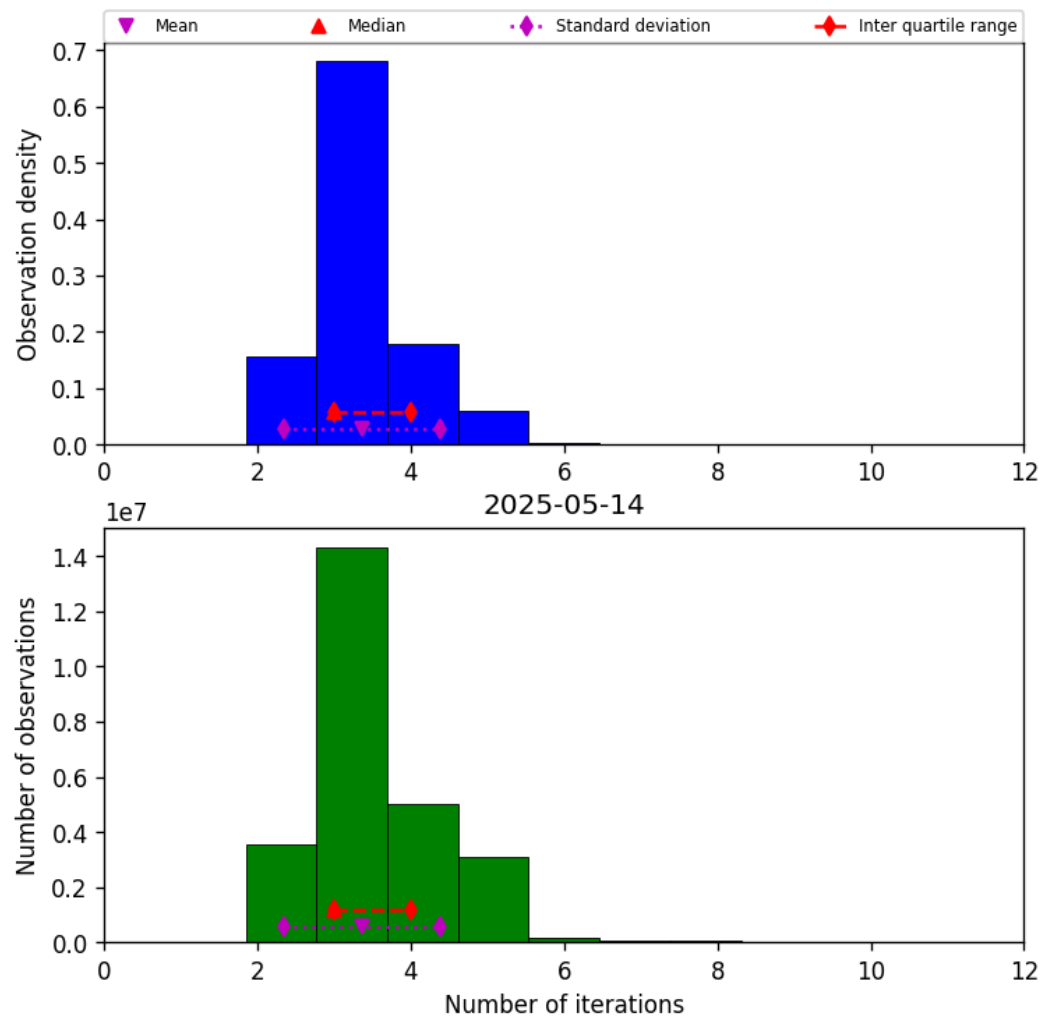
Figure 39: Histogram of “Number of iterations” for 2025-05-13 to 2025-05-15
