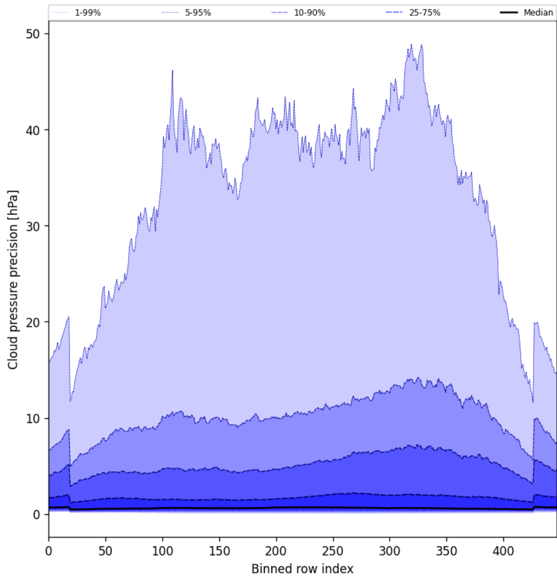
Figure 48: Along track statistics of “Cloud pressure precision” for 2025-05-13 to 2025-05-15
