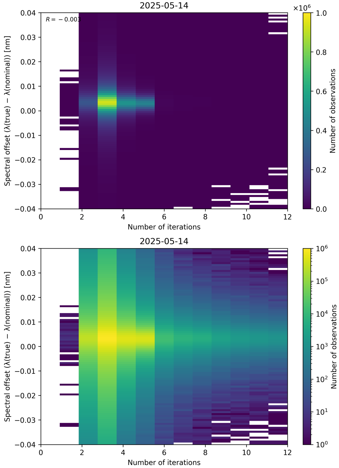
Figure 100: Scatter density plot of “Number of iterations” against “Spectral offset ( \lambda_{\text{true}} - \lambda_{\text{nominal}} )” for 2025-05-13 to 2025-05-15.
