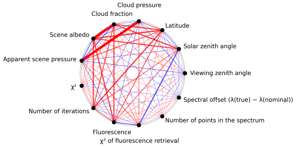
Figure 1: Map of correlation graph for 2025-05-13 to 2025-05-15.
