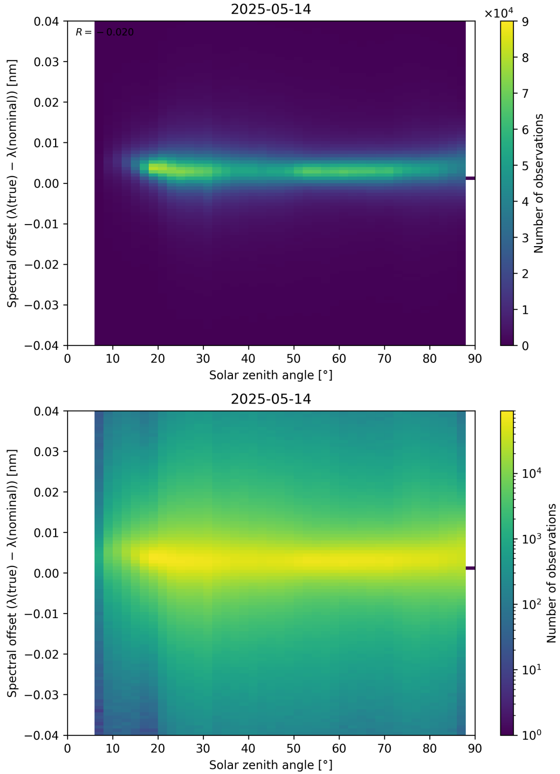
Figure 117: Scatter density plot of “Solar zenith angle” against “Spectral offset ( \lambda_{\text{true}} - \lambda_{\text{nominal}} )” for 2025-05-13 to 2025-05-15.
