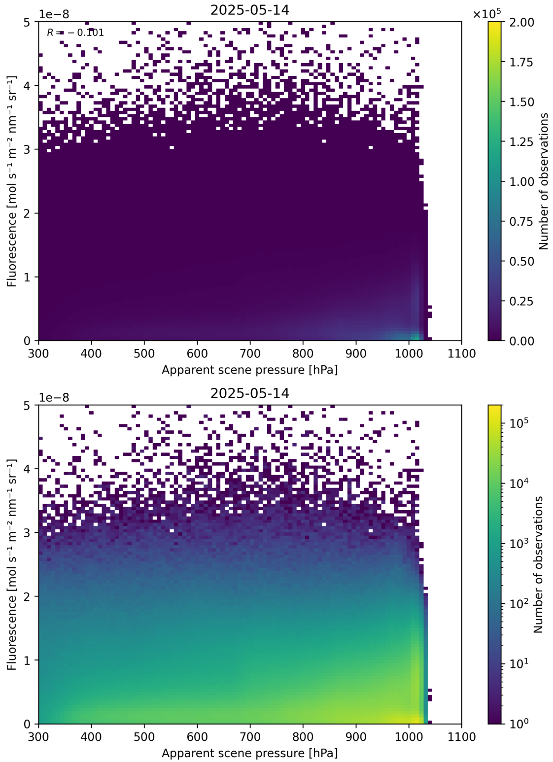
Figure 64: Scatter density plot of “Apparent scene pressure” against “Fluorescence” for 2025-05-13 to 2025-05-15.
