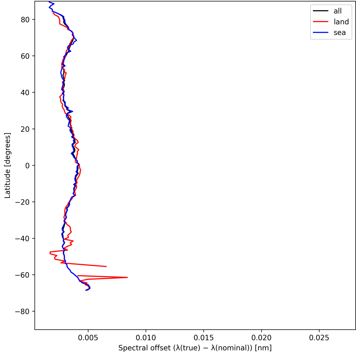
Figure 28: Zonal average of “Spectral offset ( \lambda_{\text{true}} - \lambda_{\text{nominal}} )” for 2025-05-13 to 2025-05-15.
