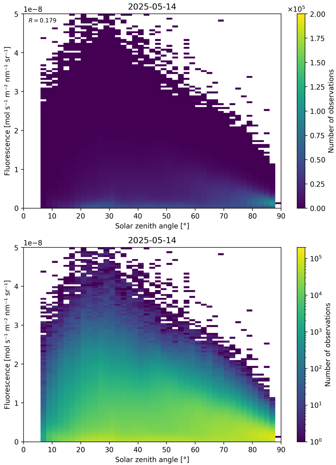
Figure 112: Scatter density plot of “Solar zenith angle” against “Fluorescence” for 2025-05-13 to 2025-05-15.
