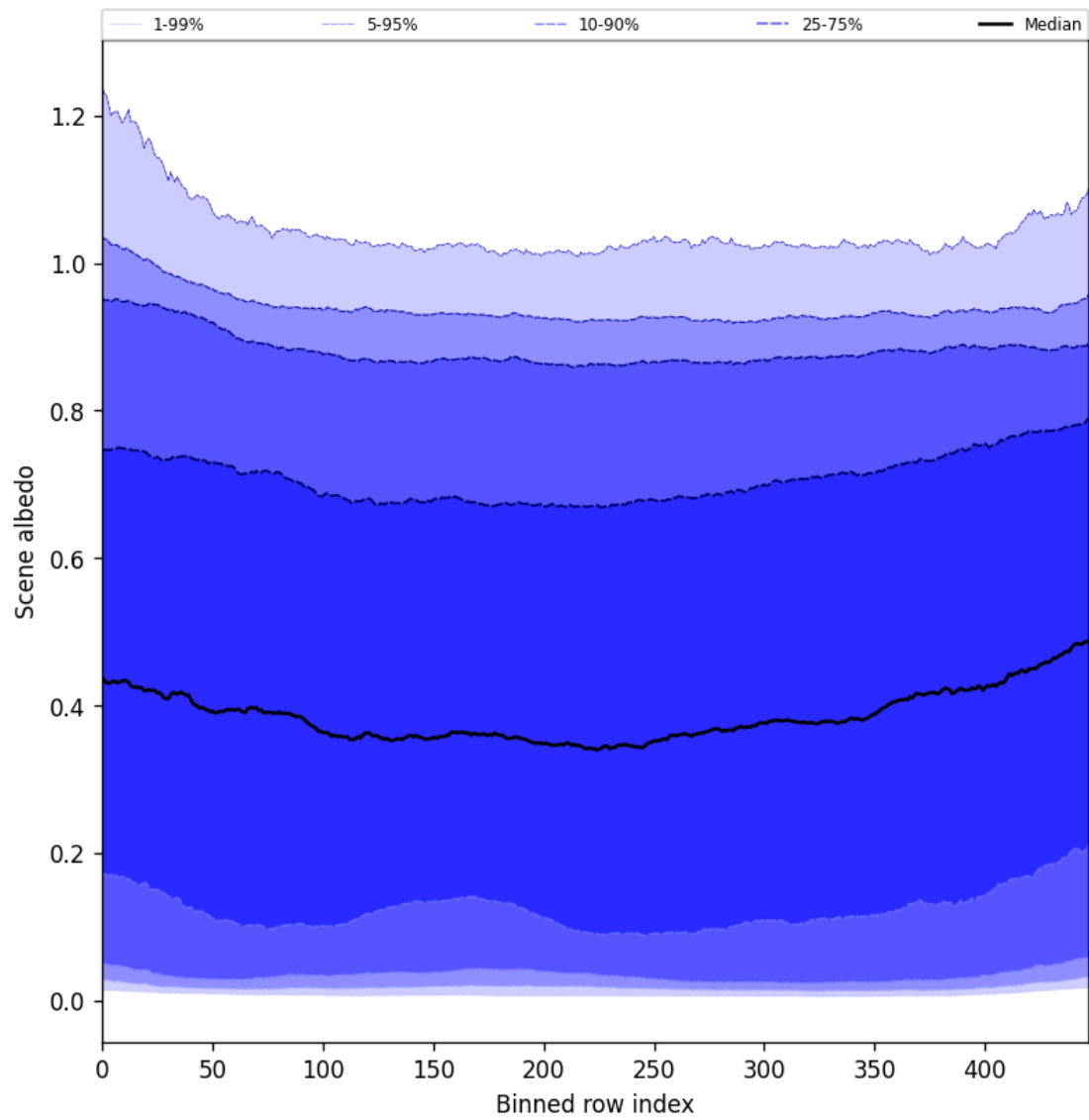
Figure 51: Along track statistics of “Scene albedo” for 2025-05-13 to 2025-05-15
