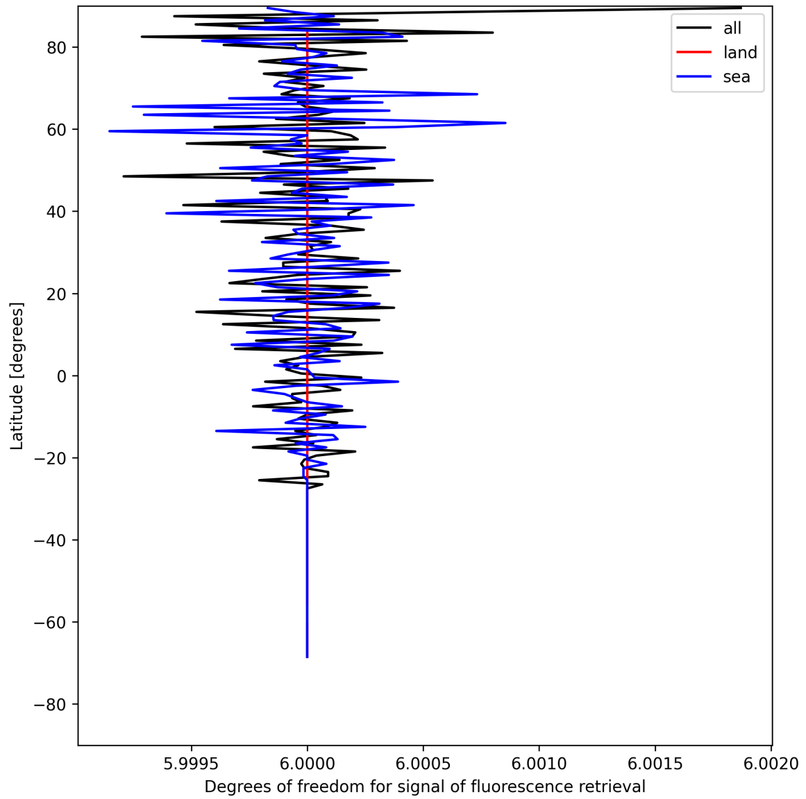
Figure 26: Zonal average of “Degrees of freedom for signal of fluorescence retrieval” for 2025-05-13 to 2025-05-15.
