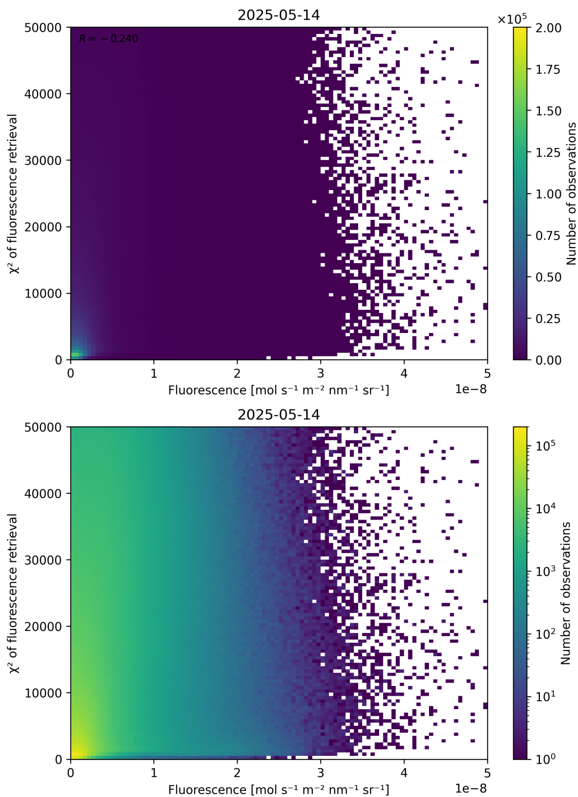
Figure 85: Scatter density plot of “Fluorescence” against “ \chi^2 of fluorescence retrieval” for 2025-05-13 to 2025-05-15.
