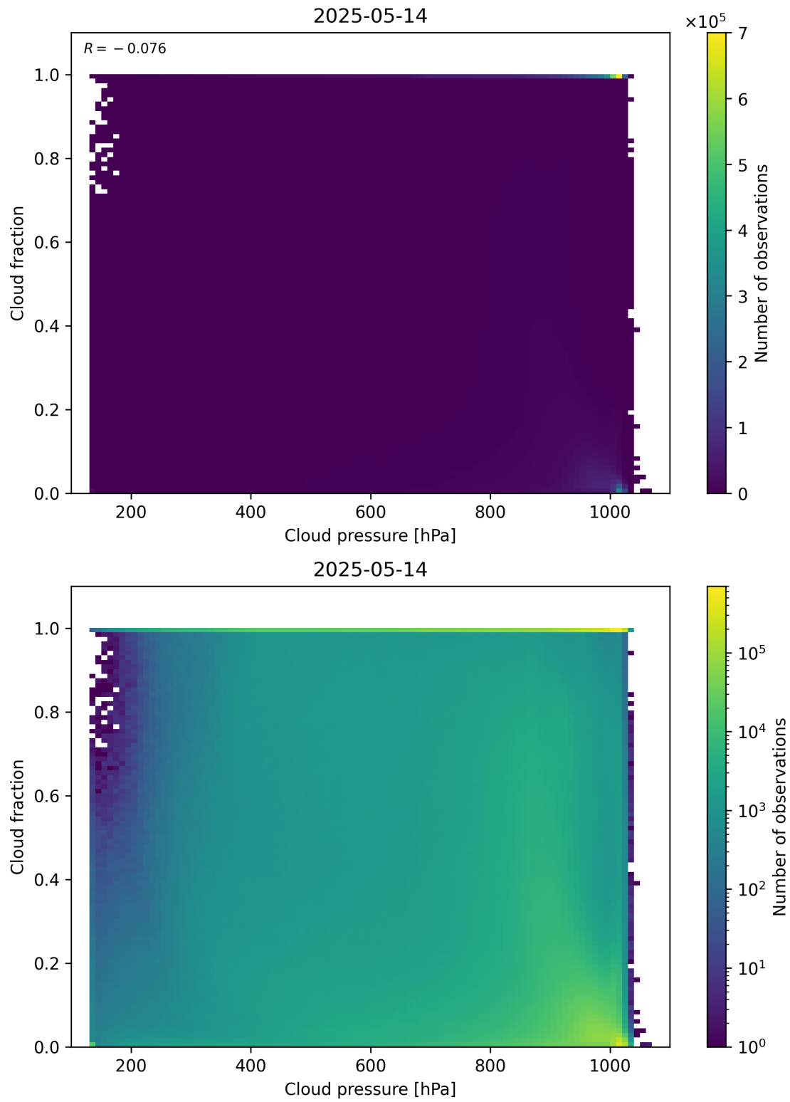
Figure 79: Scatter density plot of “Cloud pressure” against “Cloud fraction” for 2025-05-13 to 2025-05-15.
