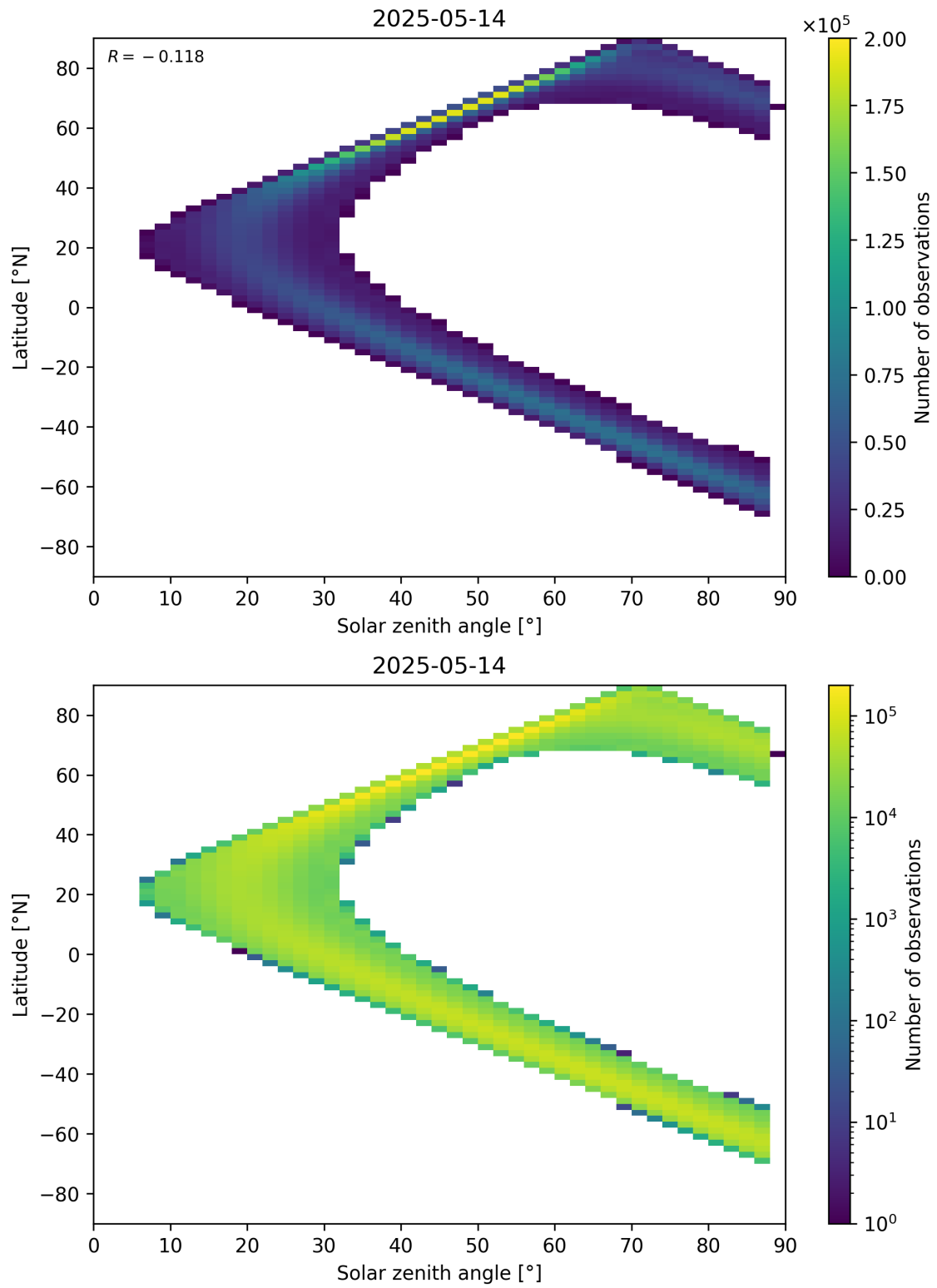
Figure 113: Scatter density plot of “Solar zenith angle” against “Latitude” for 2025-05-13 to 2025-05-15.
