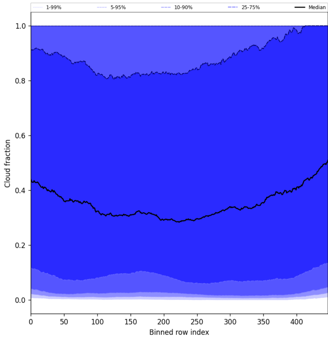
Figure 49: Along track statistics of “Cloud fraction” for 2025-05-13 to 2025-05-15
