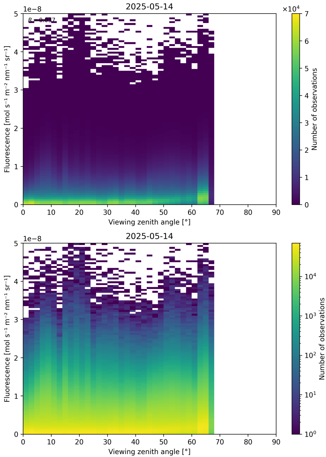
Figure 122: Scatter density plot of “Viewing zenith angle” against “Fluorescence” for 2025-05-13 to 2025-05-15.
