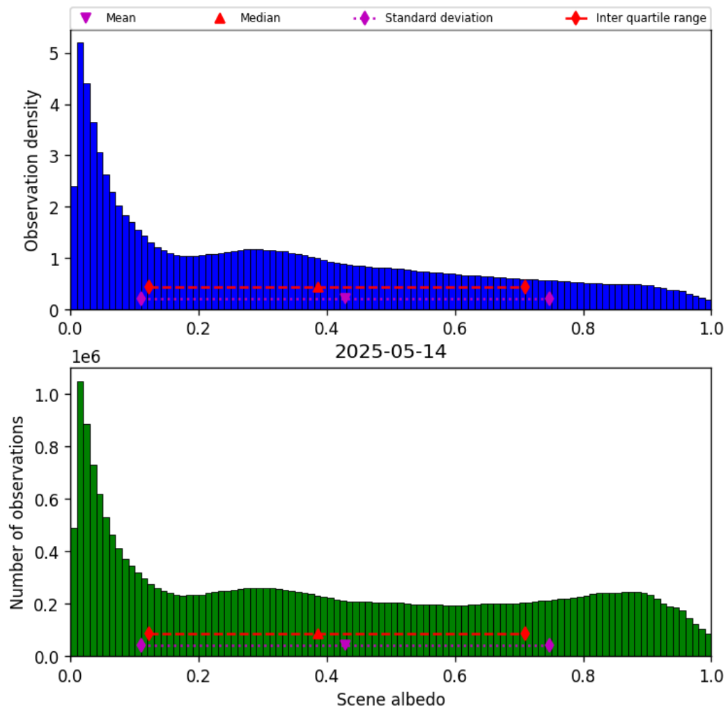
Figure 34: Histogram of “Scene albedo” for 2025-05-13 to 2025-05-15
