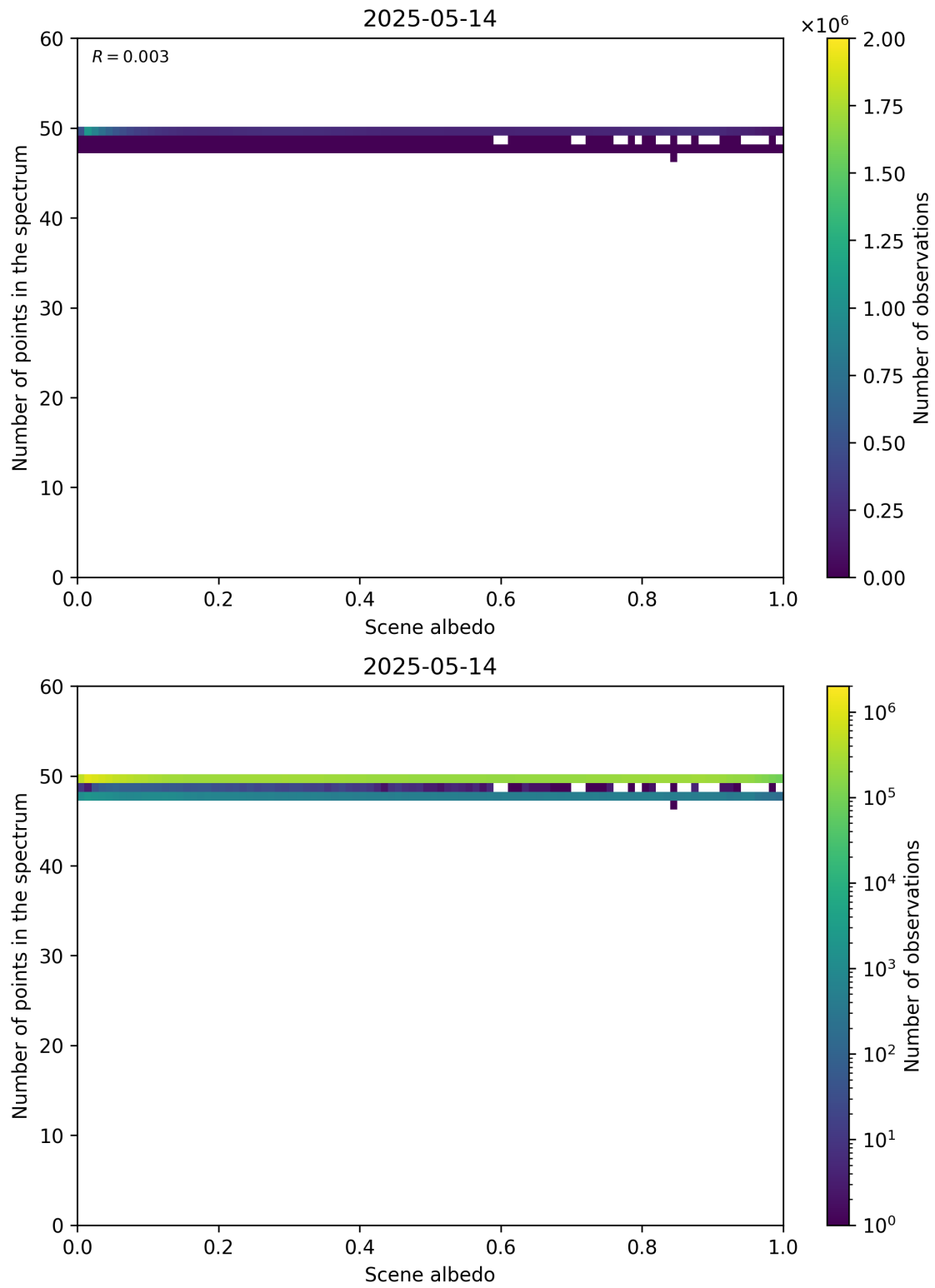
Figure 106: Scatter density plot of “Scene albedo” against “Number of points in the spectrum” for 2025-05-13 to 2025-05-15.
