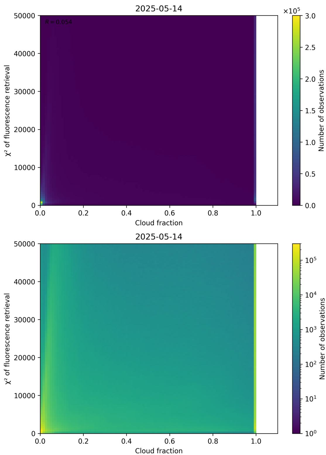
Figure 71: Scatter density plot of “Cloud fraction” against “ \chi^2 of fluorescence retrieval” for 2025-05-13 to 2025-05-15.
