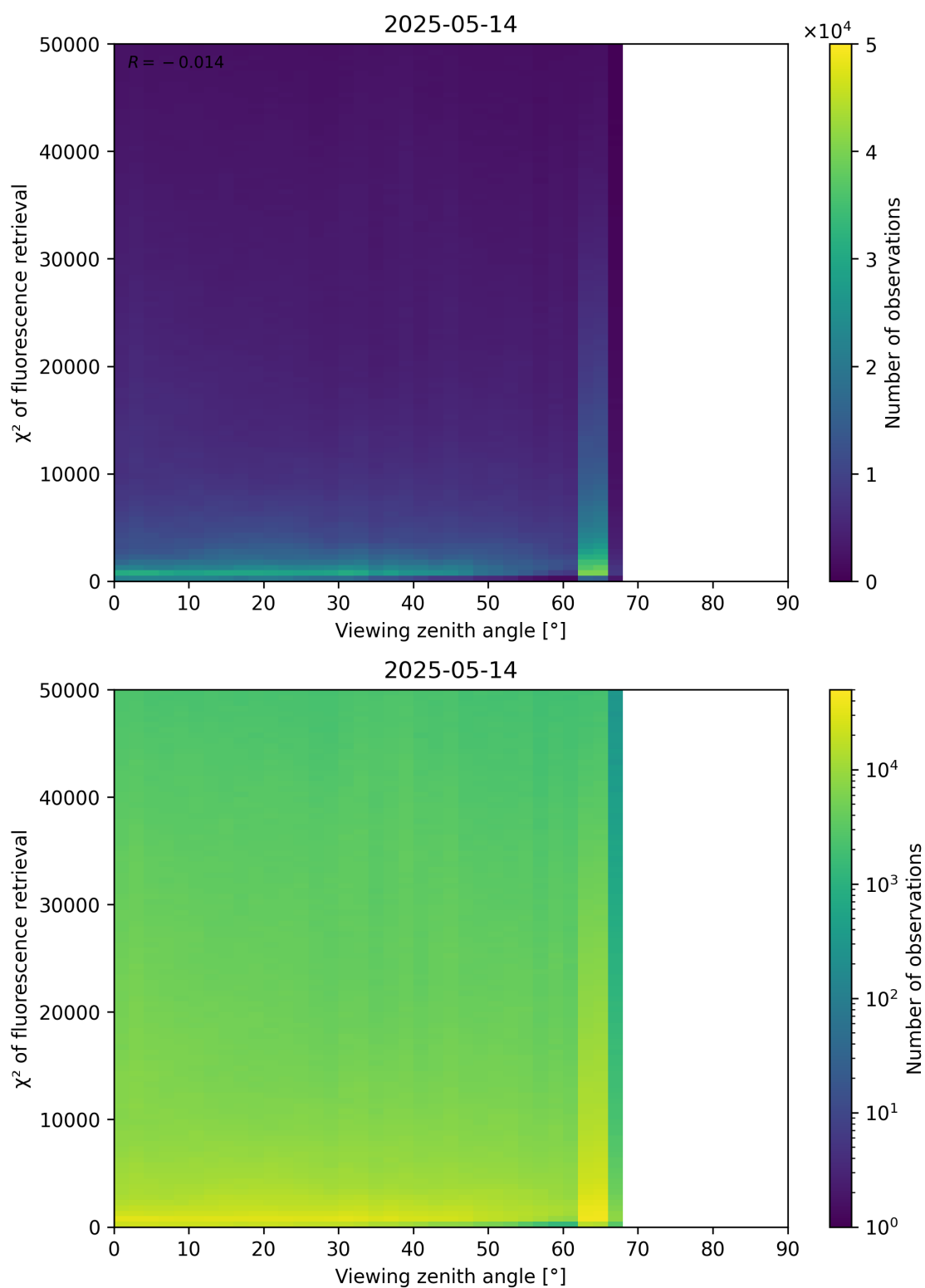
Figure 119: Scatter density plot of “Viewing zenith angle” against “ \chi^2 of fluorescence retrieval” for 2025-05-13 to 2025-05-15.
