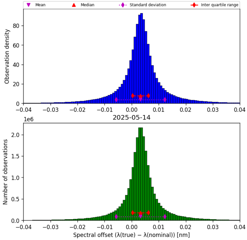
Figure 45: Histogram of “Spectral offset ( \lambda_{\text{true}} - \lambda_{\text{nominal}} )” for 2025-05-13 to 2025-05-15
