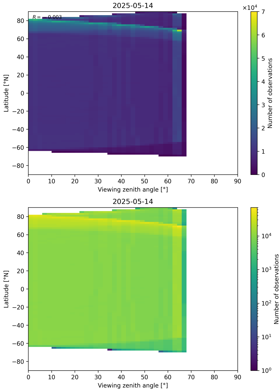
Figure 123: Scatter density plot of “Viewing zenith angle” against “Latitude” for 2025-05-13 to 2025-05-15.
