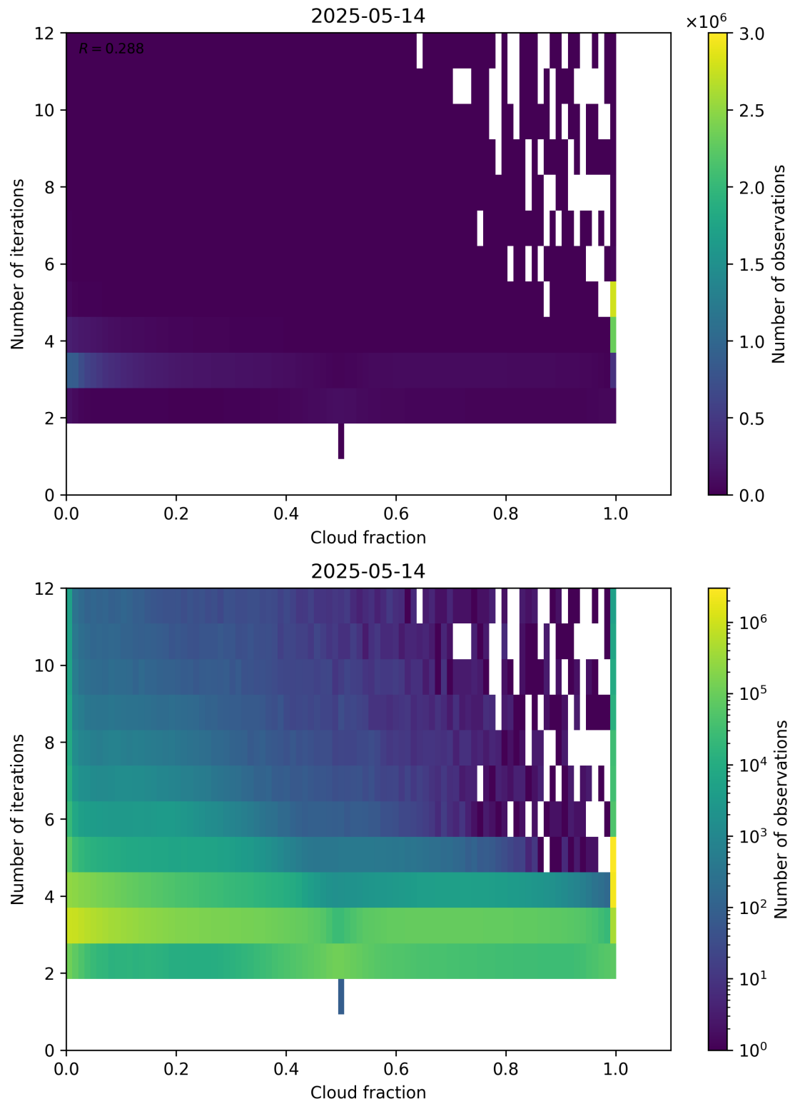
Figure 73: Scatter density plot of “Cloud fraction” against “Number of iterations” for 2025-05-13 to 2025-05-15.
