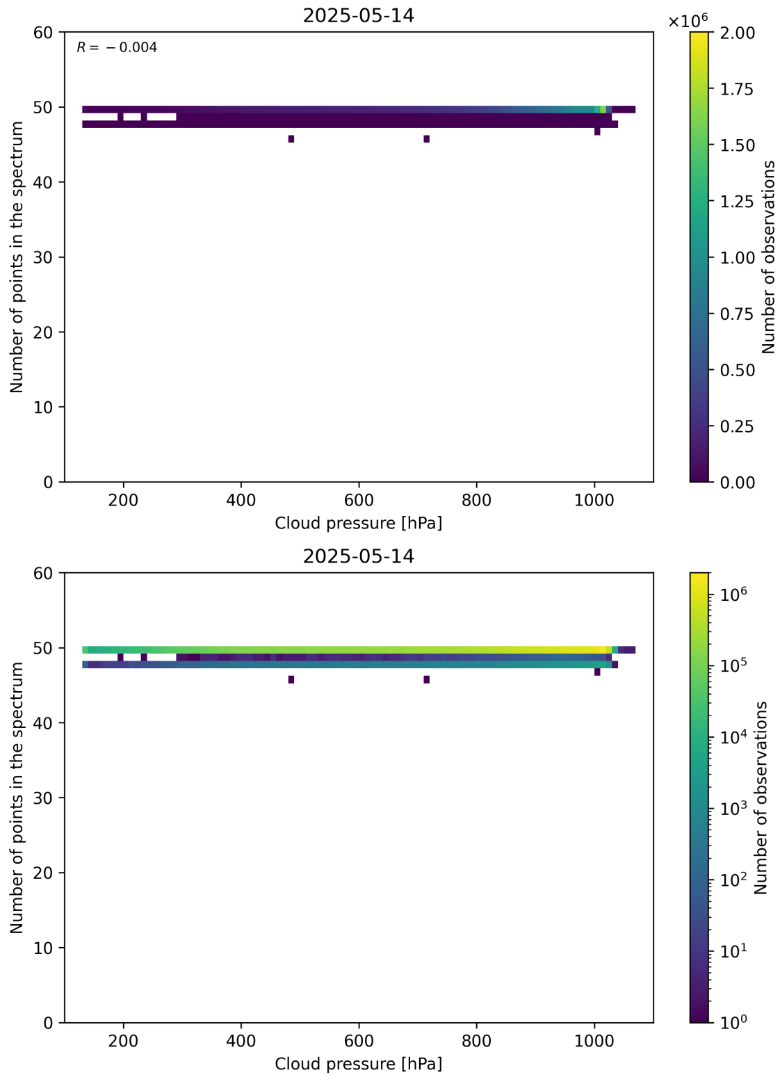
Figure 82: Scatter density plot of “Cloud pressure” against “Number of points in the spectrum” for 2025-05-13 to 2025-05-15.
