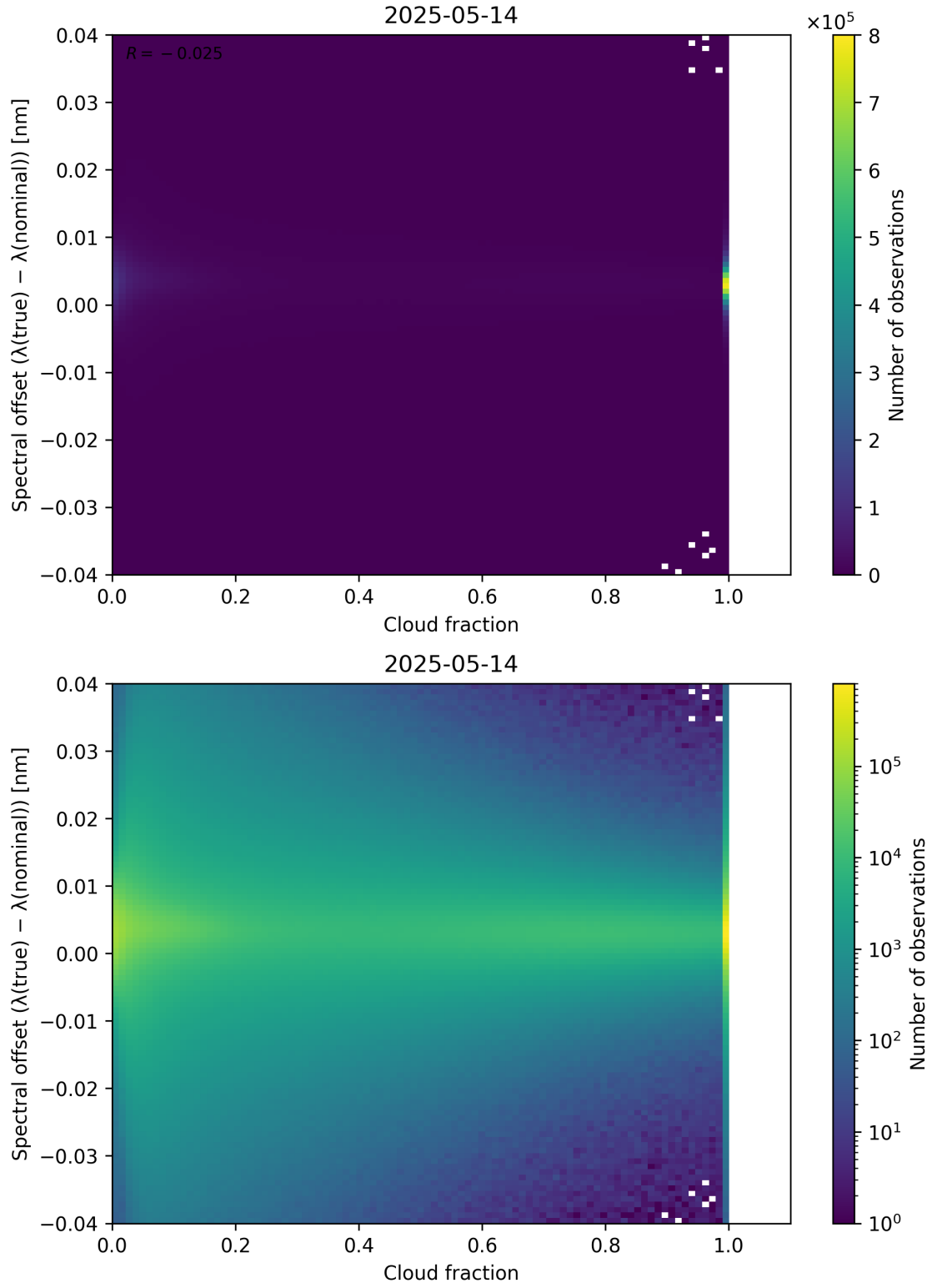
Figure 76: Scatter density plot of “Cloud fraction” against “Spectral offset ( \lambda_{\text{true}} - \lambda_{\text{nominal}} )” for 2025-05-13 to 2025-05-15.
