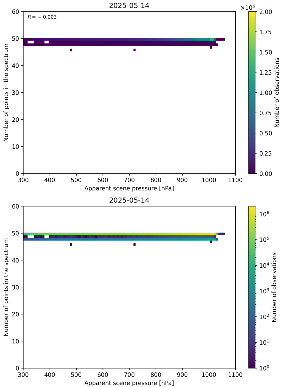
Figure 66: Scatter density plot of “Apparent scene pressure” against “Number of points in the spectrum” for 2025-05-13 to 2025-05-15.
