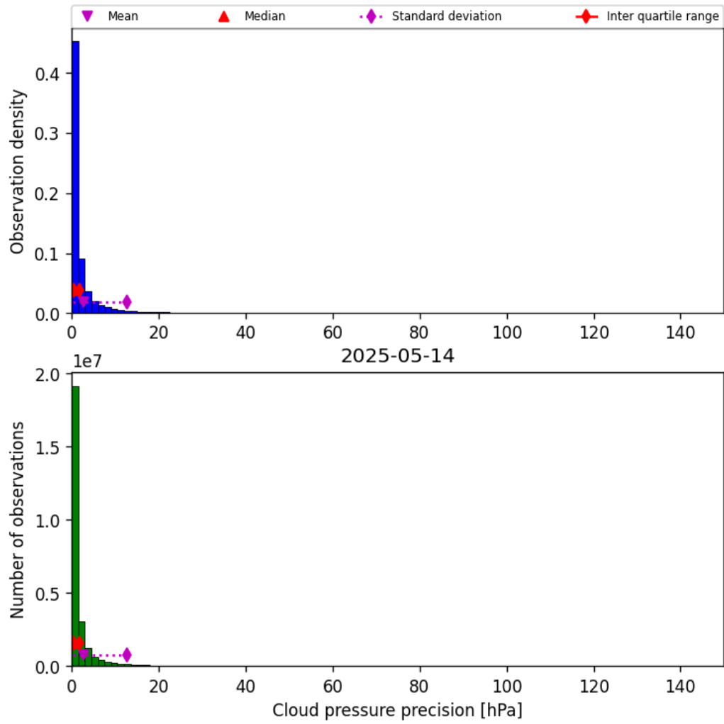
Figure 31: Histogram of “Cloud pressure precision” for 2025-05-13 to 2025-05-15
