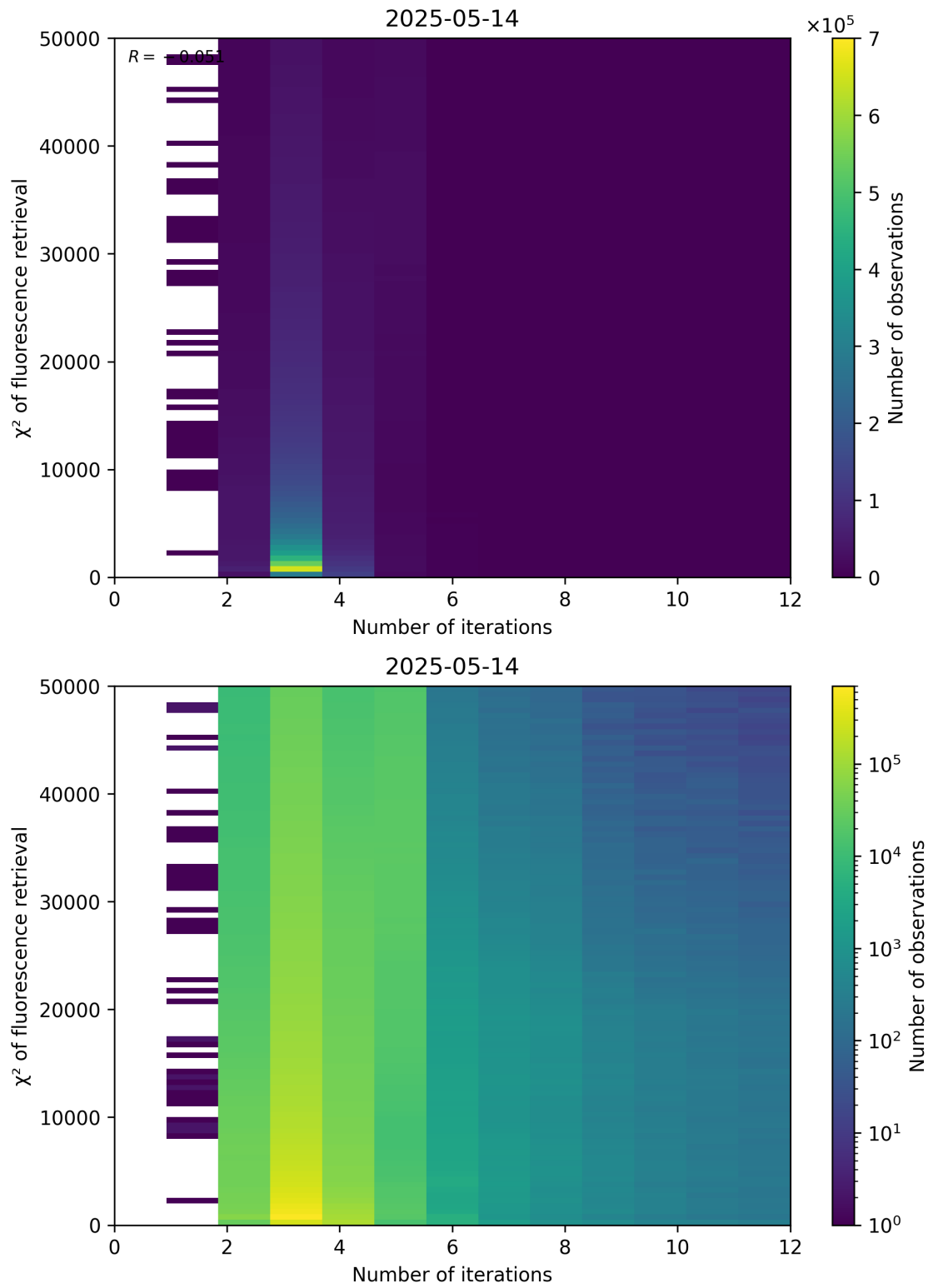
Figure 97: Scatter density plot of “Number of iterations” against “ \chi^2 of fluorescence retrieval” for 2025-05-13 to 2025-05-15.
