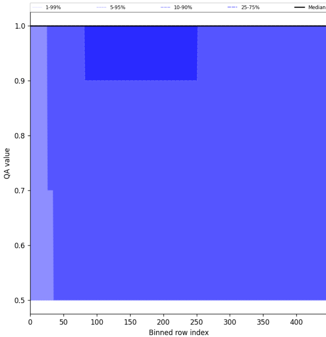
Figure 46: Along track statistics of “QA value” for 2025-05-13 to 2025-05-15
