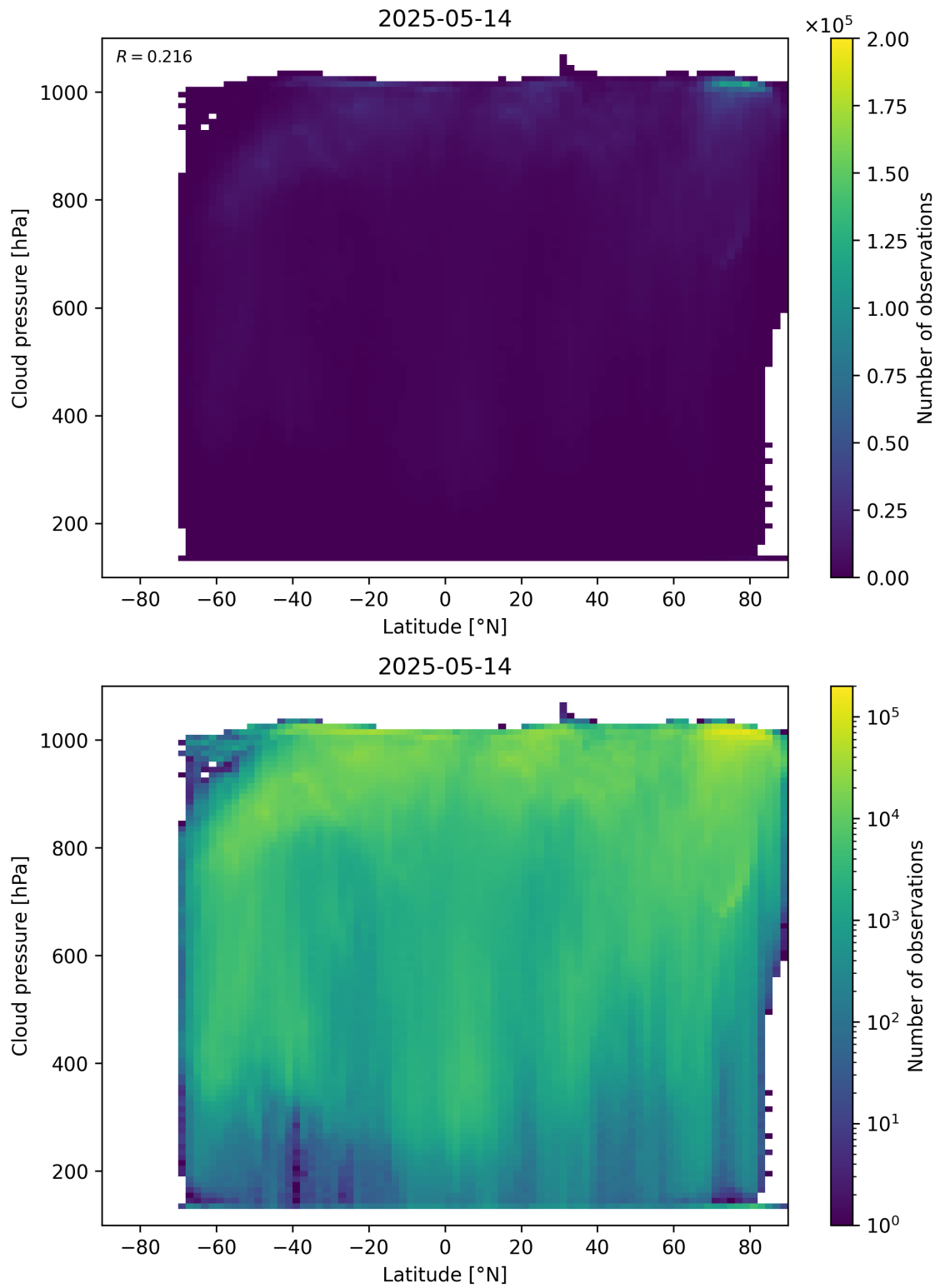
Figure 91: Scatter density plot of “Latitude” against “Cloud pressure” for 2025-05-13 to 2025-05-15.
