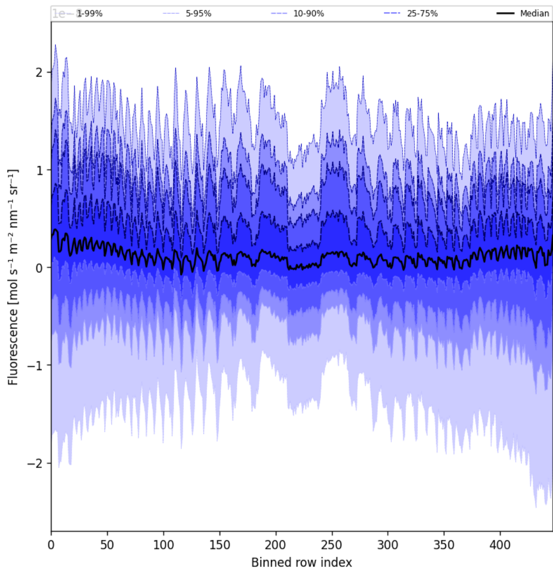
Figure 57: Along track statistics of “Fluorescence” for 2025-05-13 to 2025-05-15
