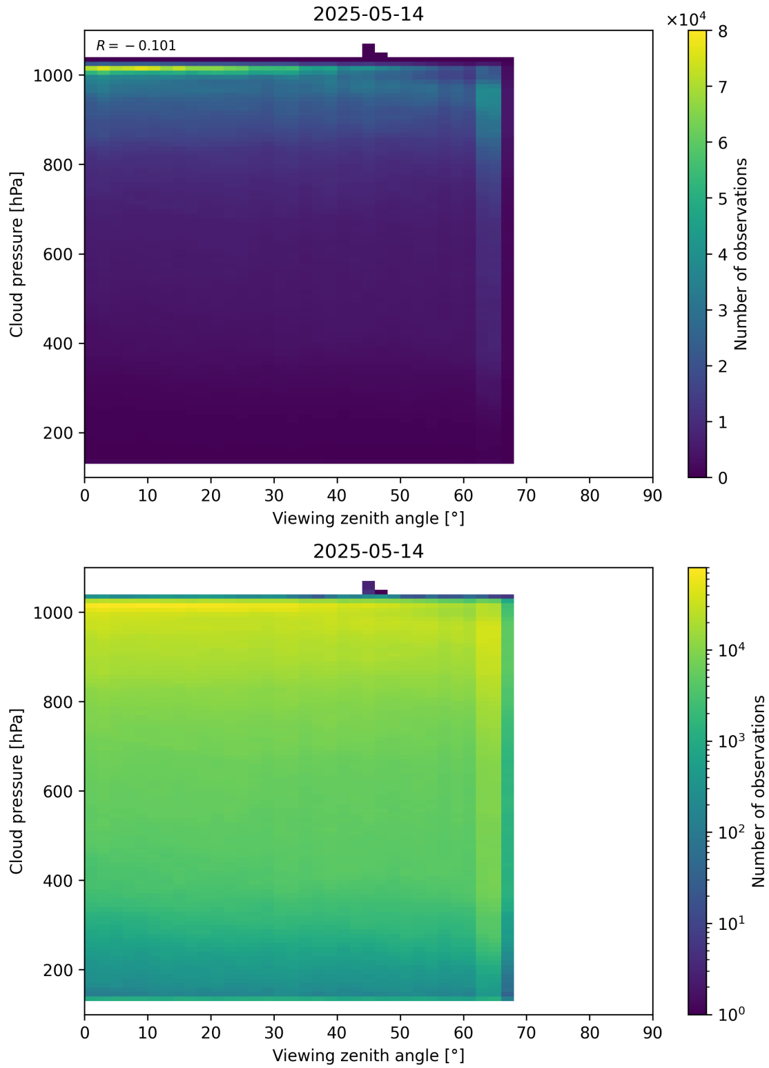
Figure 121: Scatter density plot of “Viewing zenith angle” against “Cloud pressure” for 2025-05-13 to 2025-05-15.
