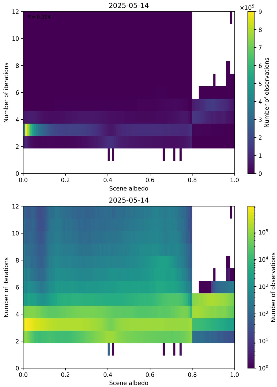
Figure 105: Scatter density plot of “Scene albedo” against “Number of iterations” for 2025-05-13 to 2025-05-15.
