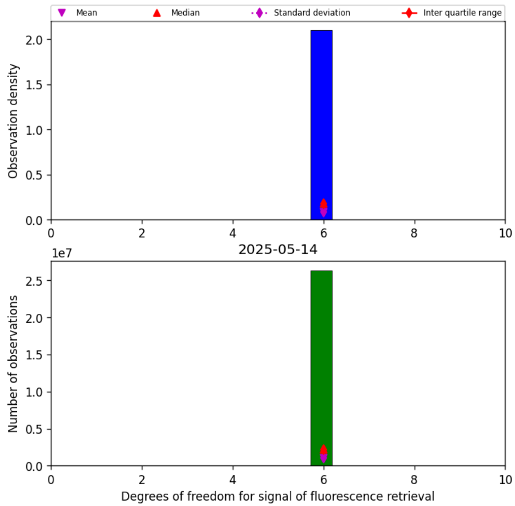
Figure 43: Histogram of “Degrees of freedom for signal of fluorescence retrieval” for 2025-05-13 to 2025-05-15
