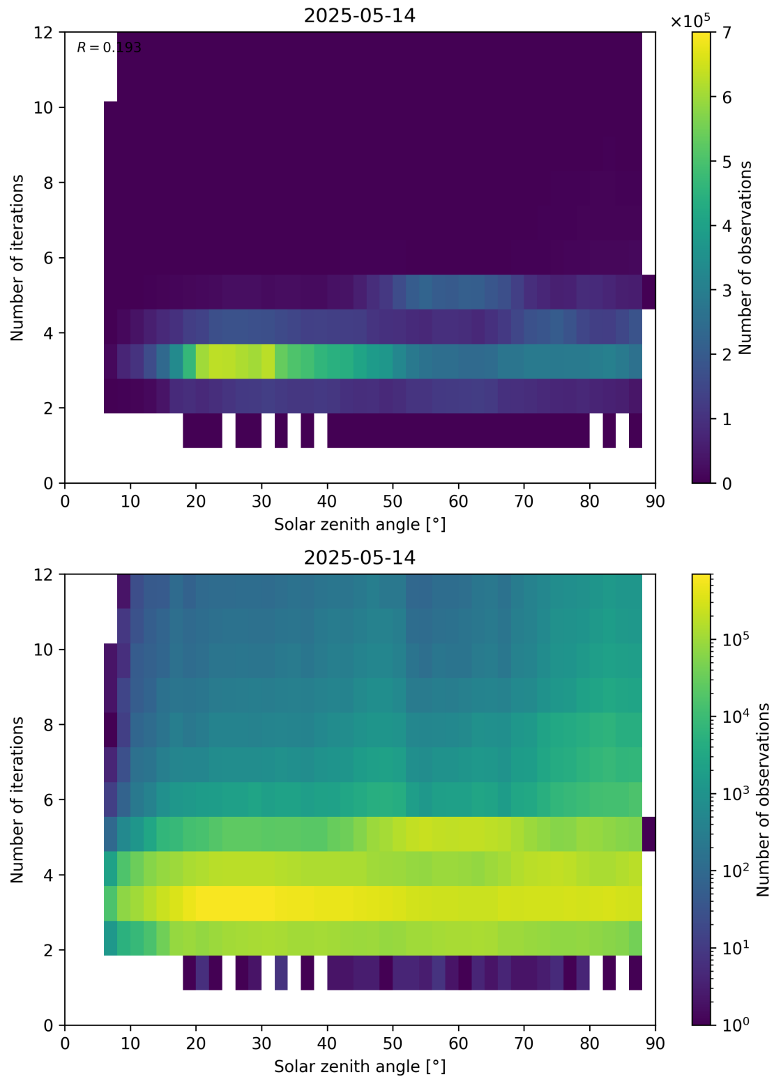
Figure 114: Scatter density plot of “Solar zenith angle” against “Number of iterations” for 2025-05-13 to 2025-05-15.
