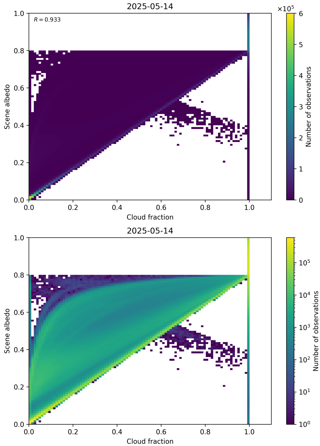
Figure 75: Scatter density plot of “Cloud fraction” against “Scene albedo” for 2025-05-13 to 2025-05-15.
