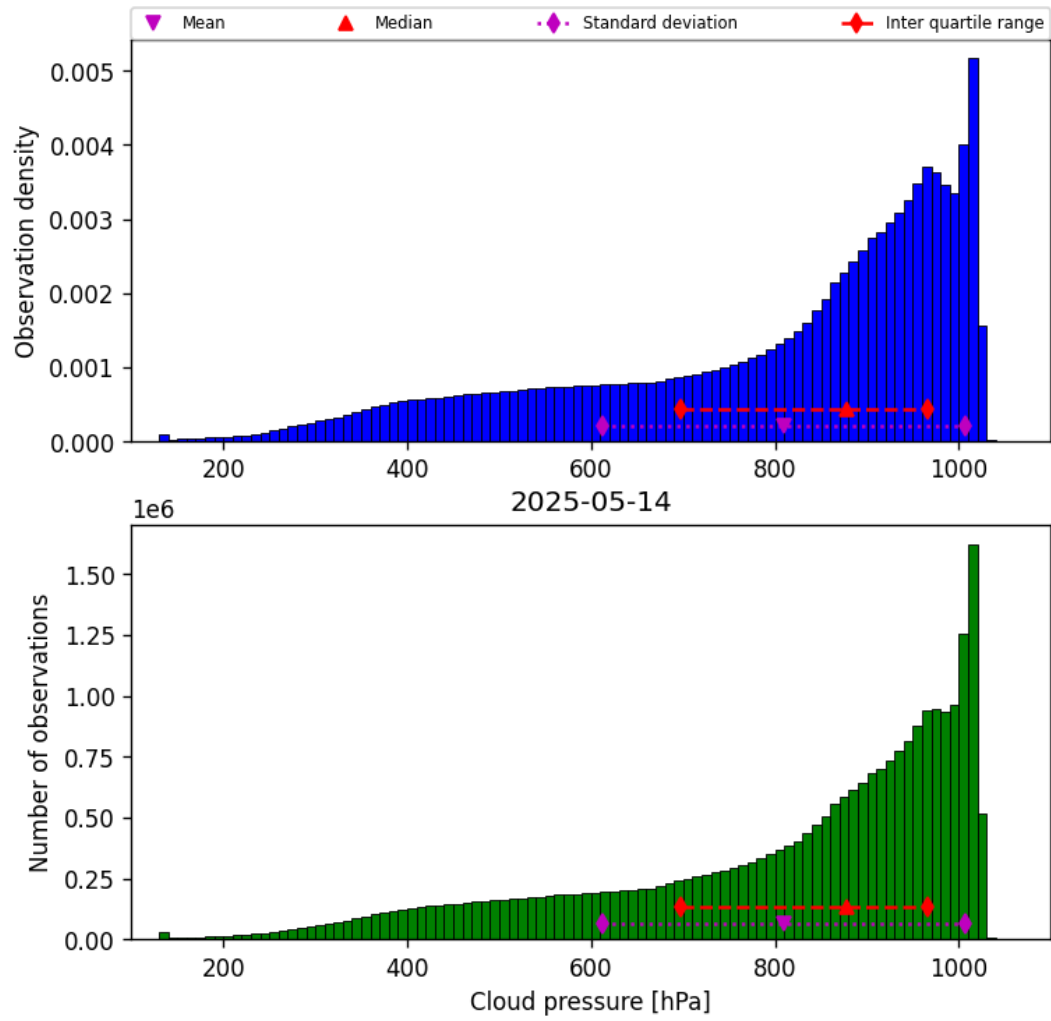
Figure 30: Histogram of “Cloud pressure” for 2025-05-13 to 2025-05-15
