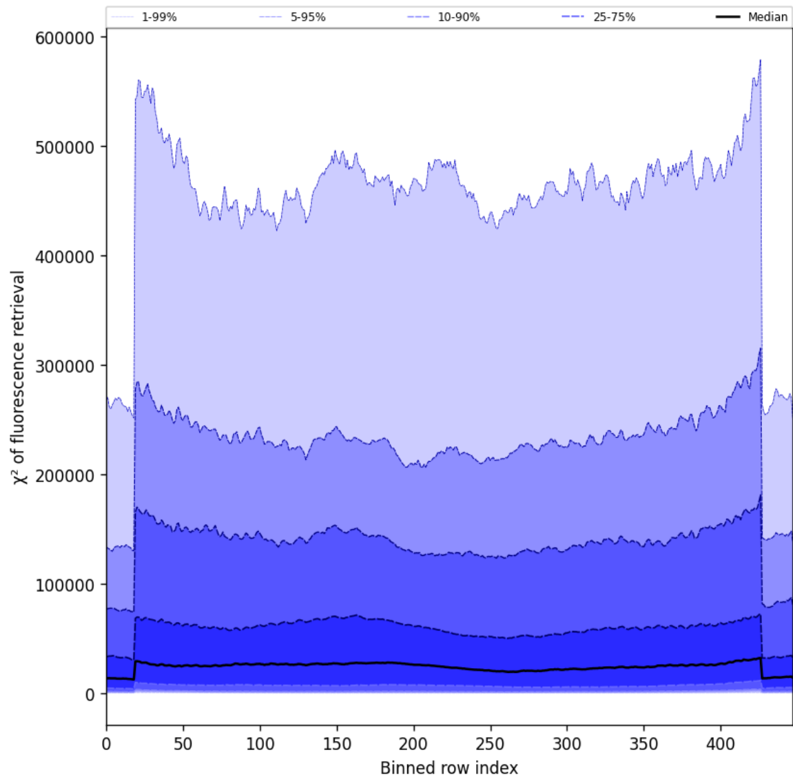
Figure 59: Along track statistics of “ \chi^2 of fluorescence retrieval” for 2025-05-13 to 2025-05-15
