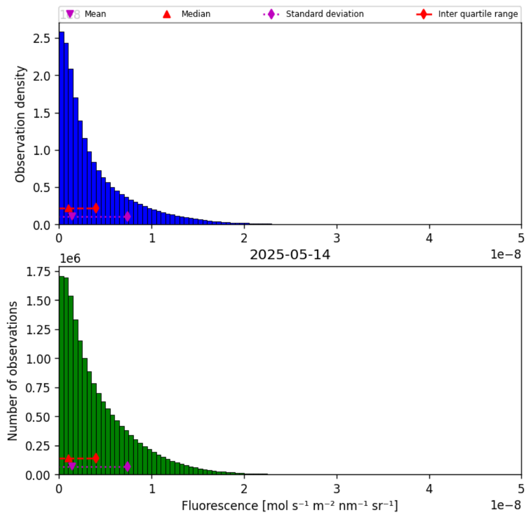
Figure 40: Histogram of “Fluorescence” for 2025-05-13 to 2025-05-15
