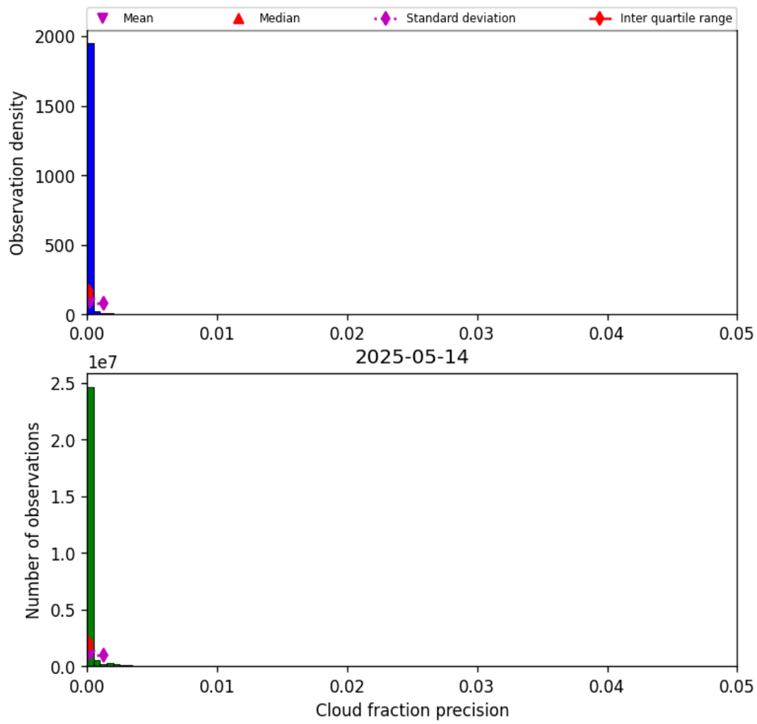
Figure 33: Histogram of “Cloud fraction precision” for 2025-05-13 to 2025-05-15
