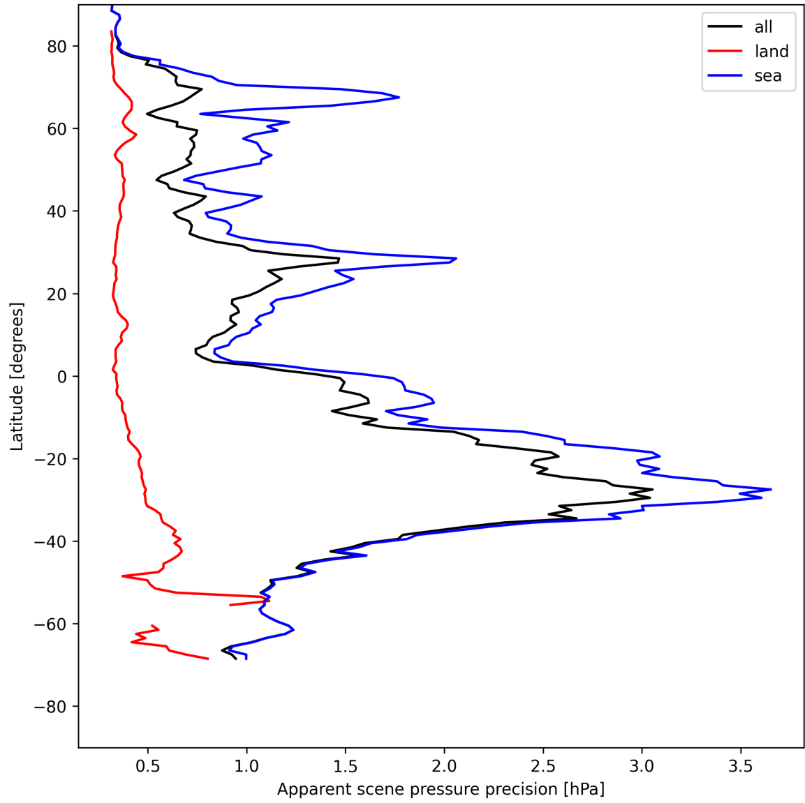
Figure 20: Zonal average of “Apparent scene pressure precision” for 2025-05-13 to 2025-05-15.
