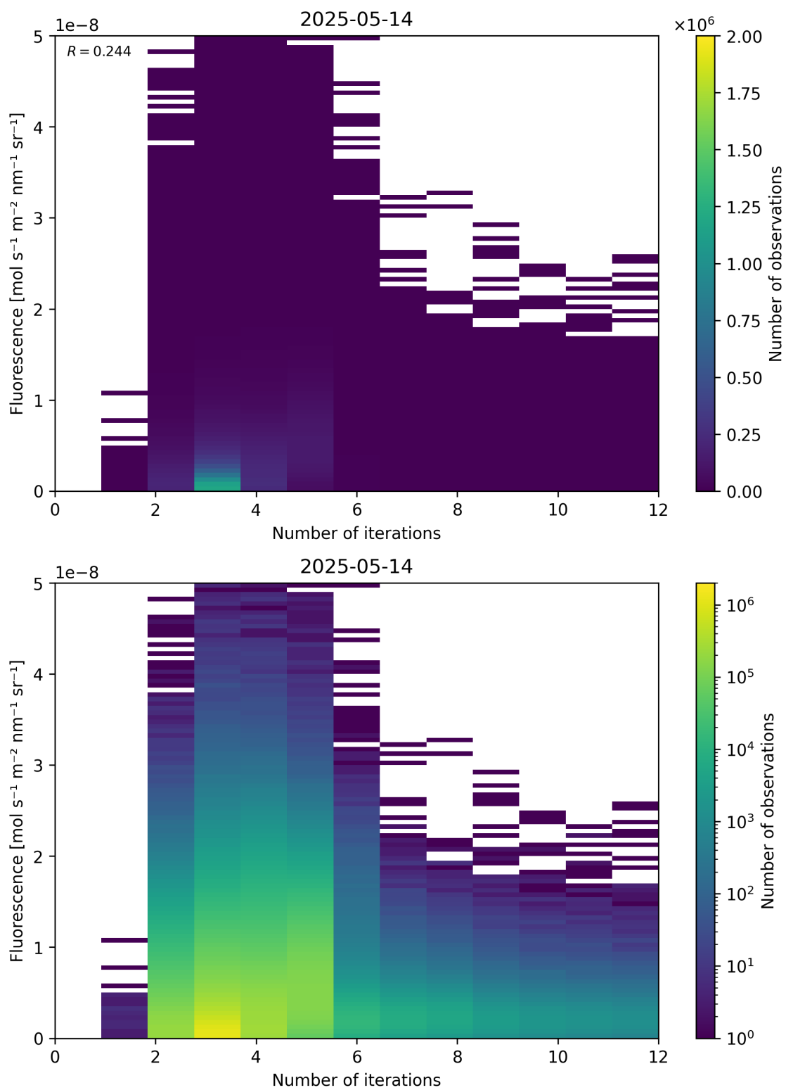
Figure 98: Scatter density plot of “Number of iterations” against “Fluorescence” for 2025-05-13 to 2025-05-15.
