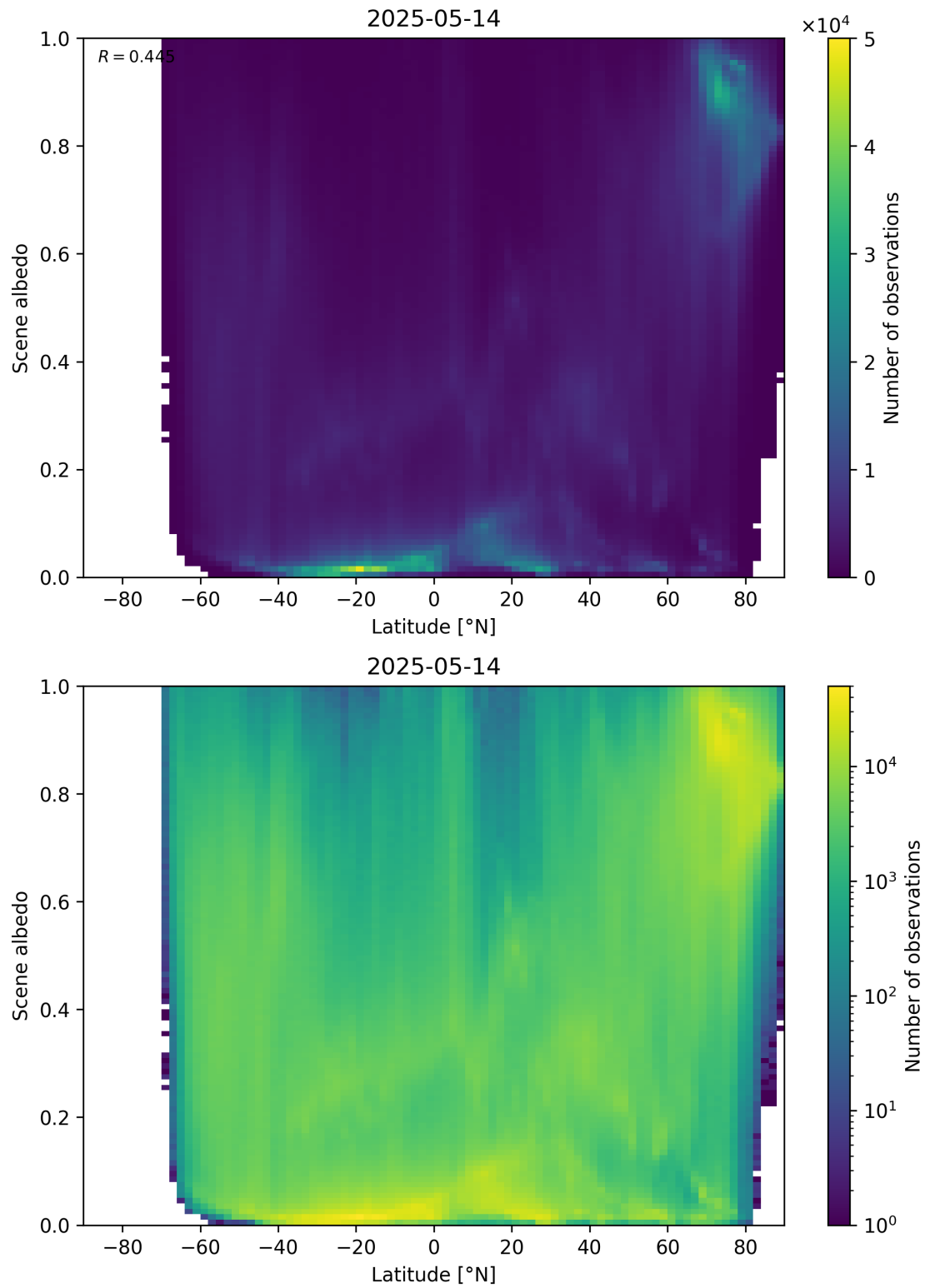
Figure 95: Scatter density plot of “Latitude” against “Scene albedo” for 2025-05-13 to 2025-05-15.
