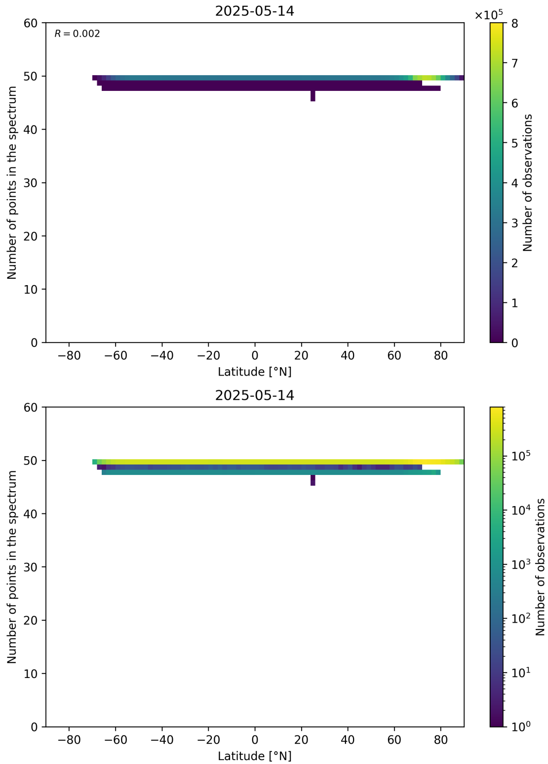
Figure 94: Scatter density plot of “Latitude” against “Number of points in the spectrum” for 2025-05-13 to 2025-05-15.
