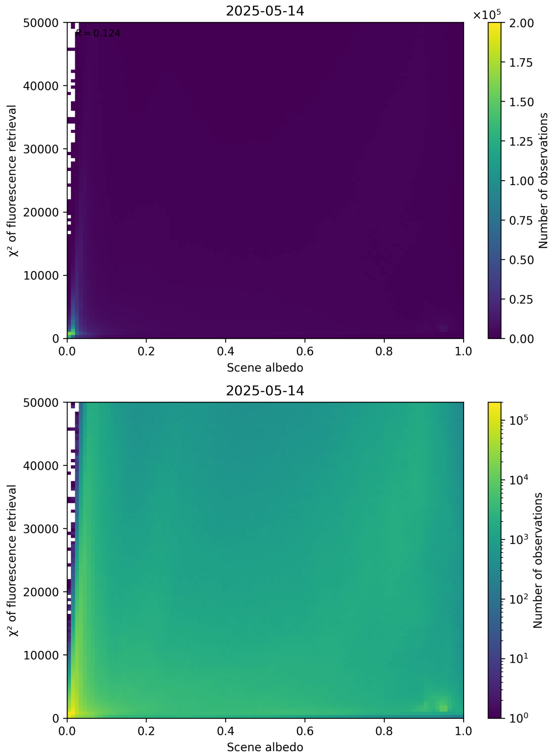
Figure 103: Scatter density plot of “Scene albedo” against “ \chi^2 of fluorescence retrieval” for 2025-05-13 to 2025-05-15.
