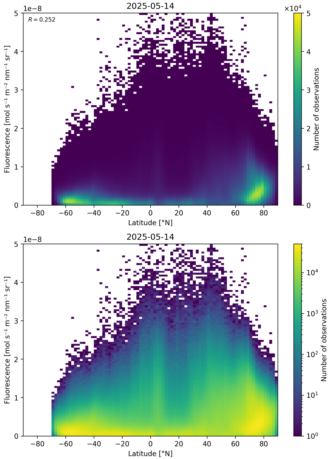
Figure 92: Scatter density plot of “Latitude” against “Fluorescence” for 2025-05-13 to 2025-05-15.
