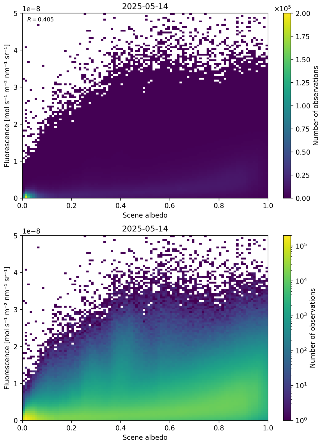
Figure 104: Scatter density plot of “Scene albedo” against “Fluorescence” for 2025-05-13 to 2025-05-15.
