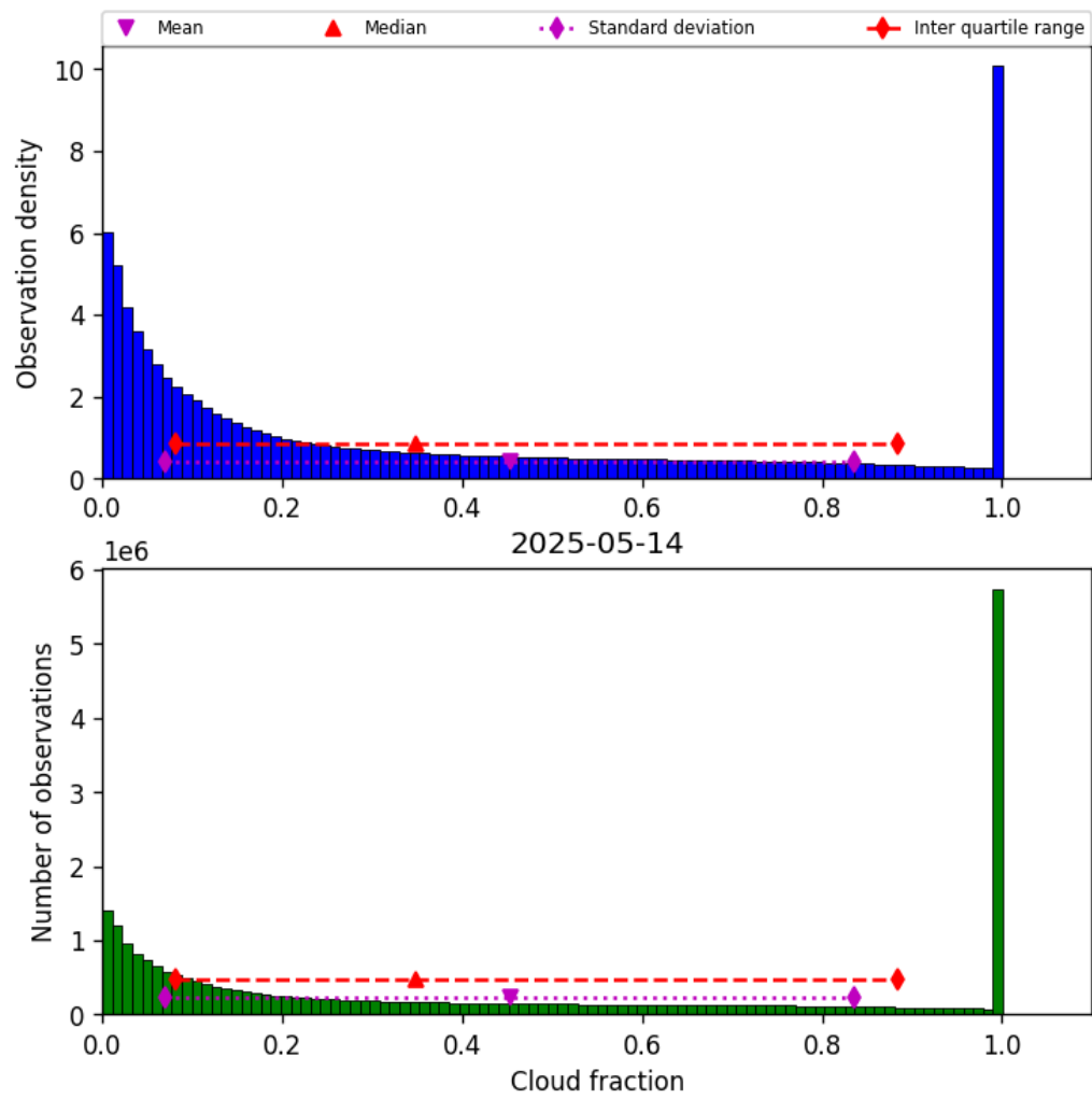
Figure 32: Histogram of “Cloud fraction” for 2025-05-13 to 2025-05-15
