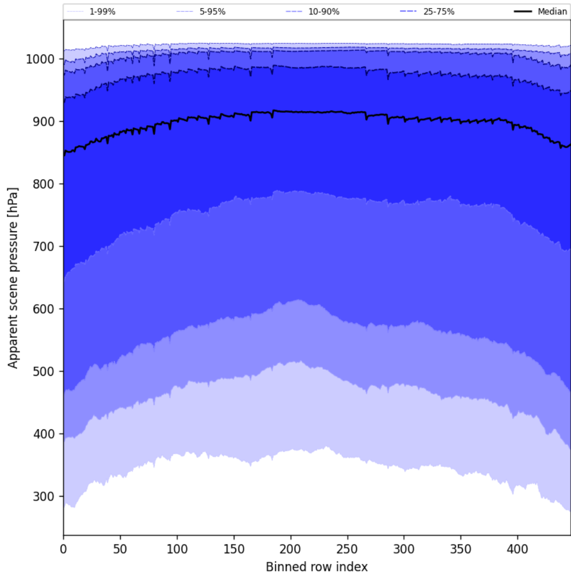
Figure 53: Along track statistics of “Apparent scene pressure” for 2025-05-13 to 2025-05-15
