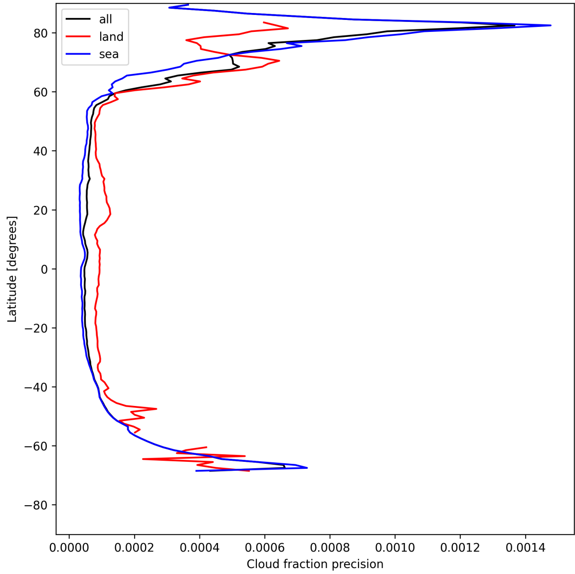
Figure 16: Zonal average of “Cloud fraction precision” for 2025-05-13 to 2025-05-15.
