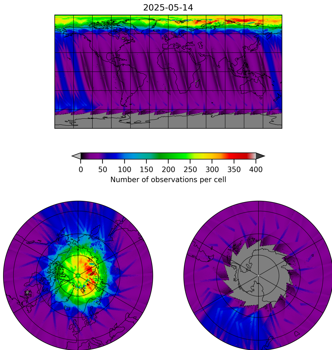
Figure 11: Map of the number of observations for 2025-05-13 to 2025-05-15
