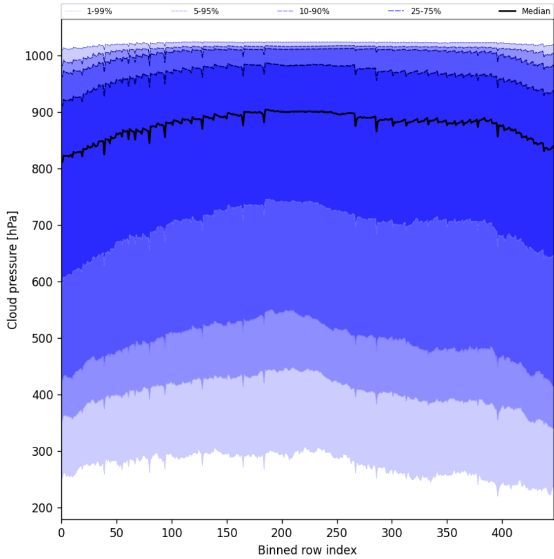
Figure 47: Along track statistics of “Cloud pressure” for 2025-05-13 to 2025-05-15
