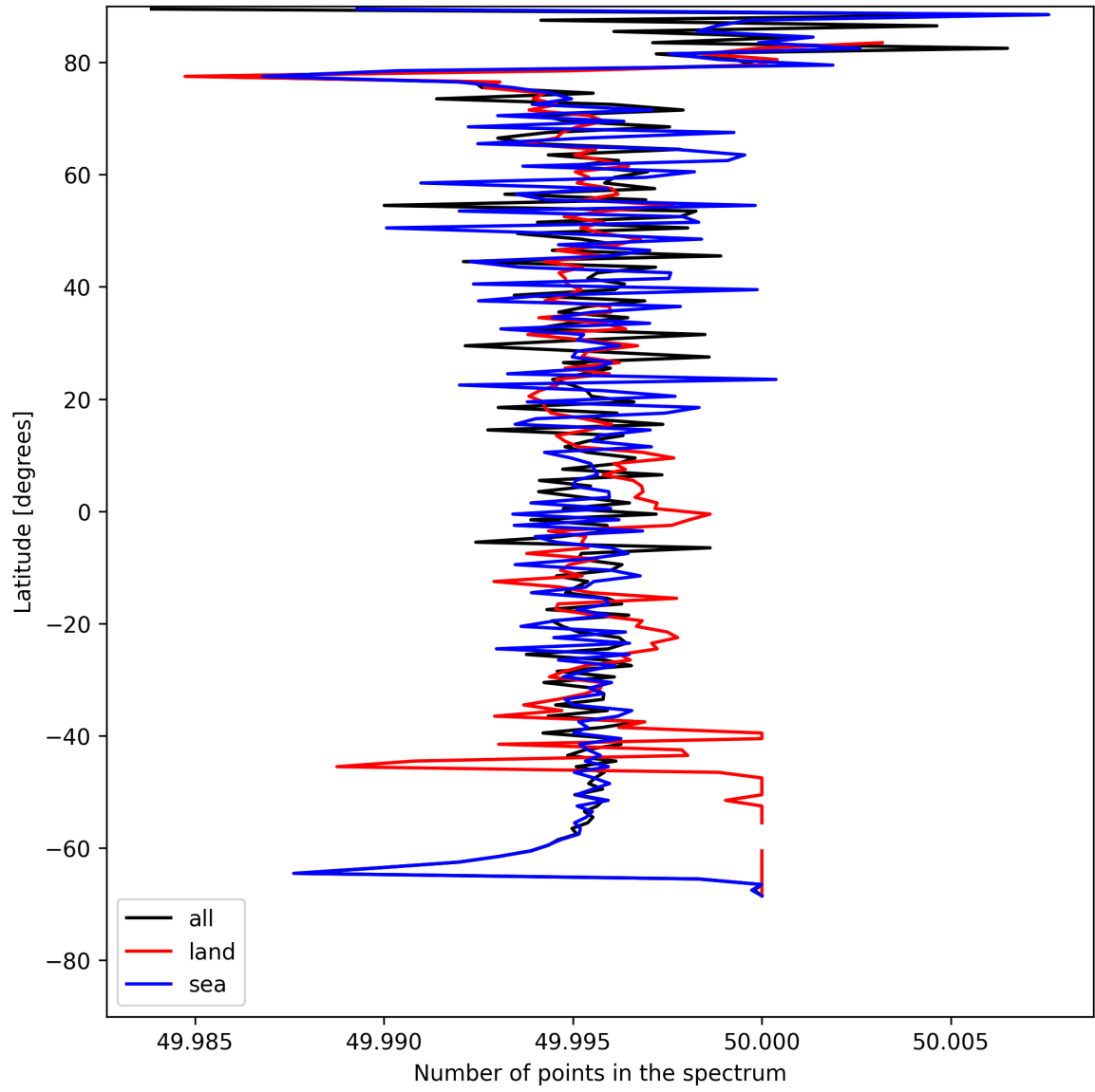
Figure 27: Zonal average of “Number of points in the spectrum” for 2025-05-13 to 2025-05-15.
