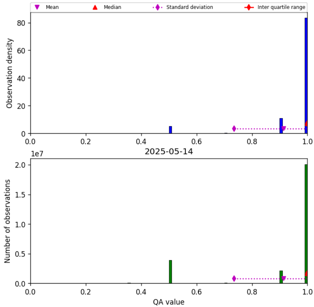
Figure 29: Histogram of “QA value” for 2025-05-13 to 2025-05-15
