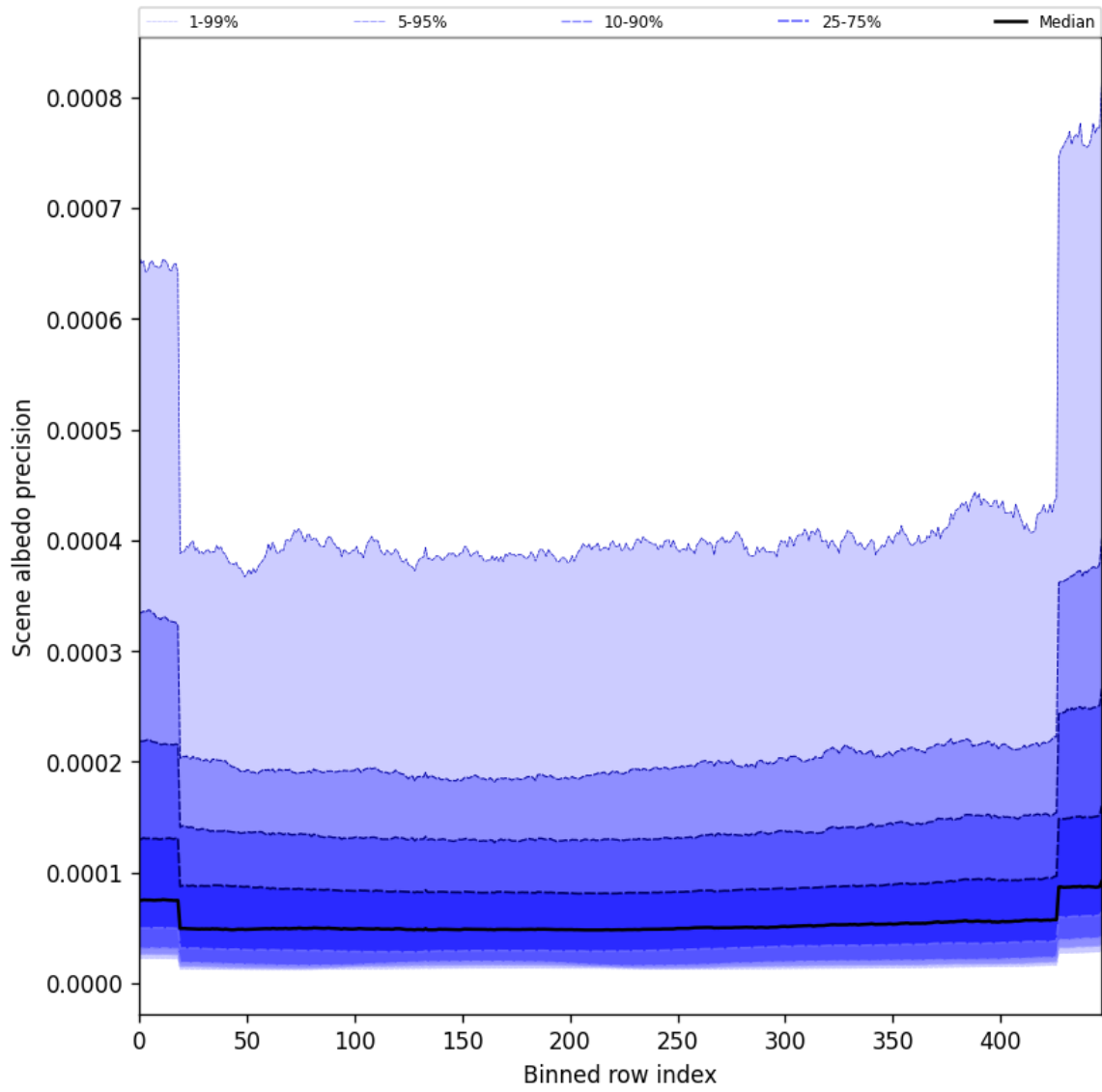
Figure 52: Along track statistics of “Scene albedo precision” for 2025-05-13 to 2025-05-15
