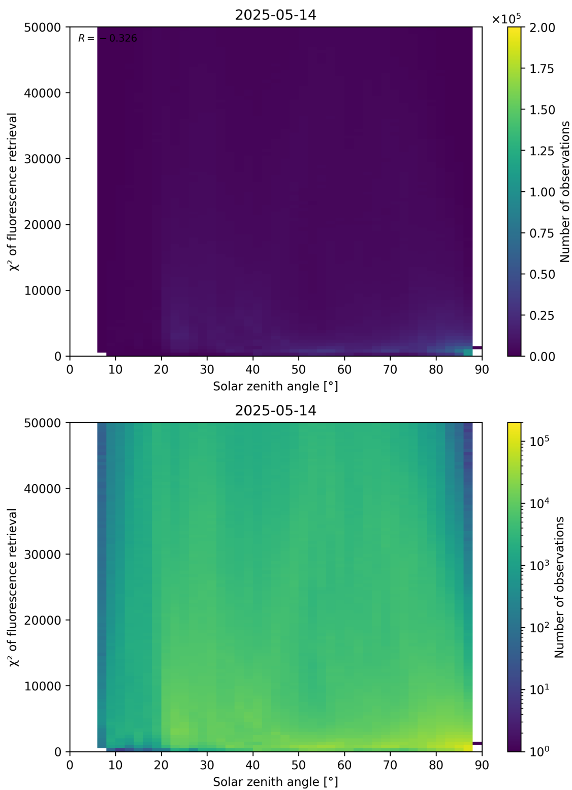
Figure 109: Scatter density plot of “Solar zenith angle” against “ \chi^2 of fluorescence retrieval” for 2025-05-13 to 2025-05-15.
