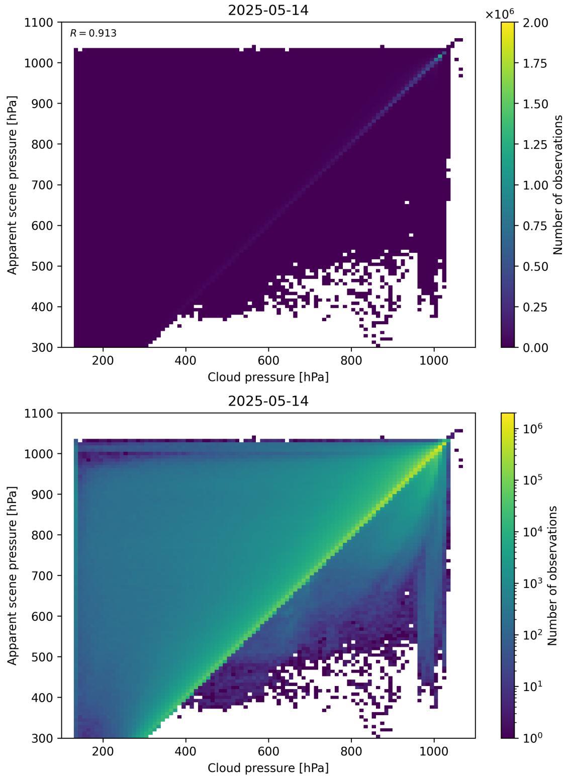
Figure 77: Scatter density plot of “Cloud pressure” against “Apparent scene pressure” for 2025-05-13 to 2025-05-15.
