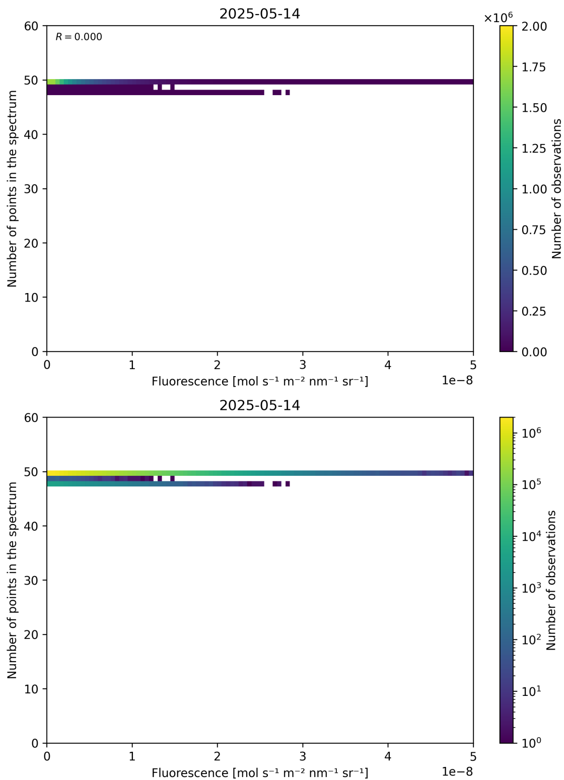
Figure 86: Scatter density plot of “Fluorescence” against “Number of points in the spectrum” for 2025-05-13 to 2025-05-15.
