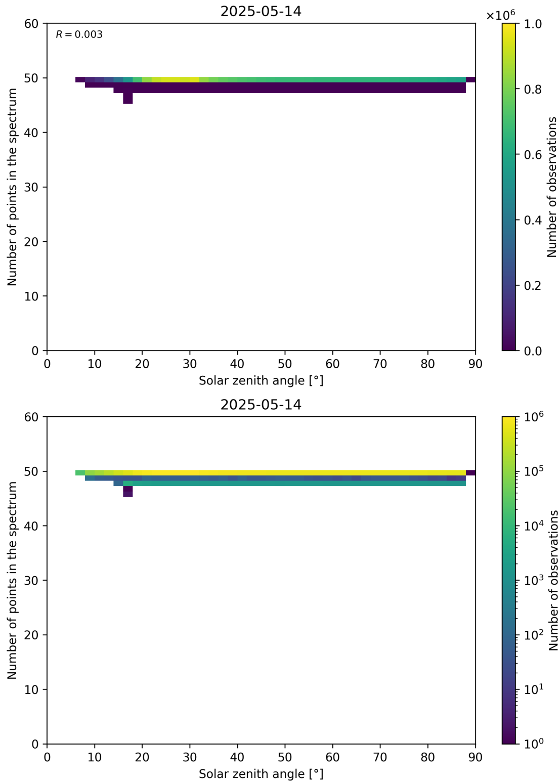
Figure 115: Scatter density plot of “Solar zenith angle” against “Number of points in the spectrum” for 2025-05-13 to 2025-05-15.
