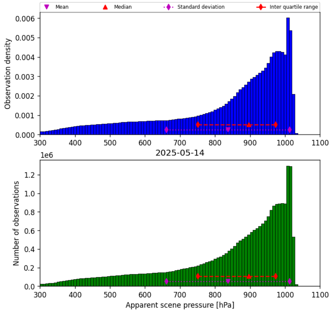
Figure 36: Histogram of “Apparent scene pressure” for 2025-05-13 to 2025-05-15
