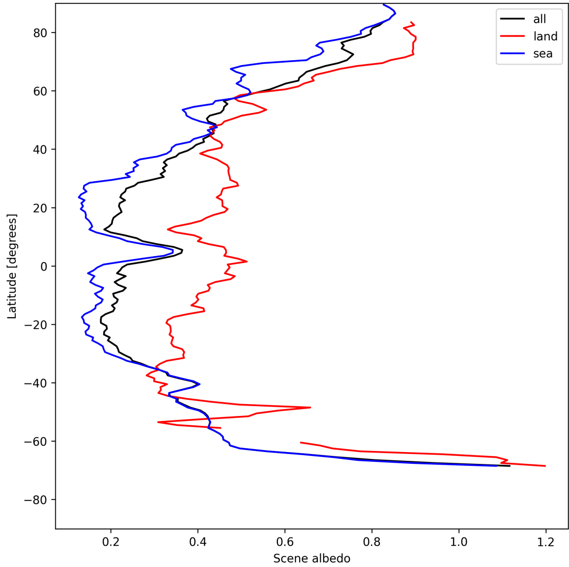
Figure 17: Zonal average of “Scene albedo” for 2025-05-13 to 2025-05-15.
