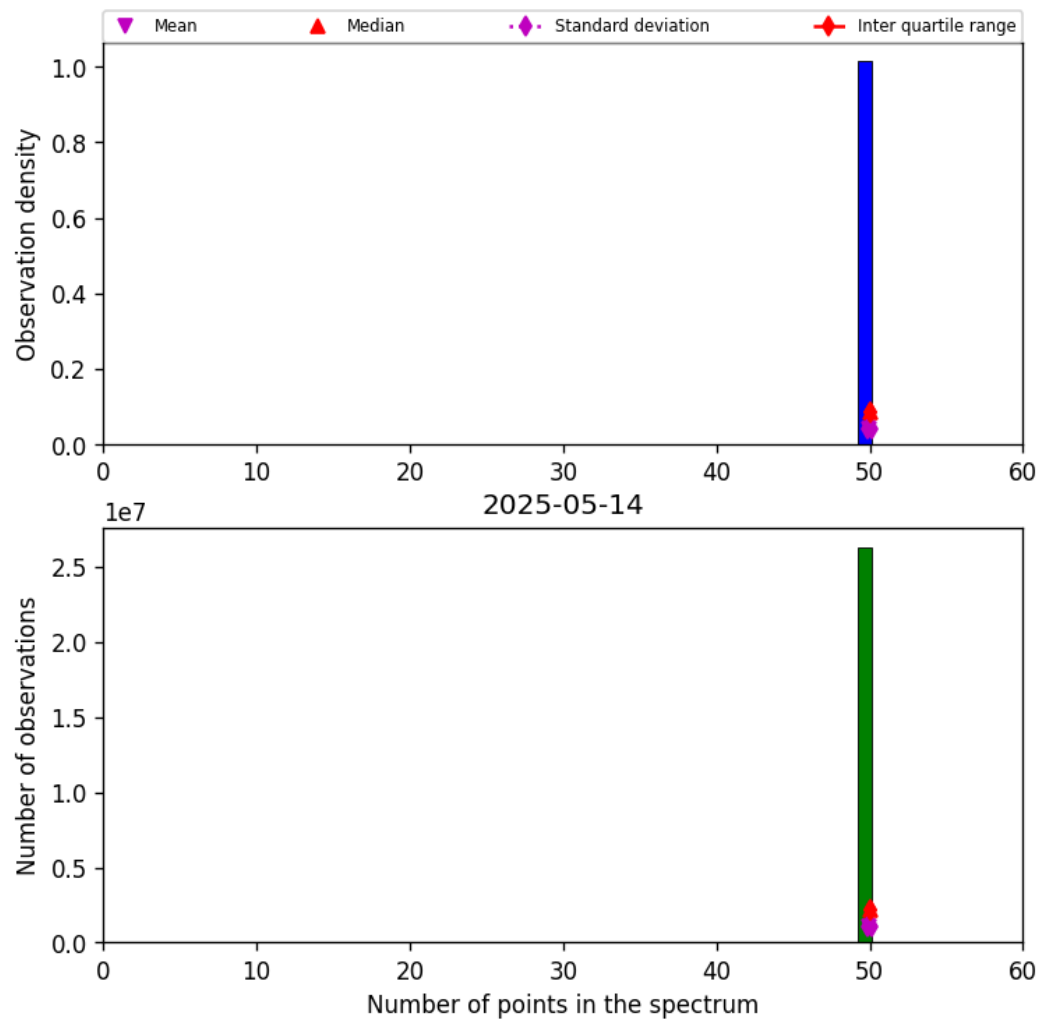
Figure 44: Histogram of "Number of points in the spectrum" for 2025-05-13 to 2025-05-15
