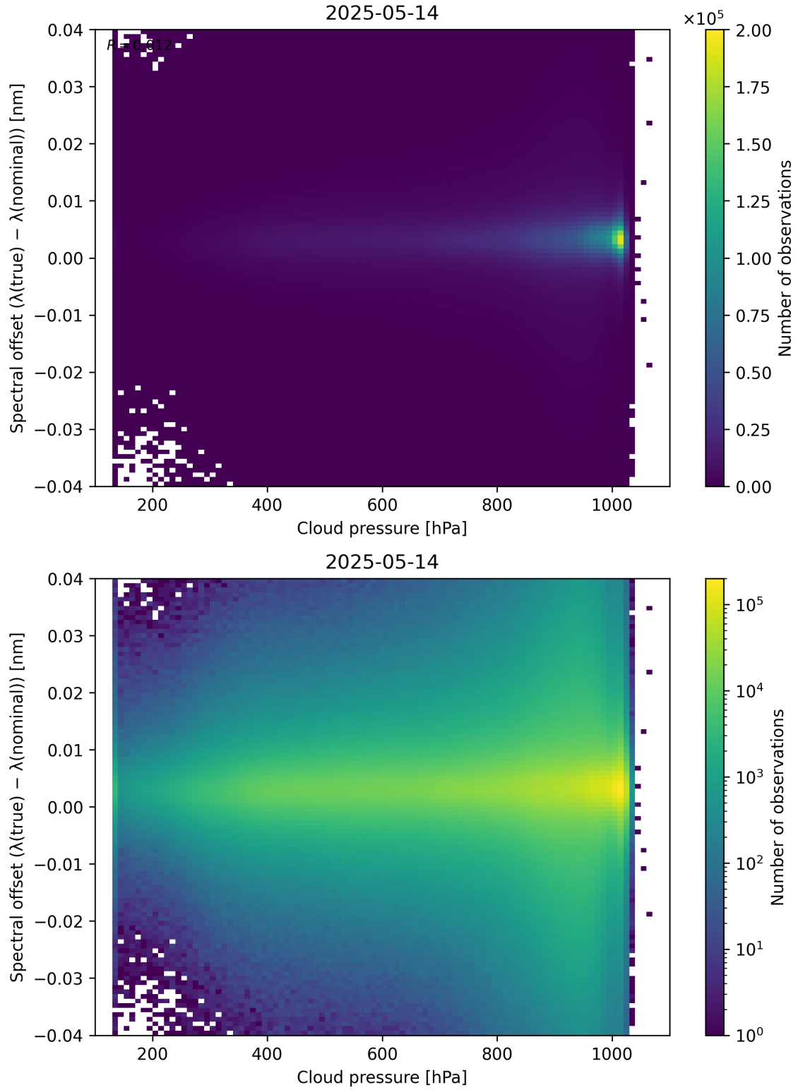
Figure 84: Scatter density plot of “Cloud pressure” against “Spectral offset ( \lambda_{\text{true}} - \lambda_{\text{nominal}} )” for 2025-05-13 to 2025-05-15.
