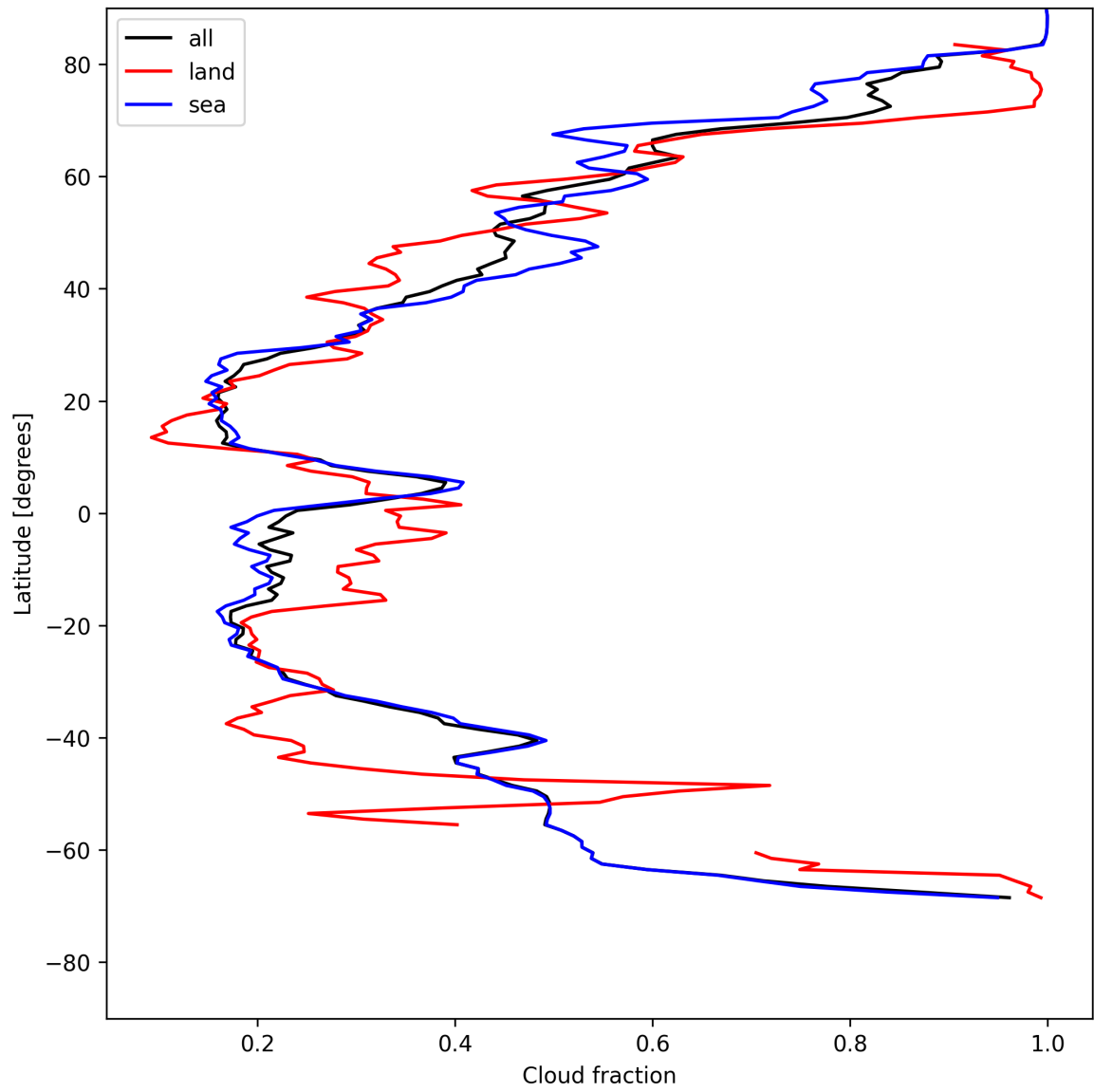
Figure 15: Zonal average of “Cloud fraction” for 2025-05-13 to 2025-05-15.
