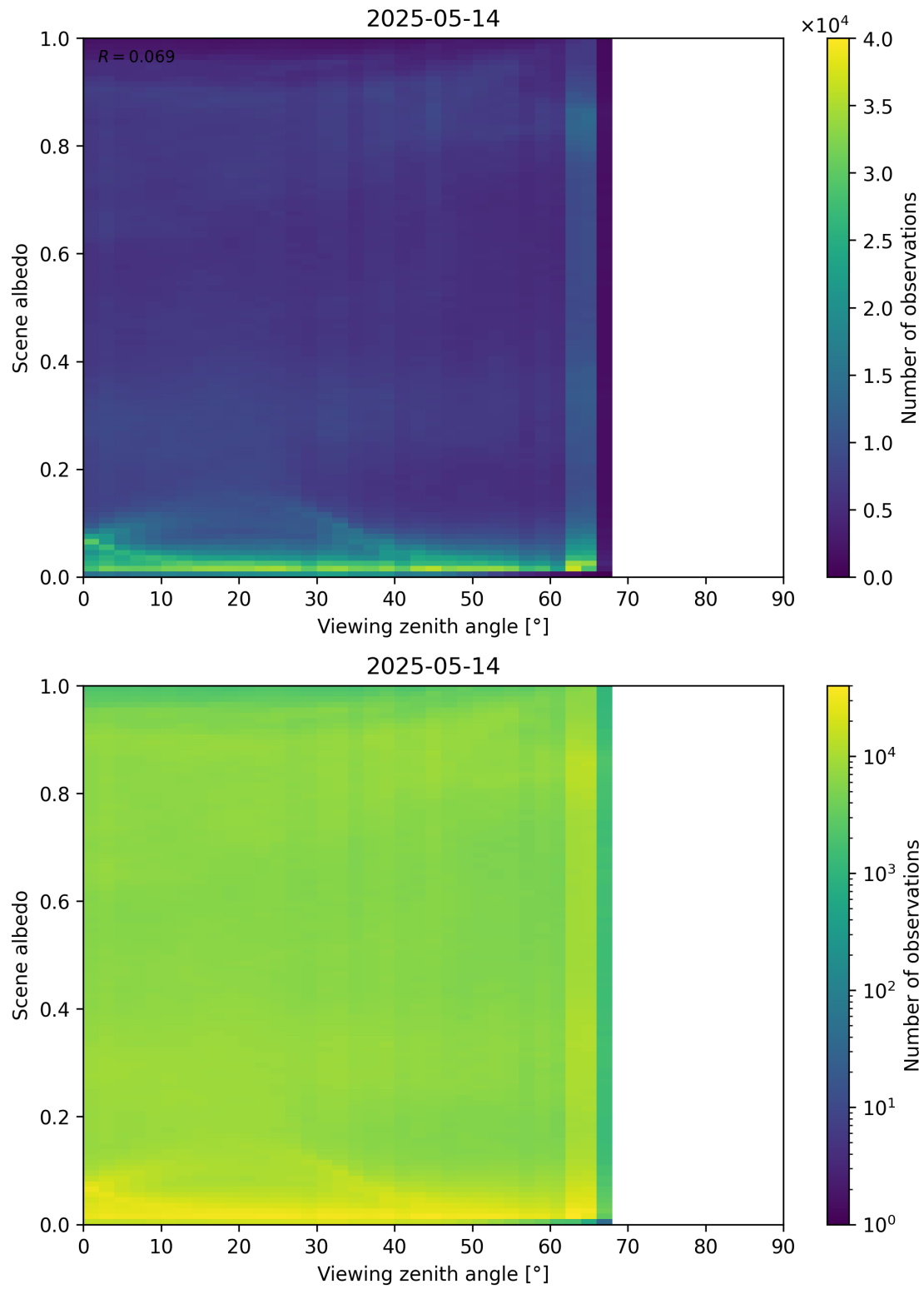
Figure 126: Scatter density plot of “Viewing zenith angle” against “Scene albedo” for 2025-05-13 to 2025-05-15.
