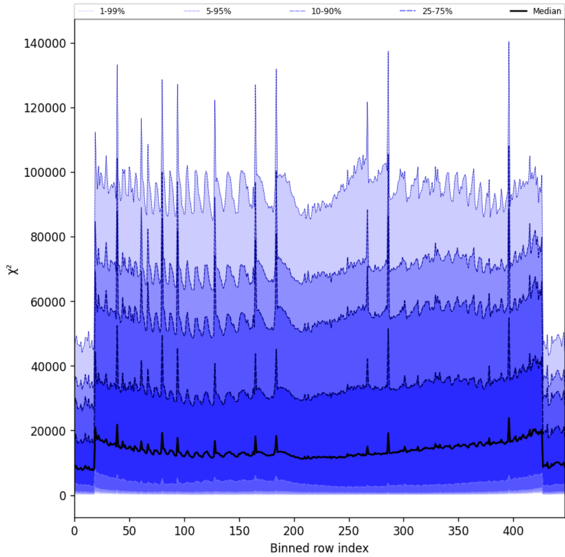
Figure 55: Along track statistics of “ \chi^2 ” for 2025-05-13 to 2025-05-15
