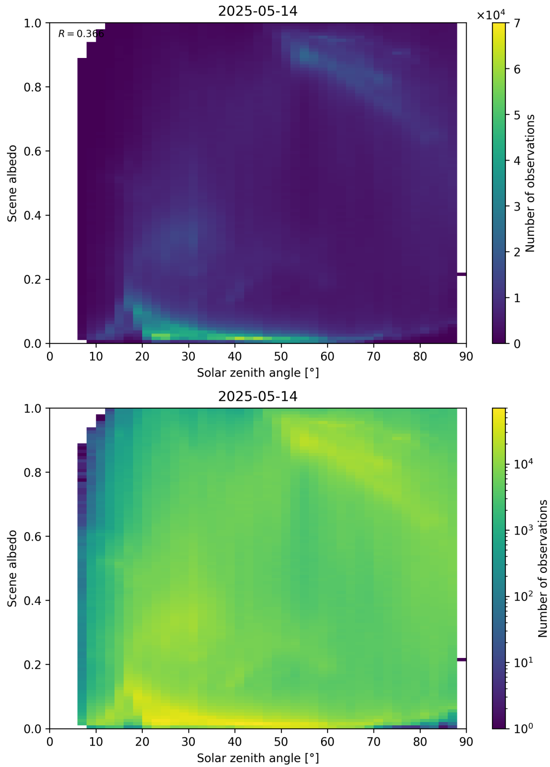
Figure 116: Scatter density plot of “Solar zenith angle” against “Scene albedo” for 2025-05-13 to 2025-05-15.
