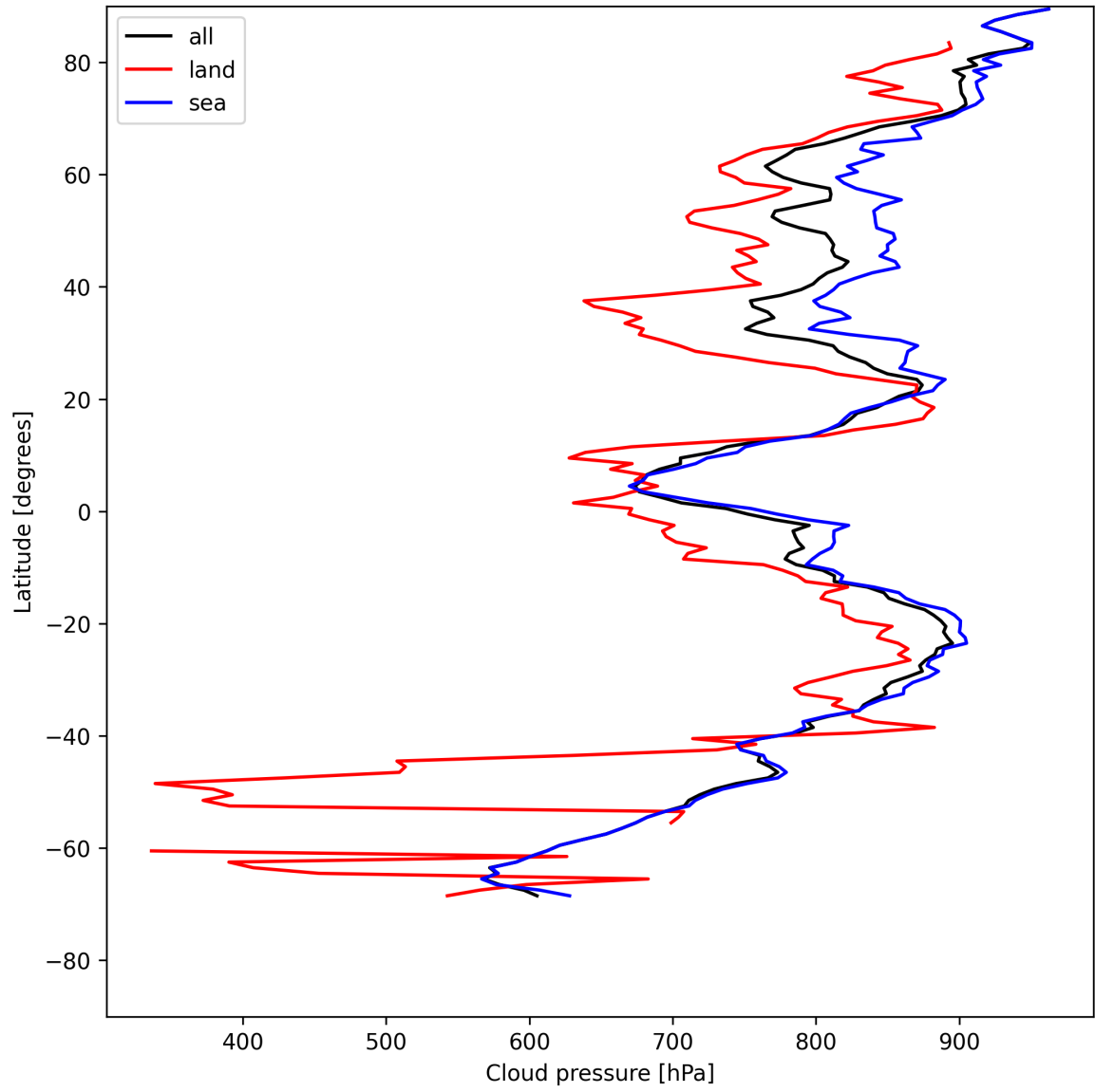
Figure 13: Zonal average of “Cloud pressure” for 2025-05-13 to 2025-05-15.
