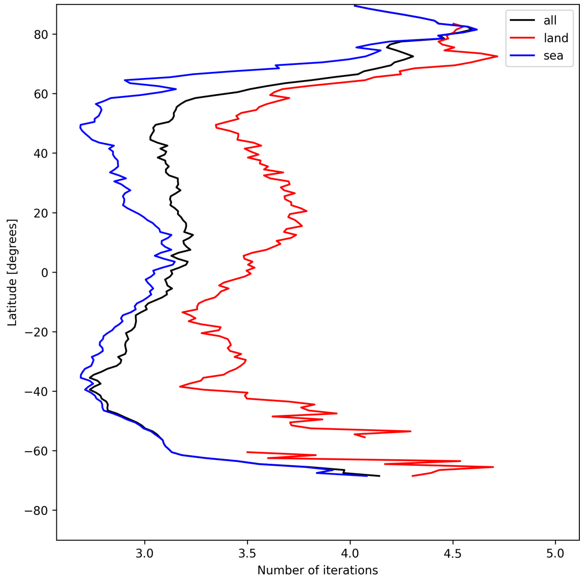
Figure 22: Zonal average of “Number of iterations” for 2025-05-13 to 2025-05-15.
