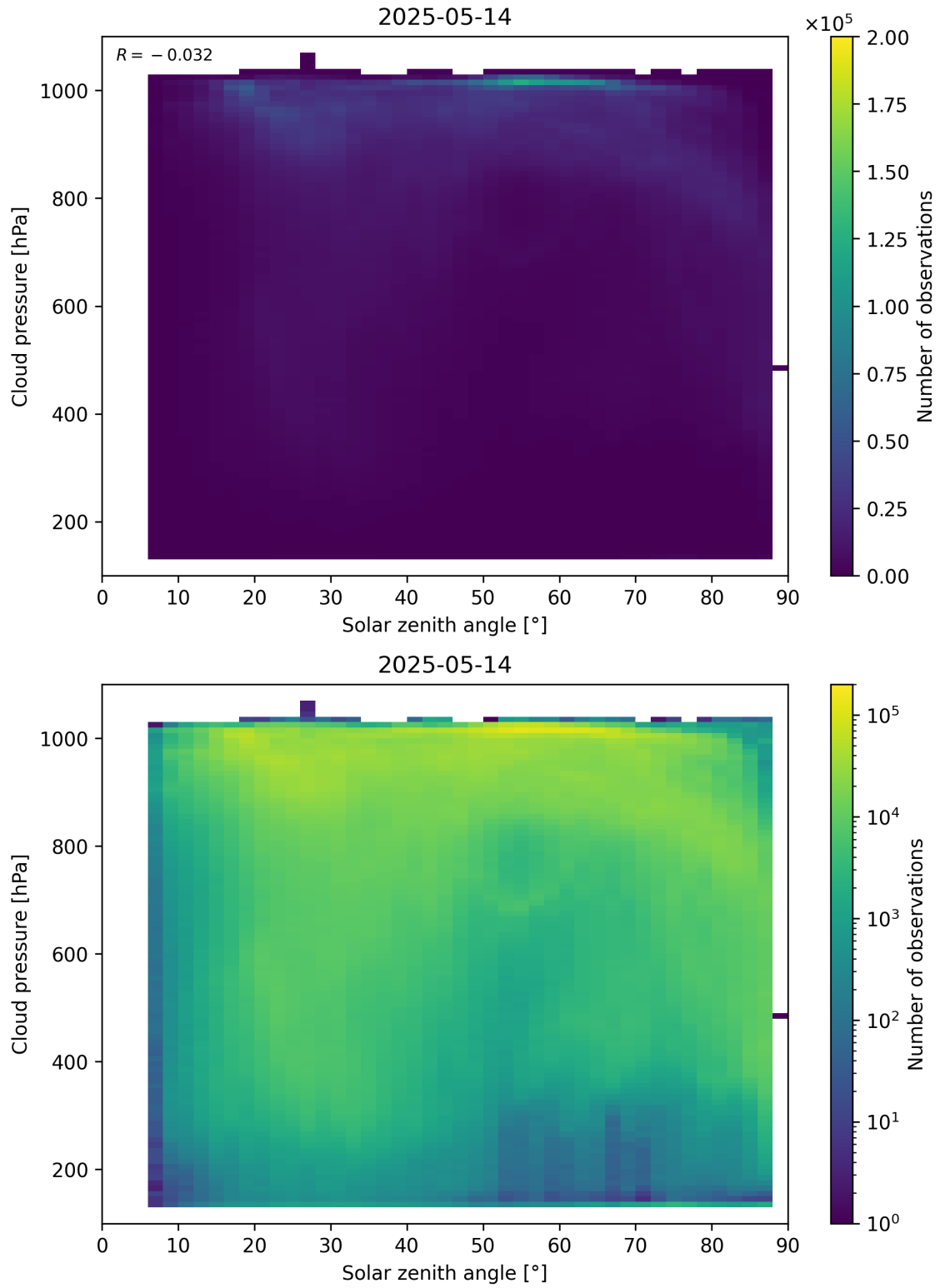
Figure 111: Scatter density plot of “Solar zenith angle” against “Cloud pressure” for 2025-05-13 to 2025-05-15.
