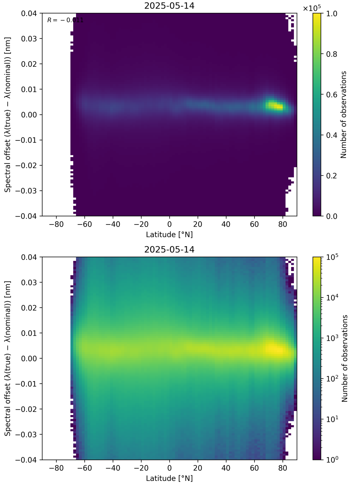
Figure 96: Scatter density plot of “Latitude” against “Spectral offset ( \lambda_{\text{true}} - \lambda_{\text{nominal}} )” for 2025-05-13 to 2025-05-15.
