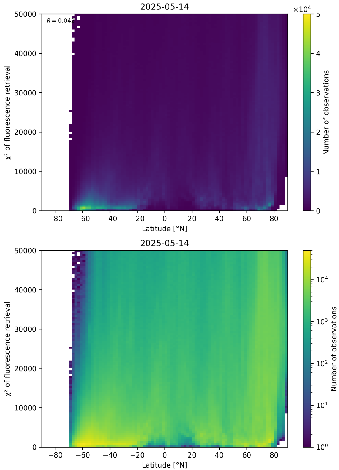
Figure 89: Scatter density plot of “Latitude” against “ \chi^2 of fluorescence retrieval” for 2025-05-13 to 2025-05-15.
