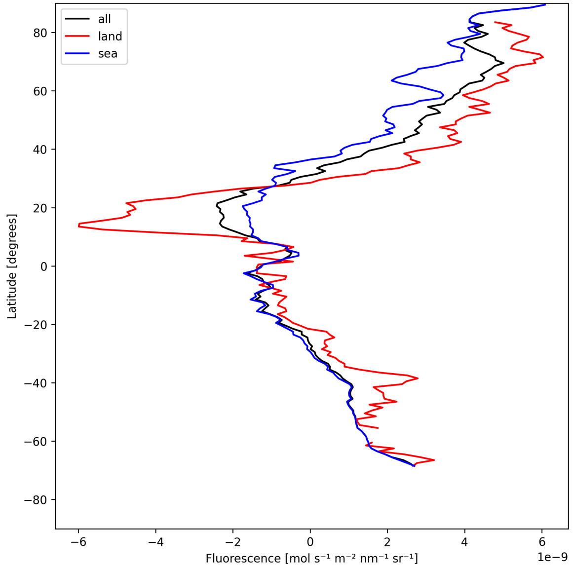
Figure 23: Zonal average of “Fluorescence” for 2025-05-13 to 2025-05-15.
