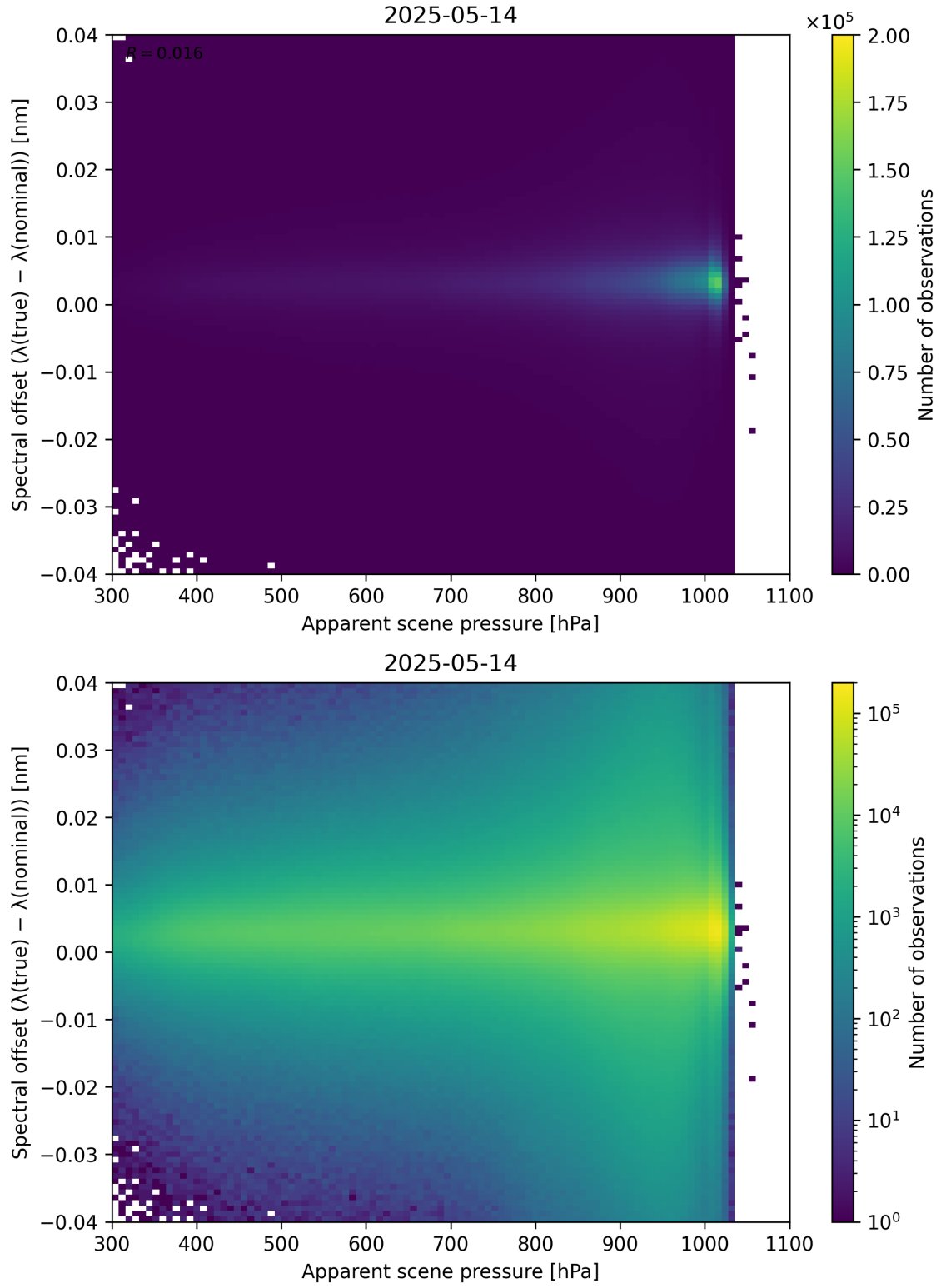
Figure 67: Scatter density plot of “Apparent scene pressure” against “Spectral offset ( \lambda_{\text{true}} - \lambda_{\text{nominal}} )” for 2025-05-13 to 2025-05-15.
