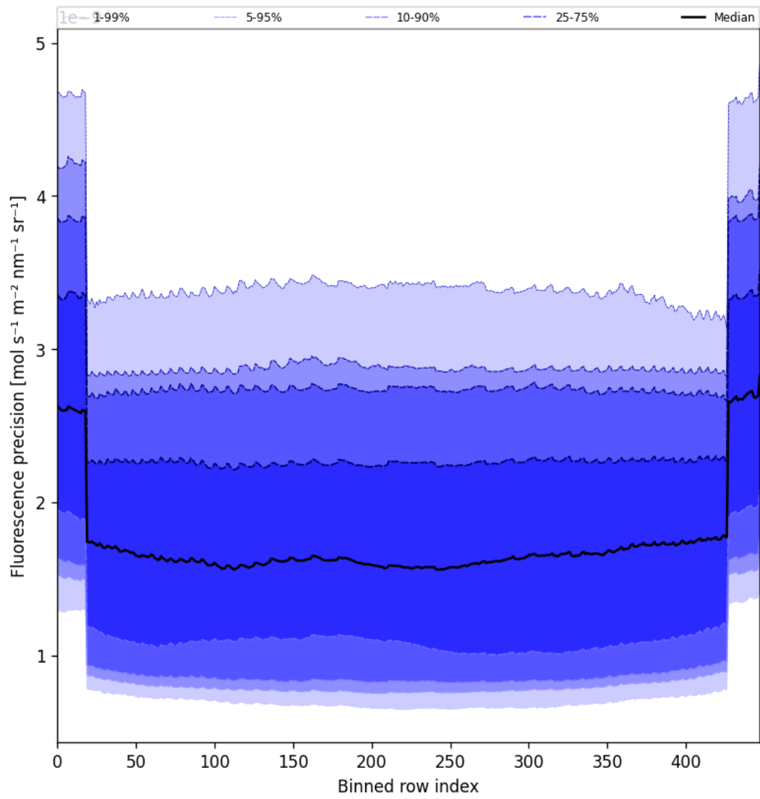
Figure 58: Along track statistics of “Fluorescence precision” for 2025-05-13 to 2025-05-15
