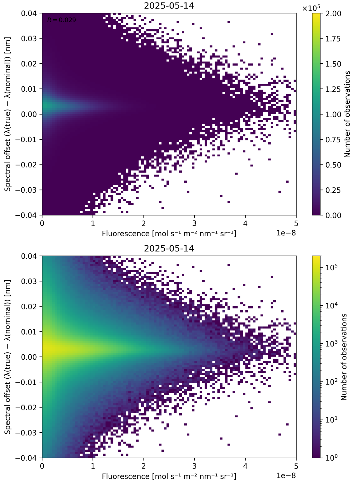
Figure 87: Scatter density plot of “Fluorescence” against “Spectral offset ( \lambda_{\text{true}} - \lambda_{\text{nominal}} )” for 2025-05-13 to 2025-05-15.
