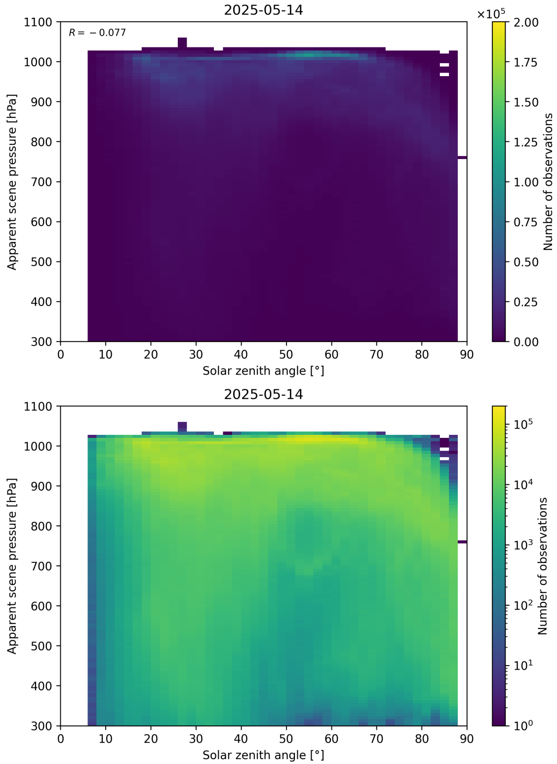
Figure 108: Scatter density plot of “Solar zenith angle” against “Apparent scene pressure” for 2025-05-13 to 2025-05-15.
