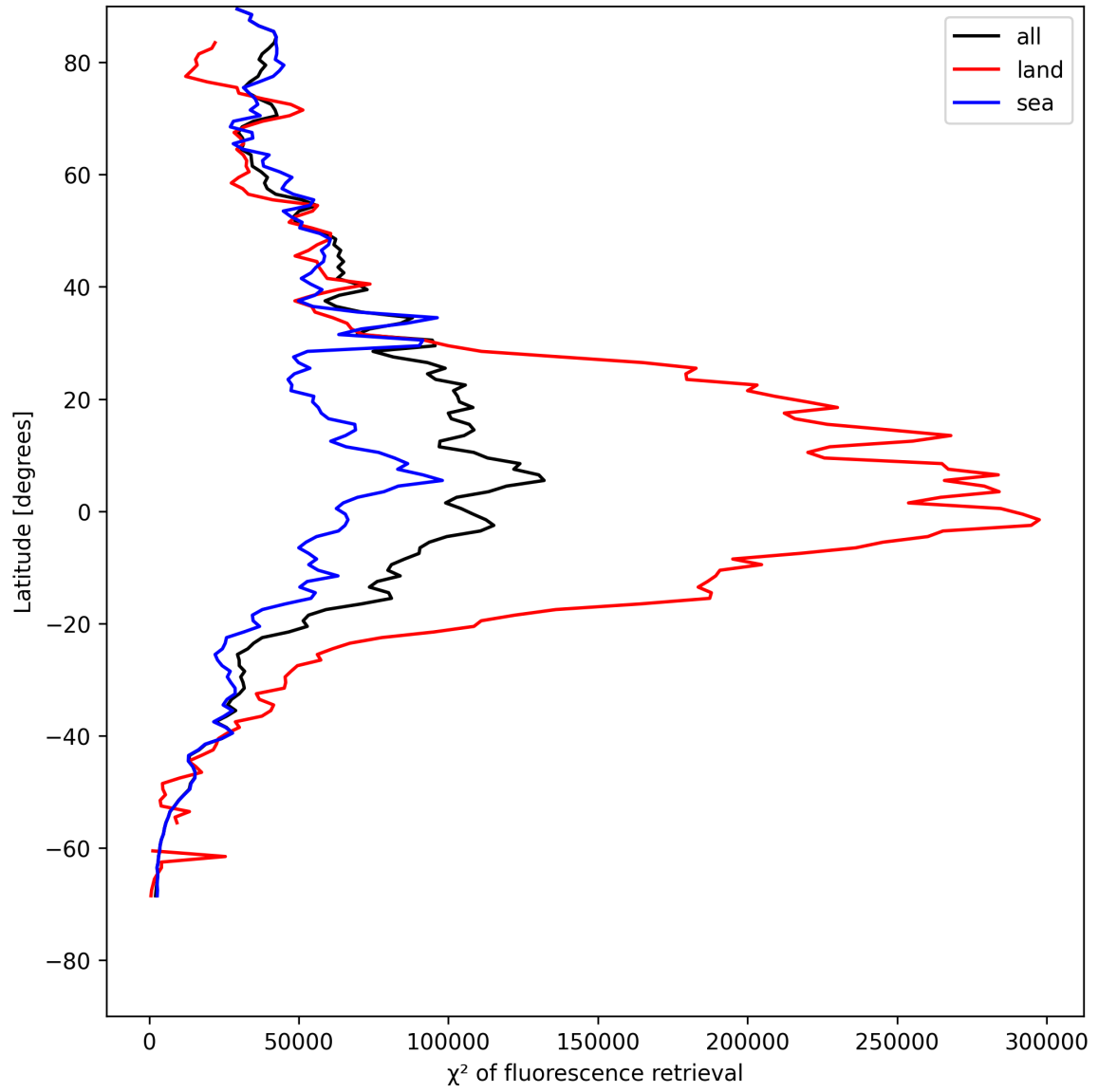
Figure 25: Zonal average of “ \chi^2 of fluorescence retrieval” for 2025-05-13 to 2025-05-15.
