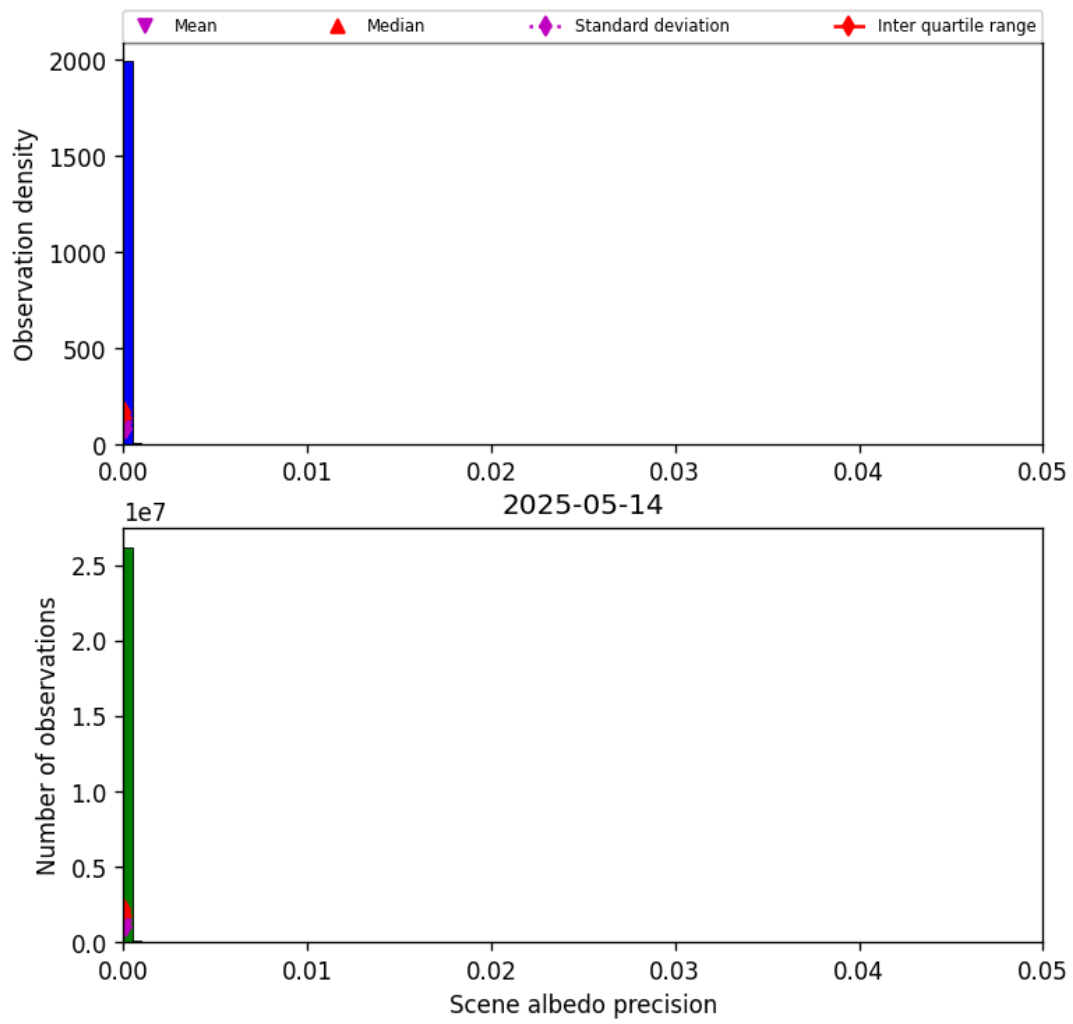
Figure 35: Histogram of “Scene albedo precision” for 2025-05-13 to 2025-05-15
