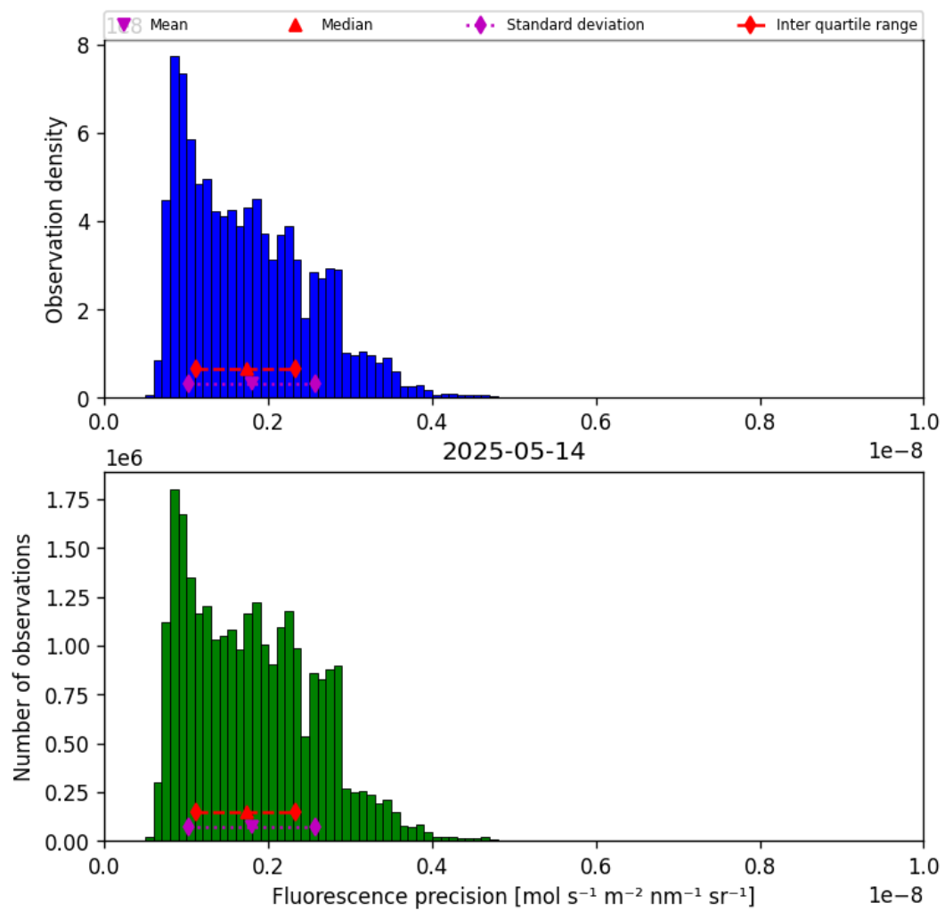
Figure 41: Histogram of “Fluorescence precision” for 2025-05-13 to 2025-05-15
