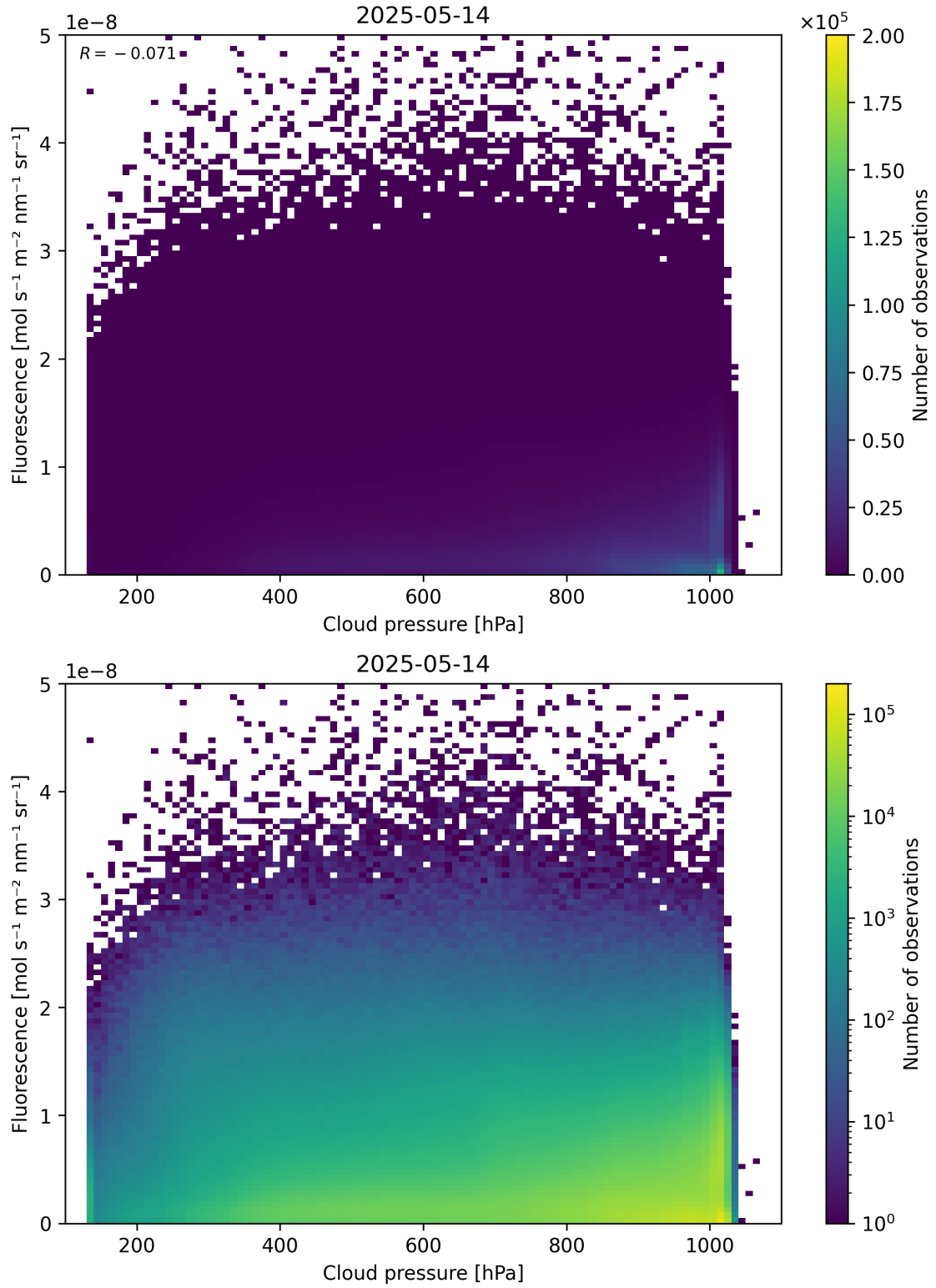
Figure 80: Scatter density plot of “Cloud pressure” against “Fluorescence” for 2025-05-13 to 2025-05-15.
