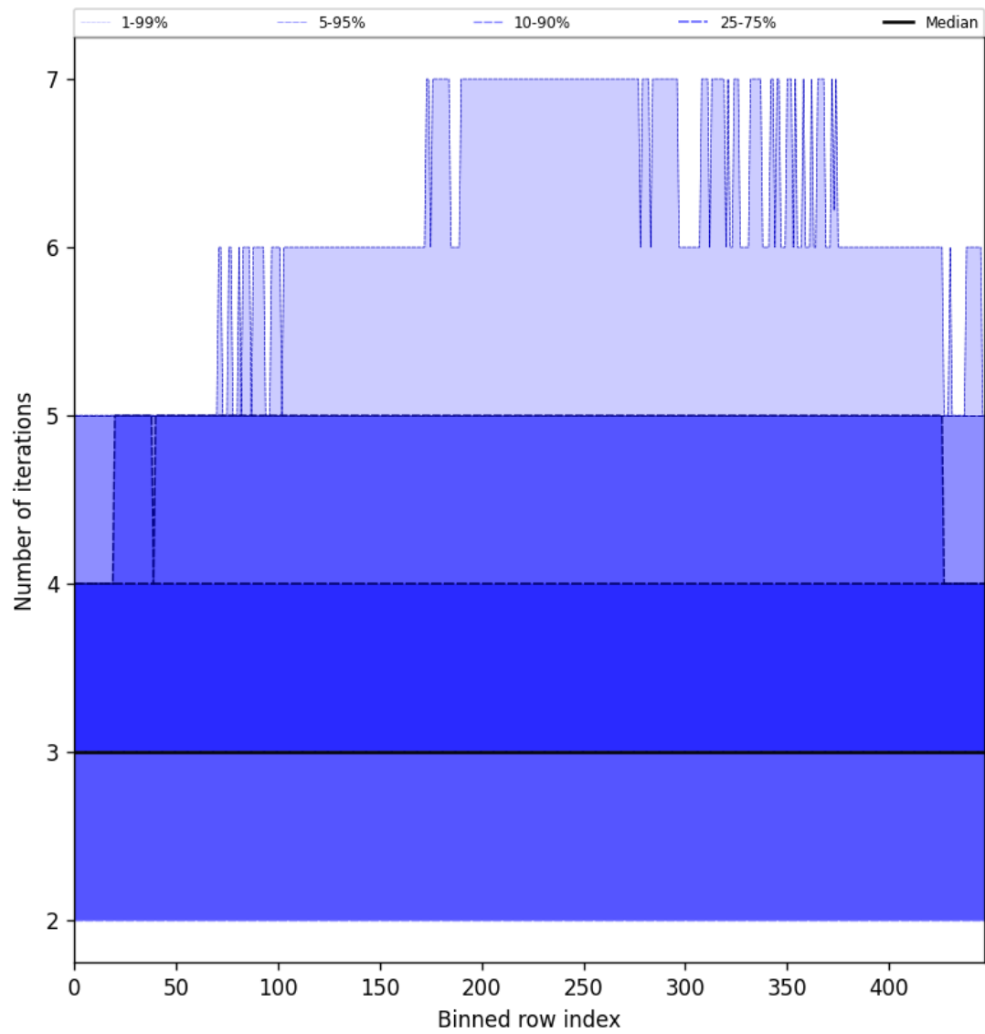
Figure 56: Along track statistics of “Number of iterations” for 2025-05-13 to 2025-05-15
