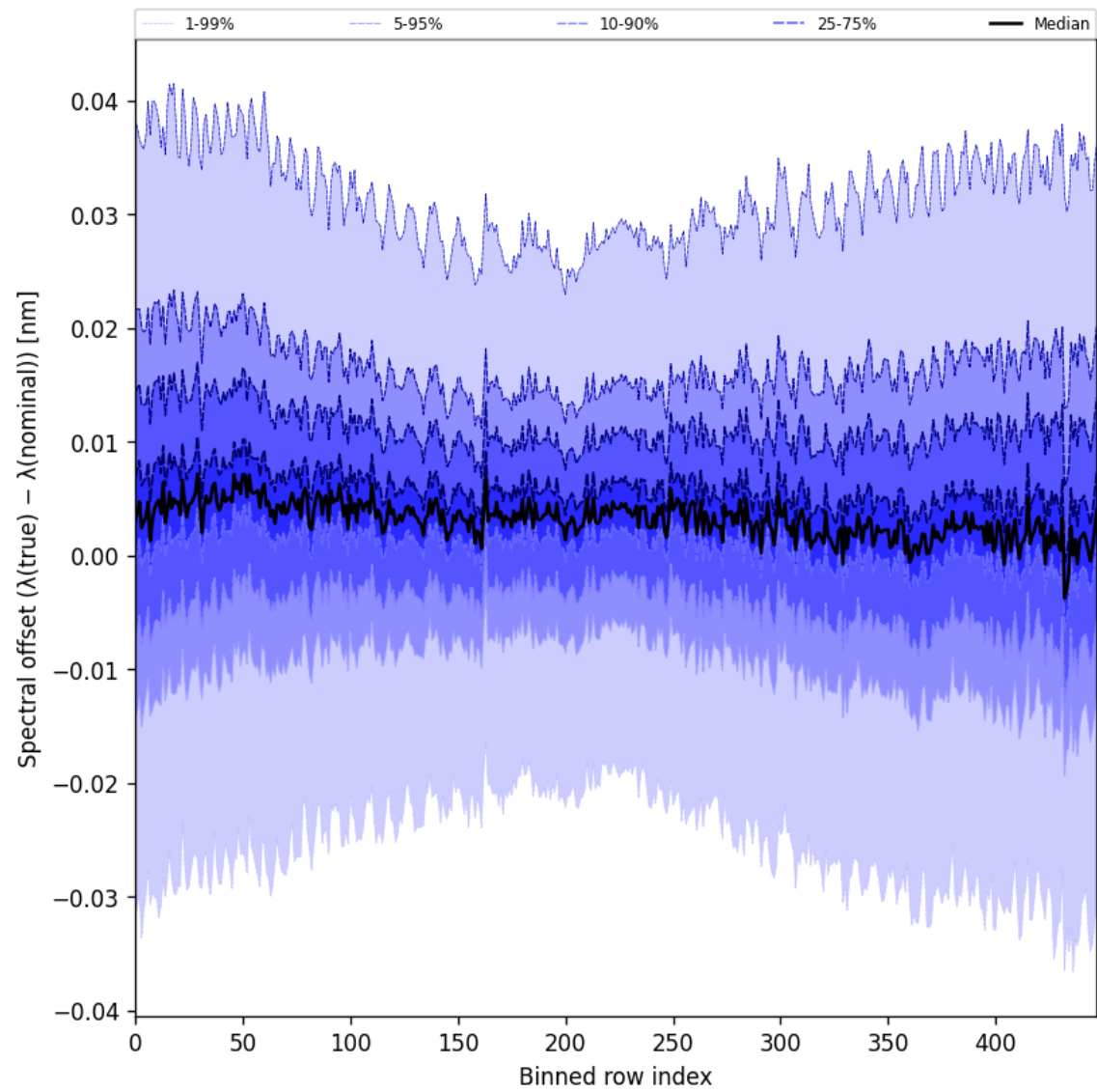
Figure 62: Along track statistics of “Spectral offset ( \lambda_{\text{true}} - \lambda_{\text{nominal}} )” for 2025-05-13 to 2025-05-15
