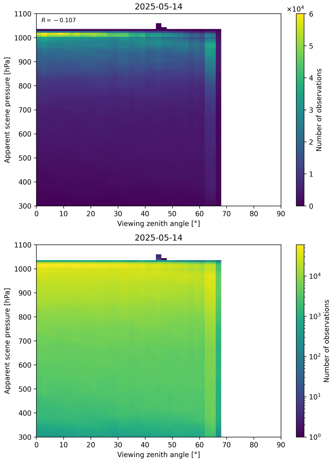
Figure 118: Scatter density plot of “Viewing zenith angle” against “Apparent scene pressure” for 2025-05-13 to 2025-05-15.
