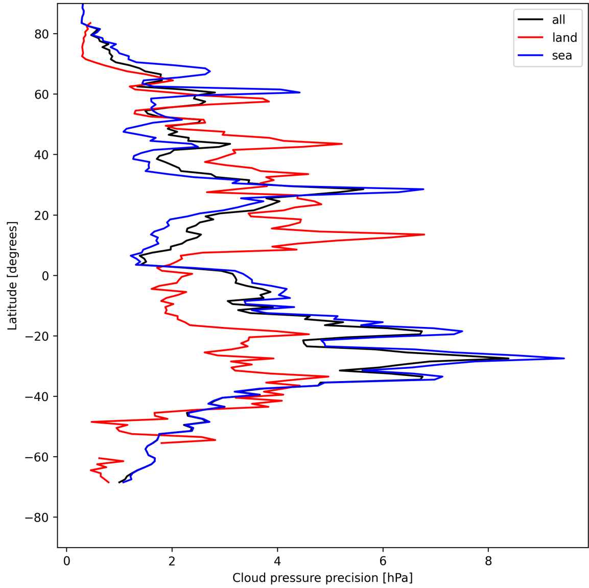
Figure 14: Zonal average of “Cloud pressure precision” for 2025-05-13 to 2025-05-15.
