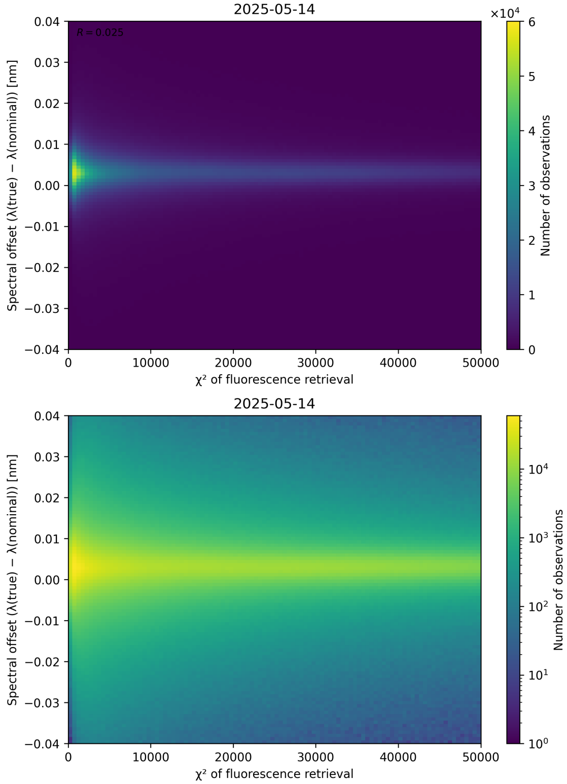
Figure 69: Scatter density plot of “ \chi^2 of fluorescence retrieval” against “Spectral offset ( \lambda_{\text{true}} - \lambda_{\text{nominal}} )” for 2025-05-13 to 2025-05-15.
