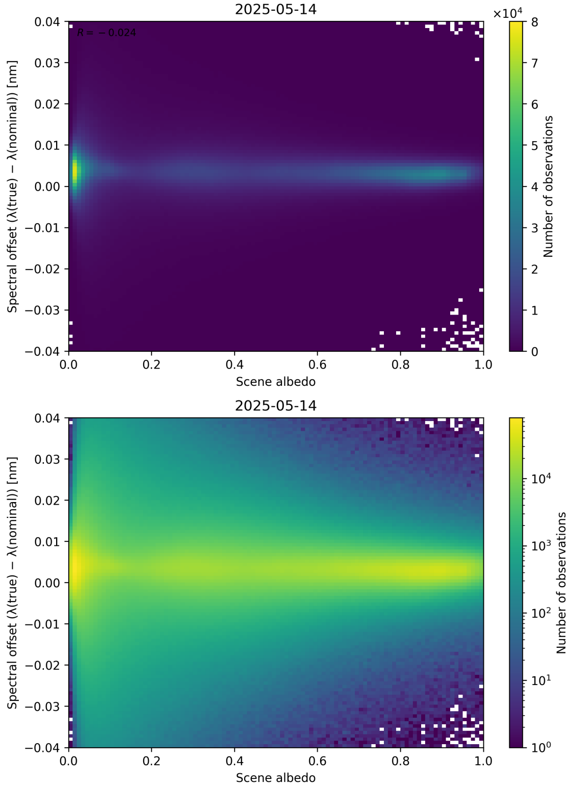
Figure 107: Scatter density plot of “Scene albedo” against “Spectral offset ( \lambda_{\text{true}} - \lambda_{\text{nominal}} )” for 2025-05-13 to 2025-05-15.
