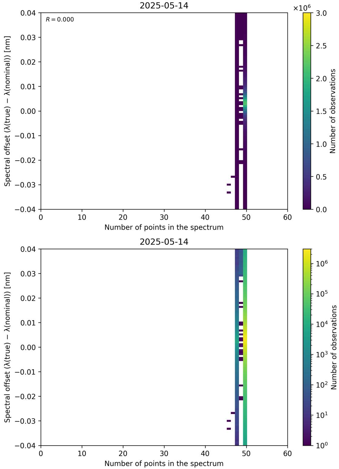
Figure 101: Scatter density plot of “Number of points in the spectrum” against “Spectral offset ( \lambda_{\text{true}} - \lambda_{\text{nominal}} )” for 2025-05-13 to 2025-05-15.
