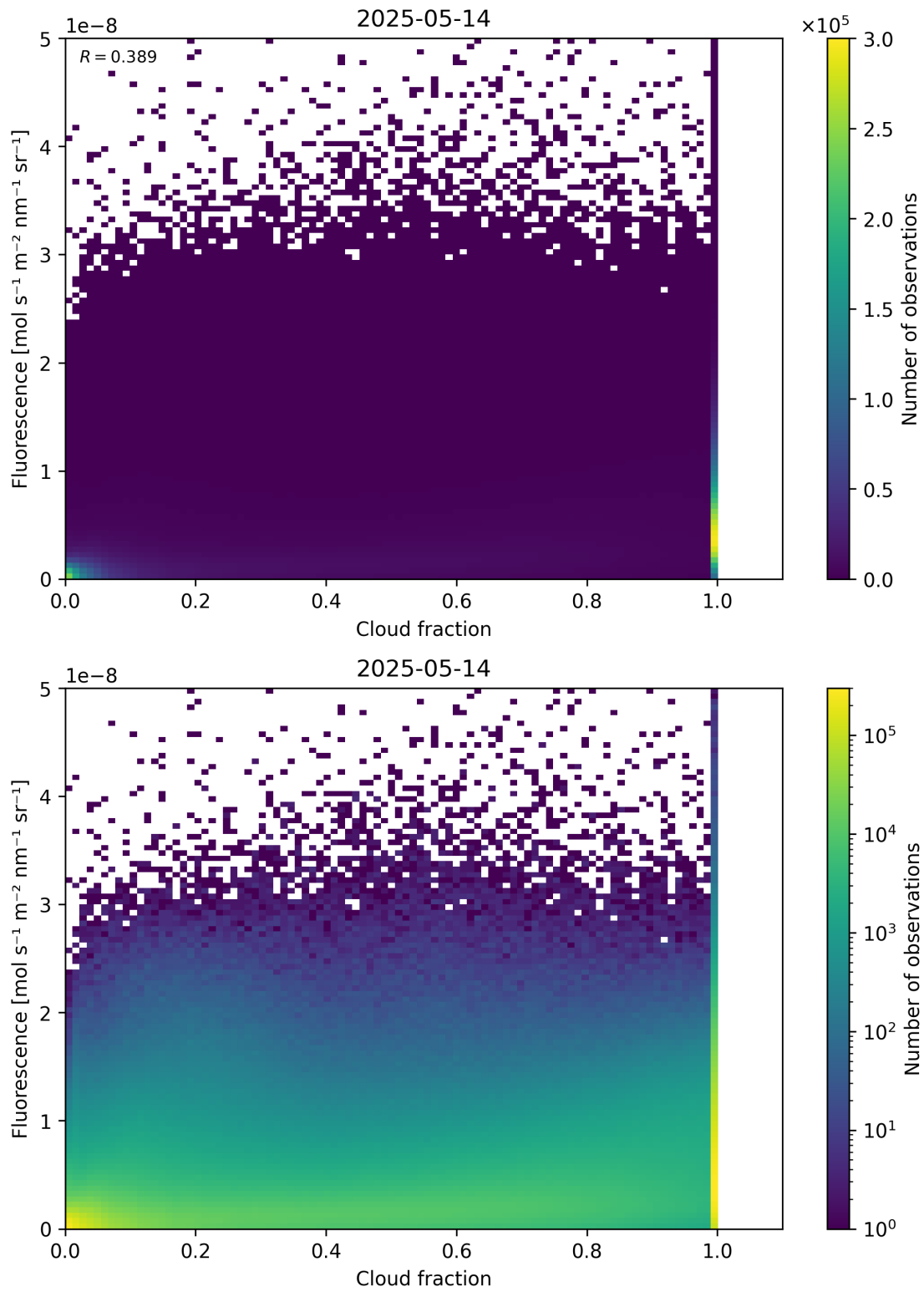
Figure 72: Scatter density plot of “Cloud fraction” against “Fluorescence” for 2025-05-13 to 2025-05-15.
