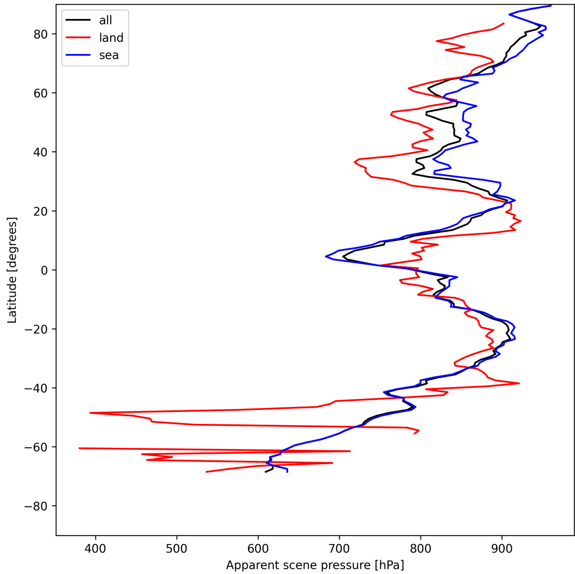
Figure 19: Zonal average of “Apparent scene pressure” for 2025-05-13 to 2025-05-15.
