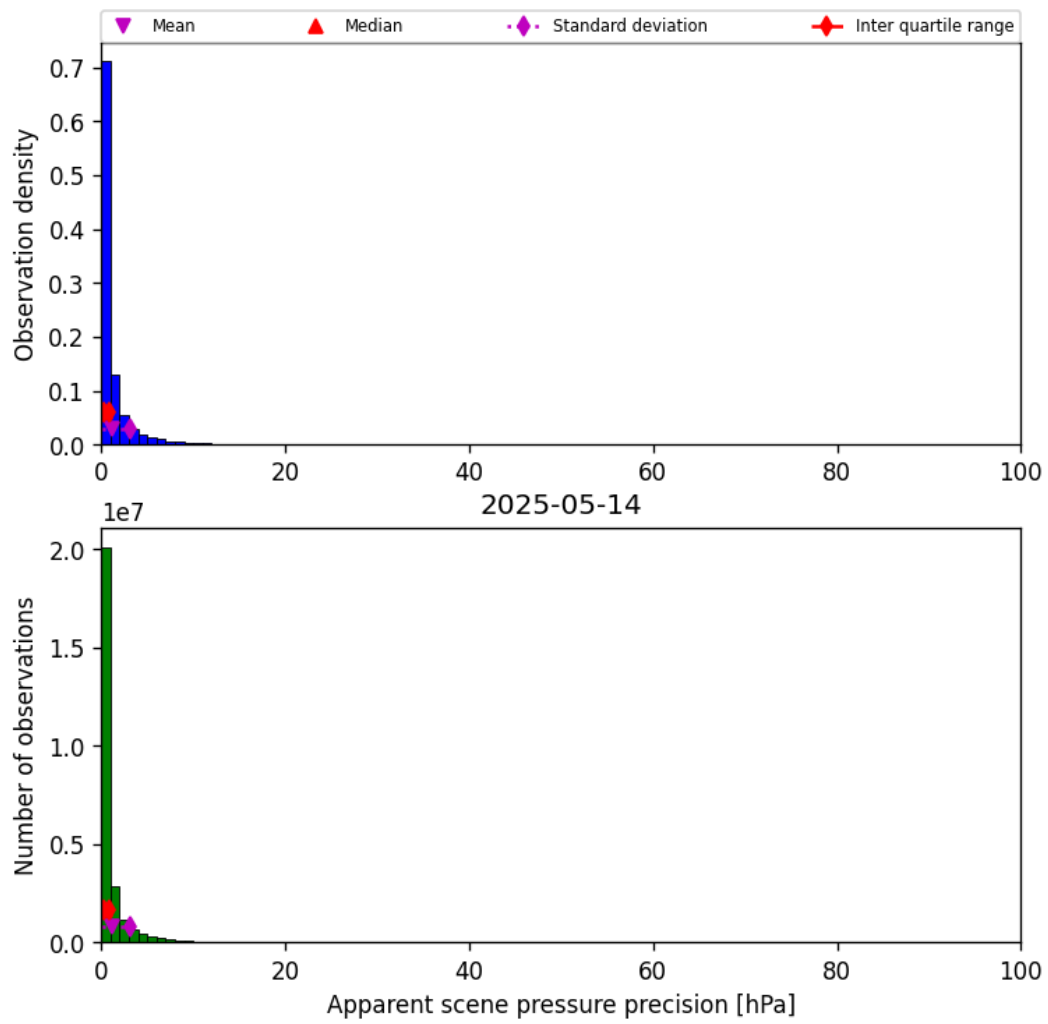
Figure 37: Histogram of “Apparent scene pressure precision” for 2025-05-13 to 2025-05-15
