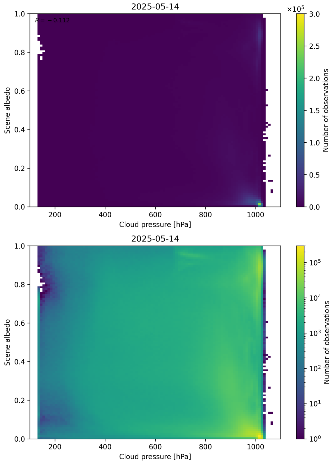
Figure 83: Scatter density plot of “Cloud pressure” against “Scene albedo” for 2025-05-13 to 2025-05-15.
