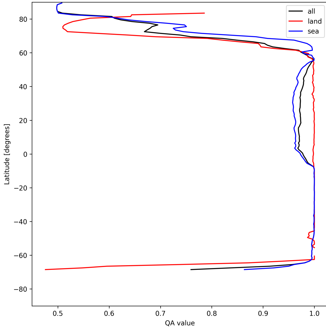
Figure 12: Zonal average of “QA value” for 2025-05-13 to 2025-05-15.
