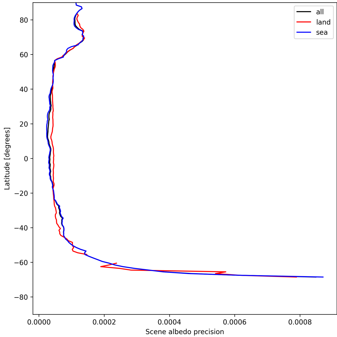
Figure 18: Zonal average of “Scene albedo precision” for 2025-05-13 to 2025-05-15.
