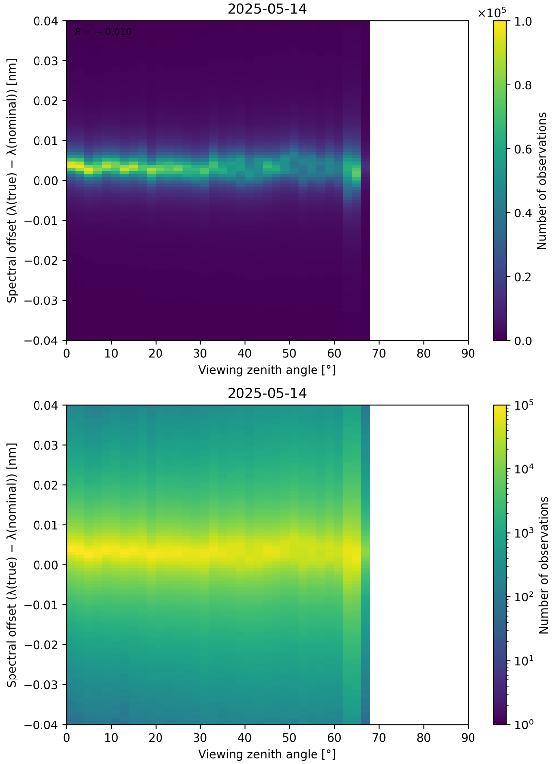
Figure 128: Scatter density plot of “Viewing zenith angle” against “Spectral offset ( \lambda_{\text{true}} - \lambda_{\text{nominal}} )” for 2025-05-13 to 2025-05-15.
