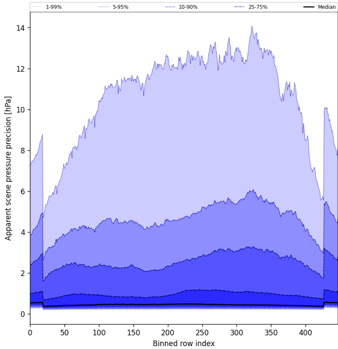
Figure 54: Along track statistics of “Apparent scene pressure precision” for 2025-05-13 to 2025-05-15
