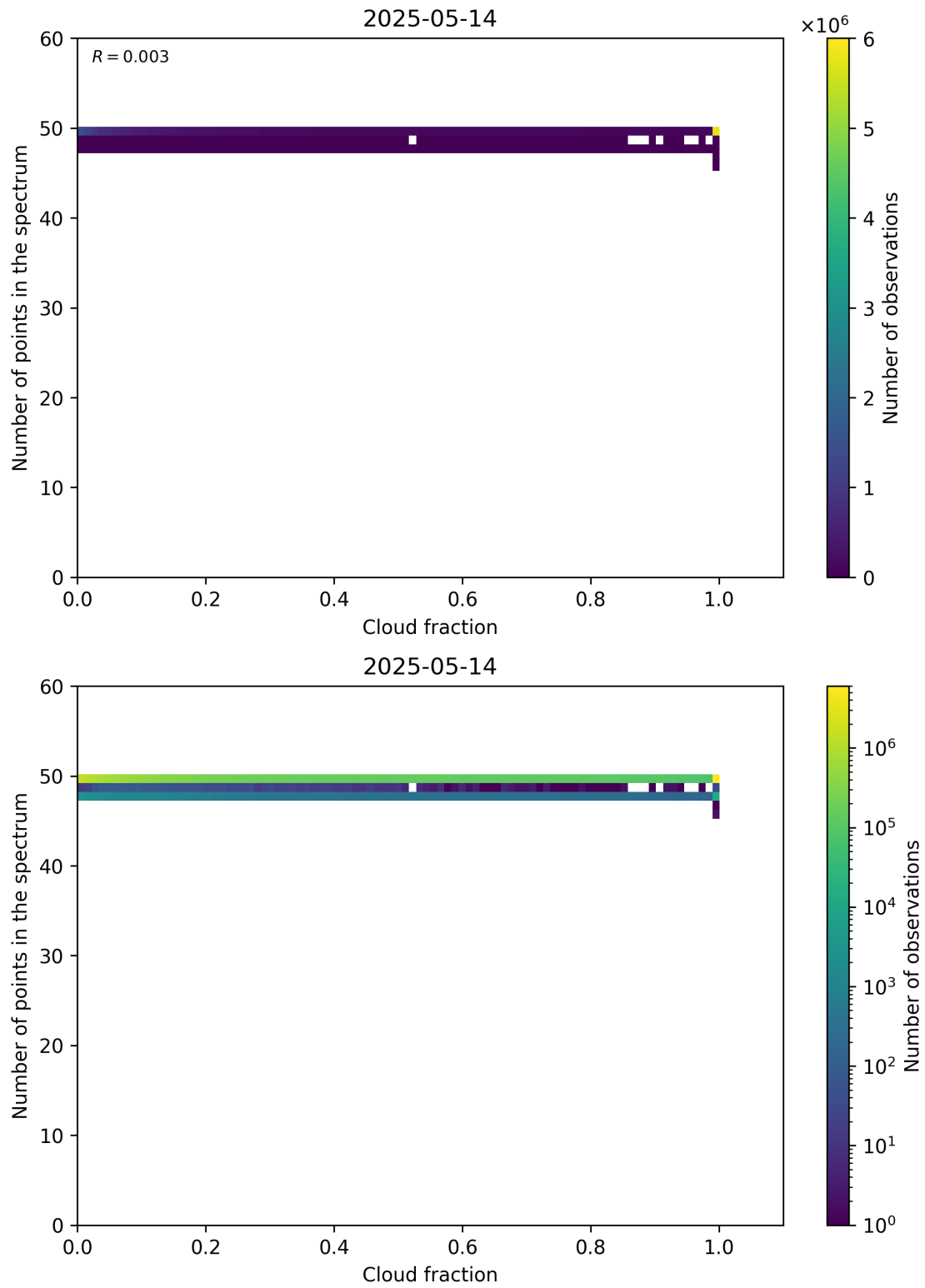
Figure 74: Scatter density plot of “Cloud fraction” against “Number of points in the spectrum” for 2025-05-13 to 2025-05-15.
