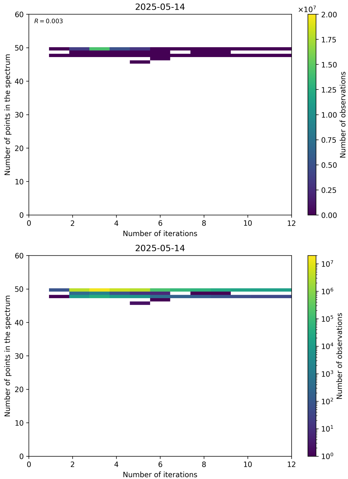
Figure 99: Scatter density plot of “Number of iterations” against “Number of points in the spectrum” for 2025-05-13 to 2025-05-15.
