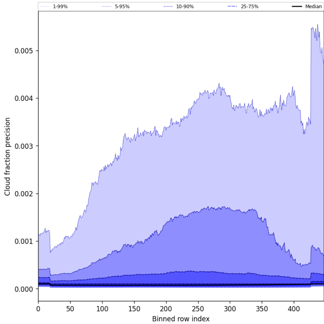
Figure 50: Along track statistics of “Cloud fraction precision” for 2025-05-13 to 2025-05-15
