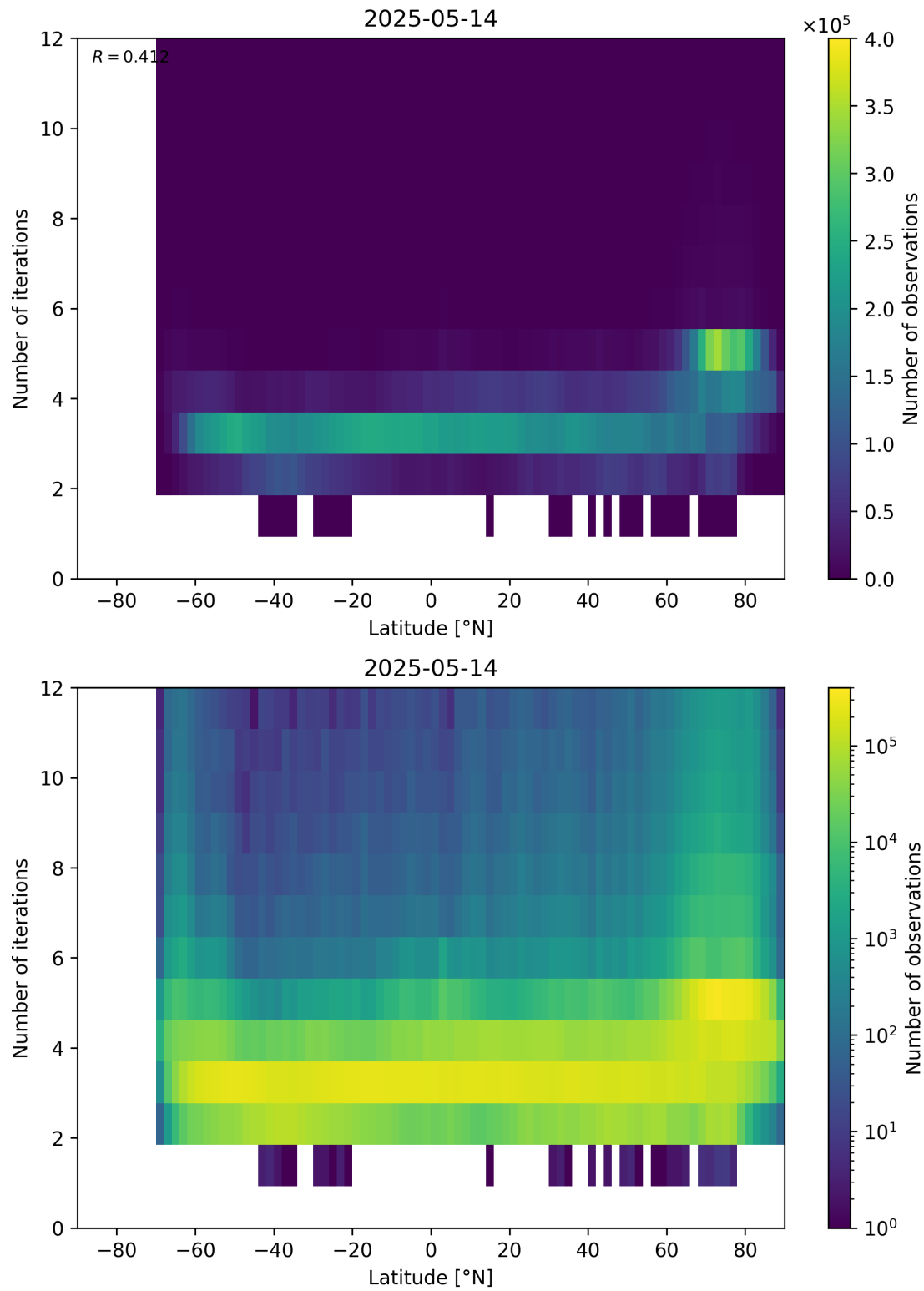
Figure 93: Scatter density plot of “Latitude” against “Number of iterations” for 2025-05-13 to 2025-05-15.
