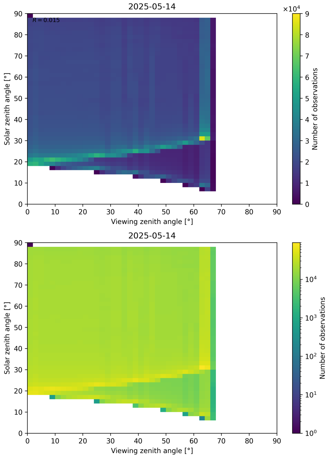
Figure 127: Scatter density plot of “Viewing zenith angle” against “Solar zenith angle” for 2025-05-13 to 2025-05-15.
