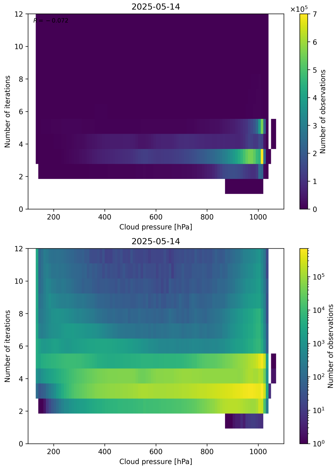
Figure 81: Scatter density plot of “Cloud pressure” against “Number of iterations” for 2025-05-13 to 2025-05-15.
