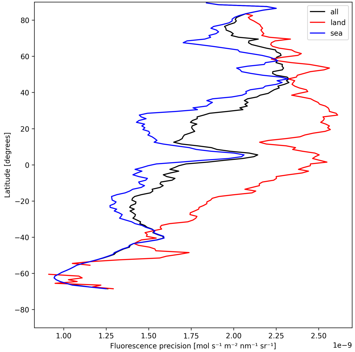
Figure 24: Zonal average of “Fluorescence precision” for 2025-05-13 to 2025-05-15.
