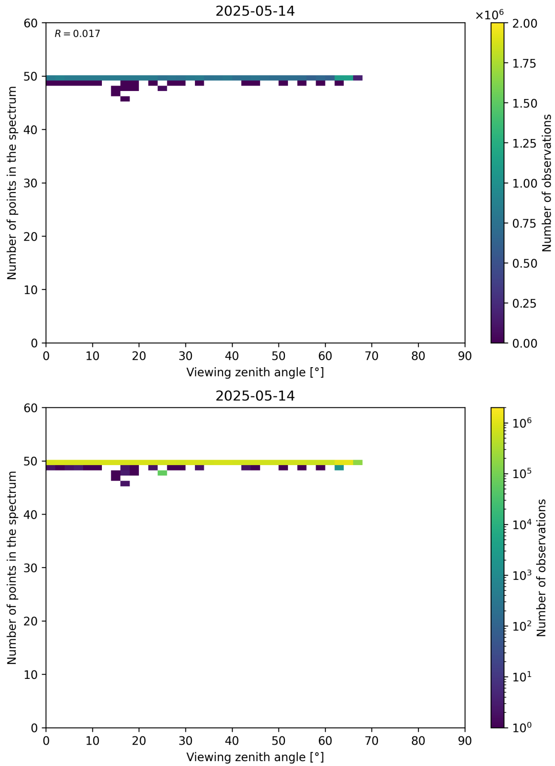
Figure 125: Scatter density plot of “Viewing zenith angle” against “Number of points in the spectrum” for 2025-05-13 to 2025-05-15.
