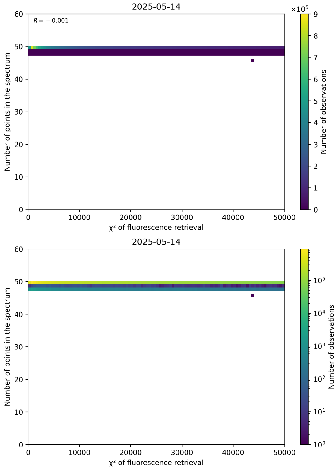
Figure 68: Scatter density plot of “ \chi^2 of fluorescence retrieval” against “Number of points in the spectrum” for 2025-05-13 to 2025-05-15.
