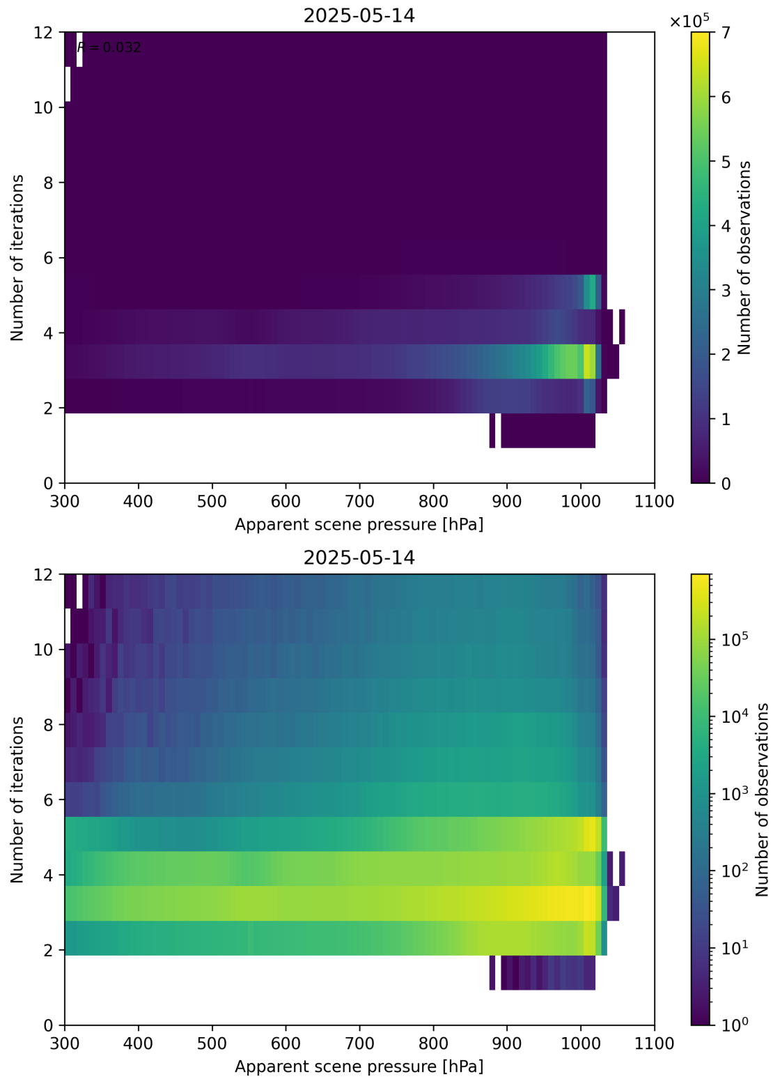
Figure 65: Scatter density plot of “Apparent scene pressure” against “Number of iterations” for 2025-05-13 to 2025-05-15.
