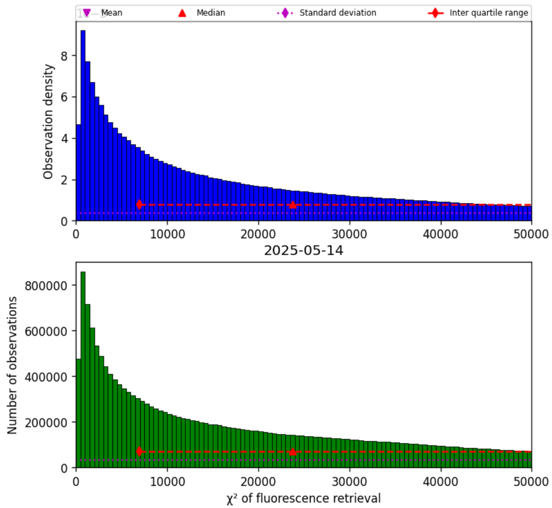
Figure 42: Histogram of “ \chi^2 of fluorescence retrieval” for 2025-05-13 to 2025-05-15
