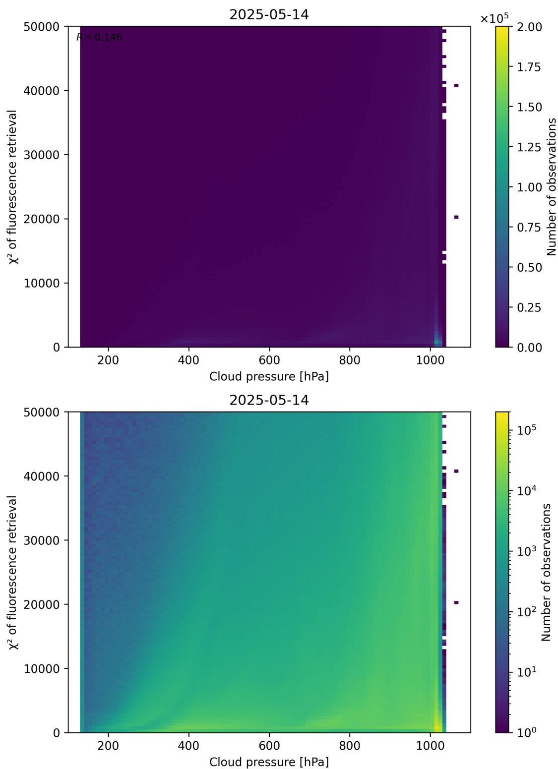
Figure 78: Scatter density plot of “Cloud pressure” against “ \chi^2 of fluorescence retrieval” for 2025-05-13 to 2025-05-15.
