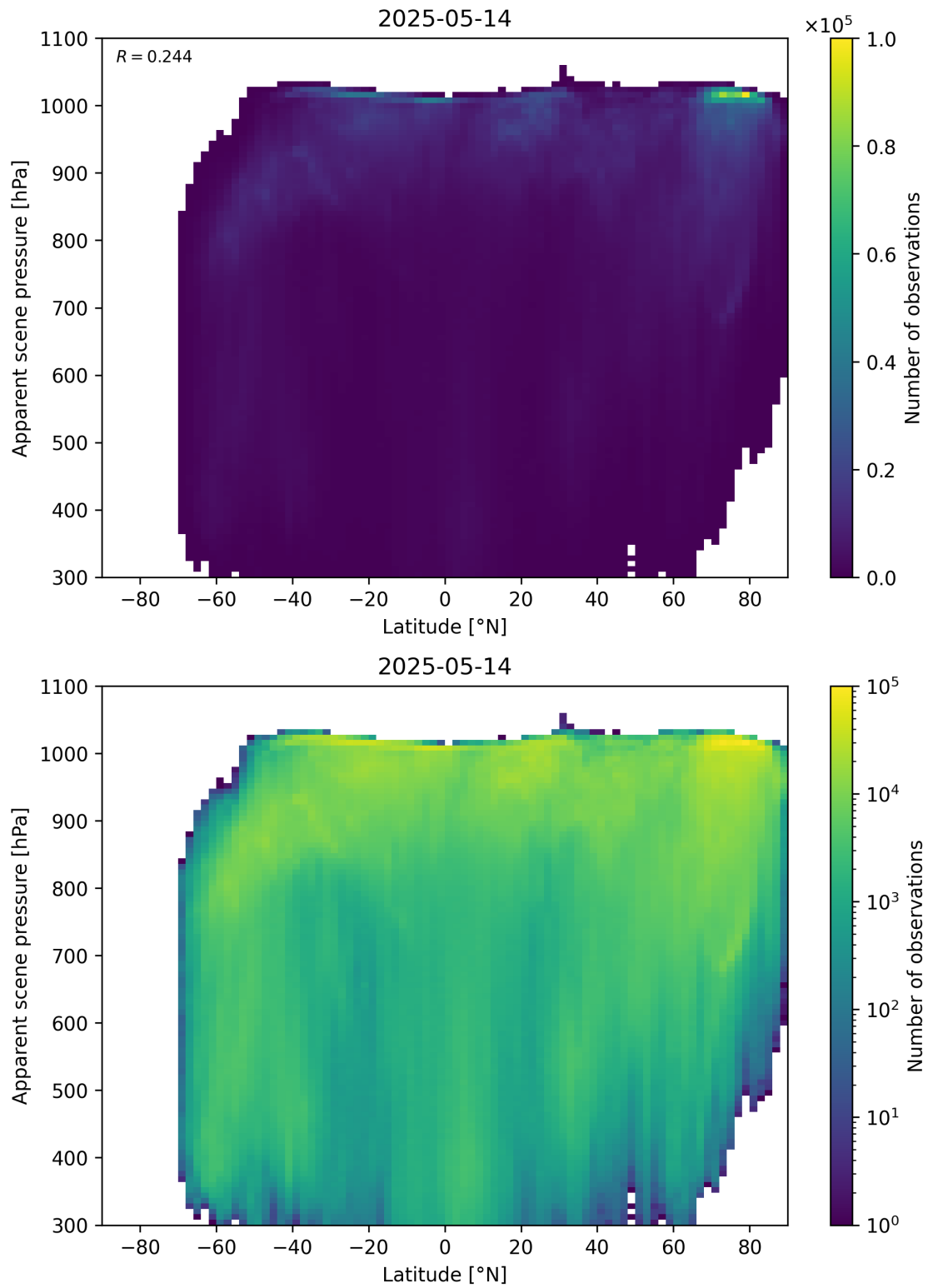
Figure 88: Scatter density plot of “Latitude” against “Apparent scene pressure” for 2025-05-13 to 2025-05-15.
