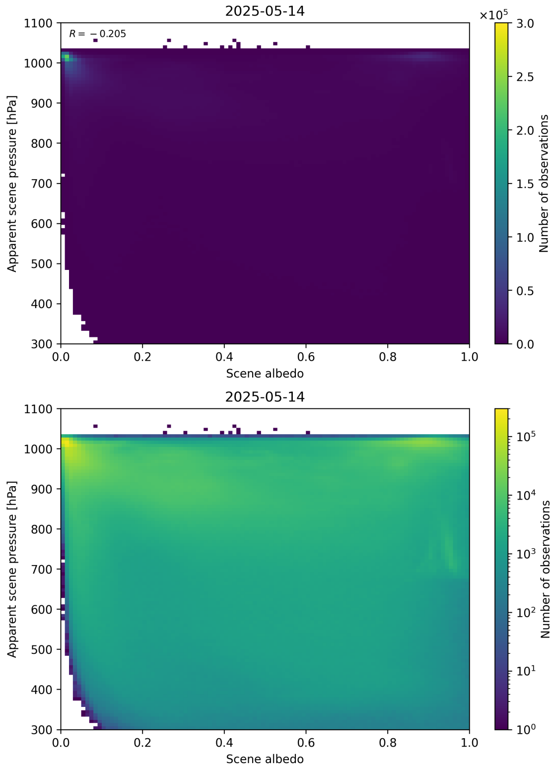
Figure 102: Scatter density plot of “Scene albedo” against “Apparent scene pressure” for 2025-05-13 to 2025-05-15.
