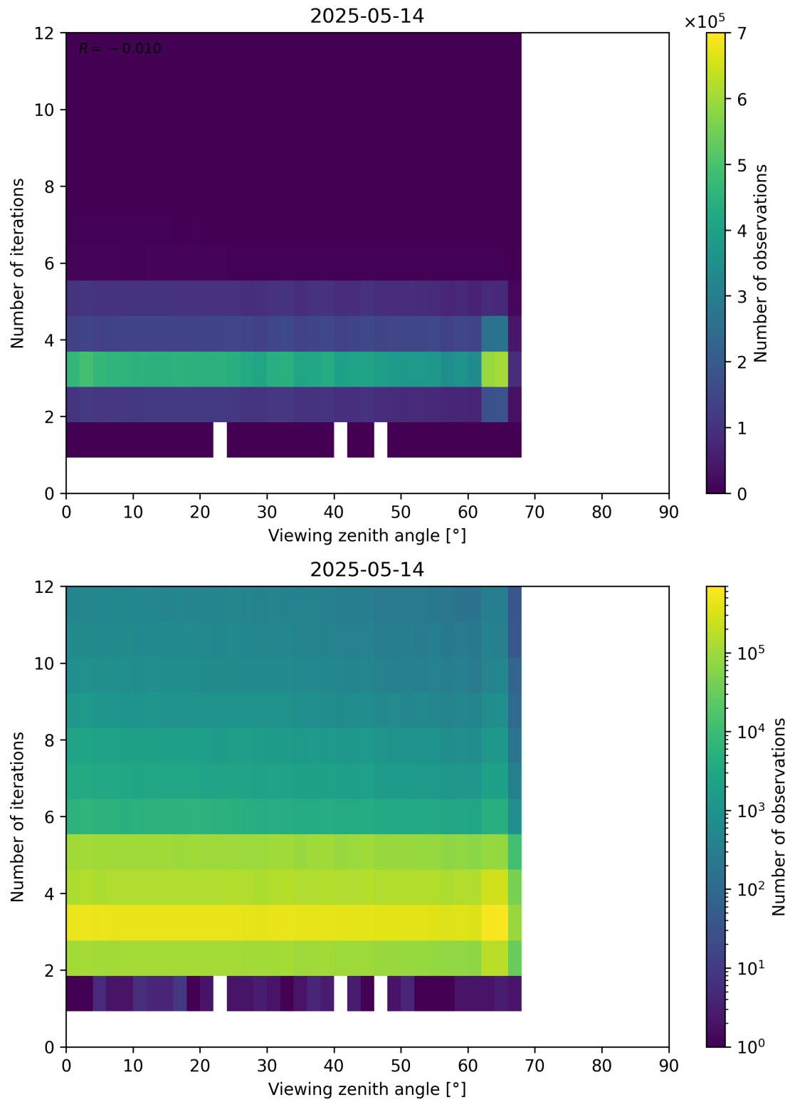
Figure 124: Scatter density plot of “Viewing zenith angle” against “Number of iterations” for 2025-05-13 to 2025-05-15.
