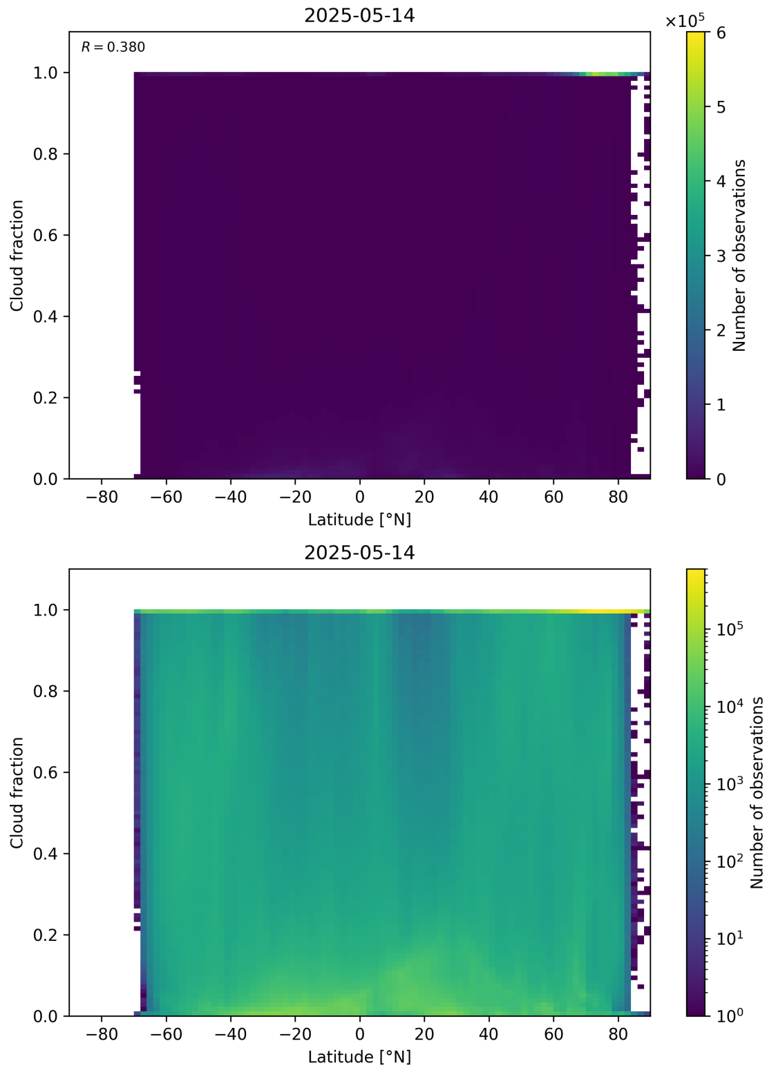
Figure 90: Scatter density plot of “Latitude” against “Cloud fraction” for 2025-05-13 to 2025-05-15.
