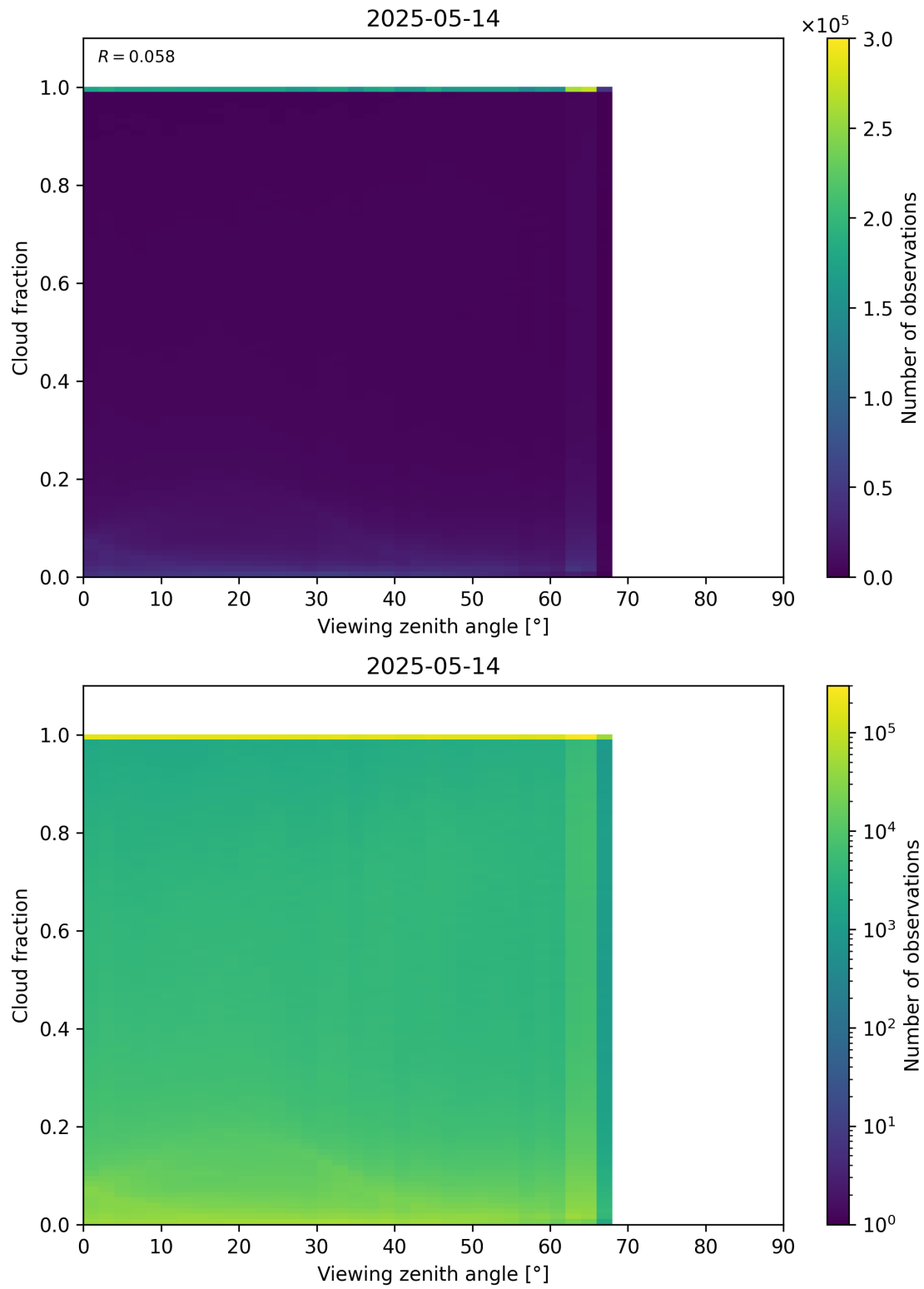
Figure 120: Scatter density plot of “Viewing zenith angle” against “Cloud fraction” for 2025-05-13 to 2025-05-15.
