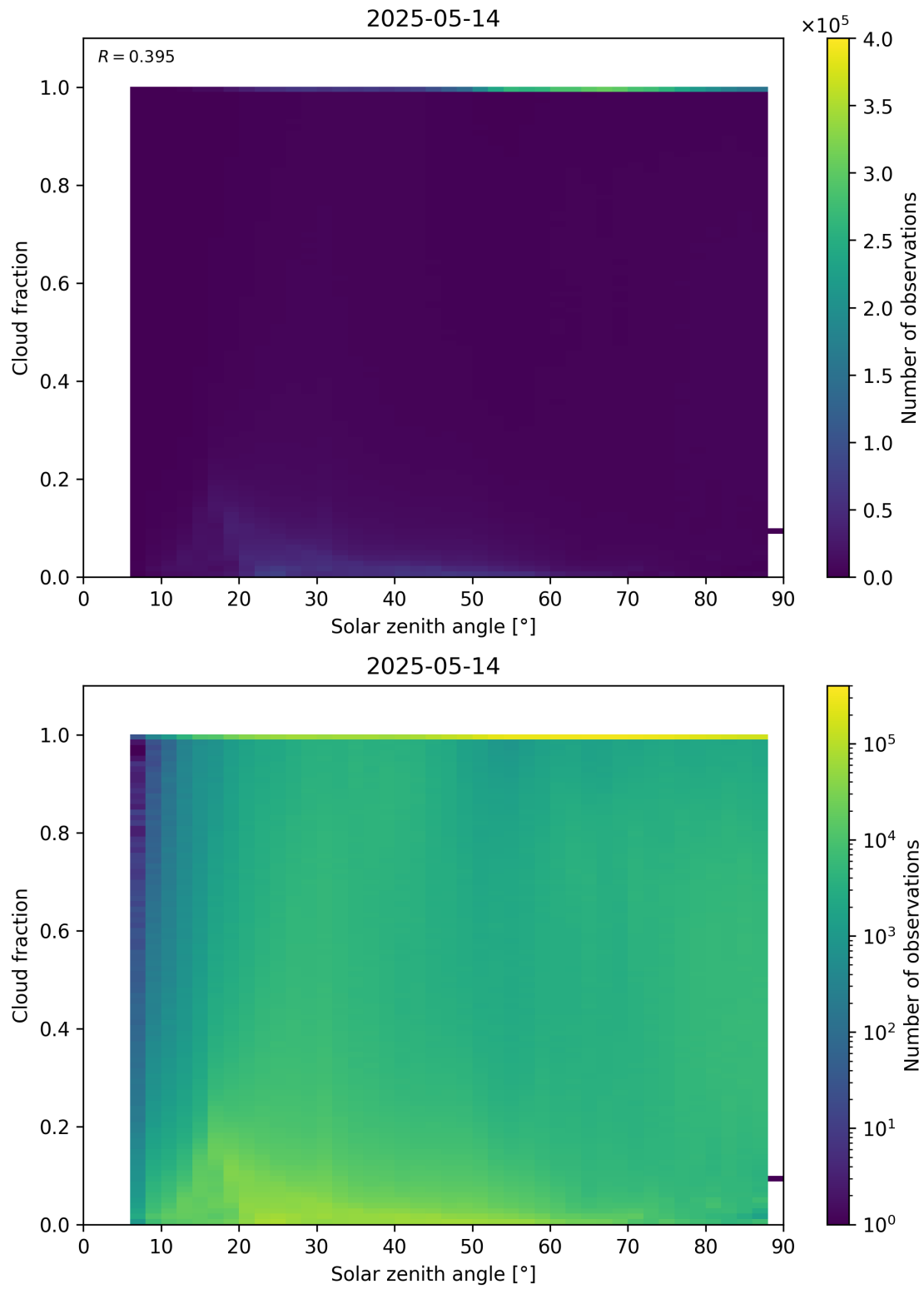
Figure 110: Scatter density plot of “Solar zenith angle” against “Cloud fraction” for 2025-05-13 to 2025-05-15.
