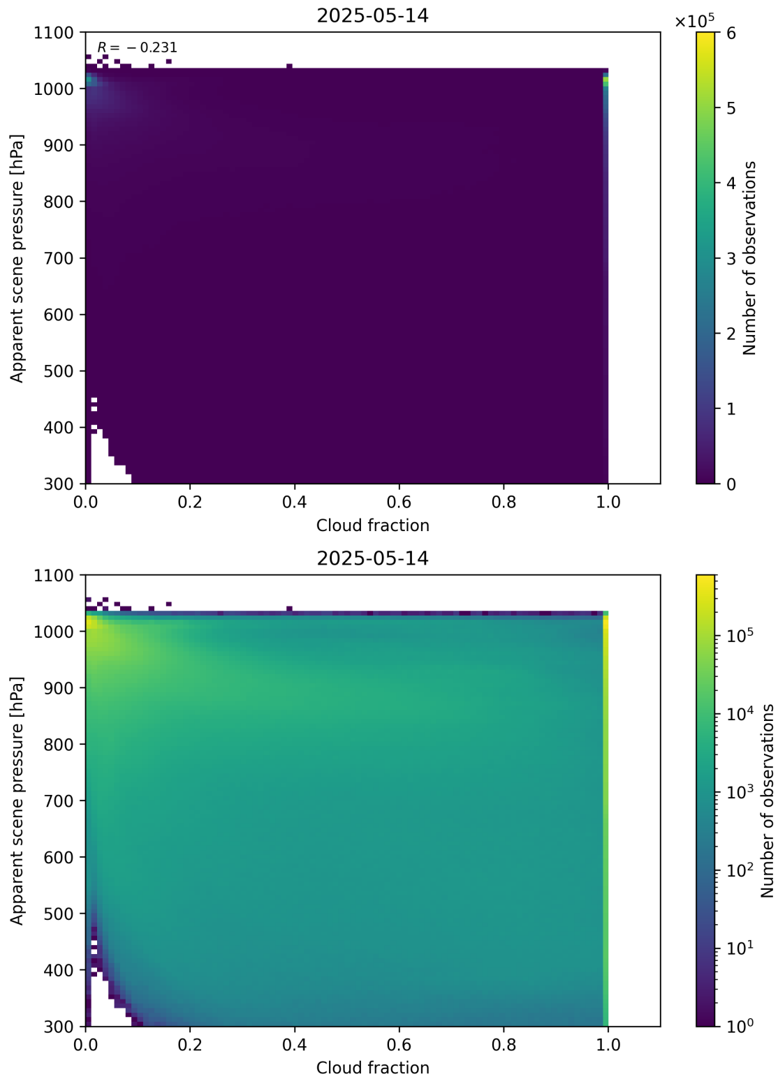
Figure 70: Scatter density plot of “Cloud fraction” against “Apparent scene pressure” for 2025-05-13 to 2025-05-15.
