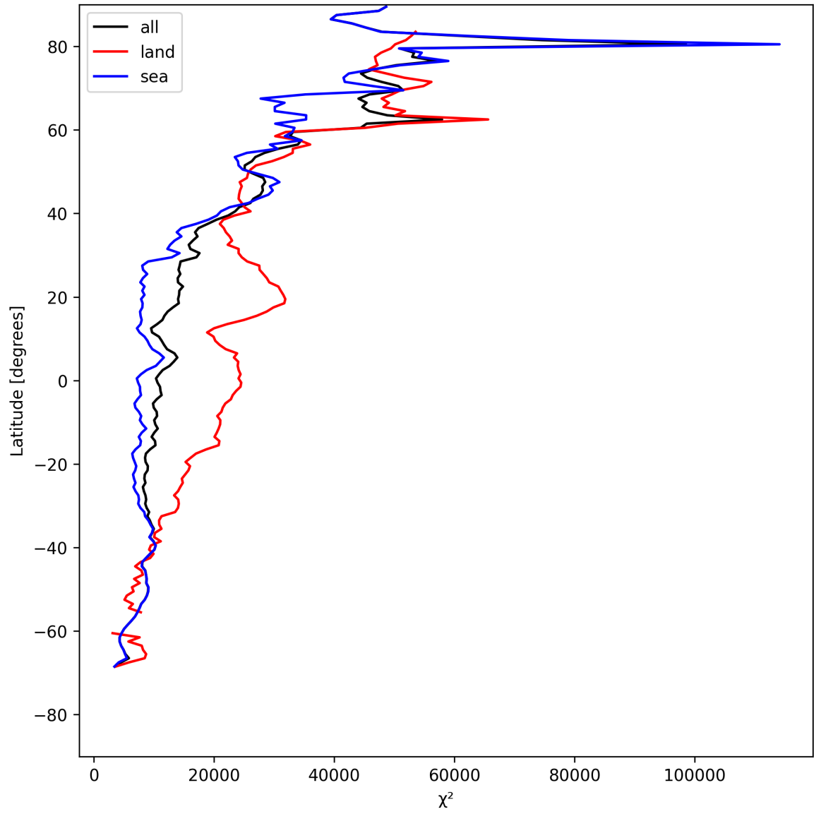
Figure 21: Zonal average of “ \chi^2 ” for 2025-05-13 to 2025-05-15.
