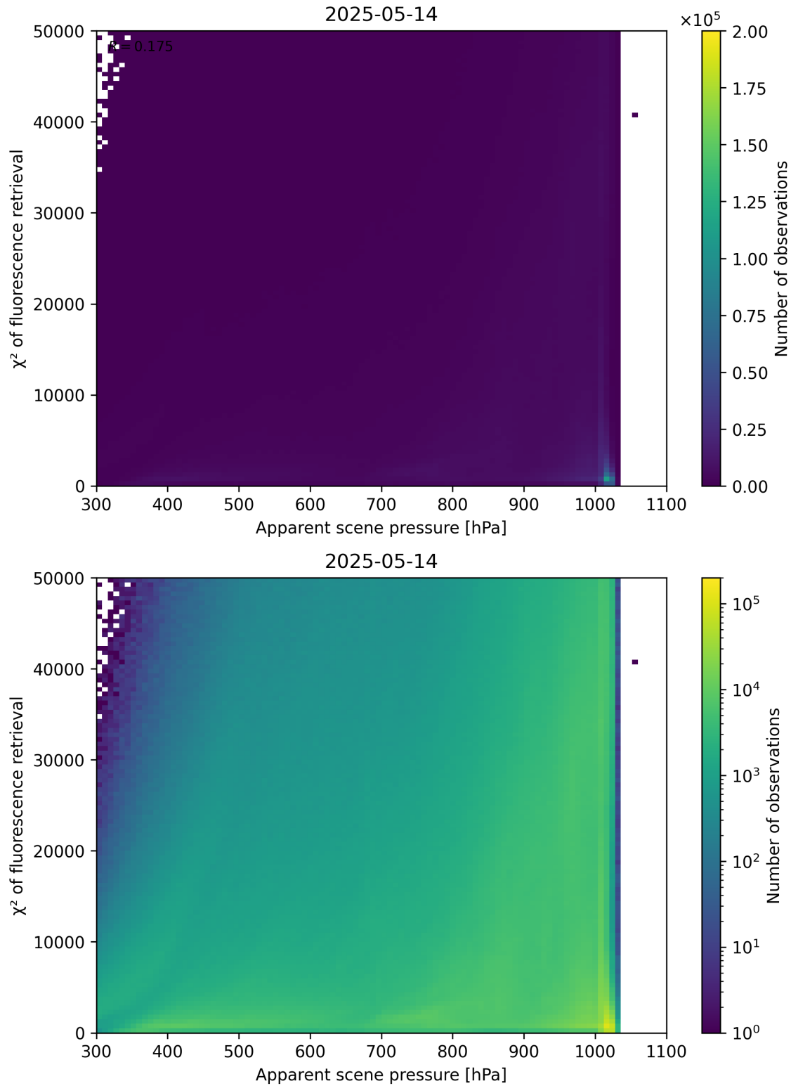
Figure 63: Scatter density plot of “Apparent scene pressure” against “ \chi^2 of fluorescence retrieval” for 2025-05-13 to 2025-05-15.
