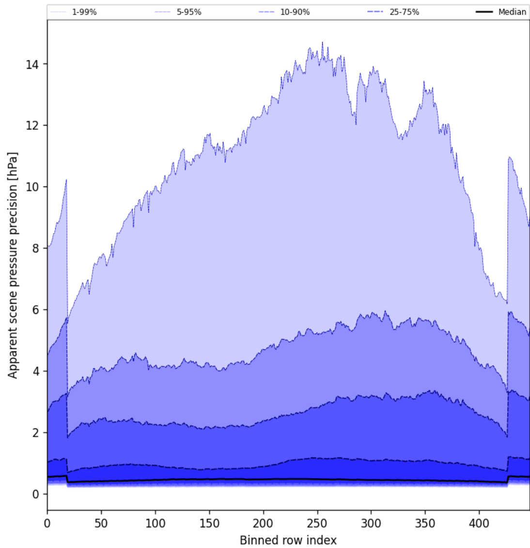
Figure 54: Along track statistics of “Apparent scene pressure precision” for 2025-05-15 to 2025-05-16
