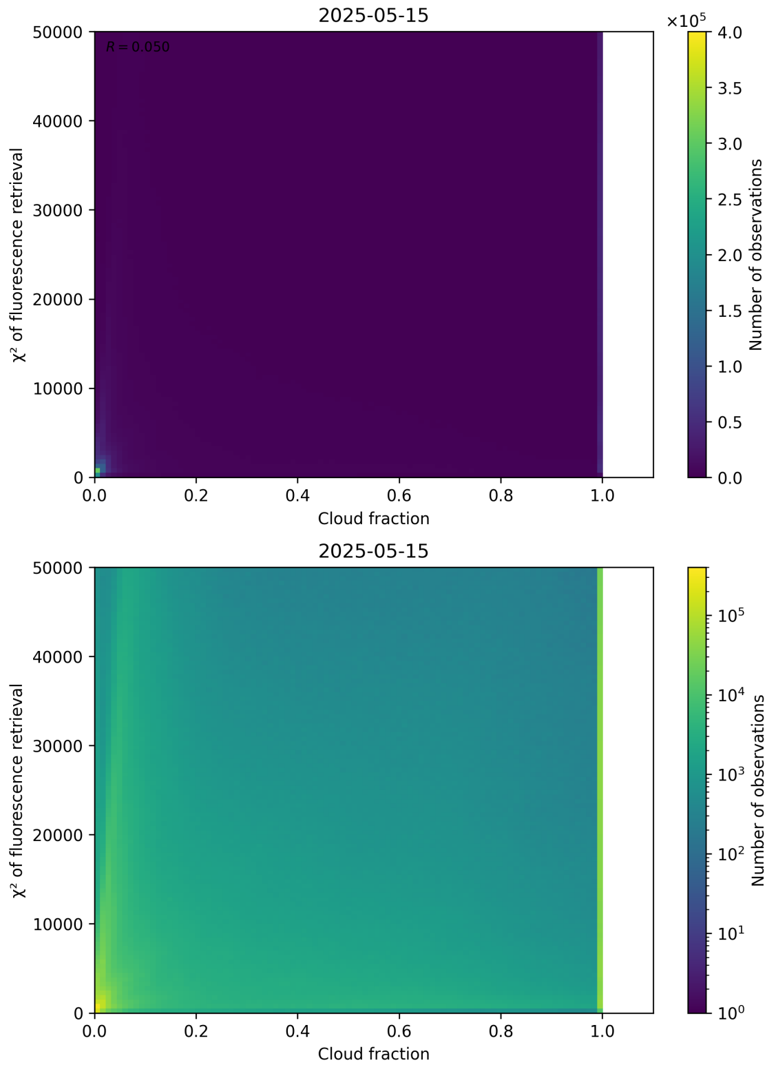
Figure 71: Scatter density plot of “Cloud fraction” against “ \chi^2 of fluorescence retrieval” for 2025-05-15 to 2025-05-16.
