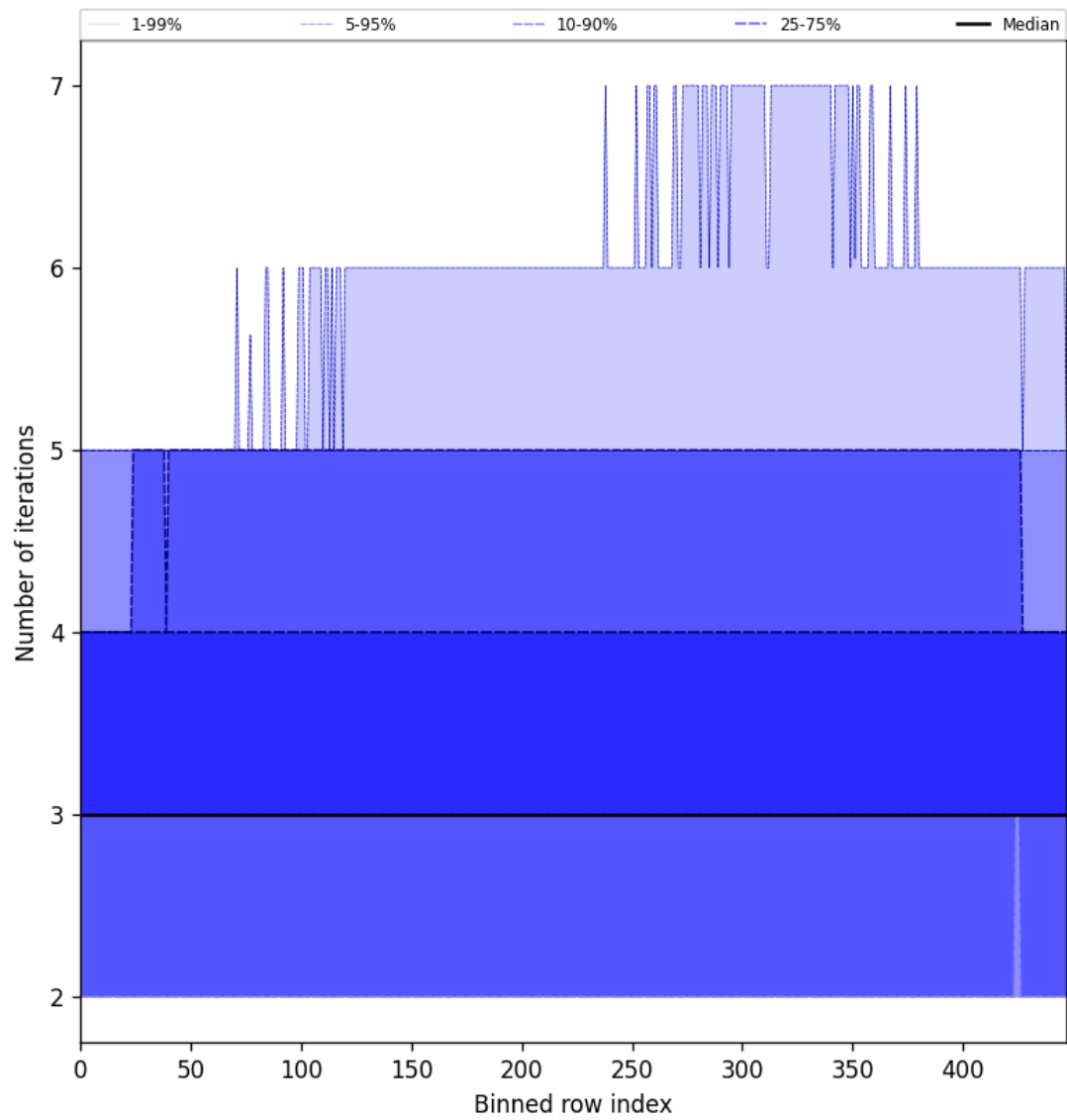
Figure 56: Along track statistics of “Number of iterations” for 2025-05-15 to 2025-05-16
