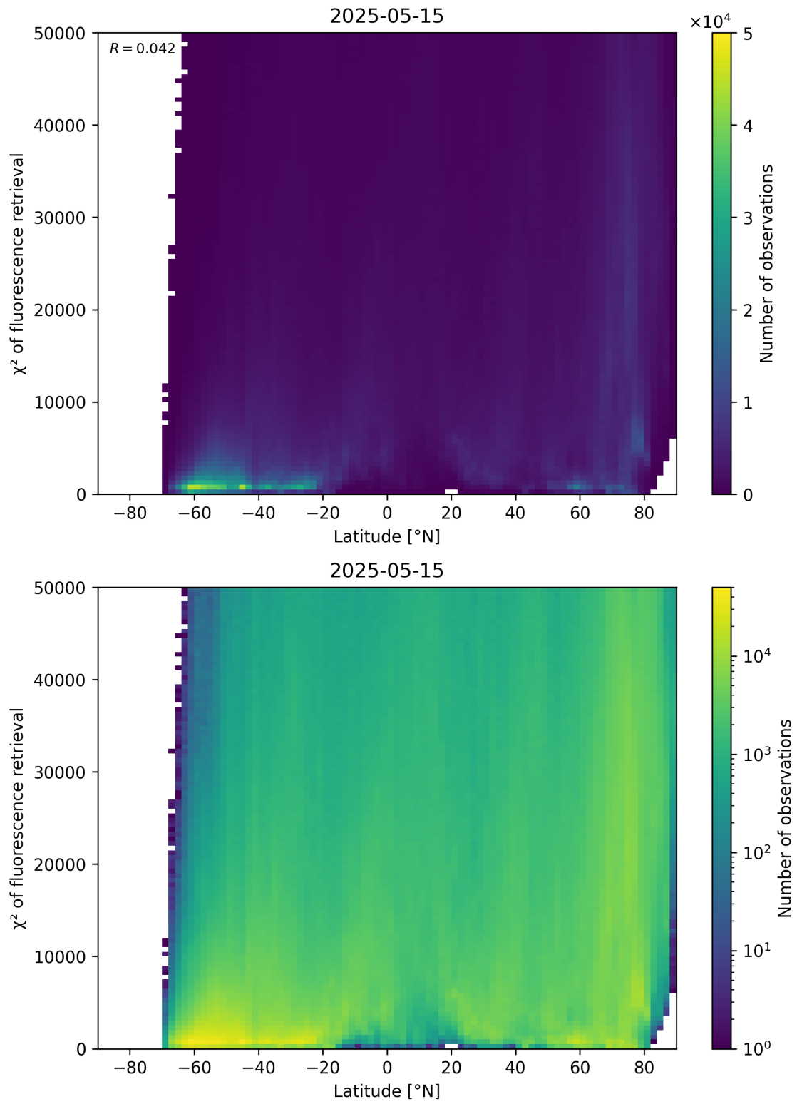
Figure 89: Scatter density plot of “Latitude” against “ \chi^2 of fluorescence retrieval” for 2025-05-15 to 2025-05-16.
