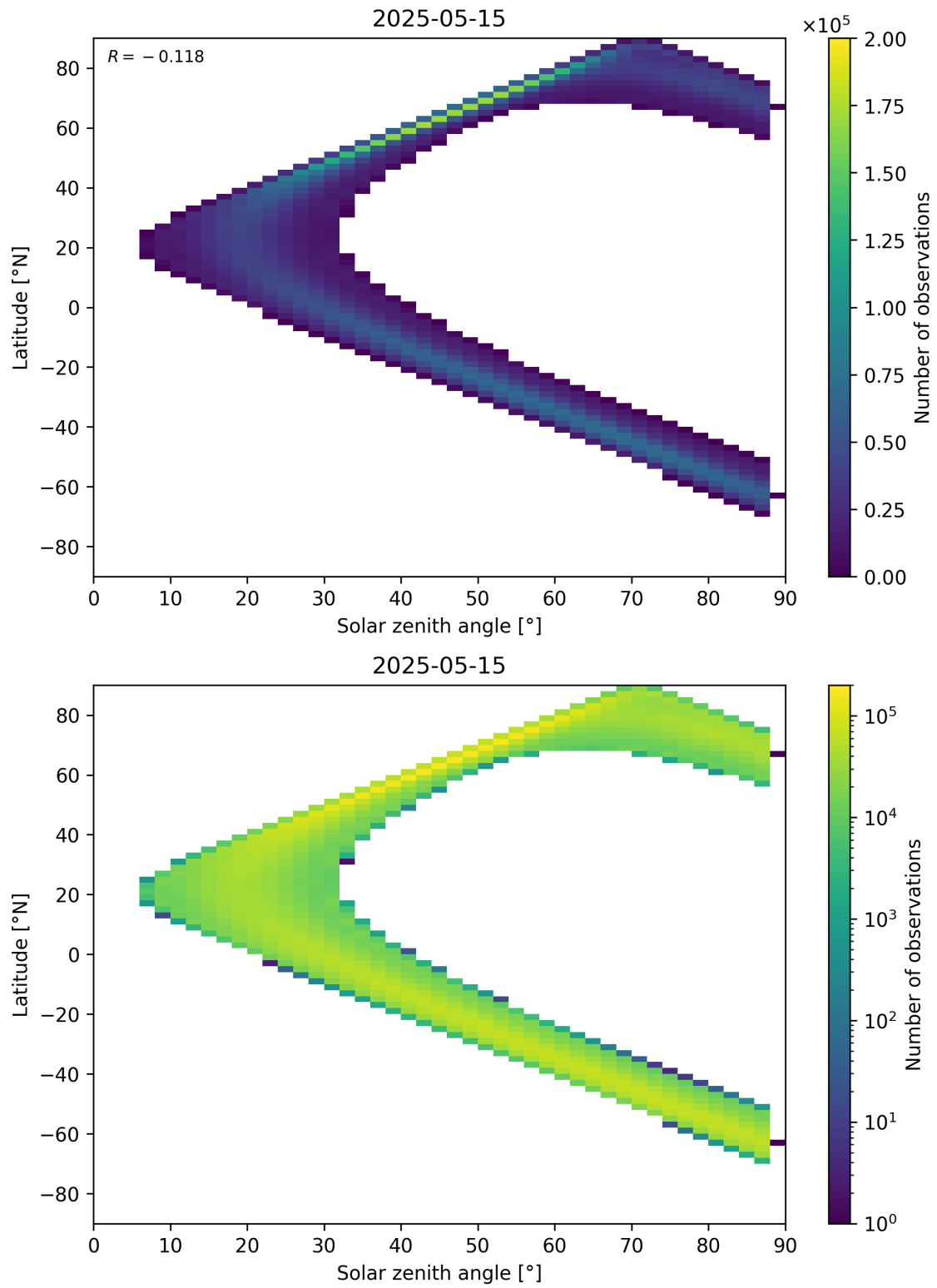
Figure 113: Scatter density plot of “Solar zenith angle” against “Latitude” for 2025-05-15 to 2025-05-16.
