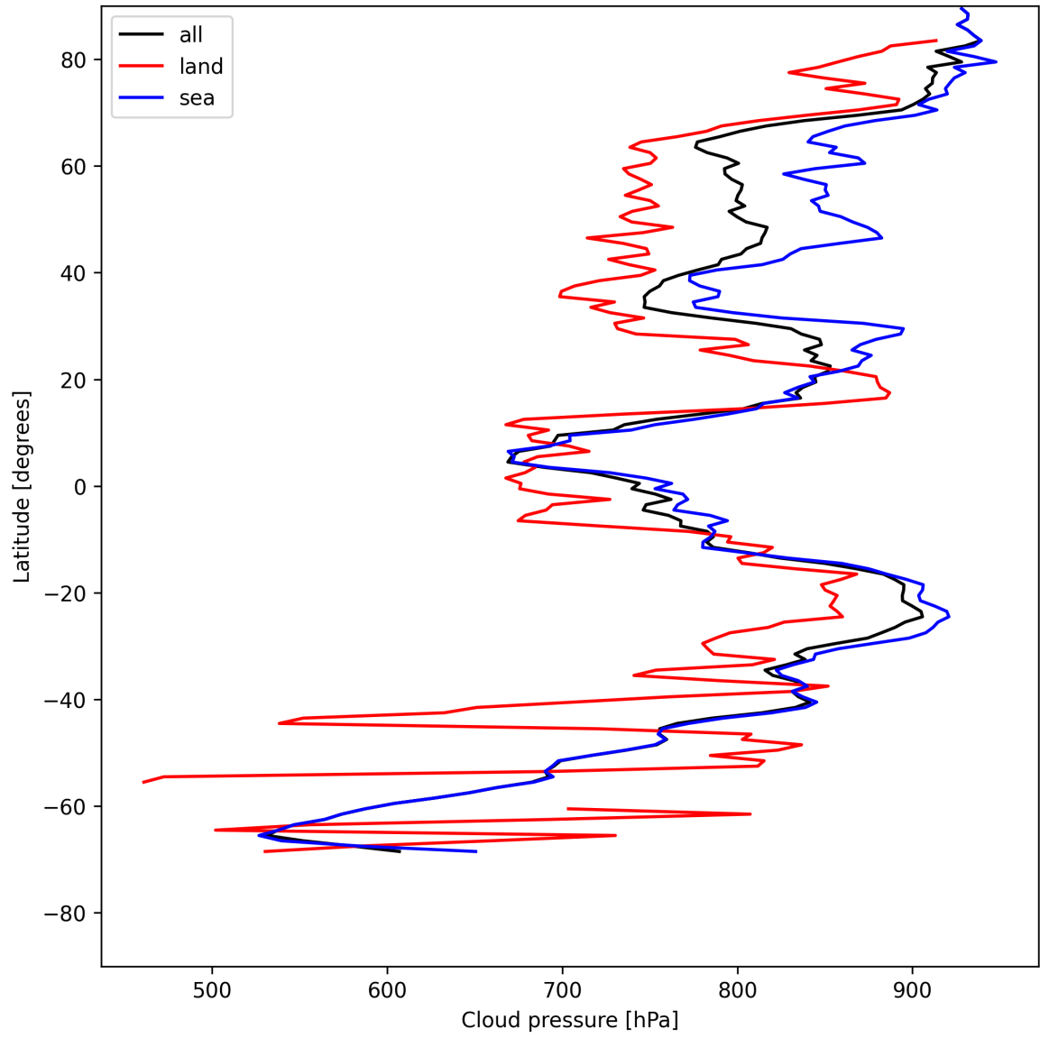
Figure 13: Zonal average of “Cloud pressure” for 2025-05-15 to 2025-05-16.
