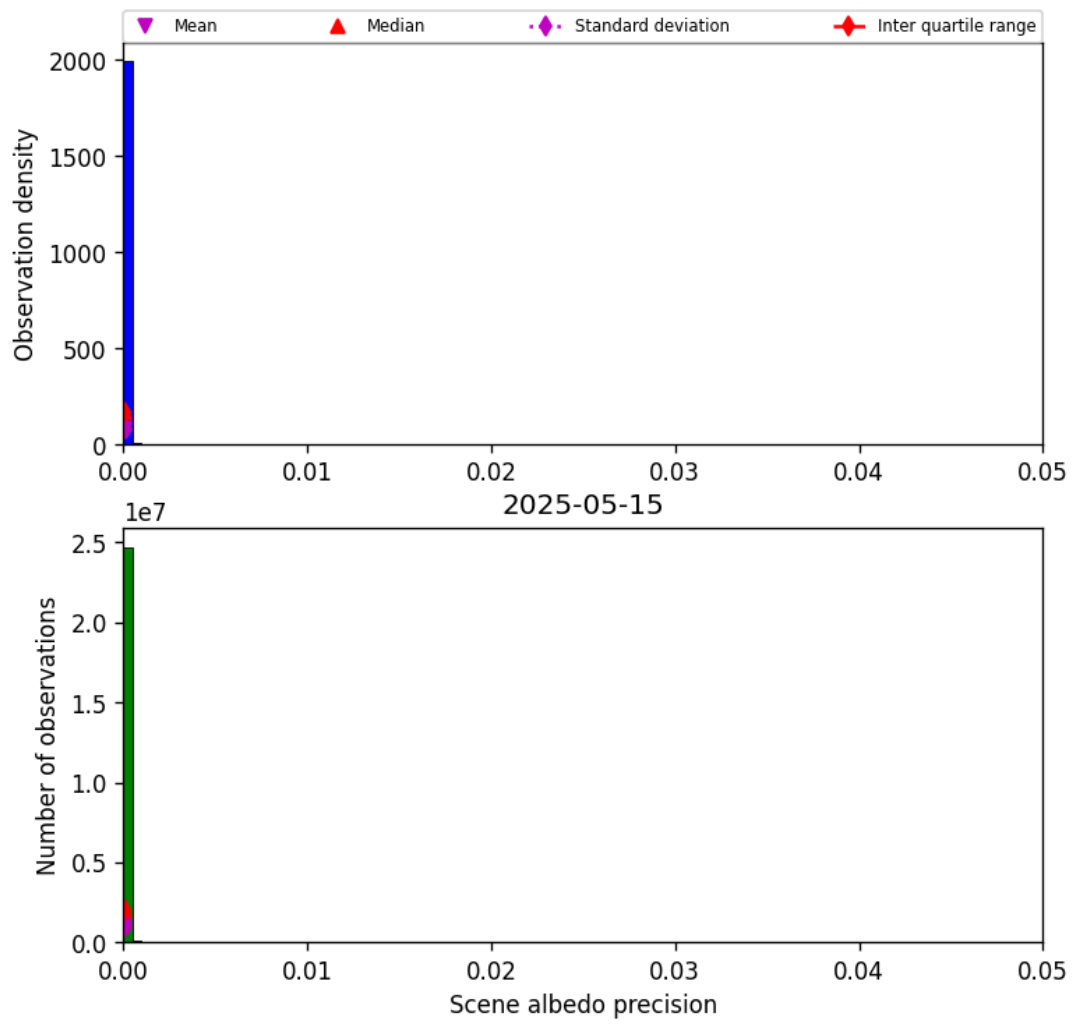
Figure 35: Histogram of “Scene albedo precision” for 2025-05-15 to 2025-05-16
