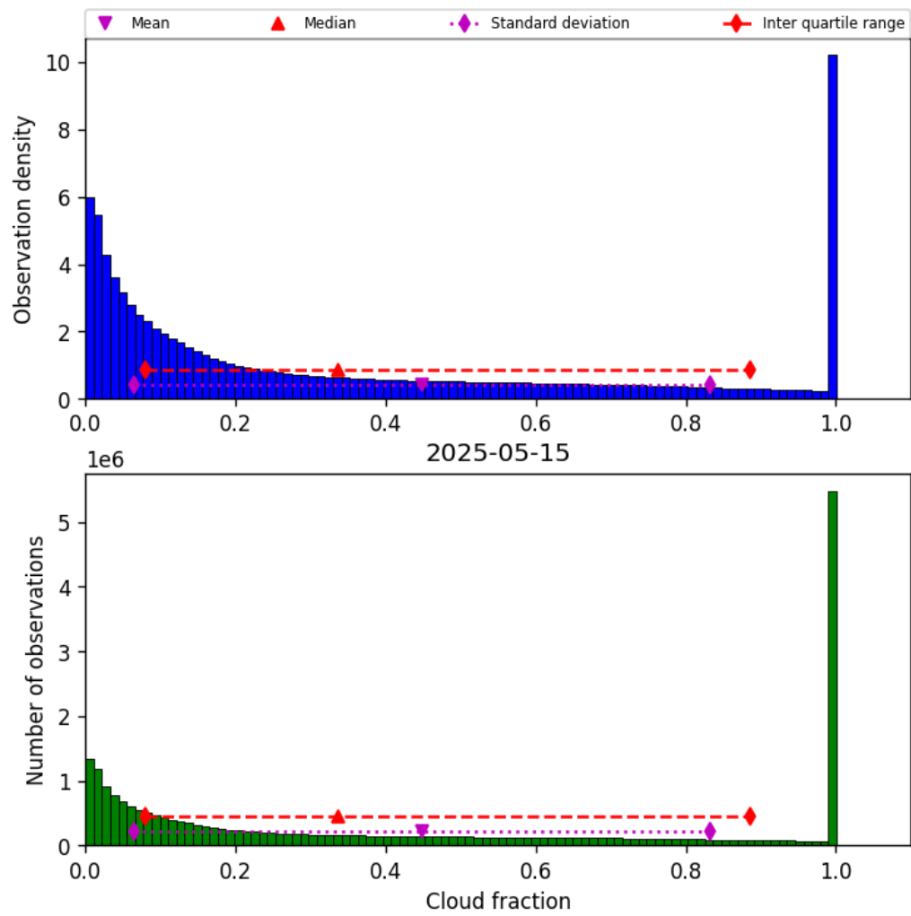
Figure 32: Histogram of “Cloud fraction” for 2025-05-15 to 2025-05-16
