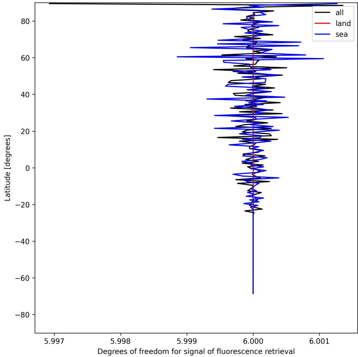
Figure 26: Zonal average of “Degrees of freedom for signal of fluorescence retrieval” for 2025-05-15 to 2025-05-16.
