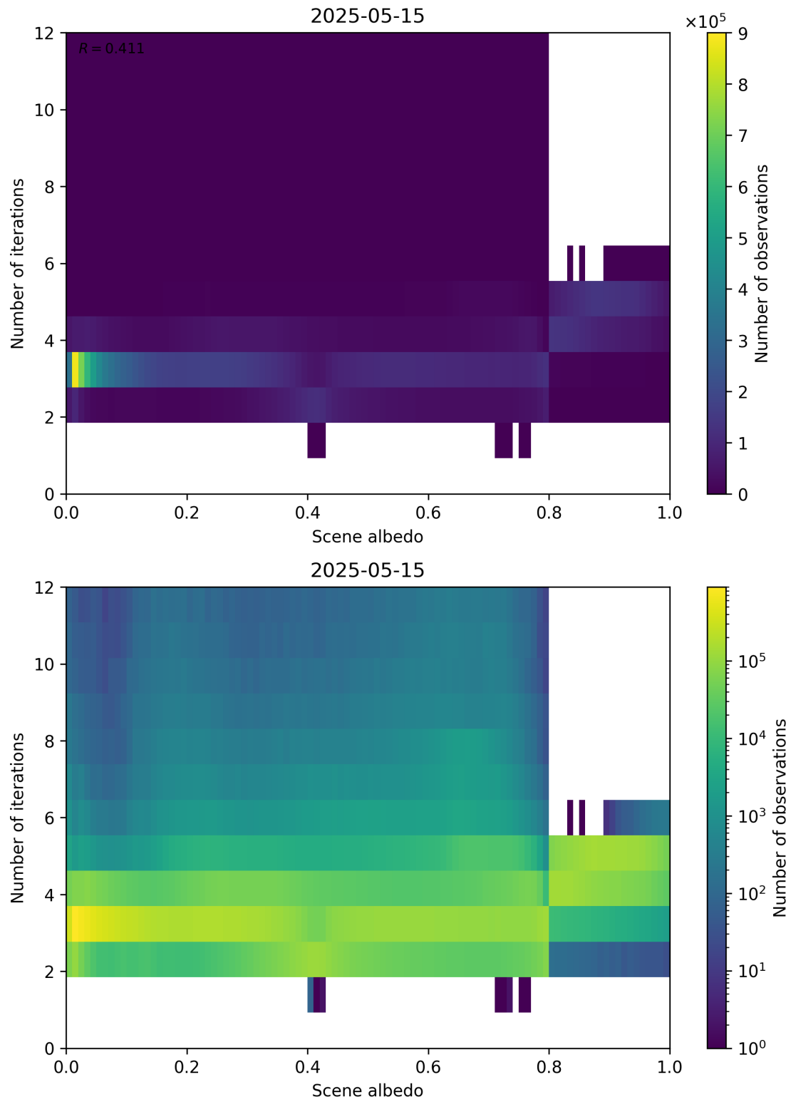
Figure 105: Scatter density plot of “Scene albedo” against “Number of iterations” for 2025-05-15 to 2025-05-16.
