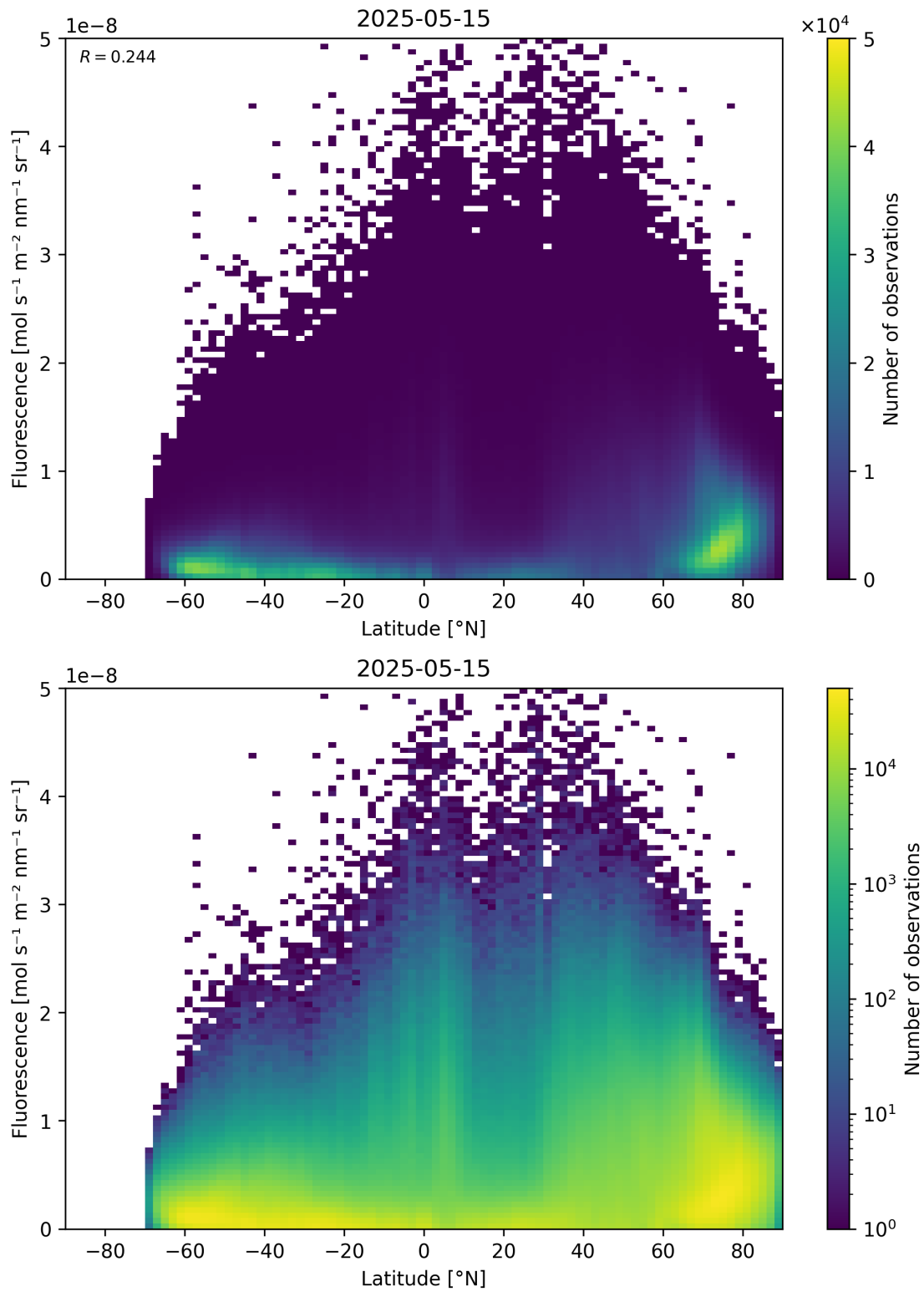
Figure 92: Scatter density plot of “Latitude” against “Fluorescence” for 2025-05-15 to 2025-05-16.
