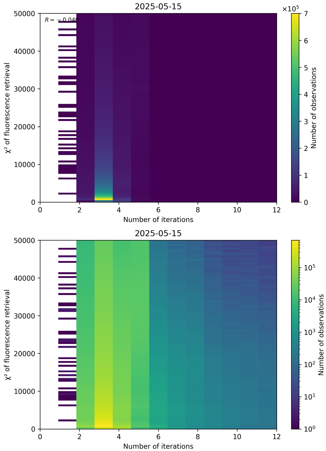
Figure 97: Scatter density plot of “Number of iterations” against “ \chi^2 of fluorescence retrieval” for 2025-05-15 to 2025-05-16.
