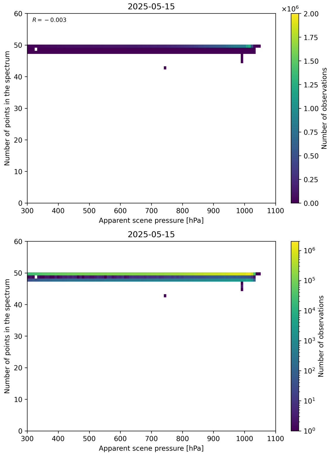
Figure 66: Scatter density plot of “Apparent scene pressure” against “Number of points in the spectrum” for 2025-05-15 to 2025-05-16.
