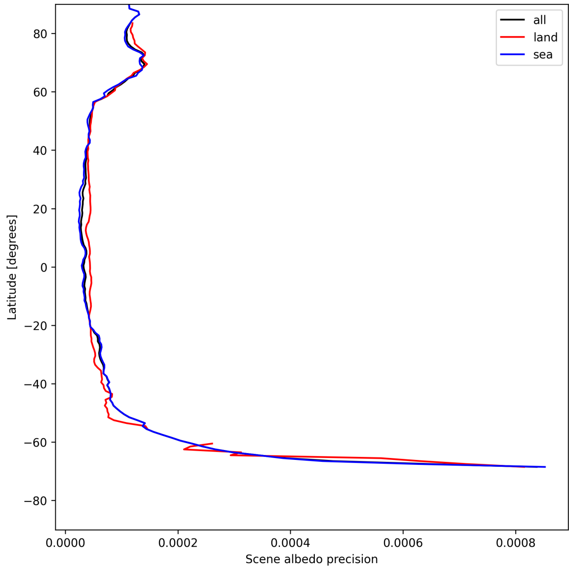
Figure 18: Zonal average of “Scene albedo precision” for 2025-05-15 to 2025-05-16.
