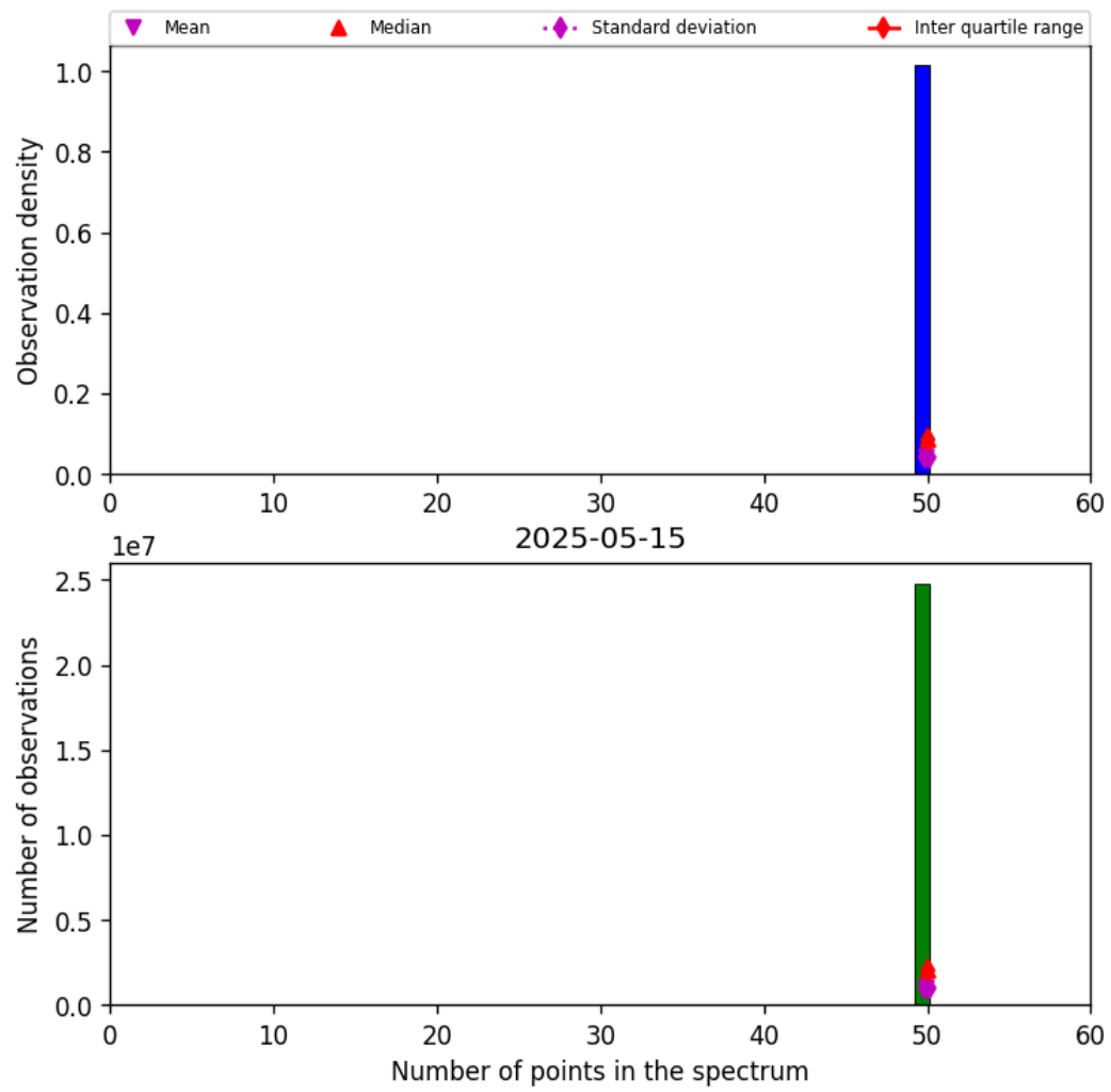
Figure 44: Histogram of “Number of points in the spectrum” for 2025-05-15 to 2025-05-16
