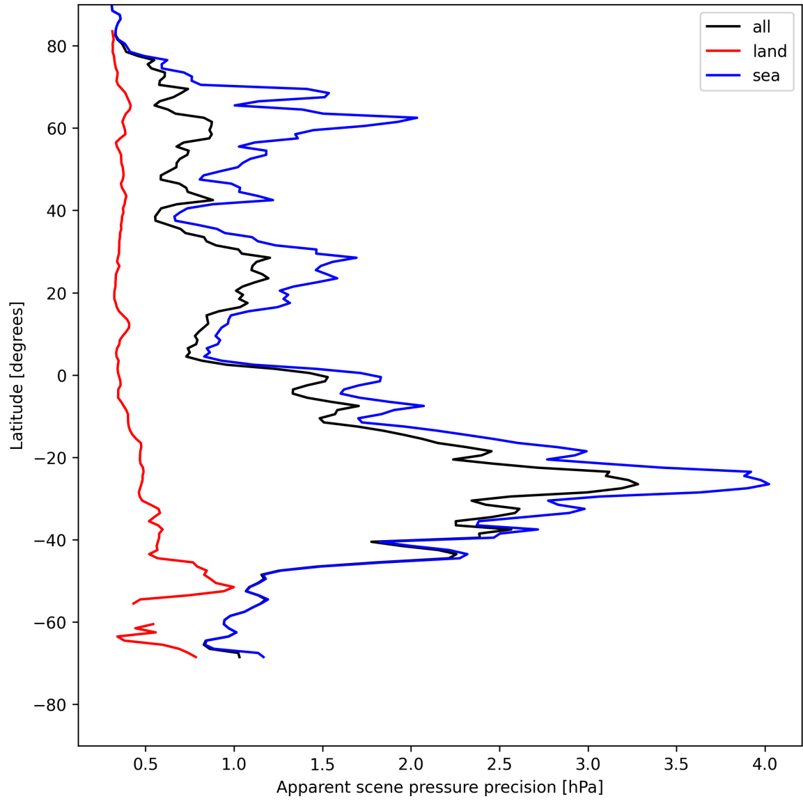
Figure 20: Zonal average of “Apparent scene pressure precision” for 2025-05-15 to 2025-05-16.
