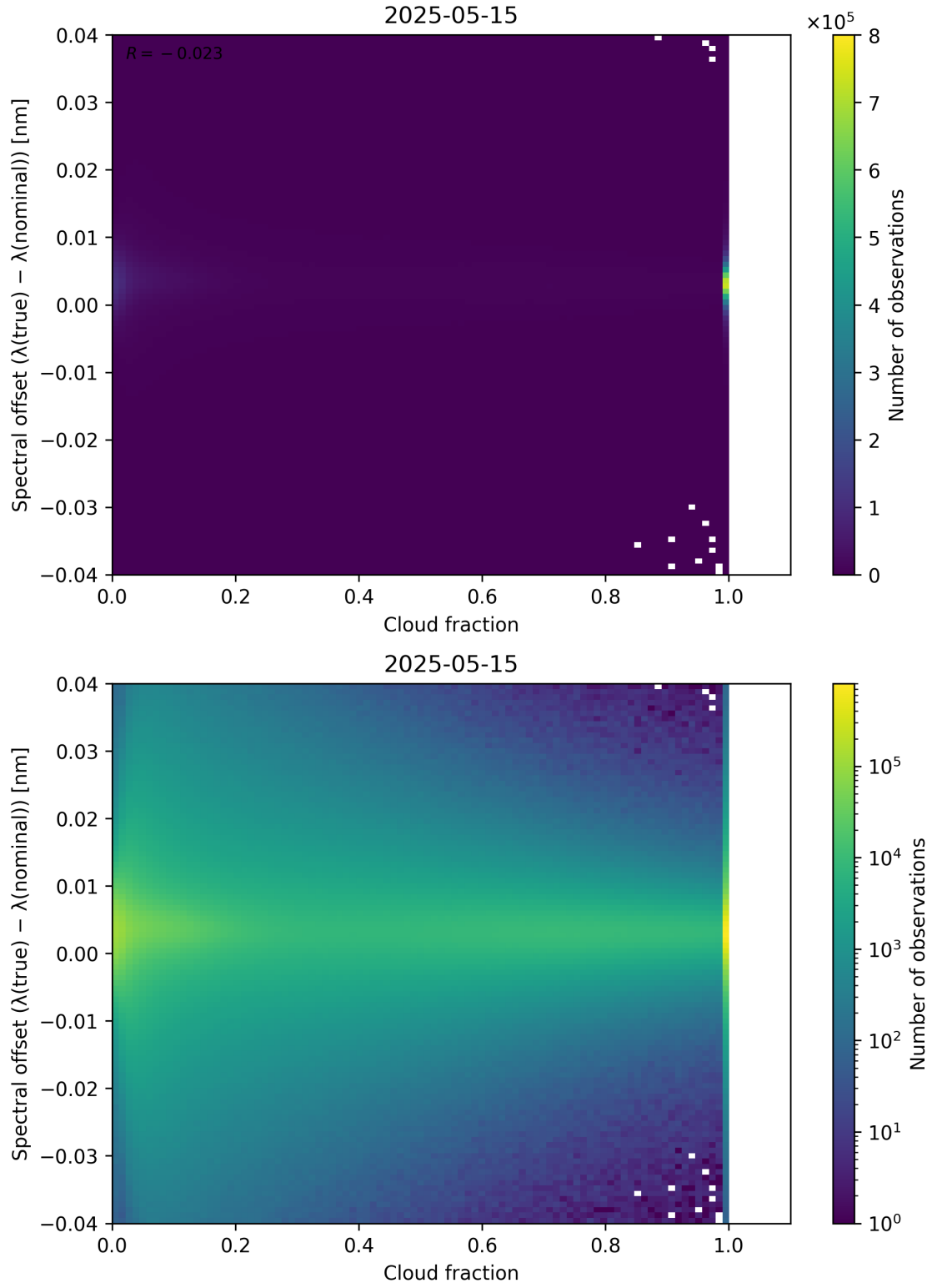
Figure 76: Scatter density plot of “Cloud fraction” against “Spectral offset ( \lambda_{\text{true}} - \lambda_{\text{nominal}} )” for 2025-05-15 to 2025-05-16.
