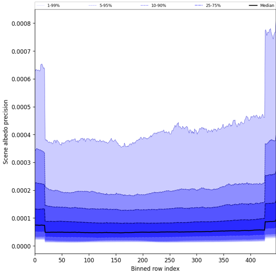
Figure 52: Along track statistics of “Scene albedo precision” for 2025-05-15 to 2025-05-16
