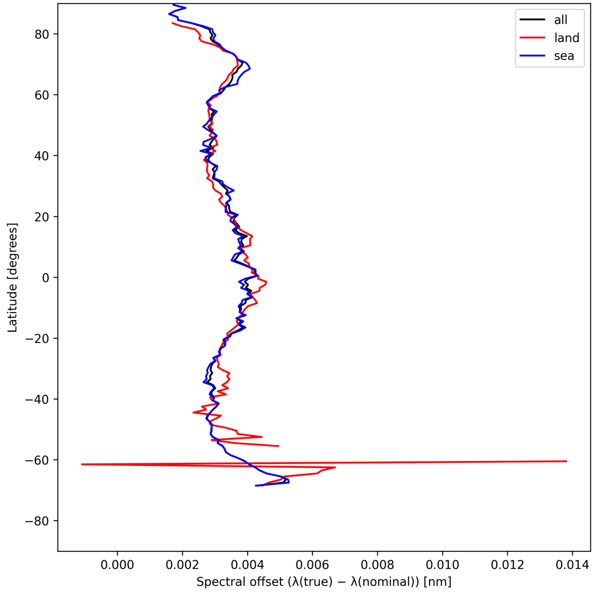
Figure 28: Zonal average of “Spectral offset ( \lambda_{\text{true}} - \lambda_{\text{nominal}} )” for 2025-05-15 to 2025-05-16.
