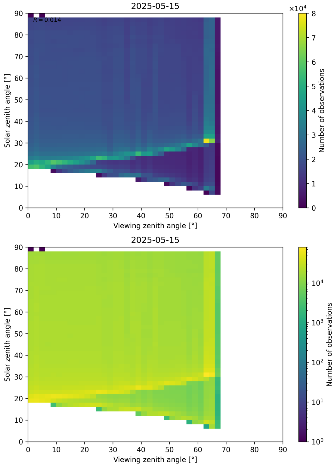
Figure 127: Scatter density plot of “Viewing zenith angle” against “Solar zenith angle” for 2025-05-15 to 2025-05-16.
