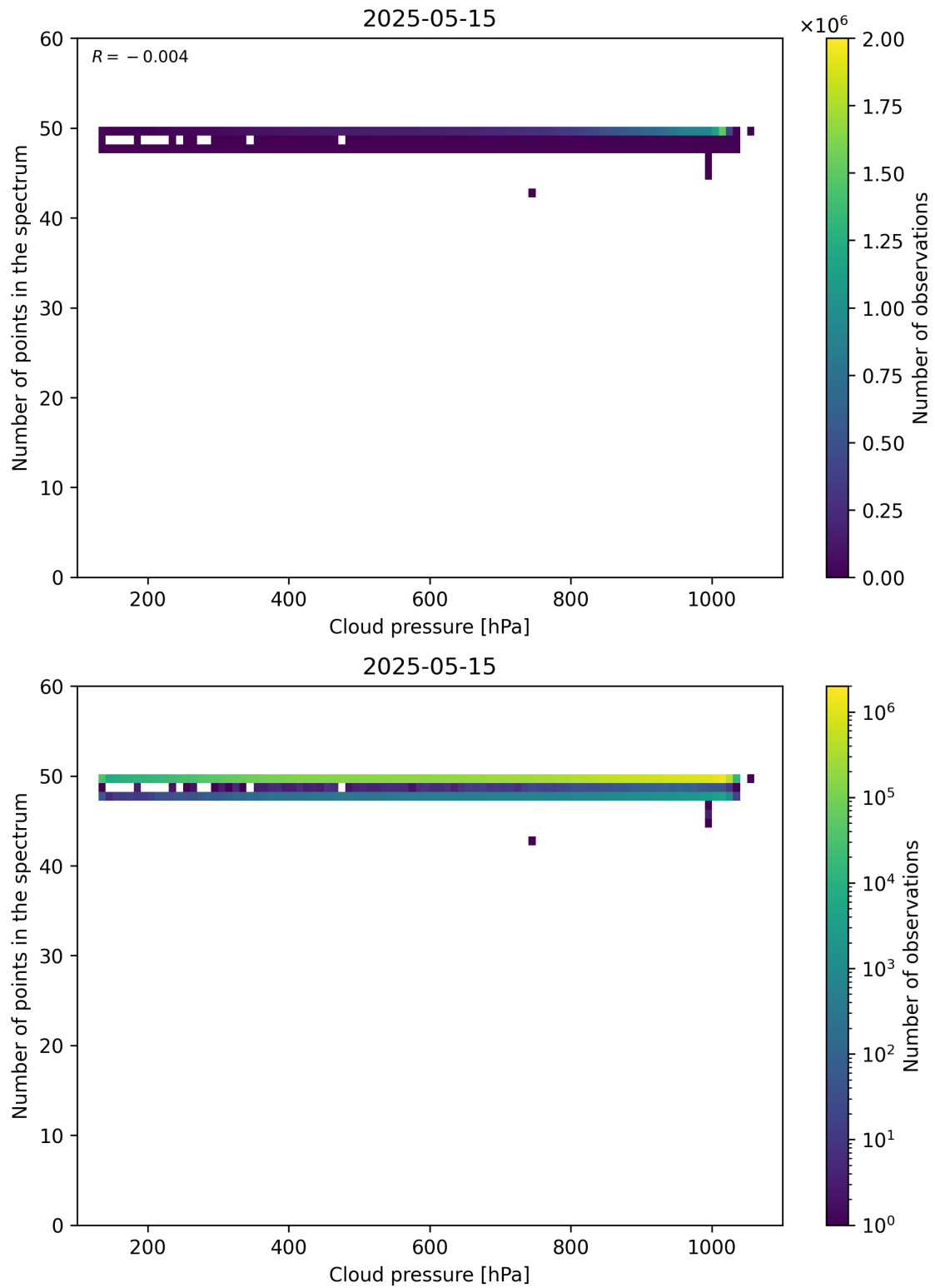
Figure 82: Scatter density plot of “Cloud pressure” against “Number of points in the spectrum” for 2025-05-15 to 2025-05-16.
