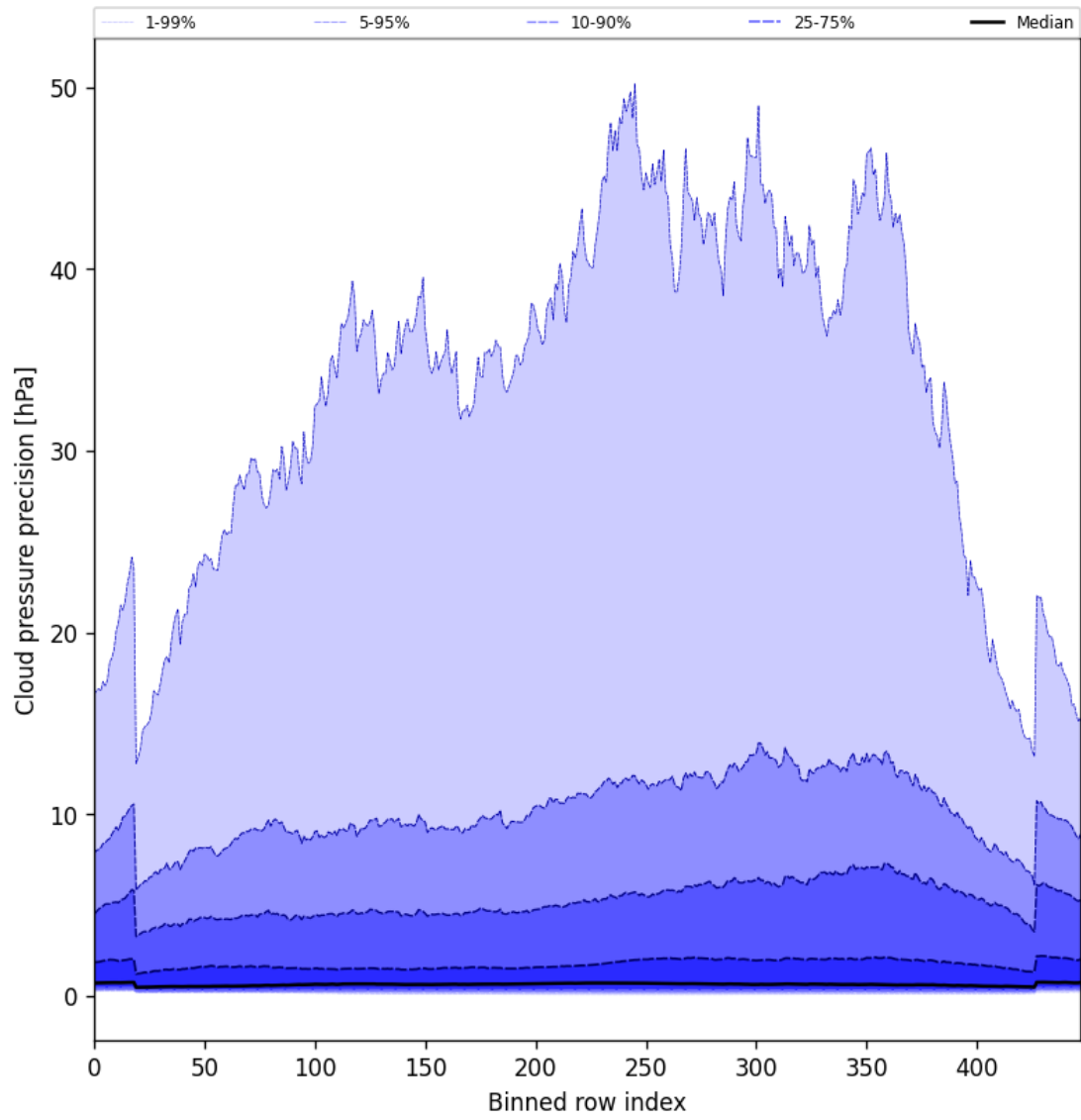
Figure 48: Along track statistics of “Cloud pressure precision” for 2025-05-15 to 2025-05-16
