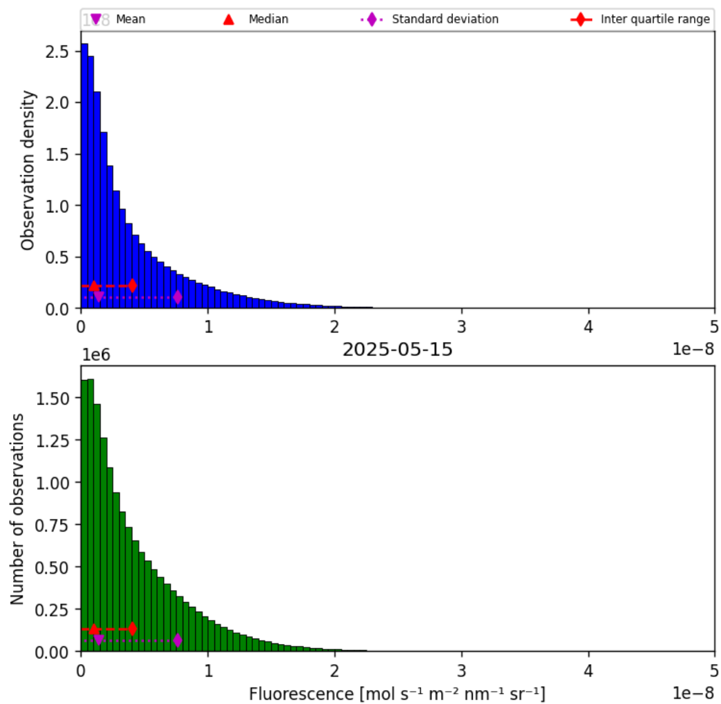
Figure 40: Histogram of “Fluorescence” for 2025-05-15 to 2025-05-16
