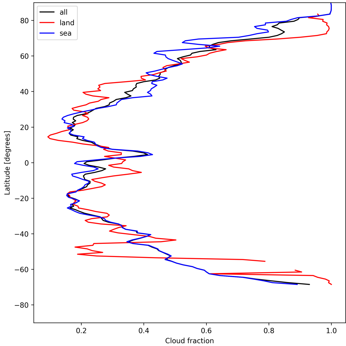
Figure 15: Zonal average of “Cloud fraction” for 2025-05-15 to 2025-05-16.
