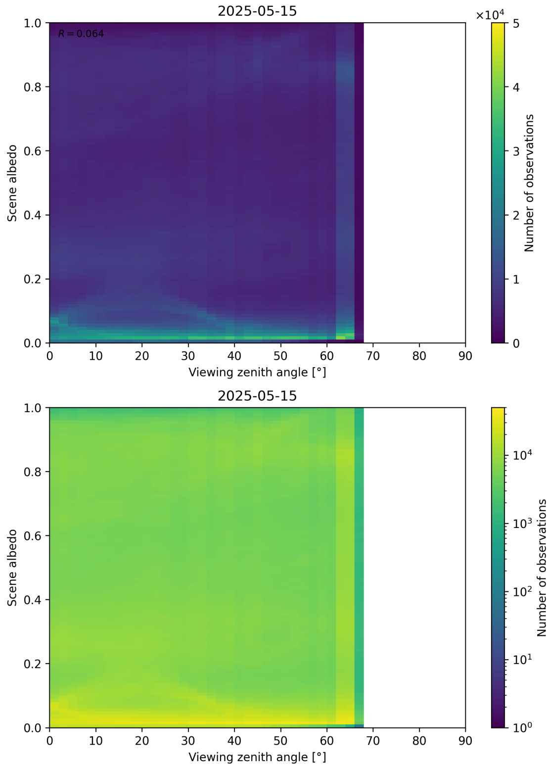
Figure 126: Scatter density plot of “Viewing zenith angle” against “Scene albedo” for 2025-05-15 to 2025-05-16.
