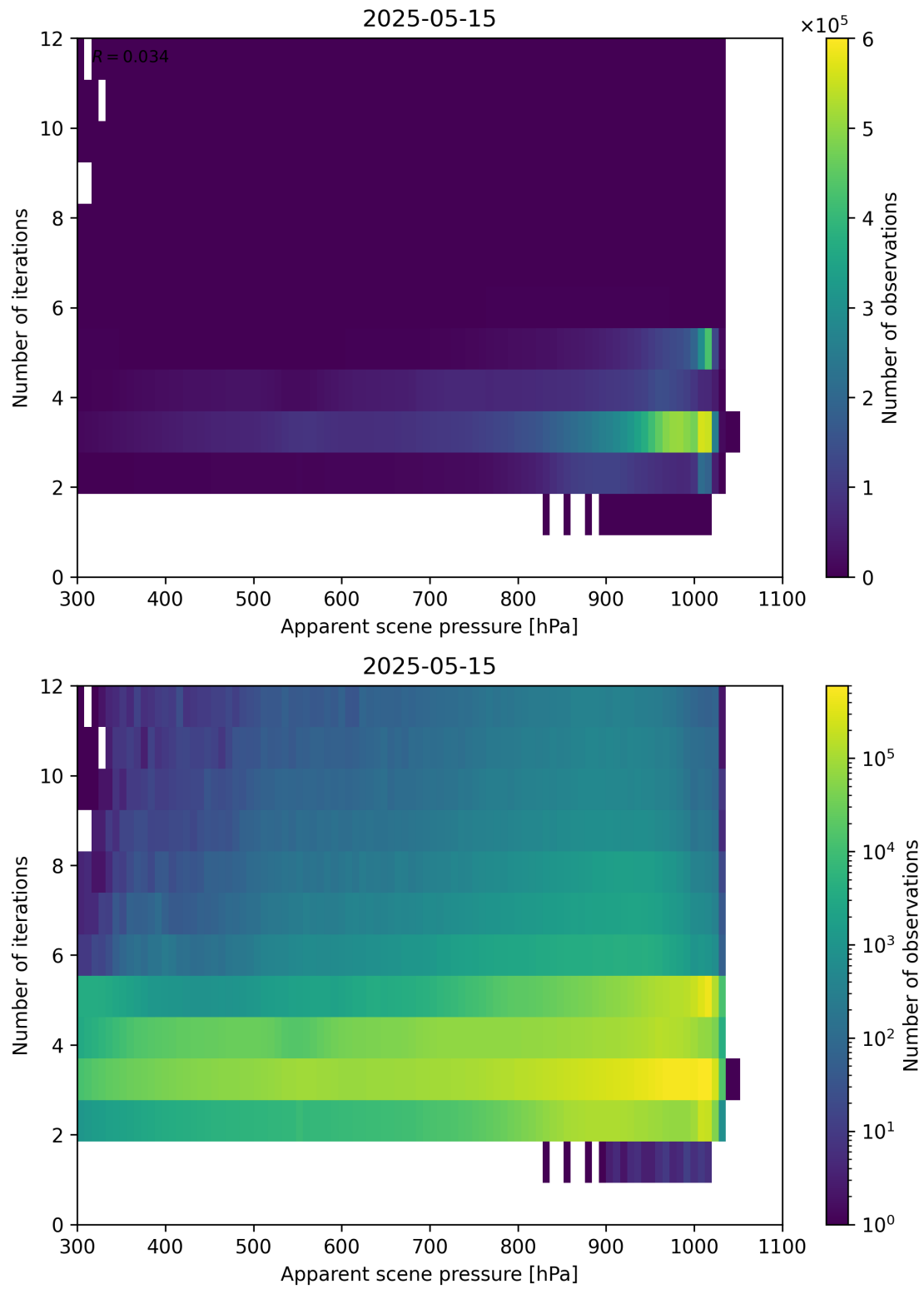
Figure 65: Scatter density plot of “Apparent scene pressure” against “Number of iterations” for 2025-05-15 to 2025-05-16.
