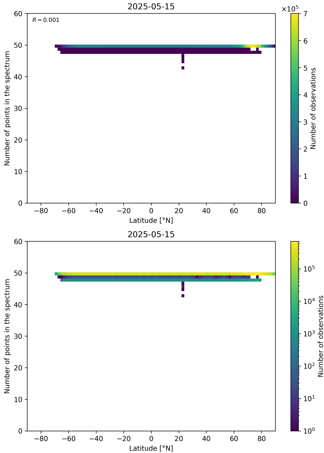
Figure 94: Scatter density plot of “Latitude” against “Number of points in the spectrum” for 2025-05-15 to 2025-05-16.
