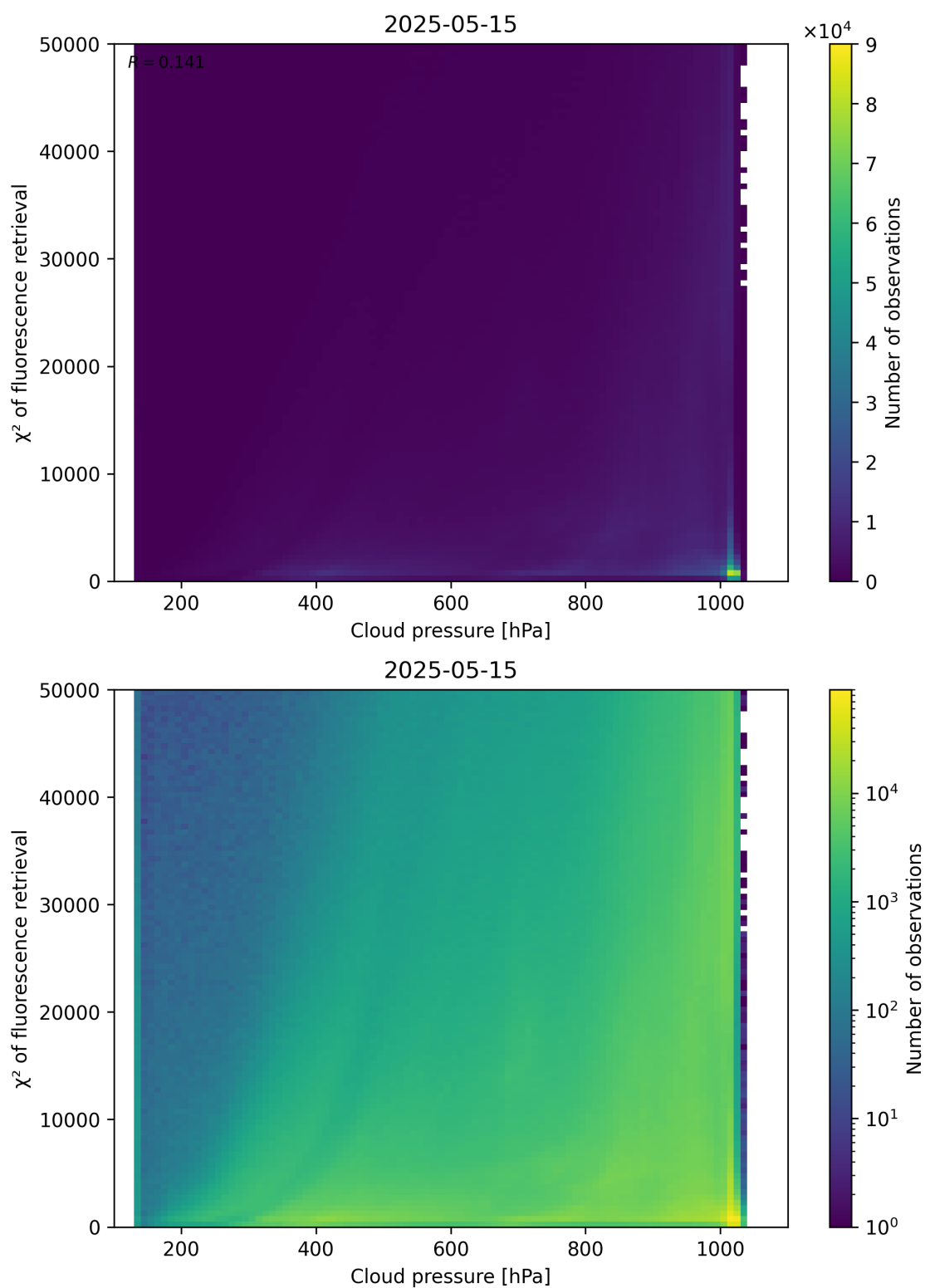
Figure 78: Scatter density plot of “Cloud pressure” against “ \chi^2 of fluorescence retrieval” for 2025-05-15 to 2025-05-16.
