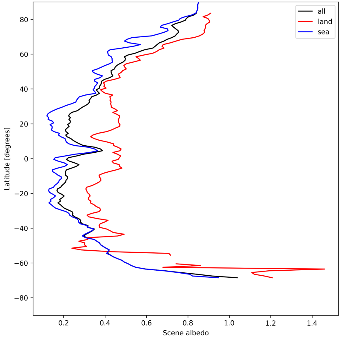
Figure 17: Zonal average of “Scene albedo” for 2025-05-15 to 2025-05-16.
