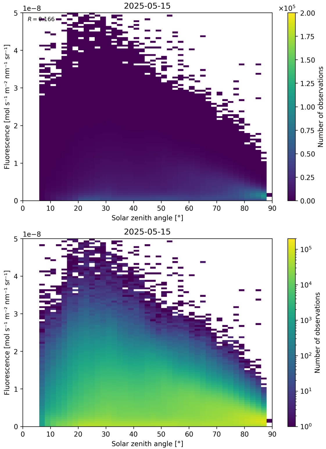
Figure 112: Scatter density plot of “Solar zenith angle” against “Fluorescence” for 2025-05-15 to 2025-05-16.
