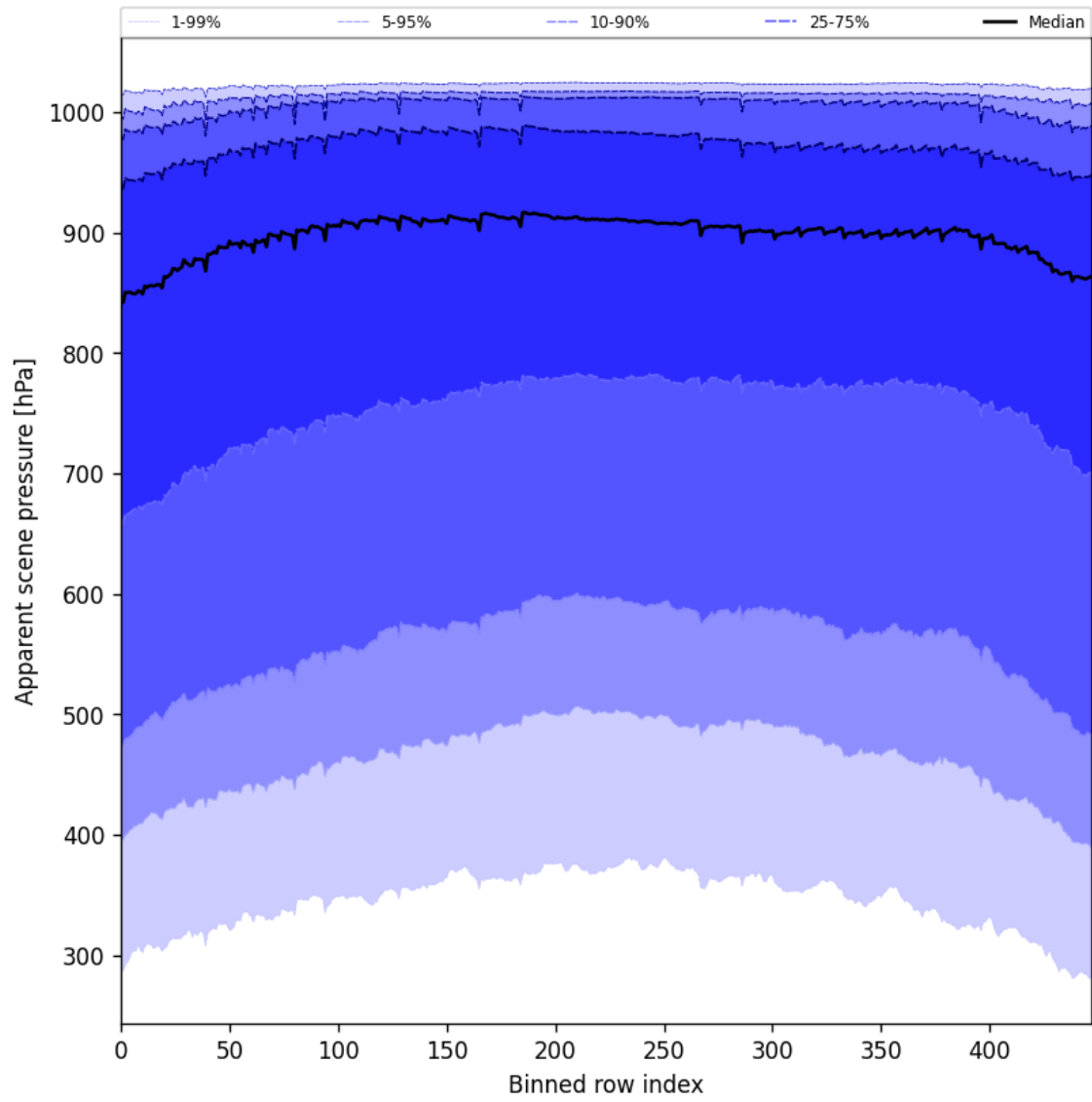
Figure 53: Along track statistics of “Apparent scene pressure” for 2025-05-15 to 2025-05-16
