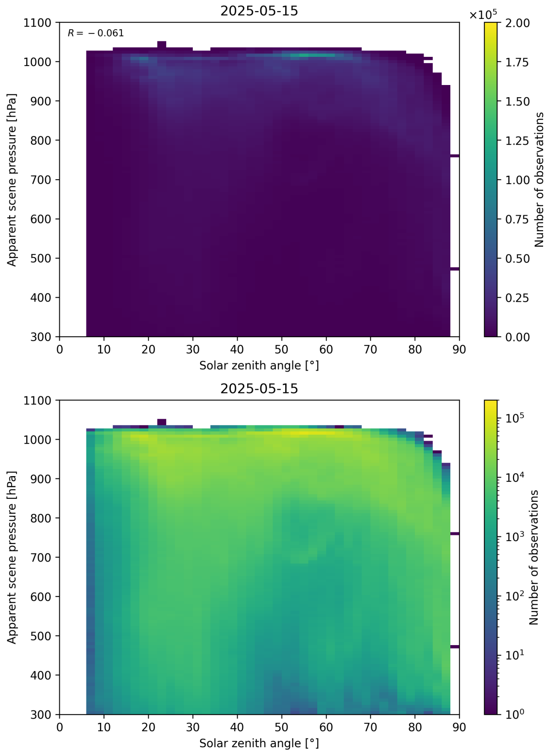
Figure 108: Scatter density plot of “Solar zenith angle” against “Apparent scene pressure” for 2025-05-15 to 2025-05-16.
