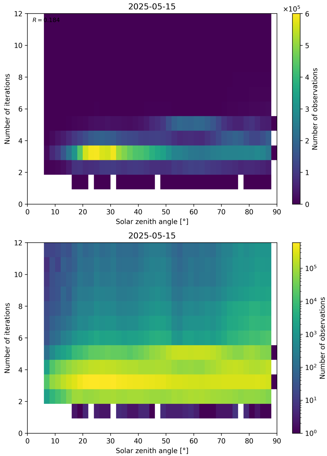
Figure 114: Scatter density plot of “Solar zenith angle” against “Number of iterations” for 2025-05-15 to 2025-05-16.
