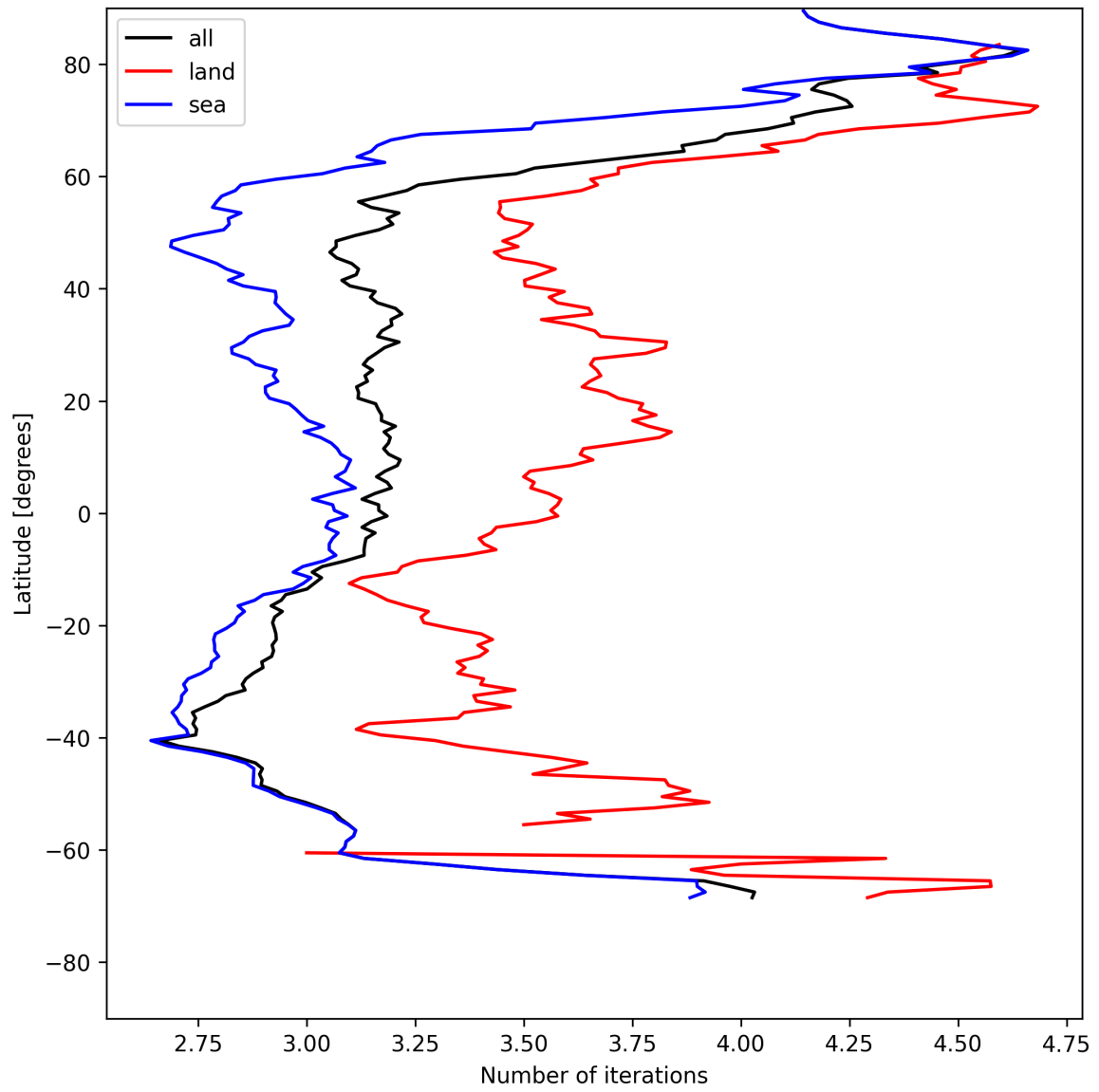
Figure 22: Zonal average of “Number of iterations” for 2025-05-15 to 2025-05-16.
