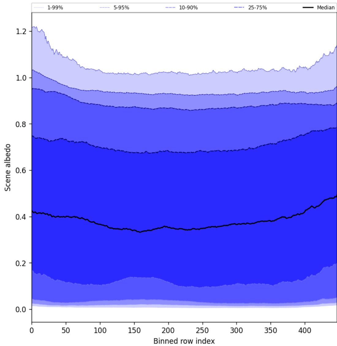
Figure 51: Along track statistics of “Scene albedo” for 2025-05-15 to 2025-05-16
