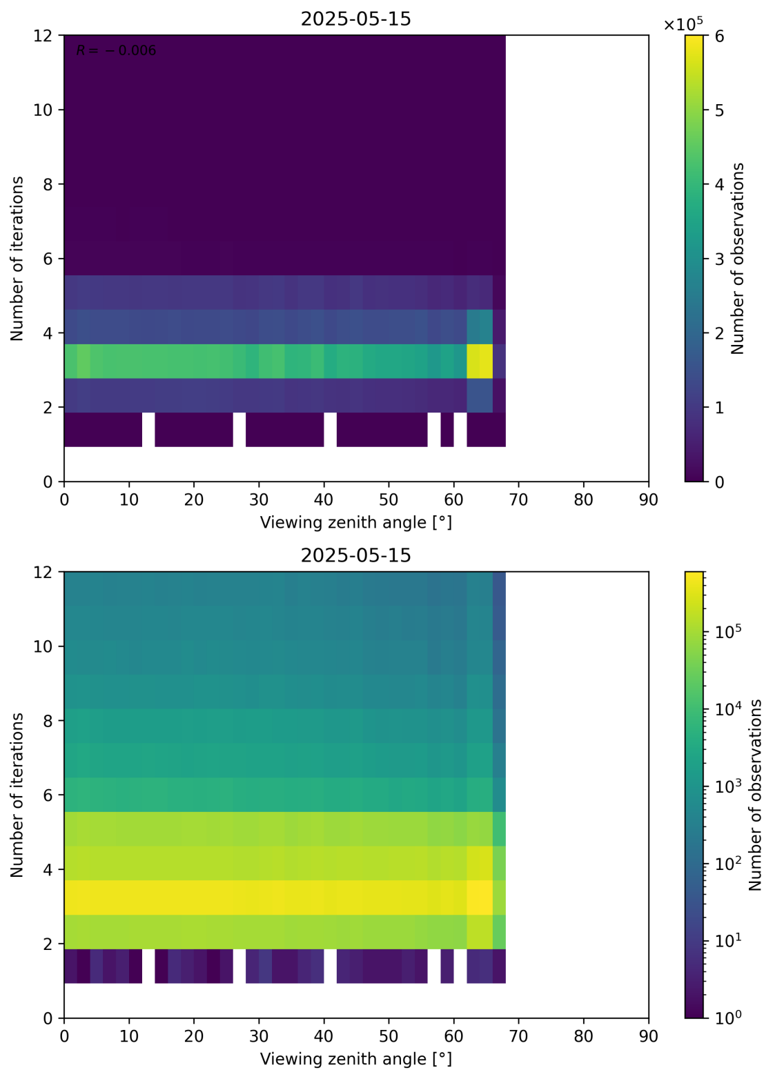
Figure 124: Scatter density plot of “Viewing zenith angle” against “Number of iterations” for 2025-05-15 to 2025-05-16.
