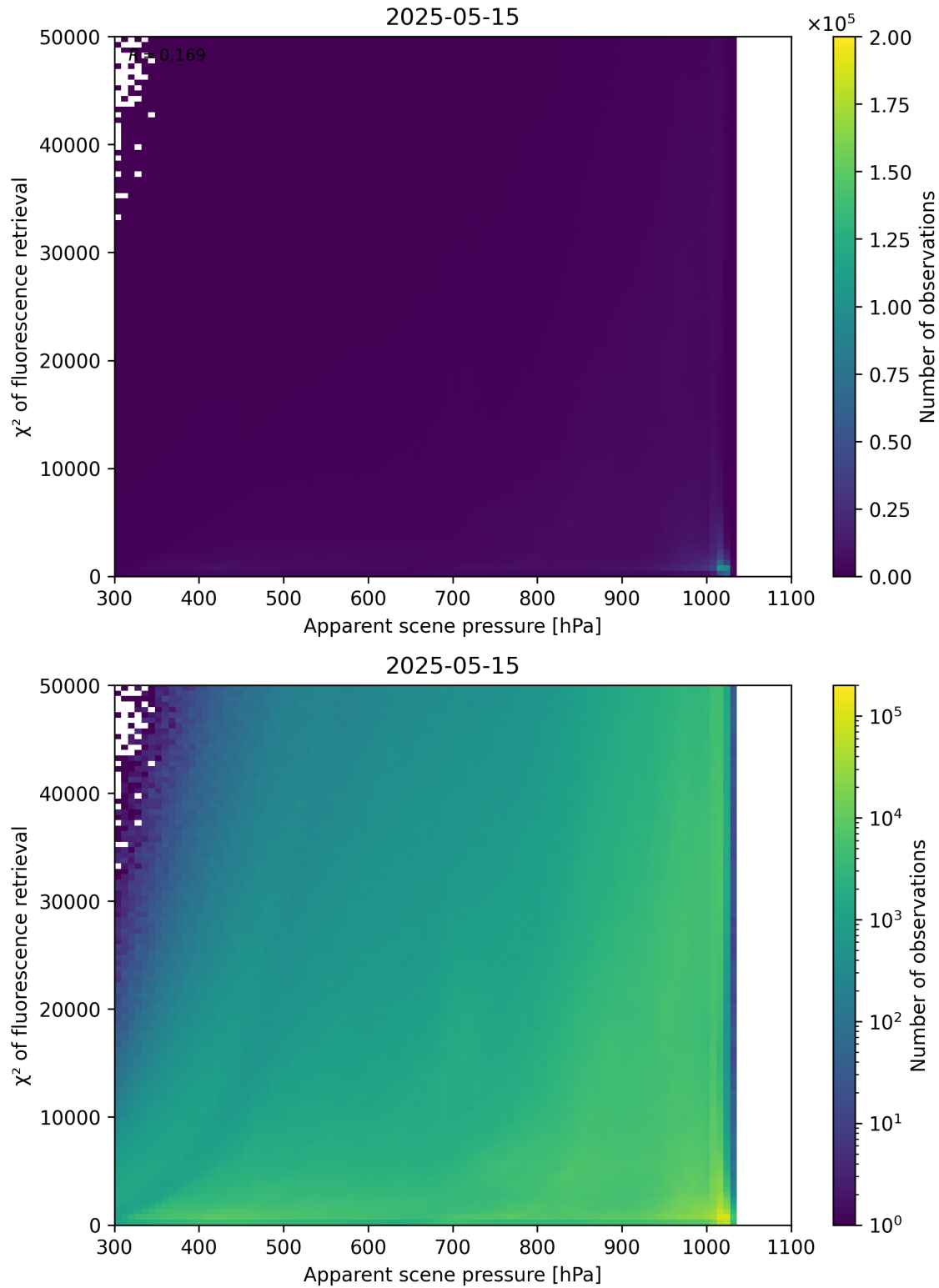
Figure 63: Scatter density plot of “Apparent scene pressure” against “ \chi^2 of fluorescence retrieval” for 2025-05-15 to 2025-05-16.
