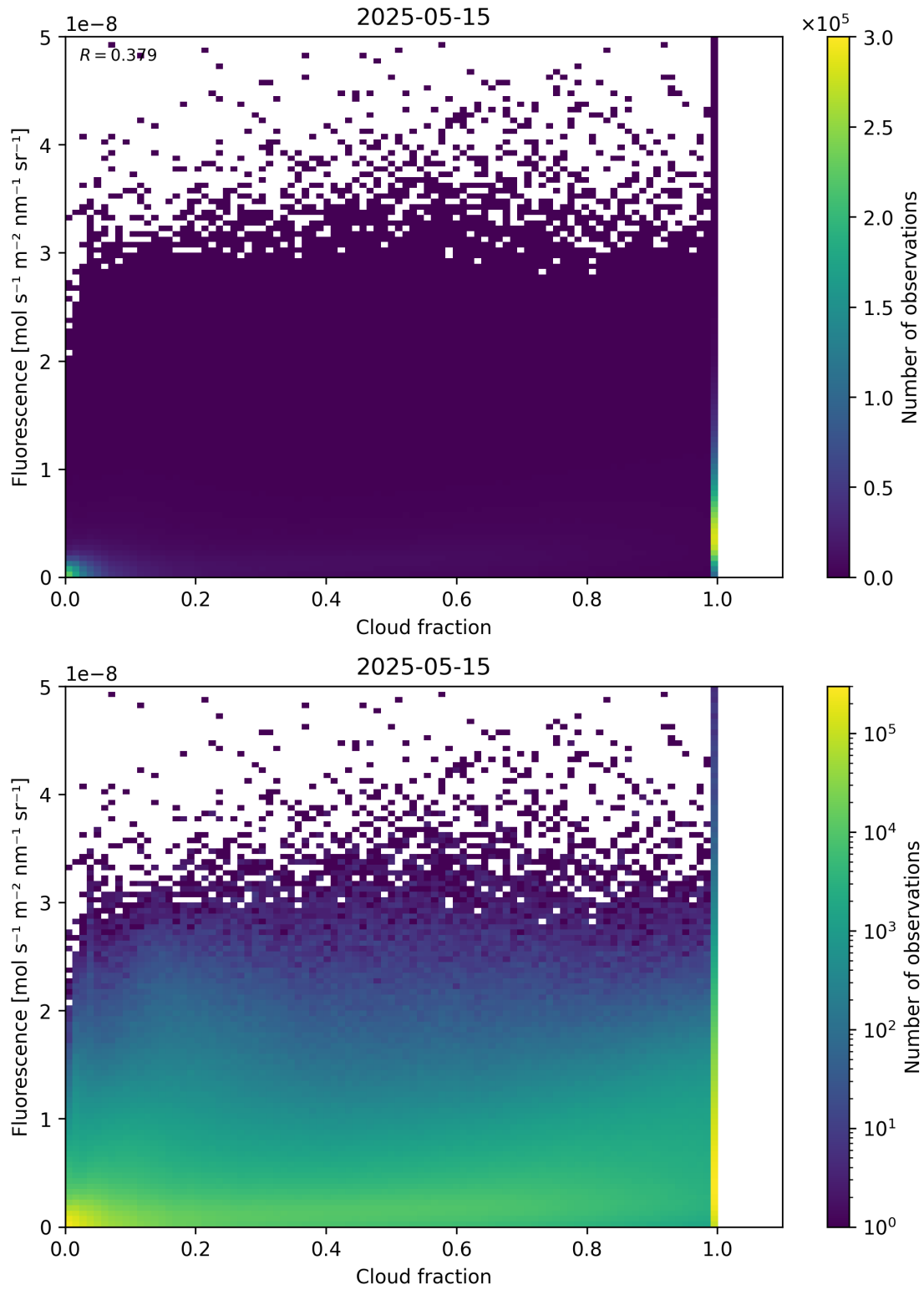
Figure 72: Scatter density plot of “Cloud fraction” against “Fluorescence” for 2025-05-15 to 2025-05-16.
