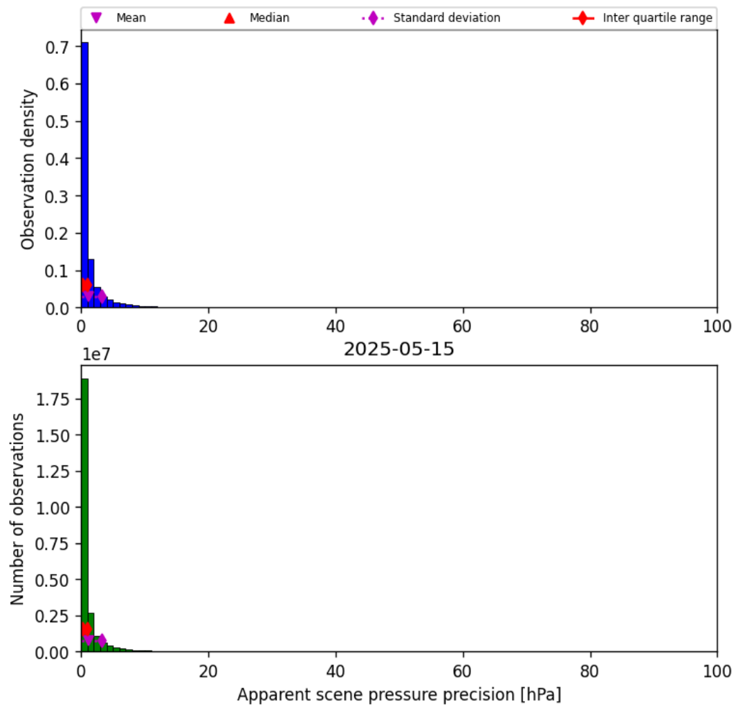
Figure 37: Histogram of “Apparent scene pressure precision” for 2025-05-15 to 2025-05-16
