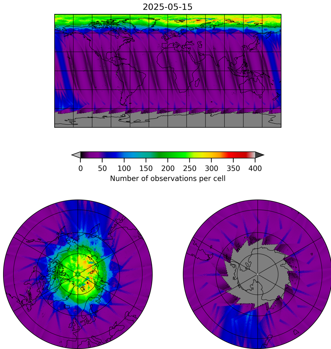
Figure 11: Map of the number of observations for 2025-05-15 to 2025-05-16
