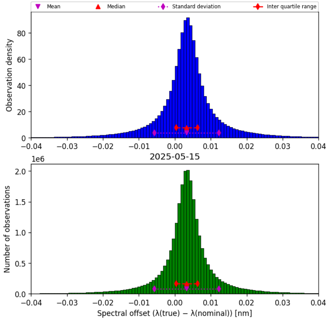
Figure 45: Histogram of “Spectral offset ( \lambda_{\text{true}} - \lambda_{\text{nominal}} )” for 2025-05-15 to 2025-05-16
