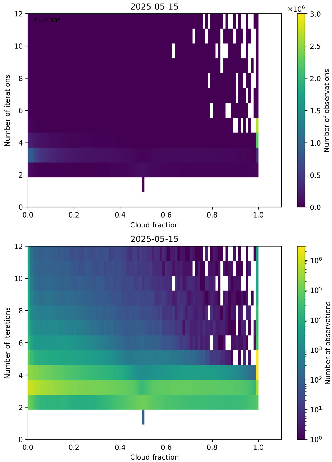
Figure 73: Scatter density plot of “Cloud fraction” against “Number of iterations” for 2025-05-15 to 2025-05-16.
