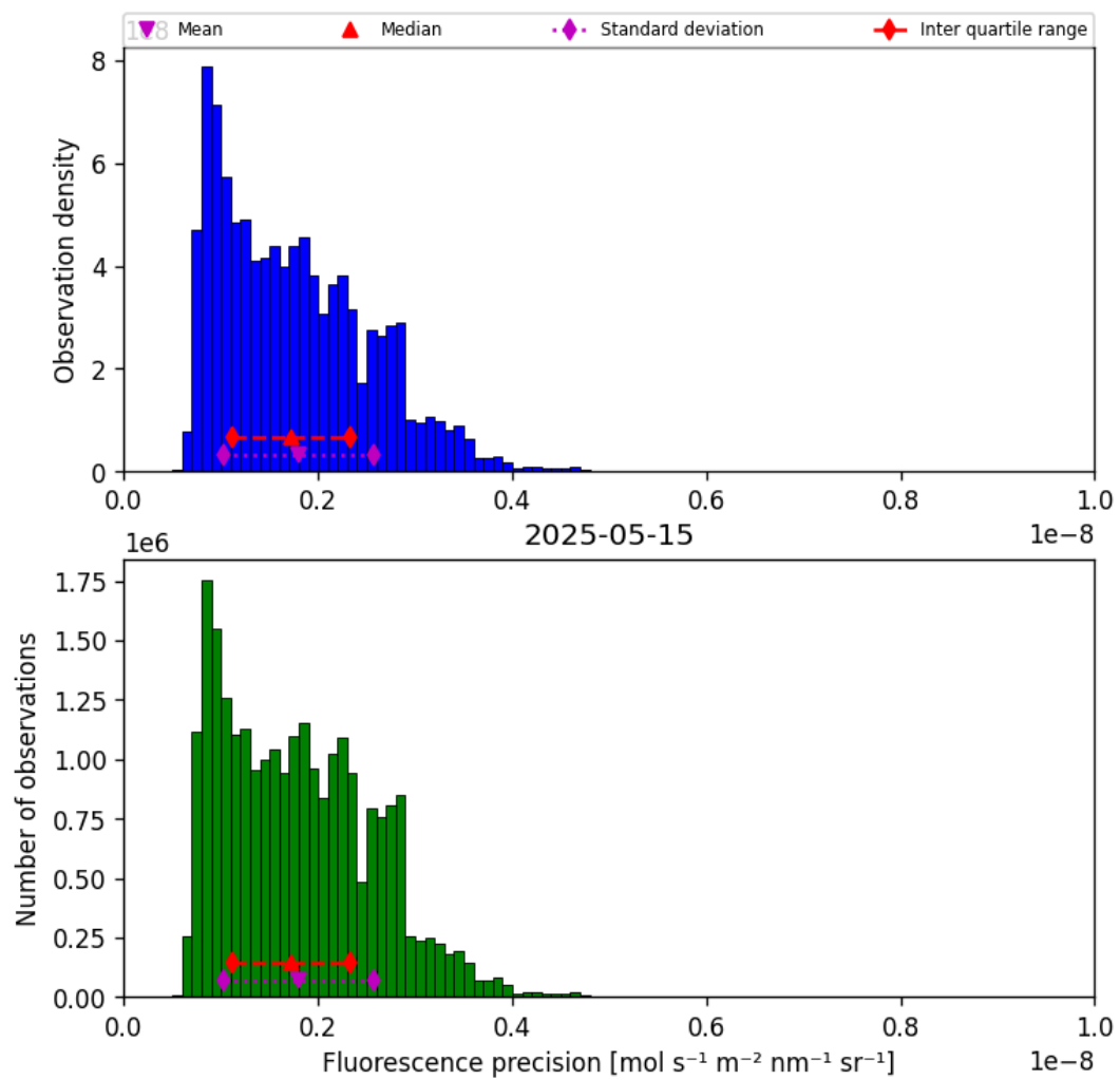
Figure 41: Histogram of “Fluorescence precision” for 2025-05-15 to 2025-05-16
