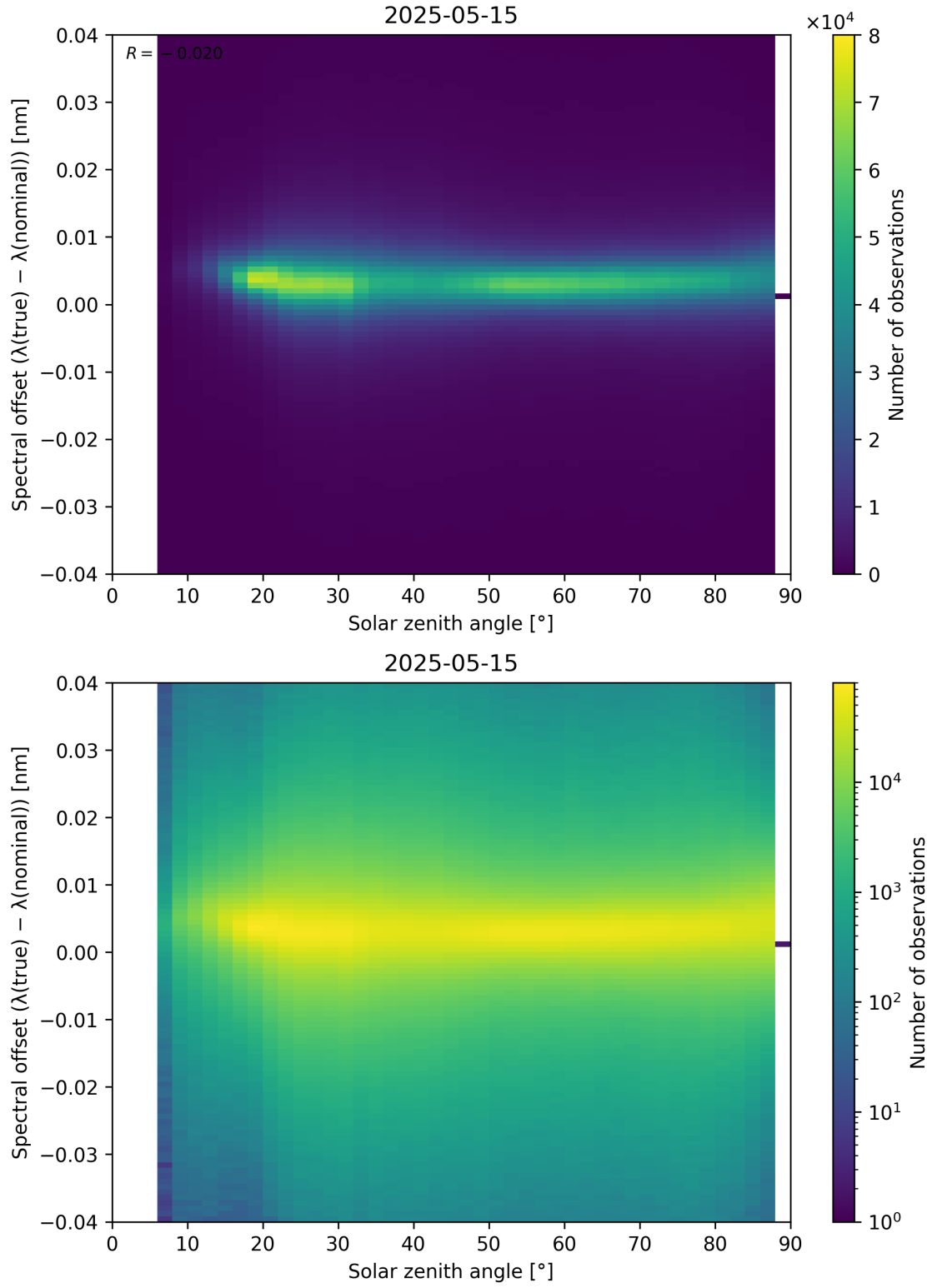
Figure 117: Scatter density plot of “Solar zenith angle” against “Spectral offset ( \lambda_{\text{true}} - \lambda_{\text{nominal}} )” for 2025-05-15 to 2025-05-16.
