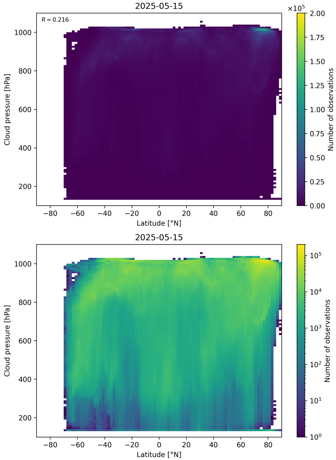
Figure 91: Scatter density plot of “Latitude” against “Cloud pressure” for 2025-05-15 to 2025-05-16.
