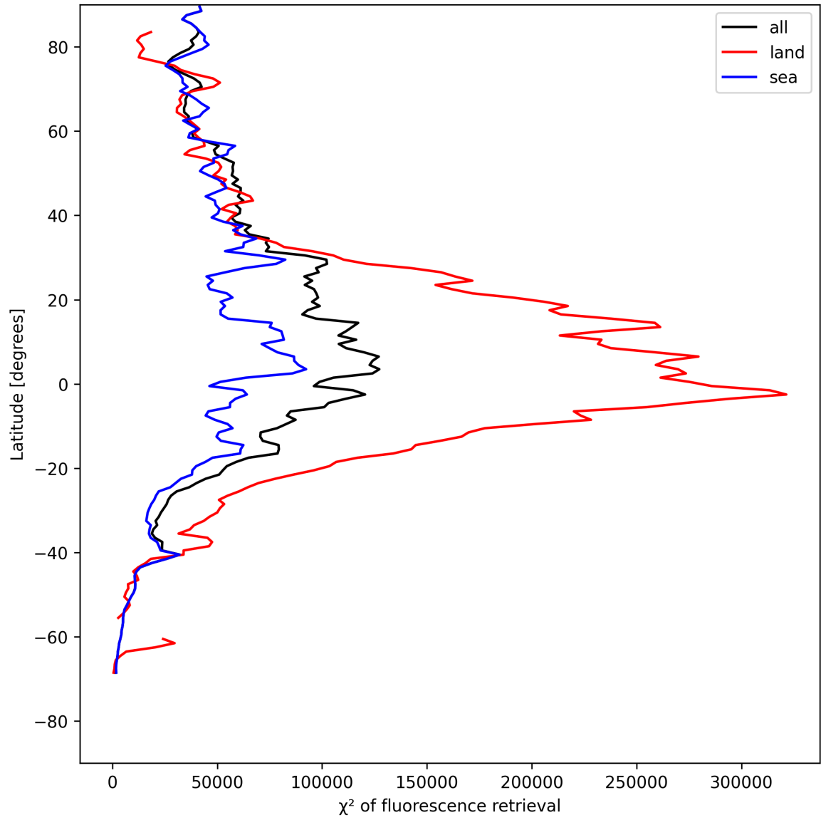
Figure 25: Zonal average of “ \chi^2 of fluorescence retrieval” for 2025-05-15 to 2025-05-16.
