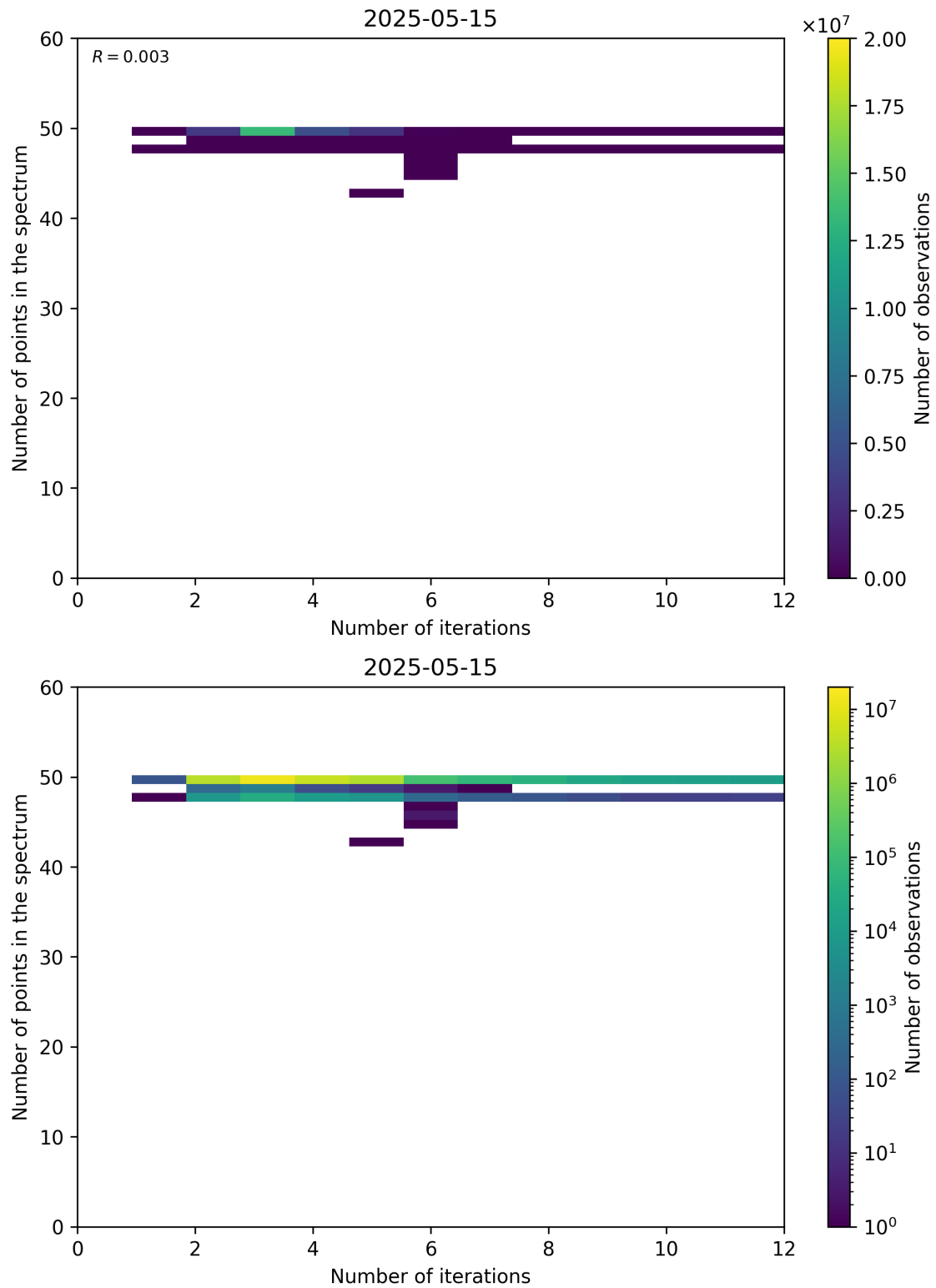
Figure 99: Scatter density plot of “Number of iterations” against “Number of points in the spectrum” for 2025-05-15 to 2025-05-16.
