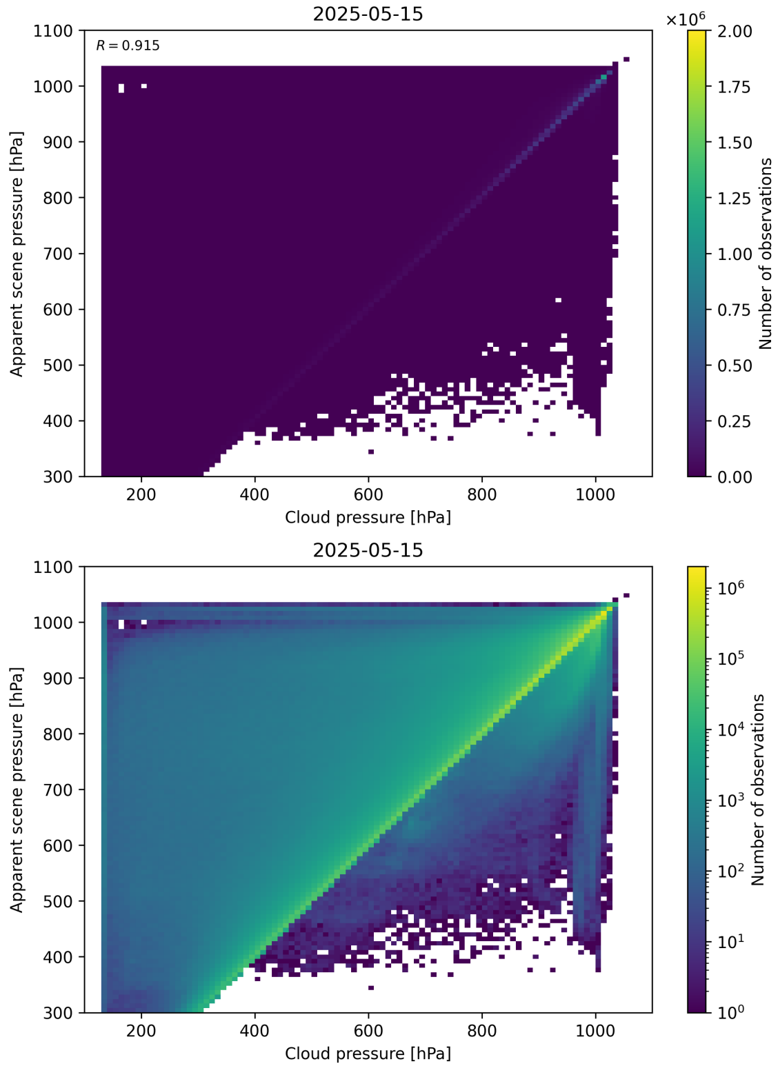
Figure 77: Scatter density plot of “Cloud pressure” against “Apparent scene pressure” for 2025-05-15 to 2025-05-16.
