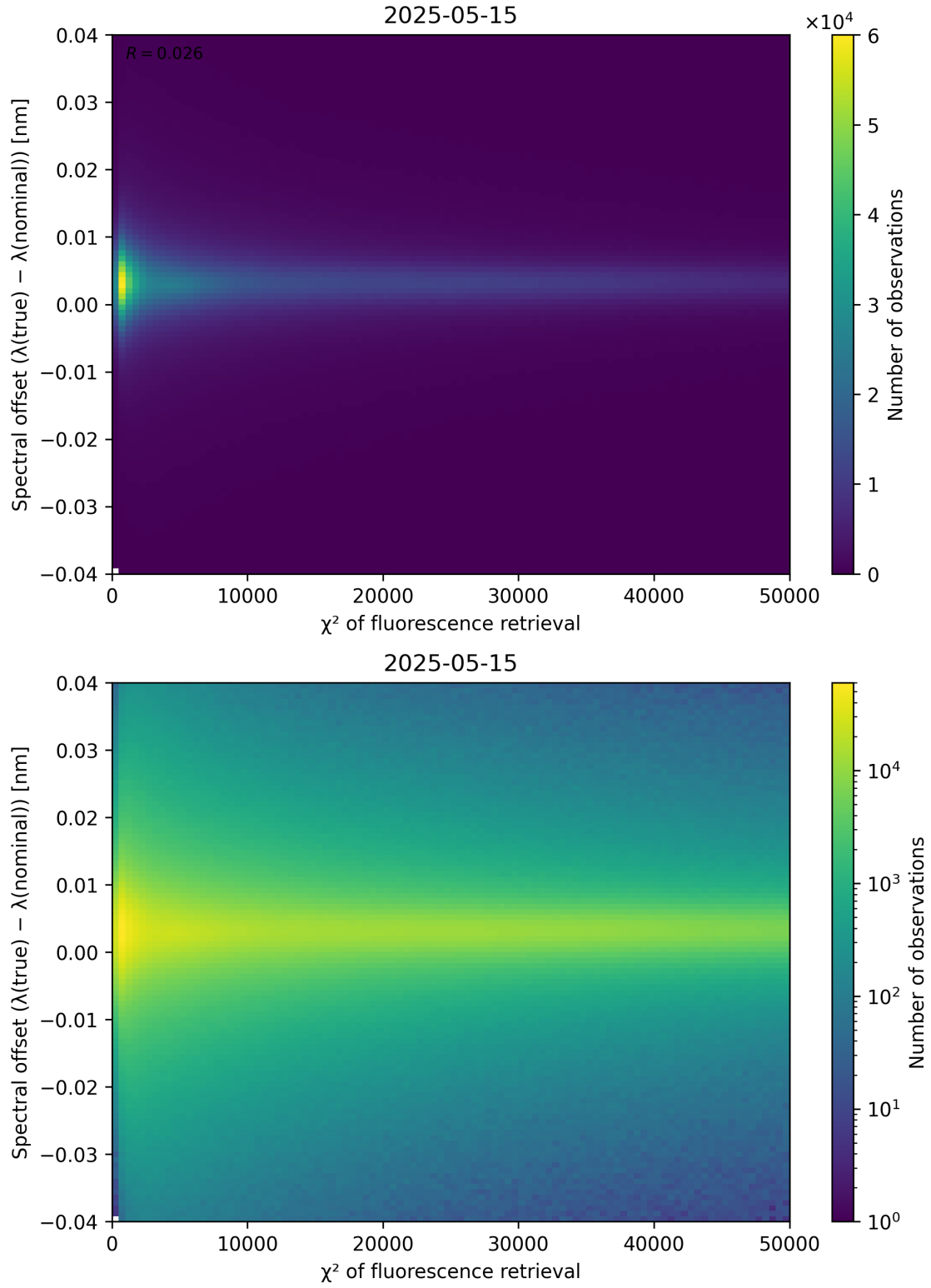
Figure 69: Scatter density plot of “ \chi^2 of fluorescence retrieval” against “Spectral offset ( \lambda_{\text{true}} - \lambda_{\text{nominal}} )” for 2025-05-15 to 2025-05-16.
