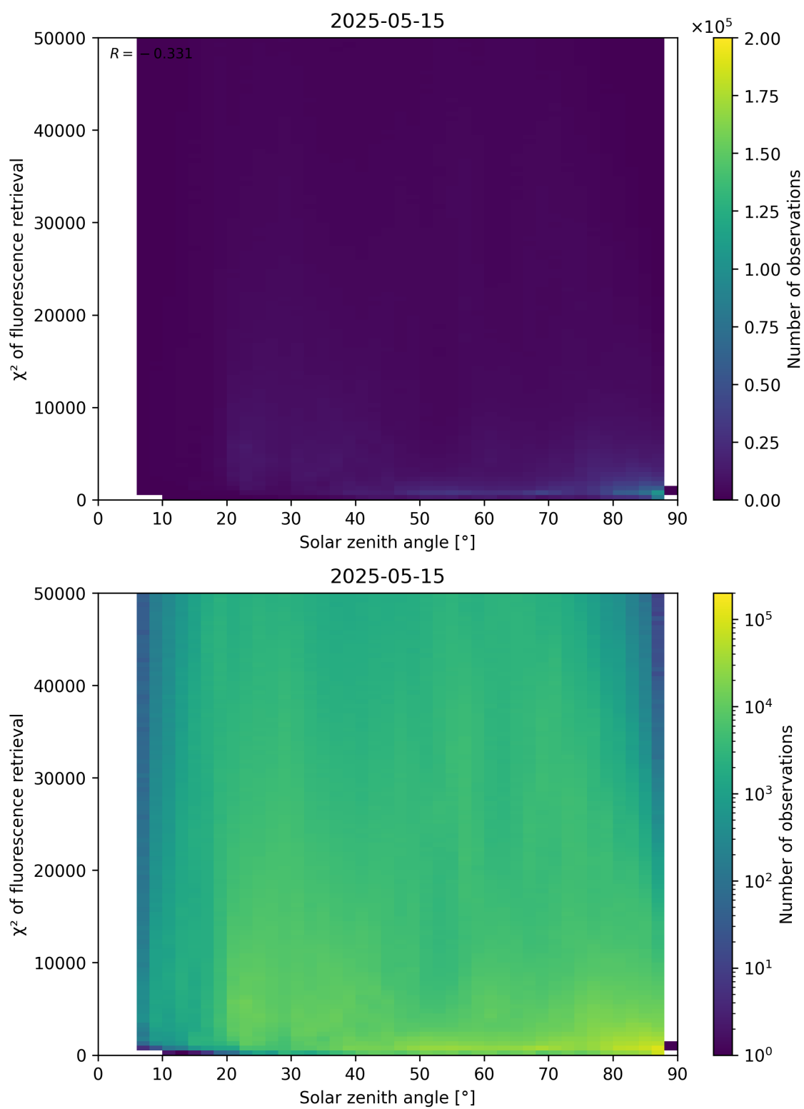
Figure 109: Scatter density plot of “Solar zenith angle” against “ \chi^2 of fluorescence retrieval” for 2025-05-15 to 2025-05-16.
