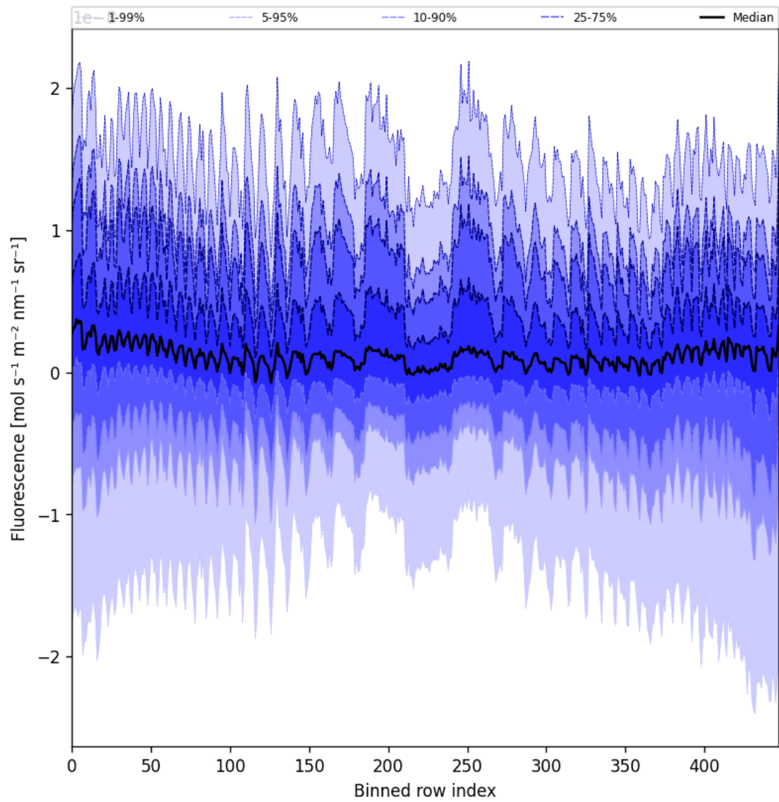
Figure 57: Along track statistics of "Fluorescence" for 2025-05-15 to 2025-05-16
