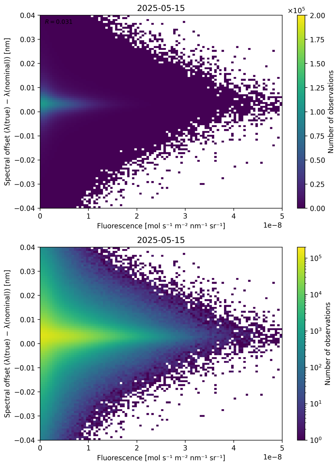
Figure 87: Scatter density plot of “Fluorescence” against “Spectral offset ( \lambda_{\text{true}} - \lambda_{\text{nominal}} )” for 2025-05-15 to 2025-05-16.
