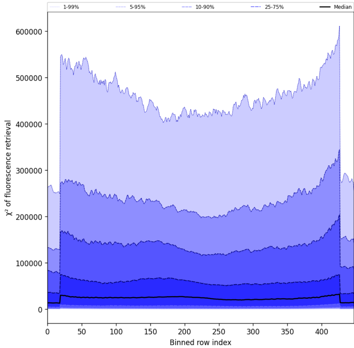
Figure 59: Along track statistics of “ \chi^2 of fluorescence retrieval” for 2025-05-15 to 2025-05-16
