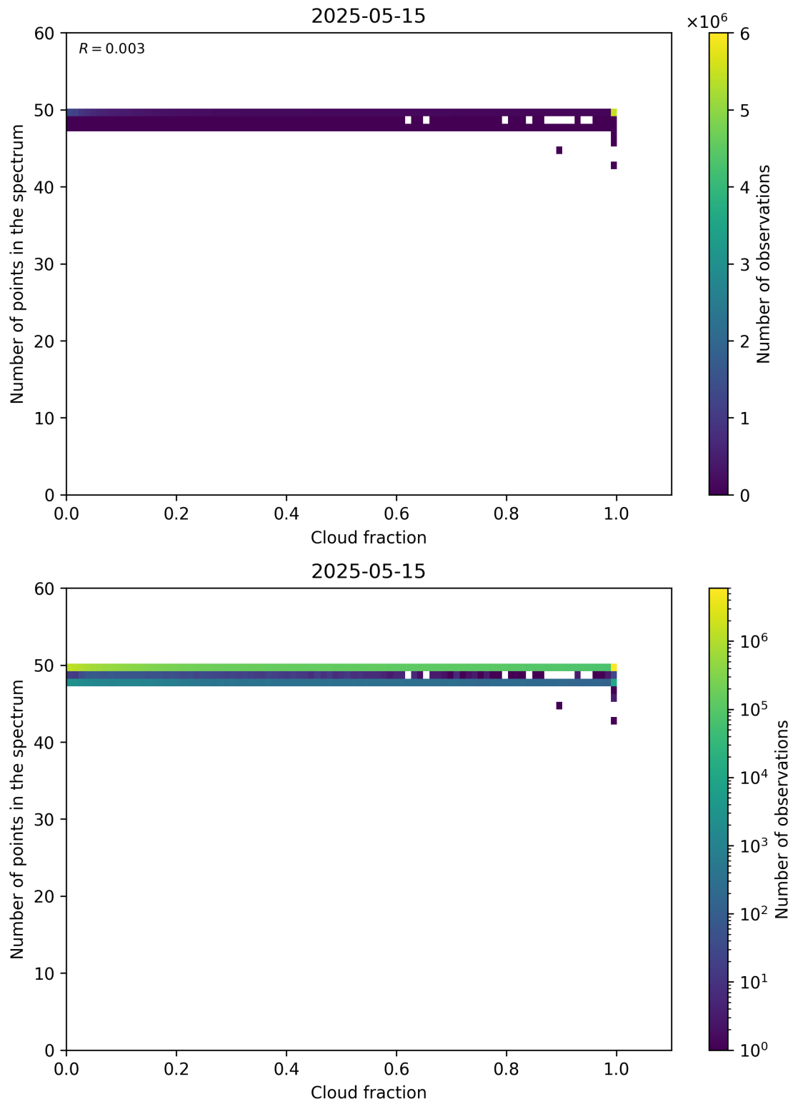
Figure 74: Scatter density plot of “Cloud fraction” against “Number of points in the spectrum” for 2025-05-15 to 2025-05-16.
