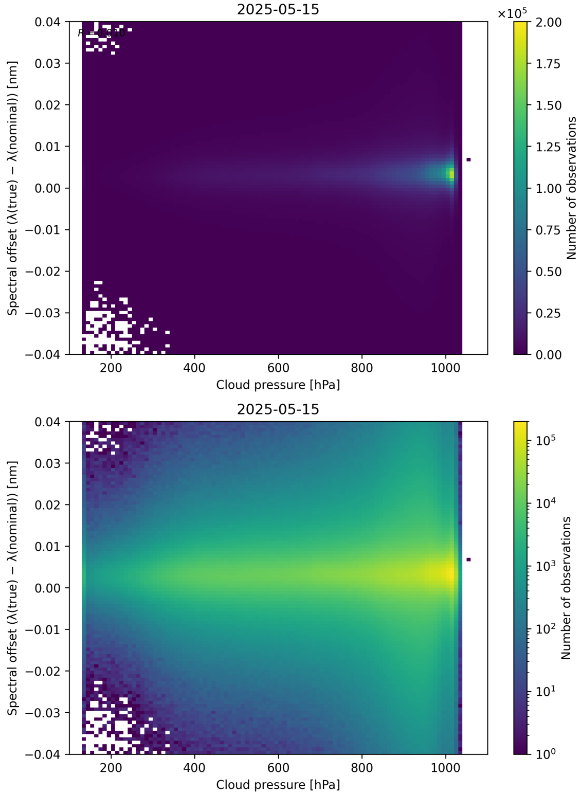
Figure 84: Scatter density plot of “Cloud pressure” against “Spectral offset ( \lambda_{\text{true}} - \lambda_{\text{nominal}} )” for 2025-05-15 to 2025-05-16.
