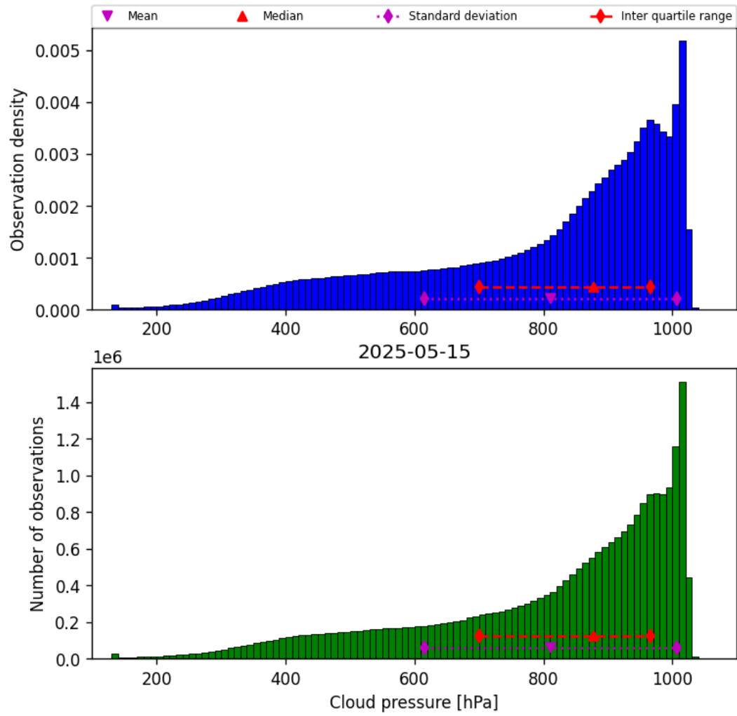
Figure 30: Histogram of “Cloud pressure” for 2025-05-15 to 2025-05-16
