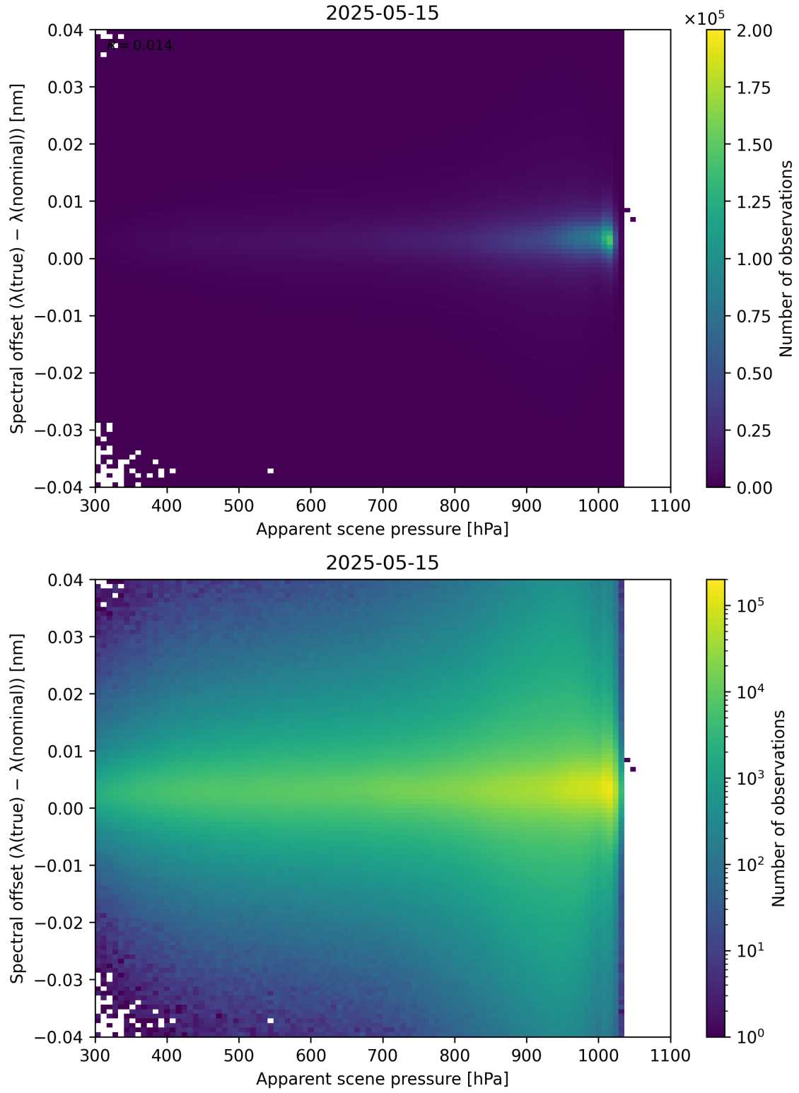
Figure 67: Scatter density plot of “Apparent scene pressure” against “Spectral offset ( \lambda_{\text{true}} - \lambda_{\text{nominal}} )” for 2025-05-15 to 2025-05-16.
