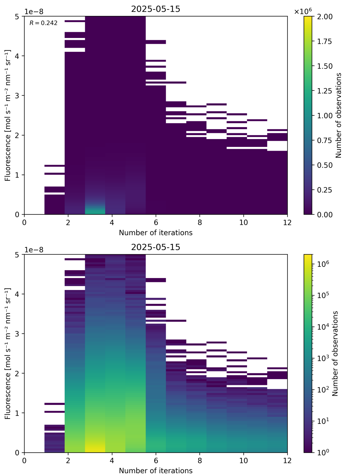
Figure 98: Scatter density plot of “Number of iterations” against “Fluorescence” for 2025-05-15 to 2025-05-16.
