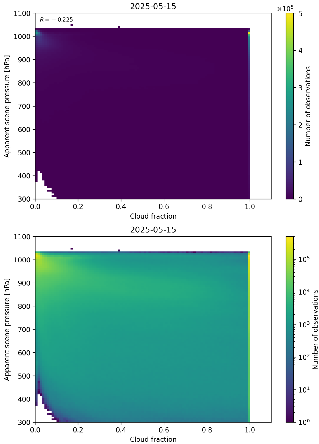
Figure 70: Scatter density plot of “Cloud fraction” against “Apparent scene pressure” for 2025-05-15 to 2025-05-16.
