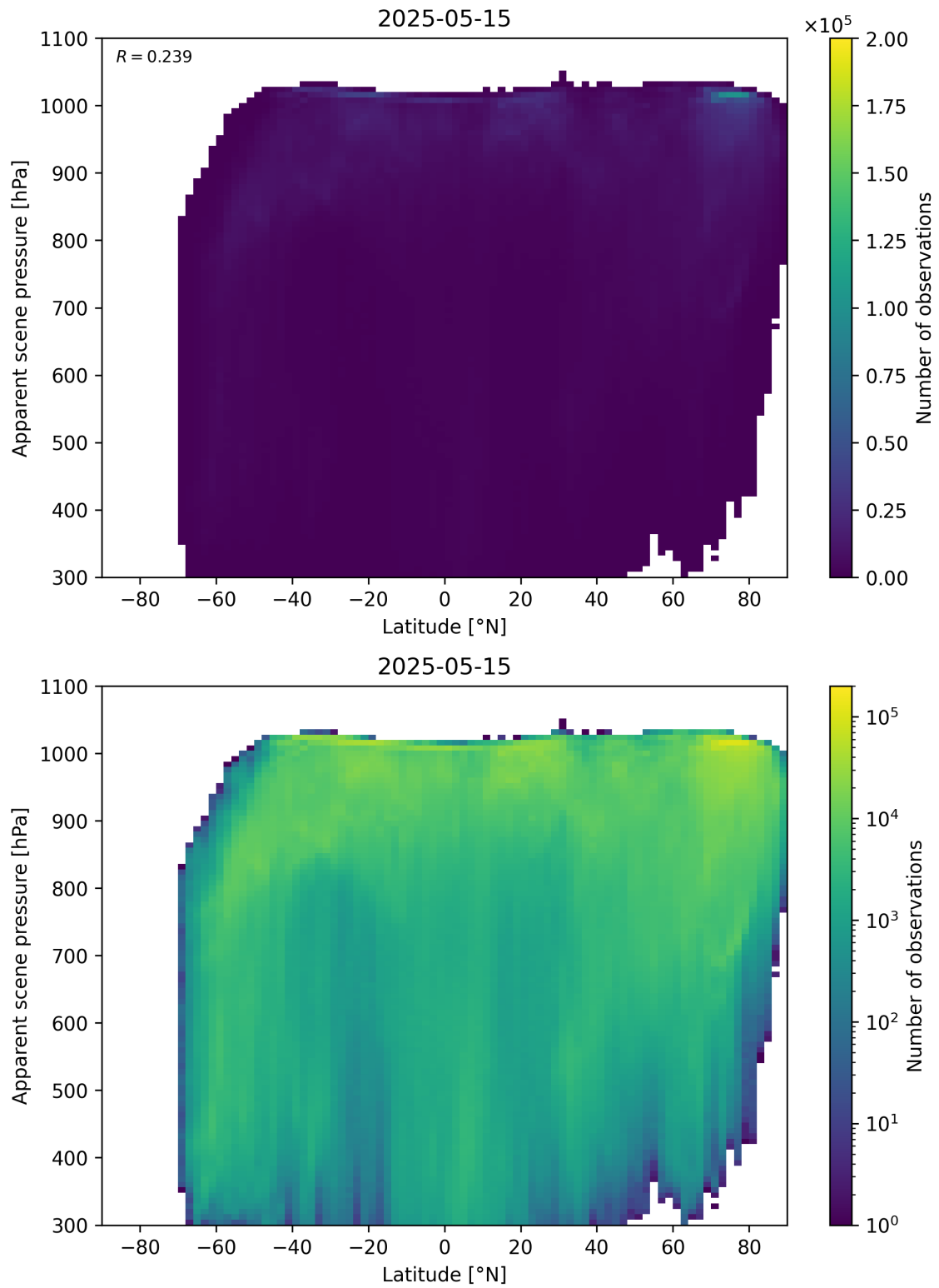
Figure 88: Scatter density plot of “Latitude” against “Apparent scene pressure” for 2025-05-15 to 2025-05-16.
