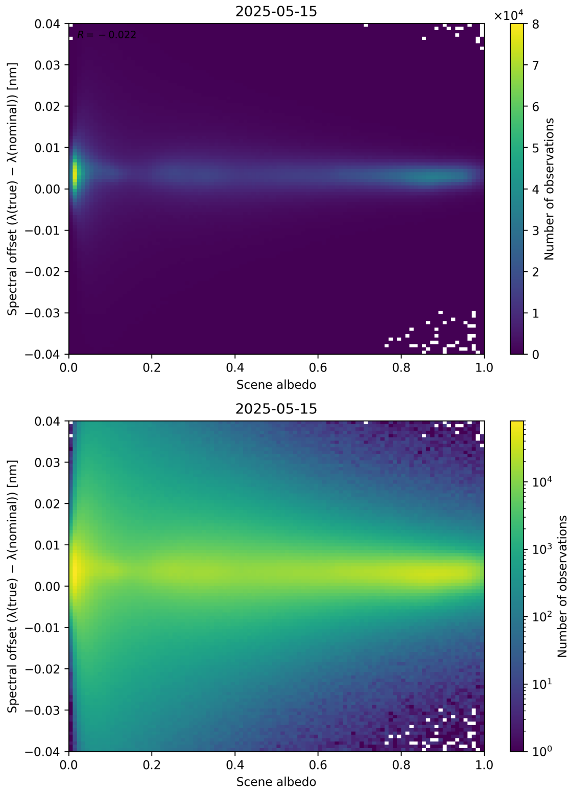
Figure 107: Scatter density plot of “Scene albedo” against “Spectral offset ( \lambda_{\text{true}} - \lambda_{\text{nominal}} )” for 2025-05-15 to 2025-05-16.
