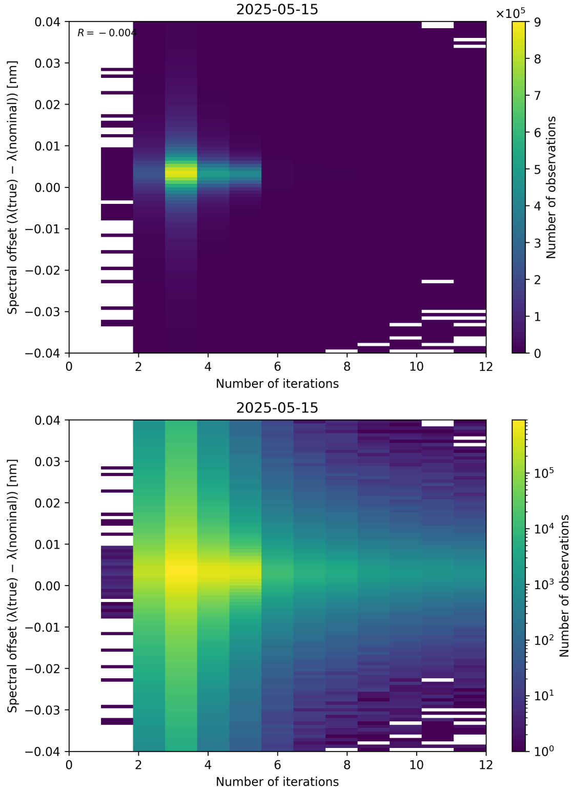
Figure 100: Scatter density plot of “Number of iterations” against “Spectral offset ( \lambda_{\text{true}} - \lambda_{\text{nominal}} )” for 2025-05-15 to 2025-05-16.
