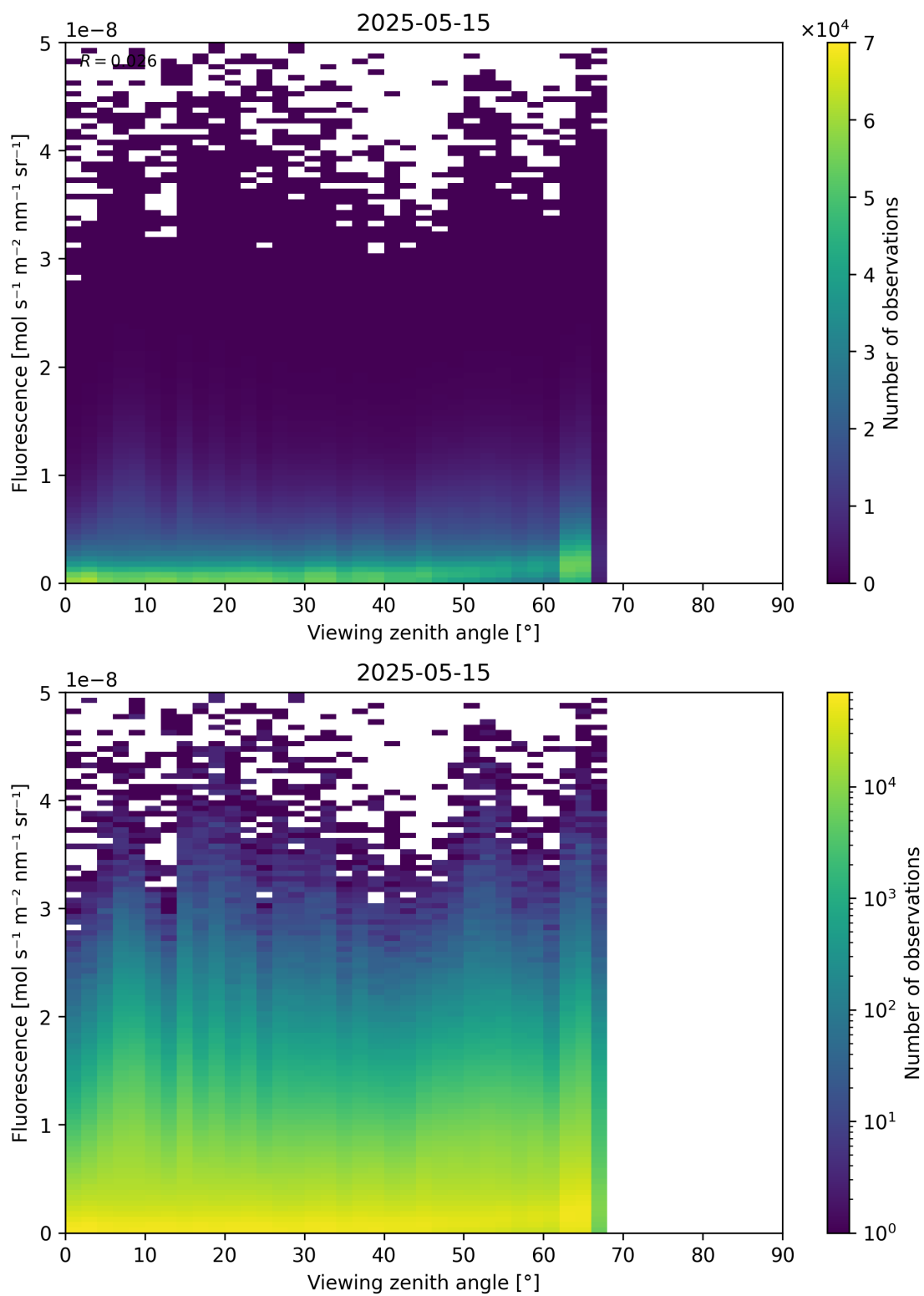
Figure 122: Scatter density plot of “Viewing zenith angle” against “Fluorescence” for 2025-05-15 to 2025-05-16.
