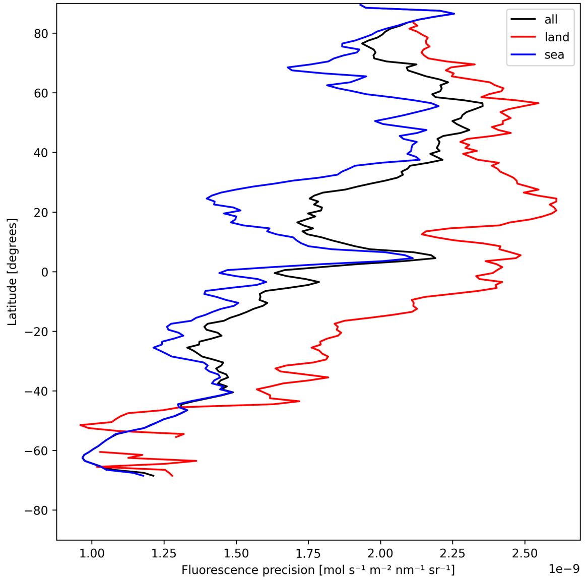
Figure 24: Zonal average of “Fluorescence precision” for 2025-05-15 to 2025-05-16.
