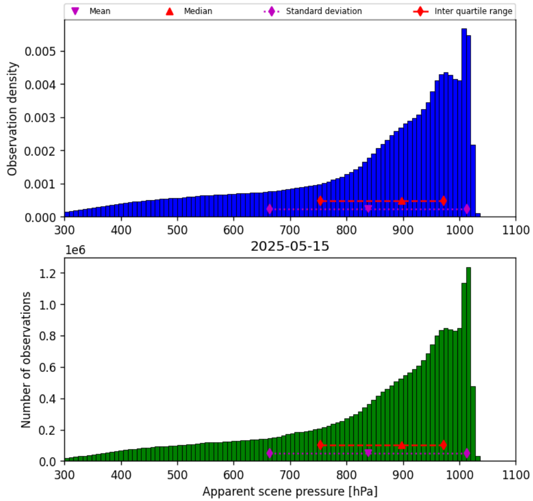
Figure 36: Histogram of “Apparent scene pressure” for 2025-05-15 to 2025-05-16
