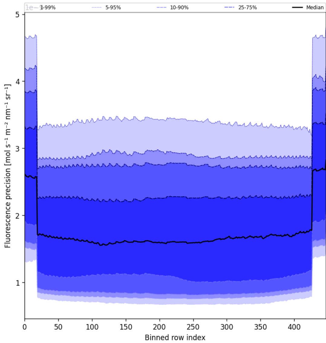
Figure 58: Along track statistics of “Fluorescence precision” for 2025-05-15 to 2025-05-16
