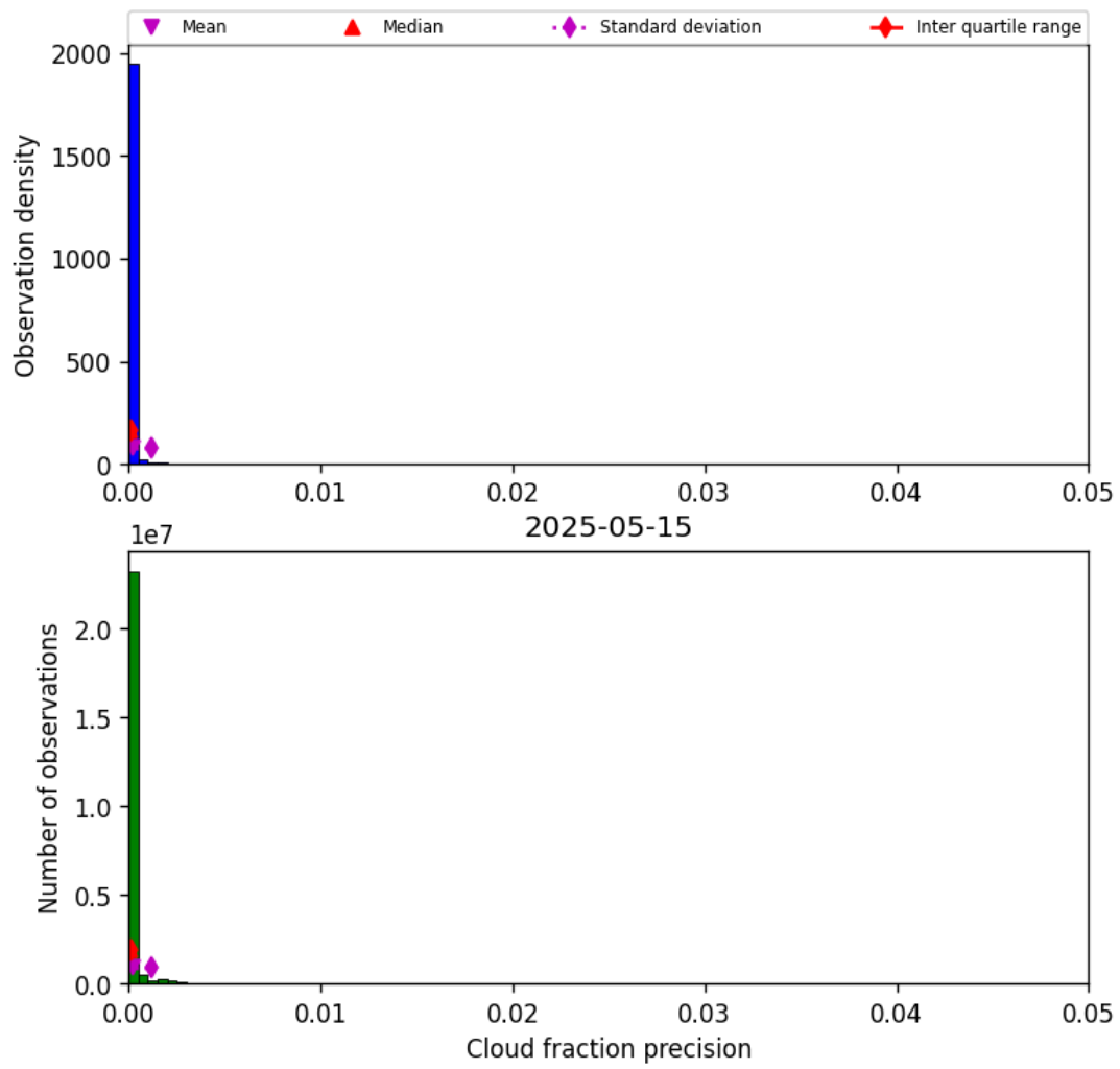
Figure 33: Histogram of “Cloud fraction precision” for 2025-05-15 to 2025-05-16
