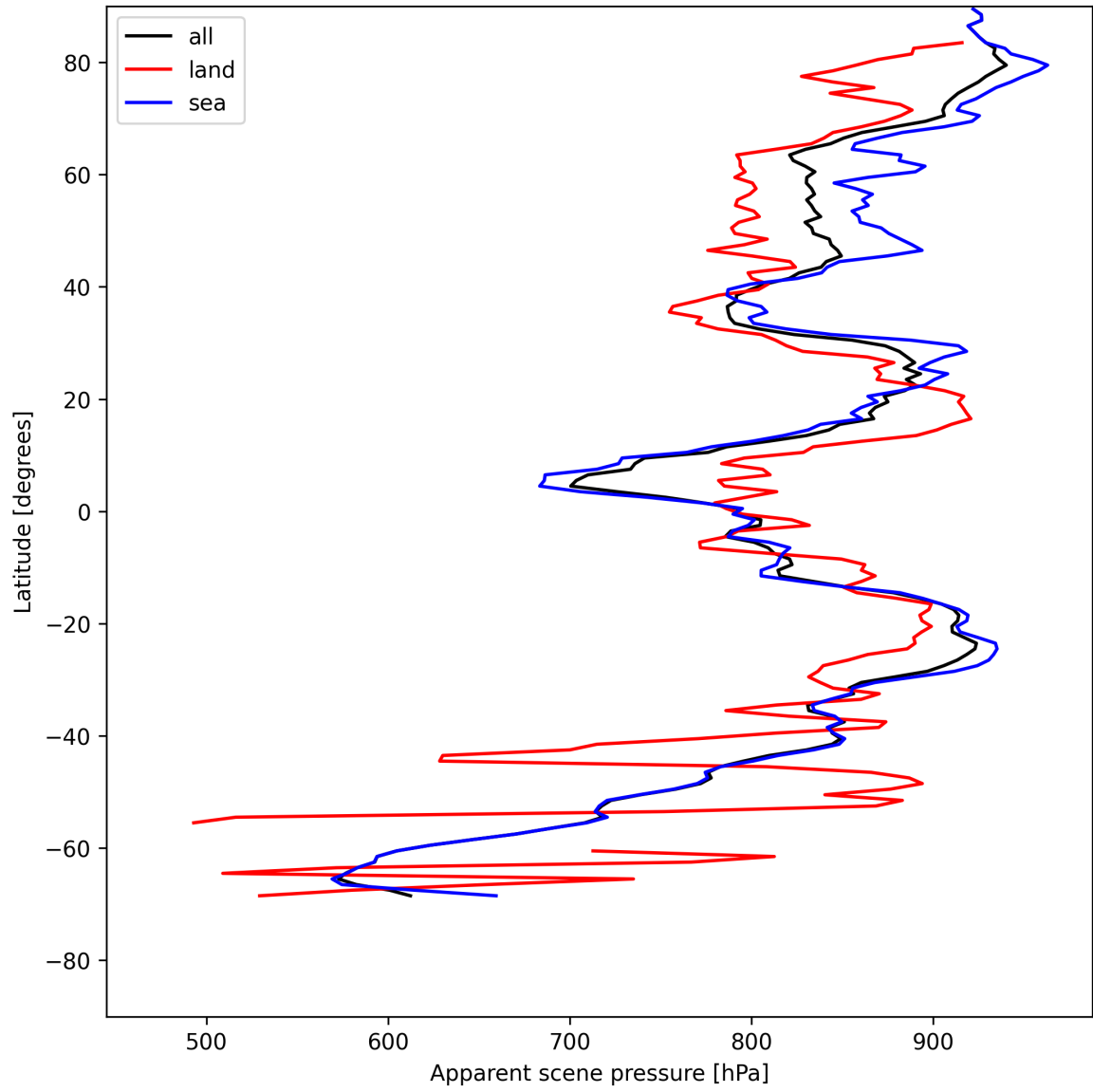
Figure 19: Zonal average of “Apparent scene pressure” for 2025-05-15 to 2025-05-16.
