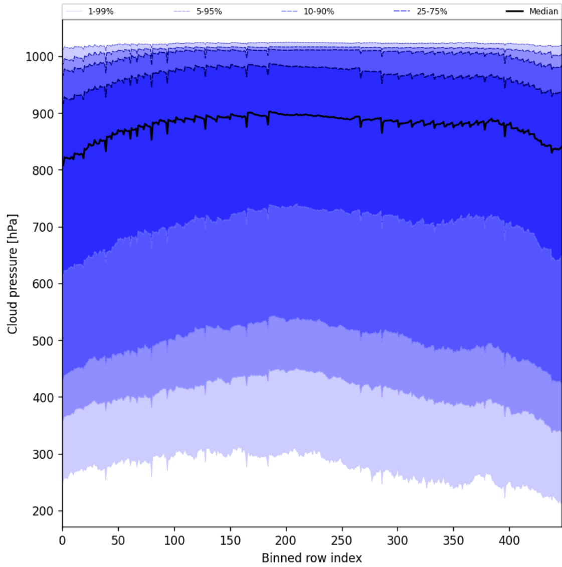
Figure 47: Along track statistics of “Cloud pressure” for 2025-05-15 to 2025-05-16
