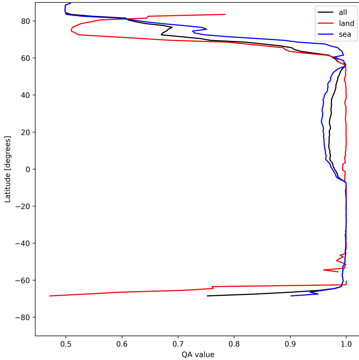
Figure 12: Zonal average of “QA value” for 2025-05-15 to 2025-05-16.
