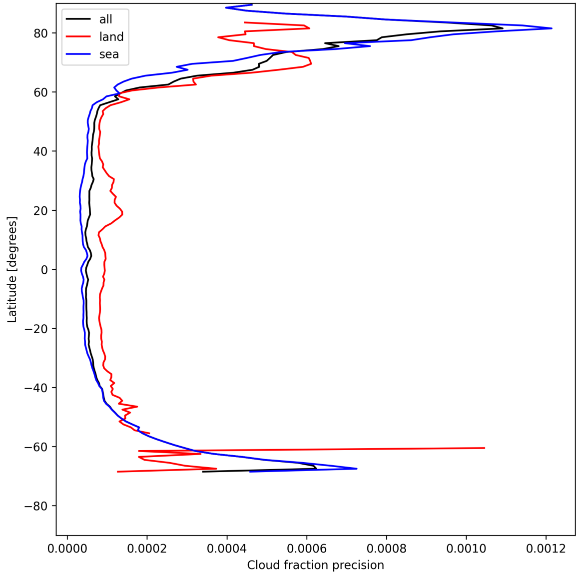
Figure 16: Zonal average of “Cloud fraction precision” for 2025-05-15 to 2025-05-16.
