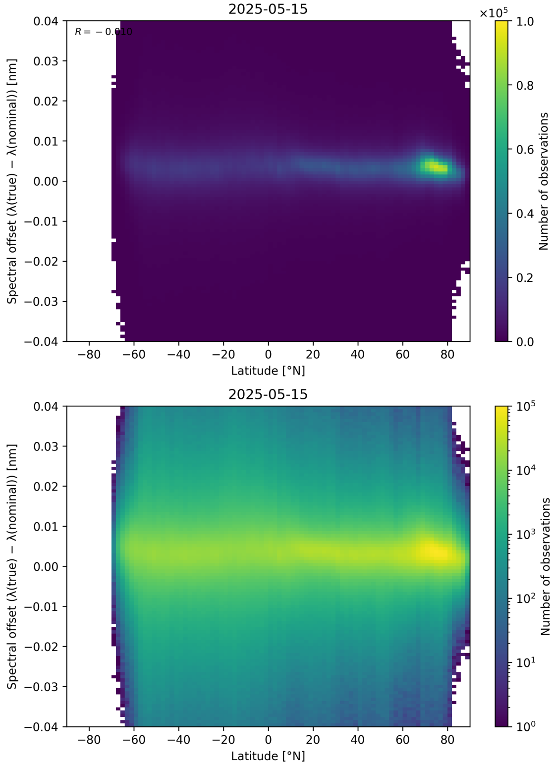
Figure 96: Scatter density plot of “Latitude” against “Spectral offset ( \lambda_{\text{true}} - \lambda_{\text{nominal}} )” for 2025-05-15 to 2025-05-16.
