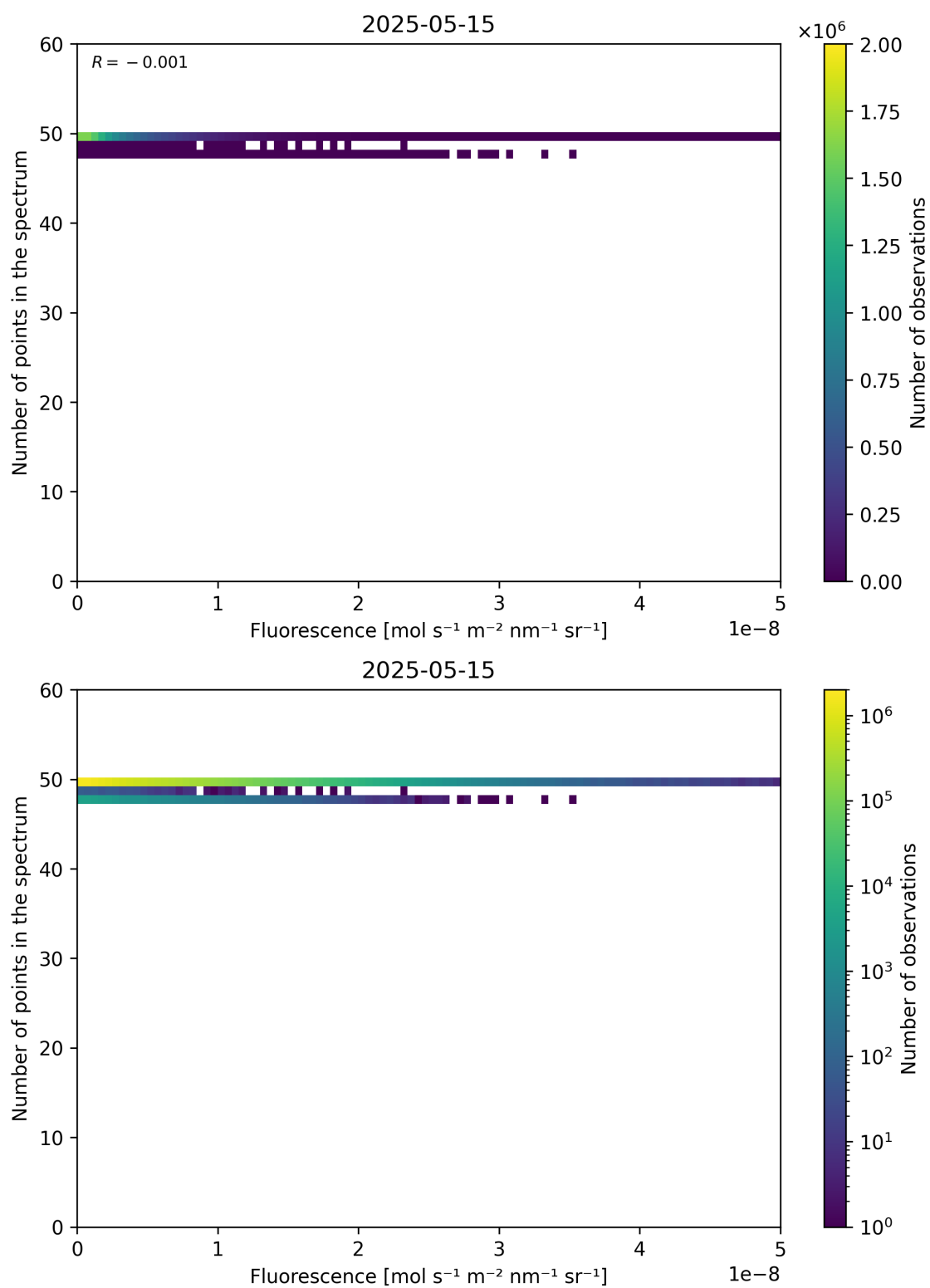
Figure 86: Scatter density plot of “Fluorescence” against “Number of points in the spectrum” for 2025-05-15 to 2025-05-16.
