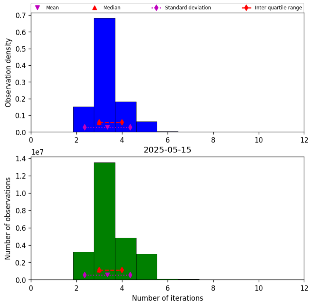
Figure 39: Histogram of “Number of iterations” for 2025-05-15 to 2025-05-16
