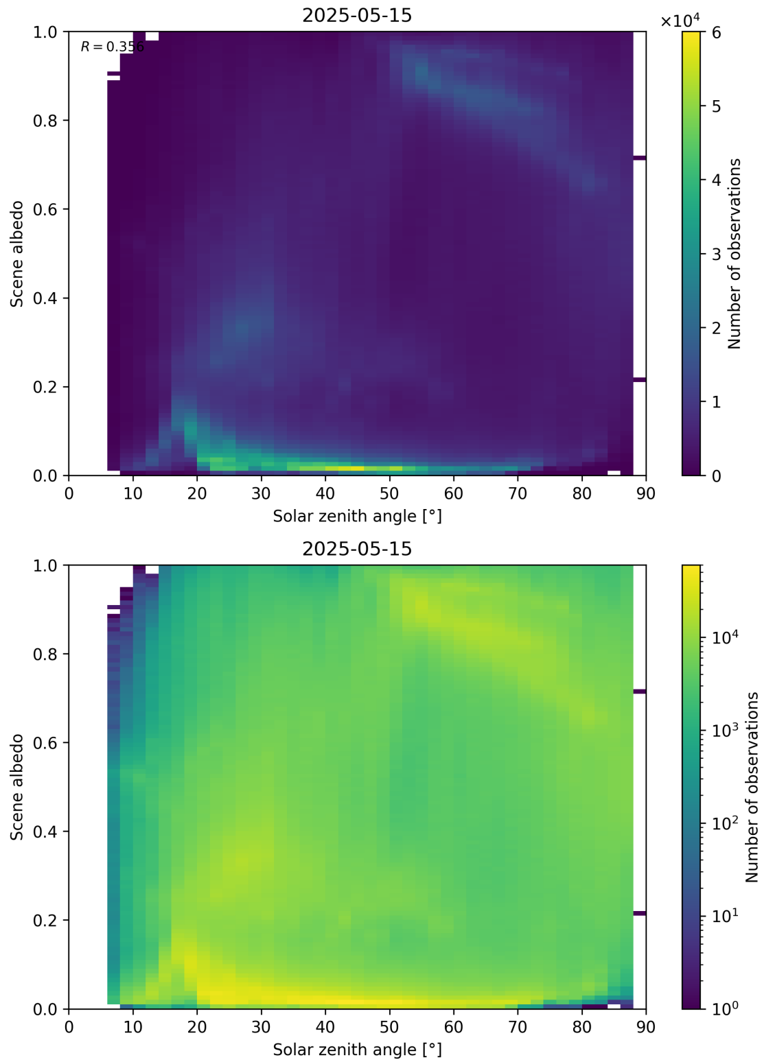
Figure 116: Scatter density plot of “Solar zenith angle” against “Scene albedo” for 2025-05-15 to 2025-05-16.
