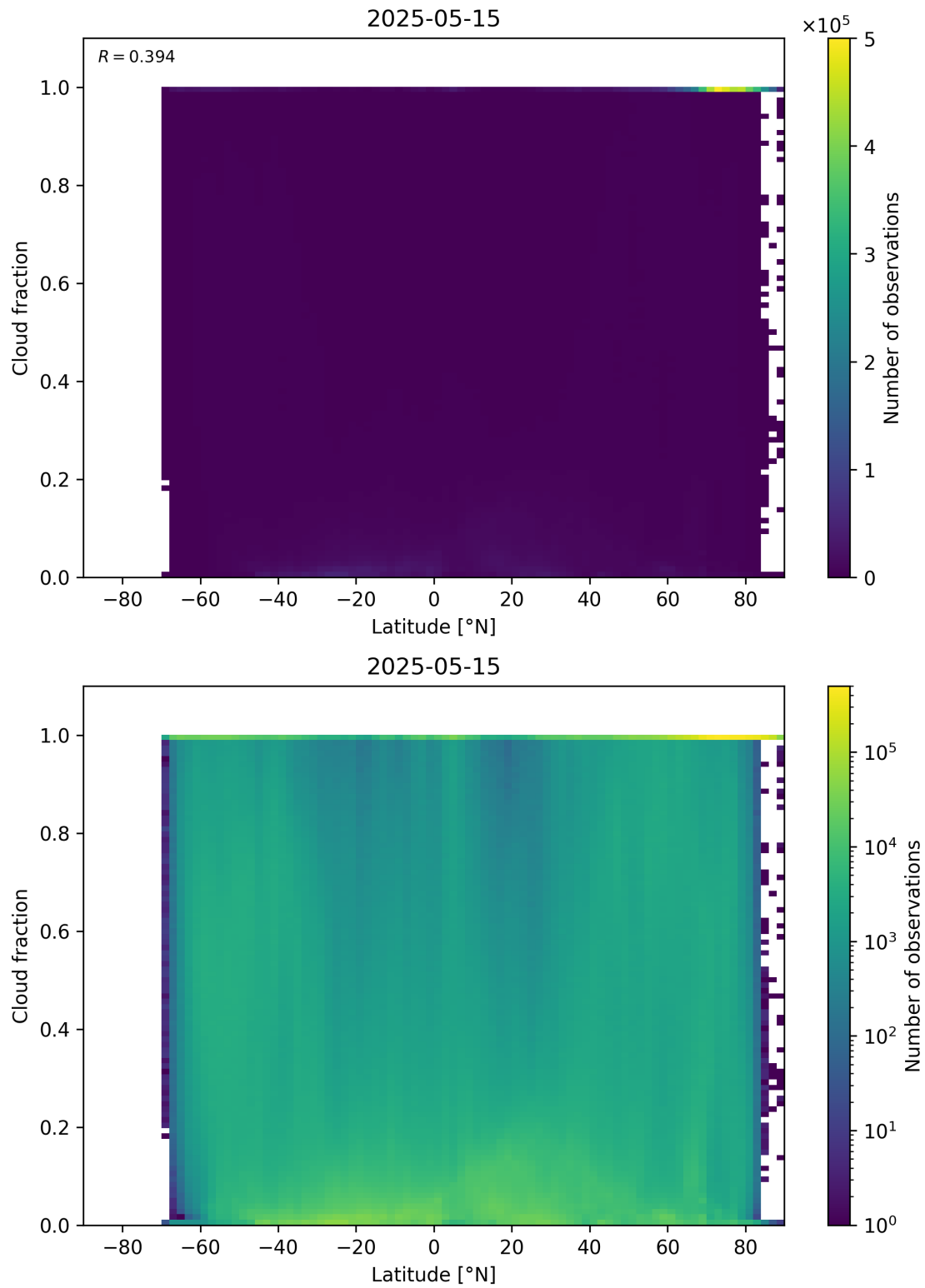
Figure 90: Scatter density plot of “Latitude” against “Cloud fraction” for 2025-05-15 to 2025-05-16.
