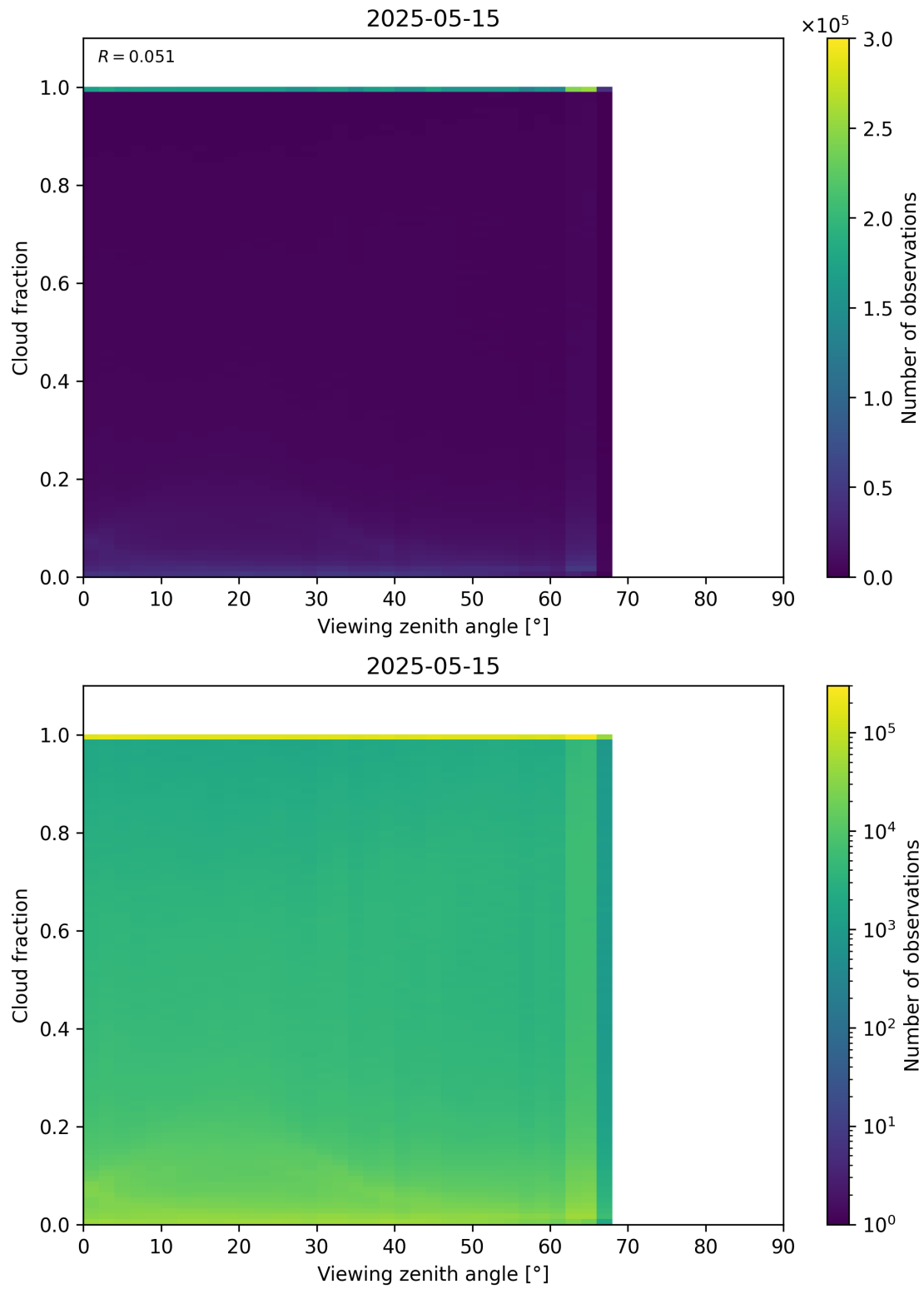
Figure 120: Scatter density plot of “Viewing zenith angle” against “Cloud fraction” for 2025-05-15 to 2025-05-16.
