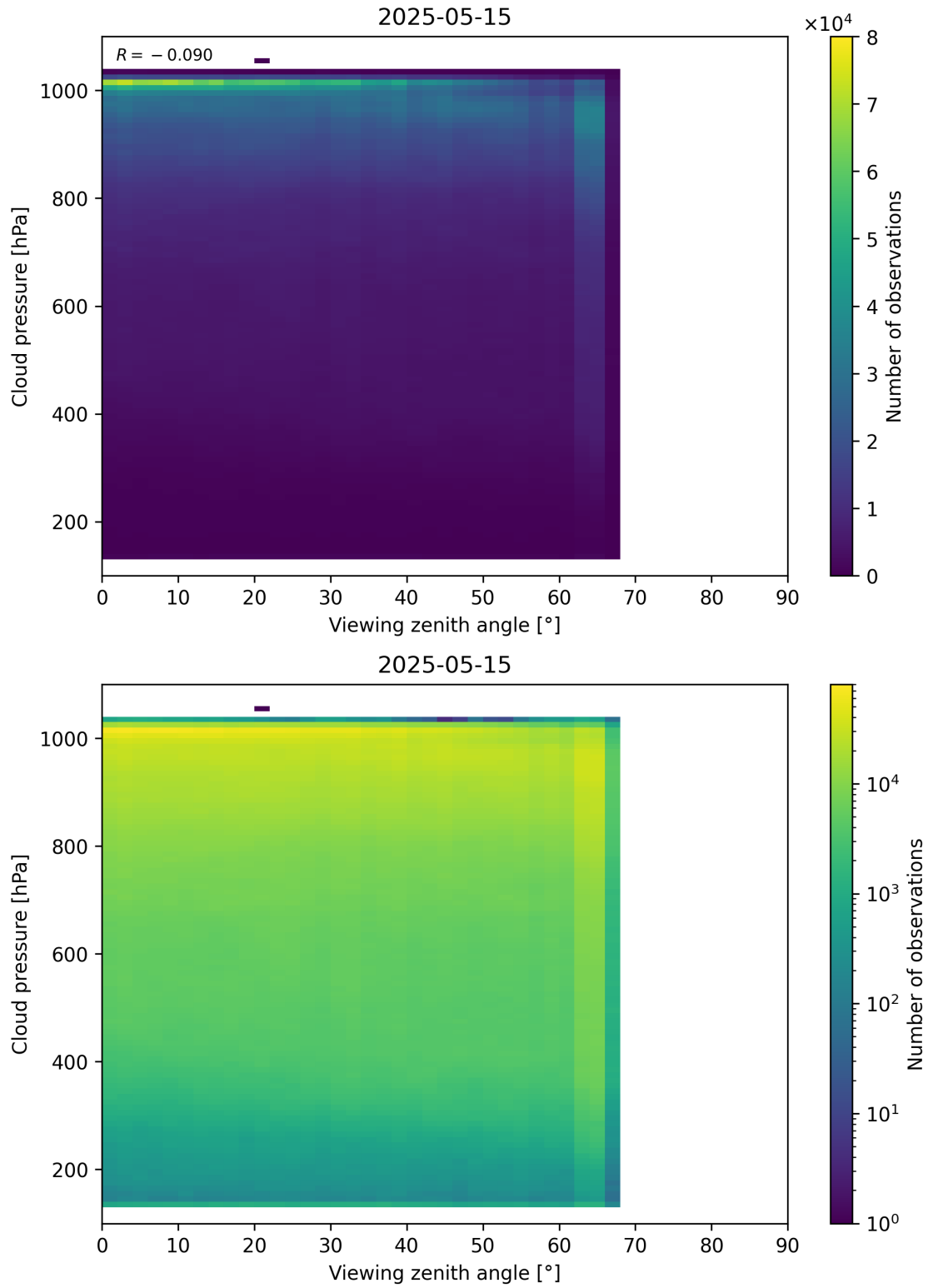
Figure 121: Scatter density plot of “Viewing zenith angle” against “Cloud pressure” for 2025-05-15 to 2025-05-16.
