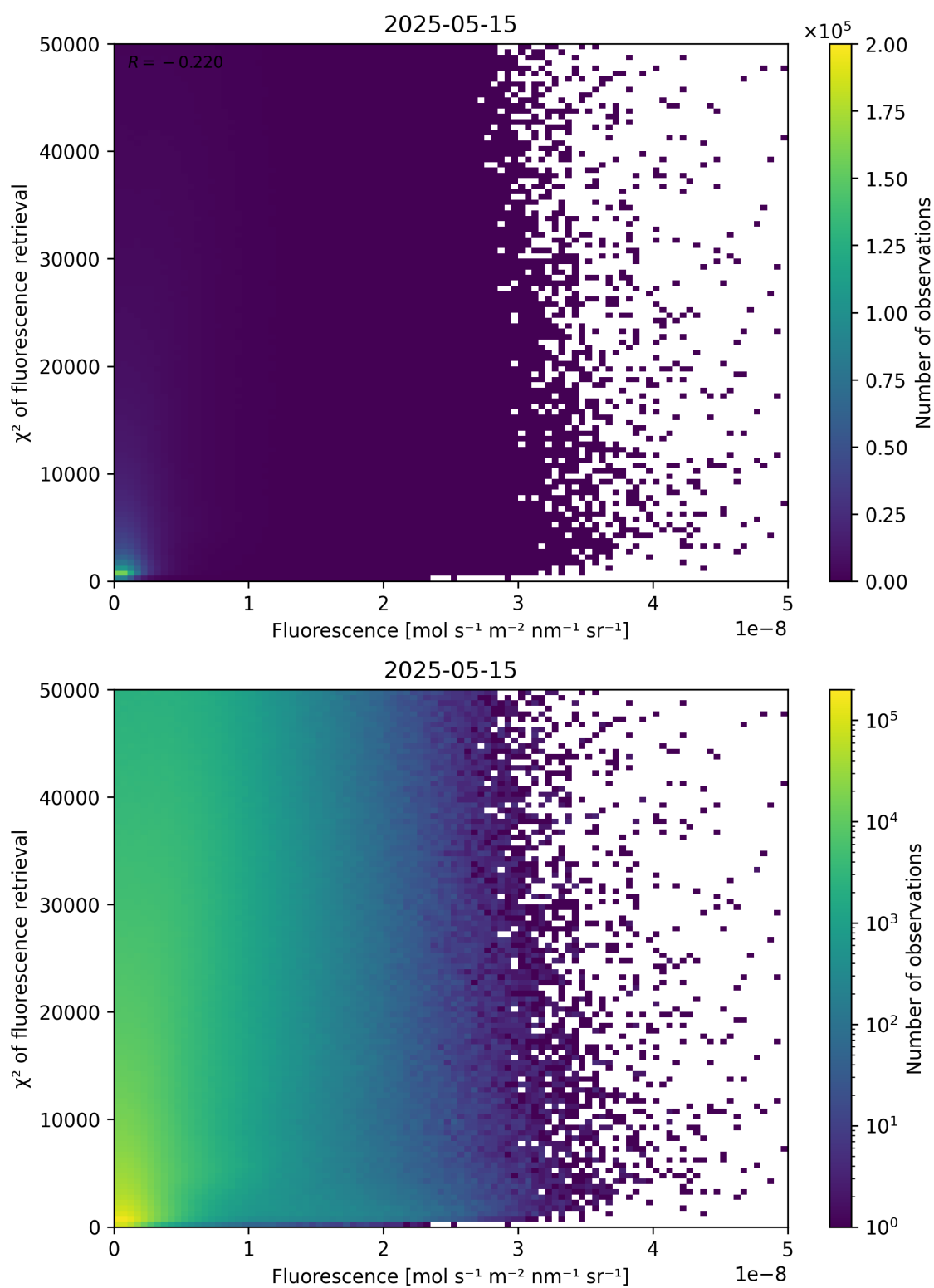
Figure 85: Scatter density plot of “Fluorescence” against “ \chi^2 of fluorescence retrieval” for 2025-05-15 to 2025-05-16.
