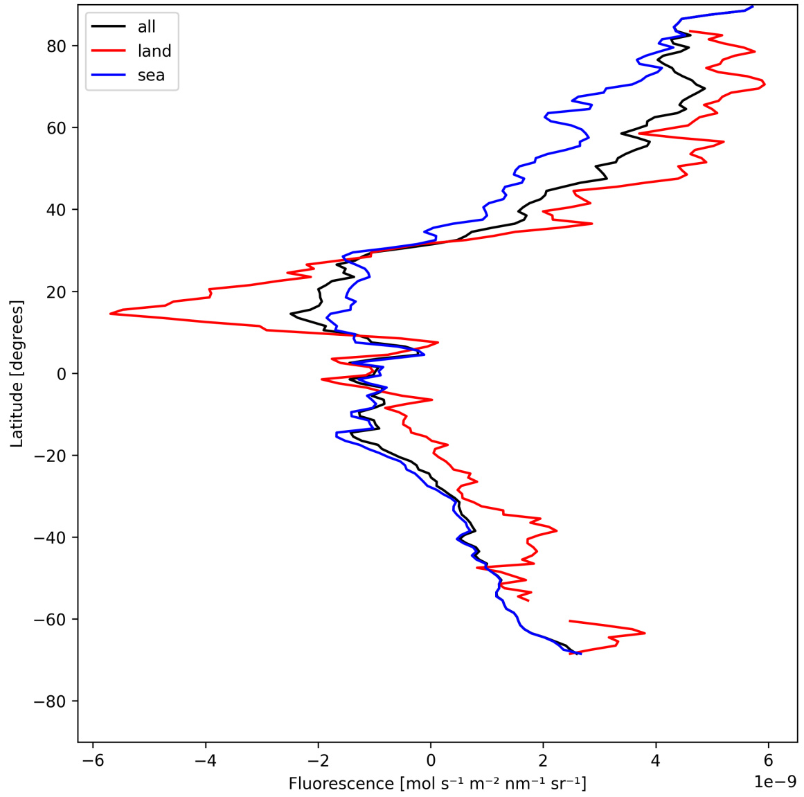
Figure 23: Zonal average of “Fluorescence” for 2025-05-15 to 2025-05-16.
