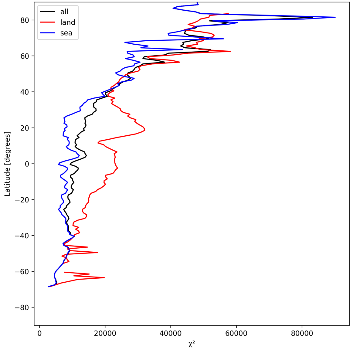
Figure 21: Zonal average of “ \chi^2 ” for 2025-05-15 to 2025-05-16.
