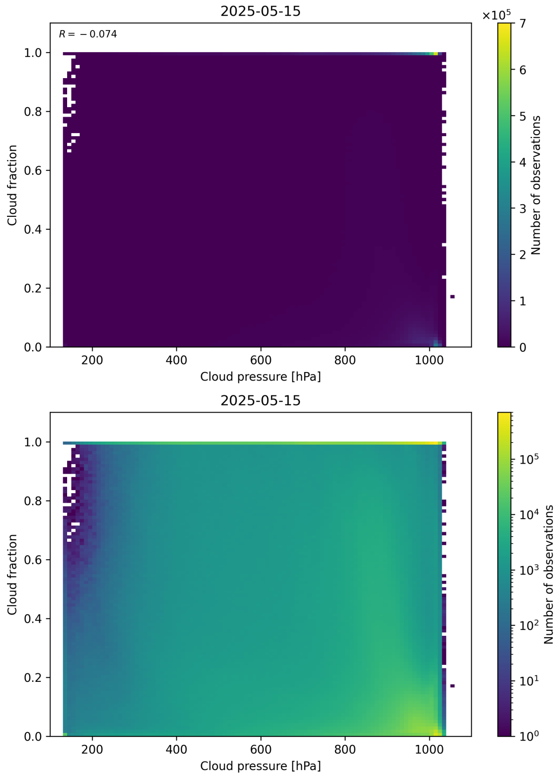
Figure 79: Scatter density plot of “Cloud pressure” against “Cloud fraction” for 2025-05-15 to 2025-05-16.
