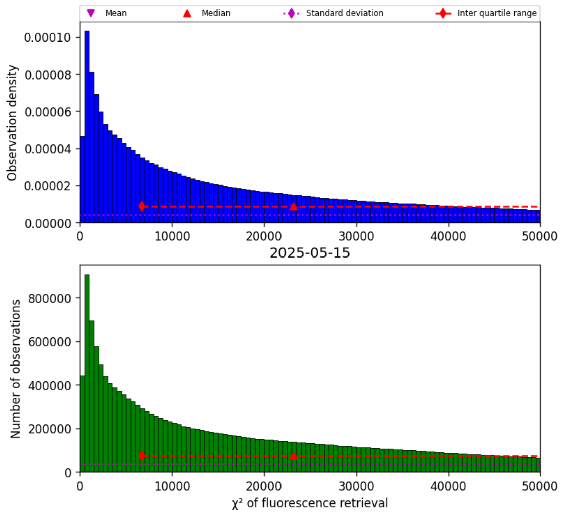
Figure 42: Histogram of “ \chi^2 of fluorescence retrieval” for 2025-05-15 to 2025-05-16
