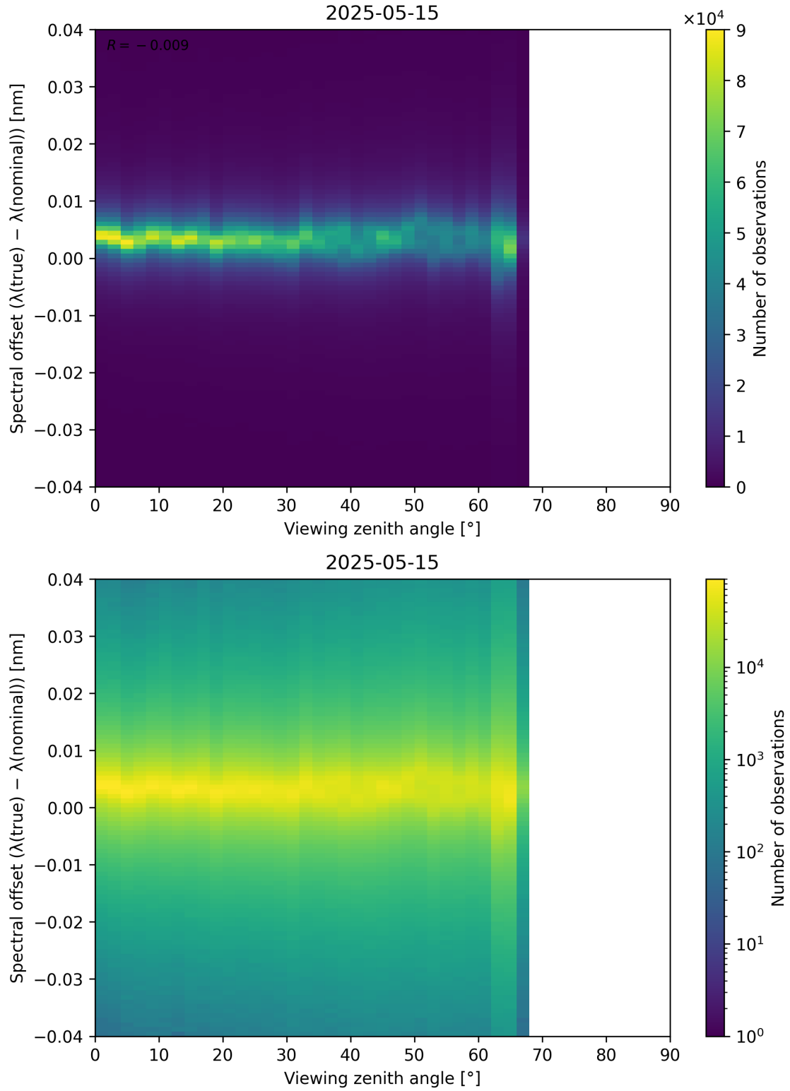
Figure 128: Scatter density plot of “Viewing zenith angle” against “Spectral offset ( \lambda_{\text{true}} - \lambda_{\text{nominal}} )” for 2025-05-15 to 2025-05-16.
