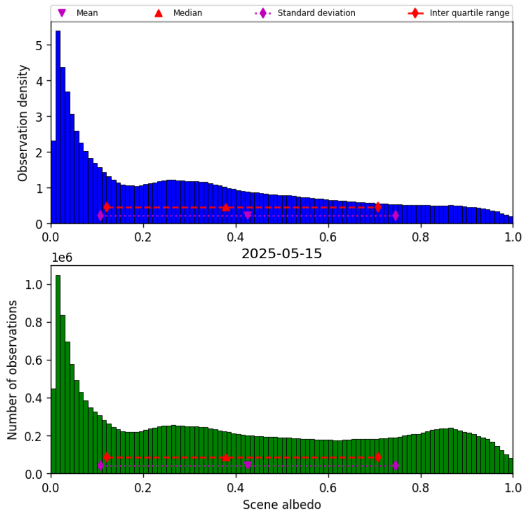
Figure 34: Histogram of “Scene albedo” for 2025-05-15 to 2025-05-16
