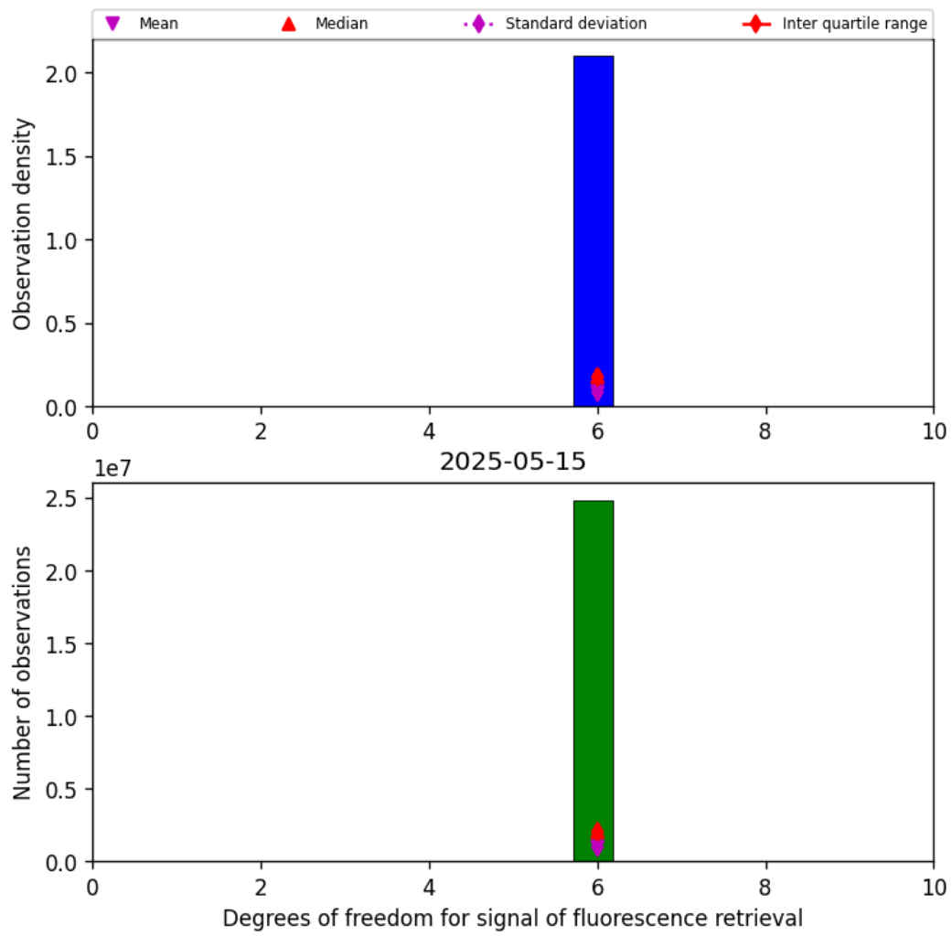
Figure 43: Histogram of “Degrees of freedom for signal of fluorescence retrieval” for 2025-05-15 to 2025-05-16
