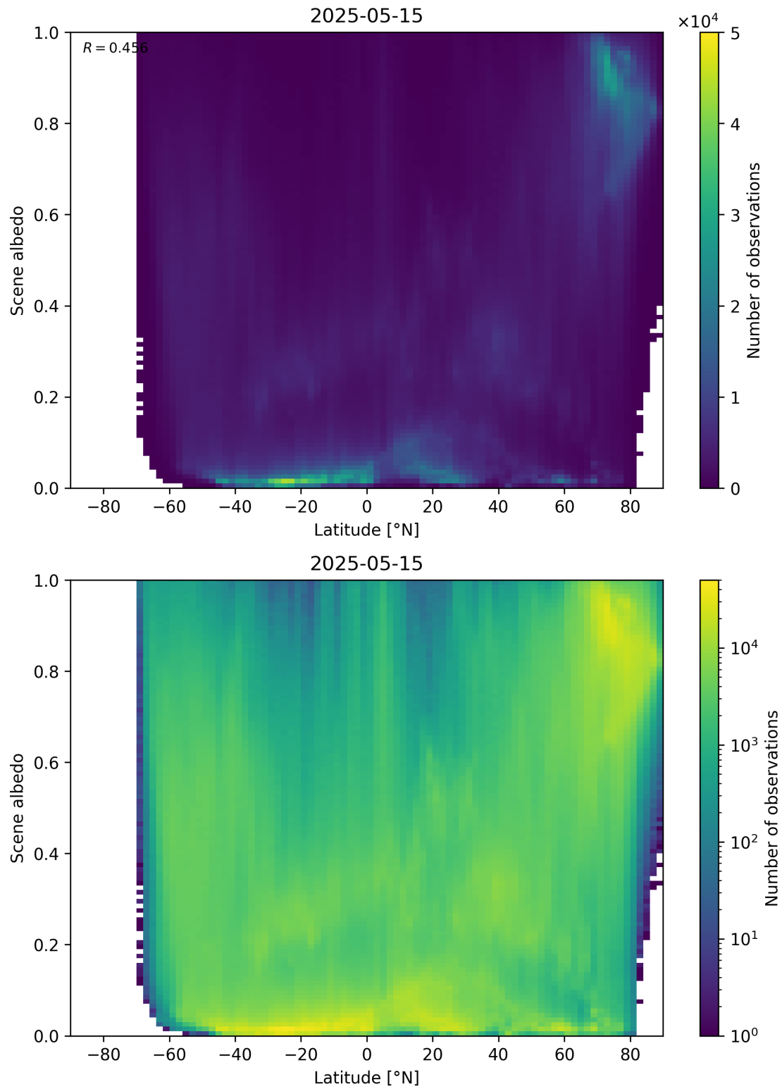
Figure 95: Scatter density plot of “Latitude” against “Scene albedo” for 2025-05-15 to 2025-05-16.
