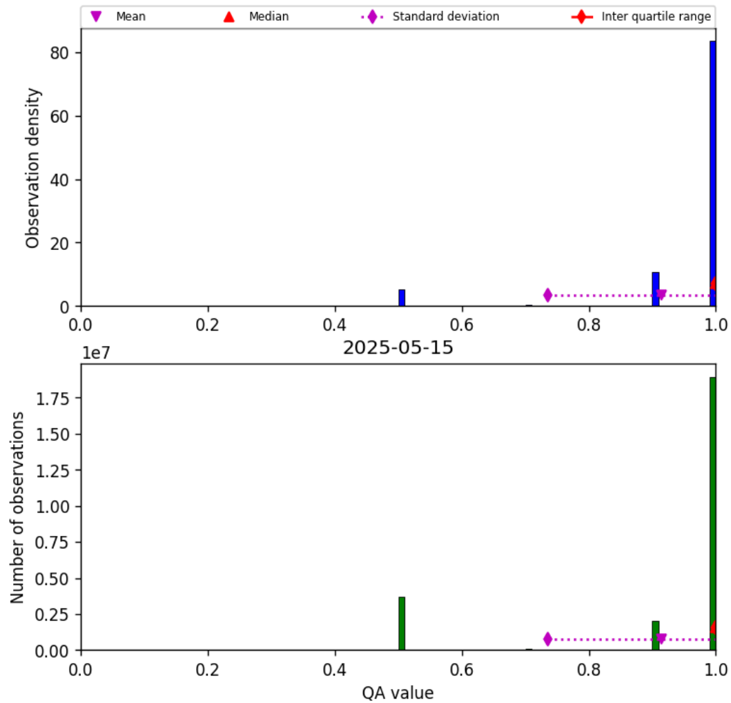
Figure 29: Histogram of “QA value” for 2025-05-15 to 2025-05-16
