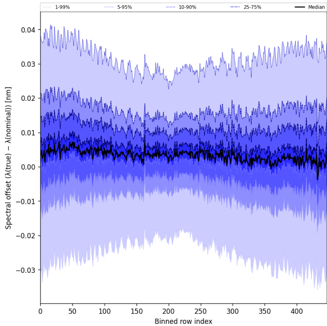
Figure 62: Along track statistics of “Spectral offset ( \lambda_{\text{true}} - \lambda_{\text{nominal}} )” for 2025-05-15 to 2025-05-16
