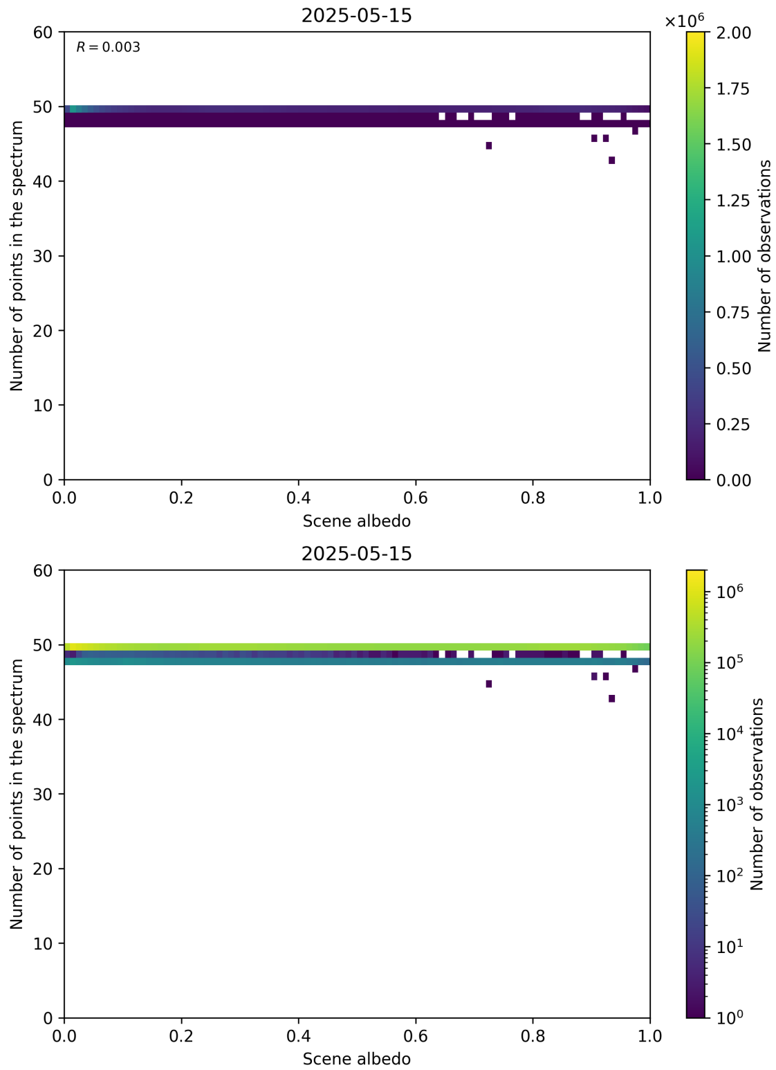
Figure 106: Scatter density plot of “Scene albedo” against “Number of points in the spectrum” for 2025-05-15 to 2025-05-16.
