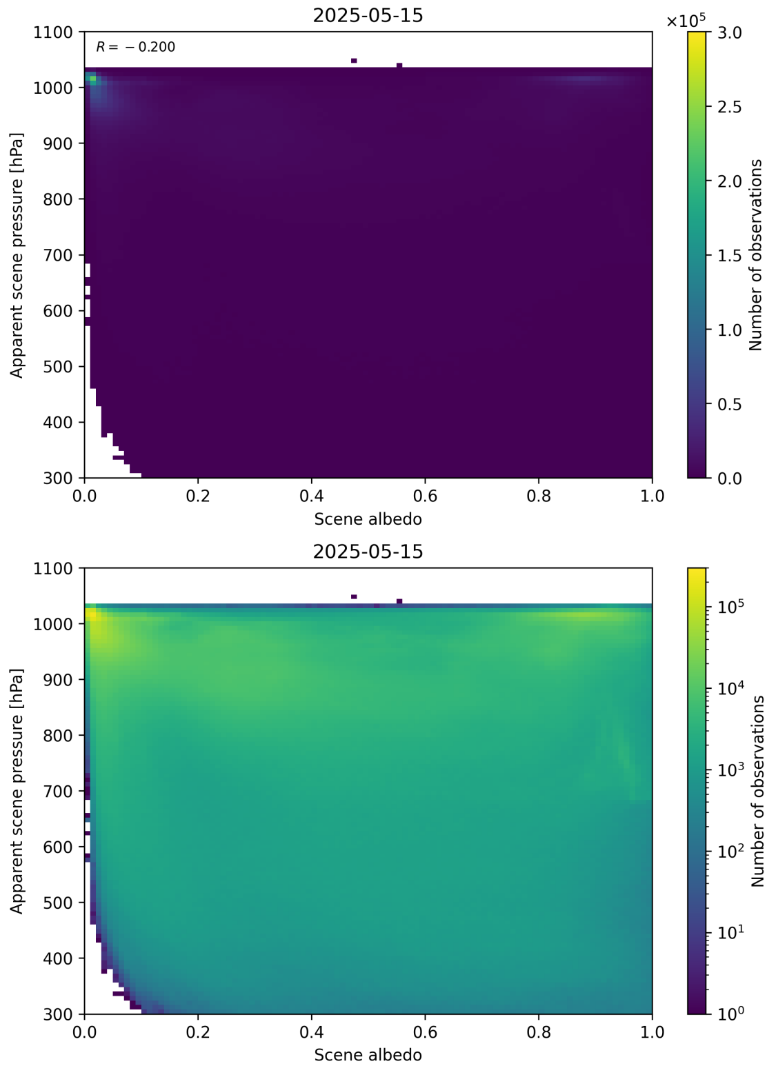
Figure 102: Scatter density plot of “Scene albedo” against “Apparent scene pressure” for 2025-05-15 to 2025-05-16.
