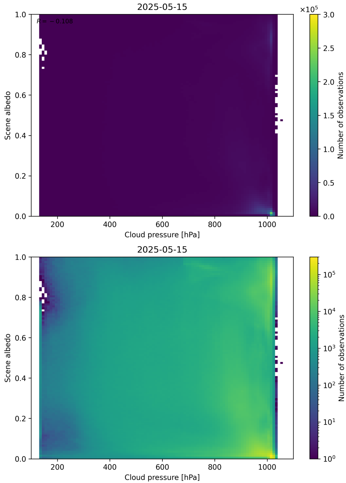
Figure 83: Scatter density plot of “Cloud pressure” against “Scene albedo” for 2025-05-15 to 2025-05-16.
