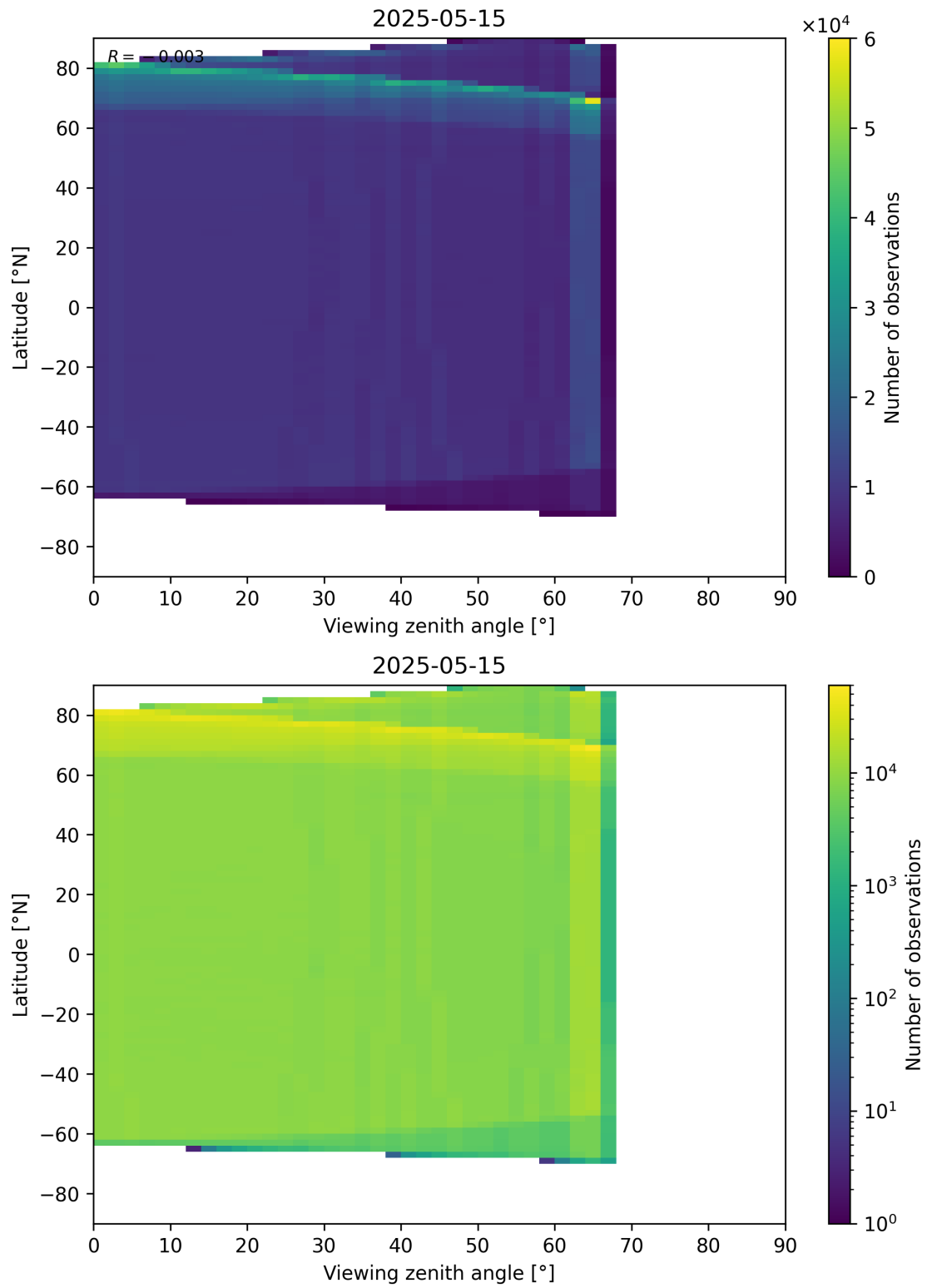
Figure 123: Scatter density plot of “Viewing zenith angle” against “Latitude” for 2025-05-15 to 2025-05-16.
