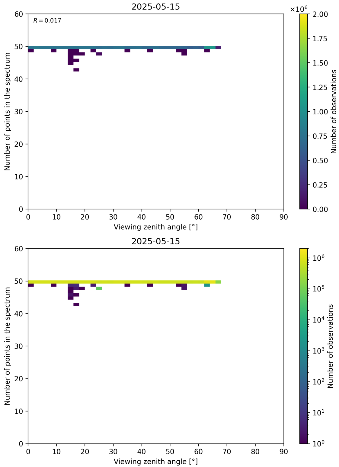
Figure 125: Scatter density plot of “Viewing zenith angle” against “Number of points in the spectrum” for 2025-05-15 to 2025-05-16.
