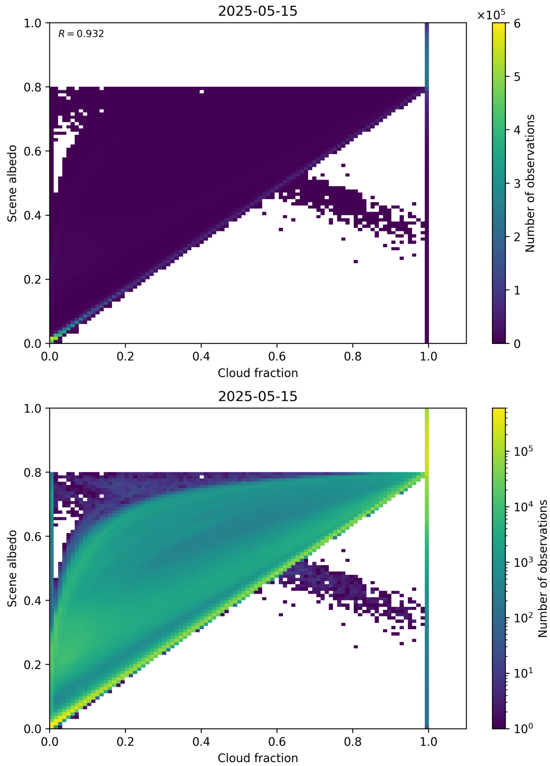
Figure 75: Scatter density plot of “Cloud fraction” against “Scene albedo” for 2025-05-15 to 2025-05-16.
