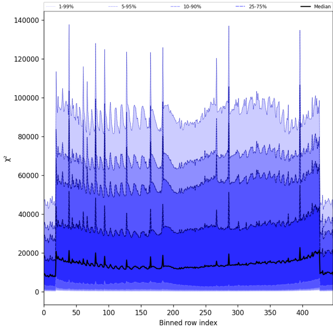
Figure 55: Along track statistics of “ \chi^2 ” for 2025-05-15 to 2025-05-16
