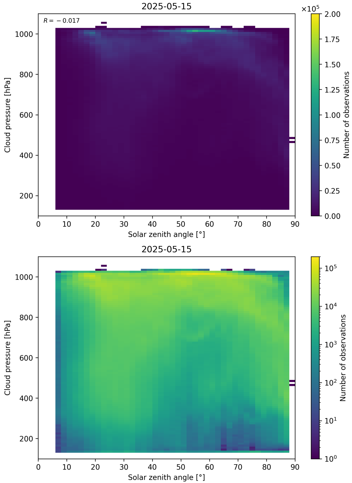
Figure 111: Scatter density plot of “Solar zenith angle” against “Cloud pressure” for 2025-05-15 to 2025-05-16.
