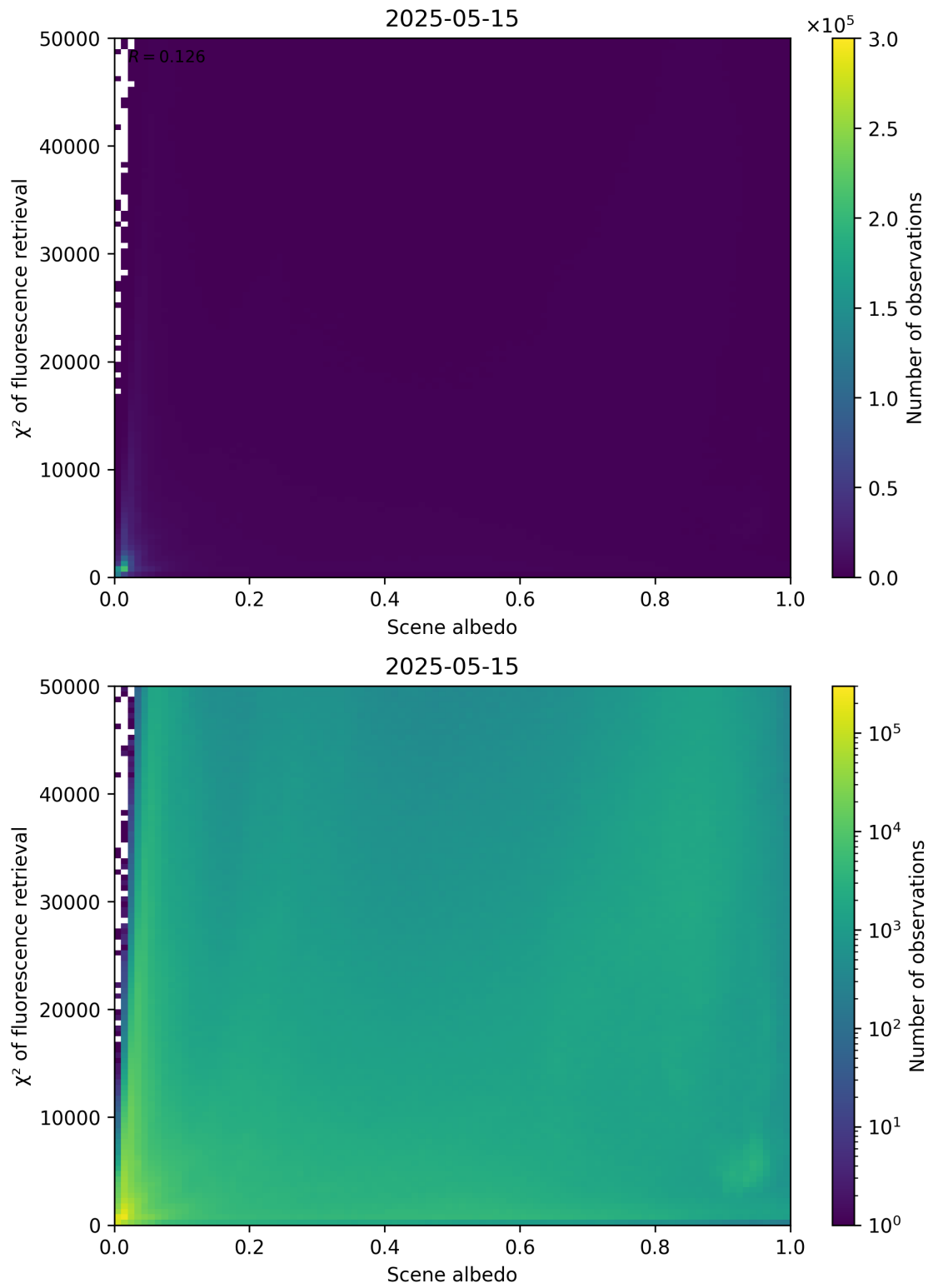
Figure 103: Scatter density plot of “Scene albedo” against “ \chi^2 of fluorescence retrieval” for 2025-05-15 to 2025-05-16.
