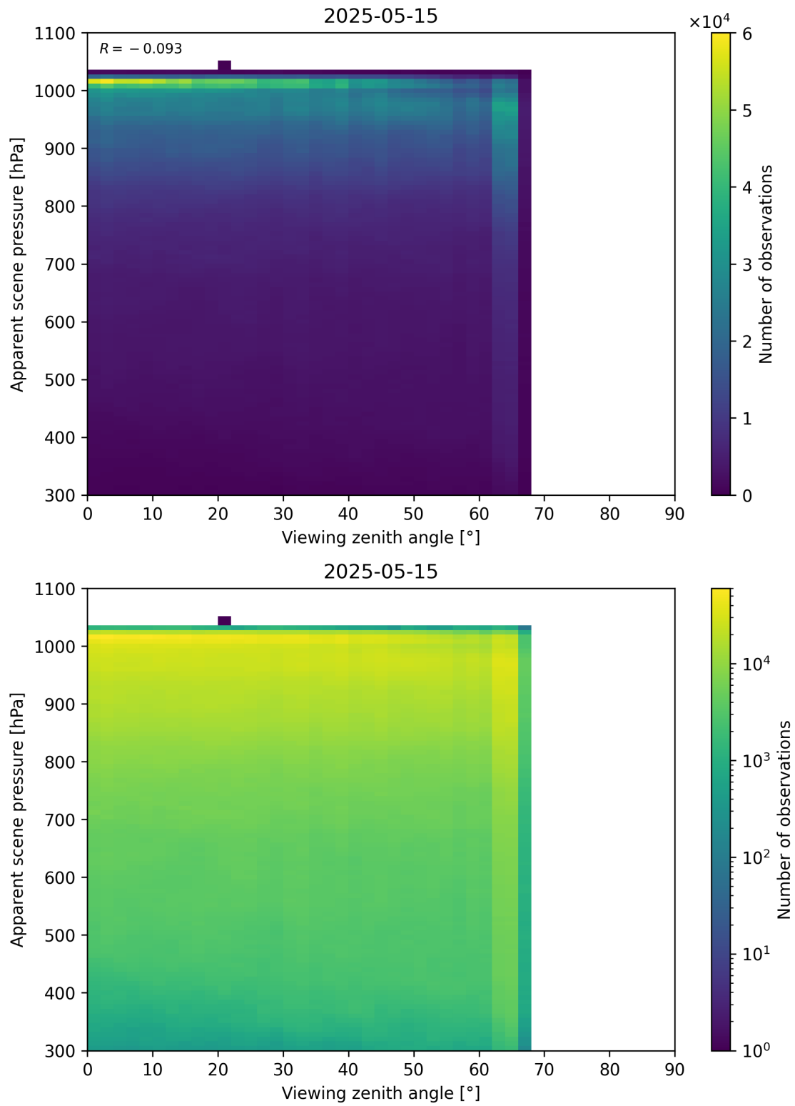
Figure 118: Scatter density plot of “Viewing zenith angle” against “Apparent scene pressure” for 2025-05-15 to 2025-05-16.
