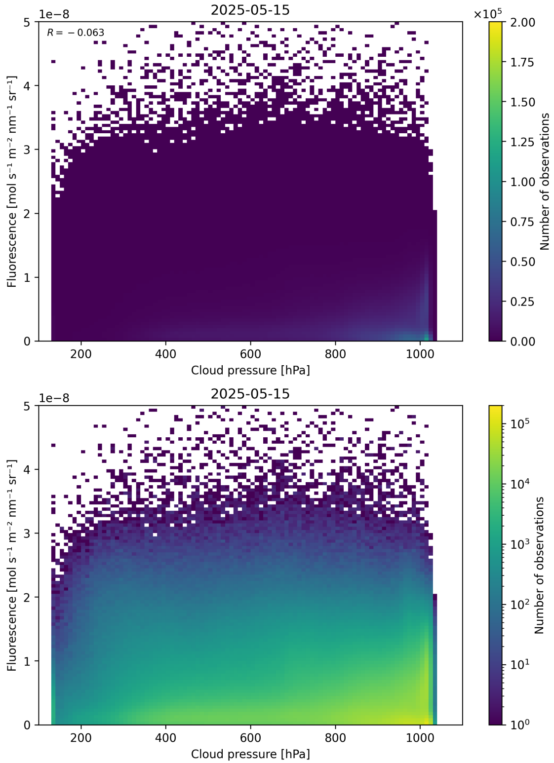
Figure 80: Scatter density plot of “Cloud pressure” against “Fluorescence” for 2025-05-15 to 2025-05-16.
