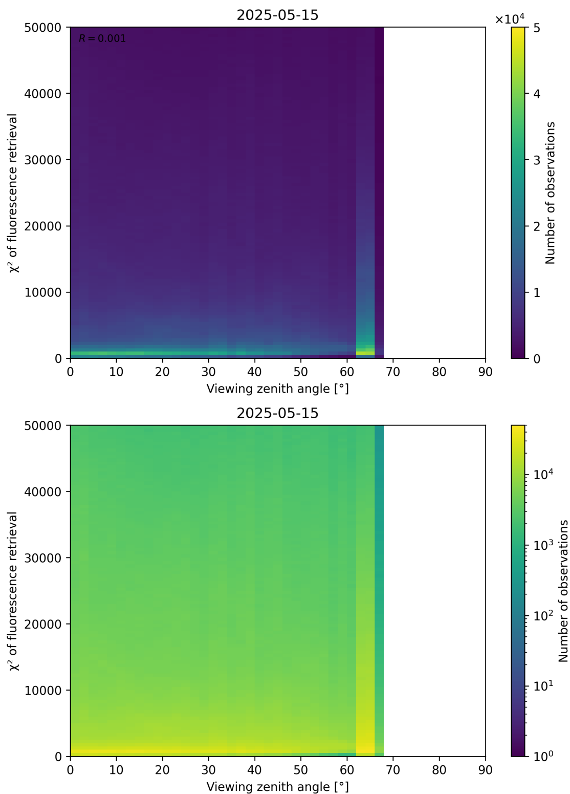
Figure 119: Scatter density plot of “Viewing zenith angle” against “ \chi^2 of fluorescence retrieval” for 2025-05-15 to 2025-05-16.
