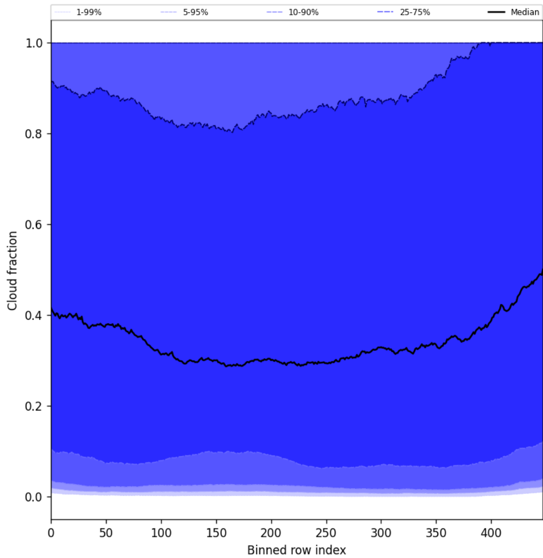
Figure 49: Along track statistics of “Cloud fraction” for 2025-05-15 to 2025-05-16
