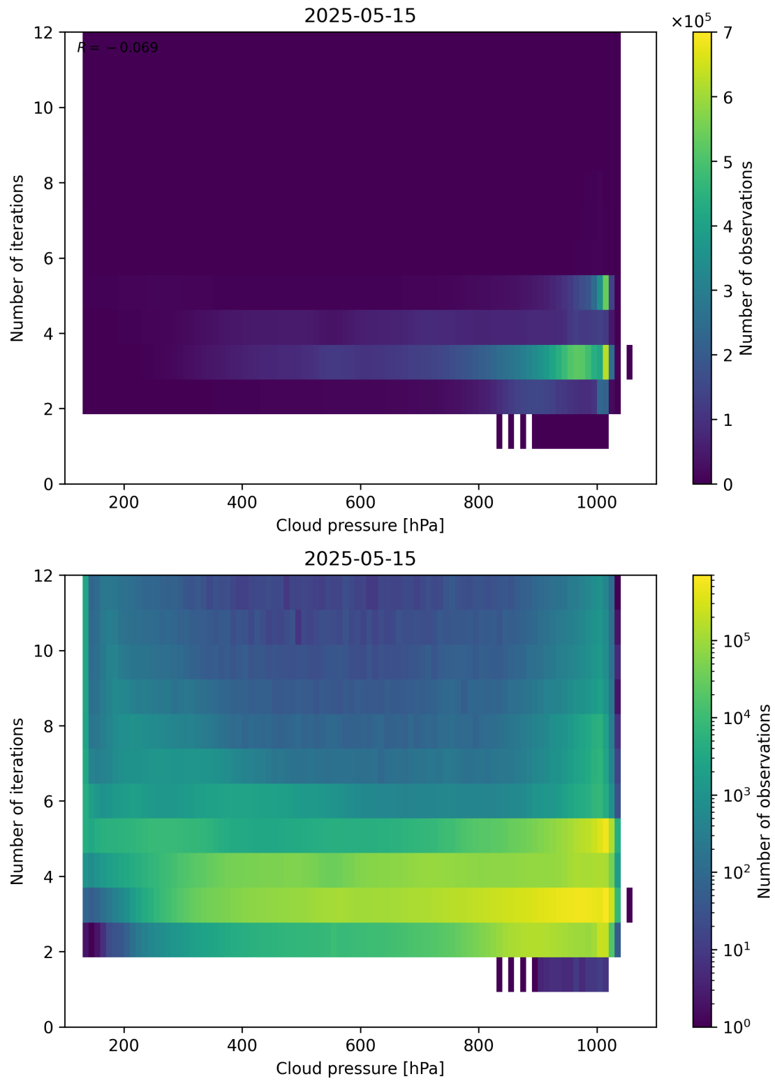
Figure 81: Scatter density plot of “Cloud pressure” against “Number of iterations” for 2025-05-15 to 2025-05-16.
