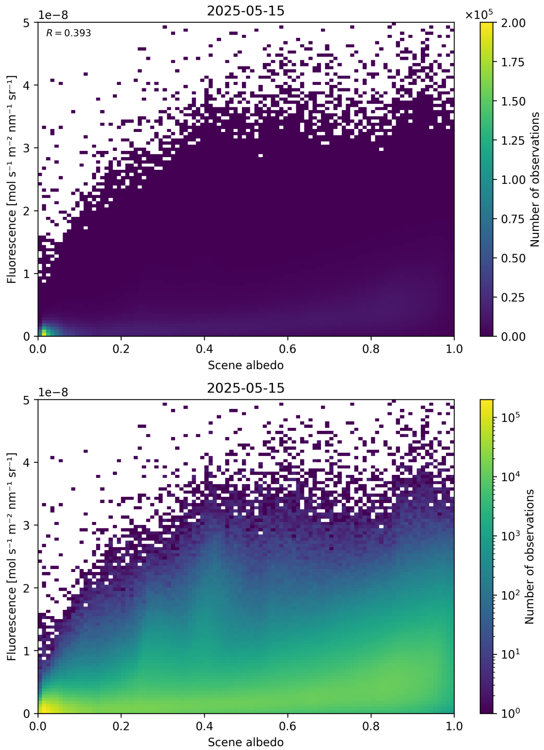
Figure 104: Scatter density plot of “Scene albedo” against “Fluorescence” for 2025-05-15 to 2025-05-16.
