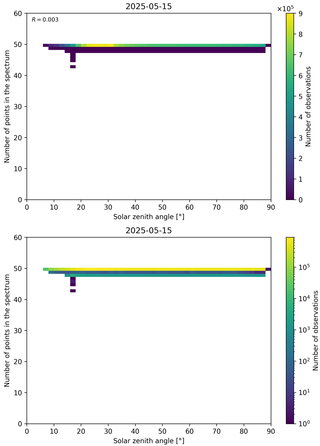
Figure 115: Scatter density plot of “Solar zenith angle” against “Number of points in the spectrum” for 2025-05-15 to 2025-05-16.
