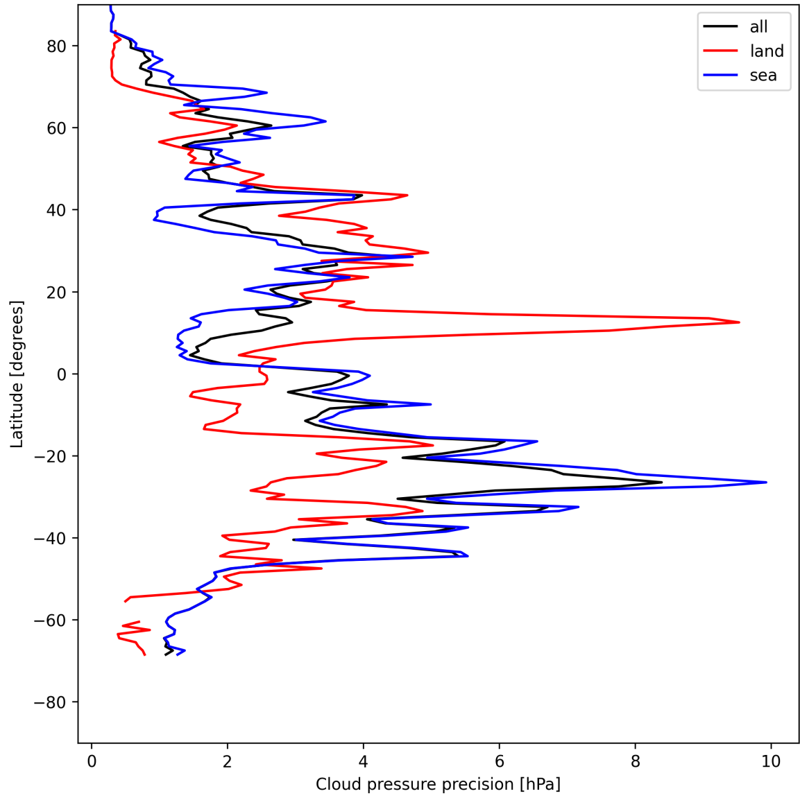
Figure 14: Zonal average of “Cloud pressure precision” for 2025-05-15 to 2025-05-16.
