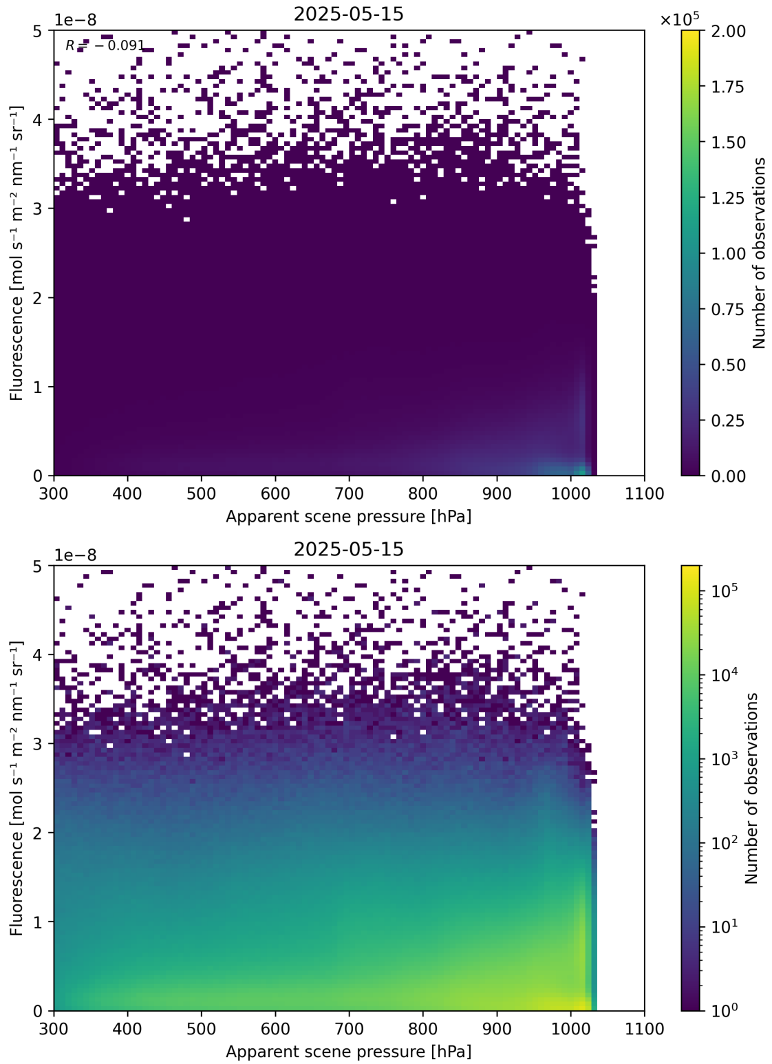
Figure 64: Scatter density plot of “Apparent scene pressure” against “Fluorescence” for 2025-05-15 to 2025-05-16.
