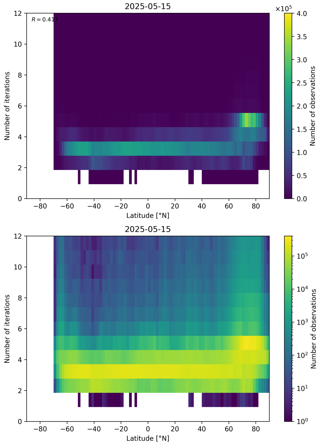
Figure 93: Scatter density plot of “Latitude” against “Number of iterations” for 2025-05-15 to 2025-05-16.
