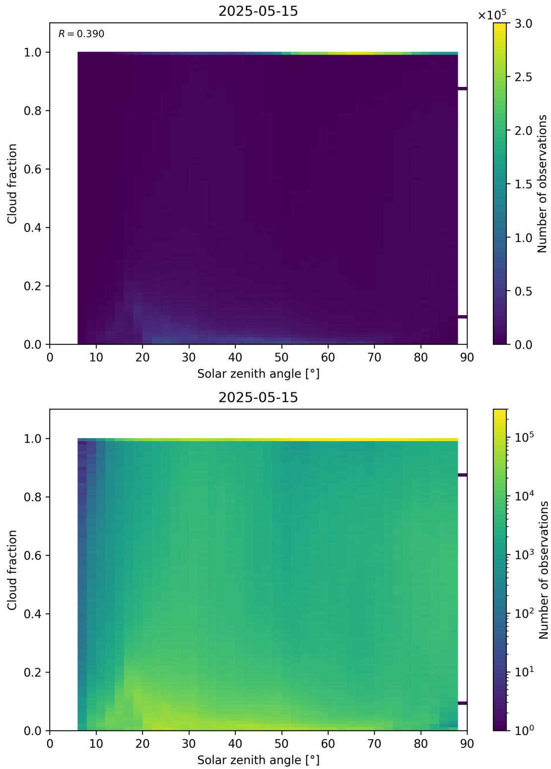
Figure 110: Scatter density plot of “Solar zenith angle” against “Cloud fraction” for 2025-05-15 to 2025-05-16.
