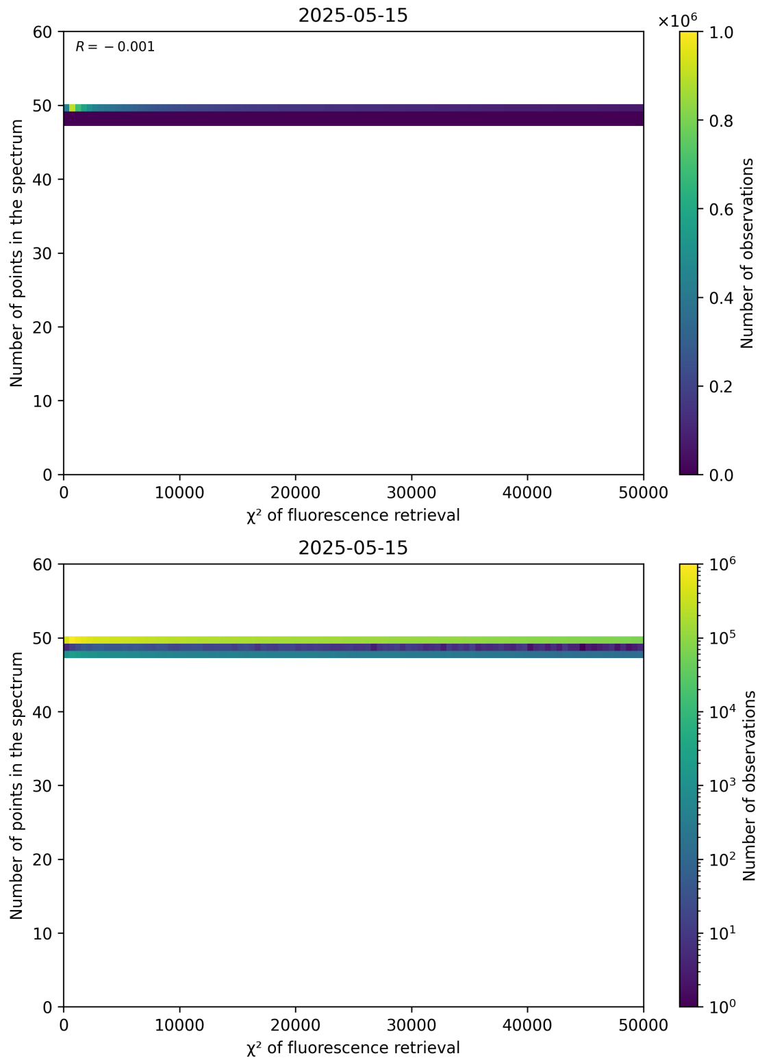
Figure 68: Scatter density plot of " \chi^2 of fluorescence retrieval" against "Number of points in the spectrum" for 2025-05-15 to 2025-05-16.
