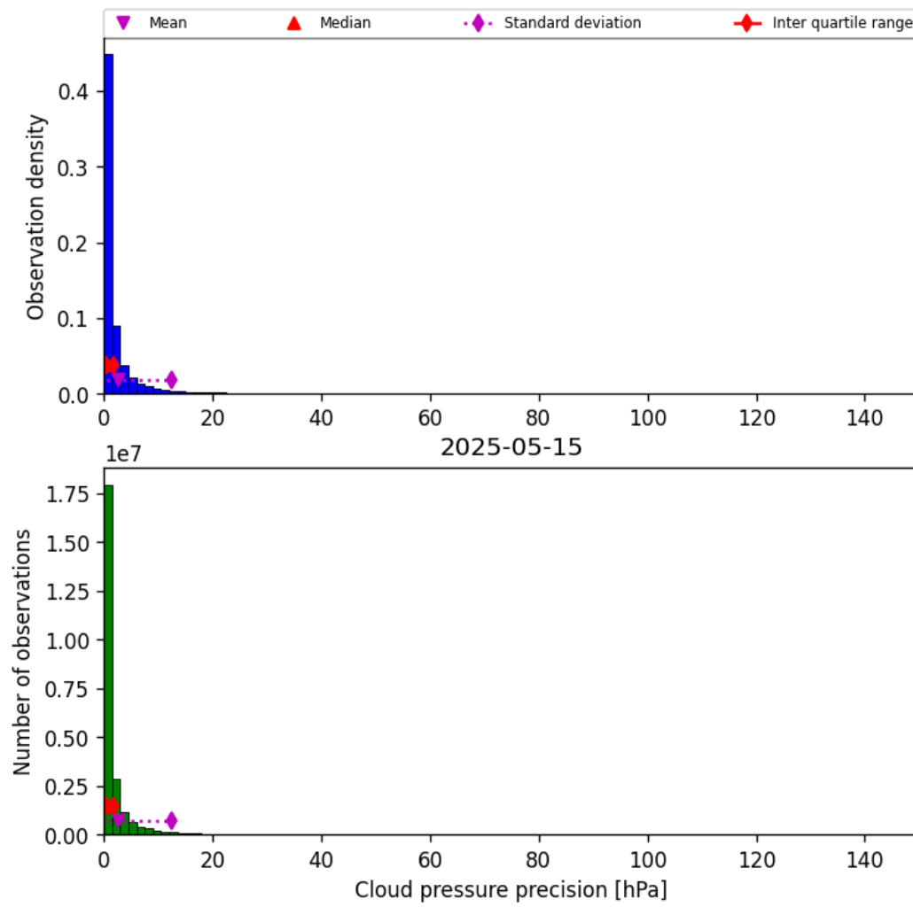
Figure 31: Histogram of “Cloud pressure precision” for 2025-05-15 to 2025-05-16
