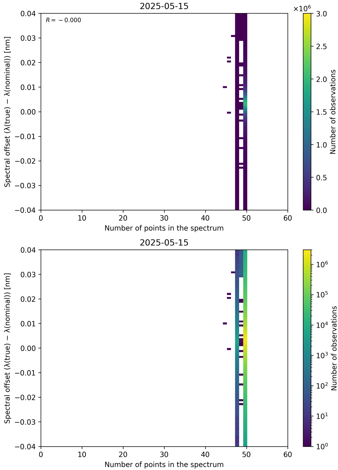
Figure 101: Scatter density plot of “Number of points in the spectrum” against “Spectral offset ( \lambda_{\text{true}} - \lambda_{\text{nominal}} )” for 2025-05-15 to 2025-05-16.
