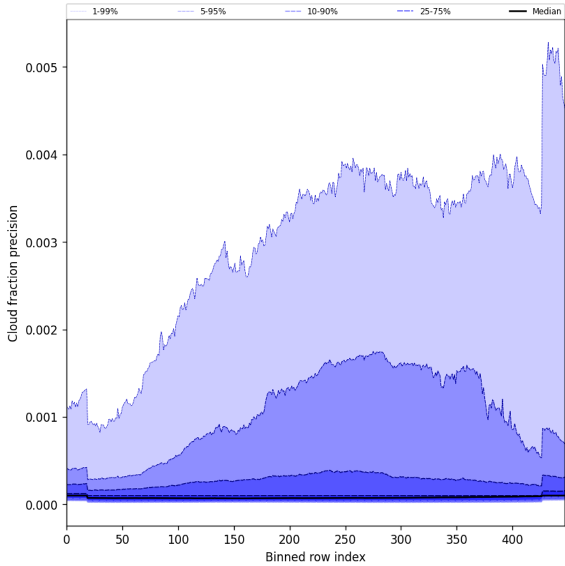
Figure 50: Along track statistics of “Cloud fraction precision” for 2025-05-15 to 2025-05-16
