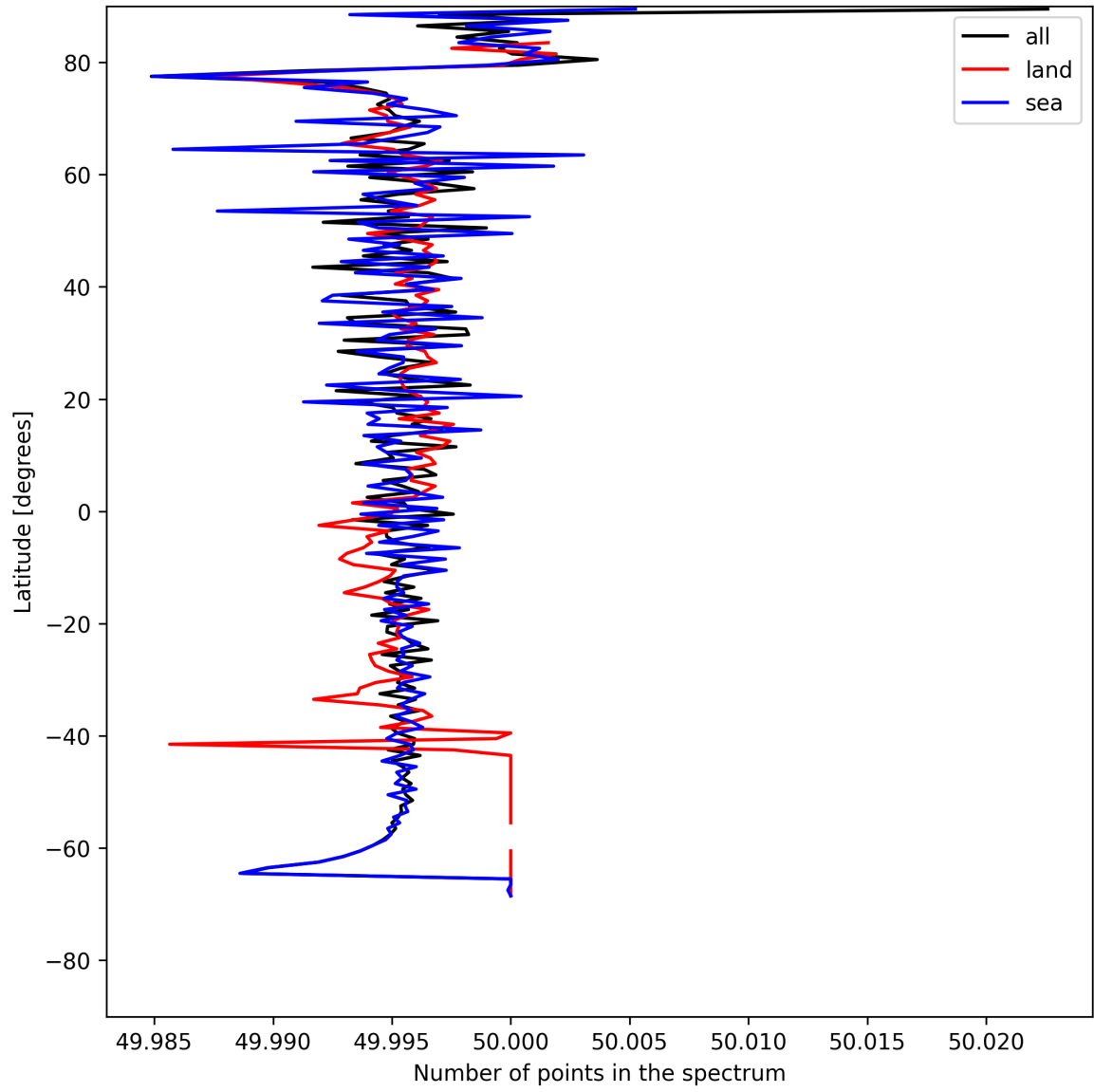
Figure 27: Zonal average of “Number of points in the spectrum” for 2025-05-15 to 2025-05-16.
