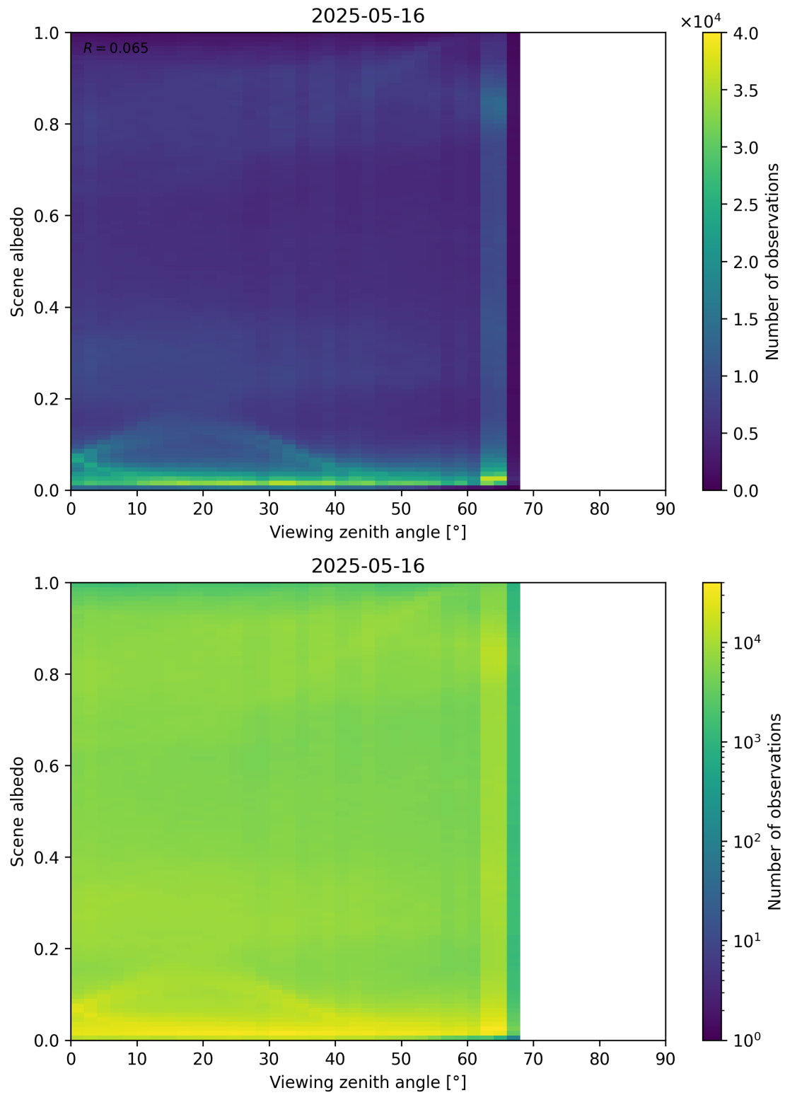
Figure 126: Scatter density plot of “Viewing zenith angle” against “Scene albedo” for 2025-05-15 to 2025-05-17.
