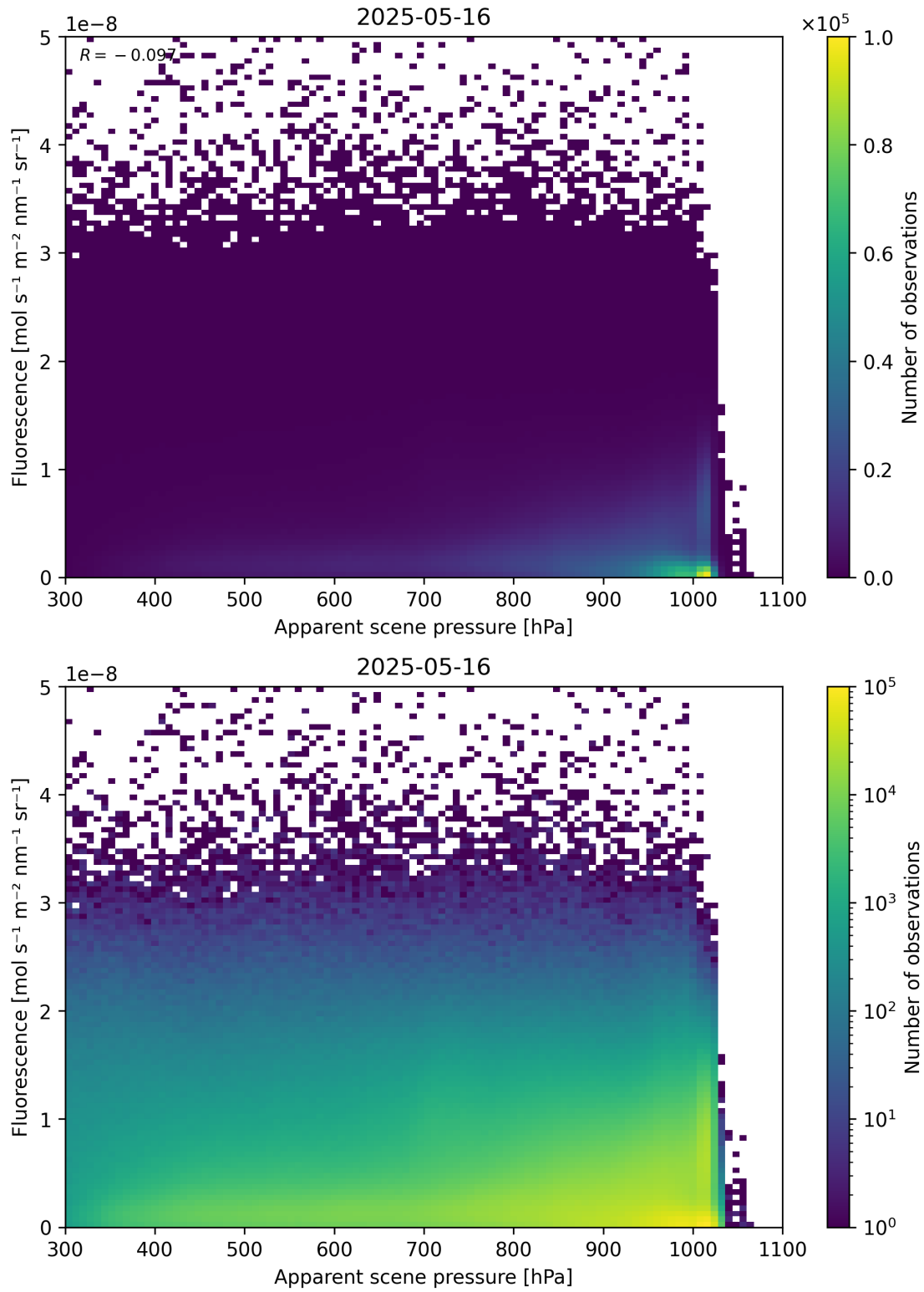
Figure 64: Scatter density plot of “Apparent scene pressure” against “Fluorescence” for 2025-05-15 to 2025-05-17.
