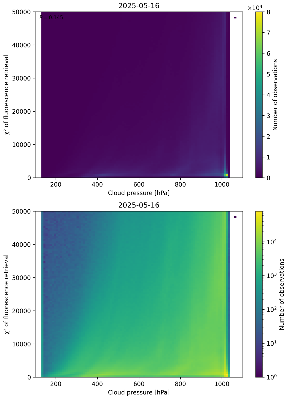
Figure 78: Scatter density plot of “Cloud pressure” against “ \chi^2 of fluorescence retrieval” for 2025-05-15 to 2025-05-17.
