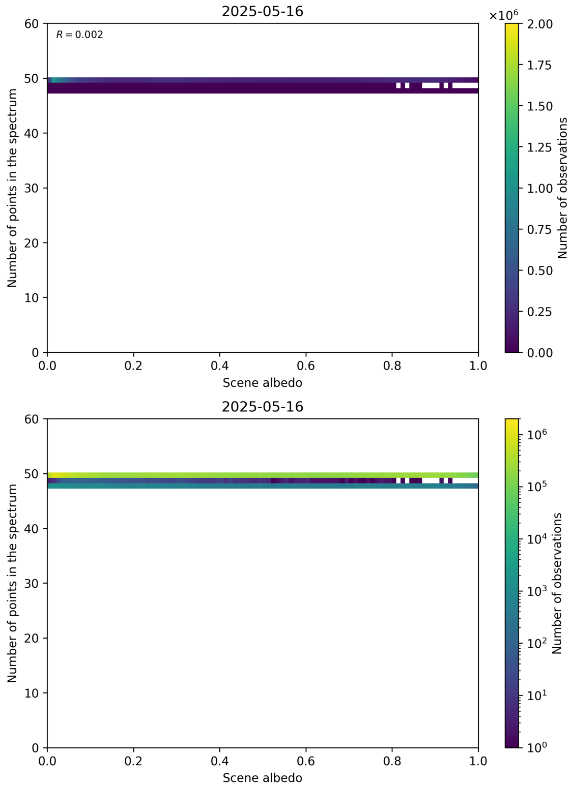
Figure 106: Scatter density plot of “Scene albedo” against “Number of points in the spectrum” for 2025-05-15 to 2025-05-17.
