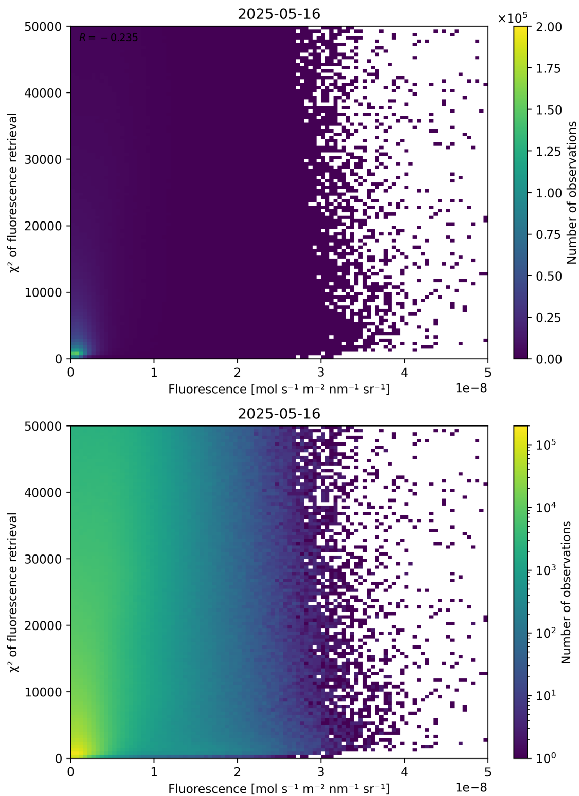
Figure 85: Scatter density plot of “Fluorescence” against “ \chi^2 of fluorescence retrieval” for 2025-05-15 to 2025-05-17.
