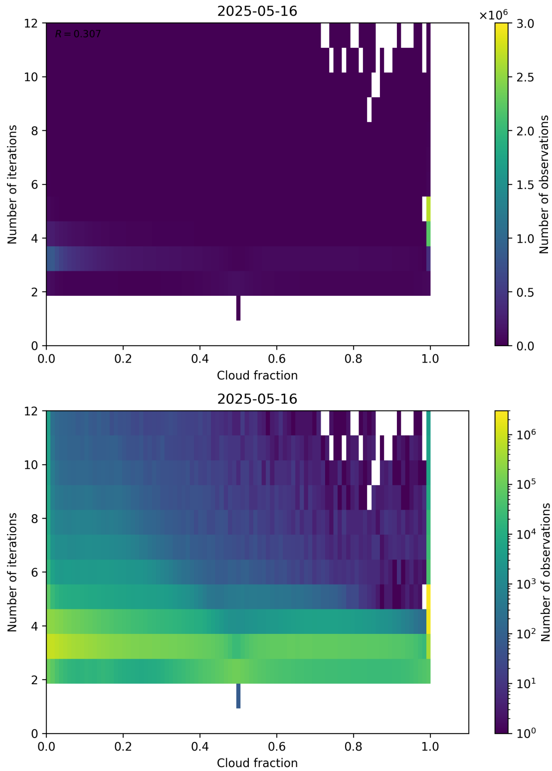
Figure 73: Scatter density plot of “Cloud fraction” against “Number of iterations” for 2025-05-15 to 2025-05-17.
