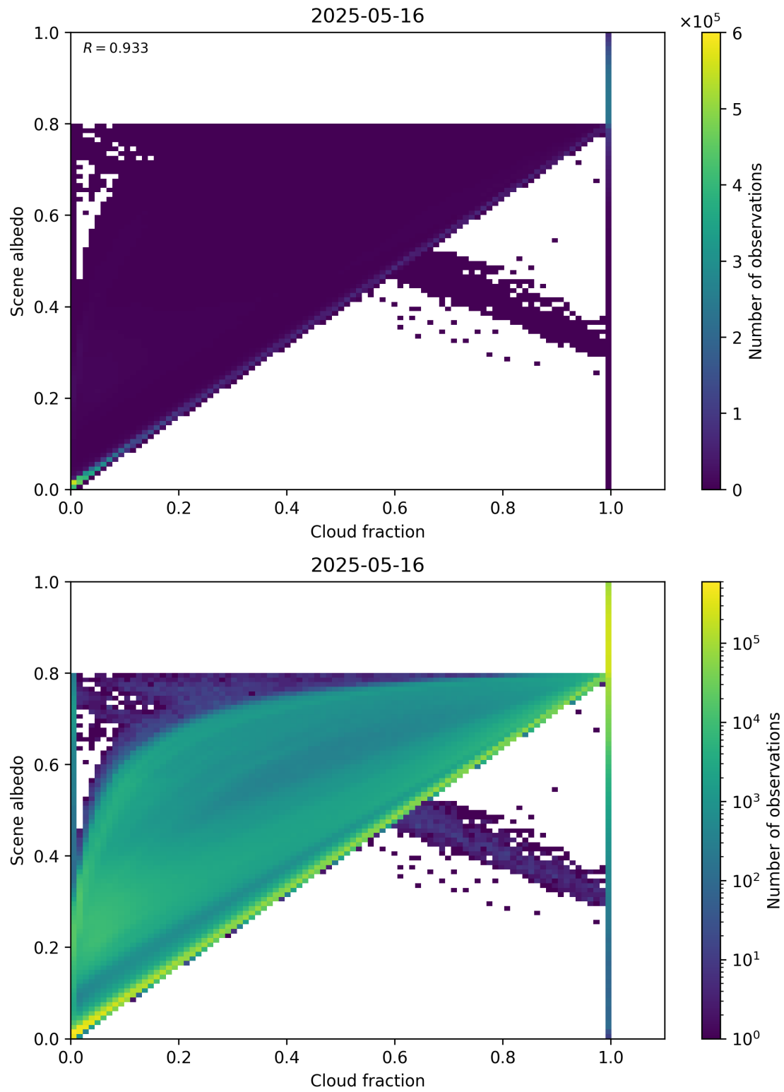
Figure 75: Scatter density plot of “Cloud fraction” against “Scene albedo” for 2025-05-15 to 2025-05-17.
