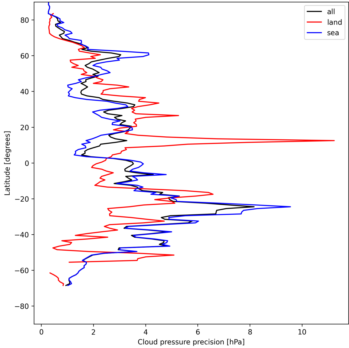
Figure 14: Zonal average of "Cloud pressure precision" for 2025-05-15 to 2025-05-17.
