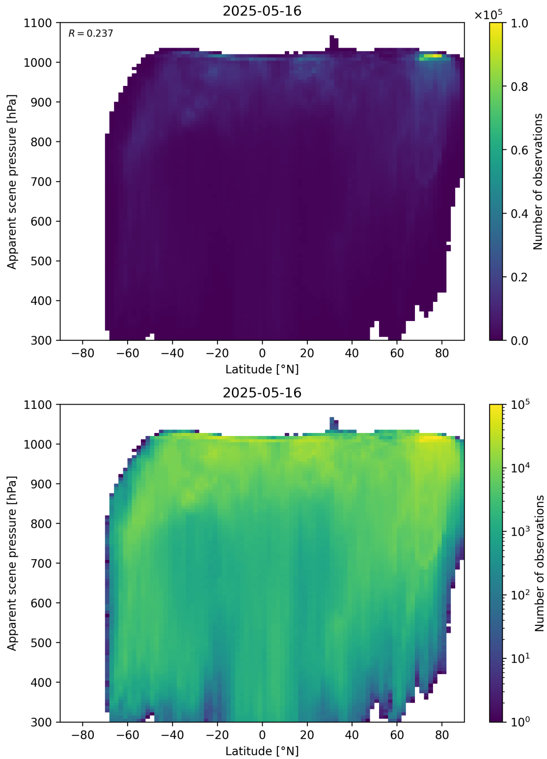
Figure 88: Scatter density plot of “Latitude” against “Apparent scene pressure” for 2025-05-15 to 2025-05-17.
