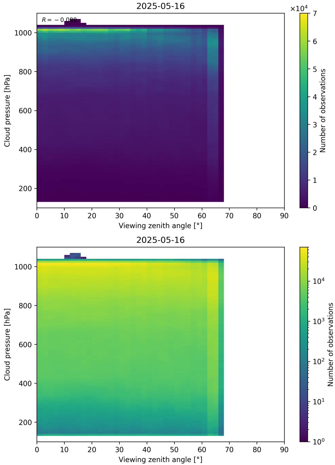
Figure 121: Scatter density plot of “Viewing zenith angle” against “Cloud pressure” for 2025-05-15 to 2025-05-17.
