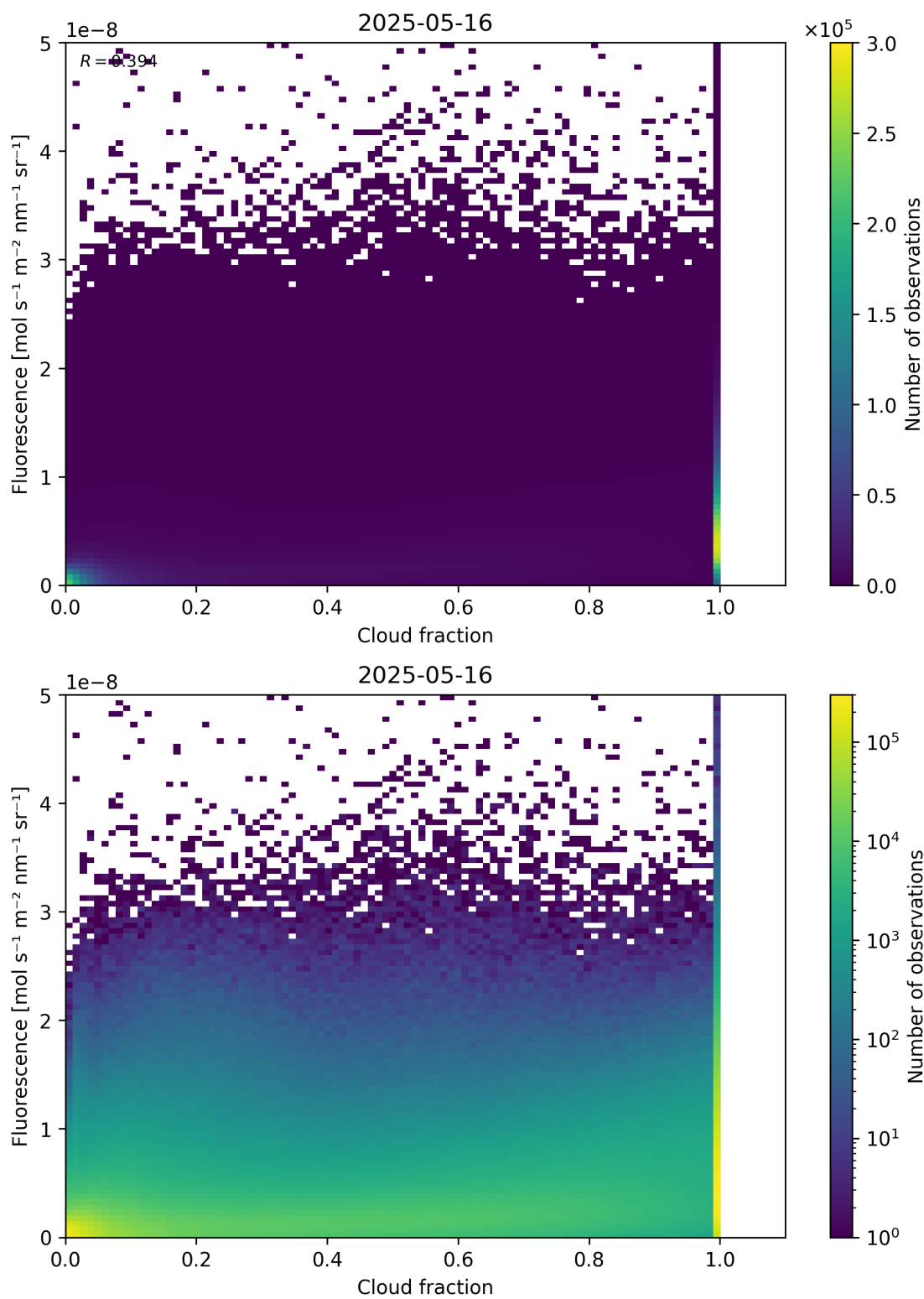
Figure 72: Scatter density plot of “Cloud fraction” against “Fluorescence” for 2025-05-15 to 2025-05-17.
