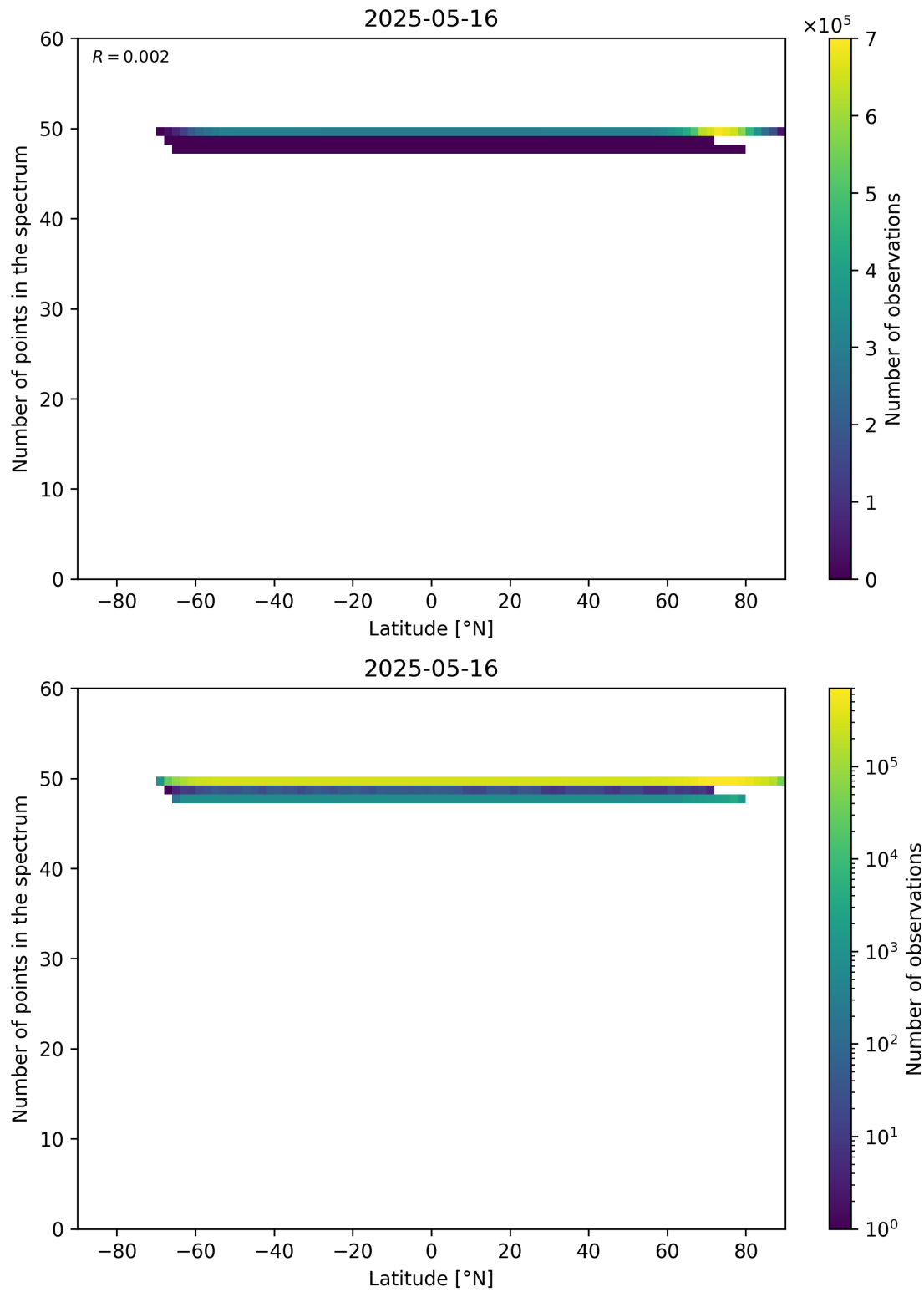
Figure 94: Scatter density plot of “Latitude” against “Number of points in the spectrum” for 2025-05-15 to 2025-05-17.
