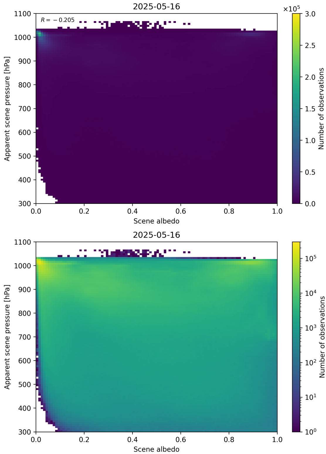
Figure 102: Scatter density plot of “Scene albedo” against “Apparent scene pressure” for 2025-05-15 to 2025-05-17.
