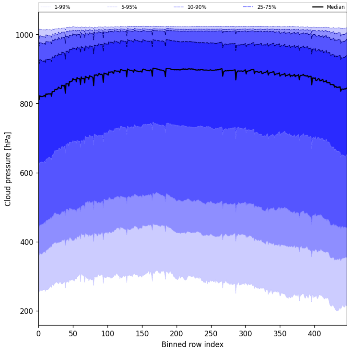
Figure 47: Along track statistics of “Cloud pressure” for 2025-05-15 to 2025-05-17
