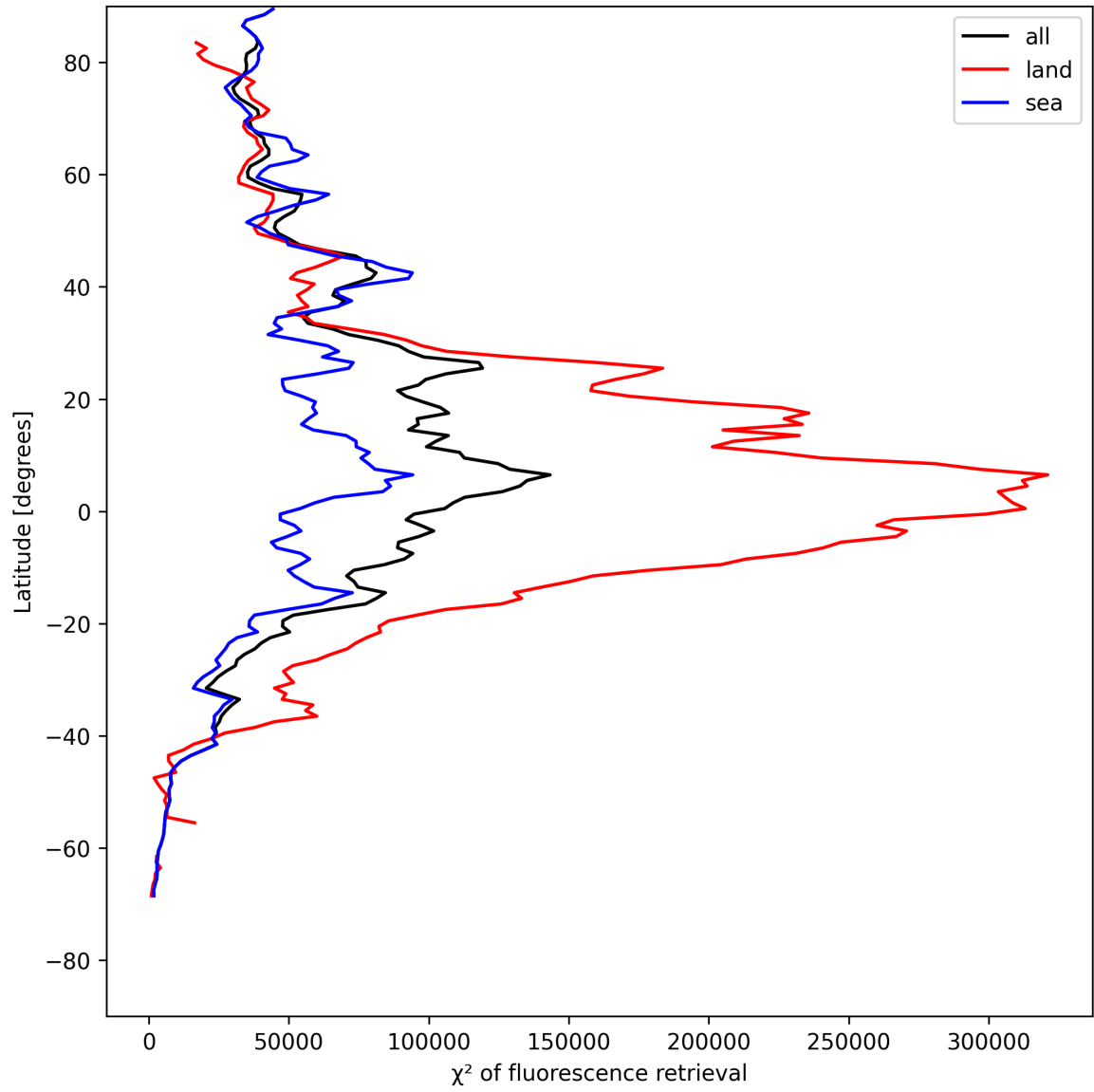
Figure 25: Zonal average of “ \chi^2 of fluorescence retrieval” for 2025-05-15 to 2025-05-17.
