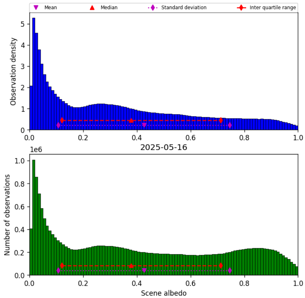
Figure 34: Histogram of “Scene albedo” for 2025-05-15 to 2025-05-17
