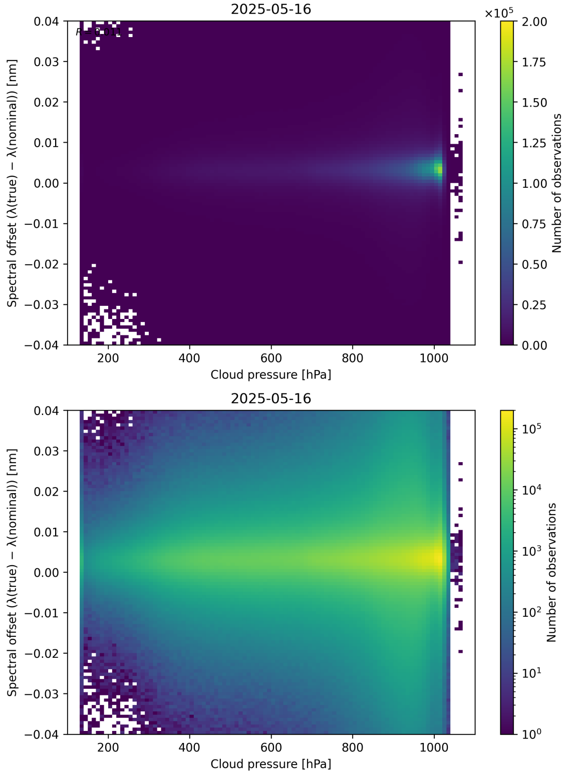
Figure 84: Scatter density plot of “Cloud pressure” against “Spectral offset ( \lambda_{\text{true}} - \lambda_{\text{nominal}} )” for 2025-05-15 to 2025-05-17.
