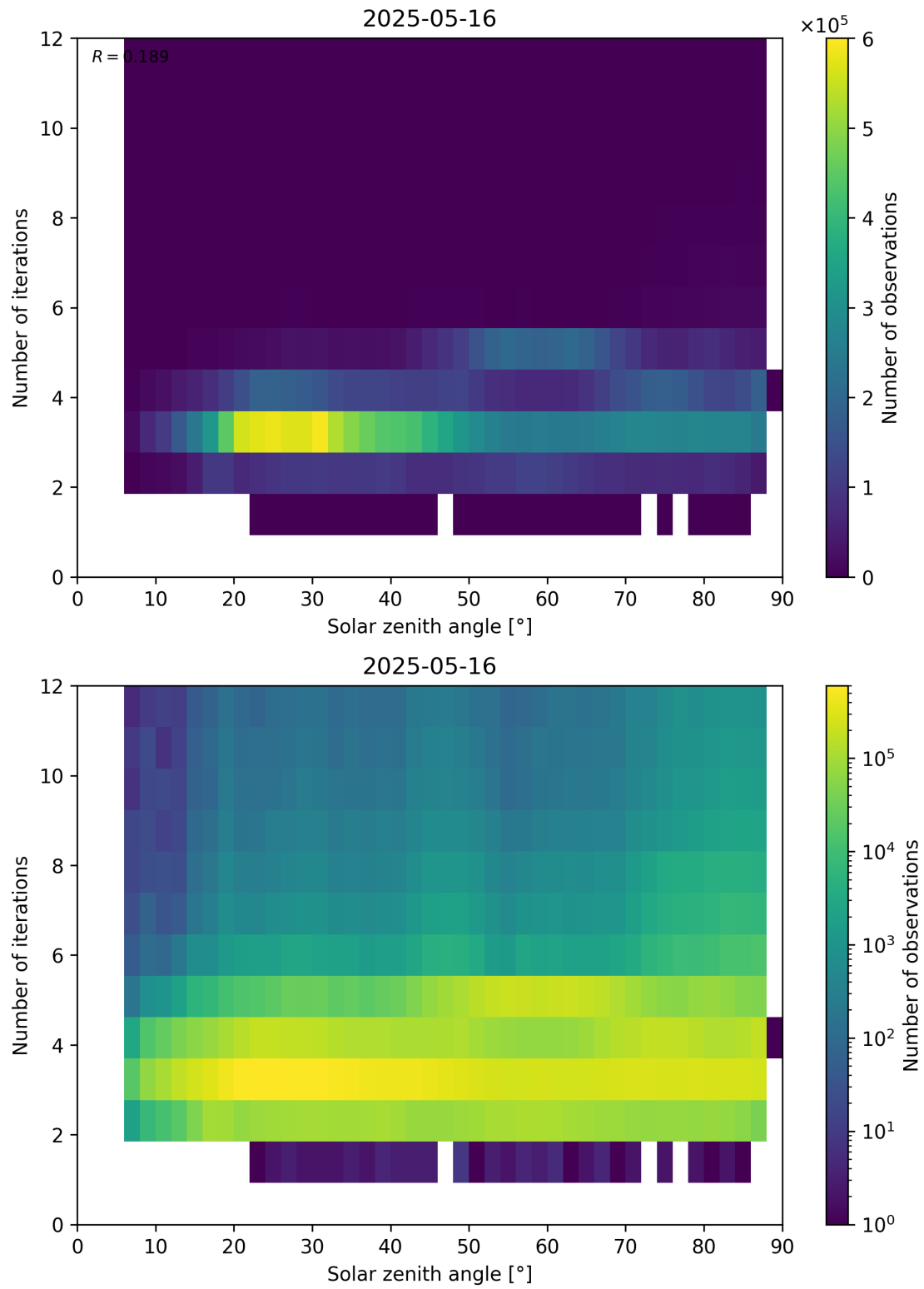
Figure 114: Scatter density plot of “Solar zenith angle” against “Number of iterations” for 2025-05-15 to 2025-05-17.
