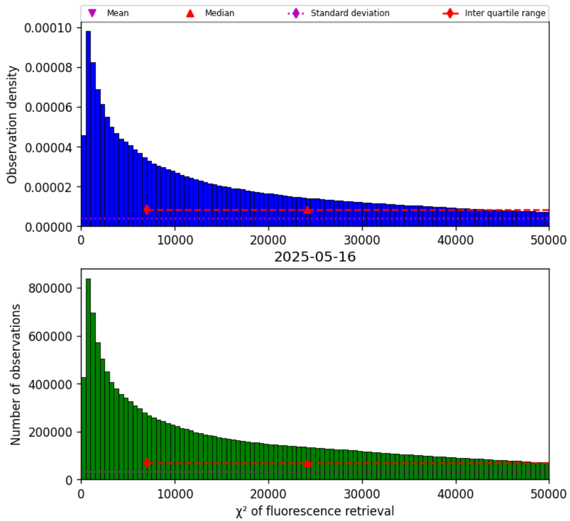
Figure 42: Histogram of “ \chi^2 of fluorescence retrieval” for 2025-05-15 to 2025-05-17
