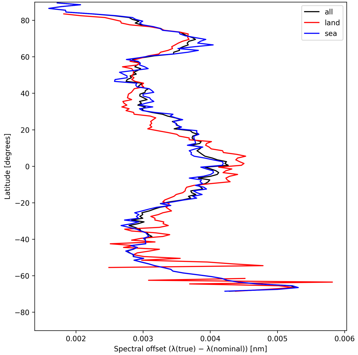
Figure 28: Zonal average of “Spectral offset ( \lambda_{\text{true}} - \lambda_{\text{nominal}} )” for 2025-05-15 to 2025-05-17.
