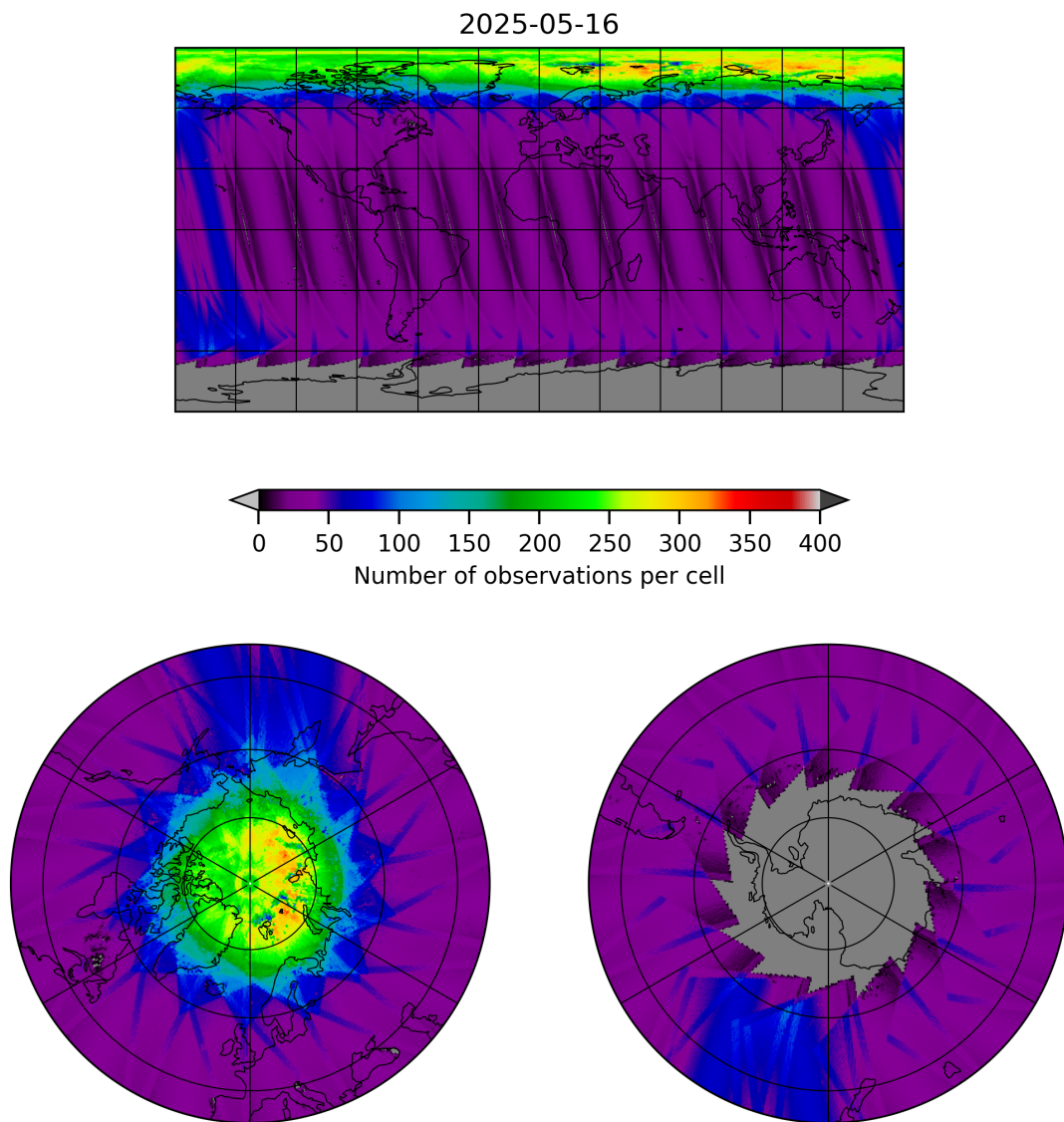
Figure 11: Map of the number of observations for 2025-05-15 to 2025-05-17
