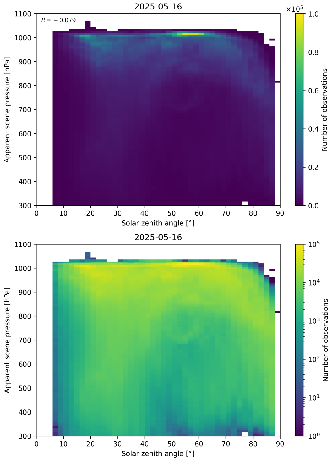
Figure 108: Scatter density plot of “Solar zenith angle” against “Apparent scene pressure” for 2025-05-15 to 2025-05-17.
