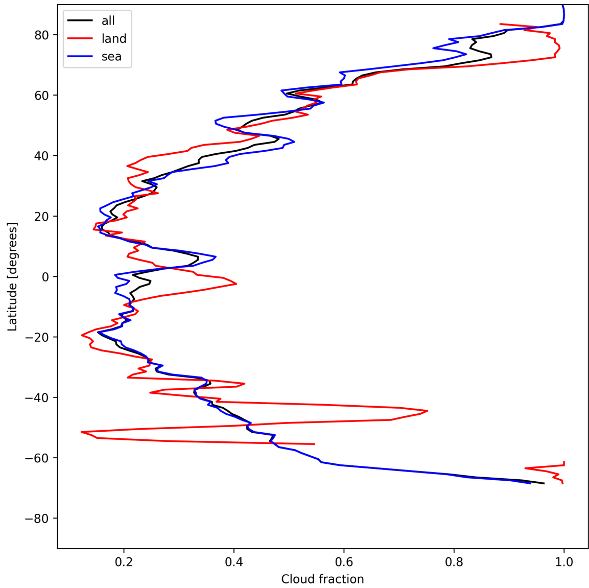
Figure 15: Zonal average of “Cloud fraction” for 2025-05-15 to 2025-05-17.
