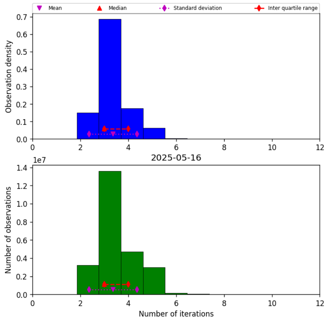
Figure 39: Histogram of “Number of iterations” for 2025-05-15 to 2025-05-17
