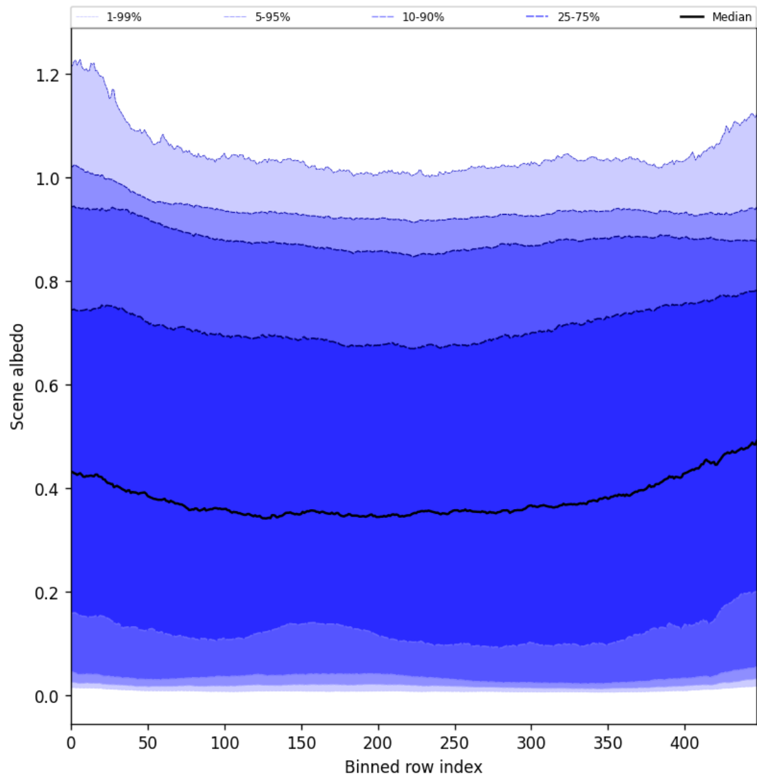
Figure 51: Along track statistics of “Scene albedo” for 2025-05-15 to 2025-05-17
