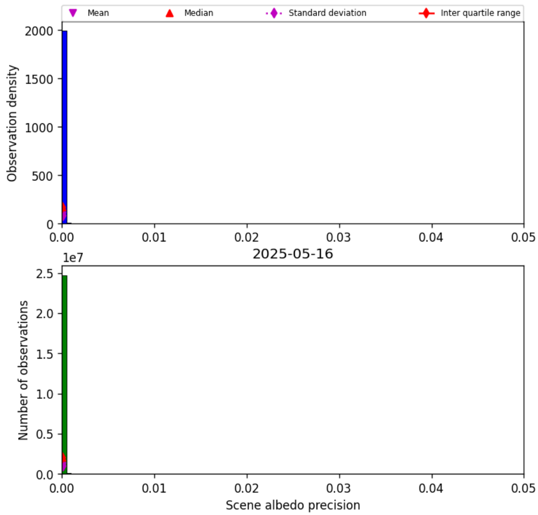
Figure 35: Histogram of “Scene albedo precision” for 2025-05-15 to 2025-05-17
