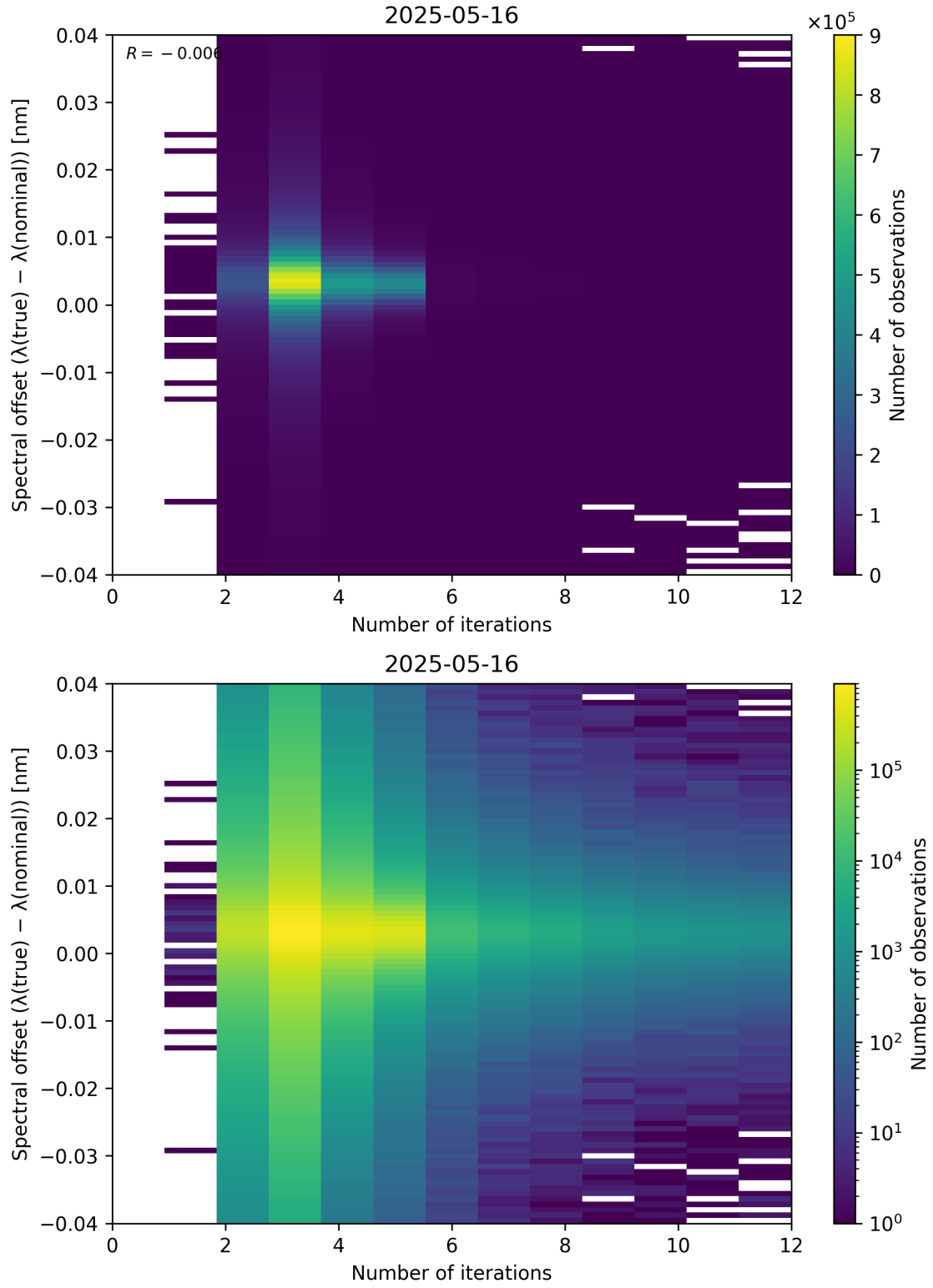
Figure 100: Scatter density plot of “Number of iterations” against “Spectral offset ( \lambda_{\text{true}} - \lambda_{\text{nominal}} )” for 2025-05-15 to 2025-05-17.
