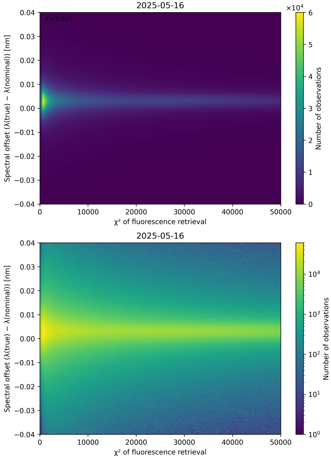
Figure 69: Scatter density plot of “ \chi^2 of fluorescence retrieval” against “Spectral offset ( \lambda_{\text{true}} - \lambda_{\text{nominal}} )” for 2025-05-15 to 2025-05-17.
