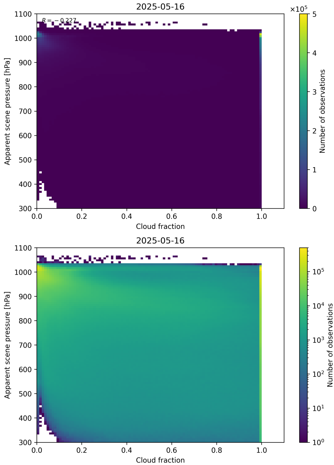
Figure 70: Scatter density plot of “Cloud fraction” against “Apparent scene pressure” for 2025-05-15 to 2025-05-17.
