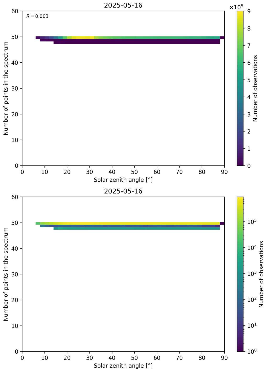
Figure 115: Scatter density plot of “Solar zenith angle” against “Number of points in the spectrum” for 2025-05-15 to 2025-05-17.
