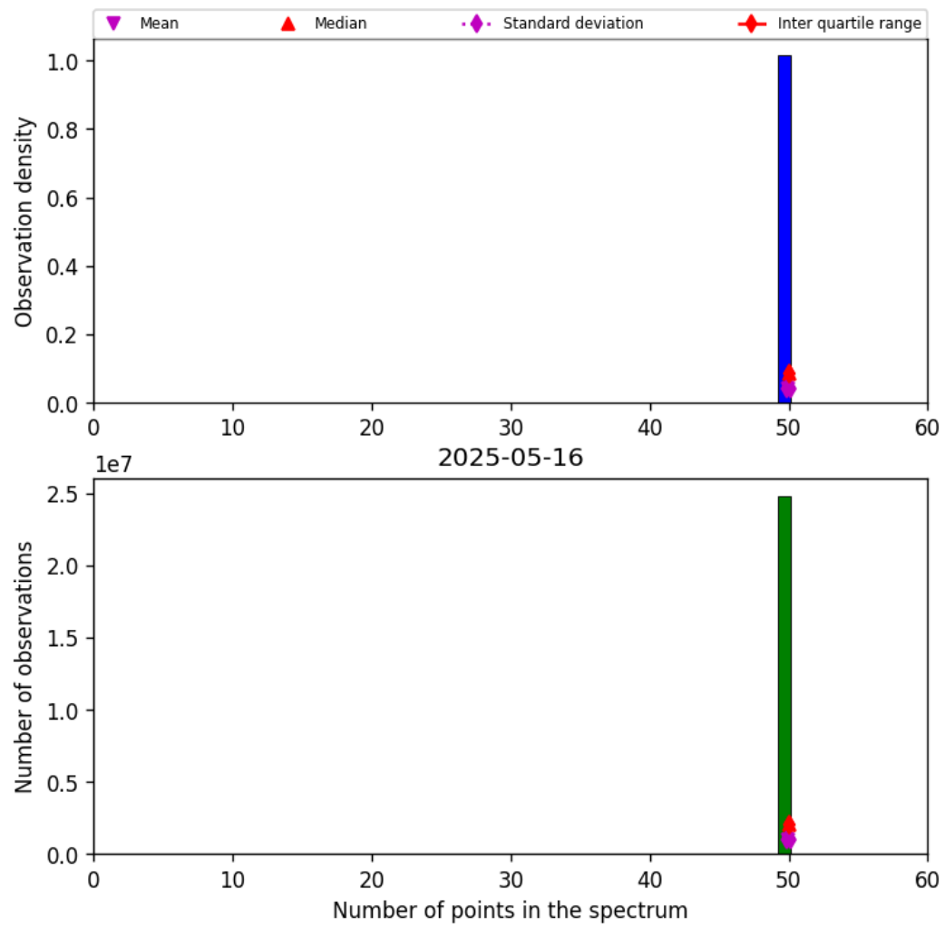
Figure 44: Histogram of “Number of points in the spectrum” for 2025-05-15 to 2025-05-17
