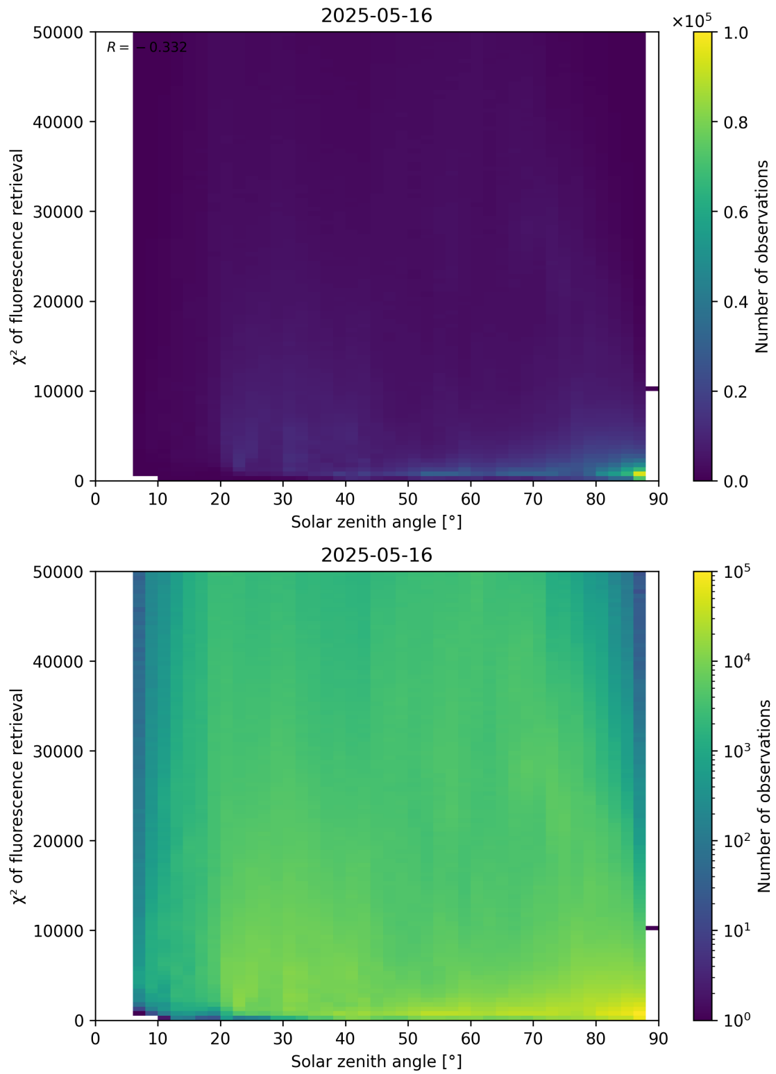
Figure 109: Scatter density plot of “Solar zenith angle” against “ \chi^2 of fluorescence retrieval” for 2025-05-15 to 2025-05-17.
