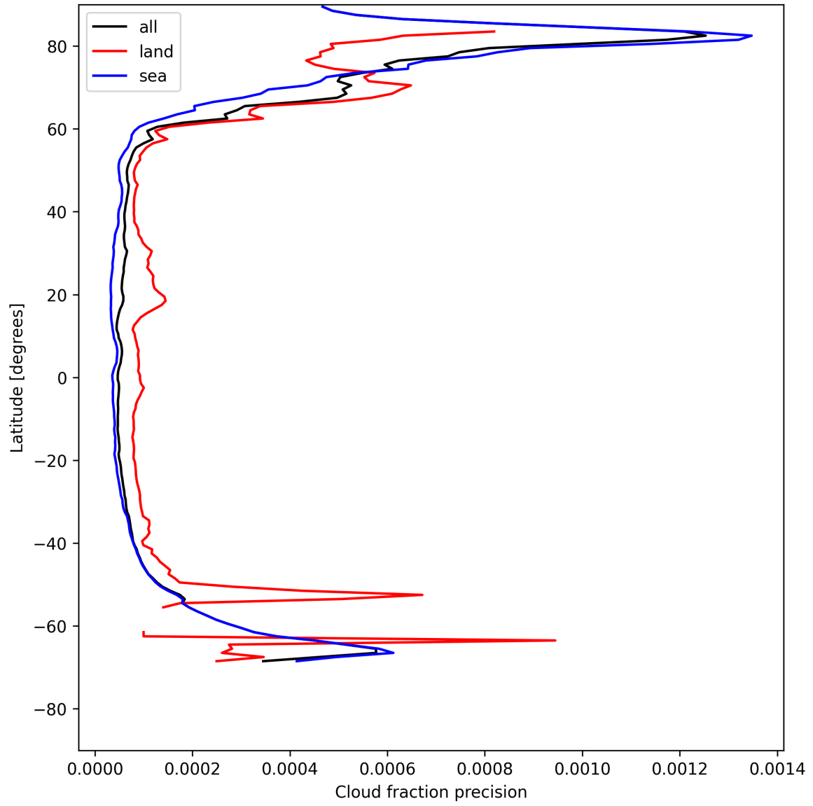
Figure 16: Zonal average of “Cloud fraction precision” for 2025-05-15 to 2025-05-17.
