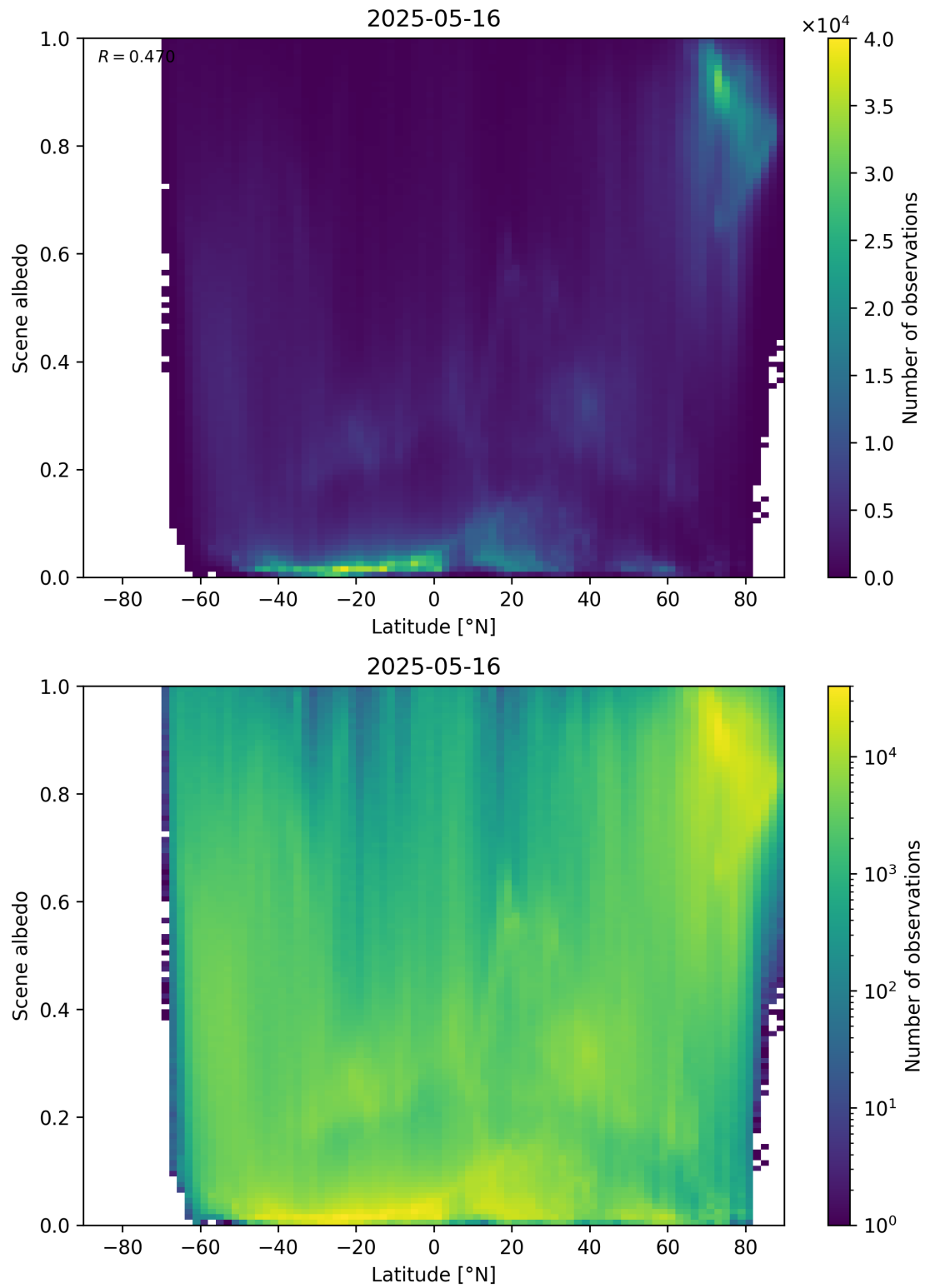
Figure 95: Scatter density plot of “Latitude” against “Scene albedo” for 2025-05-15 to 2025-05-17.
