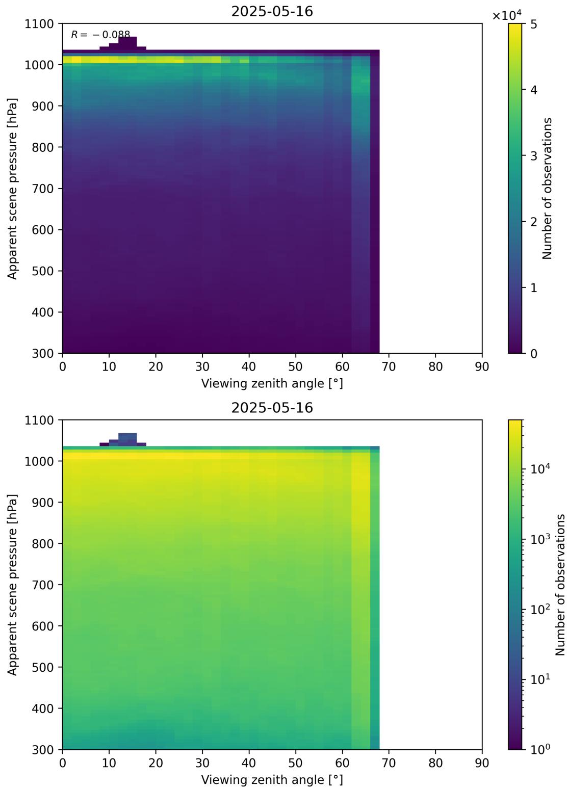
Figure 118: Scatter density plot of “Viewing zenith angle” against “Apparent scene pressure” for 2025-05-15 to 2025-05-17.
