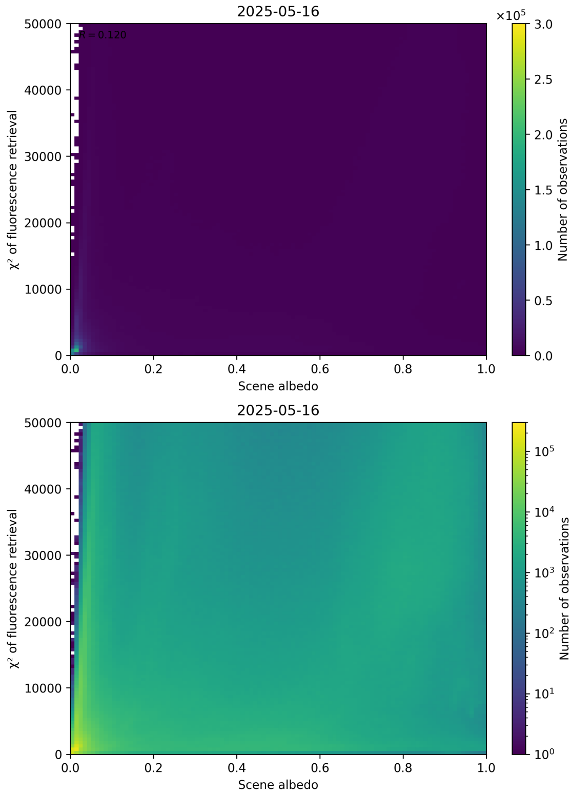
Figure 103: Scatter density plot of “Scene albedo” against “ \chi^2 of fluorescence retrieval” for 2025-05-15 to 2025-05-17.
