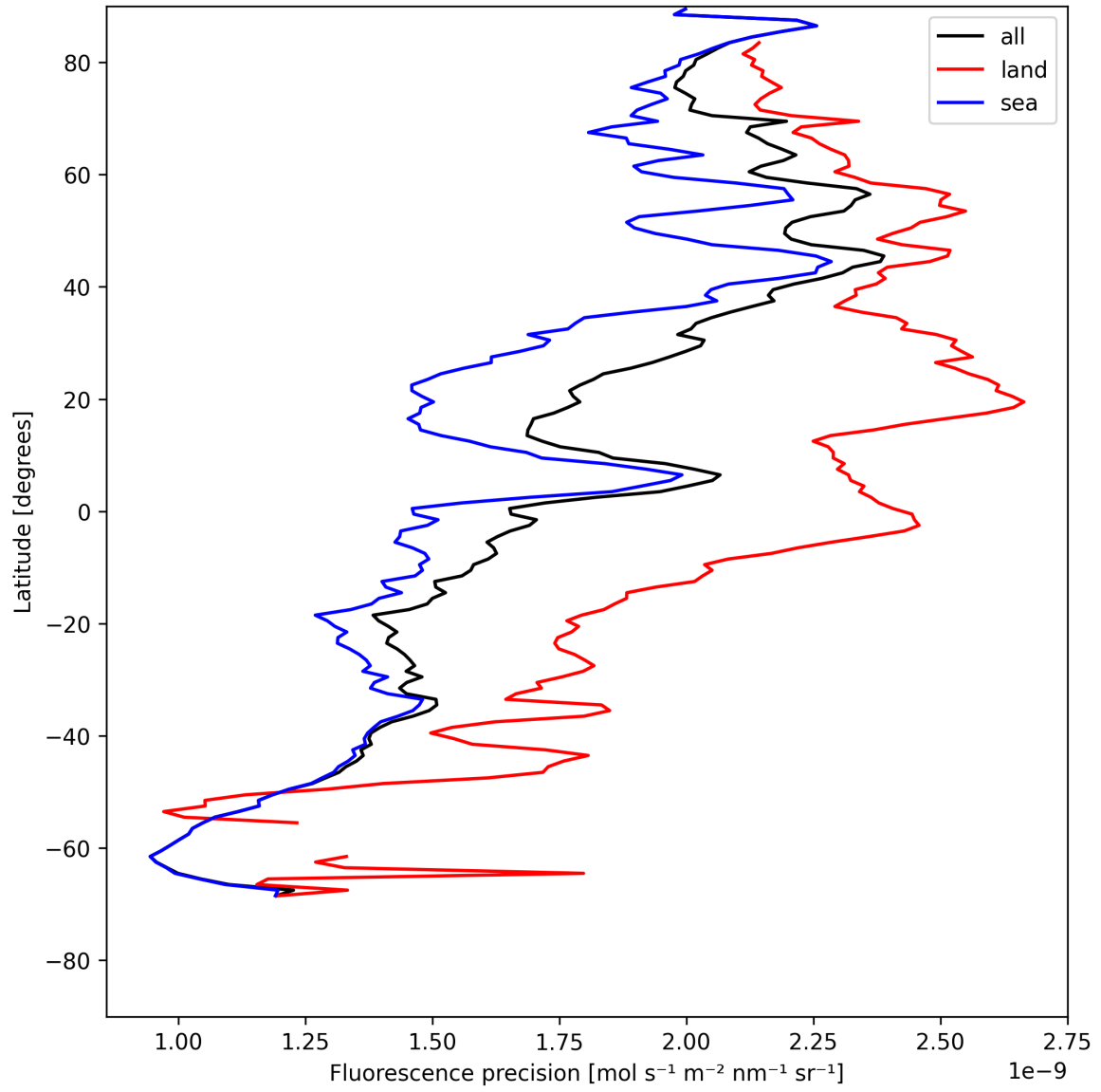
Figure 24: Zonal average of “Fluorescence precision” for 2025-05-15 to 2025-05-17.
