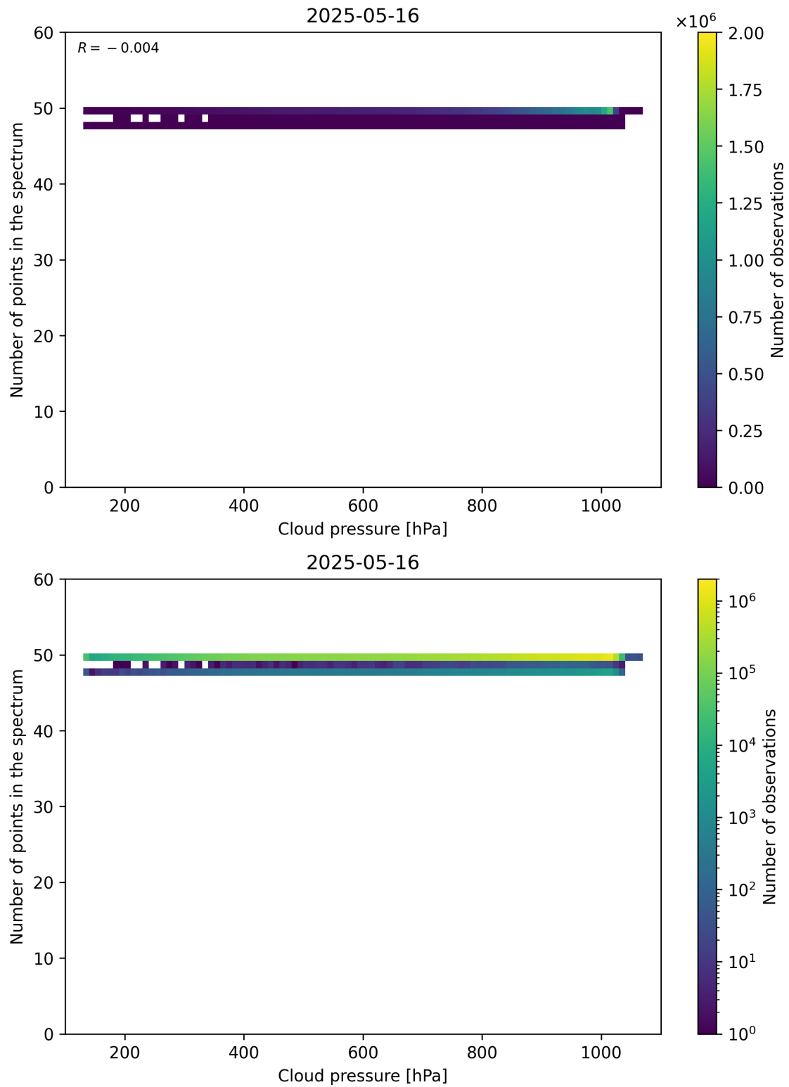
Figure 82: Scatter density plot of “Cloud pressure” against “Number of points in the spectrum” for 2025-05-15 to 2025-05-17.
