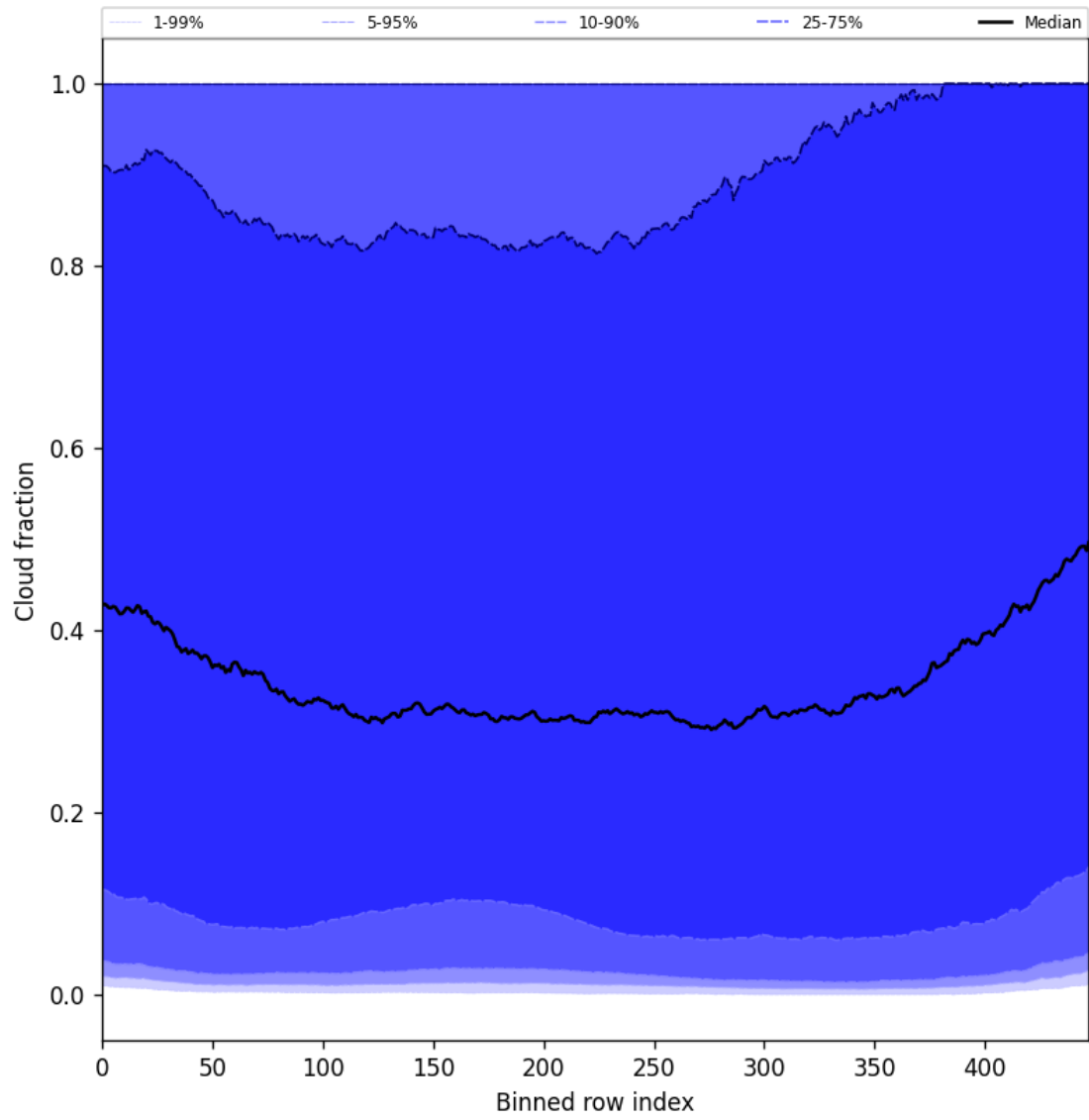
Figure 49: Along track statistics of “Cloud fraction” for 2025-05-15 to 2025-05-17
