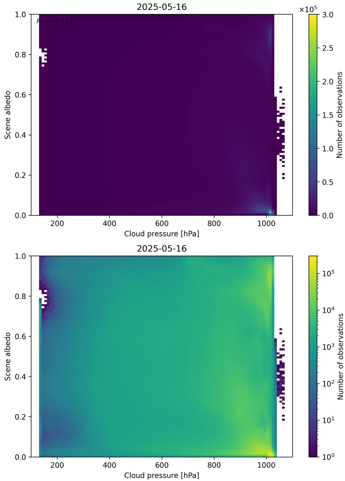
Figure 83: Scatter density plot of “Cloud pressure” against “Scene albedo” for 2025-05-15 to 2025-05-17.
