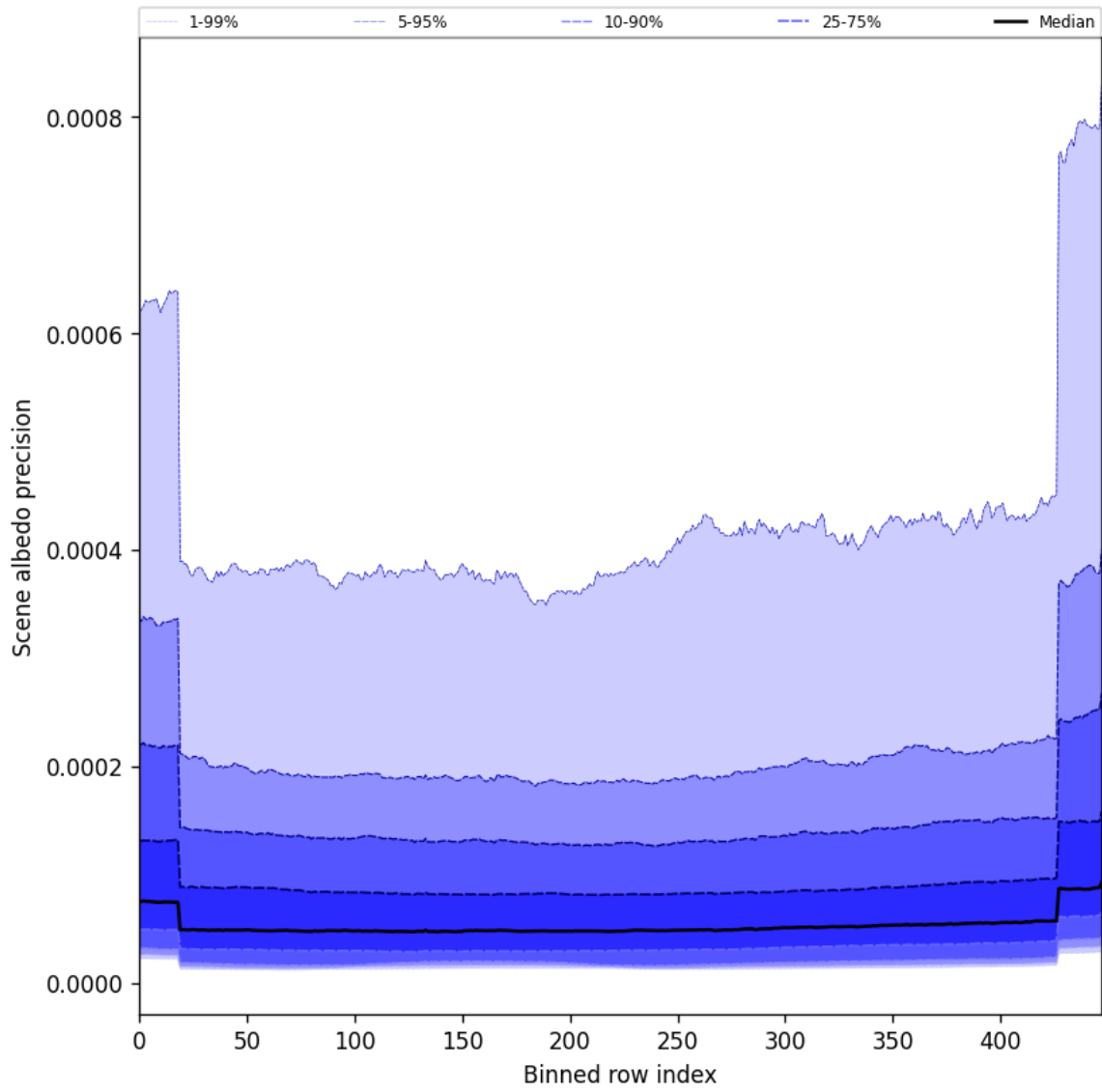
Figure 52: Along track statistics of “Scene albedo precision” for 2025-05-15 to 2025-05-17
