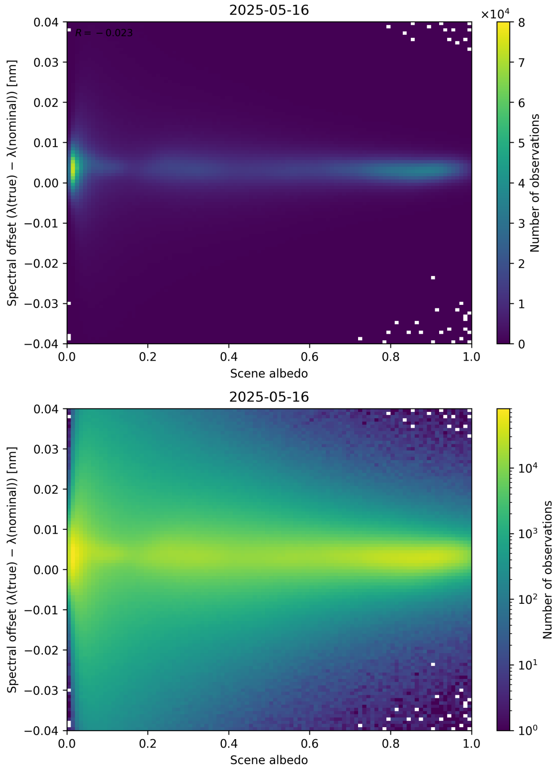
Figure 107: Scatter density plot of “Scene albedo” against “Spectral offset ( \lambda_{\text{true}} - \lambda_{\text{nominal}} )” for 2025-05-15 to 2025-05-17.
