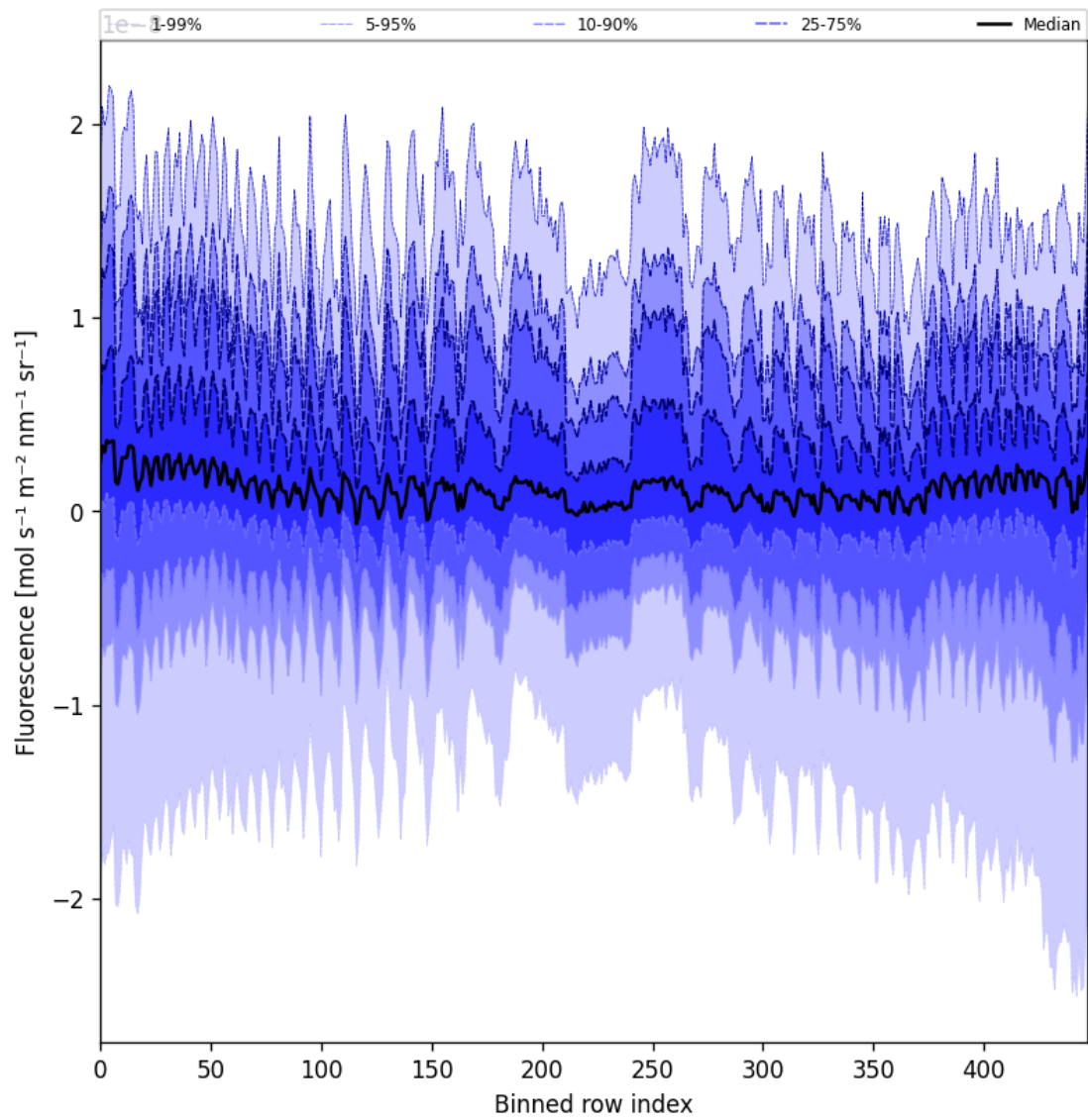
Figure 57: Along track statistics of “Fluorescence” for 2025-05-15 to 2025-05-17
