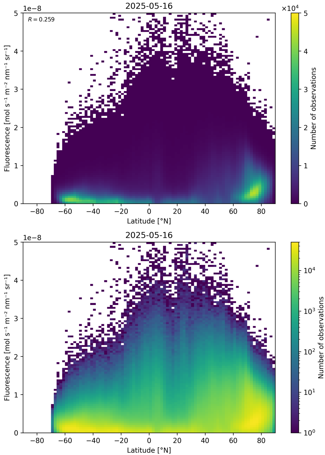
Figure 92: Scatter density plot of “Latitude” against “Fluorescence” for 2025-05-15 to 2025-05-17.
