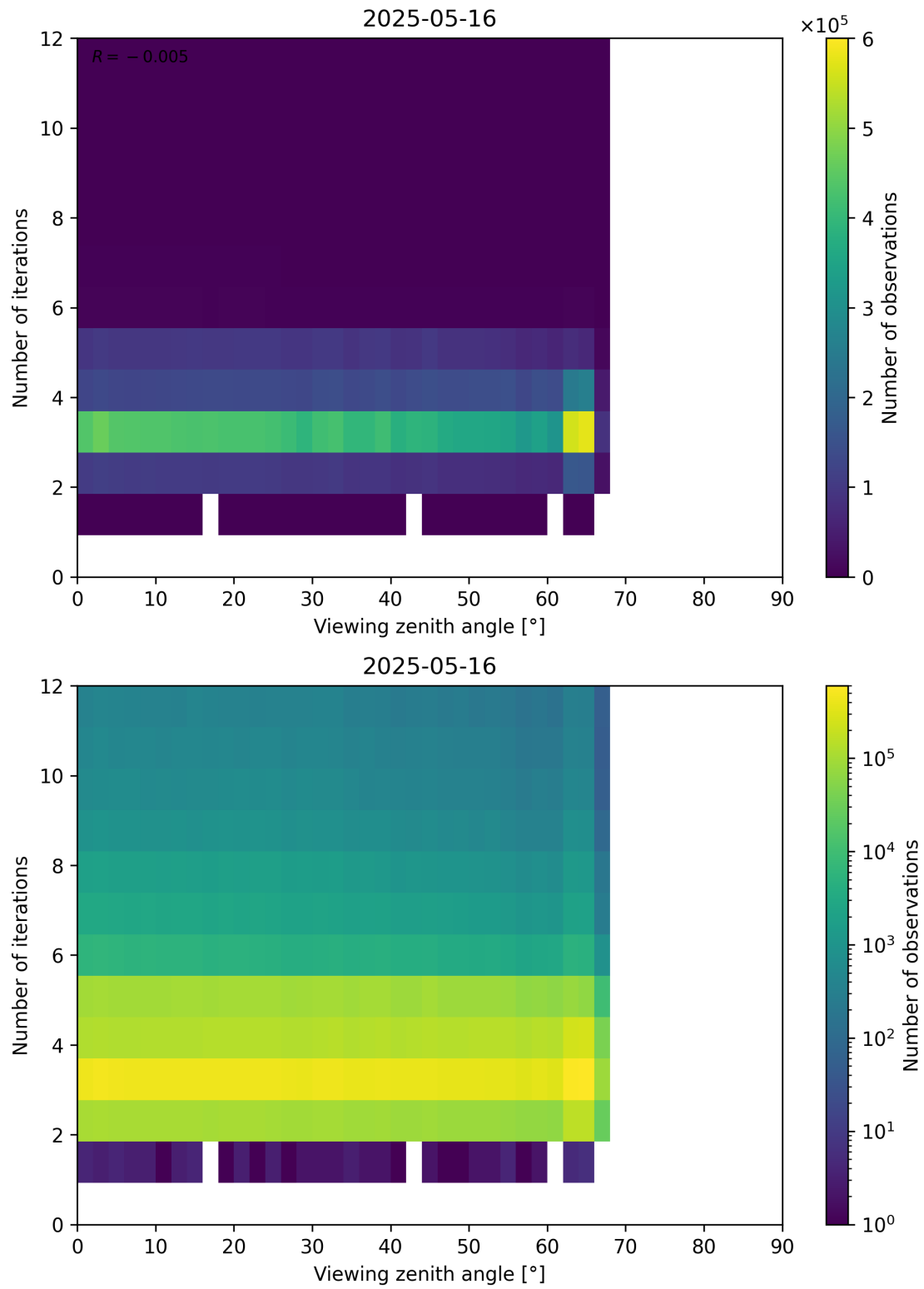
Figure 124: Scatter density plot of “Viewing zenith angle” against “Number of iterations” for 2025-05-15 to 2025-05-17.
