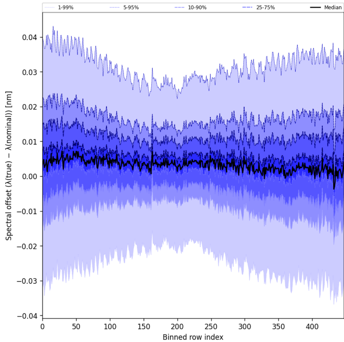
Figure 62: Along track statistics of “Spectral offset ( \lambda_{\text{true}} - \lambda_{\text{nominal}} )” for 2025-05-15 to 2025-05-17
