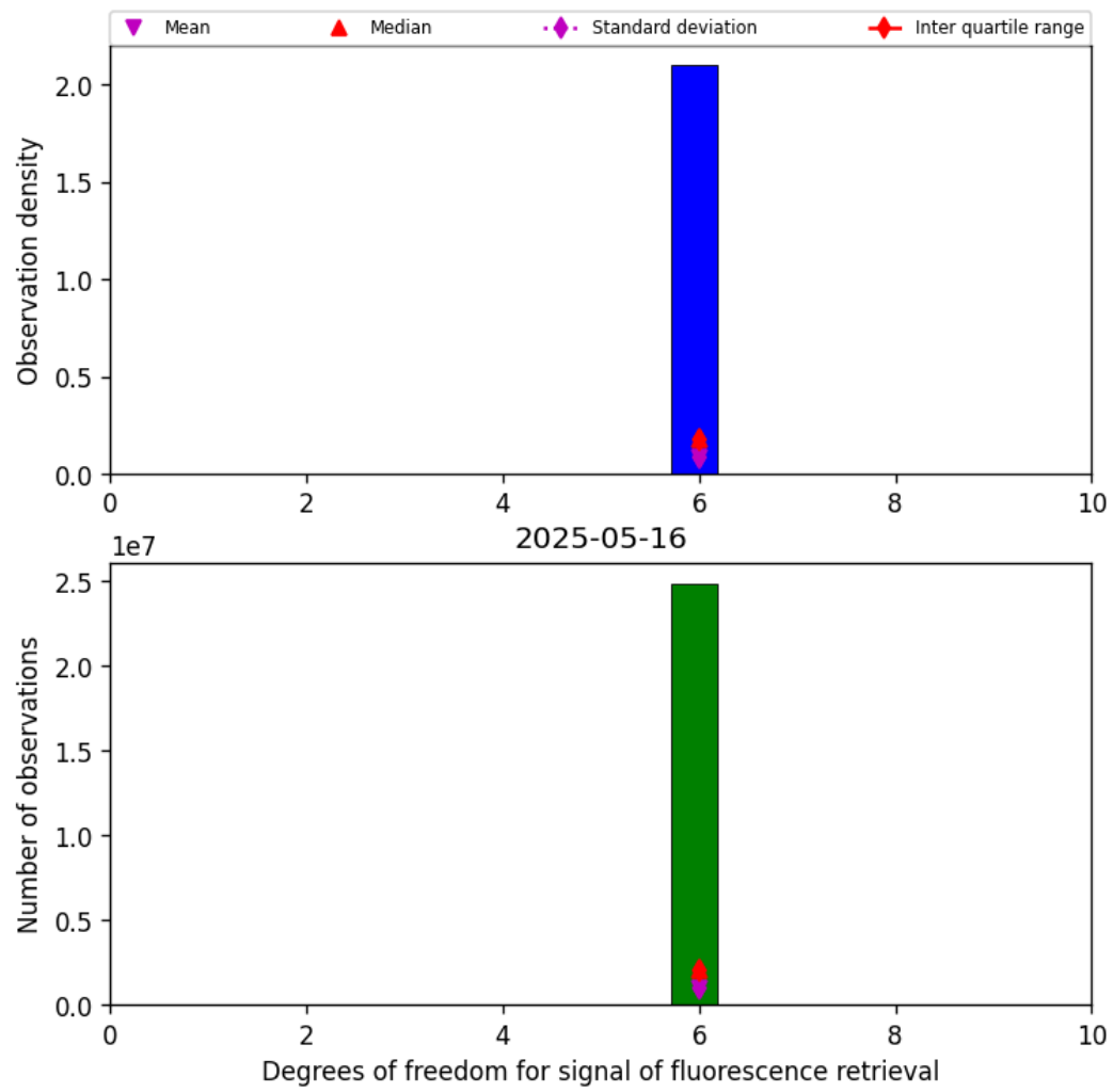
Figure 43: Histogram of “Degrees of freedom for signal of fluorescence retrieval” for 2025-05-15 to 2025-05-17
