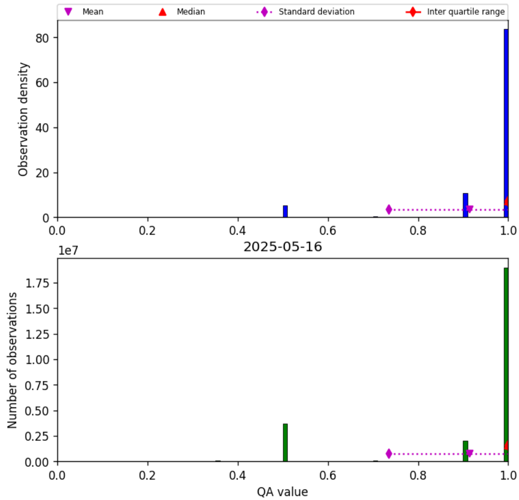
Figure 29: Histogram of “QA value” for 2025-05-15 to 2025-05-17
