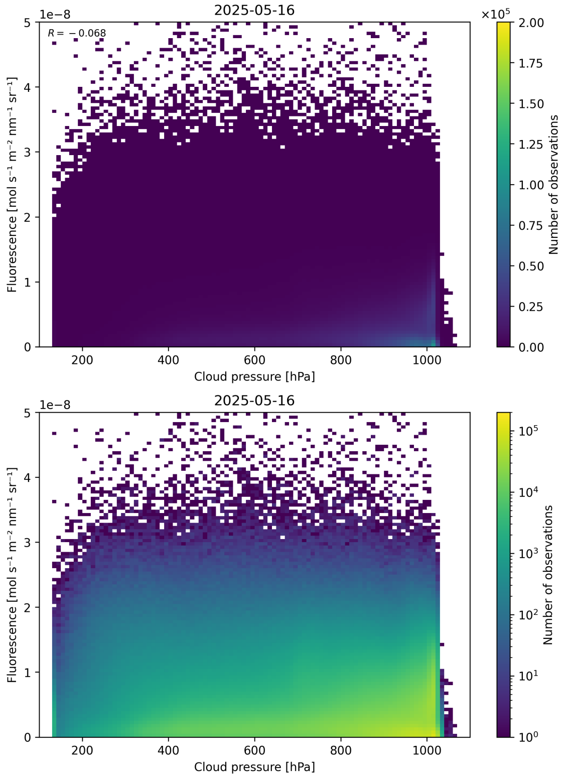
Figure 80: Scatter density plot of “Cloud pressure” against “Fluorescence” for 2025-05-15 to 2025-05-17.
