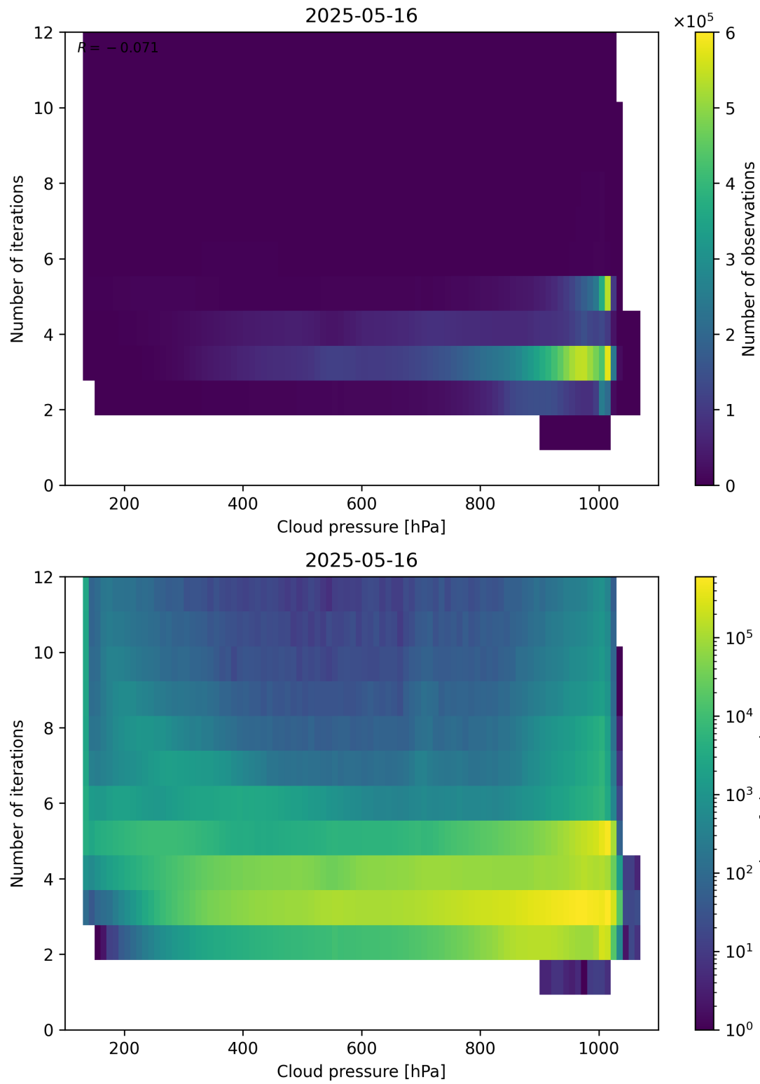
Figure 81: Scatter density plot of “Cloud pressure” against “Number of iterations” for 2025-05-15 to 2025-05-17.
