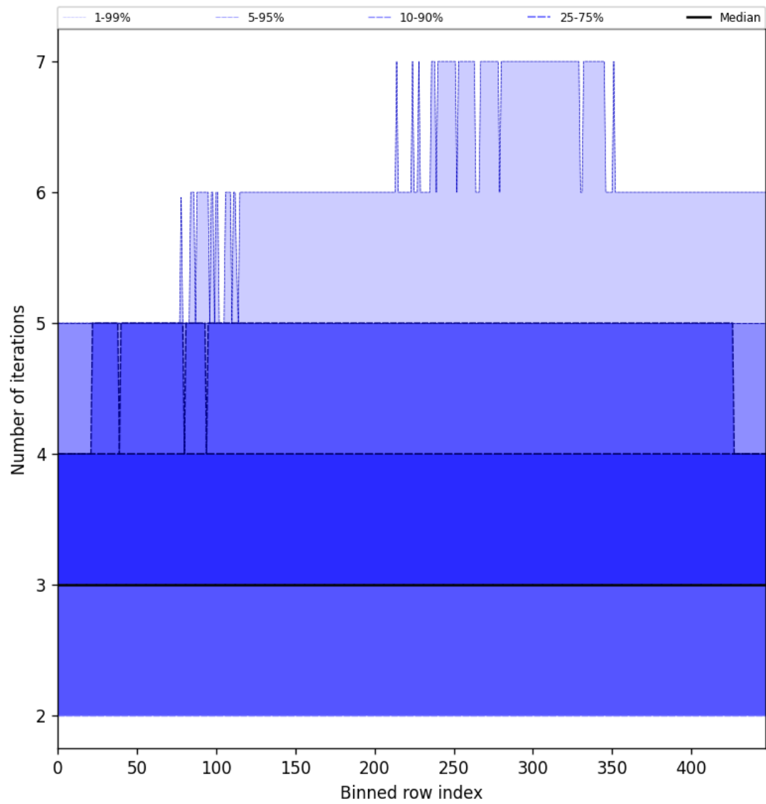
Figure 56: Along track statistics of “Number of iterations” for 2025-05-15 to 2025-05-17
