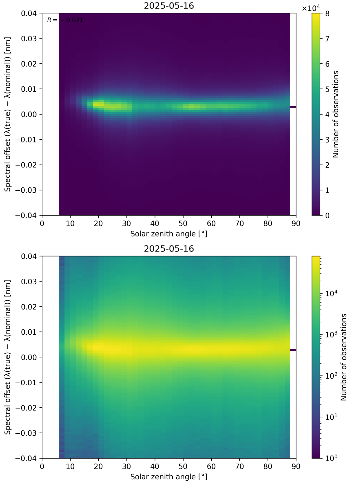
Figure 117: Scatter density plot of “Solar zenith angle” against “Spectral offset ( \lambda_{\text{true}} - \lambda_{\text{nominal}} )” for 2025-05-15 to 2025-05-17.
