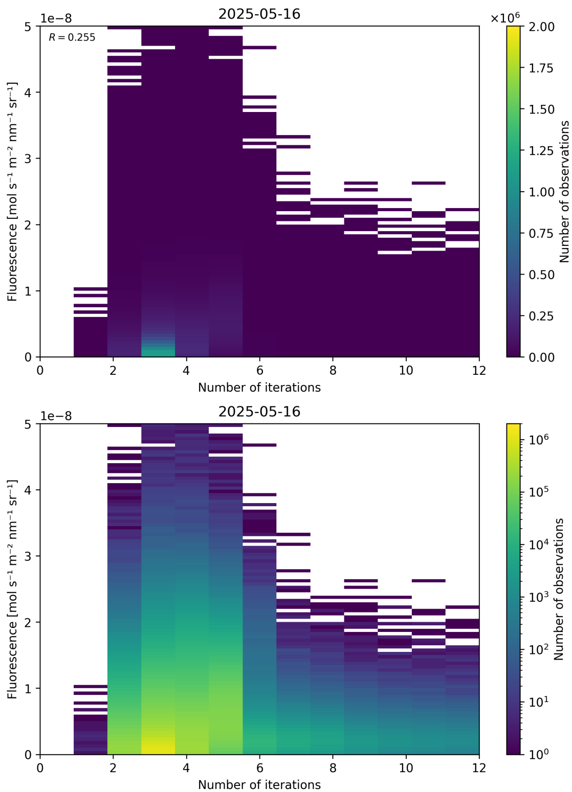
Figure 98: Scatter density plot of “Number of iterations” against “Fluorescence” for 2025-05-15 to 2025-05-17.
