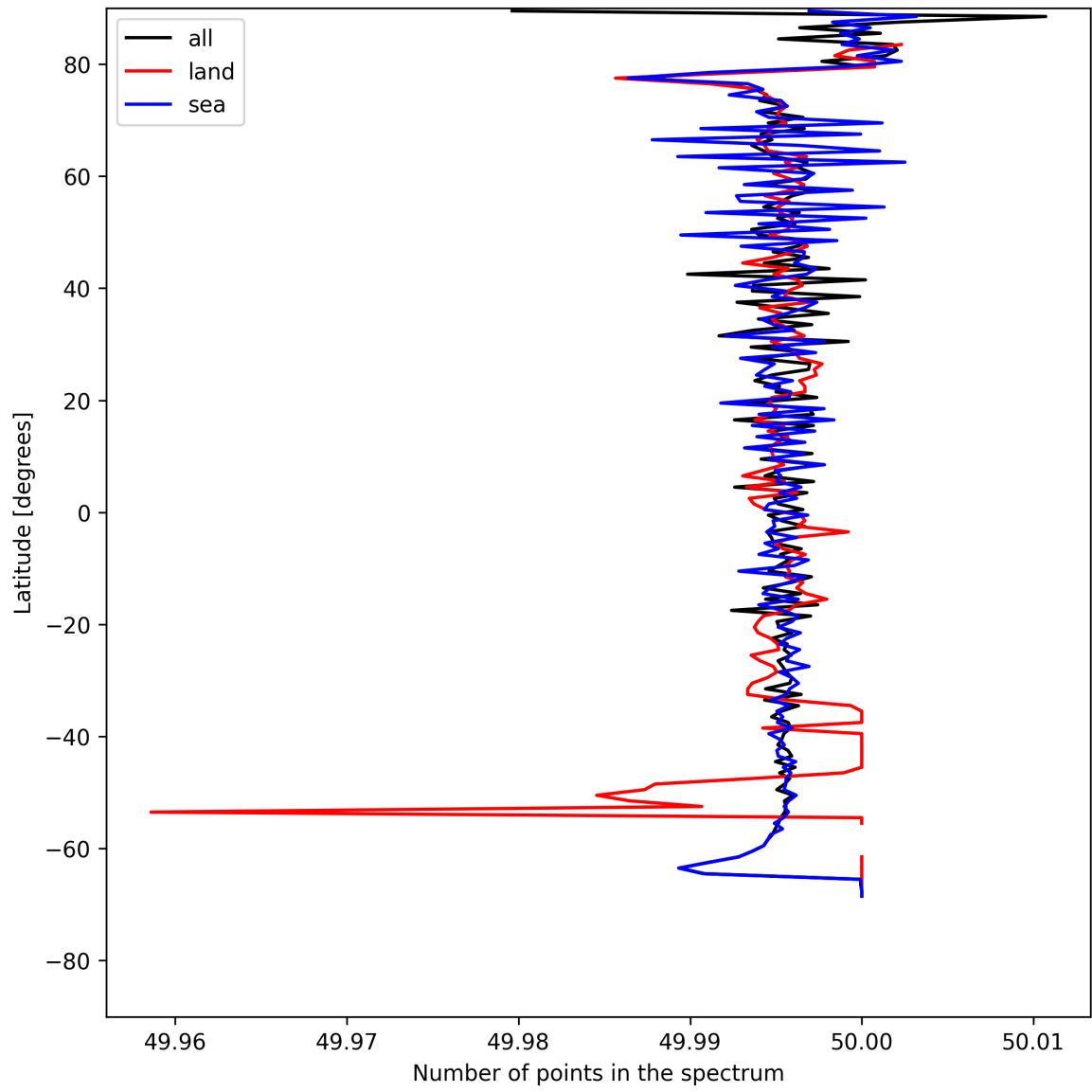
Figure 27: Zonal average of “Number of points in the spectrum” for 2025-05-15 to 2025-05-17.
