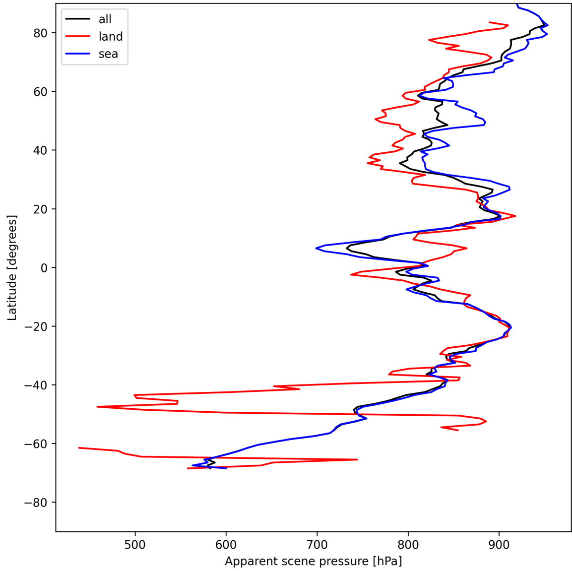
Figure 19: Zonal average of “Apparent scene pressure” for 2025-05-15 to 2025-05-17.
