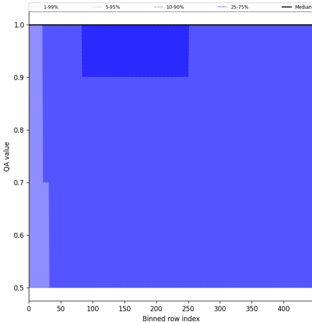
Figure 46: Along track statistics of “QA value” for 2025-05-15 to 2025-05-17
