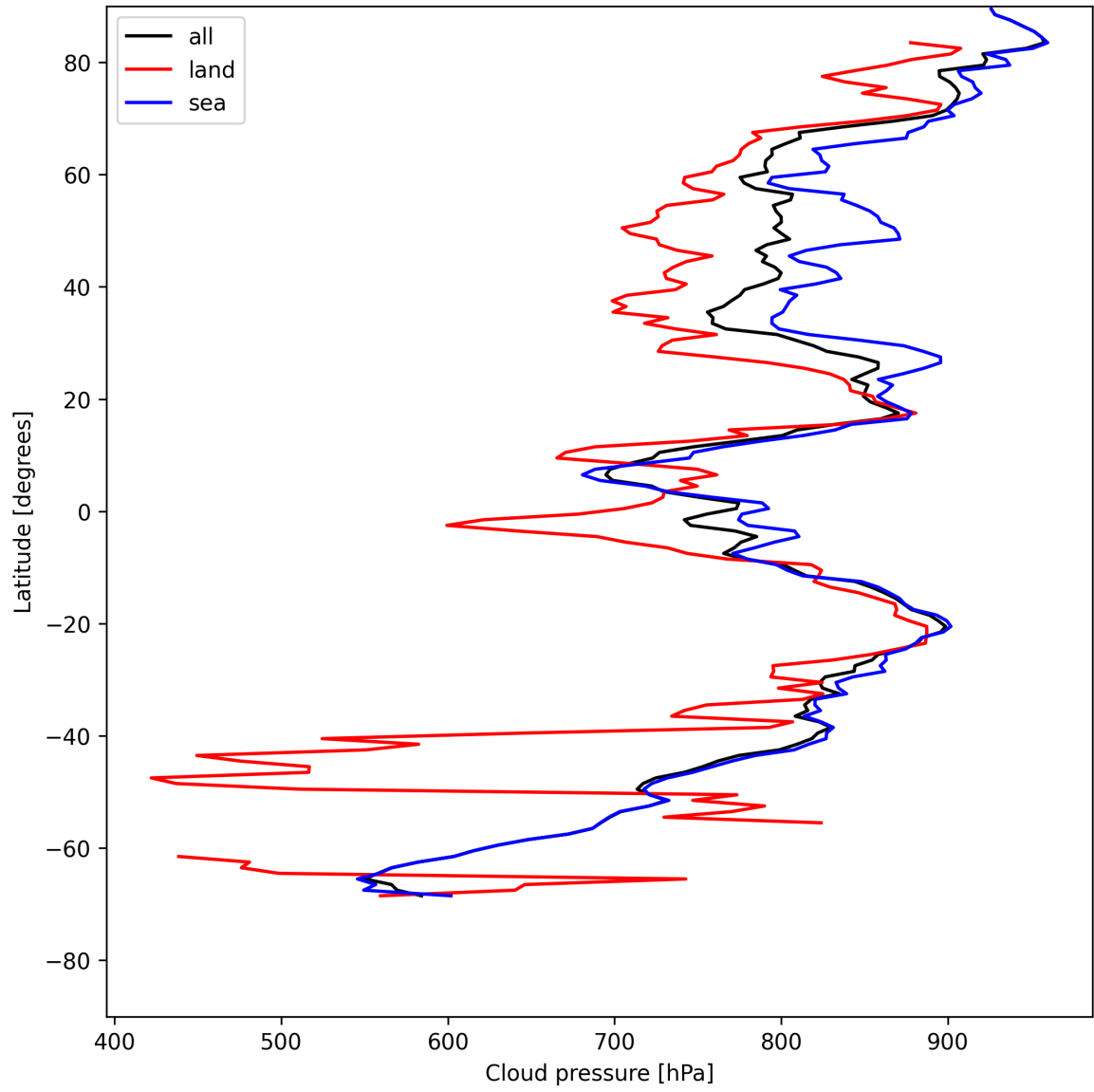
Figure 13: Zonal average of “Cloud pressure” for 2025-05-15 to 2025-05-17.
