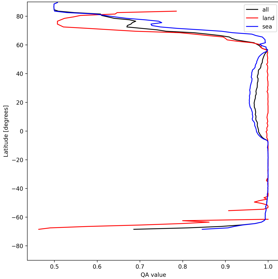
Figure 12: Zonal average of “QA value” for 2025-05-15 to 2025-05-17.
