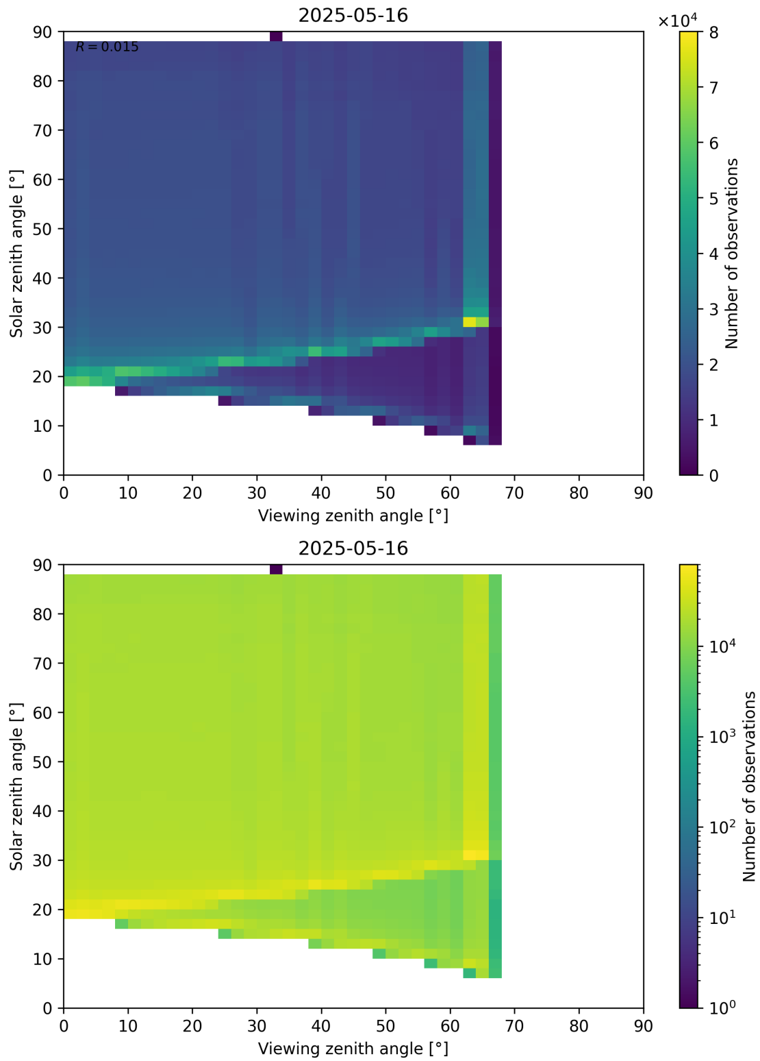
Figure 127: Scatter density plot of “Viewing zenith angle” against “Solar zenith angle” for 2025-05-15 to 2025-05-17.
