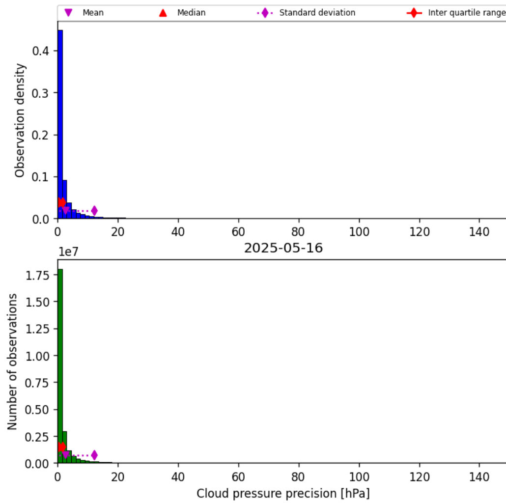
Figure 31: Histogram of “Cloud pressure precision” for 2025-05-15 to 2025-05-17
