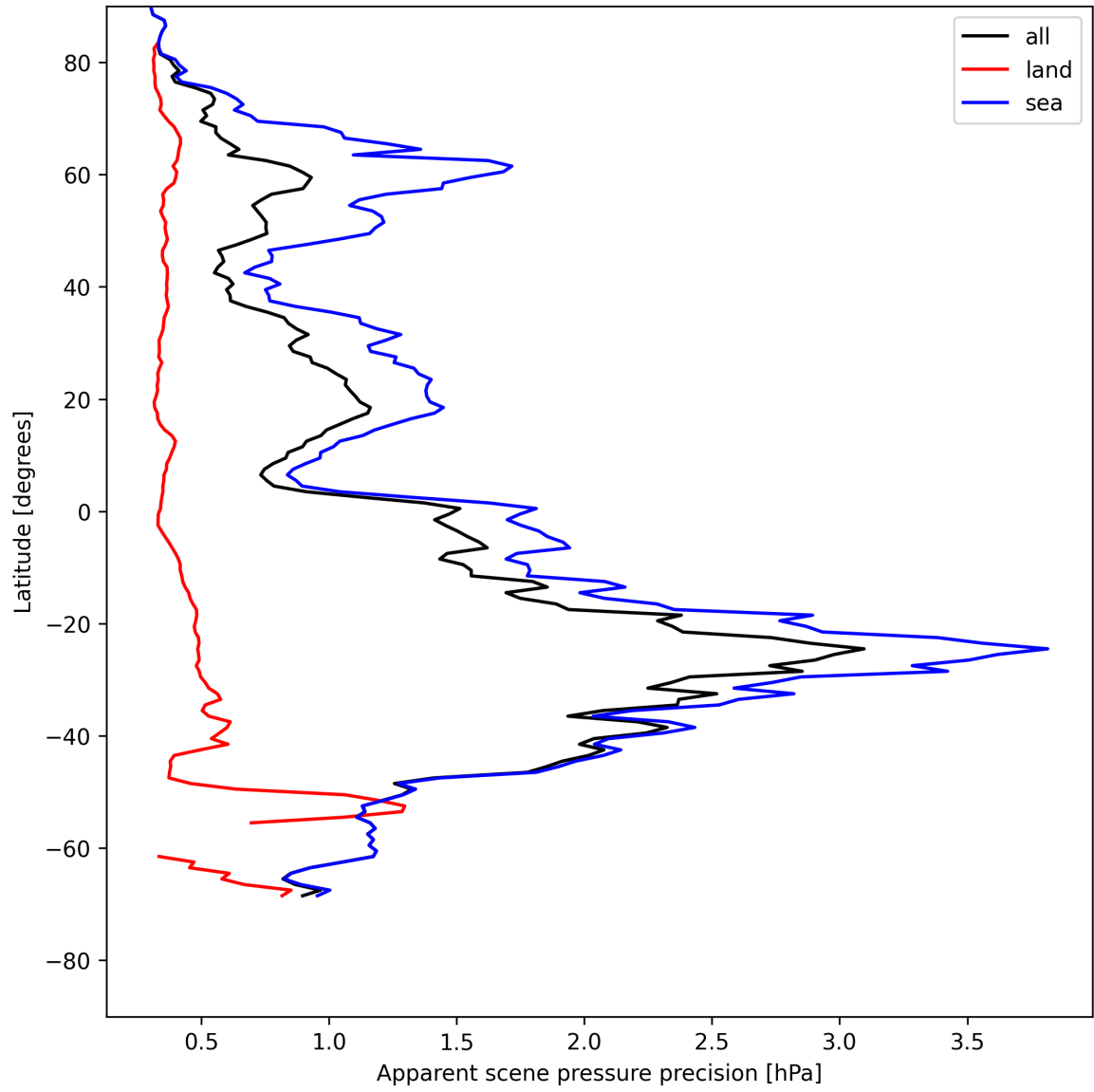
Figure 20: Zonal average of “Apparent scene pressure precision” for 2025-05-15 to 2025-05-17.
