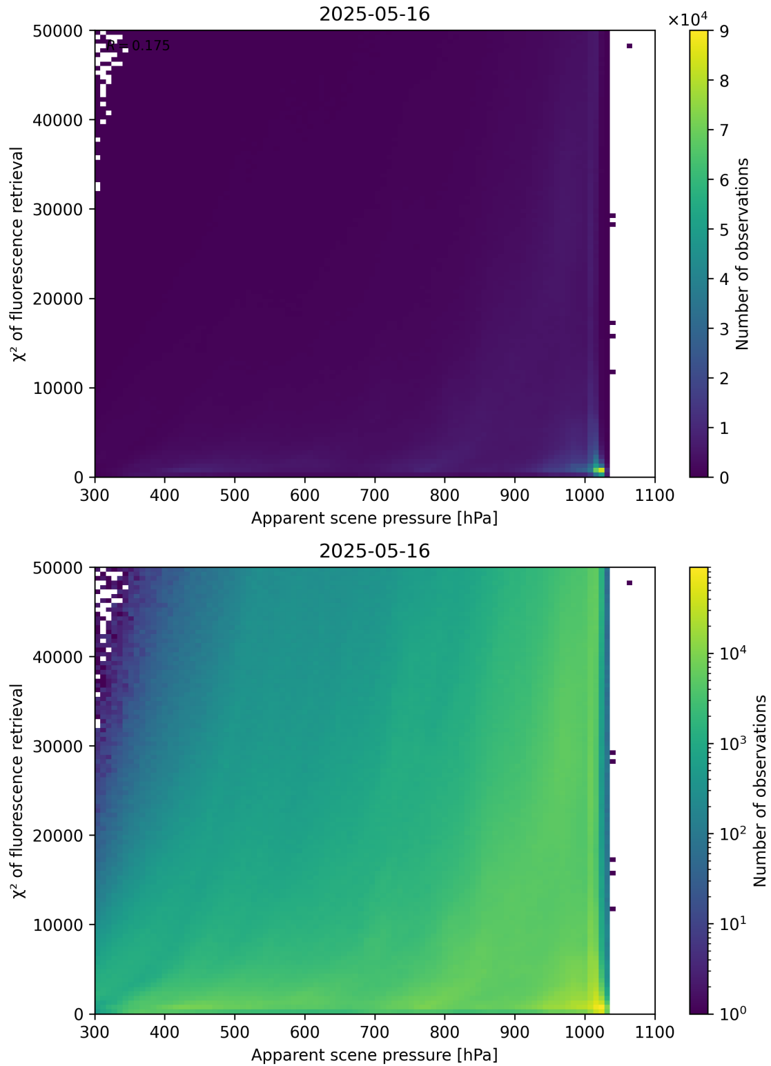
Figure 63: Scatter density plot of “Apparent scene pressure” against “ \chi^2 of fluorescence retrieval” for 2025-05-15 to 2025-05-17.
