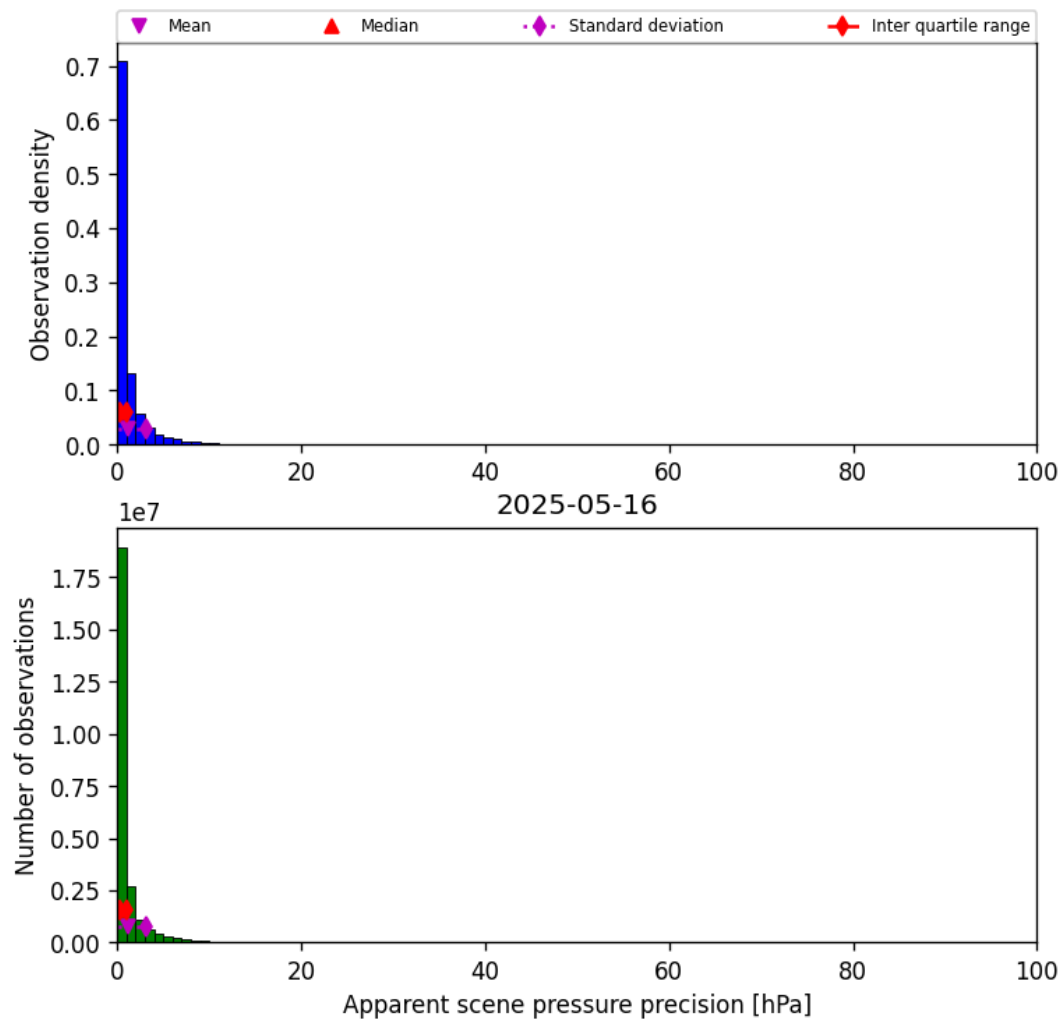
Figure 37: Histogram of “Apparent scene pressure precision” for 2025-05-15 to 2025-05-17
