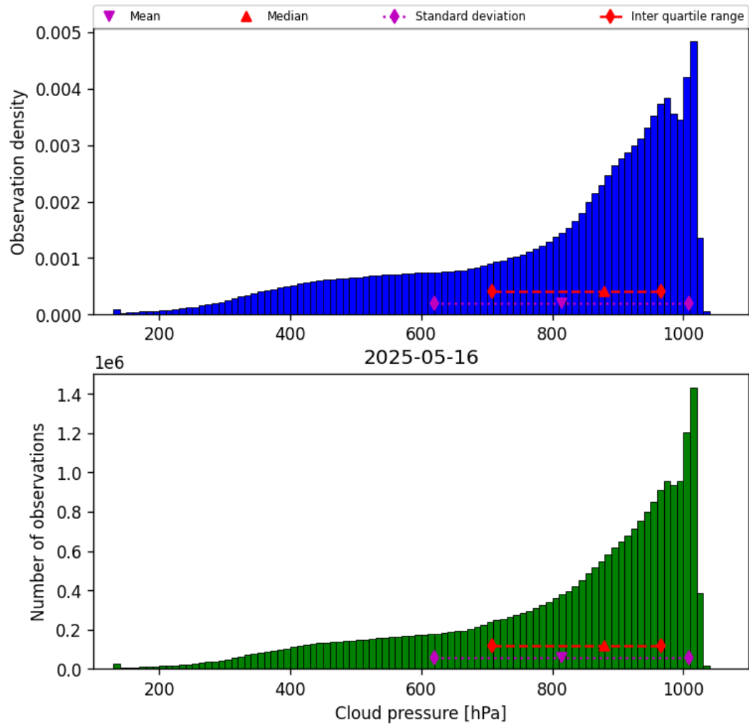
Figure 30: Histogram of “Cloud pressure” for 2025-05-15 to 2025-05-17
