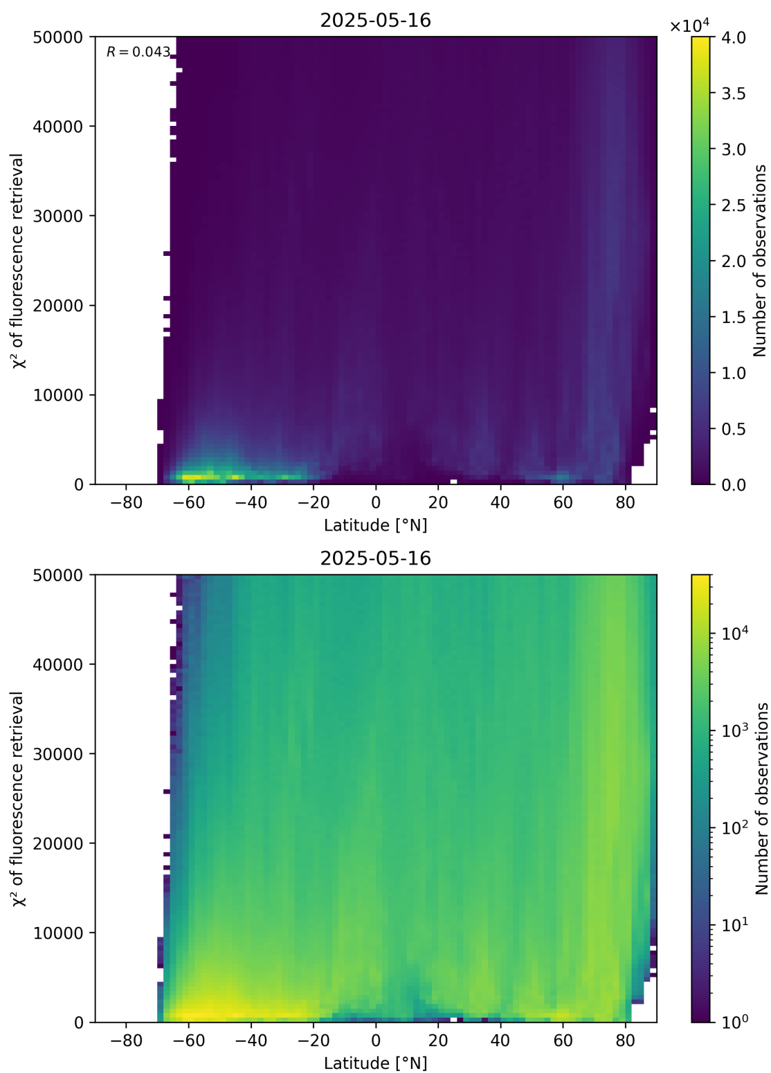
Figure 89: Scatter density plot of “Latitude” against “ \chi^2 of fluorescence retrieval” for 2025-05-15 to 2025-05-17.
