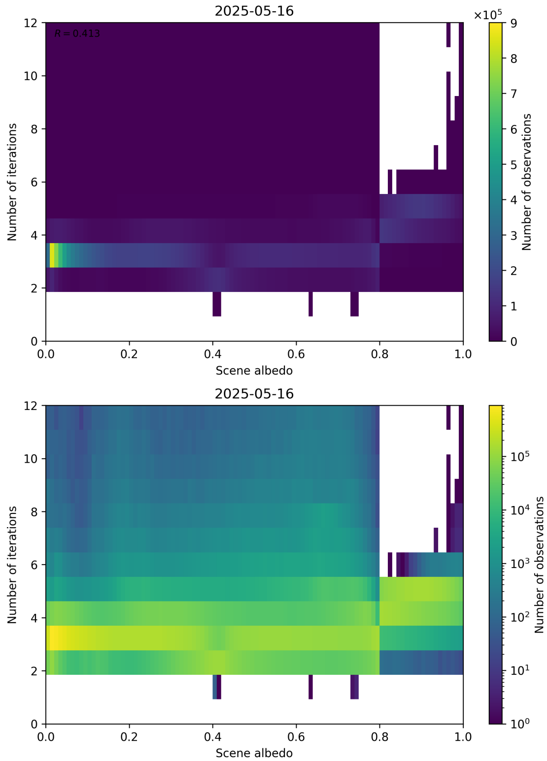
Figure 105: Scatter density plot of “Scene albedo” against “Number of iterations” for 2025-05-15 to 2025-05-17.
