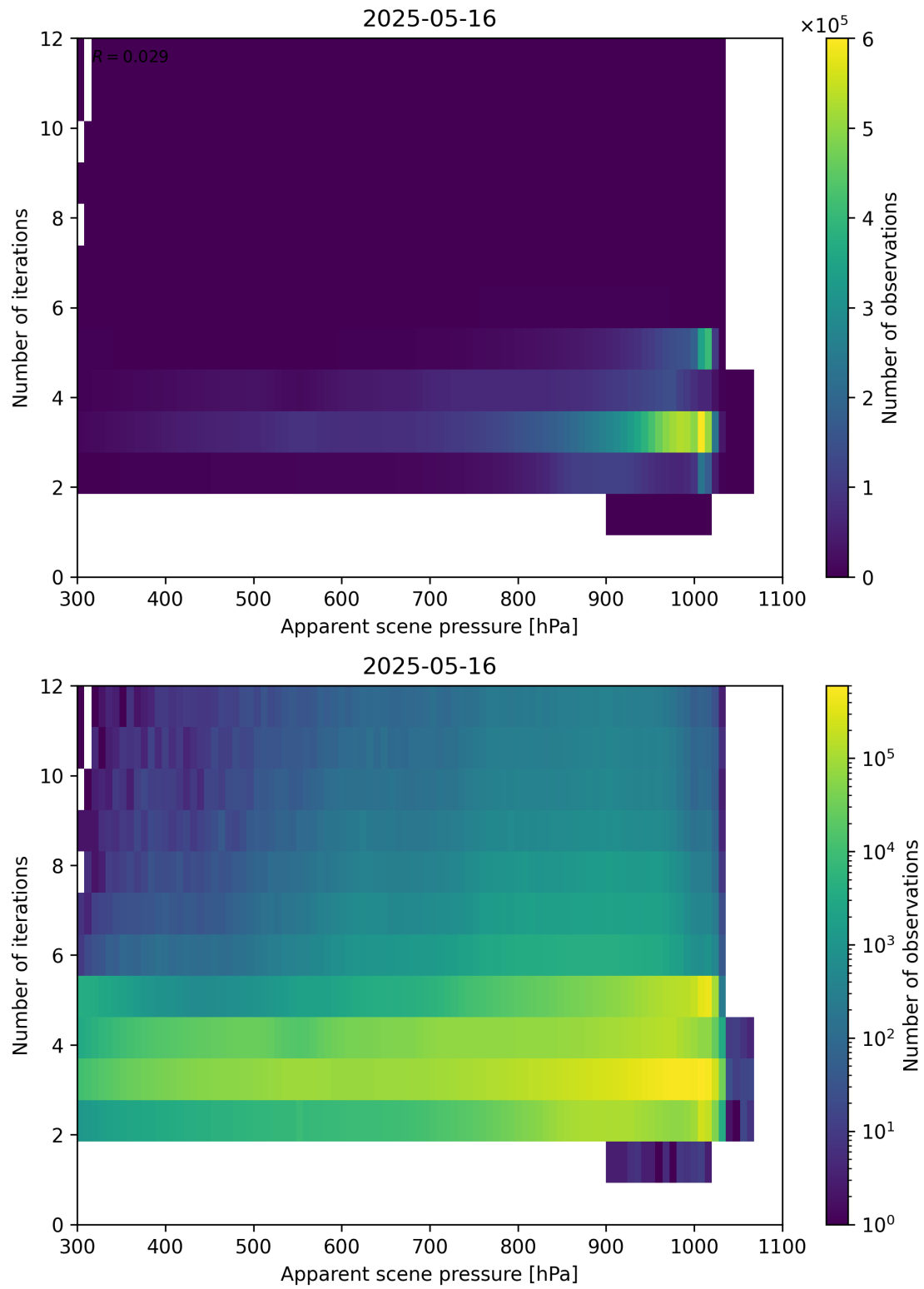
Figure 65: Scatter density plot of “Apparent scene pressure” against “Number of iterations” for 2025-05-15 to 2025-05-17.
