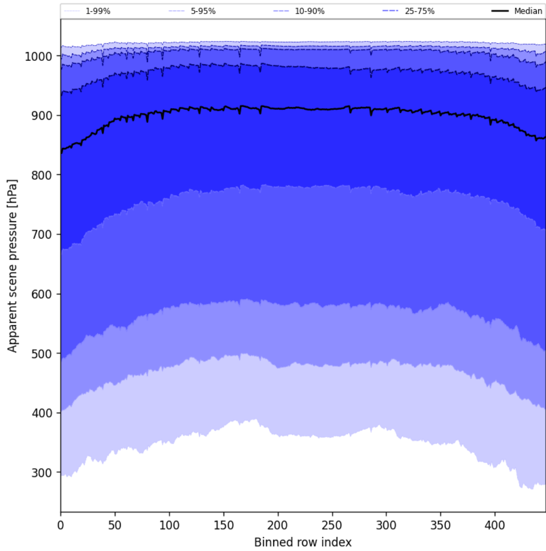
Figure 53: Along track statistics of “Apparent scene pressure” for 2025-05-15 to 2025-05-17
