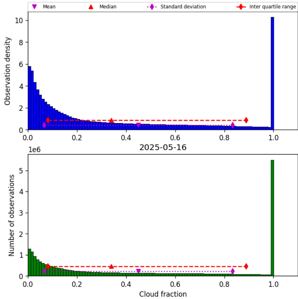
Figure 32: Histogram of “Cloud fraction” for 2025-05-15 to 2025-05-17
