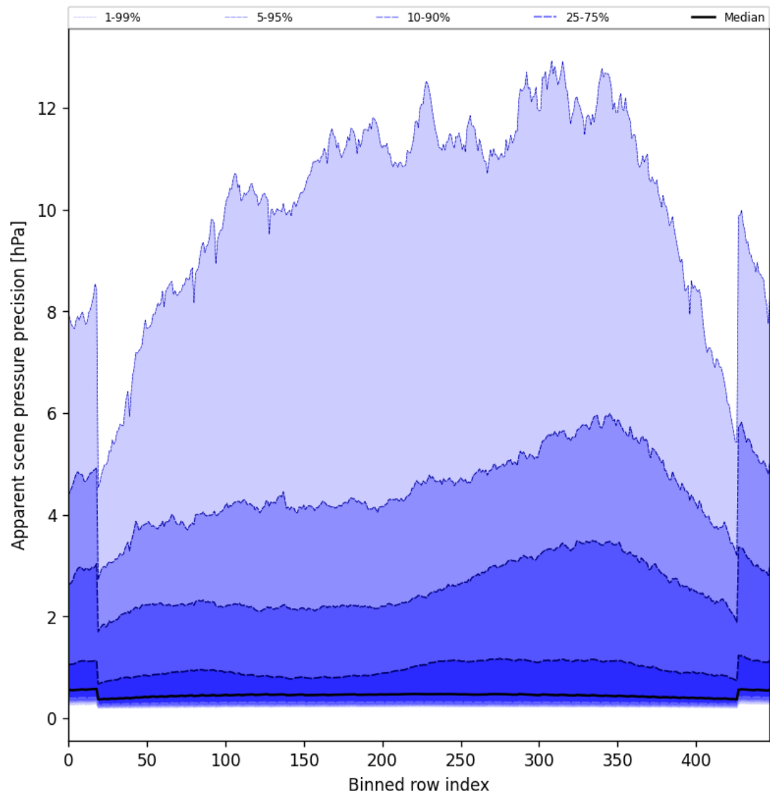
Figure 54: Along track statistics of “Apparent scene pressure precision” for 2025-05-15 to 2025-05-17
