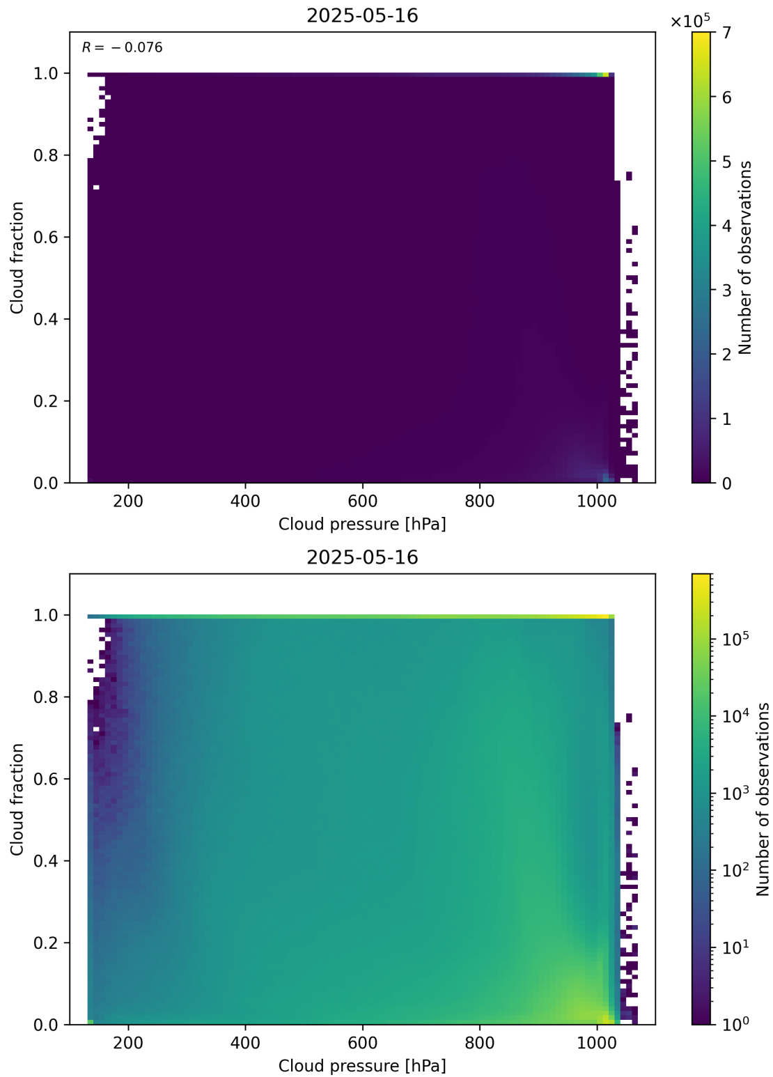
Figure 79: Scatter density plot of “Cloud pressure” against “Cloud fraction” for 2025-05-15 to 2025-05-17.
