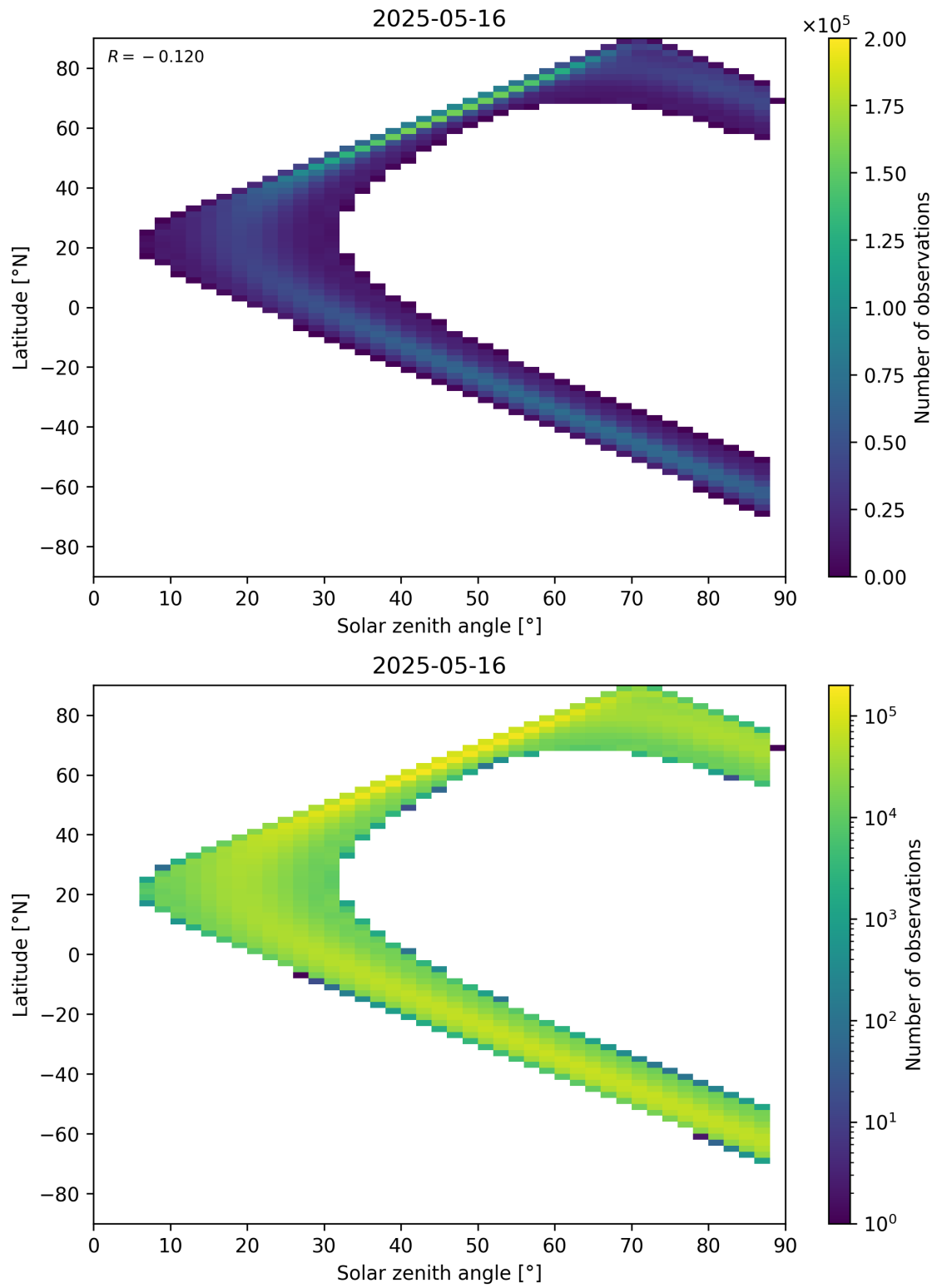
Figure 113: Scatter density plot of “Solar zenith angle” against “Latitude” for 2025-05-15 to 2025-05-17.
