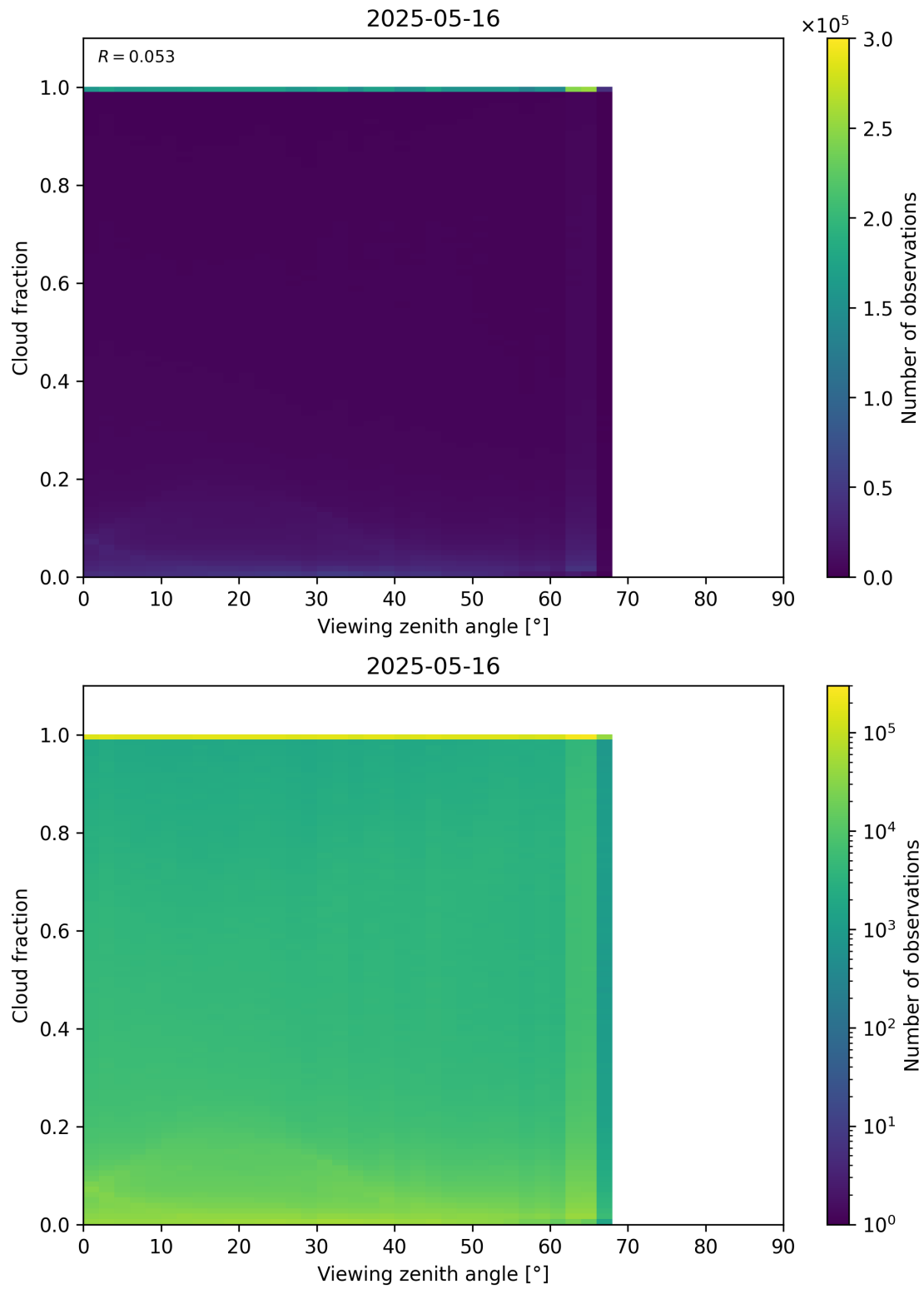
Figure 120: Scatter density plot of “Viewing zenith angle” against “Cloud fraction” for 2025-05-15 to 2025-05-17.
