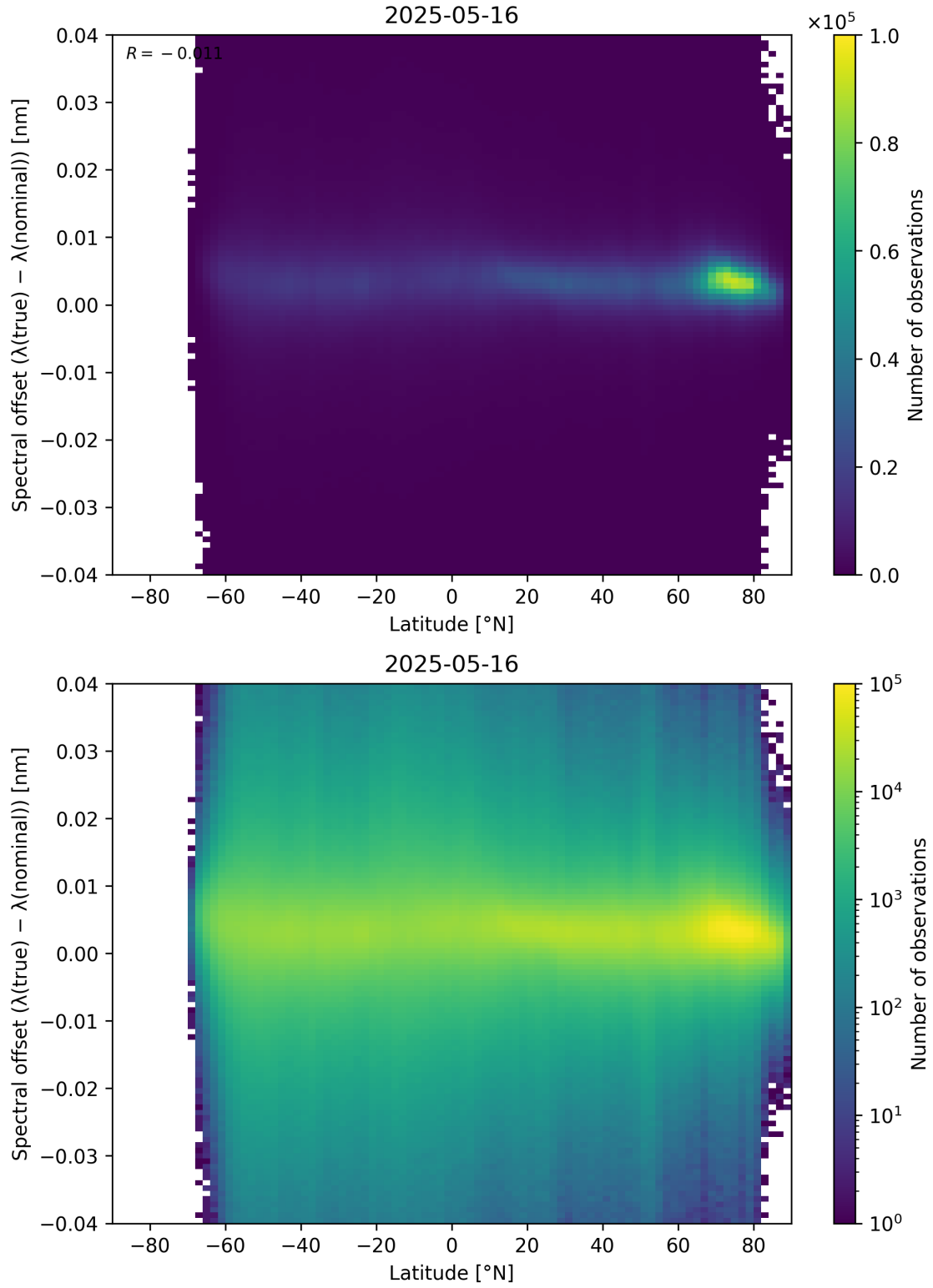
Figure 96: Scatter density plot of “Latitude” against “Spectral offset ( \lambda_{\text{true}} - \lambda_{\text{nominal}} )” for 2025-05-15 to 2025-05-17.
