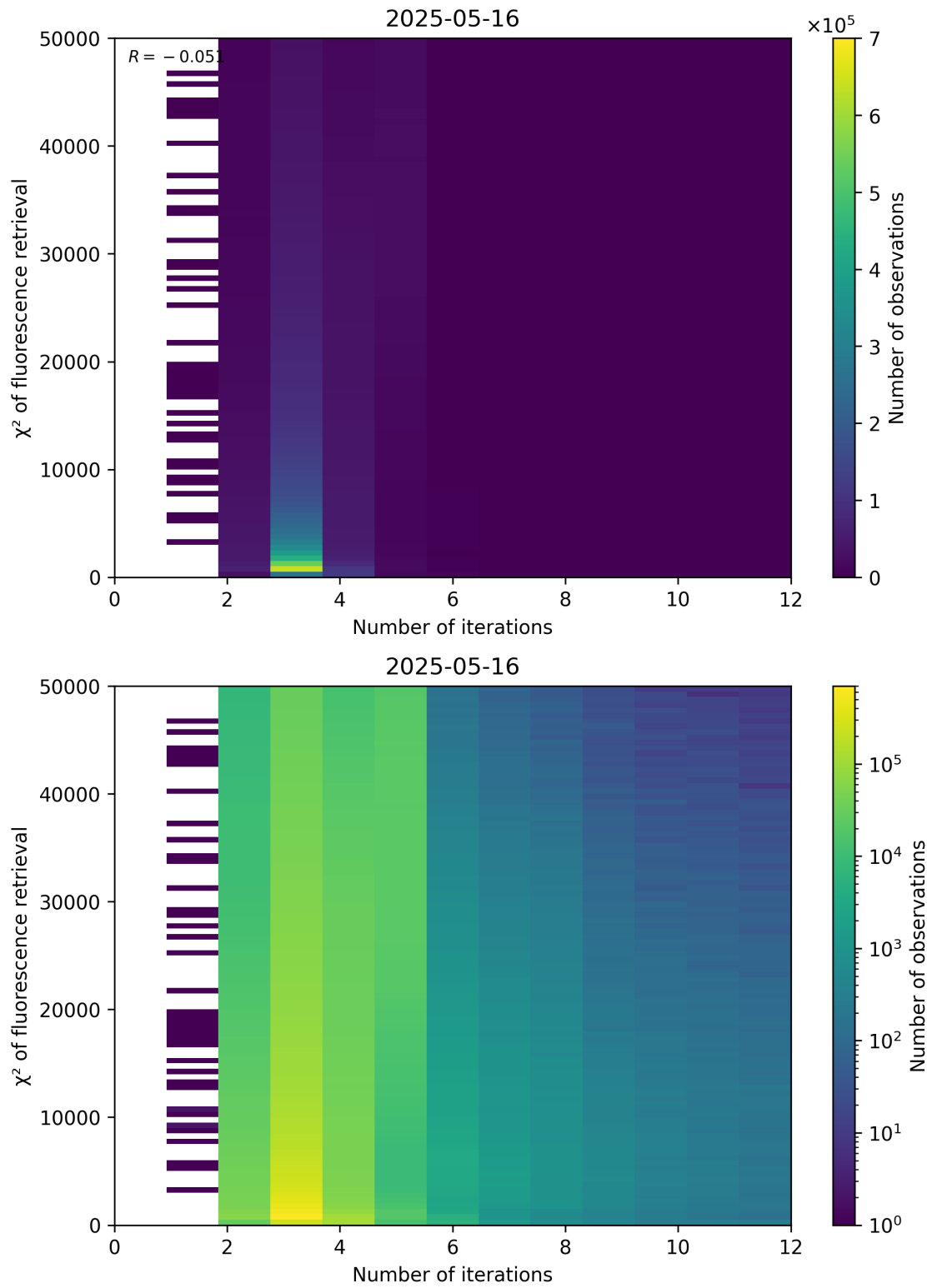
Figure 97: Scatter density plot of “Number of iterations” against “ \chi^2 of fluorescence retrieval” for 2025-05-15 to 2025-05-17.
