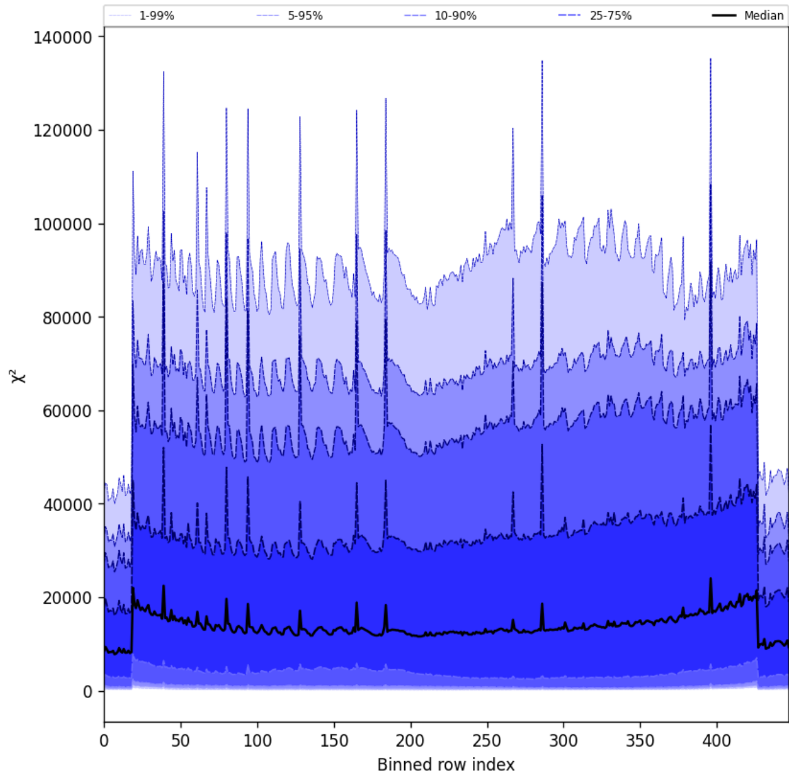
Figure 55: Along track statistics of “ \chi^2 ” for 2025-05-15 to 2025-05-17
