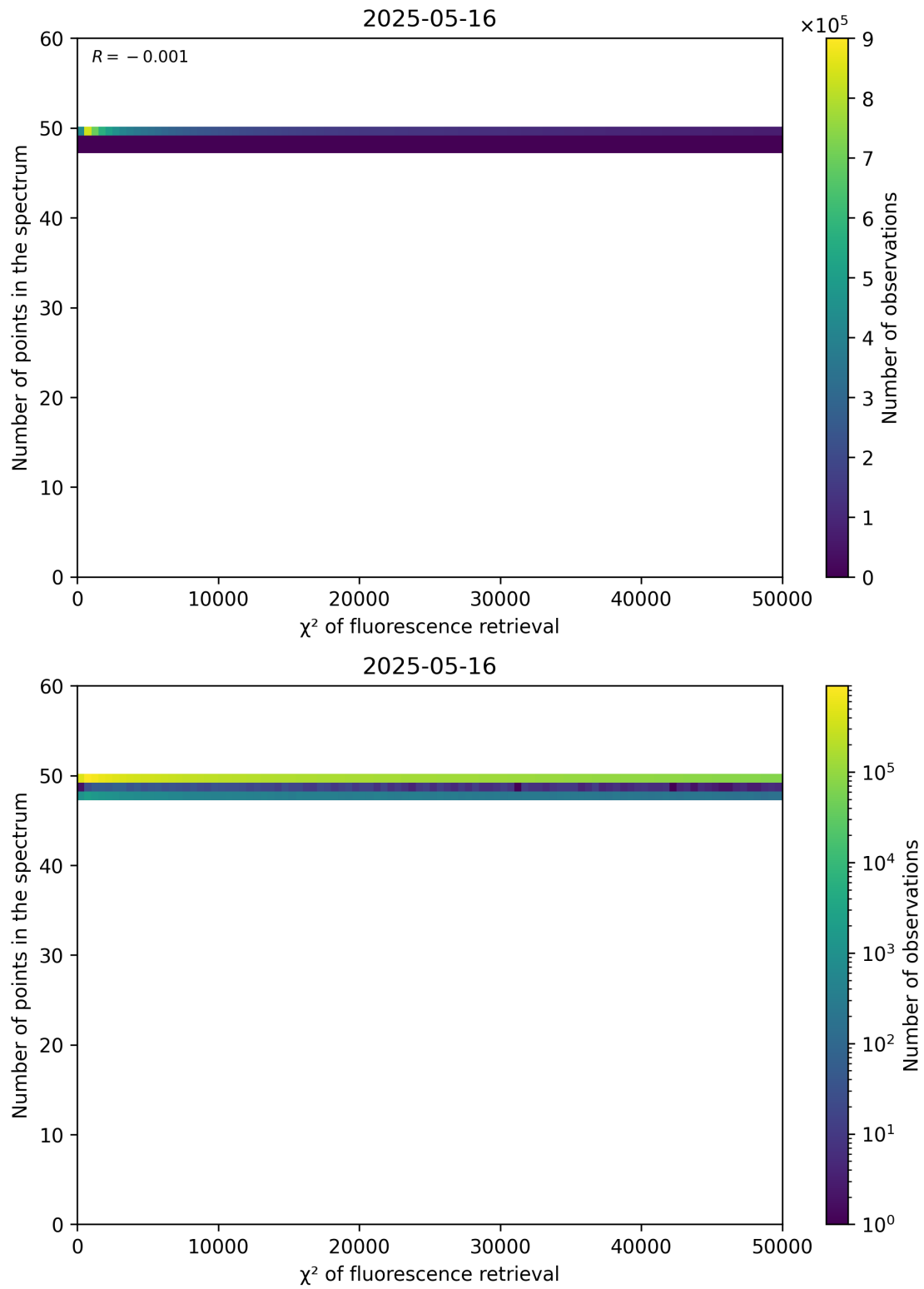
Figure 68: Scatter density plot of “ \chi^2 of fluorescence retrieval” against “Number of points in the spectrum” for 2025-05-15 to 2025-05-17.
