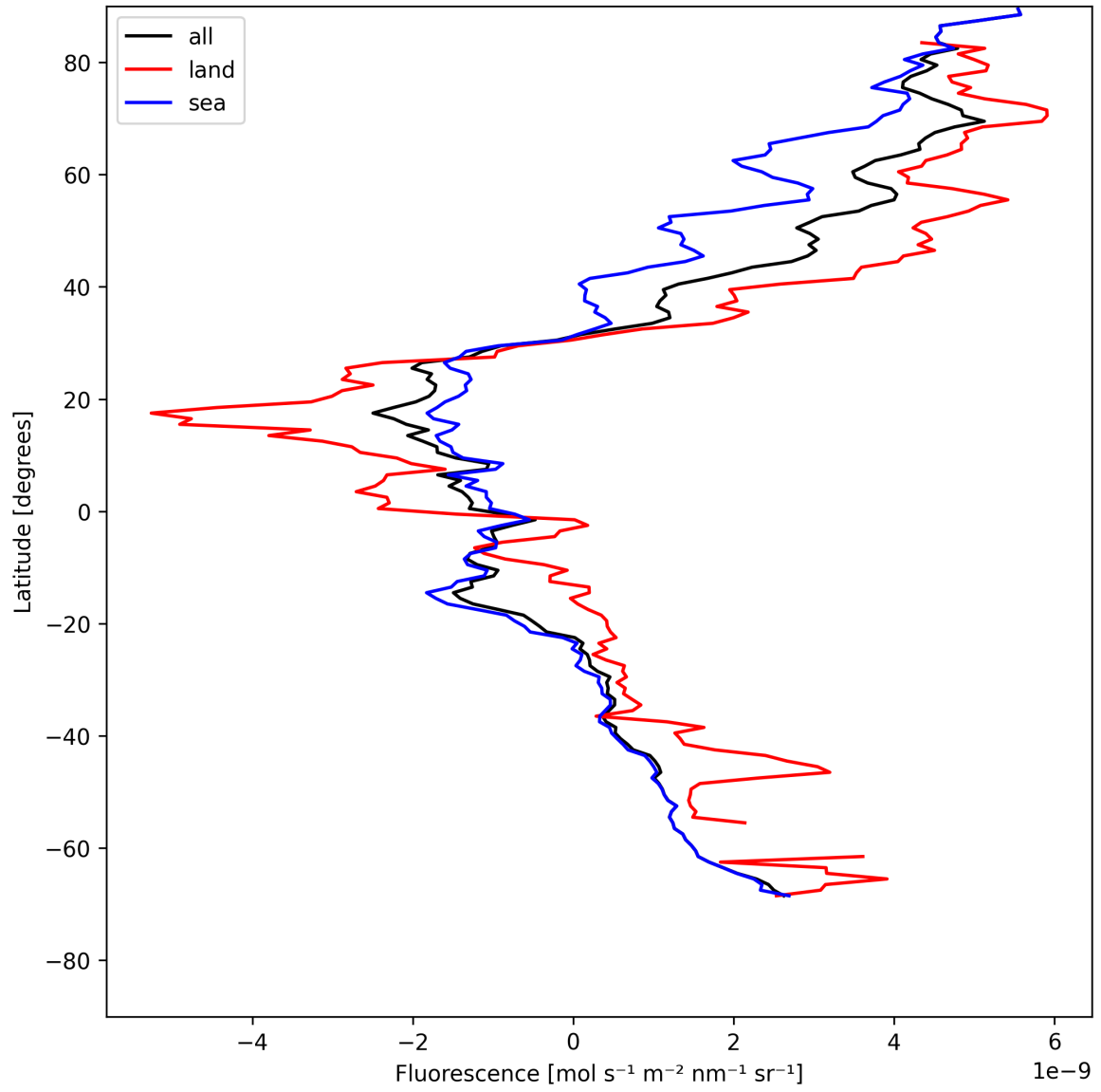
Figure 23: Zonal average of “Fluorescence” for 2025-05-15 to 2025-05-17.
