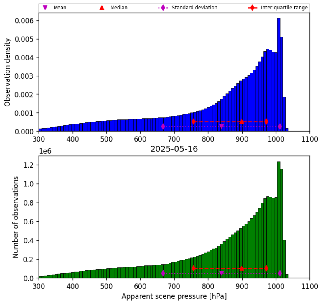
Figure 36: Histogram of “Apparent scene pressure” for 2025-05-15 to 2025-05-17
