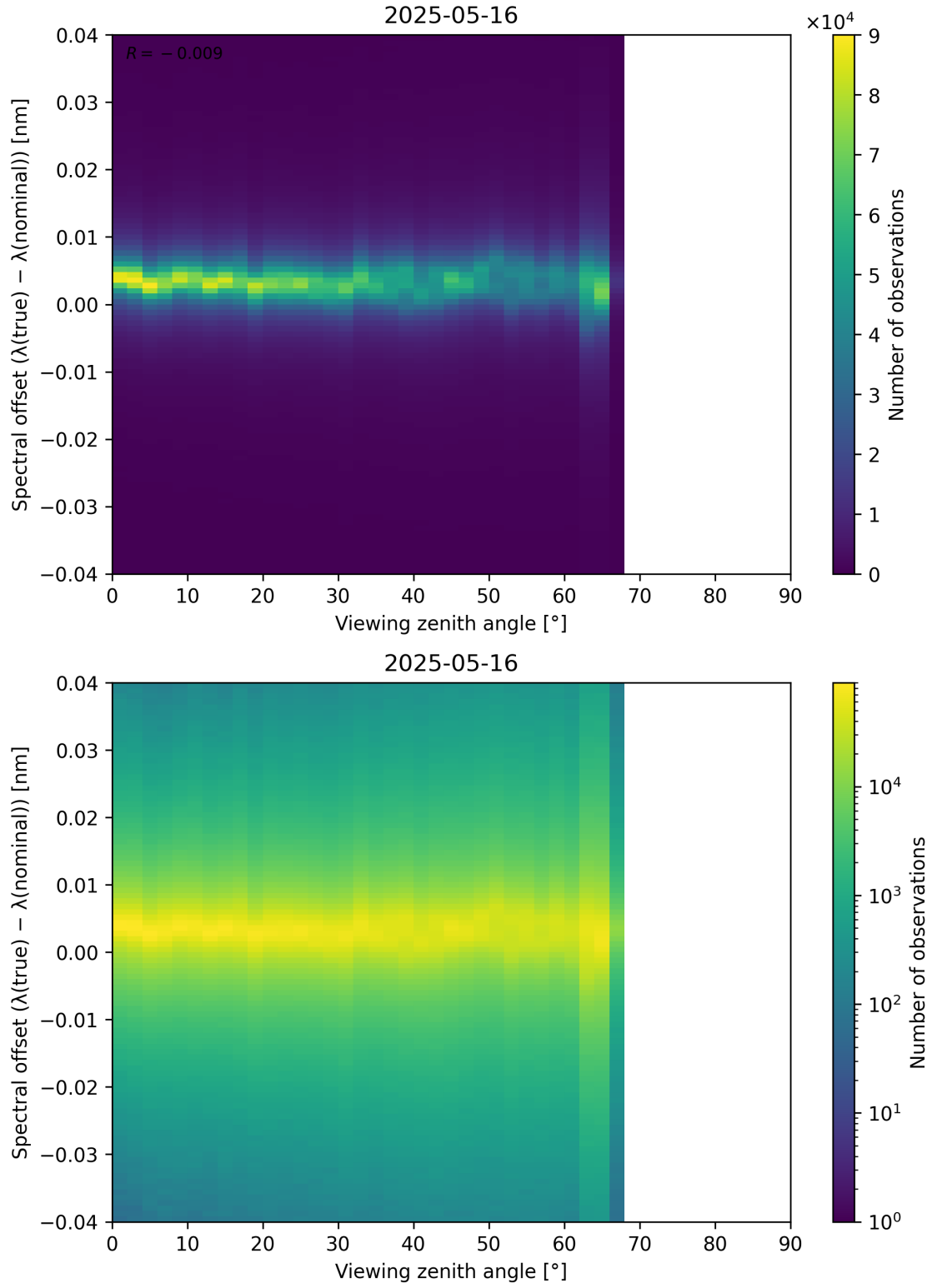
Figure 128: Scatter density plot of “Viewing zenith angle” against “Spectral offset ( \lambda_{\text{true}} - \lambda_{\text{nominal}} )” for 2025-05-15 to 2025-05-17.
