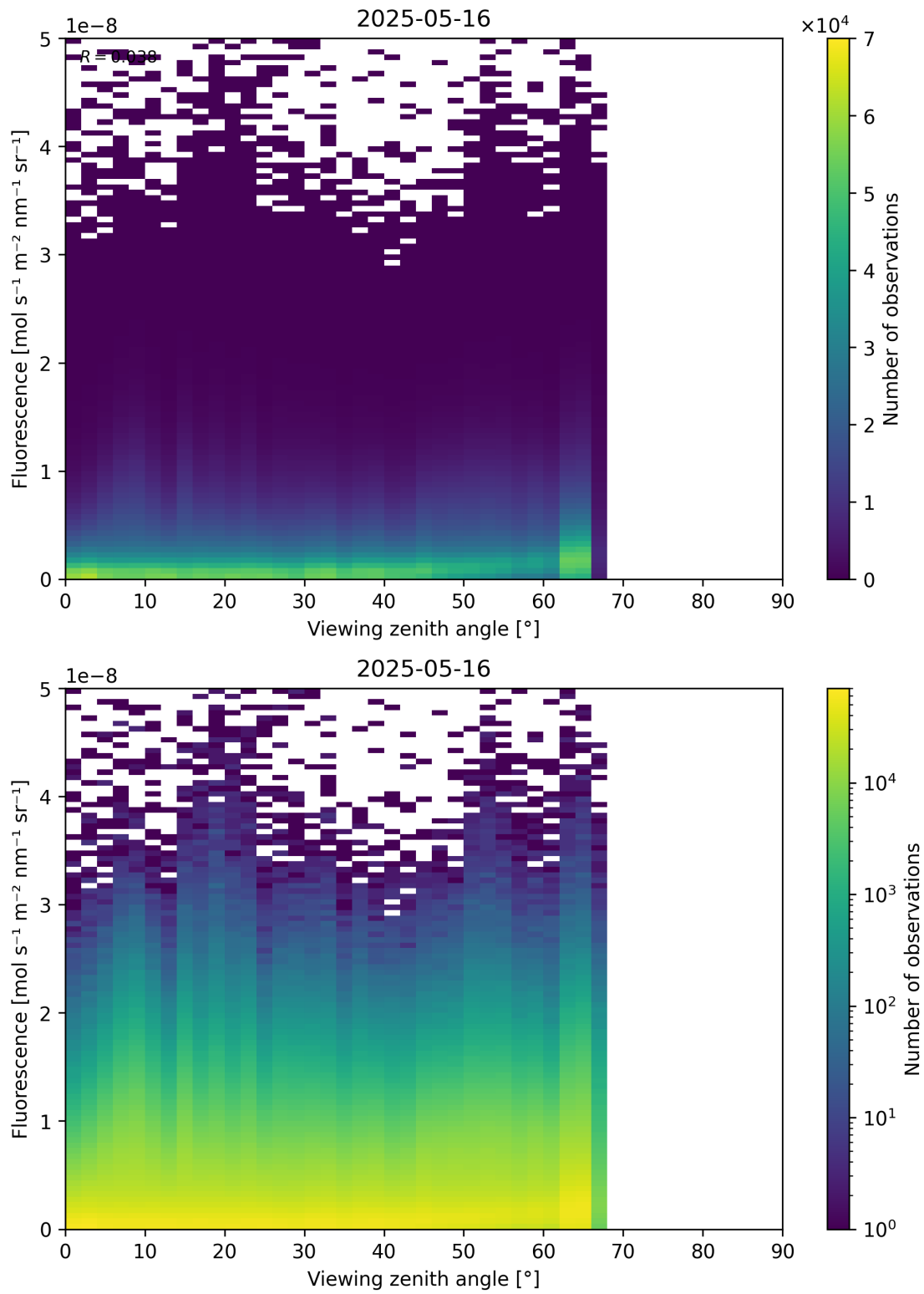
Figure 122: Scatter density plot of “Viewing zenith angle” against “Fluorescence” for 2025-05-15 to 2025-05-17.
