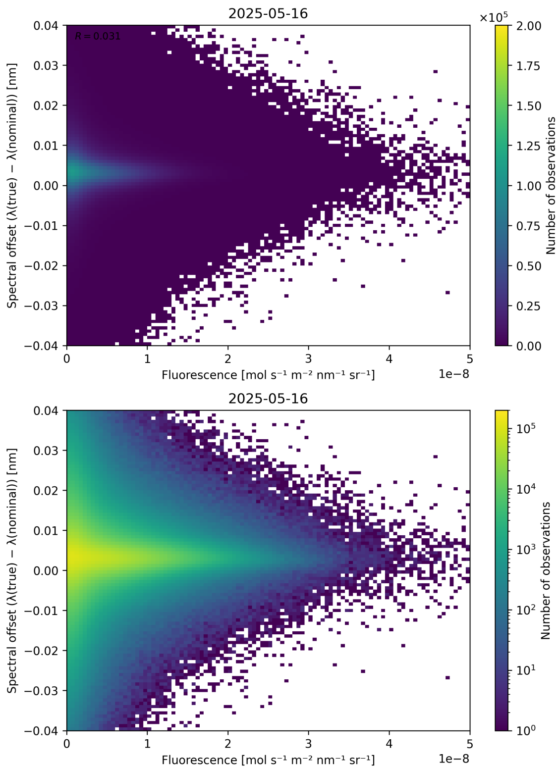
Figure 87: Scatter density plot of “Fluorescence” against “Spectral offset ( \lambda_{\text{true}} - \lambda_{\text{nominal}} )” for 2025-05-15 to 2025-05-17.
