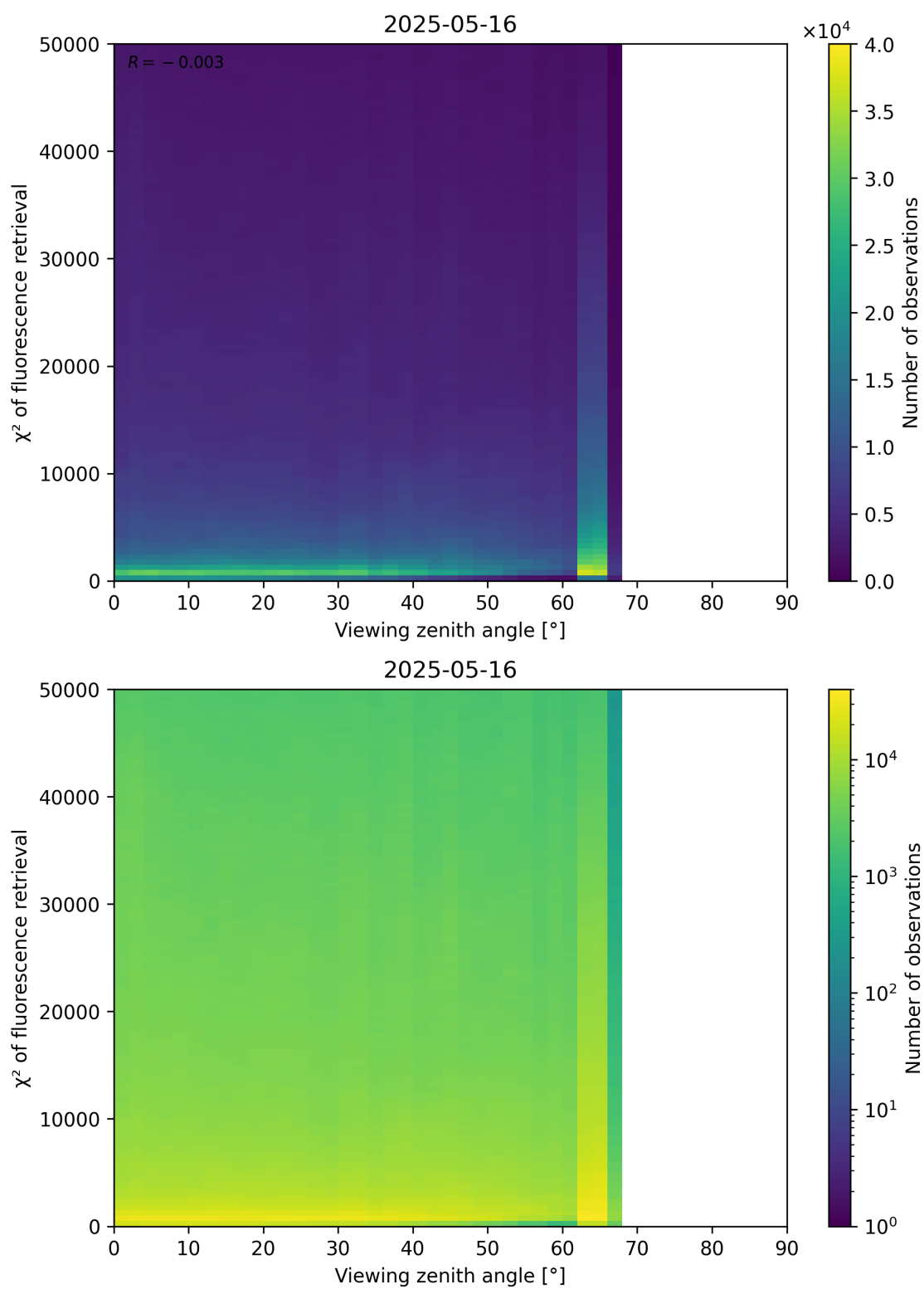
Figure 119: Scatter density plot of “Viewing zenith angle” against “ \chi^2 of fluorescence retrieval” for 2025-05-15 to 2025-05-17.
