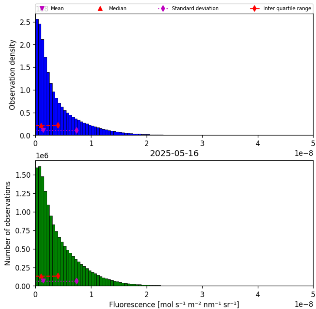
Figure 40: Histogram of “Fluorescence” for 2025-05-15 to 2025-05-17
