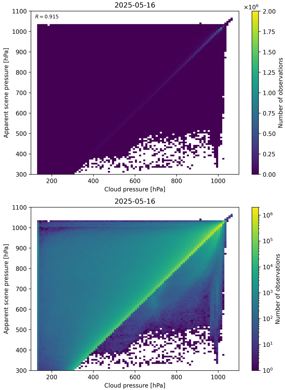
Figure 77: Scatter density plot of “Cloud pressure” against “Apparent scene pressure” for 2025-05-15 to 2025-05-17.
