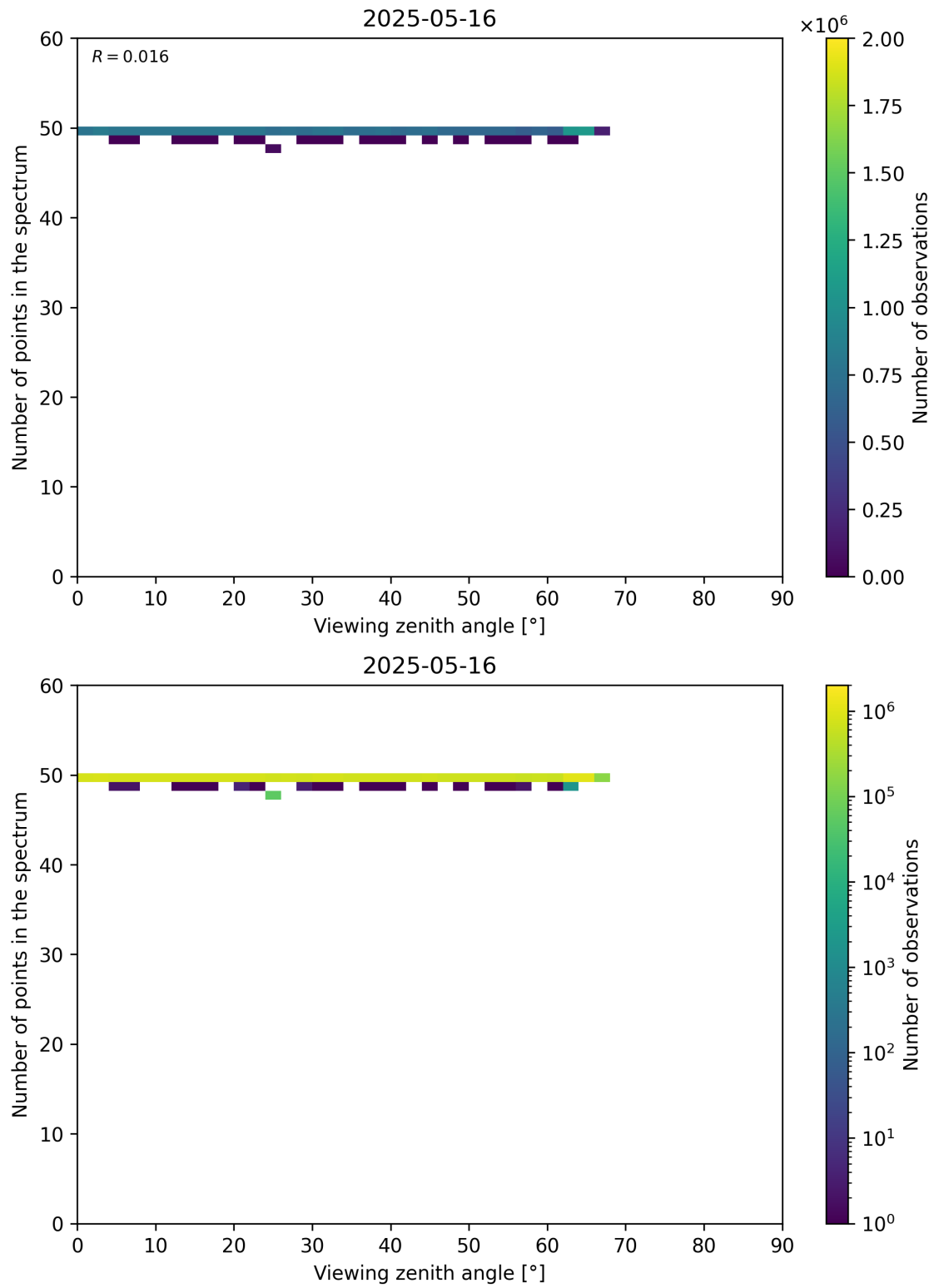
Figure 125: Scatter density plot of “Viewing zenith angle” against “Number of points in the spectrum” for 2025-05-15 to 2025-05-17.
