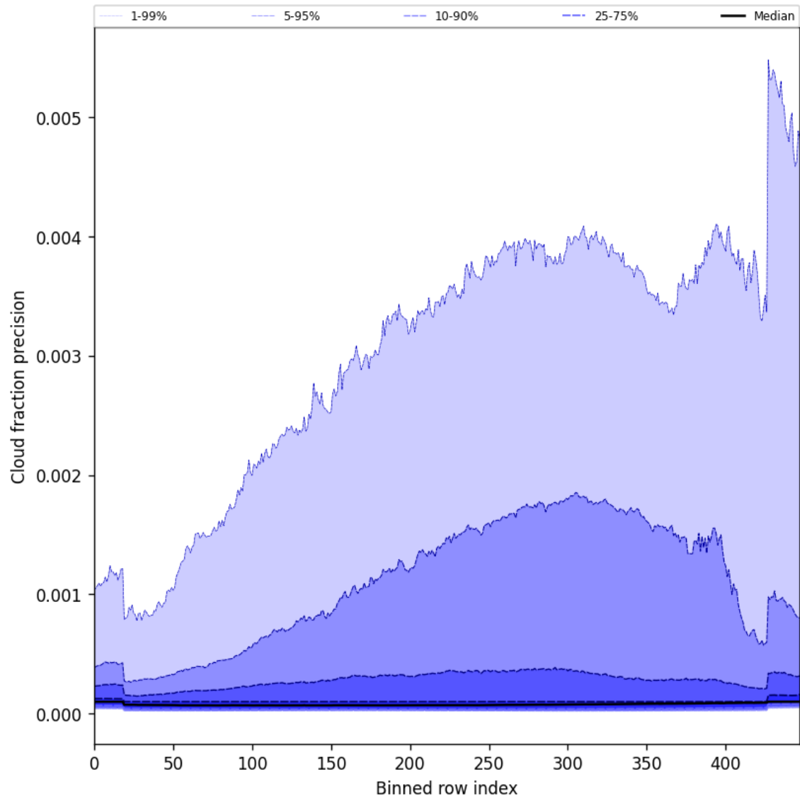
Figure 50: Along track statistics of “Cloud fraction precision” for 2025-05-15 to 2025-05-17
