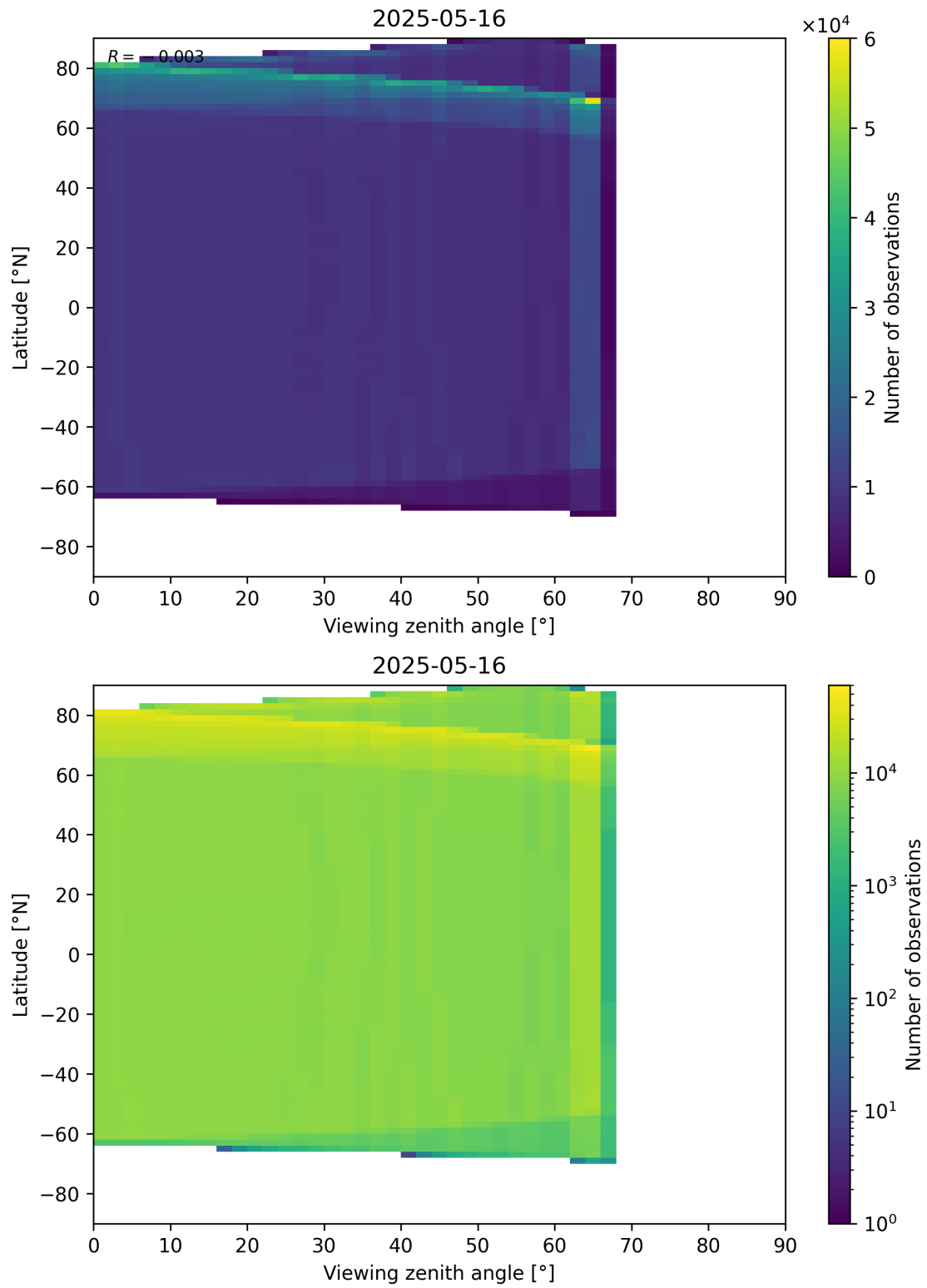
Figure 123: Scatter density plot of “Viewing zenith angle” against “Latitude” for 2025-05-15 to 2025-05-17.
