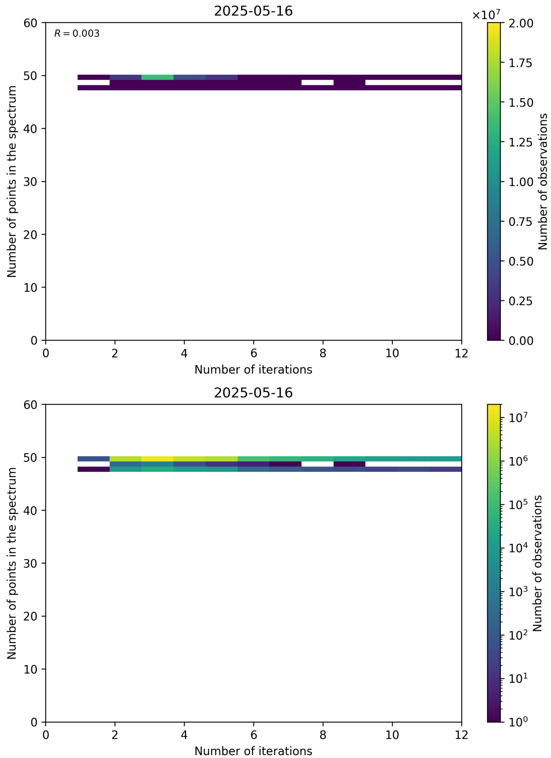
Figure 99: Scatter density plot of “Number of iterations” against “Number of points in the spectrum” for 2025-05-15 to 2025-05-17.
