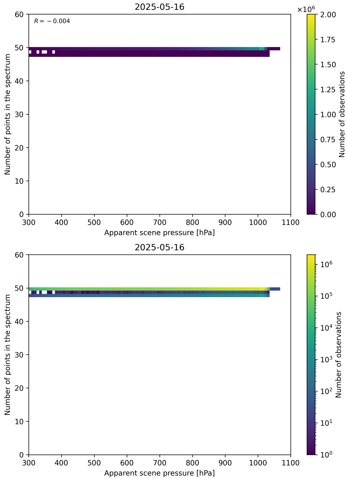
Figure 66: Scatter density plot of “Apparent scene pressure” against “Number of points in the spectrum” for 2025-05-15 to 2025-05-17.
