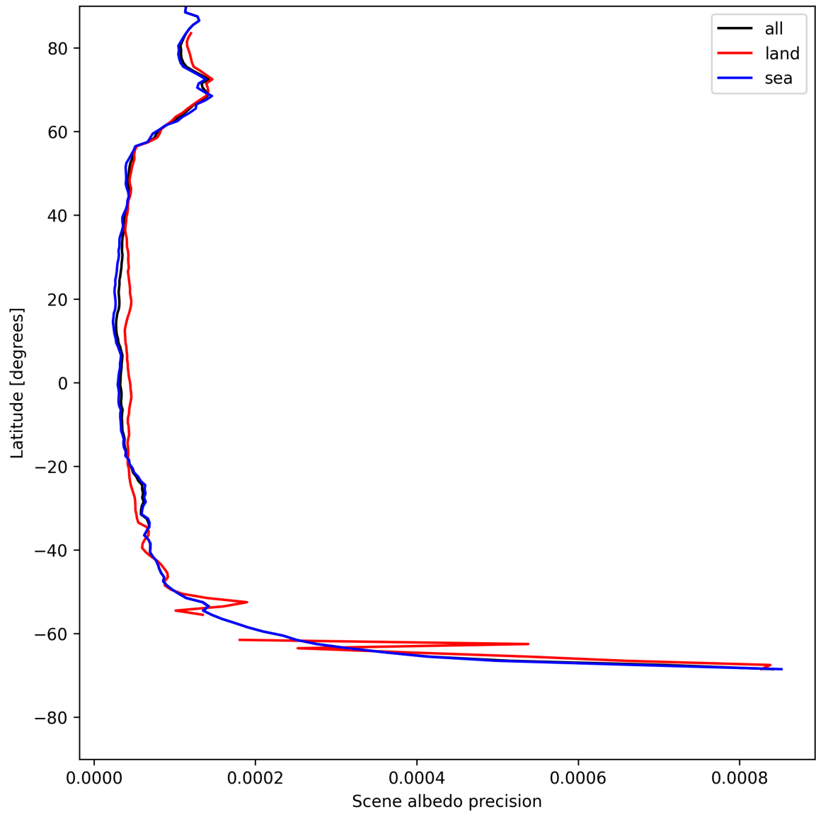
Figure 18: Zonal average of “Scene albedo precision” for 2025-05-15 to 2025-05-17.
