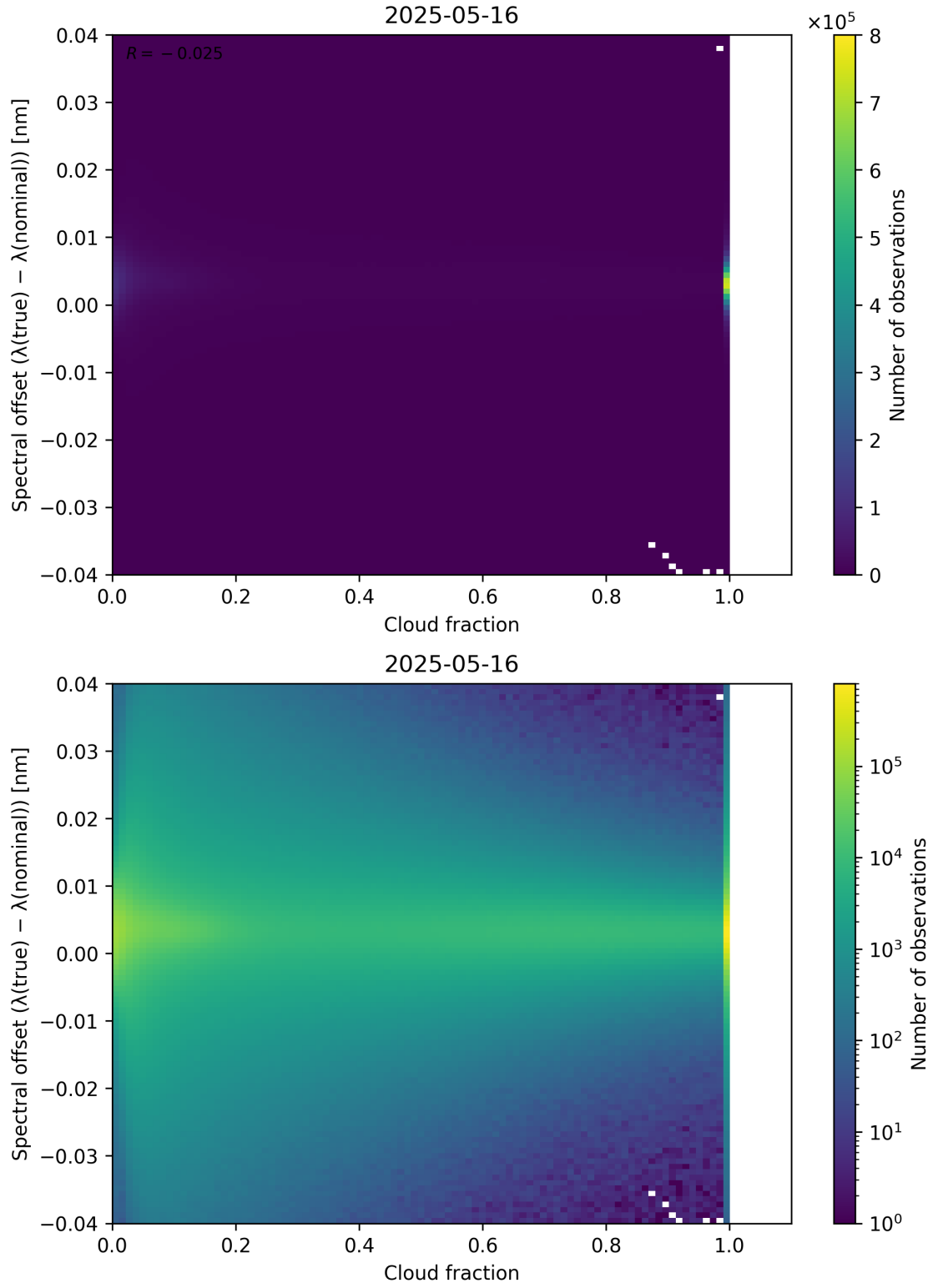
Figure 76: Scatter density plot of “Cloud fraction” against “Spectral offset ( \lambda_{\text{true}} - \lambda_{\text{nominal}} )” for 2025-05-15 to 2025-05-17.
