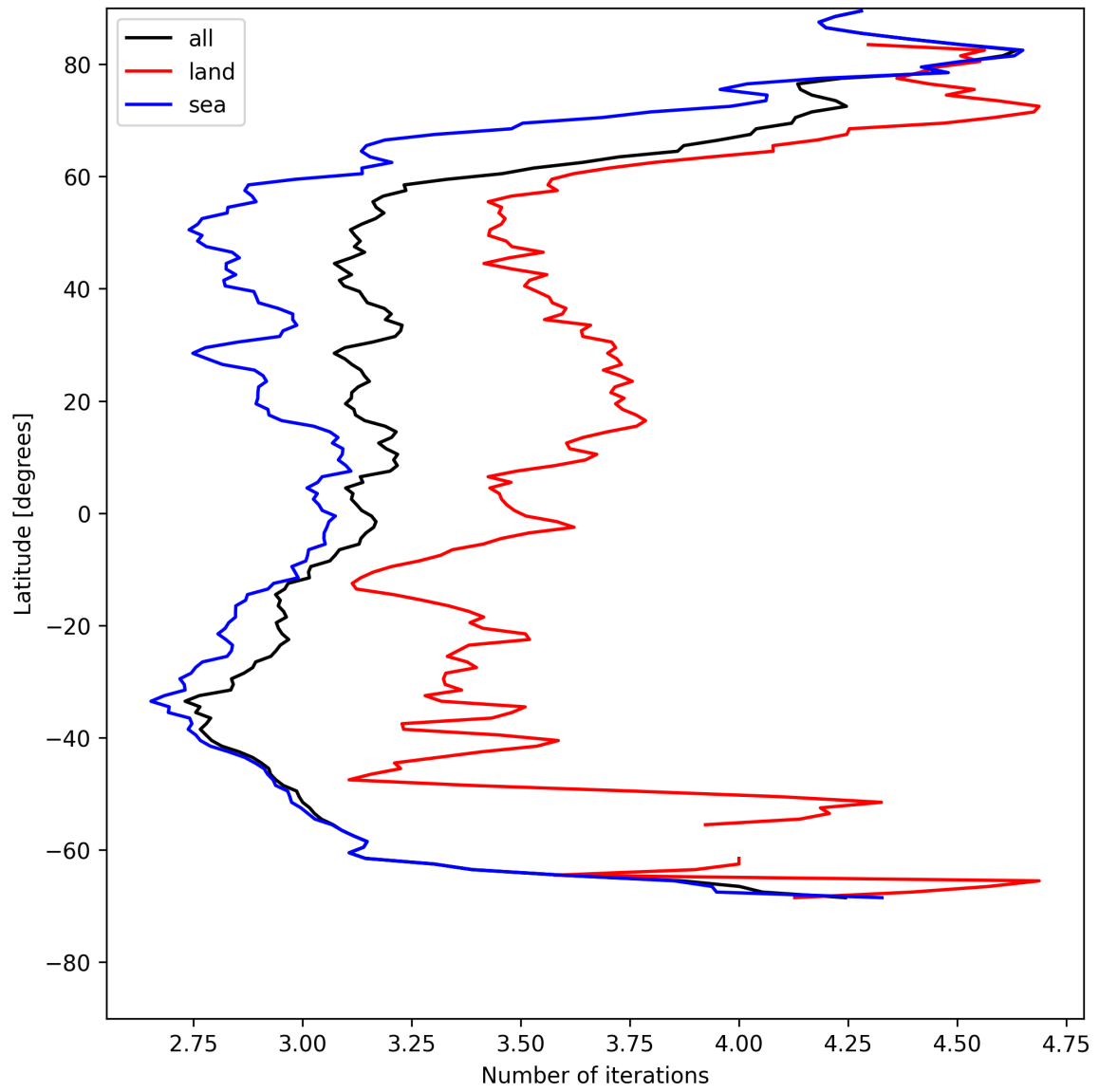
Figure 22: Zonal average of “Number of iterations” for 2025-05-15 to 2025-05-17.
