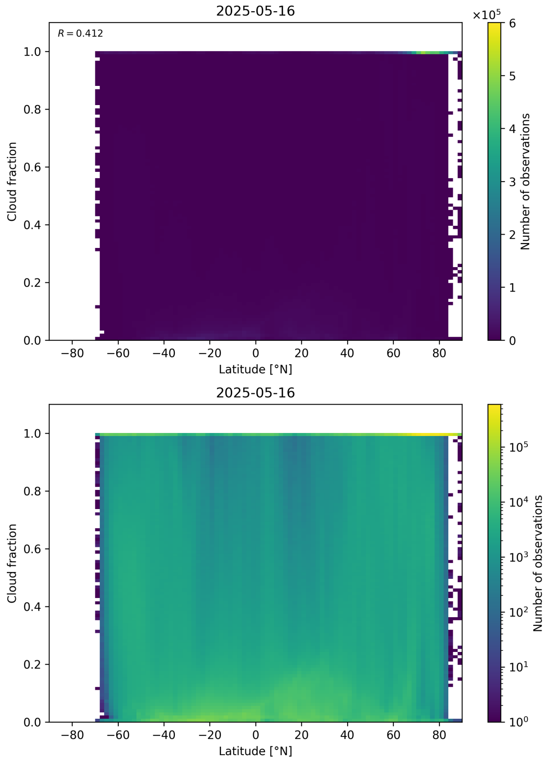
Figure 90: Scatter density plot of “Latitude” against “Cloud fraction” for 2025-05-15 to 2025-05-17.
