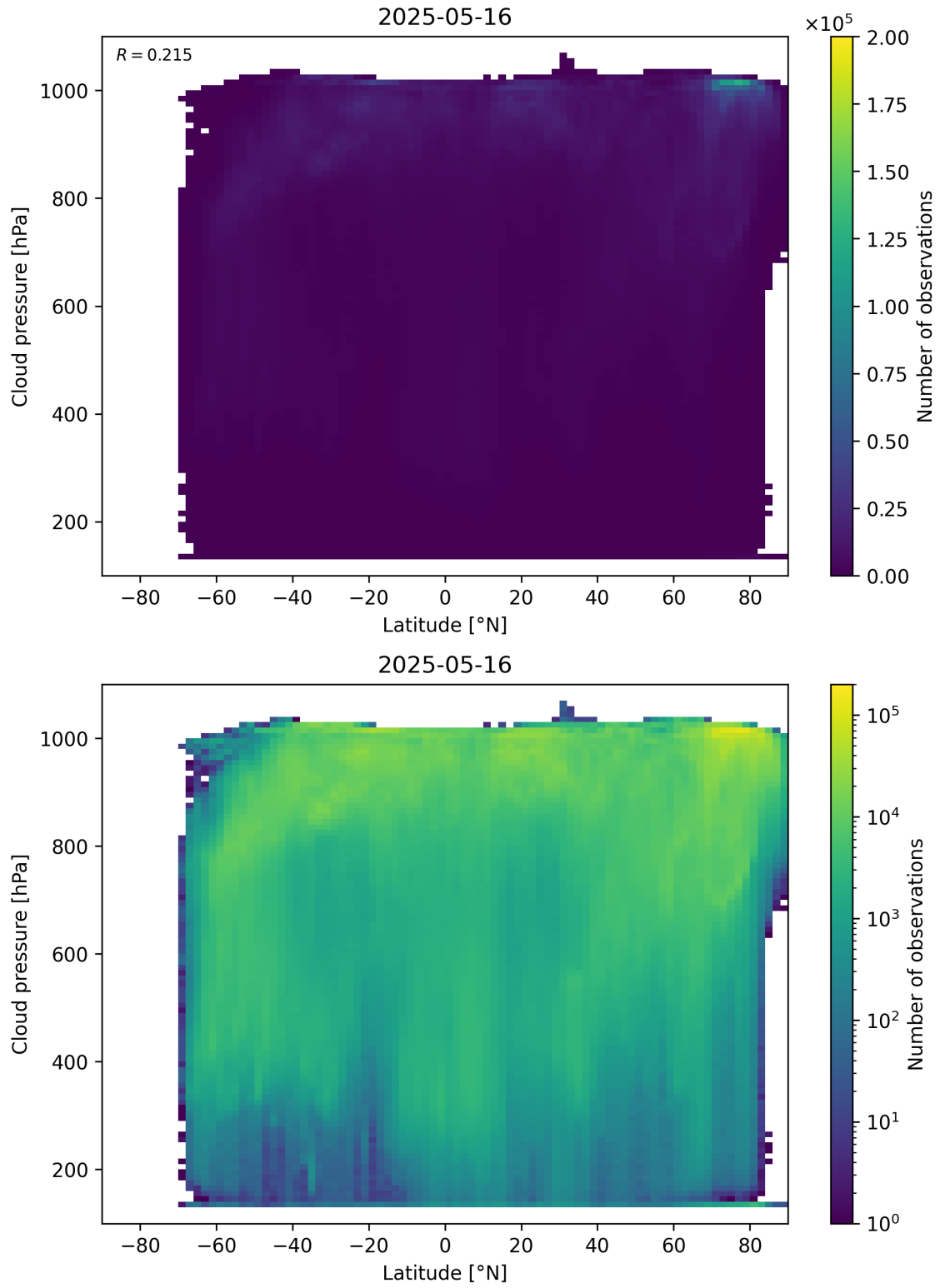
Figure 91: Scatter density plot of “Latitude” against “Cloud pressure” for 2025-05-15 to 2025-05-17.
