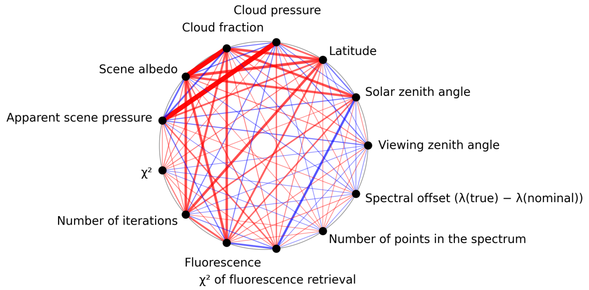
Figure 1: Map of correlation graph for 2025-05-15 to 2025-05-17.
