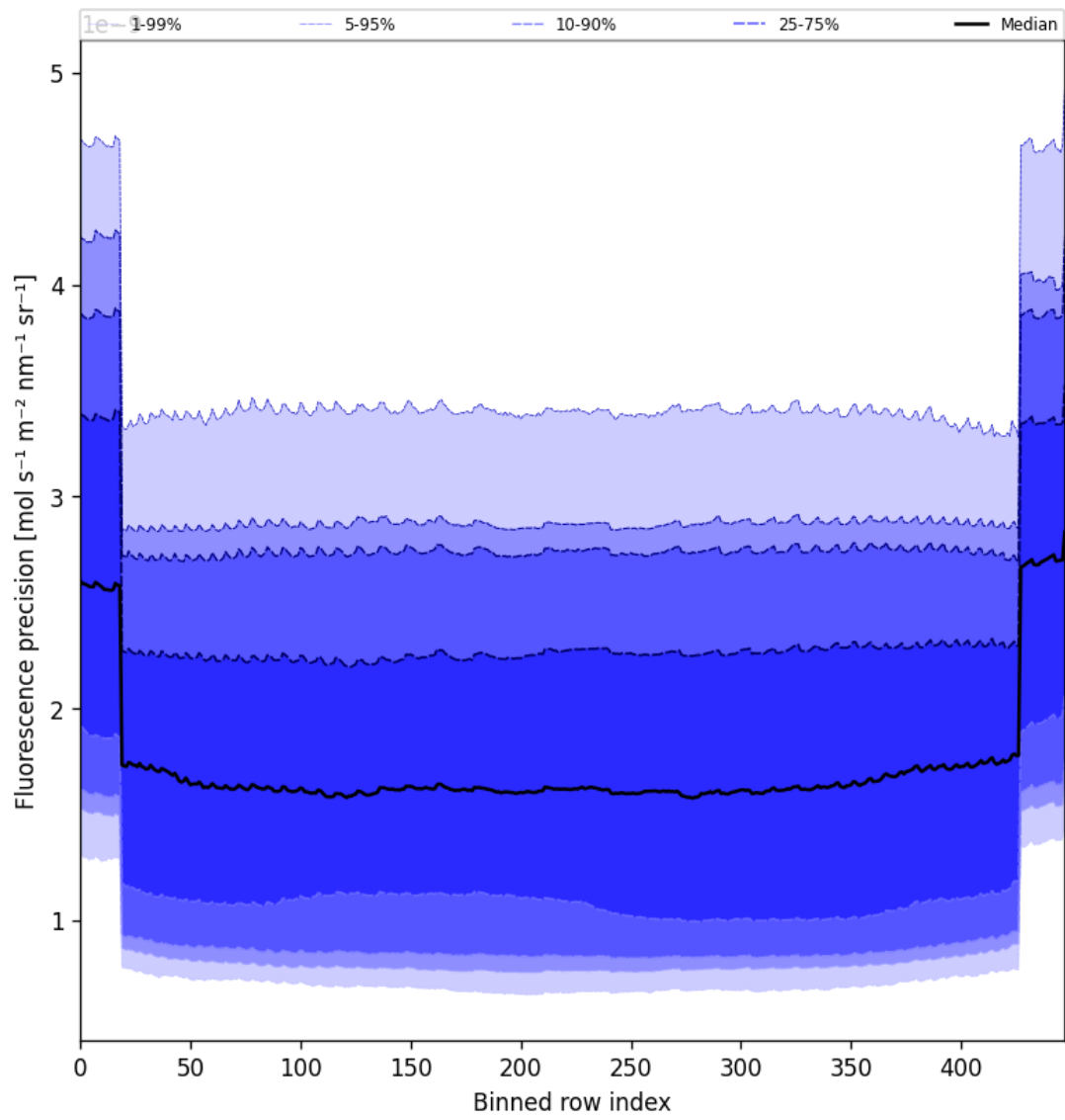
Figure 58: Along track statistics of “Fluorescence precision” for 2025-05-15 to 2025-05-17
