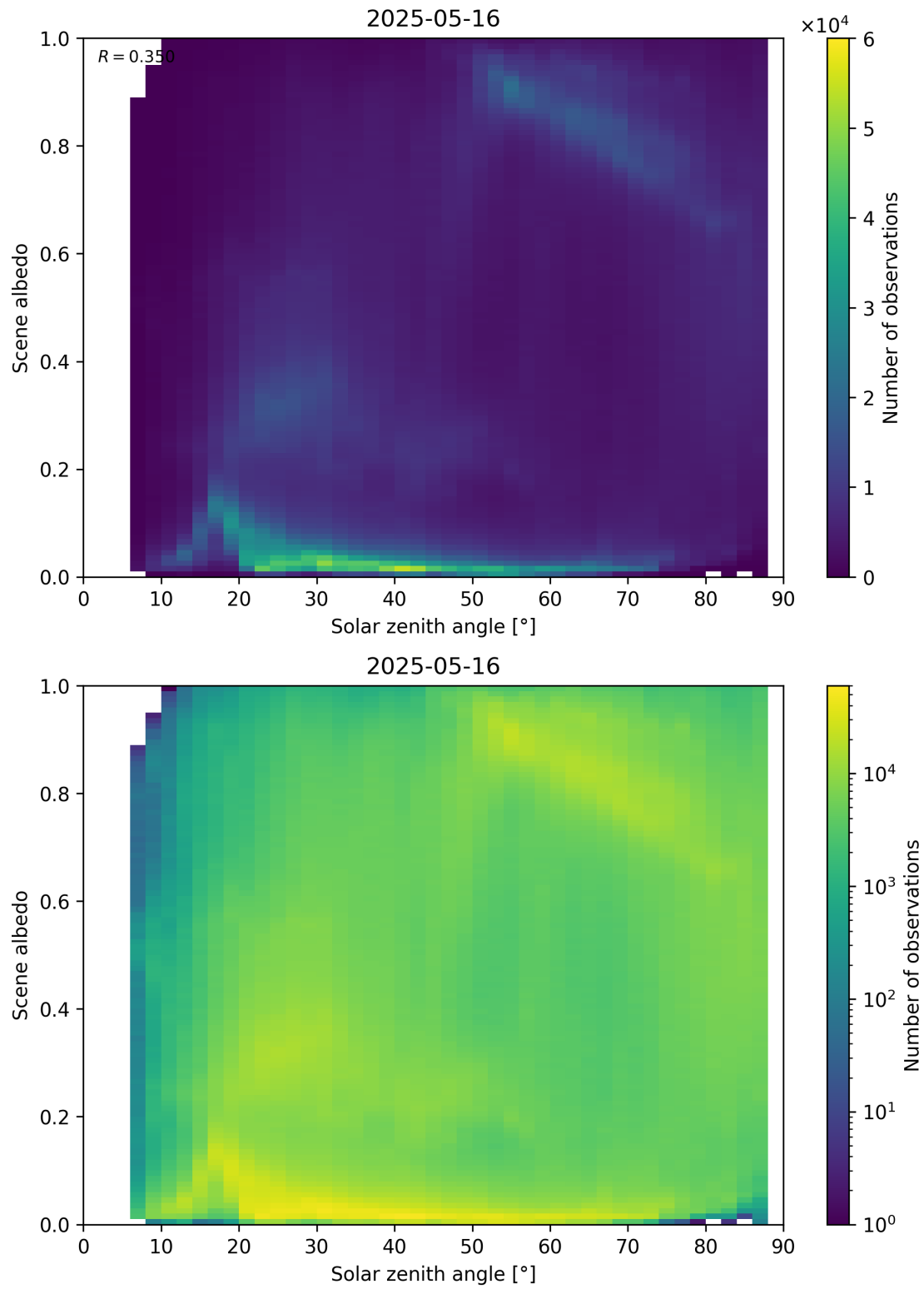
Figure 116: Scatter density plot of “Solar zenith angle” against “Scene albedo” for 2025-05-15 to 2025-05-17.
