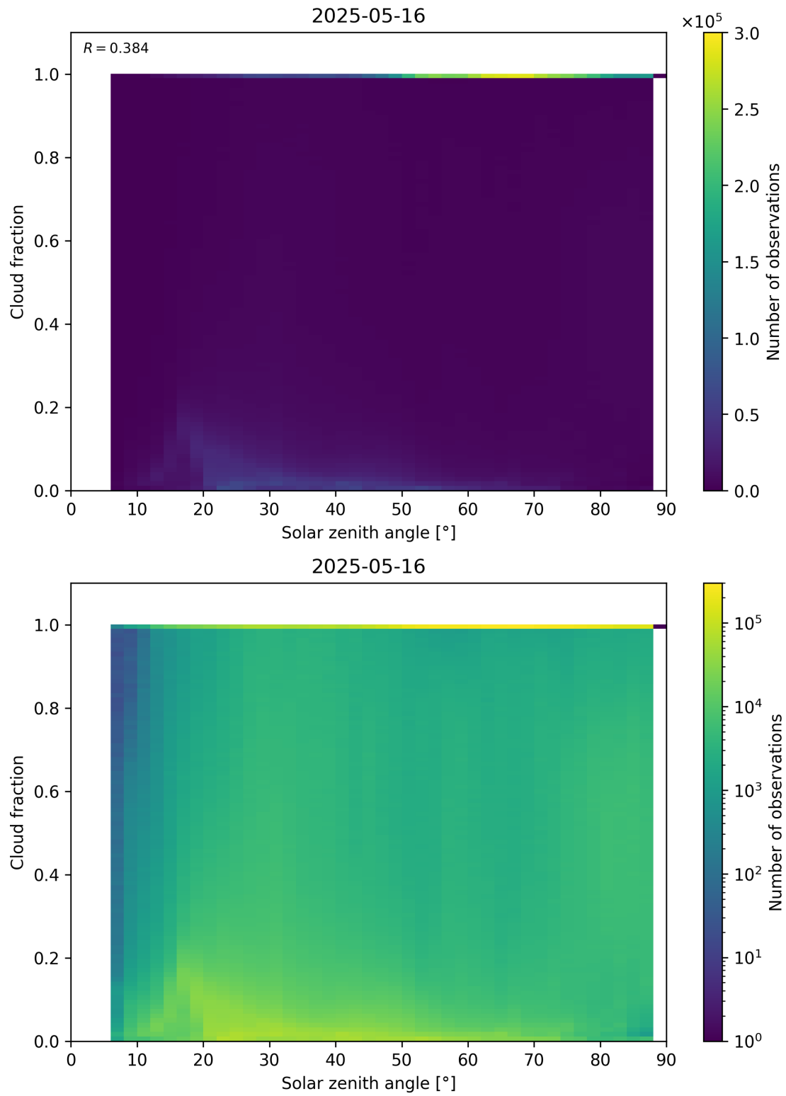
Figure 110: Scatter density plot of “Solar zenith angle” against “Cloud fraction” for 2025-05-15 to 2025-05-17.
