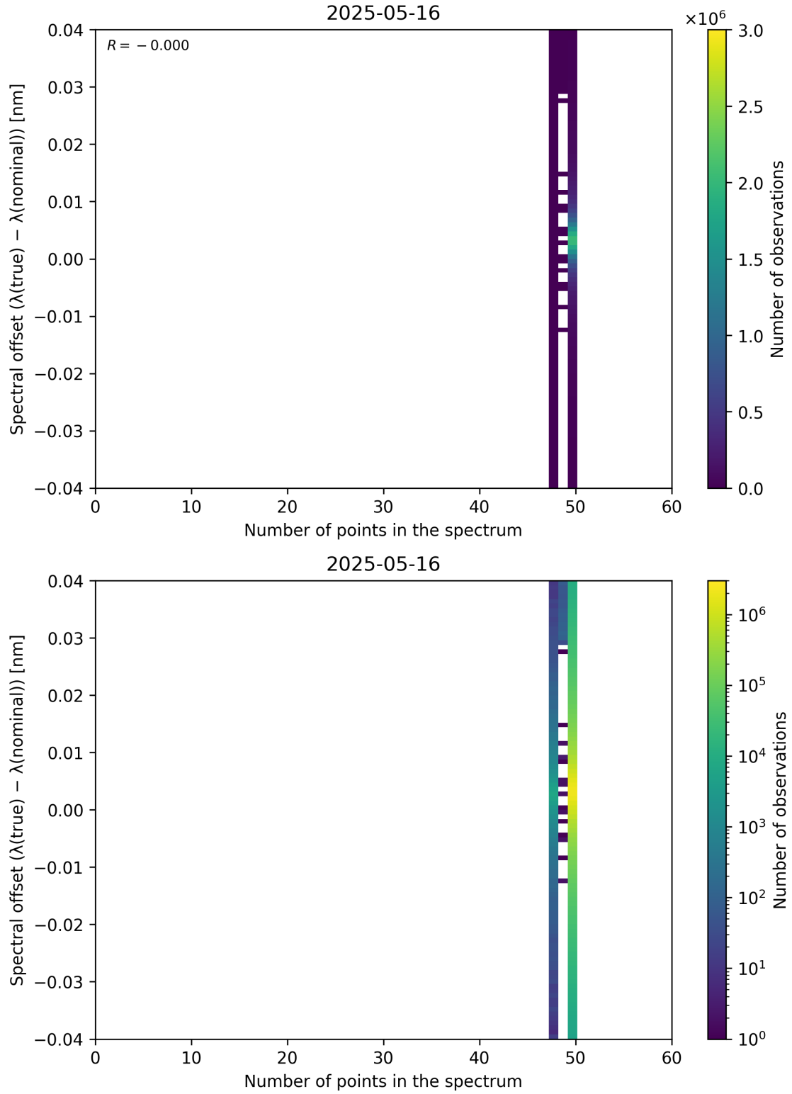
Figure 101: Scatter density plot of “Number of points in the spectrum” against “Spectral offset ( \lambda_{\text{true}} - \lambda_{\text{nominal}} )” for 2025-05-15 to 2025-05-17.
