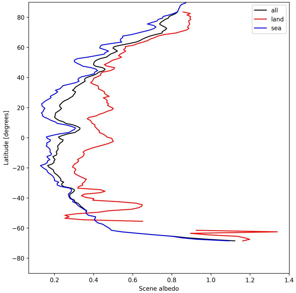
Figure 17: Zonal average of “Scene albedo” for 2025-05-15 to 2025-05-17.
