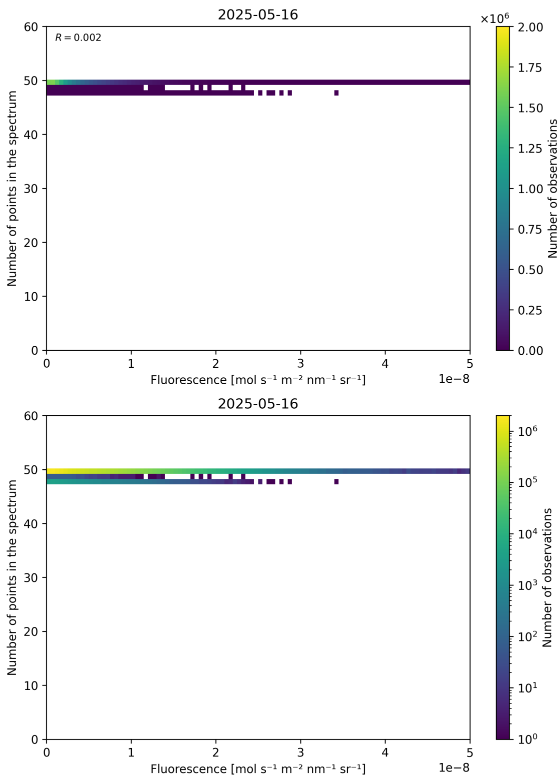
Figure 86: Scatter density plot of “Fluorescence” against “Number of points in the spectrum” for 2025-05-15 to 2025-05-17.
