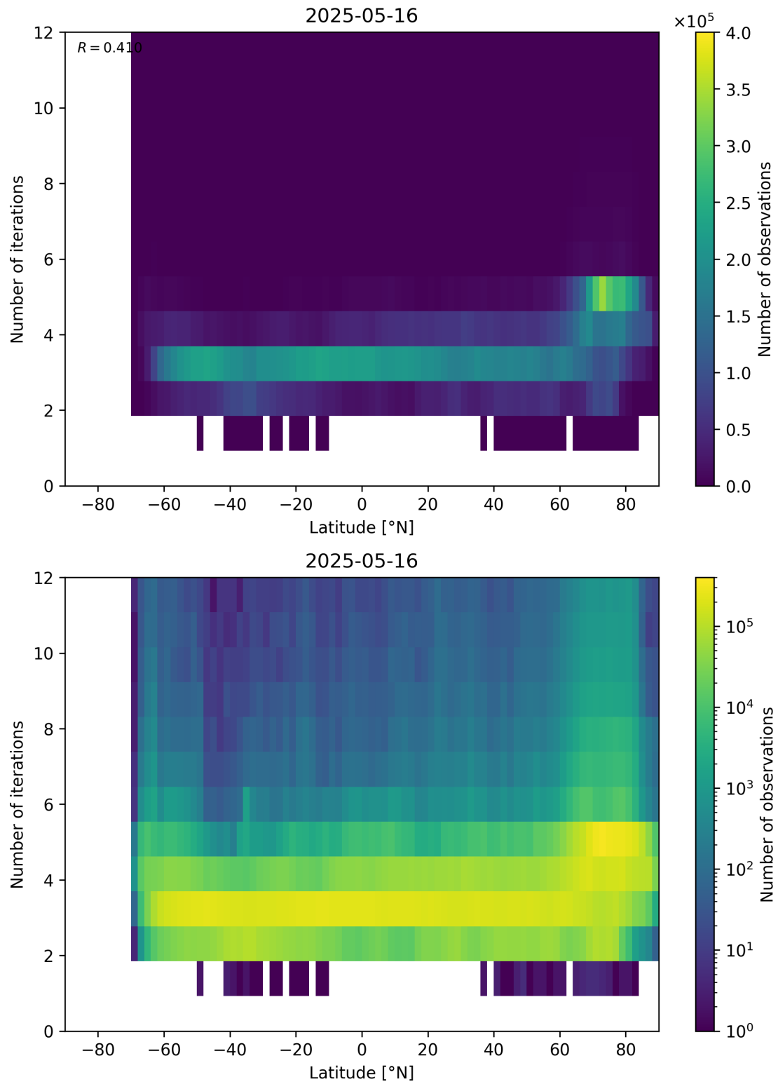
Figure 93: Scatter density plot of “Latitude” against “Number of iterations” for 2025-05-15 to 2025-05-17.
