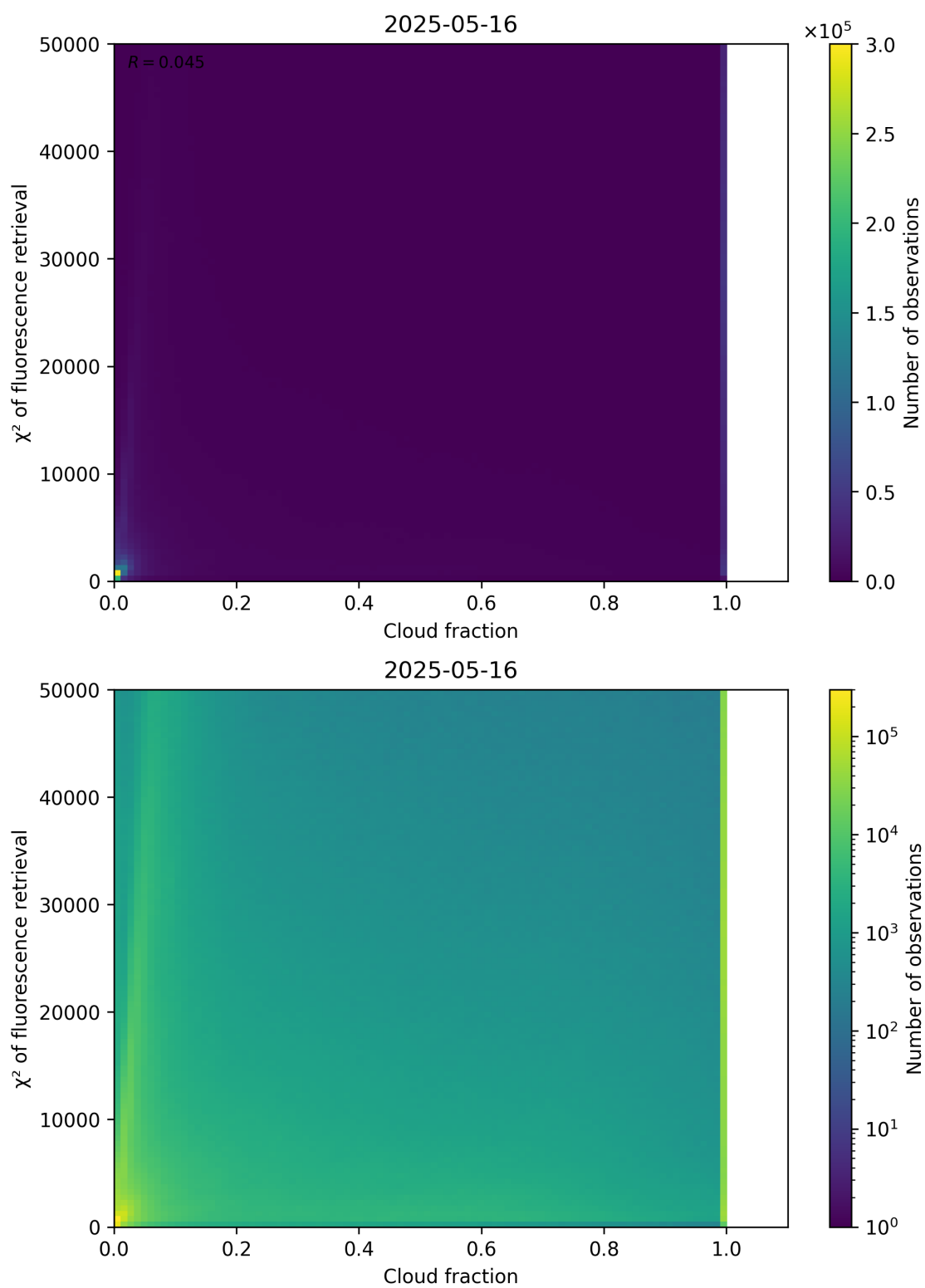
Figure 71: Scatter density plot of “Cloud fraction” against “ \chi^2 of fluorescence retrieval” for 2025-05-15 to 2025-05-17.
