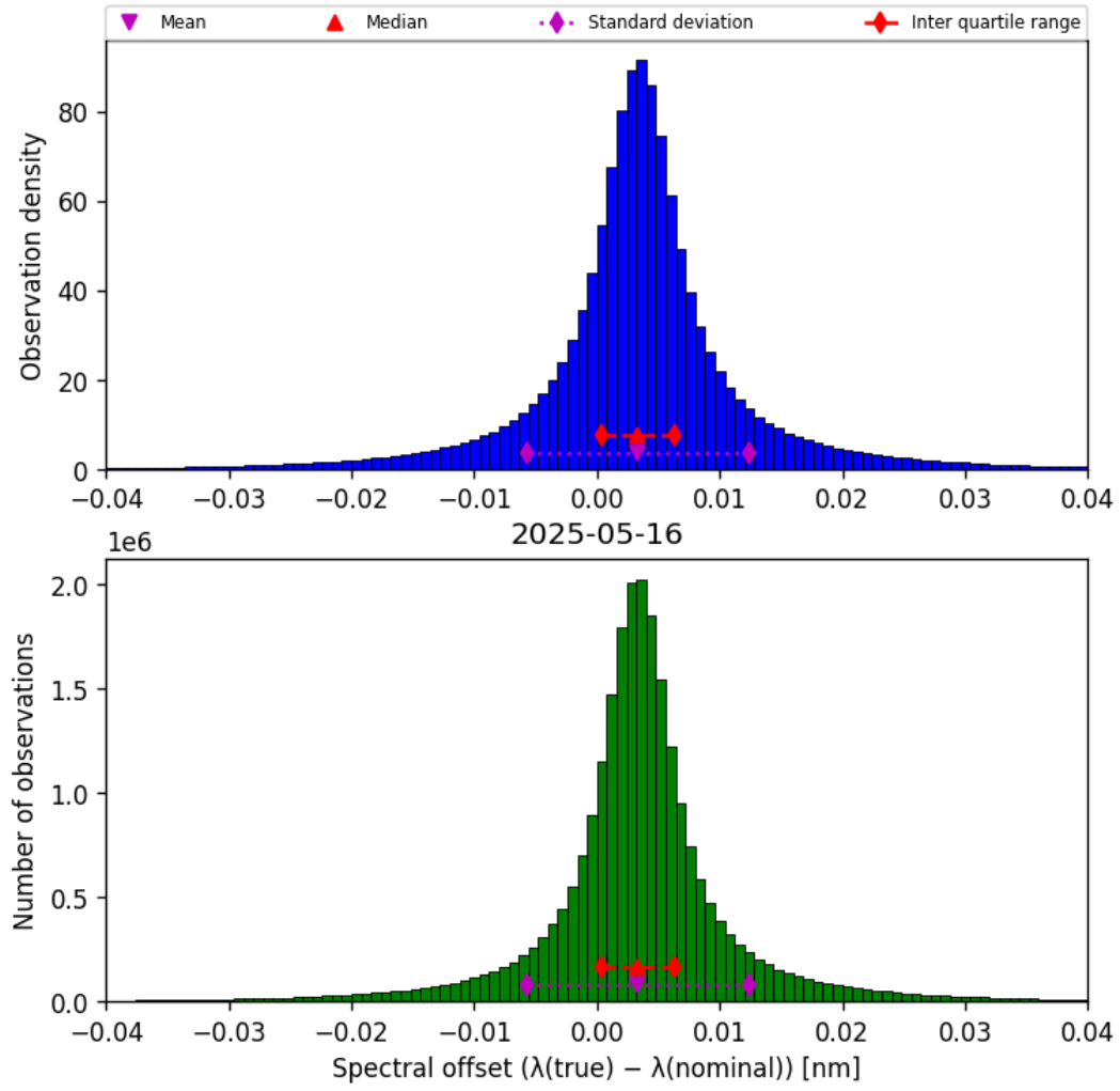
Figure 45: Histogram of “Spectral offset ( \lambda_{\text{true}} - \lambda_{\text{nominal}} )” for 2025-05-15 to 2025-05-17
