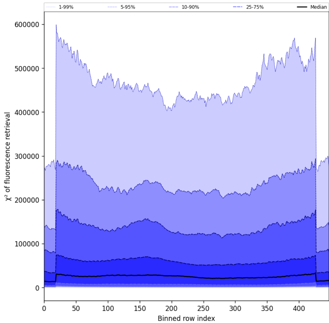
Figure 59: Along track statistics of “ \chi^2 of fluorescence retrieval” for 2025-05-15 to 2025-05-17
