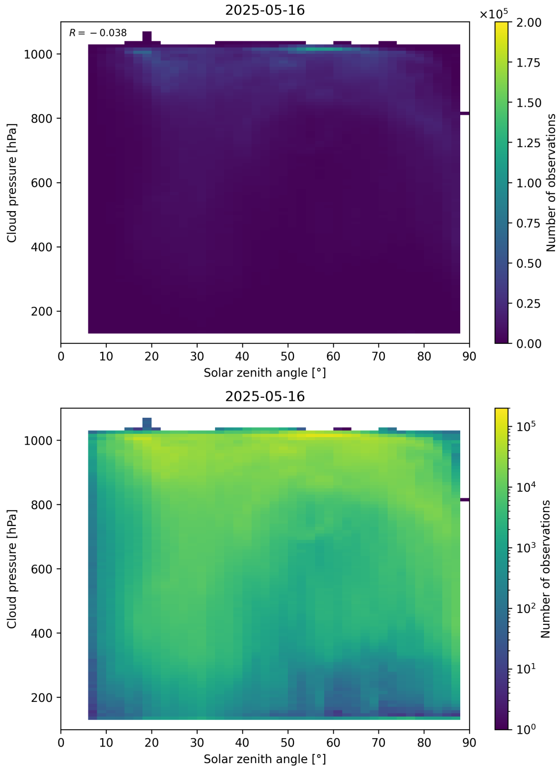
Figure 111: Scatter density plot of “Solar zenith angle” against “Cloud pressure” for 2025-05-15 to 2025-05-17.
