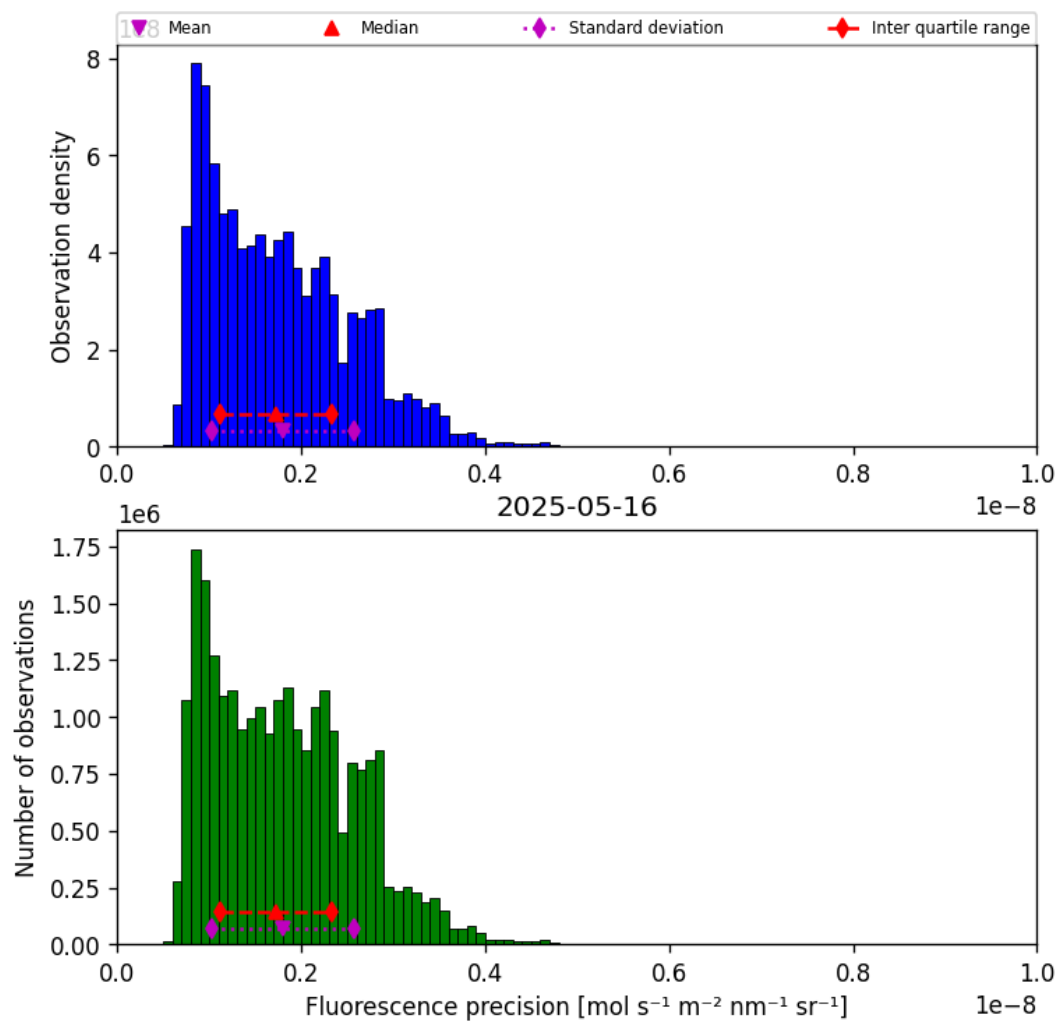
Figure 41: Histogram of “Fluorescence precision” for 2025-05-15 to 2025-05-17
