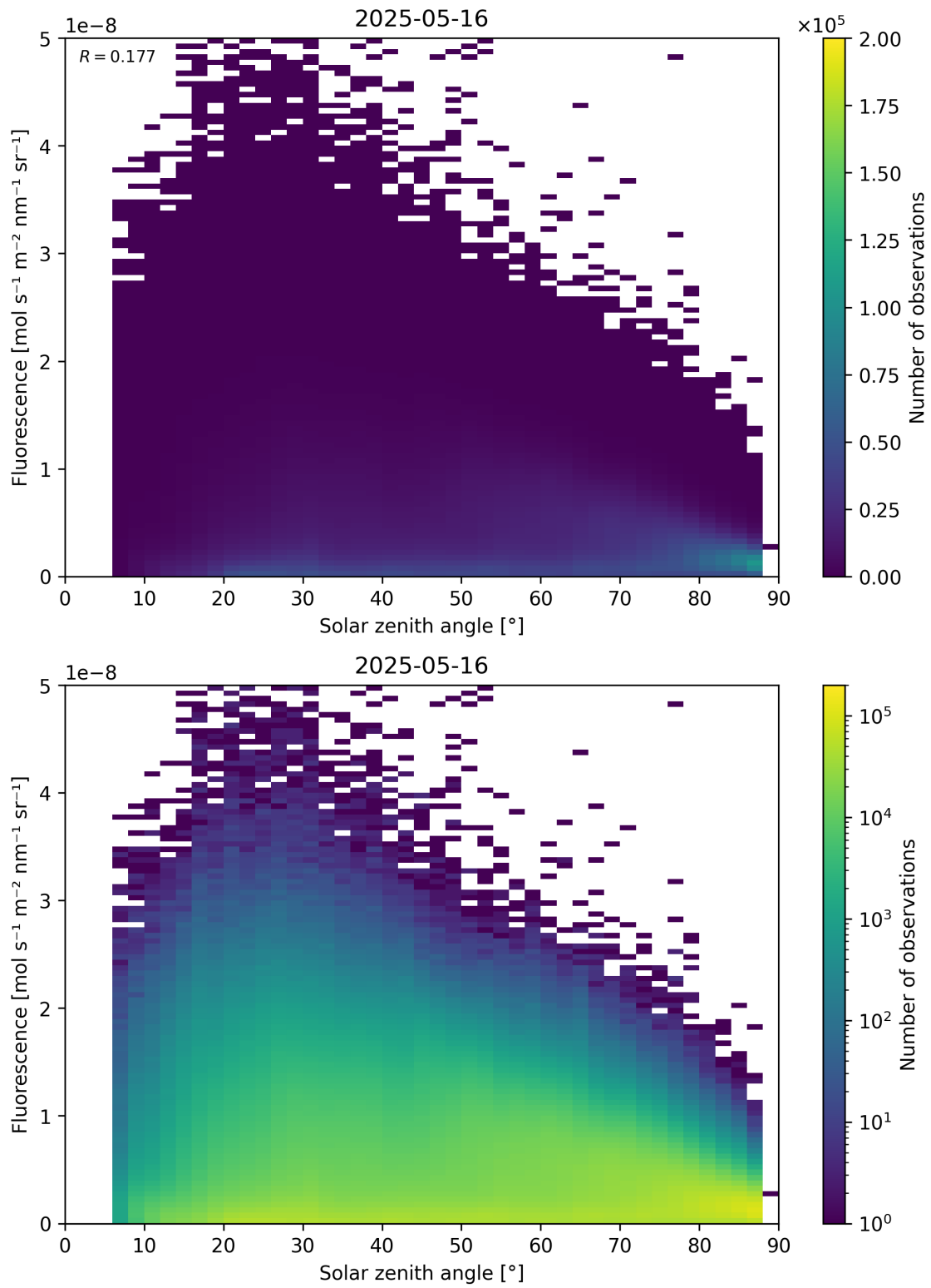
Figure 112: Scatter density plot of “Solar zenith angle” against “Fluorescence” for 2025-05-15 to 2025-05-17.
