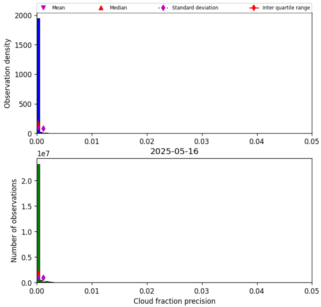
Figure 33: Histogram of “Cloud fraction precision” for 2025-05-15 to 2025-05-17
