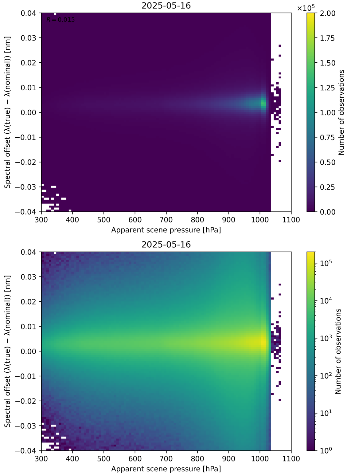
Figure 67: Scatter density plot of “Apparent scene pressure” against “Spectral offset ( \lambda_{\text{true}} - \lambda_{\text{nominal}} )” for 2025-05-15 to 2025-05-17.
