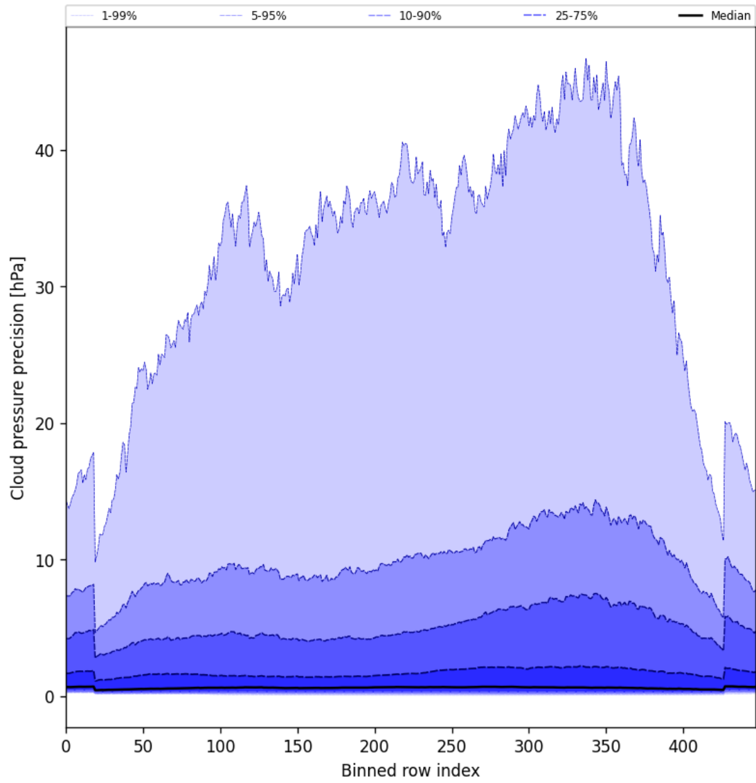
Figure 48: Along track statistics of “Cloud pressure precision” for 2025-05-15 to 2025-05-17
