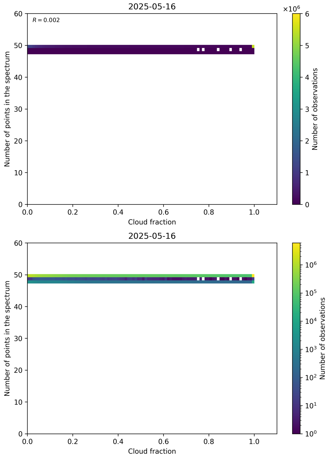
Figure 74: Scatter density plot of “Cloud fraction” against “Number of points in the spectrum” for 2025-05-15 to 2025-05-17.
