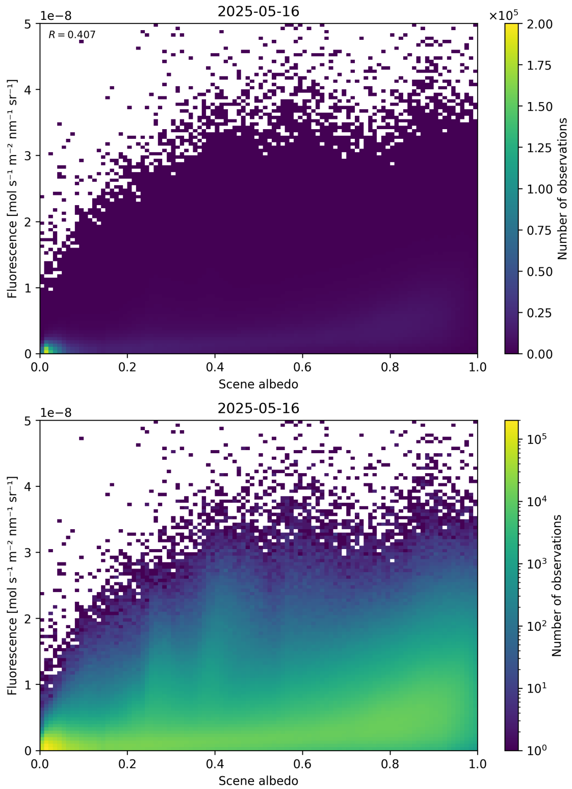
Figure 104: Scatter density plot of “Scene albedo” against “Fluorescence” for 2025-05-15 to 2025-05-17.
