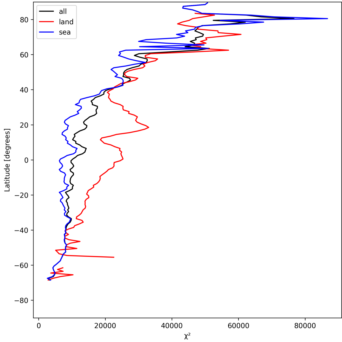
Figure 21: Zonal average of “ \chi^2 ” for 2025-05-15 to 2025-05-17.
