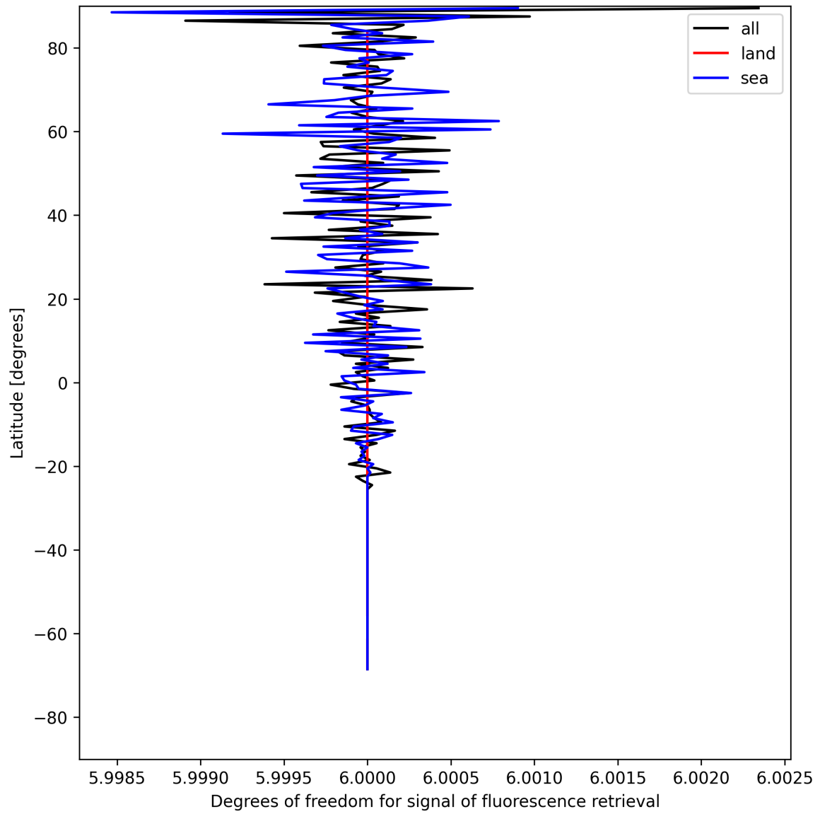
Figure 26: Zonal average of “Degrees of freedom for signal of fluorescence retrieval” for 2025-05-15 to 2025-05-17.
