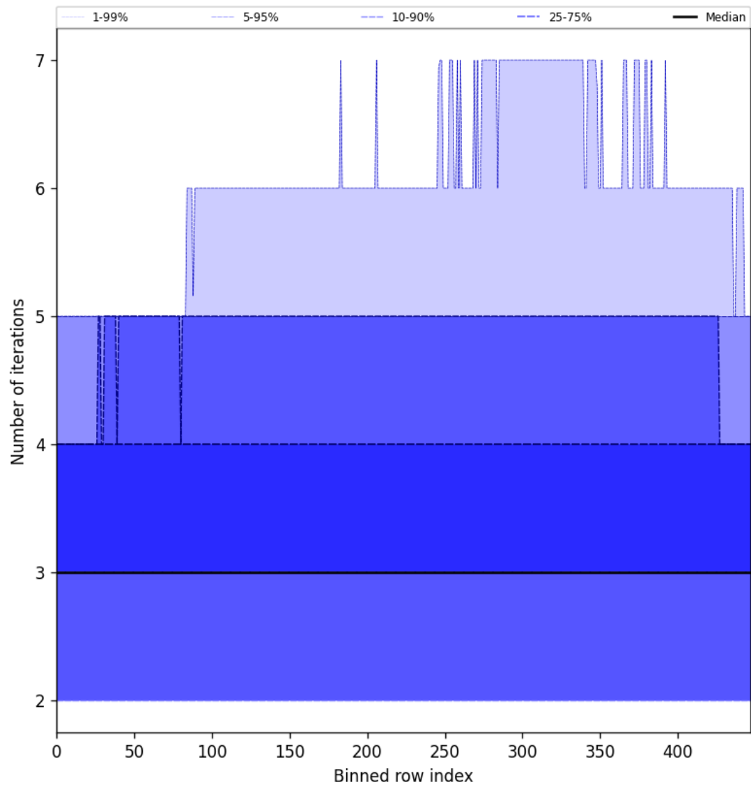
Figure 56: Along track statistics of “Number of iterations” for 2025-05-16 to 2025-05-18
