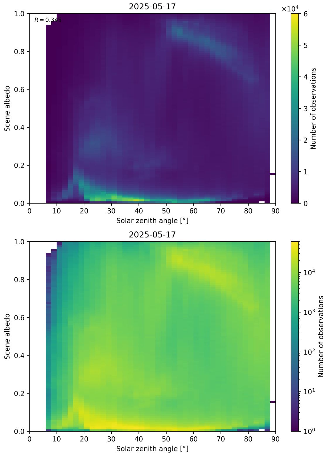
Figure 116: Scatter density plot of “Solar zenith angle” against “Scene albedo” for 2025-05-16 to 2025-05-18.
