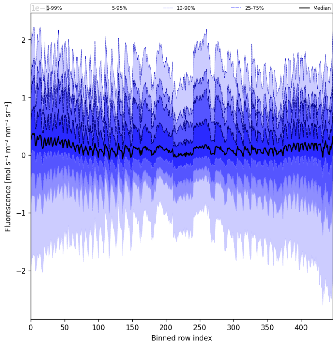
Figure 57: Along track statistics of “Fluorescence” for 2025-05-16 to 2025-05-18
