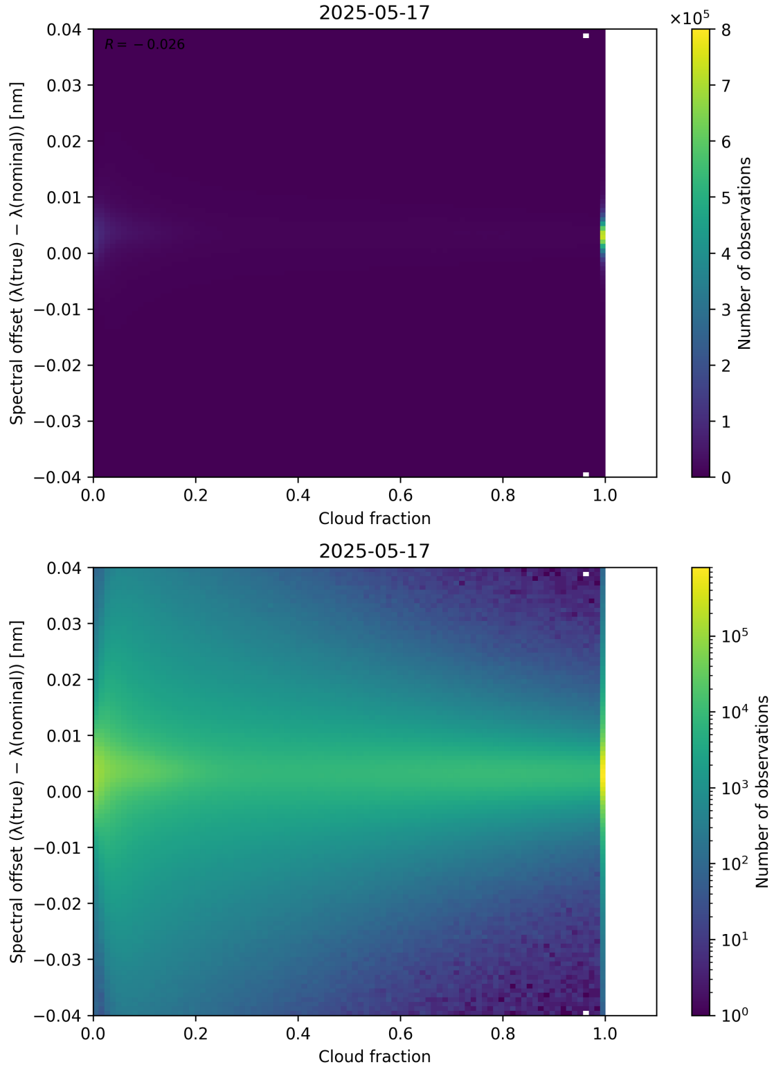
Figure 76: Scatter density plot of “Cloud fraction” against “Spectral offset ( \lambda_{\text{true}} - \lambda_{\text{nominal}} )” for 2025-05-16 to 2025-05-18.
