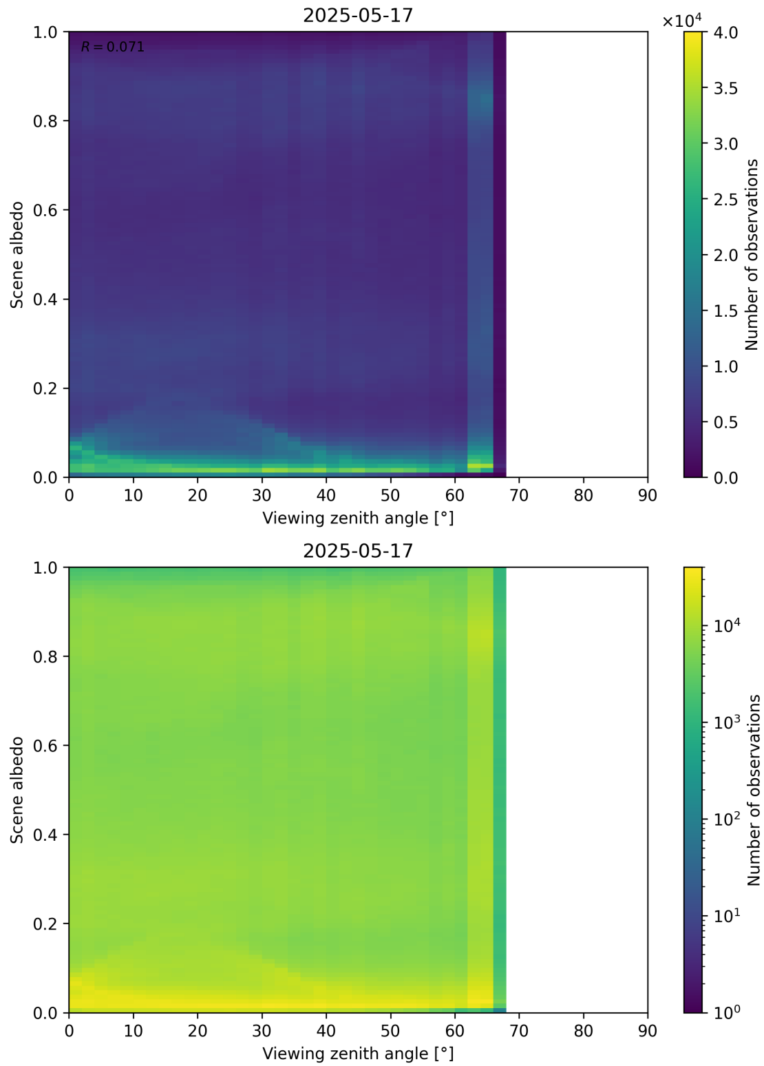
Figure 126: Scatter density plot of “Viewing zenith angle” against “Scene albedo” for 2025-05-16 to 2025-05-18.
