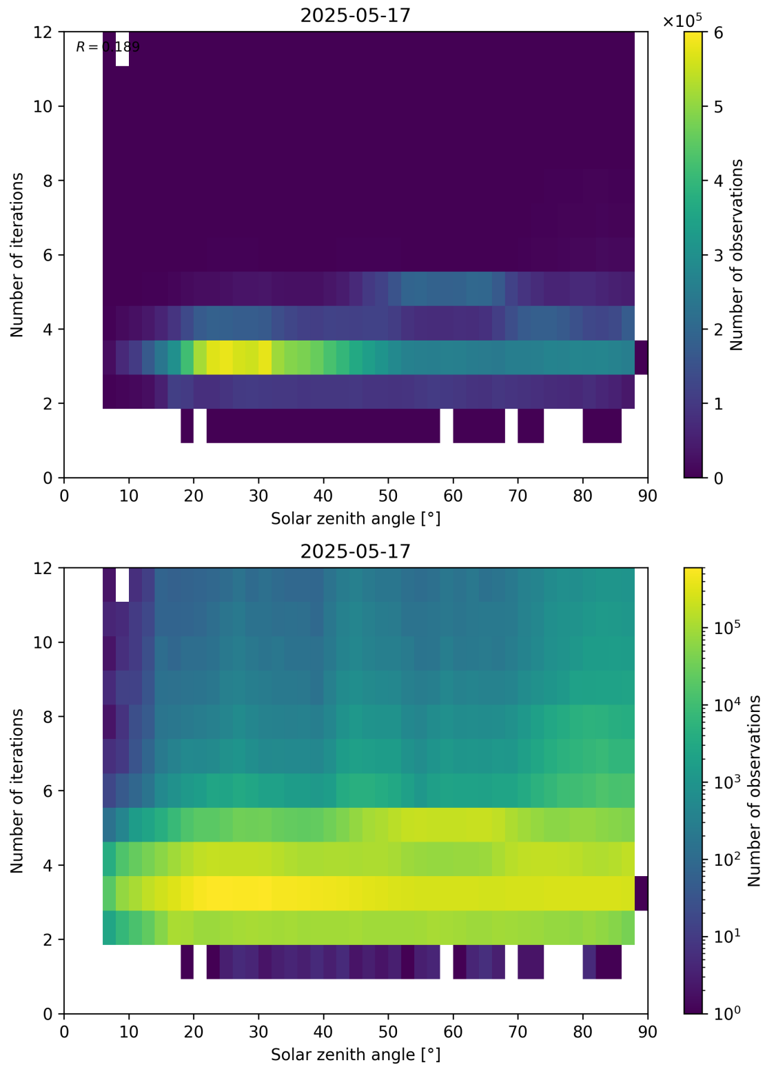
Figure 114: Scatter density plot of “Solar zenith angle” against “Number of iterations” for 2025-05-16 to 2025-05-18.
