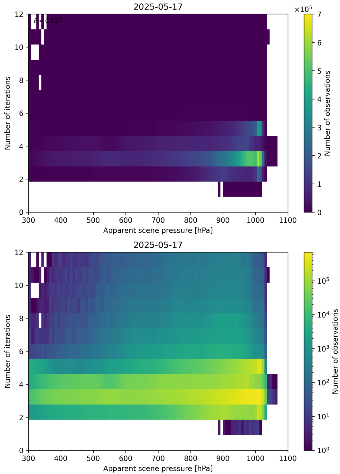
Figure 65: Scatter density plot of “Apparent scene pressure” against “Number of iterations” for 2025-05-16 to 2025-05-18.
