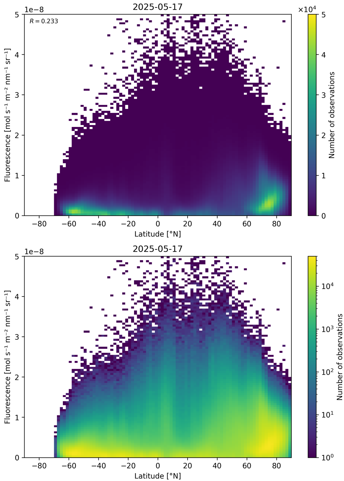
Figure 92: Scatter density plot of “Latitude” against “Fluorescence” for 2025-05-16 to 2025-05-18.
