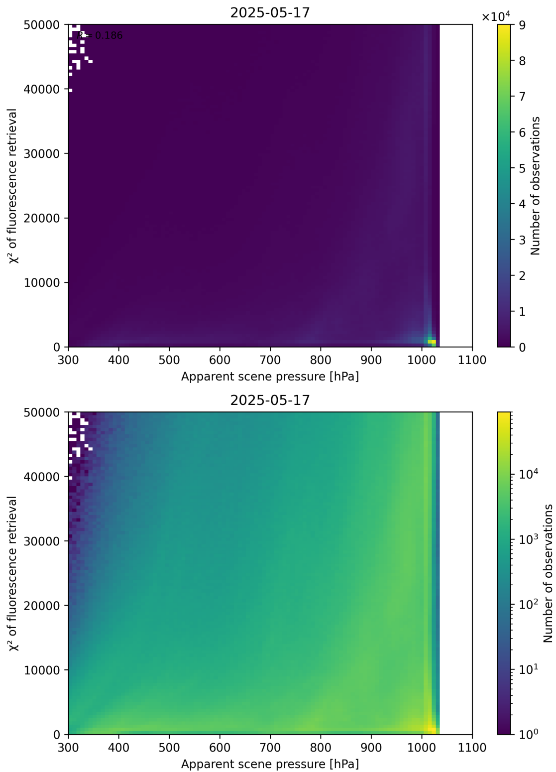
Figure 63: Scatter density plot of “Apparent scene pressure” against “ \chi^2 of fluorescence retrieval” for 2025-05-16 to 2025-05-18.
