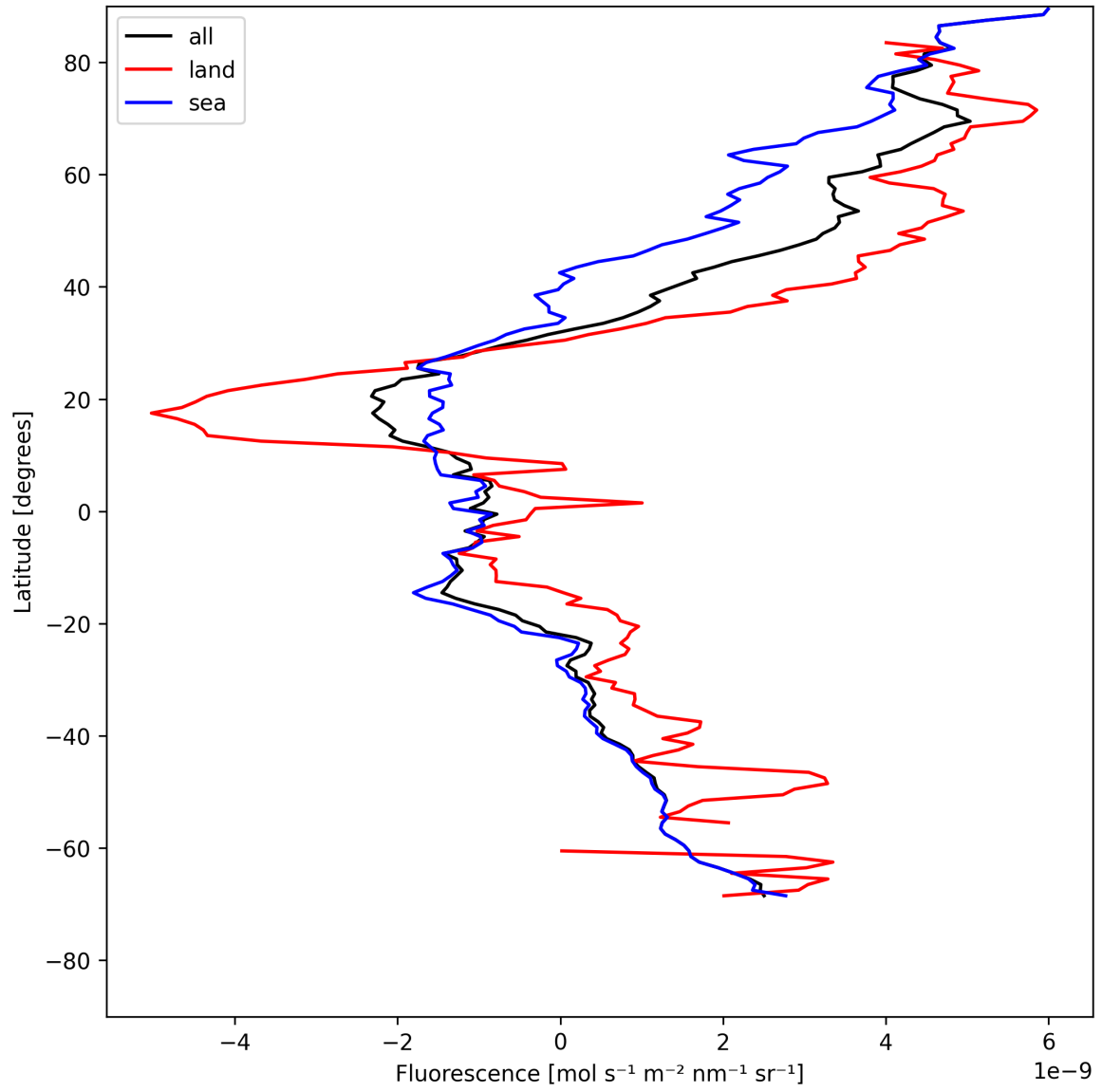
Figure 23: Zonal average of “Fluorescence” for 2025-05-16 to 2025-05-18.
