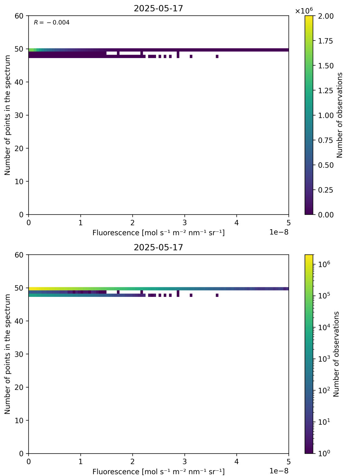
Figure 86: Scatter density plot of “Fluorescence” against “Number of points in the spectrum” for 2025-05-16 to 2025-05-18.
