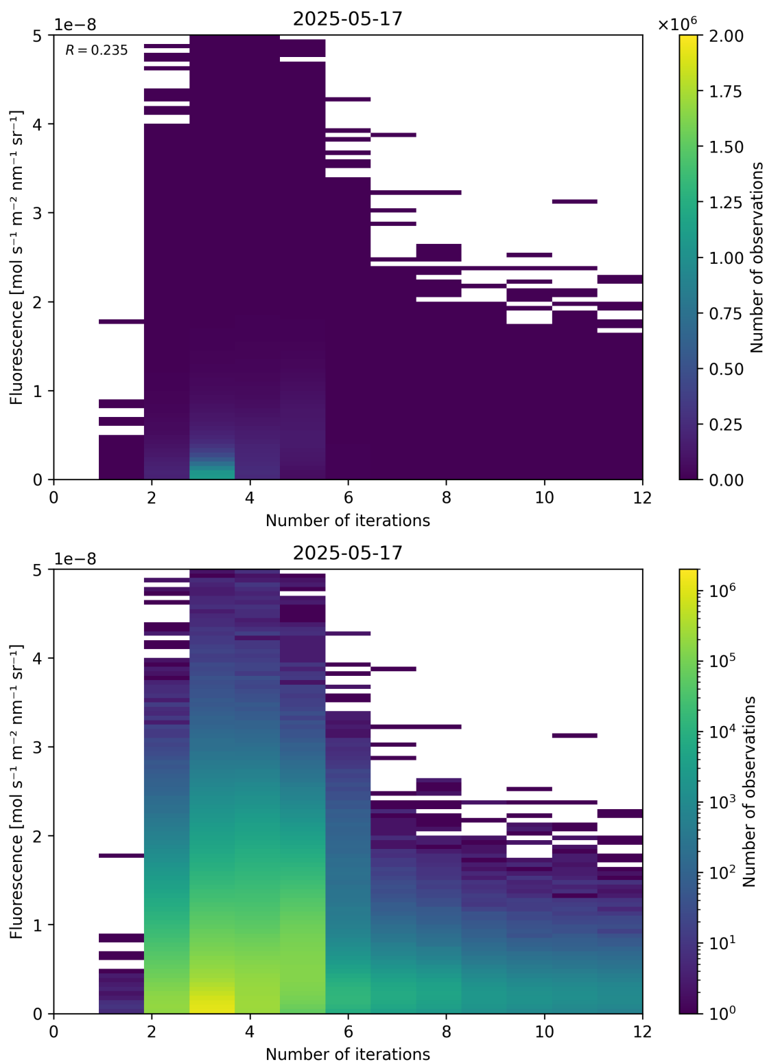
Figure 98: Scatter density plot of “Number of iterations” against “Fluorescence” for 2025-05-16 to 2025-05-18.
