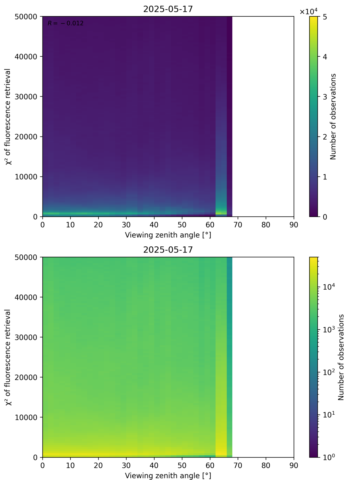
Figure 119: Scatter density plot of “Viewing zenith angle” against “ \chi^2 of fluorescence retrieval” for 2025-05-16 to 2025-05-18.
