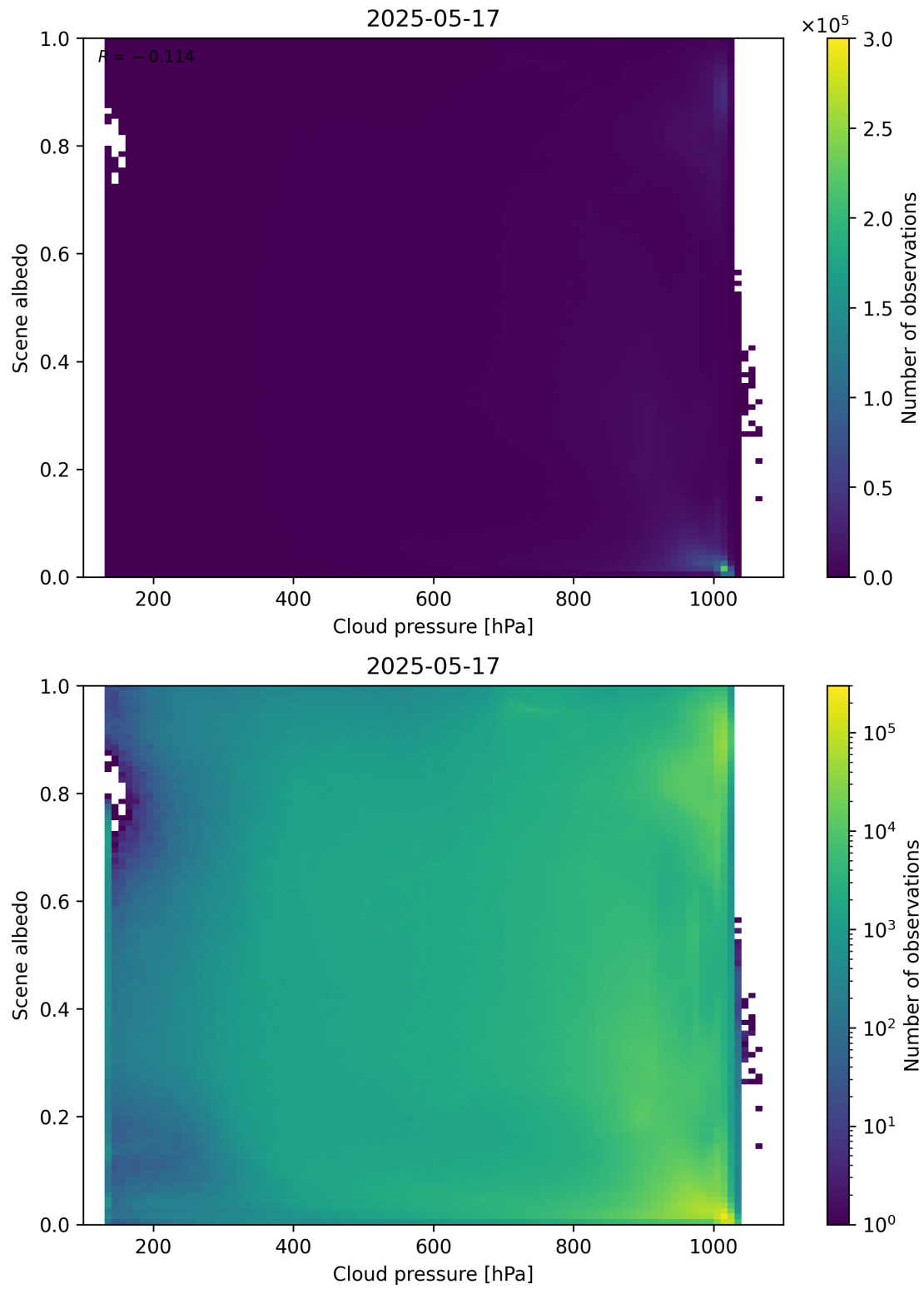
Figure 83: Scatter density plot of “Cloud pressure” against “Scene albedo” for 2025-05-16 to 2025-05-18.
