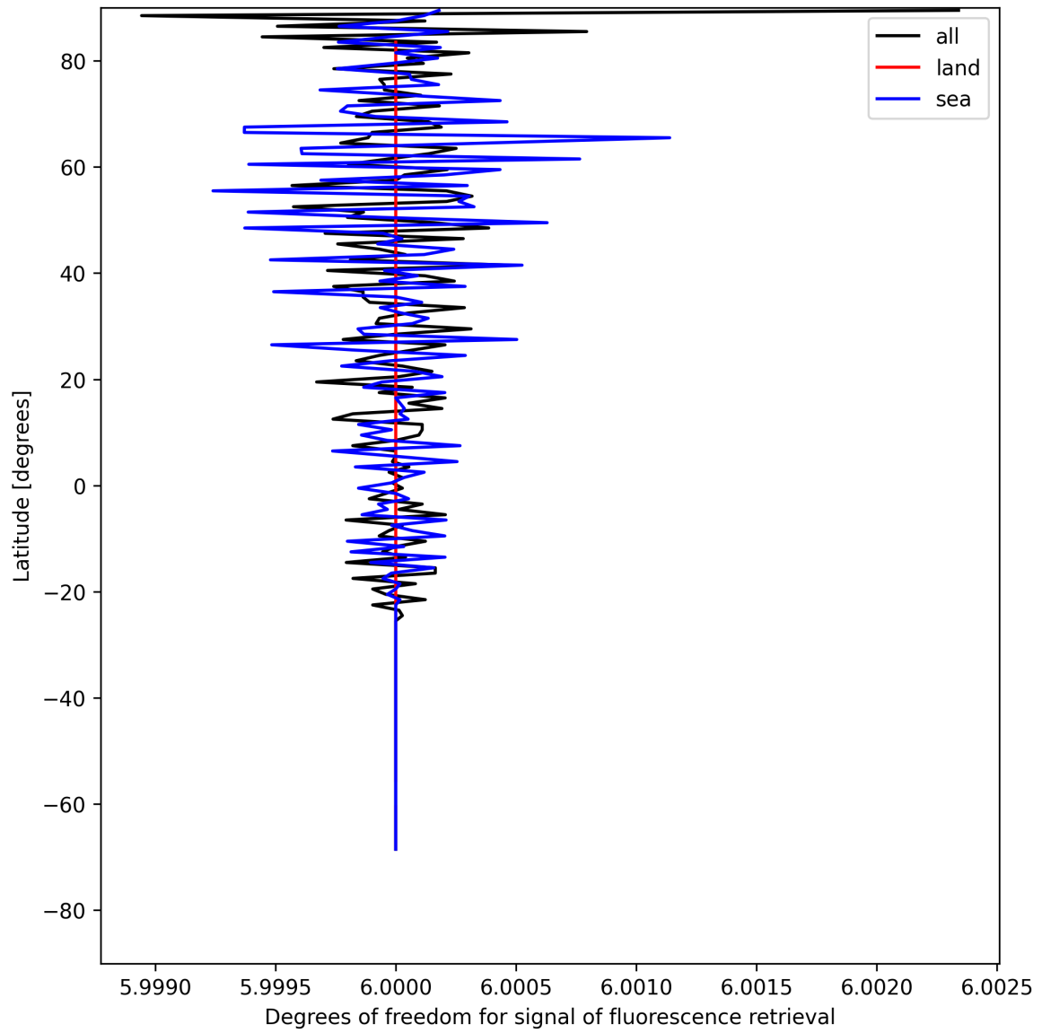
Figure 26: Zonal average of “Degrees of freedom for signal of fluorescence retrieval” for 2025-05-16 to 2025-05-18.
