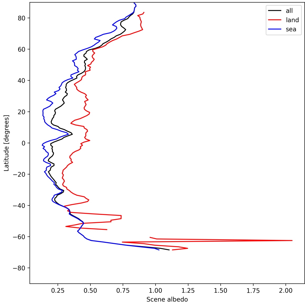
Figure 17: Zonal average of “Scene albedo” for 2025-05-16 to 2025-05-18.
