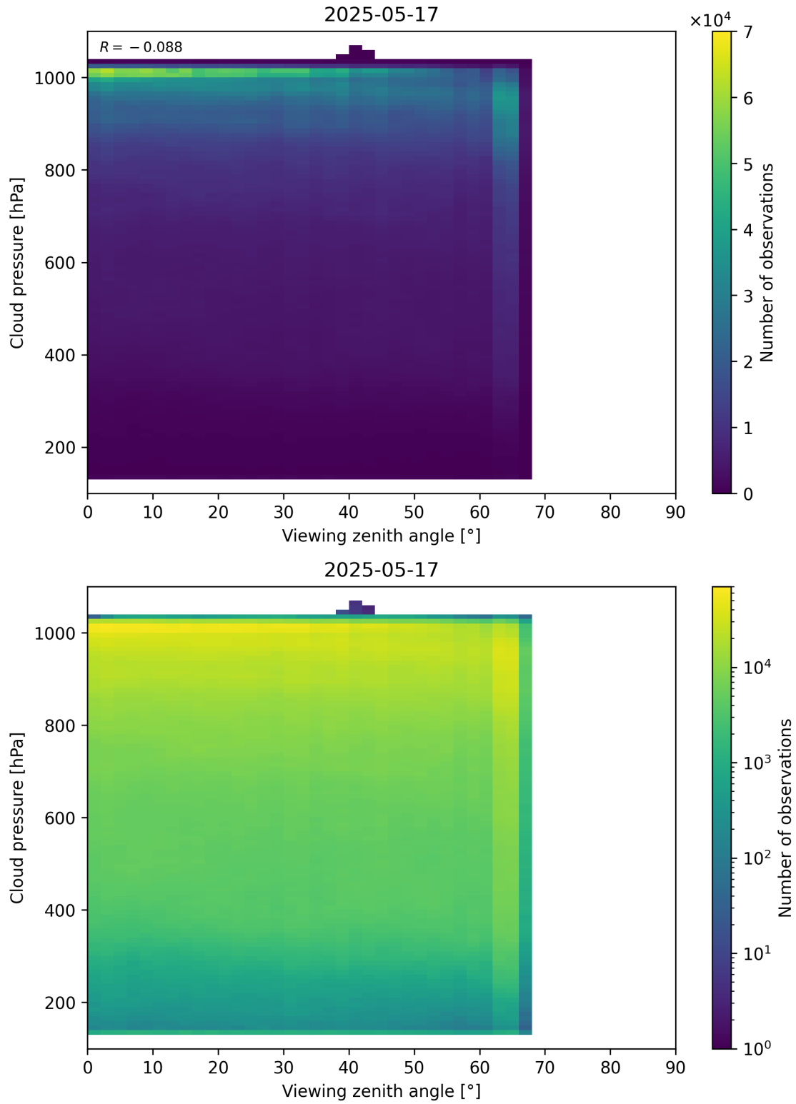
Figure 121: Scatter density plot of “Viewing zenith angle” against “Cloud pressure” for 2025-05-16 to 2025-05-18.
