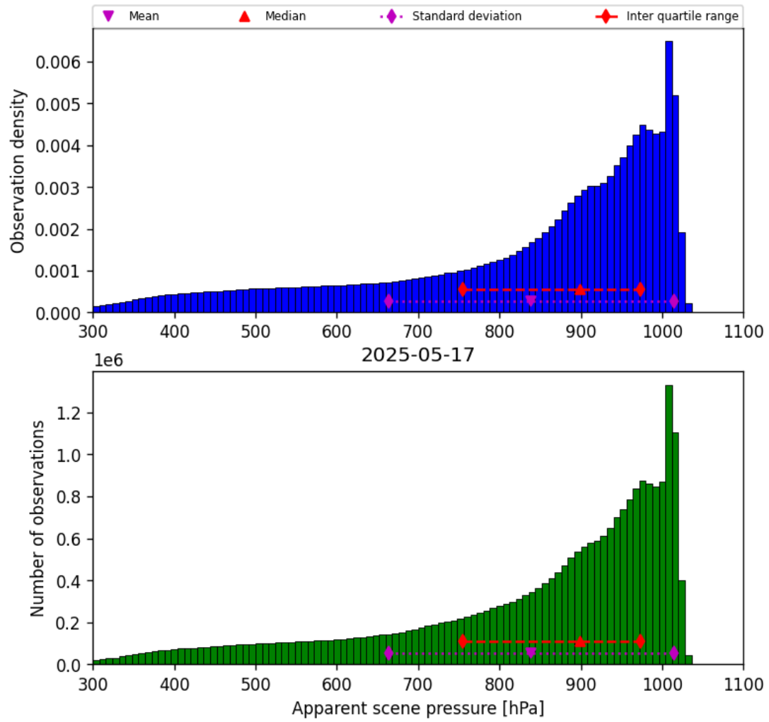
Figure 36: Histogram of “Apparent scene pressure” for 2025-05-16 to 2025-05-18
