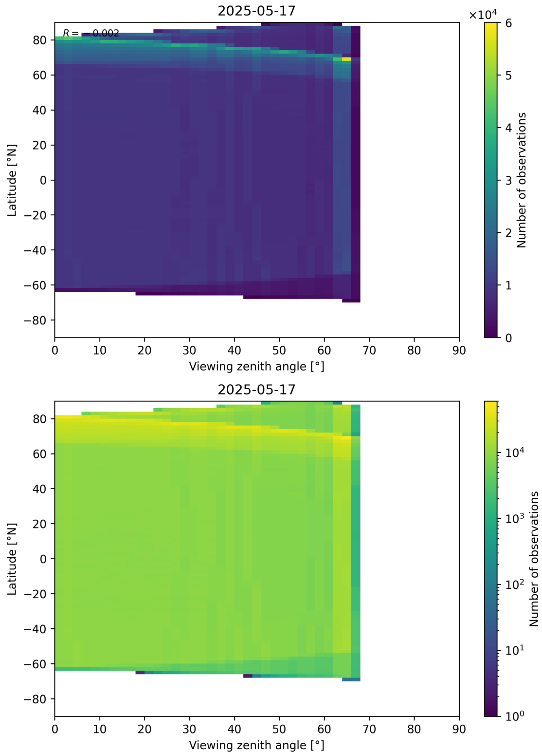
Figure 123: Scatter density plot of “Viewing zenith angle” against “Latitude” for 2025-05-16 to 2025-05-18.
