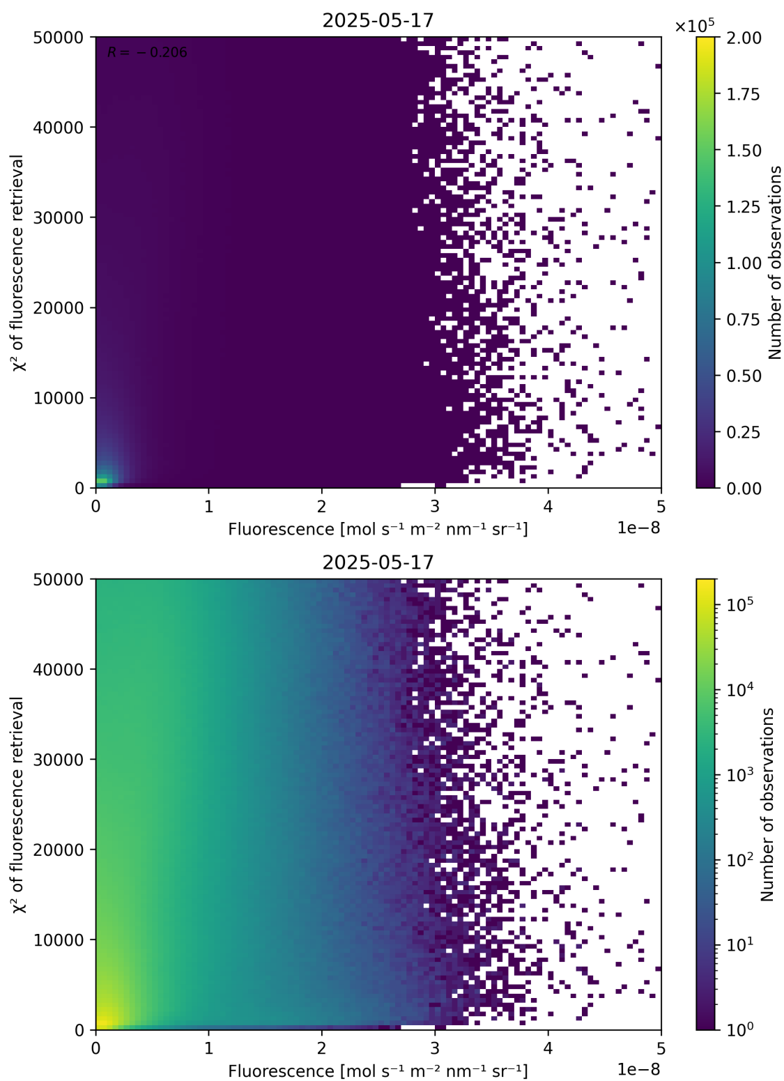
Figure 85: Scatter density plot of “Fluorescence” against “ \chi^2 of fluorescence retrieval” for 2025-05-16 to 2025-05-18.
