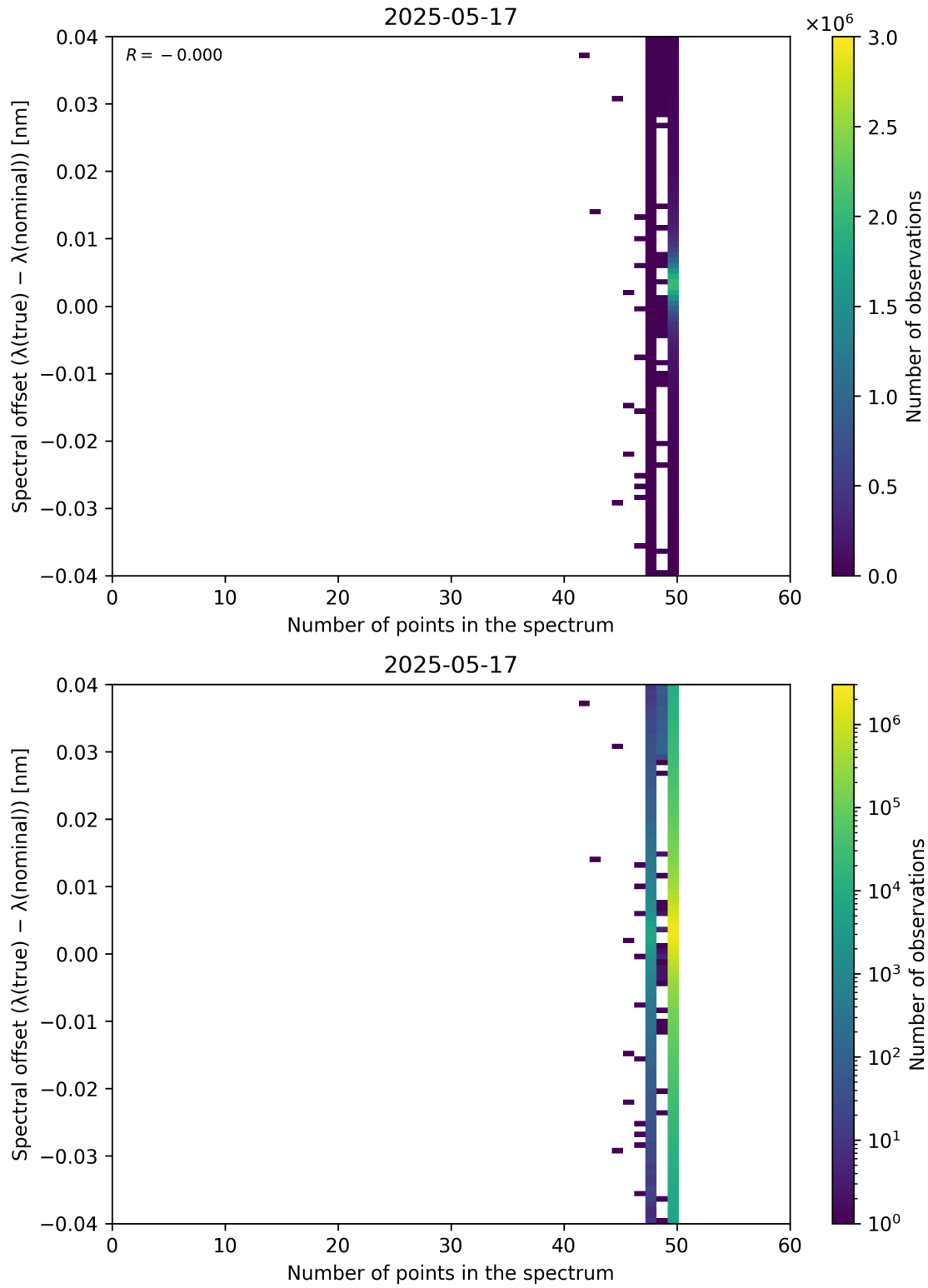
Figure 101: Scatter density plot of “Number of points in the spectrum” against “Spectral offset ( \lambda_{\text{true}} - \lambda_{\text{nominal}} )” for 2025-05-16 to 2025-05-18.
