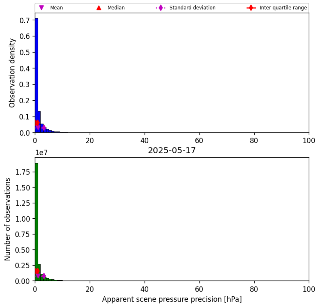
Figure 37: Histogram of “Apparent scene pressure precision” for 2025-05-16 to 2025-05-18
