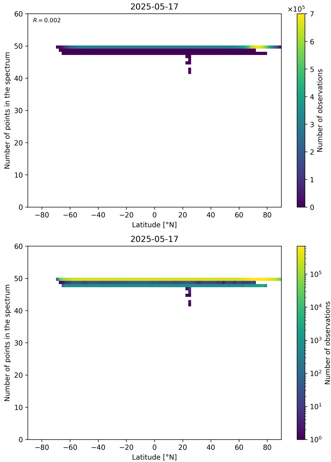
Figure 94: Scatter density plot of “Latitude” against “Number of points in the spectrum” for 2025-05-16 to 2025-05-18.
