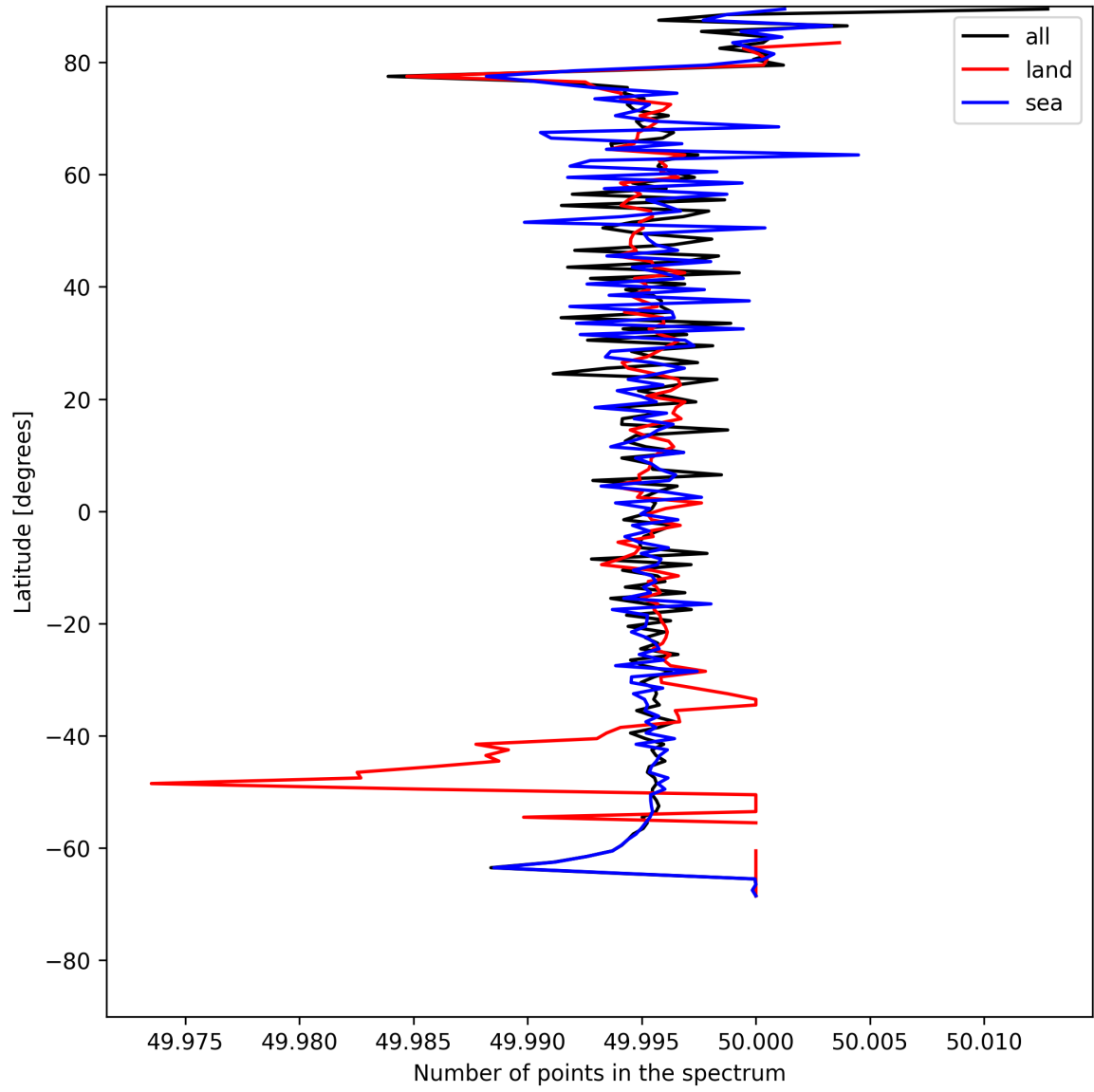
Figure 27: Zonal average of “Number of points in the spectrum” for 2025-05-16 to 2025-05-18.
