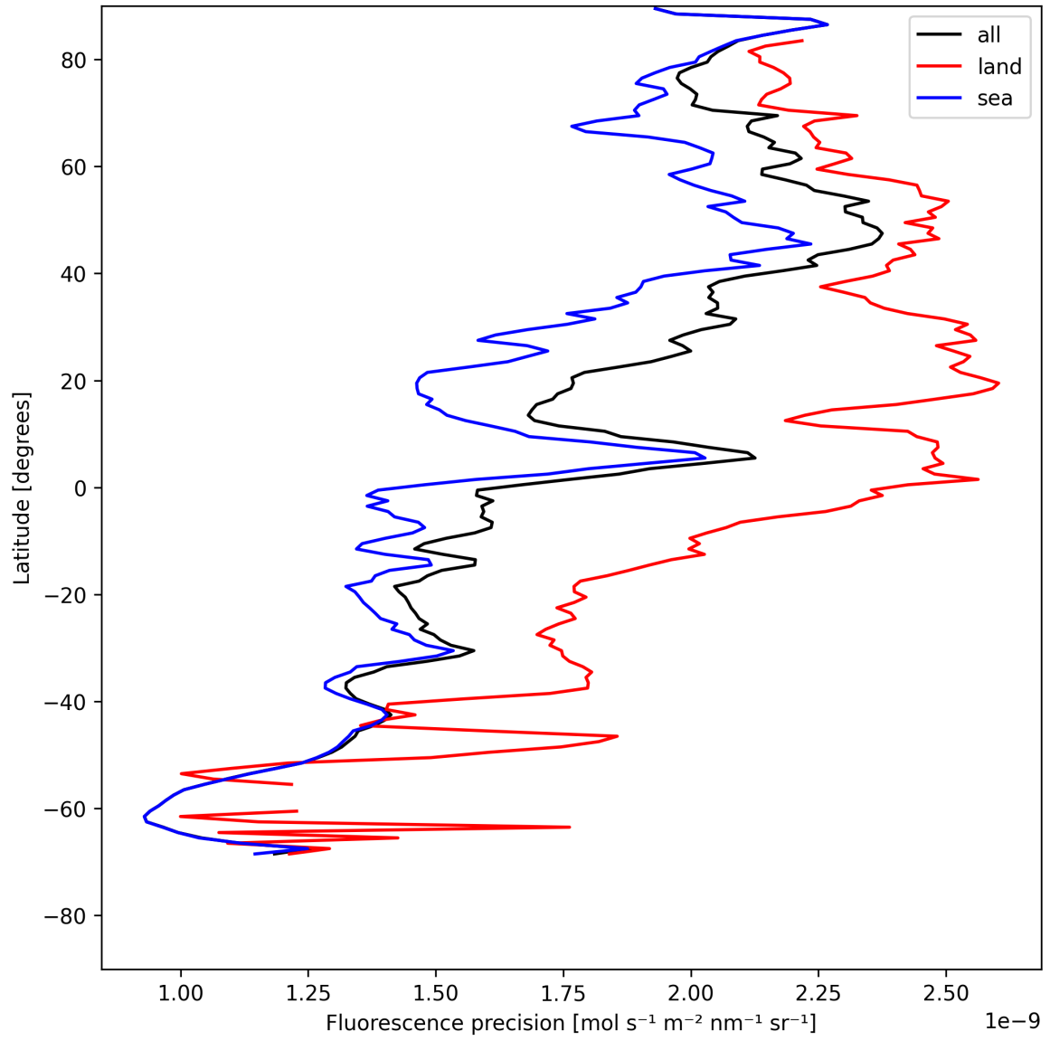
Figure 24: Zonal average of “Fluorescence precision” for 2025-05-16 to 2025-05-18.
