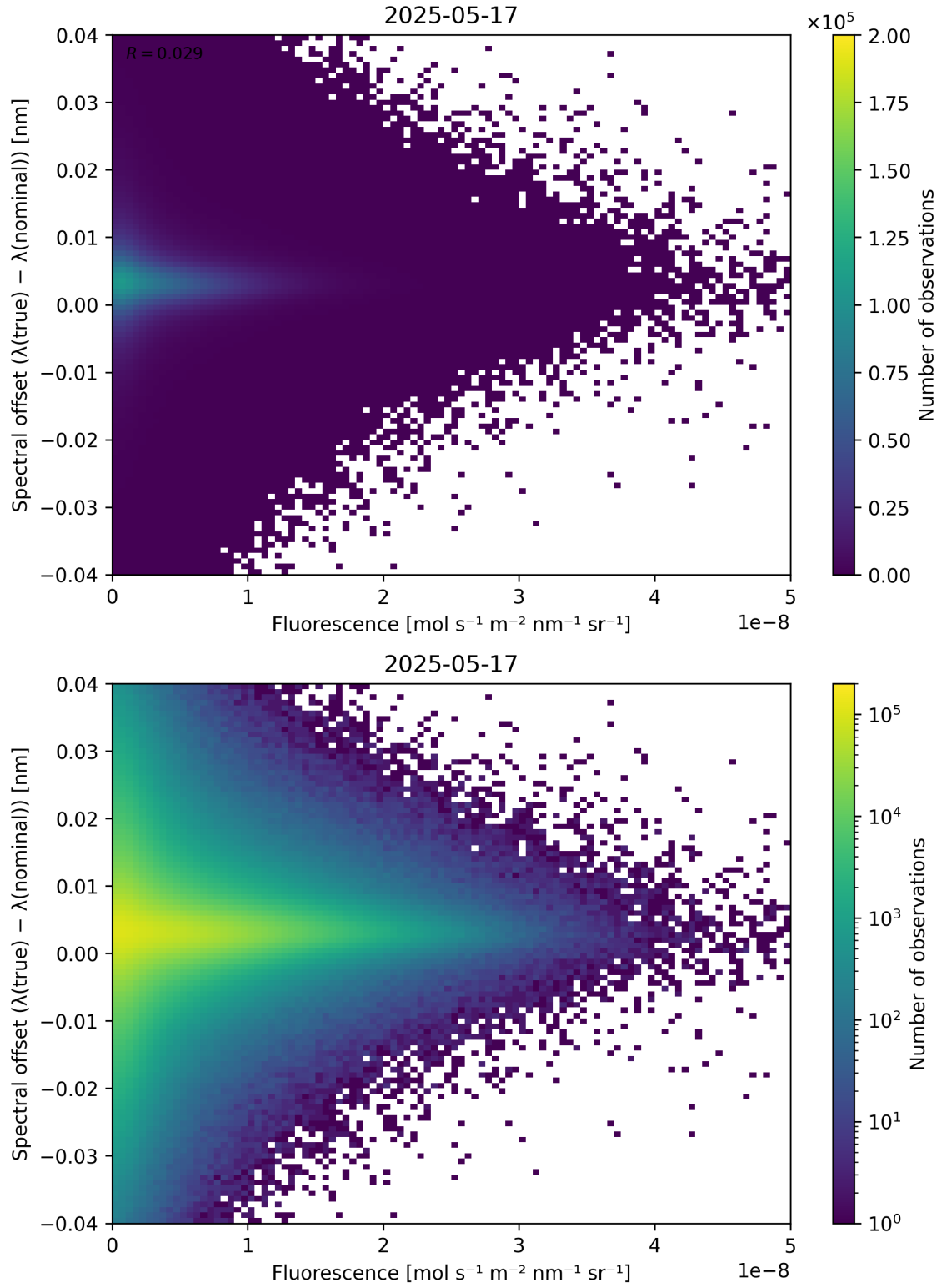
Figure 87: Scatter density plot of “Fluorescence” against “Spectral offset ( \lambda_{\text{true}} - \lambda_{\text{nominal}} )” for 2025-05-16 to 2025-05-18.
