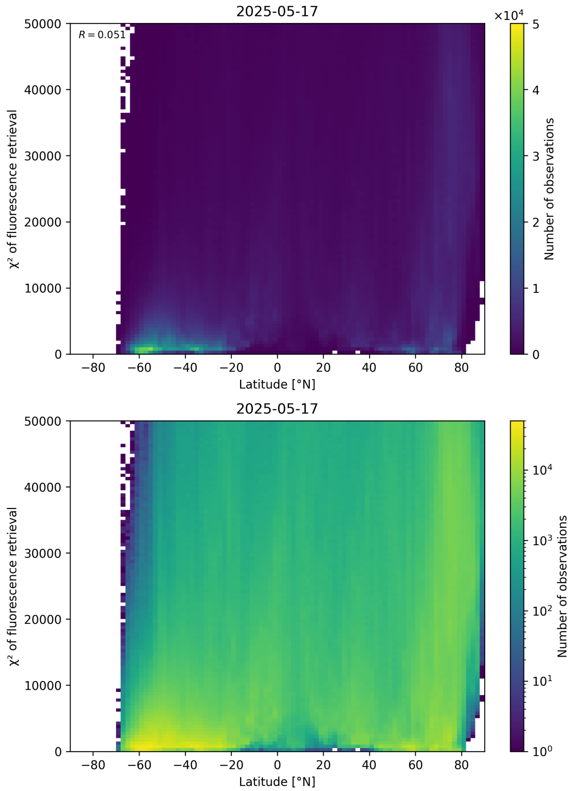
Figure 89: Scatter density plot of “Latitude” against “ \chi^2 of fluorescence retrieval” for 2025-05-16 to 2025-05-18.
