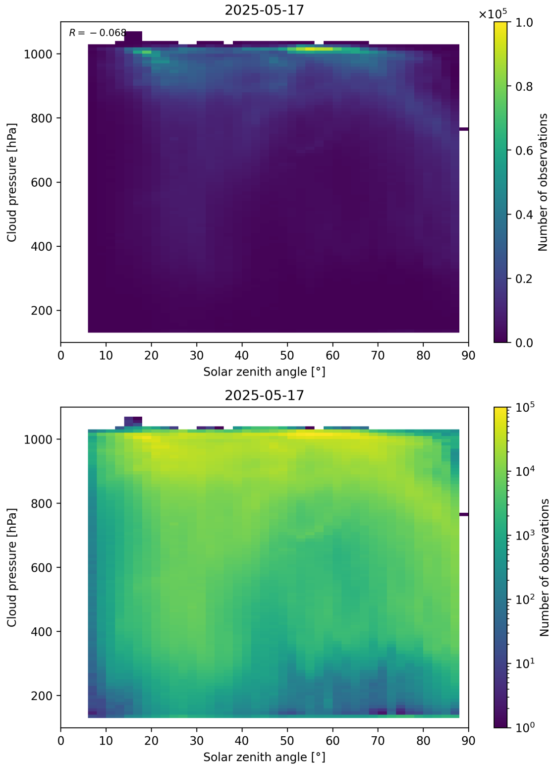
Figure 111: Scatter density plot of “Solar zenith angle” against “Cloud pressure” for 2025-05-16 to 2025-05-18.
