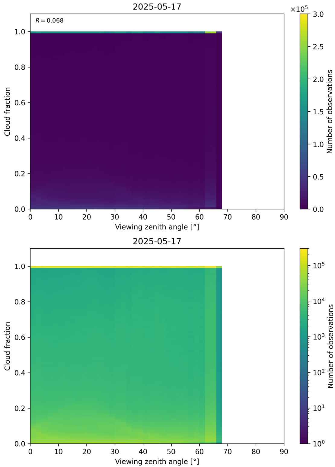
Figure 120: Scatter density plot of “Viewing zenith angle” against “Cloud fraction” for 2025-05-16 to 2025-05-18.
