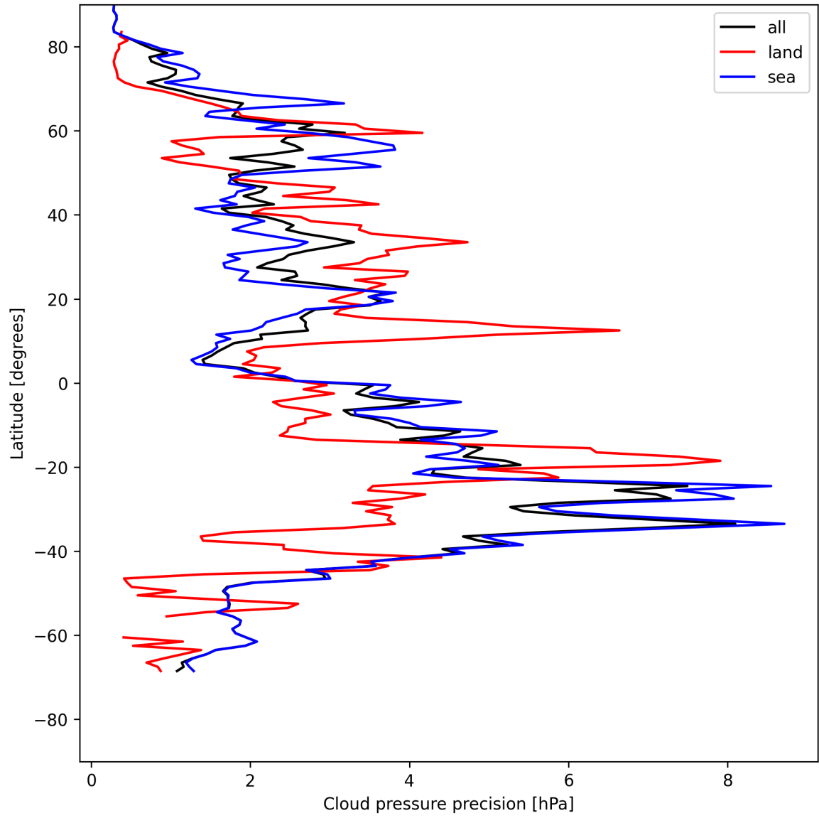
Figure 14: Zonal average of “Cloud pressure precision” for 2025-05-16 to 2025-05-18.
