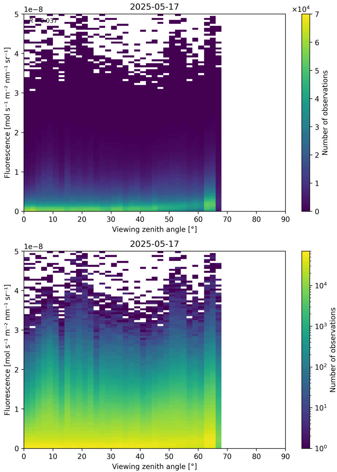
Figure 122: Scatter density plot of “Viewing zenith angle” against “Fluorescence” for 2025-05-16 to 2025-05-18.
