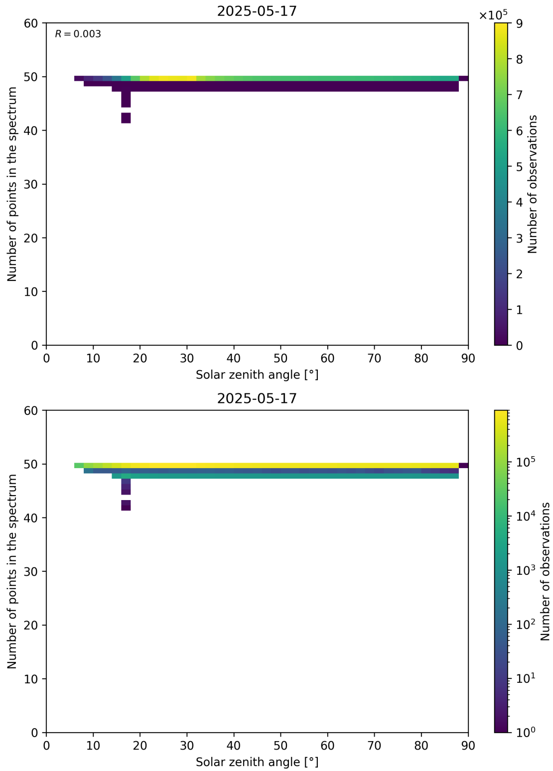
Figure 115: Scatter density plot of “Solar zenith angle” against “Number of points in the spectrum” for 2025-05-16 to 2025-05-18.
