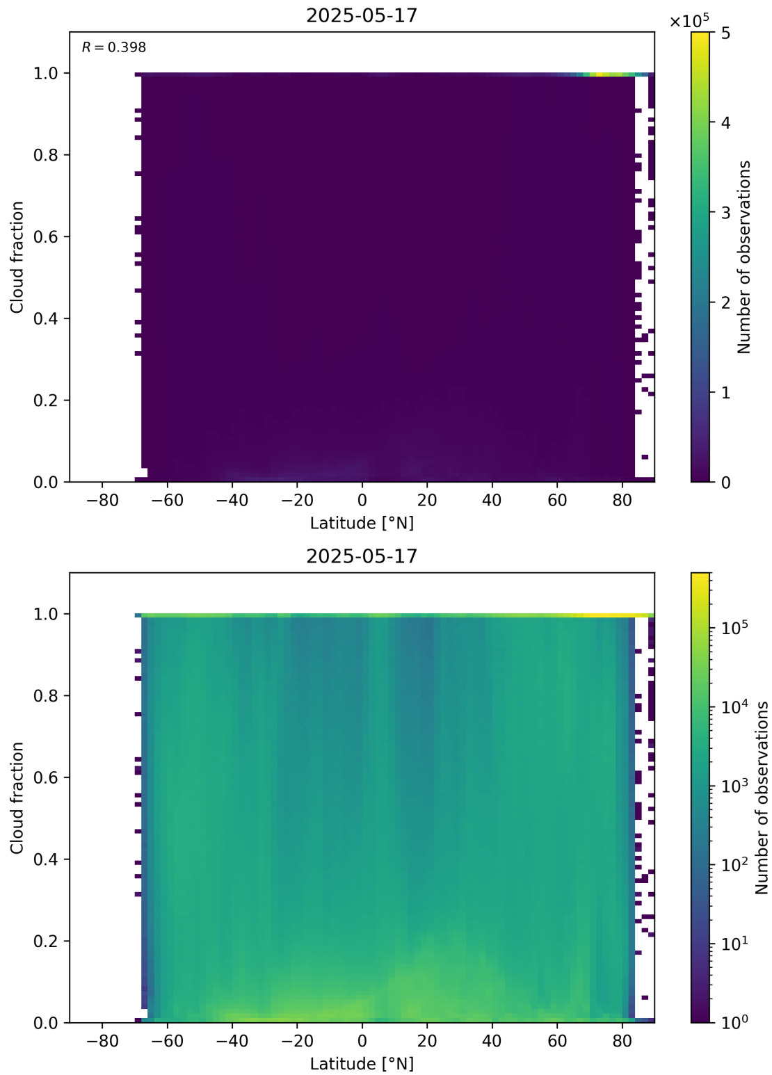
Figure 90: Scatter density plot of “Latitude” against “Cloud fraction” for 2025-05-16 to 2025-05-18.
