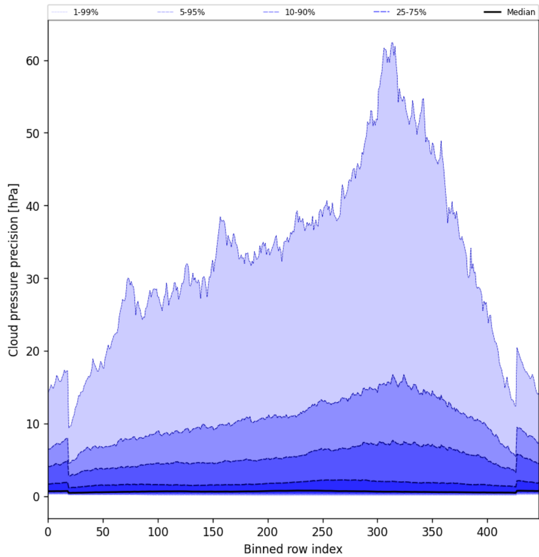
Figure 48: Along track statistics of “Cloud pressure precision” for 2025-05-16 to 2025-05-18
