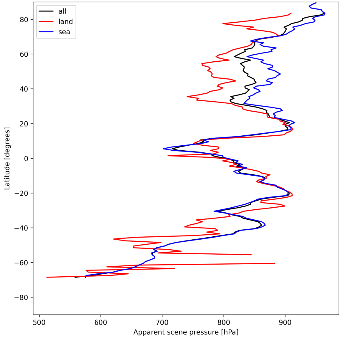
Figure 19: Zonal average of “Apparent scene pressure” for 2025-05-16 to 2025-05-18.
