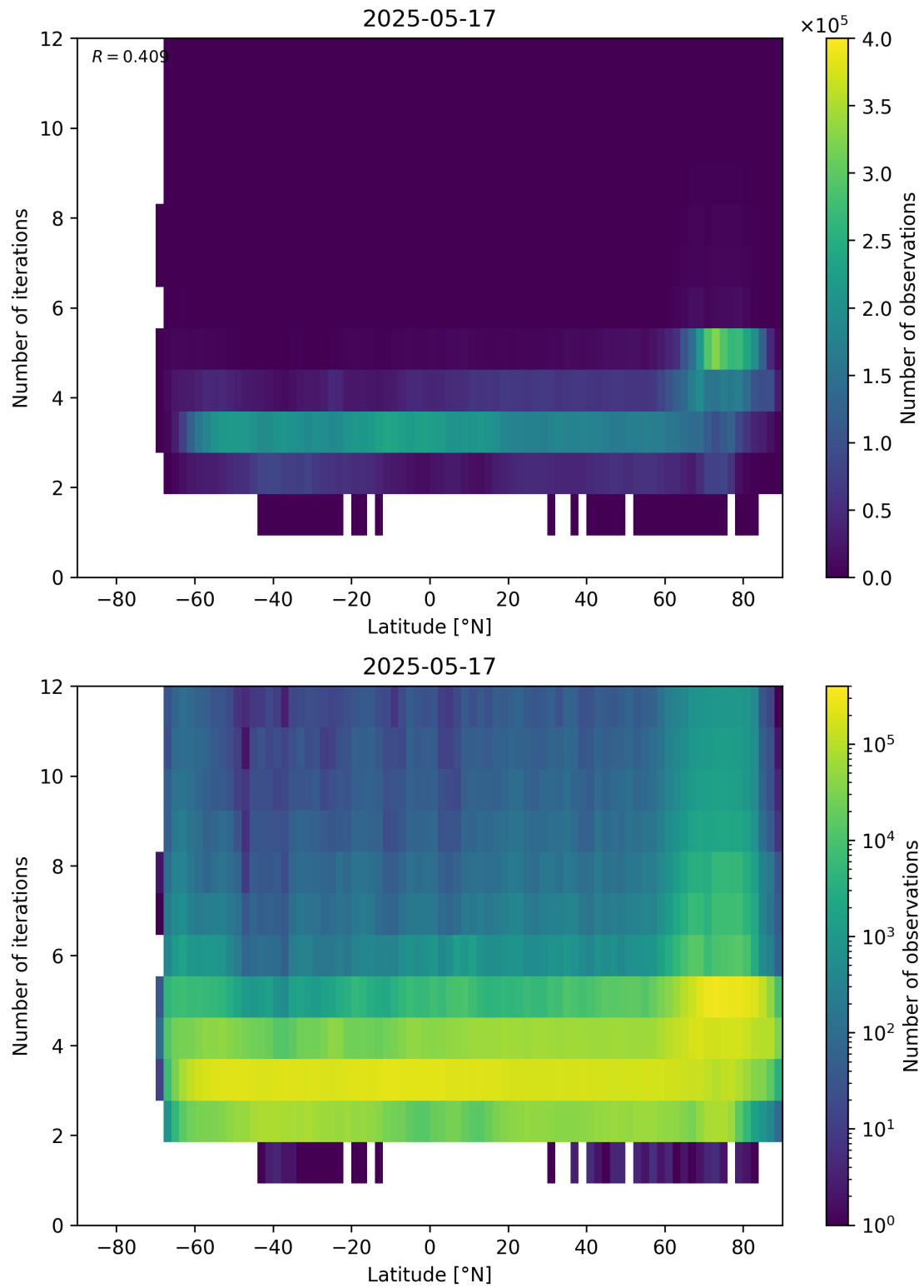
Figure 93: Scatter density plot of “Latitude” against “Number of iterations” for 2025-05-16 to 2025-05-18.
