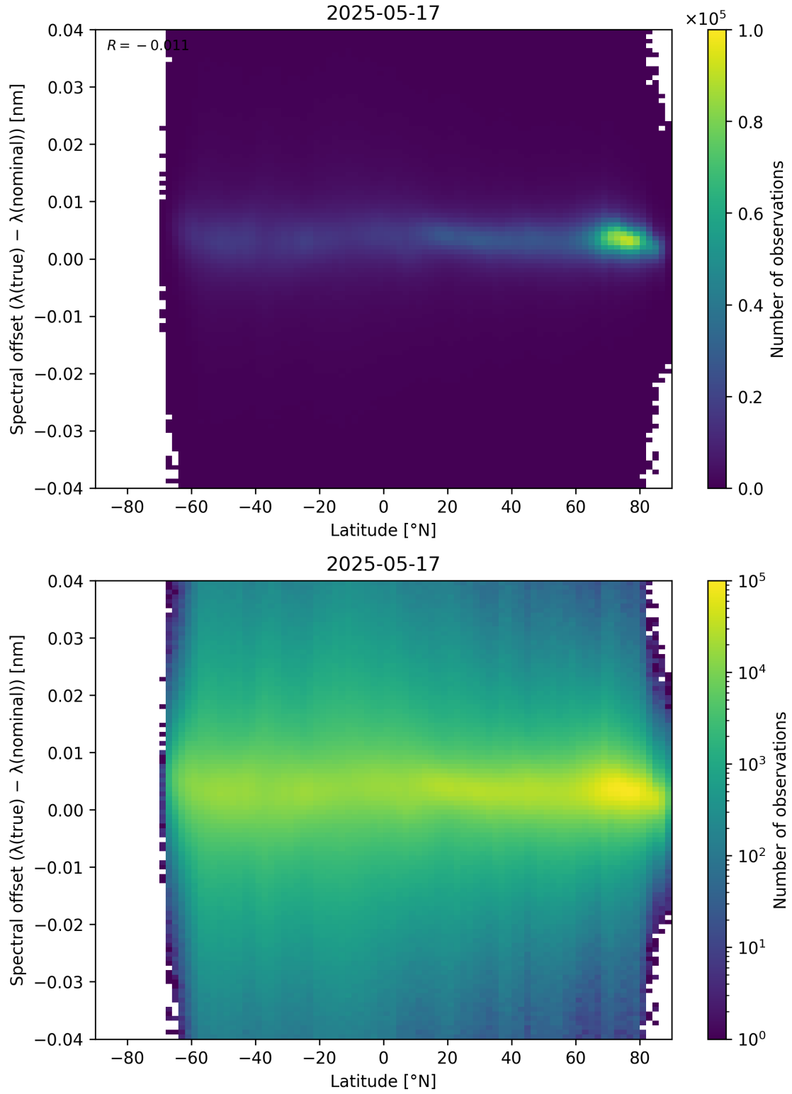
Figure 96: Scatter density plot of “Latitude” against “Spectral offset ( \lambda_{\text{true}} - \lambda_{\text{nominal}} )” for 2025-05-16 to 2025-05-18.
