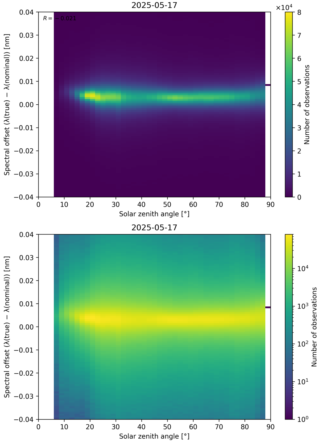
Figure 117: Scatter density plot of “Solar zenith angle” against “Spectral offset ( \lambda_{\text{true}} - \lambda_{\text{nominal}} )” for 2025-05-16 to 2025-05-18.
