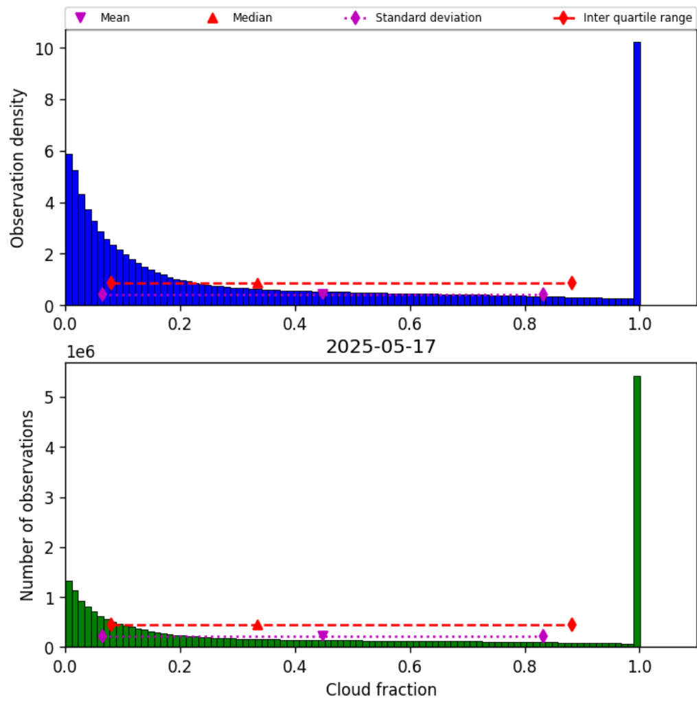
Figure 32: Histogram of “Cloud fraction” for 2025-05-16 to 2025-05-18
