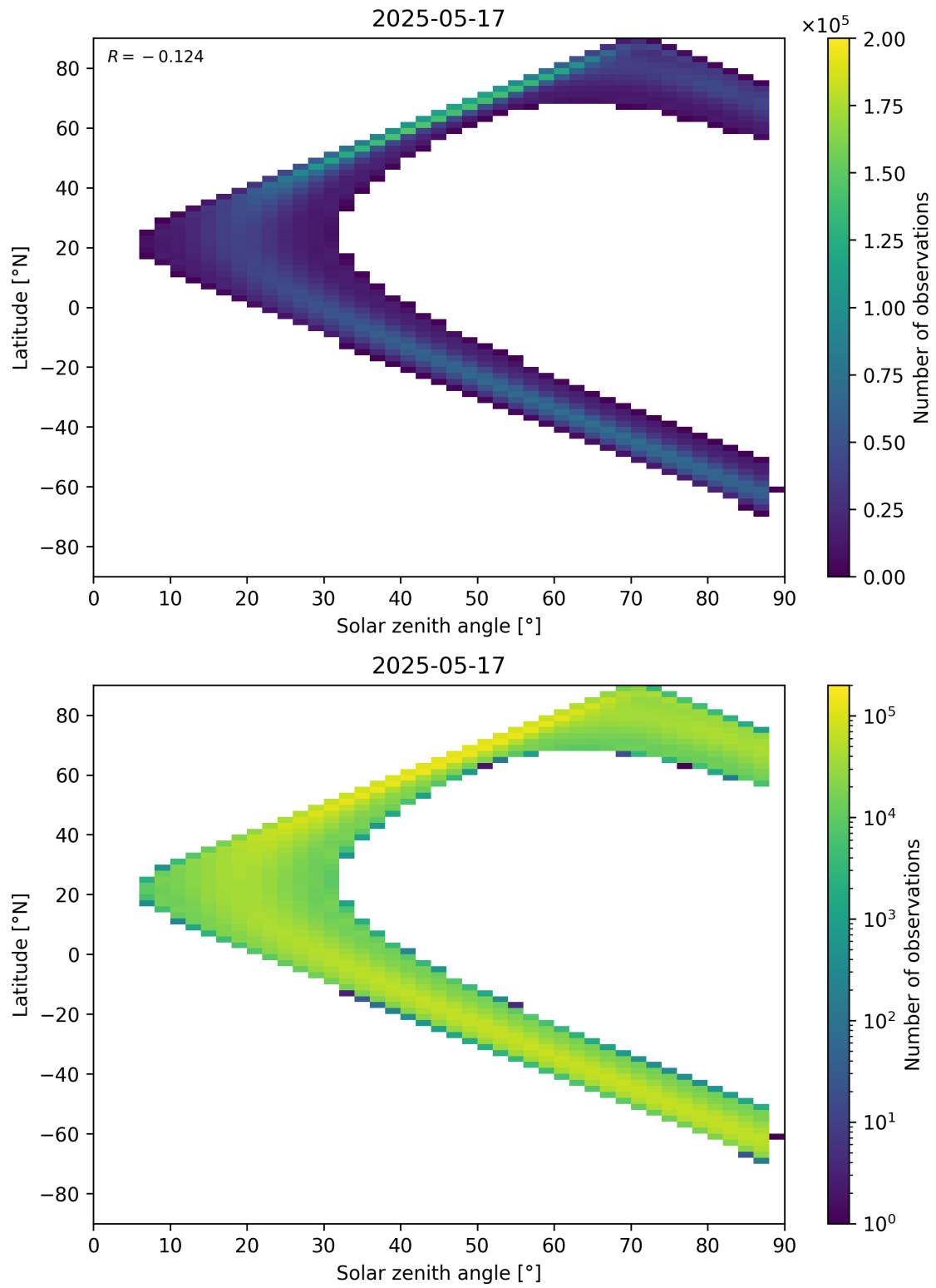
Figure 113: Scatter density plot of “Solar zenith angle” against “Latitude” for 2025-05-16 to 2025-05-18.
