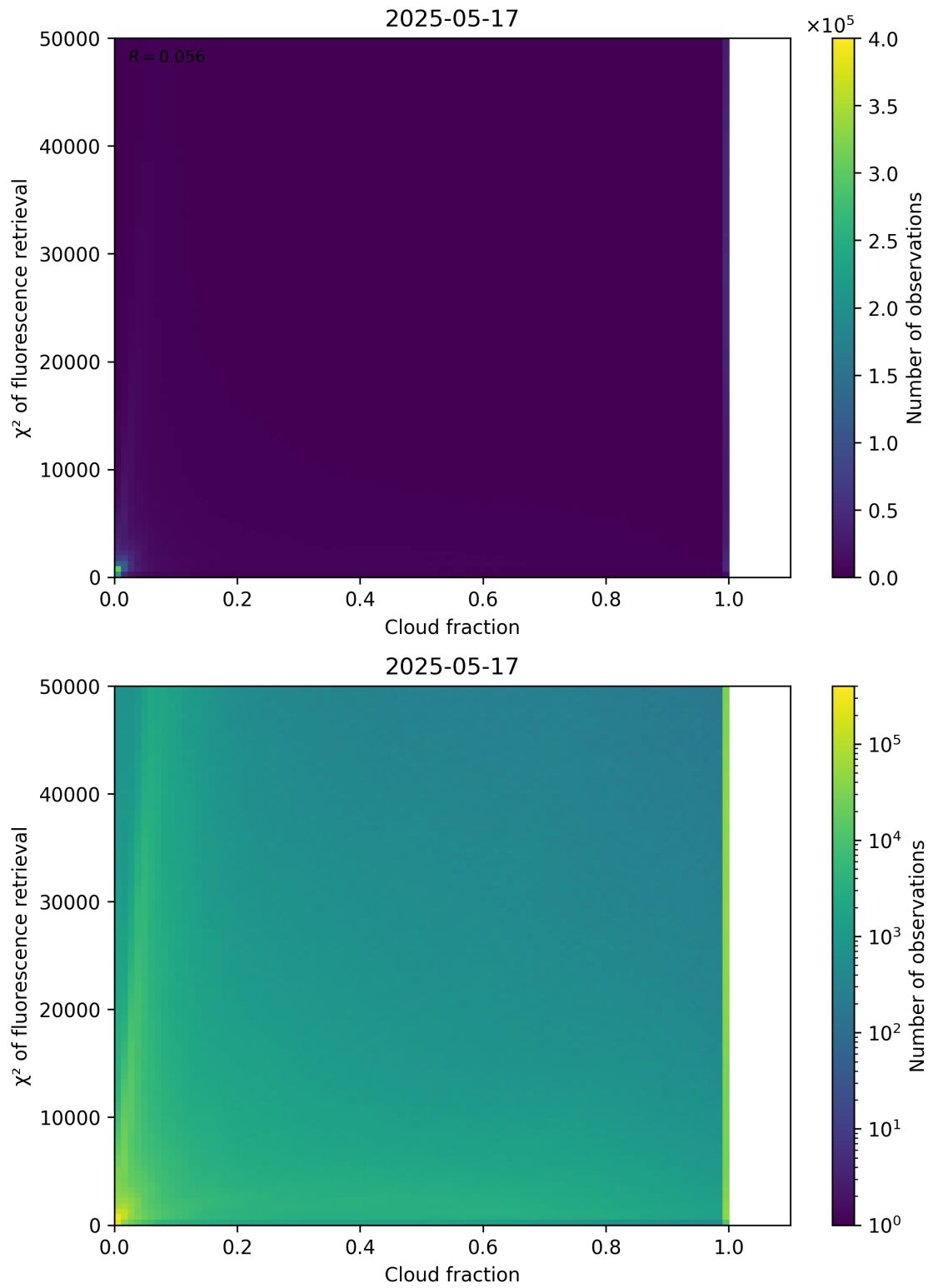
Figure 71: Scatter density plot of “Cloud fraction” against “ \chi^2 of fluorescence retrieval” for 2025-05-16 to 2025-05-18.
