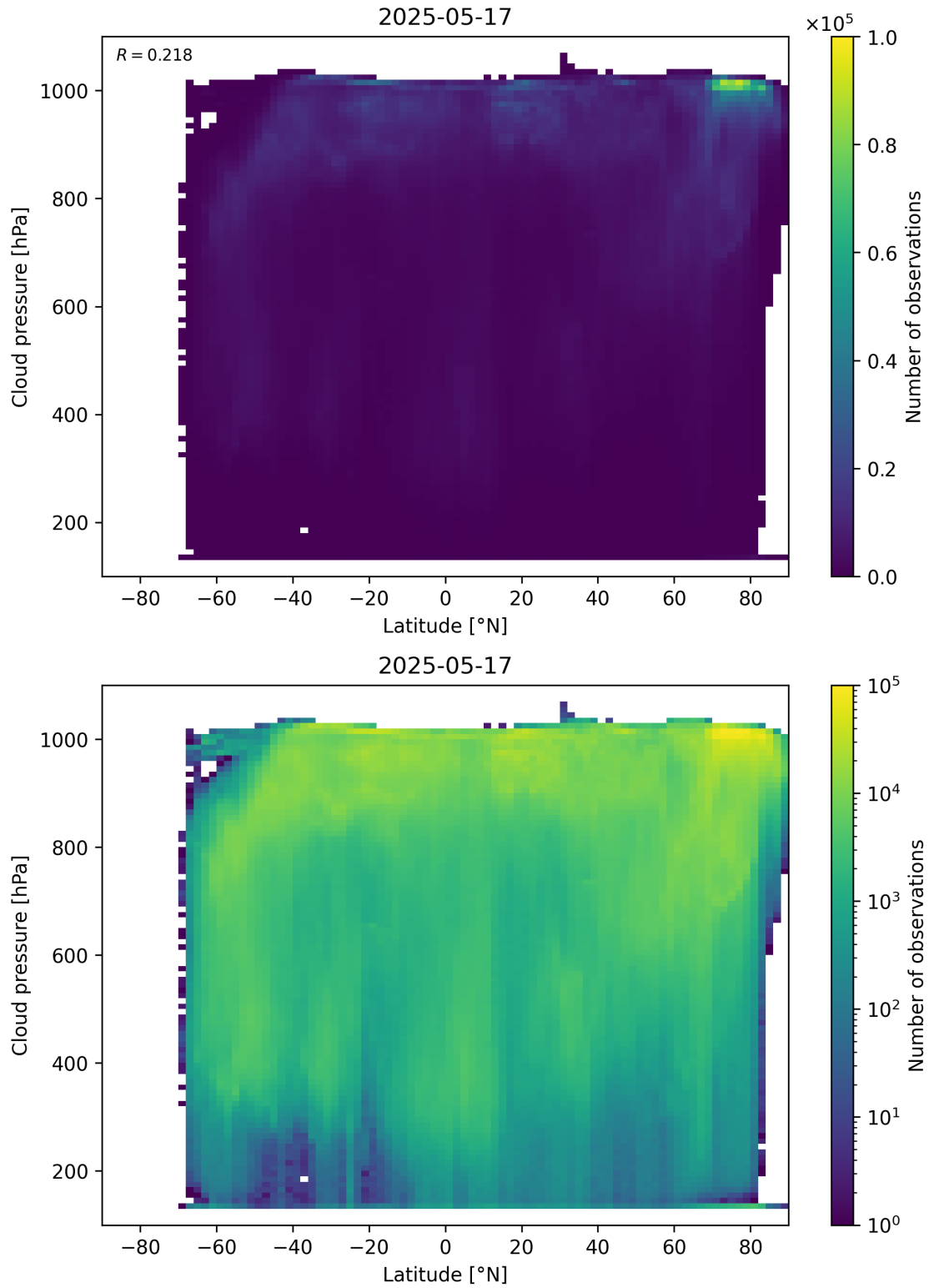
Figure 91: Scatter density plot of “Latitude” against “Cloud pressure” for 2025-05-16 to 2025-05-18.
