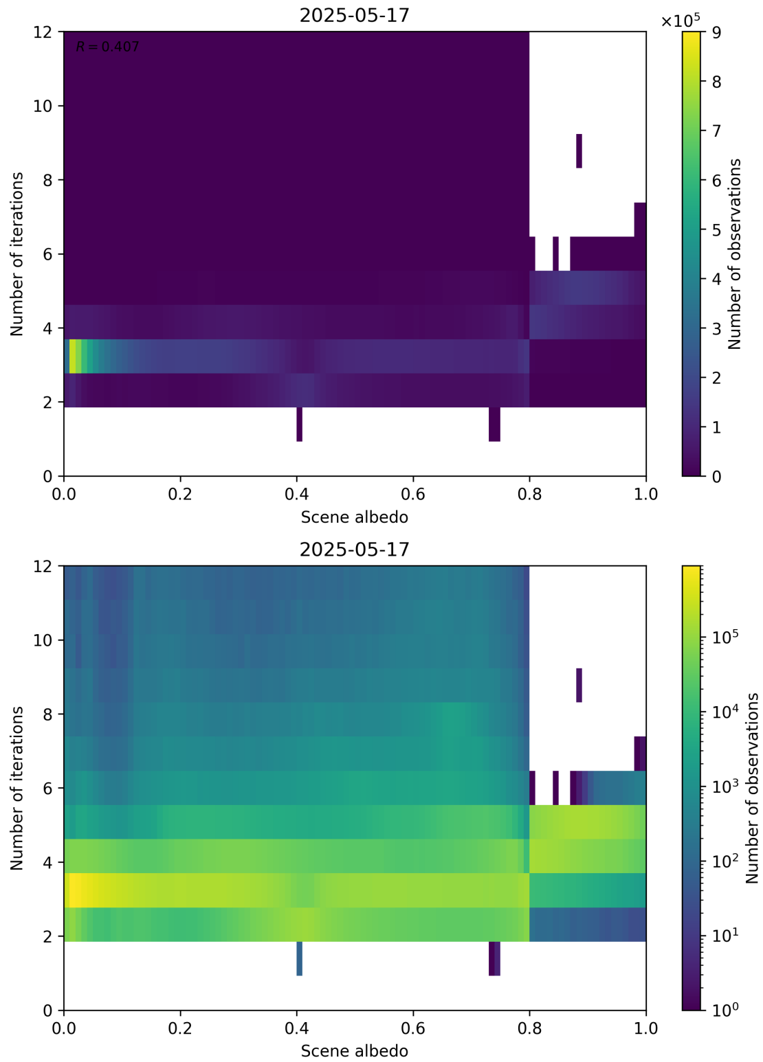
Figure 105: Scatter density plot of “Scene albedo” against “Number of iterations” for 2025-05-16 to 2025-05-18.
