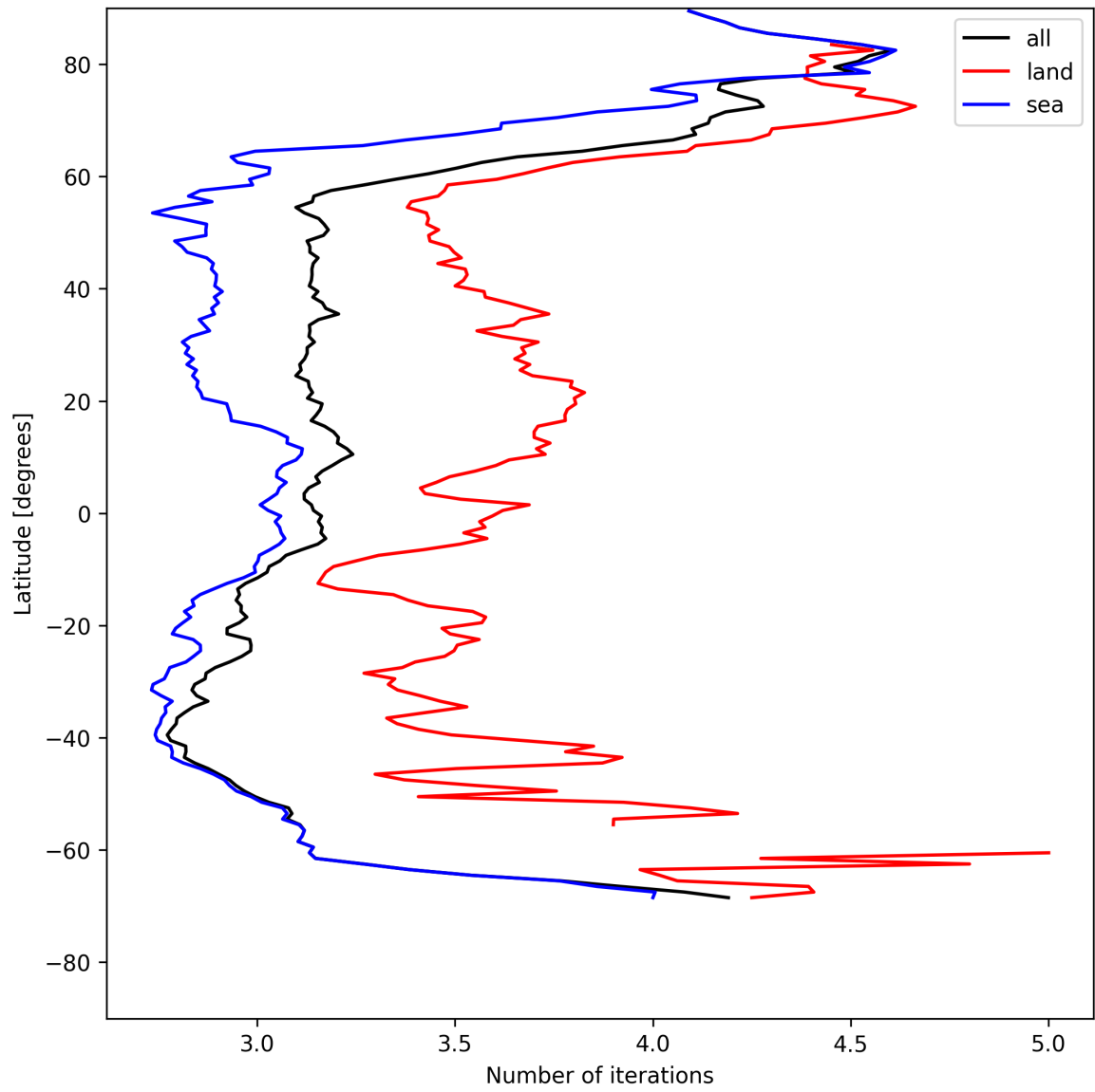
Figure 22: Zonal average of “Number of iterations” for 2025-05-16 to 2025-05-18.
