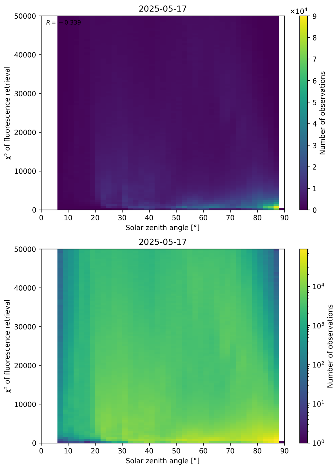
Figure 109: Scatter density plot of “Solar zenith angle” against “ \chi^2 of fluorescence retrieval” for 2025-05-16 to 2025-05-18.
