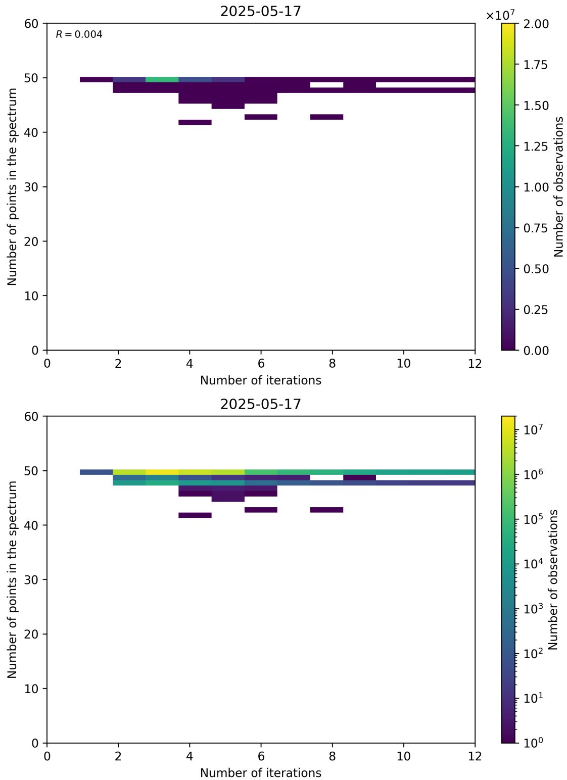
Figure 99: Scatter density plot of “Number of iterations” against “Number of points in the spectrum” for 2025-05-16 to 2025-05-18.
