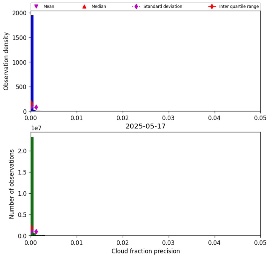
Figure 33: Histogram of “Cloud fraction precision” for 2025-05-16 to 2025-05-18
