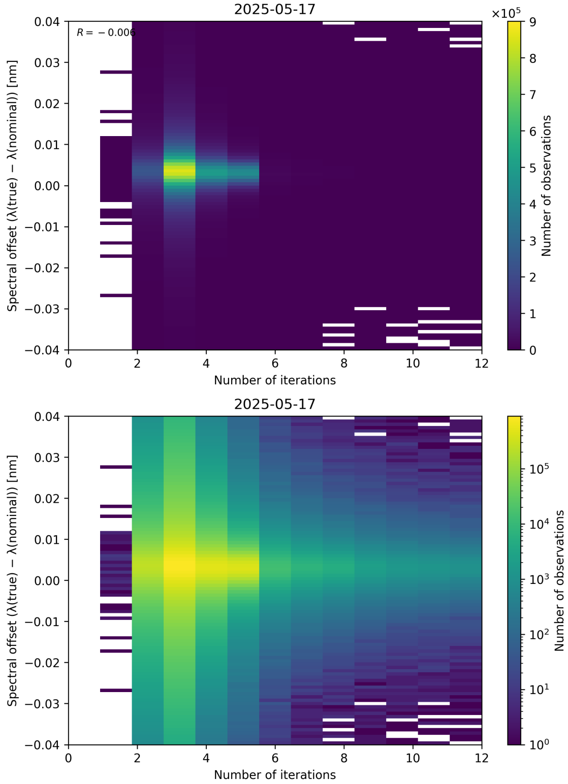
Figure 100: Scatter density plot of “Number of iterations” against “Spectral offset ( \lambda_{\text{true}} - \lambda_{\text{nominal}} )” for 2025-05-16 to 2025-05-18.
