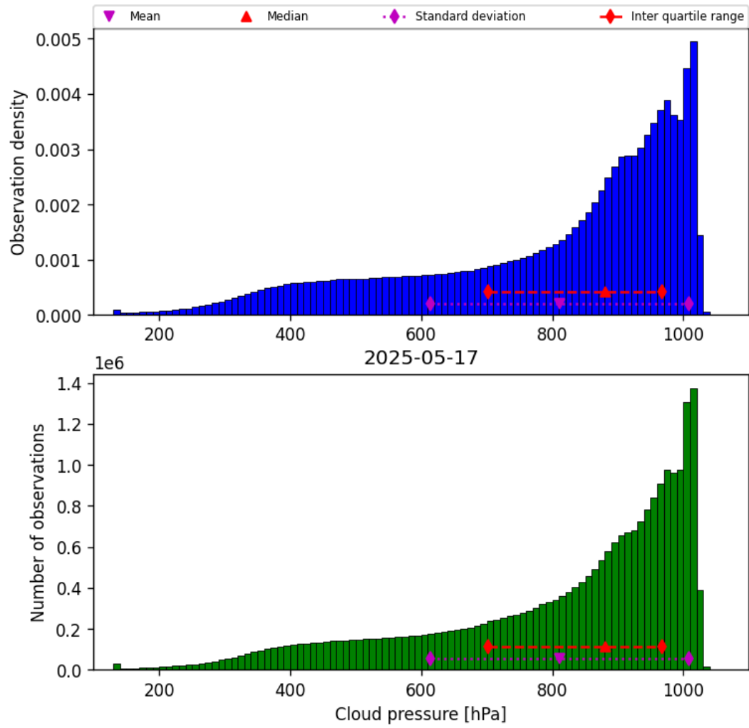
Figure 30: Histogram of “Cloud pressure” for 2025-05-16 to 2025-05-18
