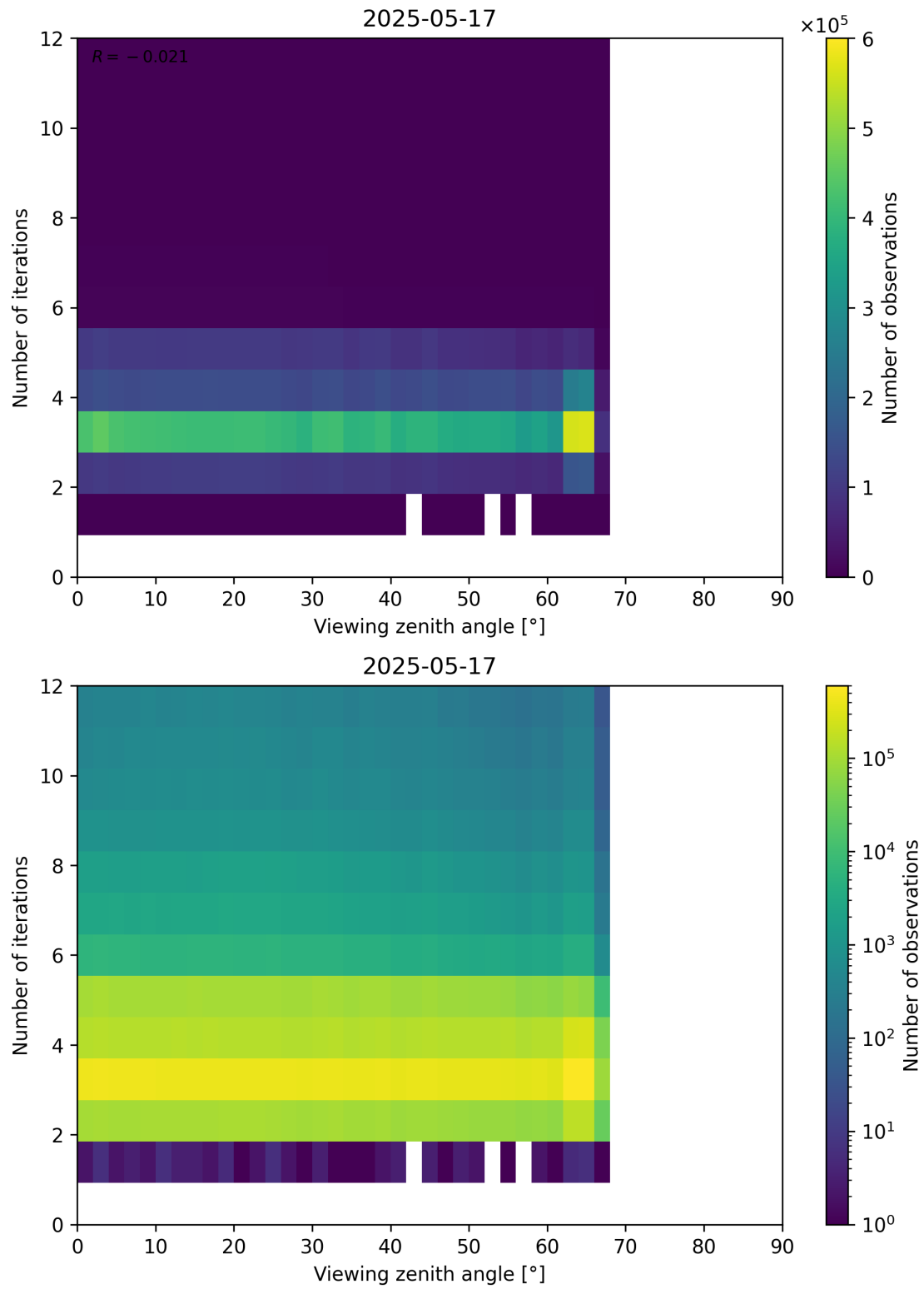
Figure 124: Scatter density plot of “Viewing zenith angle” against “Number of iterations” for 2025-05-16 to 2025-05-18.
