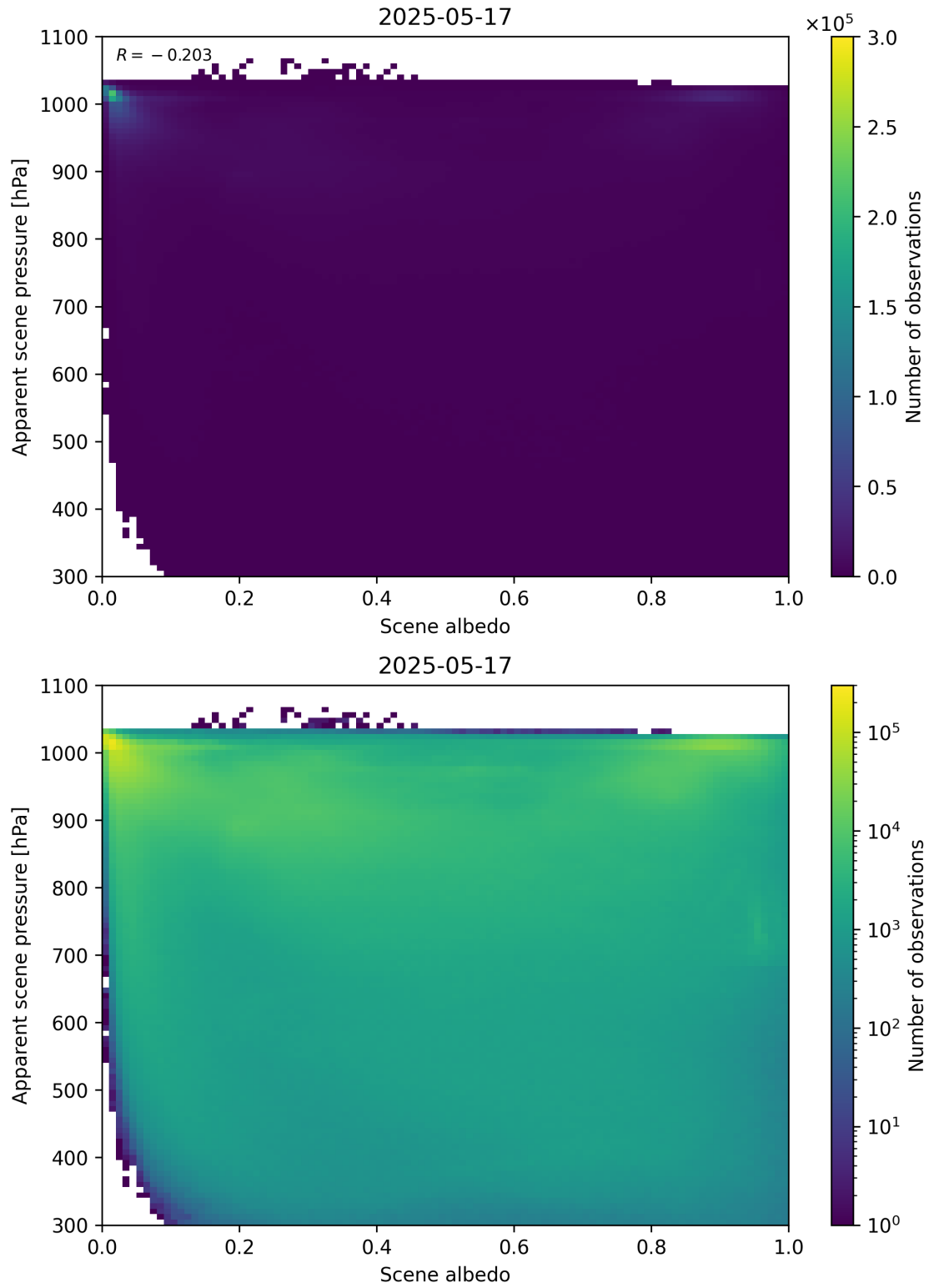
Figure 102: Scatter density plot of “Scene albedo” against “Apparent scene pressure” for 2025-05-16 to 2025-05-18.
