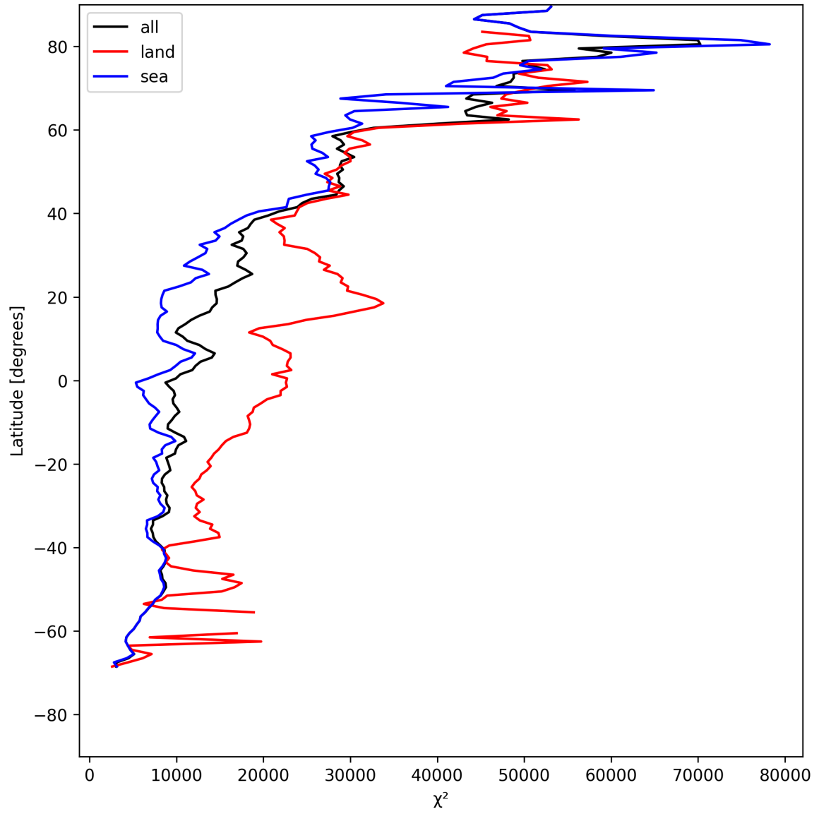
Figure 21: Zonal average of “ \chi^2 ” for 2025-05-16 to 2025-05-18.
