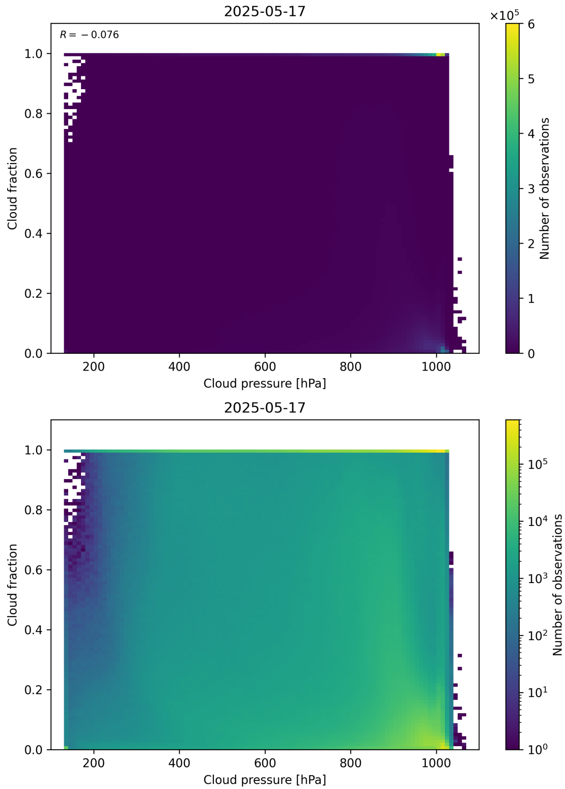
Figure 79: Scatter density plot of “Cloud pressure” against “Cloud fraction” for 2025-05-16 to 2025-05-18.
