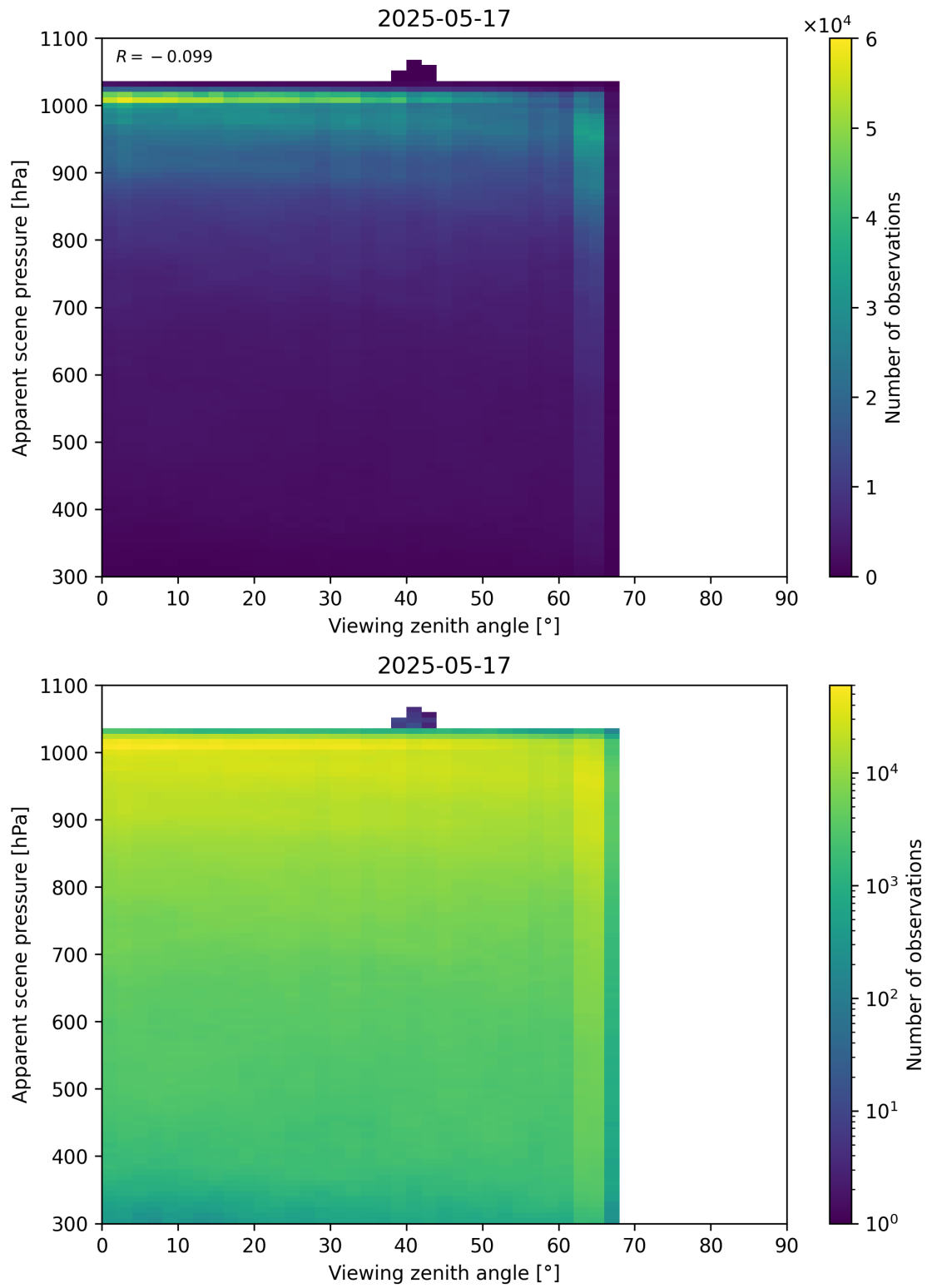
Figure 118: Scatter density plot of “Viewing zenith angle” against “Apparent scene pressure” for 2025-05-16 to 2025-05-18.
