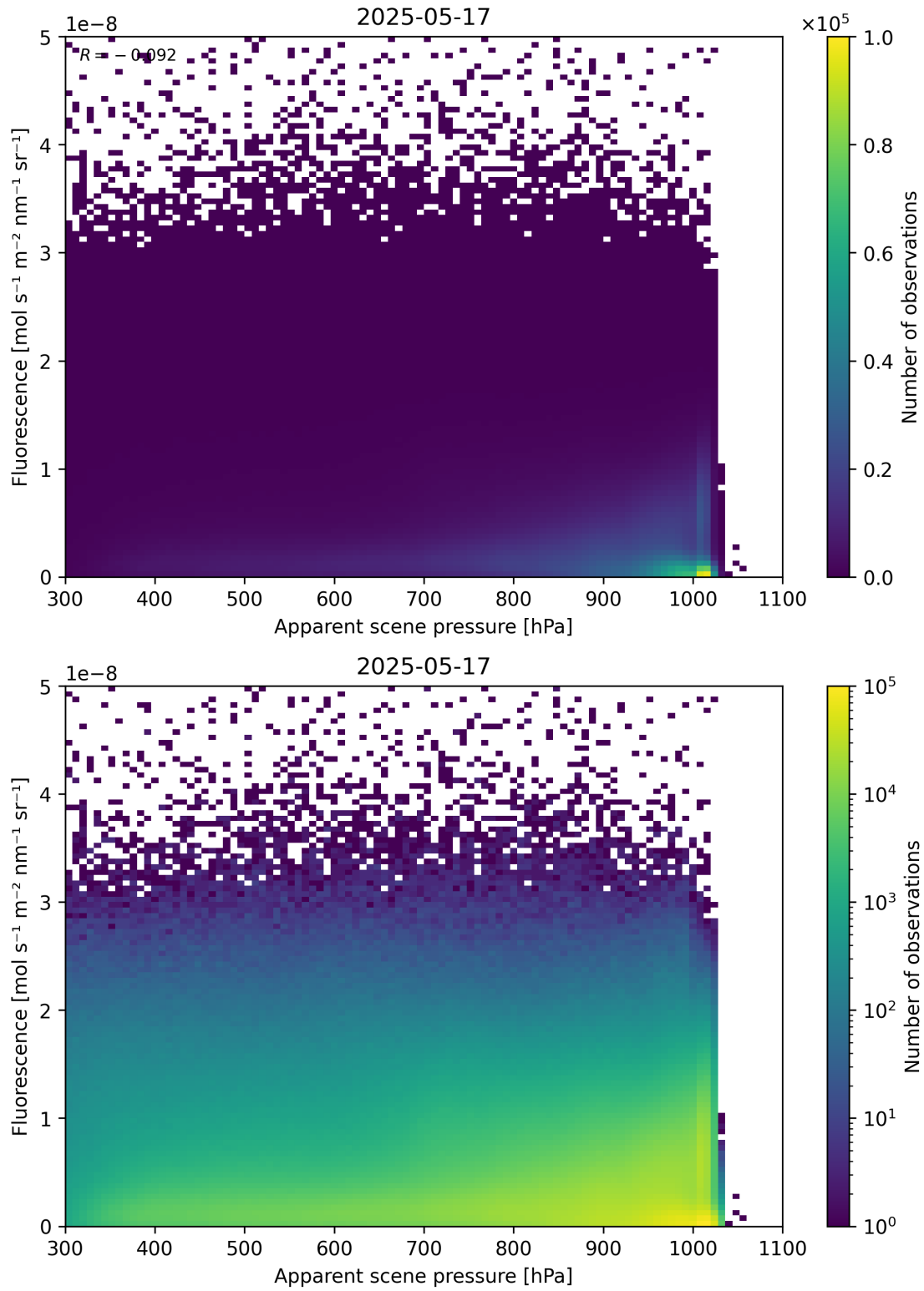
Figure 64: Scatter density plot of “Apparent scene pressure” against “Fluorescence” for 2025-05-16 to 2025-05-18.
