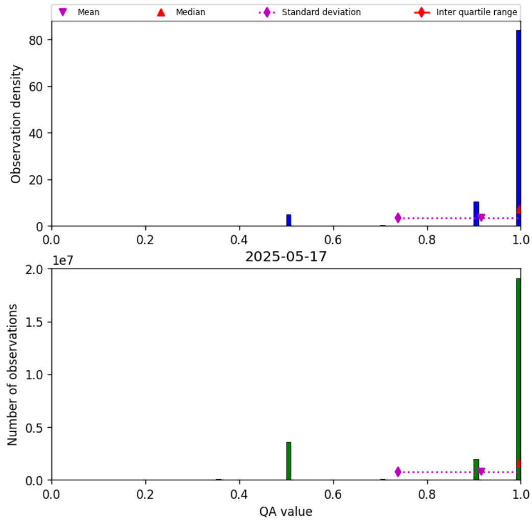
Figure 29: Histogram of “QA value” for 2025-05-16 to 2025-05-18
