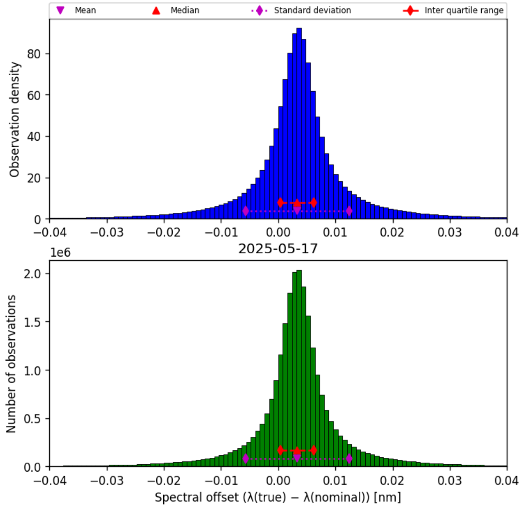
Figure 45: Histogram of “Spectral offset ( \lambda_{\text{true}} - \lambda_{\text{nominal}} )” for 2025-05-16 to 2025-05-18
