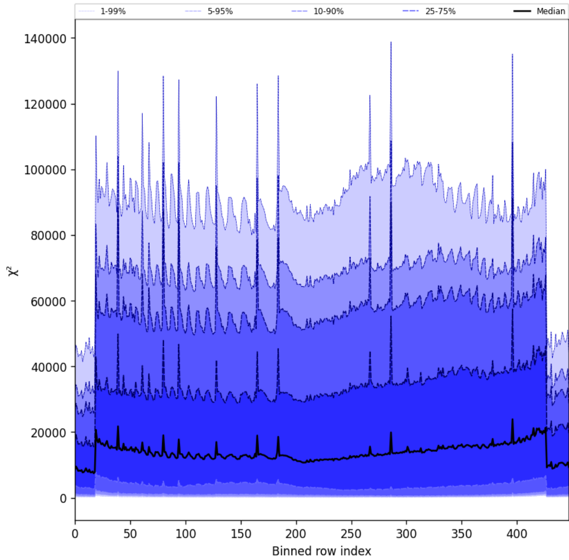
Figure 55: Along track statistics of “ \chi^2 ” for 2025-05-16 to 2025-05-18
