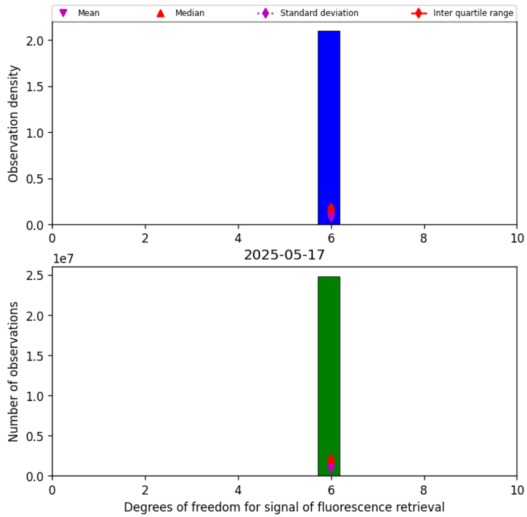
Figure 43: Histogram of “Degrees of freedom for signal of fluorescence retrieval” for 2025-05-16 to 2025-05-18
