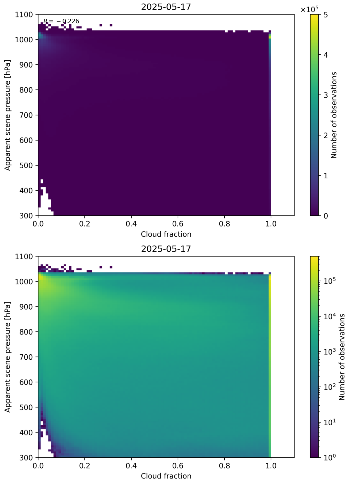
Figure 70: Scatter density plot of “Cloud fraction” against “Apparent scene pressure” for 2025-05-16 to 2025-05-18.
