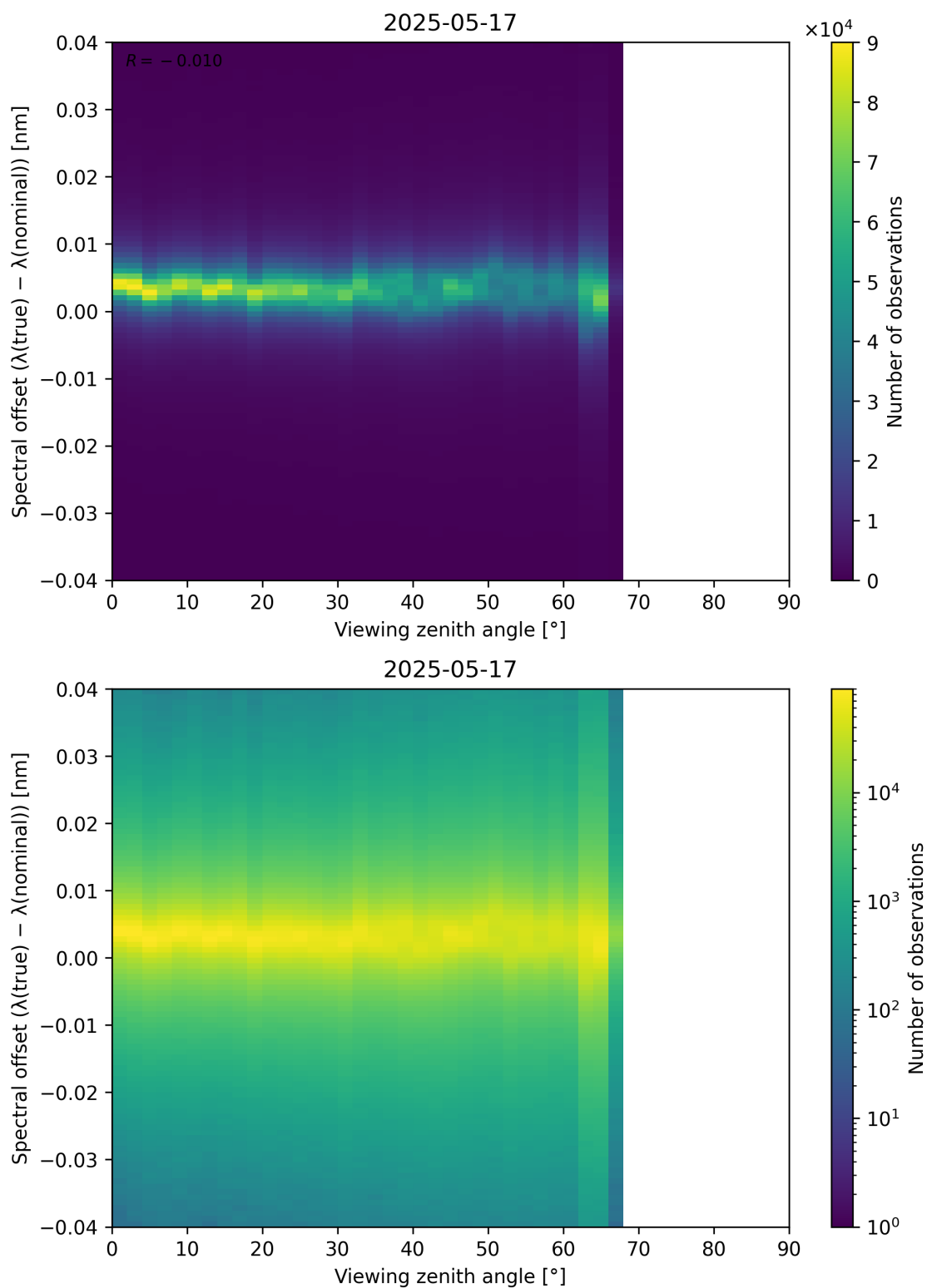
Figure 128: Scatter density plot of “Viewing zenith angle” against “Spectral offset ( \lambda_{\text{true}} - \lambda_{\text{nominal}} )” for 2025-05-16 to 2025-05-18.
