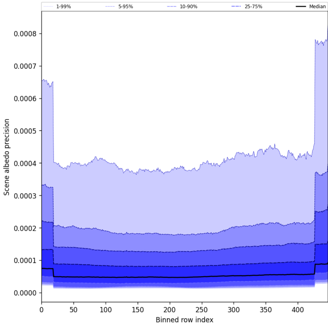
Figure 52: Along track statistics of “Scene albedo precision” for 2025-05-16 to 2025-05-18
