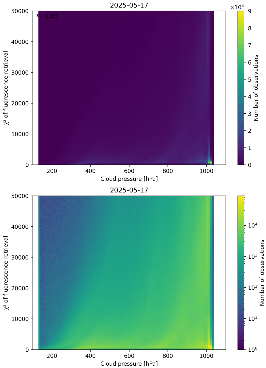
Figure 78: Scatter density plot of “Cloud pressure” against “ \chi^2 of fluorescence retrieval” for 2025-05-16 to 2025-05-18.
