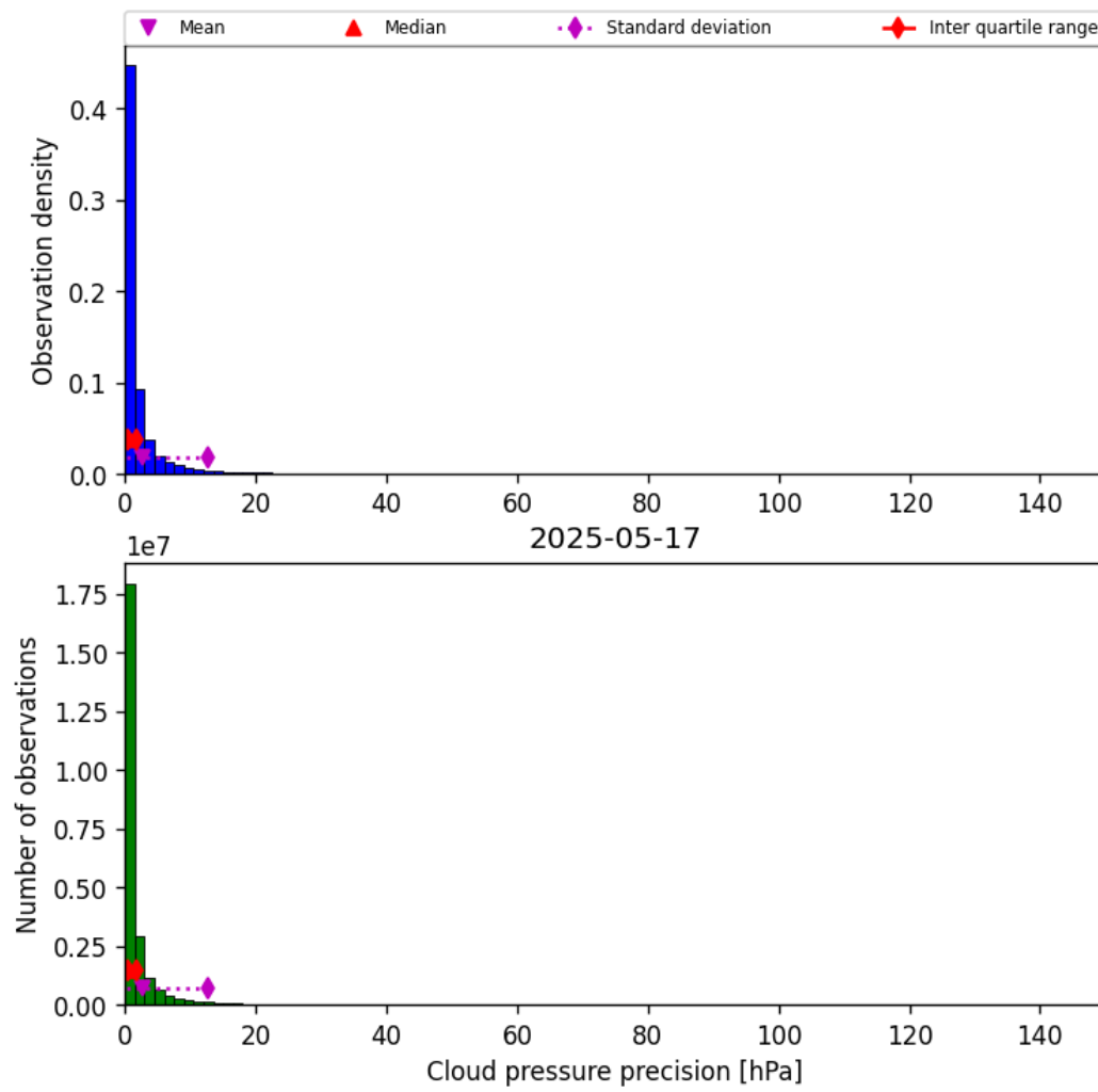
Figure 31: Histogram of “Cloud pressure precision” for 2025-05-16 to 2025-05-18
