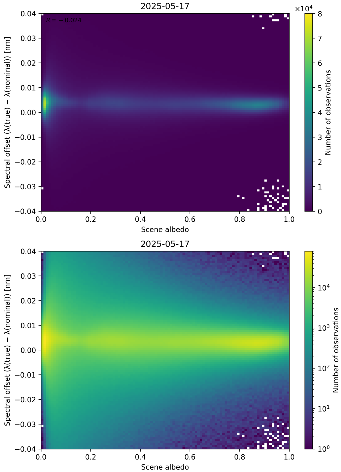
Figure 107: Scatter density plot of “Scene albedo” against “Spectral offset ( \lambda_{\text{true}} - \lambda_{\text{nominal}} )” for 2025-05-16 to 2025-05-18.
