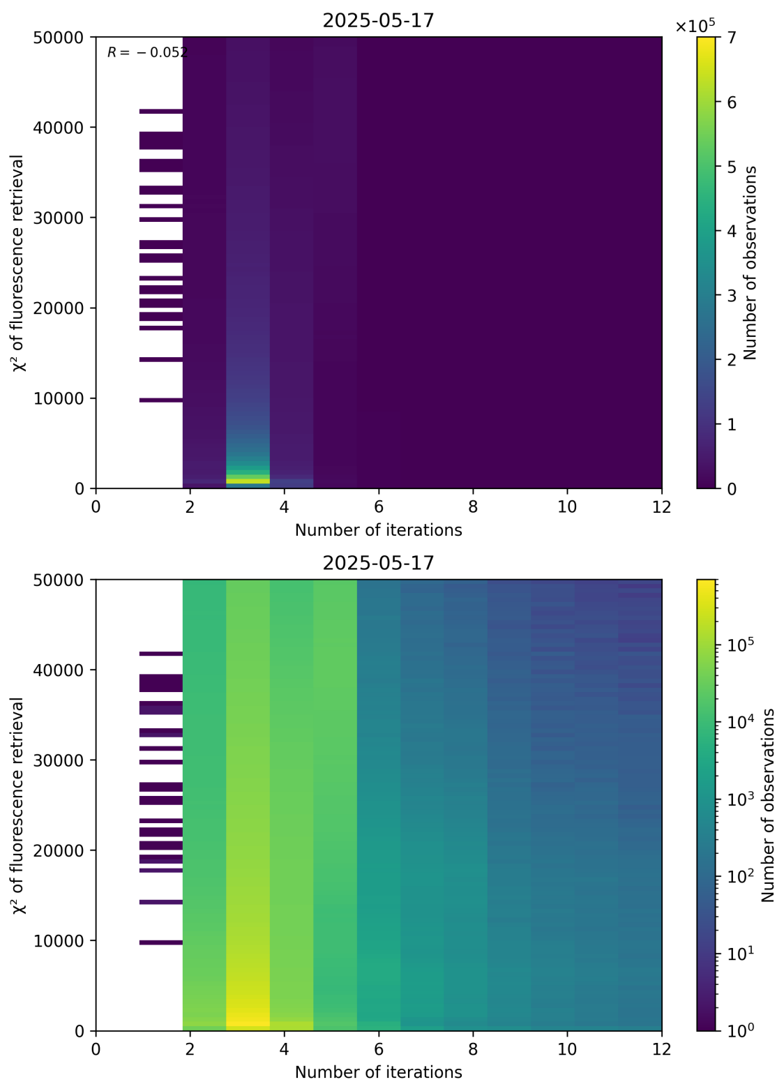
Figure 97: Scatter density plot of “Number of iterations” against “ \chi^2 of fluorescence retrieval” for 2025-05-16 to 2025-05-18.
