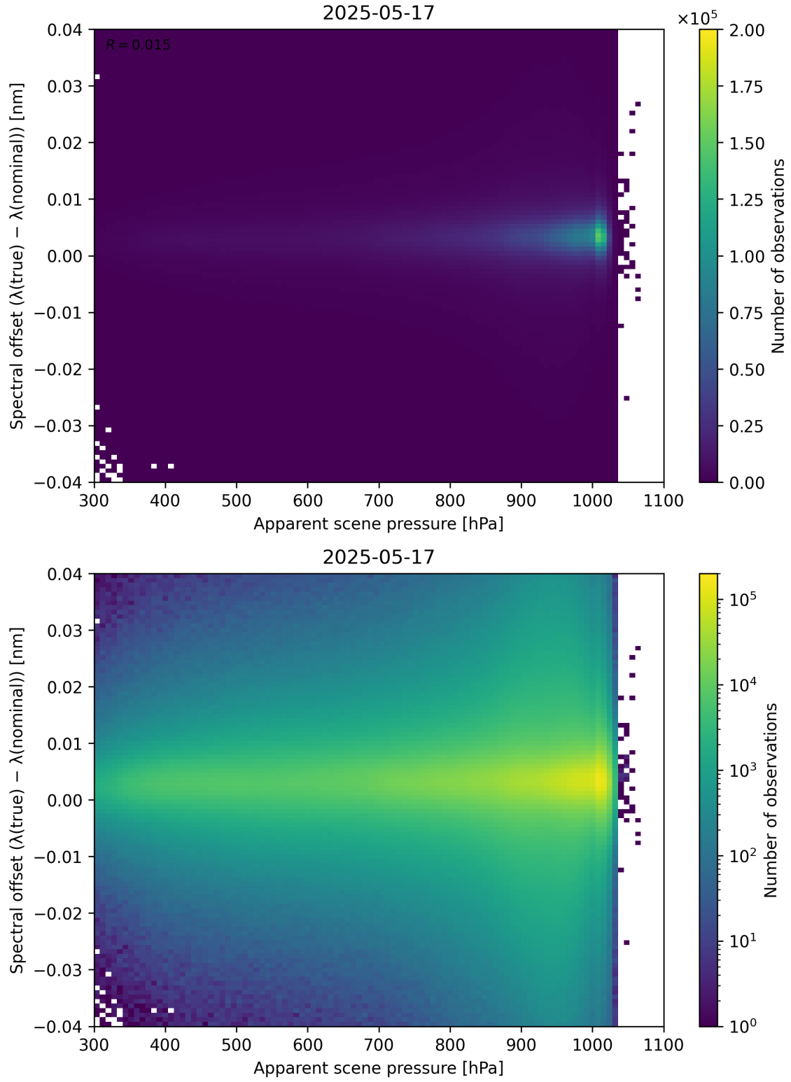
Figure 67: Scatter density plot of “Apparent scene pressure” against “Spectral offset ( \lambda_{\text{true}} - \lambda_{\text{nominal}} )” for 2025-05-16 to 2025-05-18.
