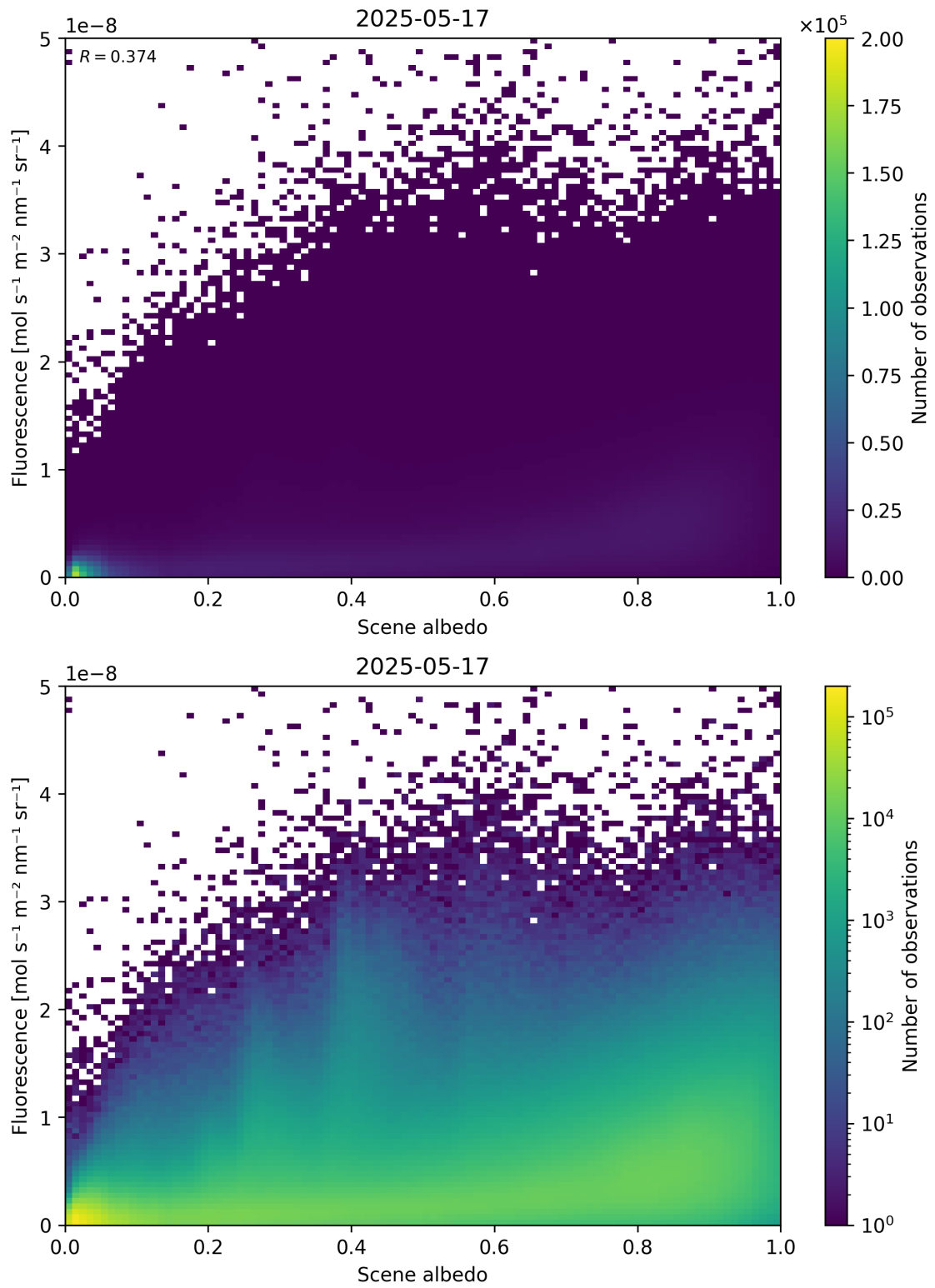
Figure 104: Scatter density plot of “Scene albedo” against “Fluorescence” for 2025-05-16 to 2025-05-18.
