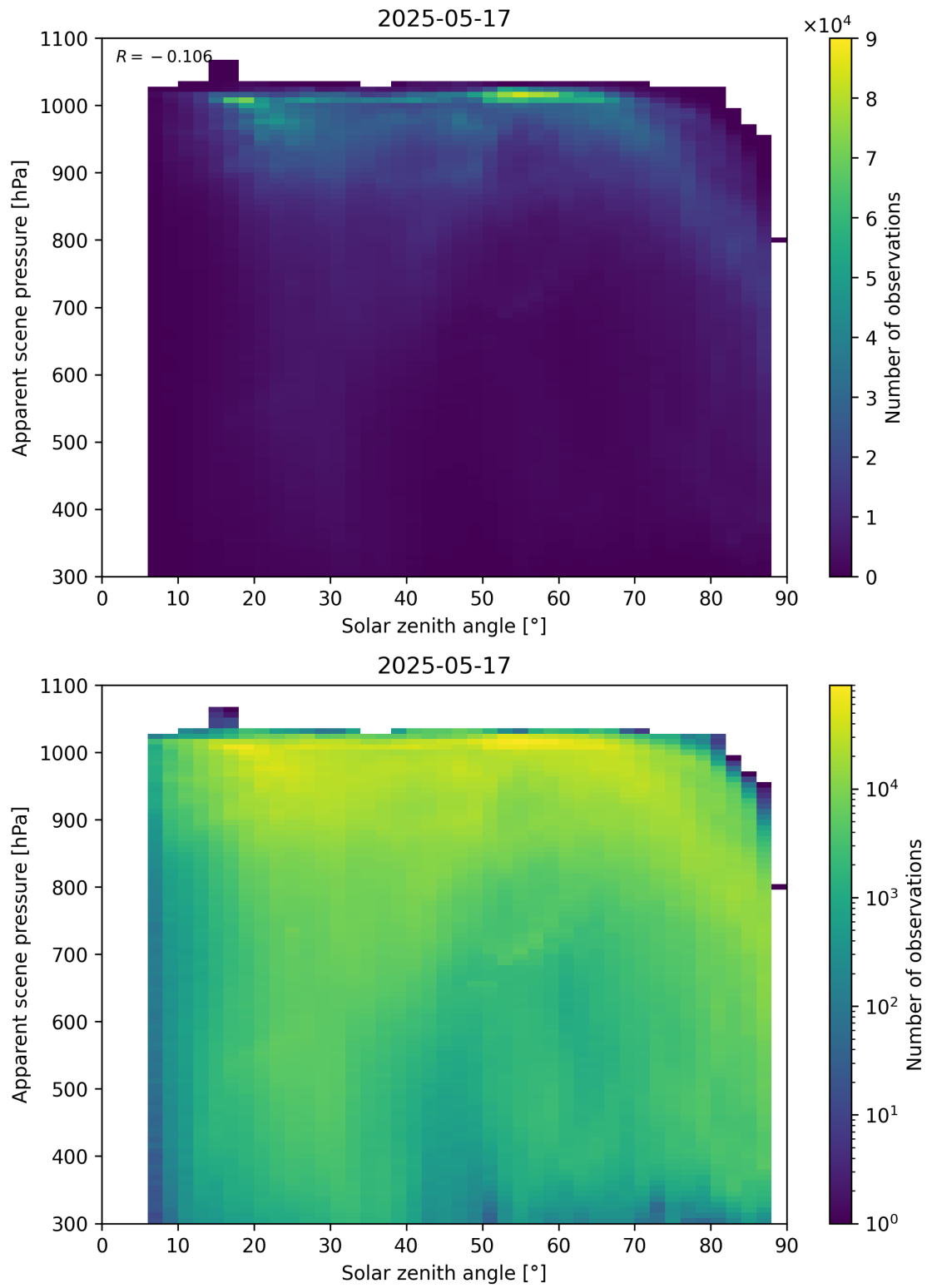
Figure 108: Scatter density plot of “Solar zenith angle” against “Apparent scene pressure” for 2025-05-16 to 2025-05-18.
