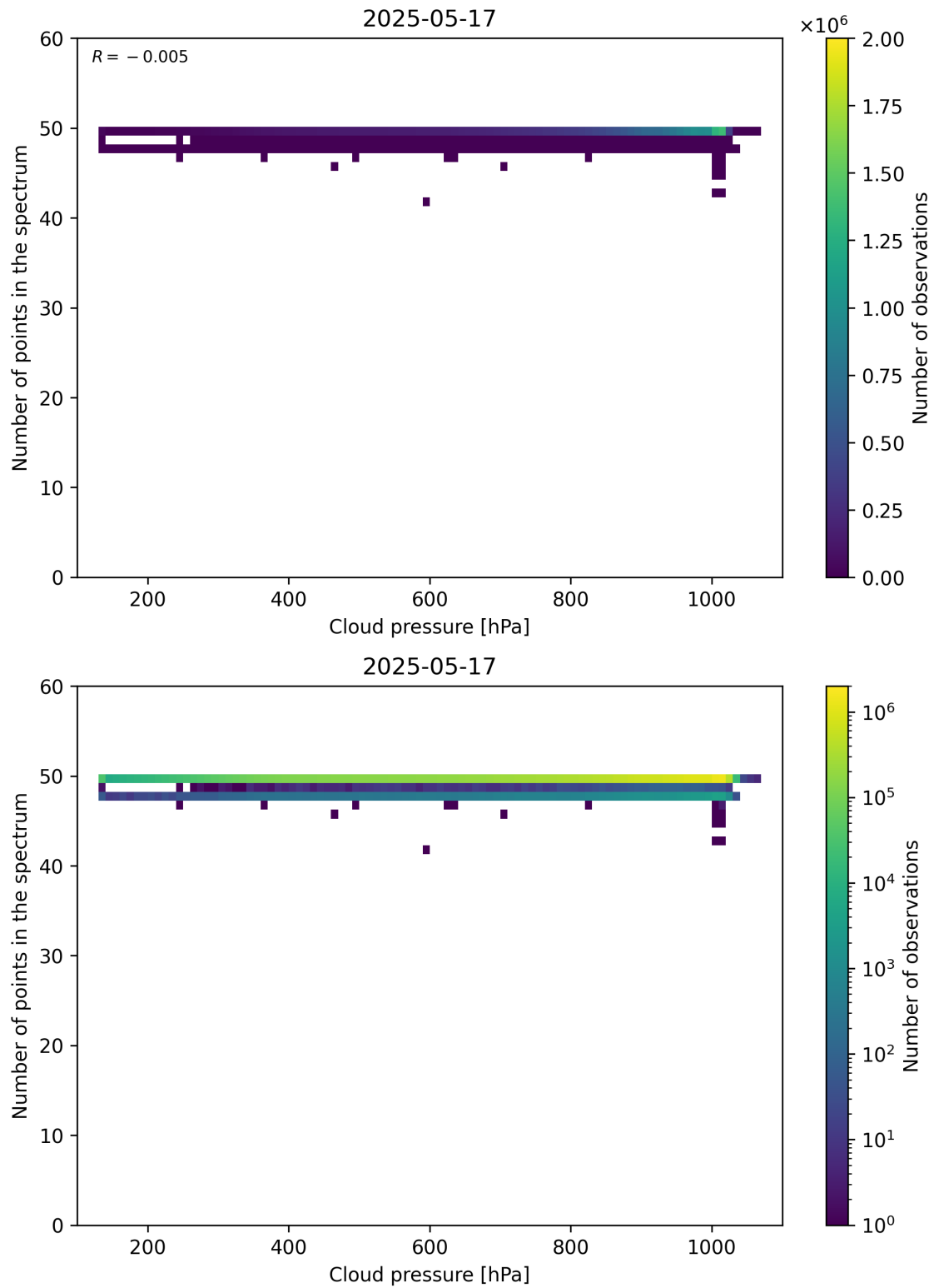
Figure 82: Scatter density plot of “Cloud pressure” against “Number of points in the spectrum” for 2025-05-16 to 2025-05-18.
