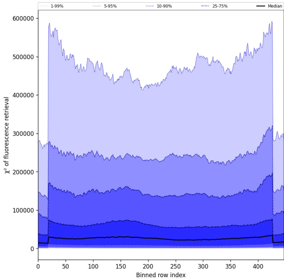
Figure 59: Along track statistics of “ \chi^2 of fluorescence retrieval” for 2025-05-16 to 2025-05-18
