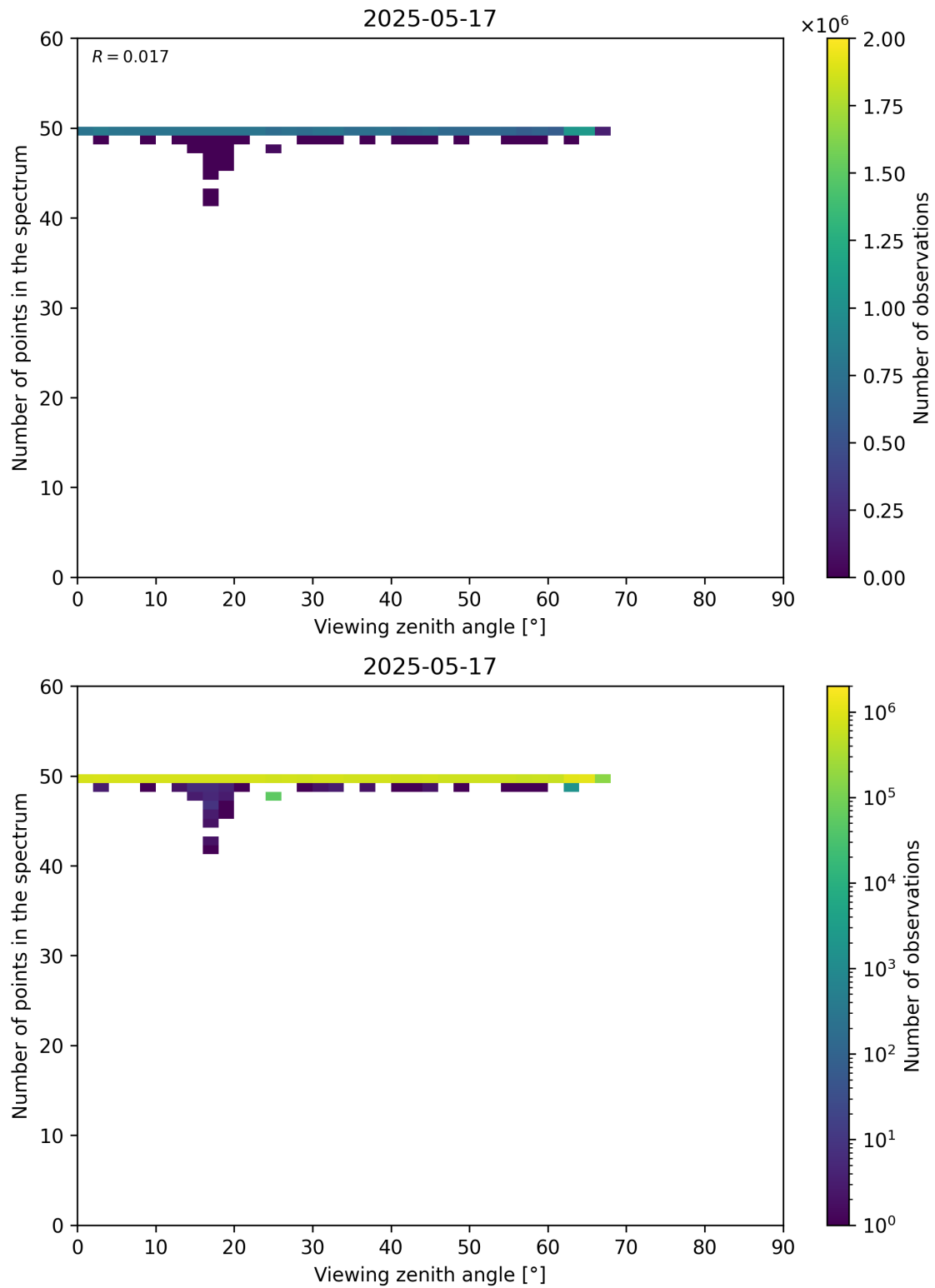
Figure 125: Scatter density plot of “Viewing zenith angle” against “Number of points in the spectrum” for 2025-05-16 to 2025-05-18.
