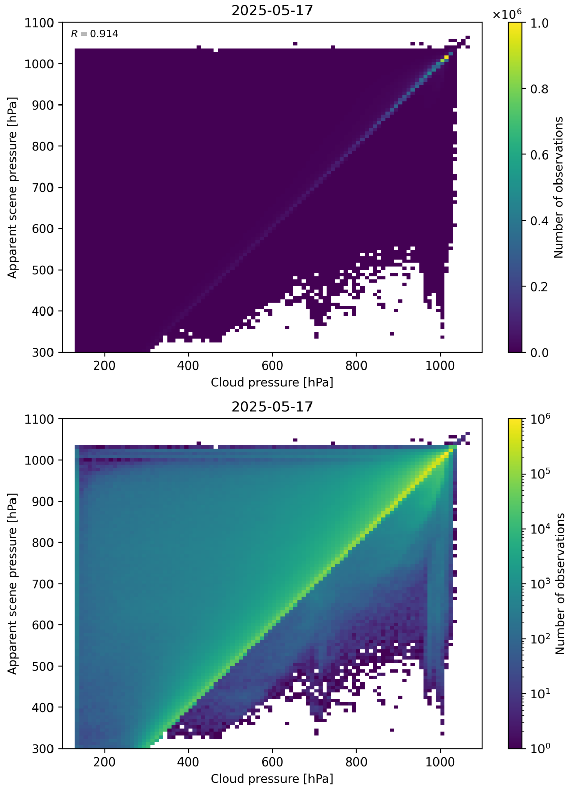
Figure 77: Scatter density plot of “Cloud pressure” against “Apparent scene pressure” for 2025-05-16 to 2025-05-18.
