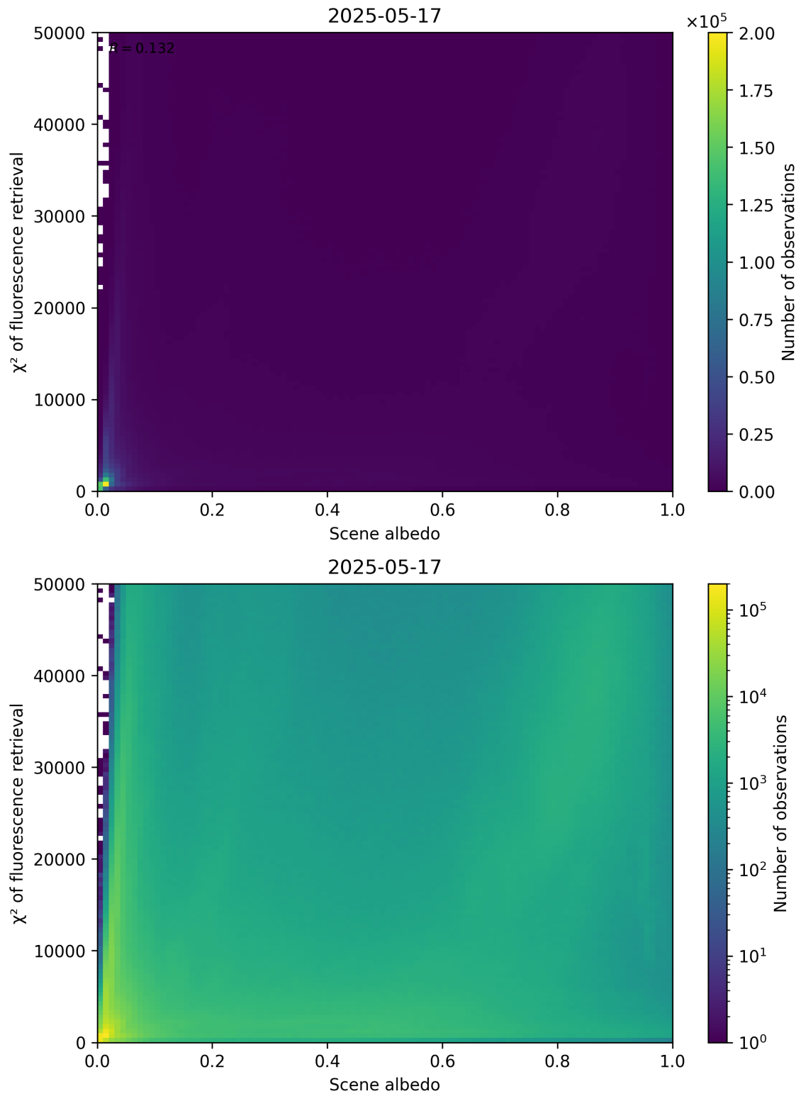
Figure 103: Scatter density plot of “Scene albedo” against “ \chi^2 of fluorescence retrieval” for 2025-05-16 to 2025-05-18.
