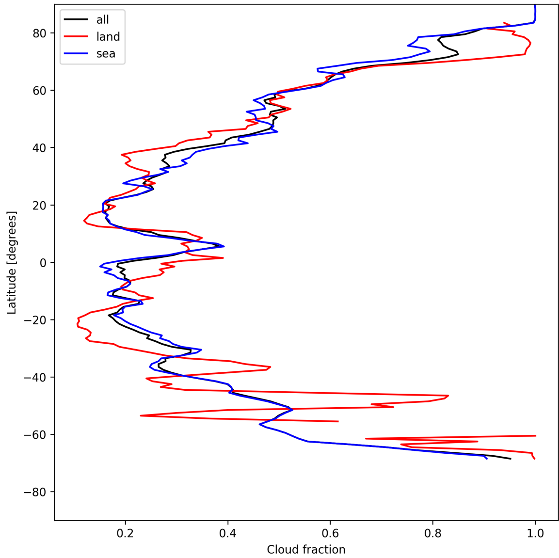
Figure 15: Zonal average of “Cloud fraction” for 2025-05-16 to 2025-05-18.
