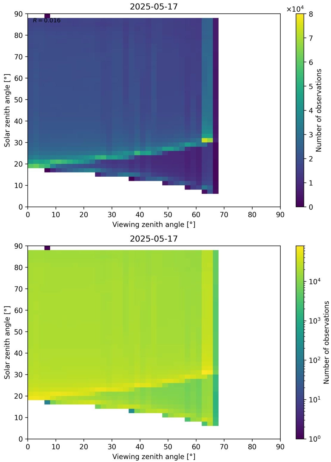
Figure 127: Scatter density plot of “Viewing zenith angle” against “Solar zenith angle” for 2025-05-16 to 2025-05-18.
