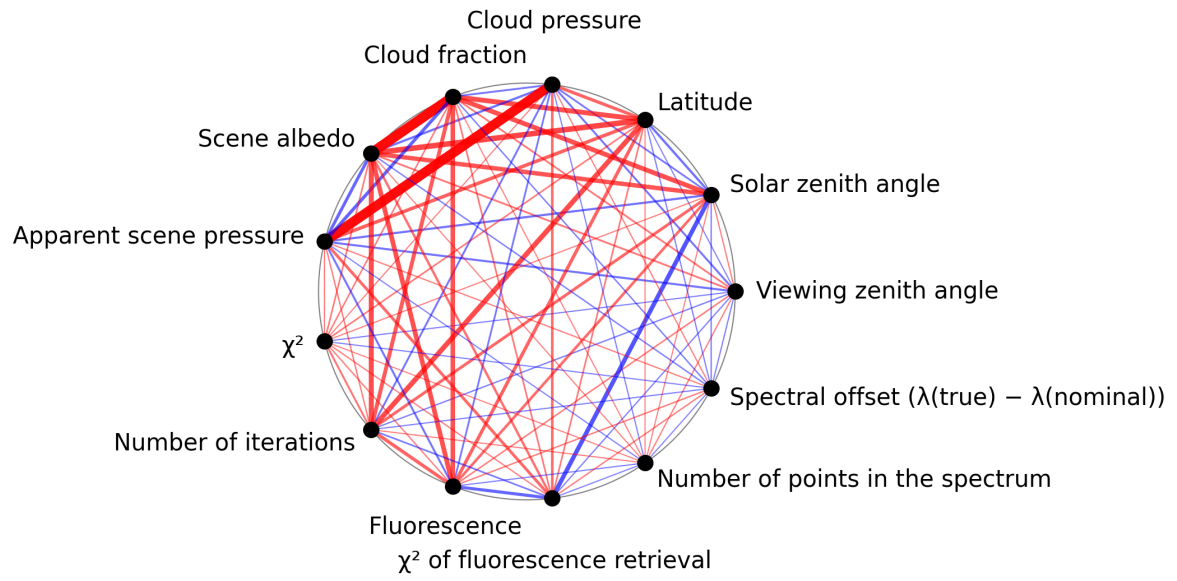
Figure 1: Map of correlation graph for 2025-05-16 to 2025-05-18.
