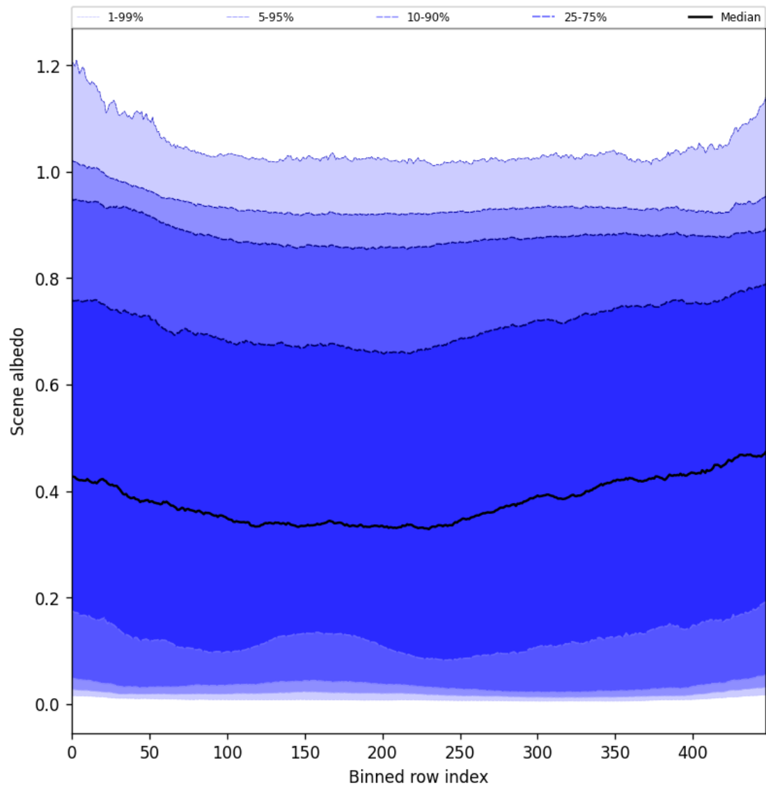
Figure 51: Along track statistics of “Scene albedo” for 2025-05-16 to 2025-05-18
