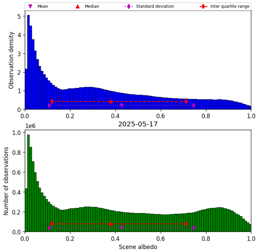
Figure 34: Histogram of “Scene albedo” for 2025-05-16 to 2025-05-18
