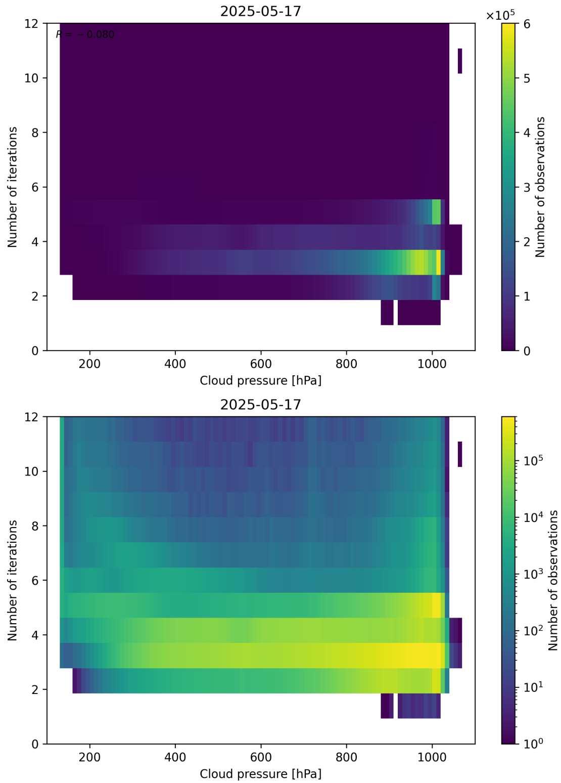
Figure 81: Scatter density plot of “Cloud pressure” against “Number of iterations” for 2025-05-16 to 2025-05-18.
