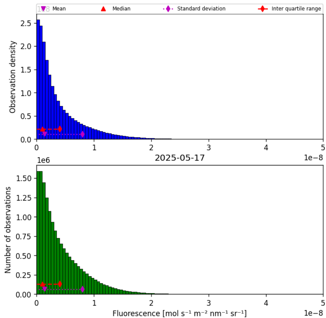
Figure 40: Histogram of “Fluorescence” for 2025-05-16 to 2025-05-18
