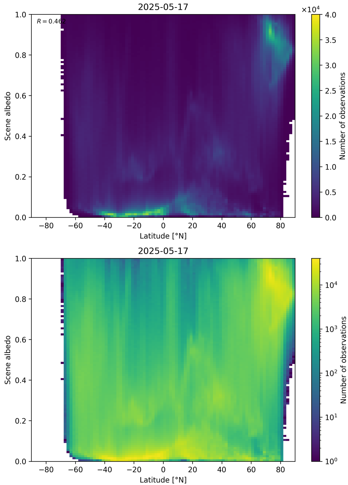
Figure 95: Scatter density plot of “Latitude” against “Scene albedo” for 2025-05-16 to 2025-05-18.
