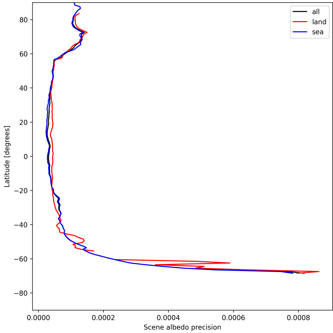
Figure 18: Zonal average of “Scene albedo precision” for 2025-05-16 to 2025-05-18.
