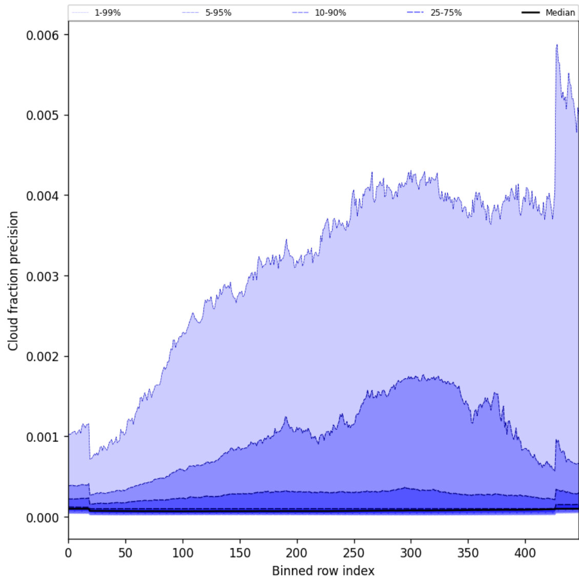
Figure 50: Along track statistics of “Cloud fraction precision” for 2025-05-16 to 2025-05-18
