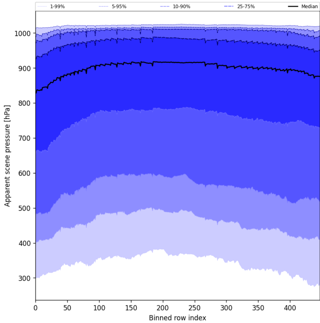
Figure 53: Along track statistics of “Apparent scene pressure” for 2025-05-16 to 2025-05-18
