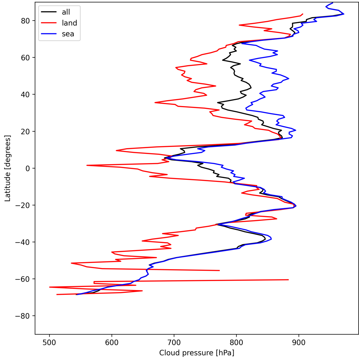
Figure 13: Zonal average of “Cloud pressure” for 2025-05-16 to 2025-05-18.
