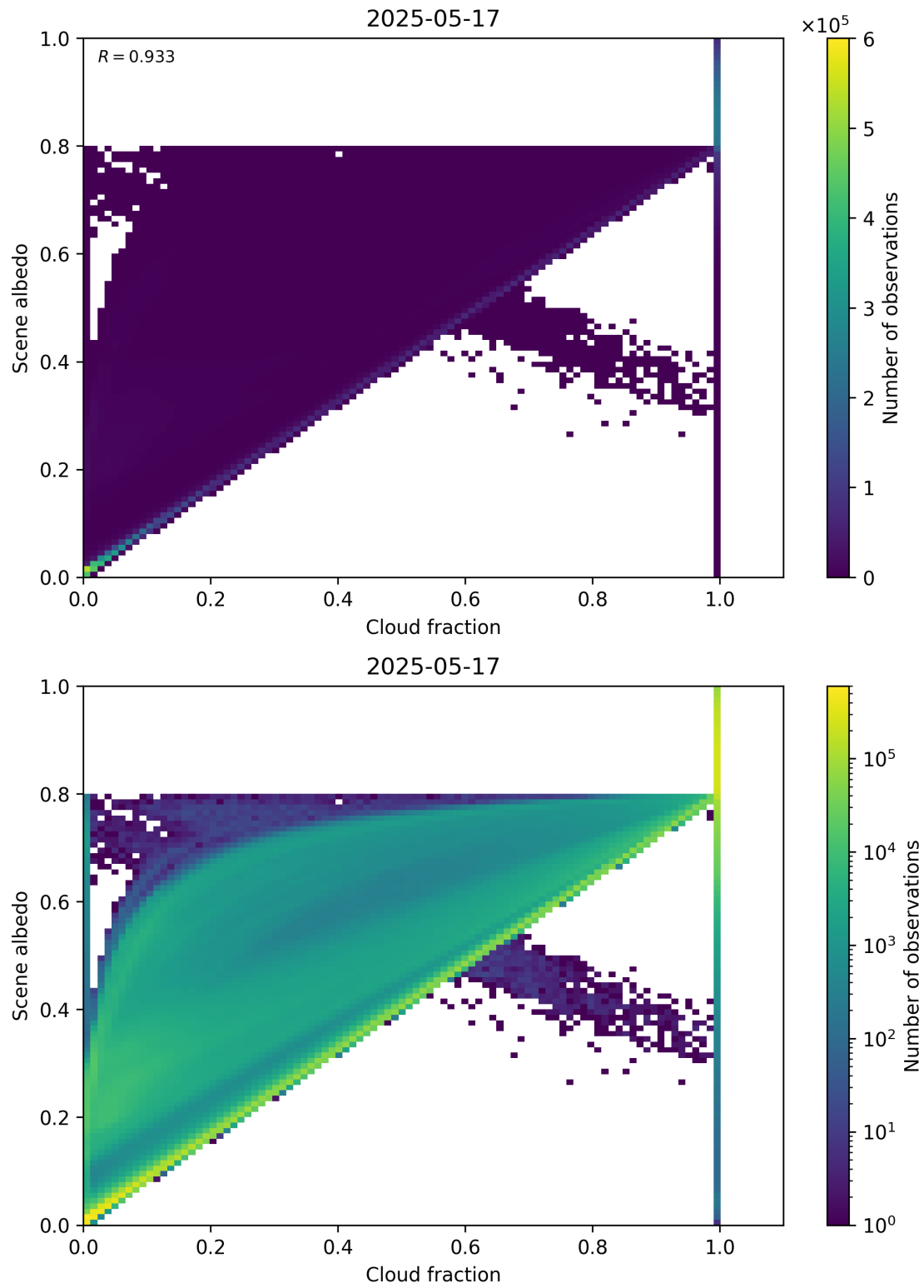
Figure 75: Scatter density plot of “Cloud fraction” against “Scene albedo” for 2025-05-16 to 2025-05-18.
