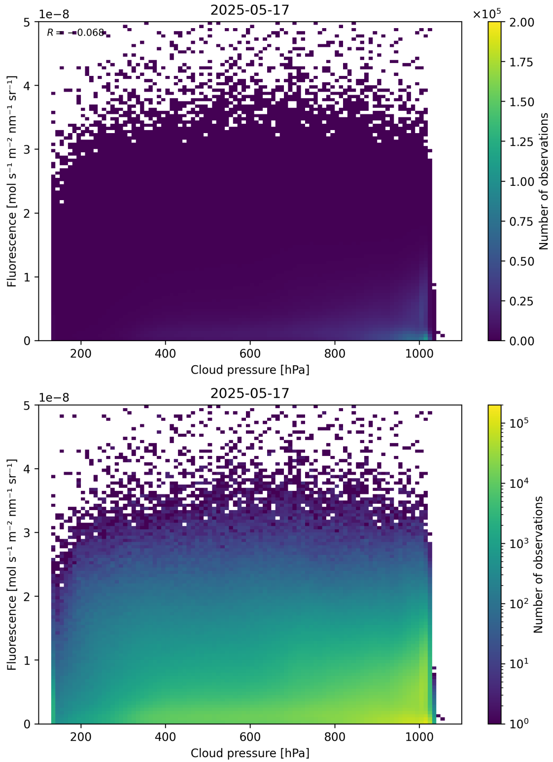
Figure 80: Scatter density plot of “Cloud pressure” against “Fluorescence” for 2025-05-16 to 2025-05-18.
