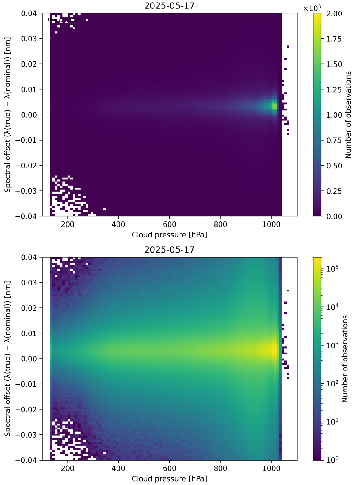
Figure 84: Scatter density plot of “Cloud pressure” against “Spectral offset ( \lambda_{\text{true}} - \lambda_{\text{nominal}} )” for 2025-05-16 to 2025-05-18.
