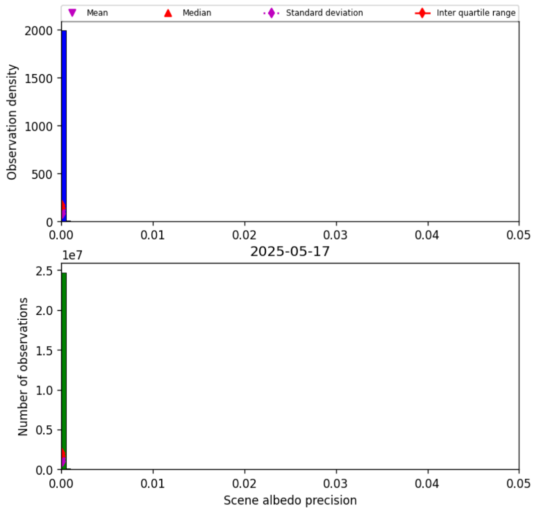
Figure 35: Histogram of “Scene albedo precision” for 2025-05-16 to 2025-05-18
