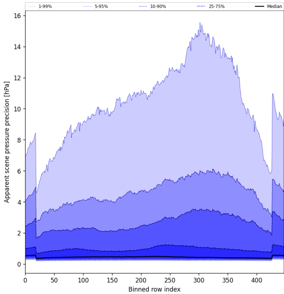
Figure 54: Along track statistics of “Apparent scene pressure precision” for 2025-05-16 to 2025-05-18
