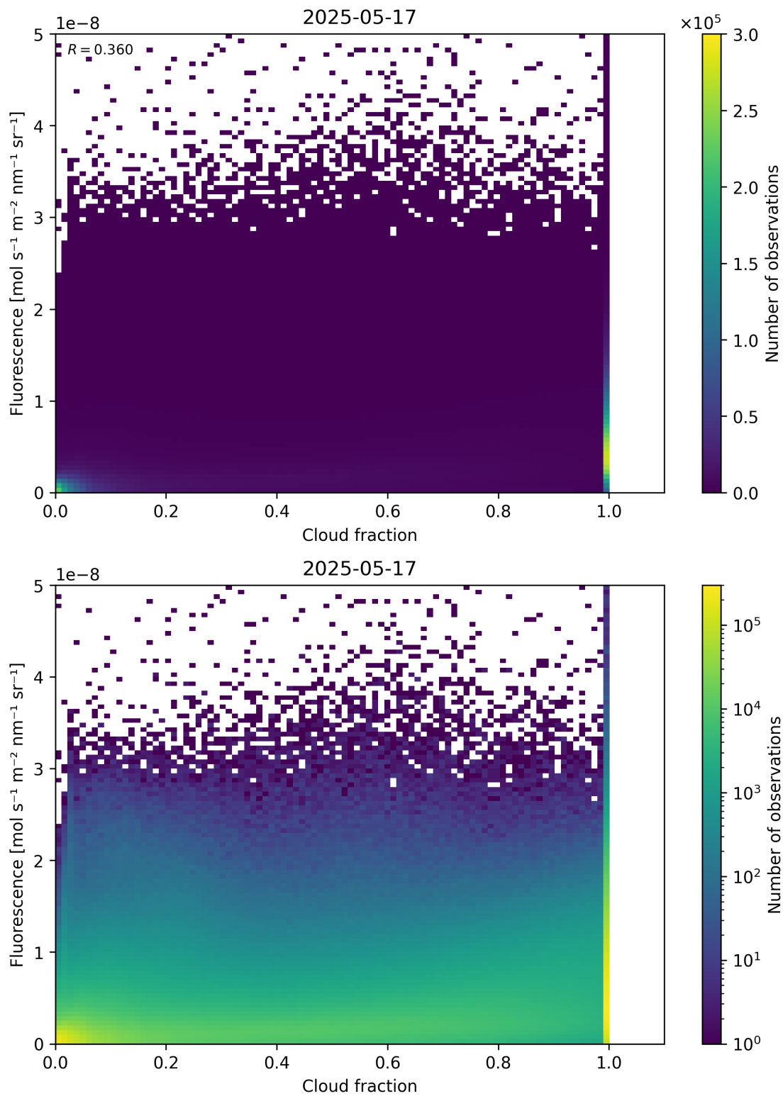
Figure 72: Scatter density plot of “Cloud fraction” against “Fluorescence” for 2025-05-16 to 2025-05-18.
