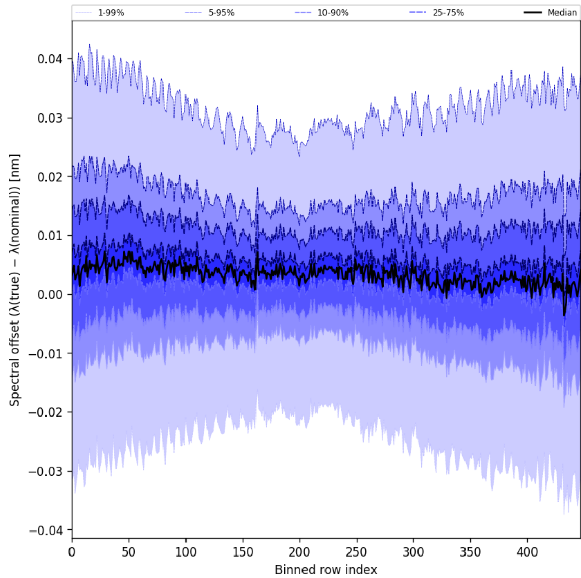
Figure 62: Along track statistics of “Spectral offset ( \lambda_{\text{true}} - \lambda_{\text{nominal}} )” for 2025-05-16 to 2025-05-18
