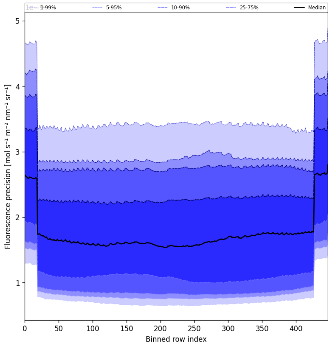
Figure 58: Along track statistics of “Fluorescence precision” for 2025-05-16 to 2025-05-18
