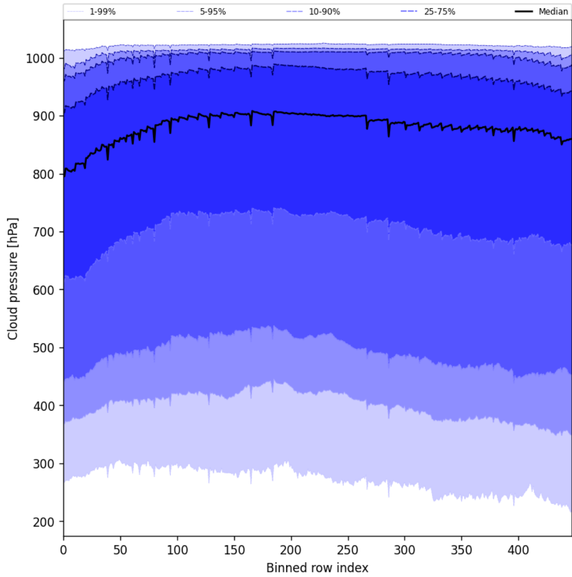
Figure 47: Along track statistics of “Cloud pressure” for 2025-05-16 to 2025-05-18
