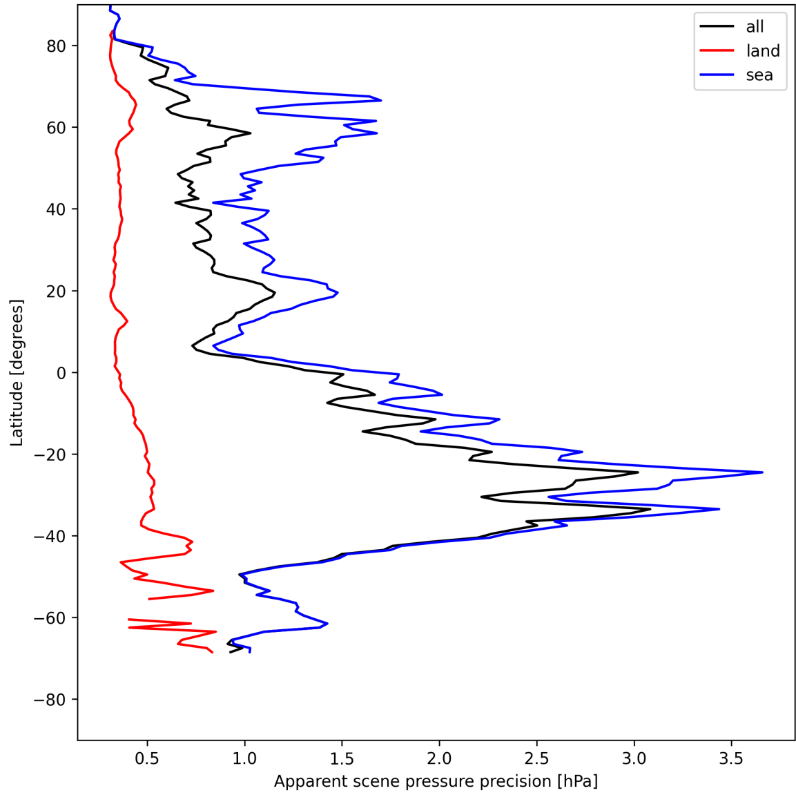
Figure 20: Zonal average of “Apparent scene pressure precision” for 2025-05-16 to 2025-05-18.
