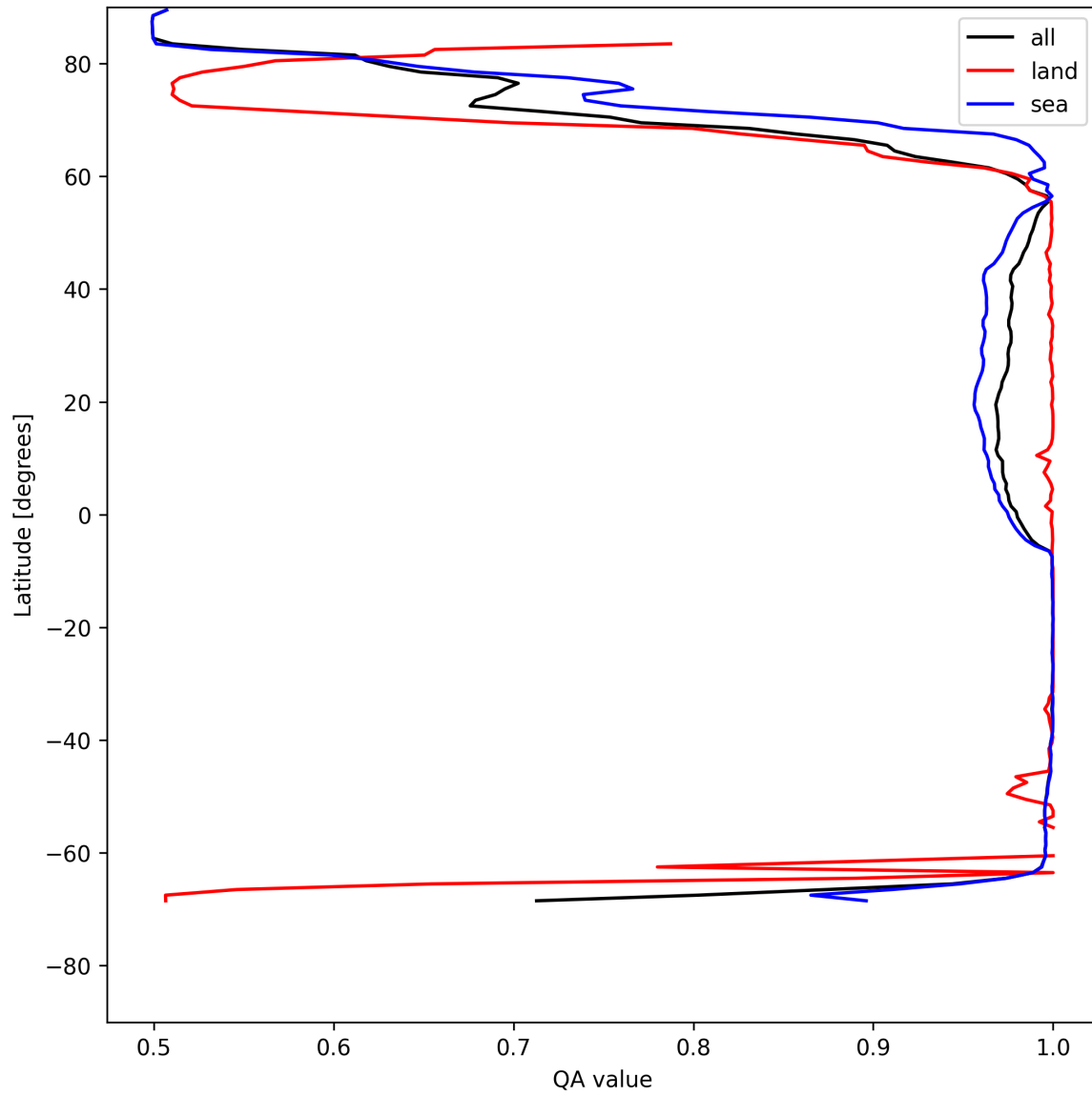
Figure 12: Zonal average of “QA value” for 2025-05-16 to 2025-05-18.
