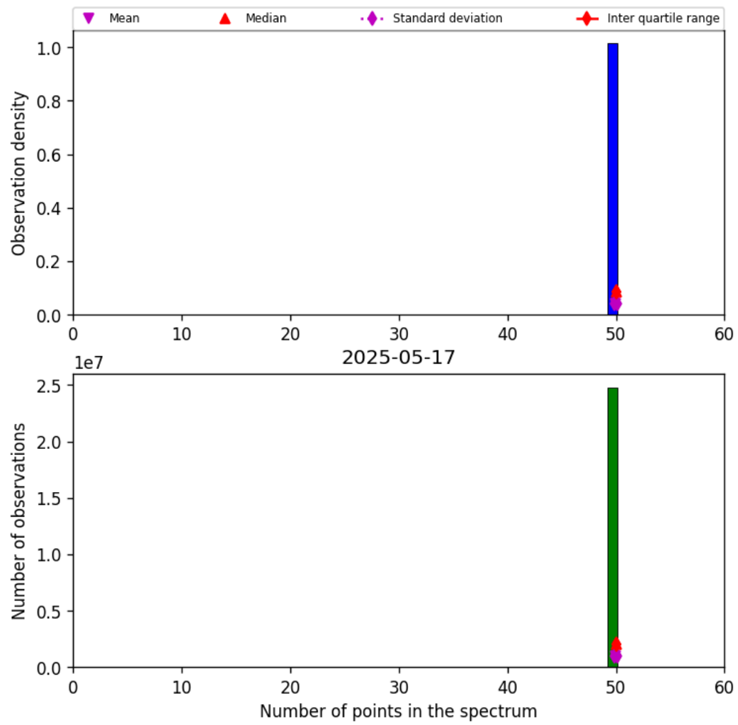
Figure 44: Histogram of “Number of points in the spectrum” for 2025-05-16 to 2025-05-18
