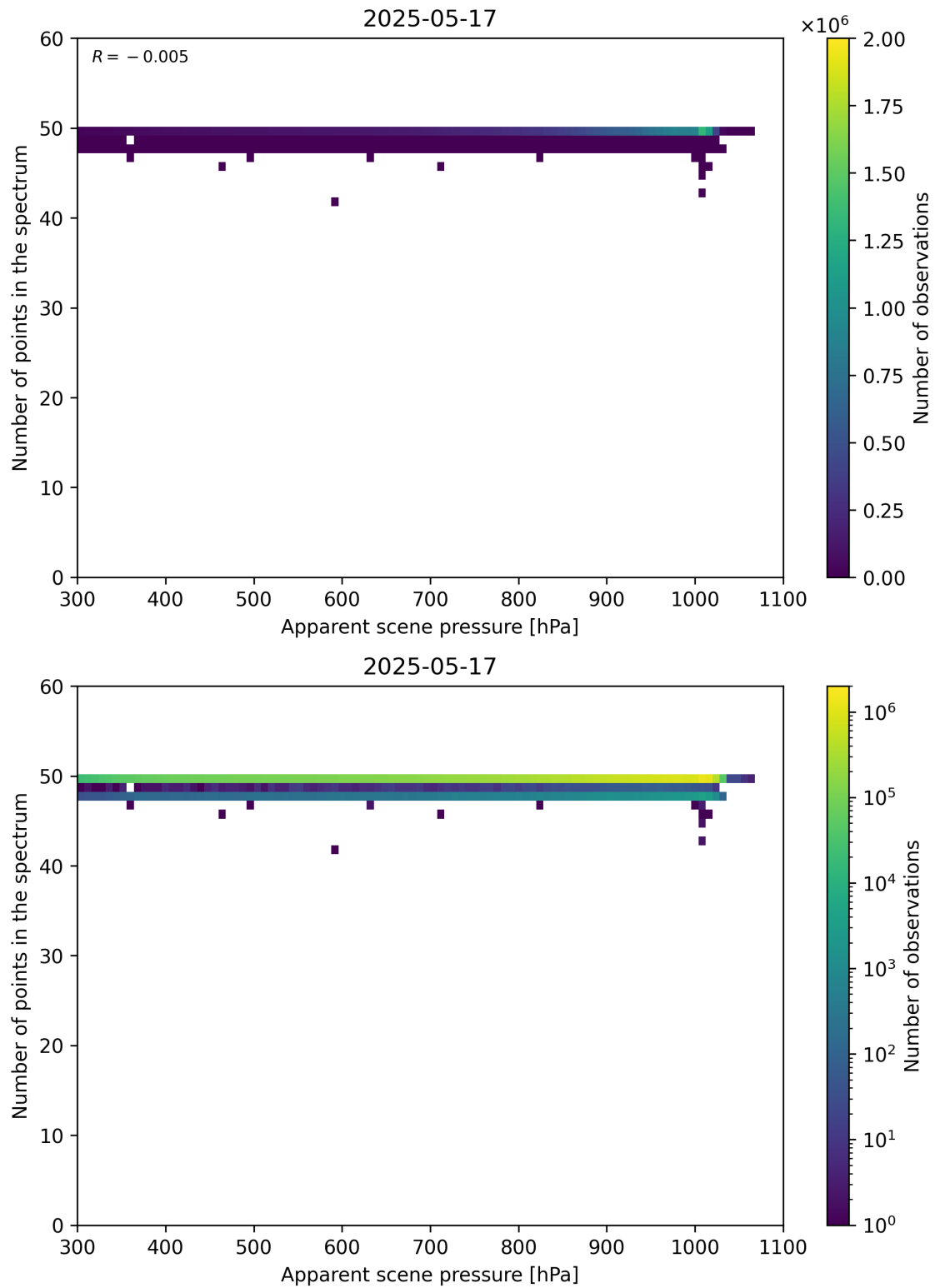
Figure 66: Scatter density plot of “Apparent scene pressure” against “Number of points in the spectrum” for 2025-05-16 to 2025-05-18.
