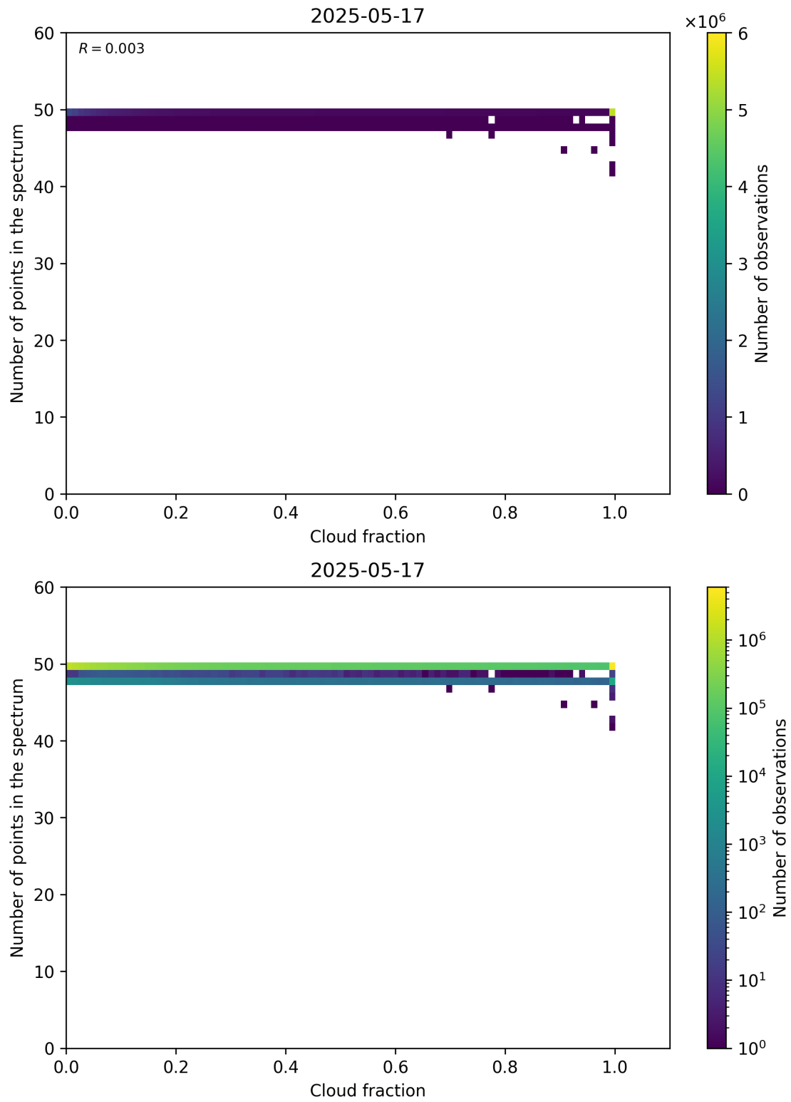
Figure 74: Scatter density plot of “Cloud fraction” against “Number of points in the spectrum” for 2025-05-16 to 2025-05-18.
