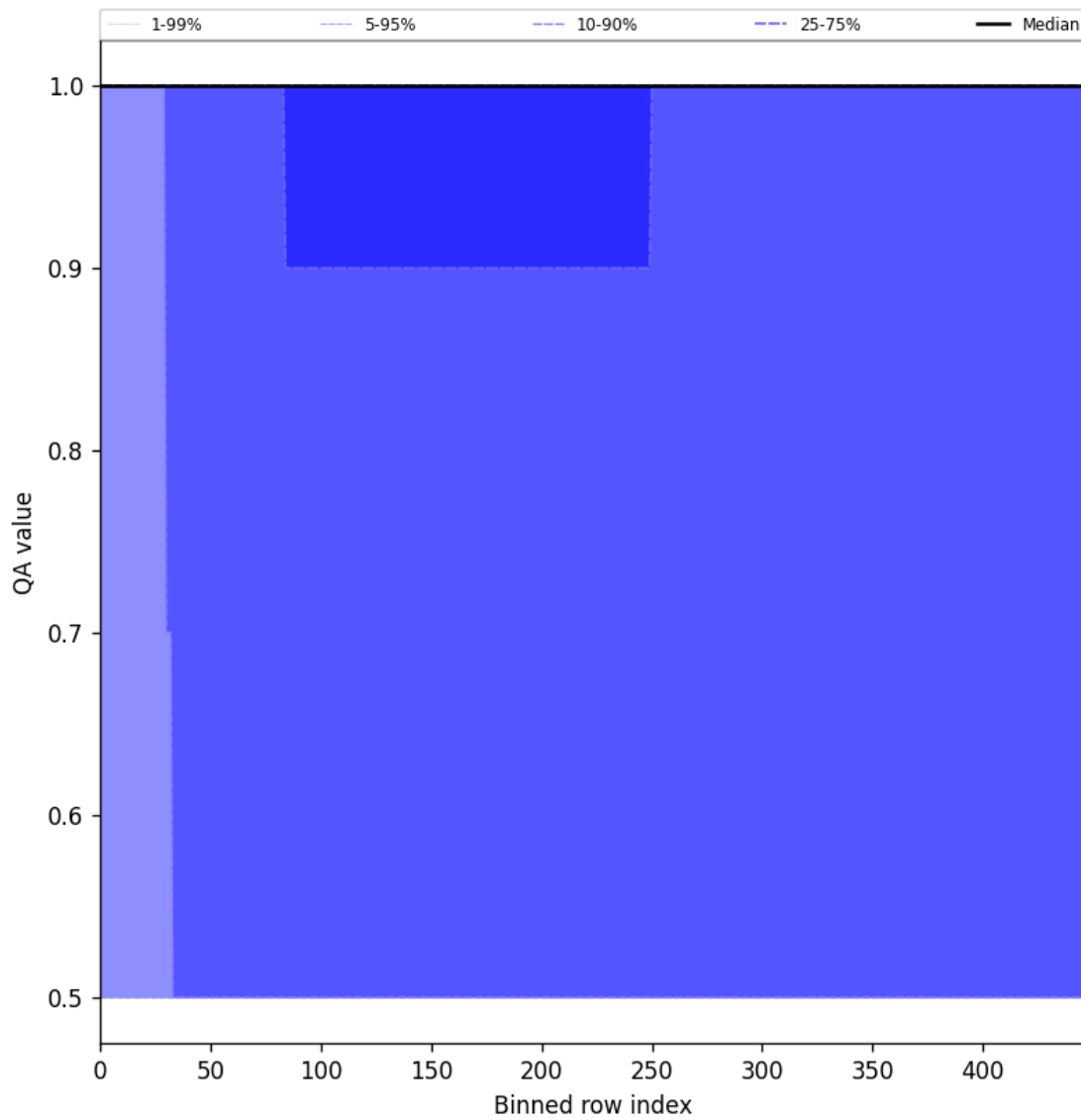
Figure 46: Along track statistics of “QA value” for 2025-05-16 to 2025-05-18
