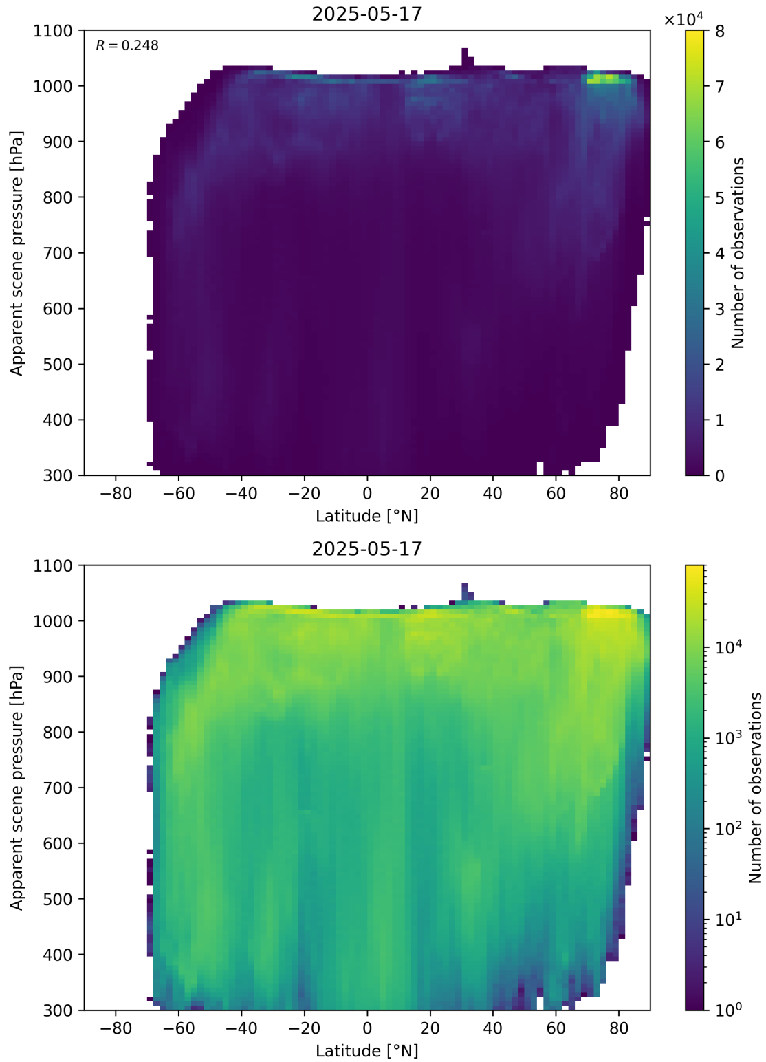
Figure 88: Scatter density plot of “Latitude” against “Apparent scene pressure” for 2025-05-16 to 2025-05-18.
