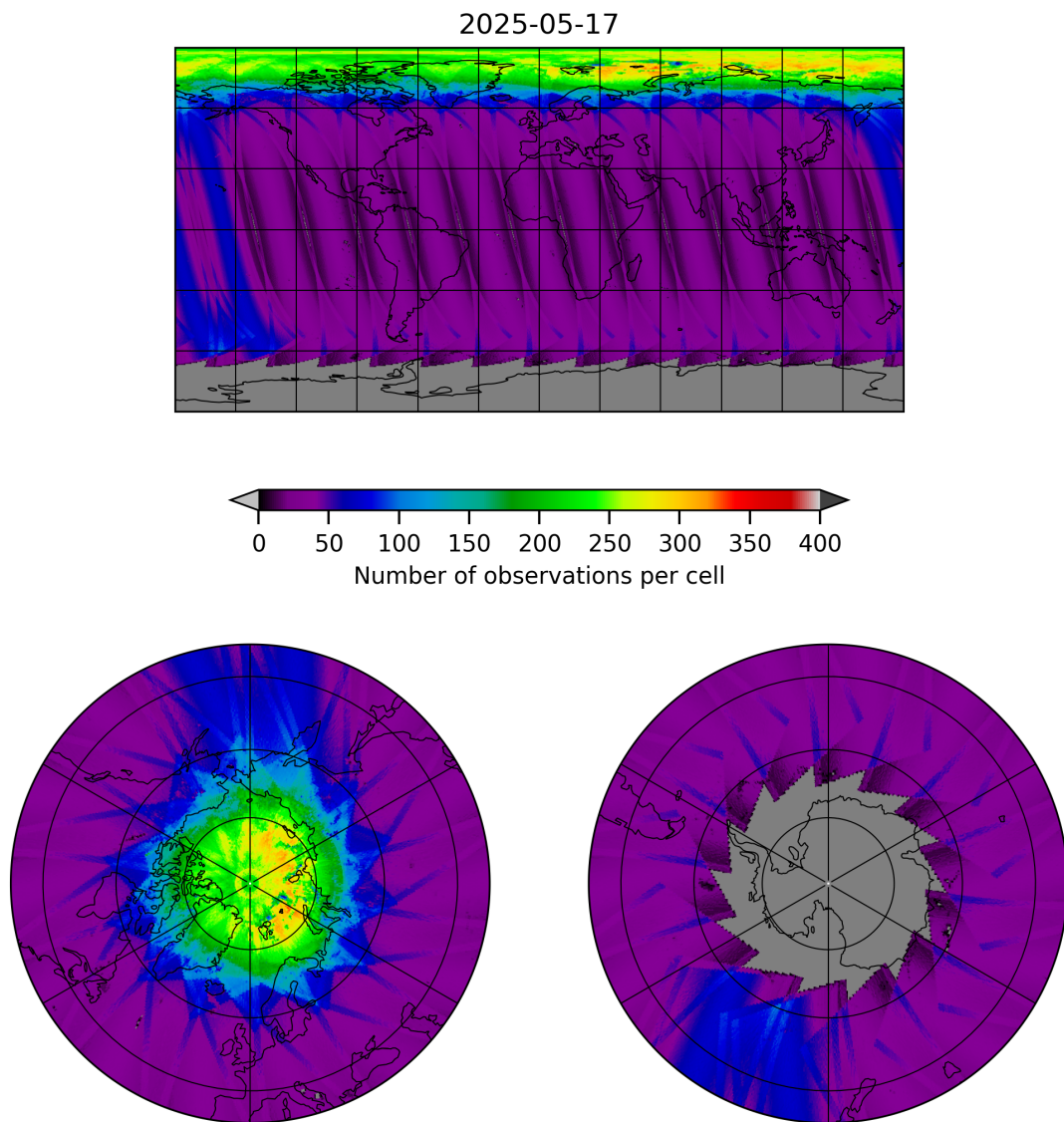
Figure 11: Map of the number of observations for 2025-05-16 to 2025-05-18
