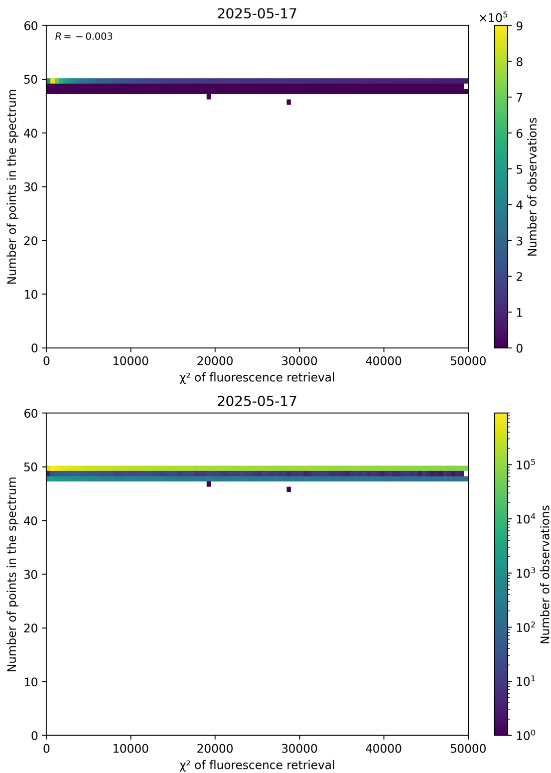
Figure 68: Scatter density plot of “ \chi^2 of fluorescence retrieval” against “Number of points in the spectrum” for 2025-05-16 to 2025-05-18.
