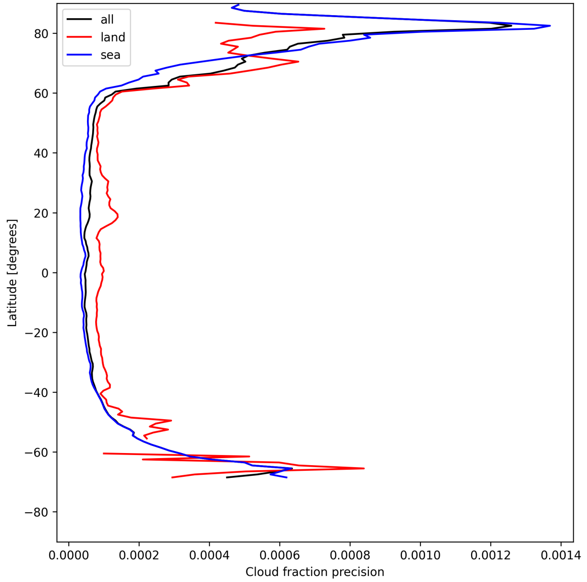
Figure 16: Zonal average of “Cloud fraction precision” for 2025-05-16 to 2025-05-18.
