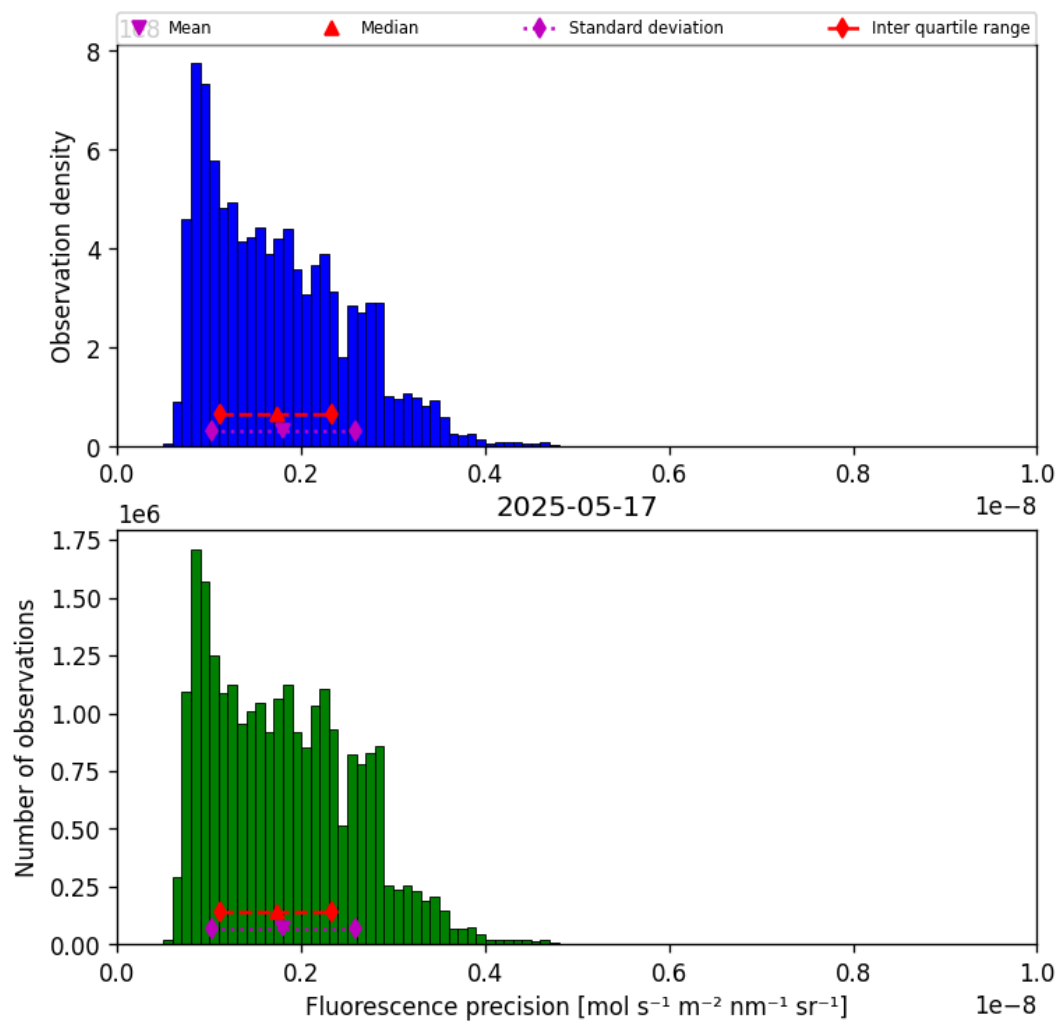
Figure 41: Histogram of “Fluorescence precision” for 2025-05-16 to 2025-05-18
