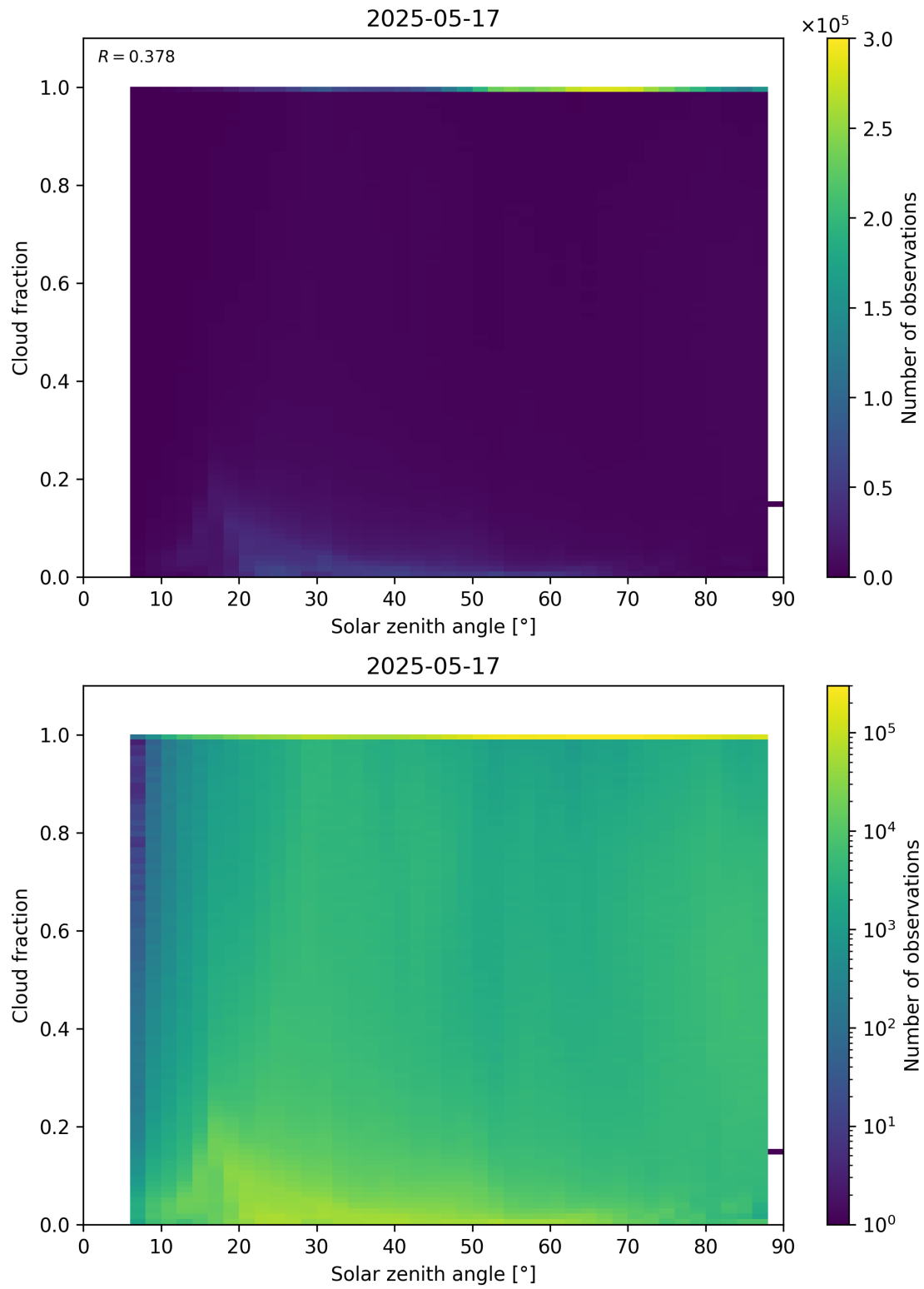
Figure 110: Scatter density plot of “Solar zenith angle” against “Cloud fraction” for 2025-05-16 to 2025-05-18.
