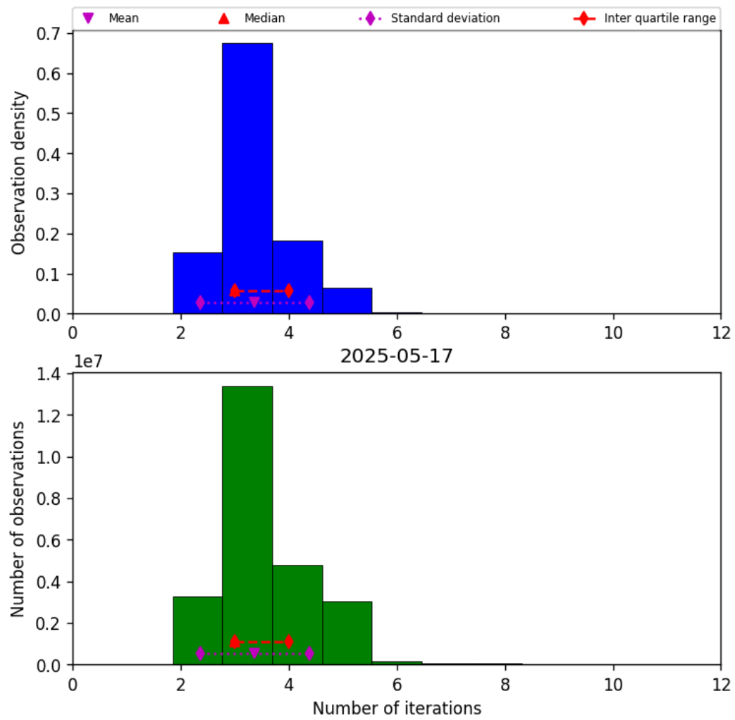
Figure 39: Histogram of “Number of iterations” for 2025-05-16 to 2025-05-18
