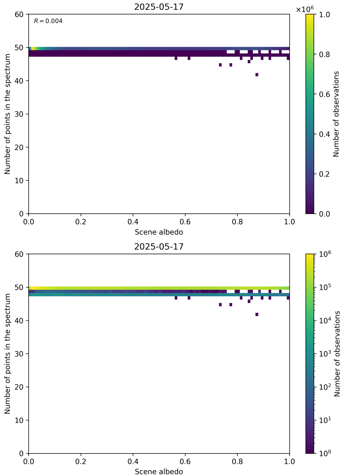
Figure 106: Scatter density plot of “Scene albedo” against “Number of points in the spectrum” for 2025-05-16 to 2025-05-18.
