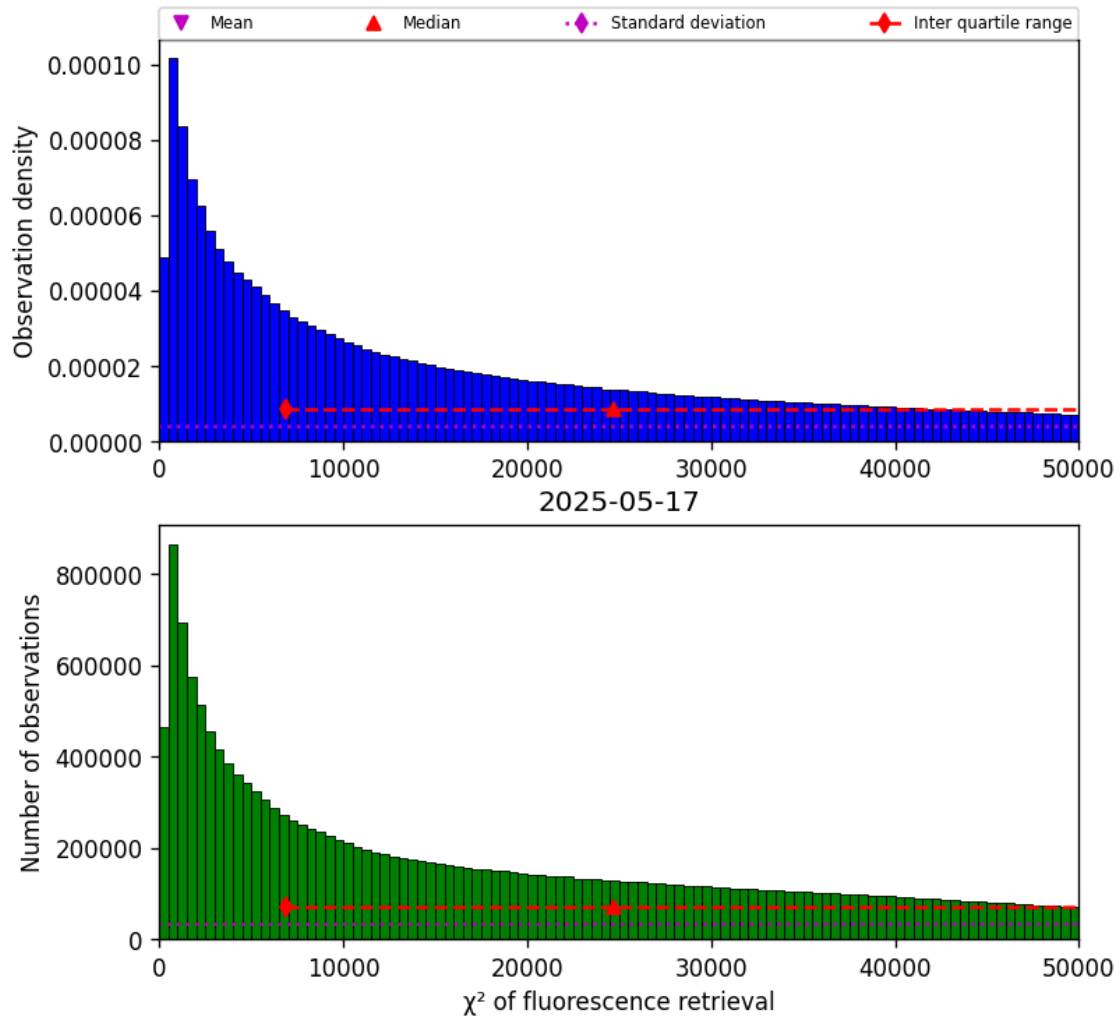
Figure 42: Histogram of “ \chi^2 of fluorescence retrieval” for 2025-05-16 to 2025-05-18
