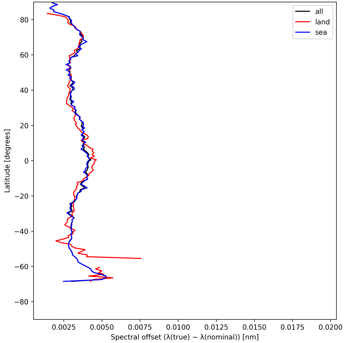
Figure 28: Zonal average of “Spectral offset ( \lambda_{\text{true}} - \lambda_{\text{nominal}} )” for 2025-05-16 to 2025-05-18.
