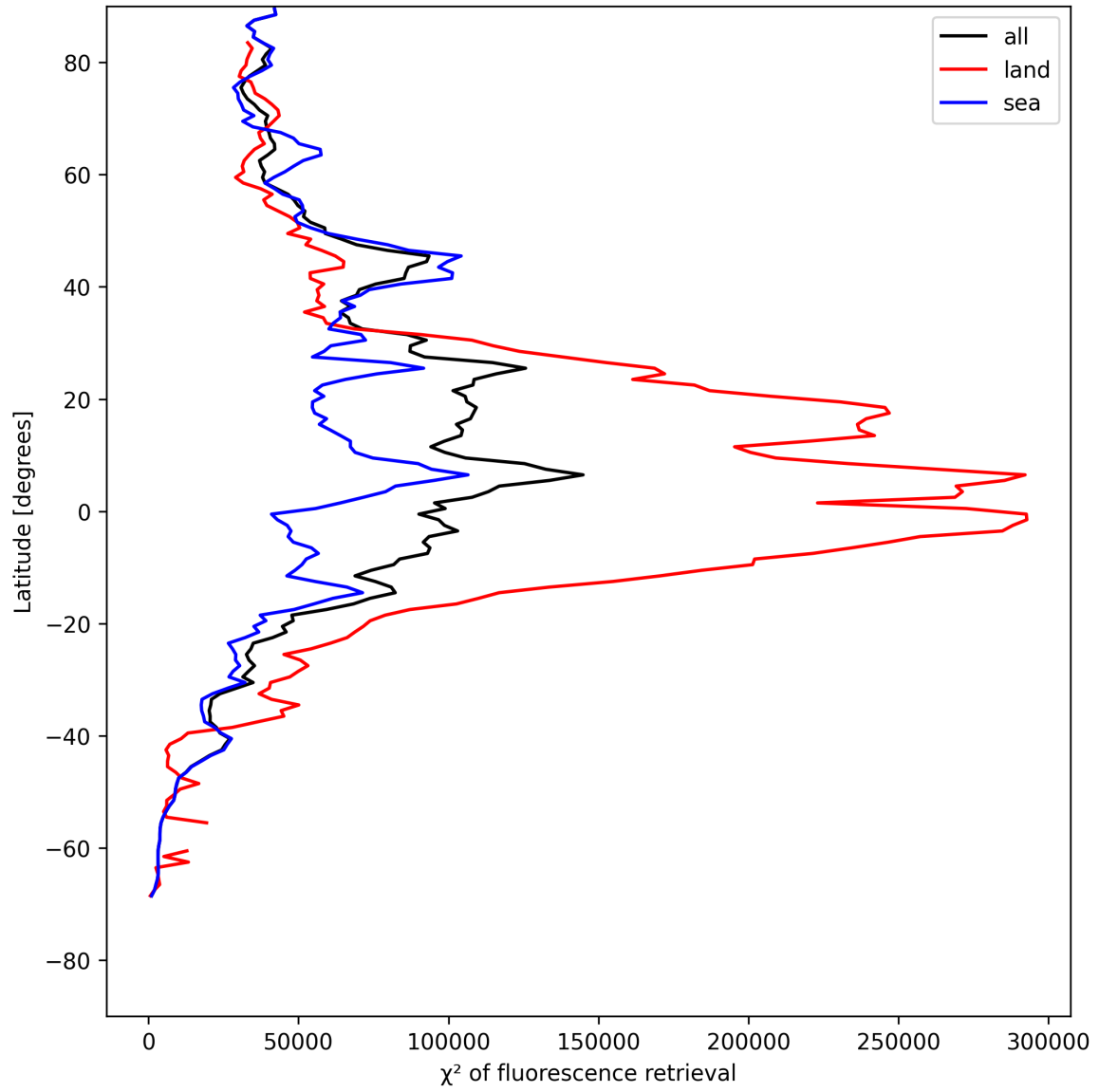
Figure 25: Zonal average of “ \chi^2 of fluorescence retrieval” for 2025-05-16 to 2025-05-18.
