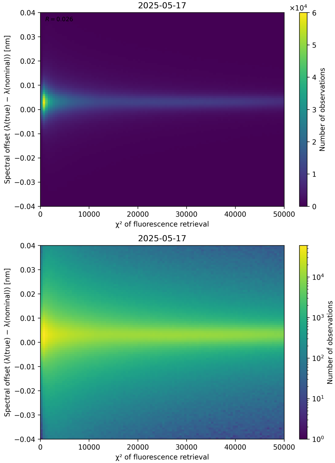
Figure 69: Scatter density plot of “ \chi^2 of fluorescence retrieval” against “Spectral offset ( \lambda_{\text{true}} - \lambda_{\text{nominal}} )” for 2025-05-16 to 2025-05-18.
