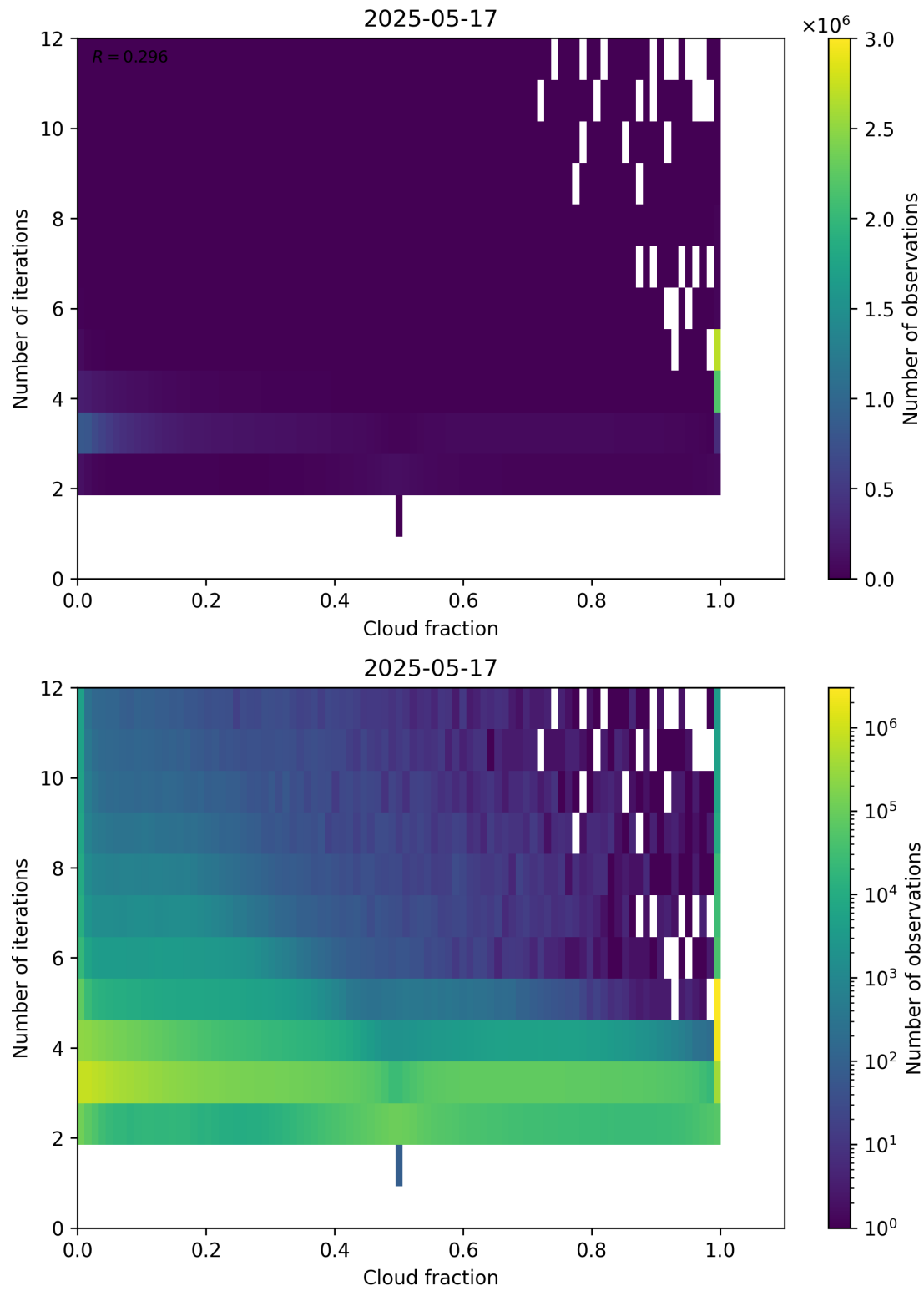
Figure 73: Scatter density plot of “Cloud fraction” against “Number of iterations” for 2025-05-16 to 2025-05-18.
