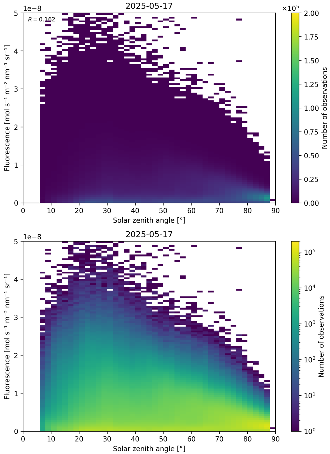
Figure 112: Scatter density plot of “Solar zenith angle” against “Fluorescence” for 2025-05-16 to 2025-05-18.
