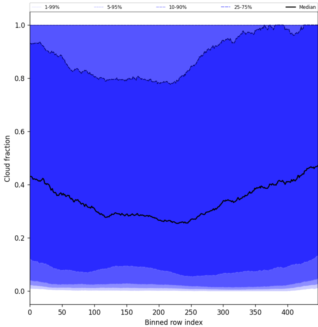
Figure 49: Along track statistics of “Cloud fraction” for 2025-05-16 to 2025-05-18
