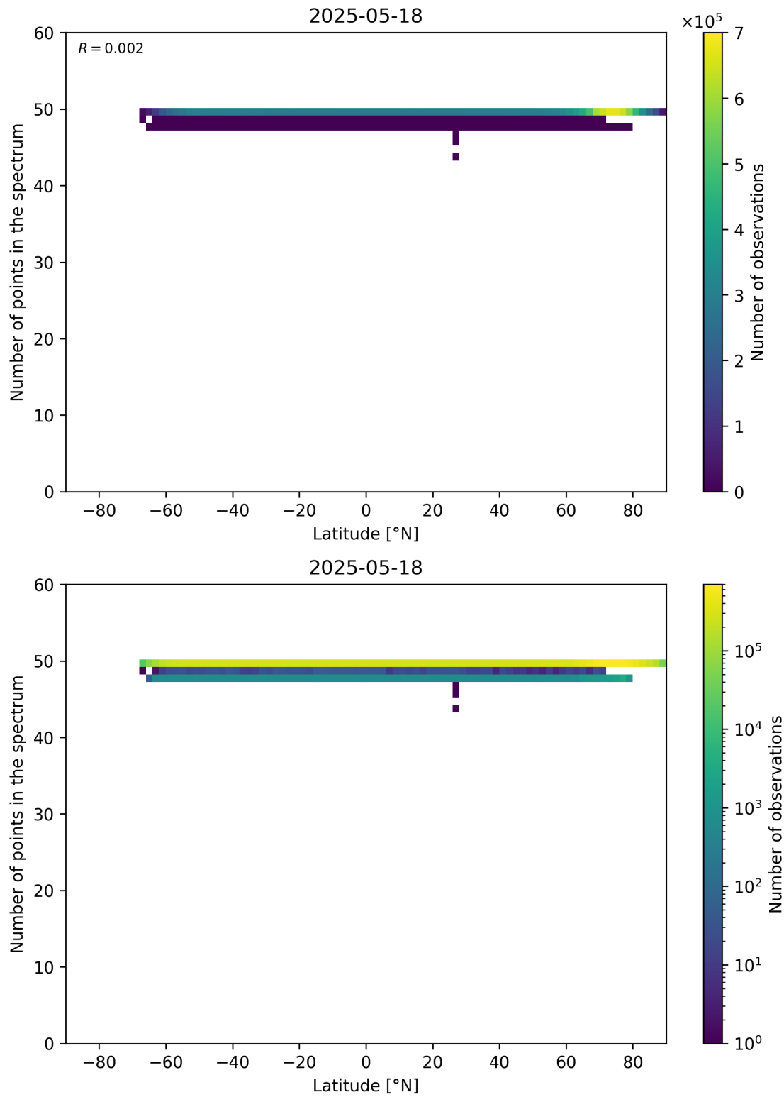
Figure 94: Scatter density plot of “Latitude” against “Number of points in the spectrum” for 2025-05-17 to 2025-05-19.
