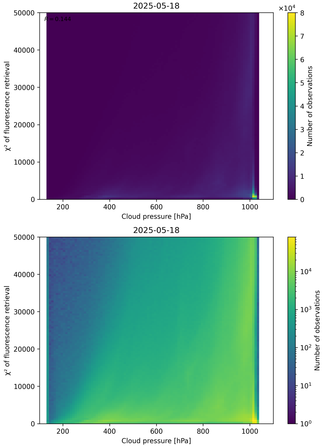
Figure 78: Scatter density plot of “Cloud pressure” against “ \chi^2 of fluorescence retrieval” for 2025-05-17 to 2025-05-19.
