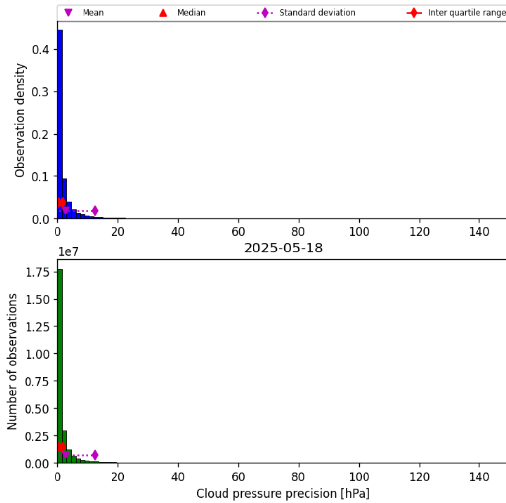
Figure 31: Histogram of “Cloud pressure precision” for 2025-05-17 to 2025-05-19
