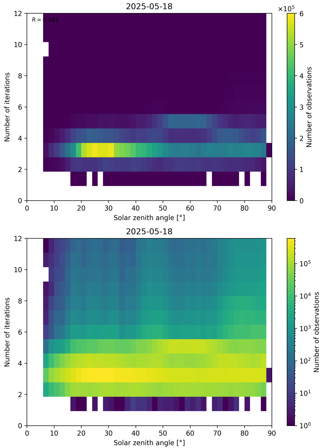
Figure 114: Scatter density plot of “Solar zenith angle” against “Number of iterations” for 2025-05-17 to 2025-05-19.
