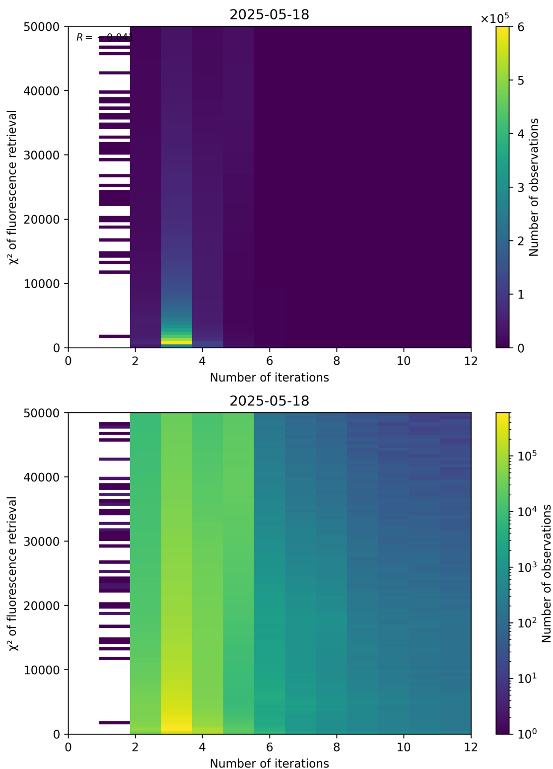
Figure 97: Scatter density plot of “Number of iterations” against “ \chi^2 of fluorescence retrieval” for 2025-05-17 to 2025-05-19.
