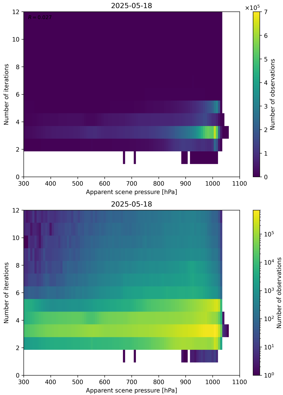
Figure 65: Scatter density plot of “Apparent scene pressure” against “Number of iterations” for 2025-05-17 to 2025-05-19.
