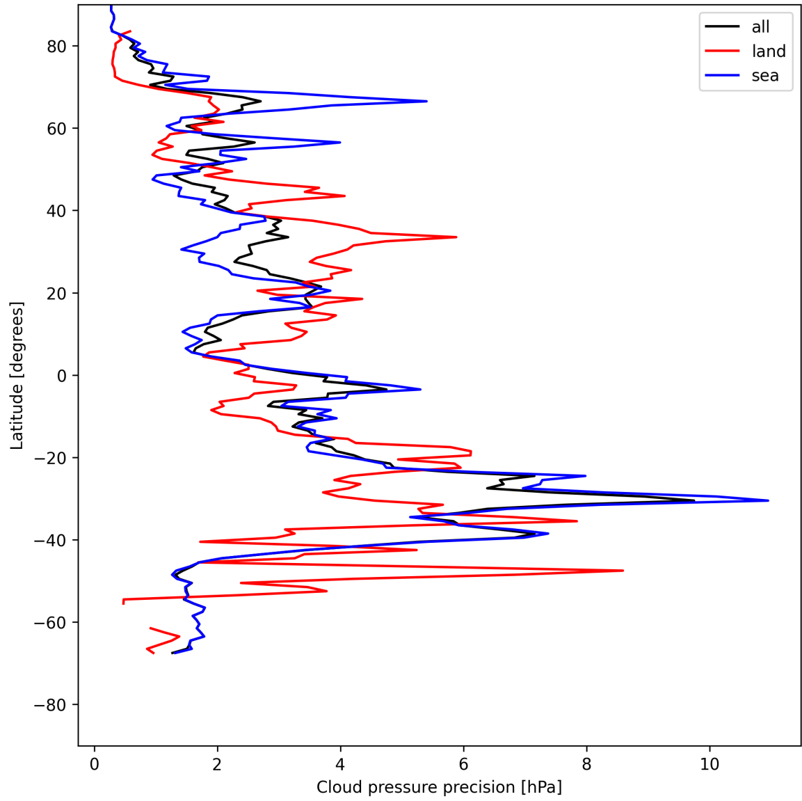
Figure 14: Zonal average of “Cloud pressure precision” for 2025-05-17 to 2025-05-19.
