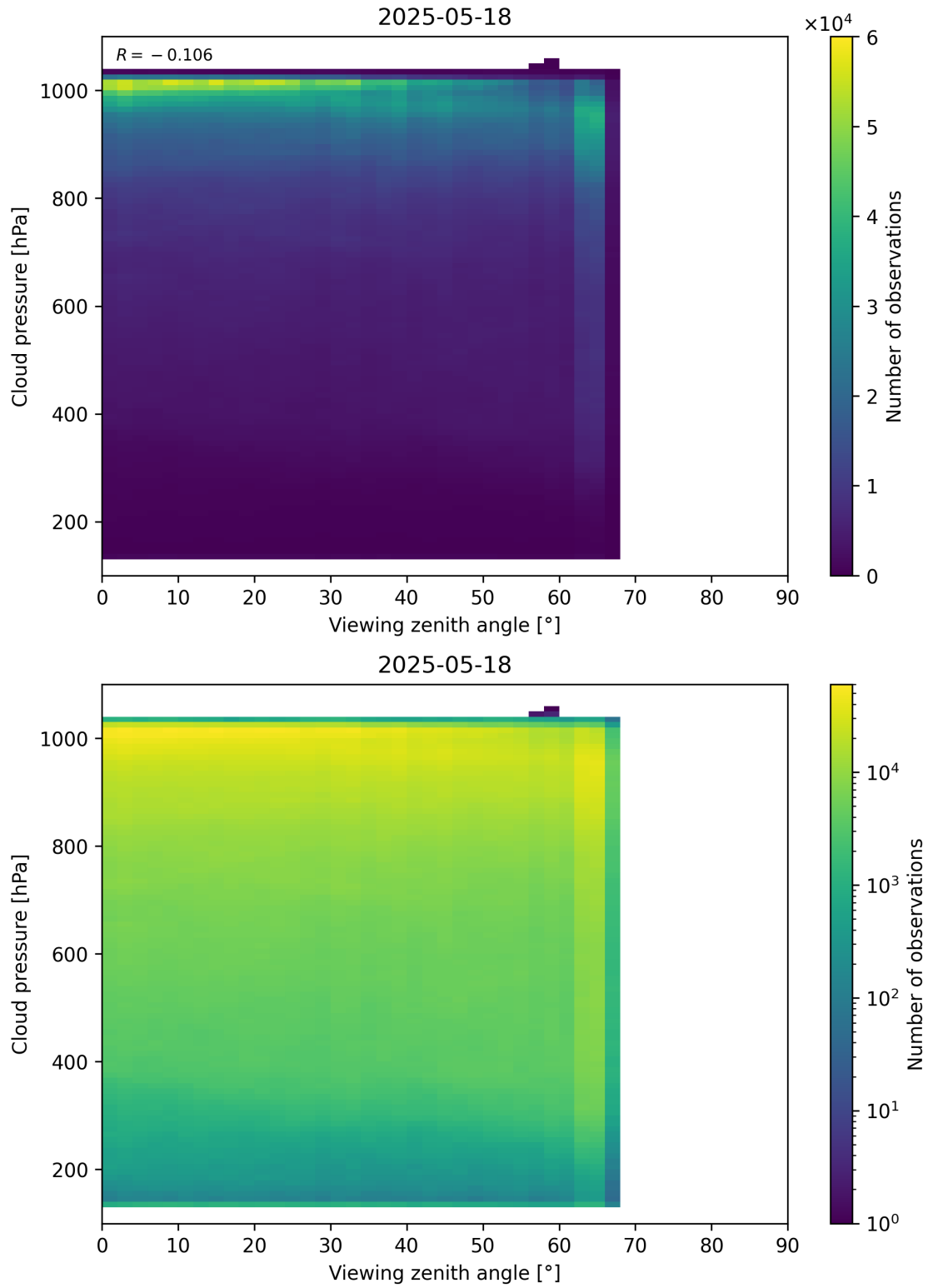
Figure 121: Scatter density plot of “Viewing zenith angle” against “Cloud pressure” for 2025-05-17 to 2025-05-19.
