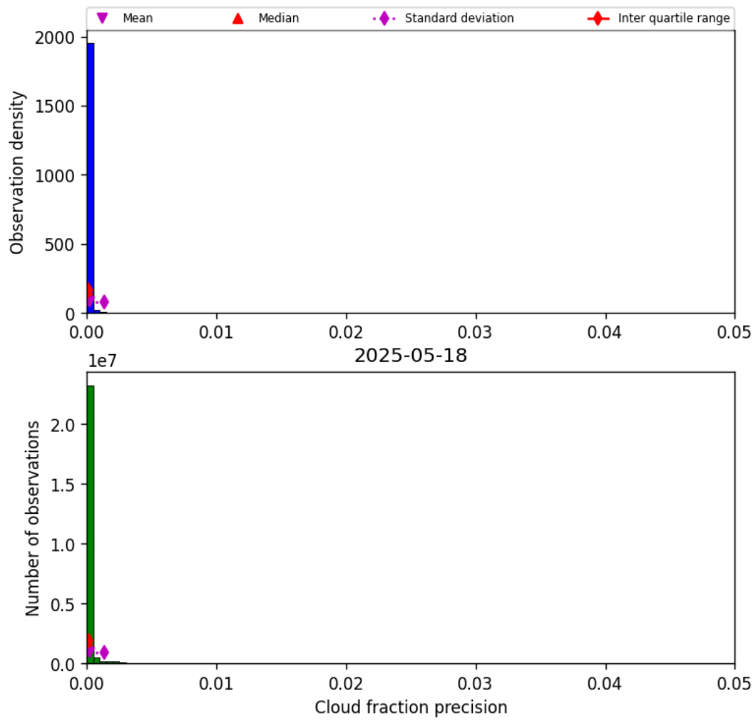
Figure 33: Histogram of “Cloud fraction precision” for 2025-05-17 to 2025-05-19
