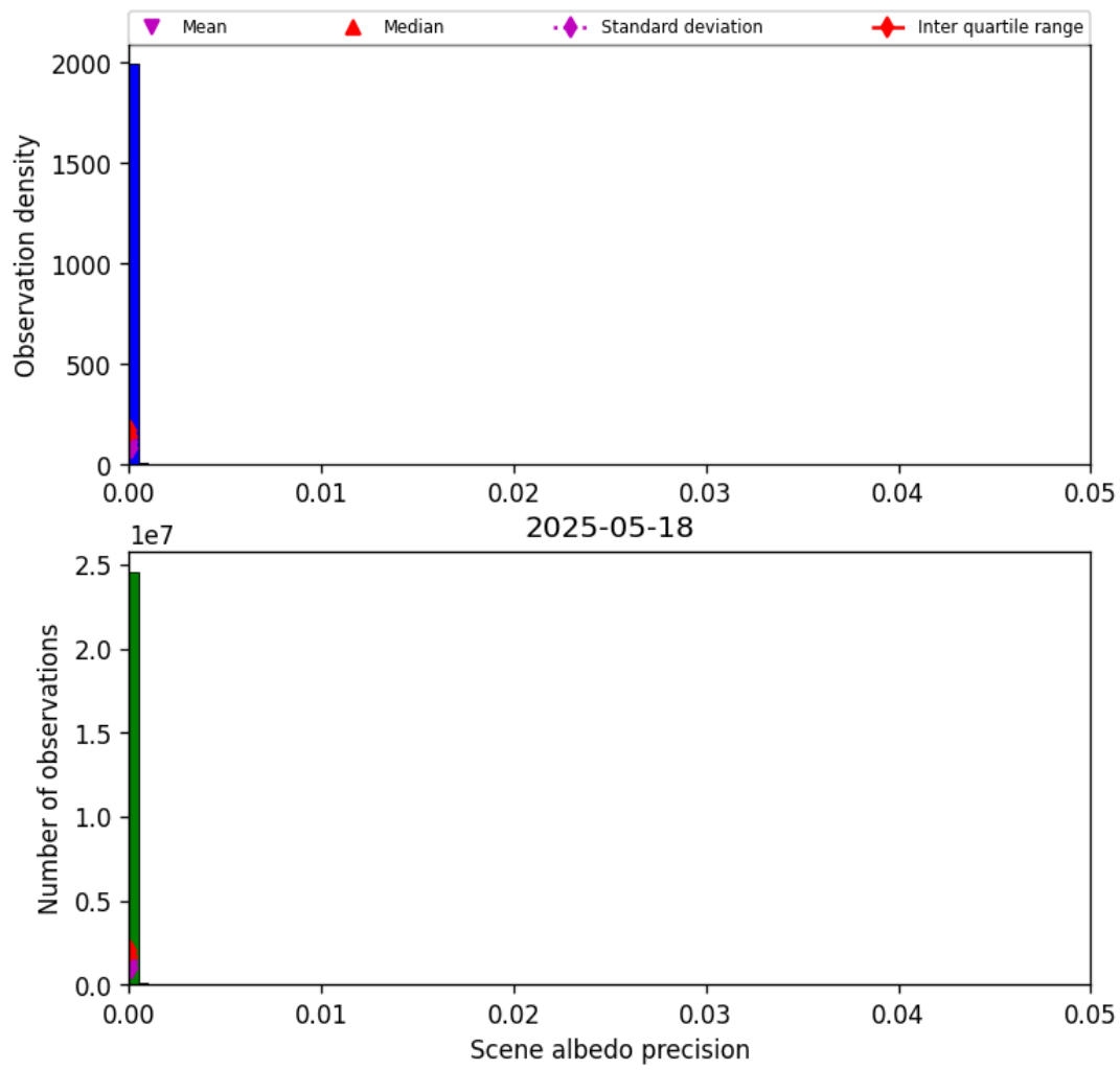
Figure 35: Histogram of “Scene albedo precision” for 2025-05-17 to 2025-05-19
