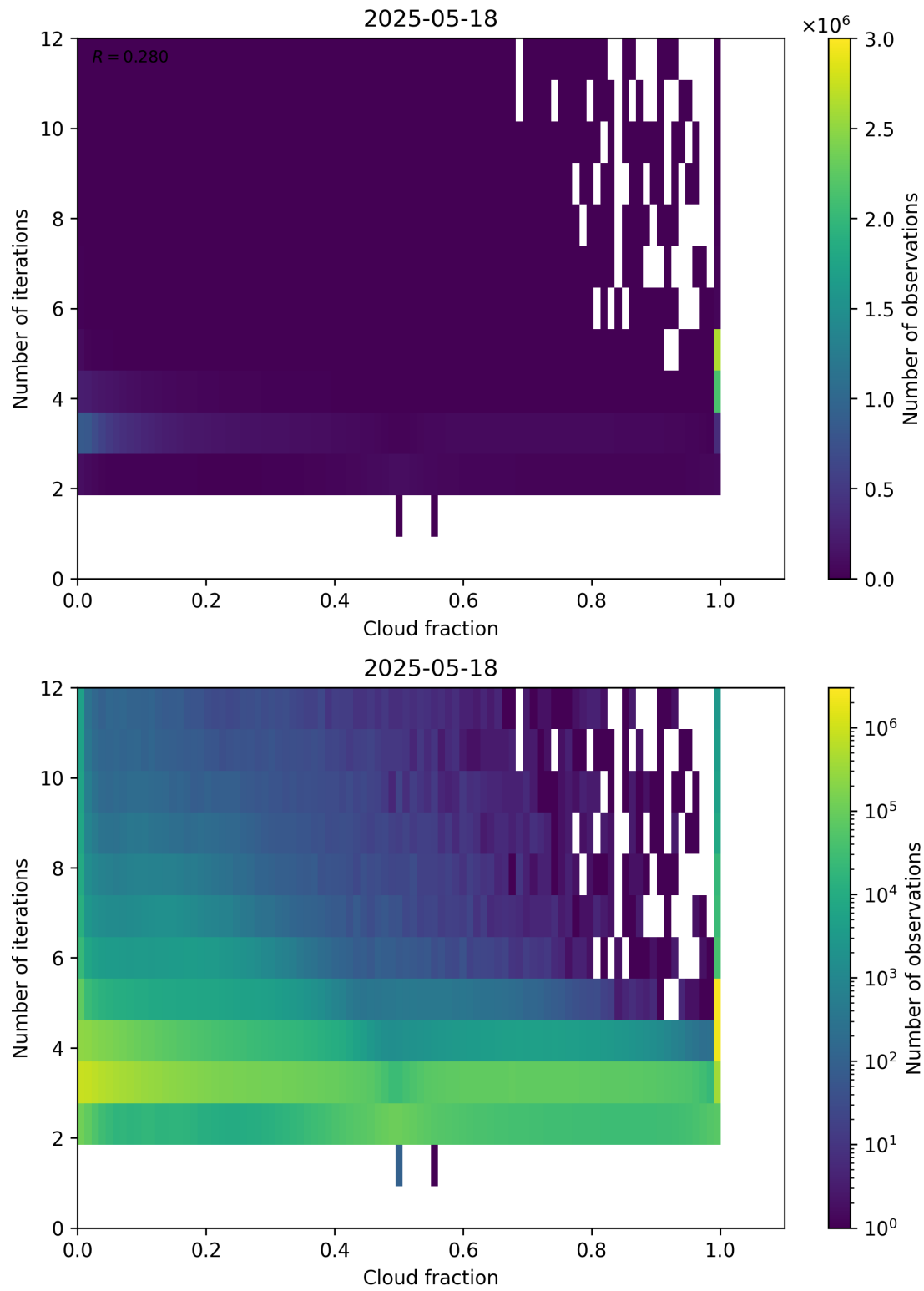
Figure 73: Scatter density plot of “Cloud fraction” against “Number of iterations” for 2025-05-17 to 2025-05-19.
