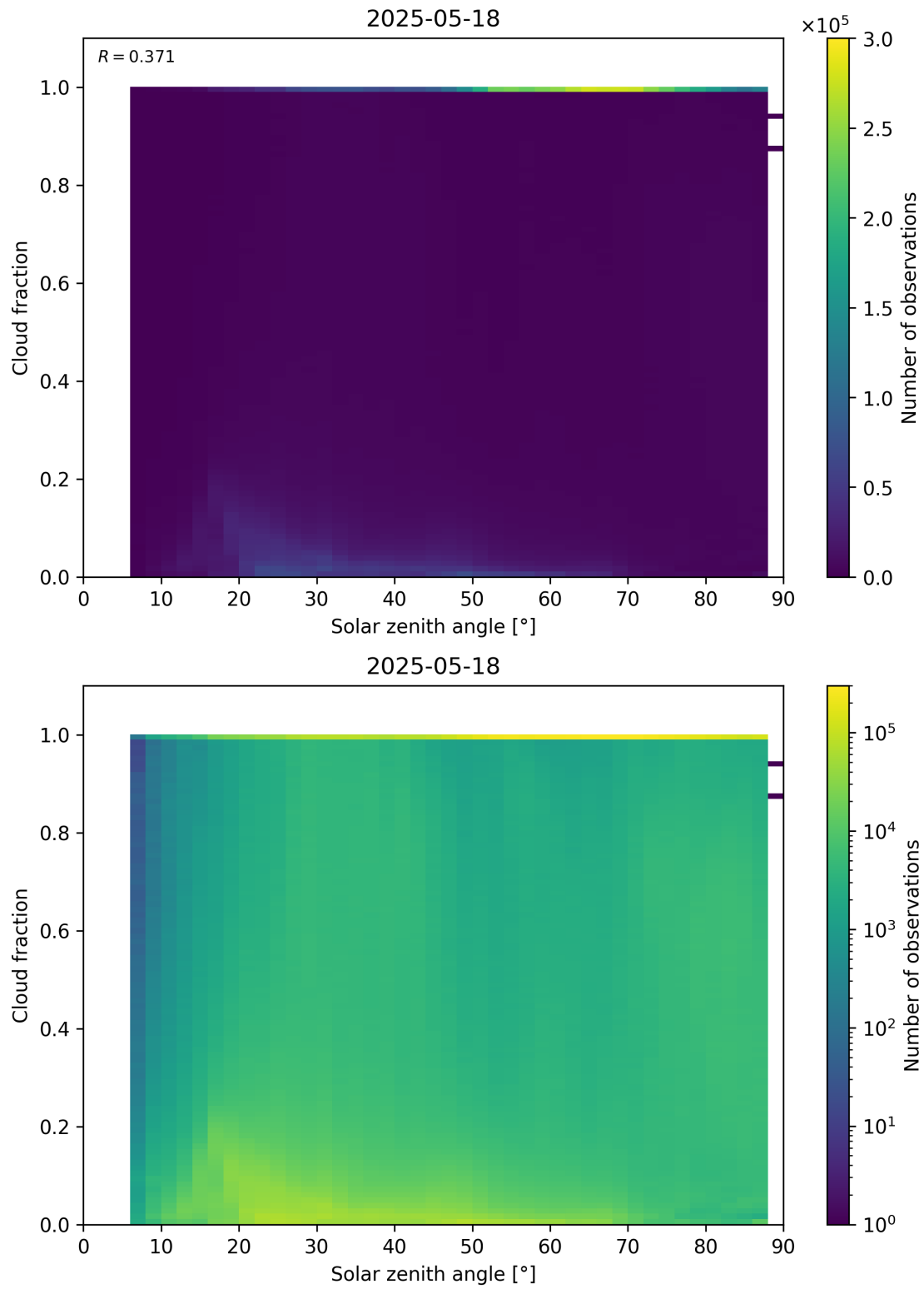
Figure 110: Scatter density plot of “Solar zenith angle” against “Cloud fraction” for 2025-05-17 to 2025-05-19.
