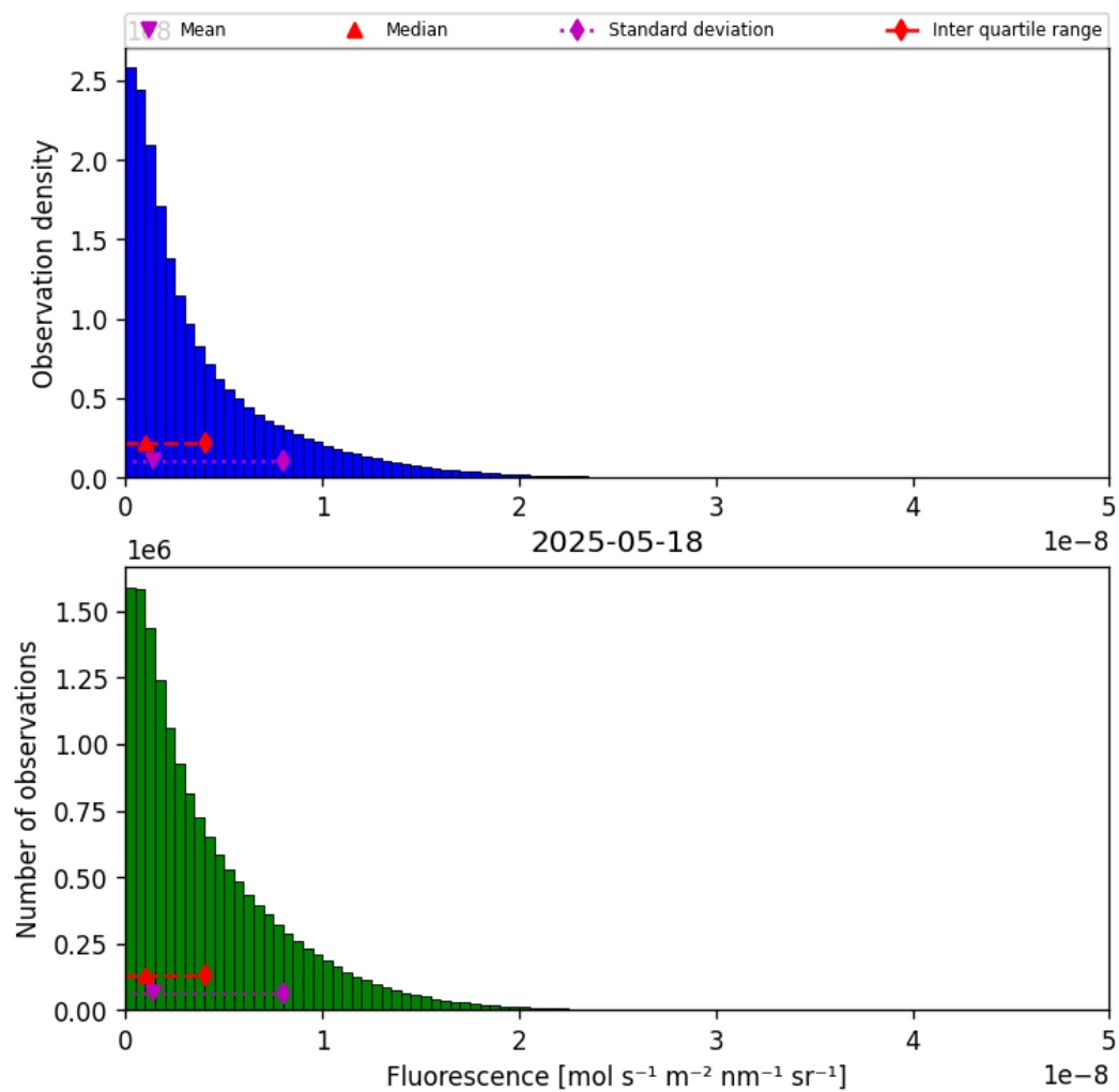
Figure 40: Histogram of “Fluorescence” for 2025-05-17 to 2025-05-19
