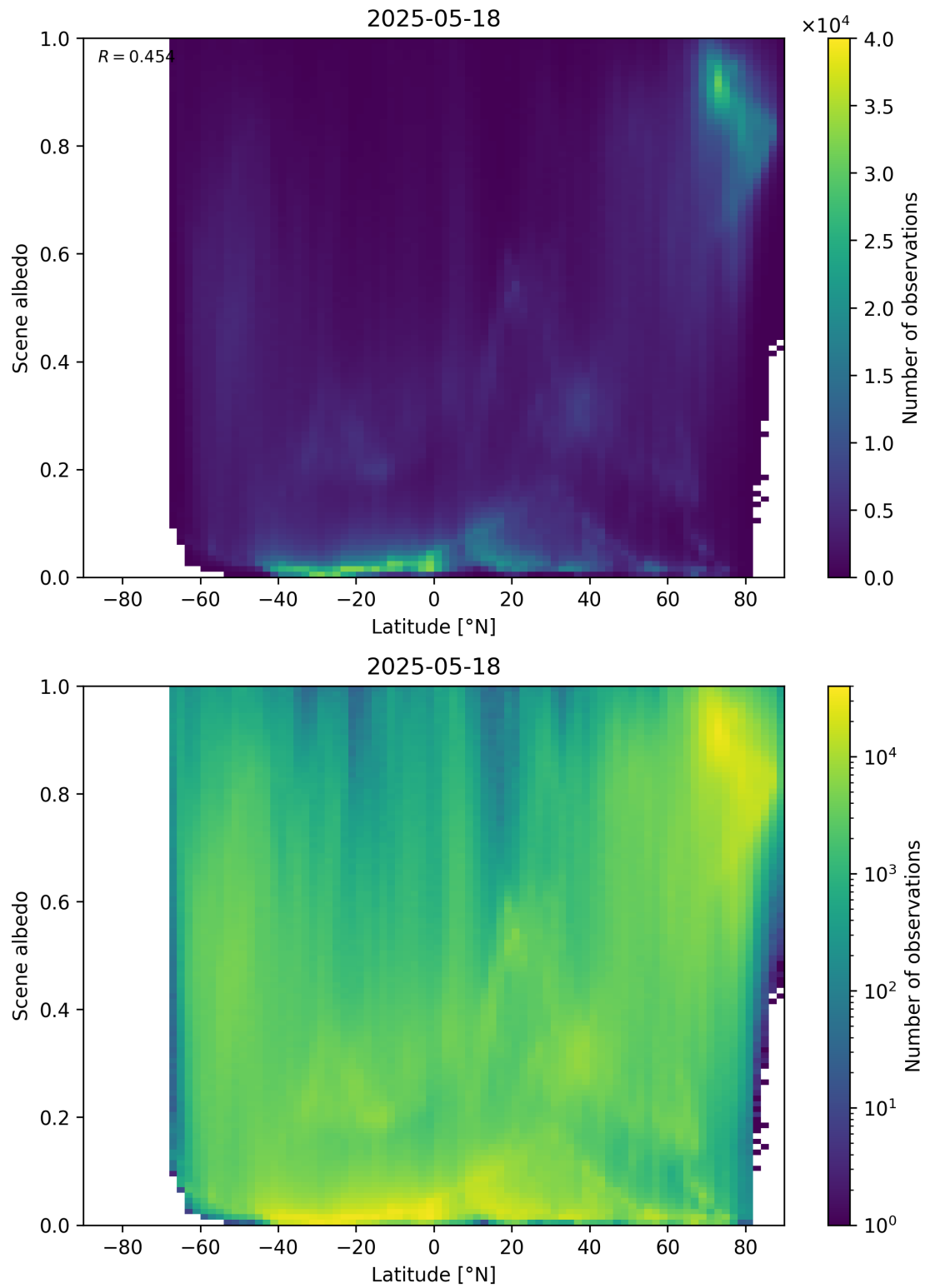
Figure 95: Scatter density plot of “Latitude” against “Scene albedo” for 2025-05-17 to 2025-05-19.
