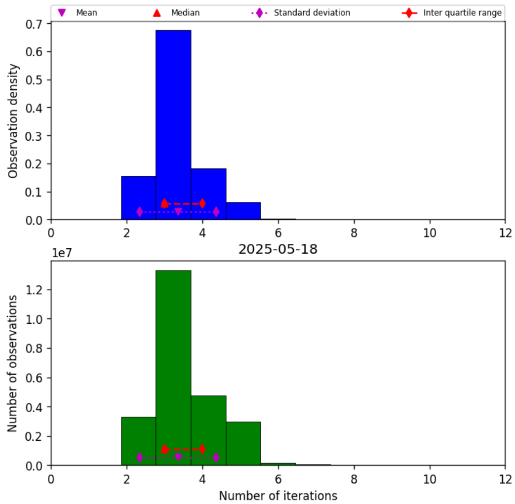
Figure 39: Histogram of “Number of iterations” for 2025-05-17 to 2025-05-19
