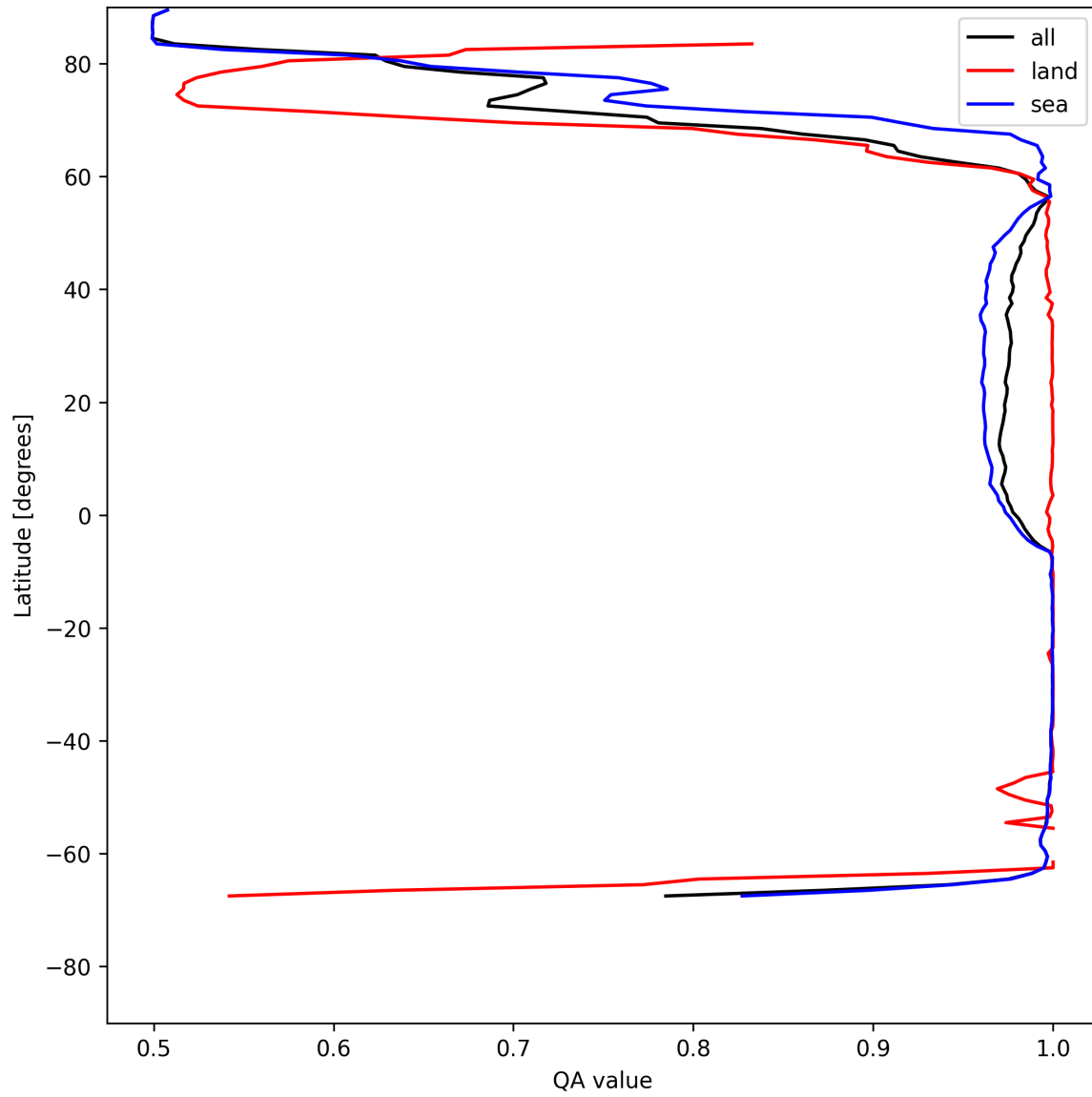
Figure 12: Zonal average of “QA value” for 2025-05-17 to 2025-05-19.
