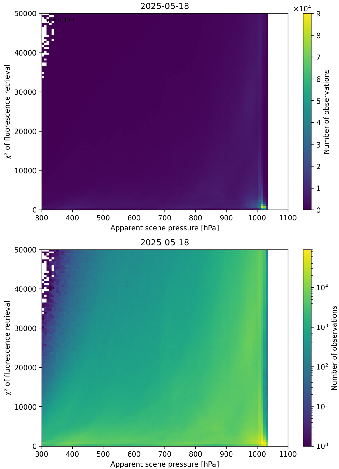
Figure 63: Scatter density plot of “Apparent scene pressure” against “ \chi^2 of fluorescence retrieval” for 2025-05-17 to 2025-05-19.
