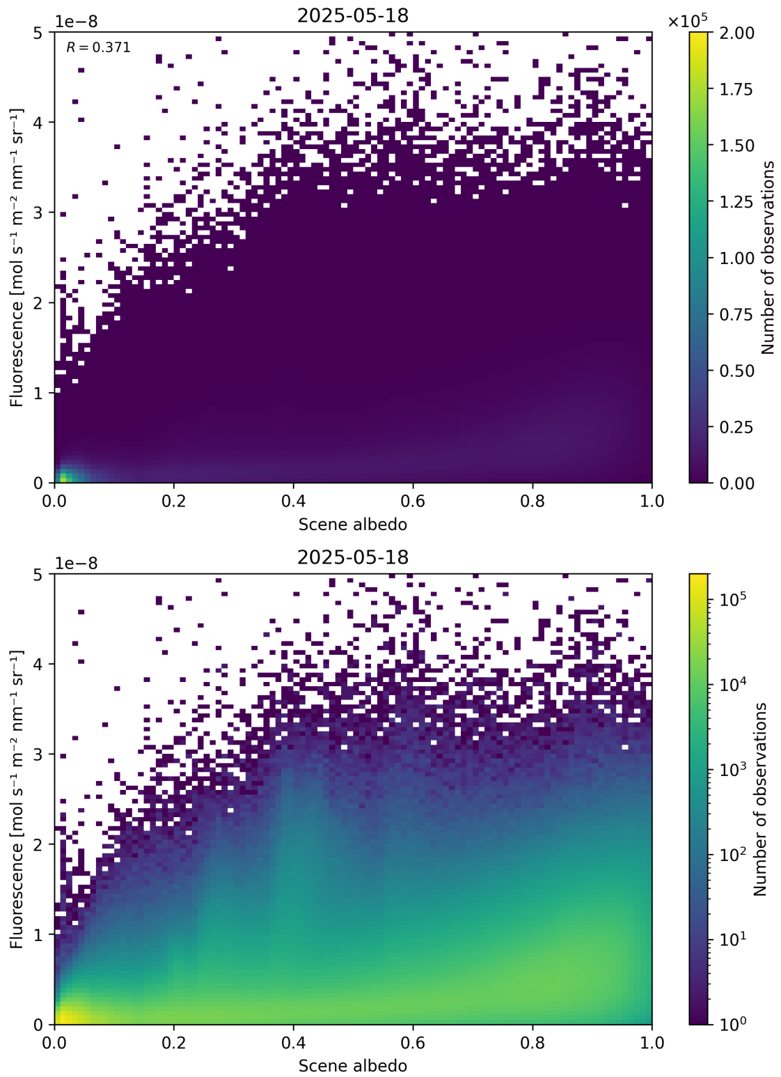
Figure 104: Scatter density plot of “Scene albedo” against “Fluorescence” for 2025-05-17 to 2025-05-19.
