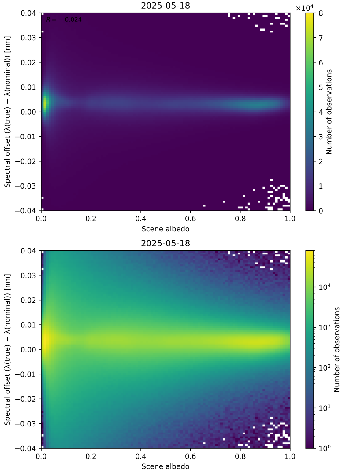
Figure 107: Scatter density plot of “Scene albedo” against “Spectral offset ( \lambda_{\text{true}} - \lambda_{\text{nominal}} )” for 2025-05-17 to 2025-05-19.
