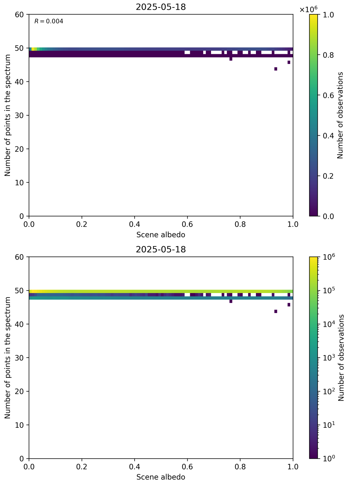
Figure 106: Scatter density plot of “Scene albedo” against “Number of points in the spectrum” for 2025-05-17 to 2025-05-19.
