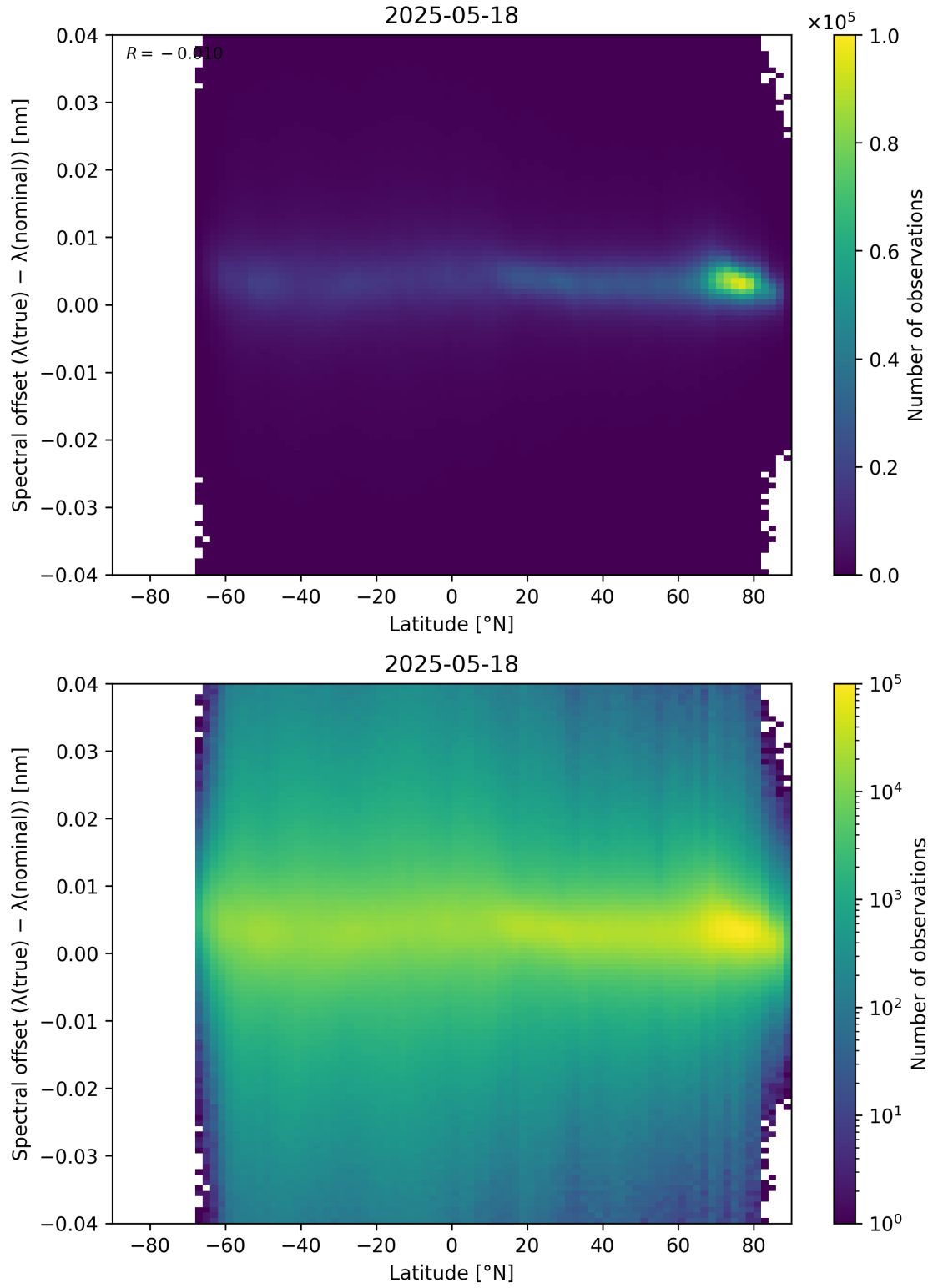
Figure 96: Scatter density plot of “Latitude” against “Spectral offset ( \lambda_{\text{true}} - \lambda_{\text{nominal}} )” for 2025-05-17 to 2025-05-19.
