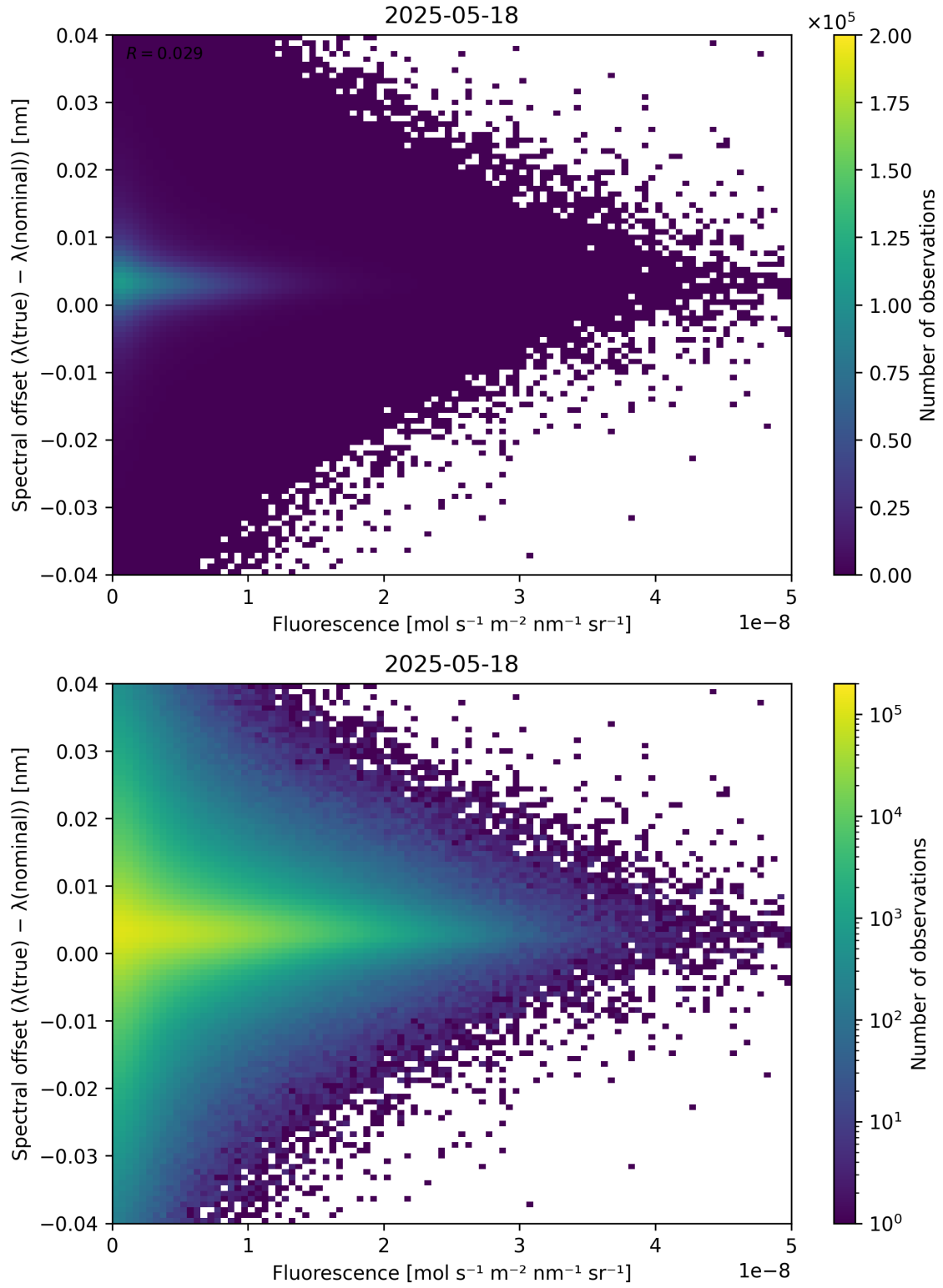
Figure 87: Scatter density plot of “Fluorescence” against “Spectral offset ( \lambda_{\text{true}} - \lambda_{\text{nominal}} )” for 2025-05-17 to 2025-05-19.
