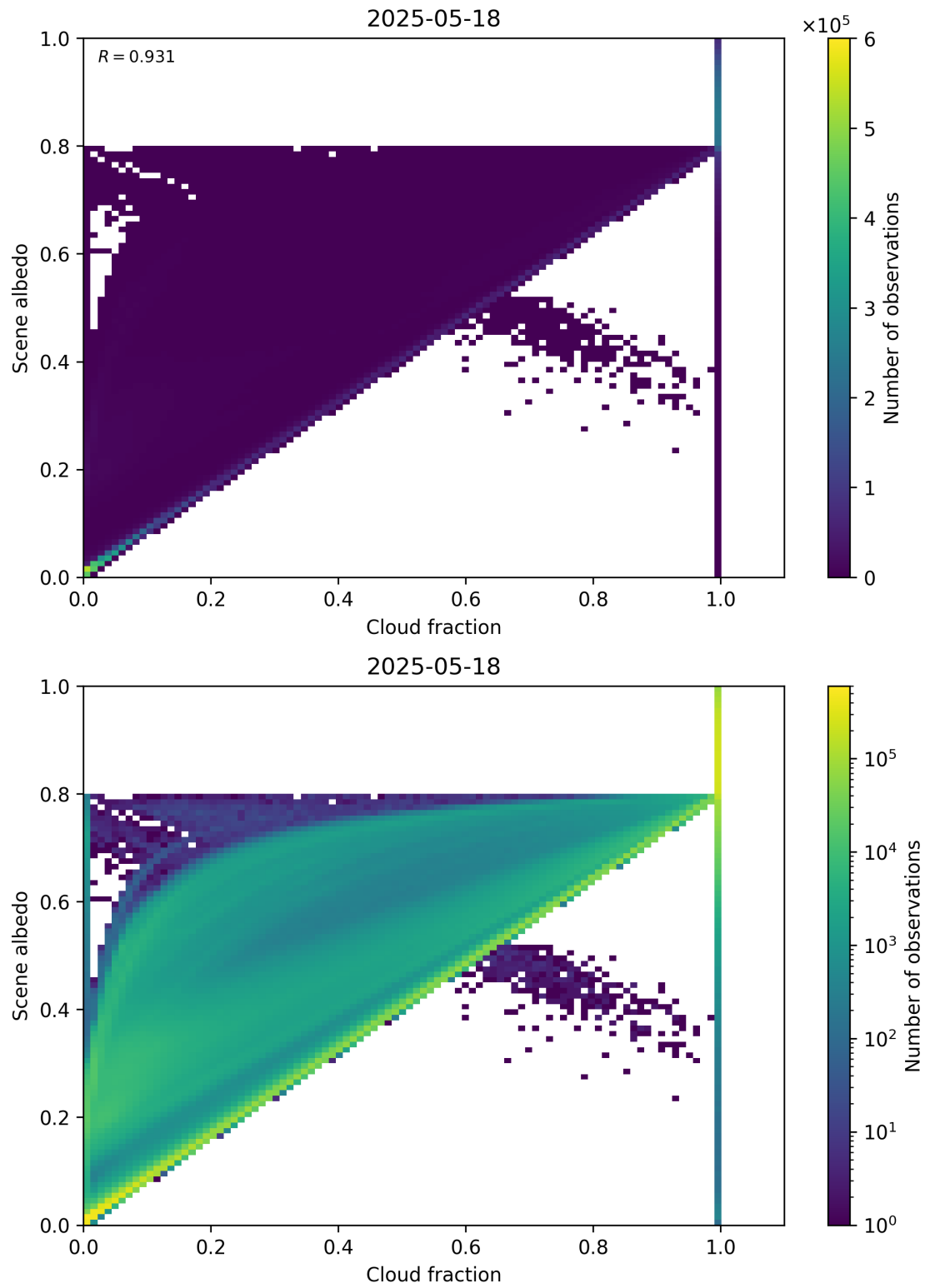
Figure 75: Scatter density plot of “Cloud fraction” against “Scene albedo” for 2025-05-17 to 2025-05-19.
