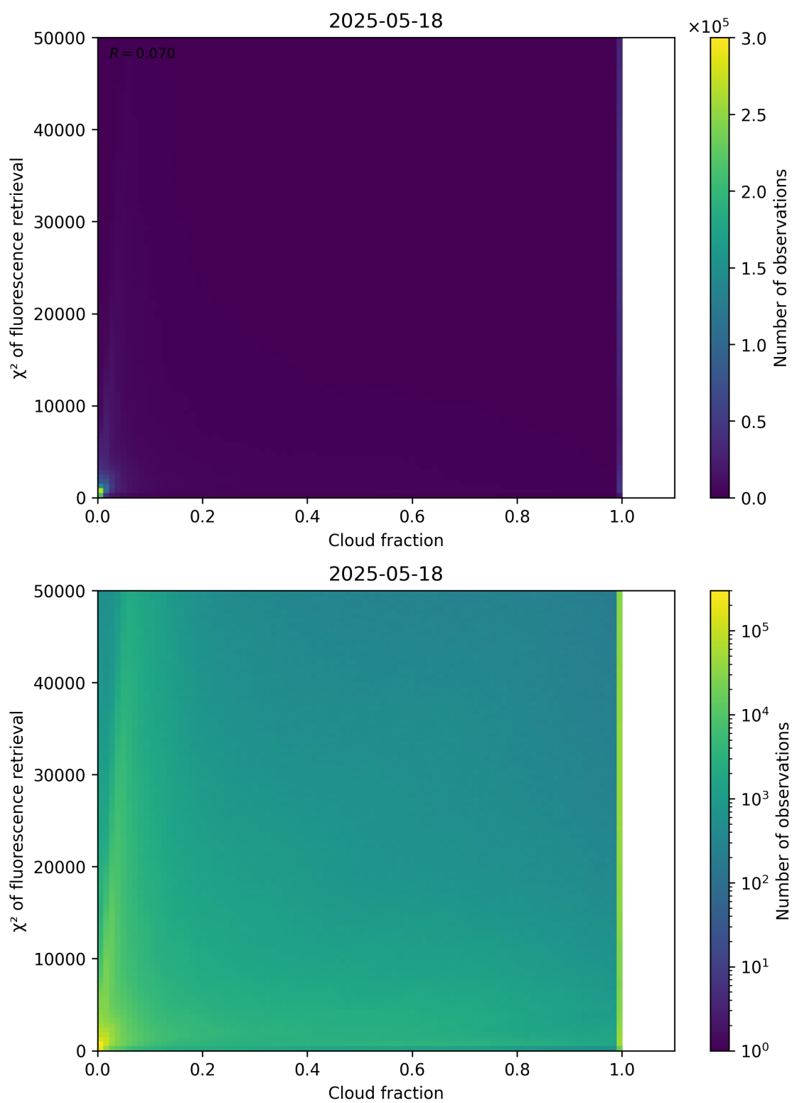
Figure 71: Scatter density plot of “Cloud fraction” against “ \chi^2 of fluorescence retrieval” for 2025-05-17 to 2025-05-19.
