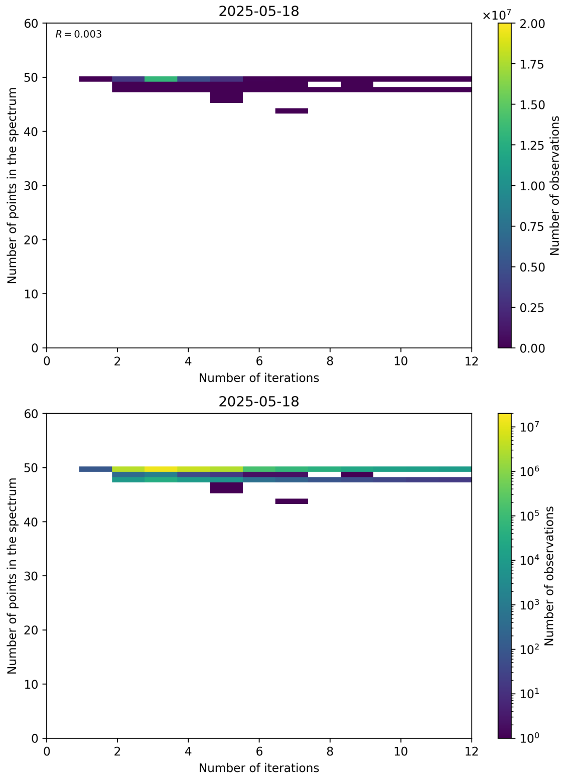
Figure 99: Scatter density plot of “Number of iterations” against “Number of points in the spectrum” for 2025-05-17 to 2025-05-19.
