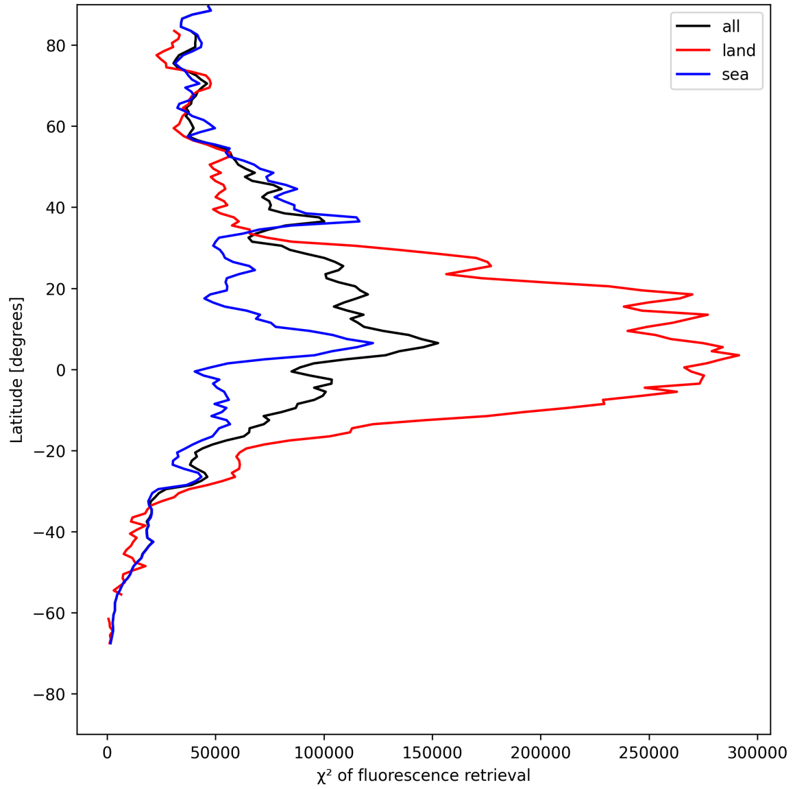
Figure 25: Zonal average of “ \chi^2 of fluorescence retrieval” for 2025-05-17 to 2025-05-19.
