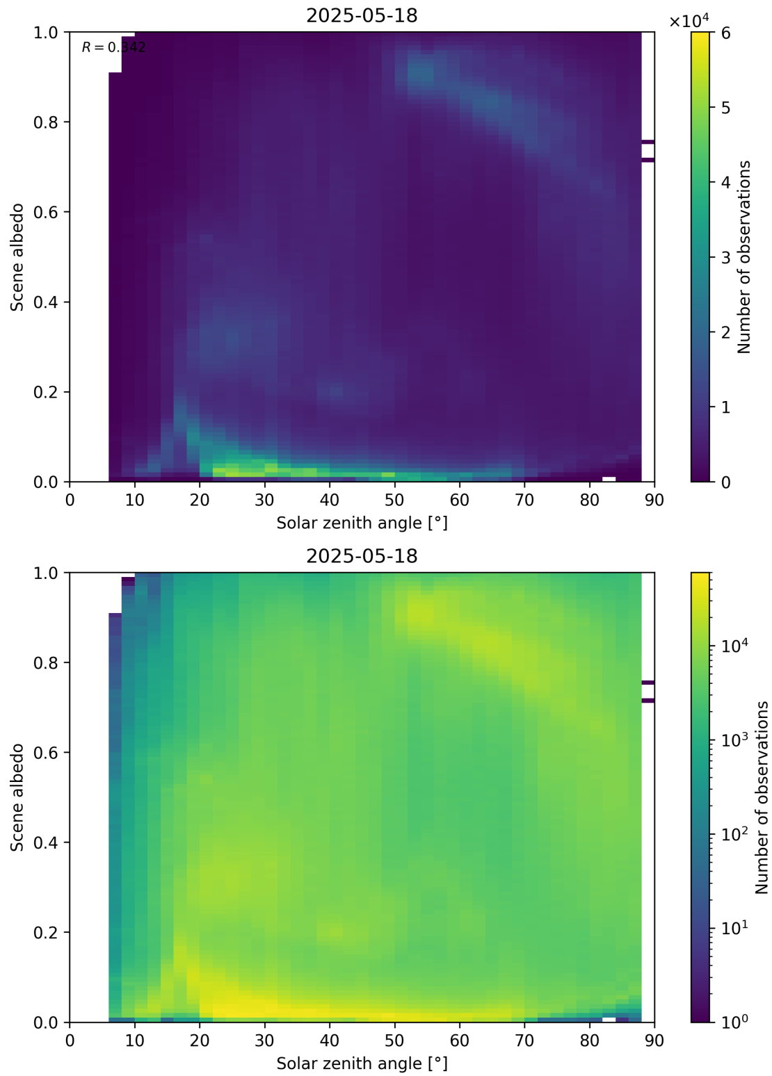
Figure 116: Scatter density plot of “Solar zenith angle” against “Scene albedo” for 2025-05-17 to 2025-05-19.
