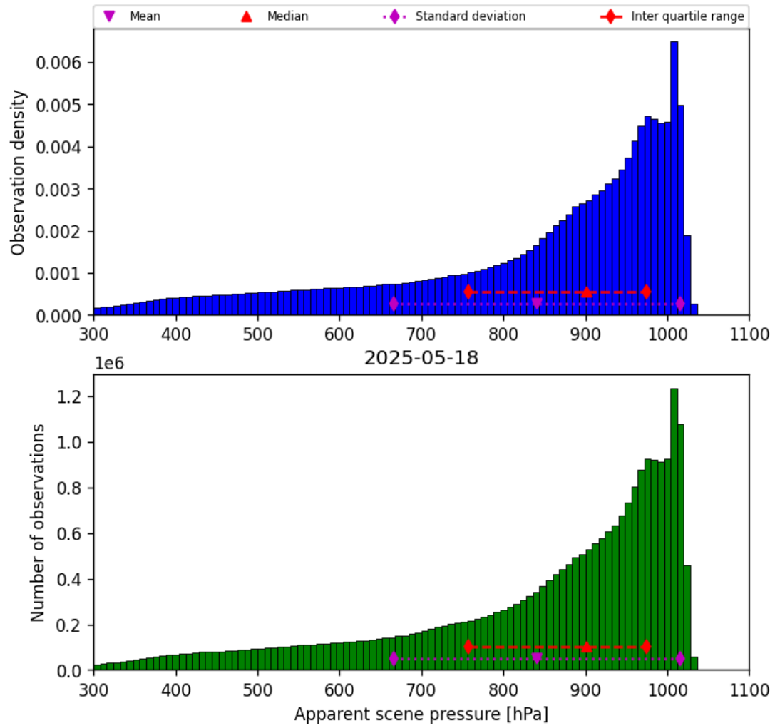
Figure 36: Histogram of “Apparent scene pressure” for 2025-05-17 to 2025-05-19
