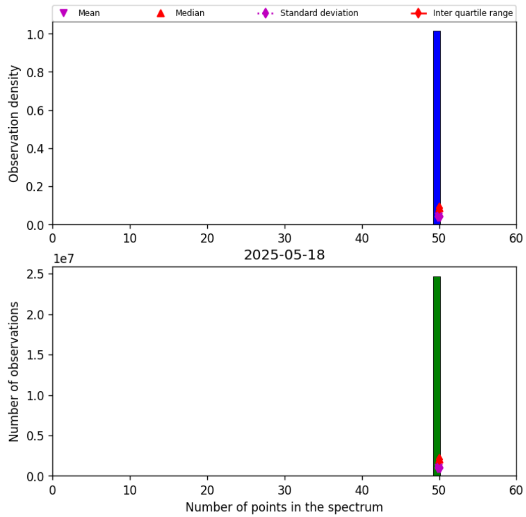
Figure 44: Histogram of “Number of points in the spectrum” for 2025-05-17 to 2025-05-19
