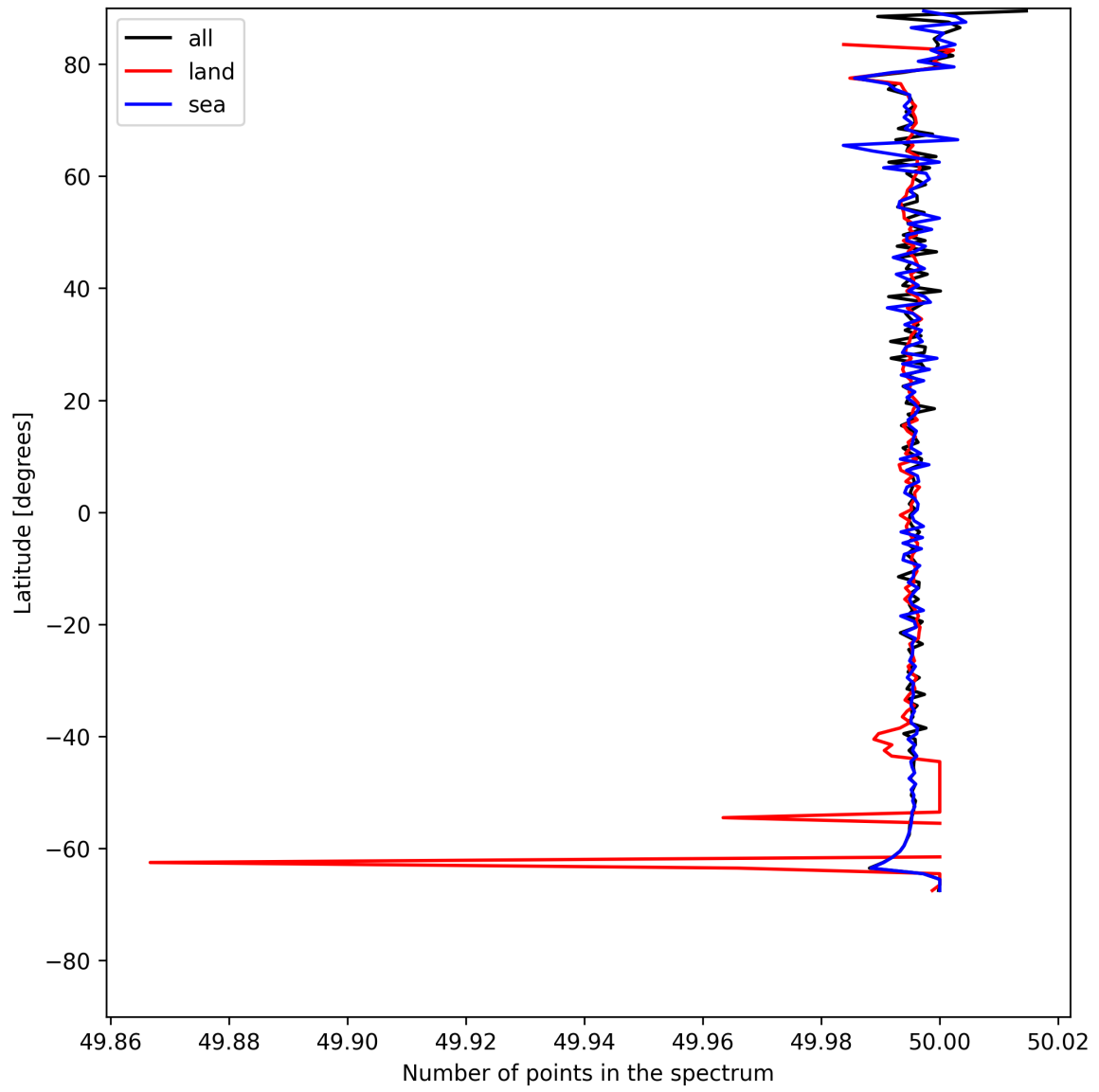
Figure 27: Zonal average of “Number of points in the spectrum” for 2025-05-17 to 2025-05-19.
