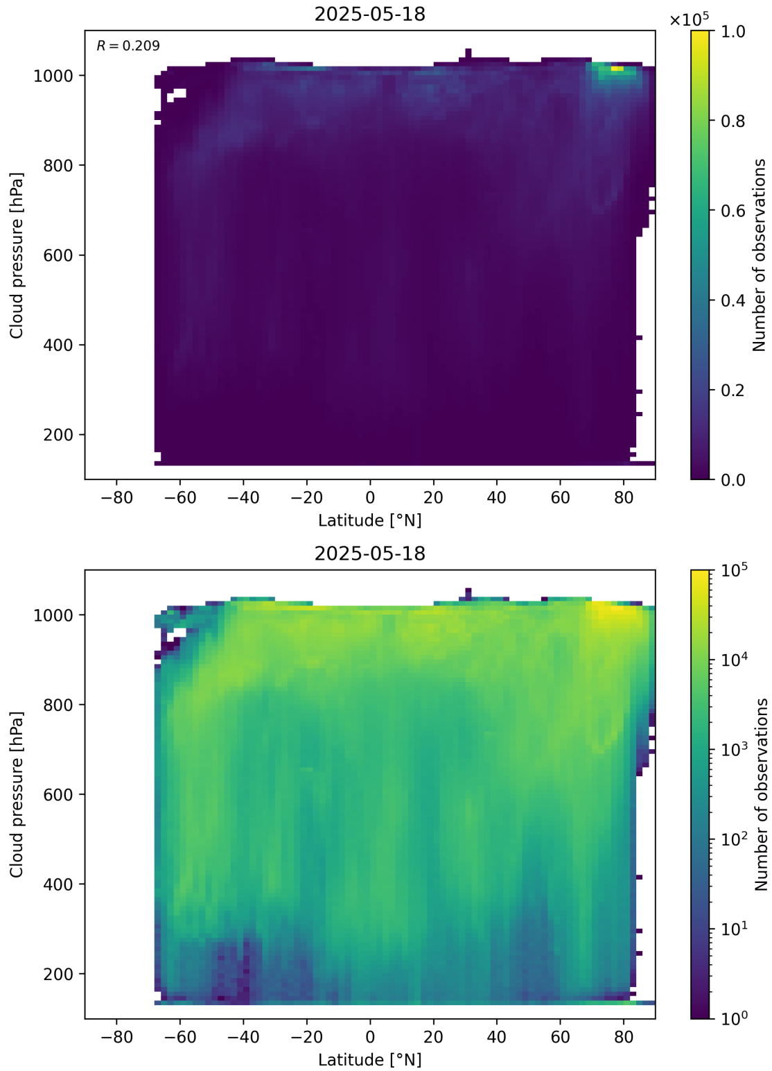
Figure 91: Scatter density plot of “Latitude” against “Cloud pressure” for 2025-05-17 to 2025-05-19.
