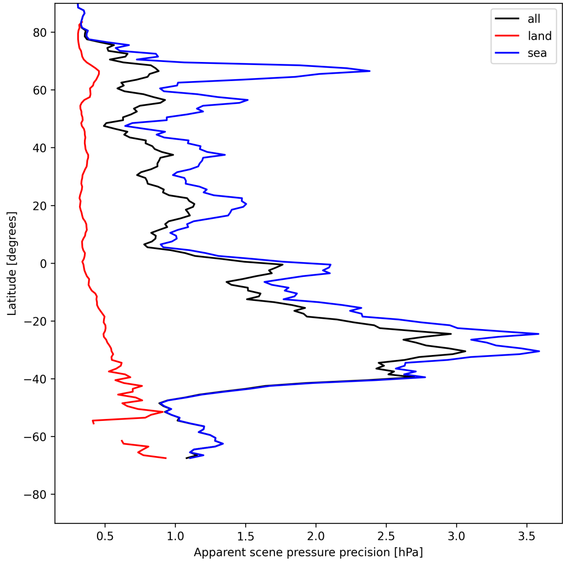
Figure 20: Zonal average of “Apparent scene pressure precision” for 2025-05-17 to 2025-05-19.
