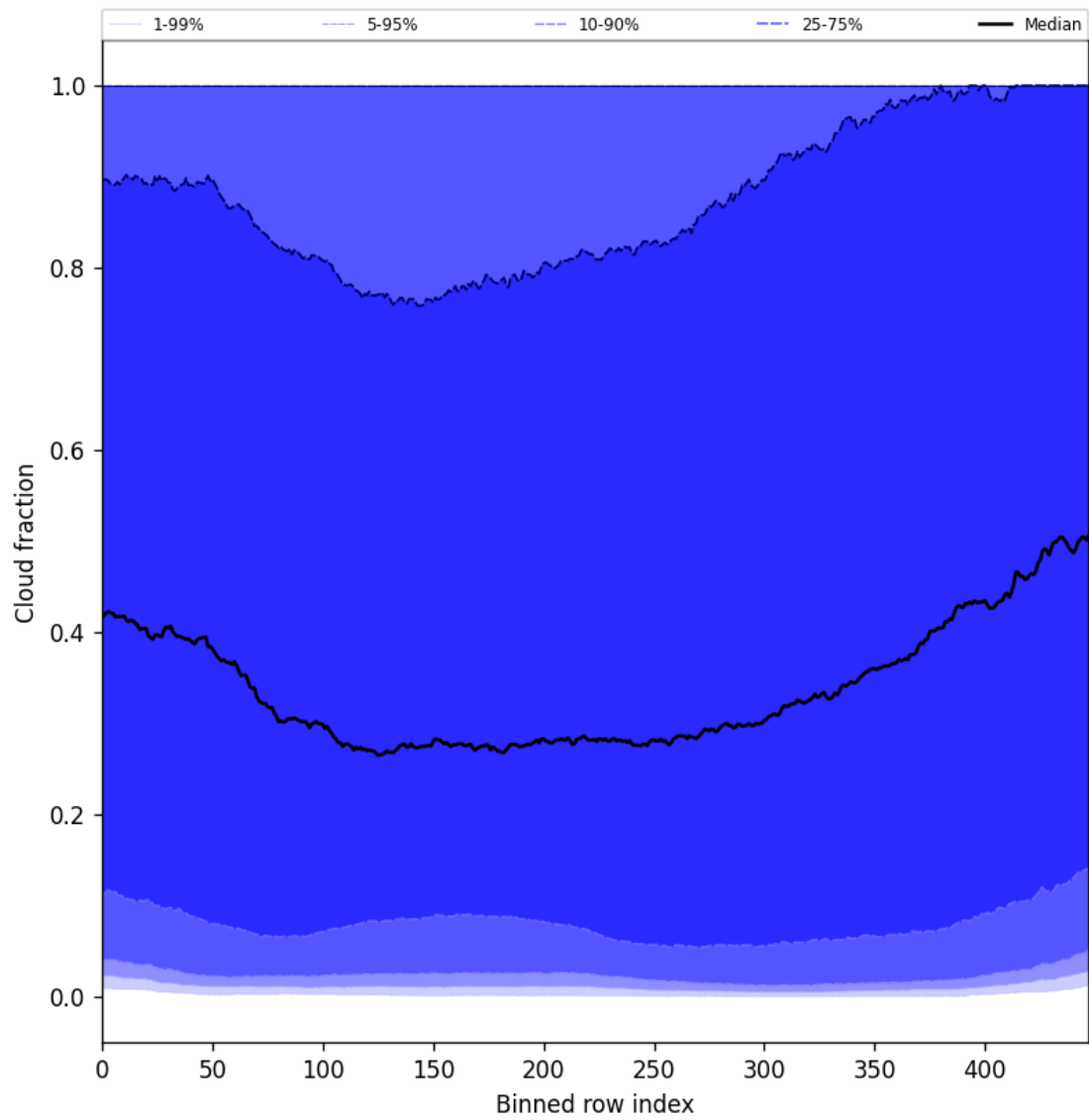
Figure 49: Along track statistics of “Cloud fraction” for 2025-05-17 to 2025-05-19
