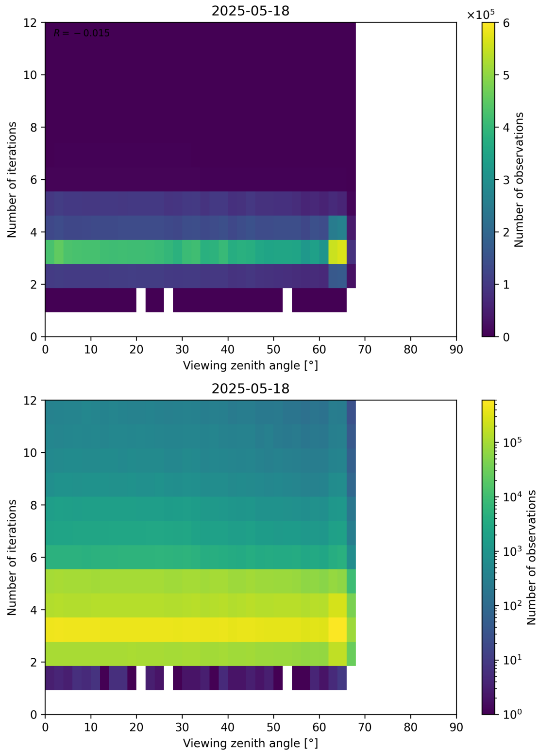
Figure 124: Scatter density plot of “Viewing zenith angle” against “Number of iterations” for 2025-05-17 to 2025-05-19.
