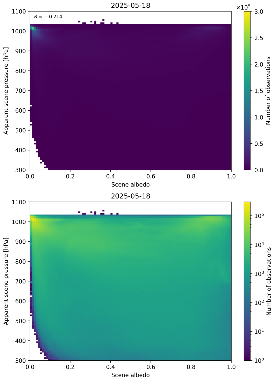
Figure 102: Scatter density plot of “Scene albedo” against “Apparent scene pressure” for 2025-05-17 to 2025-05-19.
