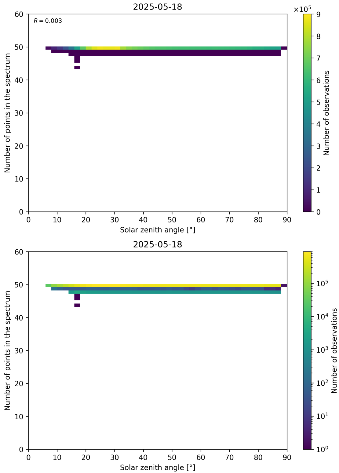
Figure 115: Scatter density plot of “Solar zenith angle” against “Number of points in the spectrum” for 2025-05-17 to 2025-05-19.
