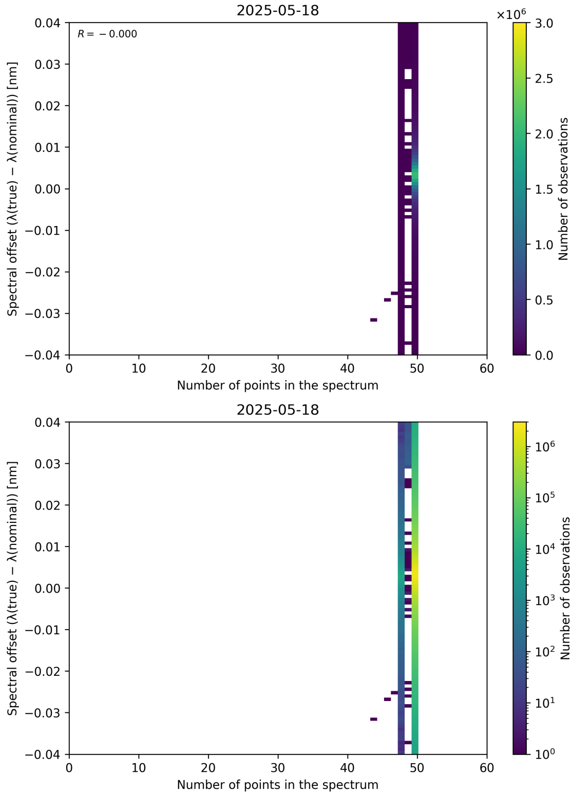
Figure 101: Scatter density plot of “Number of points in the spectrum” against “Spectral offset ( \lambda_{\text{true}} - \lambda_{\text{nominal}} )” for 2025-05-17 to 2025-05-19.
