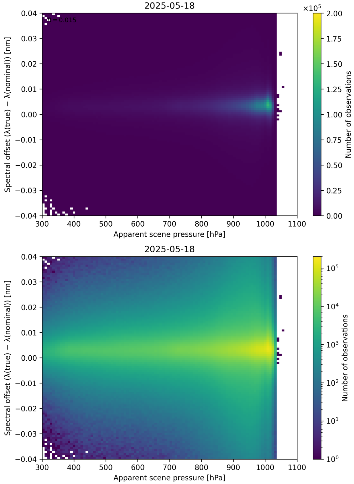
Figure 67: Scatter density plot of “Apparent scene pressure” against “Spectral offset ( \lambda_{\text{true}} - \lambda_{\text{nominal}} )” for 2025-05-17 to 2025-05-19.
