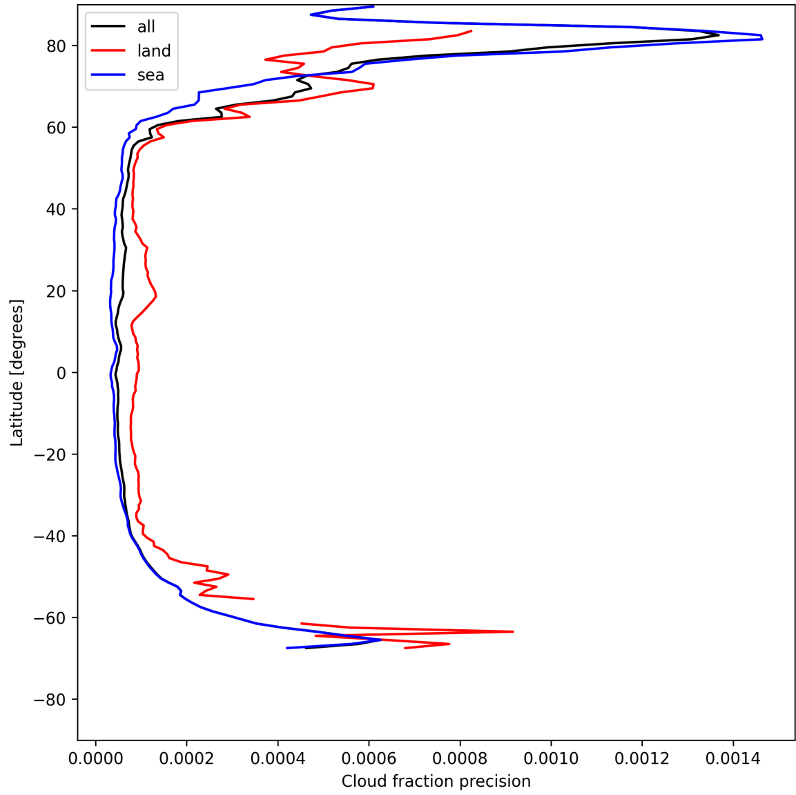
Figure 16: Zonal average of “Cloud fraction precision” for 2025-05-17 to 2025-05-19.
