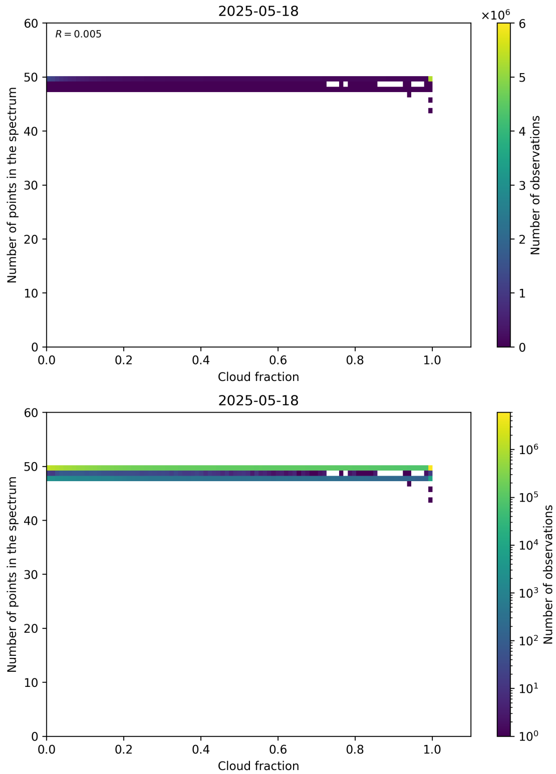
Figure 74: Scatter density plot of “Cloud fraction” against “Number of points in the spectrum” for 2025-05-17 to 2025-05-19.
