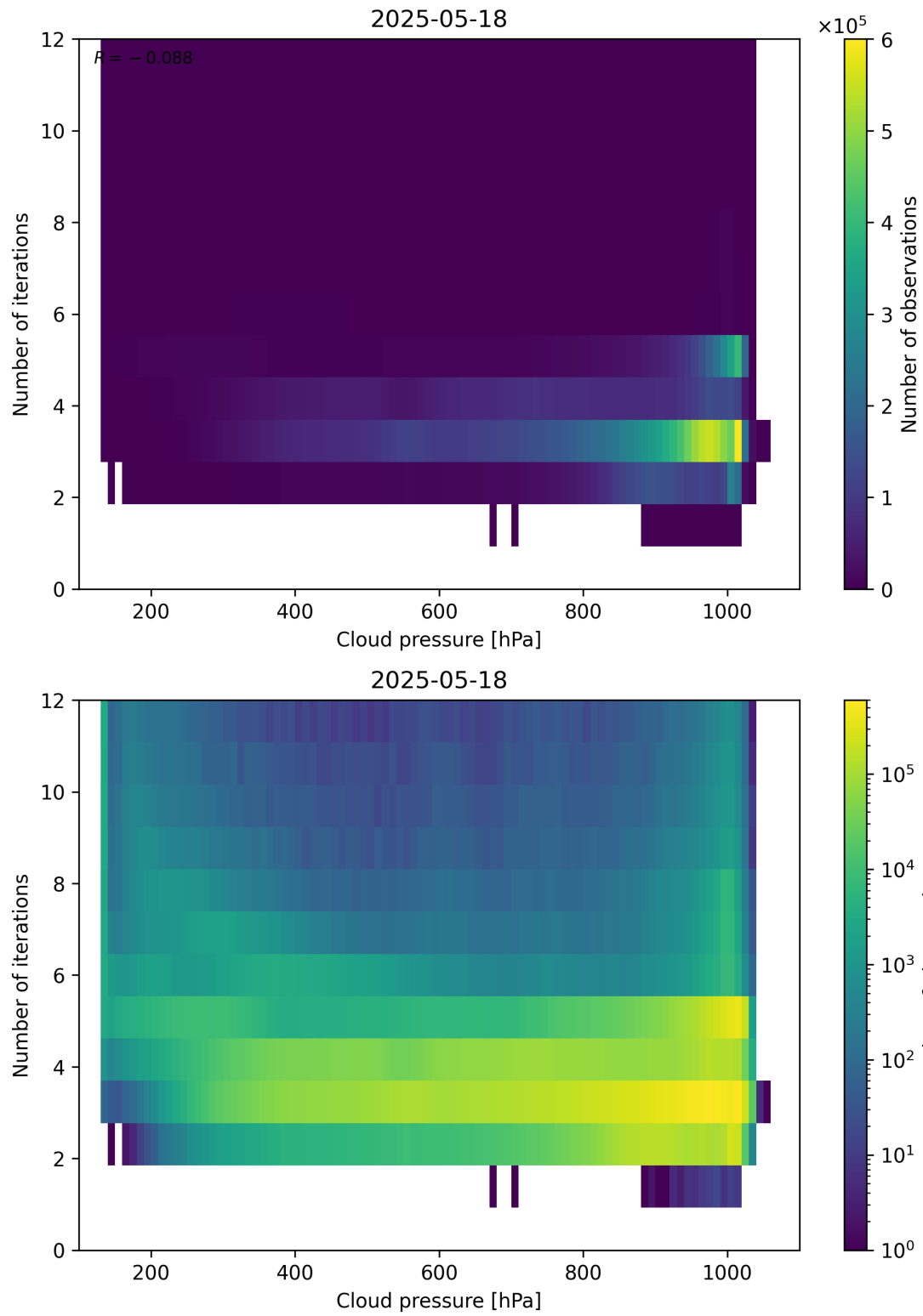
Figure 81: Scatter density plot of “Cloud pressure” against “Number of iterations” for 2025-05-17 to 2025-05-19.
