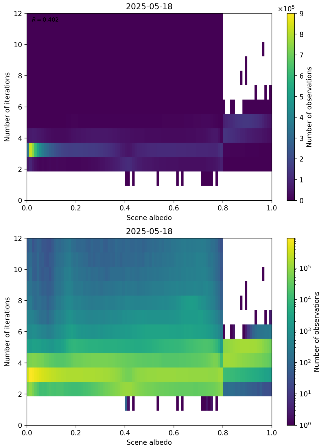
Figure 105: Scatter density plot of “Scene albedo” against “Number of iterations” for 2025-05-17 to 2025-05-19.
