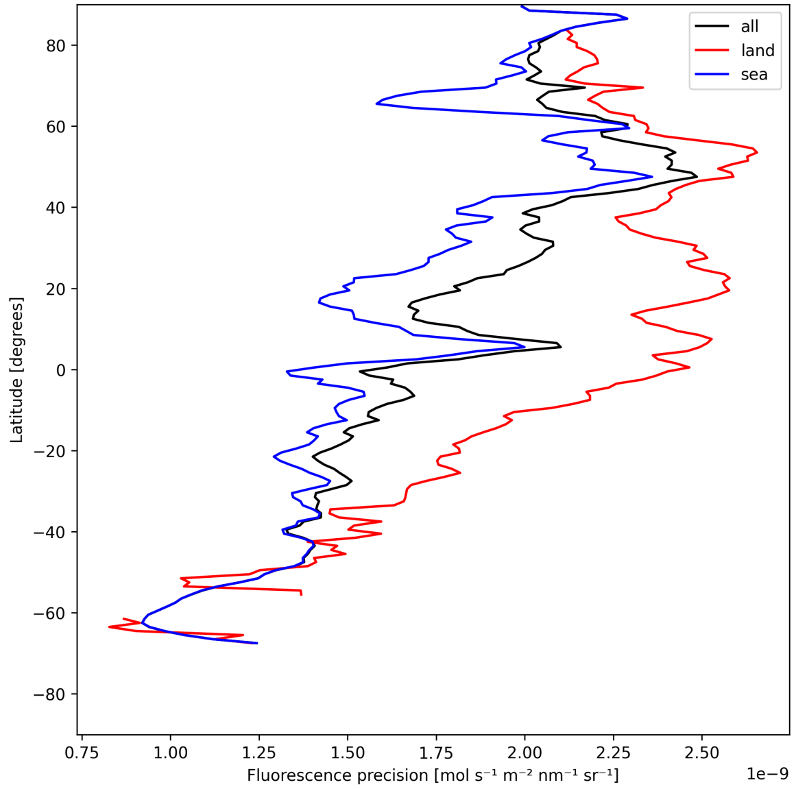
Figure 24: Zonal average of “Fluorescence precision” for 2025-05-17 to 2025-05-19.
