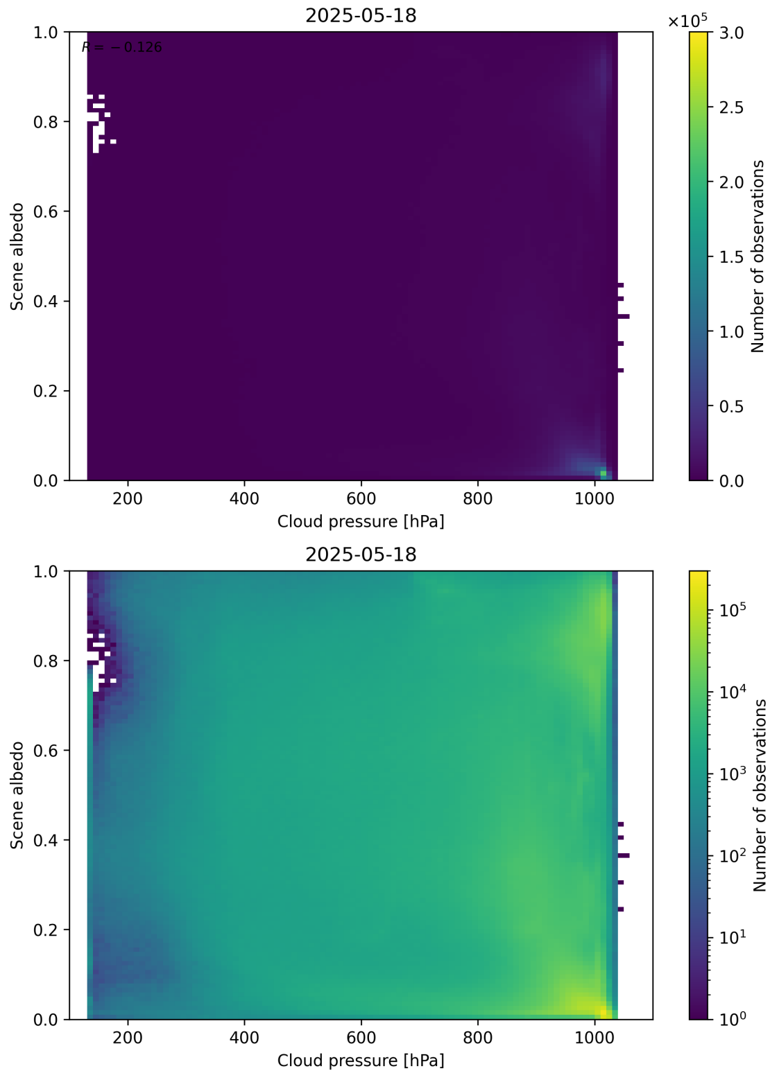
Figure 83: Scatter density plot of “Cloud pressure” against “Scene albedo” for 2025-05-17 to 2025-05-19.
