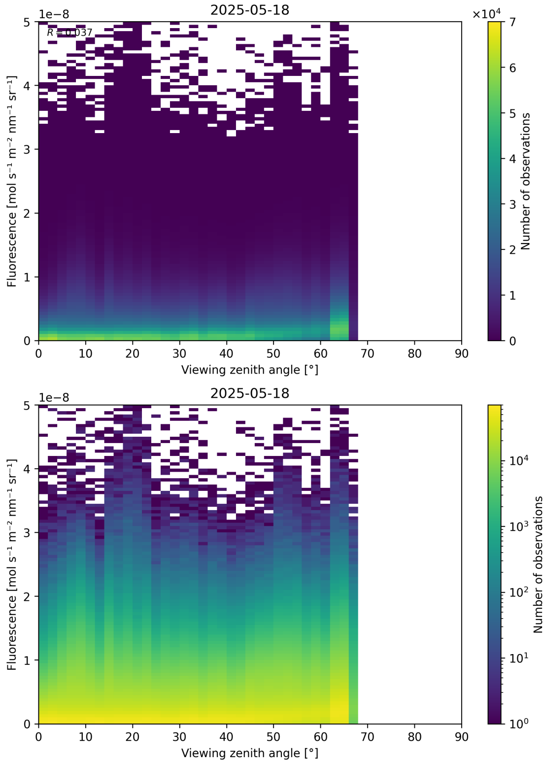
Figure 122: Scatter density plot of “Viewing zenith angle” against “Fluorescence” for 2025-05-17 to 2025-05-19.
