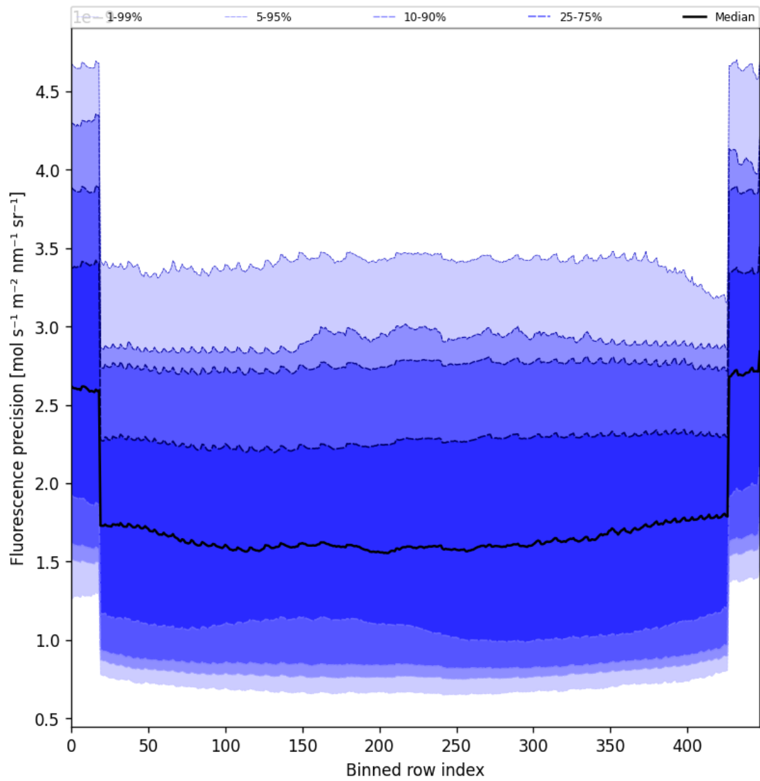
Figure 58: Along track statistics of “Fluorescence precision” for 2025-05-17 to 2025-05-19
