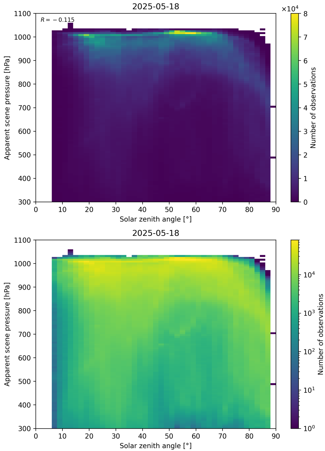
Figure 108: Scatter density plot of “Solar zenith angle” against “Apparent scene pressure” for 2025-05-17 to 2025-05-19.
