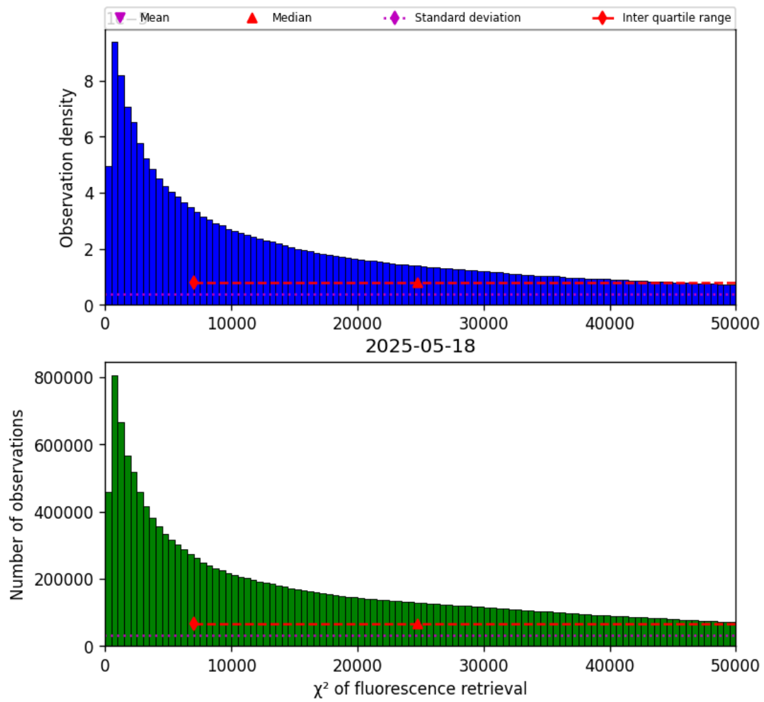
Figure 42: Histogram of “ \chi^2 of fluorescence retrieval” for 2025-05-17 to 2025-05-19
