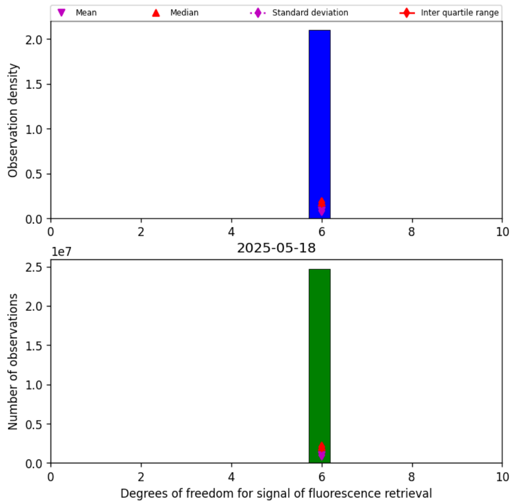
Figure 43: Histogram of “Degrees of freedom for signal of fluorescence retrieval” for 2025-05-17 to 2025-05-19
