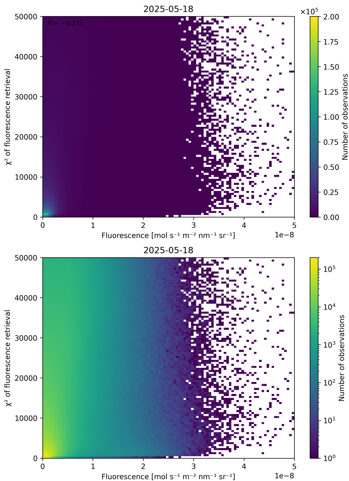
Figure 85: Scatter density plot of “Fluorescence” against “ \chi^2 of fluorescence retrieval” for 2025-05-17 to 2025-05-19.
