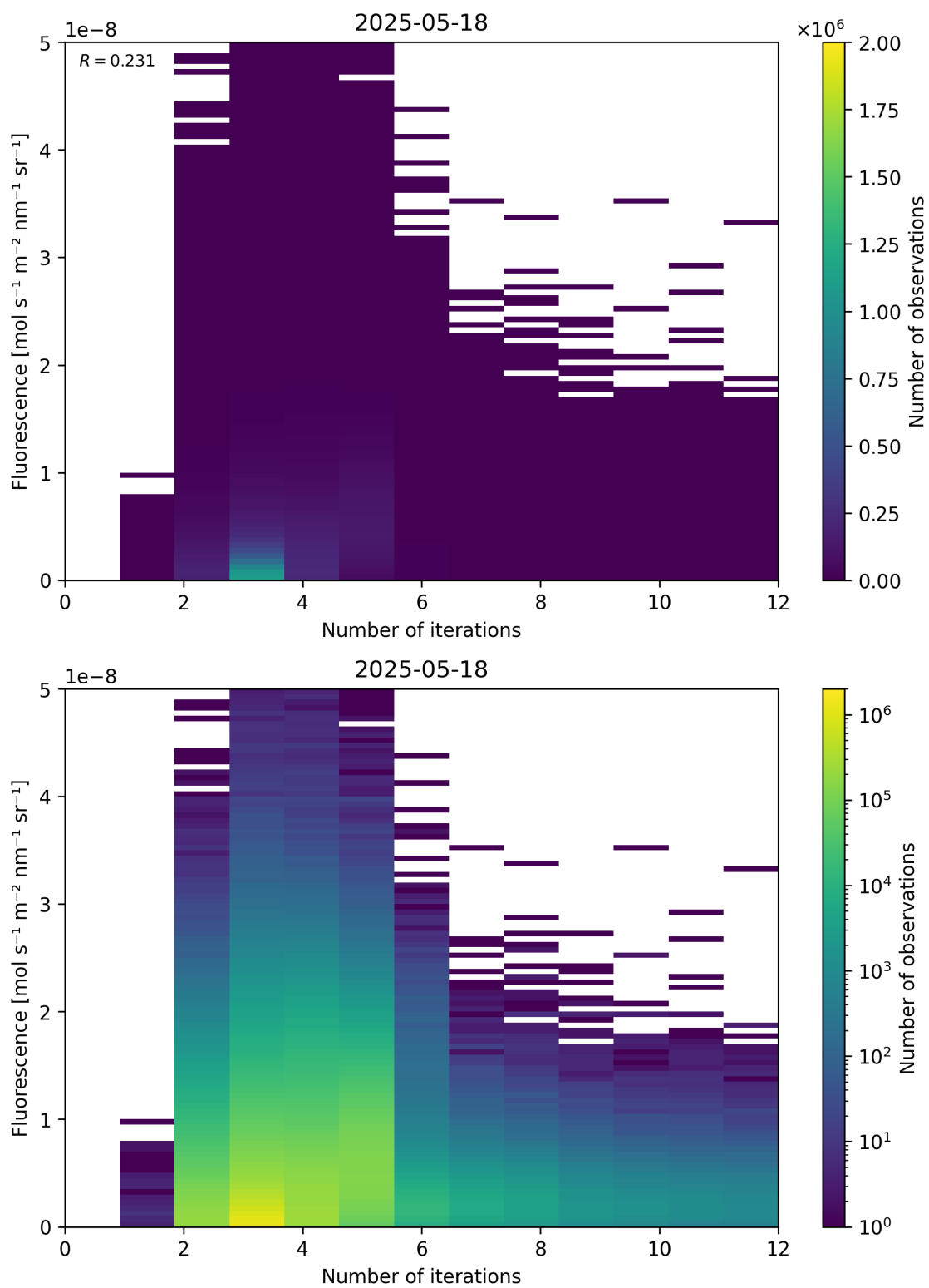
Figure 98: Scatter density plot of “Number of iterations” against “Fluorescence” for 2025-05-17 to 2025-05-19.
