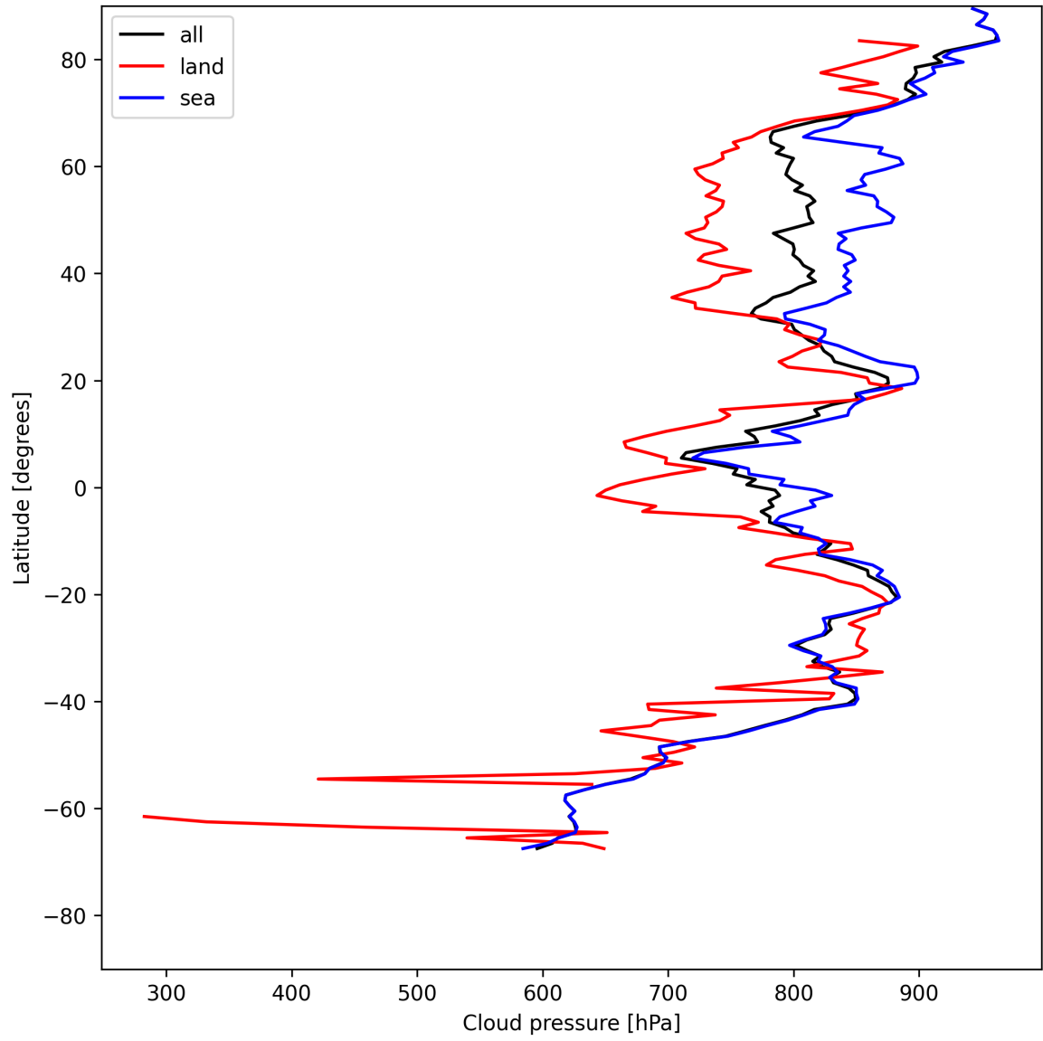
Figure 13: Zonal average of “Cloud pressure” for 2025-05-17 to 2025-05-19.
