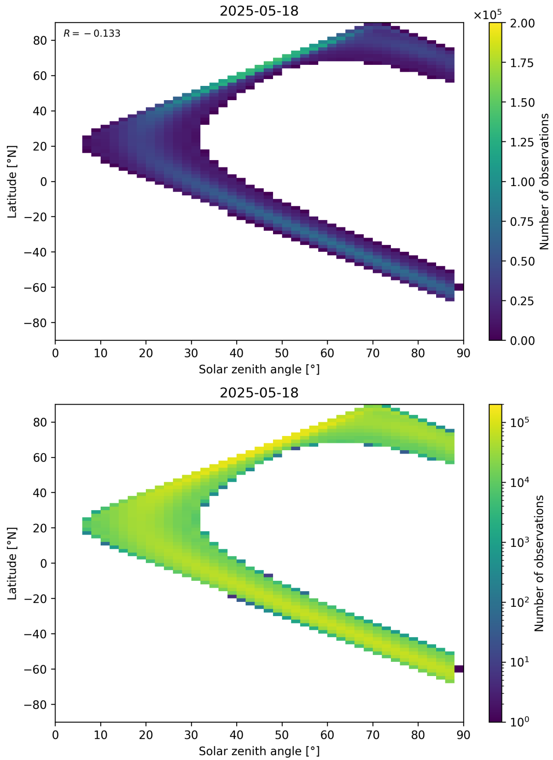
Figure 113: Scatter density plot of “Solar zenith angle” against “Latitude” for 2025-05-17 to 2025-05-19.
