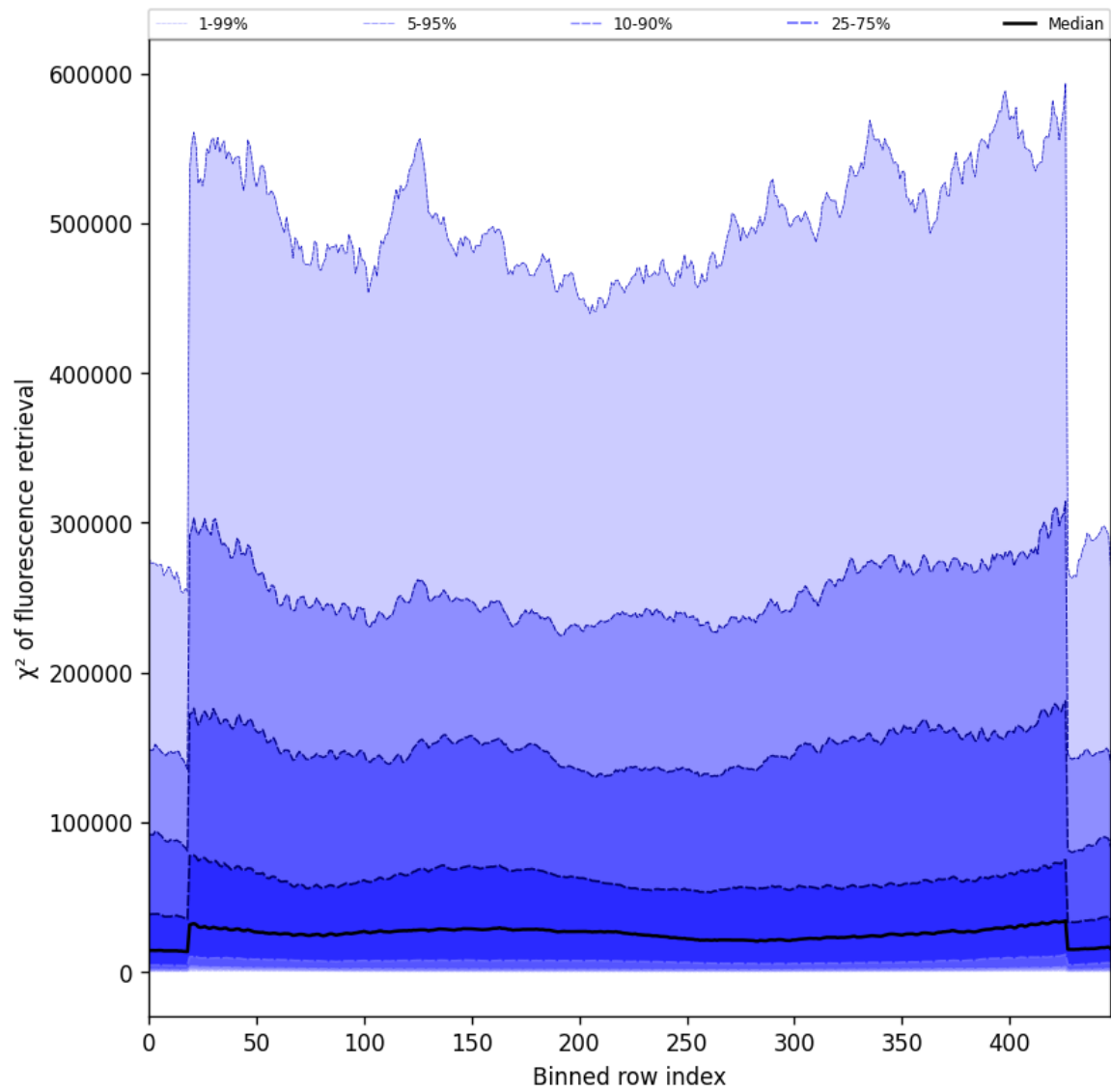
Figure 59: Along track statistics of “ \chi^2 of fluorescence retrieval” for 2025-05-17 to 2025-05-19
