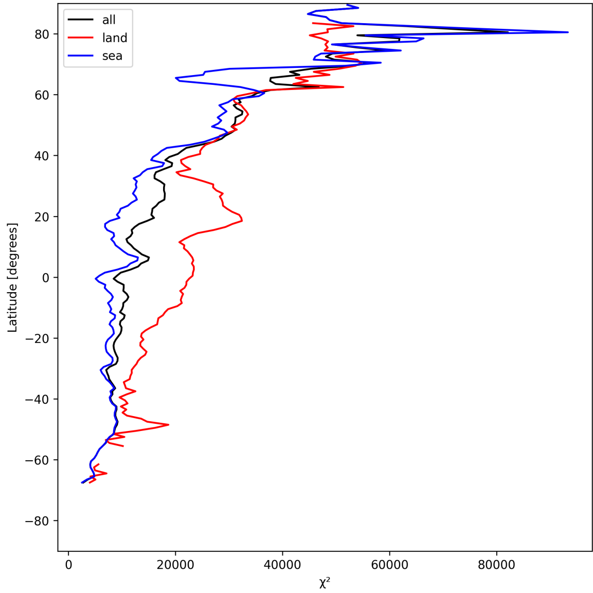
Figure 21: Zonal average of “ \chi^2 ” for 2025-05-17 to 2025-05-19.
