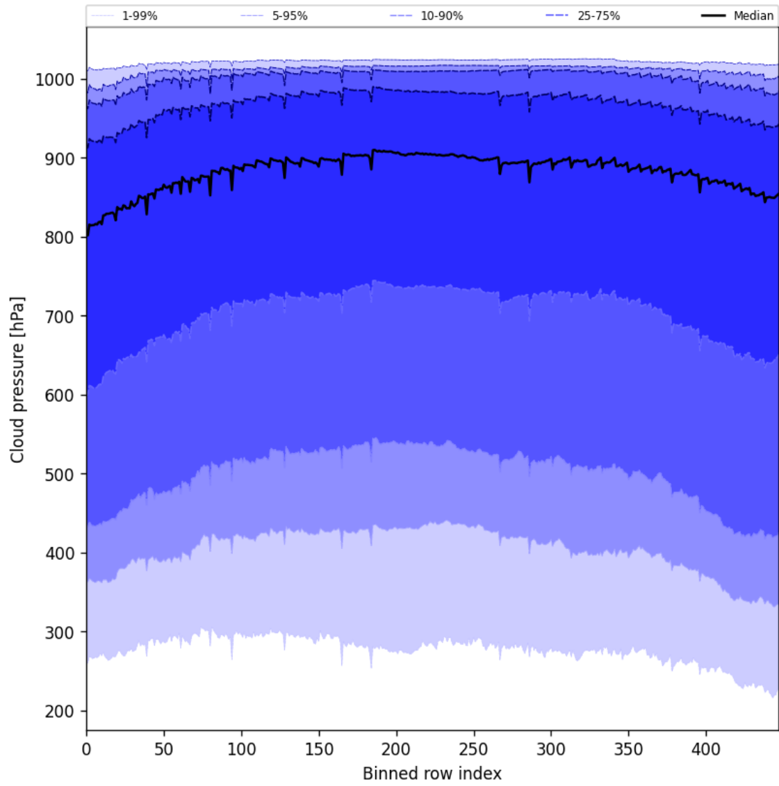
Figure 47: Along track statistics of “Cloud pressure” for 2025-05-17 to 2025-05-19
