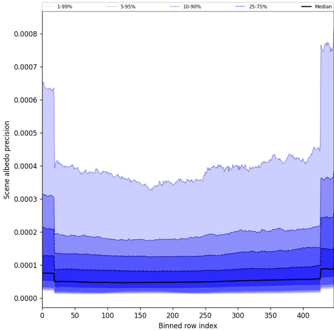
Figure 52: Along track statistics of “Scene albedo precision” for 2025-05-17 to 2025-05-19
