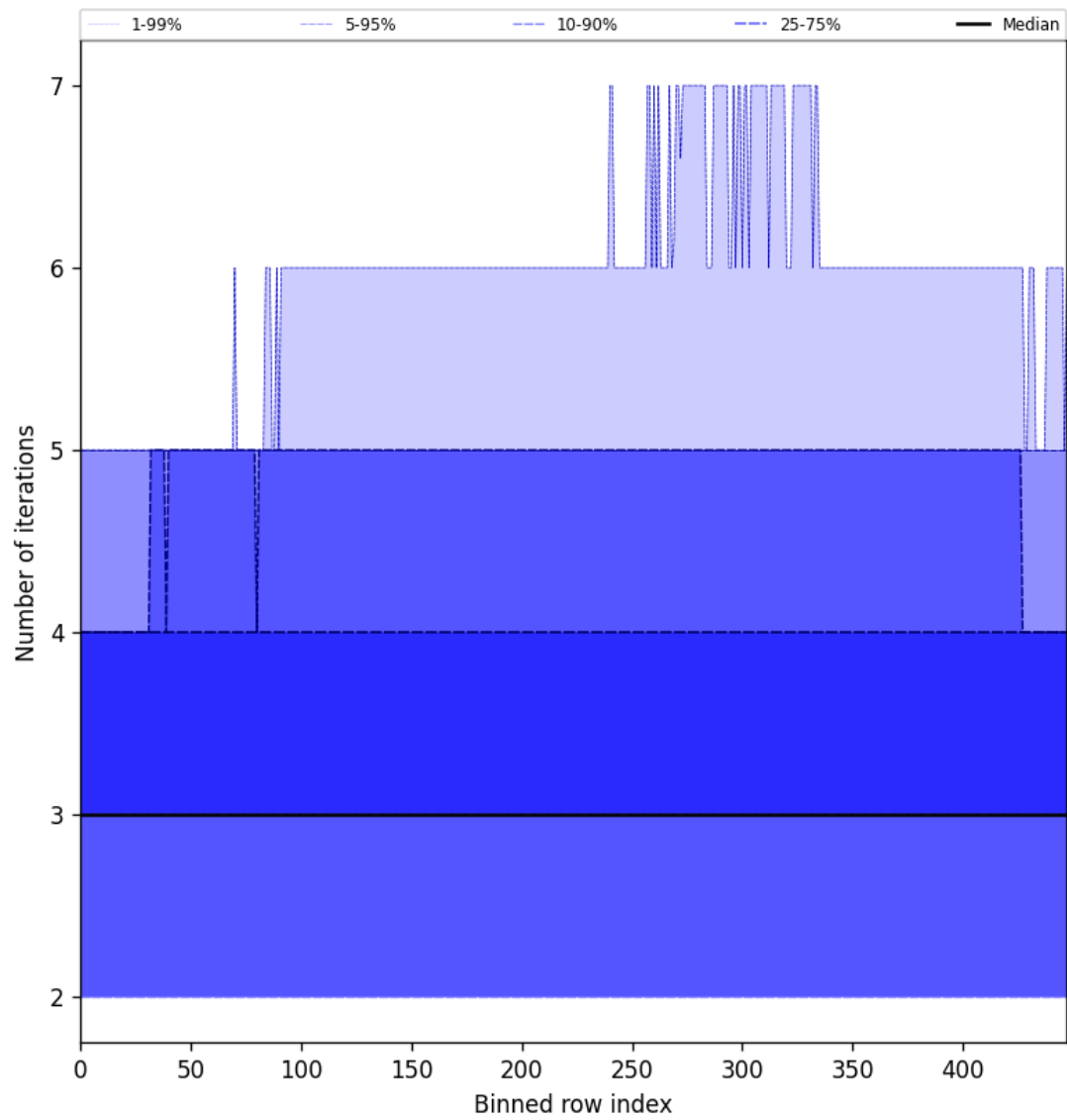
Figure 56: Along track statistics of “Number of iterations” for 2025-05-17 to 2025-05-19
