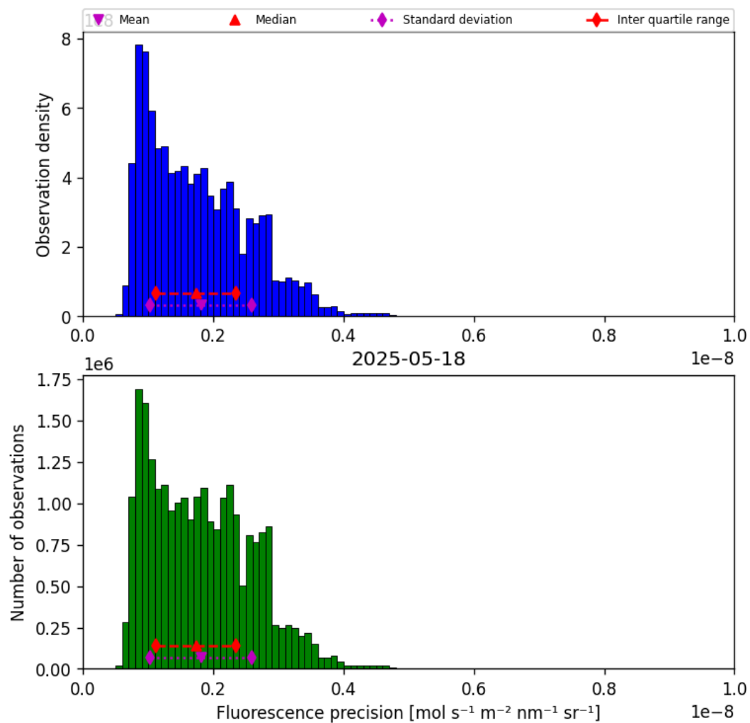
Figure 41: Histogram of “Fluorescence precision” for 2025-05-17 to 2025-05-19
