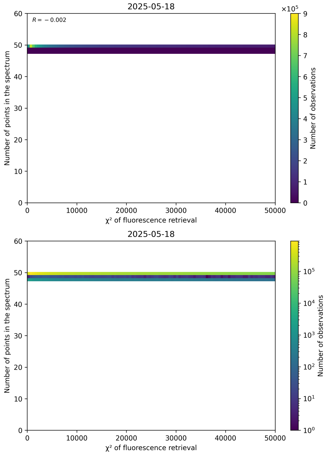
Figure 68: Scatter density plot of “ \chi^2 of fluorescence retrieval” against “Number of points in the spectrum” for 2025-05-17 to 2025-05-19.
