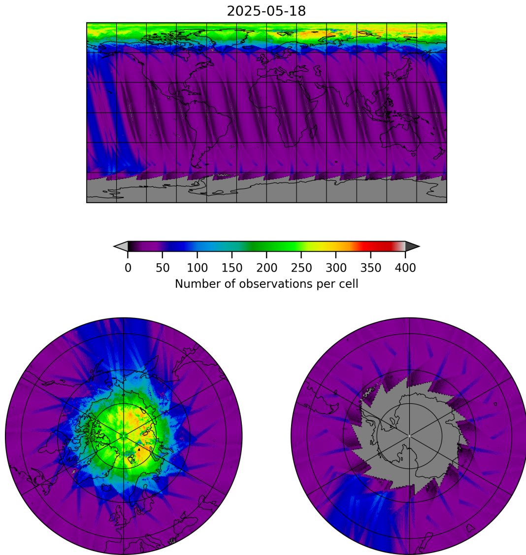
Figure 11: Map of the number of observations for 2025-05-17 to 2025-05-19
