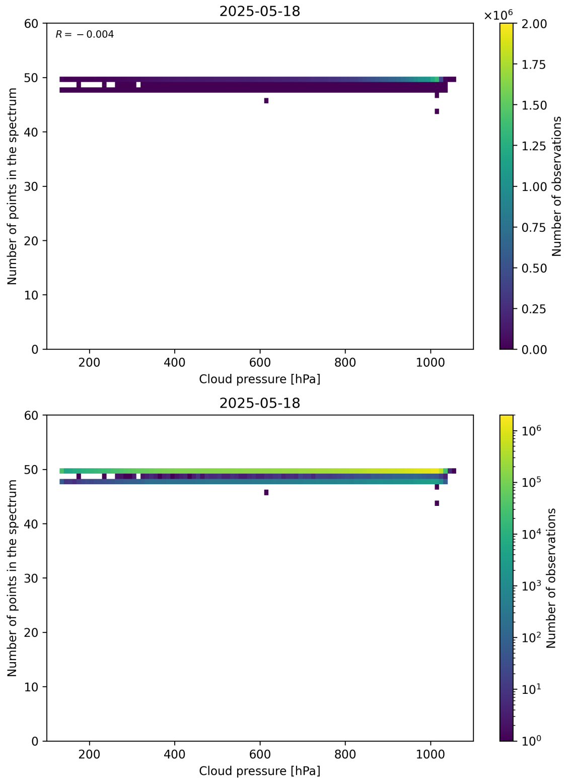
Figure 82: Scatter density plot of “Cloud pressure” against “Number of points in the spectrum” for 2025-05-17 to 2025-05-19.
