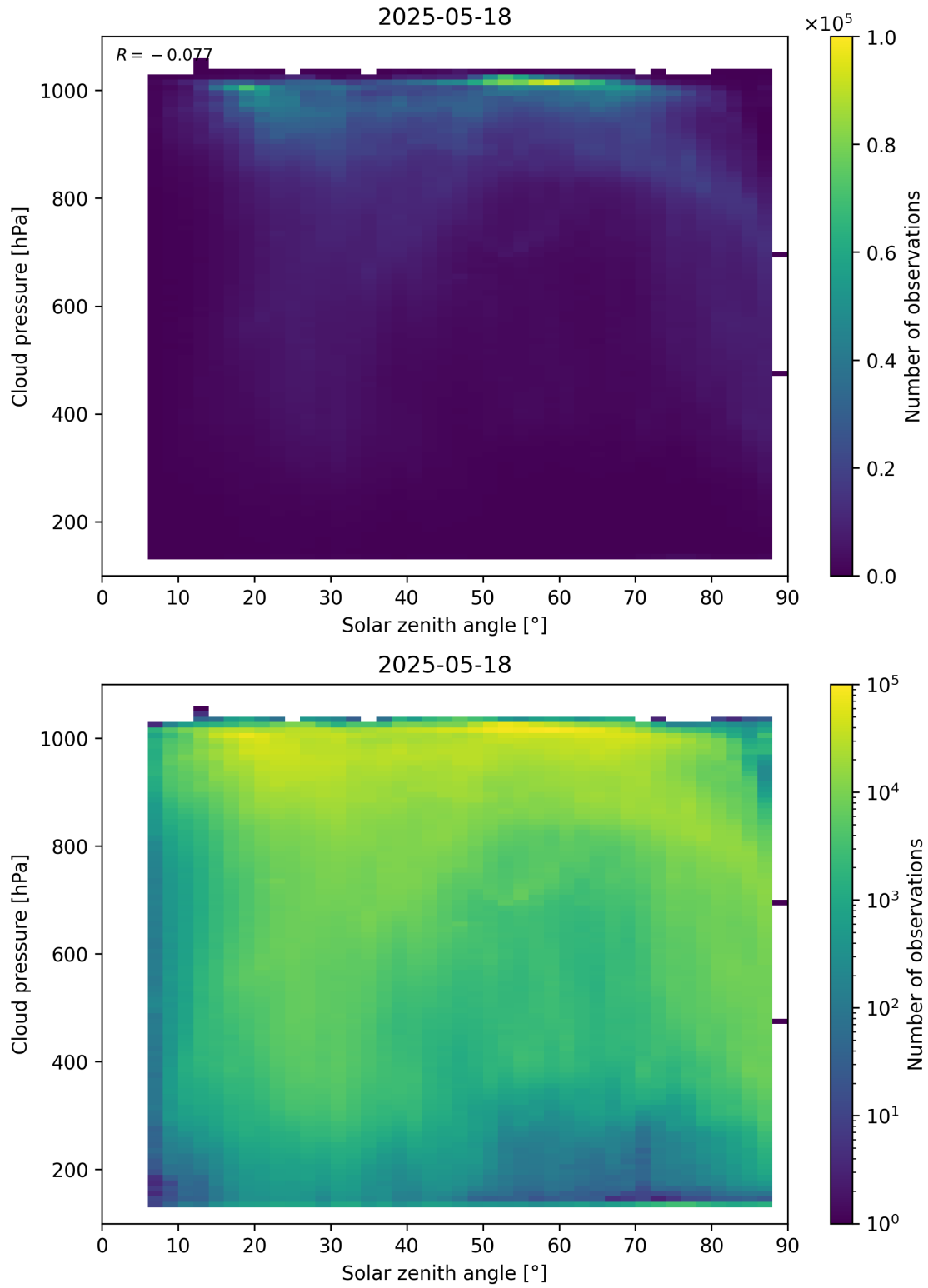
Figure 111: Scatter density plot of “Solar zenith angle” against “Cloud pressure” for 2025-05-17 to 2025-05-19.
