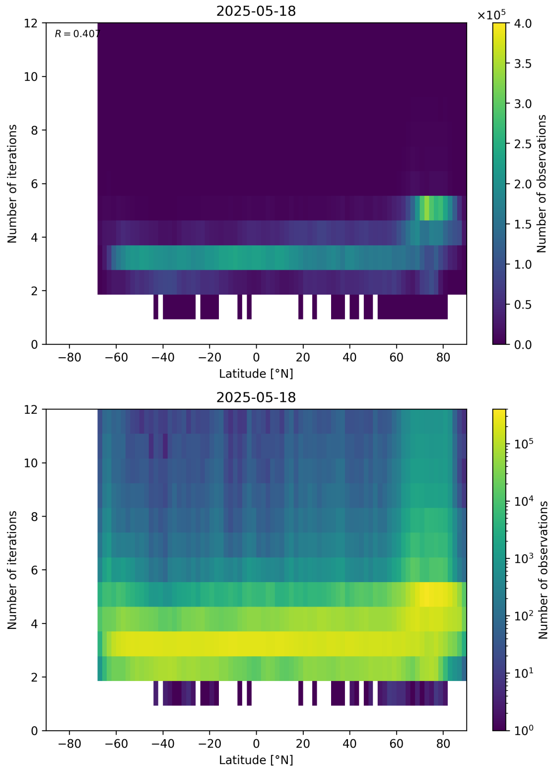
Figure 93: Scatter density plot of “Latitude” against “Number of iterations” for 2025-05-17 to 2025-05-19.
