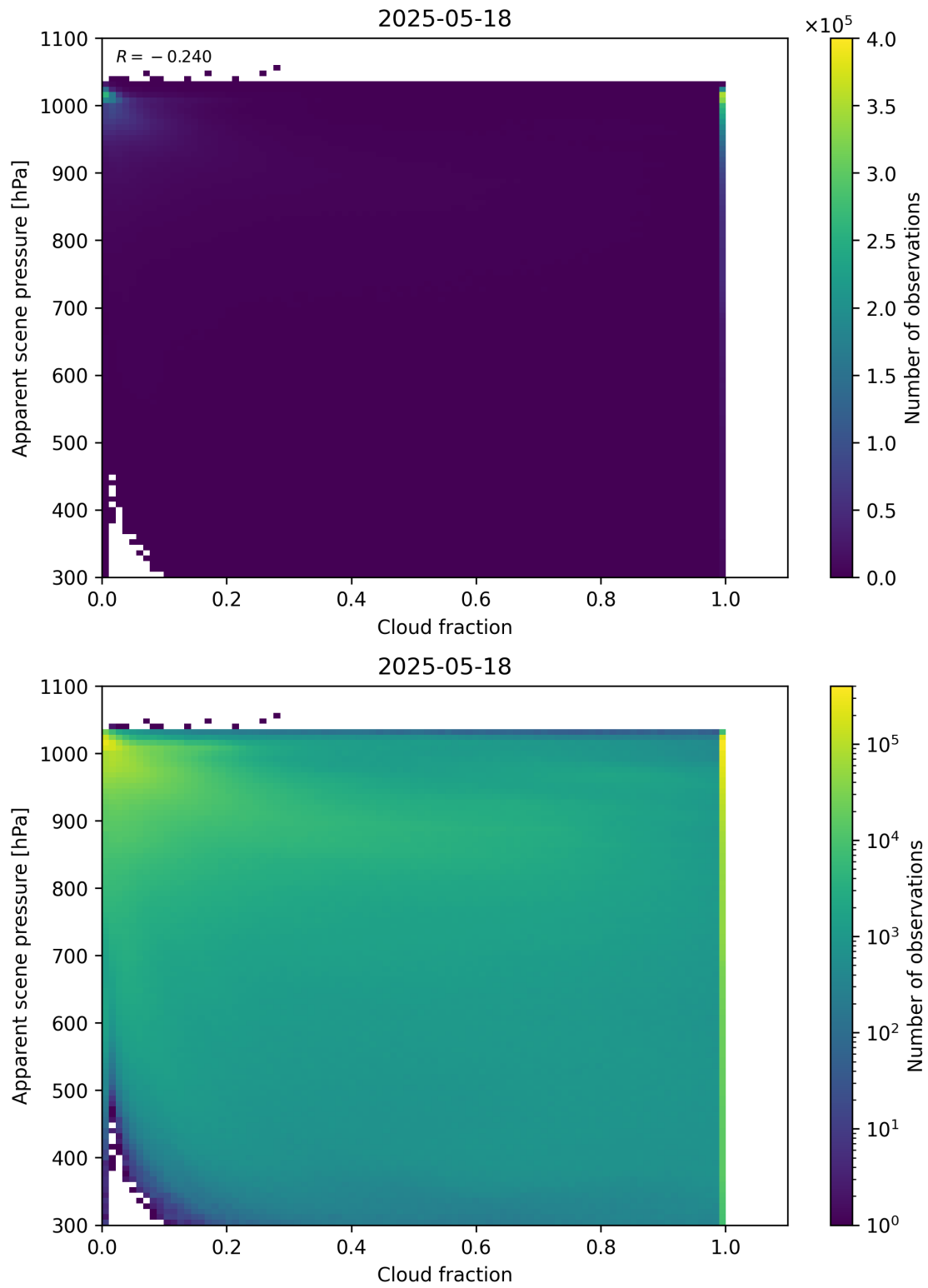
Figure 70: Scatter density plot of “Cloud fraction” against “Apparent scene pressure” for 2025-05-17 to 2025-05-19.
