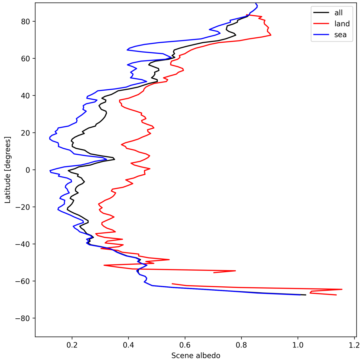
Figure 17: Zonal average of “Scene albedo” for 2025-05-17 to 2025-05-19.
