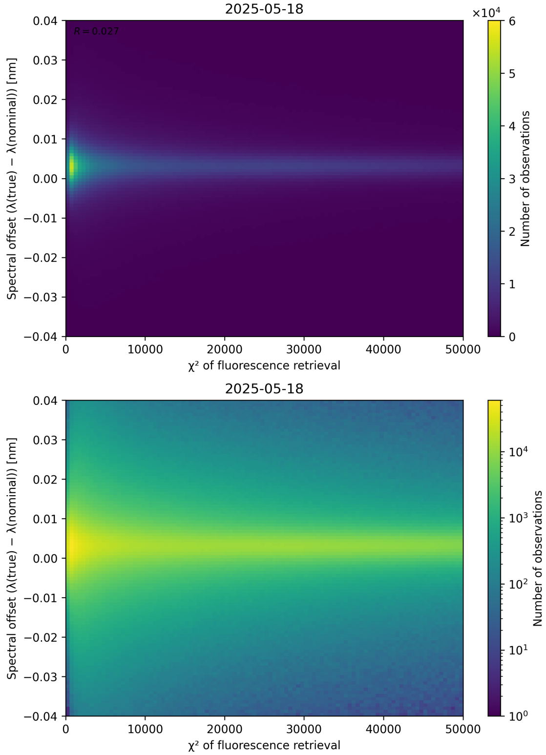
Figure 69: Scatter density plot of “ \chi^2 of fluorescence retrieval” against “Spectral offset ( \lambda_{\text{true}} - \lambda_{\text{nominal}} )” for 2025-05-17 to 2025-05-19.
