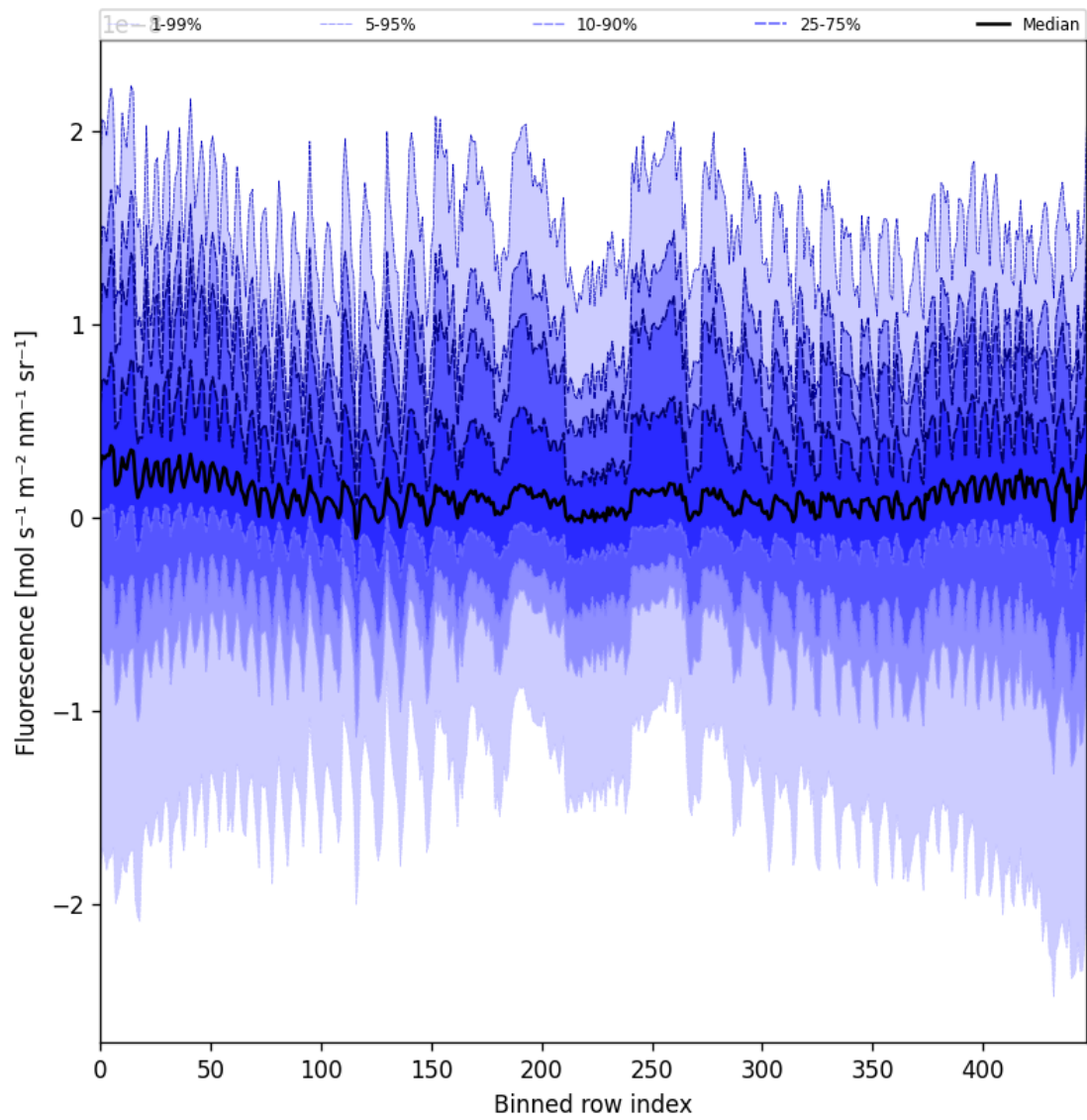
Figure 57: Along track statistics of “Fluorescence” for 2025-05-17 to 2025-05-19
