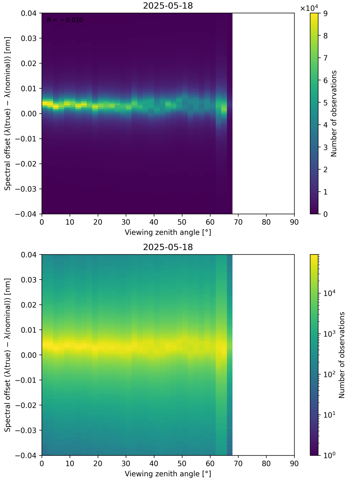
Figure 128: Scatter density plot of “Viewing zenith angle” against “Spectral offset ( \lambda_{\text{true}} - \lambda_{\text{nominal}} )” for 2025-05-17 to 2025-05-19.
