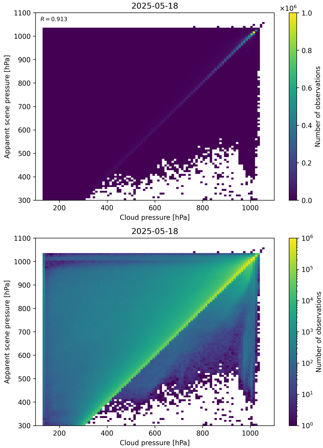
Figure 77: Scatter density plot of “Cloud pressure” against “Apparent scene pressure” for 2025-05-17 to 2025-05-19.
