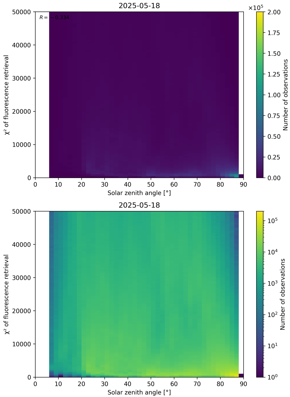
Figure 109: Scatter density plot of “Solar zenith angle” against “ \chi^2 of fluorescence retrieval” for 2025-05-17 to 2025-05-19.
