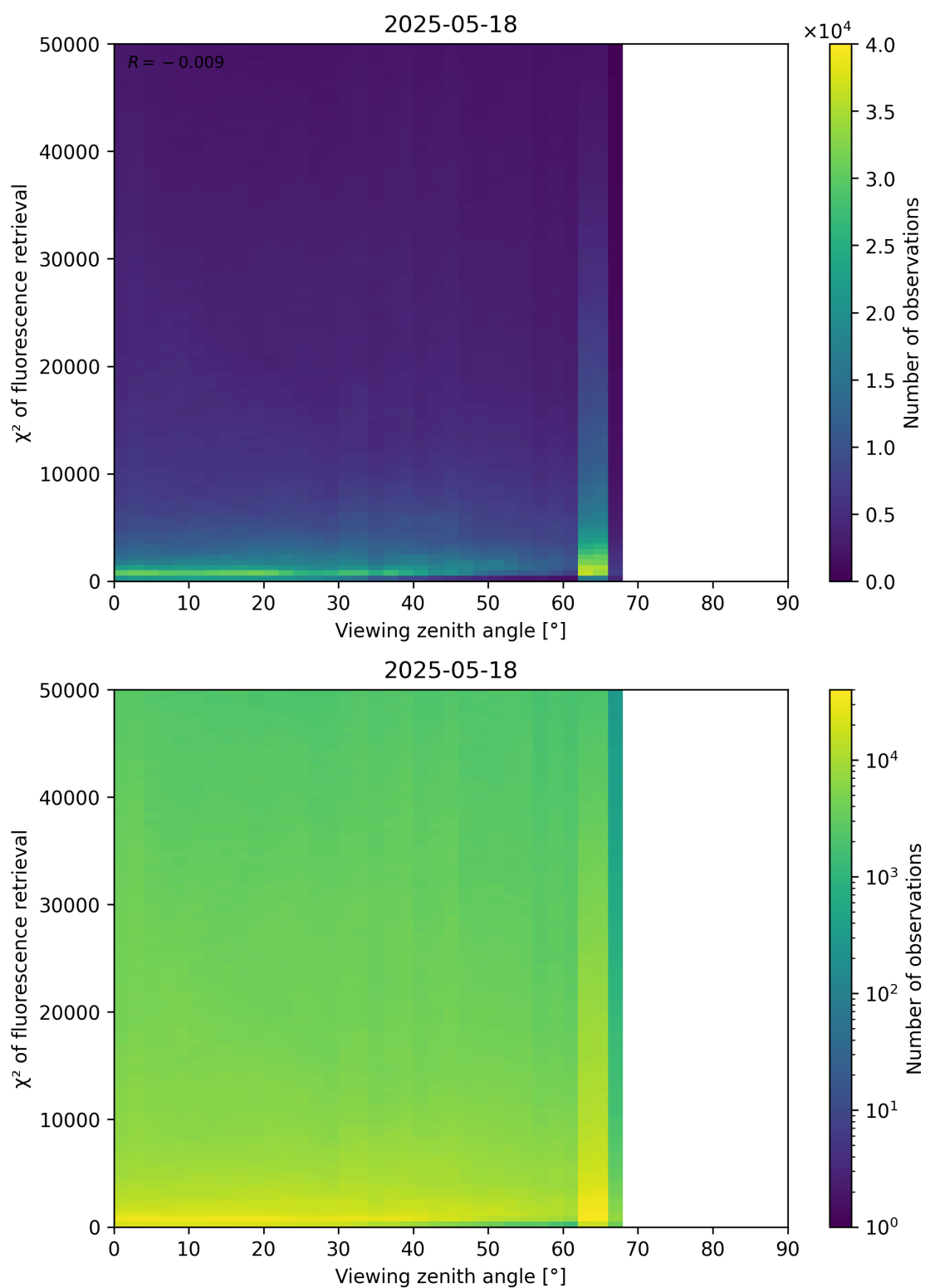
Figure 119: Scatter density plot of “Viewing zenith angle” against “ \chi^2 of fluorescence retrieval” for 2025-05-17 to 2025-05-19.
