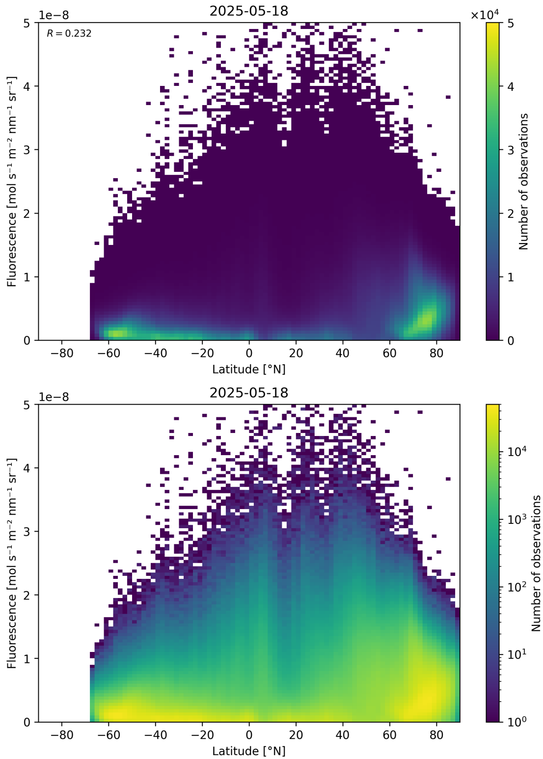
Figure 92: Scatter density plot of “Latitude” against “Fluorescence” for 2025-05-17 to 2025-05-19.
