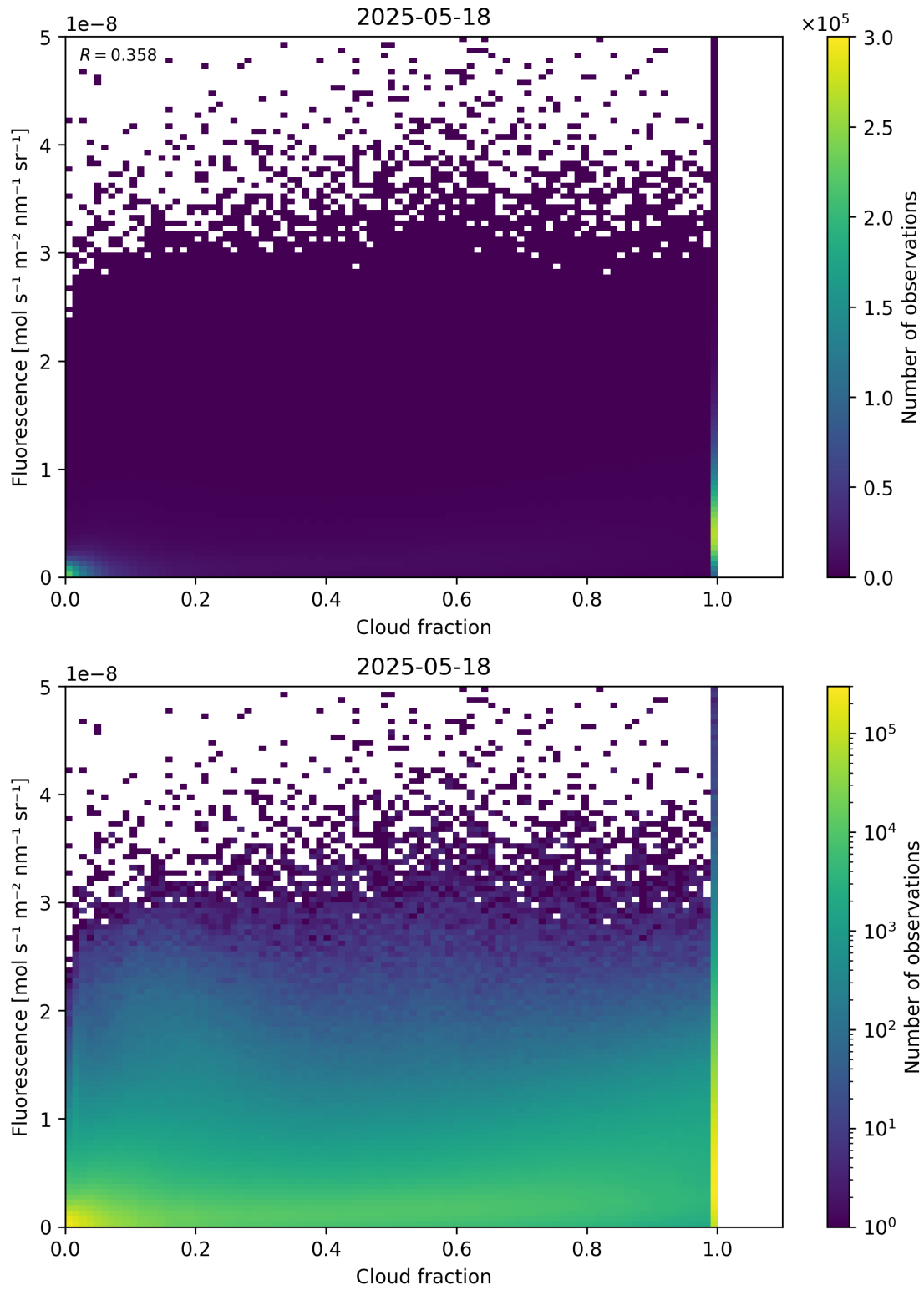
Figure 72: Scatter density plot of “Cloud fraction” against “Fluorescence” for 2025-05-17 to 2025-05-19.
