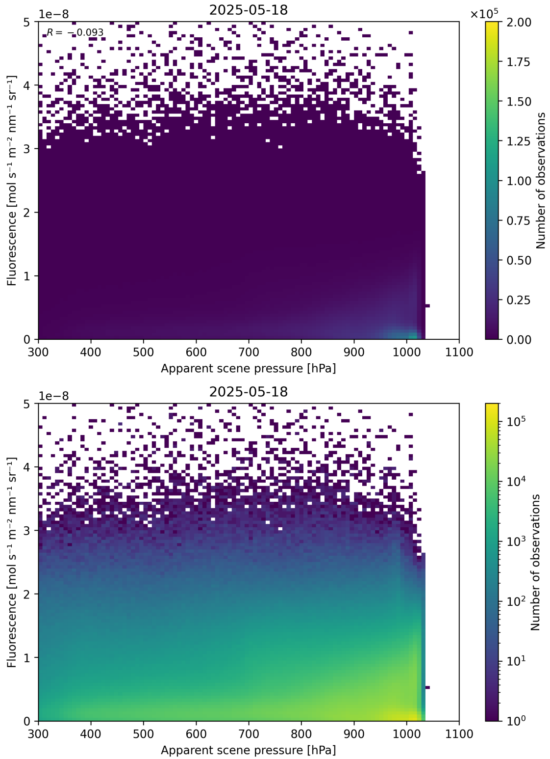
Figure 64: Scatter density plot of “Apparent scene pressure” against “Fluorescence” for 2025-05-17 to 2025-05-19.
