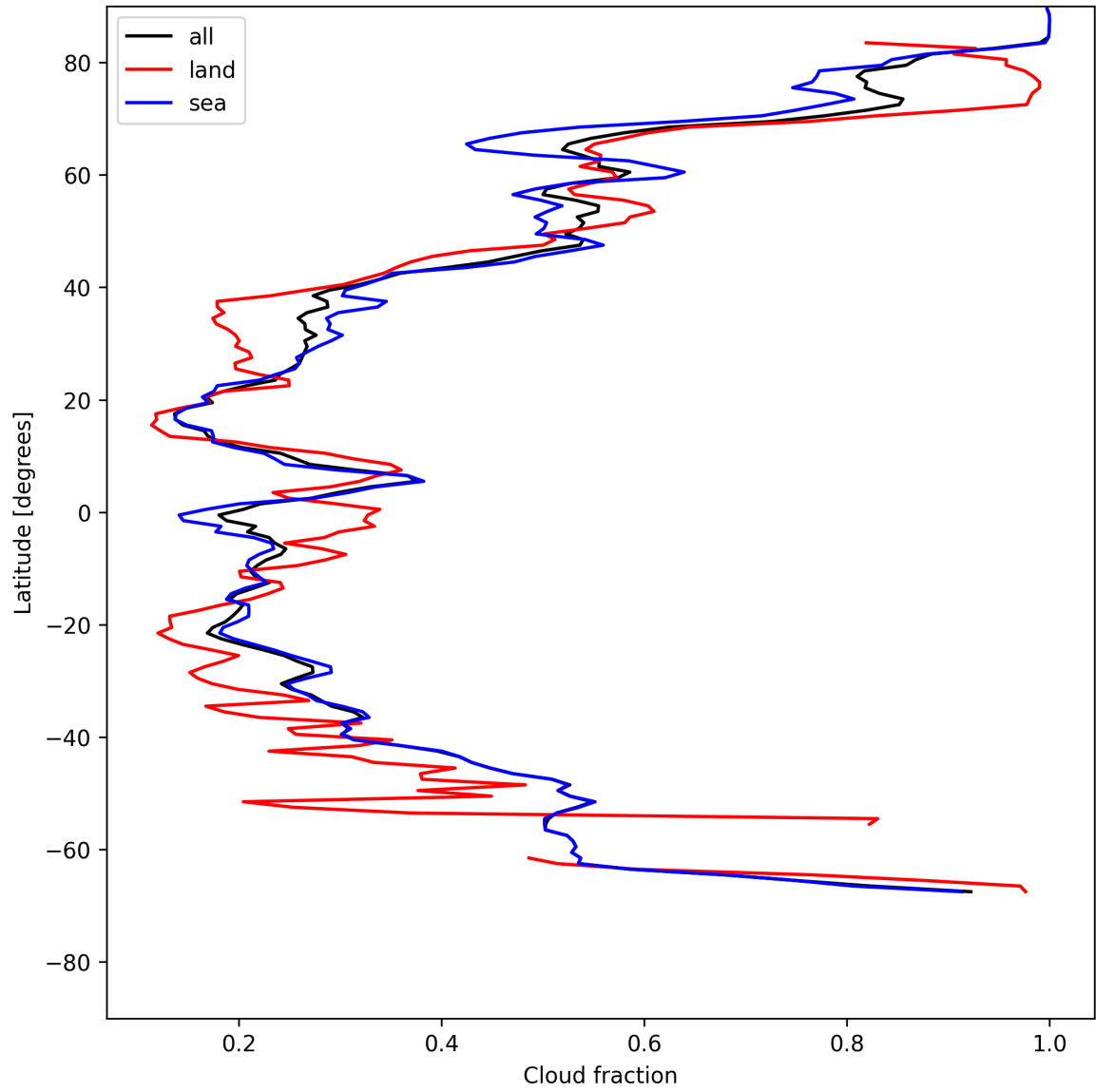
Figure 15: Zonal average of “Cloud fraction” for 2025-05-17 to 2025-05-19.
