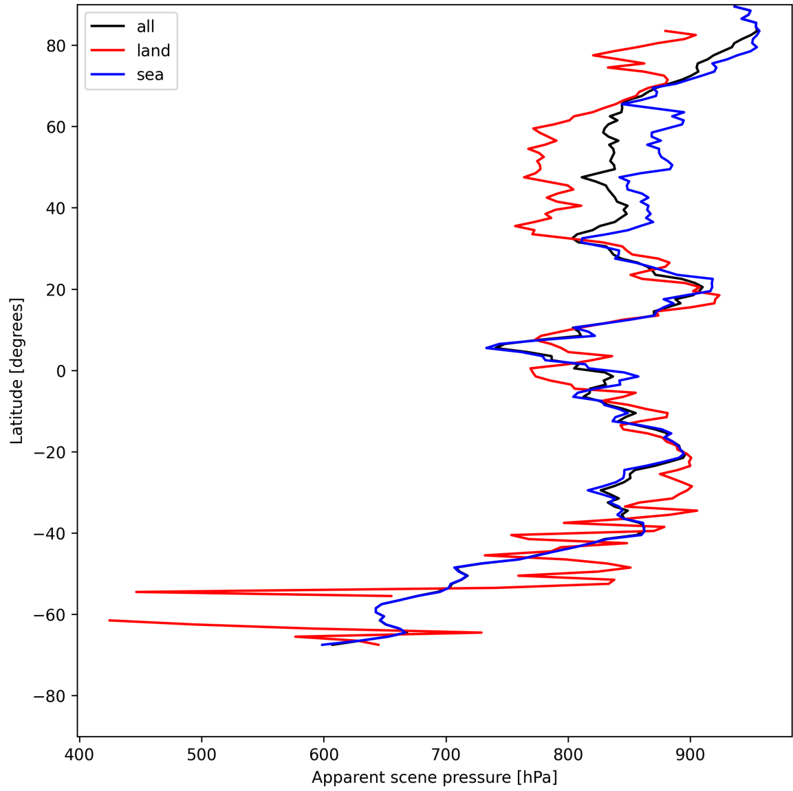
Figure 19: Zonal average of “Apparent scene pressure” for 2025-05-17 to 2025-05-19.
