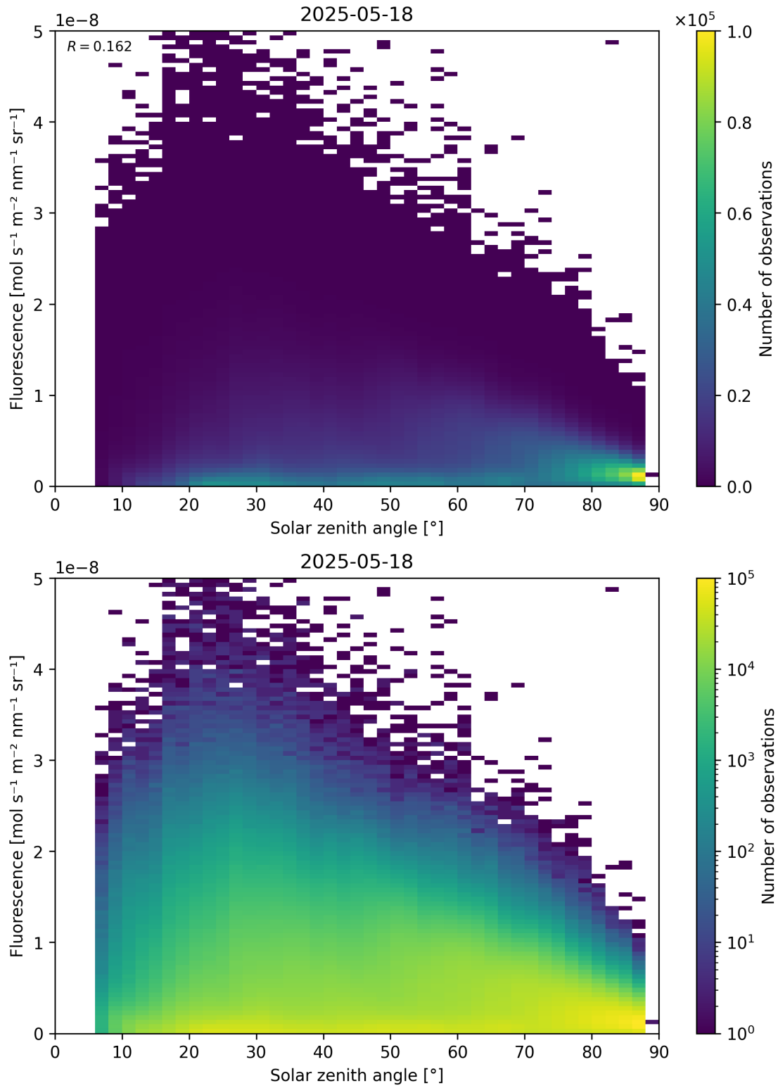
Figure 112: Scatter density plot of “Solar zenith angle” against “Fluorescence” for 2025-05-17 to 2025-05-19.
