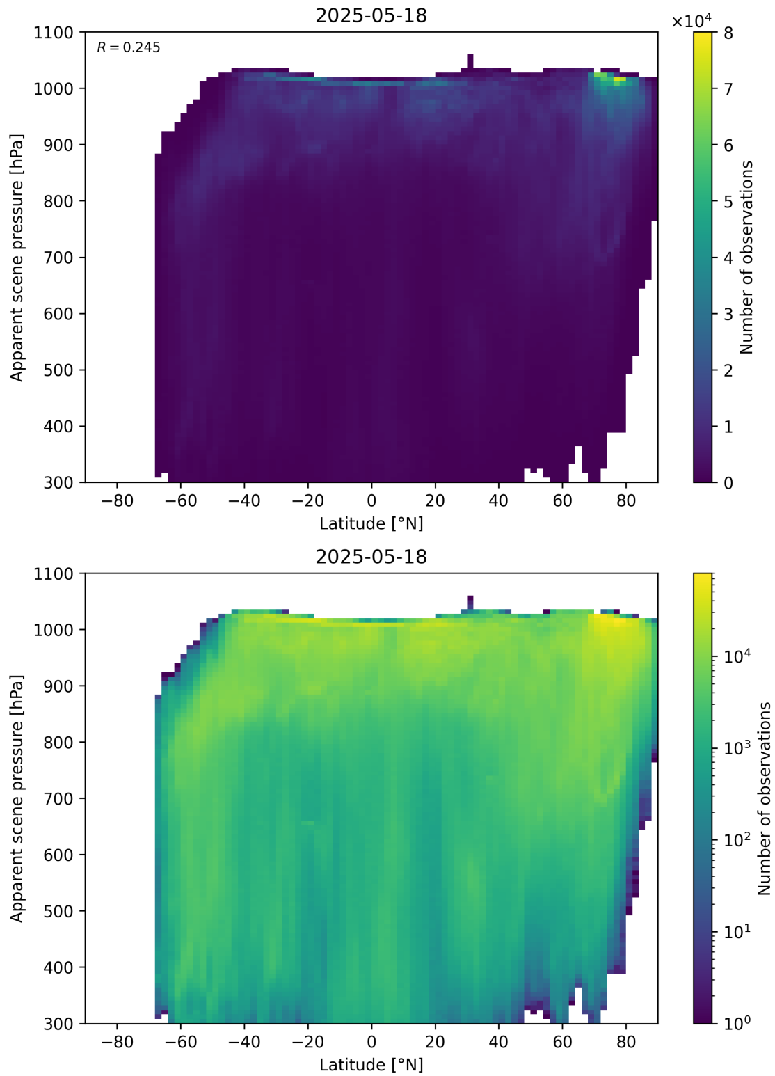
Figure 88: Scatter density plot of “Latitude” against “Apparent scene pressure” for 2025-05-17 to 2025-05-19.
