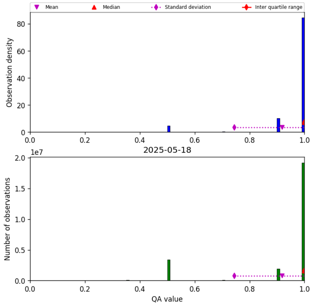
Figure 29: Histogram of “QA value” for 2025-05-17 to 2025-05-19
