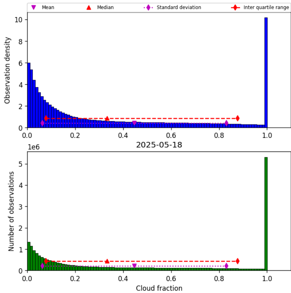
Figure 32: Histogram of “Cloud fraction” for 2025-05-17 to 2025-05-19
