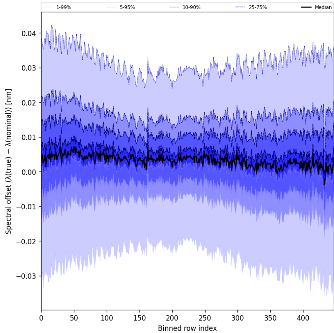
Figure 62: Along track statistics of “Spectral offset ( \lambda_{\text{true}} - \lambda_{\text{nominal}} )” for 2025-05-17 to 2025-05-19
