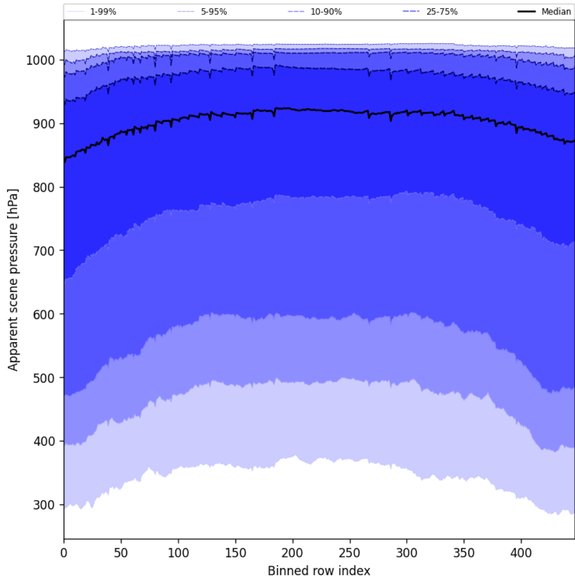
Figure 53: Along track statistics of “Apparent scene pressure” for 2025-05-17 to 2025-05-19
