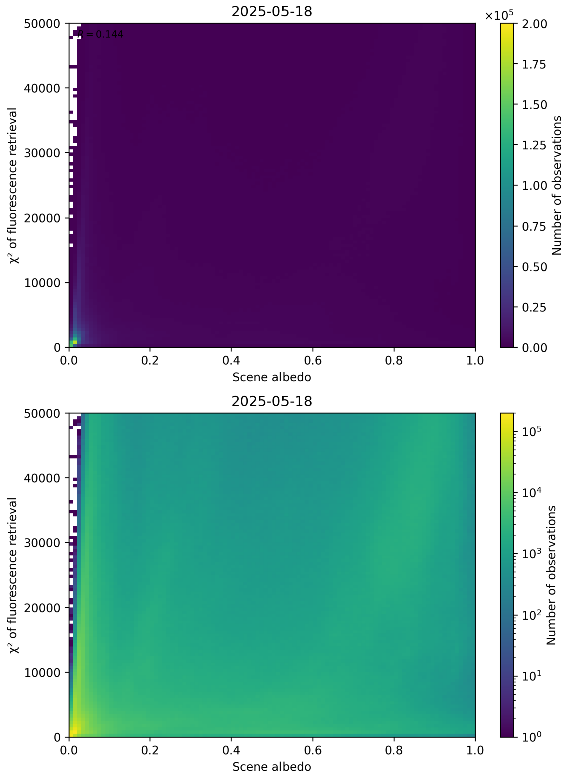
Figure 103: Scatter density plot of “Scene albedo” against “ \chi^2 of fluorescence retrieval” for 2025-05-17 to 2025-05-19.
