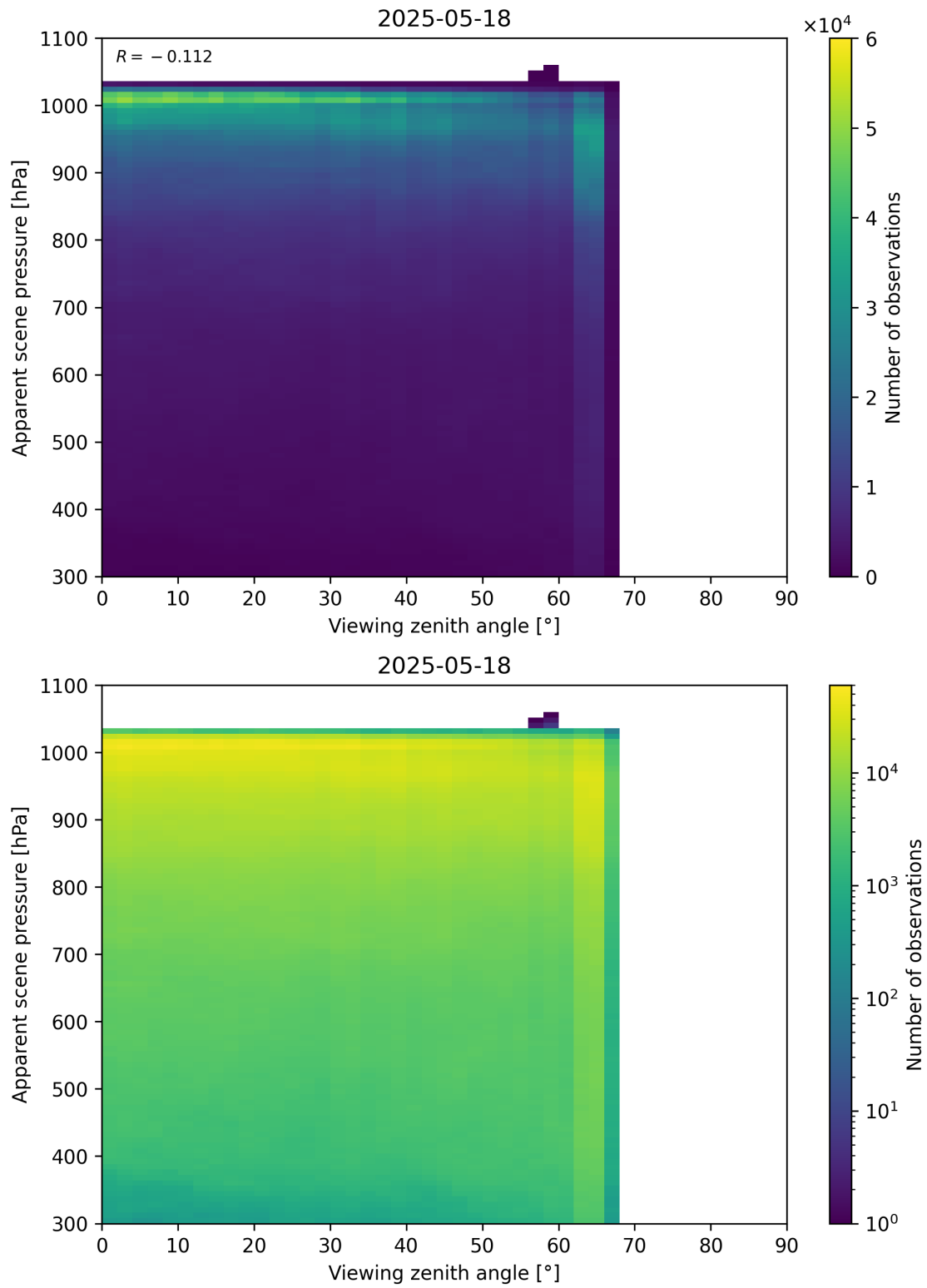
Figure 118: Scatter density plot of “Viewing zenith angle” against “Apparent scene pressure” for 2025-05-17 to 2025-05-19.
