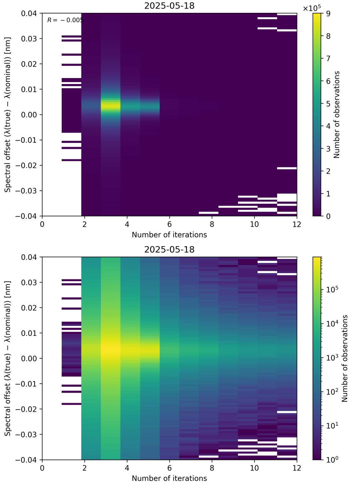
Figure 100: Scatter density plot of “Number of iterations” against “Spectral offset ( \lambda_{\text{true}} - \lambda_{\text{nominal}} )” for 2025-05-17 to 2025-05-19.
