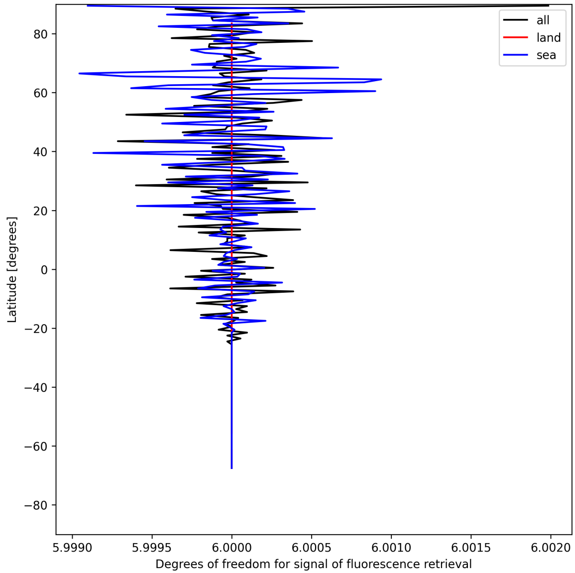
Figure 26: Zonal average of “Degrees of freedom for signal of fluorescence retrieval” for 2025-05-17 to 2025-05-19.
