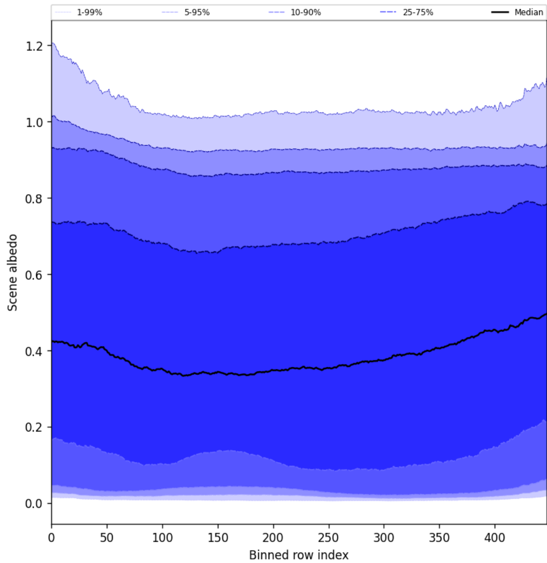
Figure 51: Along track statistics of “Scene albedo” for 2025-05-17 to 2025-05-19
