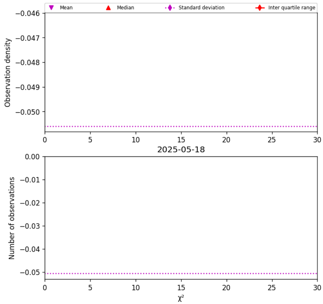
Figure 38: Histogram of " \chi^2 " for 2025-05-17 to 2025-05-19
