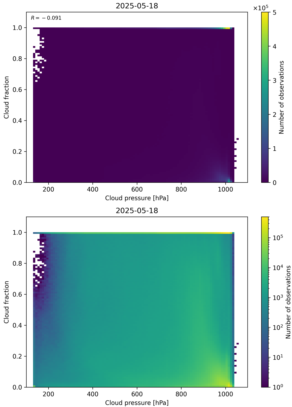
Figure 79: Scatter density plot of “Cloud pressure” against “Cloud fraction” for 2025-05-17 to 2025-05-19.
