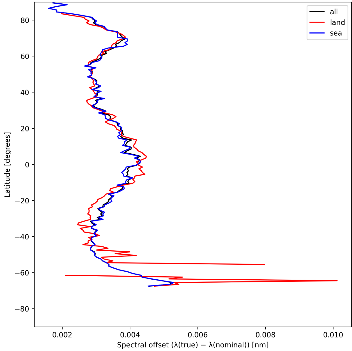
Figure 28: Zonal average of “Spectral offset ( \lambda_{\text{true}} - \lambda_{\text{nominal}} )” for 2025-05-17 to 2025-05-19.
