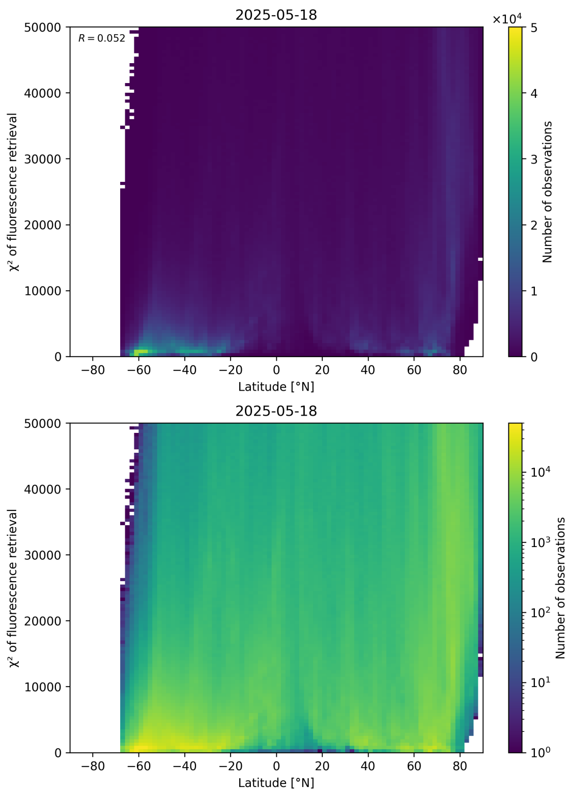
Figure 89: Scatter density plot of “Latitude” against “ \chi^2 of fluorescence retrieval” for 2025-05-17 to 2025-05-19.
