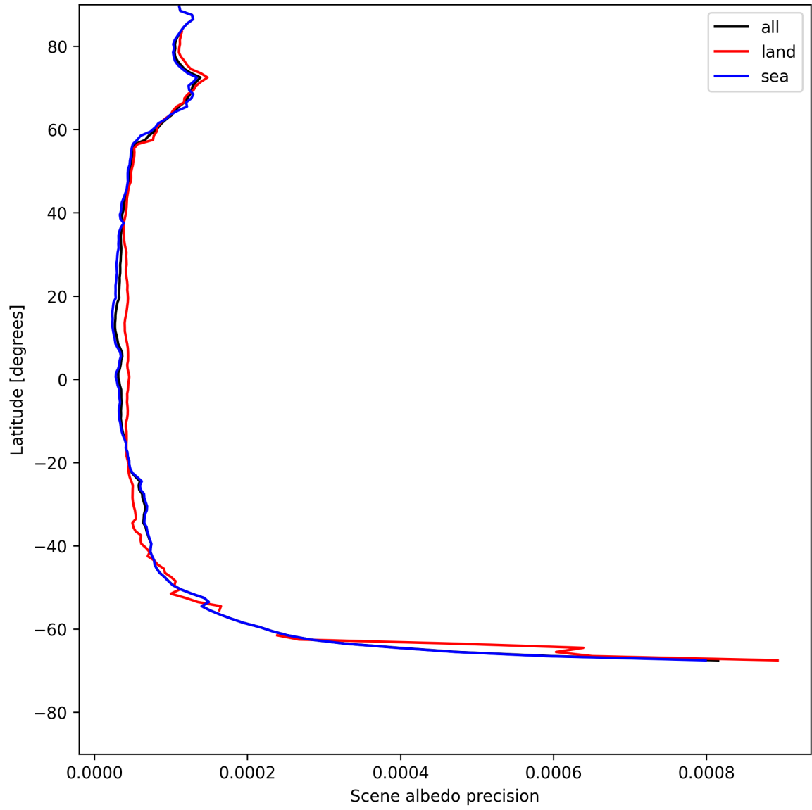
Figure 18: Zonal average of “Scene albedo precision” for 2025-05-17 to 2025-05-19.
