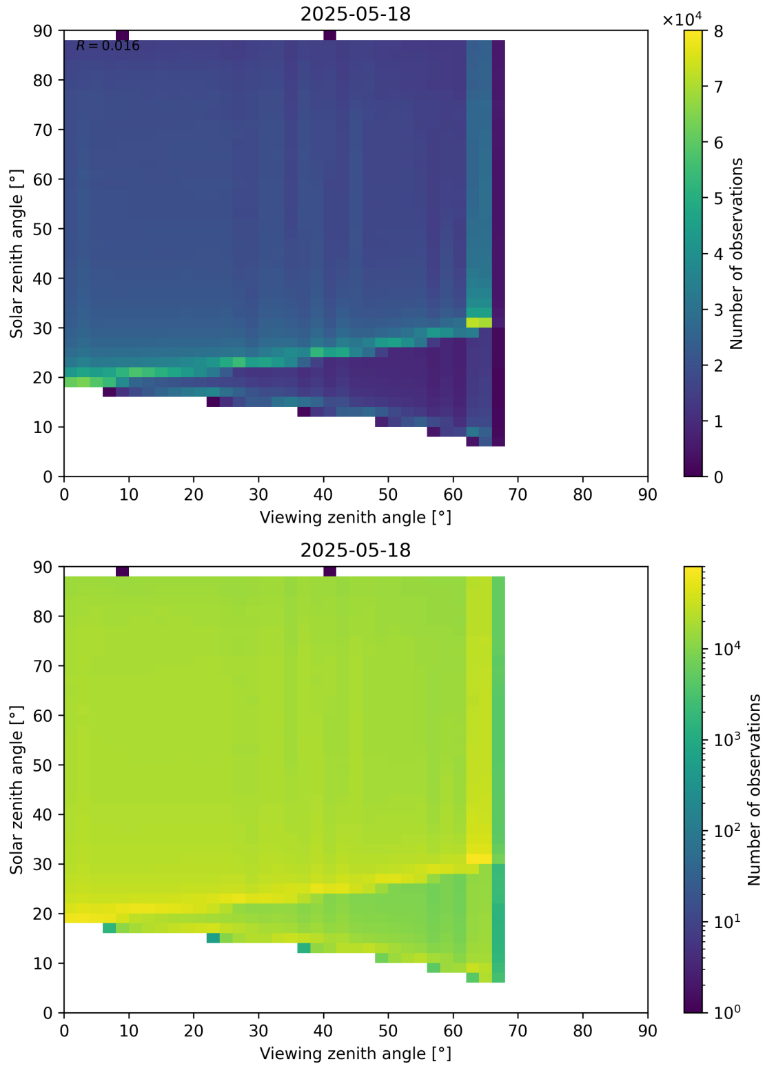
Figure 127: Scatter density plot of “Viewing zenith angle” against “Solar zenith angle” for 2025-05-17 to 2025-05-19.
