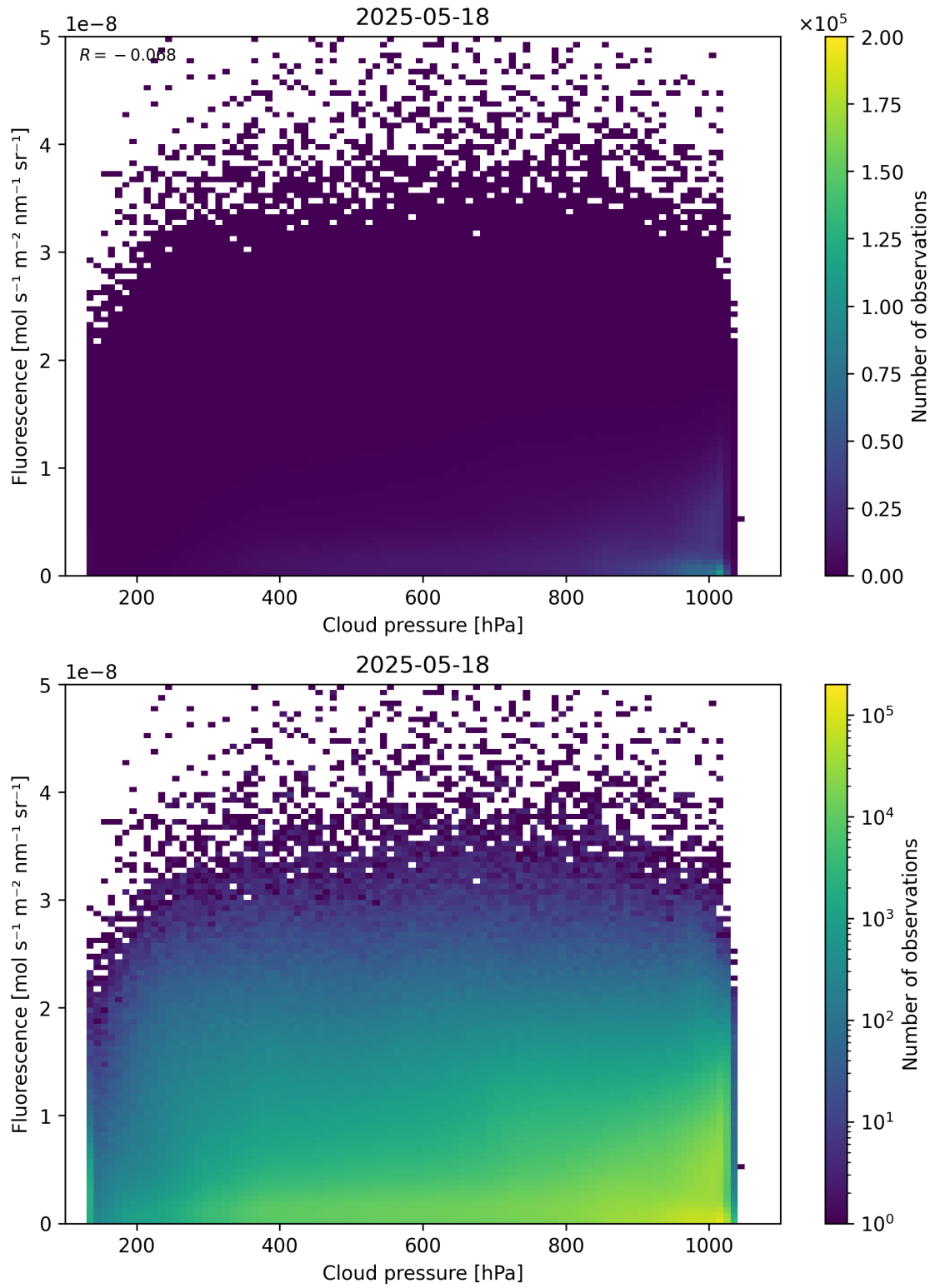
Figure 80: Scatter density plot of “Cloud pressure” against “Fluorescence” for 2025-05-17 to 2025-05-19.
