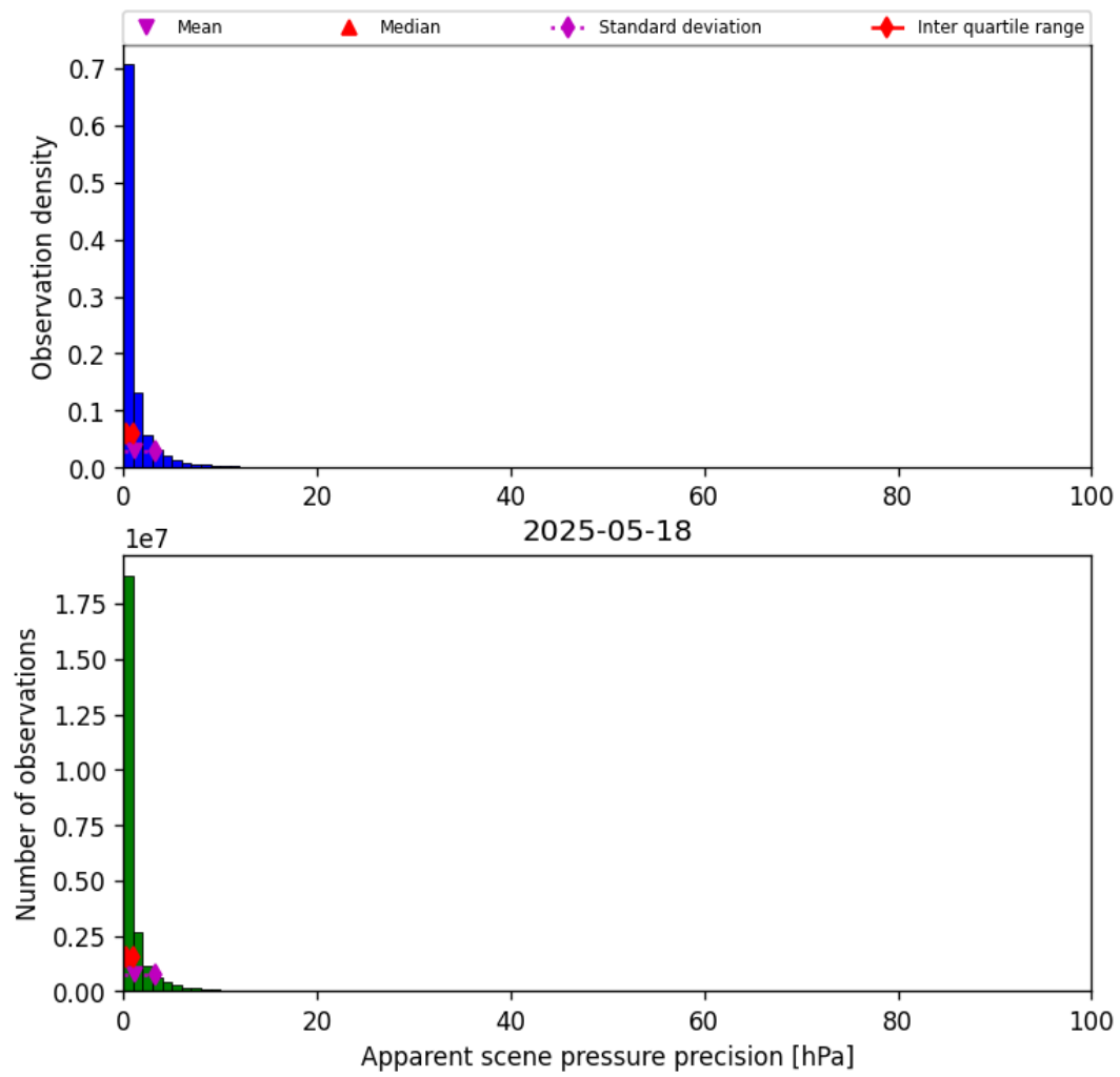
Figure 37: Histogram of “Apparent scene pressure precision” for 2025-05-17 to 2025-05-19
