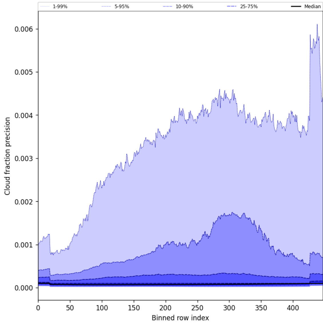
Figure 50: Along track statistics of “Cloud fraction precision” for 2025-05-17 to 2025-05-19
