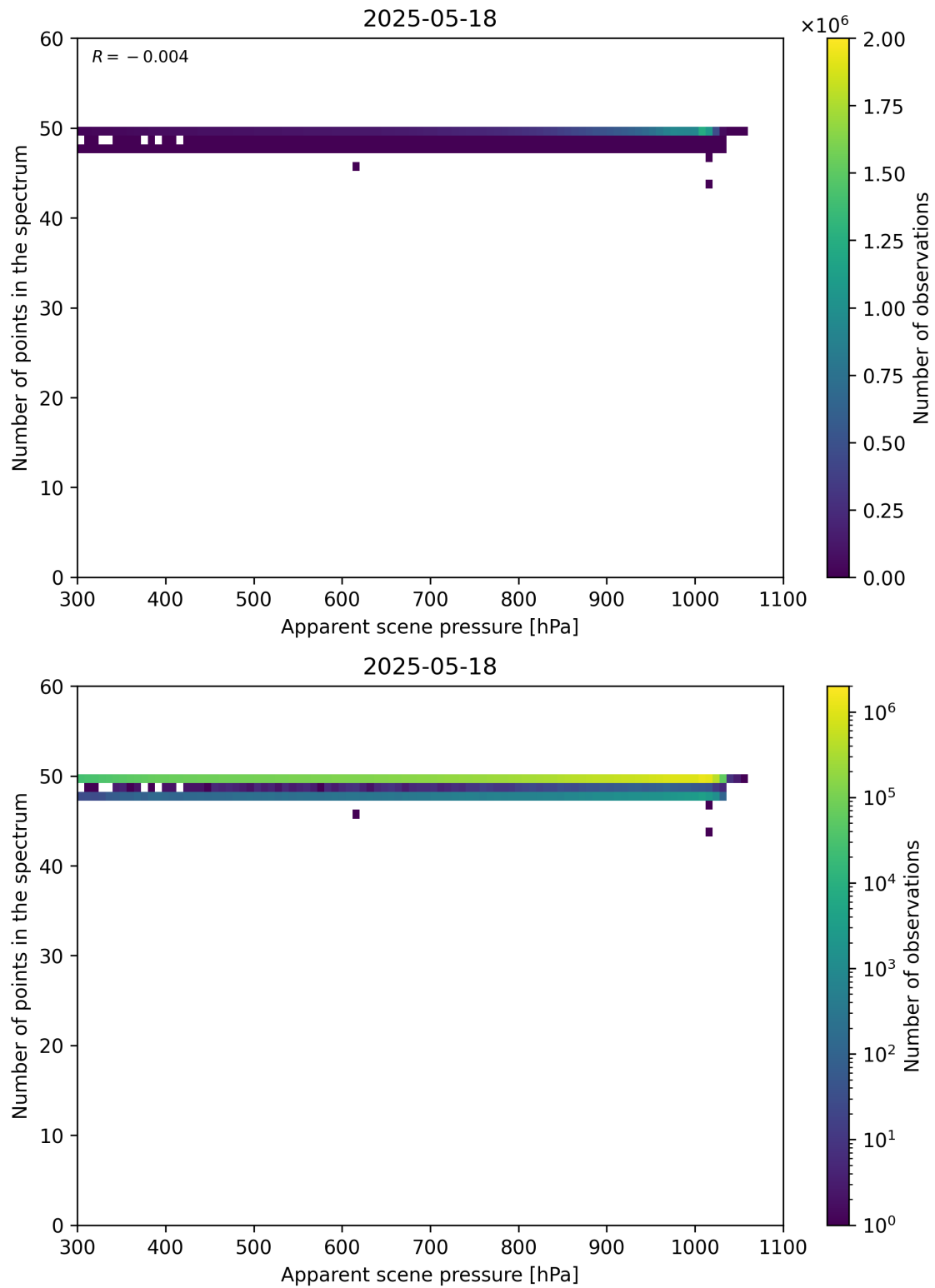
Figure 66: Scatter density plot of “Apparent scene pressure” against “Number of points in the spectrum” for 2025-05-17 to 2025-05-19.
