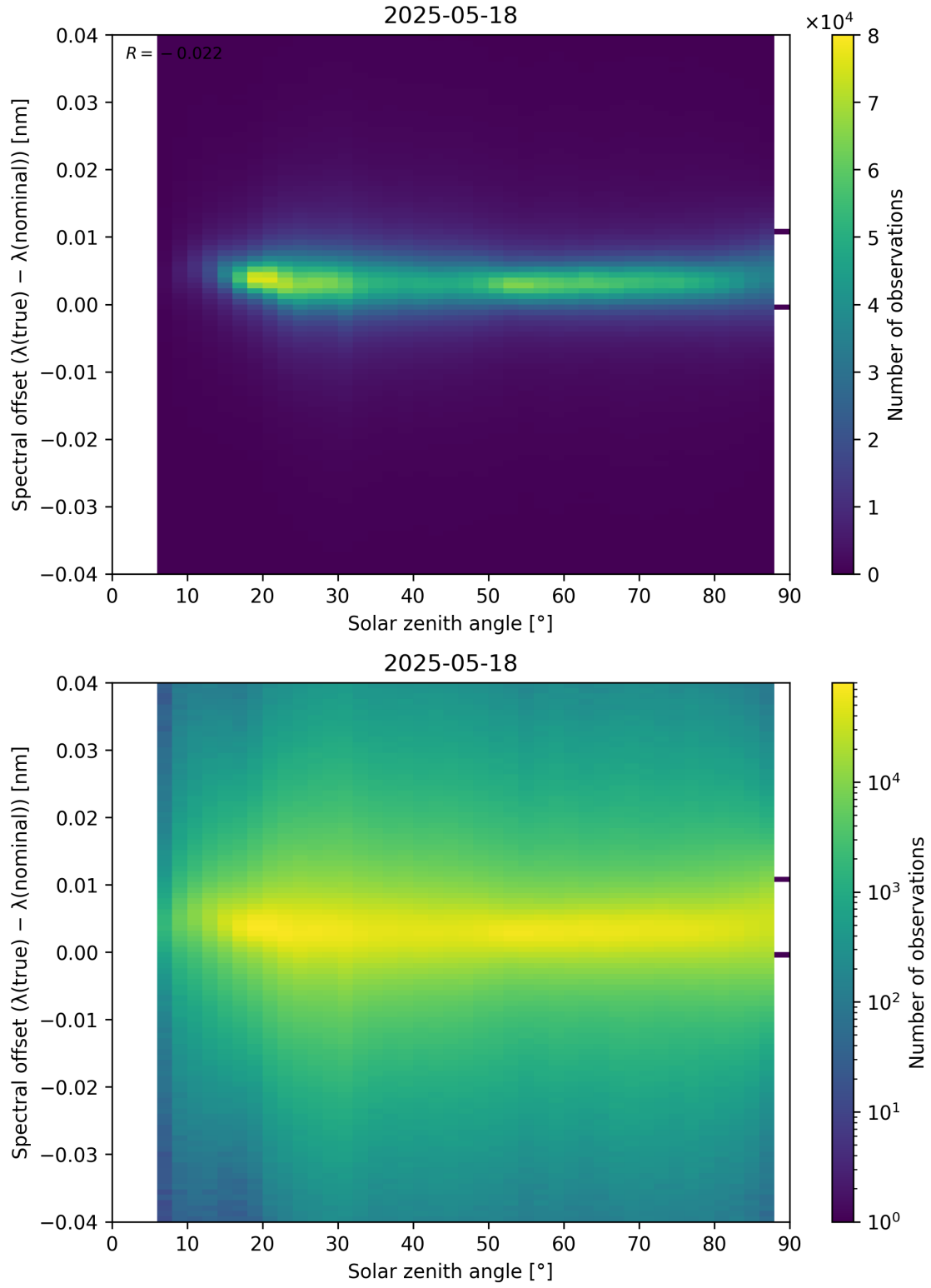
Figure 117: Scatter density plot of “Solar zenith angle” against “Spectral offset ( \lambda_{\text{true}} - \lambda_{\text{nominal}} )” for 2025-05-17 to 2025-05-19.
