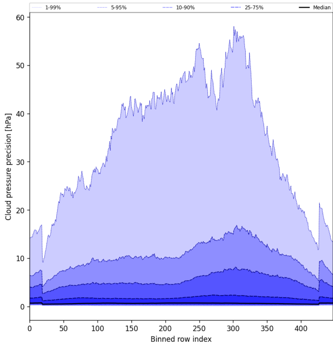
Figure 48: Along track statistics of “Cloud pressure precision” for 2025-05-17 to 2025-05-19
