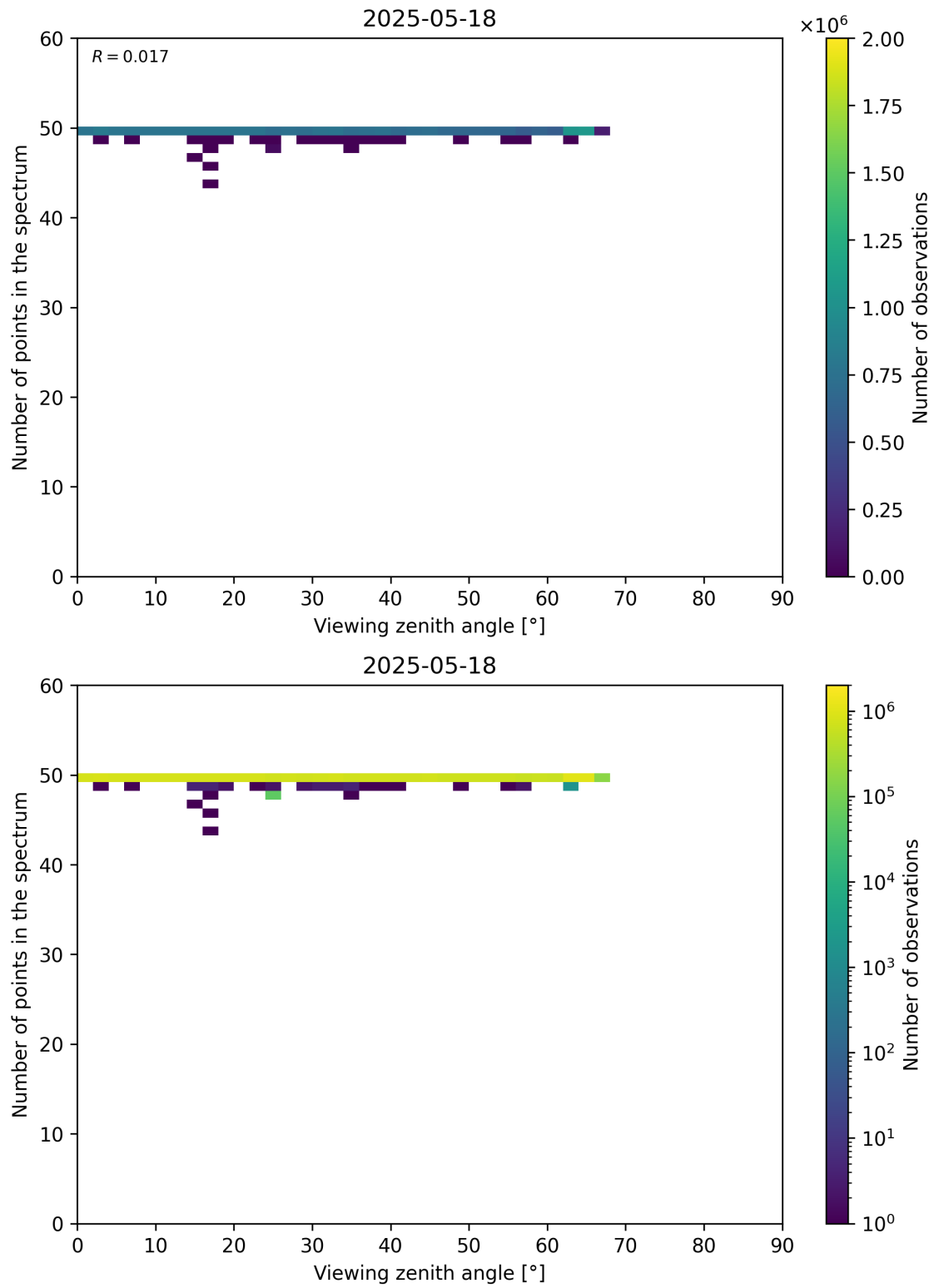
Figure 125: Scatter density plot of “Viewing zenith angle” against “Number of points in the spectrum” for 2025-05-17 to 2025-05-19.
