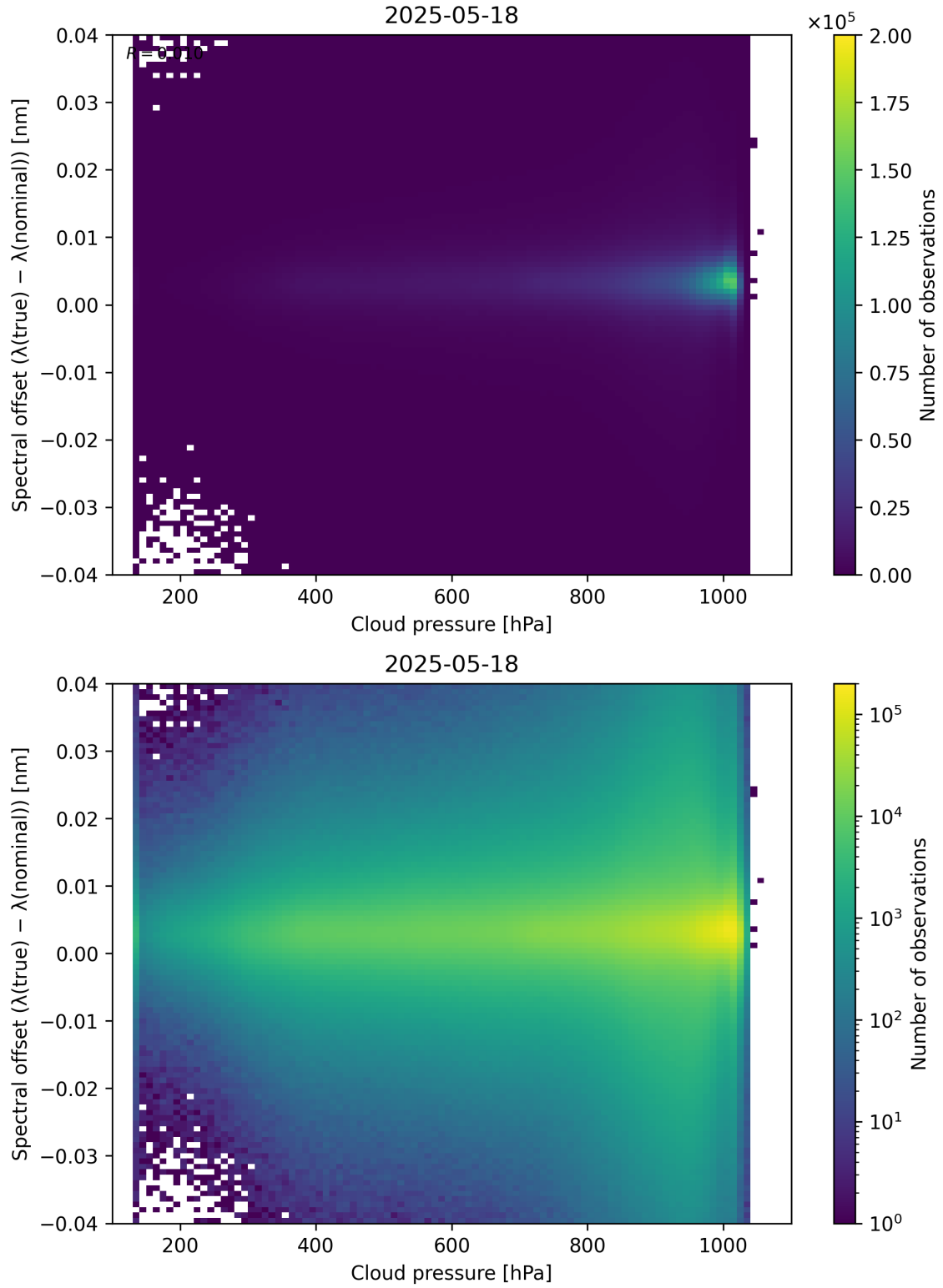
Figure 84: Scatter density plot of “Cloud pressure” against “Spectral offset ( \lambda_{\text{true}} - \lambda_{\text{nominal}} )” for 2025-05-17 to 2025-05-19.
