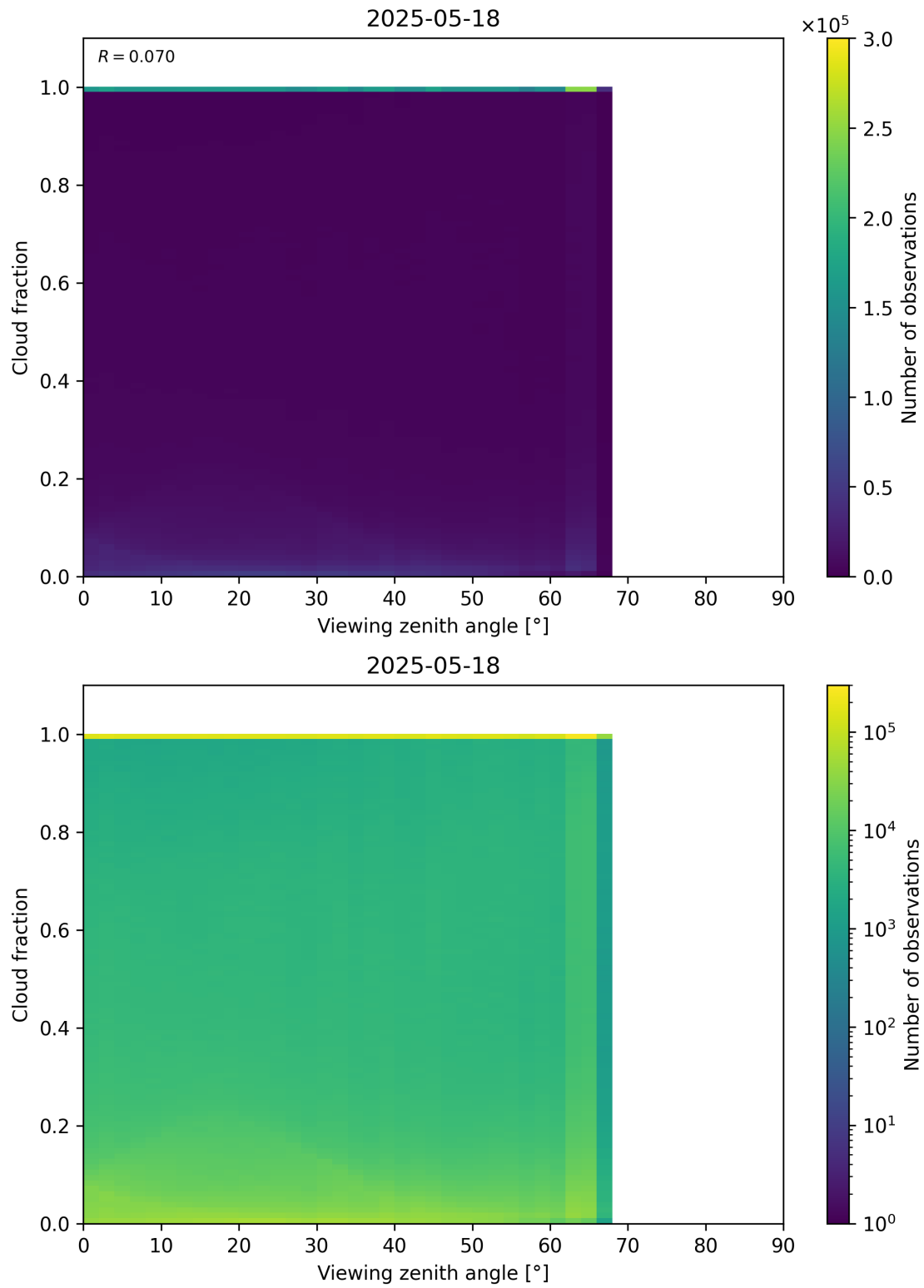
Figure 120: Scatter density plot of “Viewing zenith angle” against “Cloud fraction” for 2025-05-17 to 2025-05-19.
