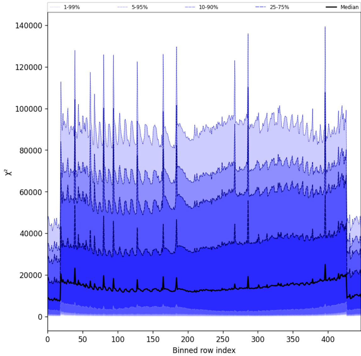
Figure 55: Along track statistics of “ \chi^2 ” for 2025-05-17 to 2025-05-19
