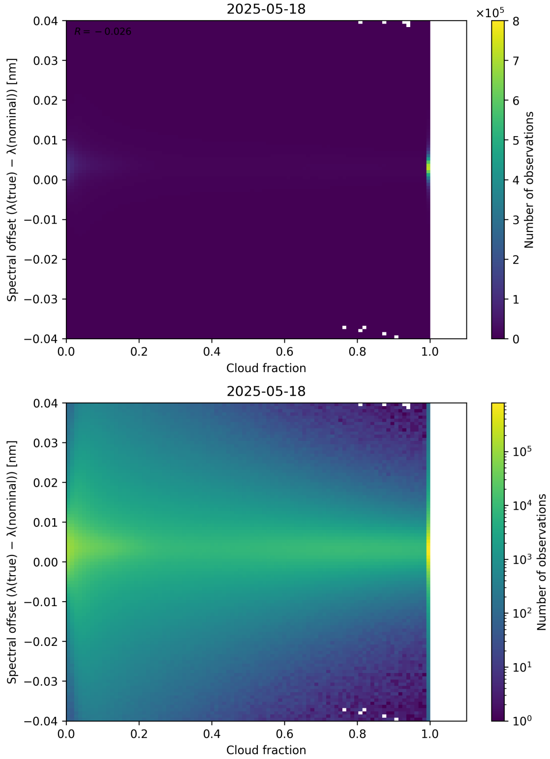
Figure 76: Scatter density plot of “Cloud fraction” against “Spectral offset ( \lambda_{\text{true}} - \lambda_{\text{nominal}} )” for 2025-05-17 to 2025-05-19.
