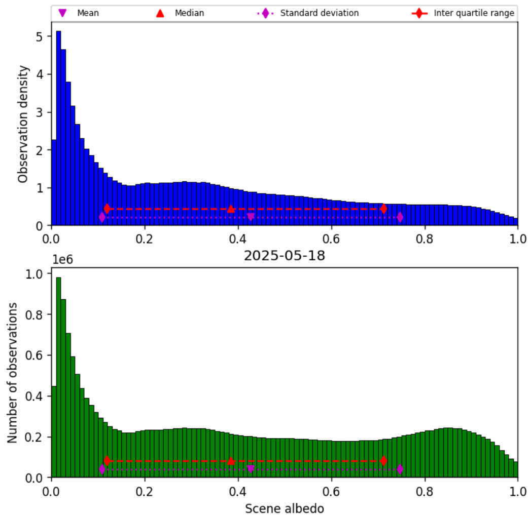
Figure 34: Histogram of “Scene albedo” for 2025-05-17 to 2025-05-19
