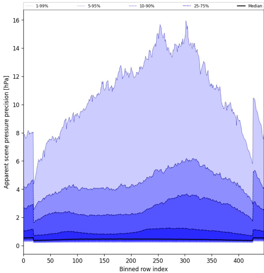
Figure 54: Along track statistics of “Apparent scene pressure precision” for 2025-05-17 to 2025-05-19
