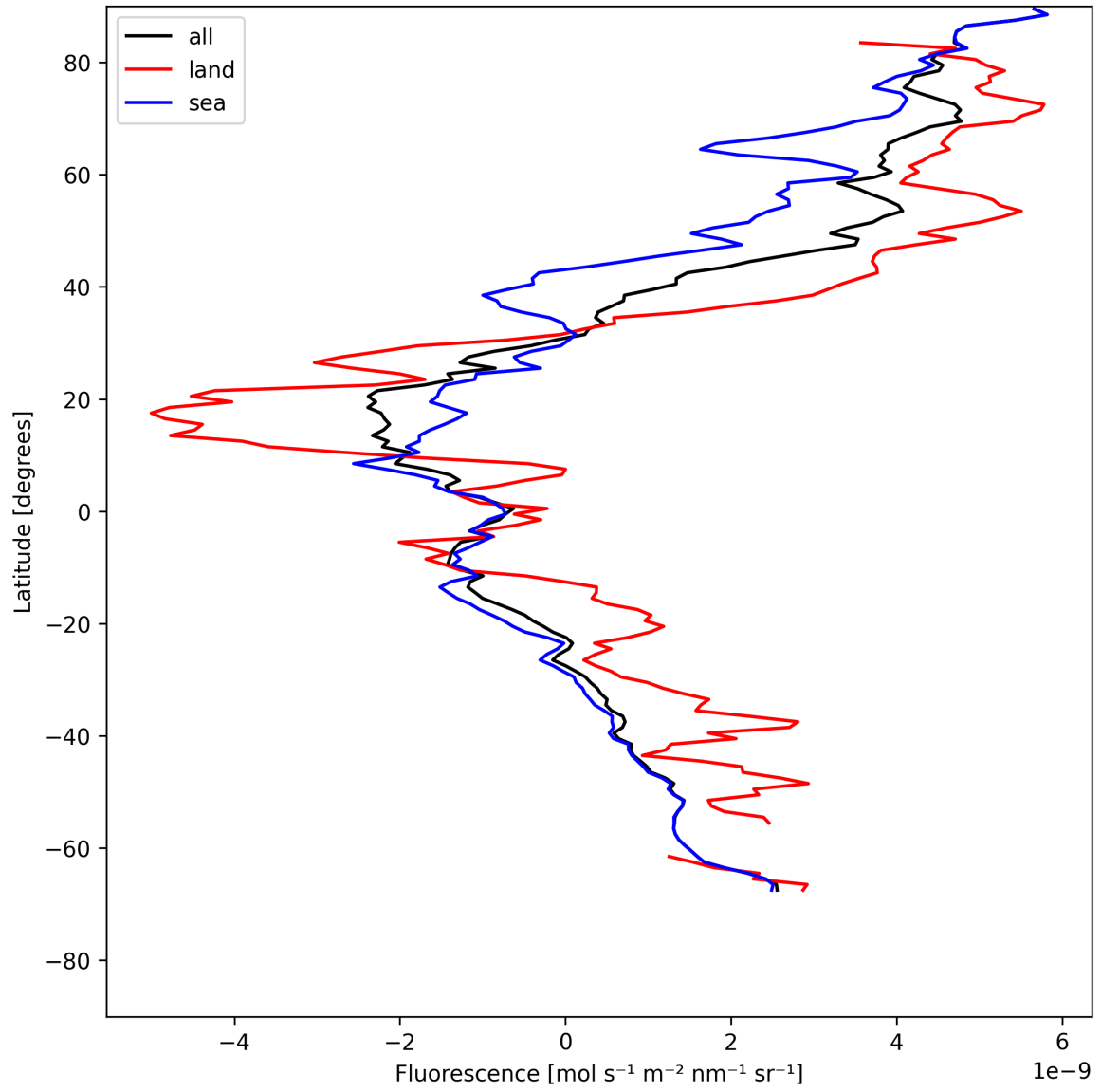
Figure 23: Zonal average of “Fluorescence” for 2025-05-17 to 2025-05-19.
