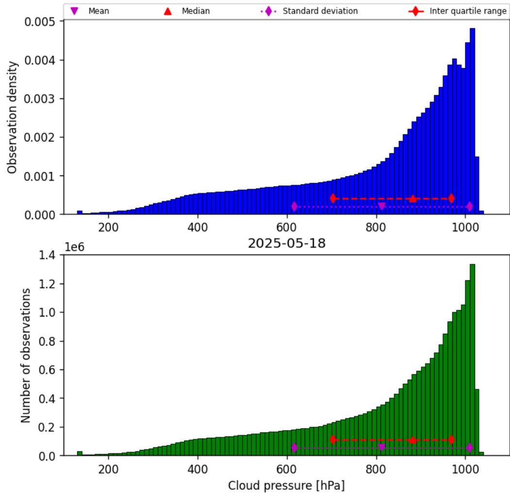
Figure 30: Histogram of “Cloud pressure” for 2025-05-17 to 2025-05-19
