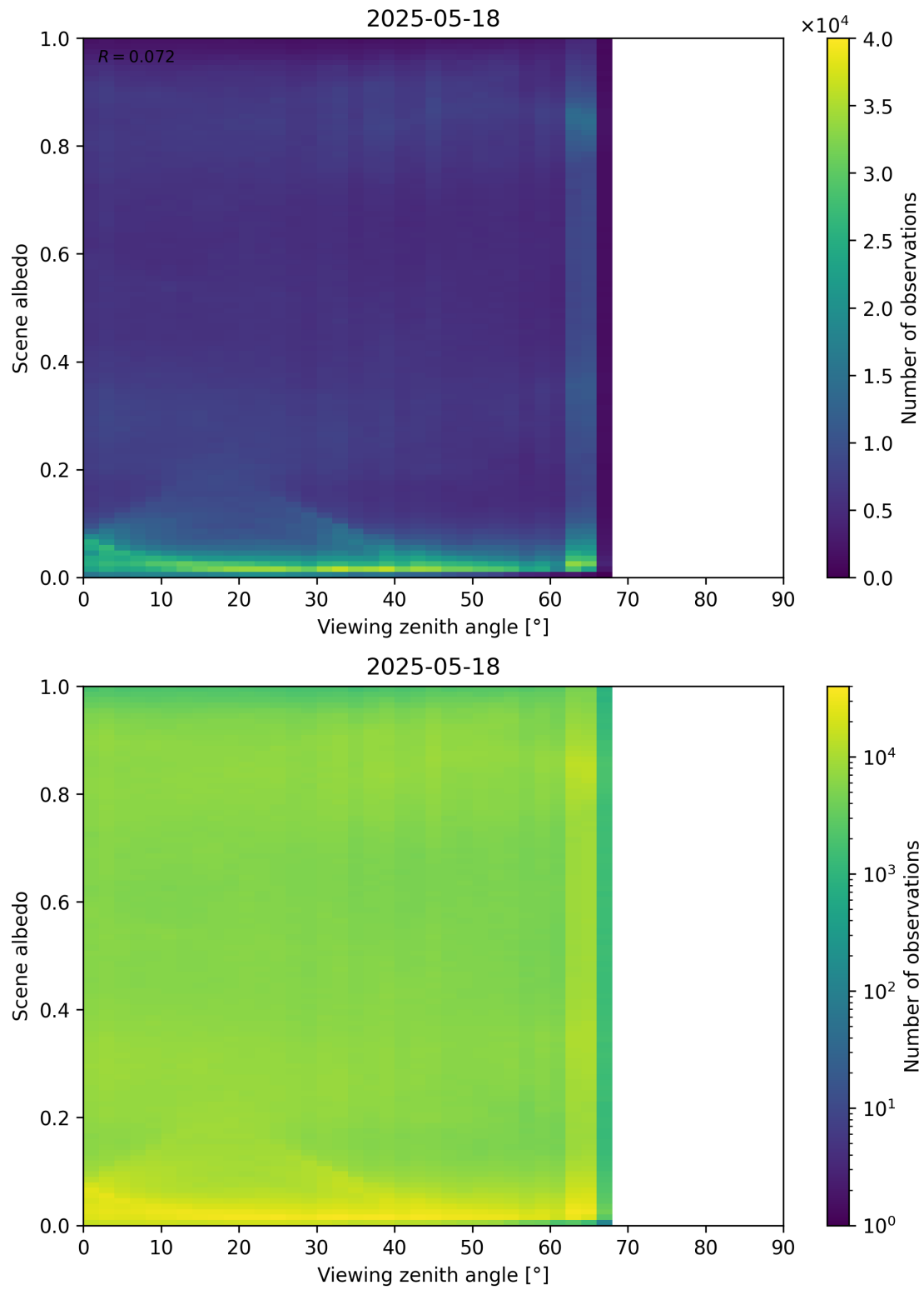
Figure 126: Scatter density plot of “Viewing zenith angle” against “Scene albedo” for 2025-05-17 to 2025-05-19.
