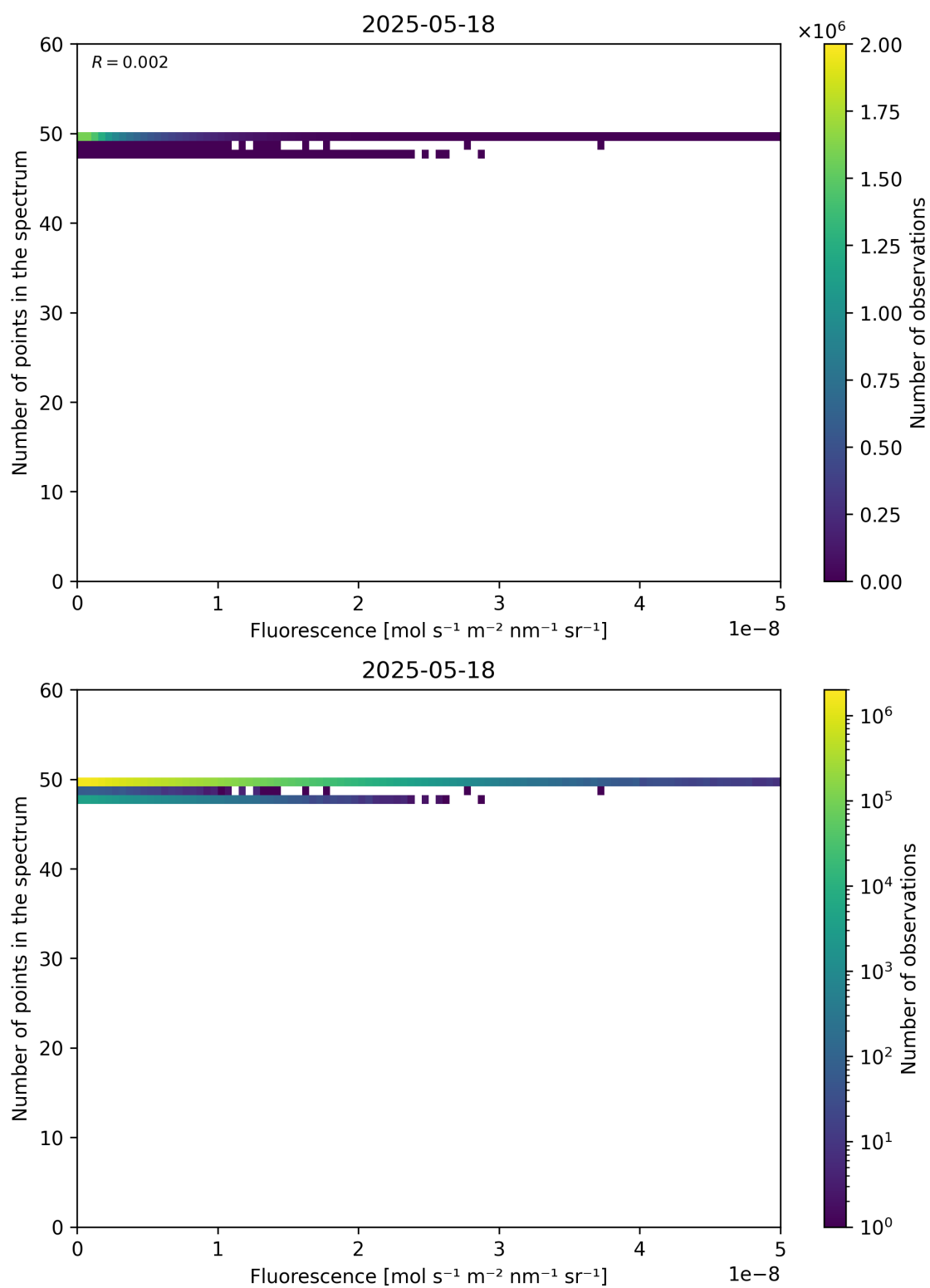
Figure 86: Scatter density plot of “Fluorescence” against “Number of points in the spectrum” for 2025-05-17 to 2025-05-19.
