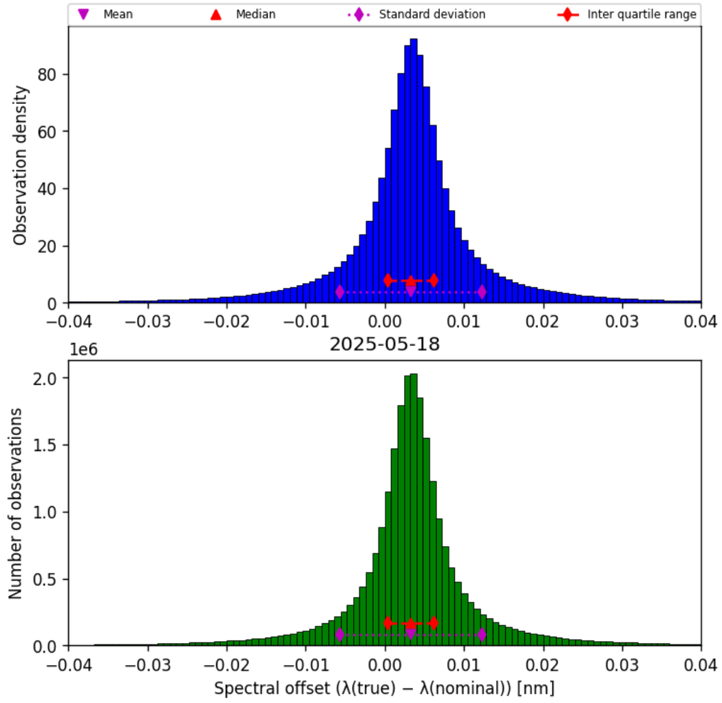
Figure 45: Histogram of “Spectral offset ( \lambda_{\text{true}} - \lambda_{\text{nominal}} )” for 2025-05-17 to 2025-05-19
