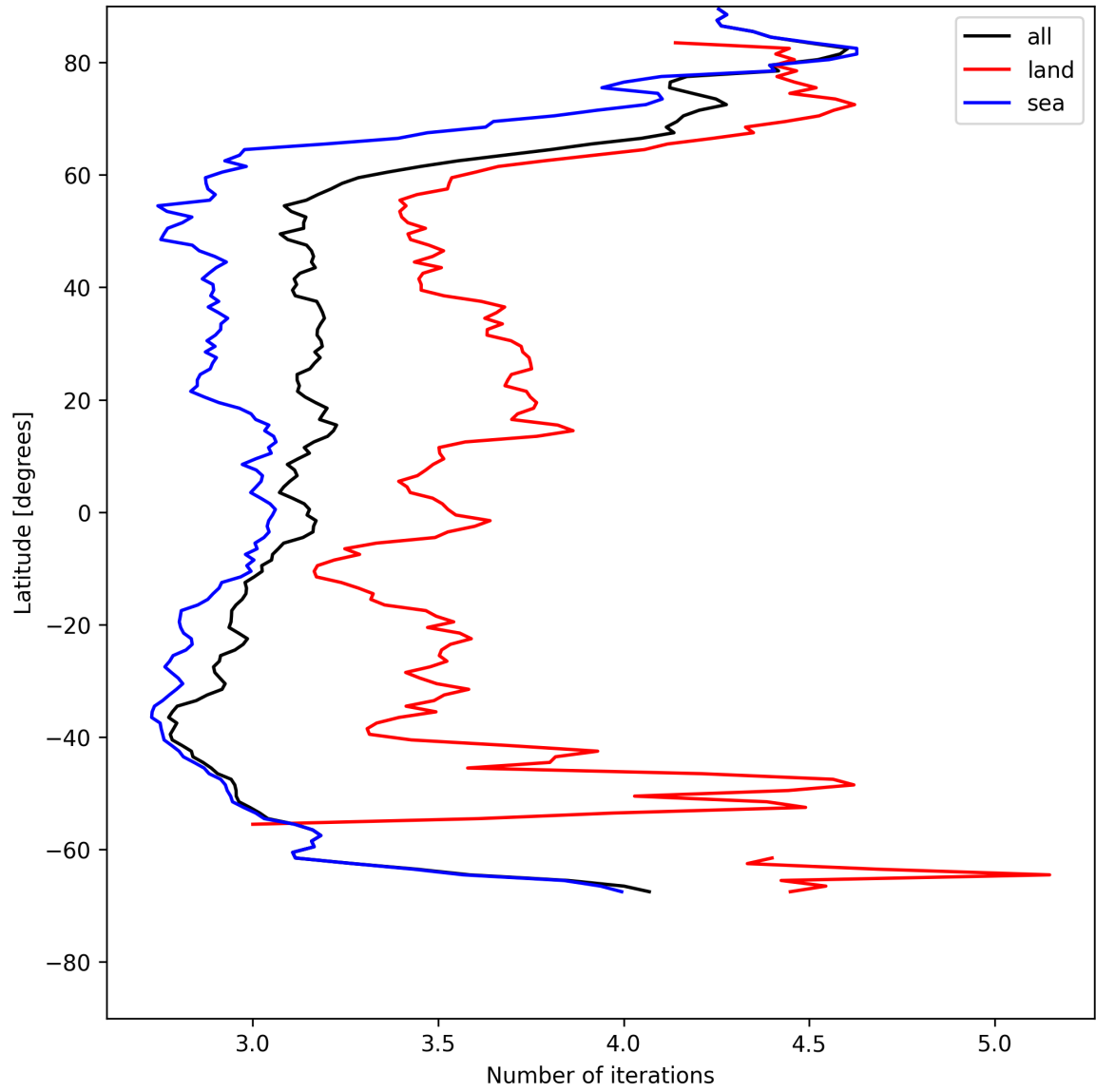
Figure 22: Zonal average of “Number of iterations” for 2025-05-17 to 2025-05-19.
