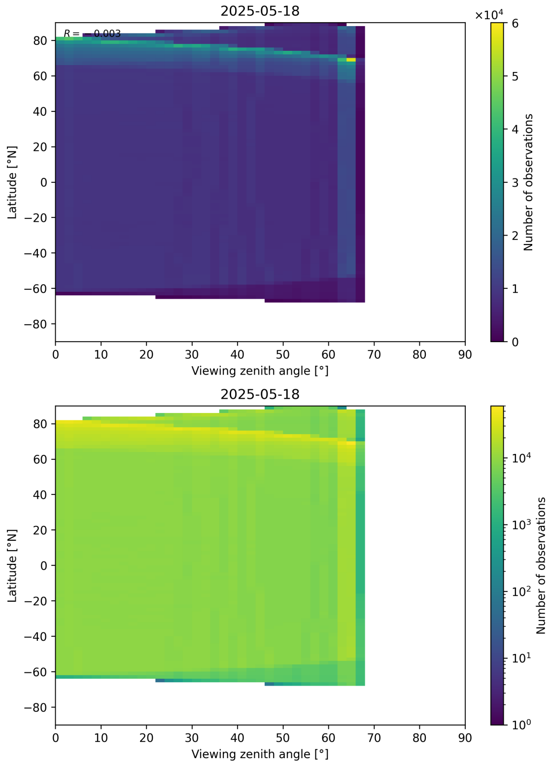
Figure 123: Scatter density plot of “Viewing zenith angle” against “Latitude” for 2025-05-17 to 2025-05-19.
