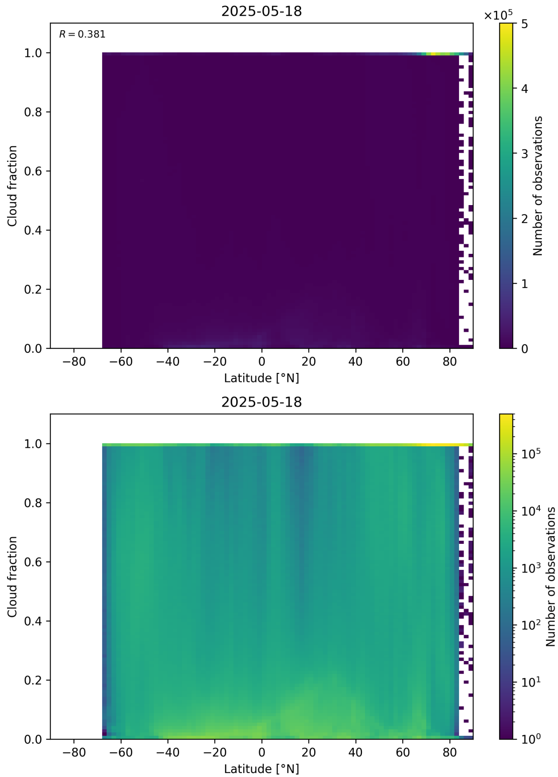
Figure 90: Scatter density plot of “Latitude” against “Cloud fraction” for 2025-05-17 to 2025-05-19.
