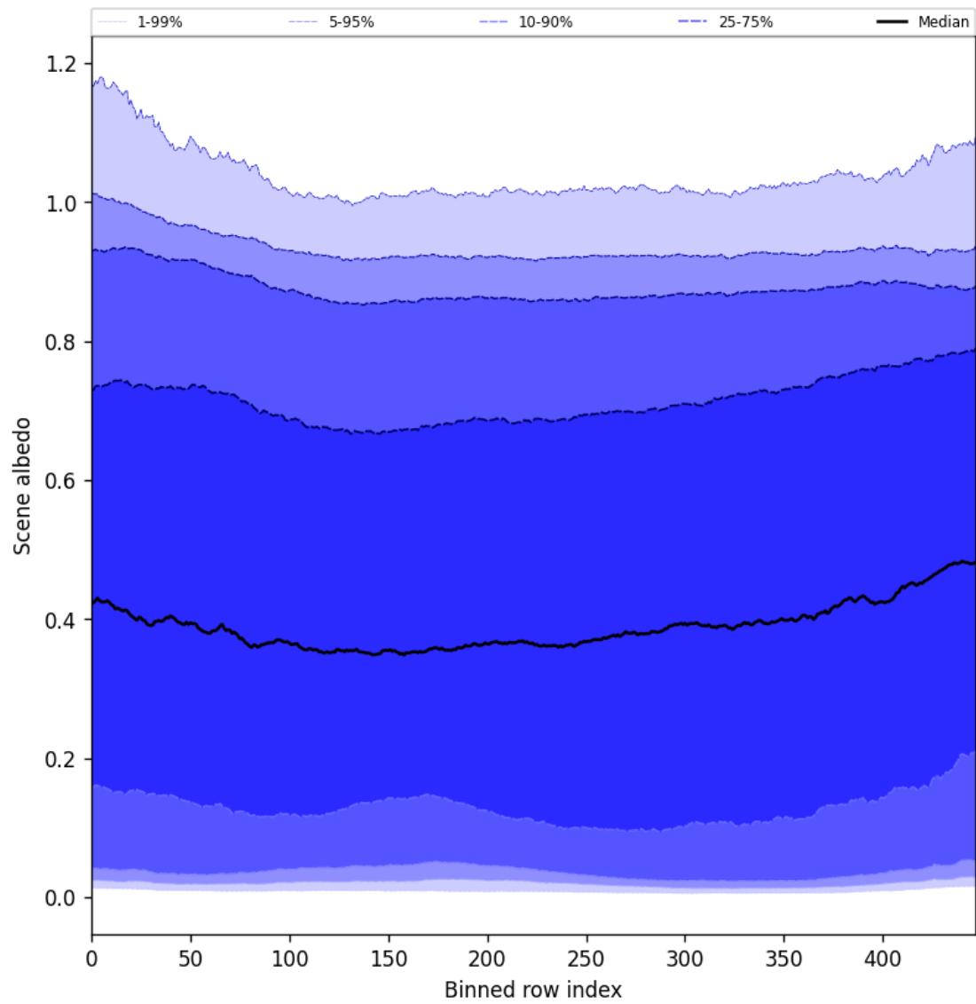
Figure 51: Along track statistics of “Scene albedo” for 2025-05-18 to 2025-05-20
