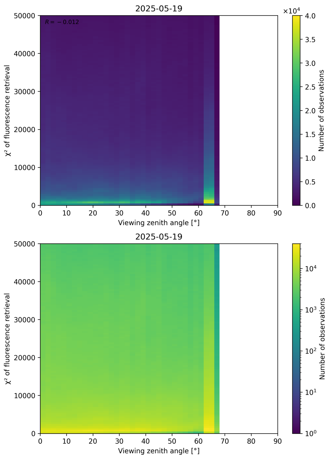
Figure 119: Scatter density plot of “Viewing zenith angle” against “ \chi^2 of fluorescence retrieval” for 2025-05-18 to 2025-05-20.
