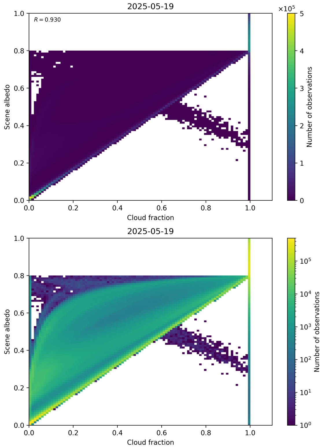
Figure 75: Scatter density plot of “Cloud fraction” against “Scene albedo” for 2025-05-18 to 2025-05-20.
