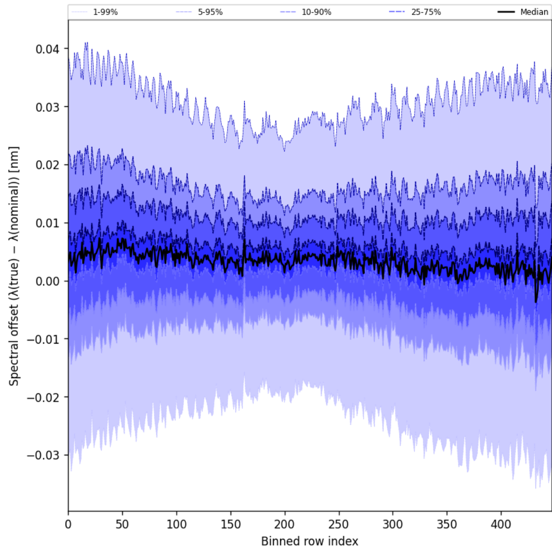
Figure 62: Along track statistics of “Spectral offset ( \lambda_{\text{true}} - \lambda_{\text{nominal}} )” for 2025-05-18 to 2025-05-20
