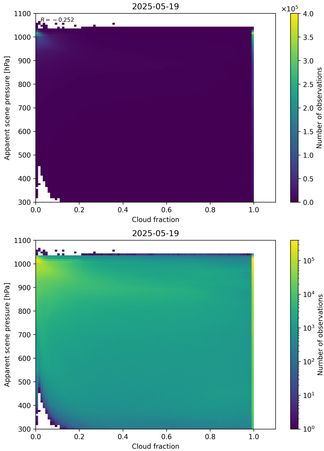
Figure 70: Scatter density plot of “Cloud fraction” against “Apparent scene pressure” for 2025-05-18 to 2025-05-20.
