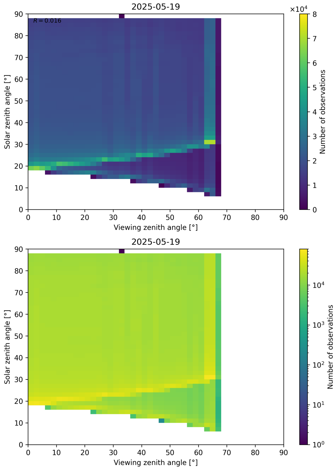
Figure 127: Scatter density plot of “Viewing zenith angle” against “Solar zenith angle” for 2025-05-18 to 2025-05-20.
