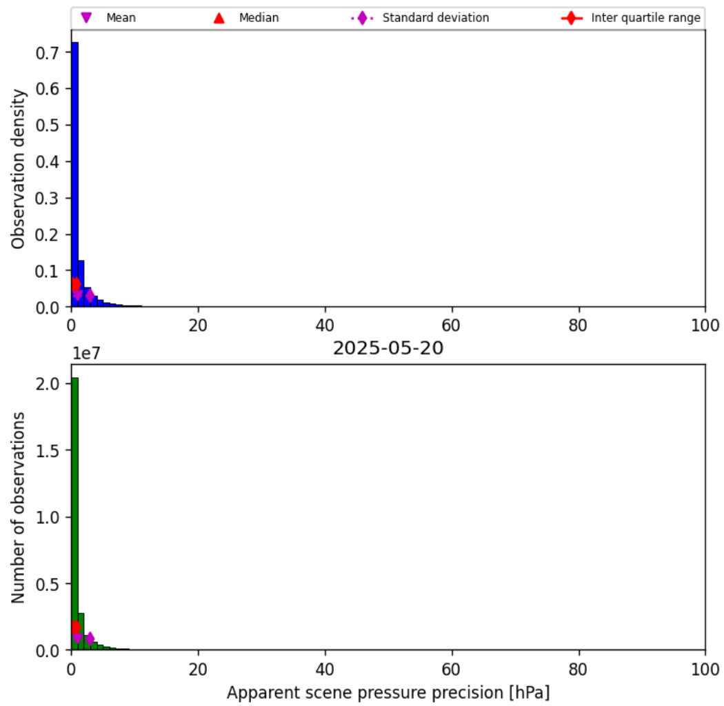
Figure 37: Histogram of “Apparent scene pressure precision” for 2025-05-19 to 2025-05-21
