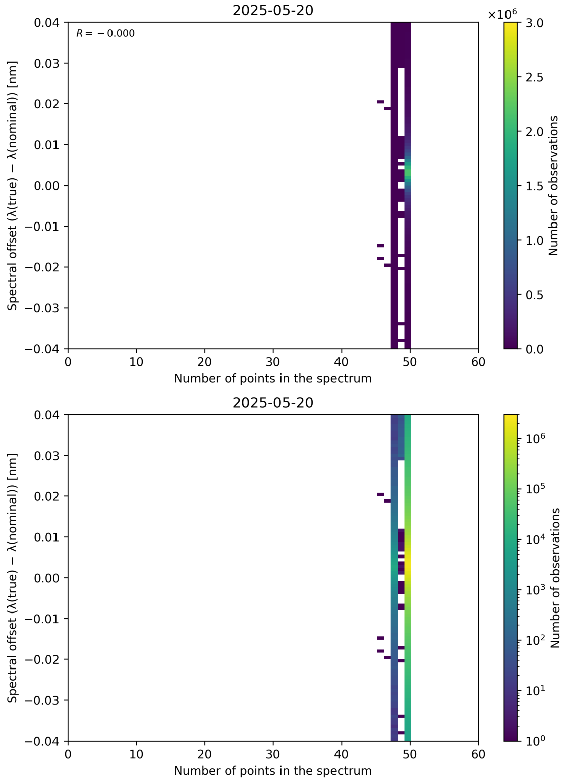
Figure 101: Scatter density plot of “Number of points in the spectrum” against “Spectral offset ( \lambda_{\text{true}} - \lambda_{\text{nominal}} )” for 2025-05-19 to 2025-05-21.
