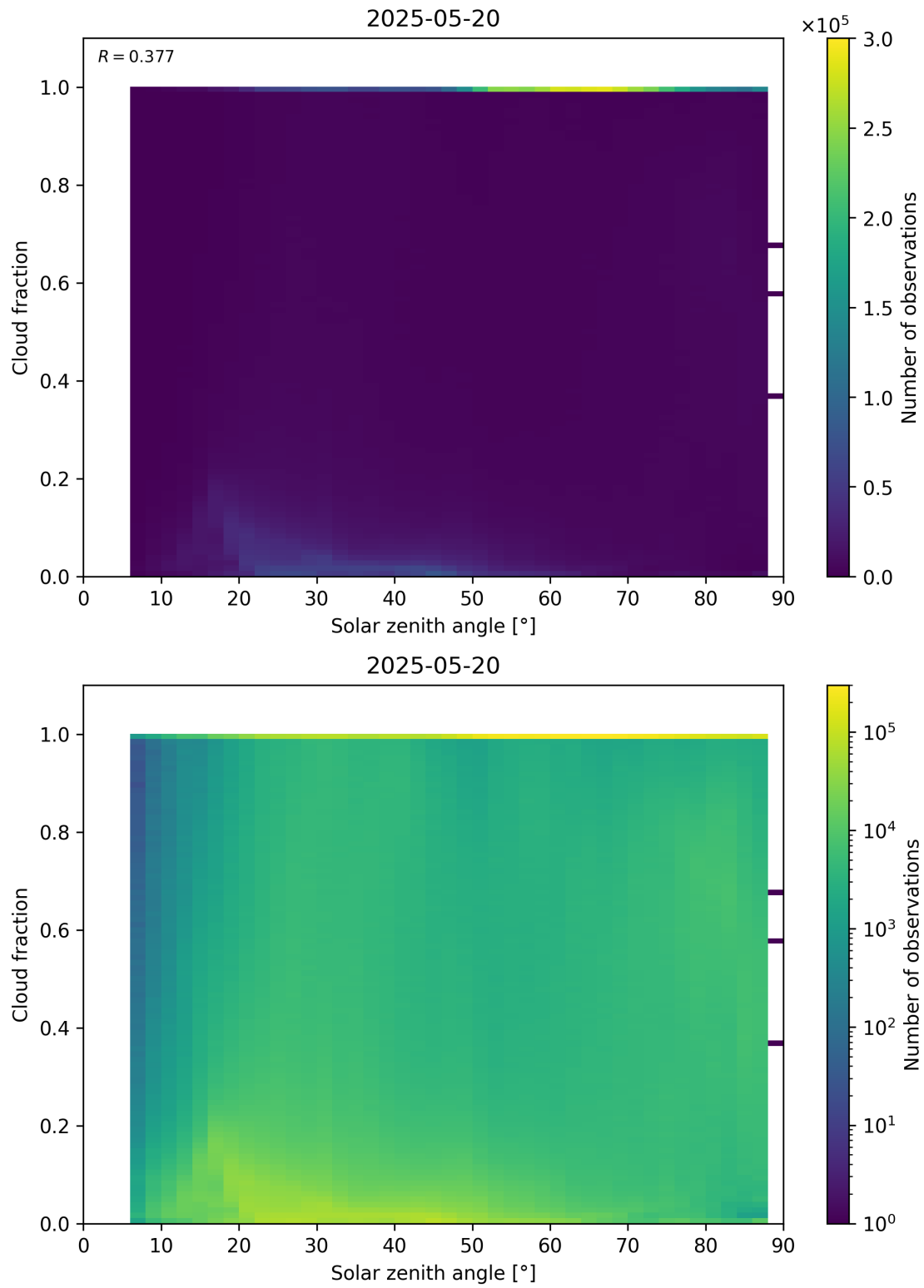
Figure 110: Scatter density plot of “Solar zenith angle” against “Cloud fraction” for 2025-05-19 to 2025-05-21.
