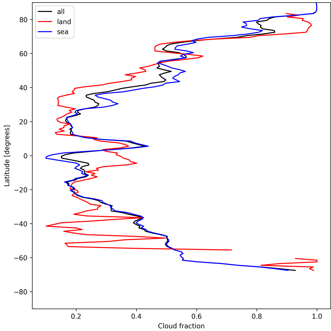
Figure 15: Zonal average of “Cloud fraction” for 2025-05-19 to 2025-05-21.
