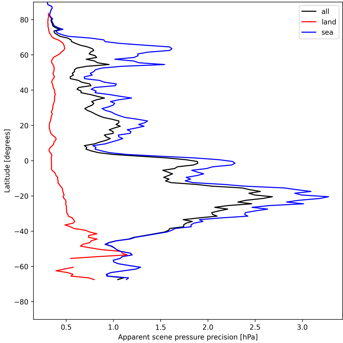
Figure 20: Zonal average of “Apparent scene pressure precision” for 2025-05-19 to 2025-05-21.
