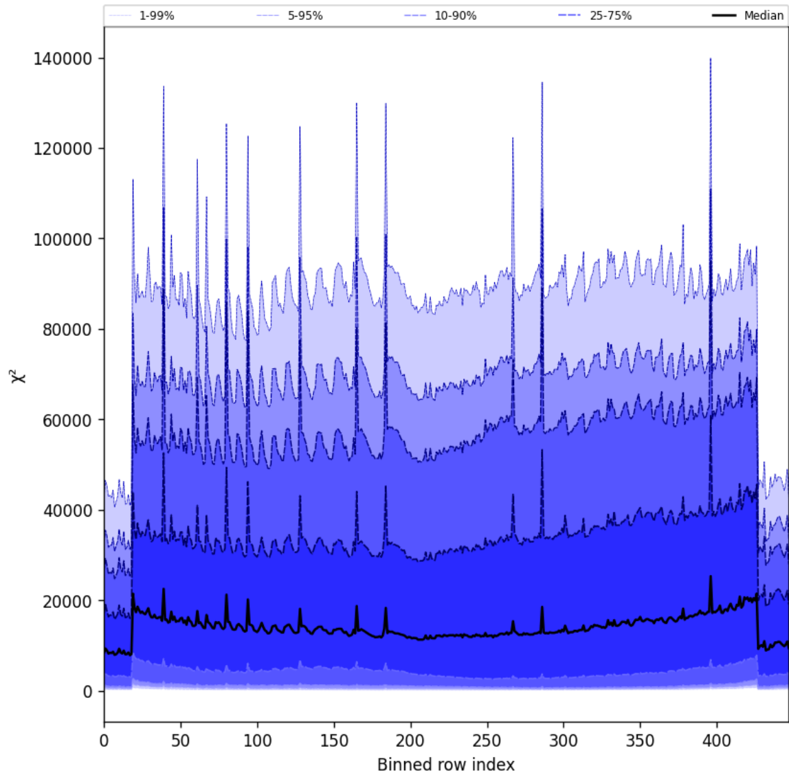
Figure 55: Along track statistics of “ \chi^2 ” for 2025-05-19 to 2025-05-21
