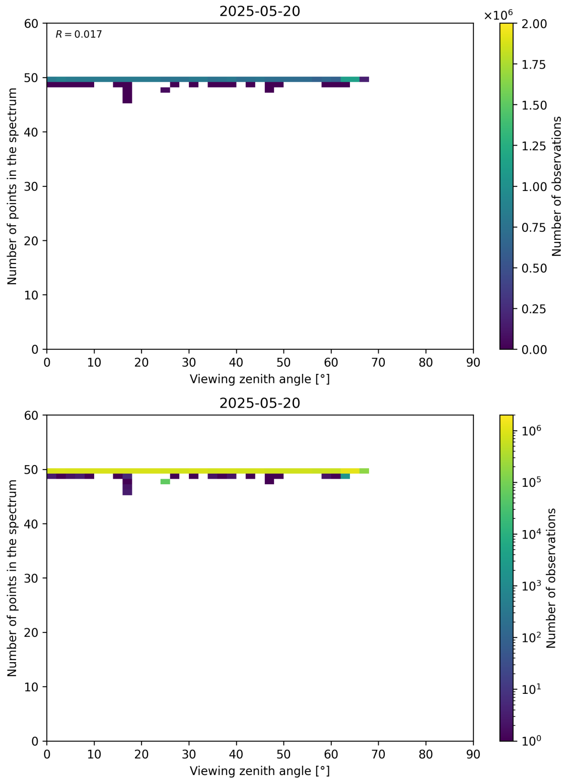
Figure 125: Scatter density plot of “Viewing zenith angle” against “Number of points in the spectrum” for 2025-05-19 to 2025-05-21.
