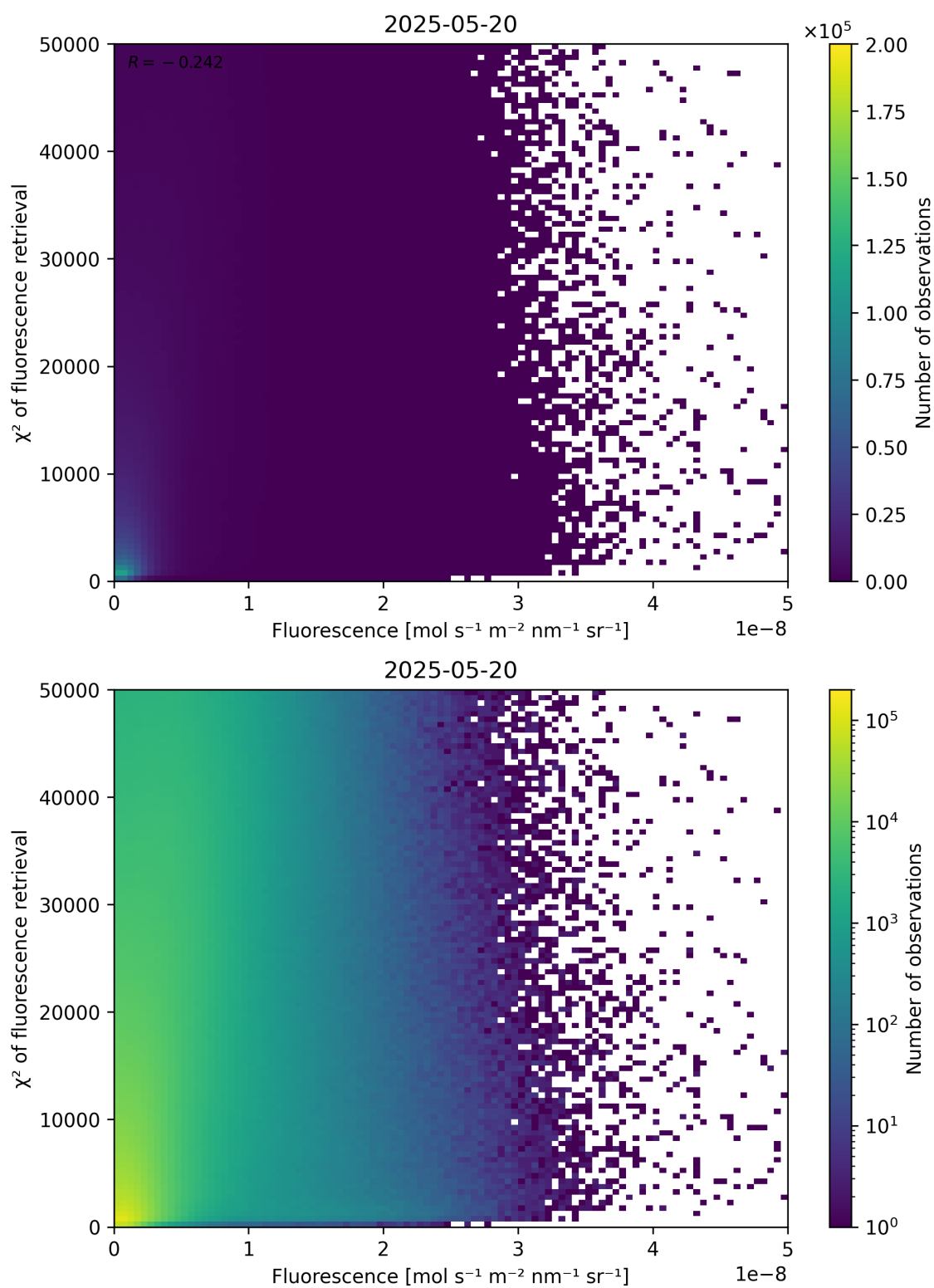
Figure 85: Scatter density plot of “Fluorescence” against “ \chi^2 of fluorescence retrieval” for 2025-05-19 to 2025-05-21.
