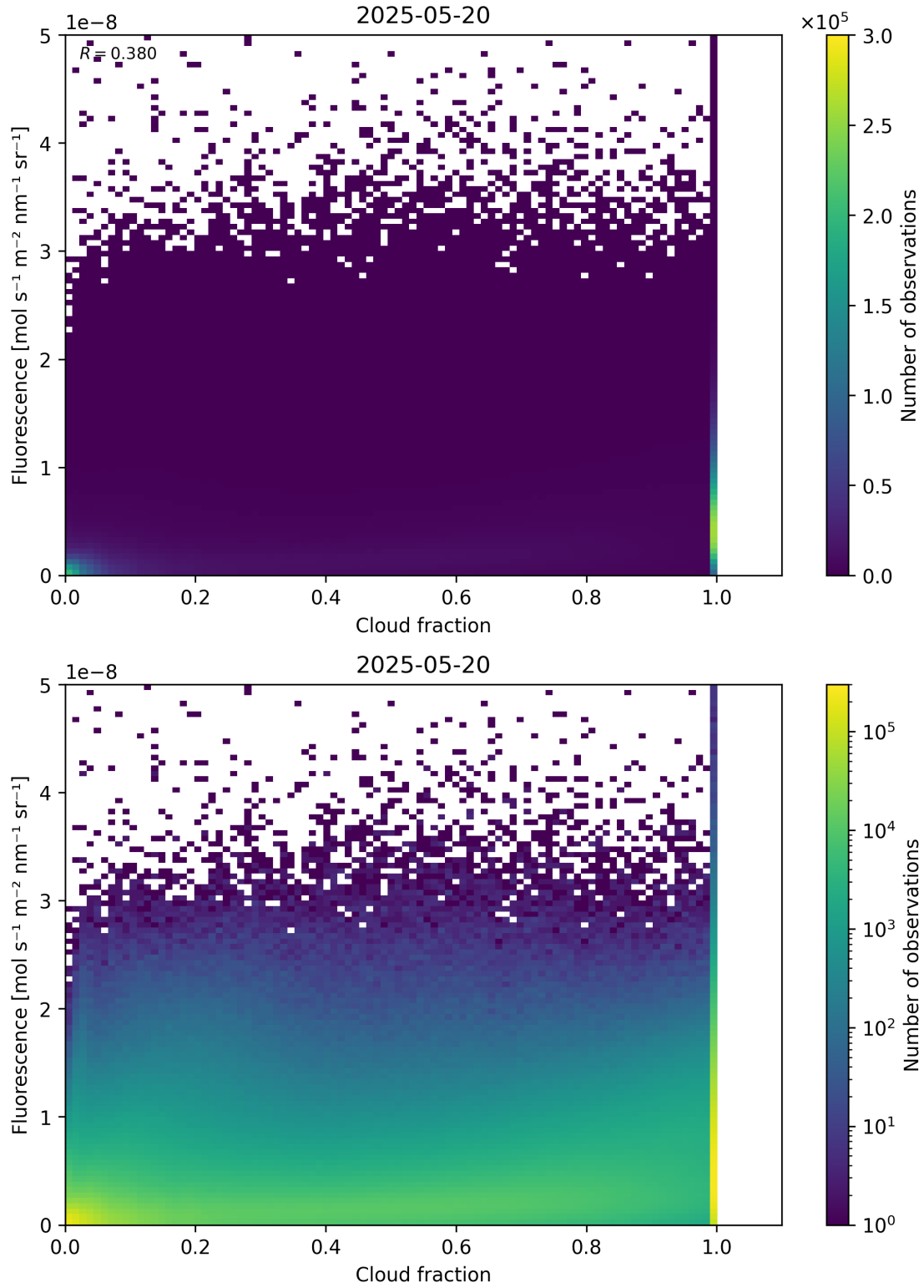
Figure 72: Scatter density plot of “Cloud fraction” against “Fluorescence” for 2025-05-19 to 2025-05-21.
