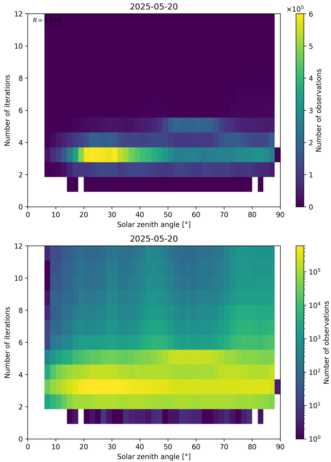
Figure 114: Scatter density plot of “Solar zenith angle” against “Number of iterations” for 2025-05-19 to 2025-05-21.
