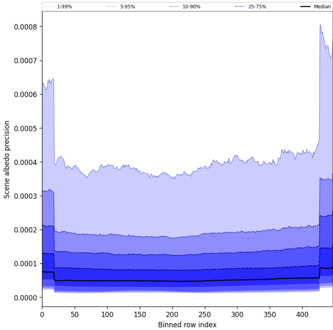
Figure 52: Along track statistics of “Scene albedo precision” for 2025-05-19 to 2025-05-21
