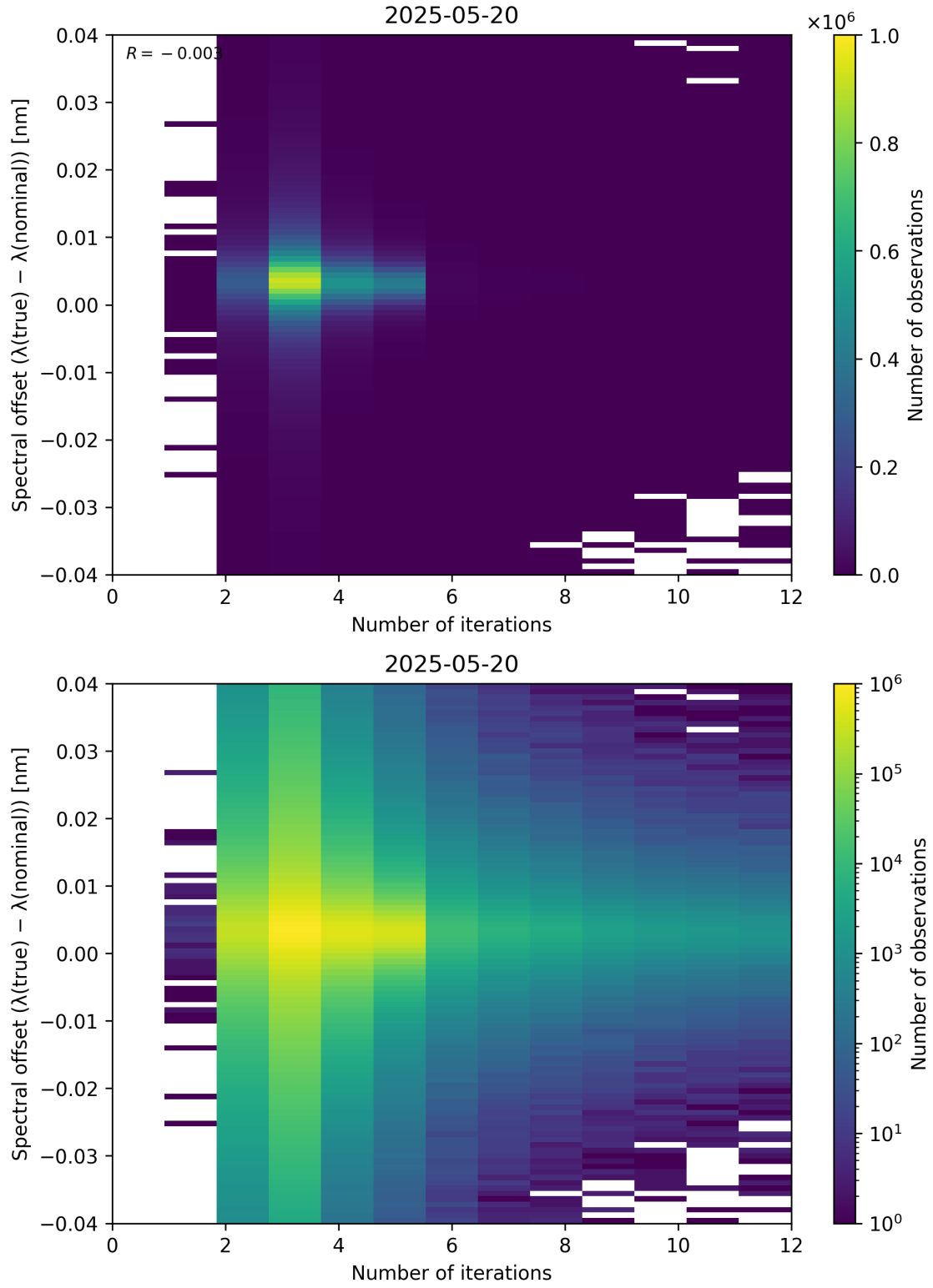
Figure 100: Scatter density plot of “Number of iterations” against “Spectral offset ( \lambda_{\text{true}} - \lambda_{\text{nominal}} )” for 2025-05-19 to 2025-05-21.
