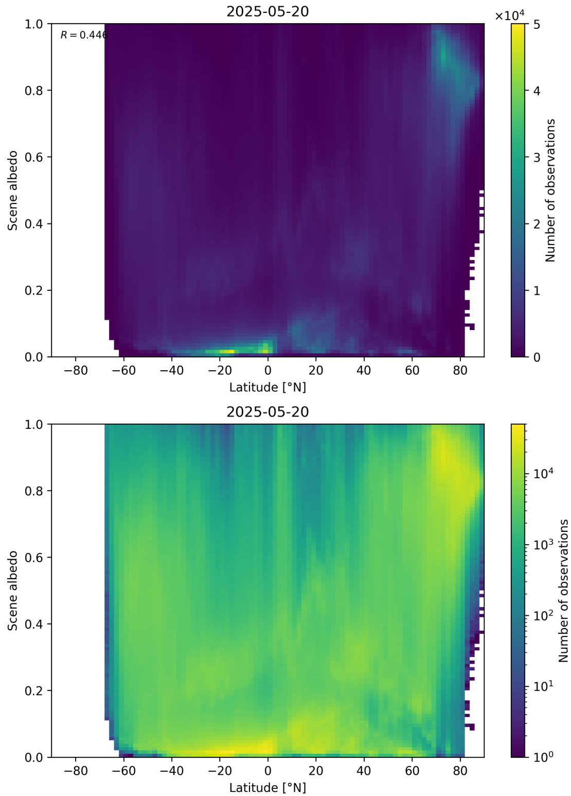
Figure 95: Scatter density plot of “Latitude” against “Scene albedo” for 2025-05-19 to 2025-05-21.
