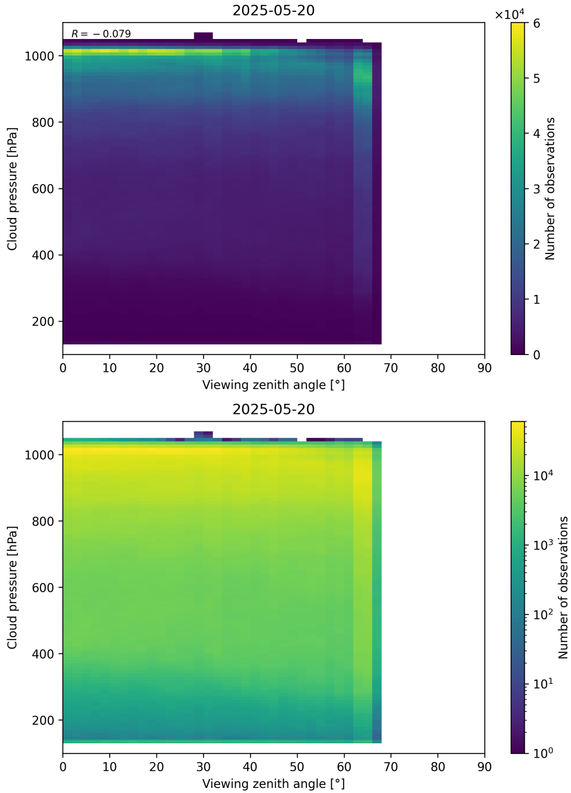
Figure 121: Scatter density plot of “Viewing zenith angle” against “Cloud pressure” for 2025-05-19 to 2025-05-21.
