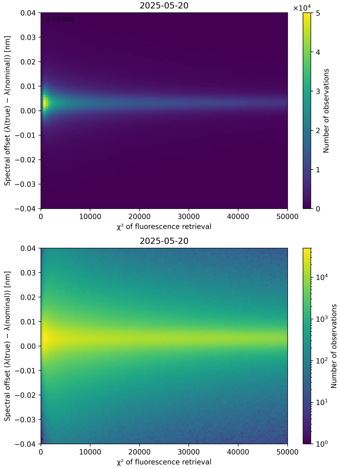
Figure 69: Scatter density plot of “ \chi^2 of fluorescence retrieval” against “Spectral offset ( \lambda_{\text{true}} - \lambda_{\text{nominal}} )” for 2025-05-19 to 2025-05-21.
