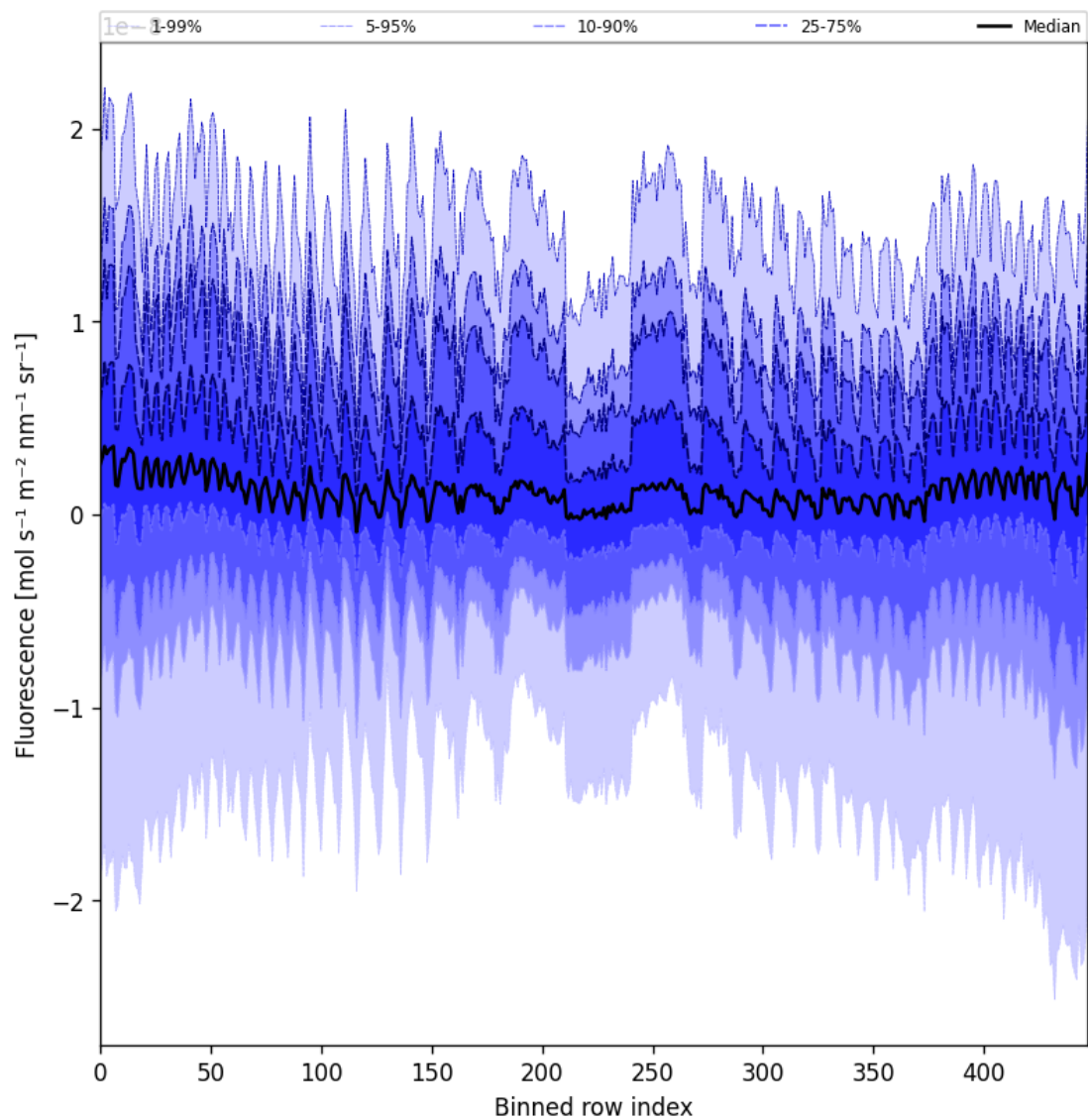
Figure 57: Along track statistics of “Fluorescence” for 2025-05-19 to 2025-05-21
