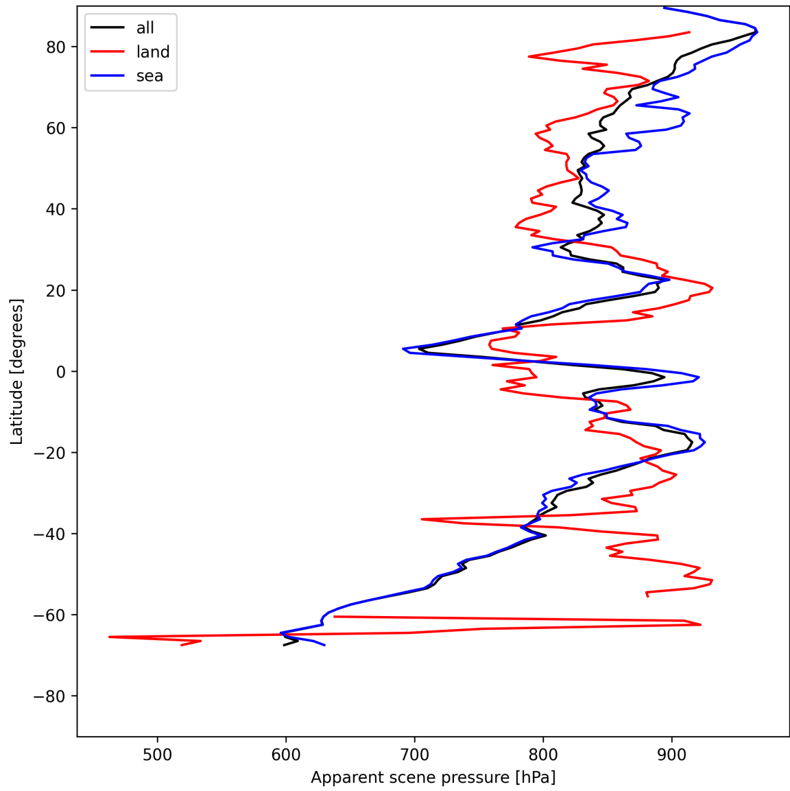
Figure 19: Zonal average of “Apparent scene pressure” for 2025-05-19 to 2025-05-21.
