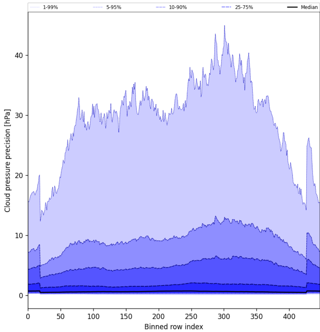
Figure 48: Along track statistics of “Cloud pressure precision” for 2025-05-19 to 2025-05-21
