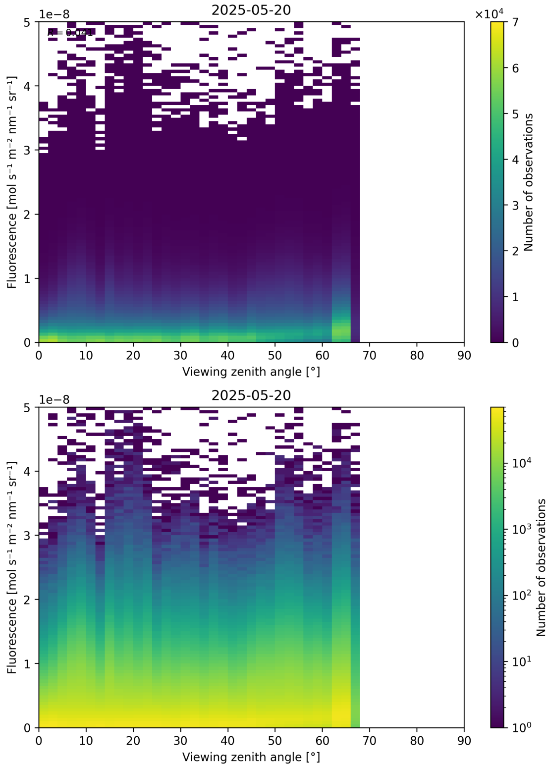
Figure 122: Scatter density plot of “Viewing zenith angle” against “Fluorescence” for 2025-05-19 to 2025-05-21.
