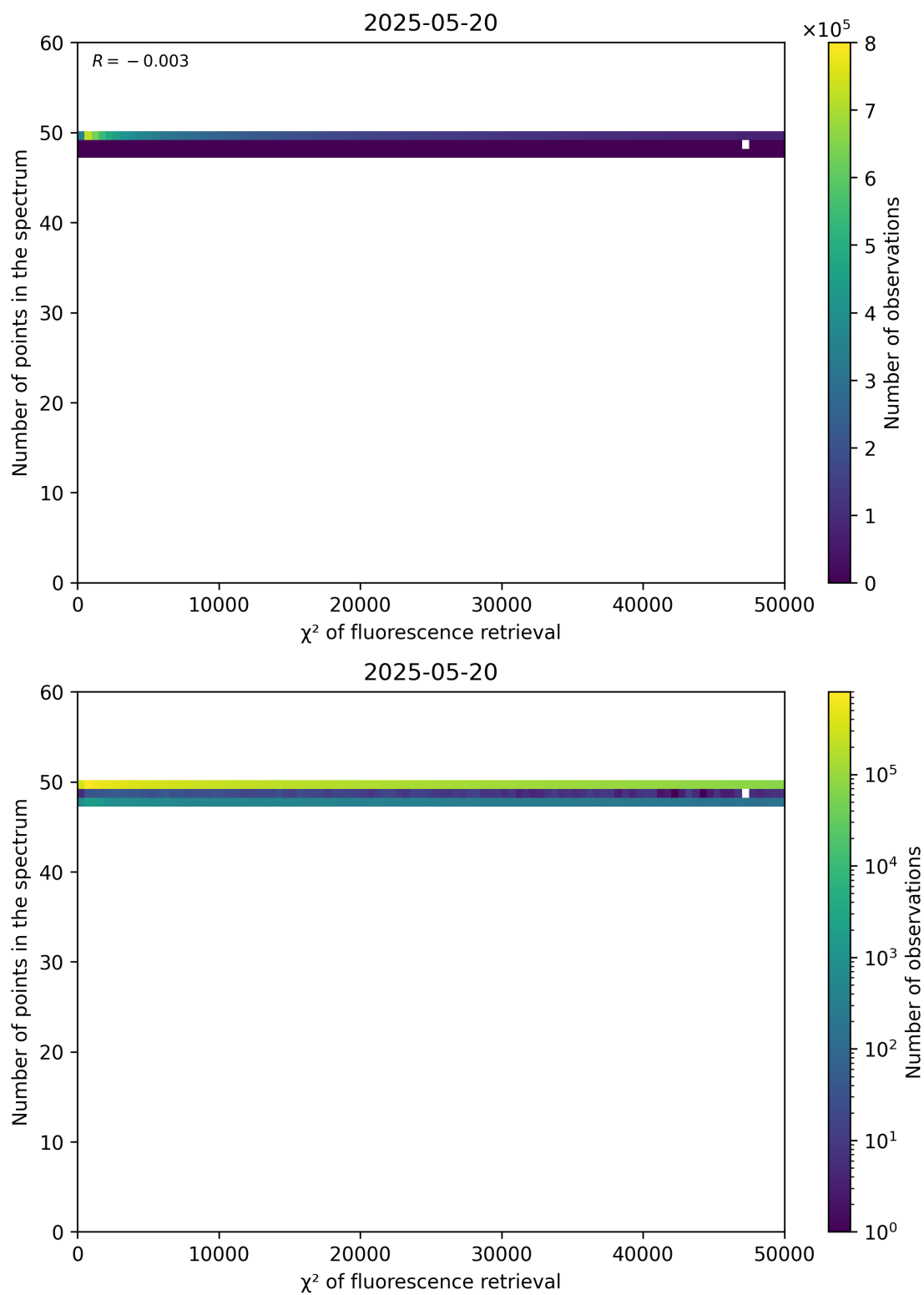
Figure 68: Scatter density plot of " \chi^2 of fluorescence retrieval" against "Number of points in the spectrum" for 2025-05-19 to 2025-05-21.
