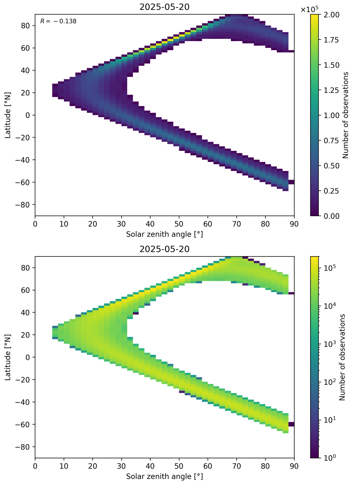
Figure 113: Scatter density plot of “Solar zenith angle” against “Latitude” for 2025-05-19 to 2025-05-21.
