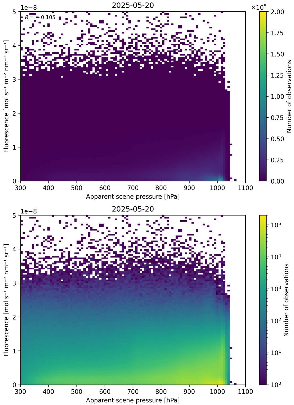
Figure 64: Scatter density plot of “Apparent scene pressure” against “Fluorescence” for 2025-05-19 to 2025-05-21.
