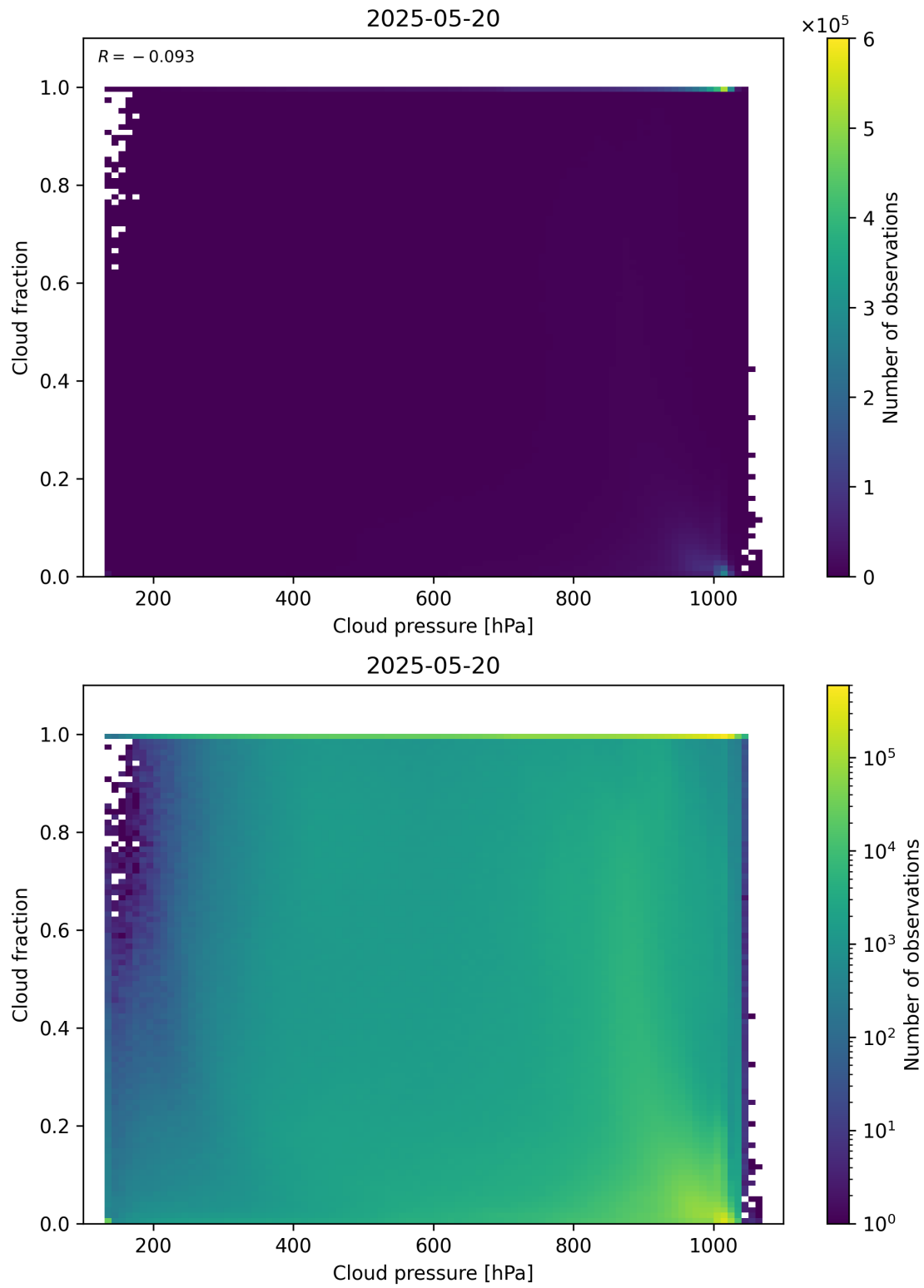
Figure 79: Scatter density plot of “Cloud pressure” against “Cloud fraction” for 2025-05-19 to 2025-05-21.
