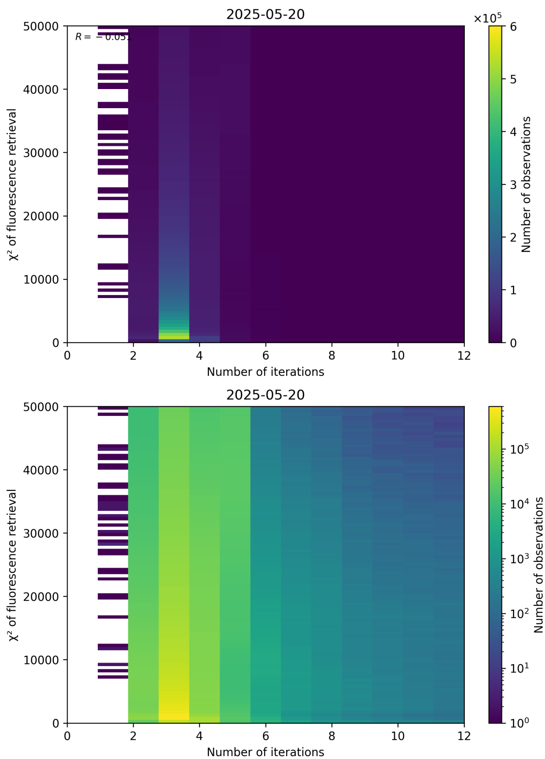
Figure 97: Scatter density plot of “Number of iterations” against “ \chi^2 of fluorescence retrieval” for 2025-05-19 to 2025-05-21.
