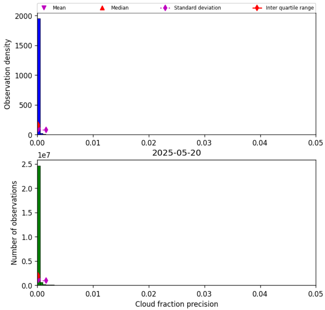
Figure 33: Histogram of “Cloud fraction precision” for 2025-05-19 to 2025-05-21
