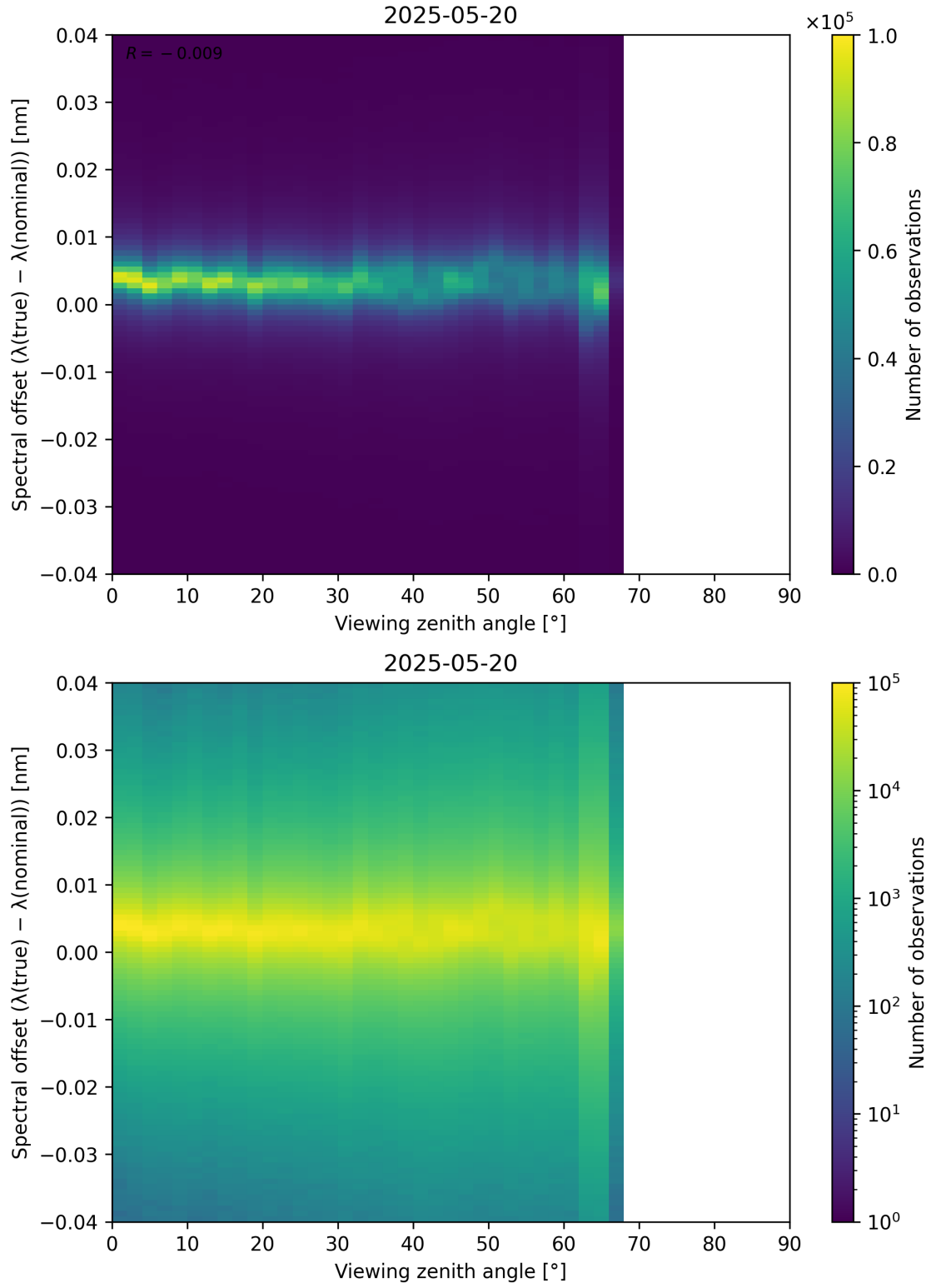
Figure 128: Scatter density plot of “Viewing zenith angle” against “Spectral offset ( \lambda_{\text{true}} - \lambda_{\text{nominal}} )” for 2025-05-19 to 2025-05-21.
