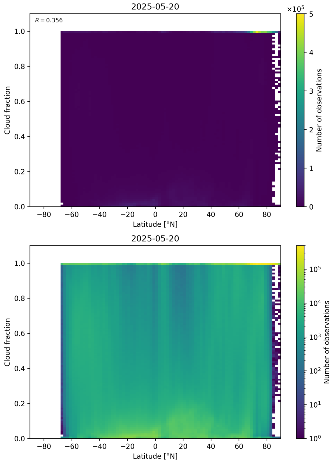
Figure 90: Scatter density plot of “Latitude” against “Cloud fraction” for 2025-05-19 to 2025-05-21.
