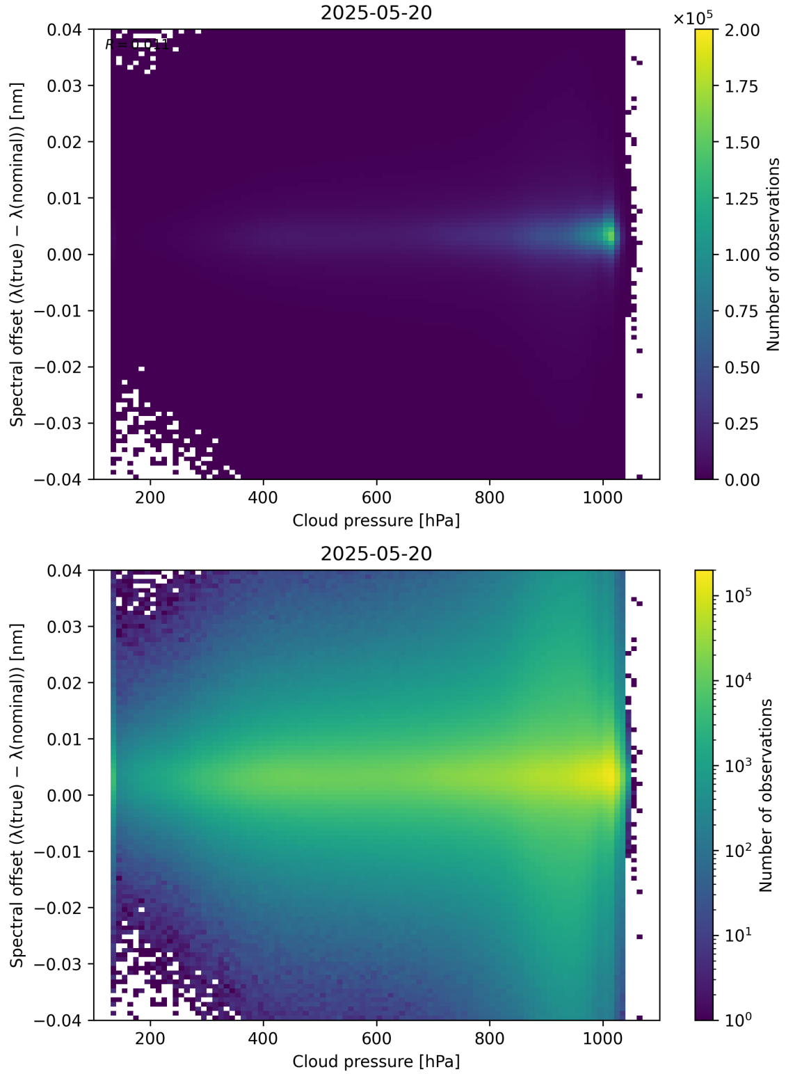
Figure 84: Scatter density plot of “Cloud pressure” against “Spectral offset ( \lambda_{\text{true}} - \lambda_{\text{nominal}} )” for 2025-05-19 to 2025-05-21.
