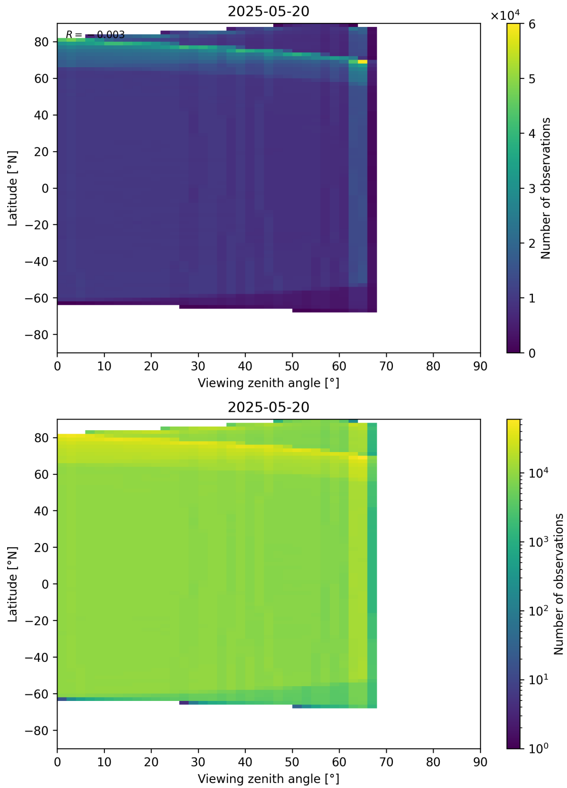
Figure 123: Scatter density plot of “Viewing zenith angle” against “Latitude” for 2025-05-19 to 2025-05-21.
