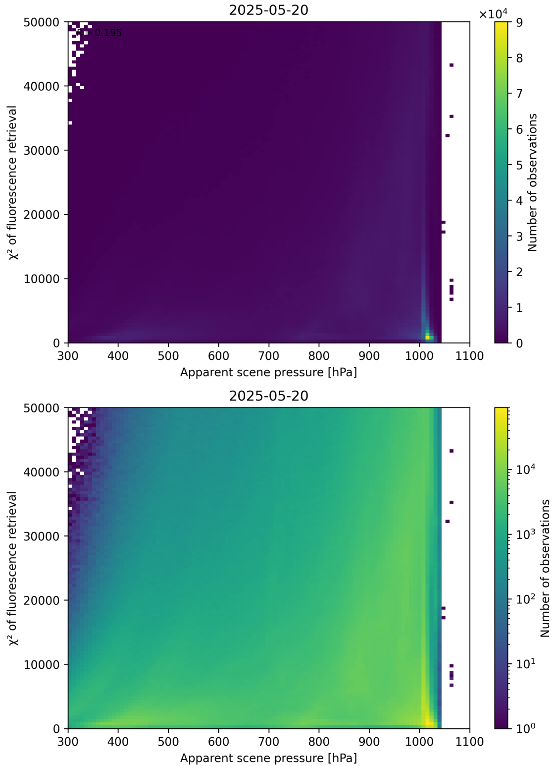
Figure 63: Scatter density plot of “Apparent scene pressure” against “ \chi^2 of fluorescence retrieval” for 2025-05-19 to 2025-05-21.
