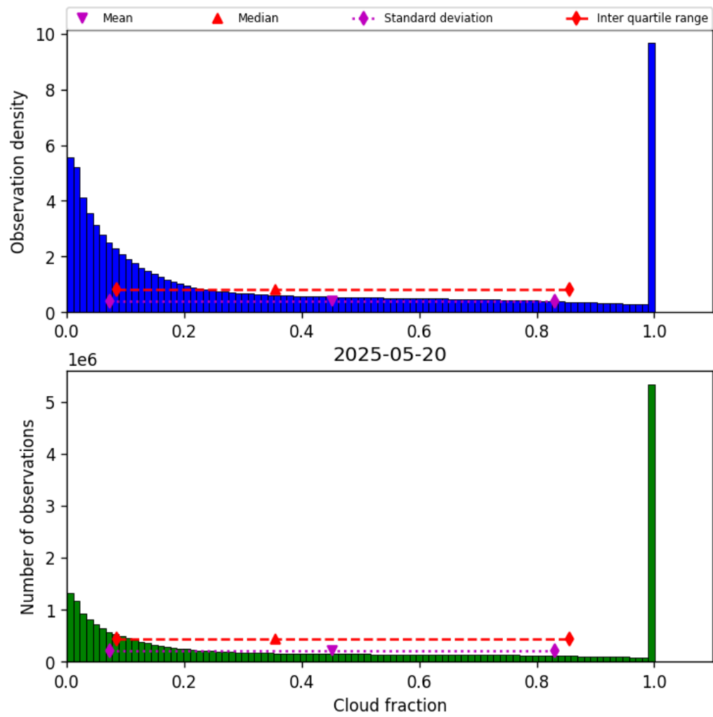
Figure 32: Histogram of “Cloud fraction” for 2025-05-19 to 2025-05-21
