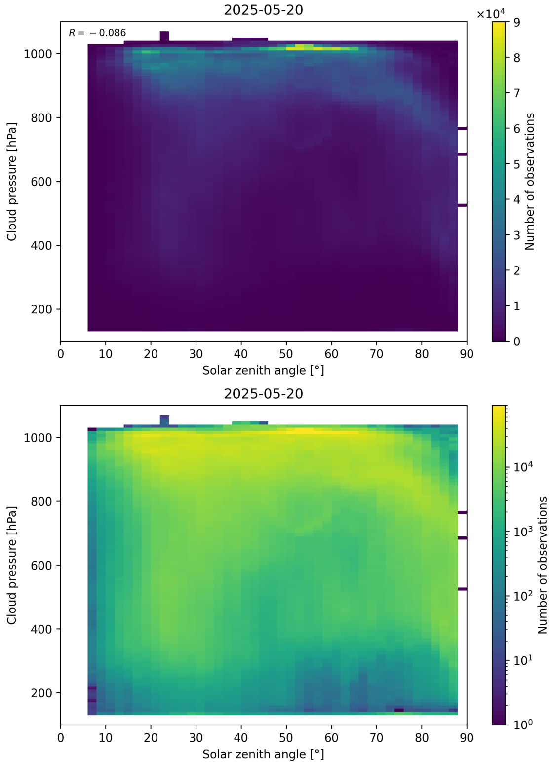
Figure 111: Scatter density plot of “Solar zenith angle” against “Cloud pressure” for 2025-05-19 to 2025-05-21.
