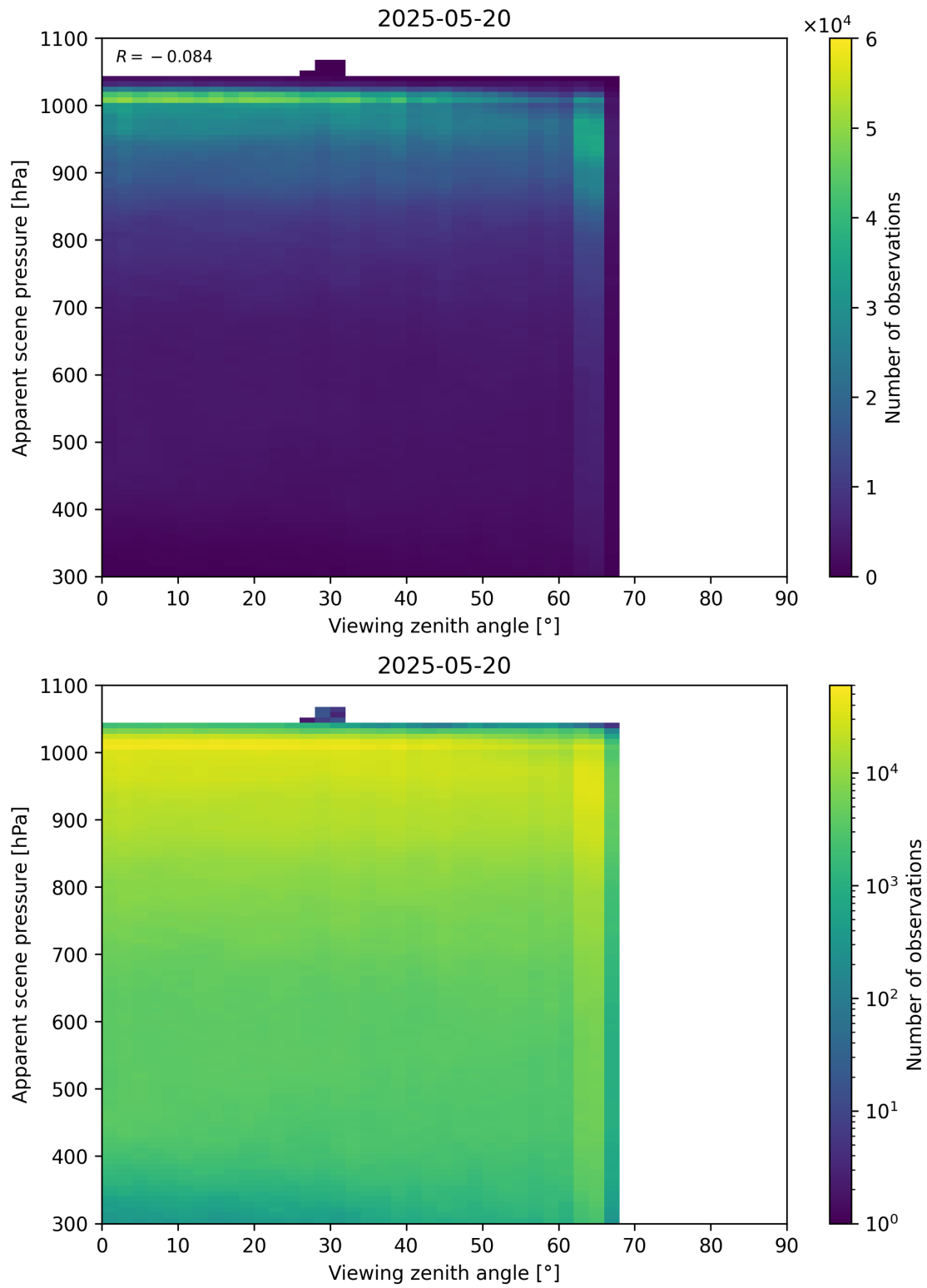
Figure 118: Scatter density plot of “Viewing zenith angle” against “Apparent scene pressure” for 2025-05-19 to 2025-05-21.
