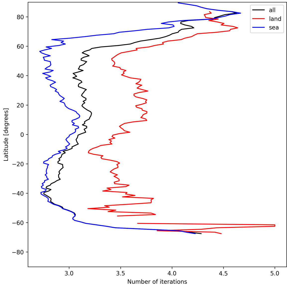
Figure 22: Zonal average of “Number of iterations” for 2025-05-19 to 2025-05-21.
