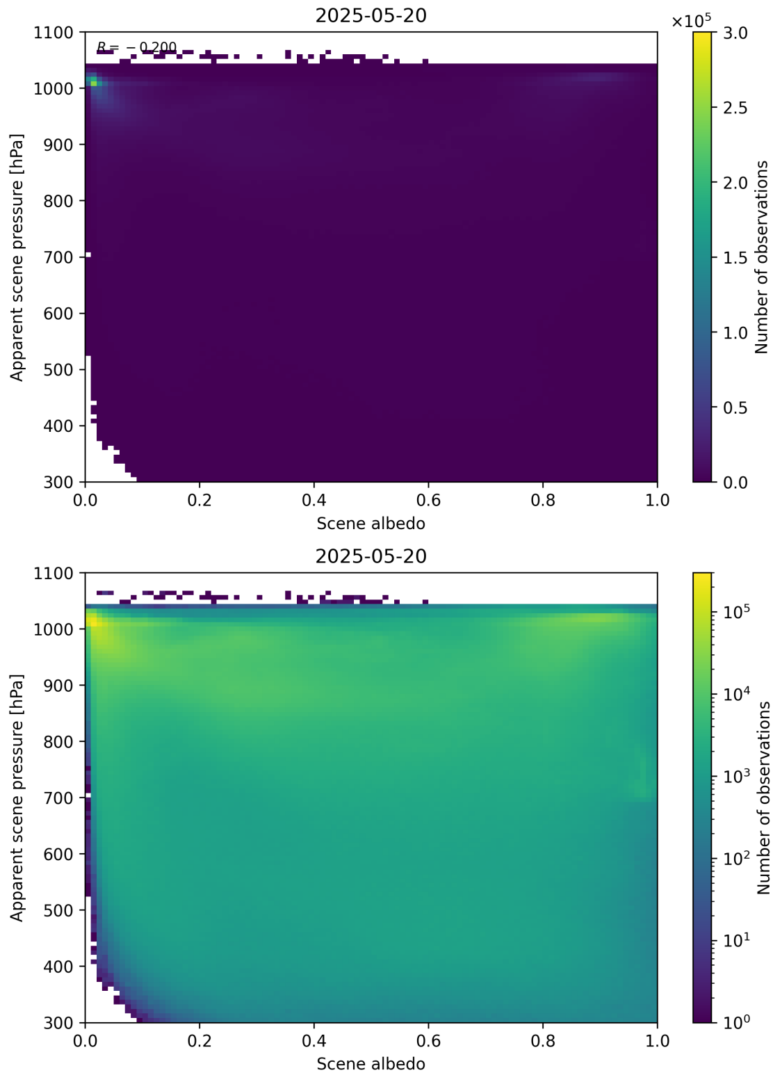
Figure 102: Scatter density plot of “Scene albedo” against “Apparent scene pressure” for 2025-05-19 to 2025-05-21.
