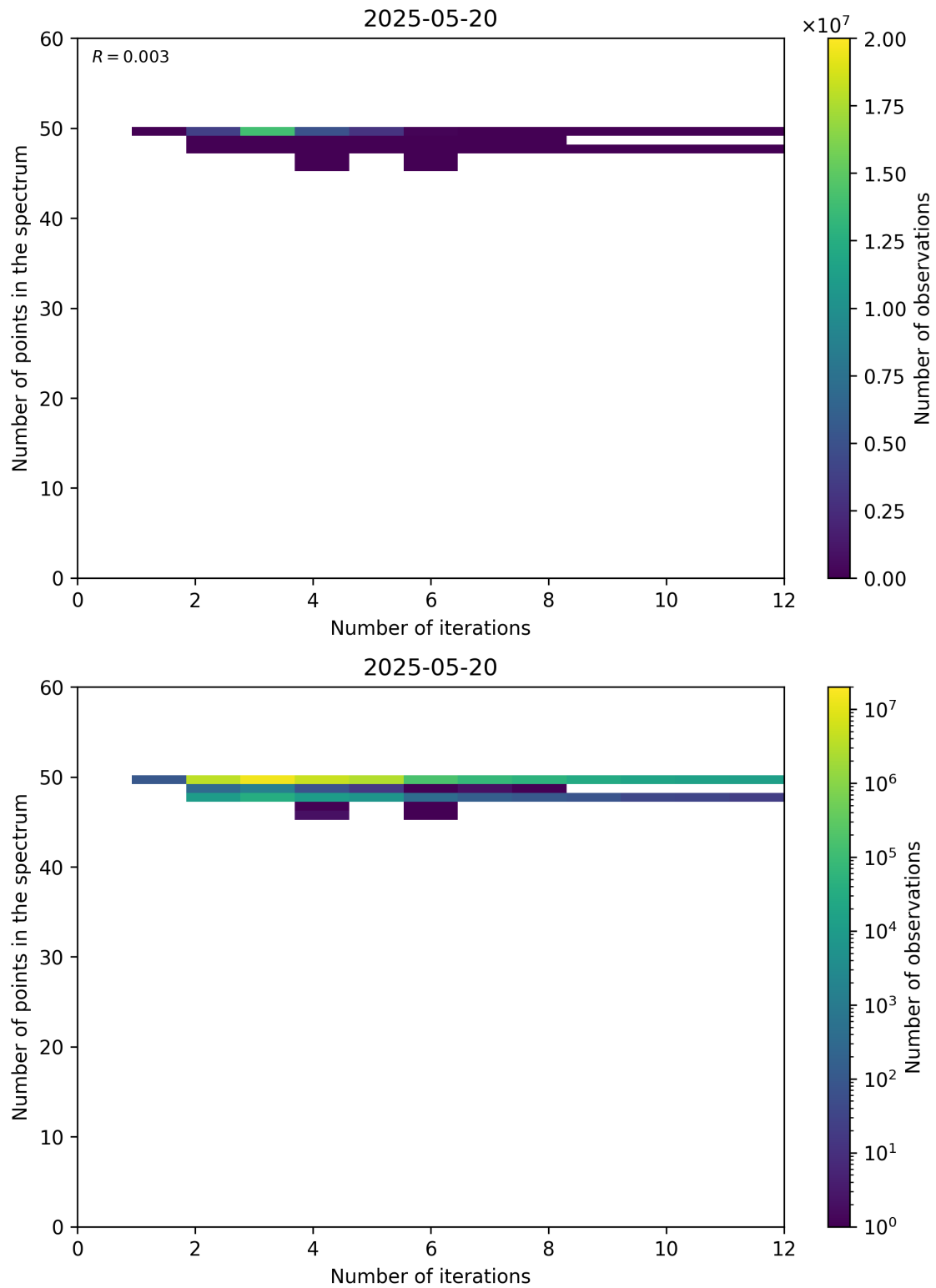
Figure 99: Scatter density plot of “Number of iterations” against “Number of points in the spectrum” for 2025-05-19 to 2025-05-21.
