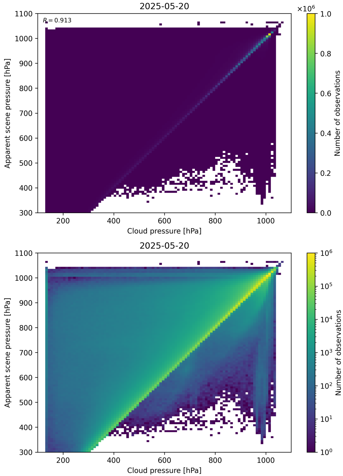
Figure 77: Scatter density plot of “Cloud pressure” against “Apparent scene pressure” for 2025-05-19 to 2025-05-21.
