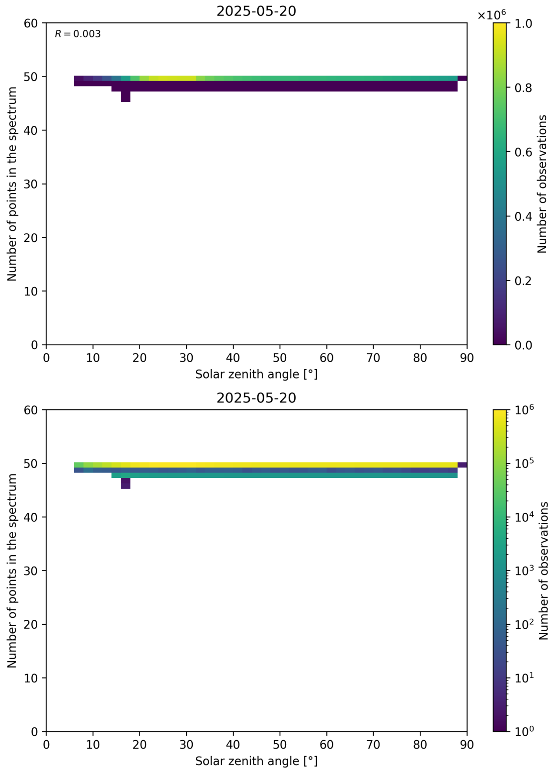
Figure 115: Scatter density plot of “Solar zenith angle” against “Number of points in the spectrum” for 2025-05-19 to 2025-05-21.
