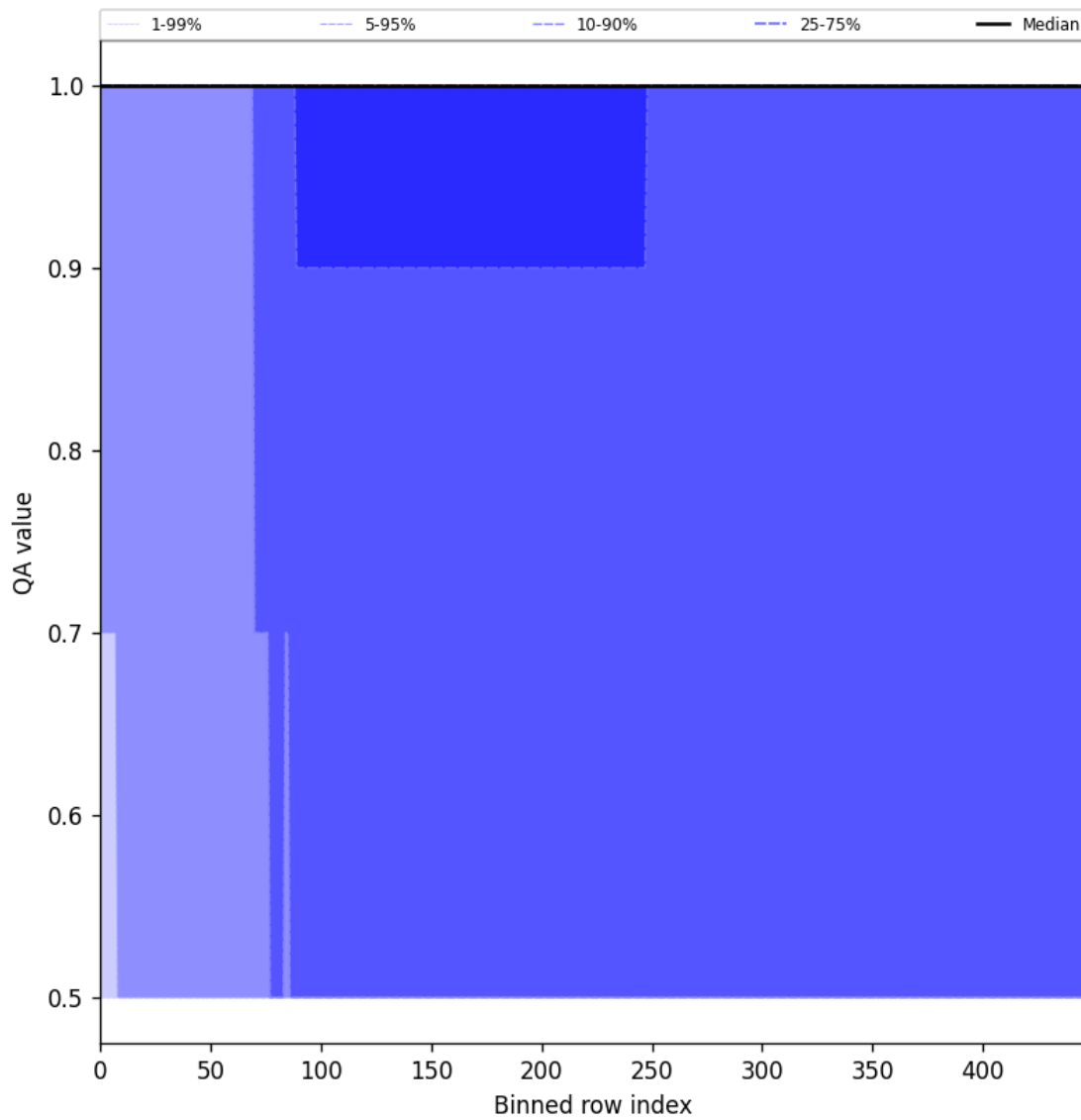
Figure 46: Along track statistics of “QA value” for 2025-05-19 to 2025-05-21
