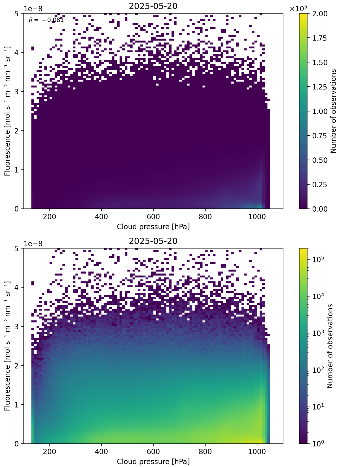
Figure 80: Scatter density plot of “Cloud pressure” against “Fluorescence” for 2025-05-19 to 2025-05-21.
