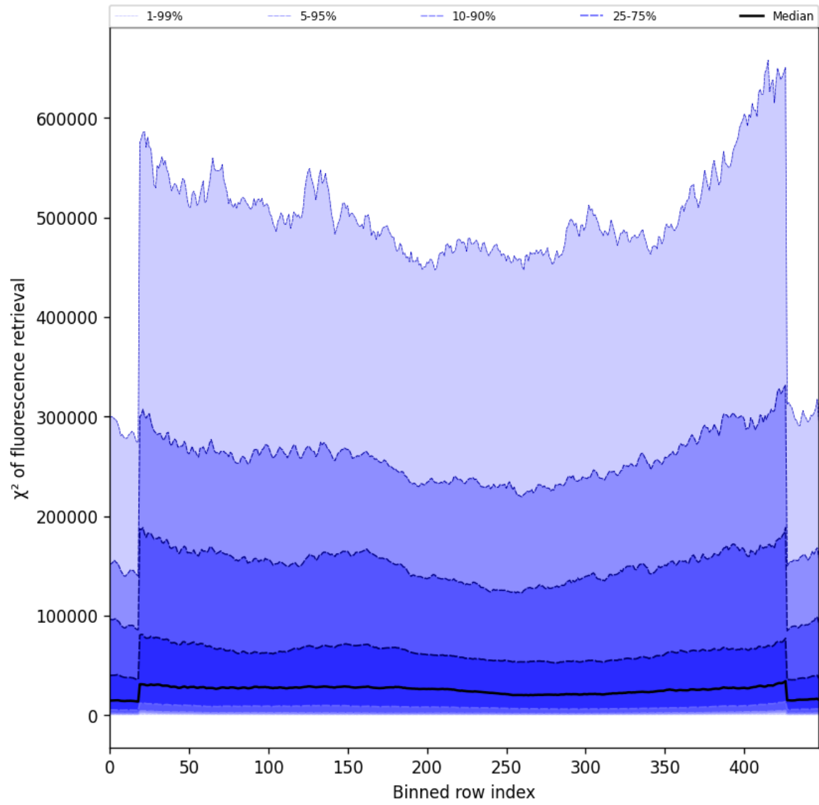
Figure 59: Along track statistics of “ \chi^2 of fluorescence retrieval” for 2025-05-19 to 2025-05-21
