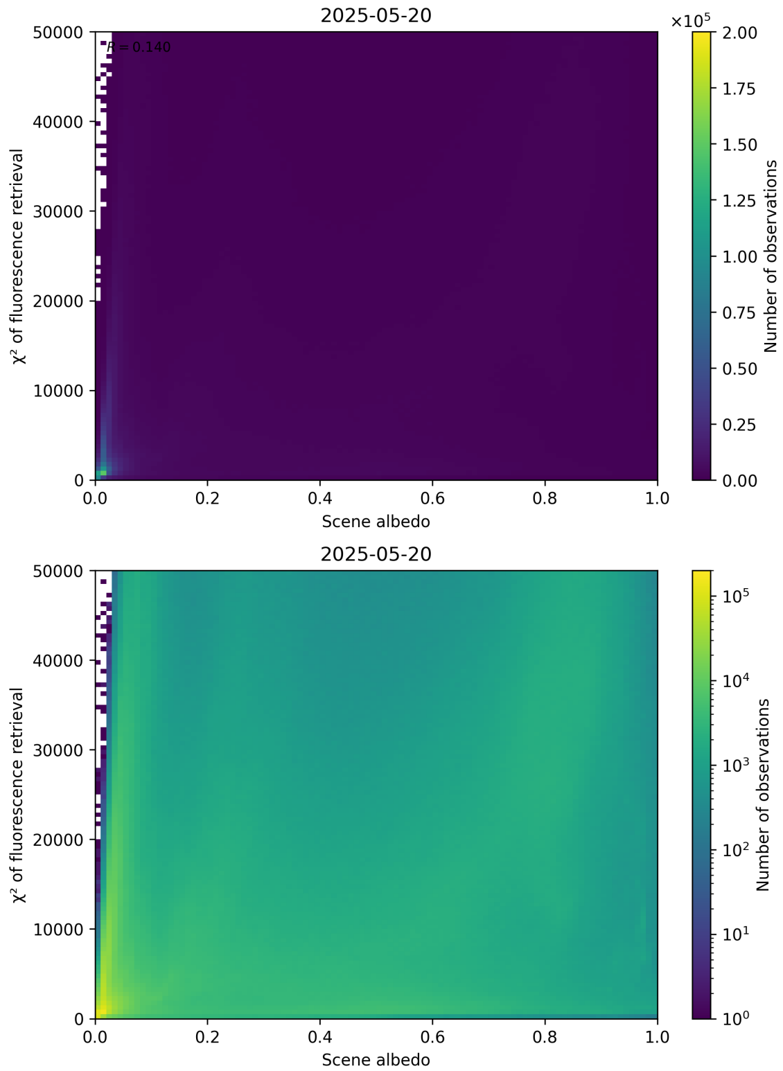
Figure 103: Scatter density plot of “Scene albedo” against “ \chi^2 of fluorescence retrieval” for 2025-05-19 to 2025-05-21.
