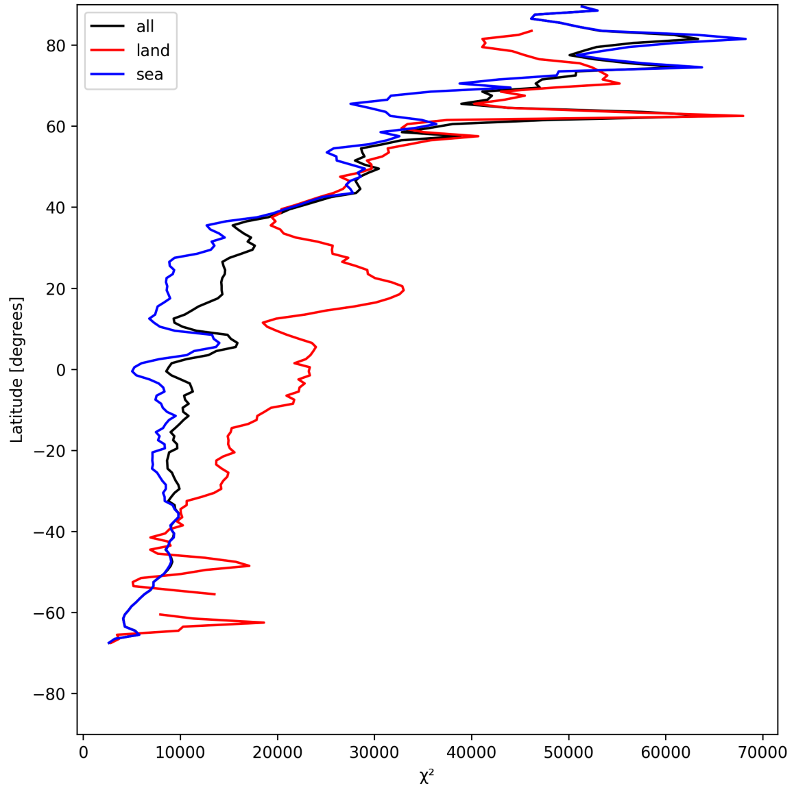
Figure 21: Zonal average of “ \chi^2 ” for 2025-05-19 to 2025-05-21.
