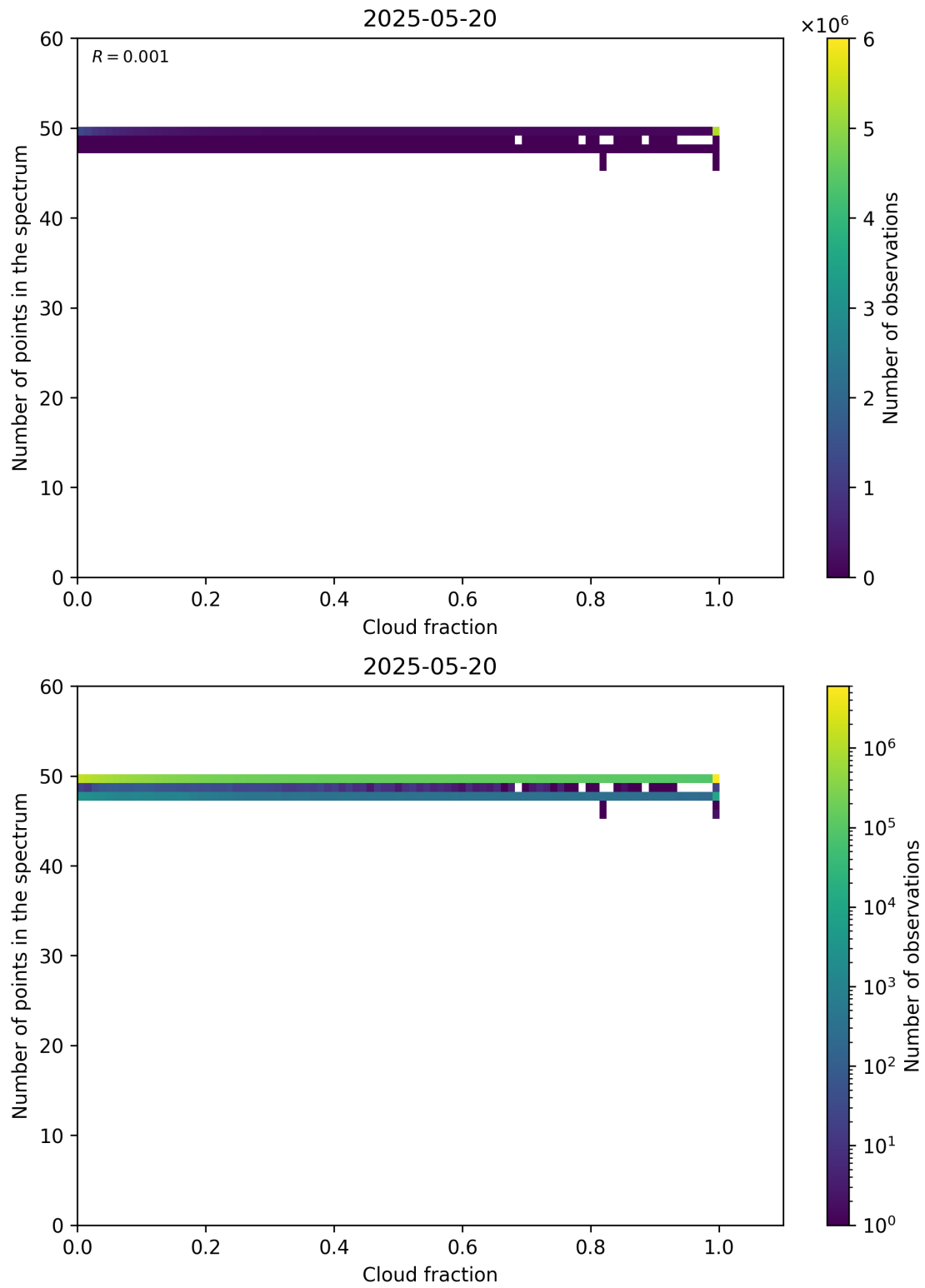
Figure 74: Scatter density plot of “Cloud fraction” against “Number of points in the spectrum” for 2025-05-19 to 2025-05-21.
