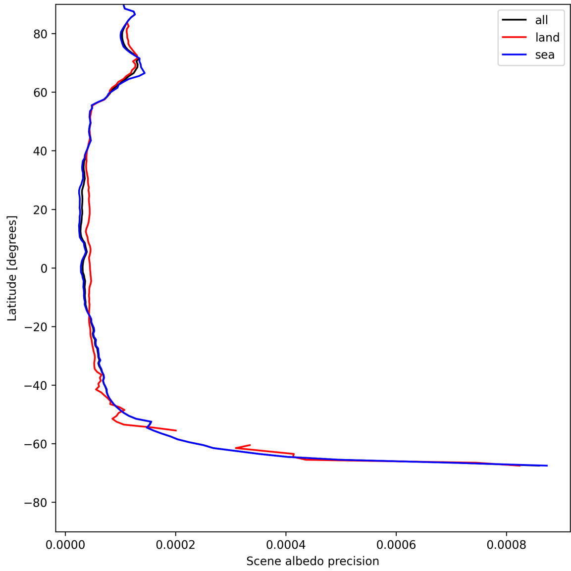
Figure 18: Zonal average of “Scene albedo precision” for 2025-05-19 to 2025-05-21.
