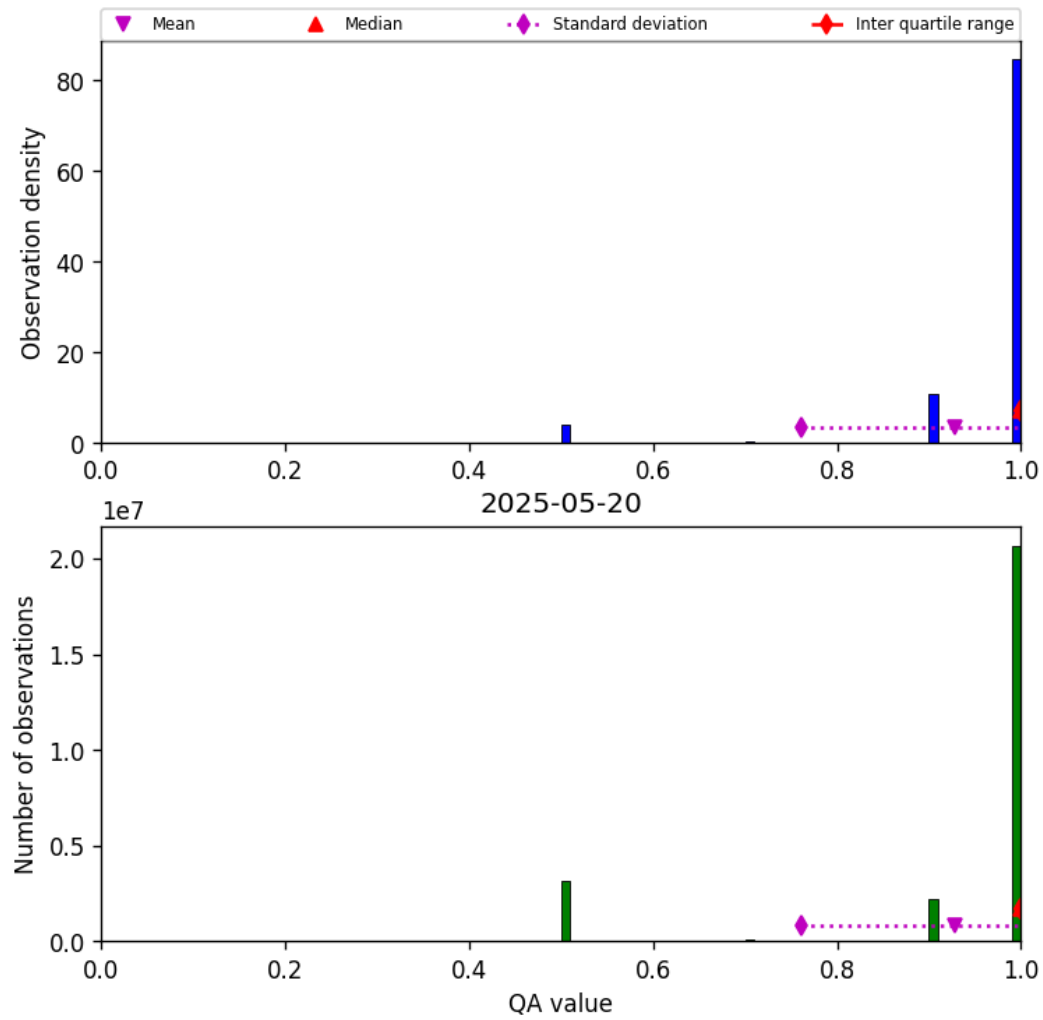
Figure 29: Histogram of “QA value” for 2025-05-19 to 2025-05-21
