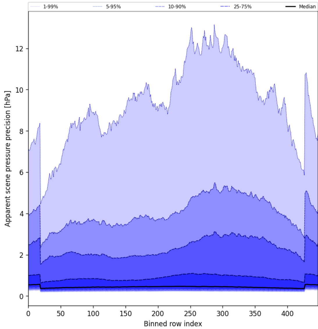
Figure 54: Along track statistics of “Apparent scene pressure precision” for 2025-05-19 to 2025-05-21
