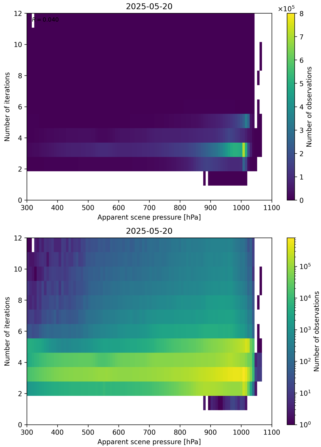
Figure 65: Scatter density plot of “Apparent scene pressure” against “Number of iterations” for 2025-05-19 to 2025-05-21.
