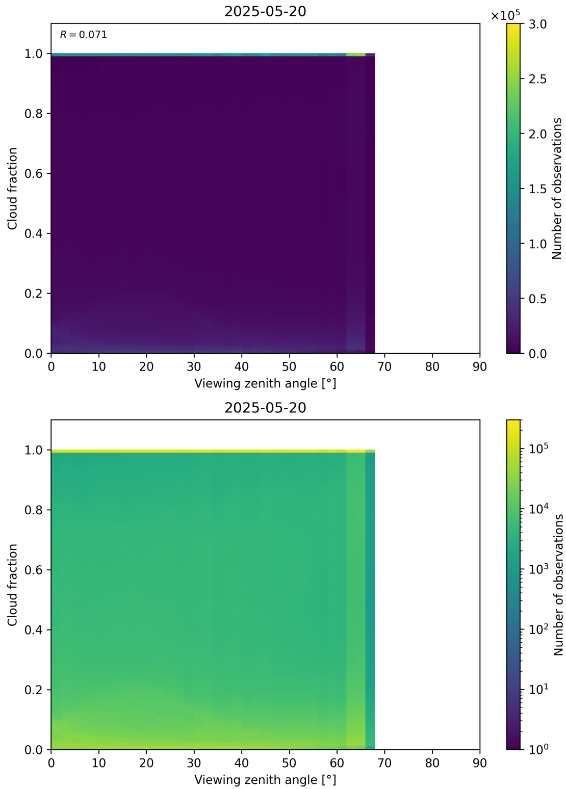
Figure 120: Scatter density plot of “Viewing zenith angle” against “Cloud fraction” for 2025-05-19 to 2025-05-21.
