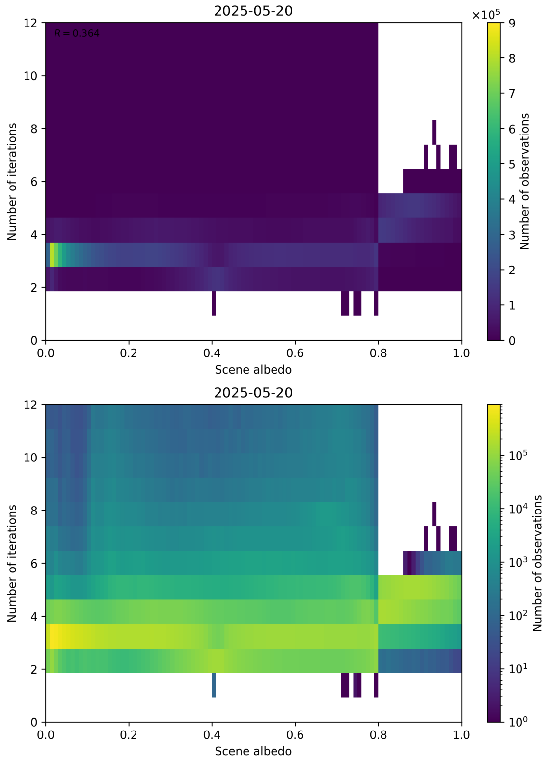
Figure 105: Scatter density plot of “Scene albedo” against “Number of iterations” for 2025-05-19 to 2025-05-21.
