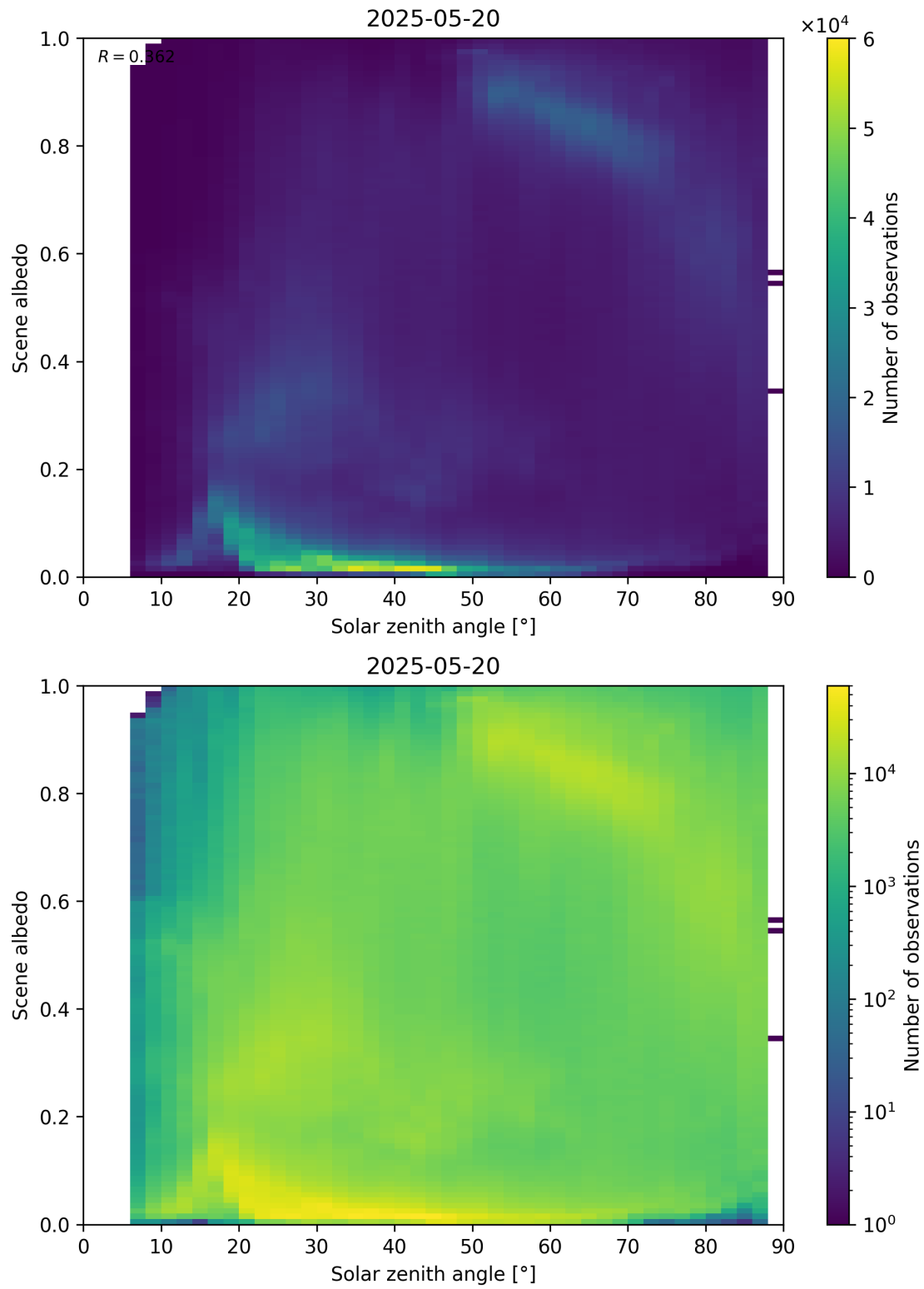
Figure 116: Scatter density plot of “Solar zenith angle” against “Scene albedo” for 2025-05-19 to 2025-05-21.
