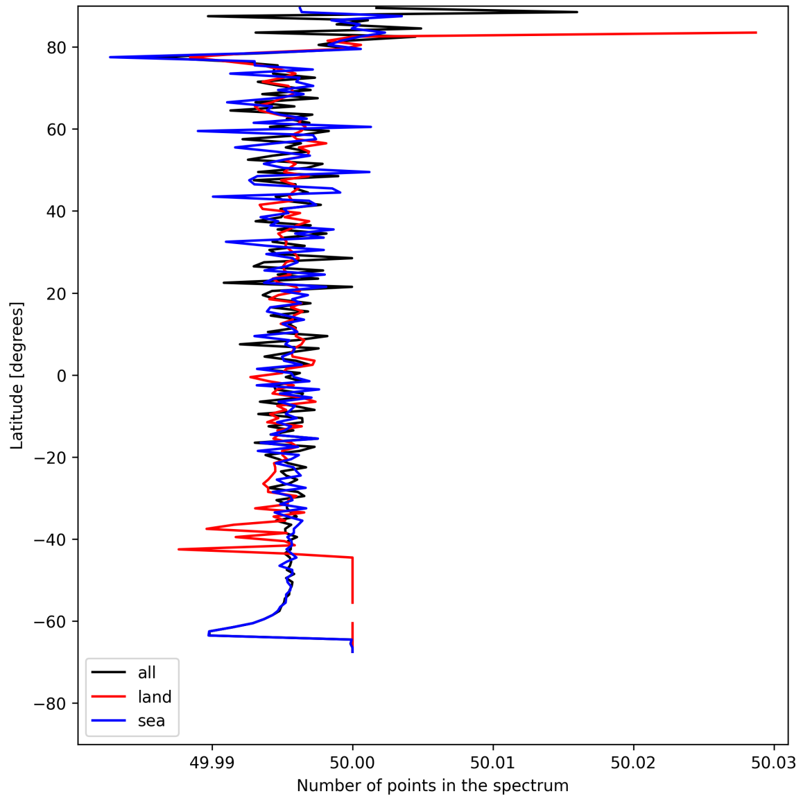
Figure 27: Zonal average of “Number of points in the spectrum” for 2025-05-19 to 2025-05-21.
