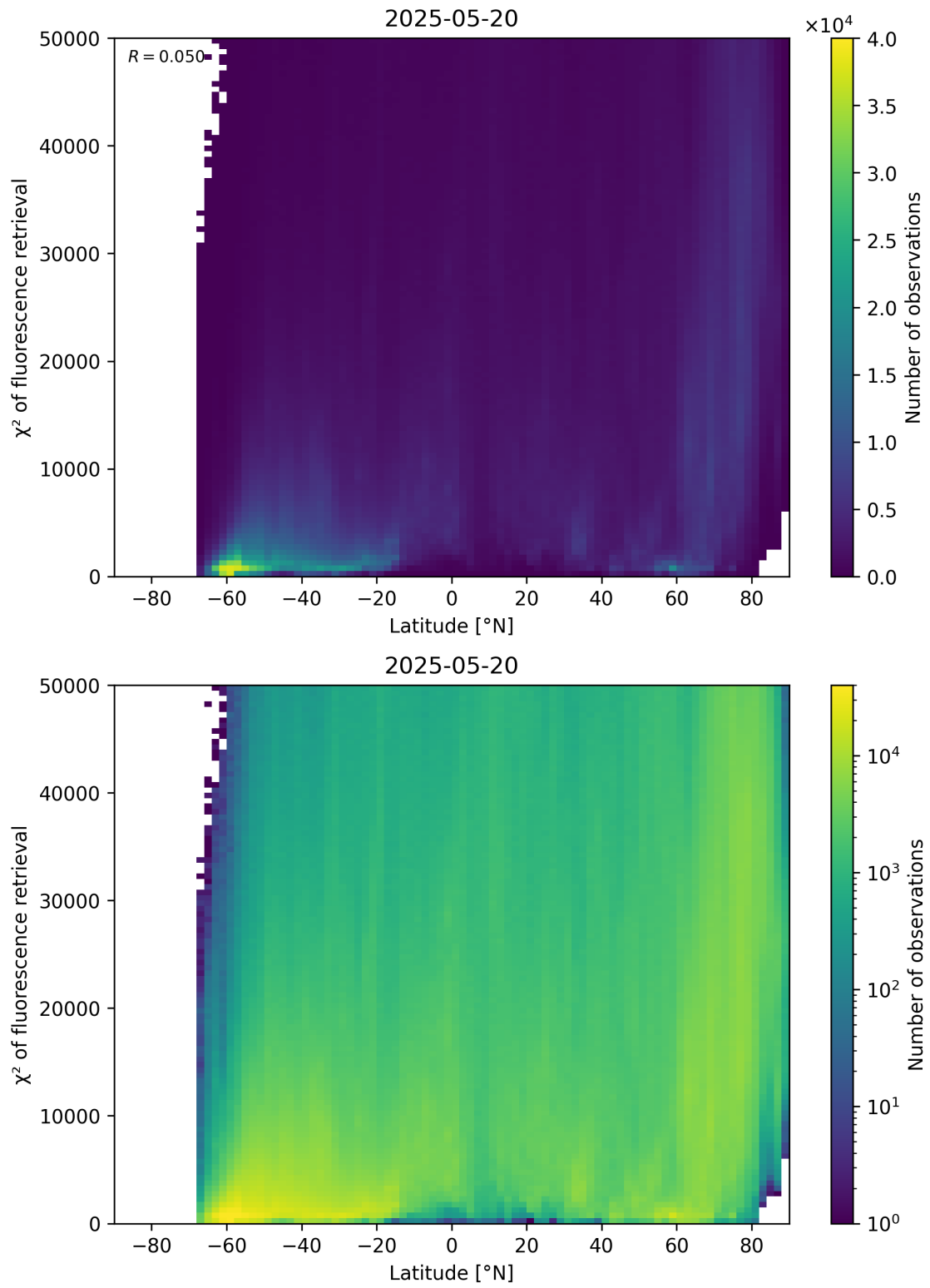
Figure 89: Scatter density plot of “Latitude” against “ \chi^2 of fluorescence retrieval” for 2025-05-19 to 2025-05-21.
