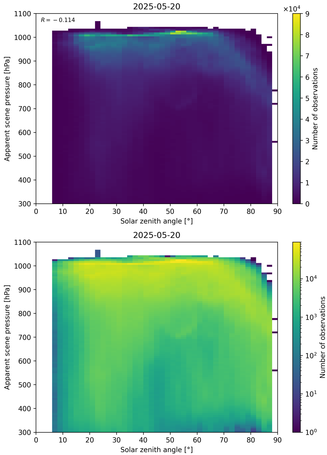
Figure 108: Scatter density plot of “Solar zenith angle” against “Apparent scene pressure” for 2025-05-19 to 2025-05-21.
