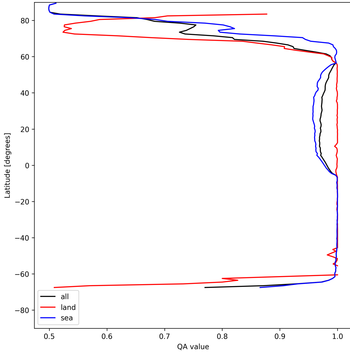
Figure 12: Zonal average of “QA value” for 2025-05-19 to 2025-05-21.
