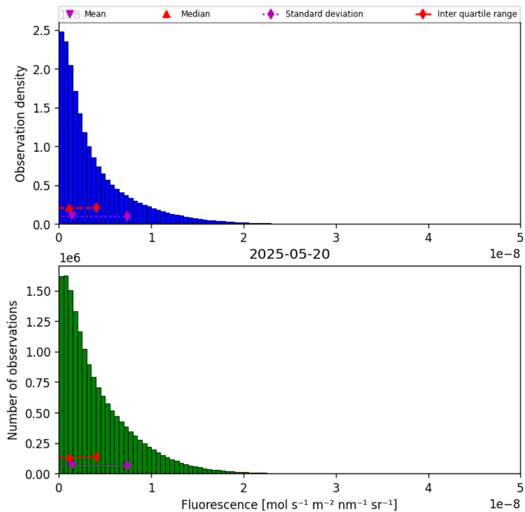
Figure 40: Histogram of “Fluorescence” for 2025-05-19 to 2025-05-21
