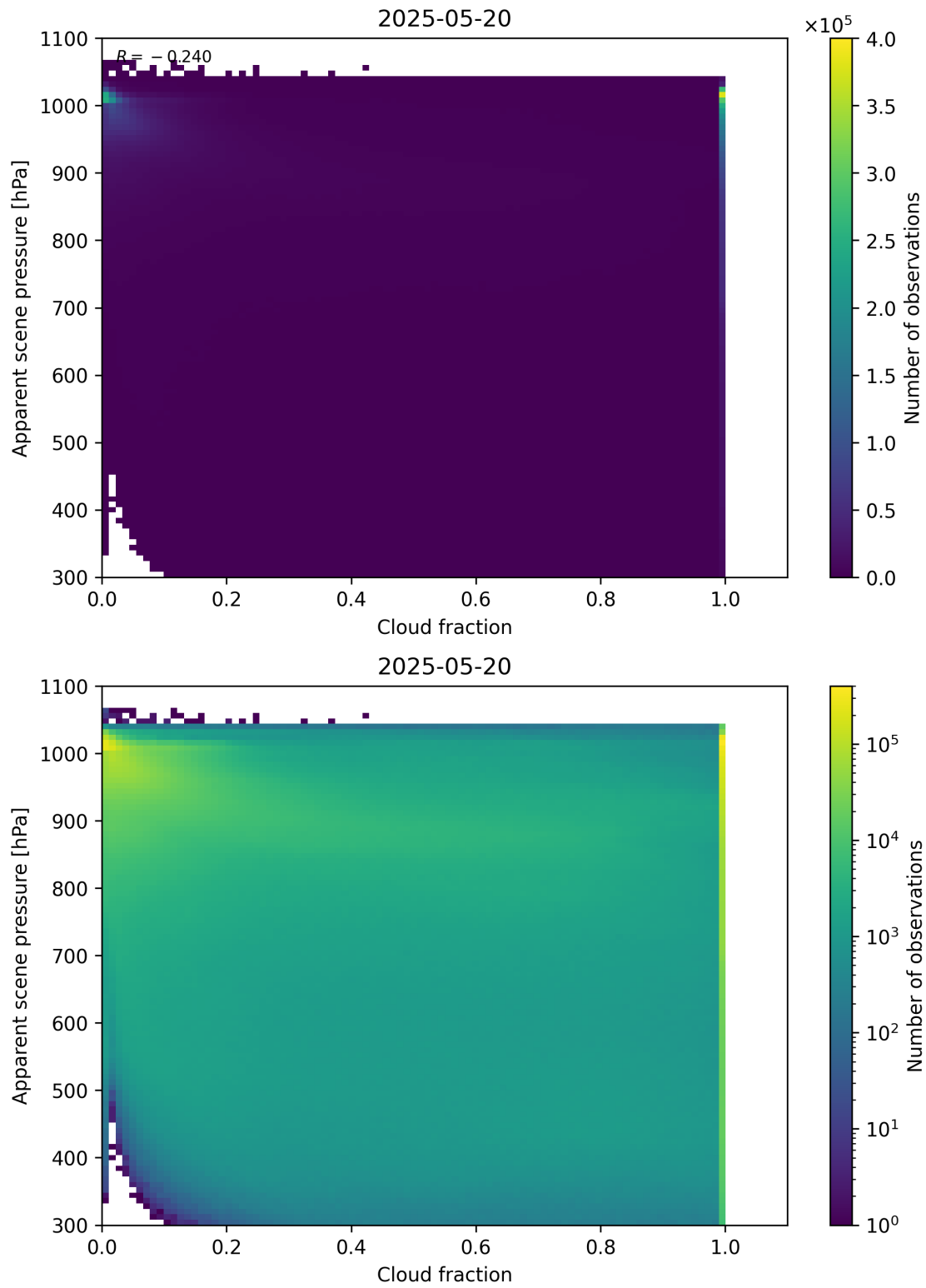
Figure 70: Scatter density plot of “Cloud fraction” against “Apparent scene pressure” for 2025-05-19 to 2025-05-21.
