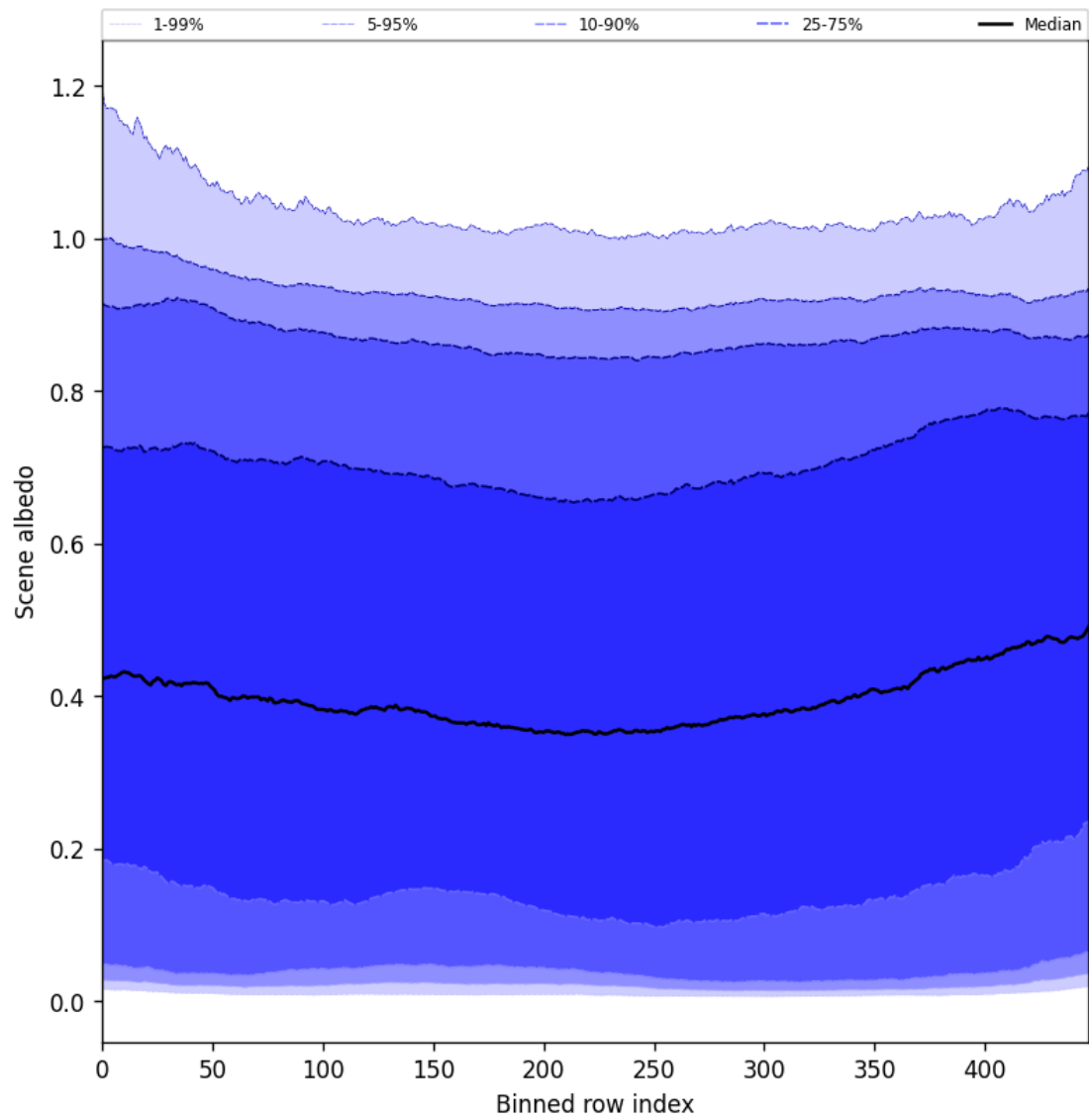
Figure 51: Along track statistics of “Scene albedo” for 2025-05-19 to 2025-05-21
