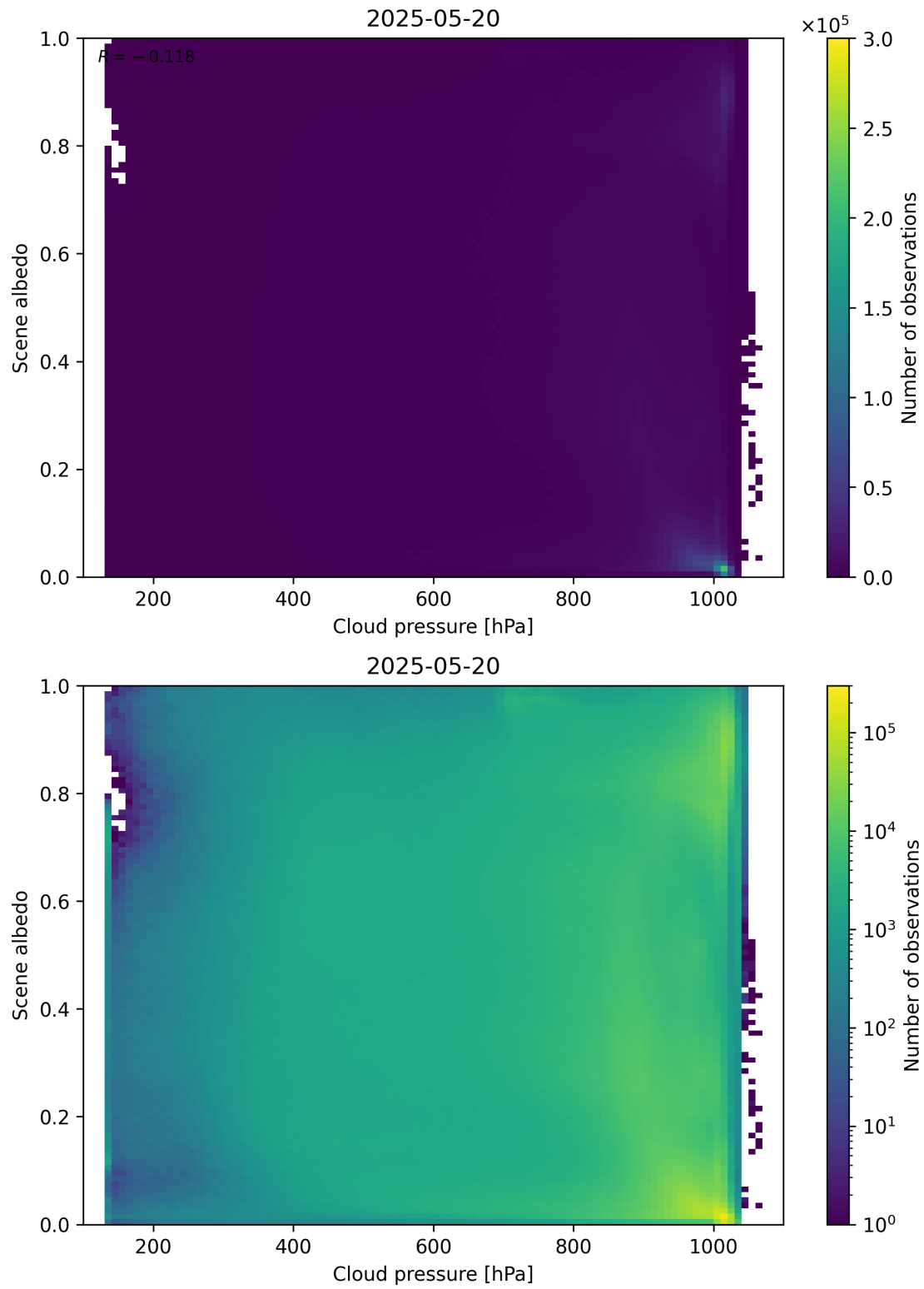
Figure 83: Scatter density plot of “Cloud pressure” against “Scene albedo” for 2025-05-19 to 2025-05-21.
