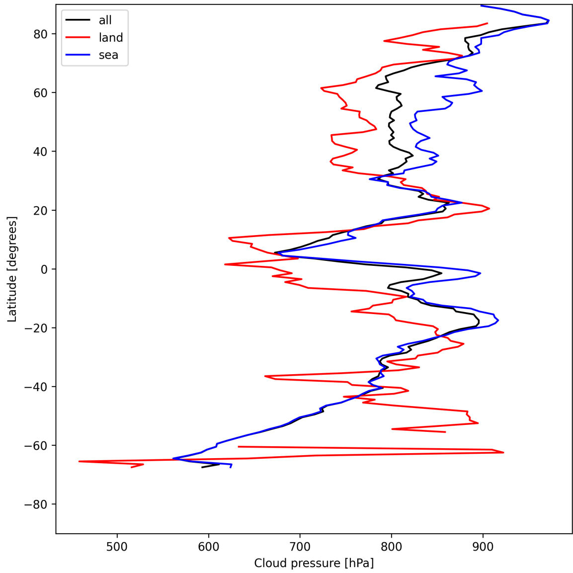
Figure 13: Zonal average of “Cloud pressure” for 2025-05-19 to 2025-05-21.
