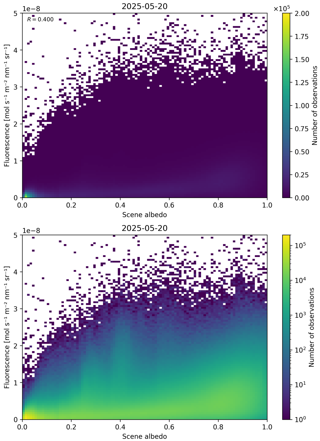
Figure 104: Scatter density plot of “Scene albedo” against “Fluorescence” for 2025-05-19 to 2025-05-21.
