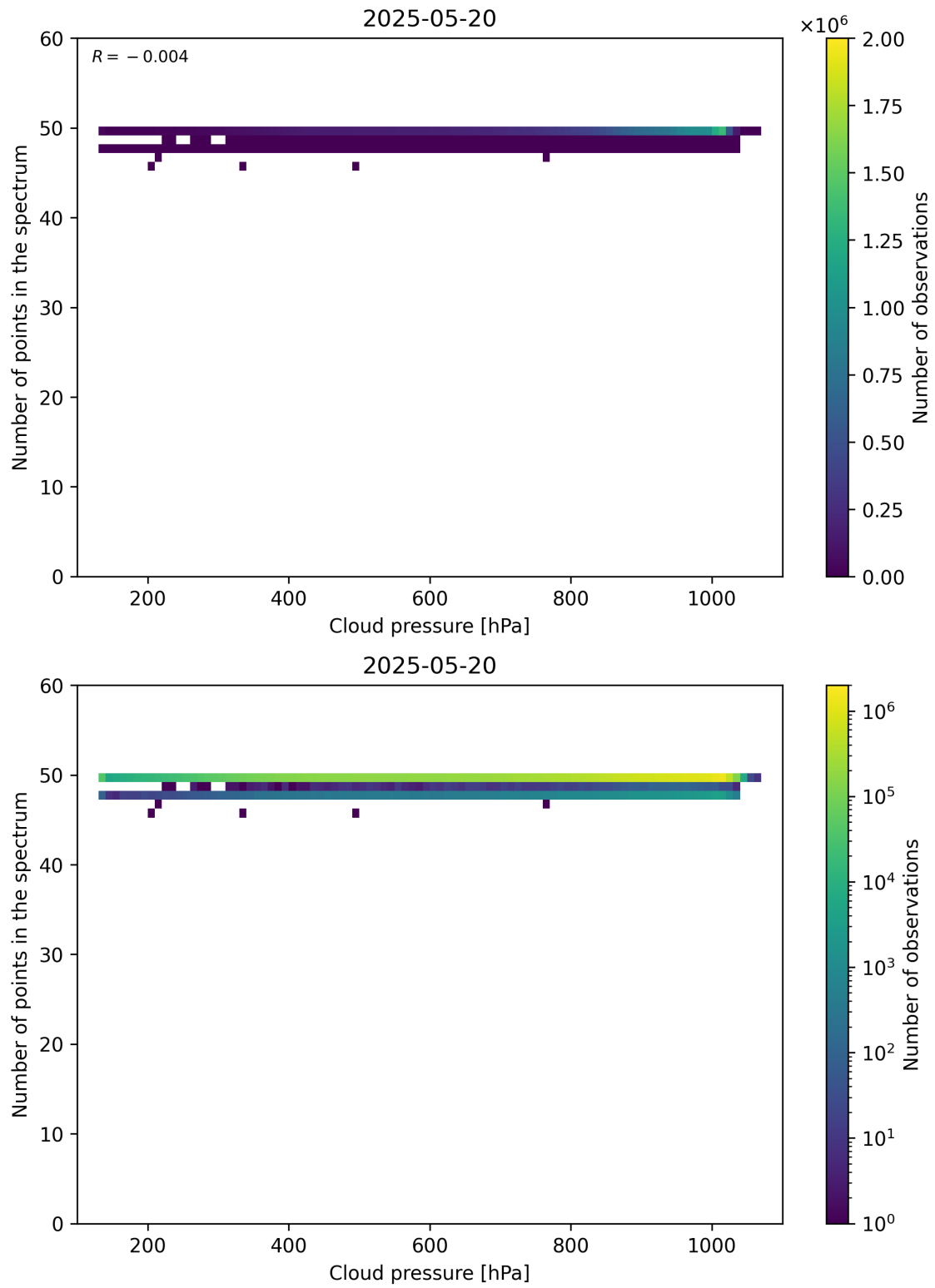
Figure 82: Scatter density plot of “Cloud pressure” against “Number of points in the spectrum” for 2025-05-19 to 2025-05-21.
