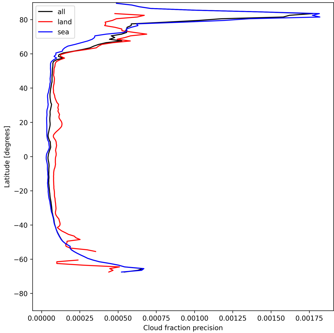
Figure 16: Zonal average of “Cloud fraction precision” for 2025-05-19 to 2025-05-21.
