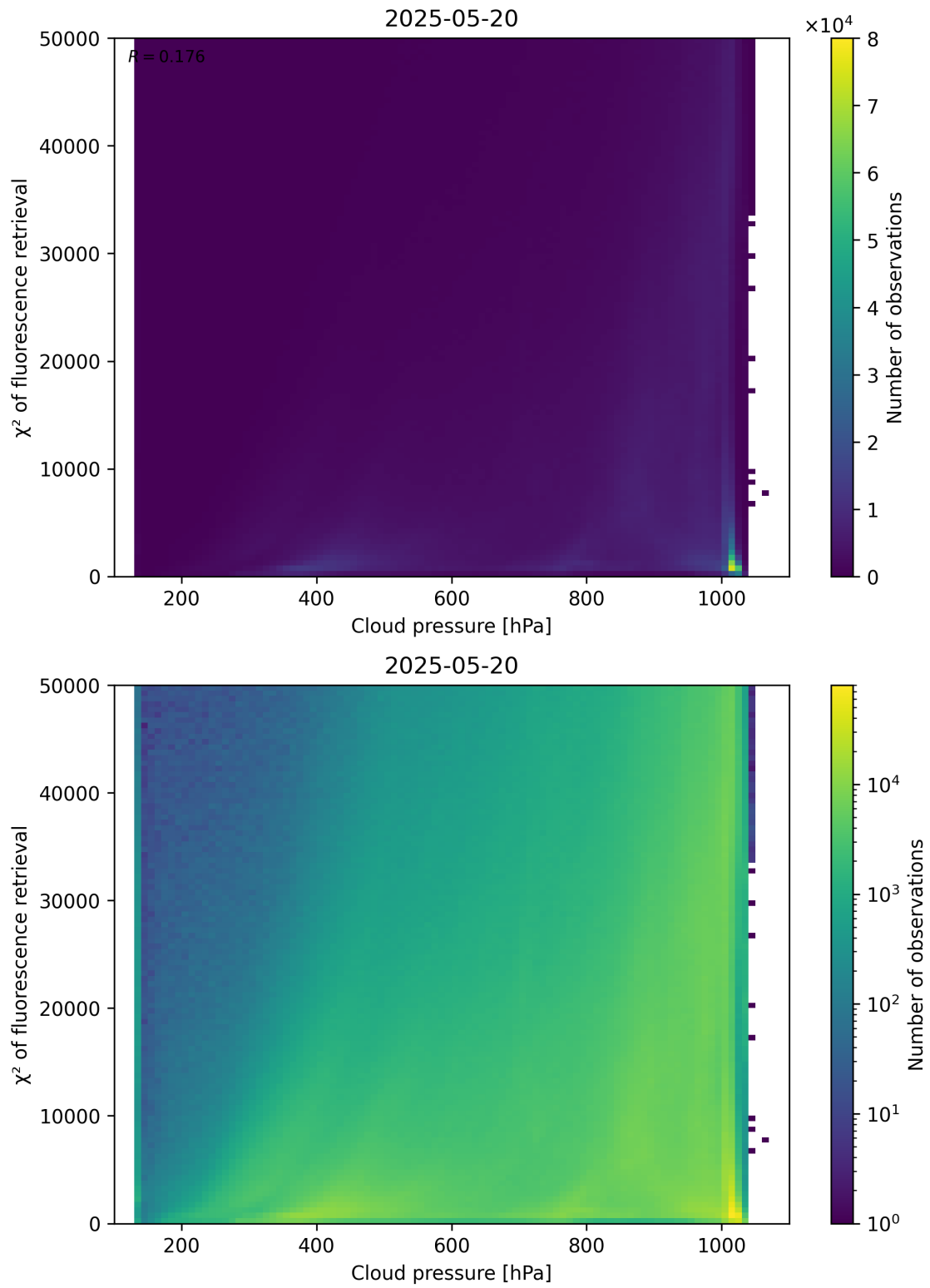
Figure 78: Scatter density plot of “Cloud pressure” against “ \chi^2 of fluorescence retrieval” for 2025-05-19 to 2025-05-21.
