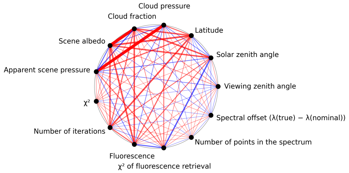
Figure 1: Map of correlation graph for 2025-05-19 to 2025-05-21.
