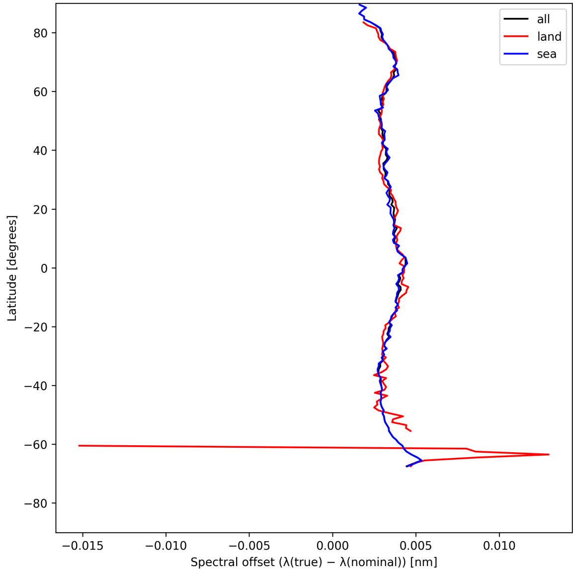
Figure 28: Zonal average of “Spectral offset ( \lambda_{\text{true}} - \lambda_{\text{nominal}} )” for 2025-05-19 to 2025-05-21.
