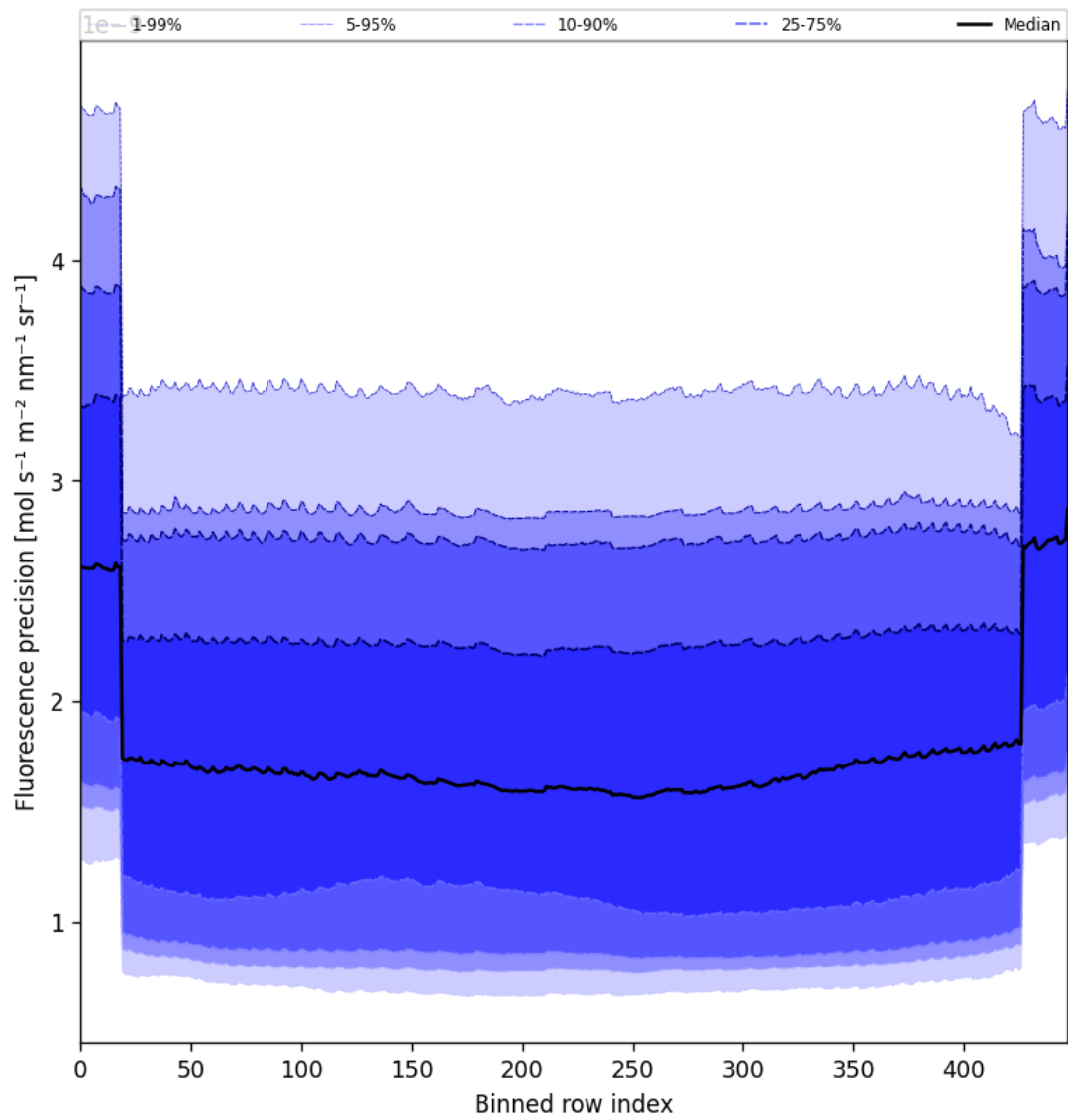
Figure 58: Along track statistics of “Fluorescence precision” for 2025-05-19 to 2025-05-21
