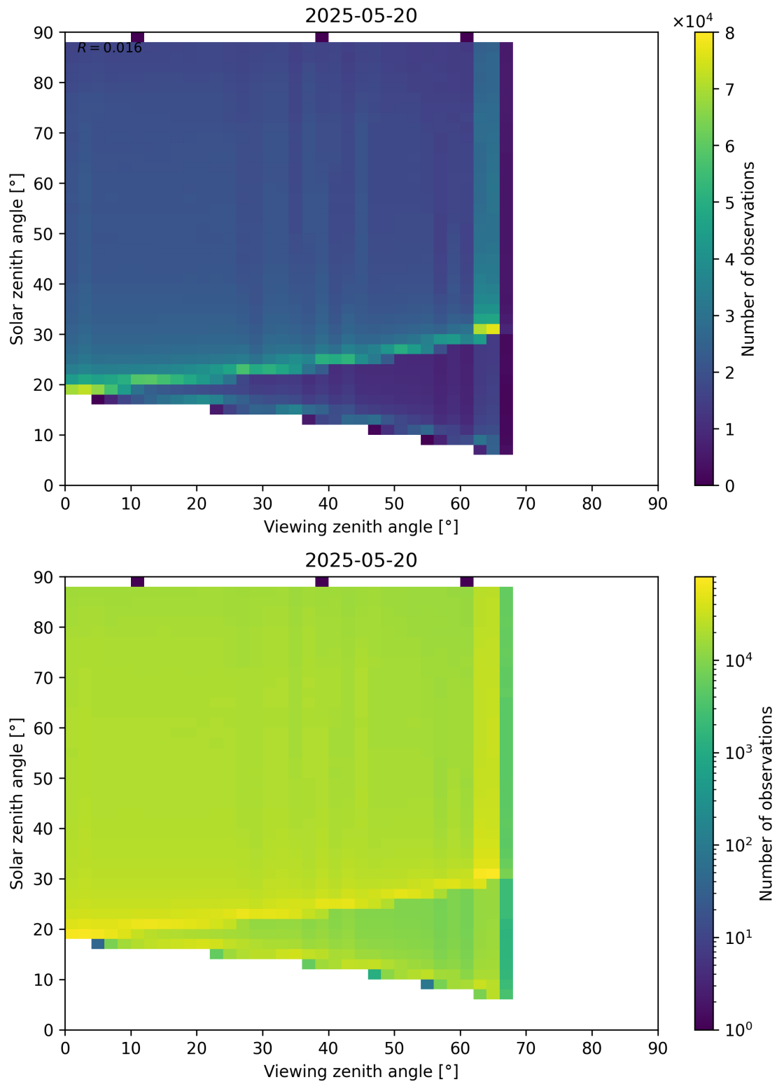
Figure 127: Scatter density plot of “Viewing zenith angle” against “Solar zenith angle” for 2025-05-19 to 2025-05-21.
