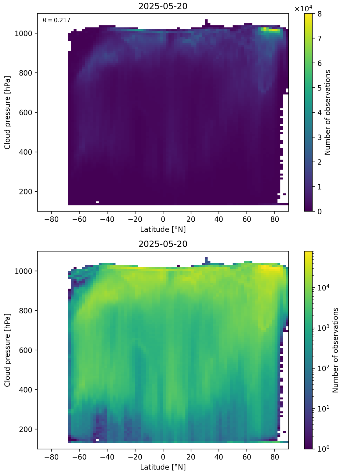
Figure 91: Scatter density plot of “Latitude” against “Cloud pressure” for 2025-05-19 to 2025-05-21.
