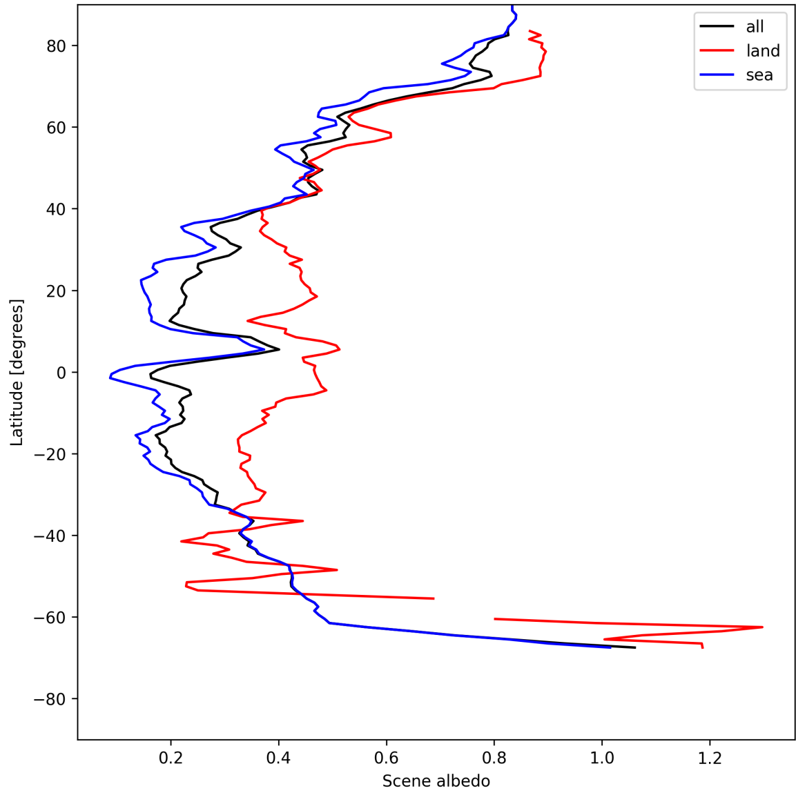
Figure 17: Zonal average of “Scene albedo” for 2025-05-19 to 2025-05-21.
