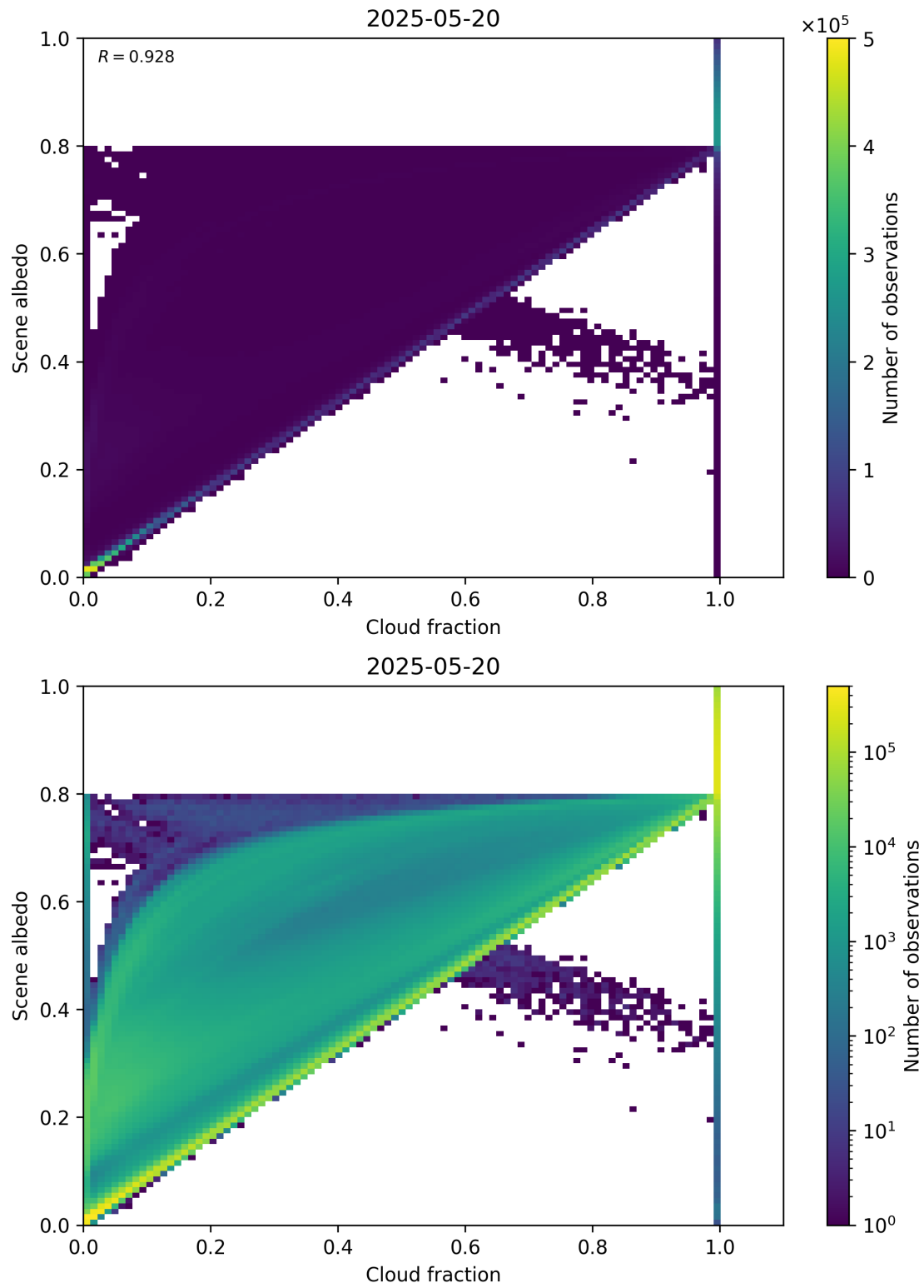
Figure 75: Scatter density plot of “Cloud fraction” against “Scene albedo” for 2025-05-19 to 2025-05-21.
