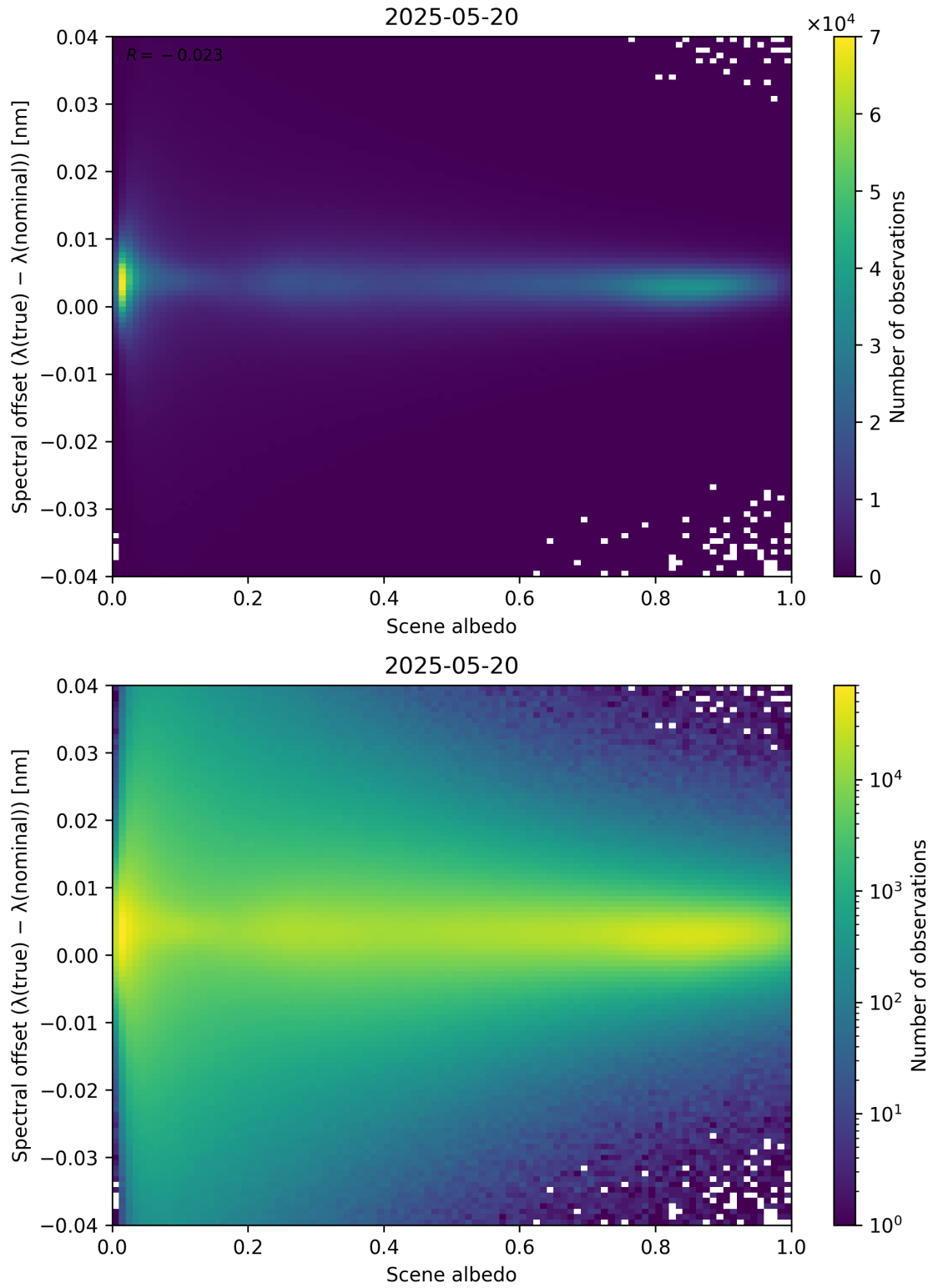
Figure 107: Scatter density plot of “Scene albedo” against “Spectral offset ( \lambda_{\text{true}} - \lambda_{\text{nominal}} )” for 2025-05-19 to 2025-05-21.
