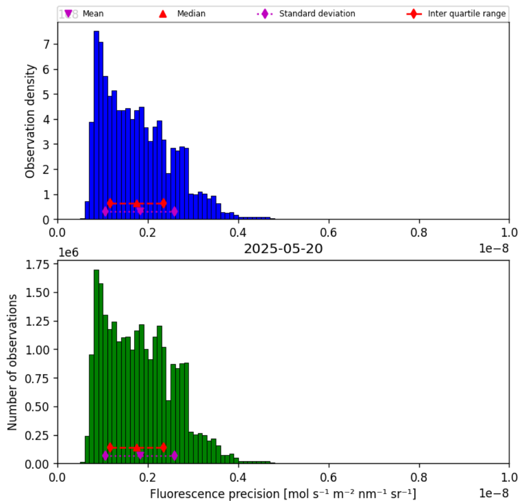
Figure 41: Histogram of “Fluorescence precision” for 2025-05-19 to 2025-05-21
