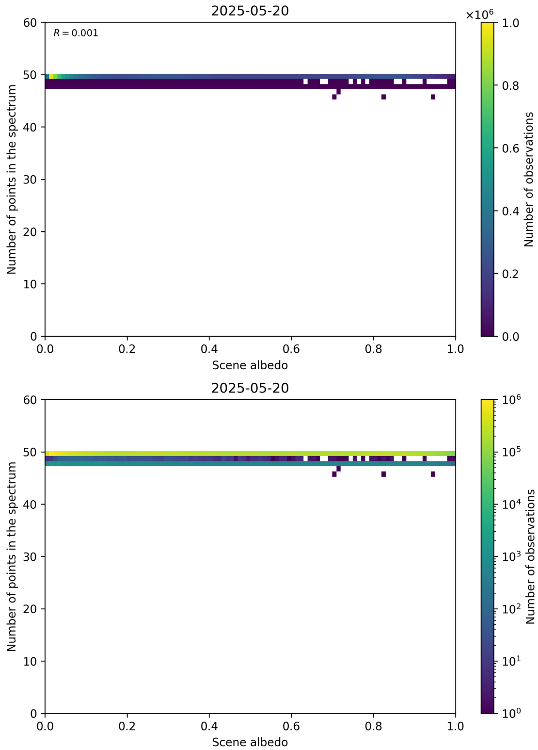
Figure 106: Scatter density plot of “Scene albedo” against “Number of points in the spectrum” for 2025-05-19 to 2025-05-21.
