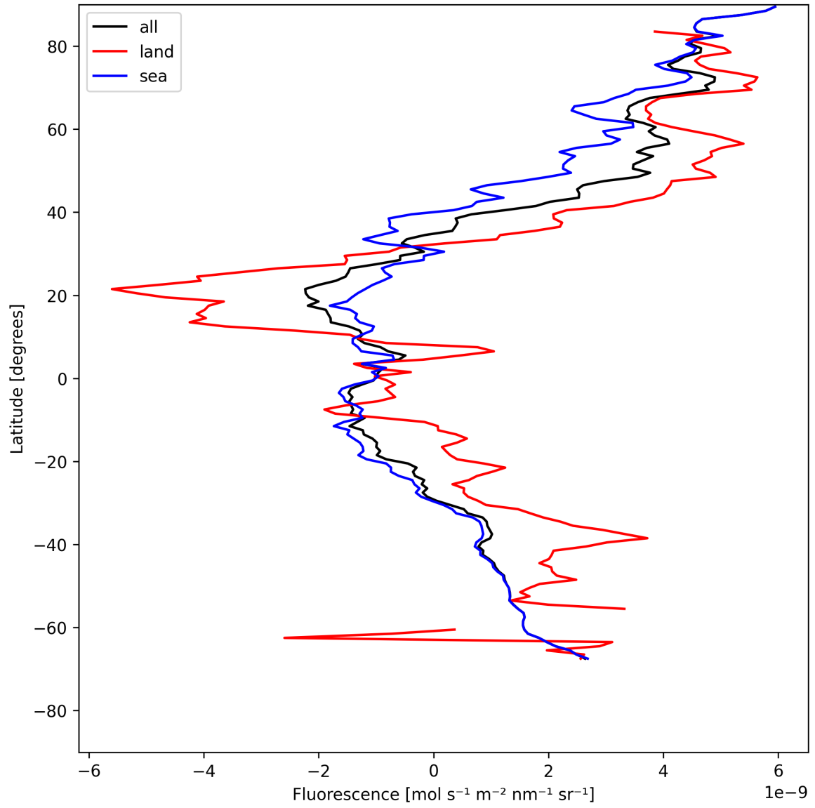
Figure 23: Zonal average of “Fluorescence” for 2025-05-19 to 2025-05-21.
