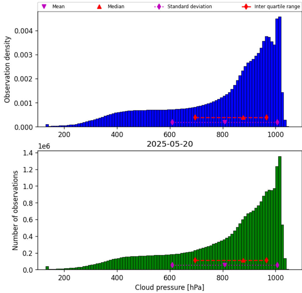
Figure 30: Histogram of “Cloud pressure” for 2025-05-19 to 2025-05-21
