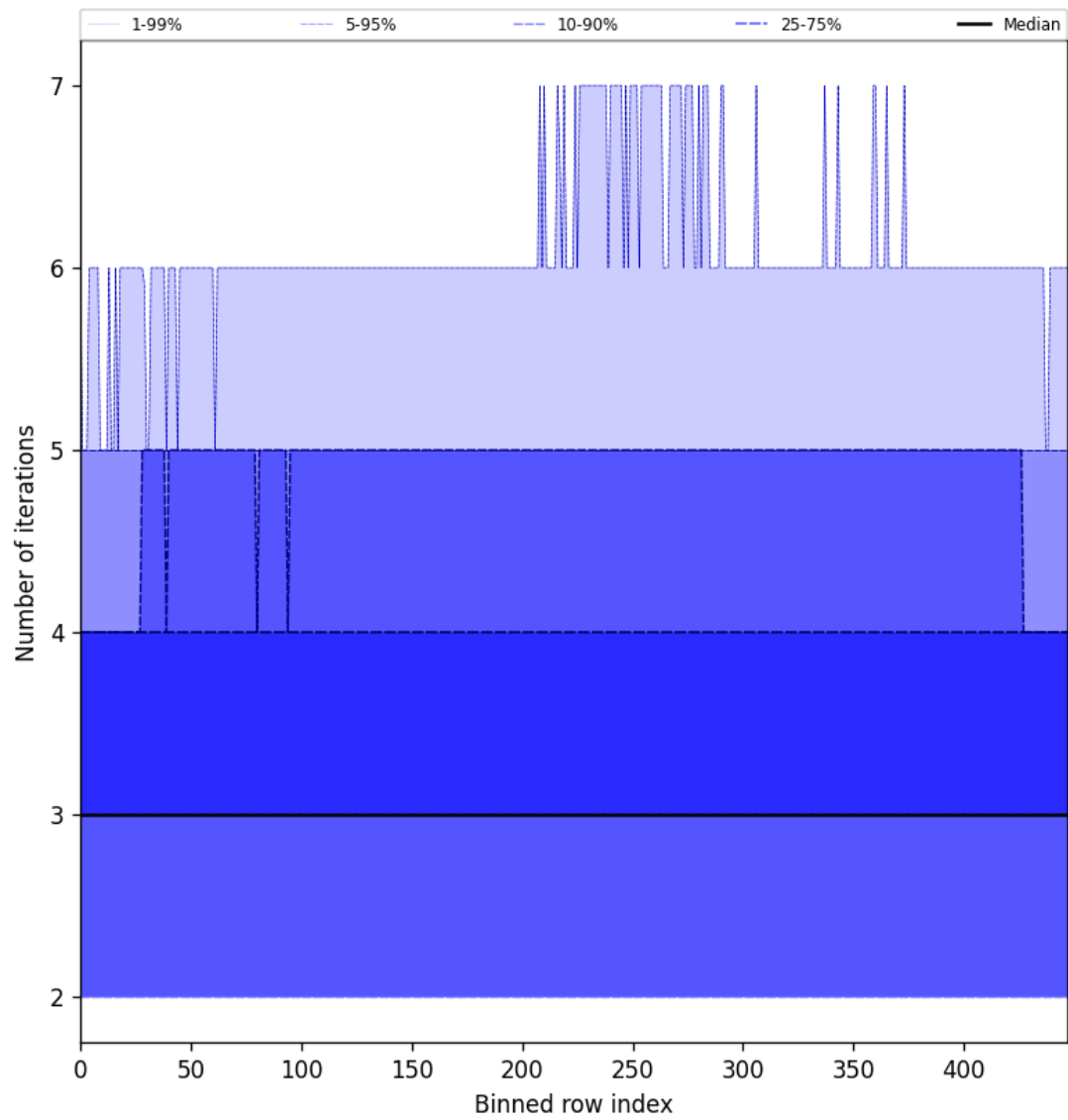
Figure 56: Along track statistics of “Number of iterations” for 2025-05-19 to 2025-05-21
