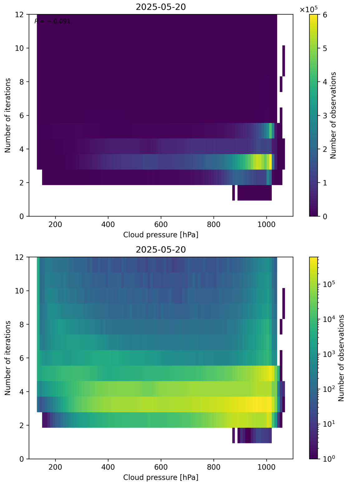
Figure 81: Scatter density plot of “Cloud pressure” against “Number of iterations” for 2025-05-19 to 2025-05-21.
