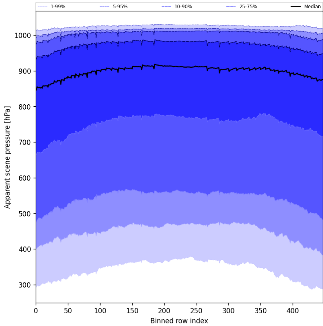
Figure 53: Along track statistics of “Apparent scene pressure” for 2025-05-19 to 2025-05-21
