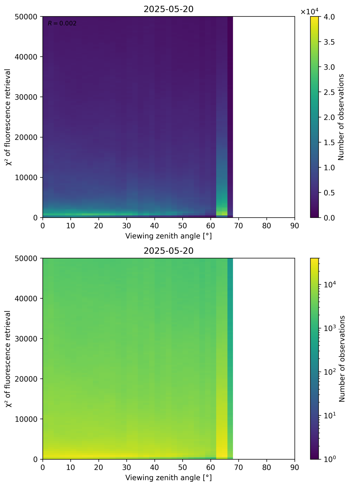
Figure 119: Scatter density plot of “Viewing zenith angle” against “ \chi^2 of fluorescence retrieval” for 2025-05-19 to 2025-05-21.
