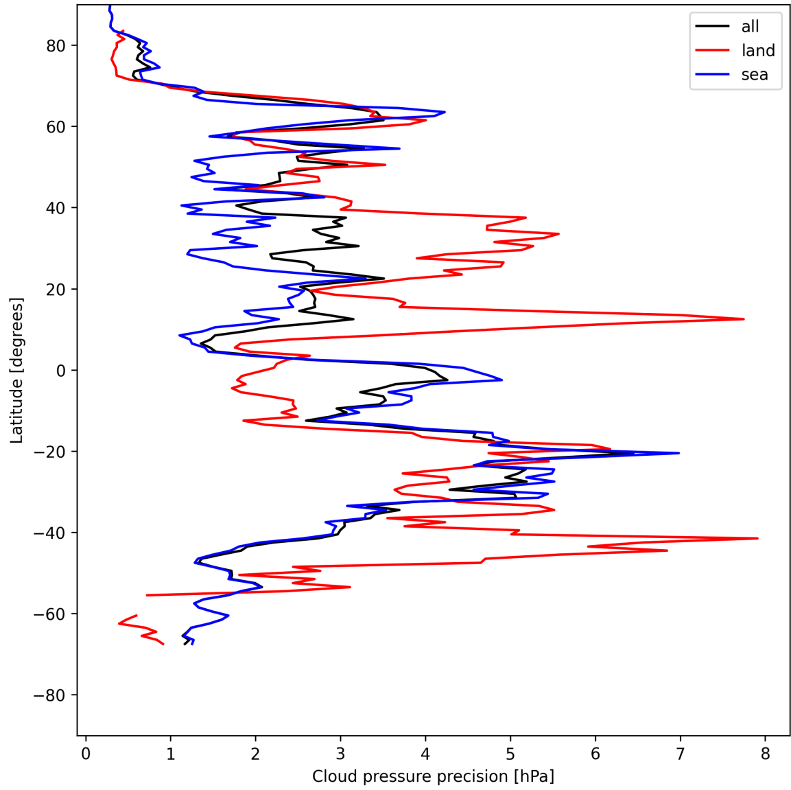
Figure 14: Zonal average of “Cloud pressure precision” for 2025-05-19 to 2025-05-21.
