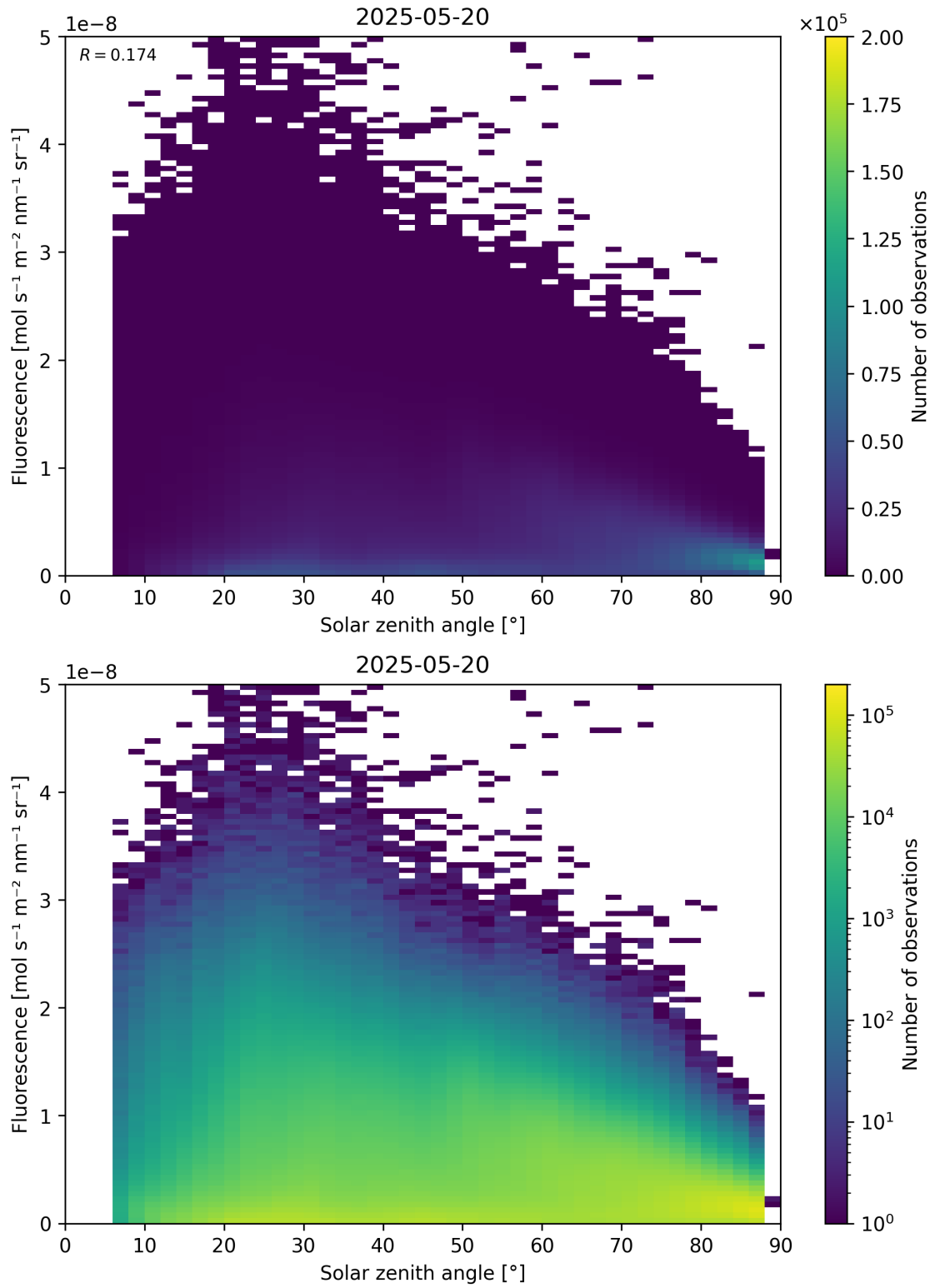
Figure 112: Scatter density plot of “Solar zenith angle” against “Fluorescence” for 2025-05-19 to 2025-05-21.
