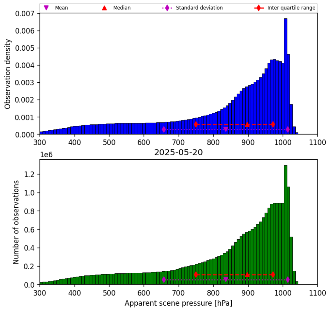
Figure 36: Histogram of “Apparent scene pressure” for 2025-05-19 to 2025-05-21
