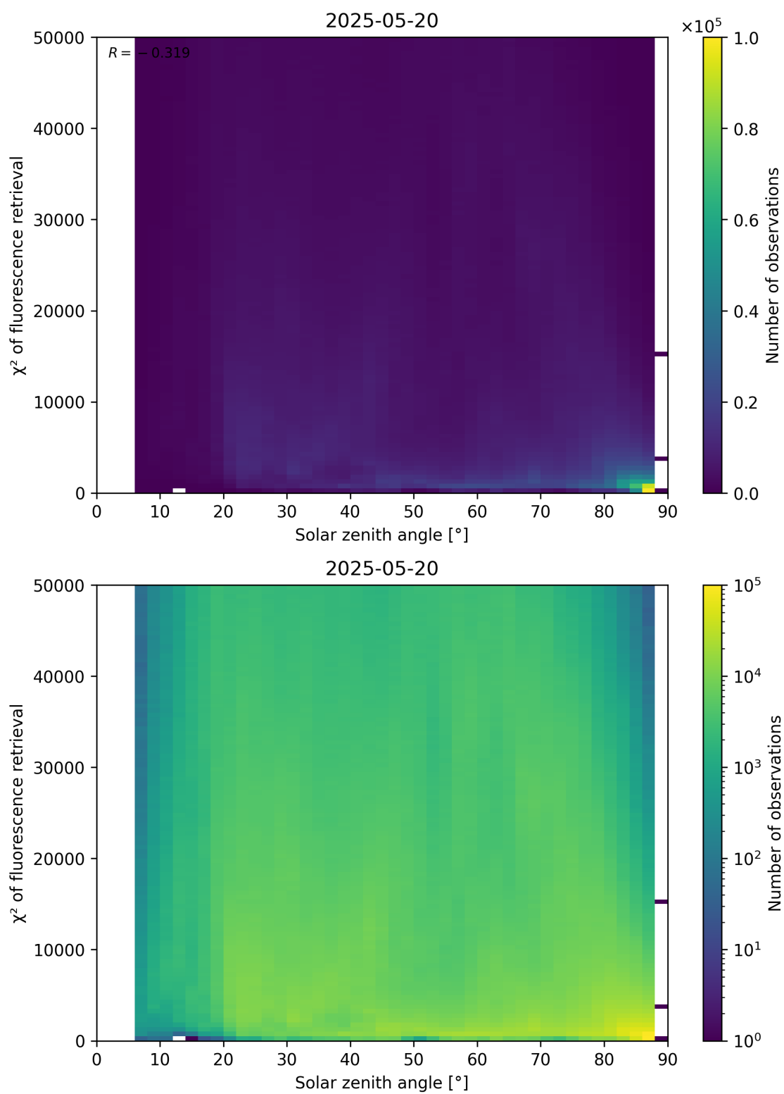
Figure 109: Scatter density plot of “Solar zenith angle” against “ \chi^2 of fluorescence retrieval” for 2025-05-19 to 2025-05-21.
