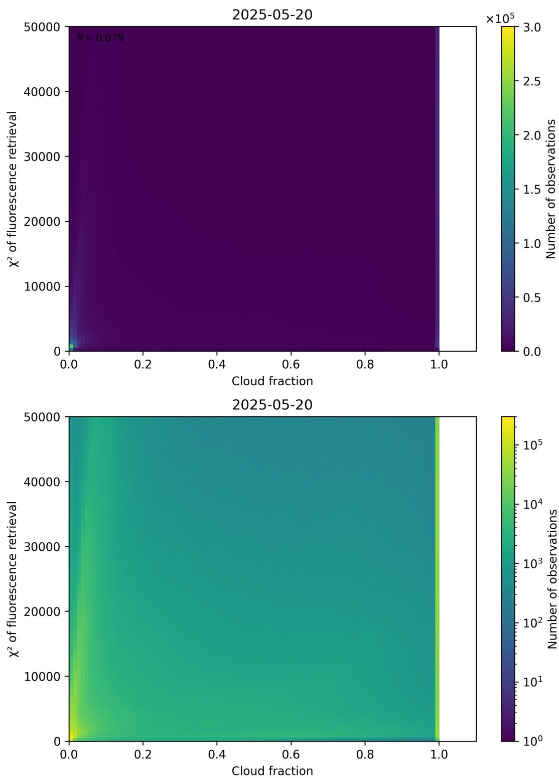
Figure 71: Scatter density plot of “Cloud fraction” against “ \chi^2 of fluorescence retrieval” for 2025-05-19 to 2025-05-21.
