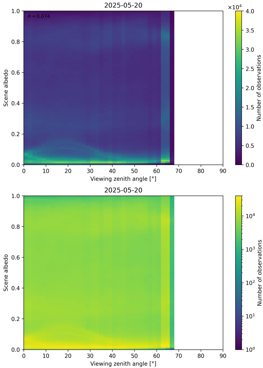
Figure 126: Scatter density plot of “Viewing zenith angle” against “Scene albedo” for 2025-05-19 to 2025-05-21.
