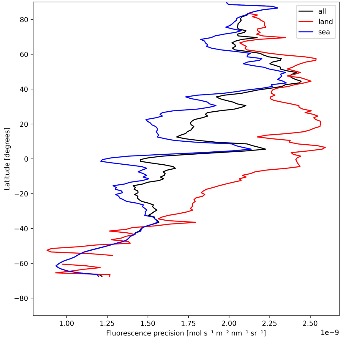
Figure 24: Zonal average of “Fluorescence precision” for 2025-05-19 to 2025-05-21.
