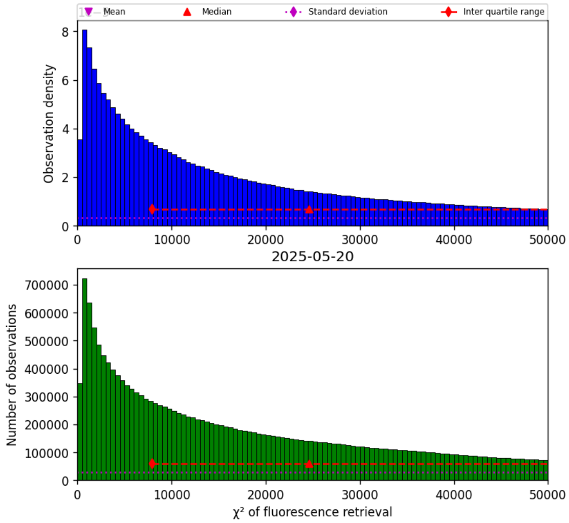
Figure 42: Histogram of “ \chi^2 of fluorescence retrieval” for 2025-05-19 to 2025-05-21
