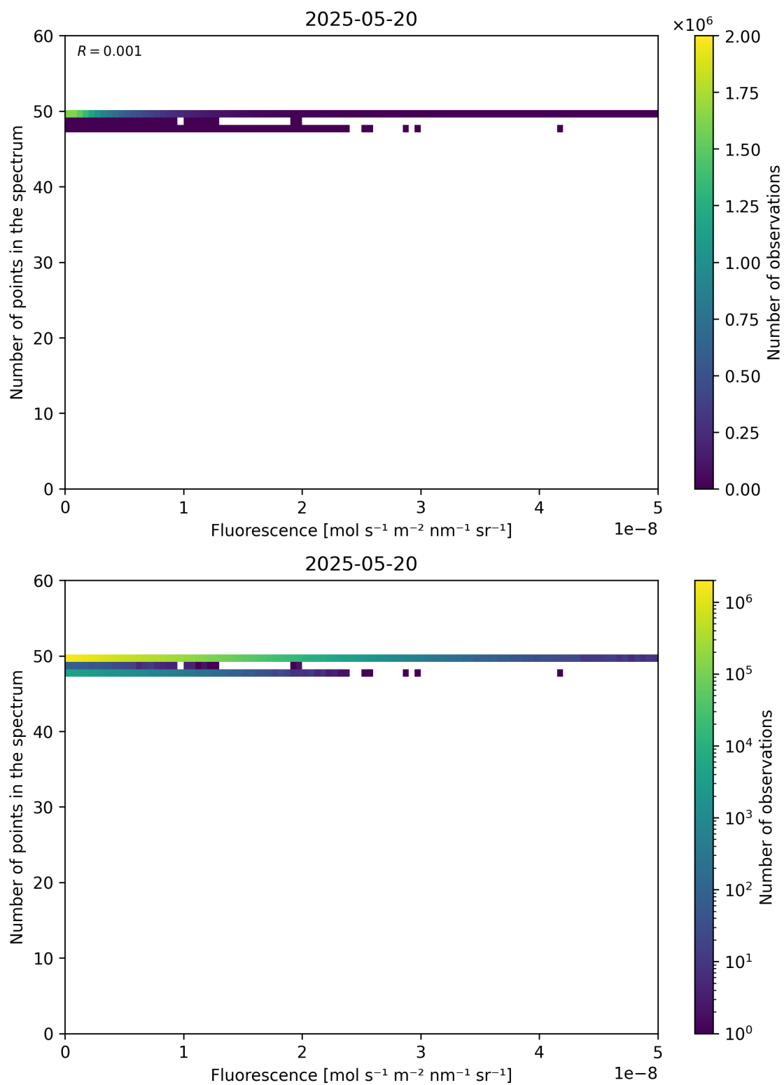
Figure 86: Scatter density plot of “Fluorescence” against “Number of points in the spectrum” for 2025-05-19 to 2025-05-21.
