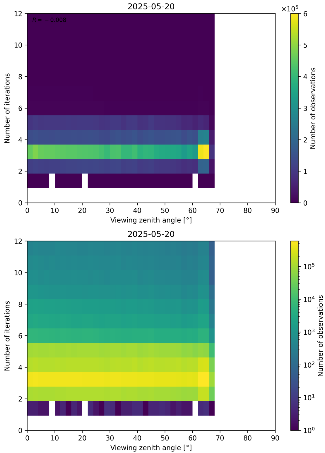
Figure 124: Scatter density plot of “Viewing zenith angle” against “Number of iterations” for 2025-05-19 to 2025-05-21.
