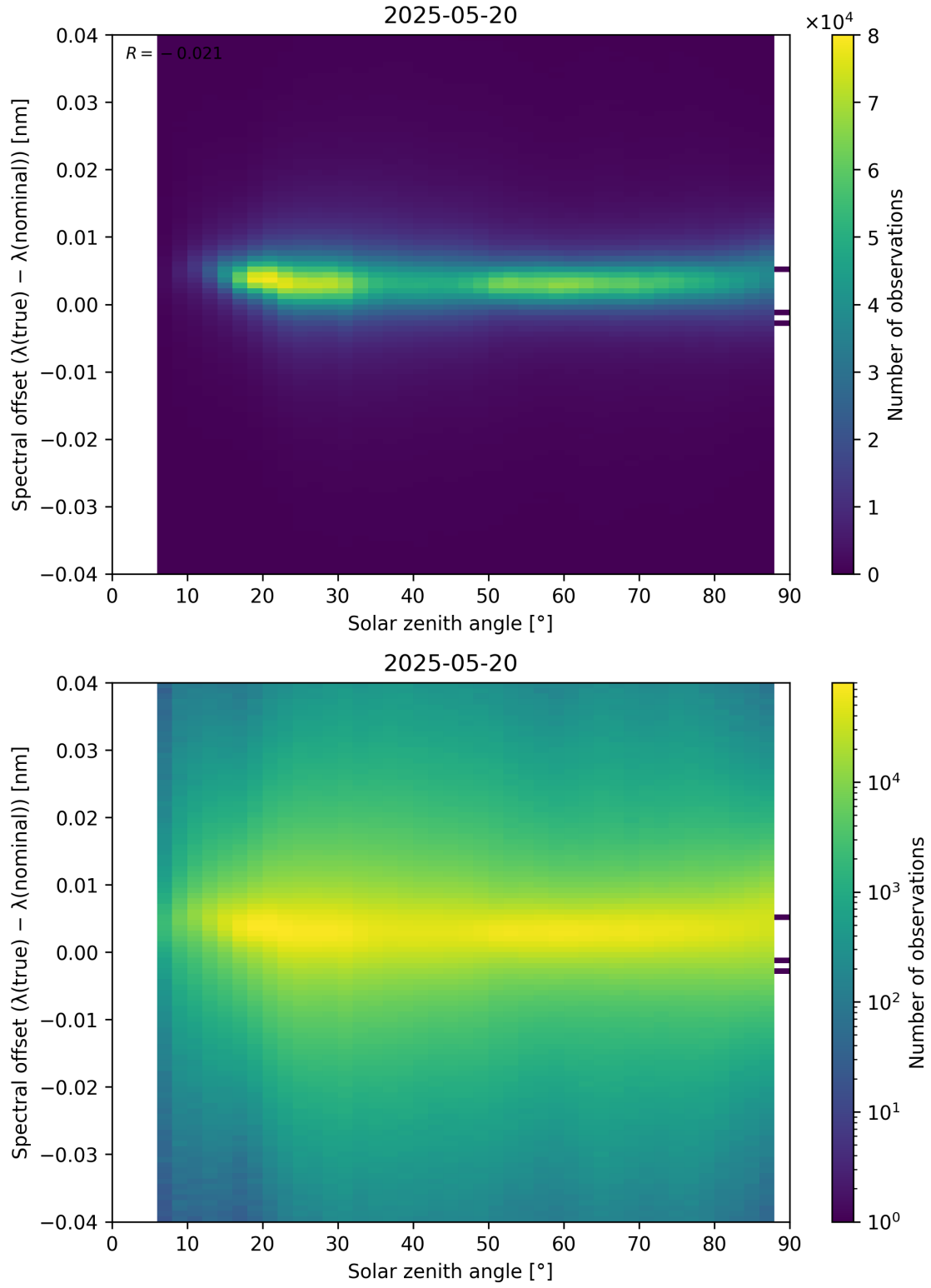
Figure 117: Scatter density plot of “Solar zenith angle” against “Spectral offset ( \lambda_{\text{true}} - \lambda_{\text{nominal}} )” for 2025-05-19 to 2025-05-21.
