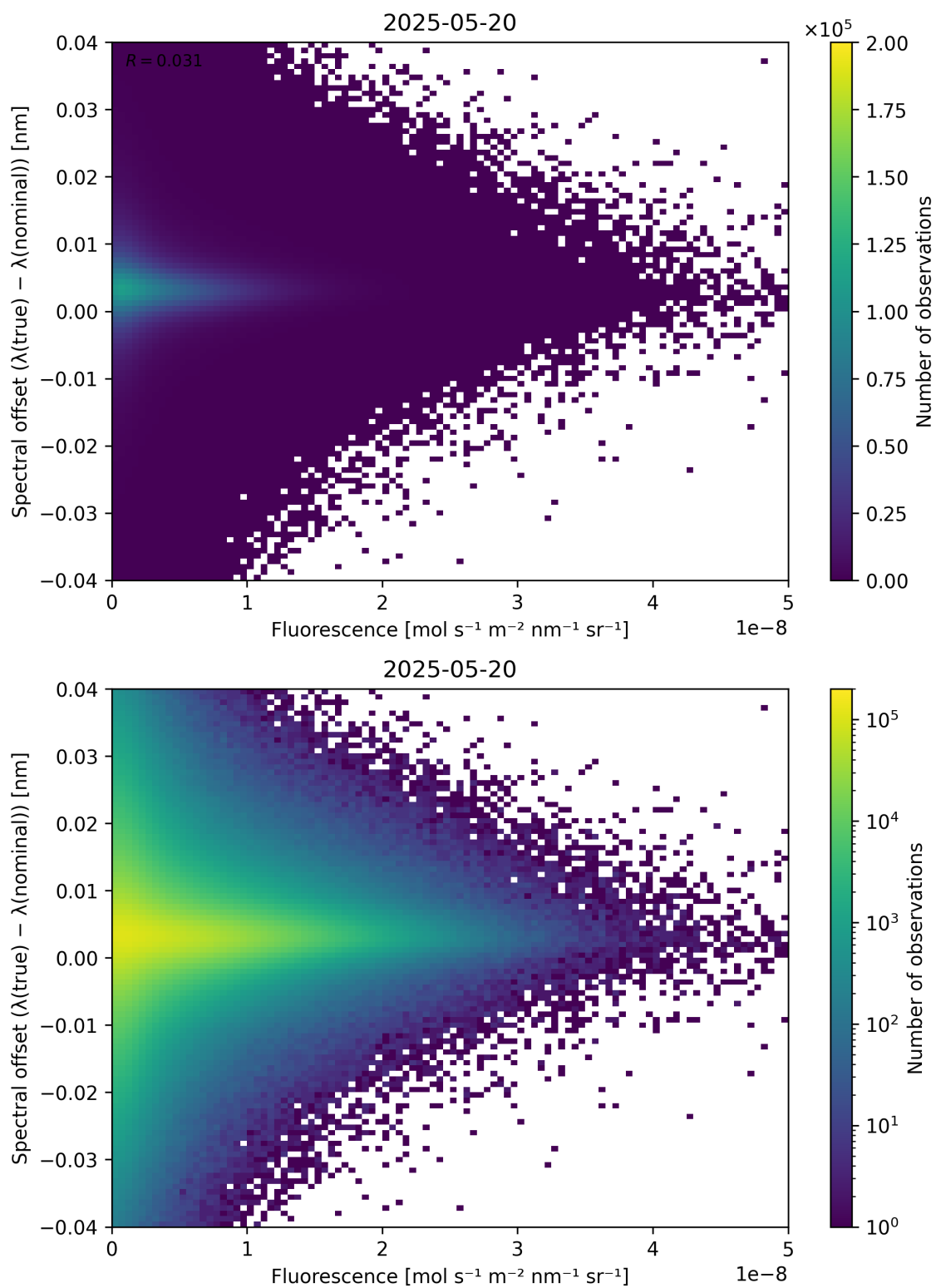
Figure 87: Scatter density plot of “Fluorescence” against “Spectral offset ( \lambda_{\text{true}} - \lambda_{\text{nominal}} )” for 2025-05-19 to 2025-05-21.
