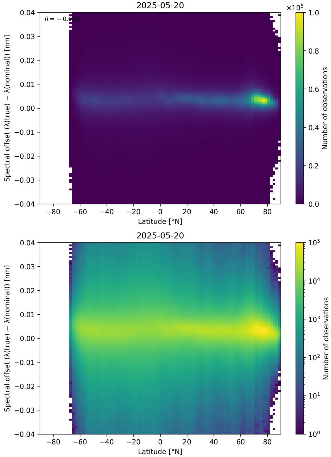
Figure 96: Scatter density plot of “Latitude” against “Spectral offset ( \lambda_{\text{true}} - \lambda_{\text{nominal}} )” for 2025-05-19 to 2025-05-21.
