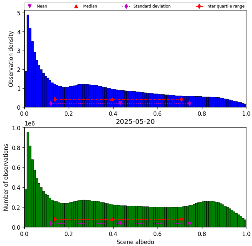
Figure 34: Histogram of “Scene albedo” for 2025-05-19 to 2025-05-21
