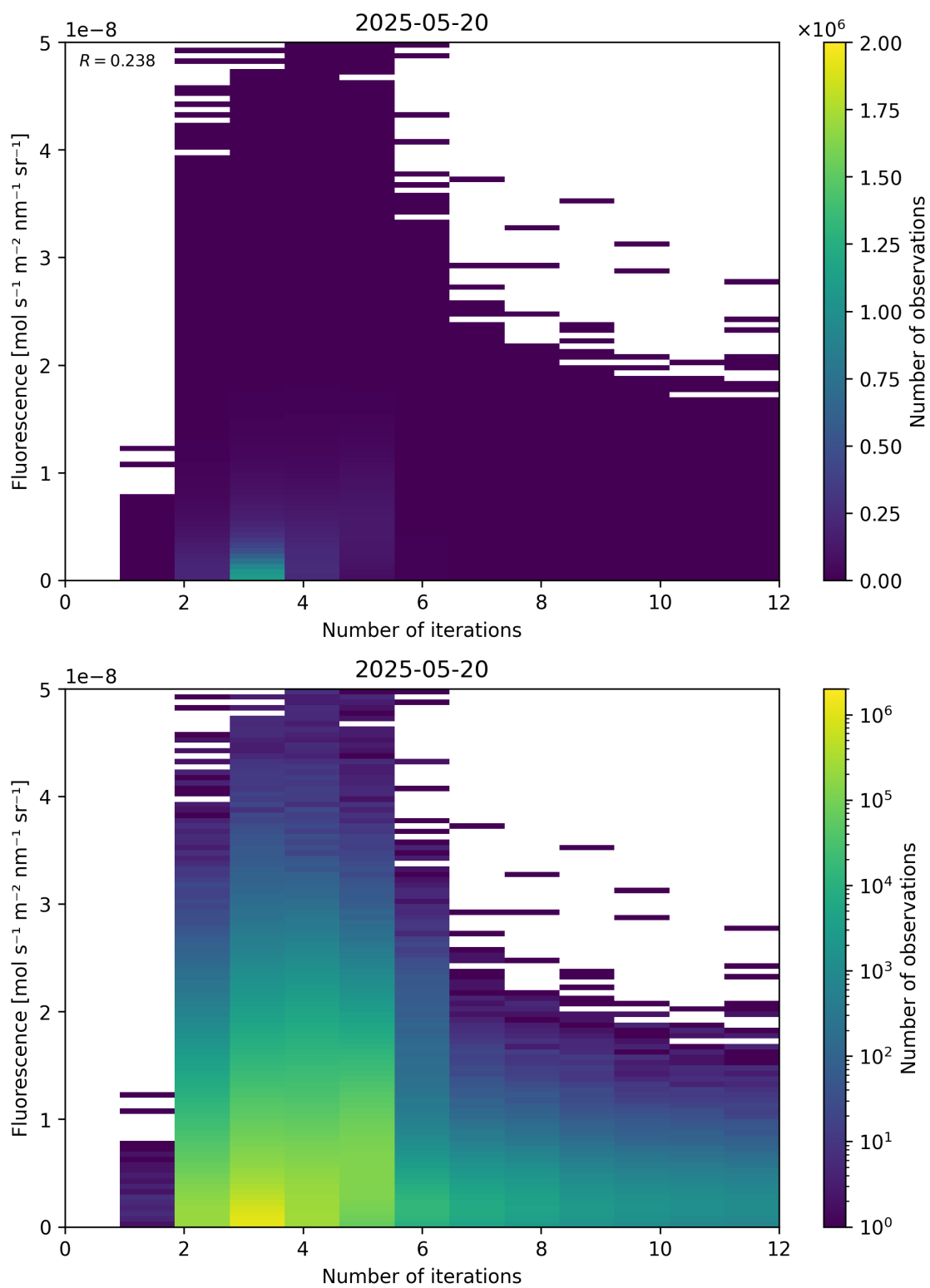
Figure 98: Scatter density plot of “Number of iterations” against “Fluorescence” for 2025-05-19 to 2025-05-21.
