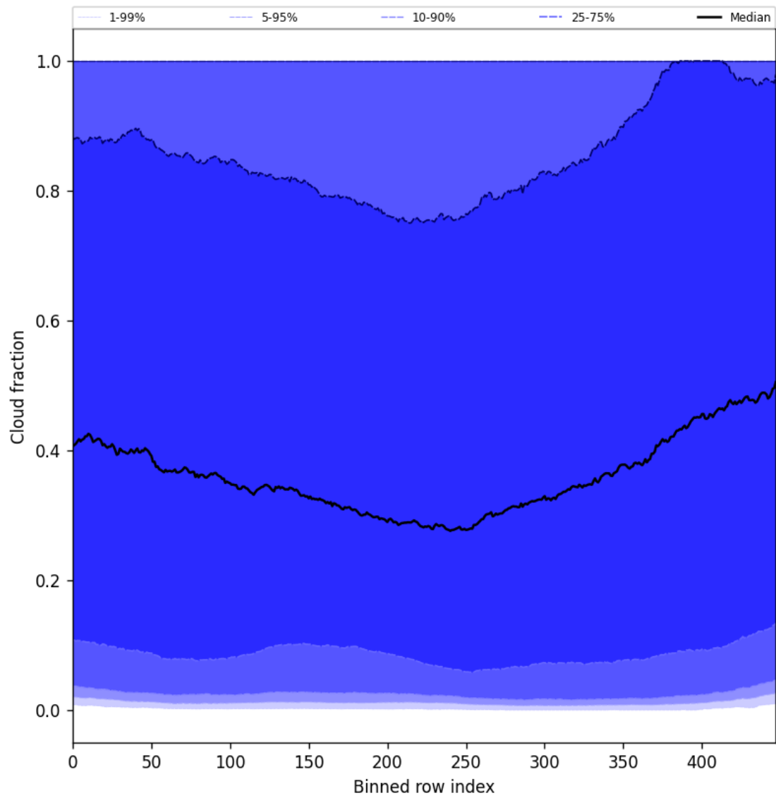
Figure 49: Along track statistics of “Cloud fraction” for 2025-05-19 to 2025-05-21
