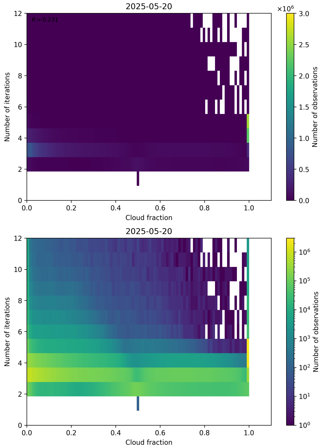
Figure 73: Scatter density plot of “Cloud fraction” against “Number of iterations” for 2025-05-19 to 2025-05-21.
