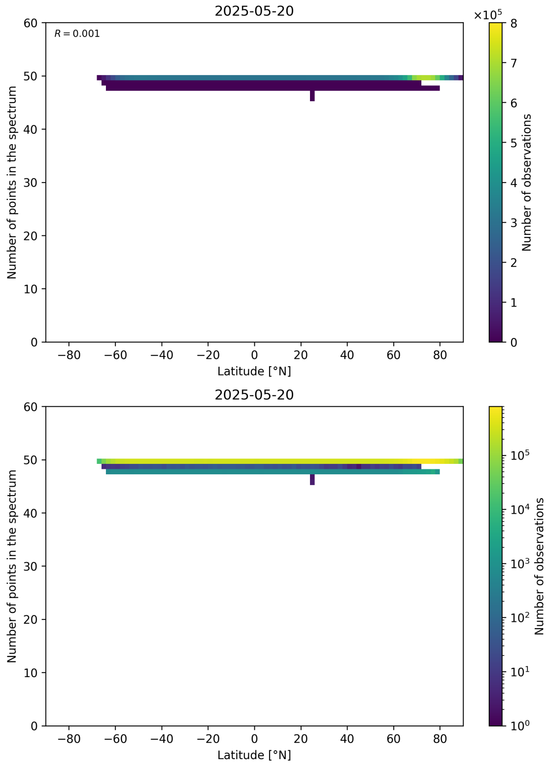
Figure 94: Scatter density plot of “Latitude” against “Number of points in the spectrum” for 2025-05-19 to 2025-05-21.
