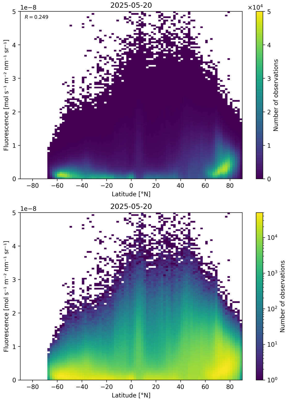
Figure 92: Scatter density plot of “Latitude” against “Fluorescence” for 2025-05-19 to 2025-05-21.
