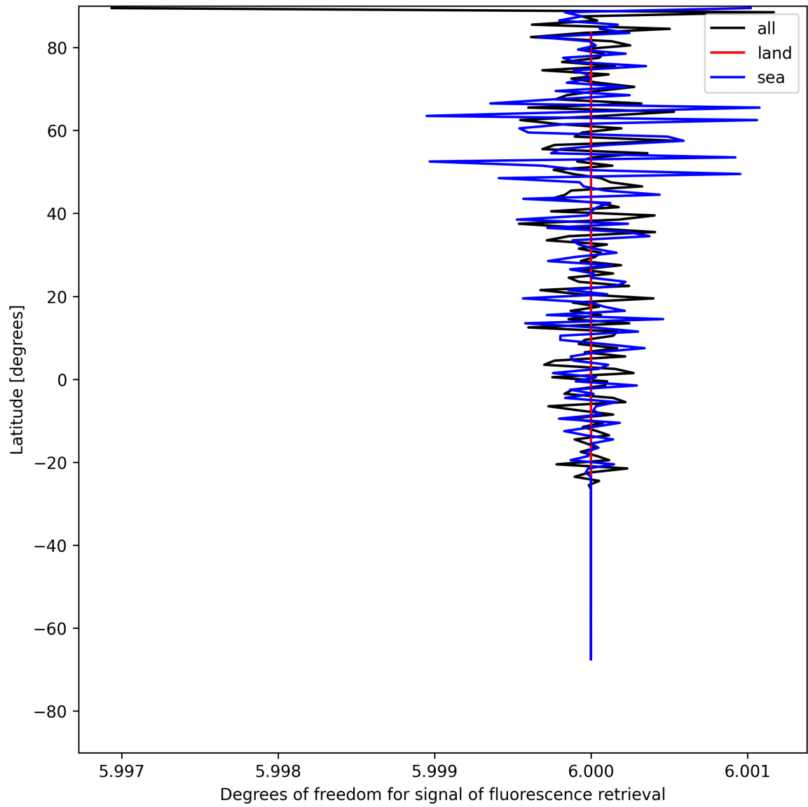
Figure 26: Zonal average of “Degrees of freedom for signal of fluorescence retrieval” for 2025-05-19 to 2025-05-21.
