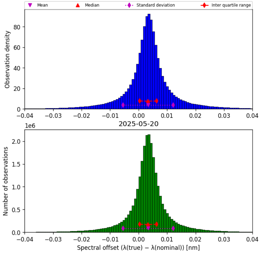
Figure 45: Histogram of “Spectral offset ( \lambda_{\text{true}} - \lambda_{\text{nominal}} )” for 2025-05-19 to 2025-05-21
