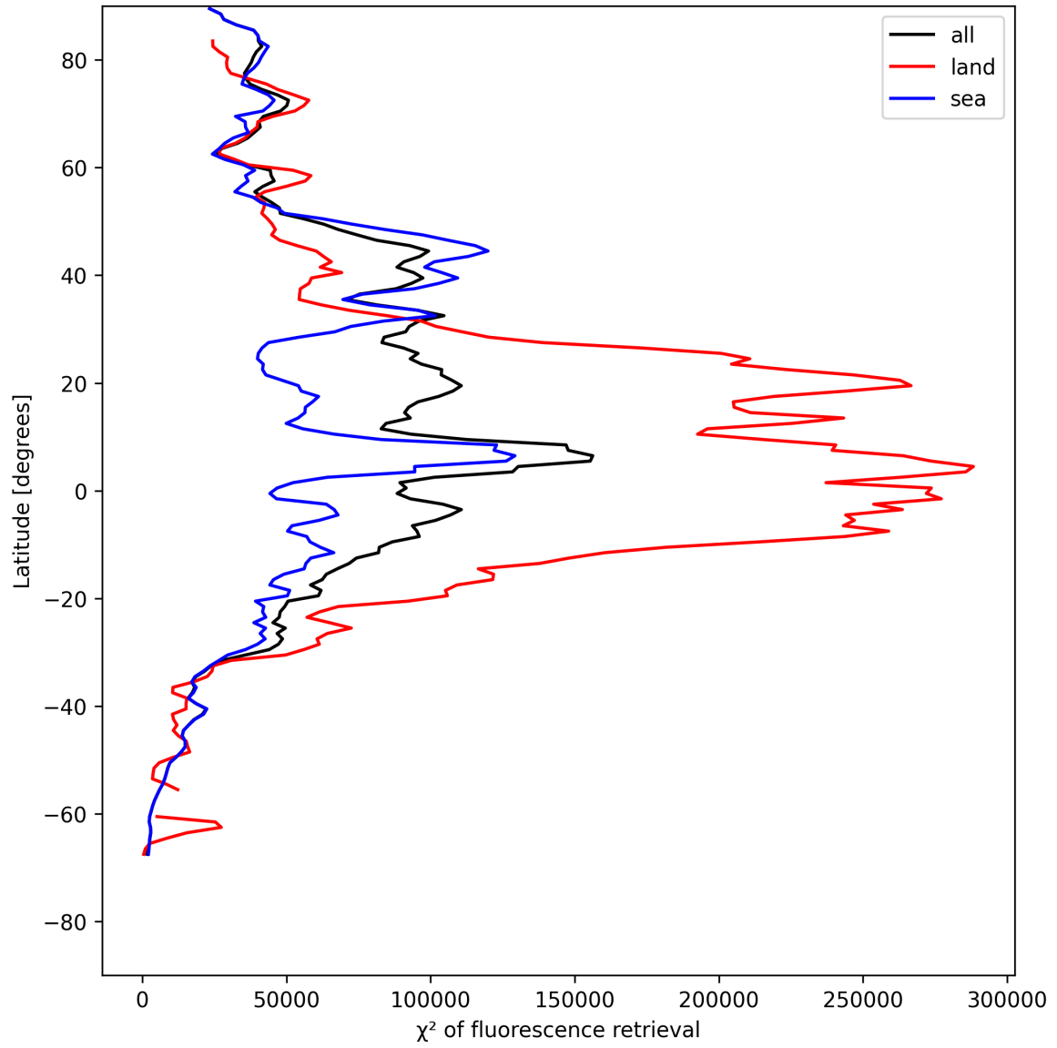
Figure 25: Zonal average of “ \chi^2 of fluorescence retrieval” for 2025-05-19 to 2025-05-21.
