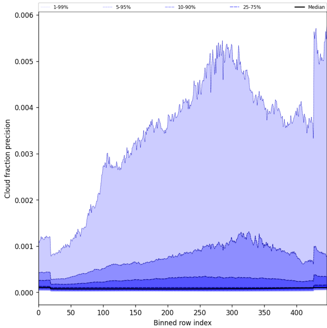
Figure 50: Along track statistics of “Cloud fraction precision” for 2025-05-19 to 2025-05-21
