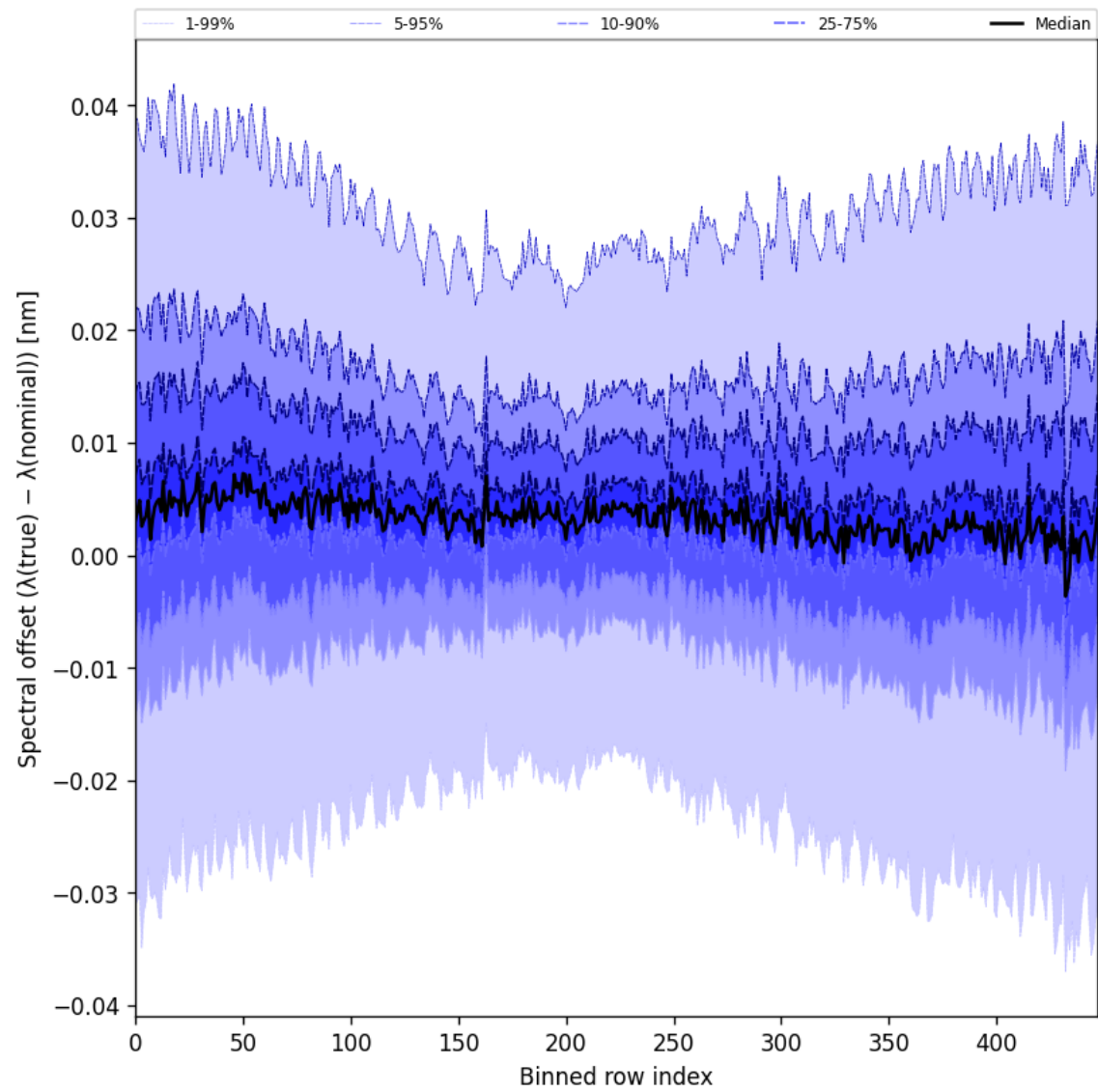
Figure 62: Along track statistics of “Spectral offset ( \lambda_{\text{true}} - \lambda_{\text{nominal}} )” for 2025-05-19 to 2025-05-21
