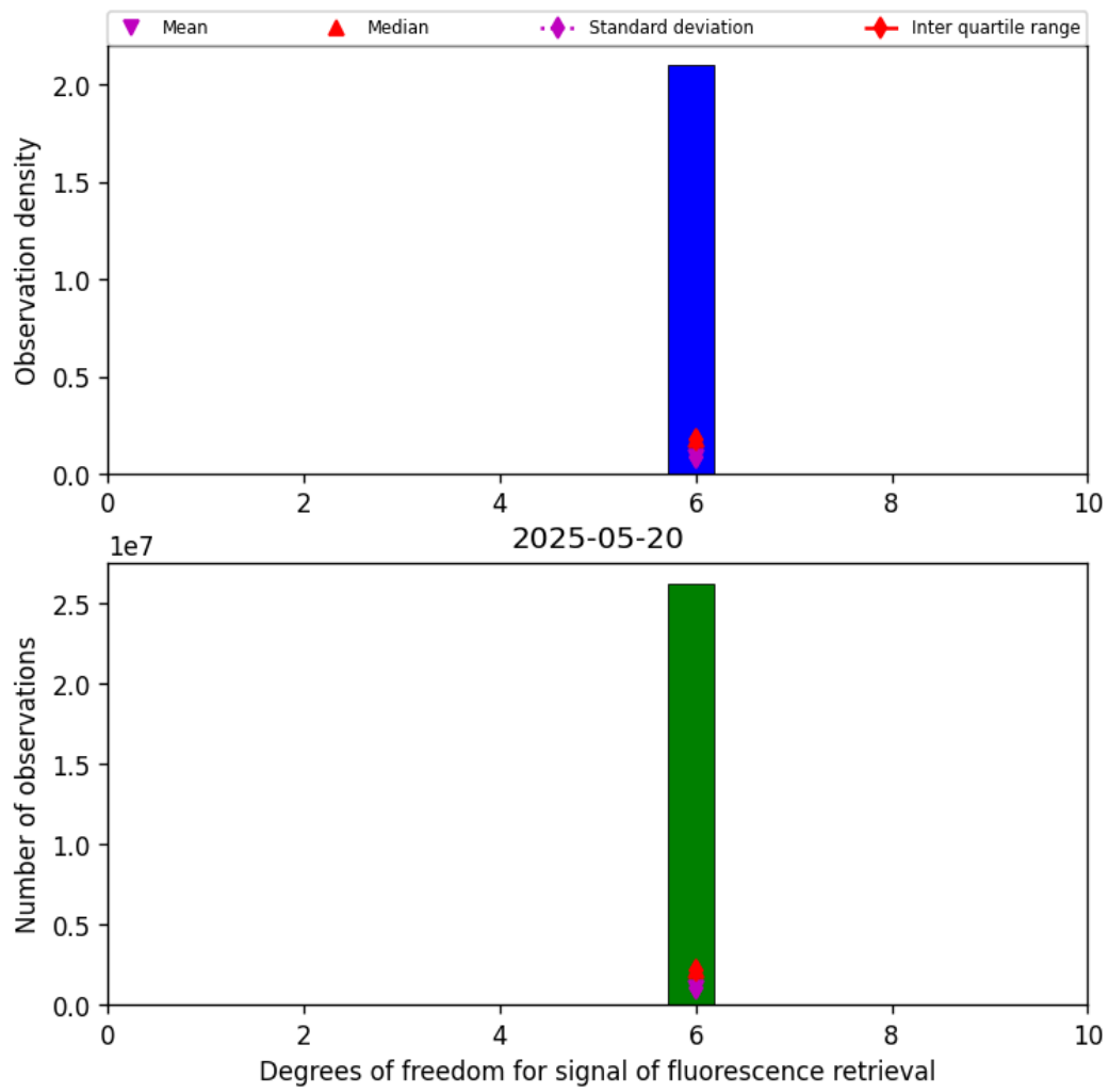
Figure 43: Histogram of "Degrees of freedom for signal of fluorescence retrieval" for 2025-05-19 to 2025-05-21
