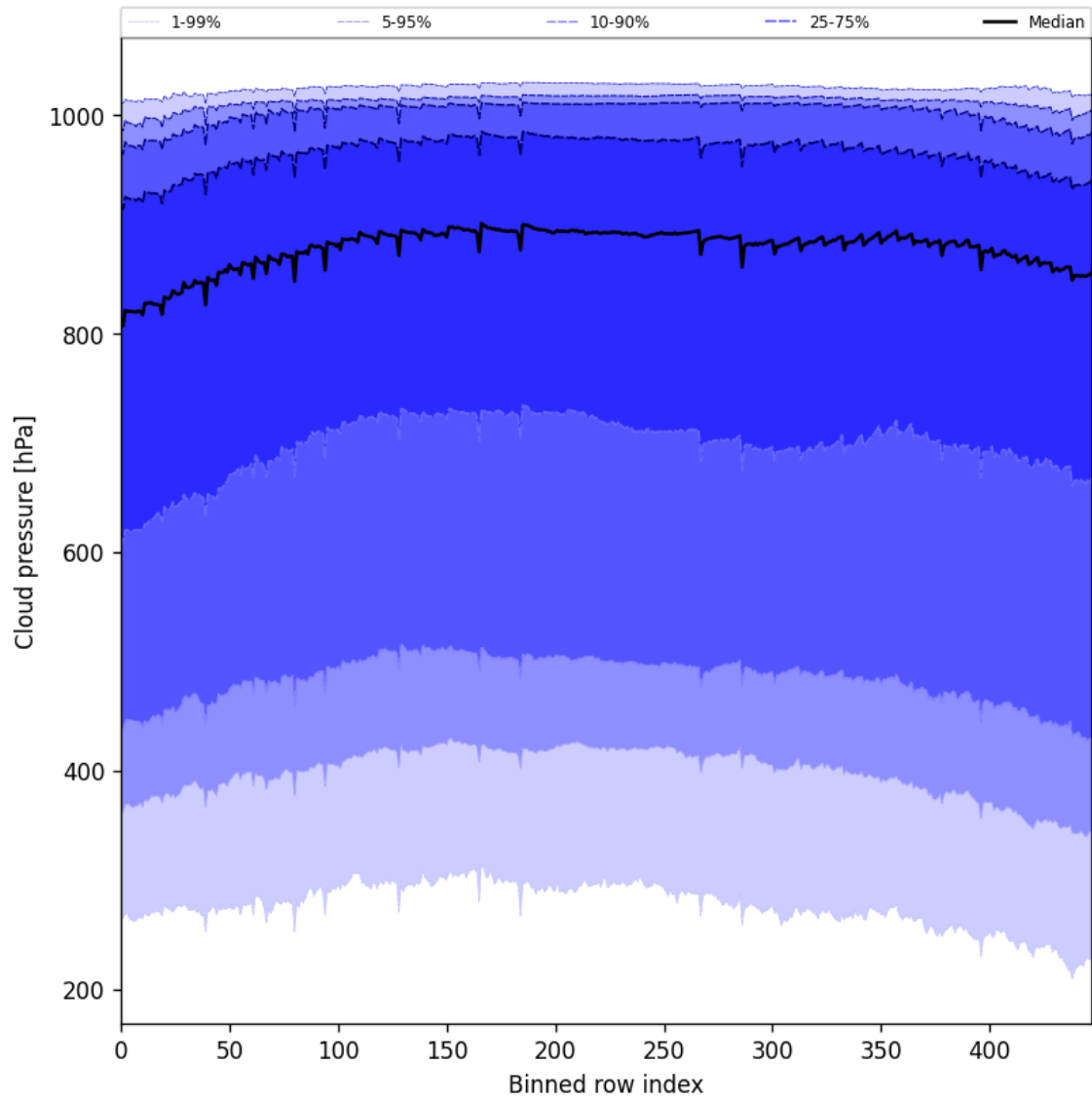
Figure 47: Along track statistics of “Cloud pressure” for 2025-05-19 to 2025-05-21
