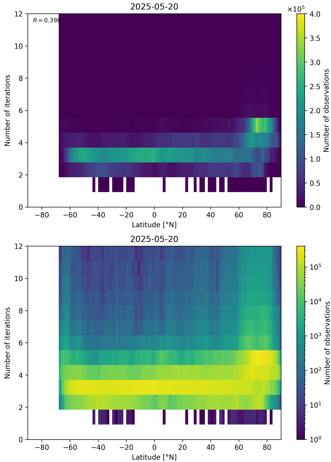
Figure 93: Scatter density plot of “Latitude” against “Number of iterations” for 2025-05-19 to 2025-05-21.
