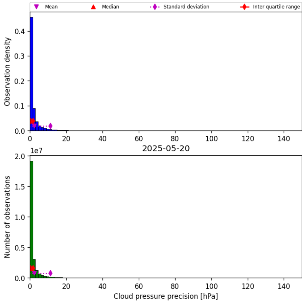
Figure 31: Histogram of “Cloud pressure precision” for 2025-05-19 to 2025-05-21
