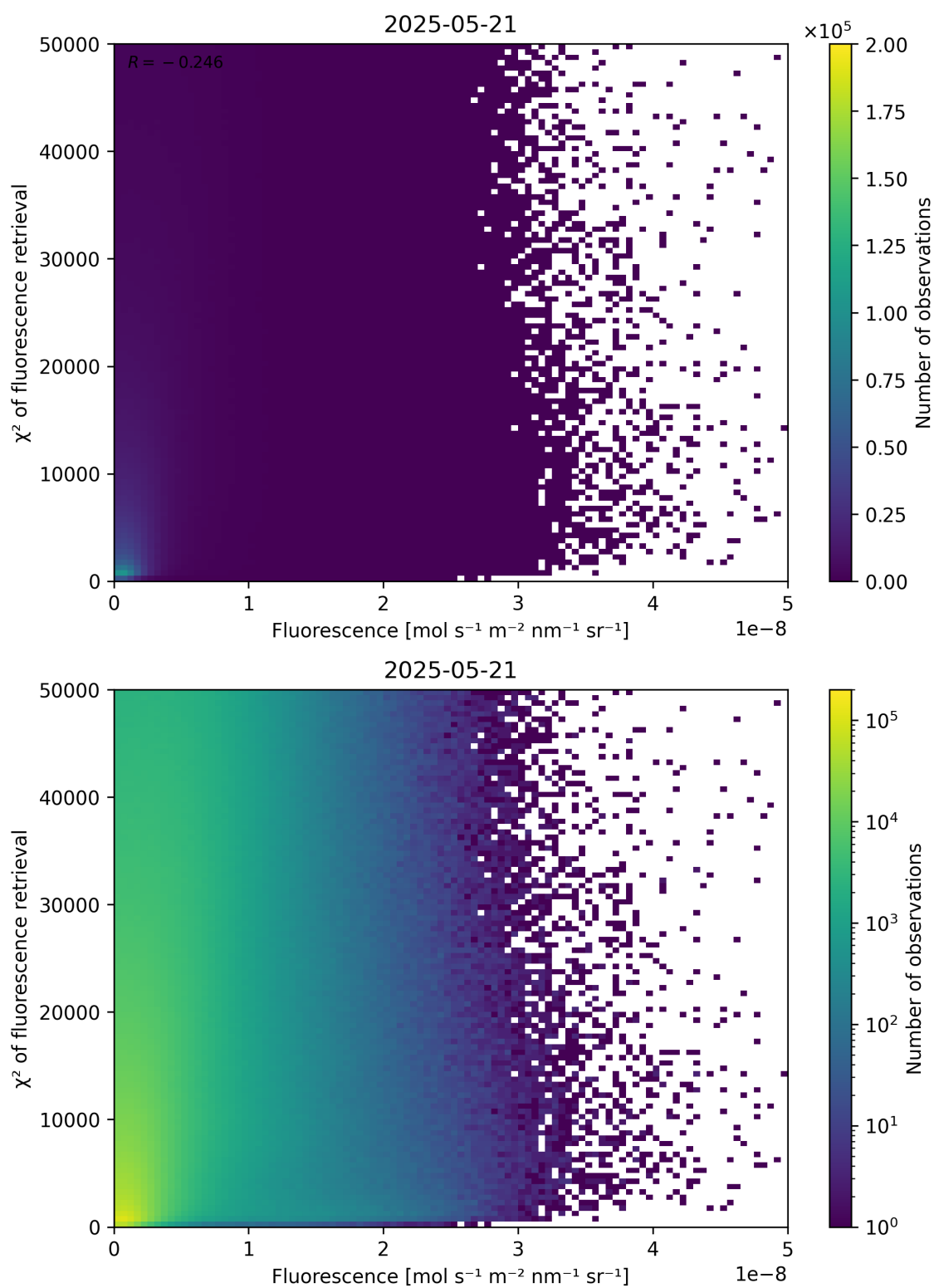
Figure 85: Scatter density plot of “Fluorescence” against “ \chi^2 of fluorescence retrieval” for 2025-05-21 to 2025-05-22.
