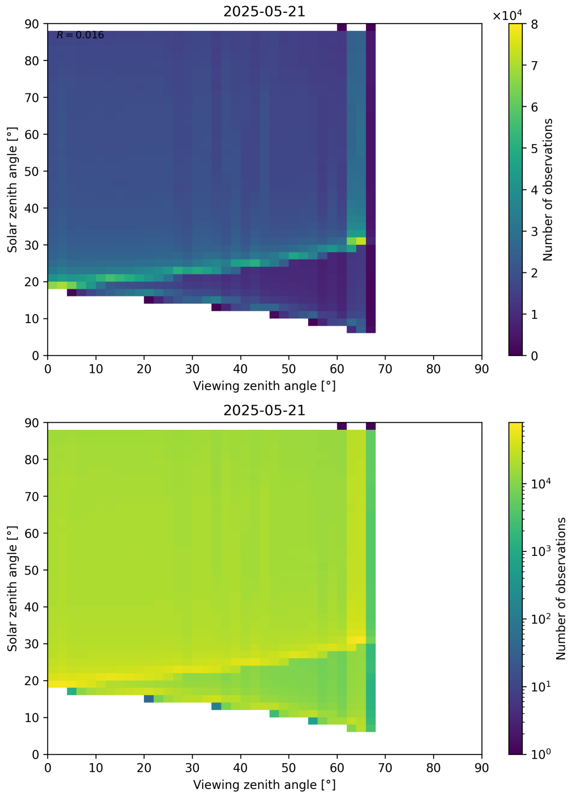
Figure 127: Scatter density plot of “Viewing zenith angle” against “Solar zenith angle” for 2025-05-21 to 2025-05-22.
