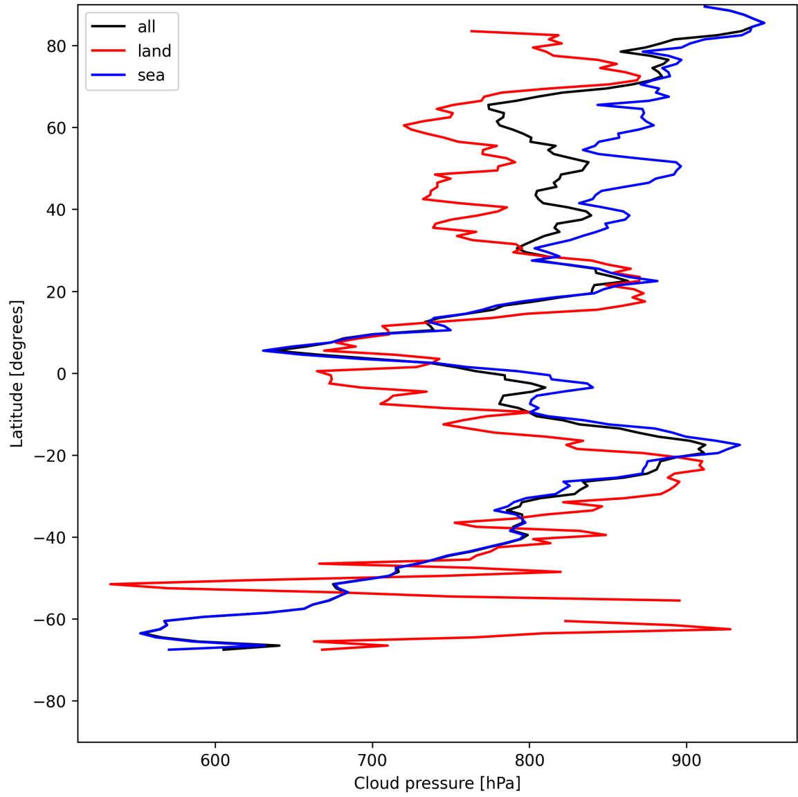
Figure 13: Zonal average of “Cloud pressure” for 2025-05-21 to 2025-05-22.
