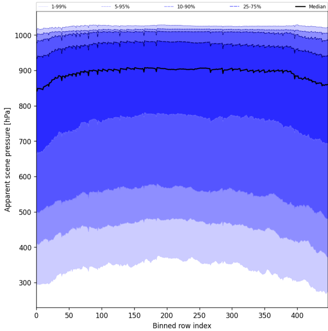
Figure 53: Along track statistics of “Apparent scene pressure” for 2025-05-21 to 2025-05-22
