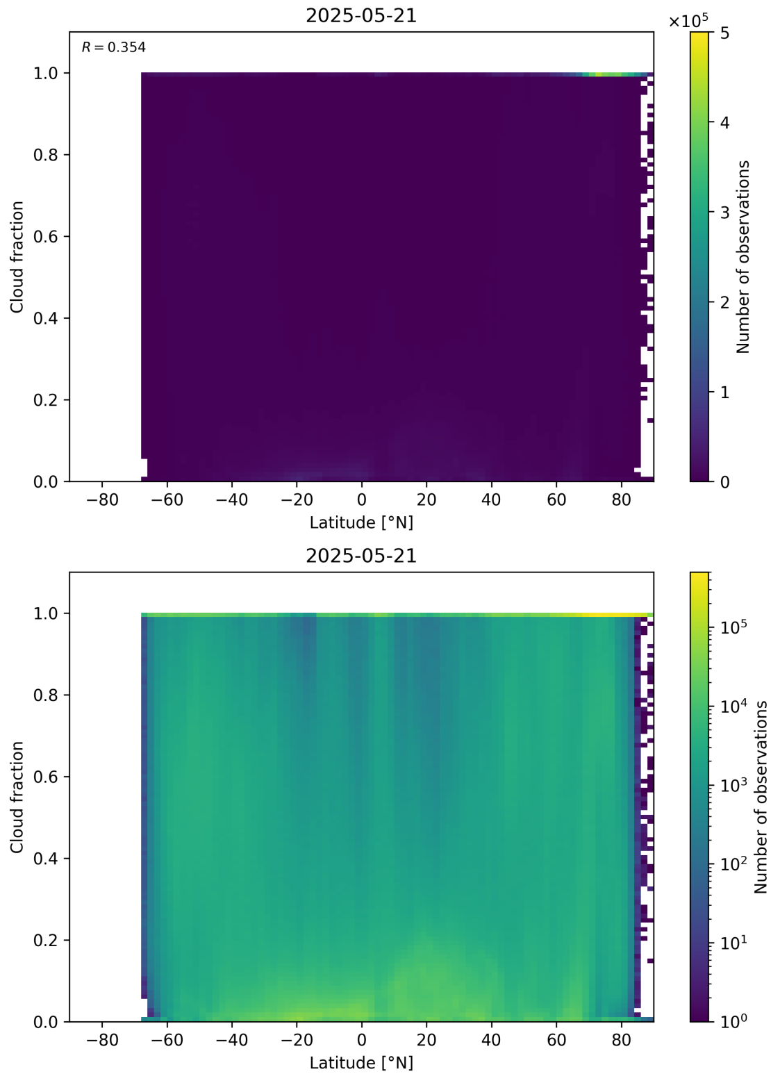
Figure 90: Scatter density plot of “Latitude” against “Cloud fraction” for 2025-05-21 to 2025-05-22.
