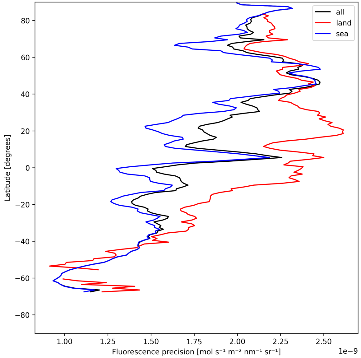
Figure 24: Zonal average of “Fluorescence precision” for 2025-05-21 to 2025-05-22.
