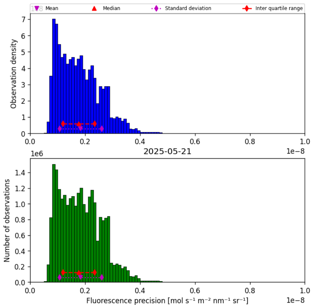
Figure 41: Histogram of “Fluorescence precision” for 2025-05-21 to 2025-05-22
