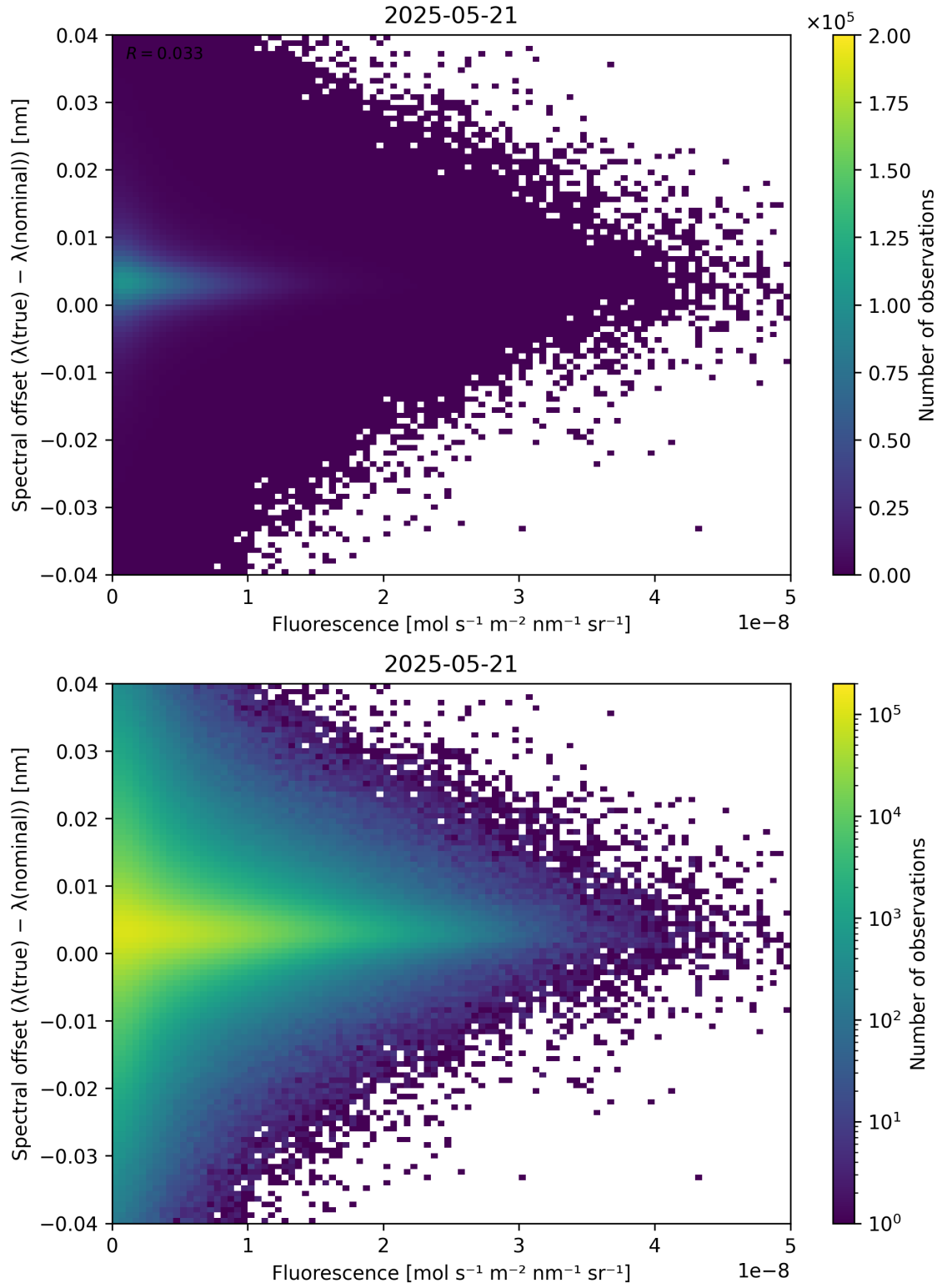
Figure 87: Scatter density plot of “Fluorescence” against “Spectral offset ( \lambda_{\text{true}} - \lambda_{\text{nominal}} )” for 2025-05-21 to 2025-05-22.
