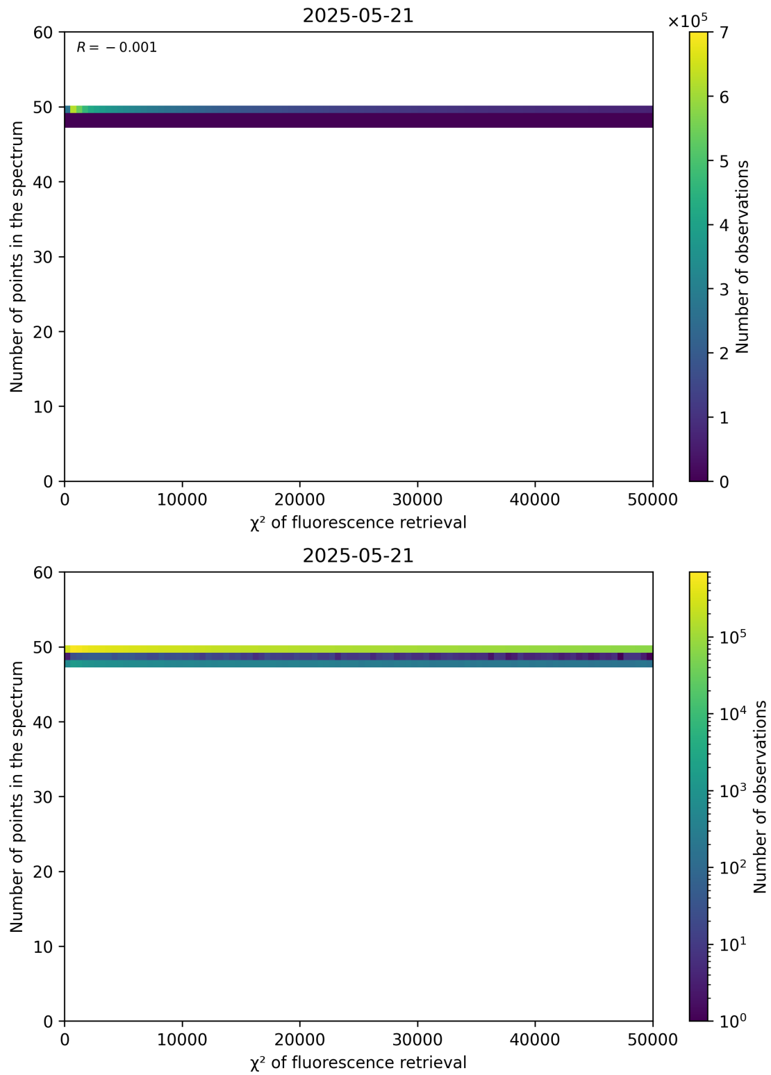
Figure 68: Scatter density plot of " \chi^2 of fluorescence retrieval" against "Number of points in the spectrum" for 2025-05-21 to 2025-05-22.
