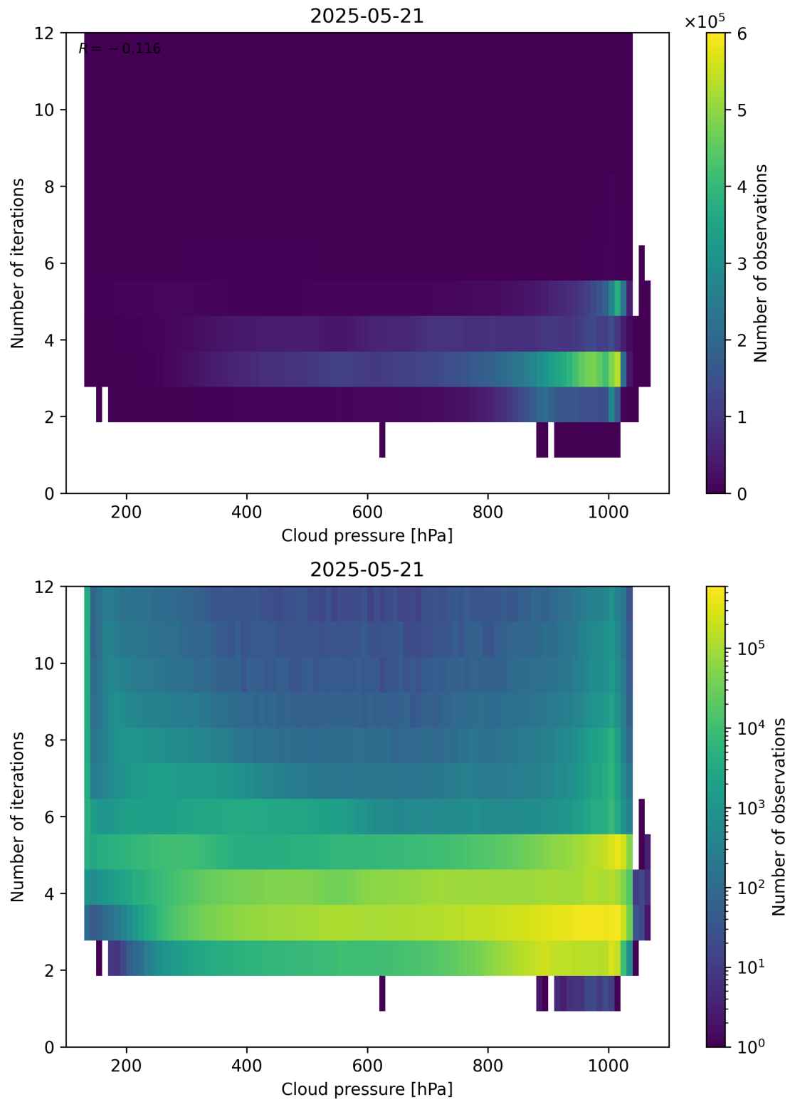
Figure 81: Scatter density plot of “Cloud pressure” against “Number of iterations” for 2025-05-21 to 2025-05-22.
