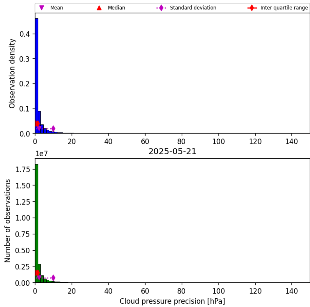
Figure 31: Histogram of “Cloud pressure precision” for 2025-05-21 to 2025-05-22
