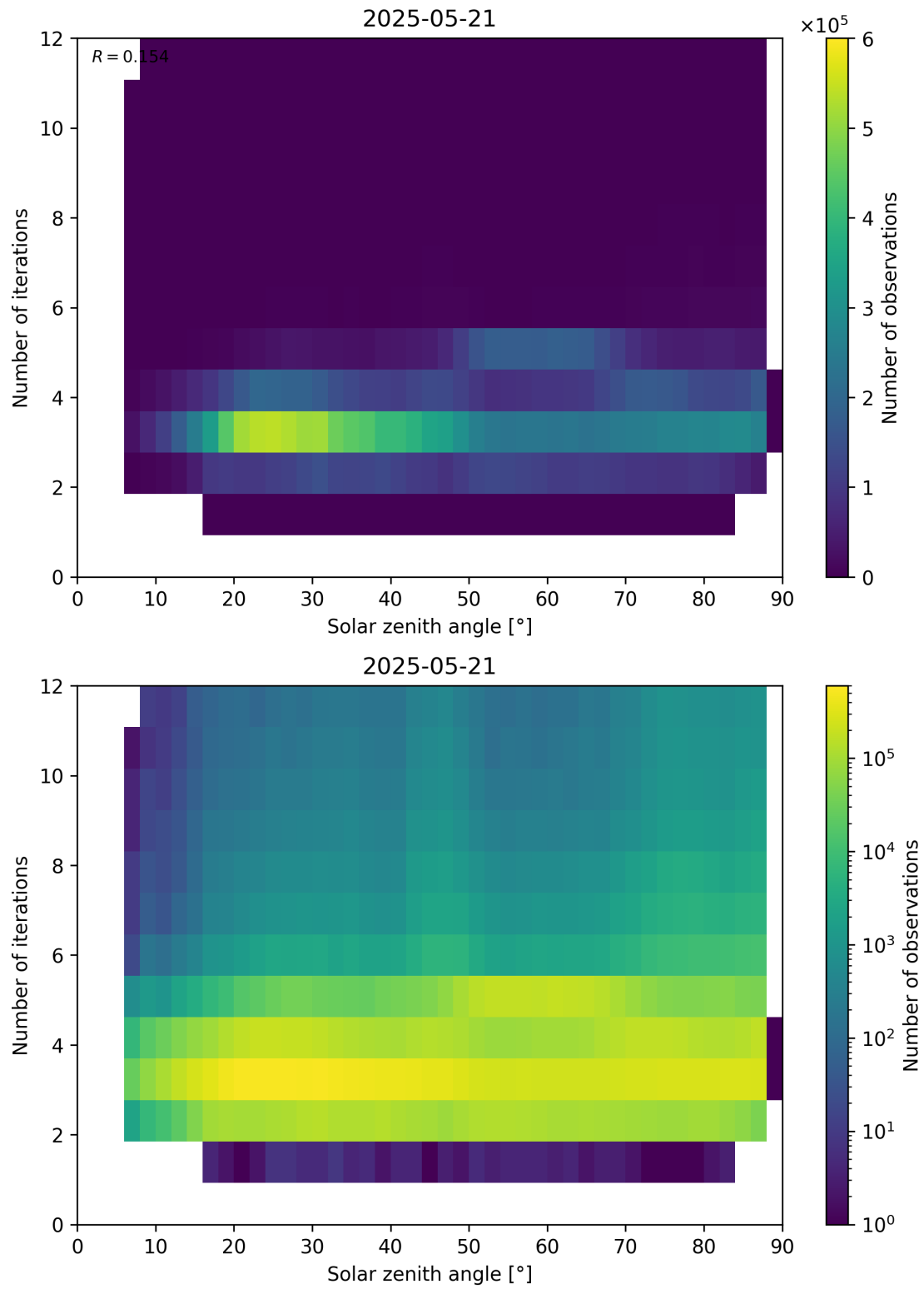
Figure 114: Scatter density plot of “Solar zenith angle” against “Number of iterations” for 2025-05-21 to 2025-05-22.
