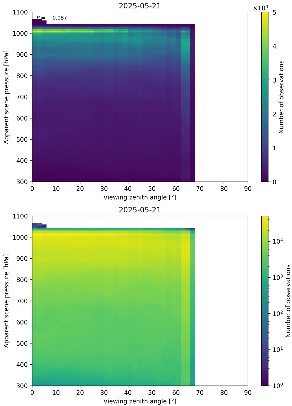
Figure 118: Scatter density plot of “Viewing zenith angle” against “Apparent scene pressure” for 2025-05-21 to 2025-05-22.
