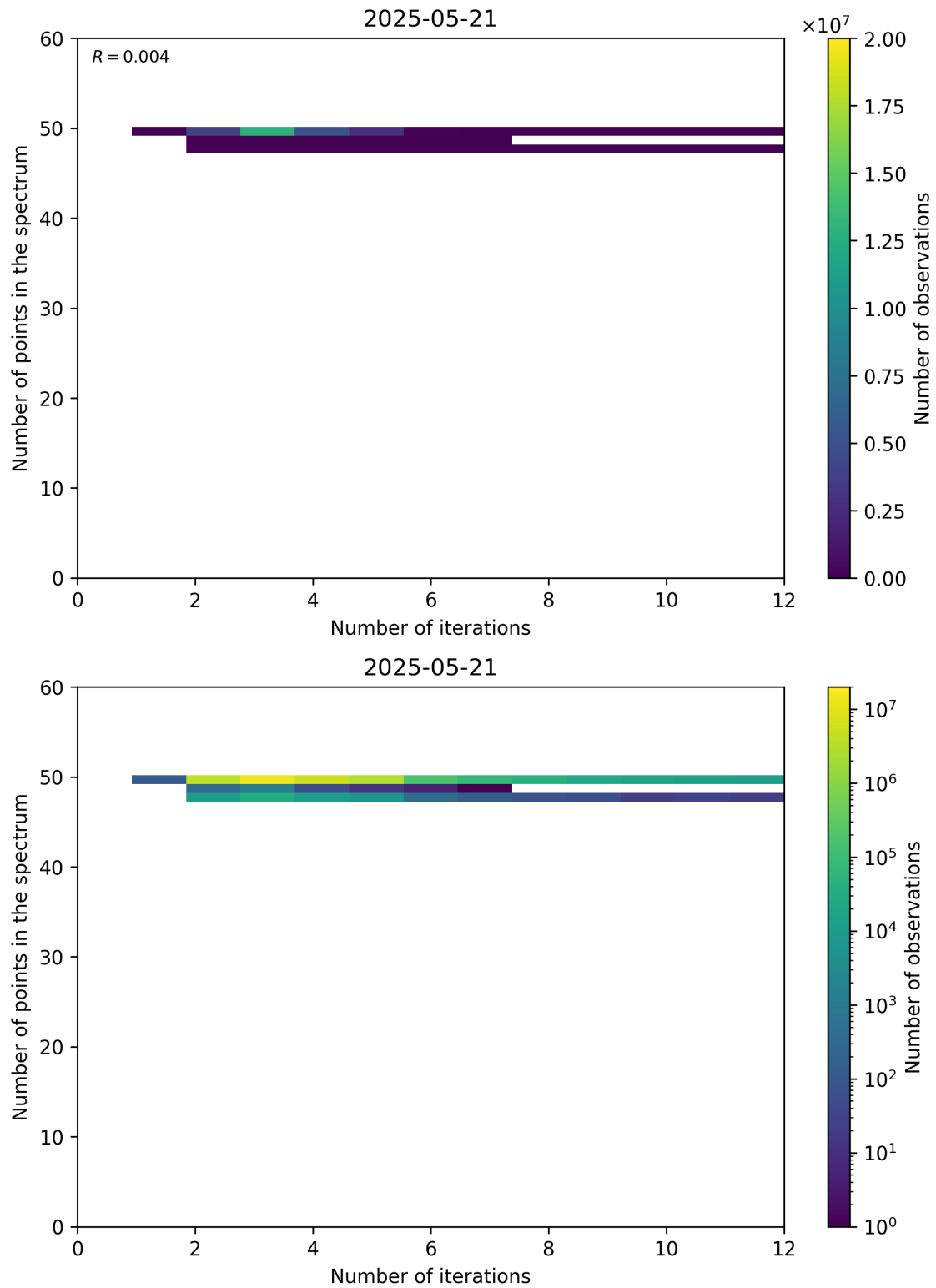
Figure 99: Scatter density plot of “Number of iterations” against “Number of points in the spectrum” for 2025-05-21 to 2025-05-22.
