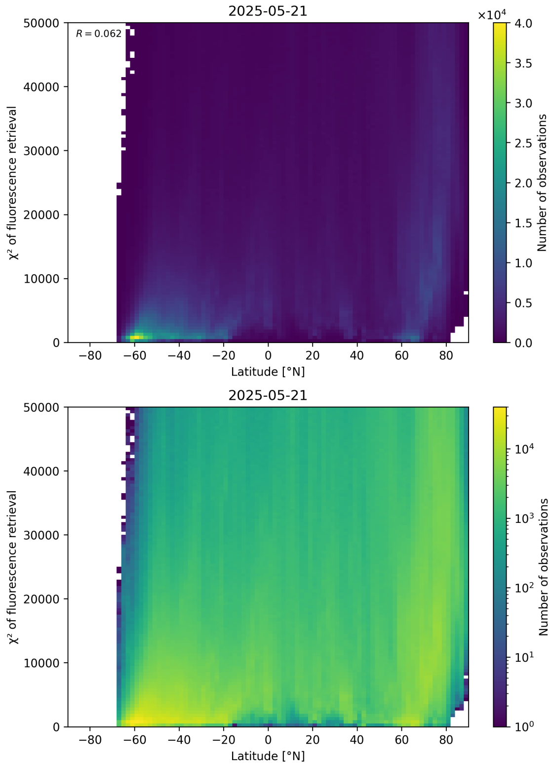
Figure 89: Scatter density plot of “Latitude” against “ \chi^2 of fluorescence retrieval” for 2025-05-21 to 2025-05-22.
