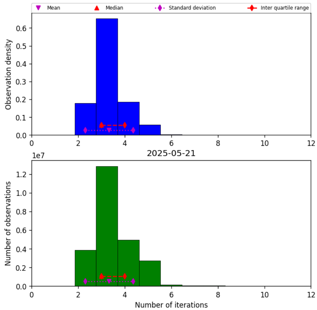
Figure 39: Histogram of “Number of iterations” for 2025-05-21 to 2025-05-22
