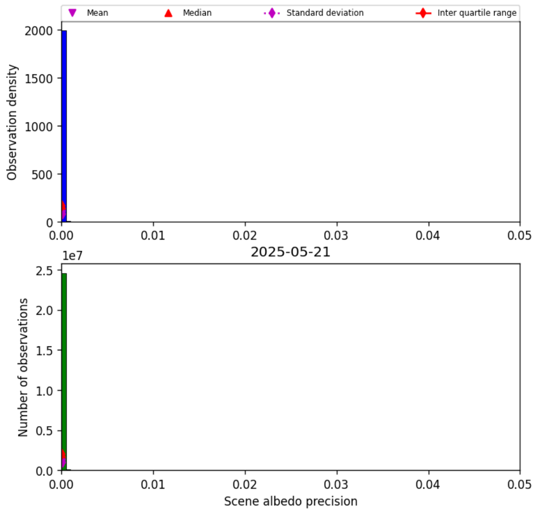
Figure 35: Histogram of “Scene albedo precision” for 2025-05-21 to 2025-05-22
