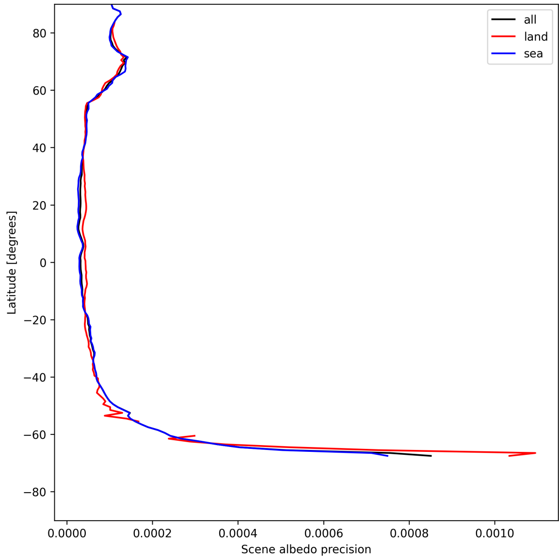
Figure 18: Zonal average of “Scene albedo precision” for 2025-05-21 to 2025-05-22.
