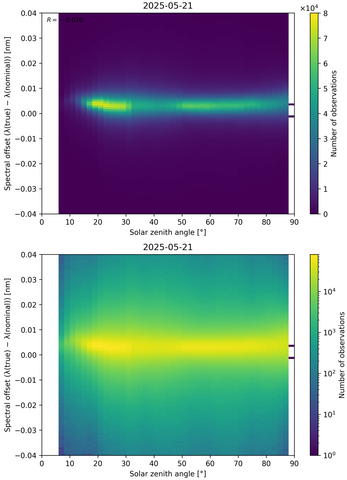
Figure 117: Scatter density plot of “Solar zenith angle” against “Spectral offset ( \lambda_{\text{true}} - \lambda_{\text{nominal}} )” for 2025-05-21 to 2025-05-22.
