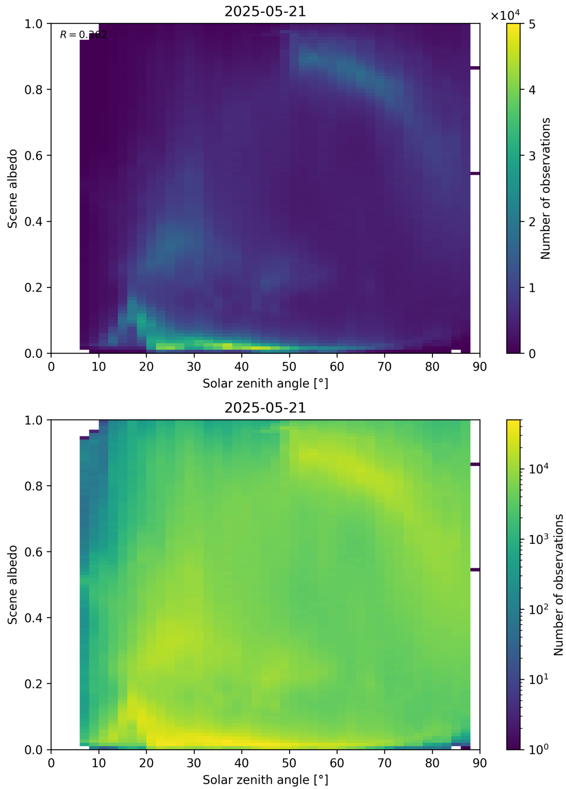
Figure 116: Scatter density plot of “Solar zenith angle” against “Scene albedo” for 2025-05-21 to 2025-05-22.
