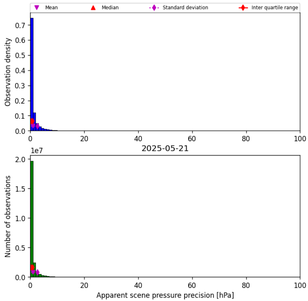
Figure 37: Histogram of “Apparent scene pressure precision” for 2025-05-21 to 2025-05-22
