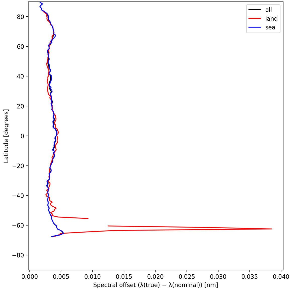
Figure 28: Zonal average of “Spectral offset ( \lambda_{\text{true}} - \lambda_{\text{nominal}} )” for 2025-05-21 to 2025-05-22.
