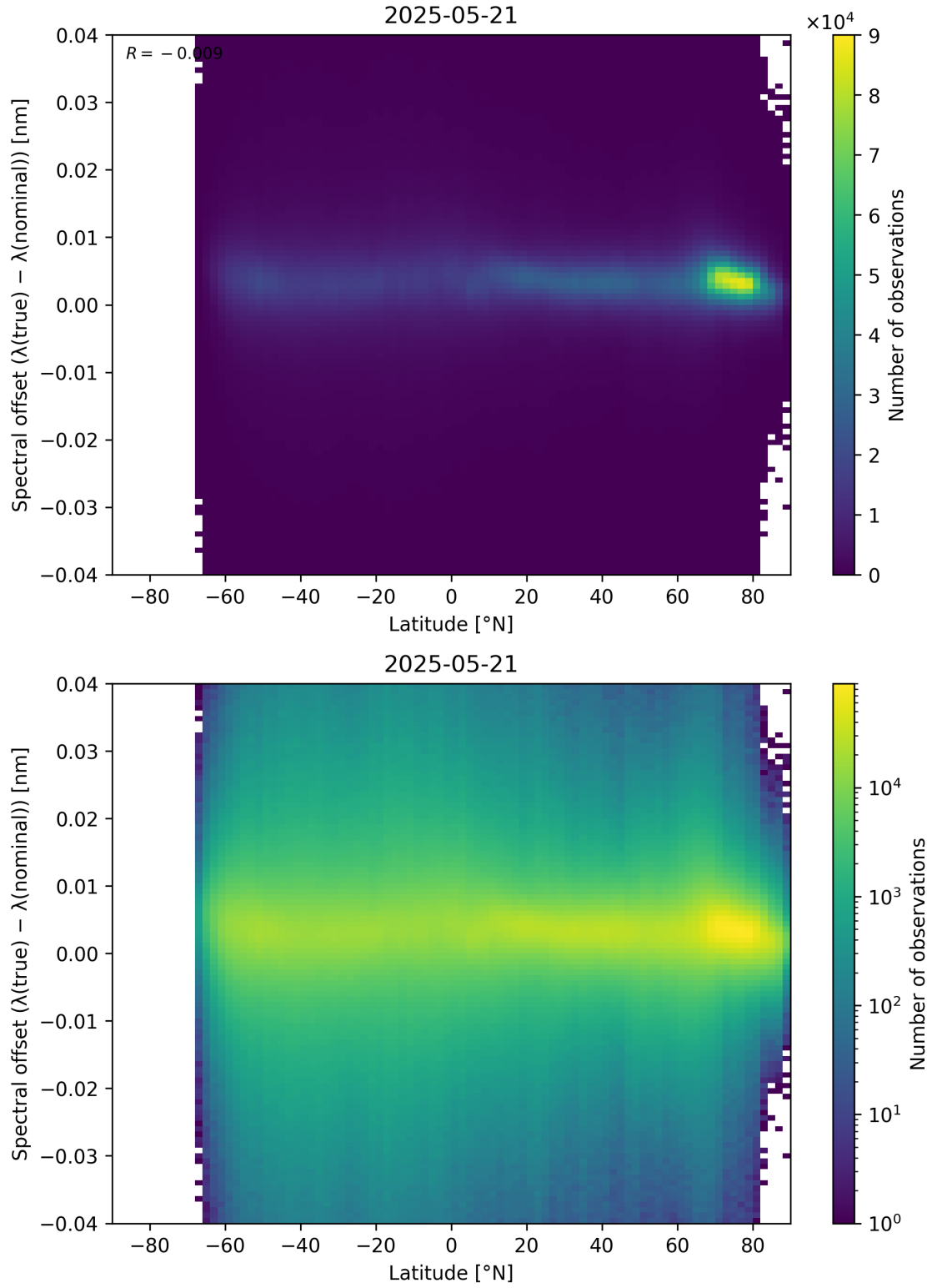
Figure 96: Scatter density plot of “Latitude” against “Spectral offset ( \lambda_{\text{true}} - \lambda_{\text{nominal}} )” for 2025-05-21 to 2025-05-22.
