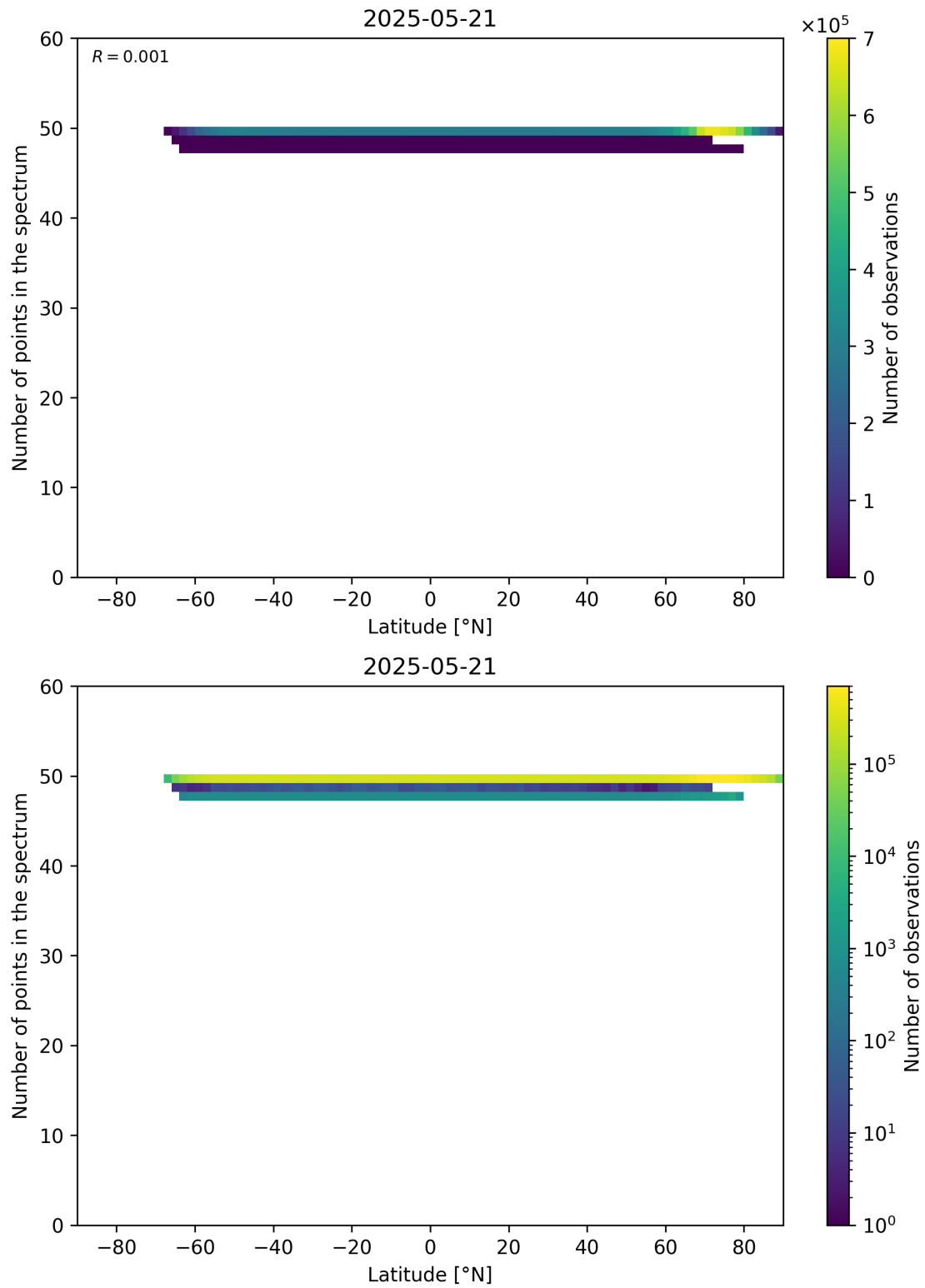
Figure 94: Scatter density plot of “Latitude” against “Number of points in the spectrum” for 2025-05-21 to 2025-05-22.
