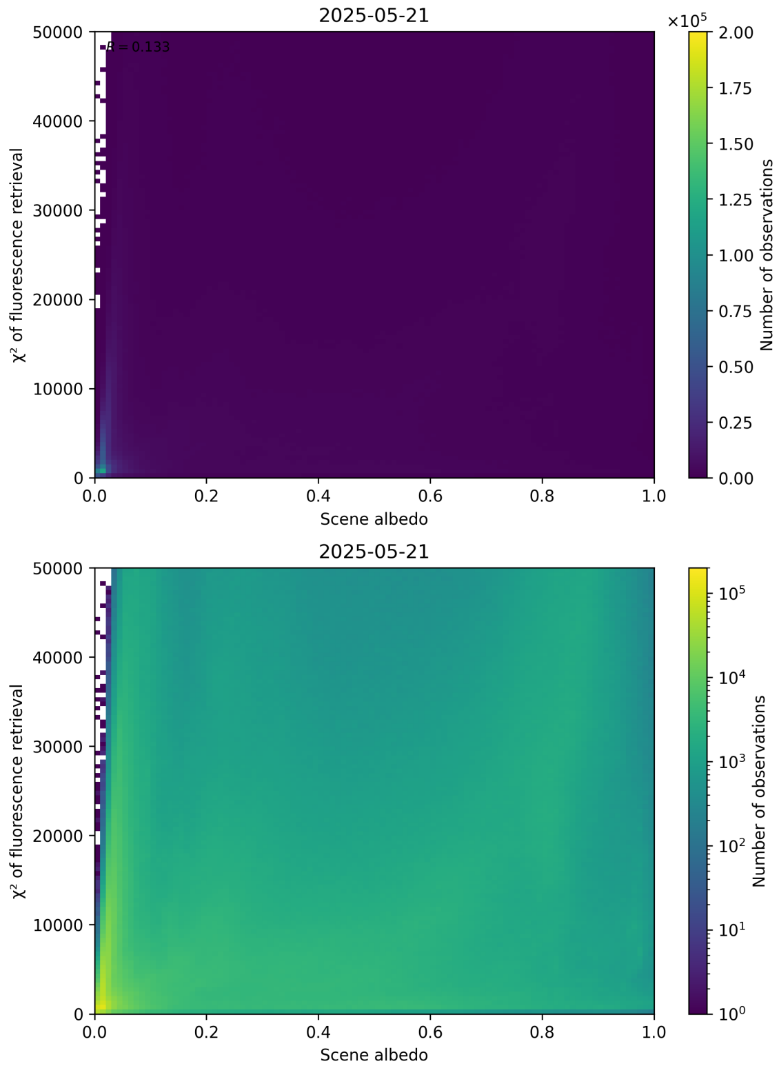
Figure 103: Scatter density plot of “Scene albedo” against “ \chi^2 of fluorescence retrieval” for 2025-05-21 to 2025-05-22.
