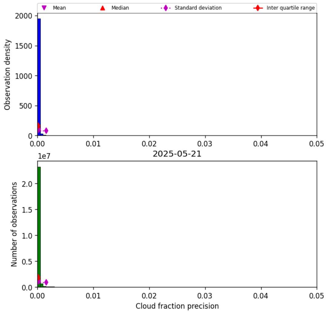
Figure 33: Histogram of “Cloud fraction precision” for 2025-05-21 to 2025-05-22
