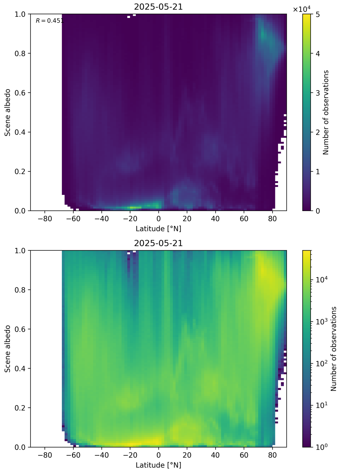
Figure 95: Scatter density plot of “Latitude” against “Scene albedo” for 2025-05-21 to 2025-05-22.
