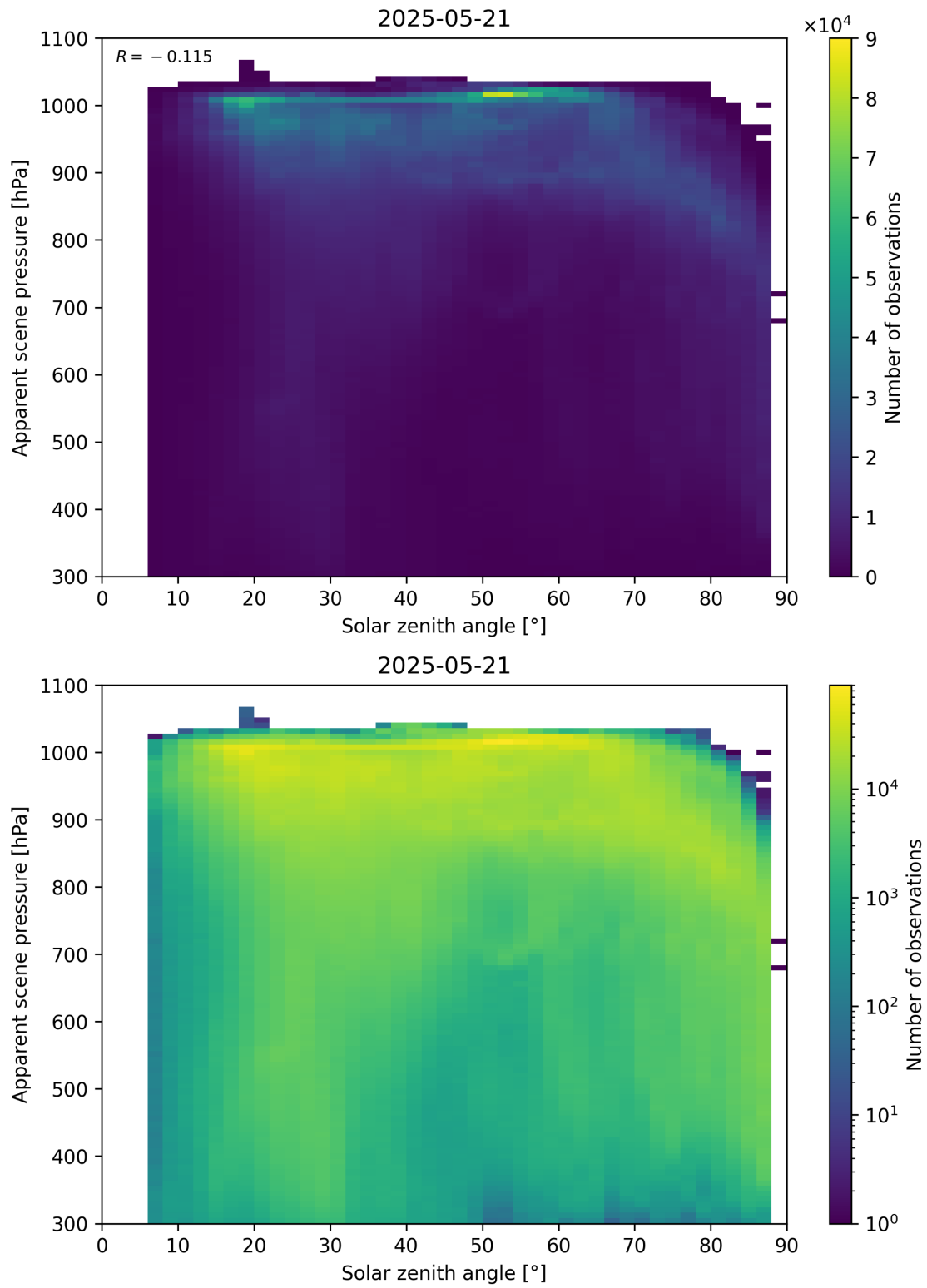
Figure 108: Scatter density plot of “Solar zenith angle” against “Apparent scene pressure” for 2025-05-21 to 2025-05-22.
