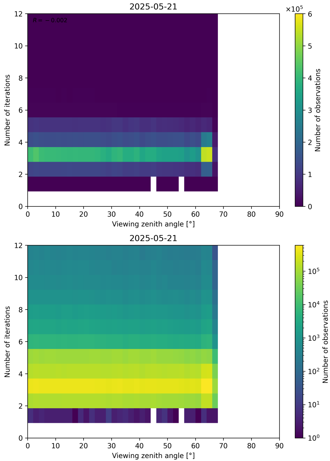
Figure 124: Scatter density plot of “Viewing zenith angle” against “Number of iterations” for 2025-05-21 to 2025-05-22.
