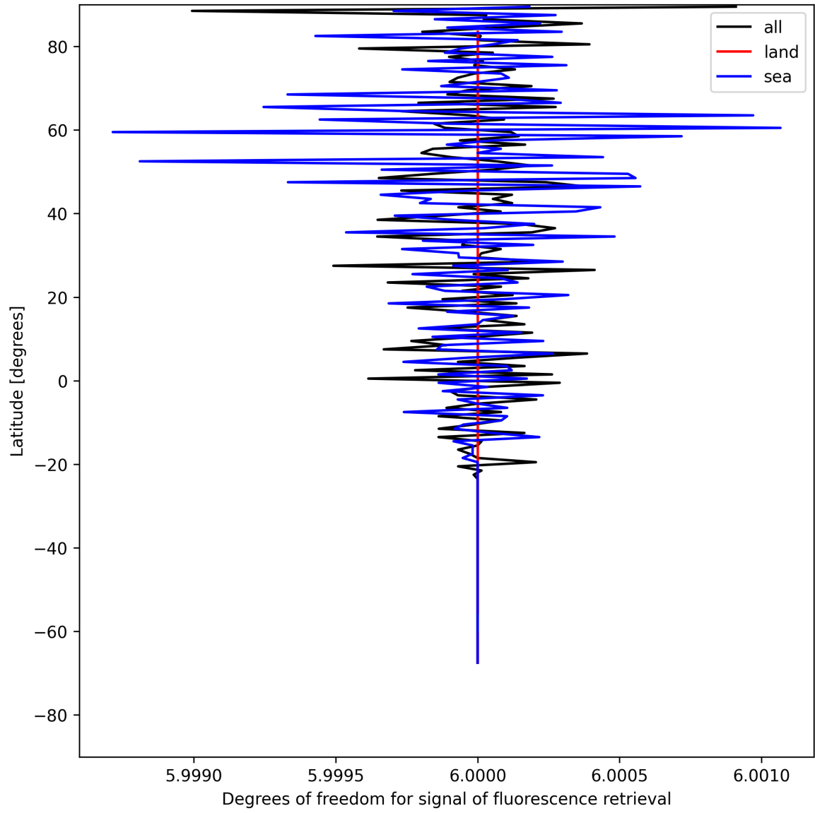
Figure 26: Zonal average of “Degrees of freedom for signal of fluorescence retrieval” for 2025-05-21 to 2025-05-22.
