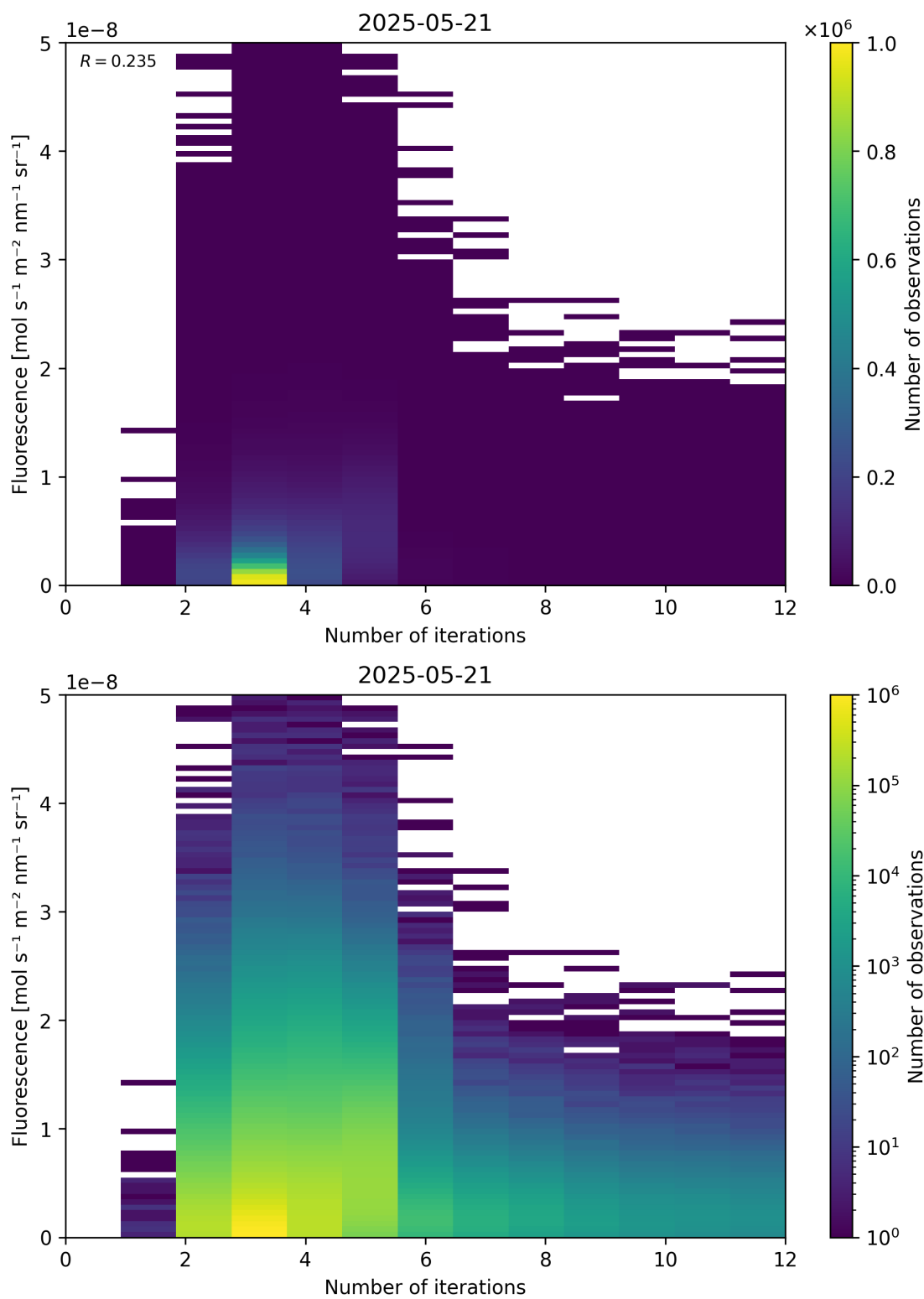
Figure 98: Scatter density plot of “Number of iterations” against “Fluorescence” for 2025-05-21 to 2025-05-22.
