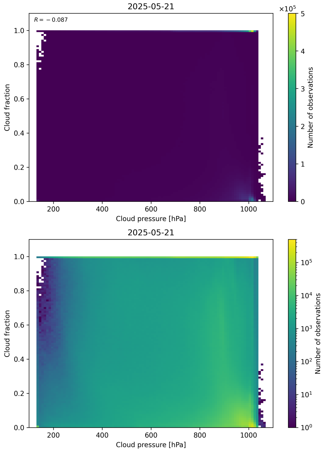
Figure 79: Scatter density plot of “Cloud pressure” against “Cloud fraction” for 2025-05-21 to 2025-05-22.
