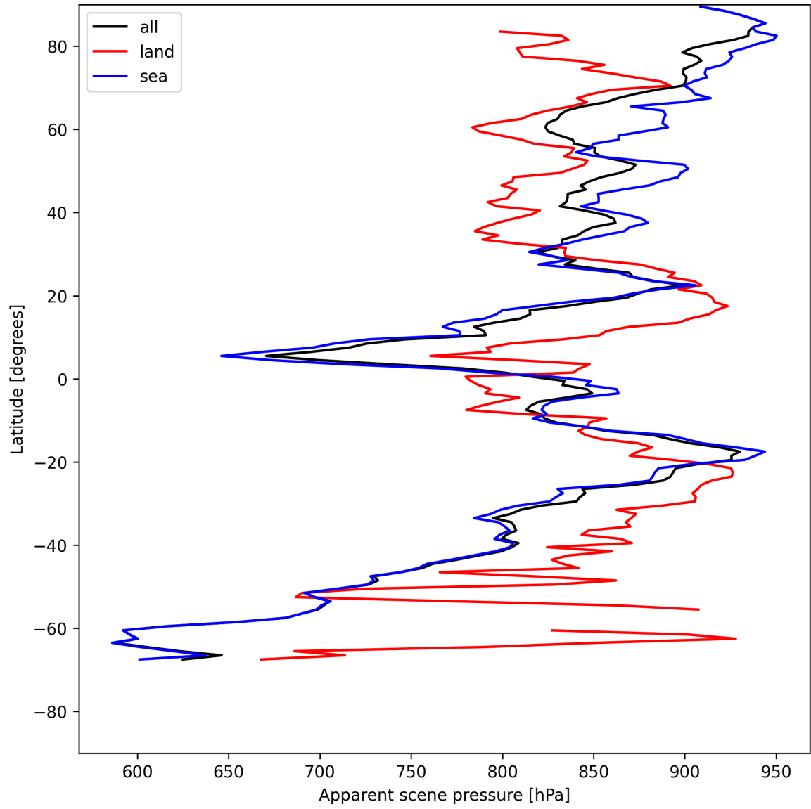
Figure 19: Zonal average of “Apparent scene pressure” for 2025-05-21 to 2025-05-22.
