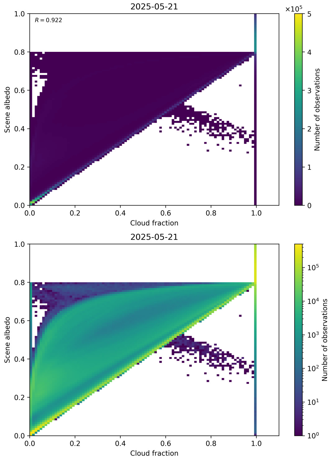
Figure 75: Scatter density plot of “Cloud fraction” against “Scene albedo” for 2025-05-21 to 2025-05-22.
