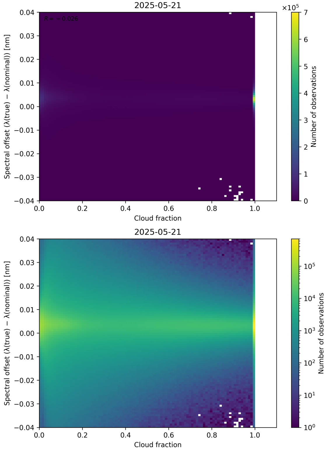
Figure 76: Scatter density plot of “Cloud fraction” against “Spectral offset ( \lambda_{\text{true}} - \lambda_{\text{nominal}} )” for 2025-05-21 to 2025-05-22.
