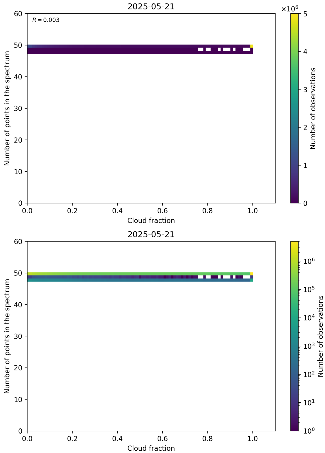
Figure 74: Scatter density plot of “Cloud fraction” against “Number of points in the spectrum” for 2025-05-21 to 2025-05-22.
