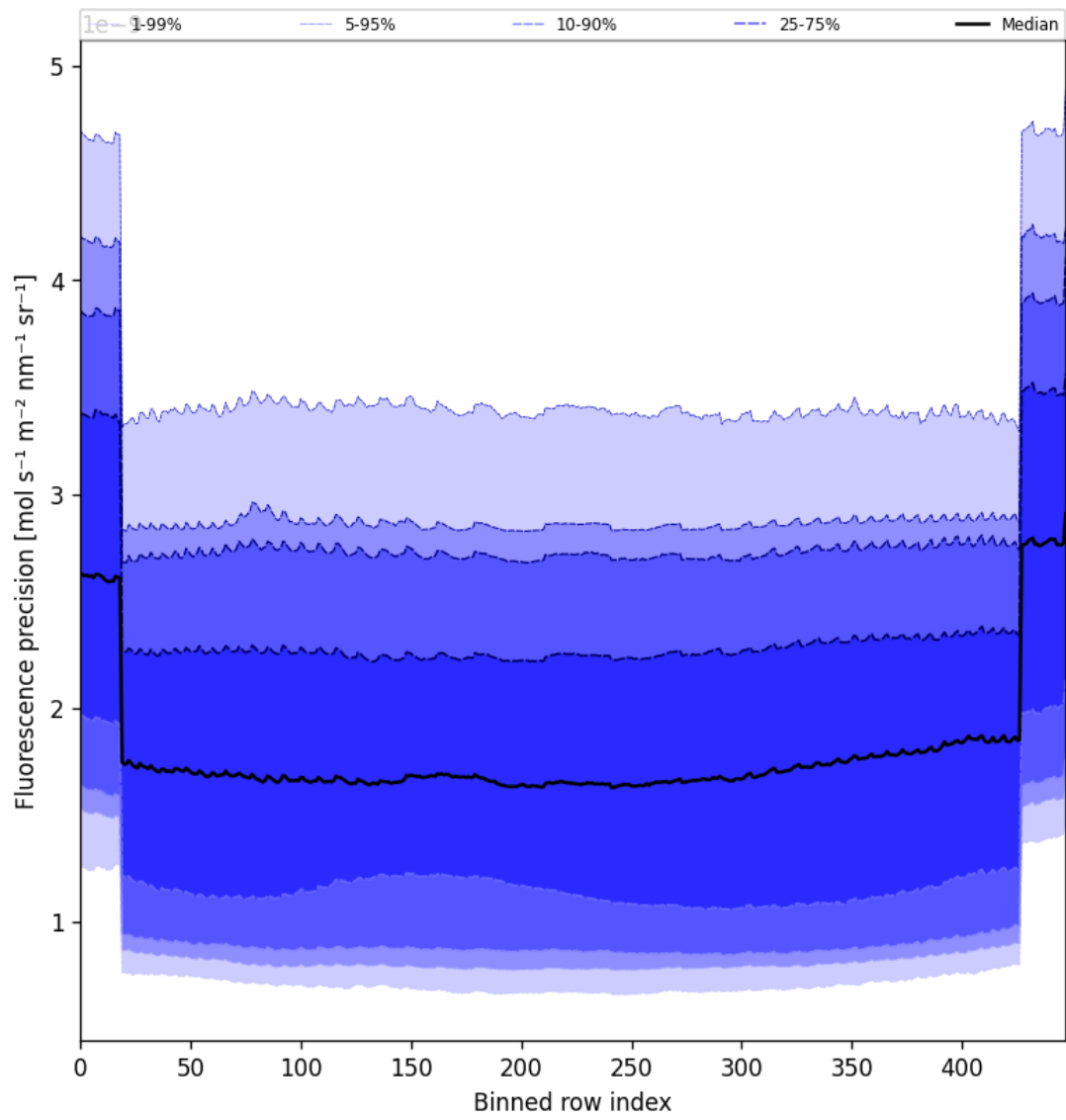
Figure 58: Along track statistics of “Fluorescence precision” for 2025-05-21 to 2025-05-22
