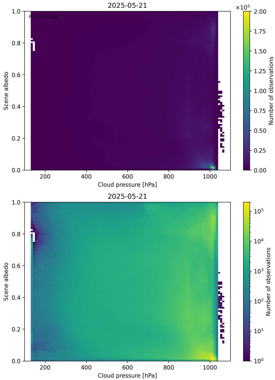
Figure 83: Scatter density plot of “Cloud pressure” against “Scene albedo” for 2025-05-21 to 2025-05-22.
