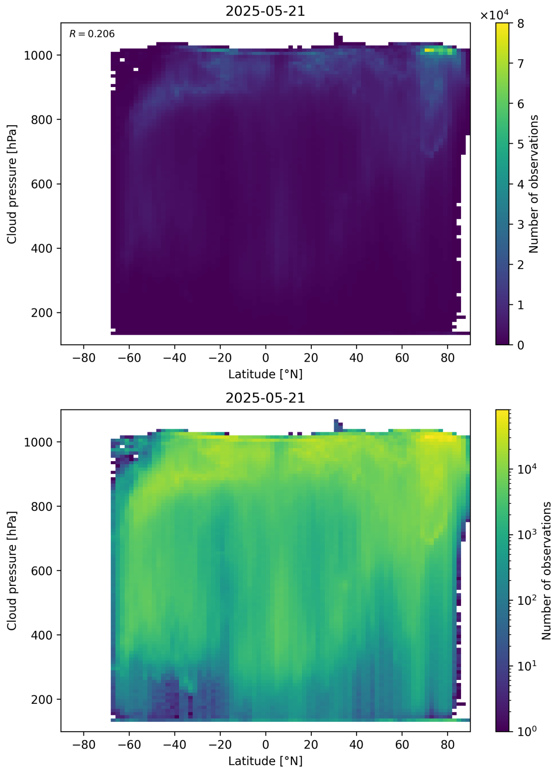
Figure 91: Scatter density plot of “Latitude” against “Cloud pressure” for 2025-05-21 to 2025-05-22.
