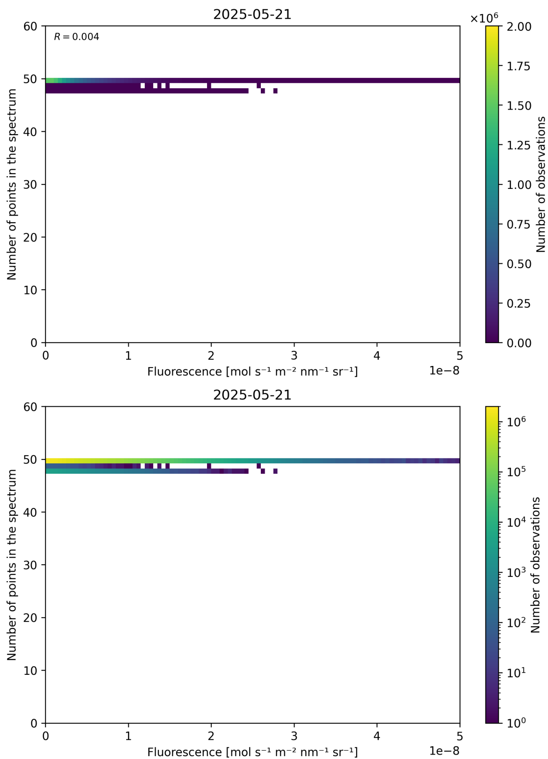
Figure 86: Scatter density plot of “Fluorescence” against “Number of points in the spectrum” for 2025-05-21 to 2025-05-22.
