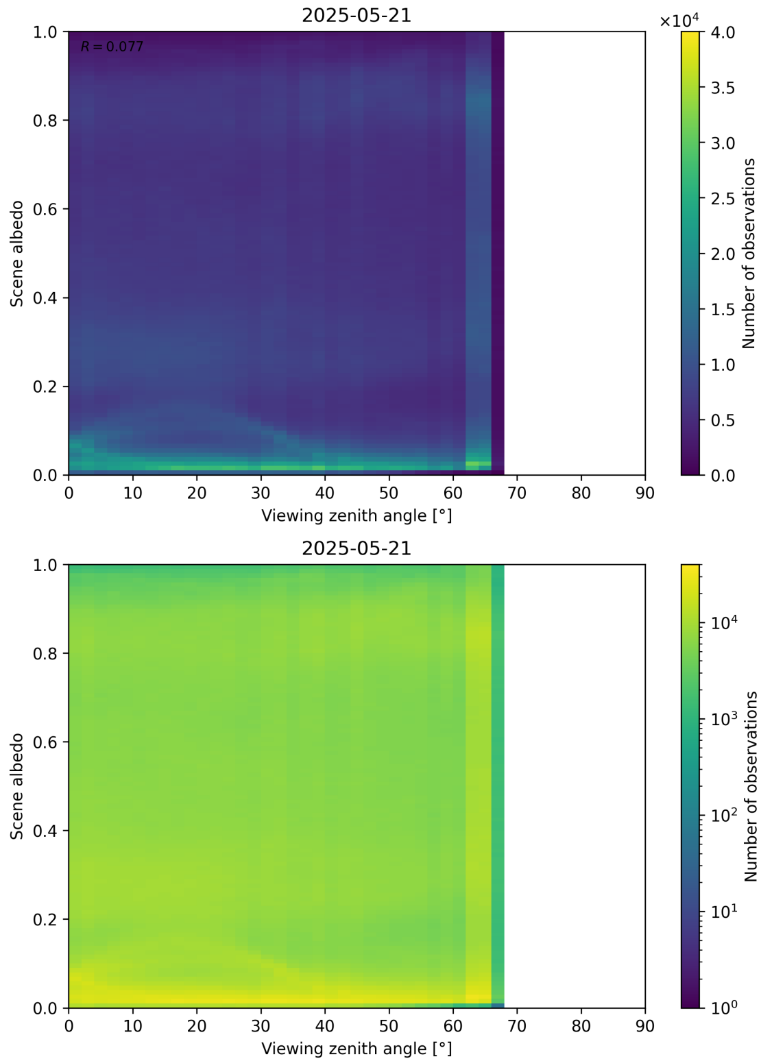
Figure 126: Scatter density plot of “Viewing zenith angle” against “Scene albedo” for 2025-05-21 to 2025-05-22.
