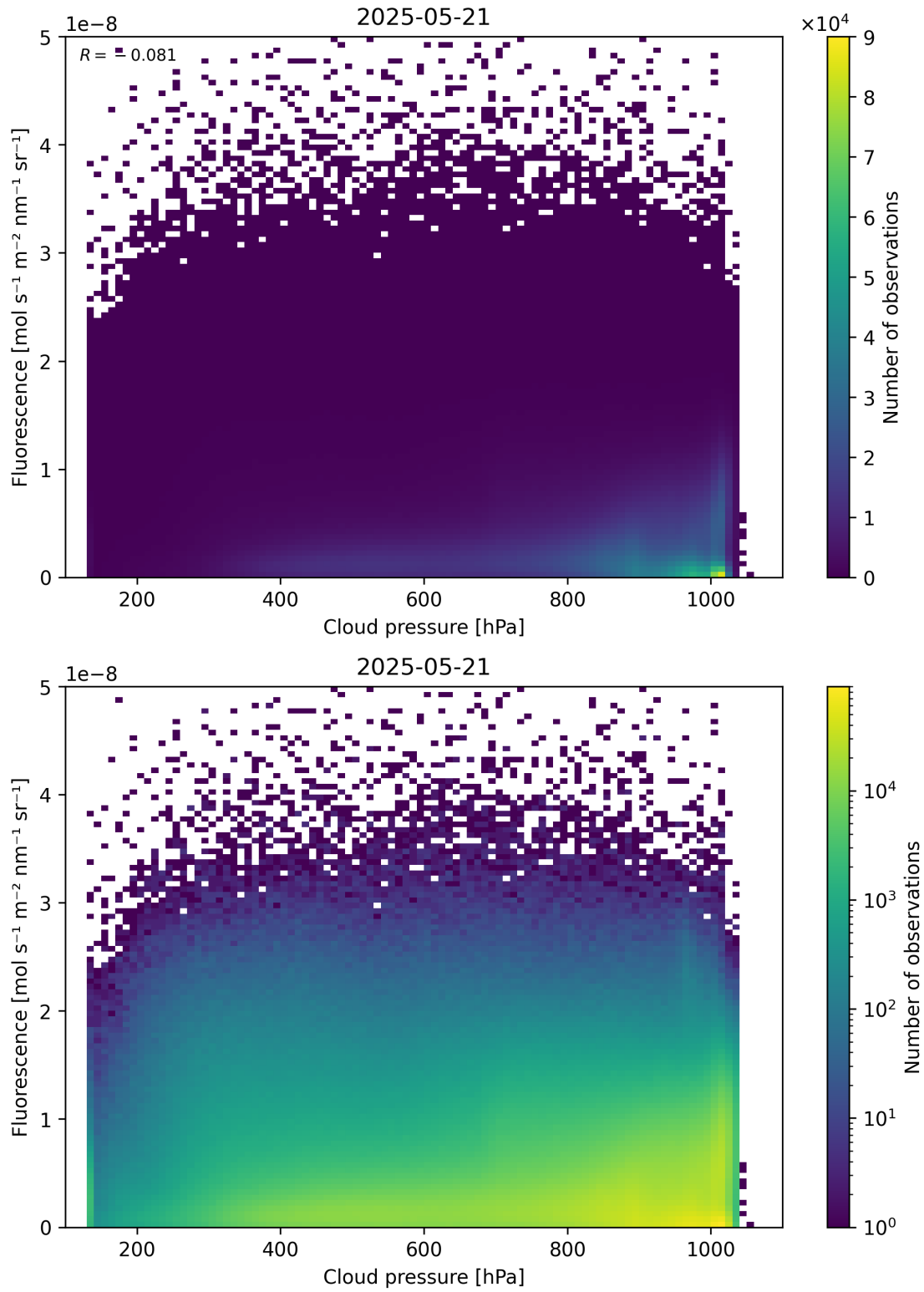
Figure 80: Scatter density plot of “Cloud pressure” against “Fluorescence” for 2025-05-21 to 2025-05-22.
