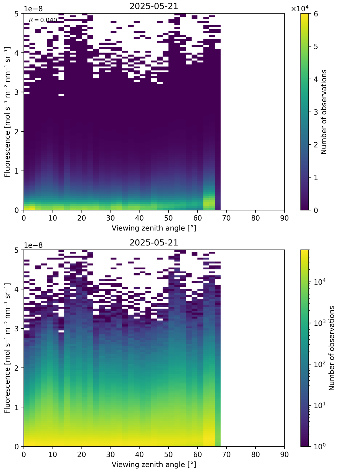
Figure 122: Scatter density plot of “Viewing zenith angle” against “Fluorescence” for 2025-05-21 to 2025-05-22.
