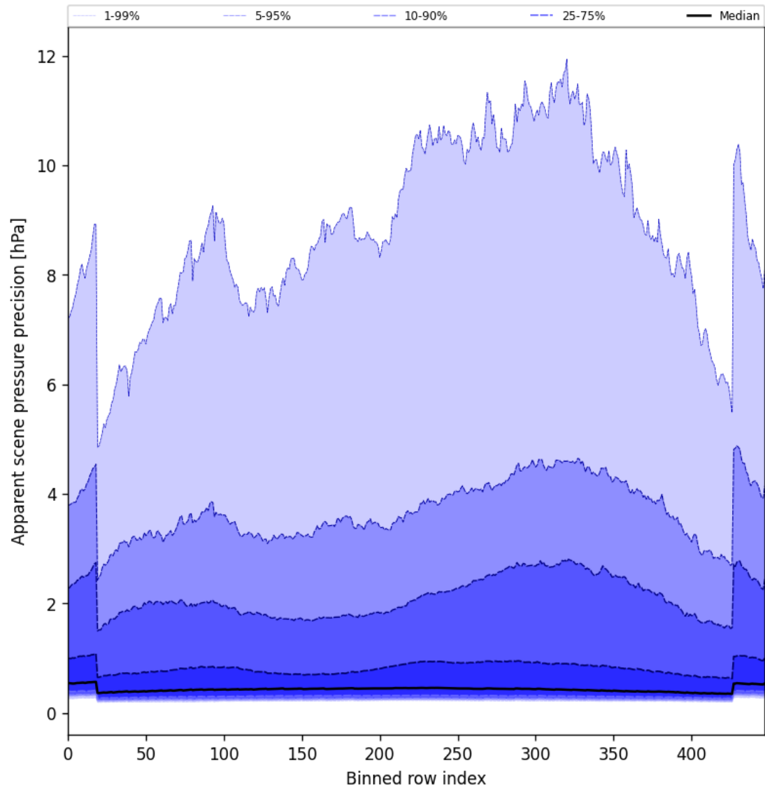
Figure 54: Along track statistics of “Apparent scene pressure precision” for 2025-05-21 to 2025-05-22
