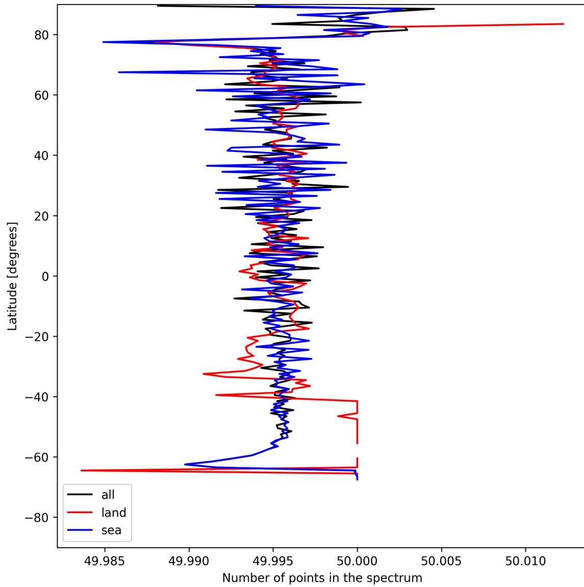
Figure 27: Zonal average of “Number of points in the spectrum” for 2025-05-21 to 2025-05-22.
