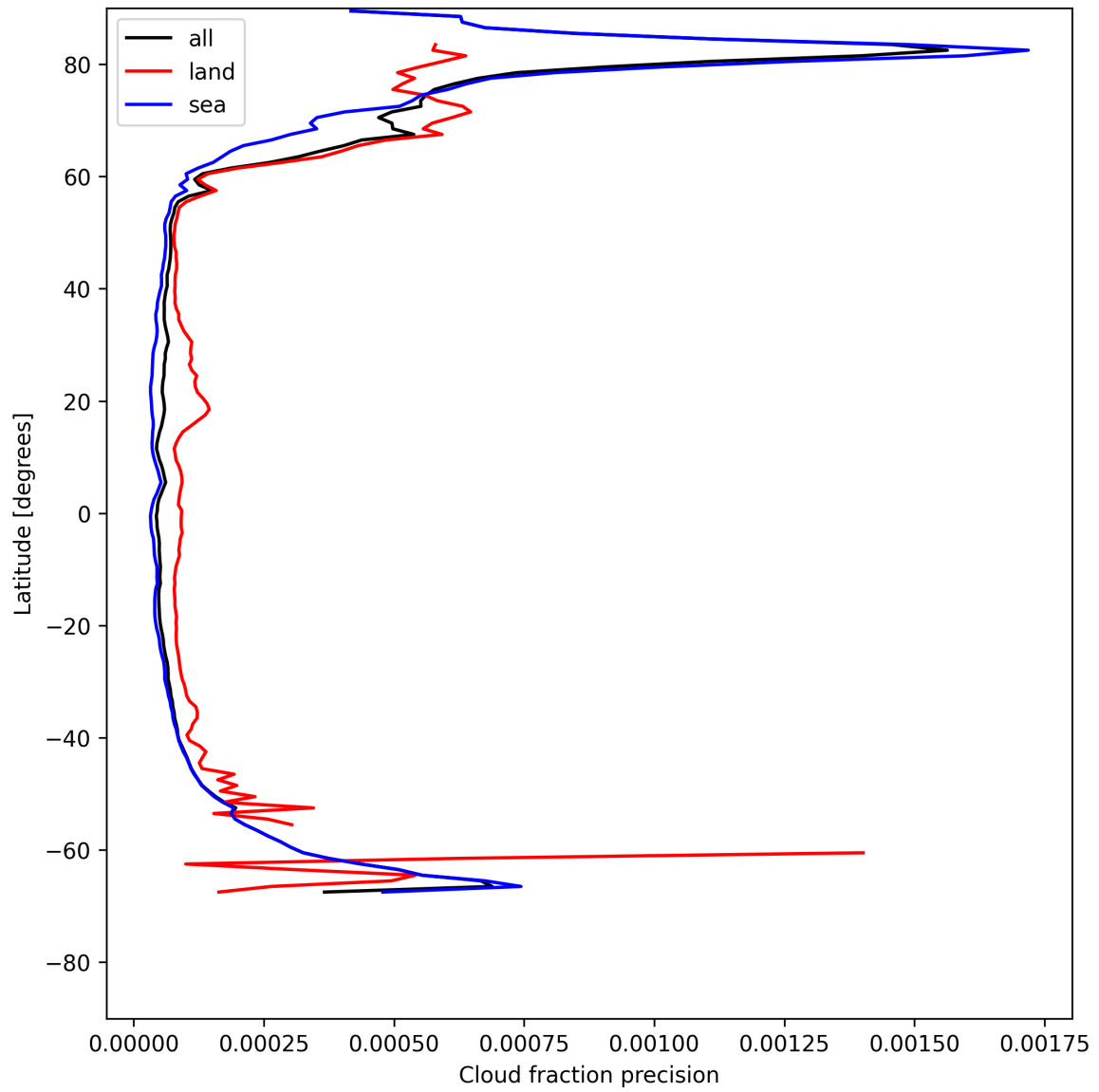
Figure 16: Zonal average of “Cloud fraction precision” for 2025-05-21 to 2025-05-22.
