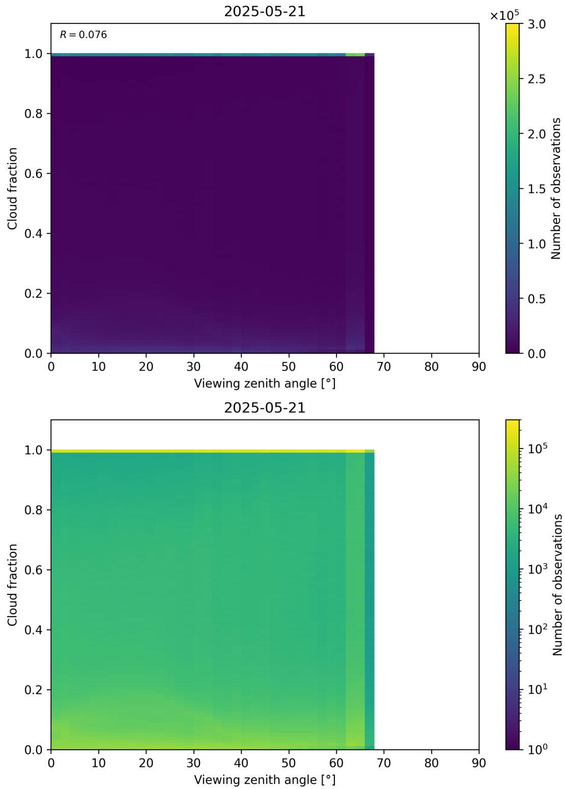
Figure 120: Scatter density plot of “Viewing zenith angle” against “Cloud fraction” for 2025-05-21 to 2025-05-22.
