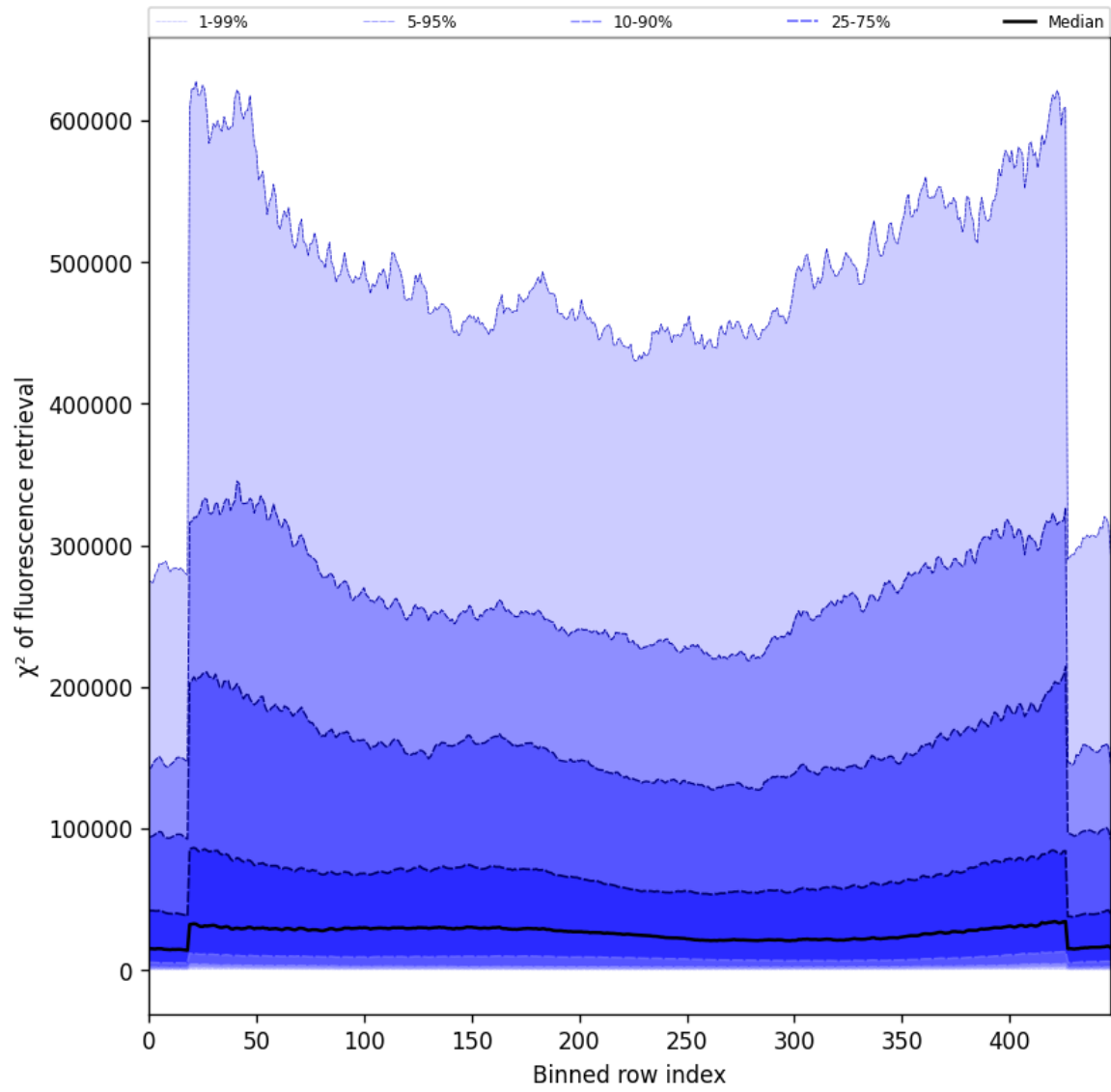
Figure 59: Along track statistics of “ \chi^2 of fluorescence retrieval” for 2025-05-21 to 2025-05-22
