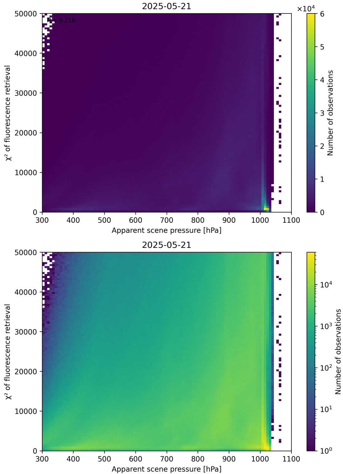
Figure 63: Scatter density plot of “Apparent scene pressure” against “ \chi^2 of fluorescence retrieval” for 2025-05-21 to 2025-05-22.
