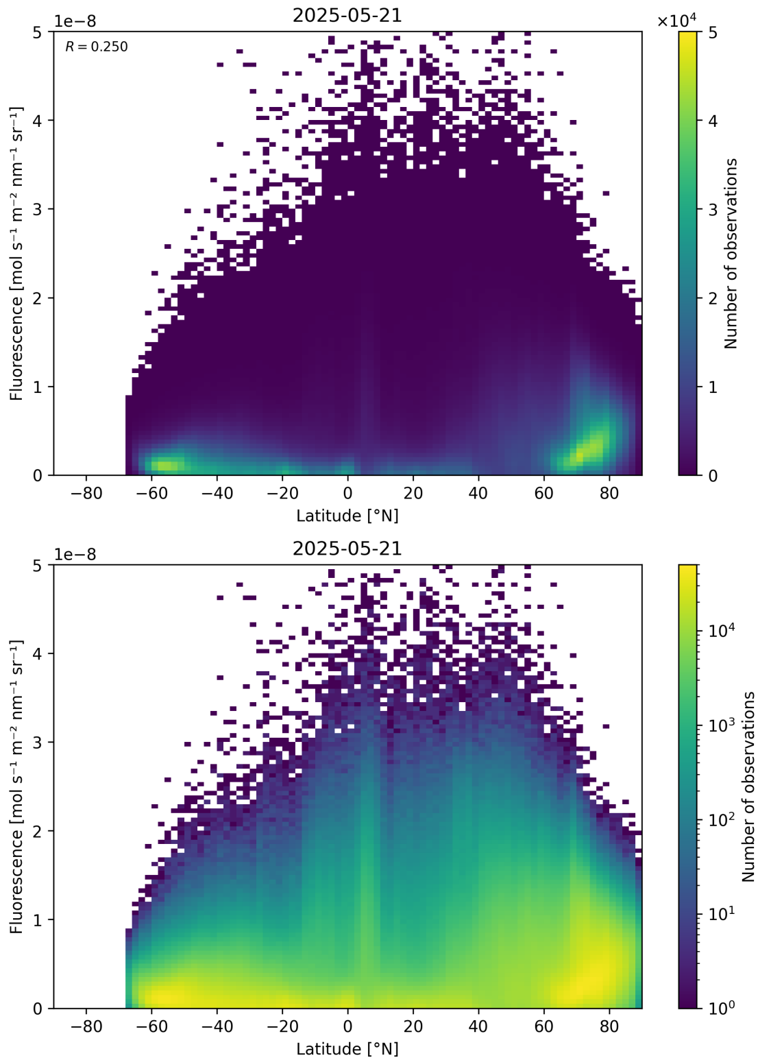
Figure 92: Scatter density plot of “Latitude” against “Fluorescence” for 2025-05-21 to 2025-05-22.
