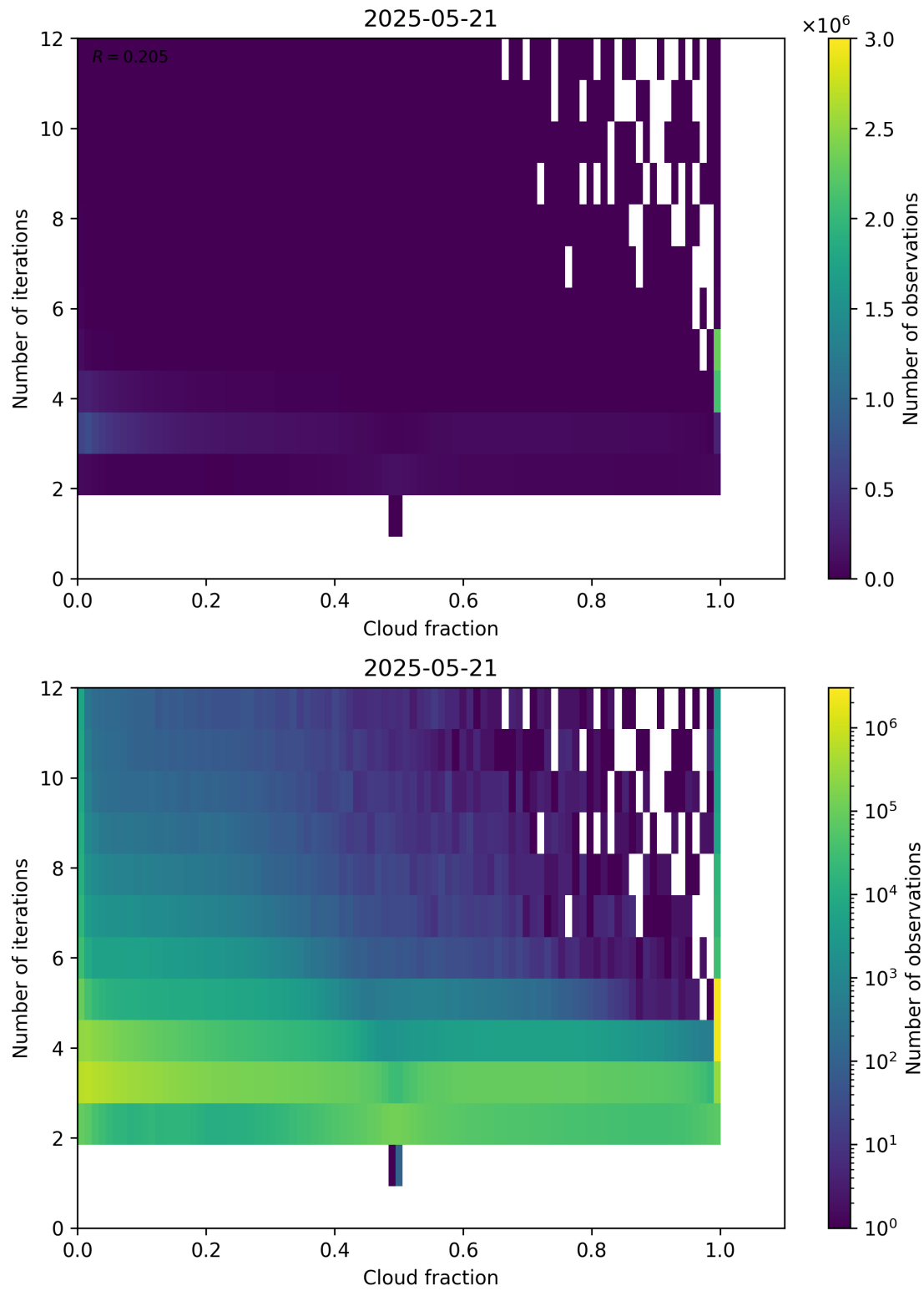
Figure 73: Scatter density plot of “Cloud fraction” against “Number of iterations” for 2025-05-21 to 2025-05-22.
