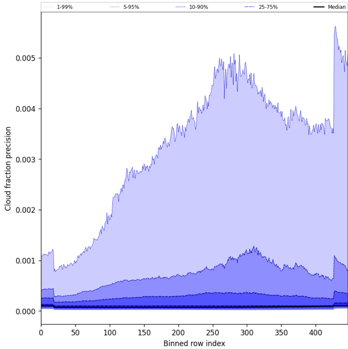
Figure 50: Along track statistics of “Cloud fraction precision” for 2025-05-21 to 2025-05-22
