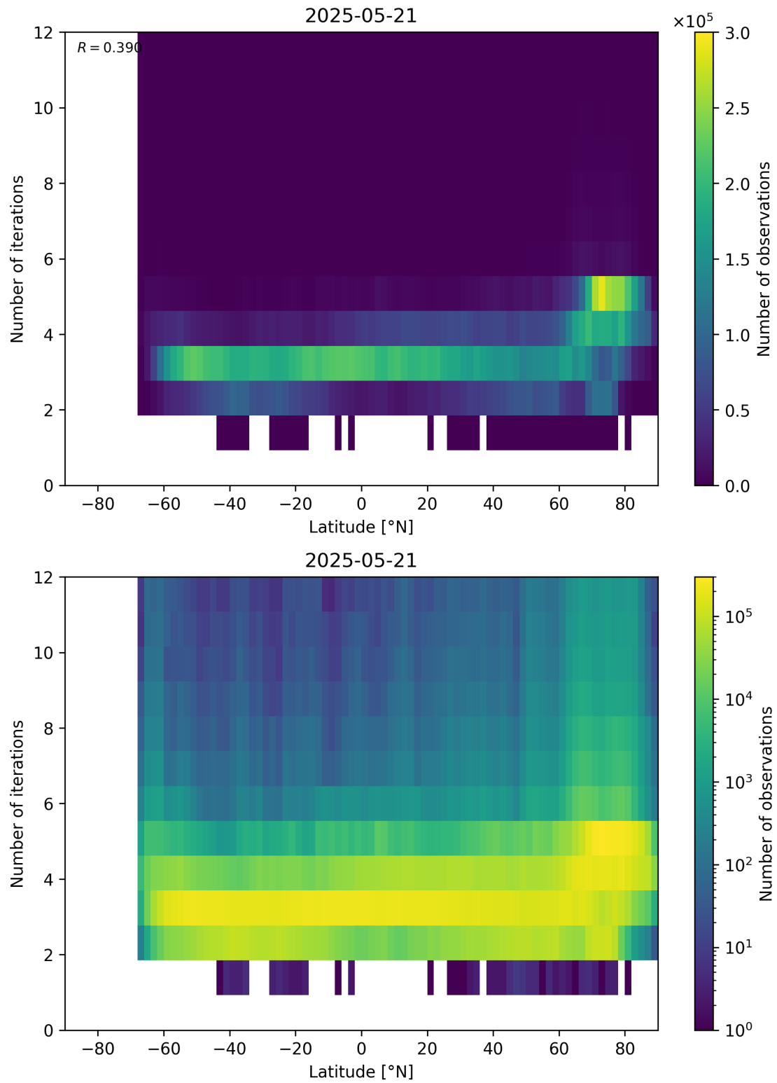
Figure 93: Scatter density plot of “Latitude” against “Number of iterations” for 2025-05-21 to 2025-05-22.
