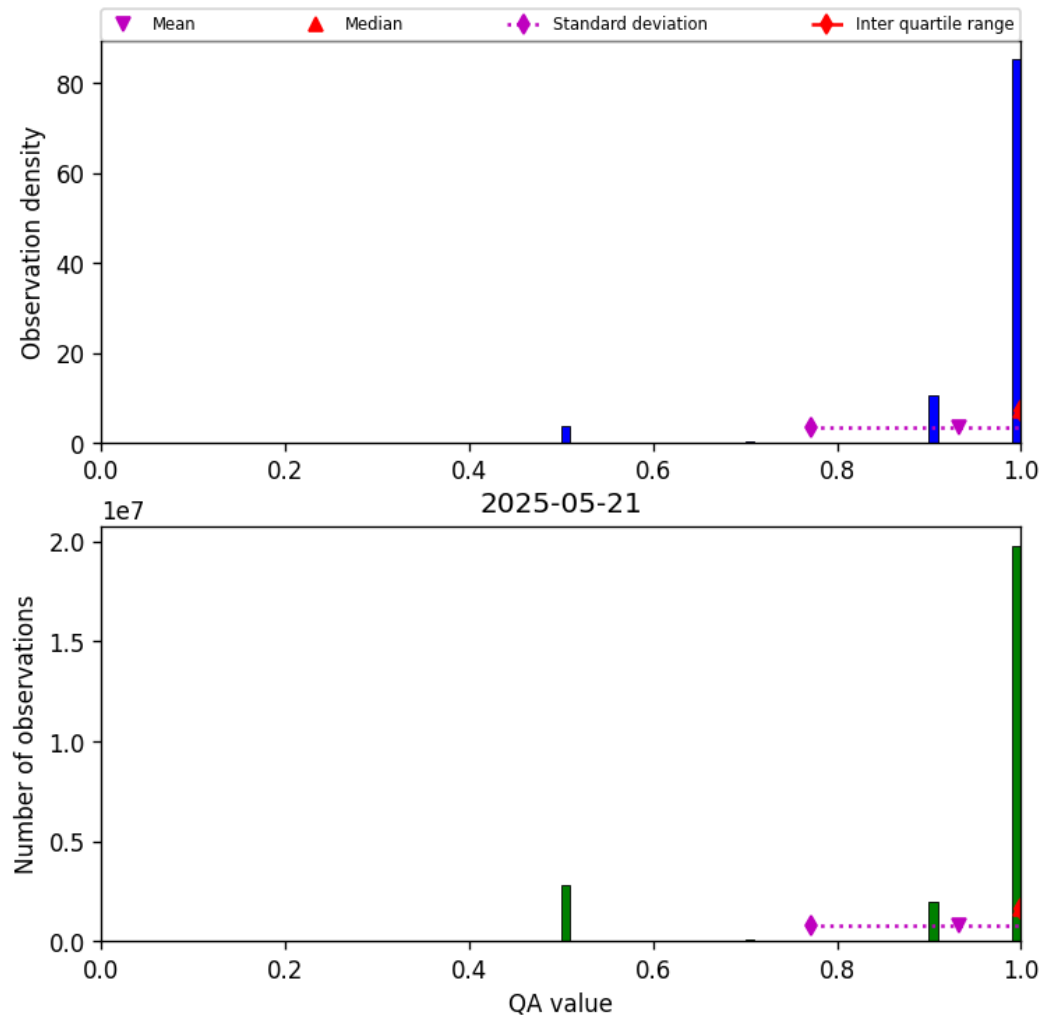
Figure 29: Histogram of “QA value” for 2025-05-21 to 2025-05-22
