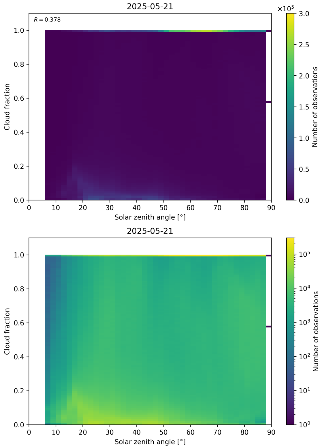
Figure 110: Scatter density plot of “Solar zenith angle” against “Cloud fraction” for 2025-05-21 to 2025-05-22.
