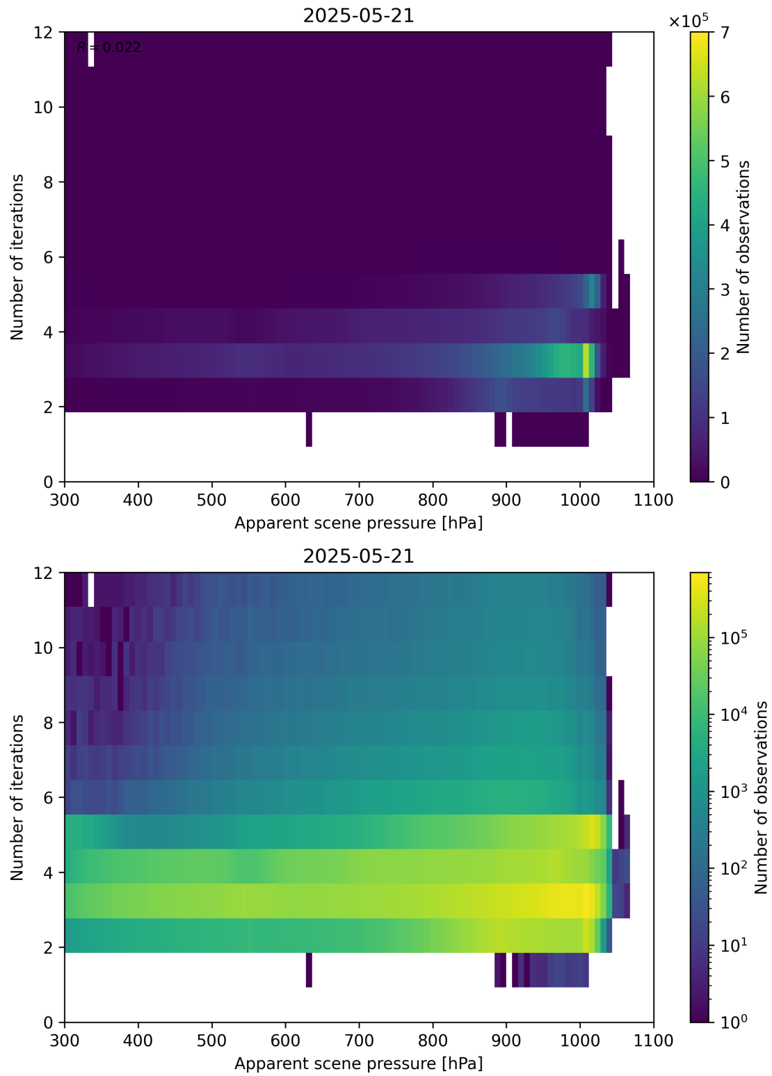
Figure 65: Scatter density plot of “Apparent scene pressure” against “Number of iterations” for 2025-05-21 to 2025-05-22.
