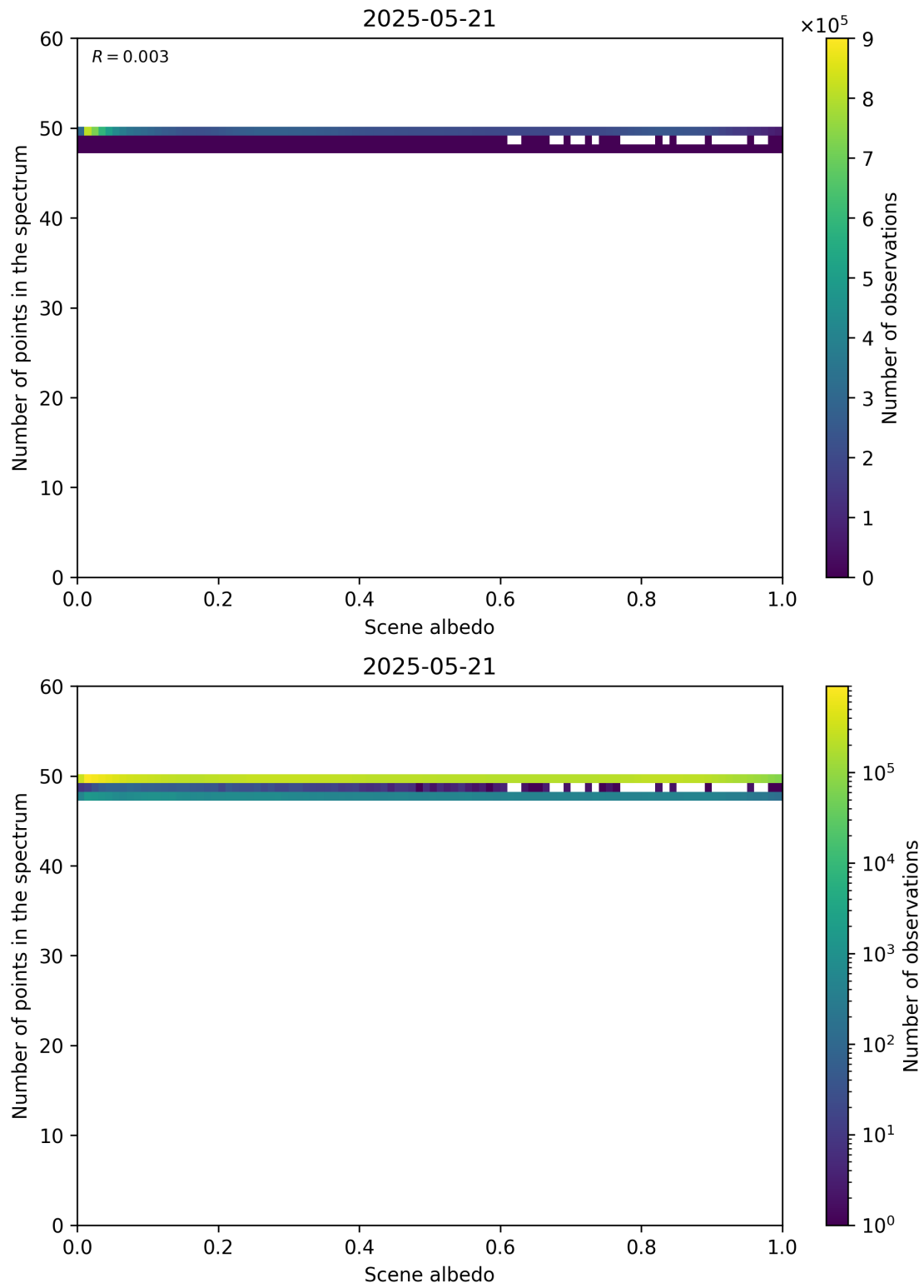
Figure 106: Scatter density plot of “Scene albedo” against “Number of points in the spectrum” for 2025-05-21 to 2025-05-22.
