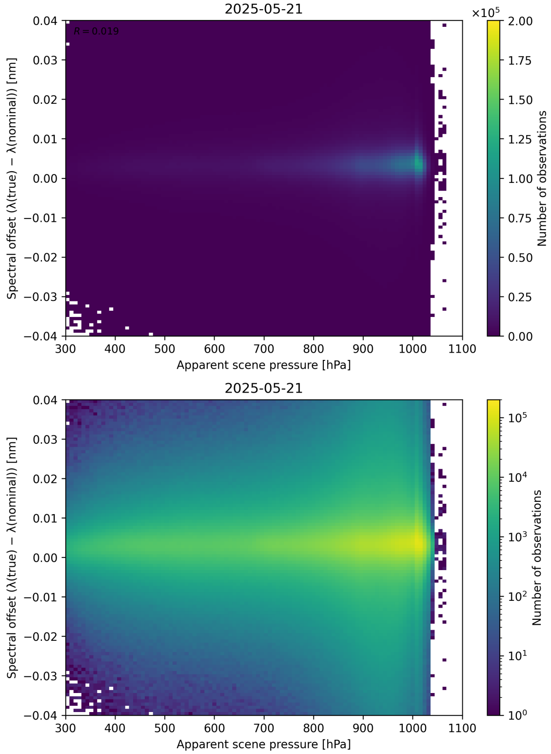
Figure 67: Scatter density plot of “Apparent scene pressure” against “Spectral offset ( \lambda_{\text{true}} - \lambda_{\text{nominal}} )” for 2025-05-21 to 2025-05-22.
