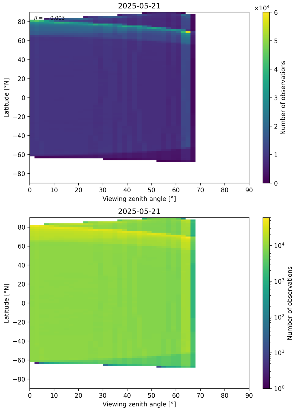
Figure 123: Scatter density plot of “Viewing zenith angle” against “Latitude” for 2025-05-21 to 2025-05-22.
