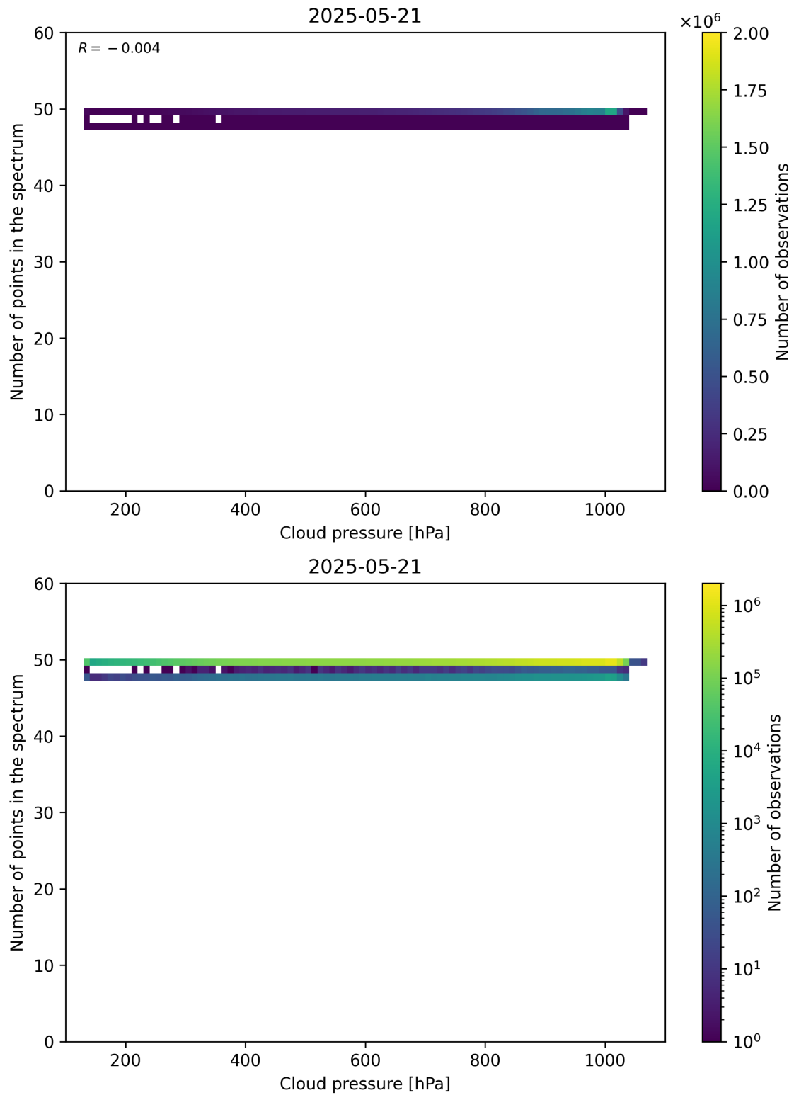
Figure 82: Scatter density plot of “Cloud pressure” against “Number of points in the spectrum” for 2025-05-21 to 2025-05-22.
