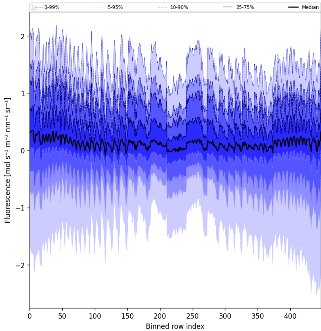
Figure 57: Along track statistics of “Fluorescence” for 2025-05-21 to 2025-05-22
