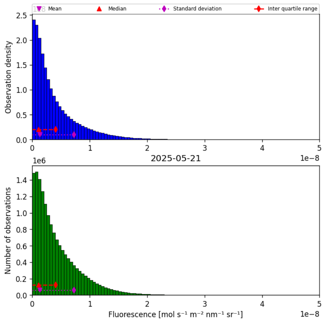
Figure 40: Histogram of “Fluorescence” for 2025-05-21 to 2025-05-22
