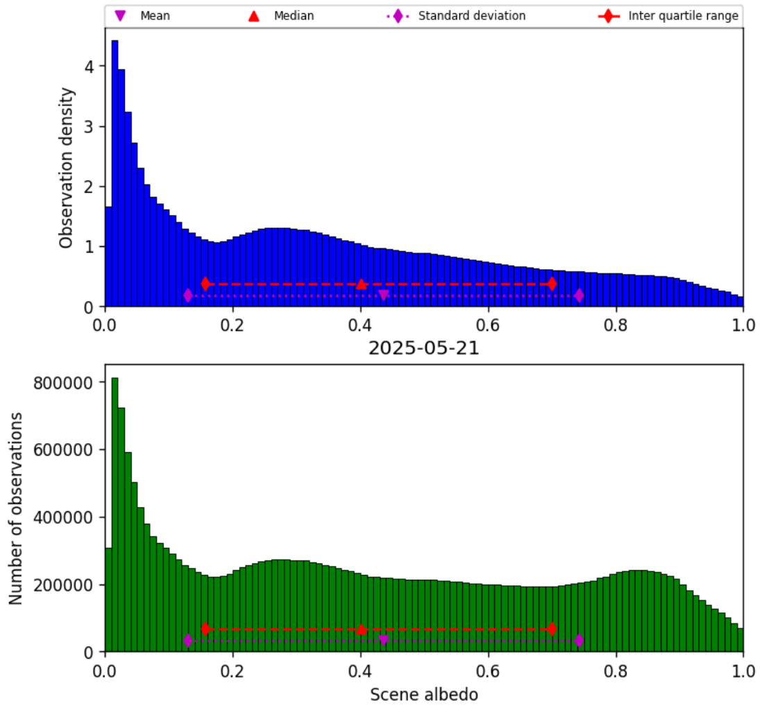
Figure 34: Histogram of “Scene albedo” for 2025-05-21 to 2025-05-22
