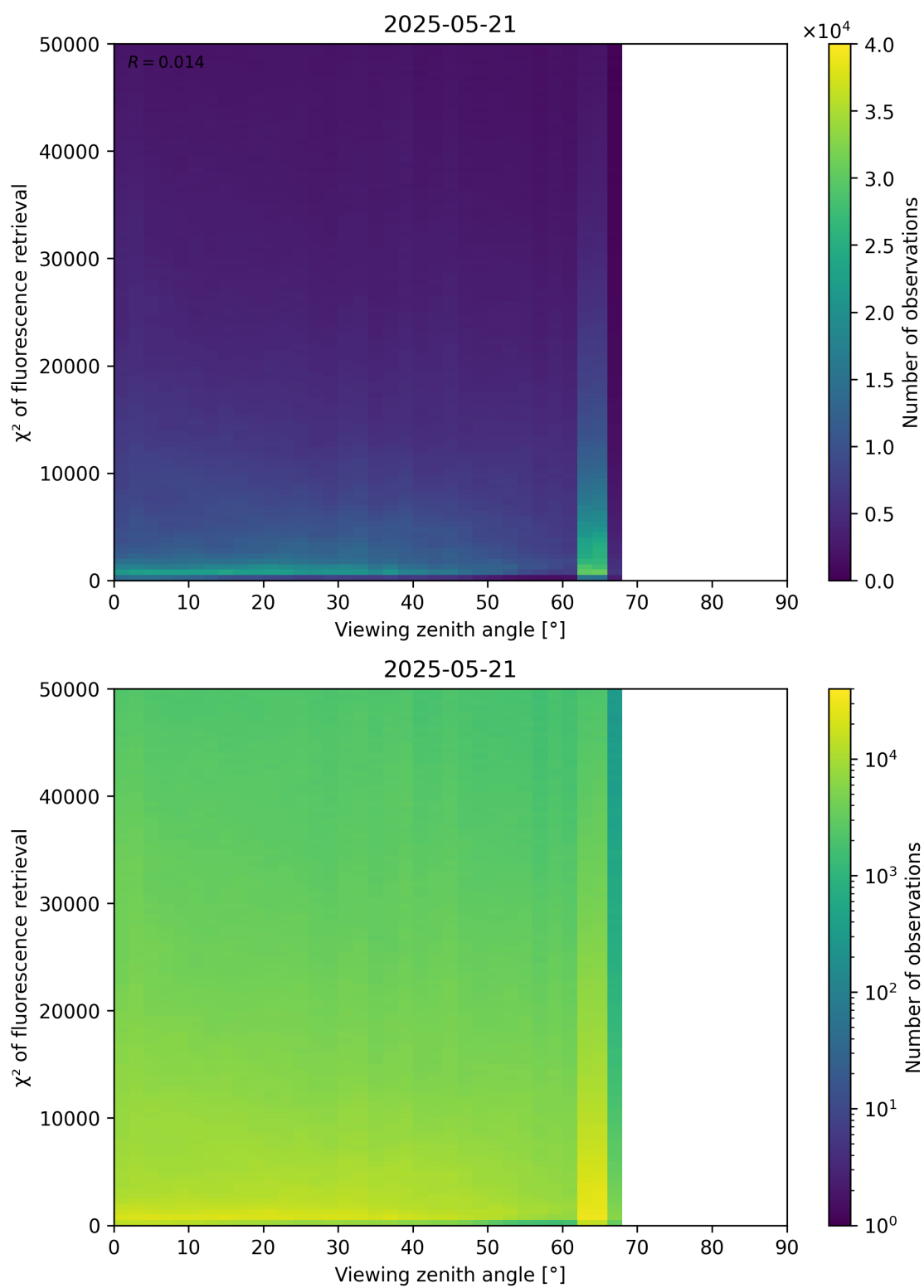
Figure 119: Scatter density plot of “Viewing zenith angle” against “ \chi^2 of fluorescence retrieval” for 2025-05-21 to 2025-05-22.
