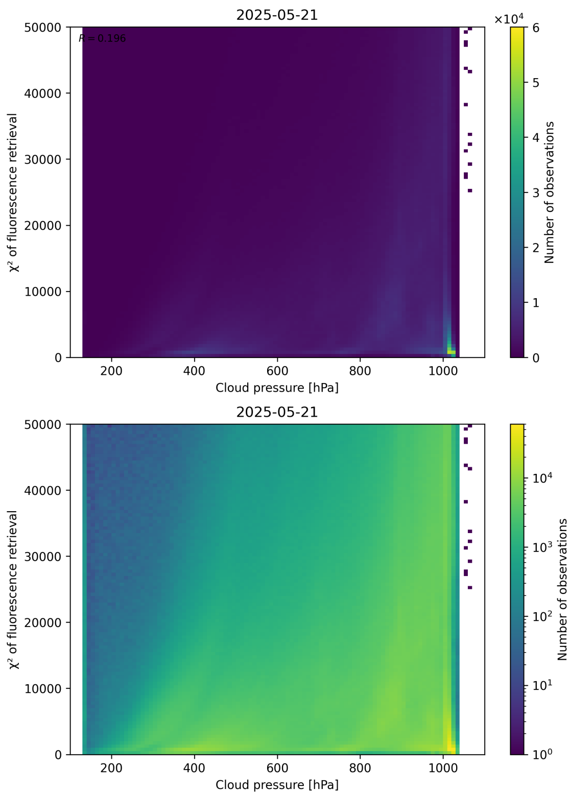
Figure 78: Scatter density plot of “Cloud pressure” against “ \chi^2 of fluorescence retrieval” for 2025-05-21 to 2025-05-22.
