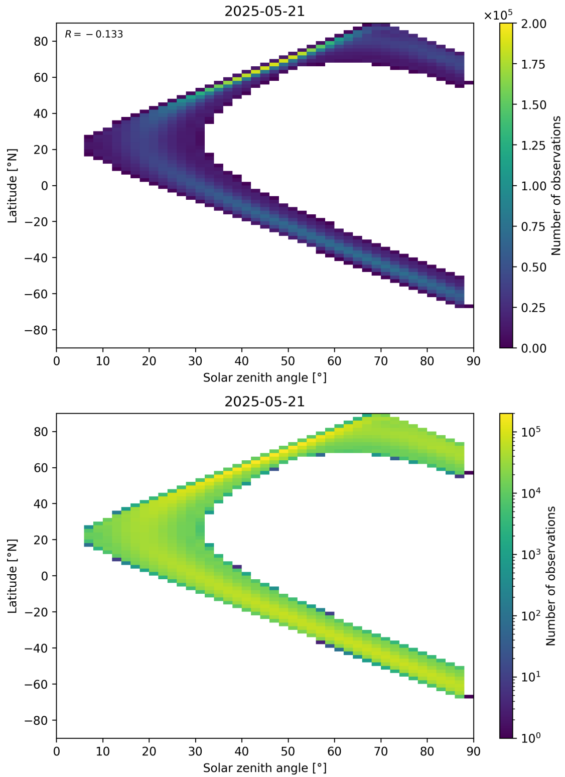
Figure 113: Scatter density plot of “Solar zenith angle” against “Latitude” for 2025-05-21 to 2025-05-22.
