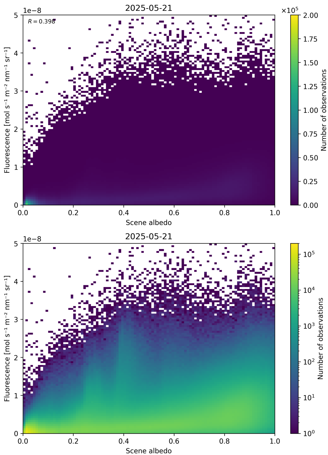
Figure 104: Scatter density plot of “Scene albedo” against “Fluorescence” for 2025-05-21 to 2025-05-22.
