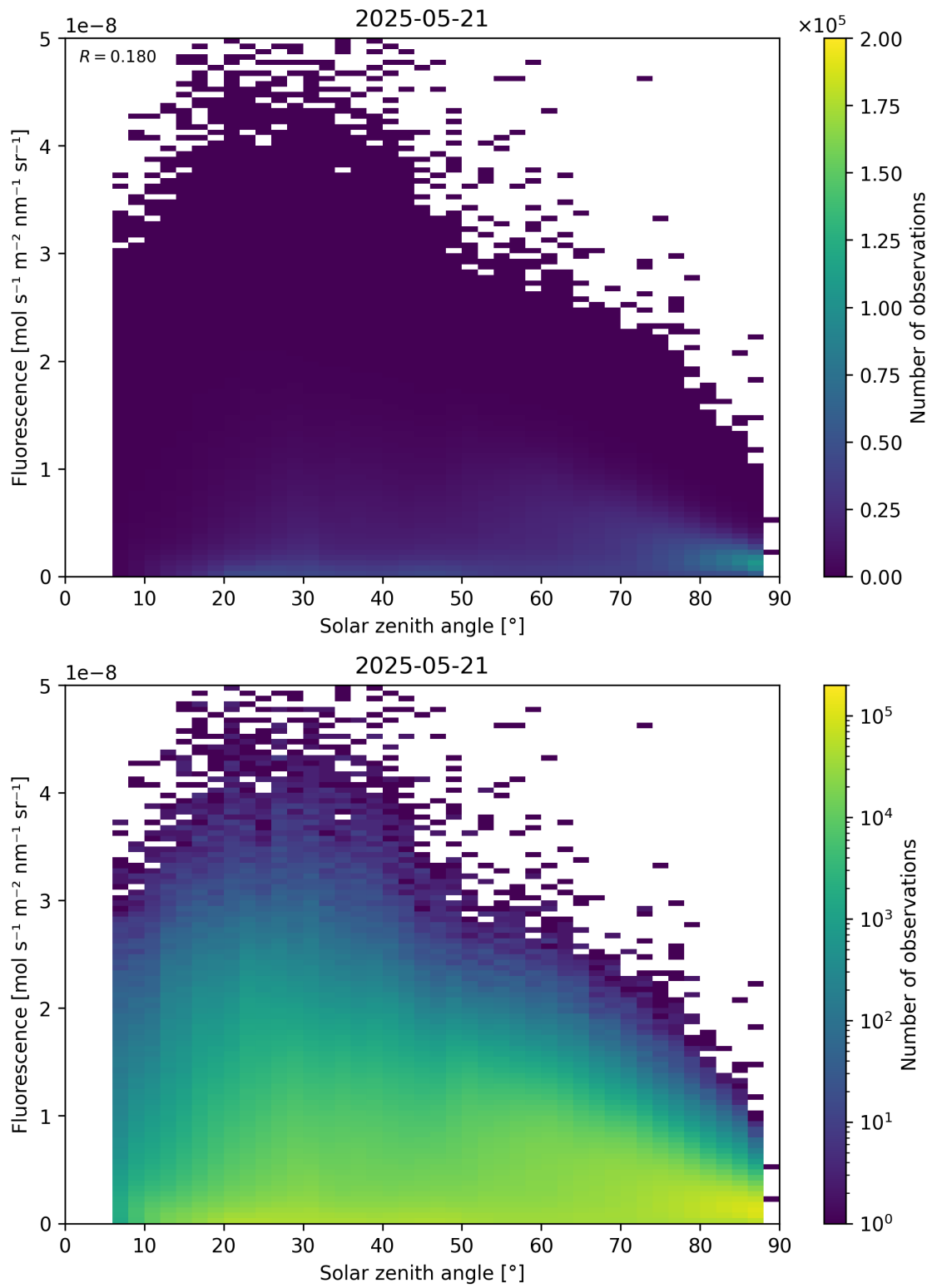
Figure 112: Scatter density plot of “Solar zenith angle” against “Fluorescence” for 2025-05-21 to 2025-05-22.
