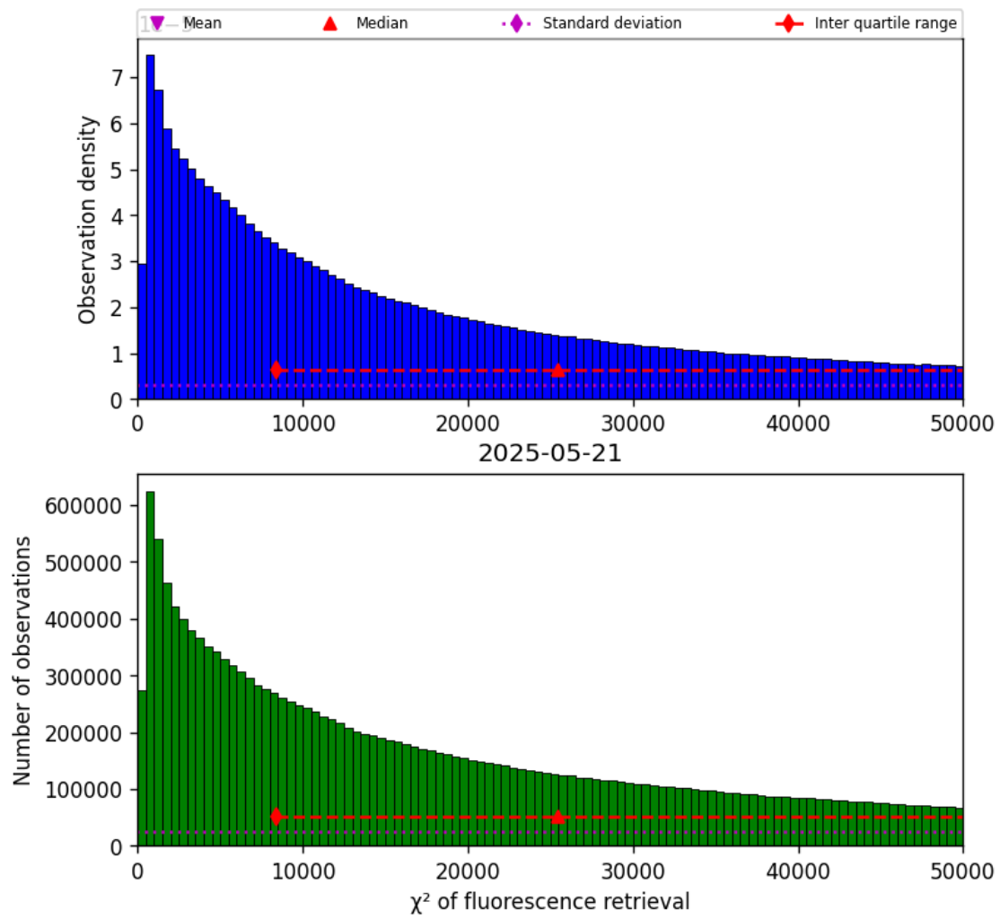
Figure 42: Histogram of “ \chi^2 of fluorescence retrieval” for 2025-05-21 to 2025-05-22
