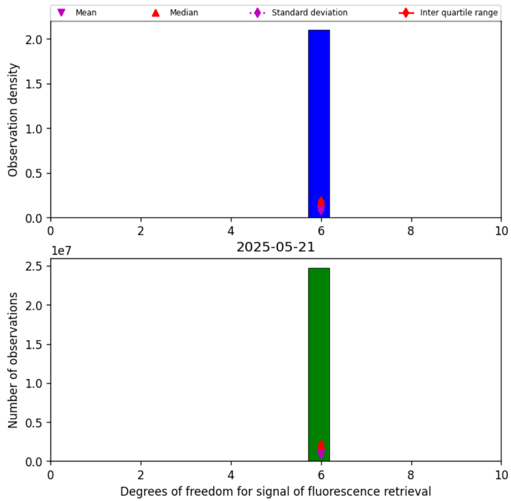
Figure 43: Histogram of “Degrees of freedom for signal of fluorescence retrieval” for 2025-05-21 to 2025-05-22
