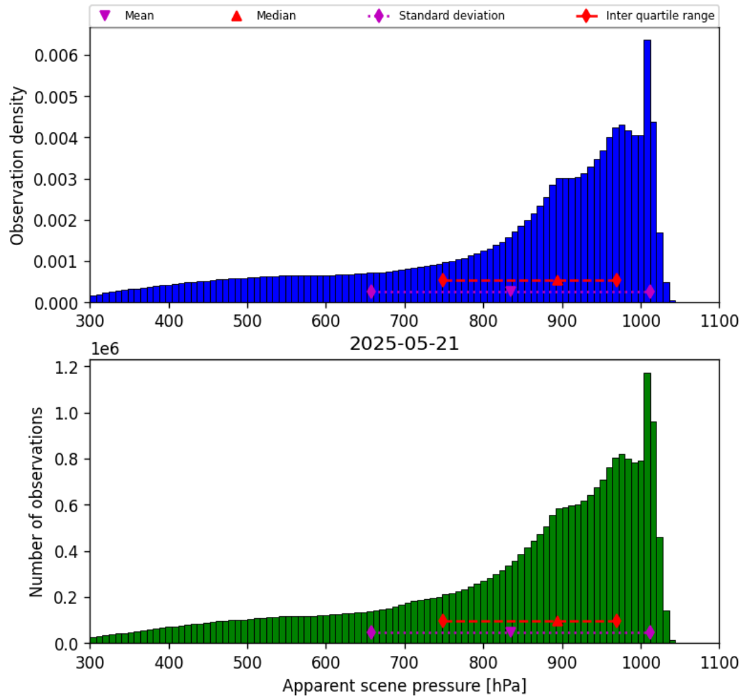
Figure 36: Histogram of “Apparent scene pressure” for 2025-05-21 to 2025-05-22
