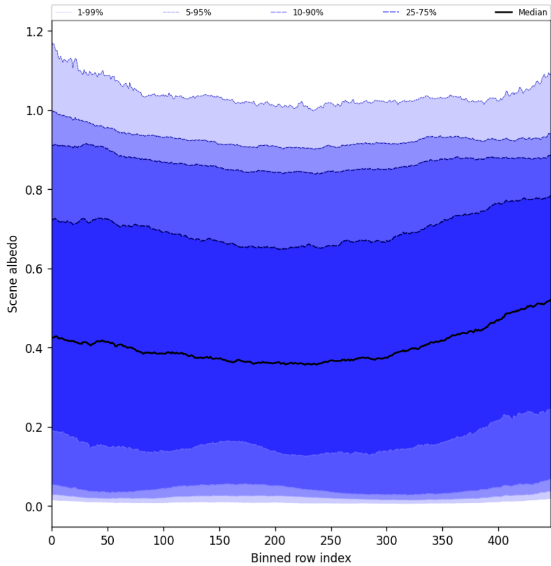
Figure 51: Along track statistics of “Scene albedo” for 2025-05-21 to 2025-05-22
