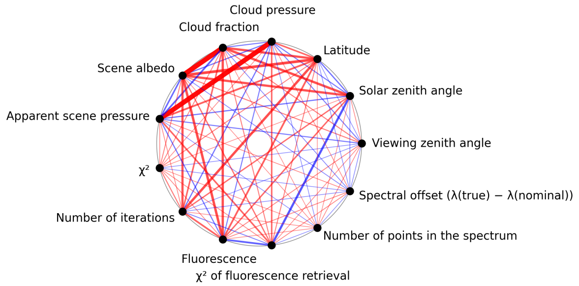
Figure 1: Map of correlation graph for 2025-05-21 to 2025-05-22.
