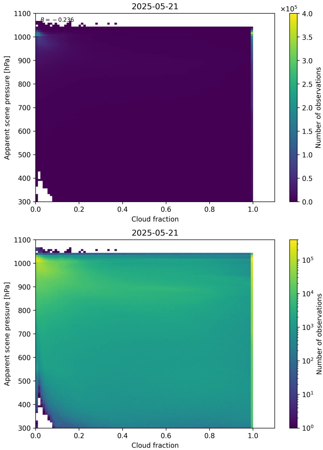
Figure 70: Scatter density plot of “Cloud fraction” against “Apparent scene pressure” for 2025-05-21 to 2025-05-22.
