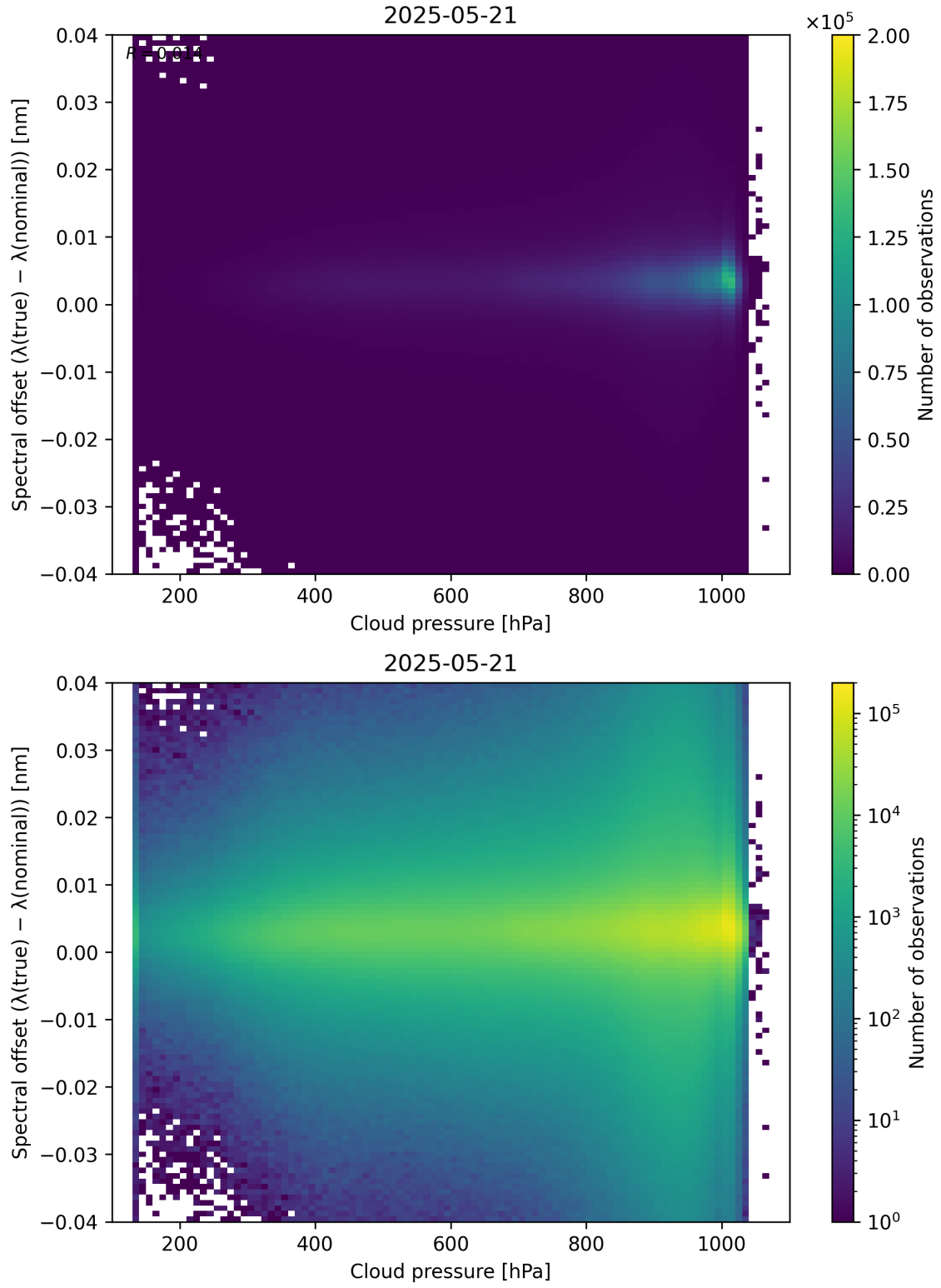
Figure 84: Scatter density plot of “Cloud pressure” against “Spectral offset ( \lambda_{\text{true}} - \lambda_{\text{nominal}} )” for 2025-05-21 to 2025-05-22.
