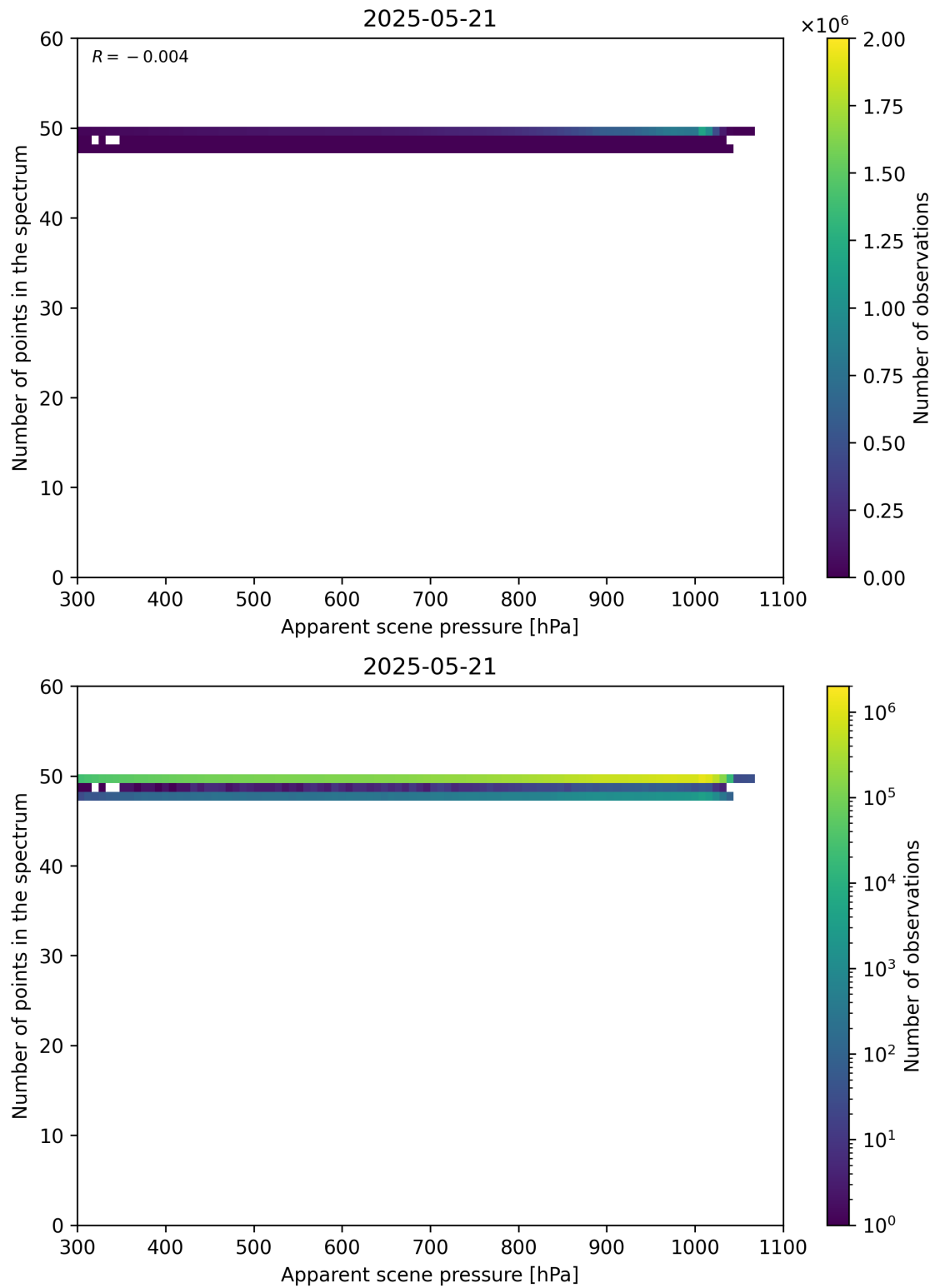
Figure 66: Scatter density plot of “Apparent scene pressure” against “Number of points in the spectrum” for 2025-05-21 to 2025-05-22.
