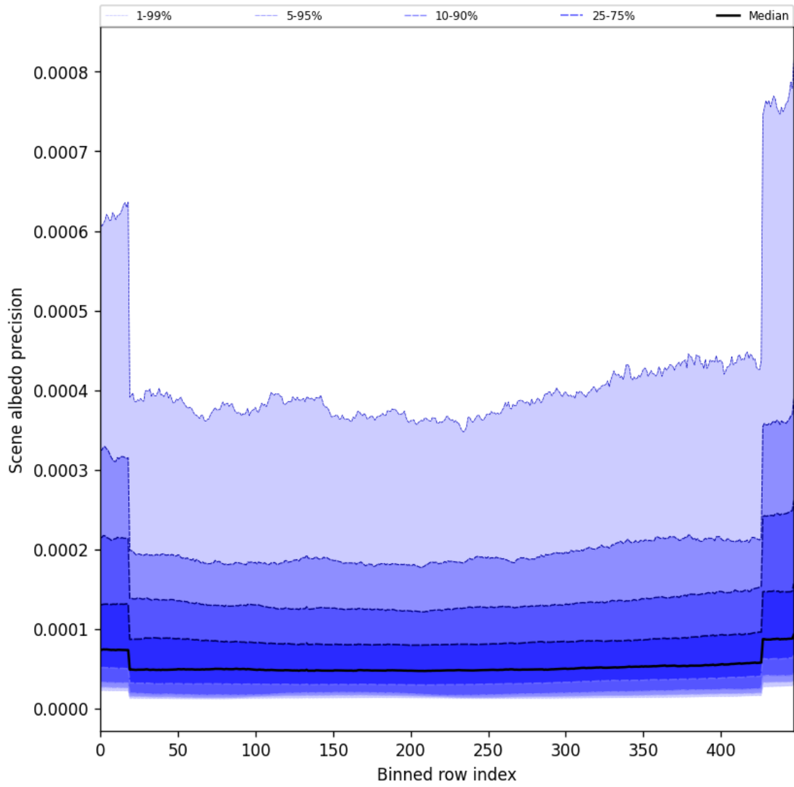
Figure 52: Along track statistics of “Scene albedo precision” for 2025-05-21 to 2025-05-22
