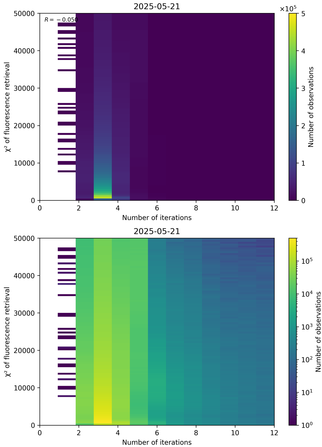
Figure 97: Scatter density plot of “Number of iterations” against “ \chi^2 of fluorescence retrieval” for 2025-05-21 to 2025-05-22.
