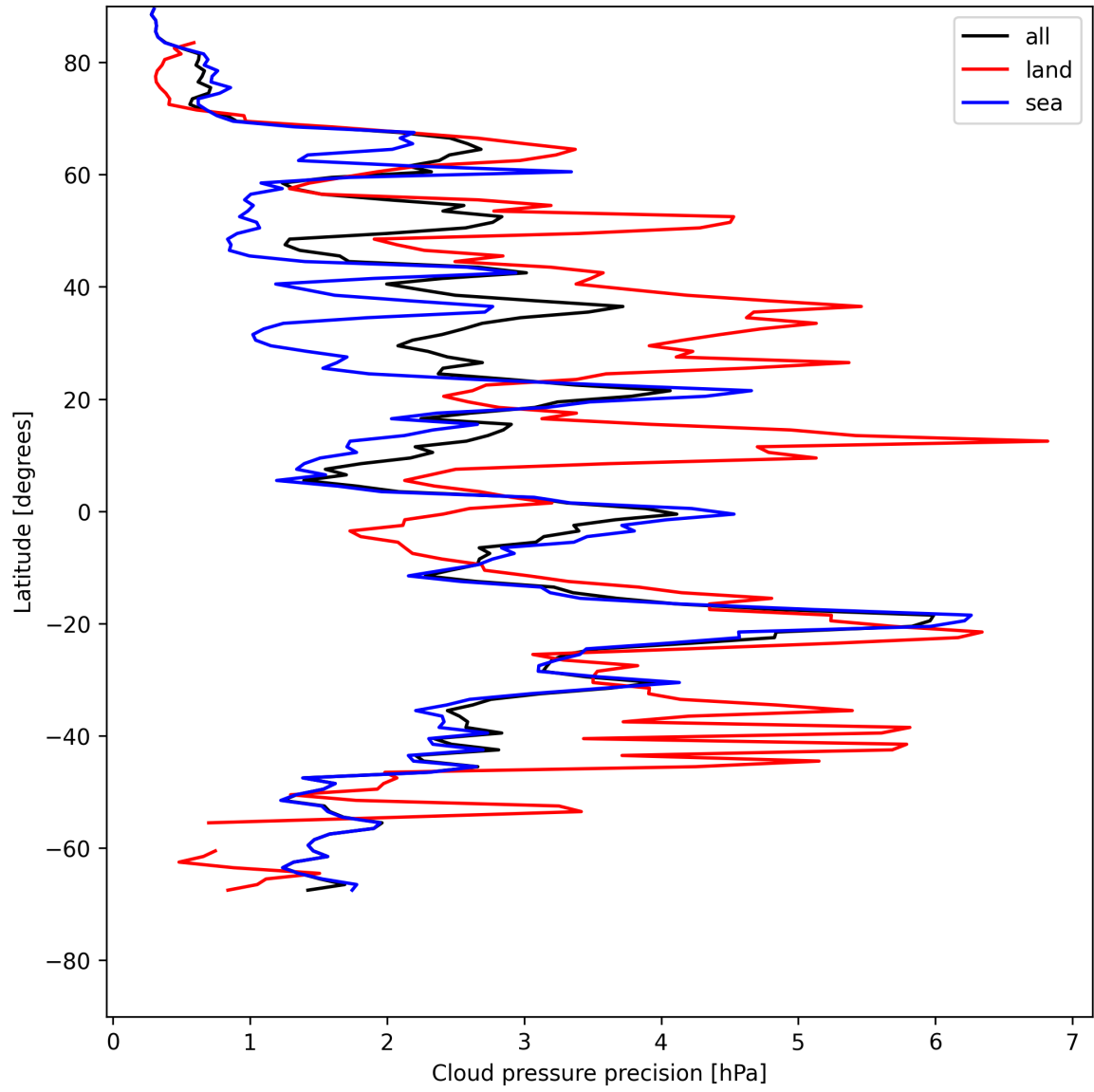
Figure 14: Zonal average of "Cloud pressure precision" for 2025-05-21 to 2025-05-22.
