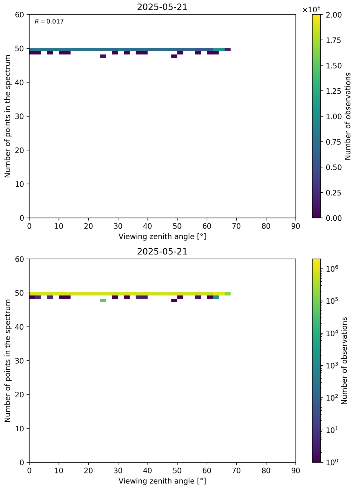
Figure 125: Scatter density plot of “Viewing zenith angle” against “Number of points in the spectrum” for 2025-05-21 to 2025-05-22.
