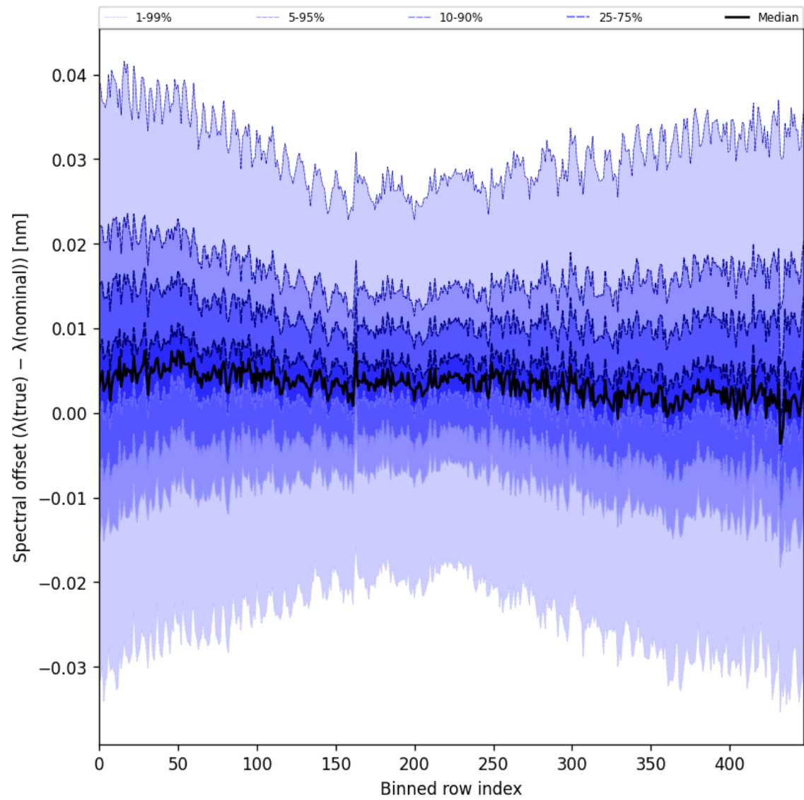
Figure 62: Along track statistics of “Spectral offset ( \lambda_{\text{true}} - \lambda_{\text{nominal}} )” for 2025-05-21 to 2025-05-22
