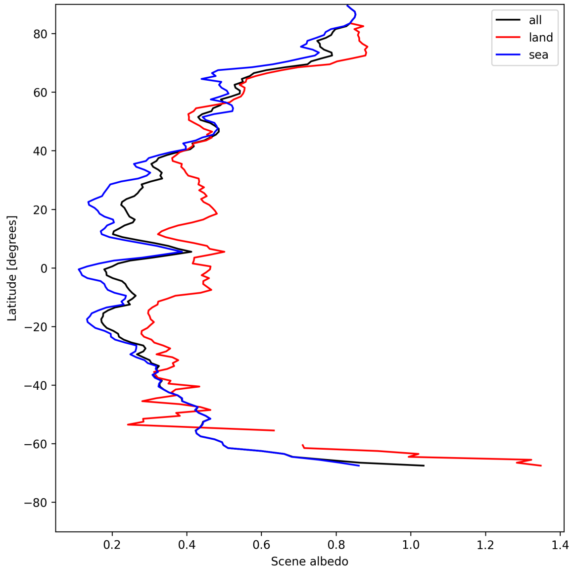
Figure 17: Zonal average of “Scene albedo” for 2025-05-21 to 2025-05-22.
