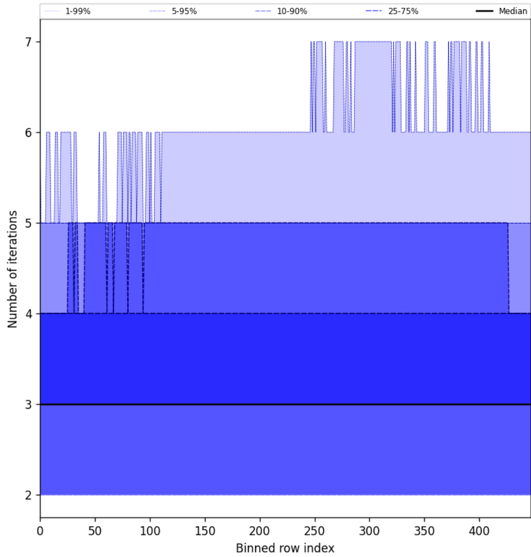
Figure 56: Along track statistics of “Number of iterations” for 2025-05-21 to 2025-05-22
