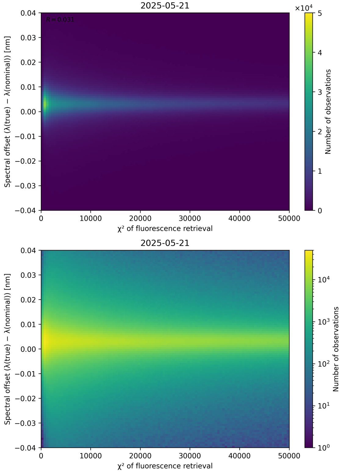
Figure 69: Scatter density plot of “ \chi^2 of fluorescence retrieval” against “Spectral offset ( \lambda_{\text{true}} - \lambda_{\text{nominal}} )” for 2025-05-21 to 2025-05-22.
