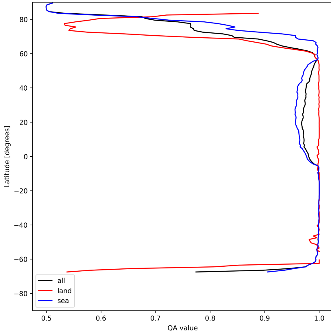
Figure 12: Zonal average of “QA value” for 2025-05-21 to 2025-05-22.
