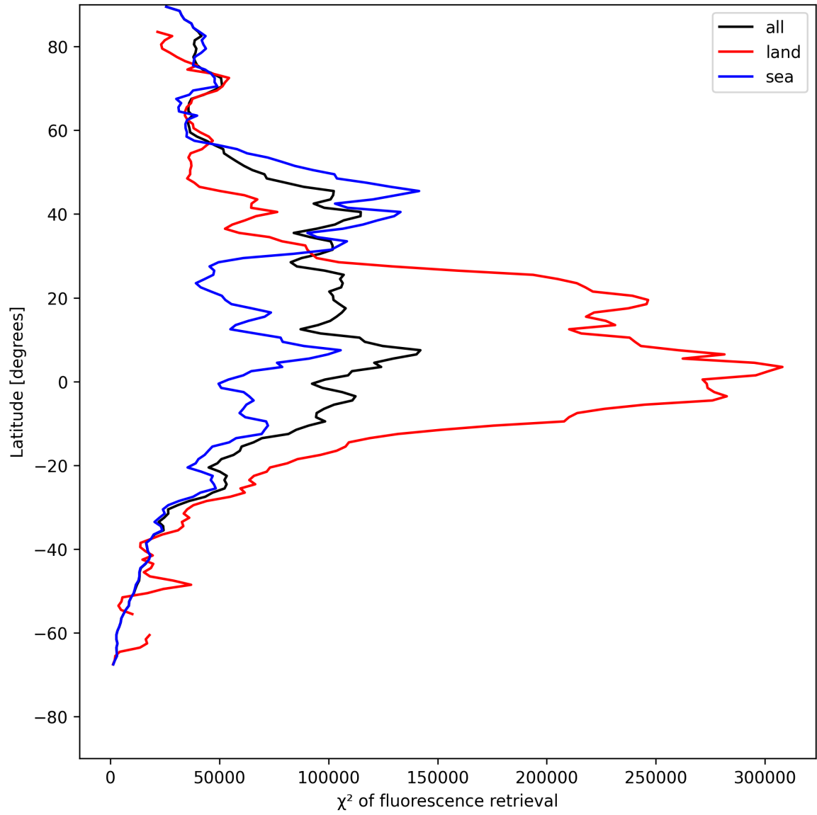
Figure 25: Zonal average of “ \chi^2 of fluorescence retrieval” for 2025-05-21 to 2025-05-22.
