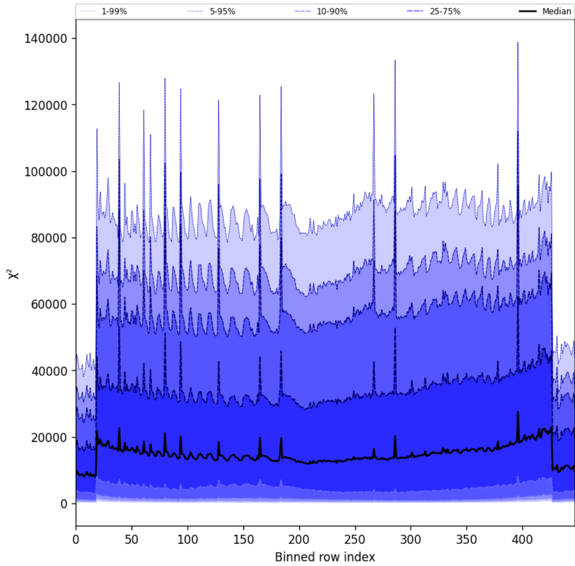
Figure 55: Along track statistics of “ \chi^2 ” for 2025-05-21 to 2025-05-22
