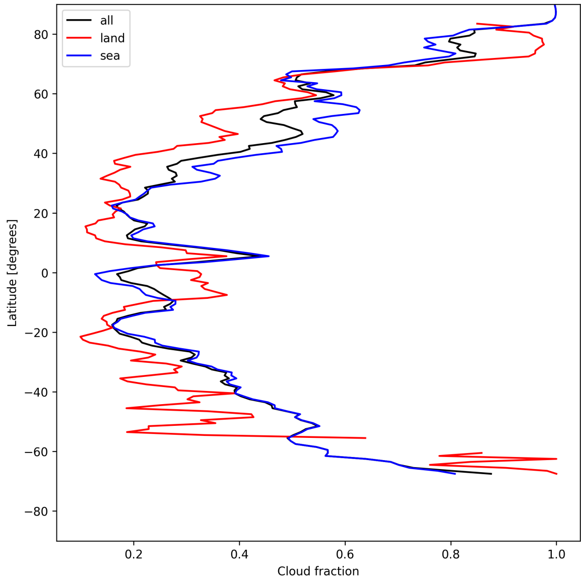
Figure 15: Zonal average of “Cloud fraction” for 2025-05-21 to 2025-05-22.
