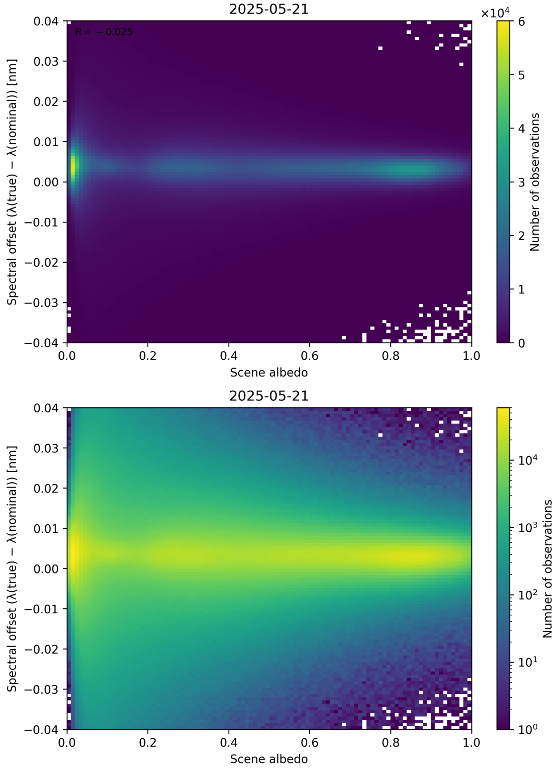
Figure 107: Scatter density plot of “Scene albedo” against “Spectral offset ( \lambda_{\text{true}} - \lambda_{\text{nominal}} )” for 2025-05-21 to 2025-05-22.
