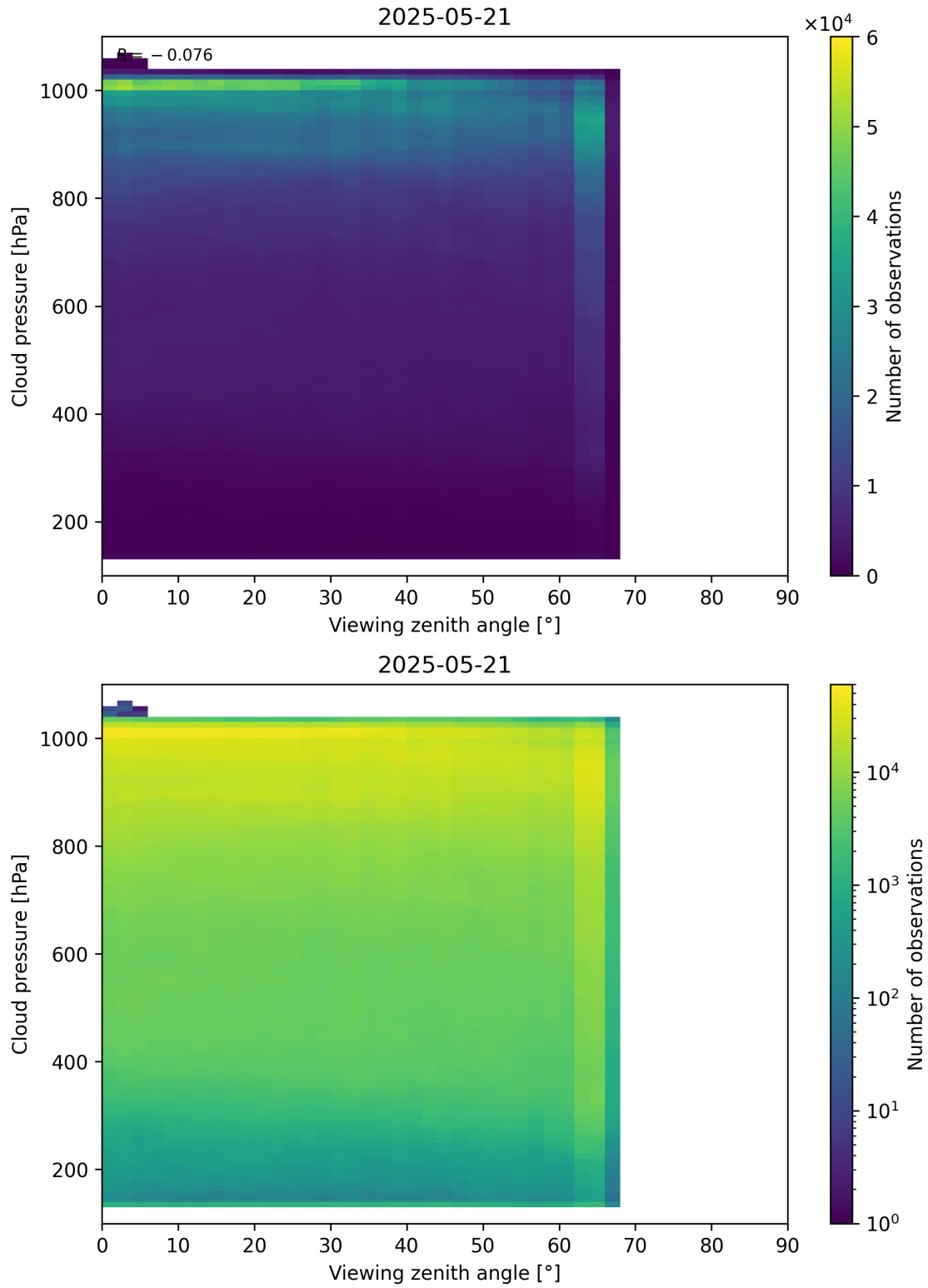
Figure 121: Scatter density plot of “Viewing zenith angle” against “Cloud pressure” for 2025-05-21 to 2025-05-22.
