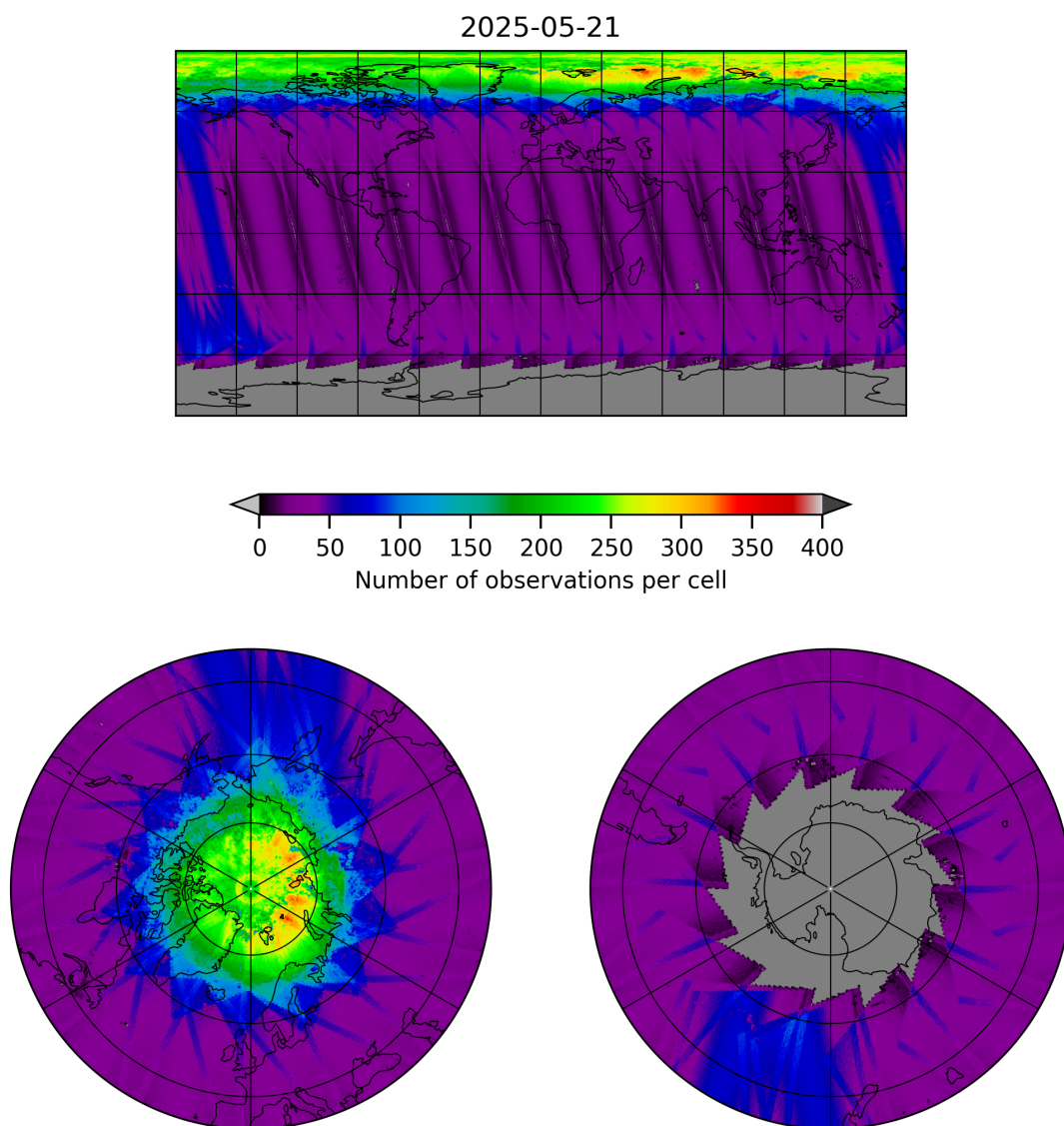
Figure 11: Map of the number of observations for 2025-05-21 to 2025-05-22
