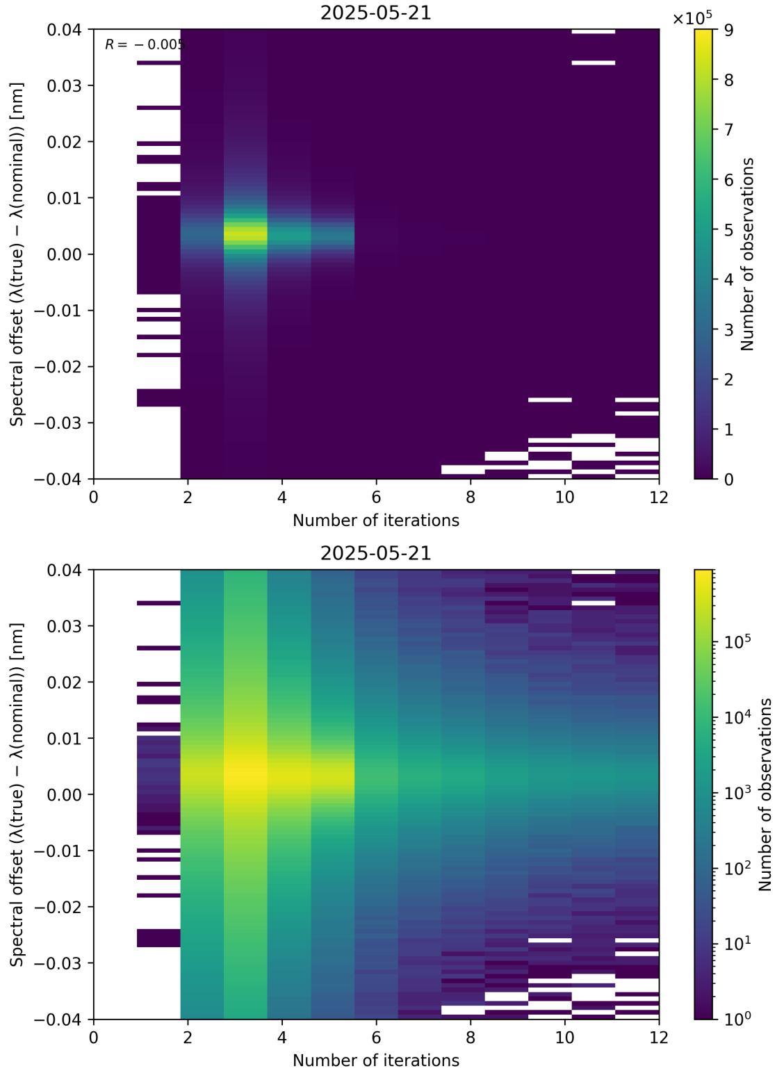
Figure 100: Scatter density plot of “Number of iterations” against “Spectral offset ( \lambda_{\text{true}} - \lambda_{\text{nominal}} )” for 2025-05-21 to 2025-05-22.
