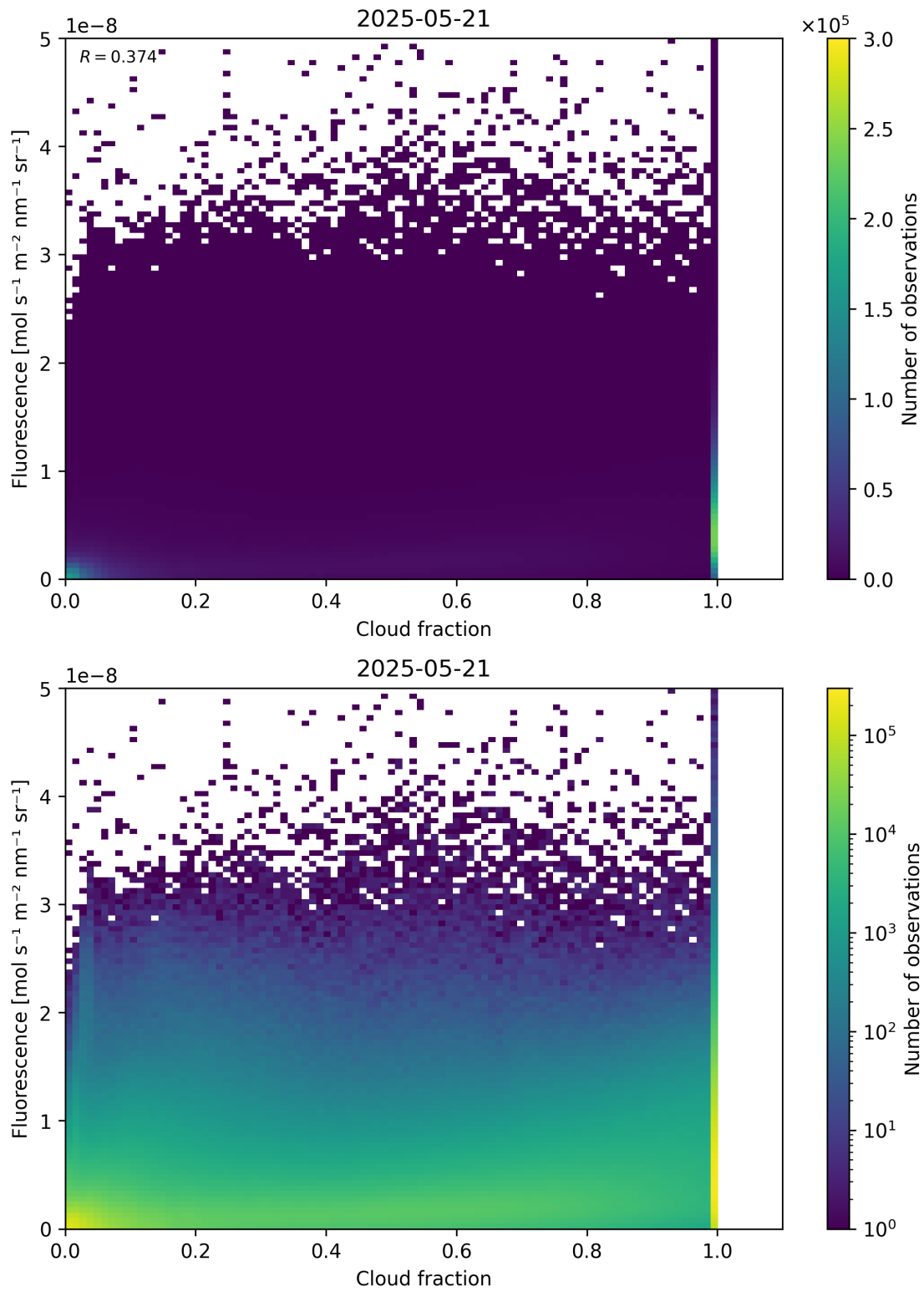
Figure 72: Scatter density plot of “Cloud fraction” against “Fluorescence” for 2025-05-21 to 2025-05-22.
