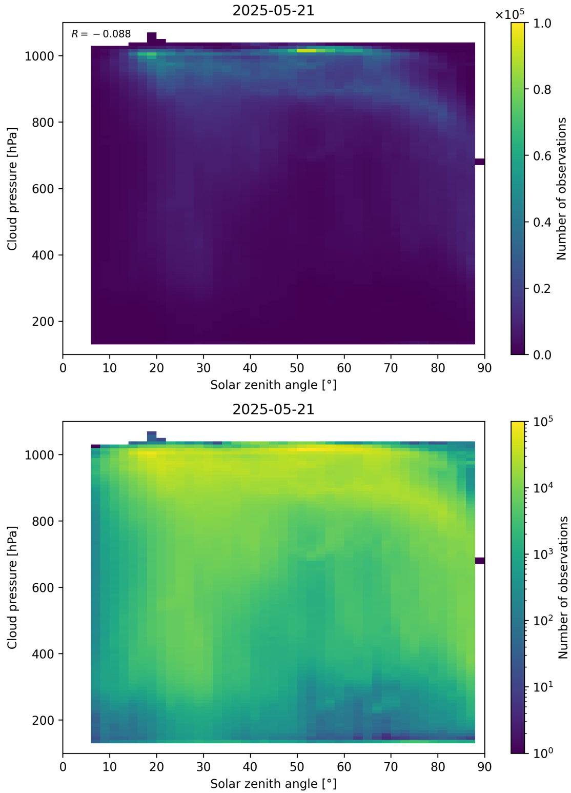
Figure 111: Scatter density plot of “Solar zenith angle” against “Cloud pressure” for 2025-05-21 to 2025-05-22.
