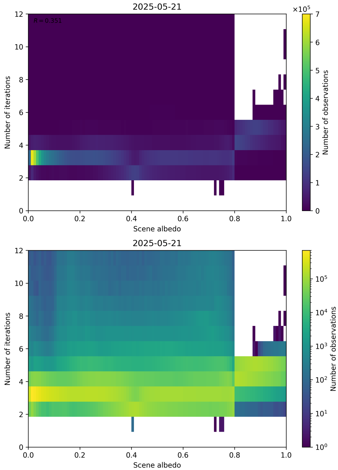
Figure 105: Scatter density plot of “Scene albedo” against “Number of iterations” for 2025-05-21 to 2025-05-22.
