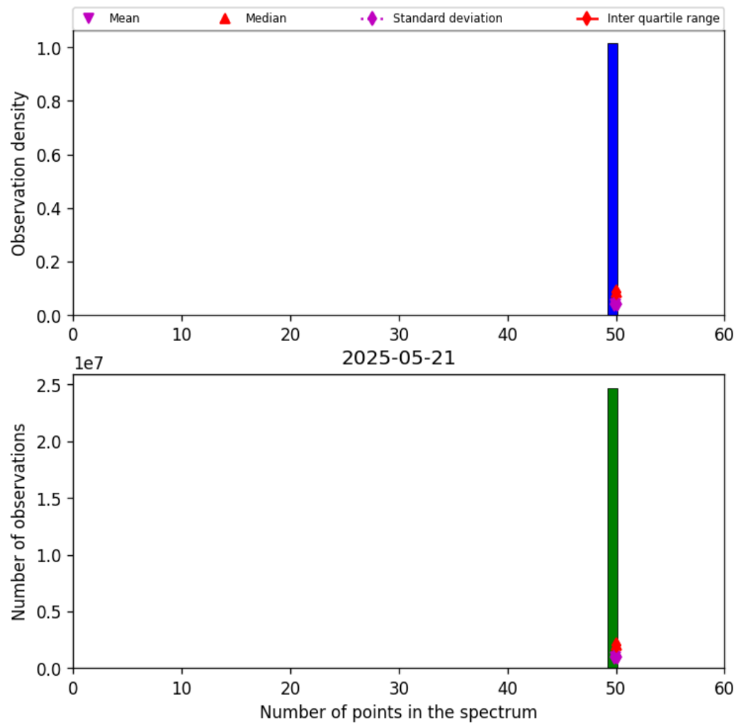
Figure 44: Histogram of “Number of points in the spectrum” for 2025-05-21 to 2025-05-22
