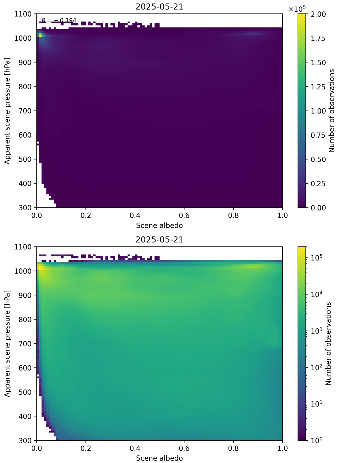
Figure 102: Scatter density plot of “Scene albedo” against “Apparent scene pressure” for 2025-05-21 to 2025-05-22.
