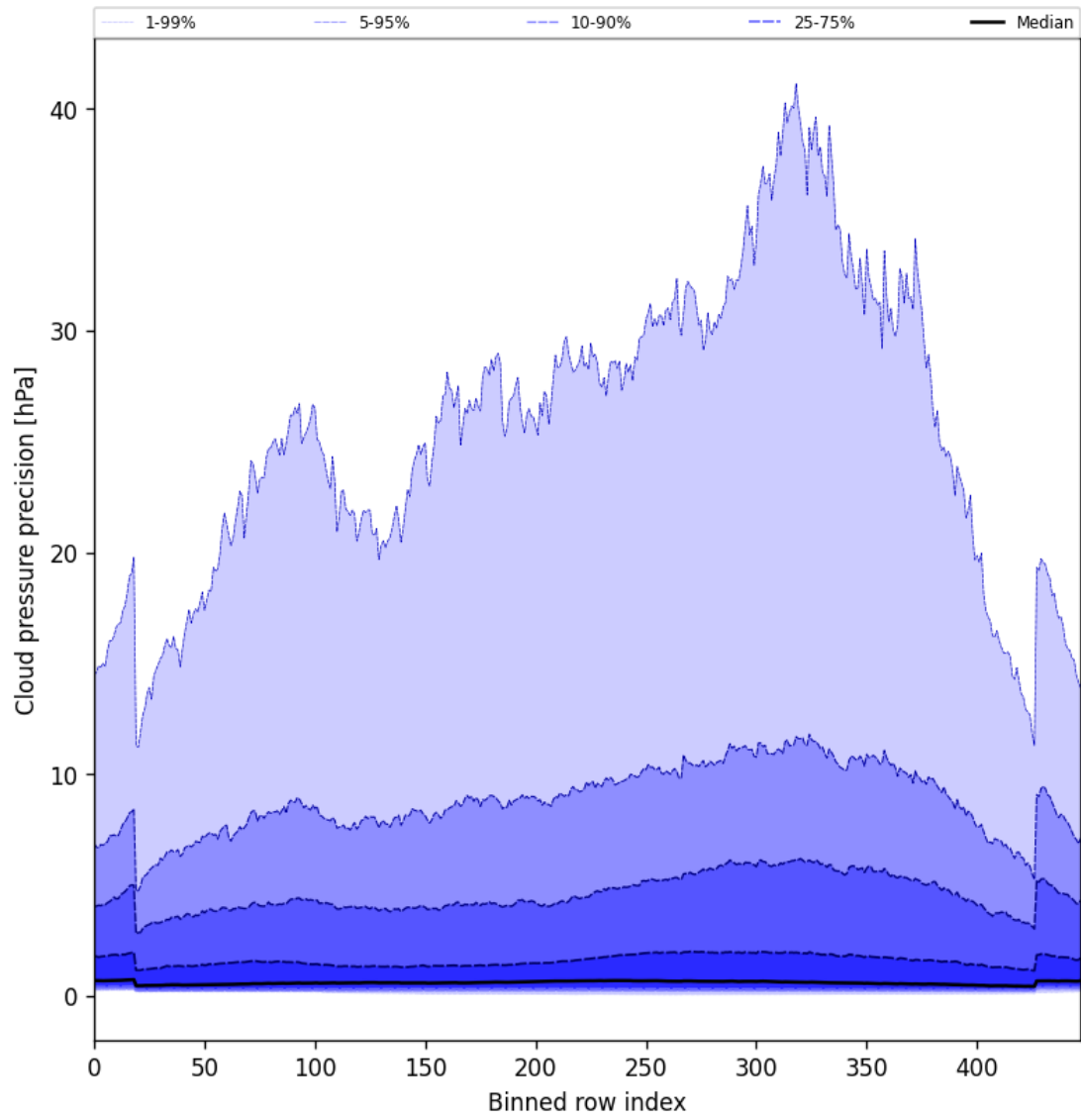
Figure 48: Along track statistics of “Cloud pressure precision” for 2025-05-21 to 2025-05-22
