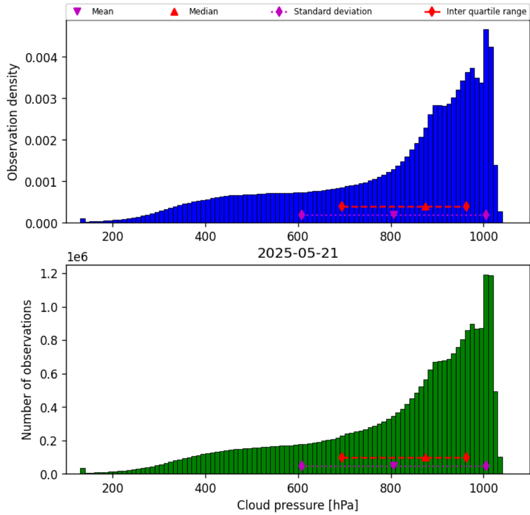
Figure 30: Histogram of “Cloud pressure” for 2025-05-21 to 2025-05-22
