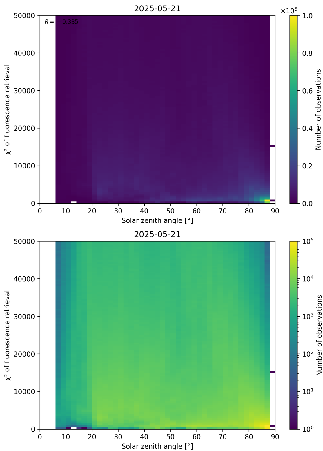
Figure 109: Scatter density plot of “Solar zenith angle” against “ \chi^2 of fluorescence retrieval” for 2025-05-21 to 2025-05-22.
