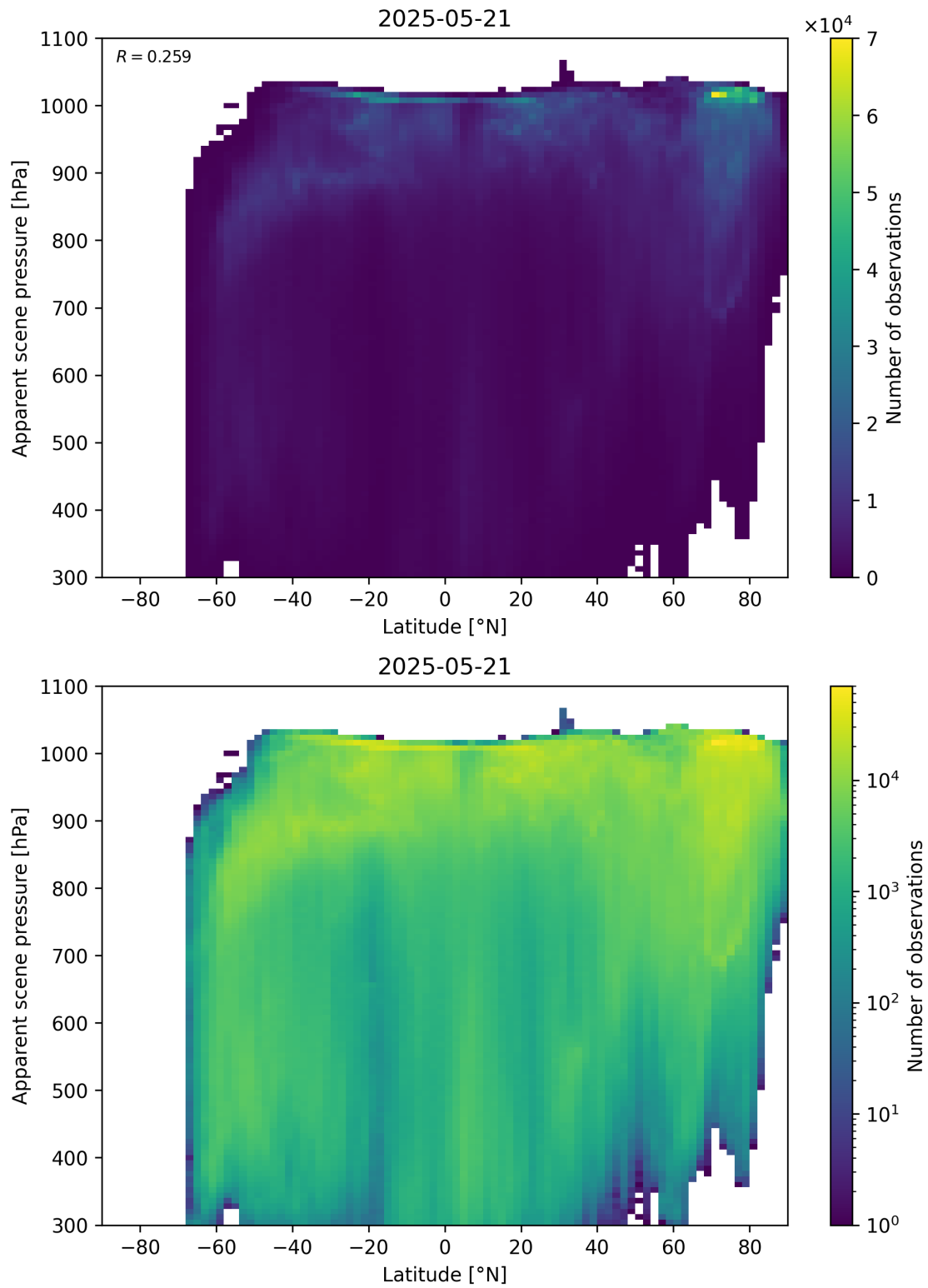
Figure 88: Scatter density plot of “Latitude” against “Apparent scene pressure” for 2025-05-21 to 2025-05-22.
