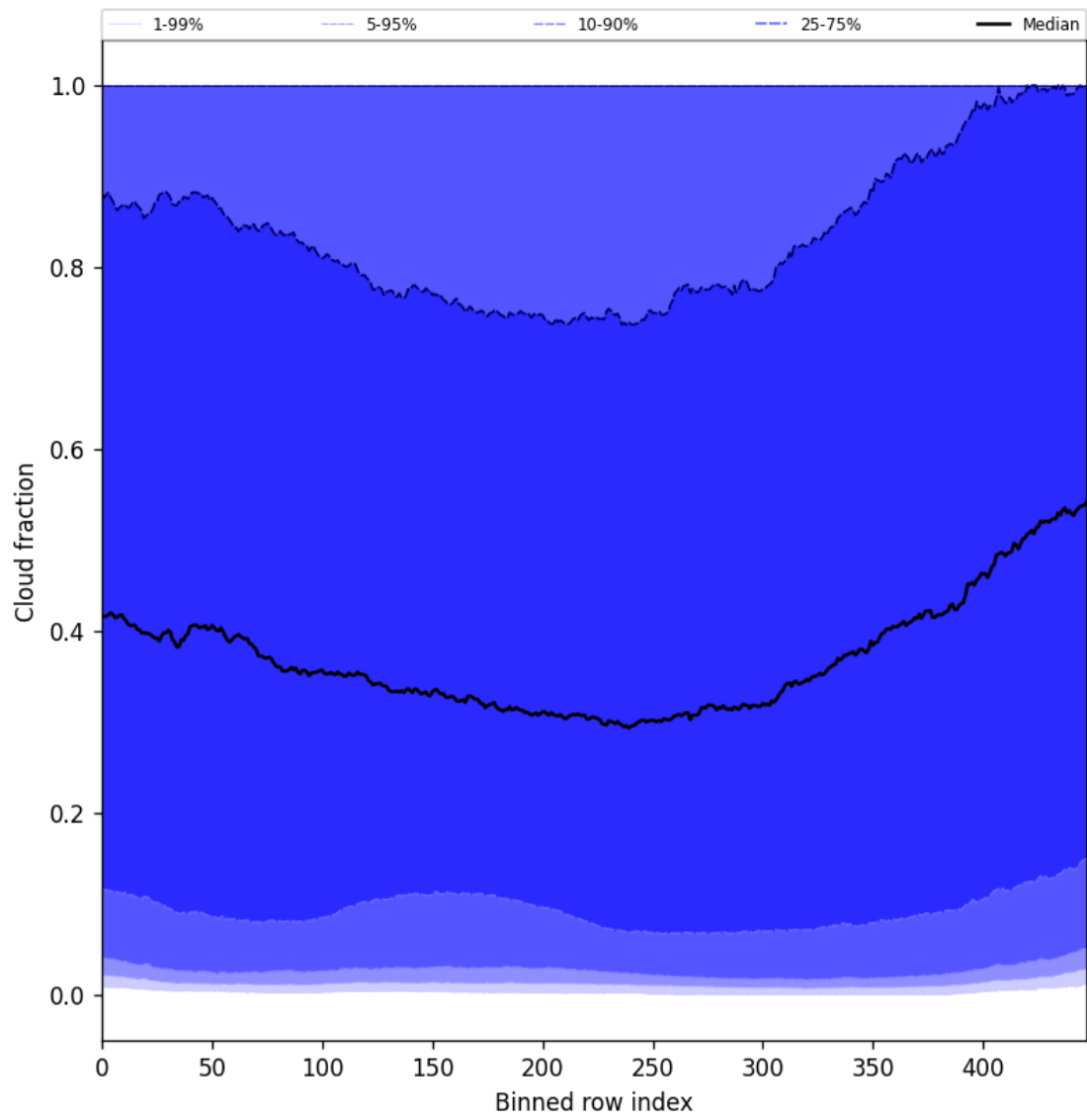
Figure 49: Along track statistics of “Cloud fraction” for 2025-05-21 to 2025-05-22
