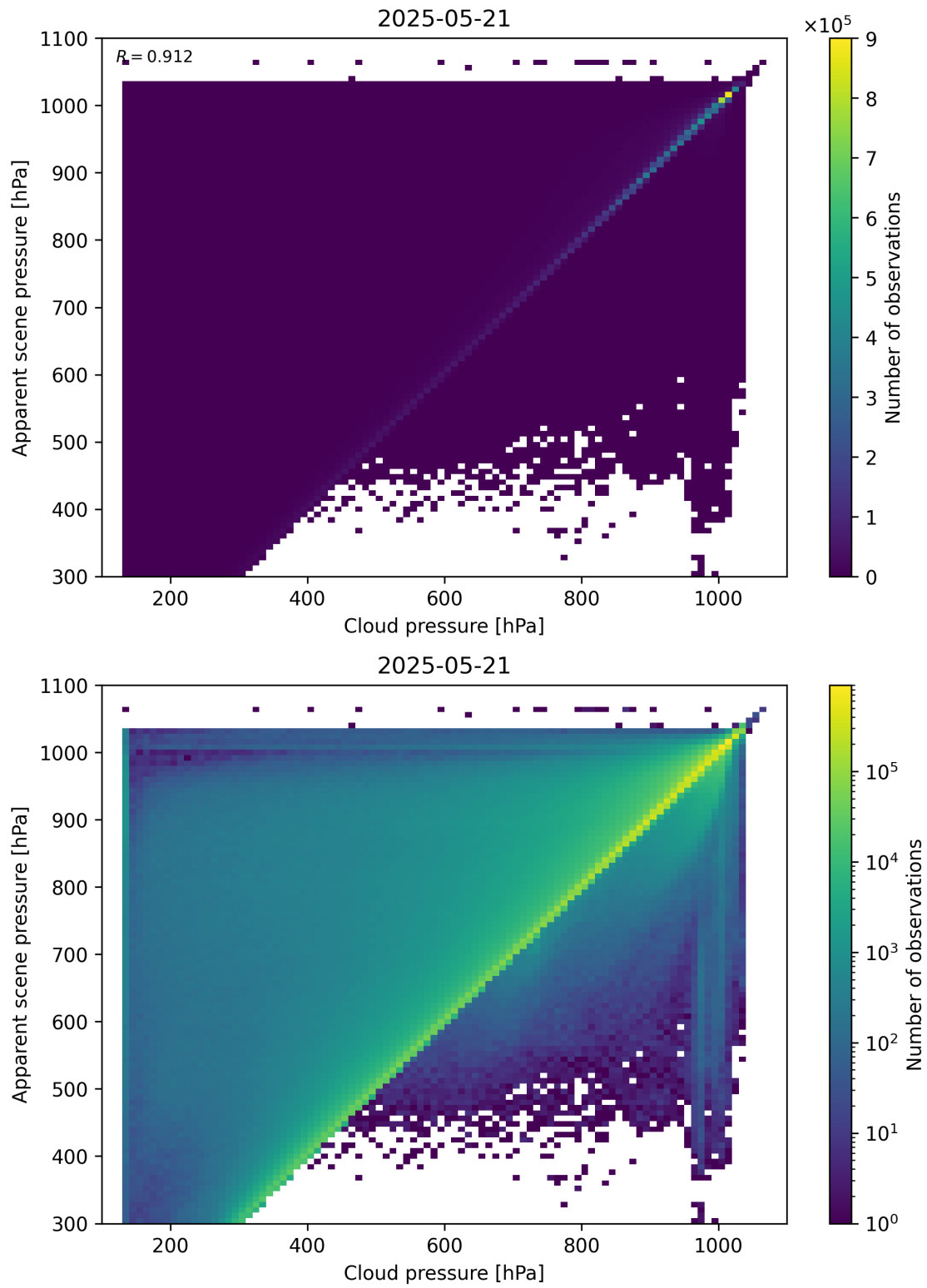
Figure 77: Scatter density plot of “Cloud pressure” against “Apparent scene pressure” for 2025-05-21 to 2025-05-22.
