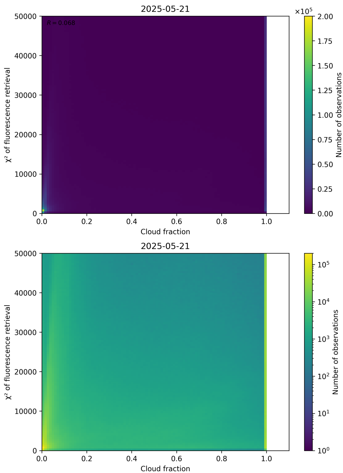
Figure 71: Scatter density plot of “Cloud fraction” against “ \chi^2 of fluorescence retrieval” for 2025-05-21 to 2025-05-22.
