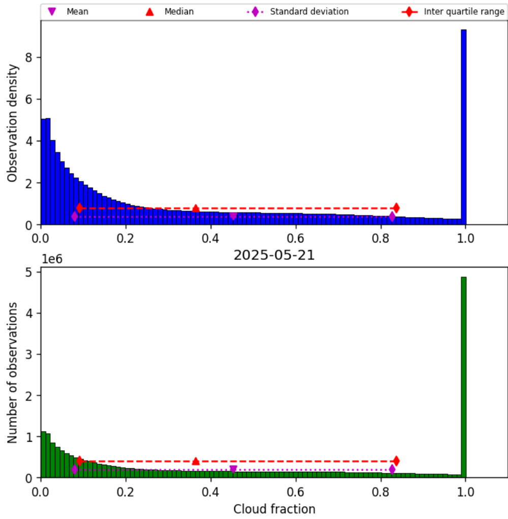
Figure 32: Histogram of “Cloud fraction” for 2025-05-21 to 2025-05-22
