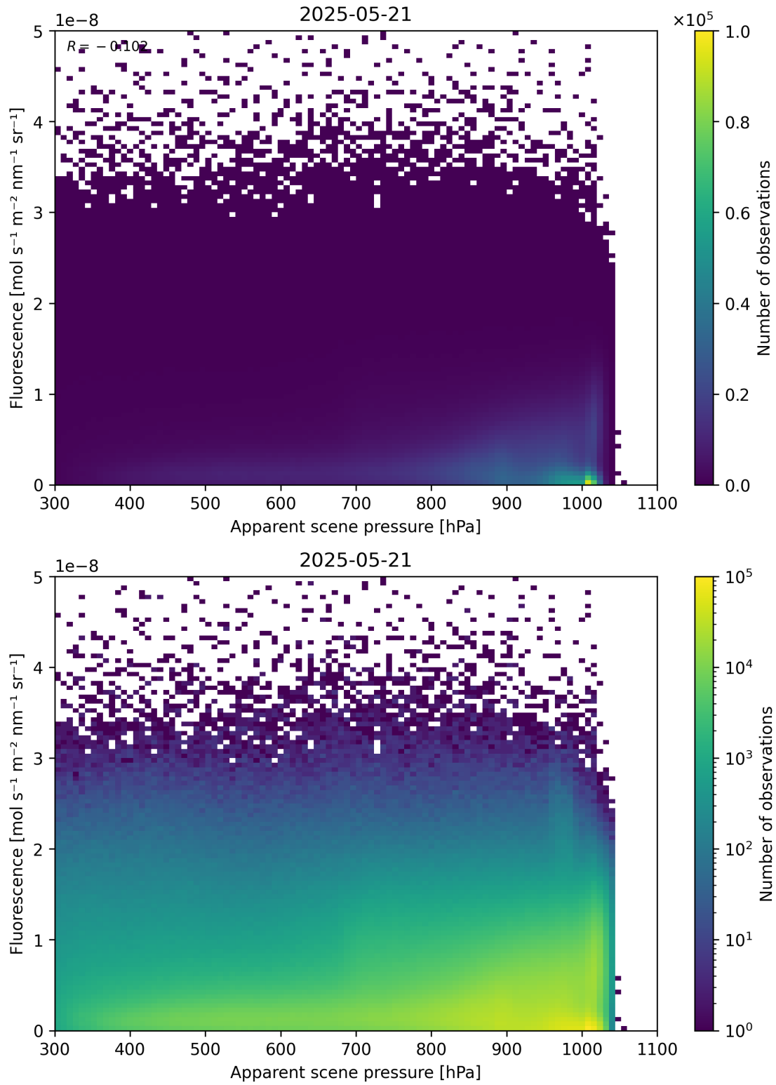
Figure 64: Scatter density plot of “Apparent scene pressure” against “Fluorescence” for 2025-05-21 to 2025-05-22.
