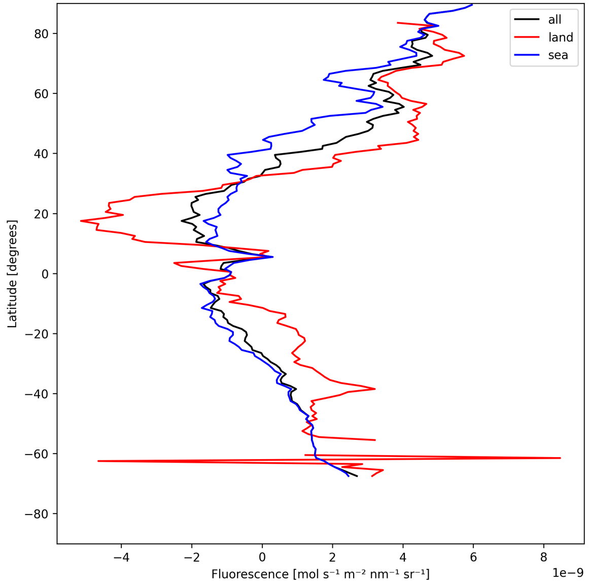
Figure 23: Zonal average of “Fluorescence” for 2025-05-21 to 2025-05-22.
