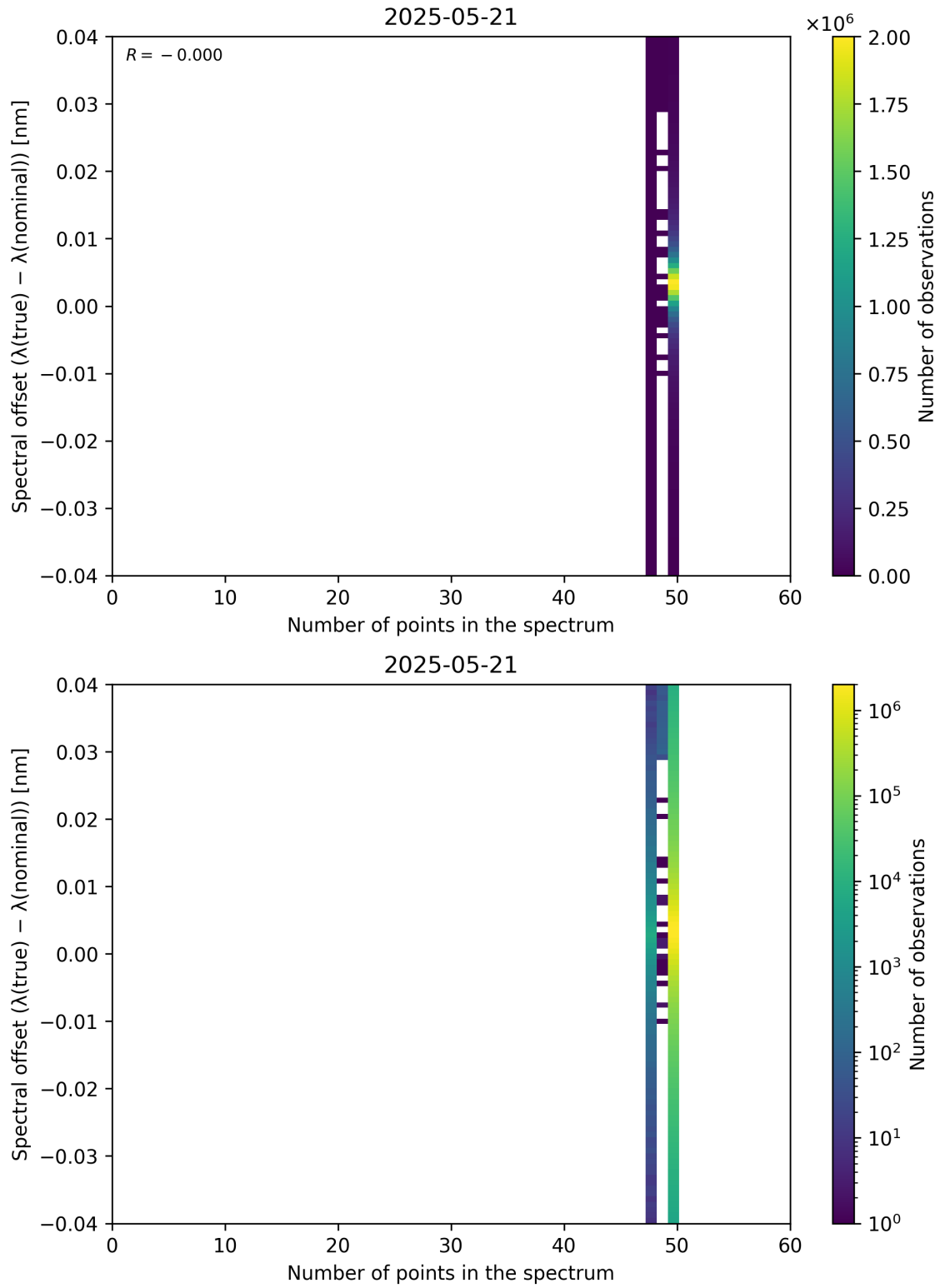
Figure 101: Scatter density plot of “Number of points in the spectrum” against “Spectral offset ( \lambda_{\text{true}} - \lambda_{\text{nominal}} )” for 2025-05-21 to 2025-05-22.
