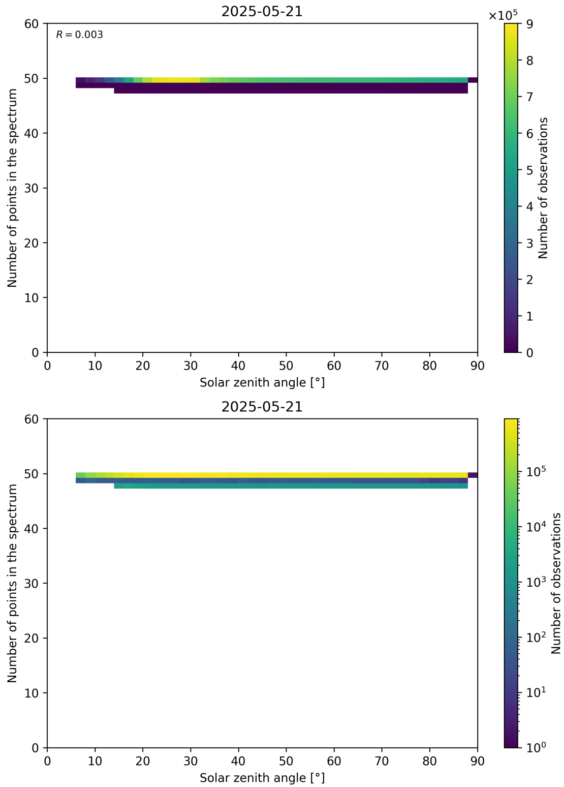
Figure 115: Scatter density plot of “Solar zenith angle” against “Number of points in the spectrum” for 2025-05-21 to 2025-05-22.
