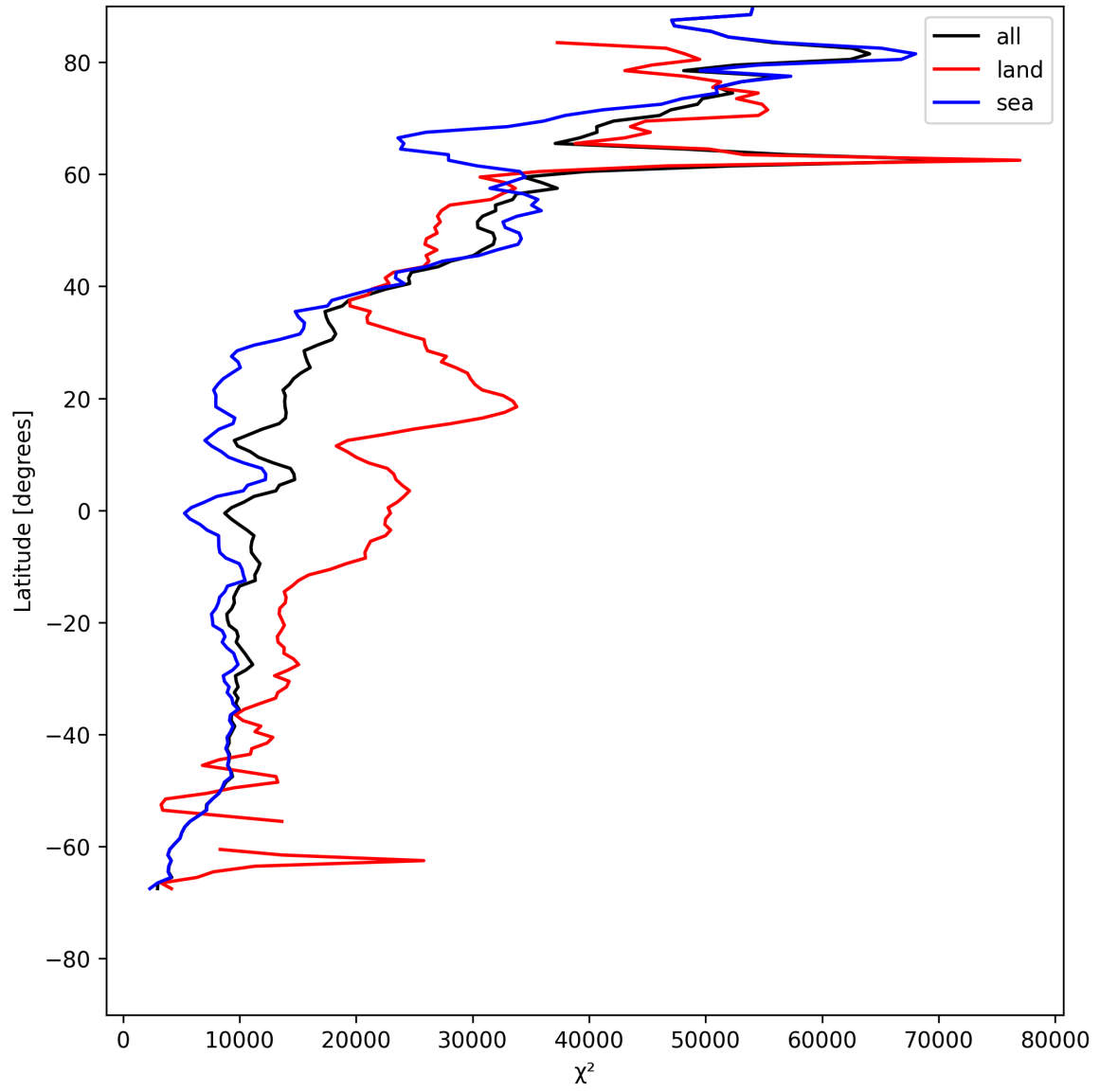
Figure 21: Zonal average of “ \chi^2 ” for 2025-05-21 to 2025-05-22.
