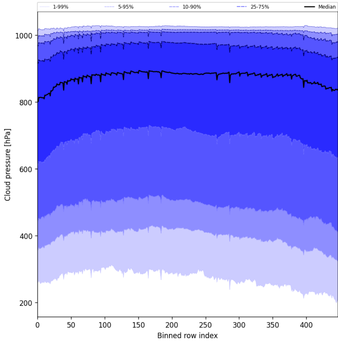
Figure 47: Along track statistics of “Cloud pressure” for 2025-05-21 to 2025-05-22
