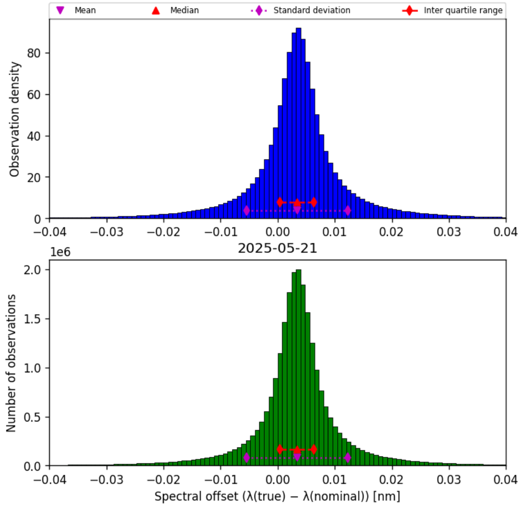
Figure 45: Histogram of “Spectral offset ( \lambda_{\text{true}} - \lambda_{\text{nominal}} )” for 2025-05-21 to 2025-05-22
