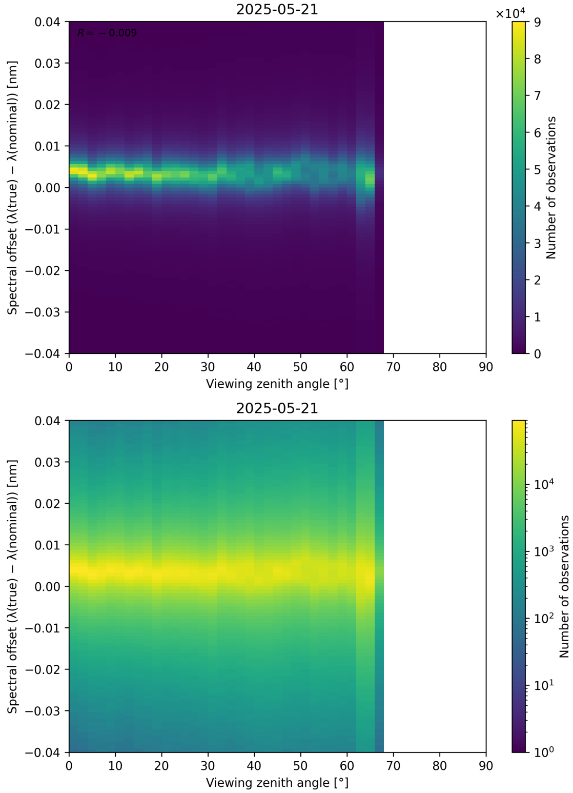
Figure 128: Scatter density plot of “Viewing zenith angle” against “Spectral offset ( \lambda_{\text{true}} - \lambda_{\text{nominal}} )” for 2025-05-21 to 2025-05-22.
