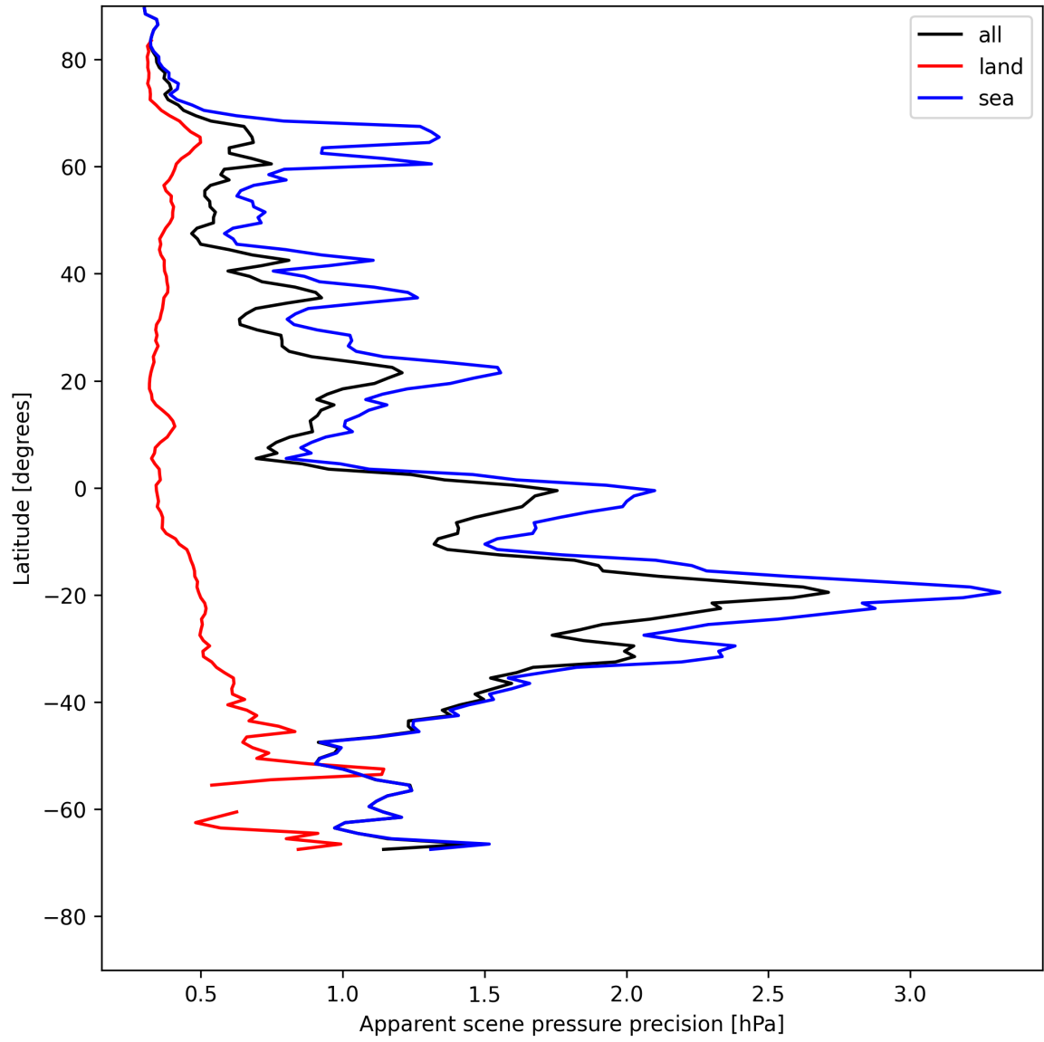
Figure 20: Zonal average of “Apparent scene pressure precision” for 2025-05-21 to 2025-05-22.
