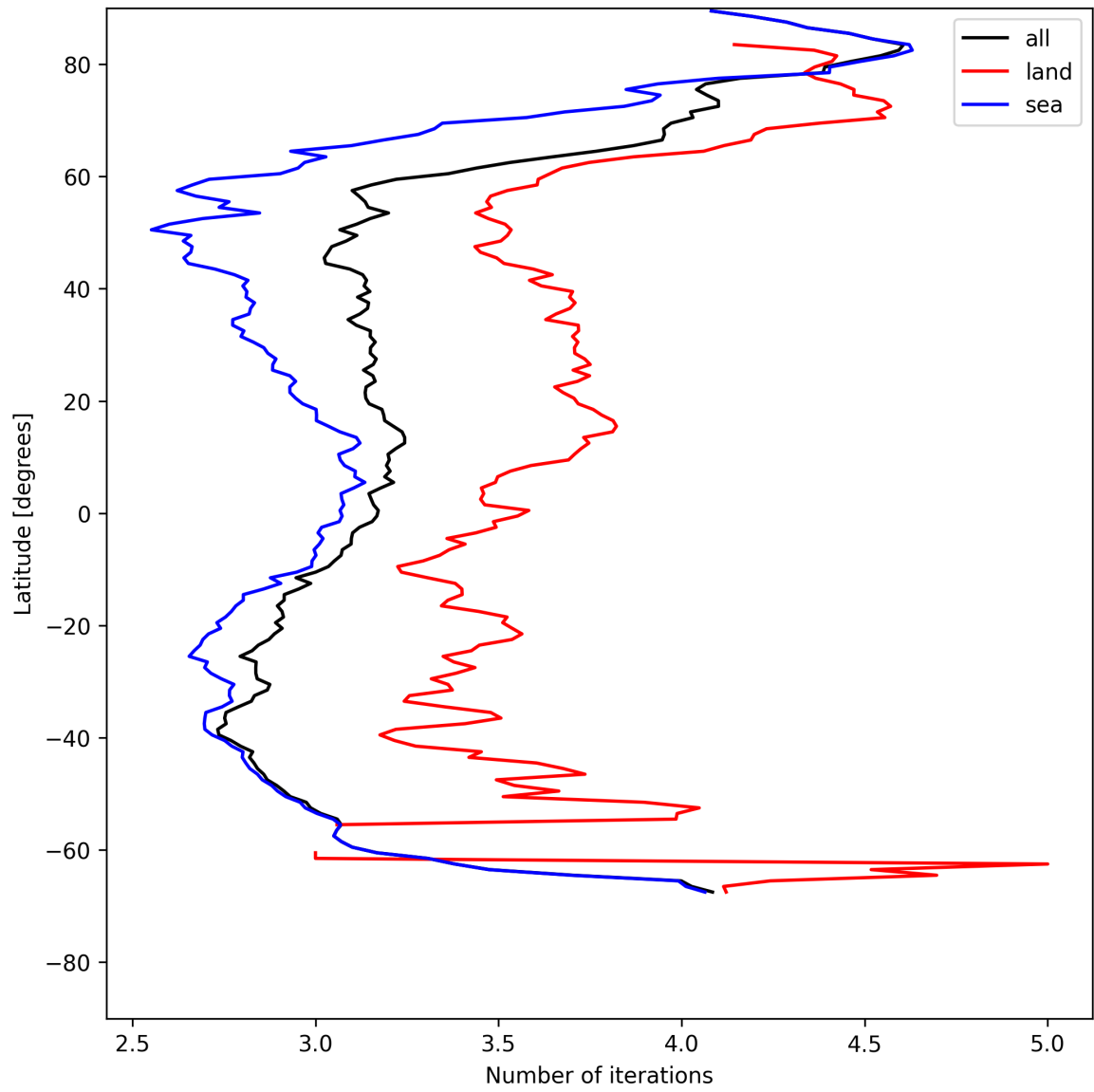
Figure 22: Zonal average of “Number of iterations” for 2025-05-21 to 2025-05-22.
