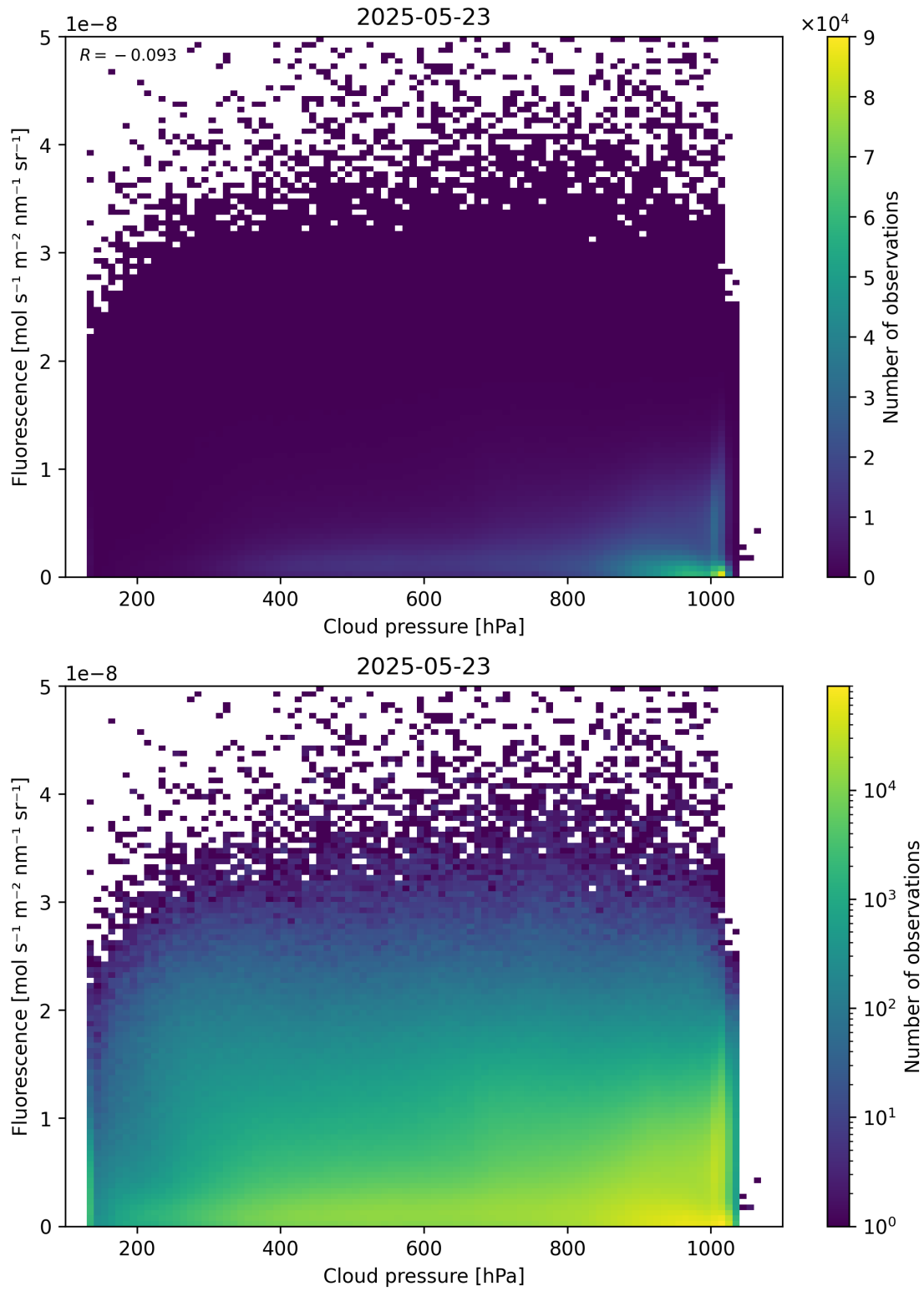
Figure 80: Scatter density plot of “Cloud pressure” against “Fluorescence” for 2025-05-22 to 2025-05-24.
