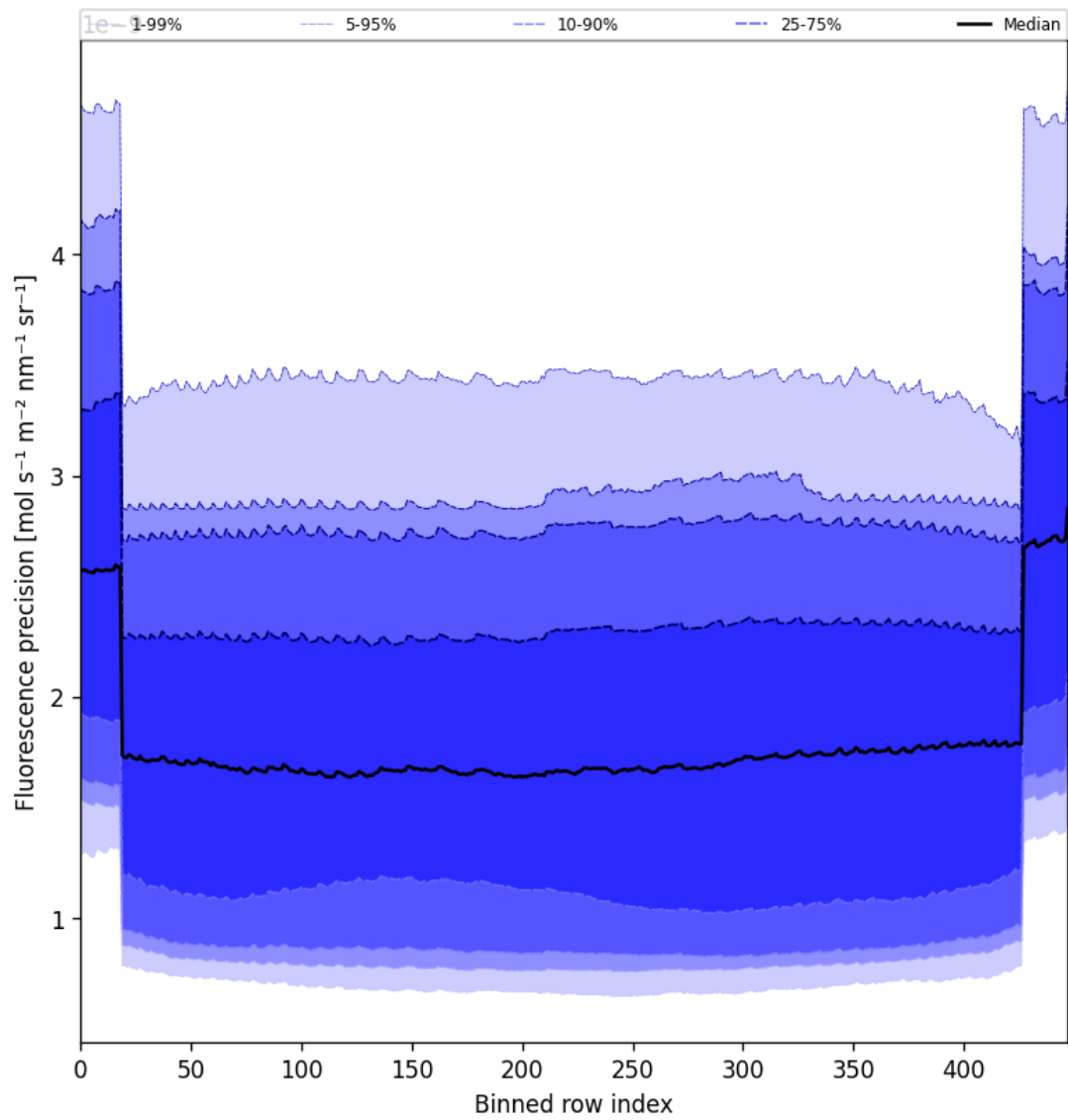
Figure 58: Along track statistics of “Fluorescence precision” for 2025-05-22 to 2025-05-24
