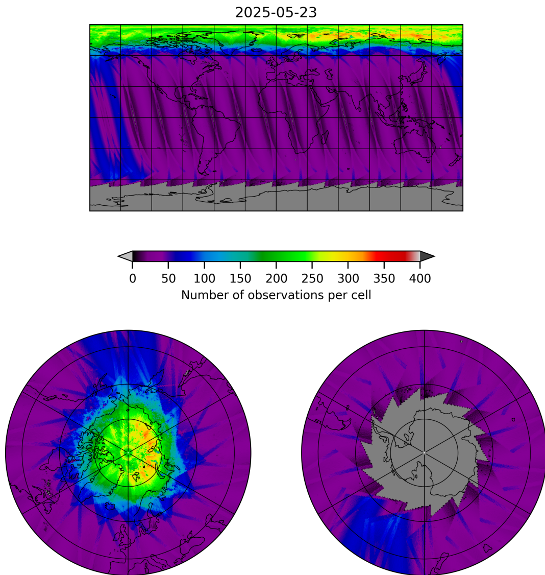
Figure 11: Map of the number of observations for 2025-05-22 to 2025-05-24
