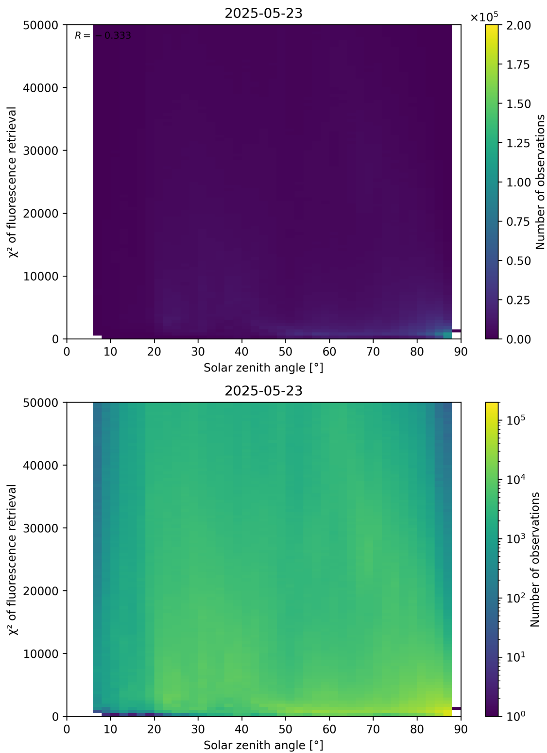
Figure 109: Scatter density plot of “Solar zenith angle” against “ \chi^2 of fluorescence retrieval” for 2025-05-22 to 2025-05-24.
