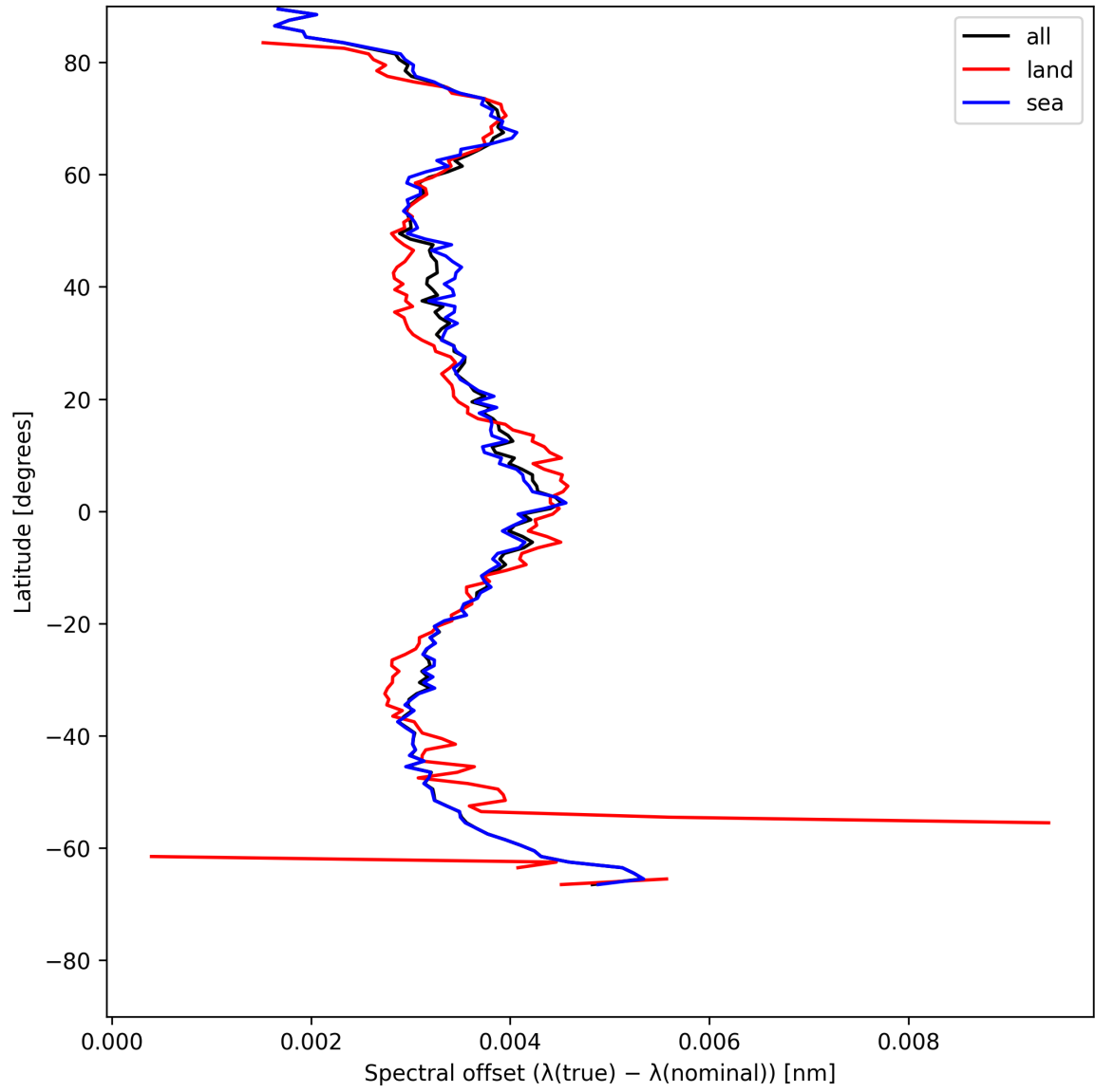
Figure 28: Zonal average of “Spectral offset ( \lambda_{\text{true}} - \lambda_{\text{nominal}} )” for 2025-05-22 to 2025-05-24.
