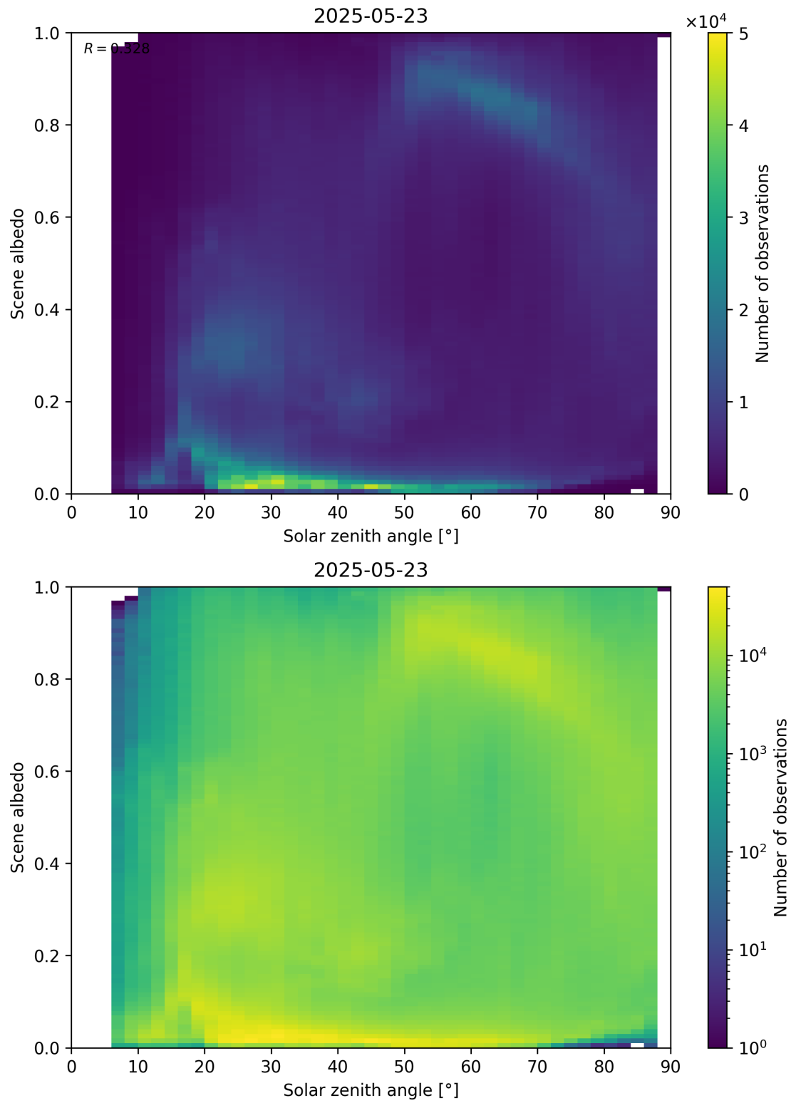
Figure 116: Scatter density plot of “Solar zenith angle” against “Scene albedo” for 2025-05-22 to 2025-05-24.
