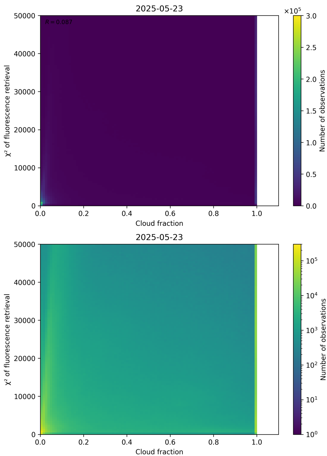
Figure 71: Scatter density plot of “Cloud fraction” against “ \chi^2 of fluorescence retrieval” for 2025-05-22 to 2025-05-24.
