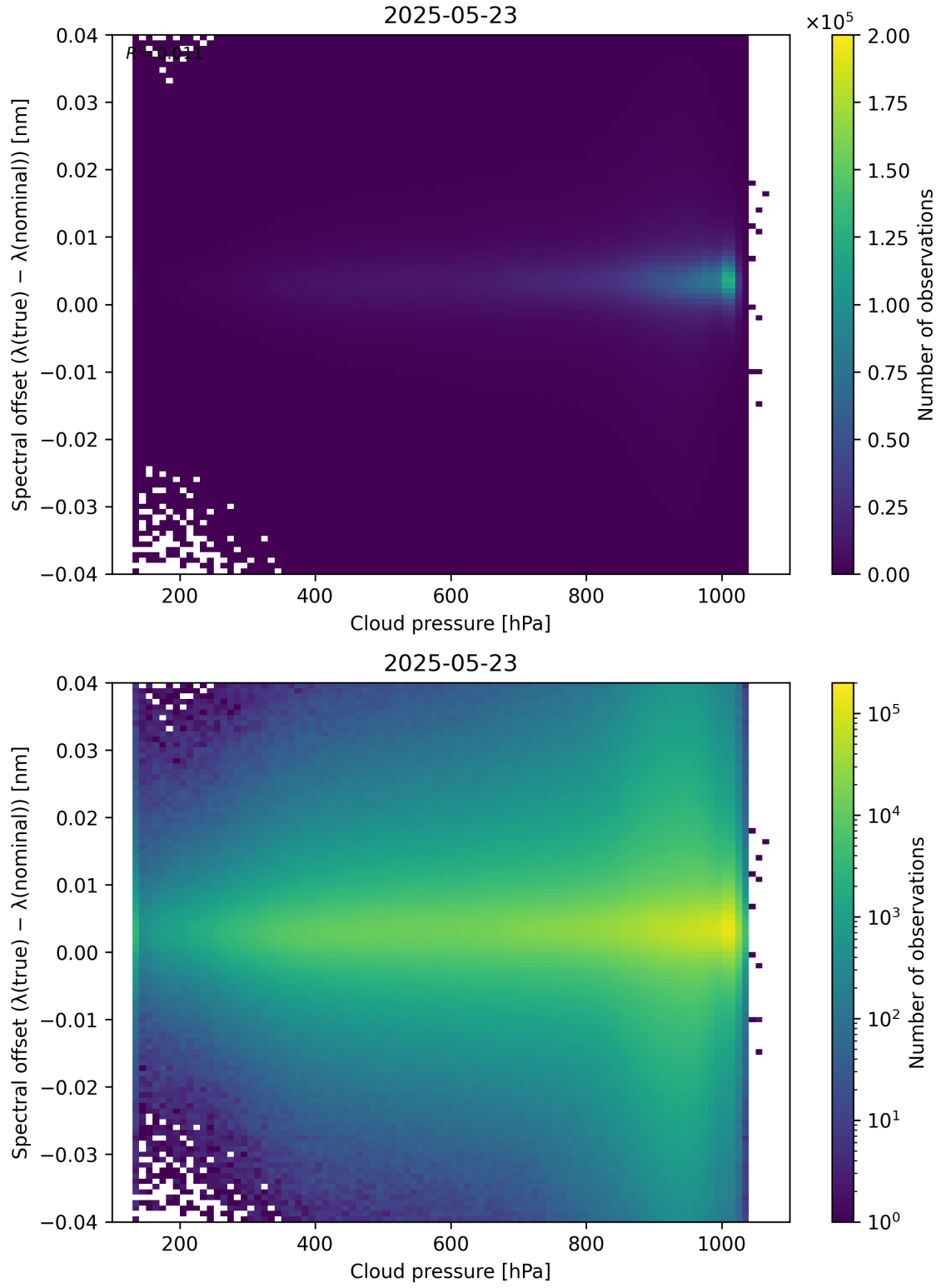
Figure 84: Scatter density plot of “Cloud pressure” against “Spectral offset ( \lambda_{\text{true}} - \lambda_{\text{nominal}} )” for 2025-05-22 to 2025-05-24.
