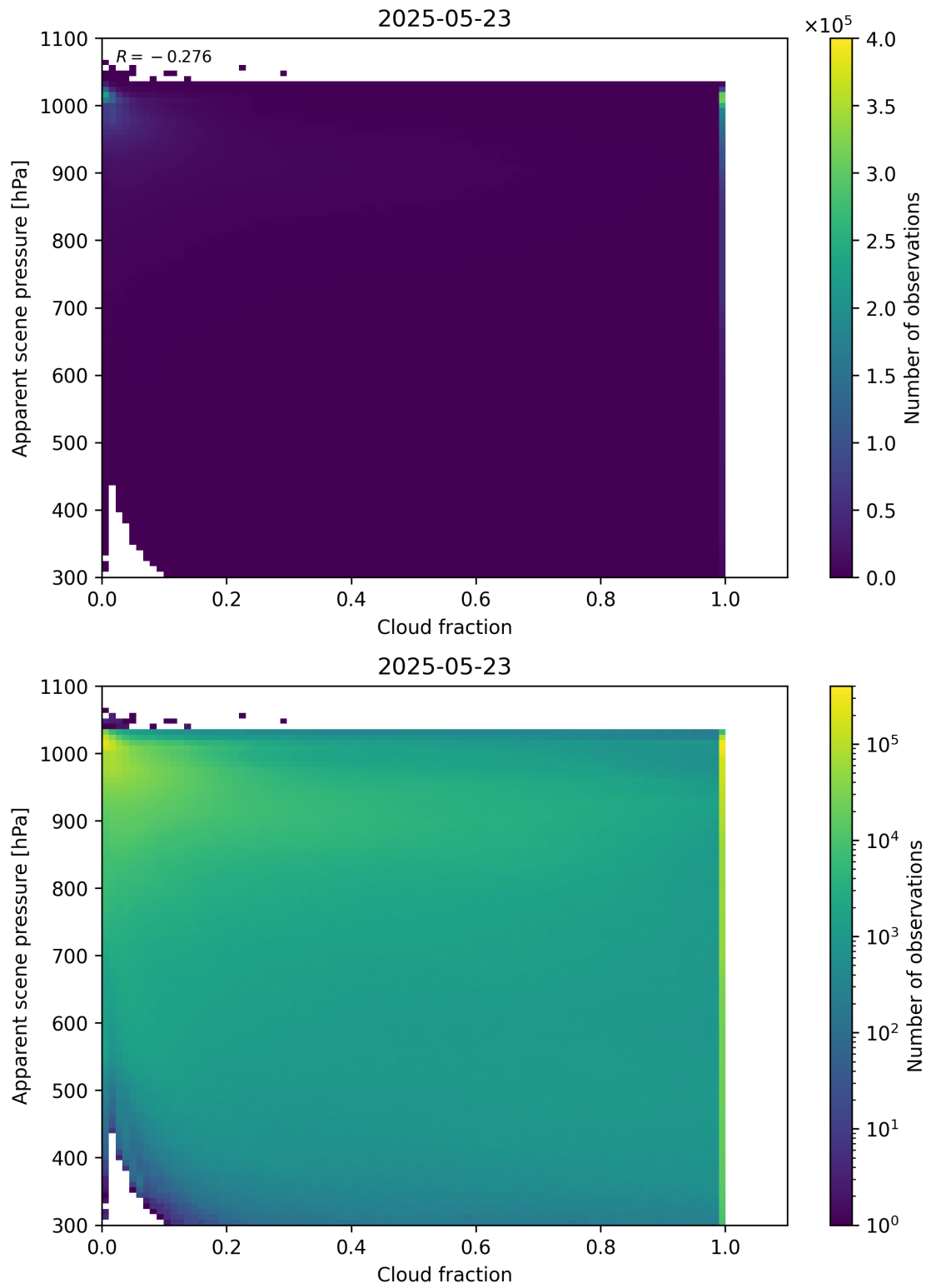
Figure 70: Scatter density plot of “Cloud fraction” against “Apparent scene pressure” for 2025-05-22 to 2025-05-24.
