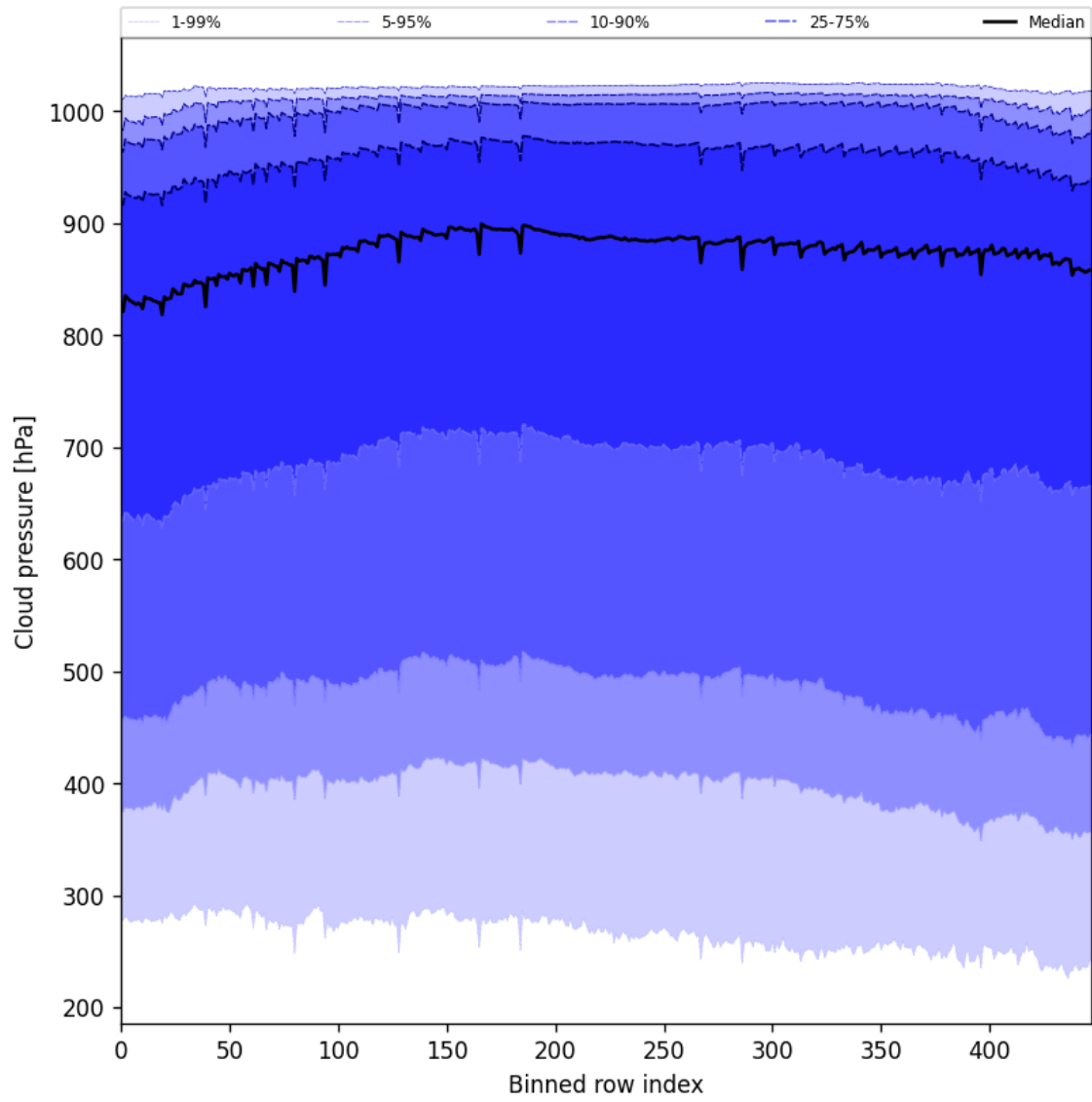
Figure 47: Along track statistics of “Cloud pressure” for 2025-05-22 to 2025-05-24
