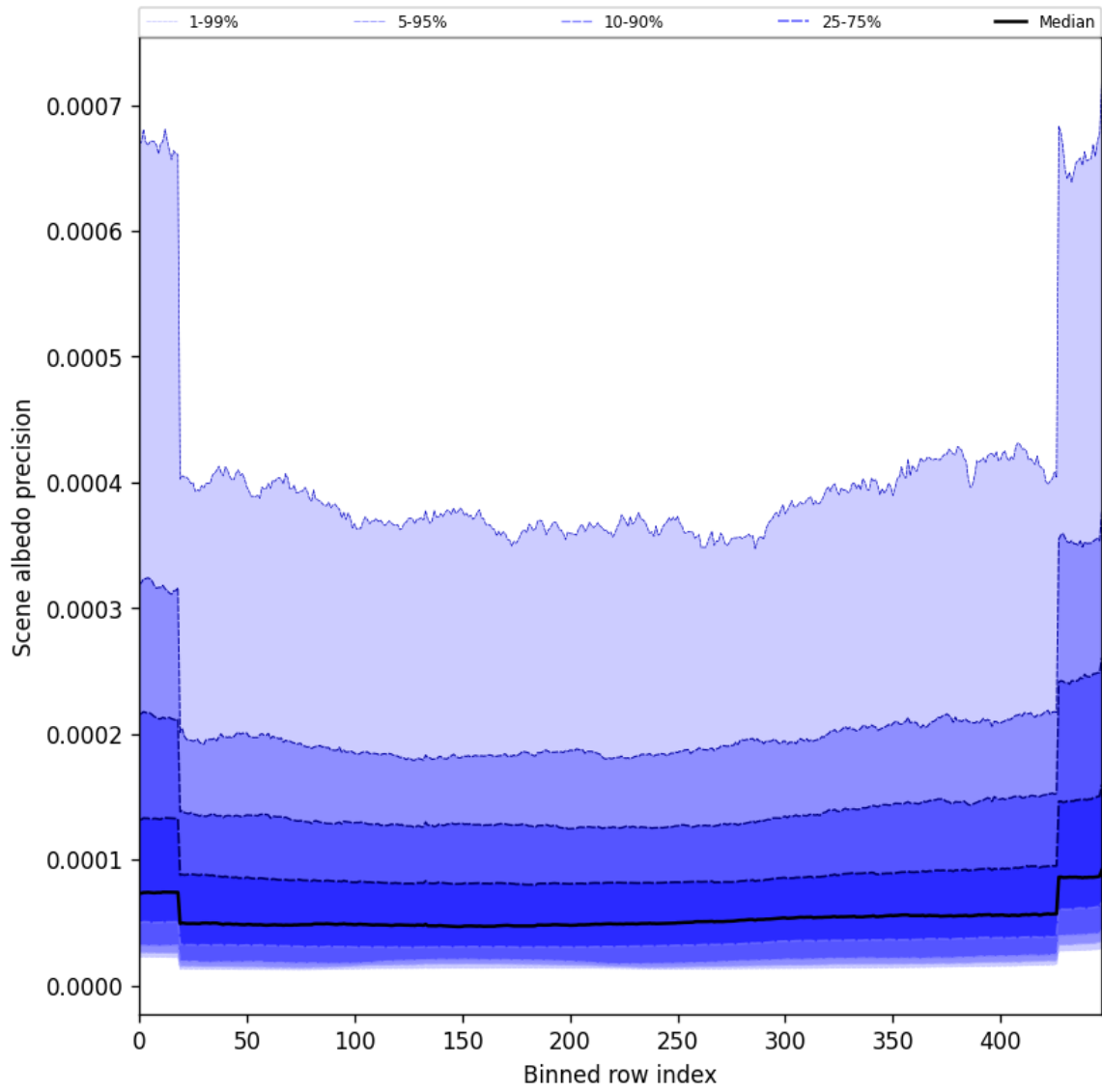
Figure 52: Along track statistics of “Scene albedo precision” for 2025-05-22 to 2025-05-24
