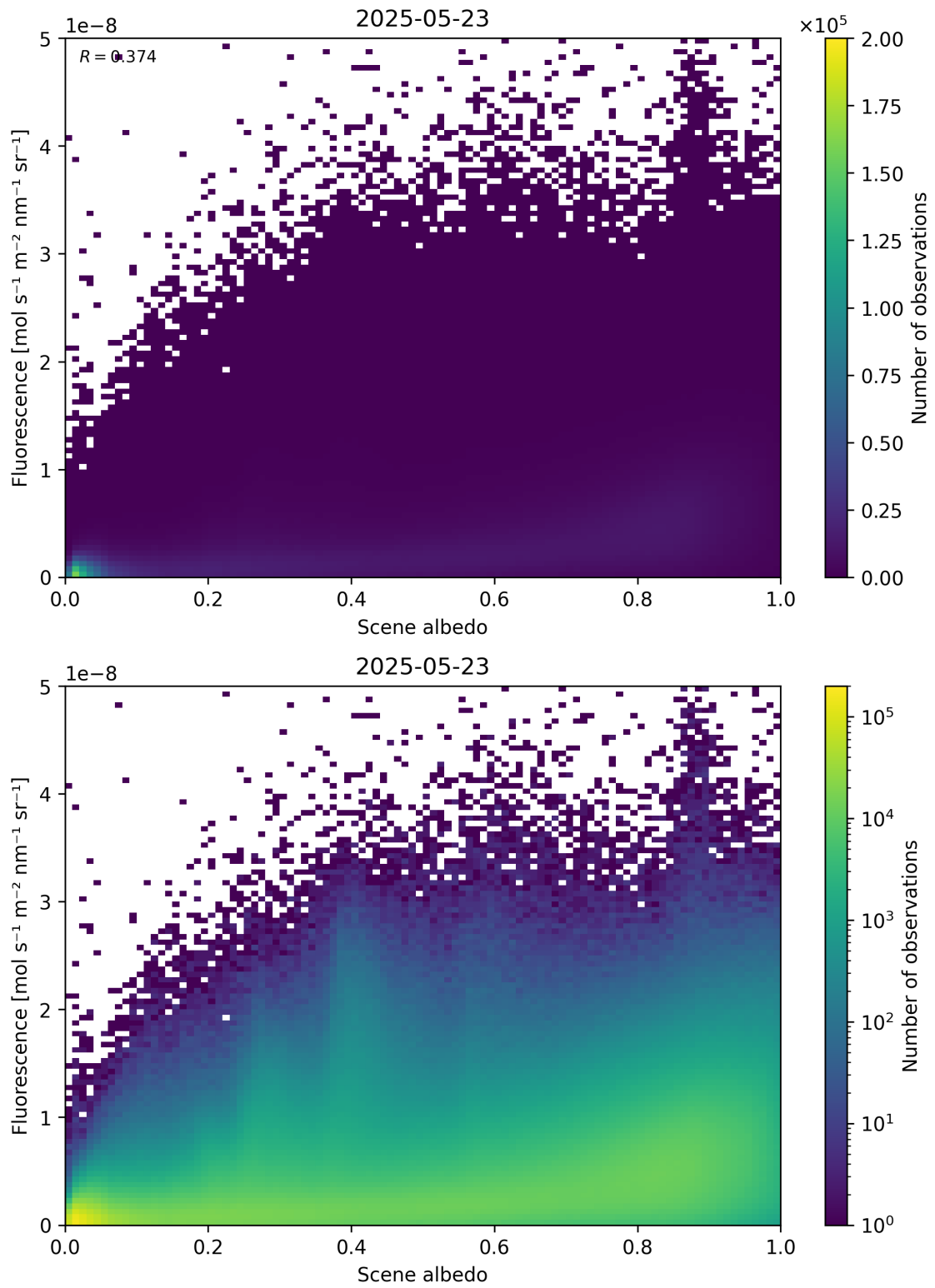
Figure 104: Scatter density plot of “Scene albedo” against “Fluorescence” for 2025-05-22 to 2025-05-24.
