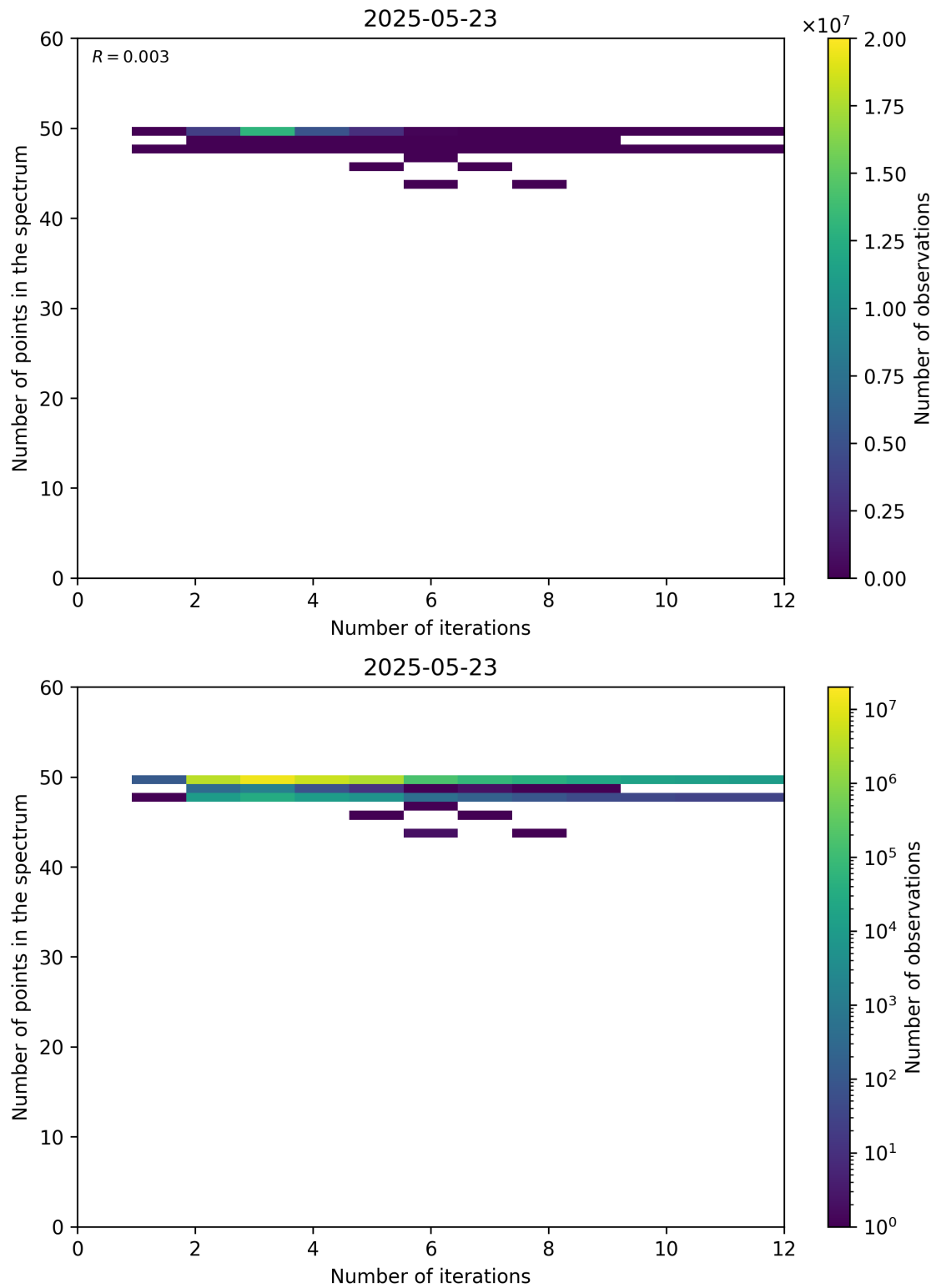
Figure 99: Scatter density plot of “Number of iterations” against “Number of points in the spectrum” for 2025-05-22 to 2025-05-24.
