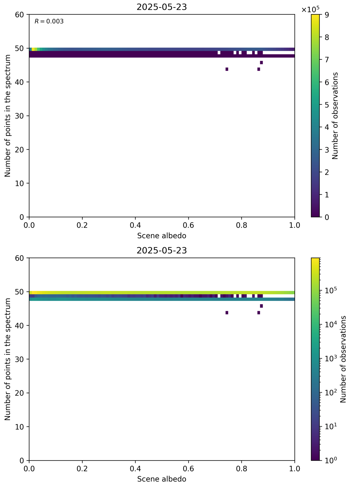
Figure 106: Scatter density plot of “Scene albedo” against “Number of points in the spectrum” for 2025-05-22 to 2025-05-24.
