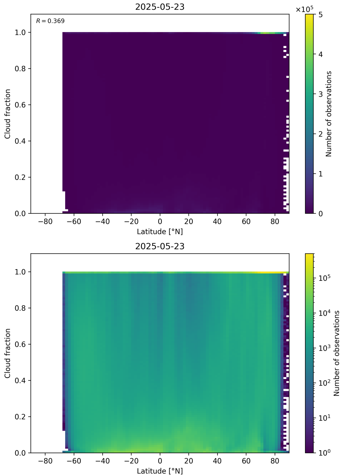
Figure 90: Scatter density plot of “Latitude” against “Cloud fraction” for 2025-05-22 to 2025-05-24.
