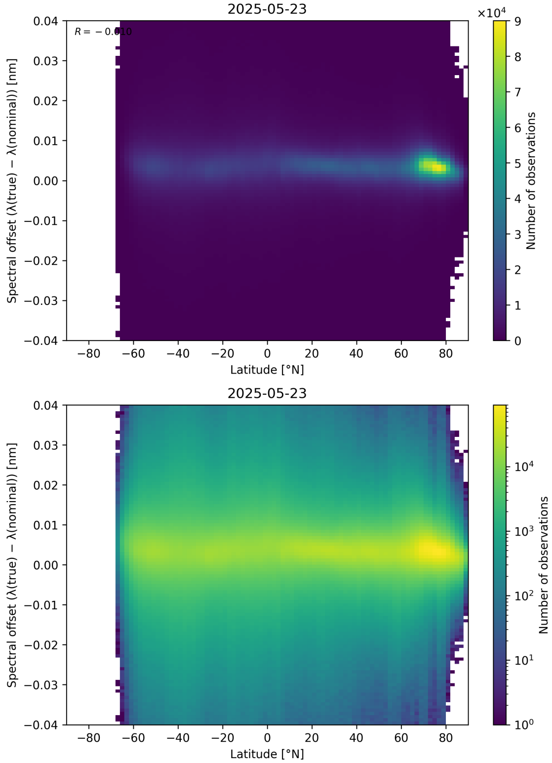
Figure 96: Scatter density plot of “Latitude” against “Spectral offset ( \lambda_{\text{true}} - \lambda_{\text{nominal}} )” for 2025-05-22 to 2025-05-24.
