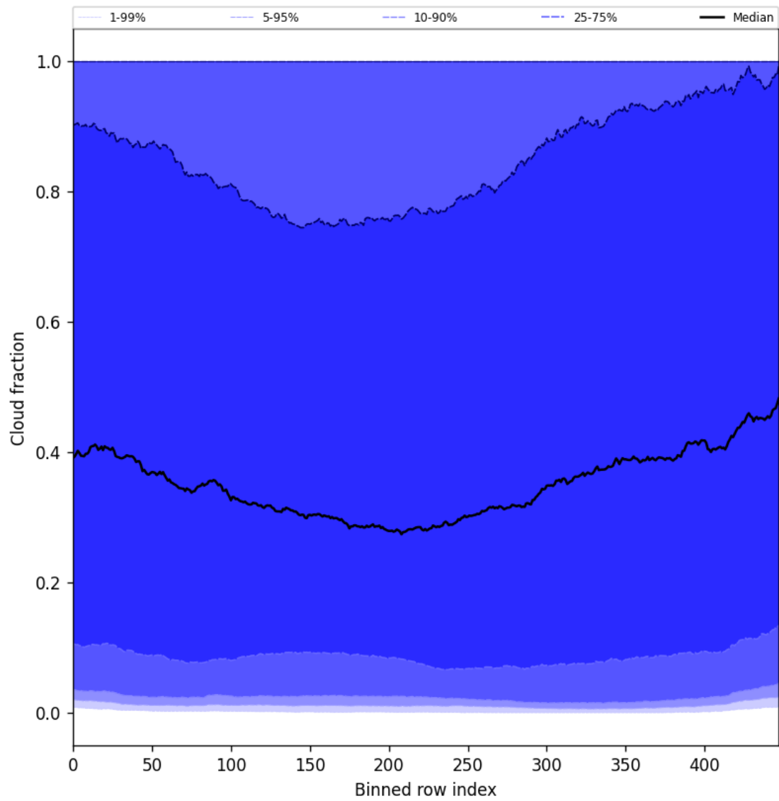
Figure 49: Along track statistics of “Cloud fraction” for 2025-05-22 to 2025-05-24
