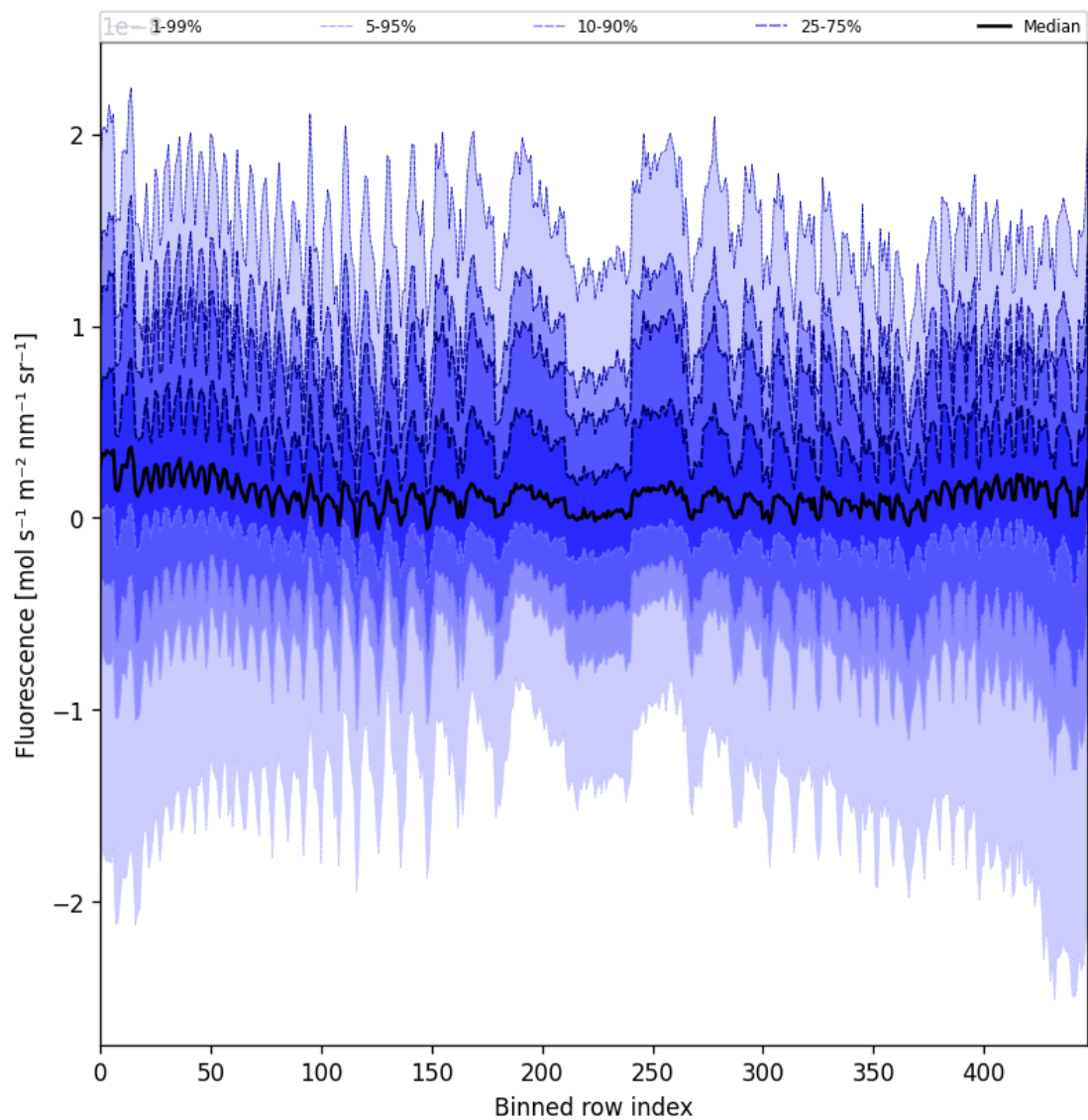
Figure 57: Along track statistics of “Fluorescence” for 2025-05-22 to 2025-05-24
