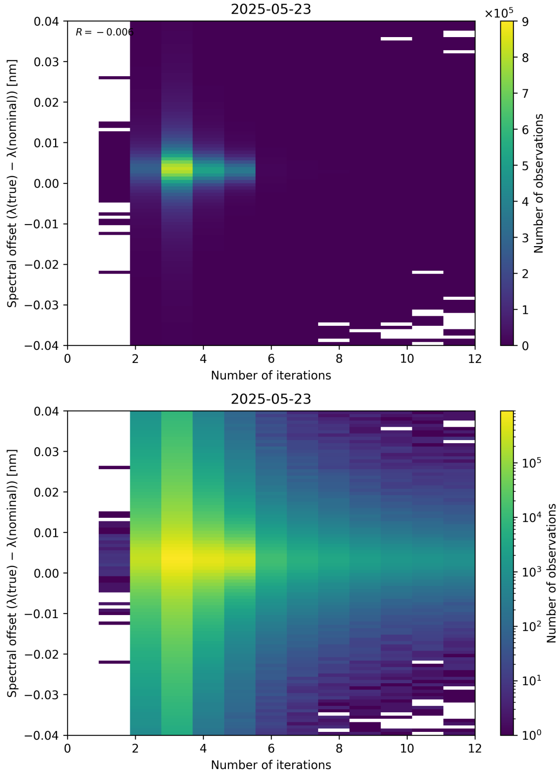
Figure 100: Scatter density plot of “Number of iterations” against “Spectral offset ( \lambda_{\text{true}} - \lambda_{\text{nominal}} )” for 2025-05-22 to 2025-05-24.
