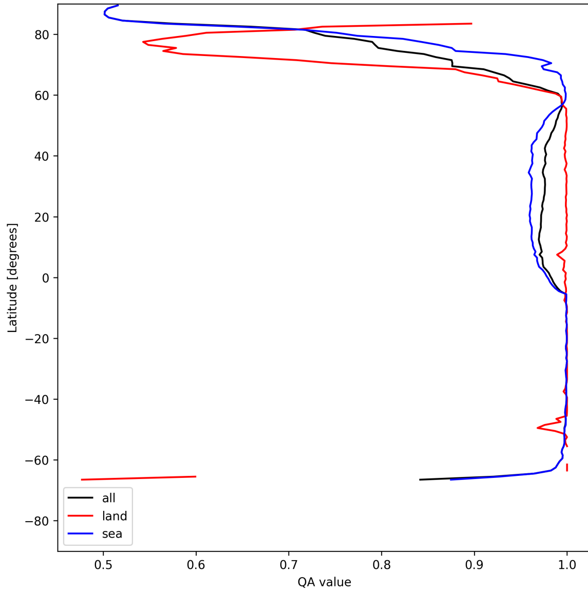
Figure 12: Zonal average of “QA value” for 2025-05-22 to 2025-05-24.
