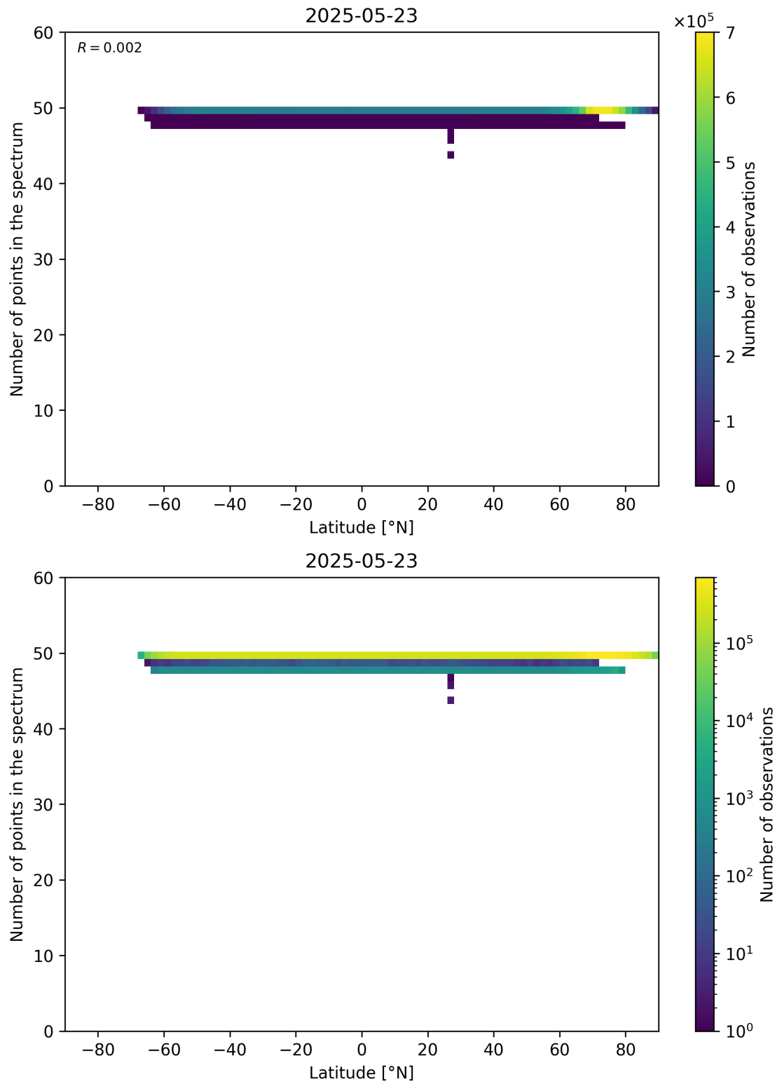
Figure 94: Scatter density plot of “Latitude” against “Number of points in the spectrum” for 2025-05-22 to 2025-05-24.
