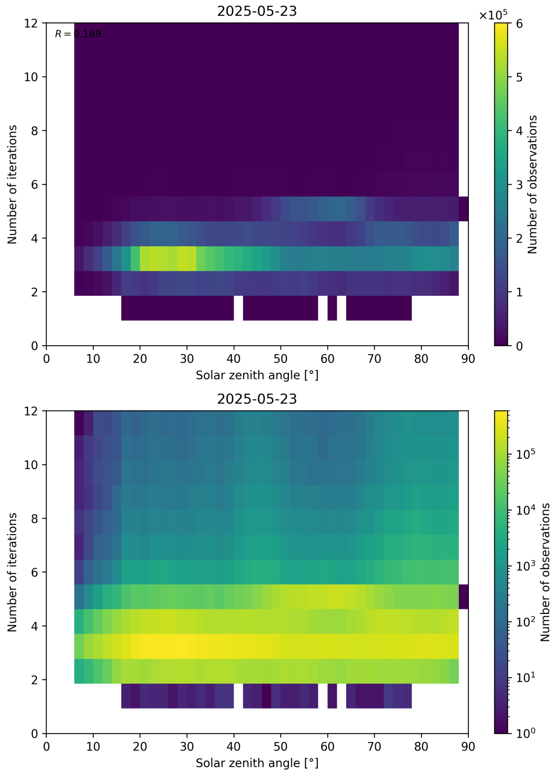
Figure 114: Scatter density plot of “Solar zenith angle” against “Number of iterations” for 2025-05-22 to 2025-05-24.
