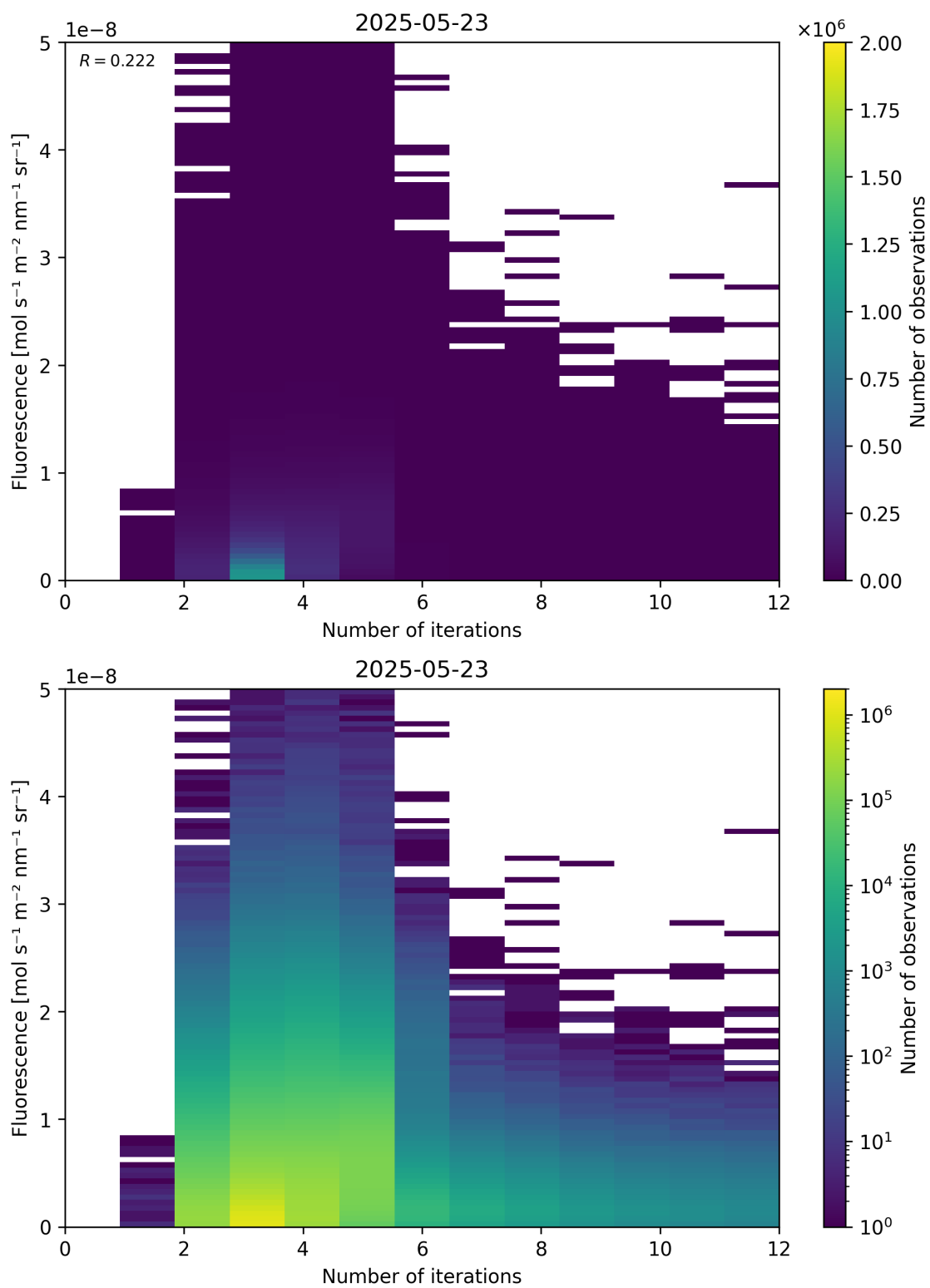
Figure 98: Scatter density plot of “Number of iterations” against “Fluorescence” for 2025-05-22 to 2025-05-24.
