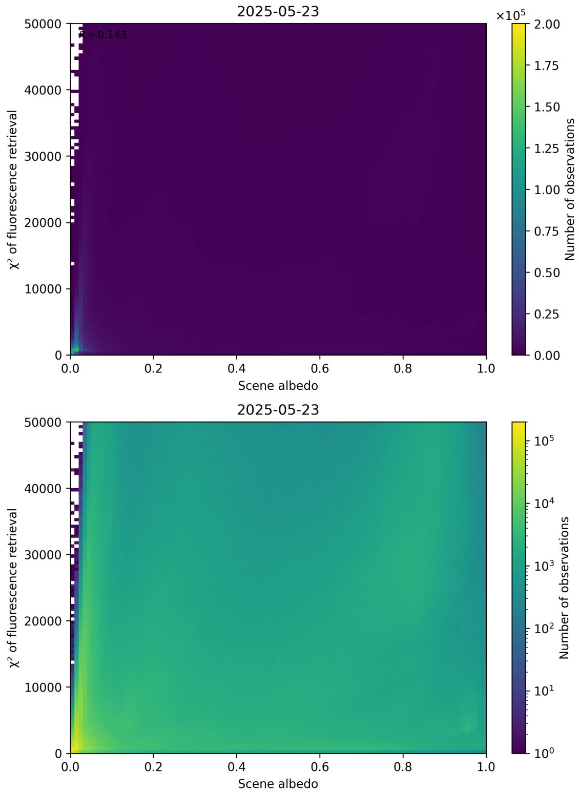
Figure 103: Scatter density plot of “Scene albedo” against “ \chi^2 of fluorescence retrieval” for 2025-05-22 to 2025-05-24.
