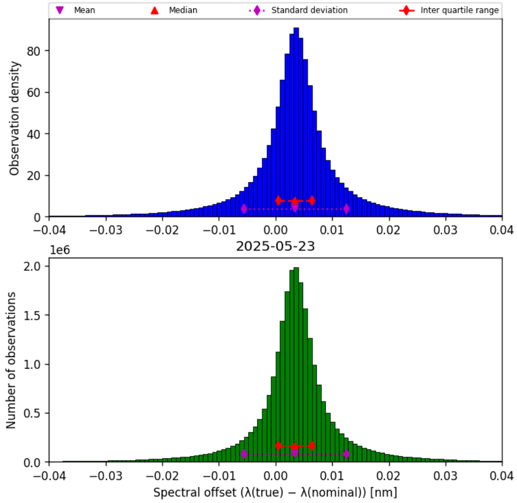
Figure 45: Histogram of “Spectral offset ( \lambda_{\text{true}} - \lambda_{\text{nominal}} )” for 2025-05-22 to 2025-05-24
