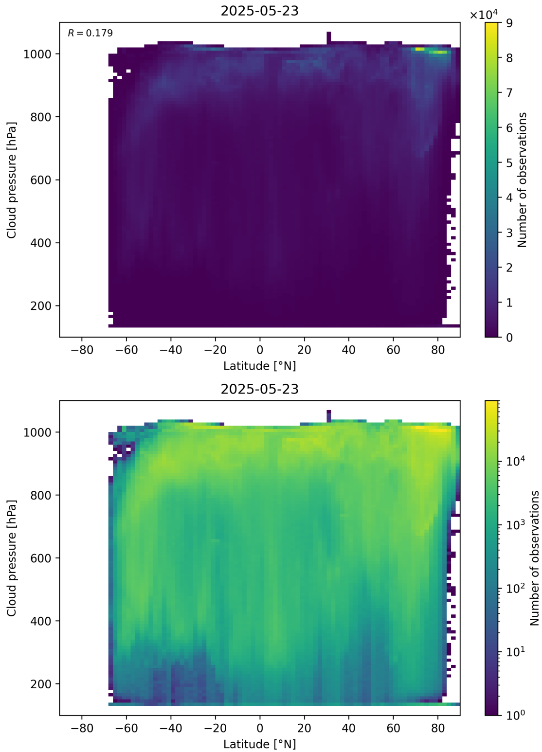
Figure 91: Scatter density plot of “Latitude” against “Cloud pressure” for 2025-05-22 to 2025-05-24.
