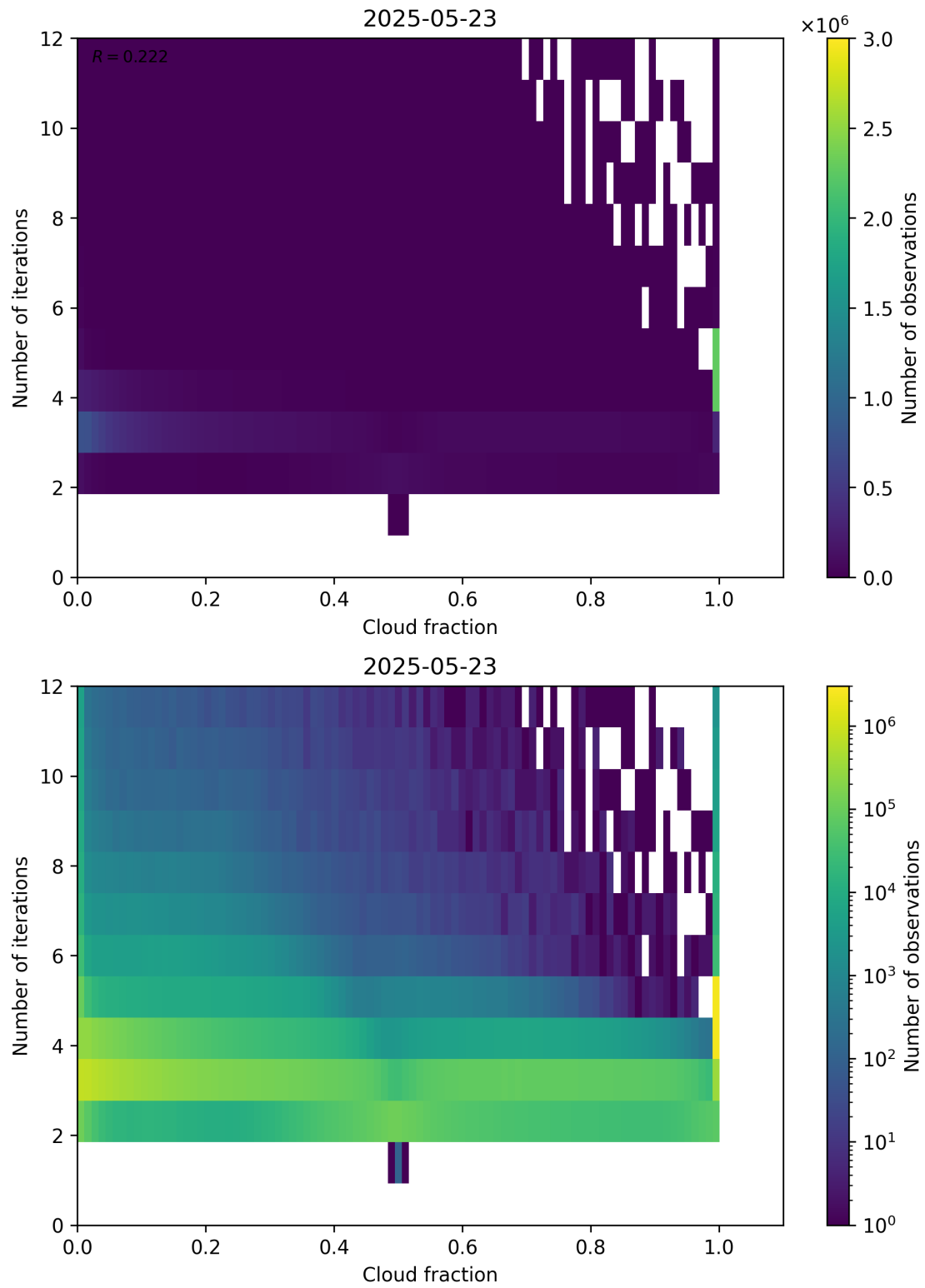
Figure 73: Scatter density plot of “Cloud fraction” against “Number of iterations” for 2025-05-22 to 2025-05-24.
