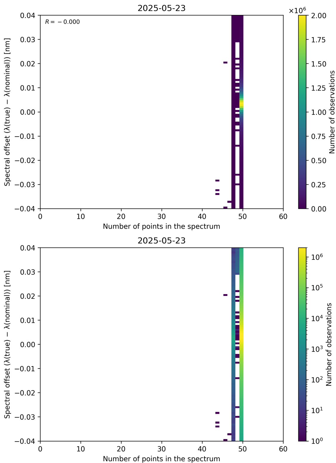
Figure 101: Scatter density plot of “Number of points in the spectrum” against “Spectral offset ( \lambda_{\text{true}} - \lambda_{\text{nominal}} )” for 2025-05-22 to 2025-05-24.
