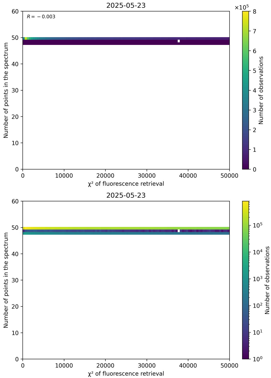
Figure 68: Scatter density plot of " \chi^2 of fluorescence retrieval" against "Number of points in the spectrum" for 2025-05-22 to 2025-05-24.
