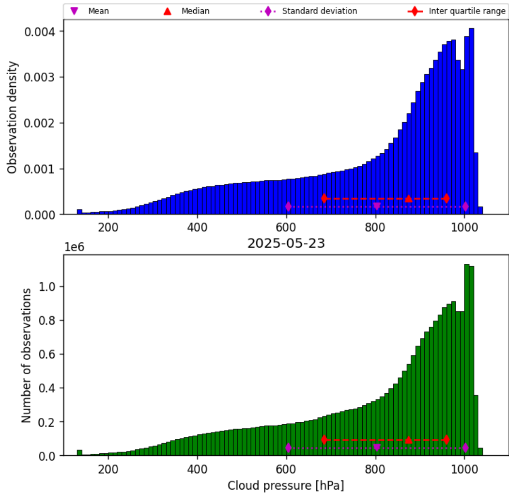
Figure 30: Histogram of “Cloud pressure” for 2025-05-22 to 2025-05-24
