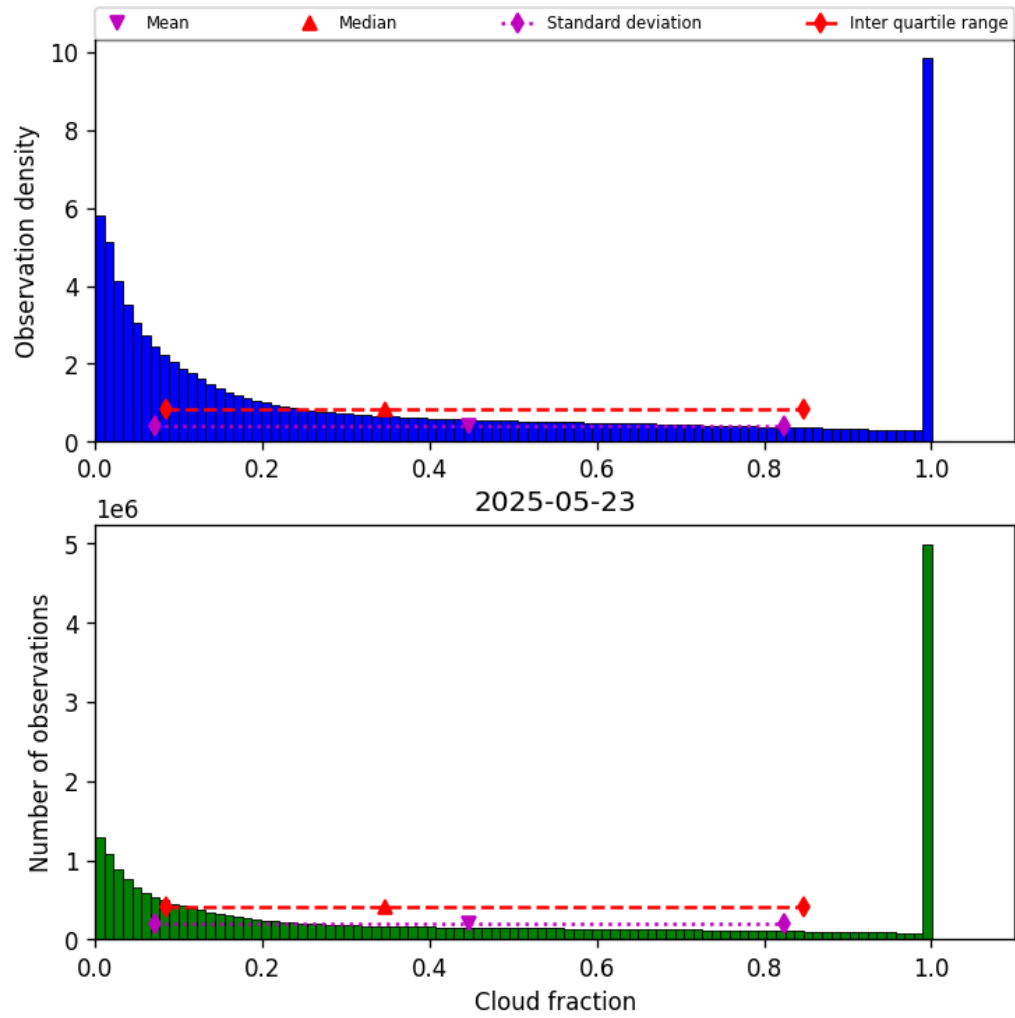
Figure 32: Histogram of “Cloud fraction” for 2025-05-22 to 2025-05-24
