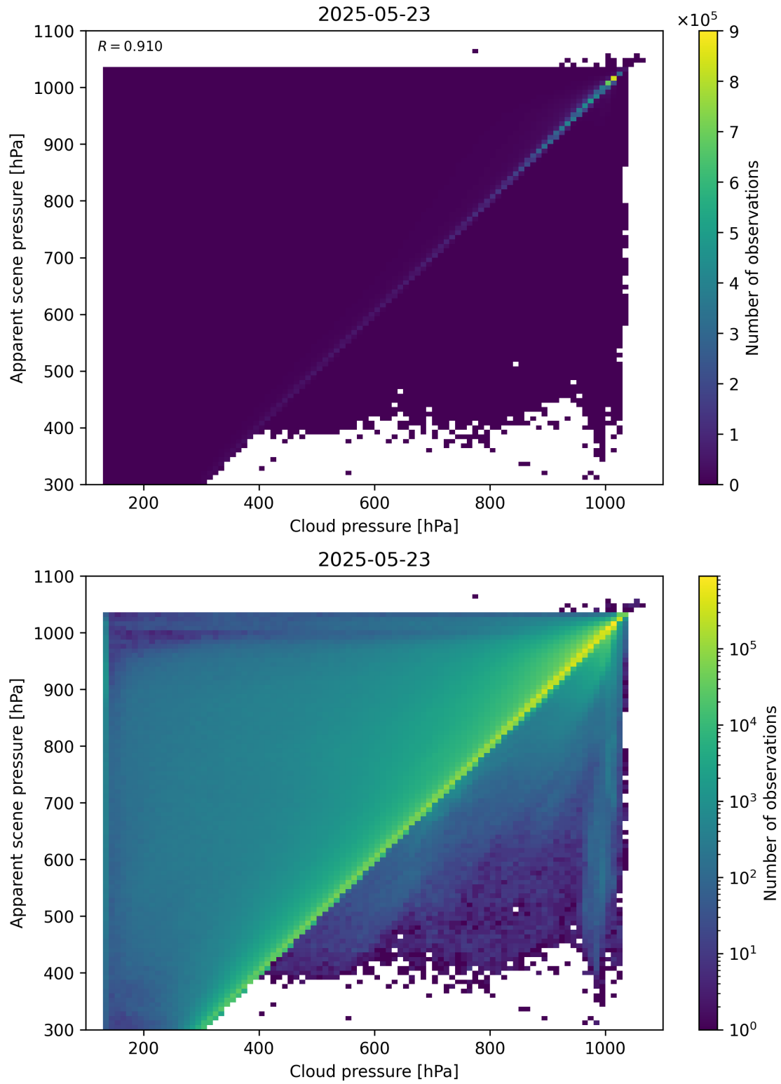
Figure 77: Scatter density plot of “Cloud pressure” against “Apparent scene pressure” for 2025-05-22 to 2025-05-24.
