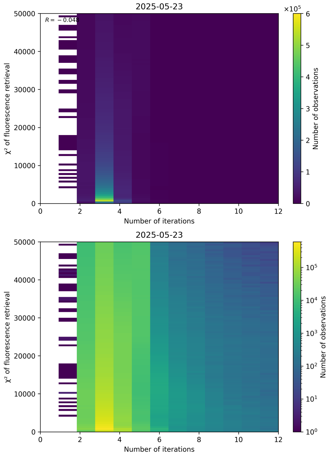
Figure 97: Scatter density plot of “Number of iterations” against “ \chi^2 of fluorescence retrieval” for 2025-05-22 to 2025-05-24.
