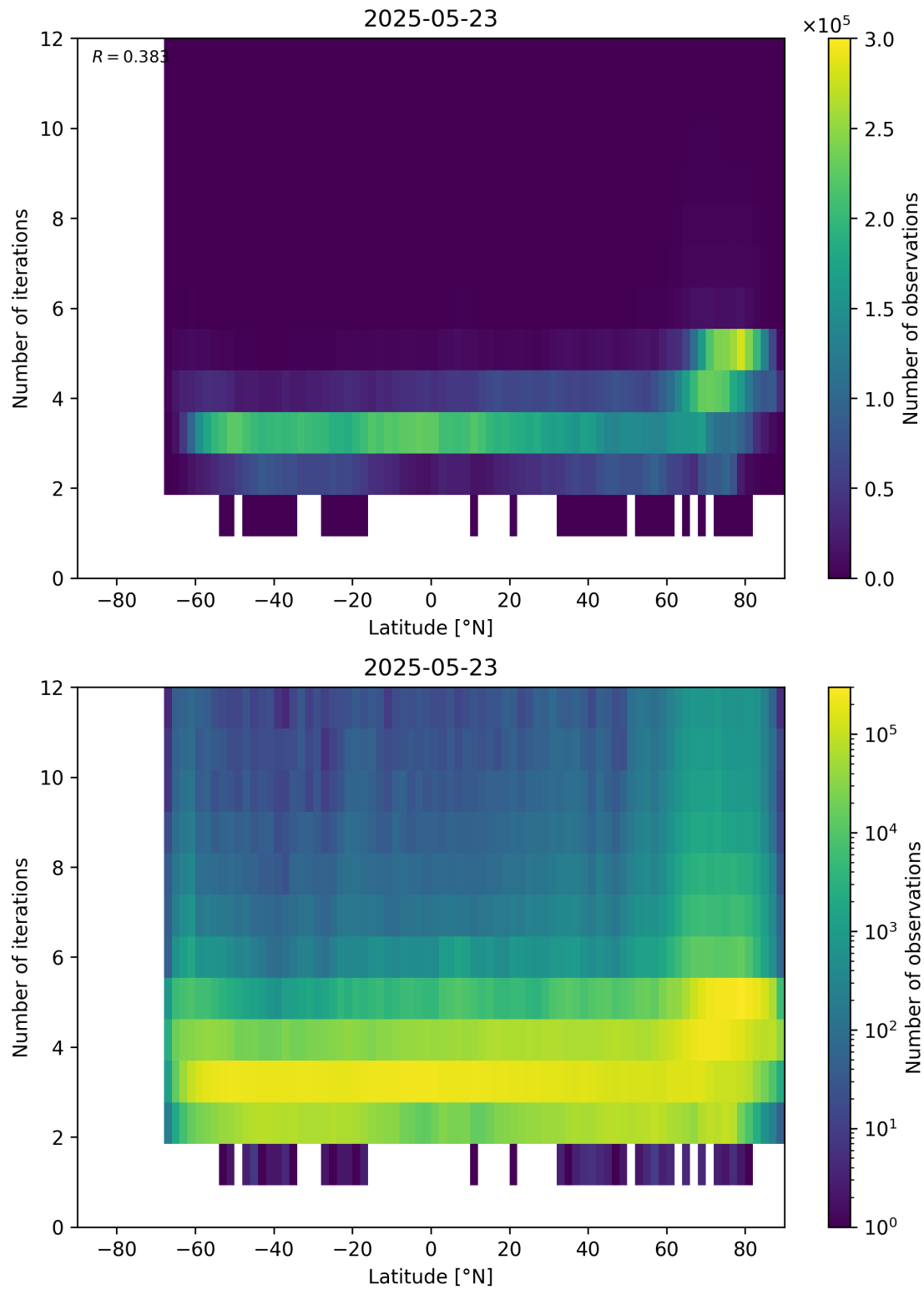
Figure 93: Scatter density plot of “Latitude” against “Number of iterations” for 2025-05-22 to 2025-05-24.
