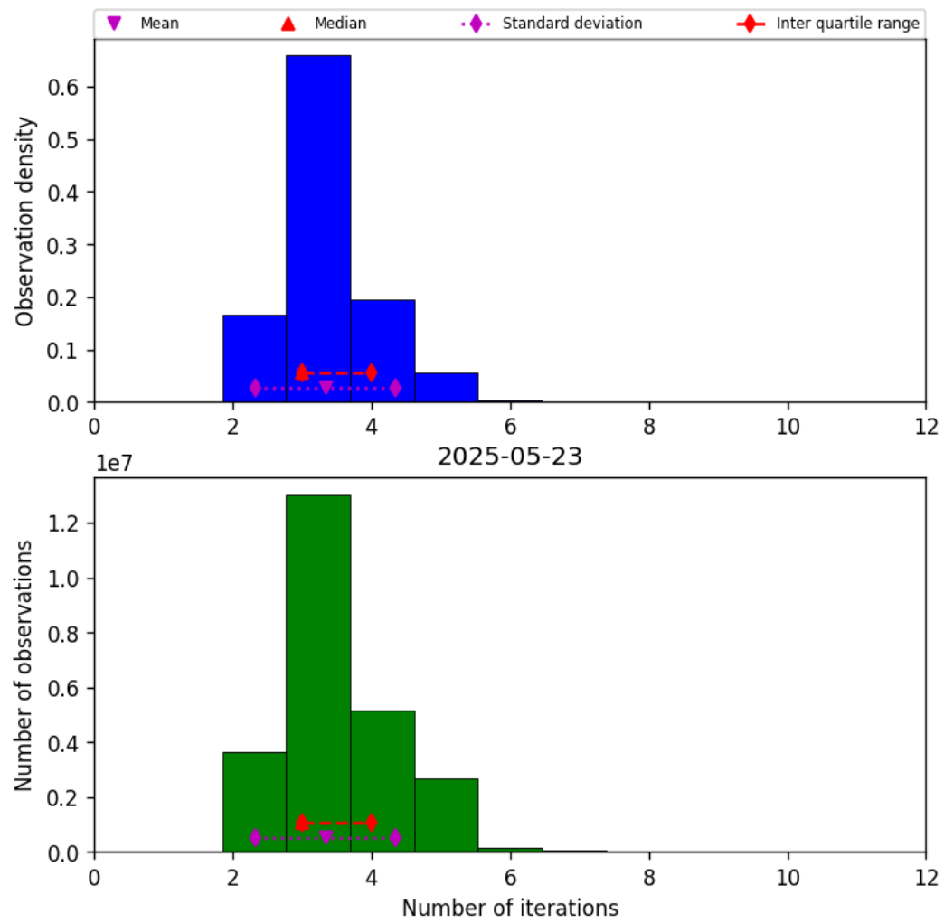
Figure 39: Histogram of “Number of iterations” for 2025-05-22 to 2025-05-24
