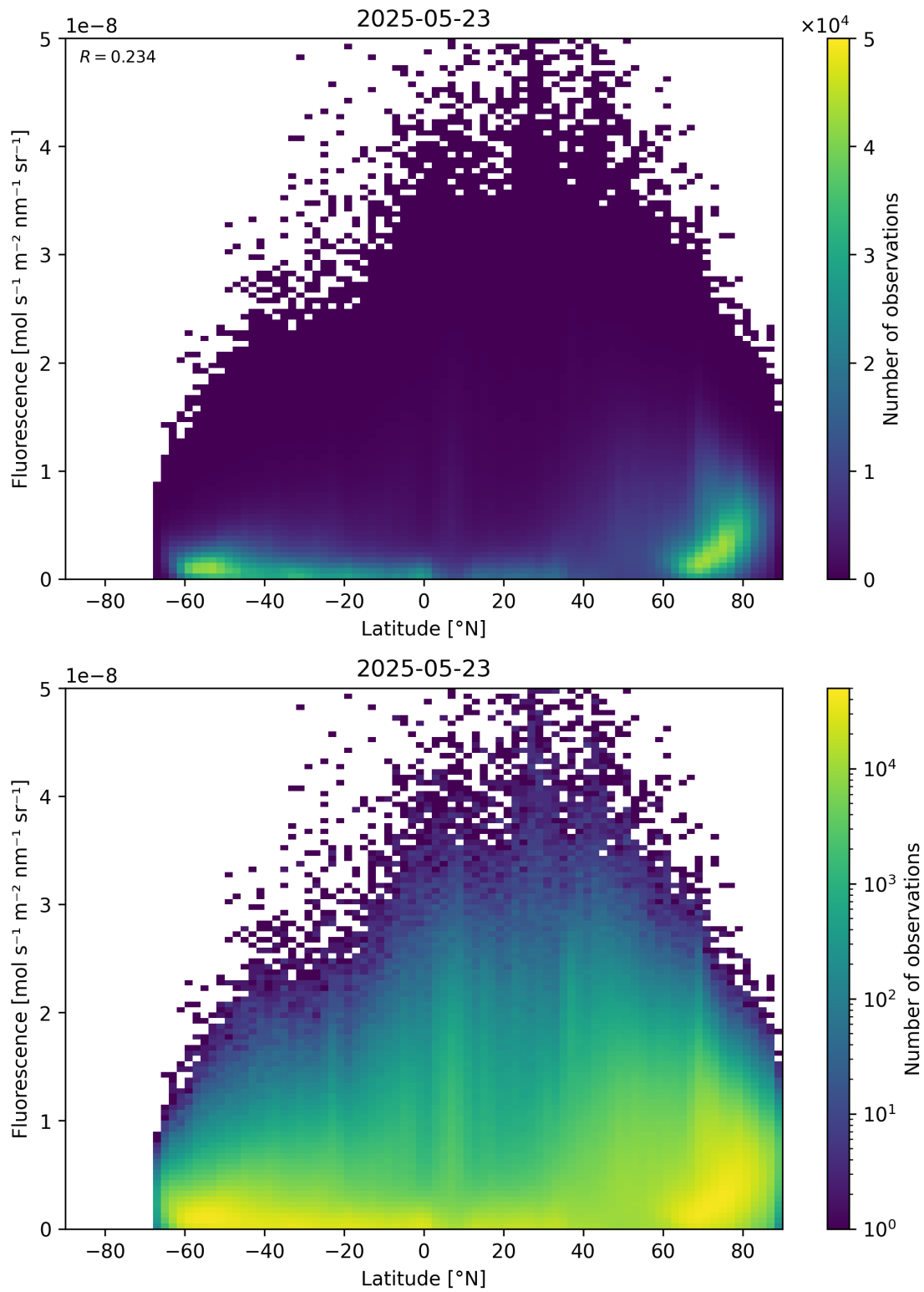
Figure 92: Scatter density plot of “Latitude” against “Fluorescence” for 2025-05-22 to 2025-05-24.
