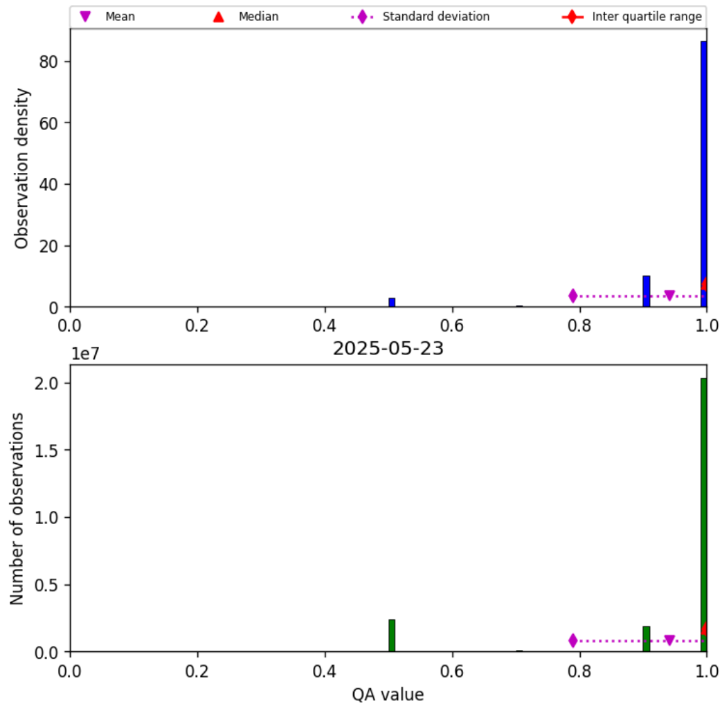
Figure 29: Histogram of “QA value” for 2025-05-22 to 2025-05-24
