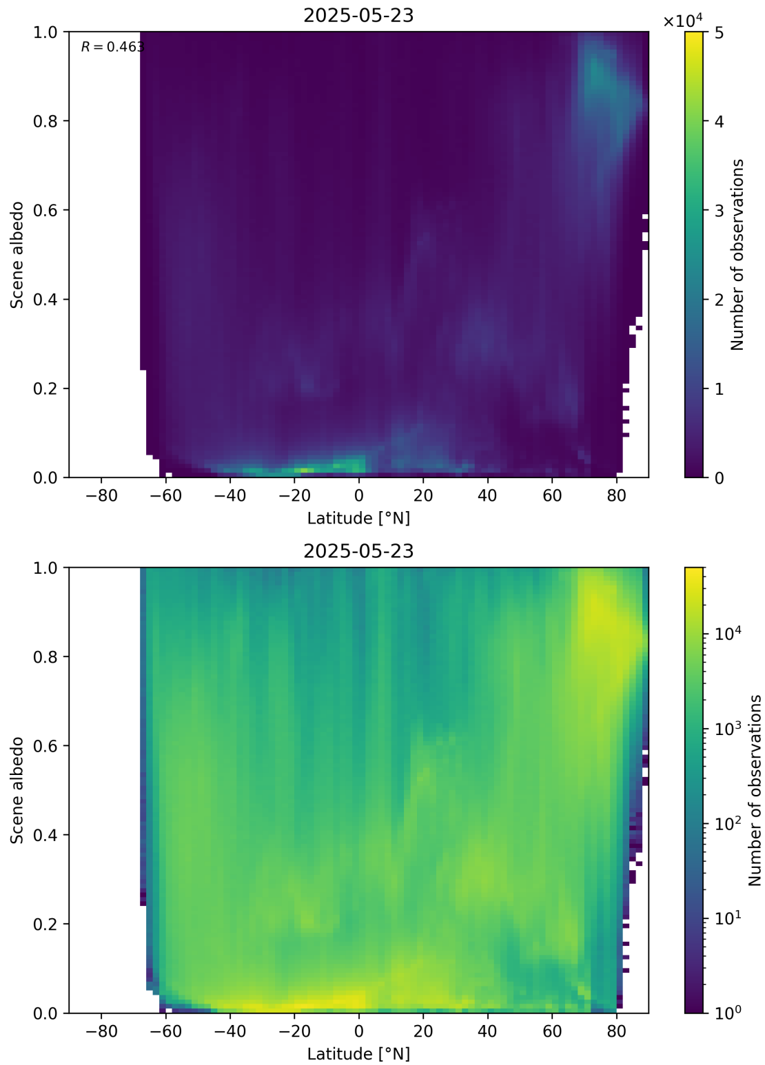
Figure 95: Scatter density plot of “Latitude” against “Scene albedo” for 2025-05-22 to 2025-05-24.
