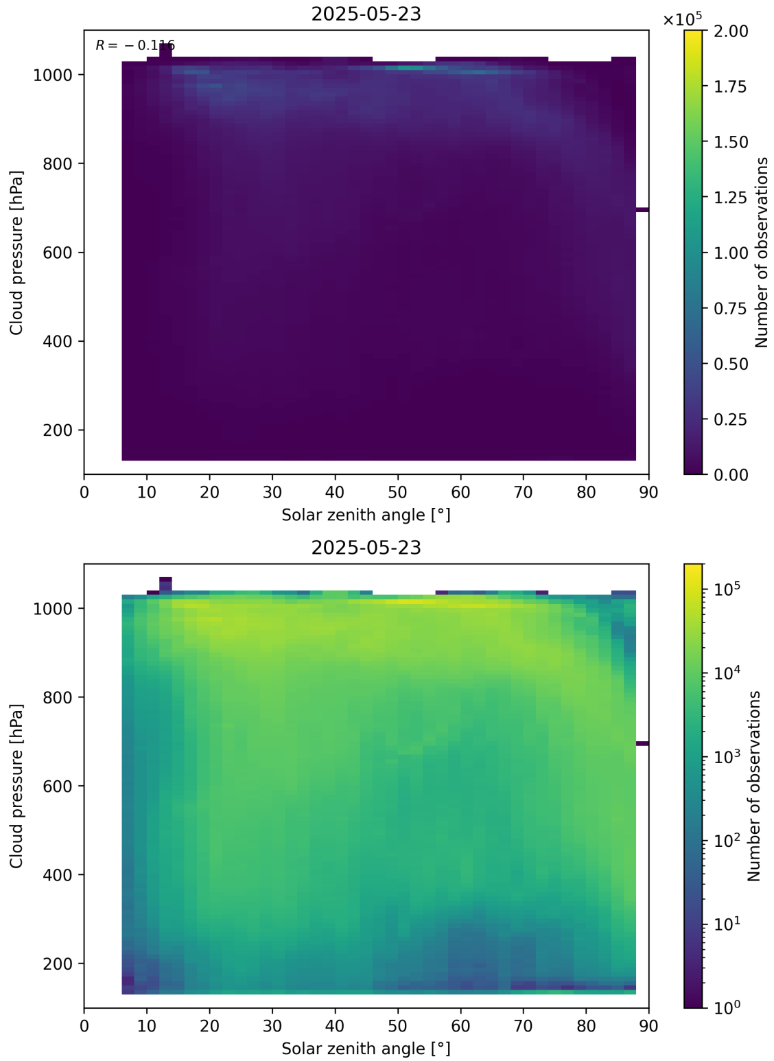
Figure 111: Scatter density plot of “Solar zenith angle” against “Cloud pressure” for 2025-05-22 to 2025-05-24.
