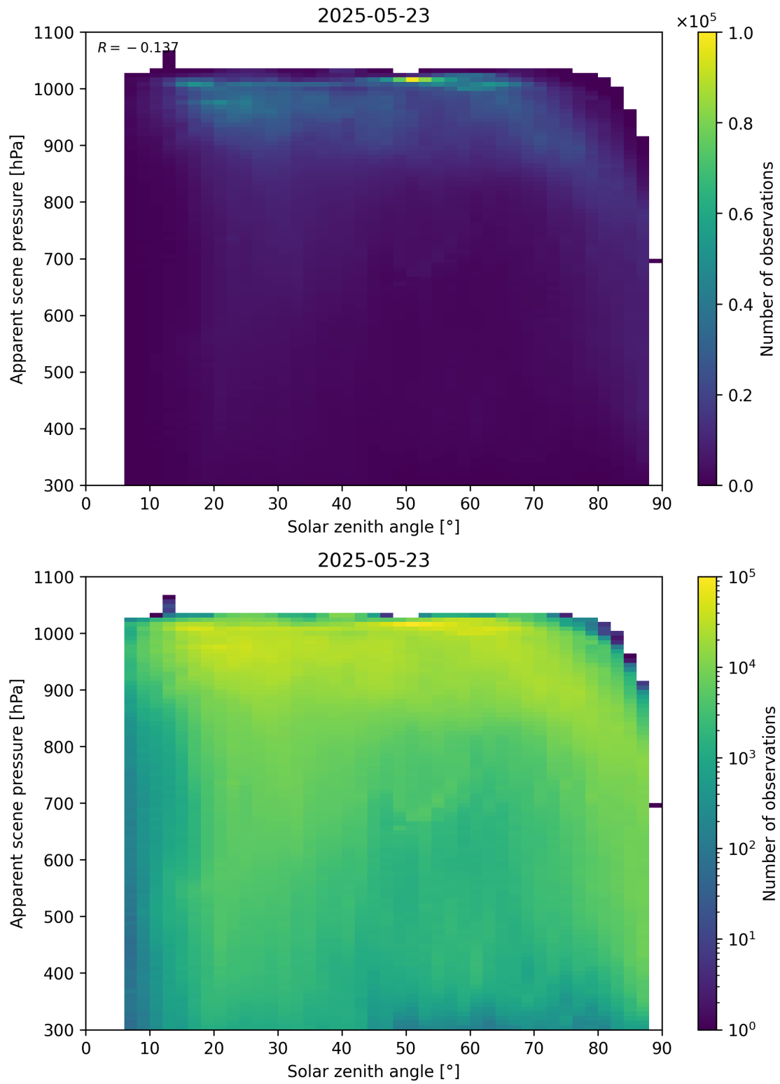
Figure 108: Scatter density plot of “Solar zenith angle” against “Apparent scene pressure” for 2025-05-22 to 2025-05-24.
