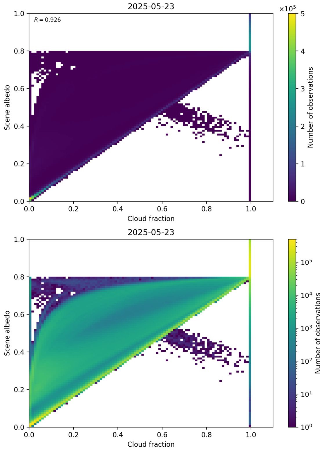
Figure 75: Scatter density plot of “Cloud fraction” against “Scene albedo” for 2025-05-22 to 2025-05-24.
