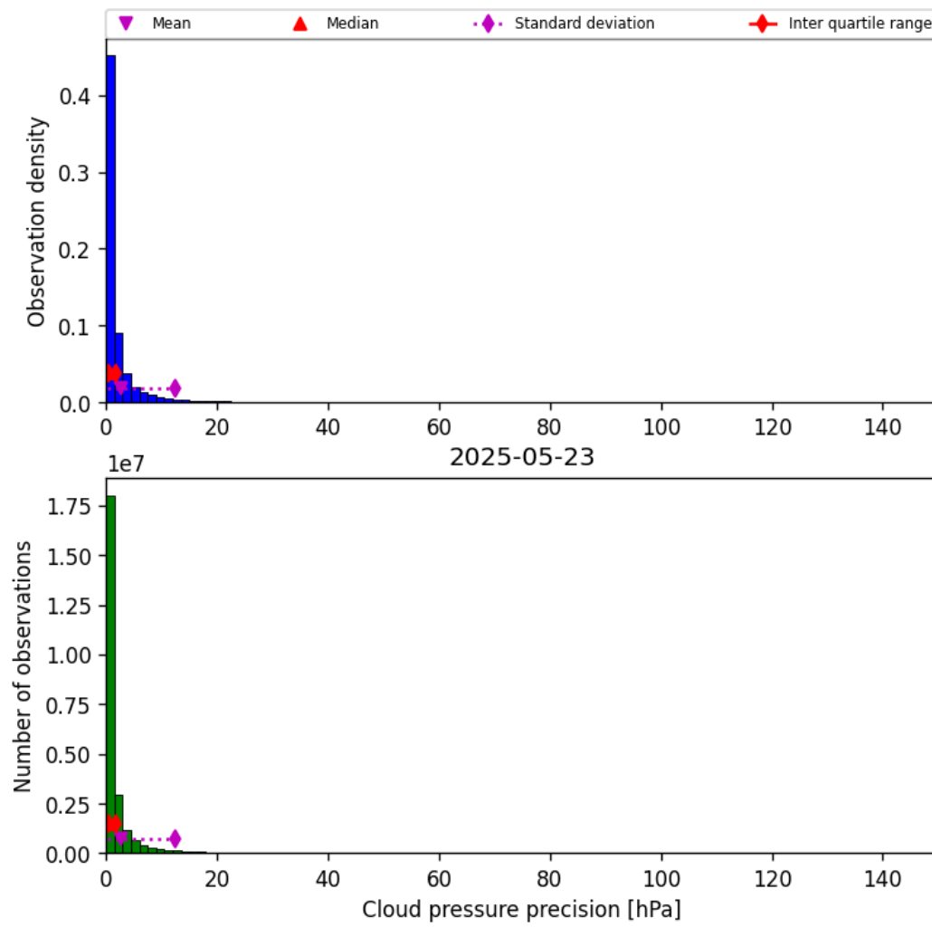
Figure 31: Histogram of “Cloud pressure precision” for 2025-05-22 to 2025-05-24
