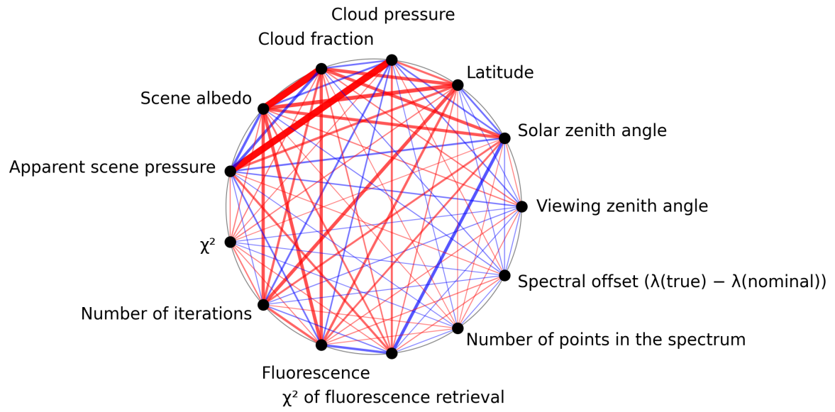
Figure 1: Map of correlation graph for 2025-05-22 to 2025-05-24.
