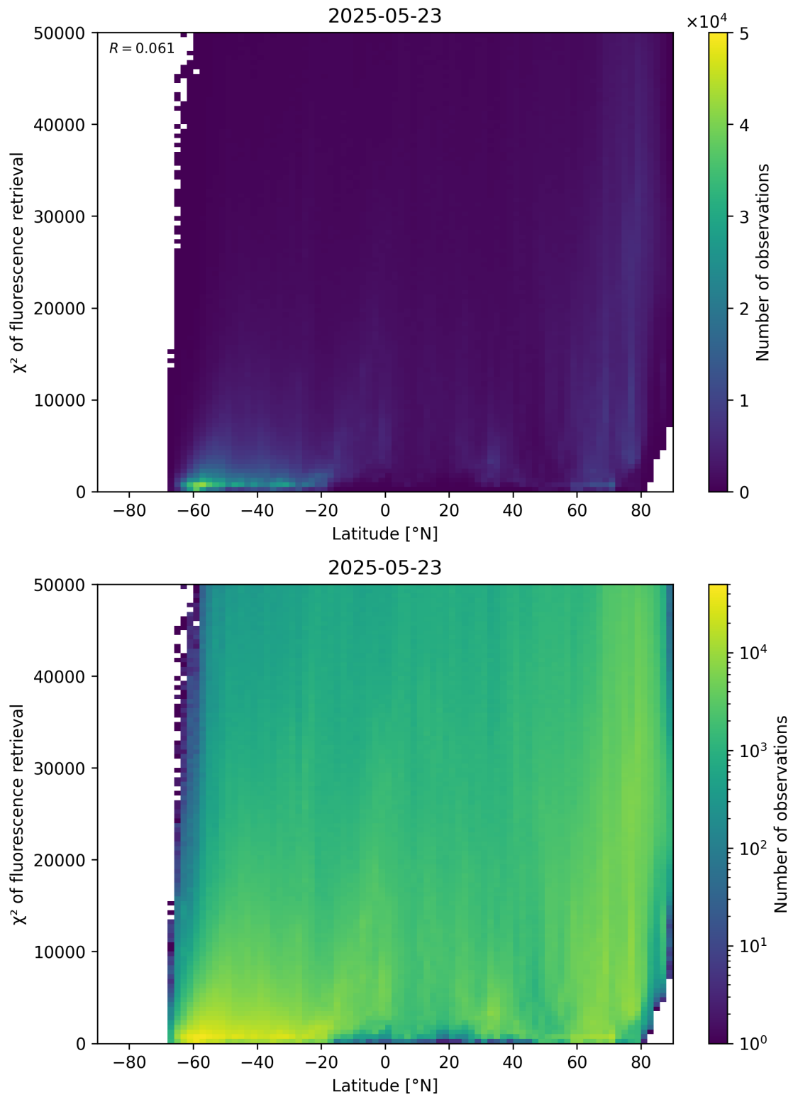
Figure 89: Scatter density plot of “Latitude” against “ \chi^2 of fluorescence retrieval” for 2025-05-22 to 2025-05-24.
