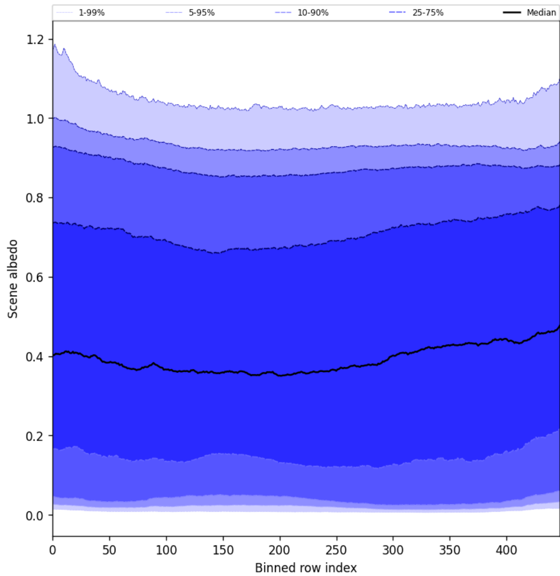
Figure 51: Along track statistics of “Scene albedo” for 2025-05-22 to 2025-05-24
