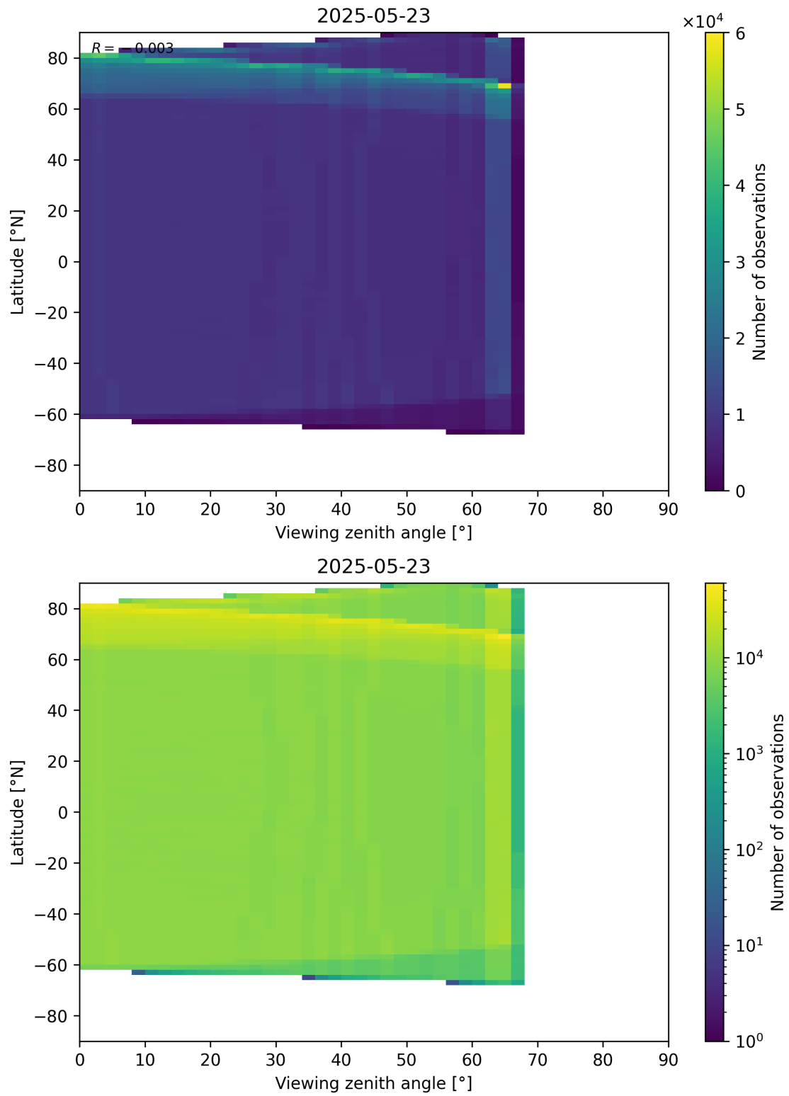
Figure 123: Scatter density plot of “Viewing zenith angle” against “Latitude” for 2025-05-22 to 2025-05-24.
