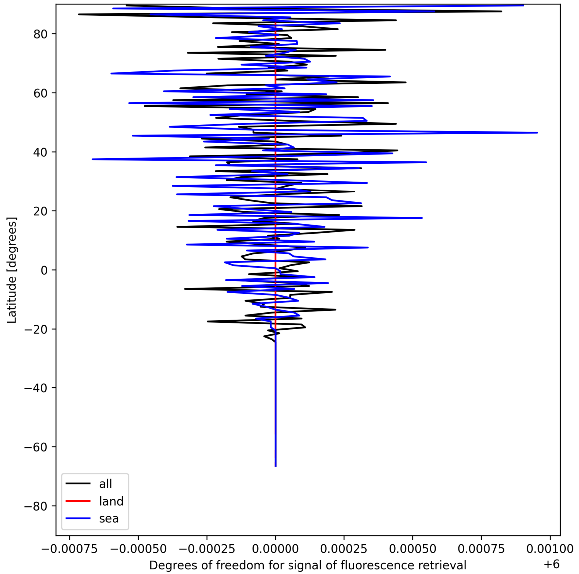
Figure 26: Zonal average of “Degrees of freedom for signal of fluorescence retrieval” for 2025-05-22 to 2025-05-24.
