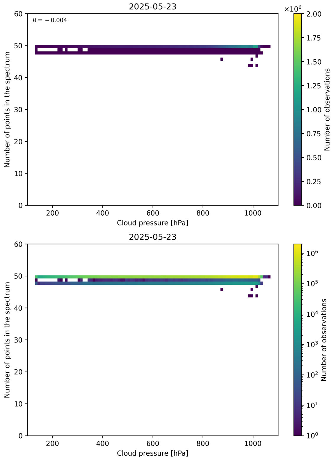
Figure 82: Scatter density plot of “Cloud pressure” against “Number of points in the spectrum” for 2025-05-22 to 2025-05-24.
