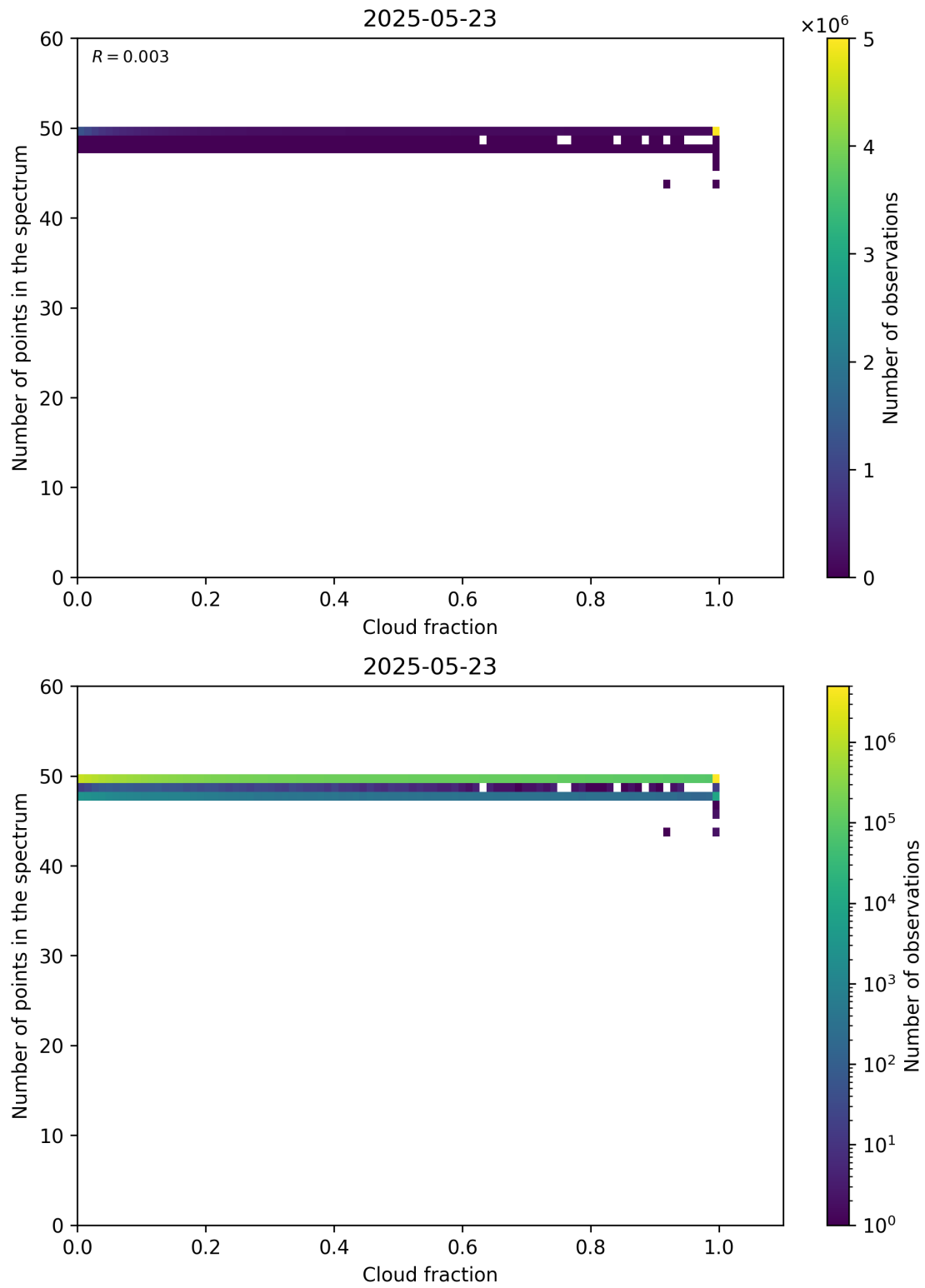
Figure 74: Scatter density plot of “Cloud fraction” against “Number of points in the spectrum” for 2025-05-22 to 2025-05-24.
