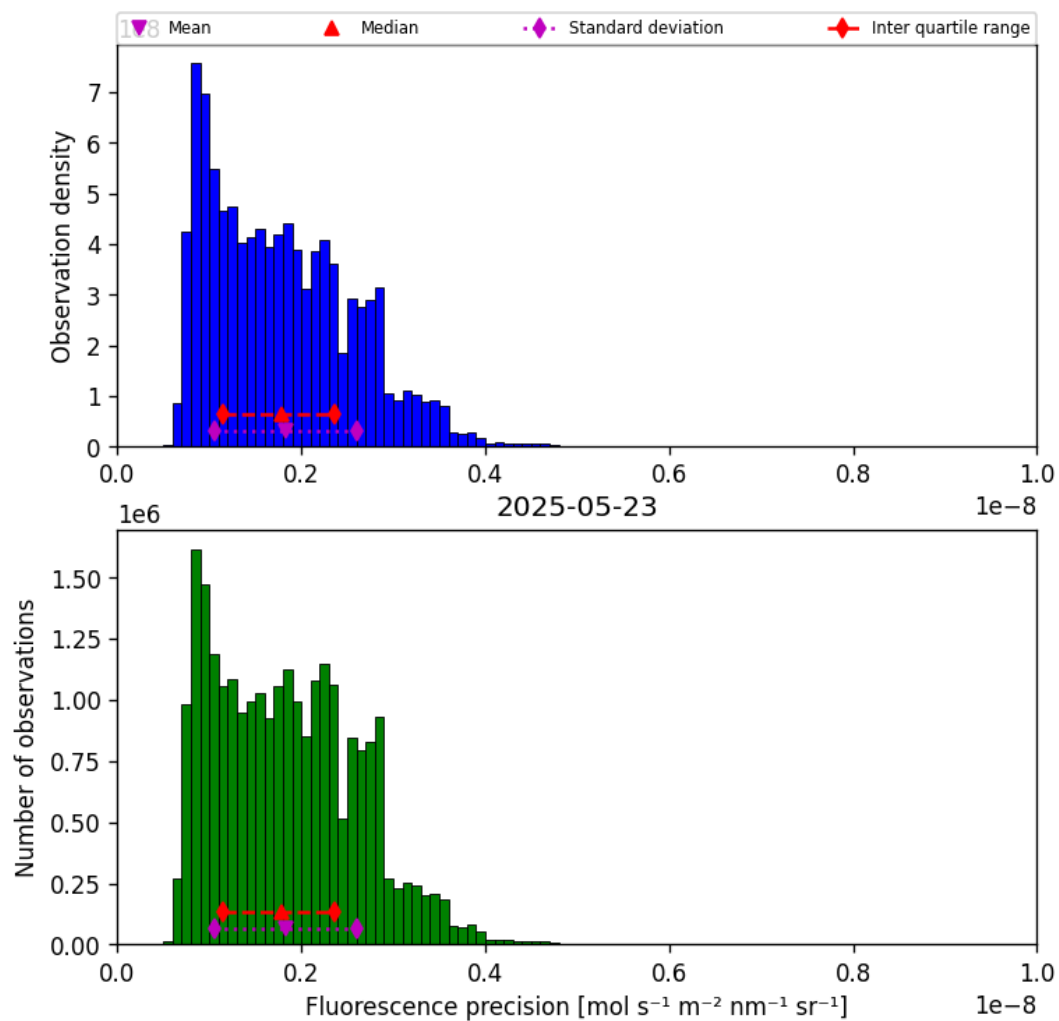
Figure 41: Histogram of “Fluorescence precision” for 2025-05-22 to 2025-05-24
