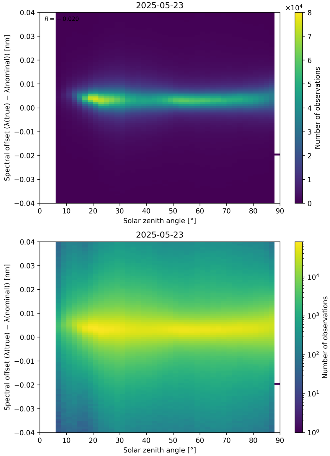
Figure 117: Scatter density plot of “Solar zenith angle” against “Spectral offset ( \lambda_{\text{true}} - \lambda_{\text{nominal}} )” for 2025-05-22 to 2025-05-24.
