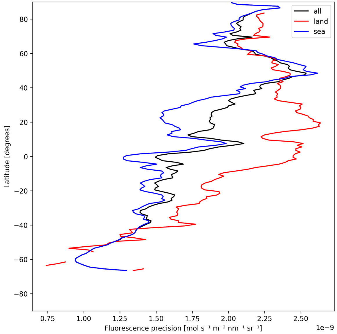
Figure 24: Zonal average of “Fluorescence precision” for 2025-05-22 to 2025-05-24.
