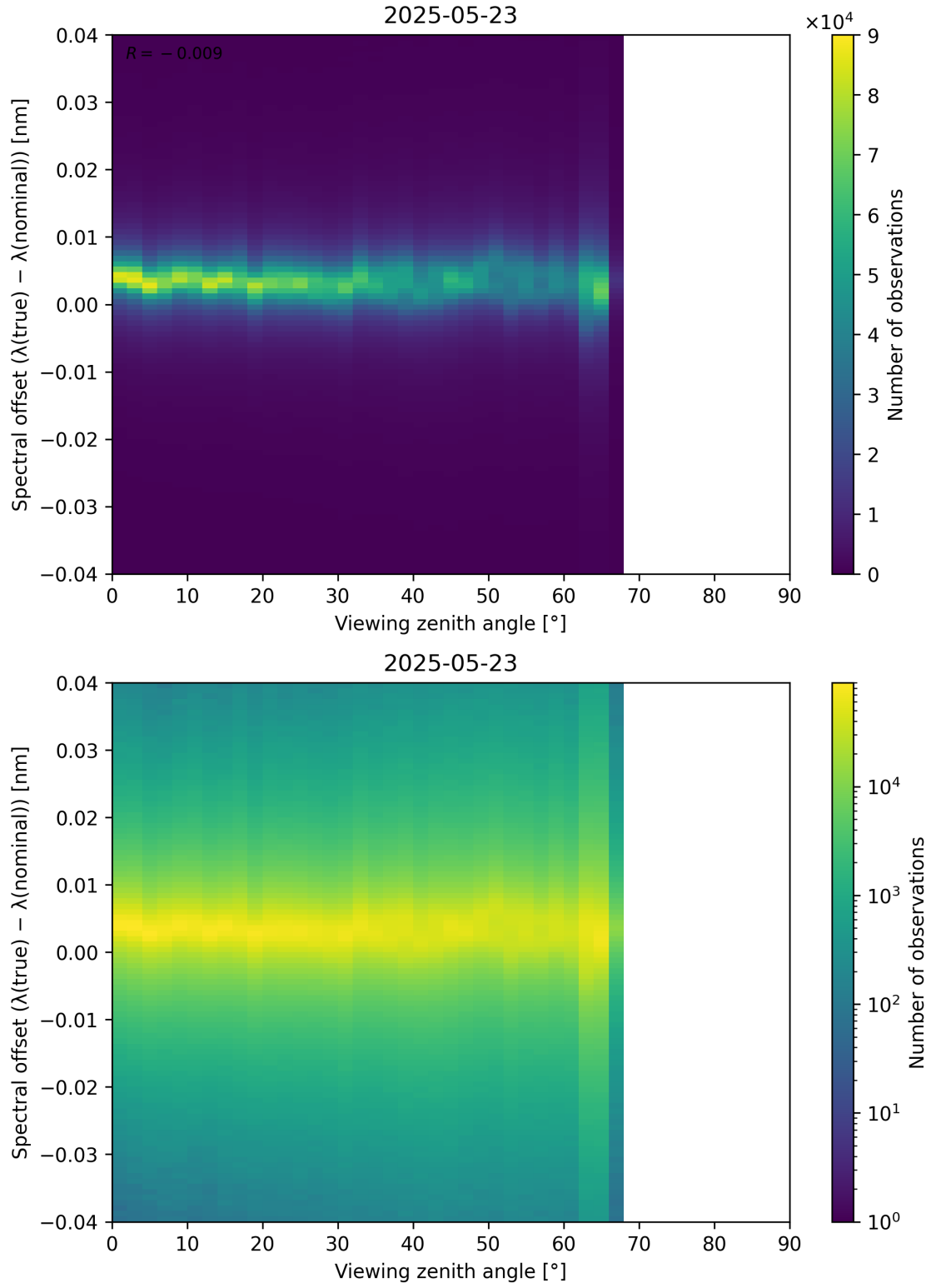
Figure 128: Scatter density plot of “Viewing zenith angle” against “Spectral offset ( \lambda_{\text{true}} - \lambda_{\text{nominal}} )” for 2025-05-22 to 2025-05-24.
