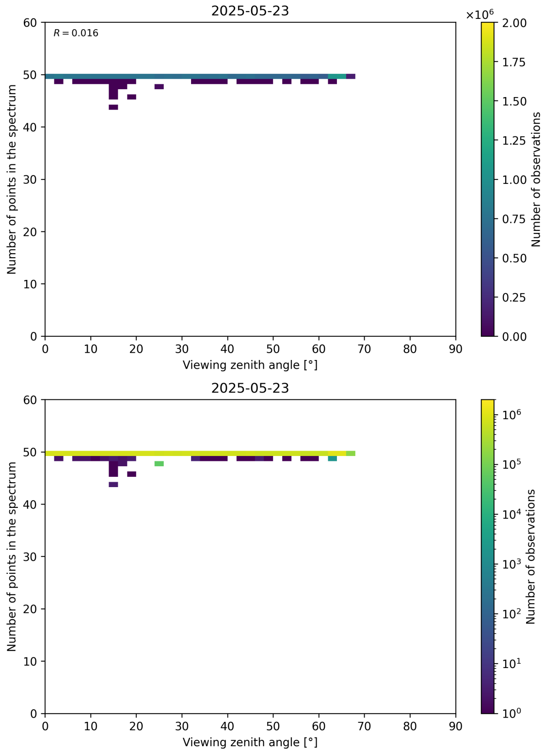
Figure 125: Scatter density plot of “Viewing zenith angle” against “Number of points in the spectrum” for 2025-05-22 to 2025-05-24.
