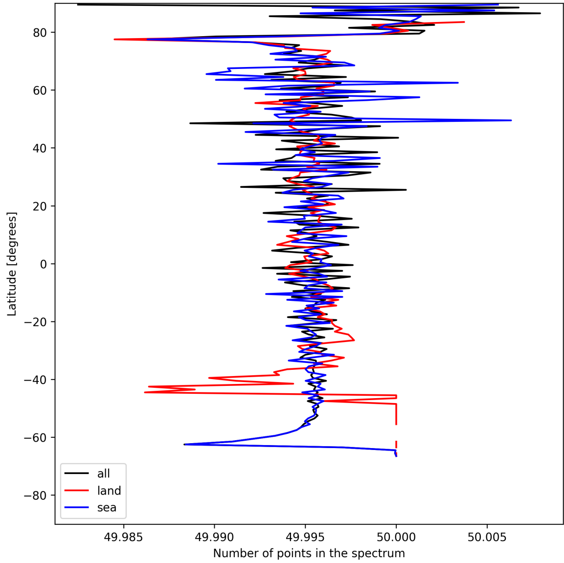
Figure 27: Zonal average of “Number of points in the spectrum” for 2025-05-22 to 2025-05-24.
