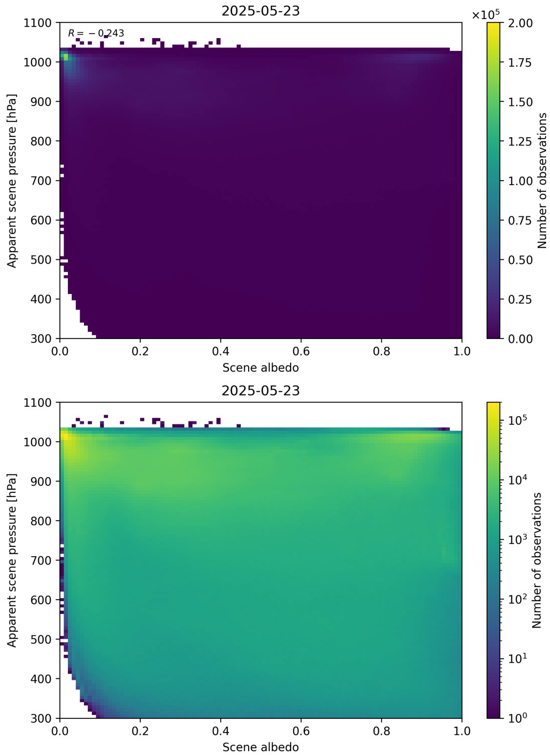
Figure 102: Scatter density plot of “Scene albedo” against “Apparent scene pressure” for 2025-05-22 to 2025-05-24.
