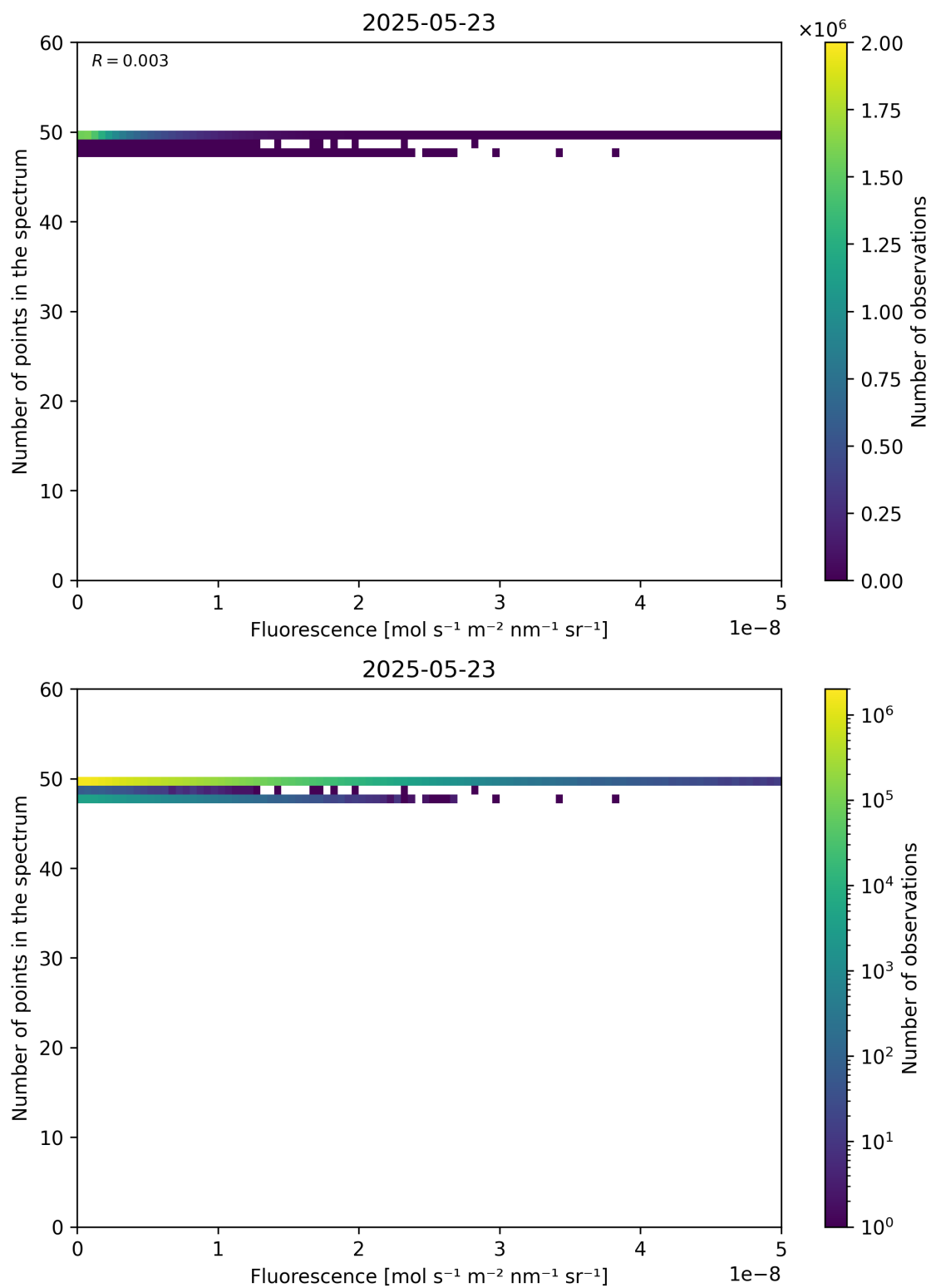
Figure 86: Scatter density plot of “Fluorescence” against “Number of points in the spectrum” for 2025-05-22 to 2025-05-24.
