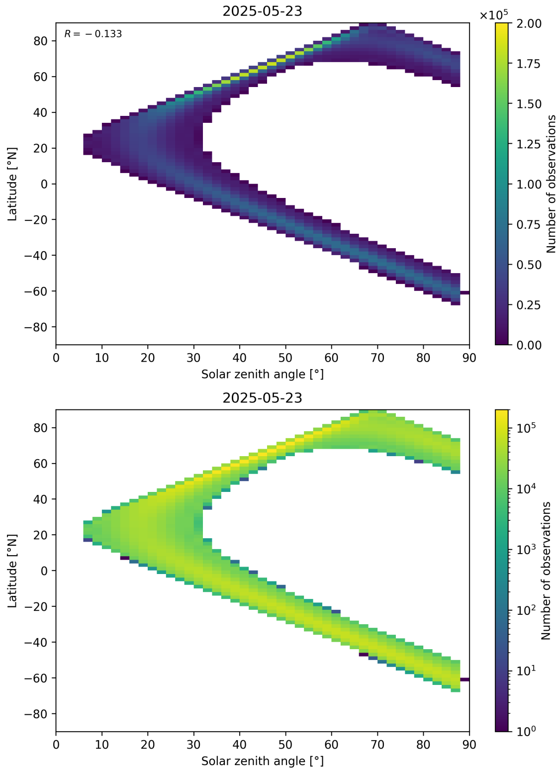
Figure 113: Scatter density plot of “Solar zenith angle” against “Latitude” for 2025-05-22 to 2025-05-24.
