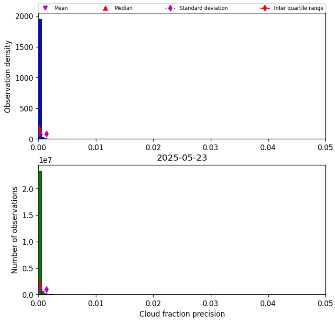
Figure 33: Histogram of “Cloud fraction precision” for 2025-05-22 to 2025-05-24
