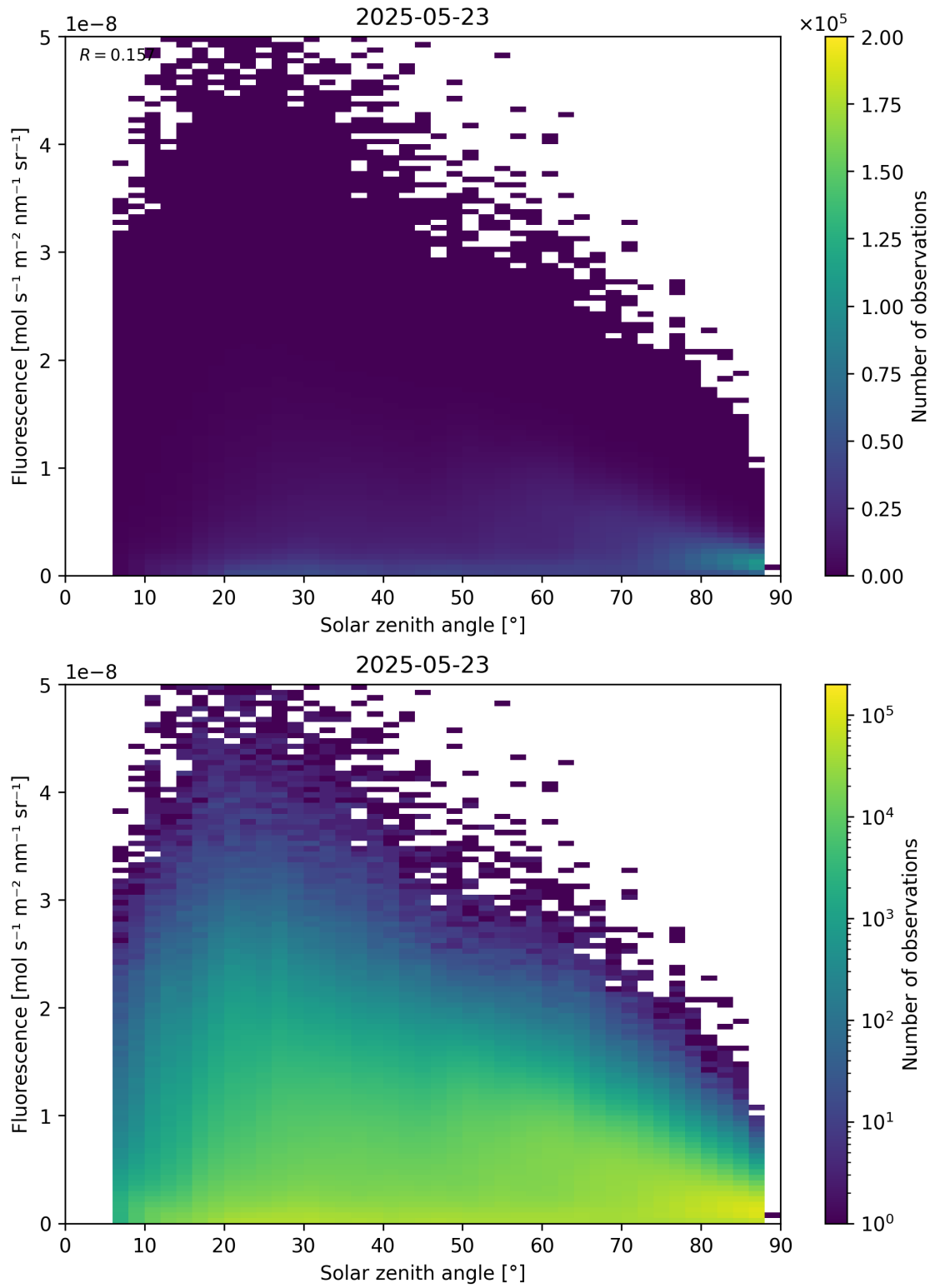
Figure 112: Scatter density plot of “Solar zenith angle” against “Fluorescence” for 2025-05-22 to 2025-05-24.
