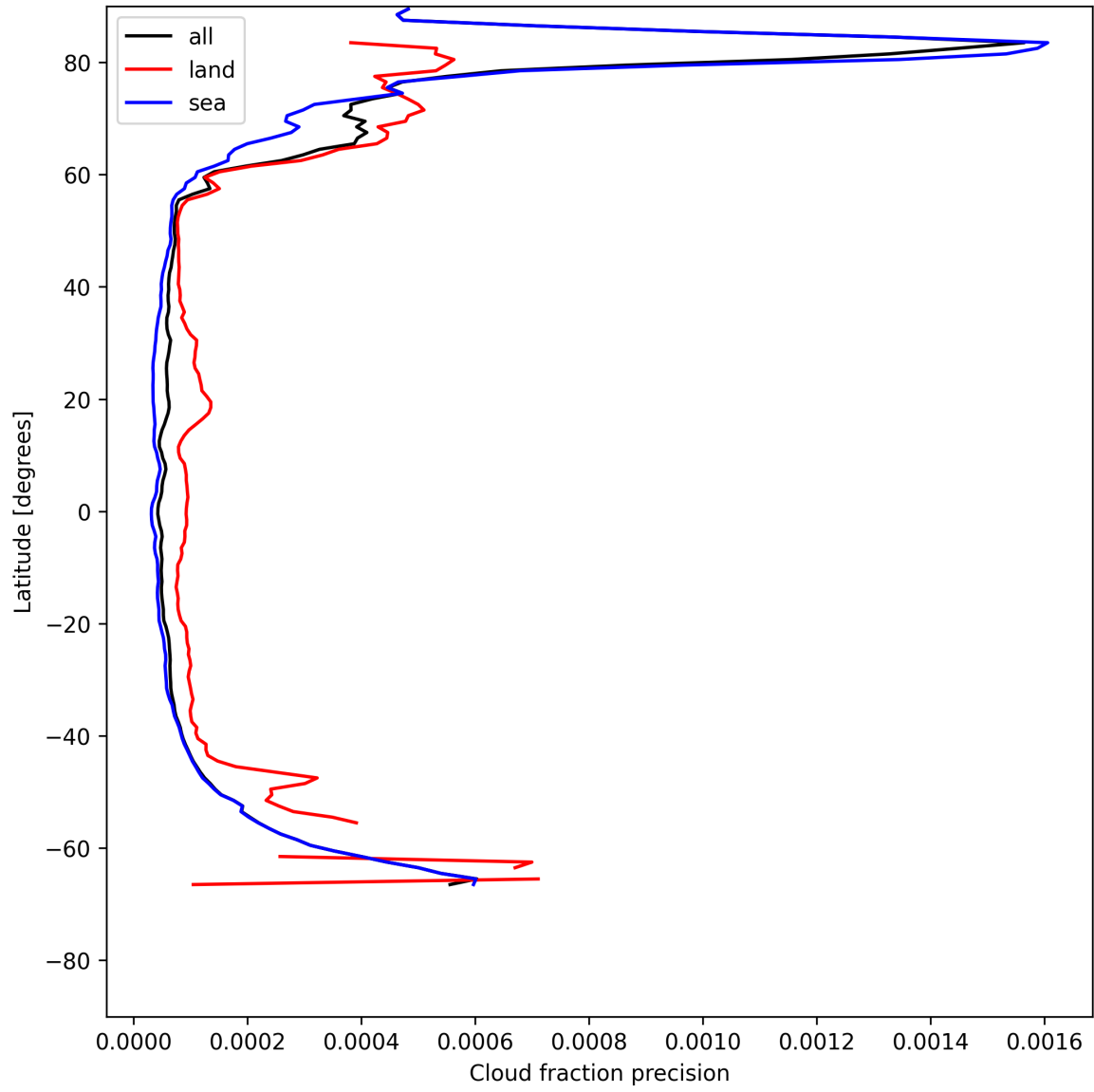
Figure 16: Zonal average of “Cloud fraction precision” for 2025-05-22 to 2025-05-24.
