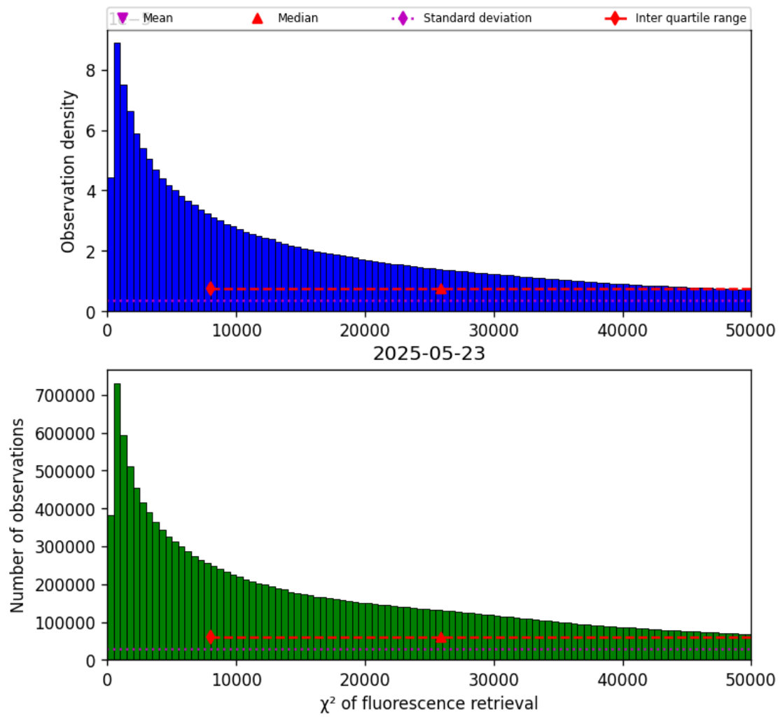
Figure 42: Histogram of “ \chi^2 of fluorescence retrieval” for 2025-05-22 to 2025-05-24
