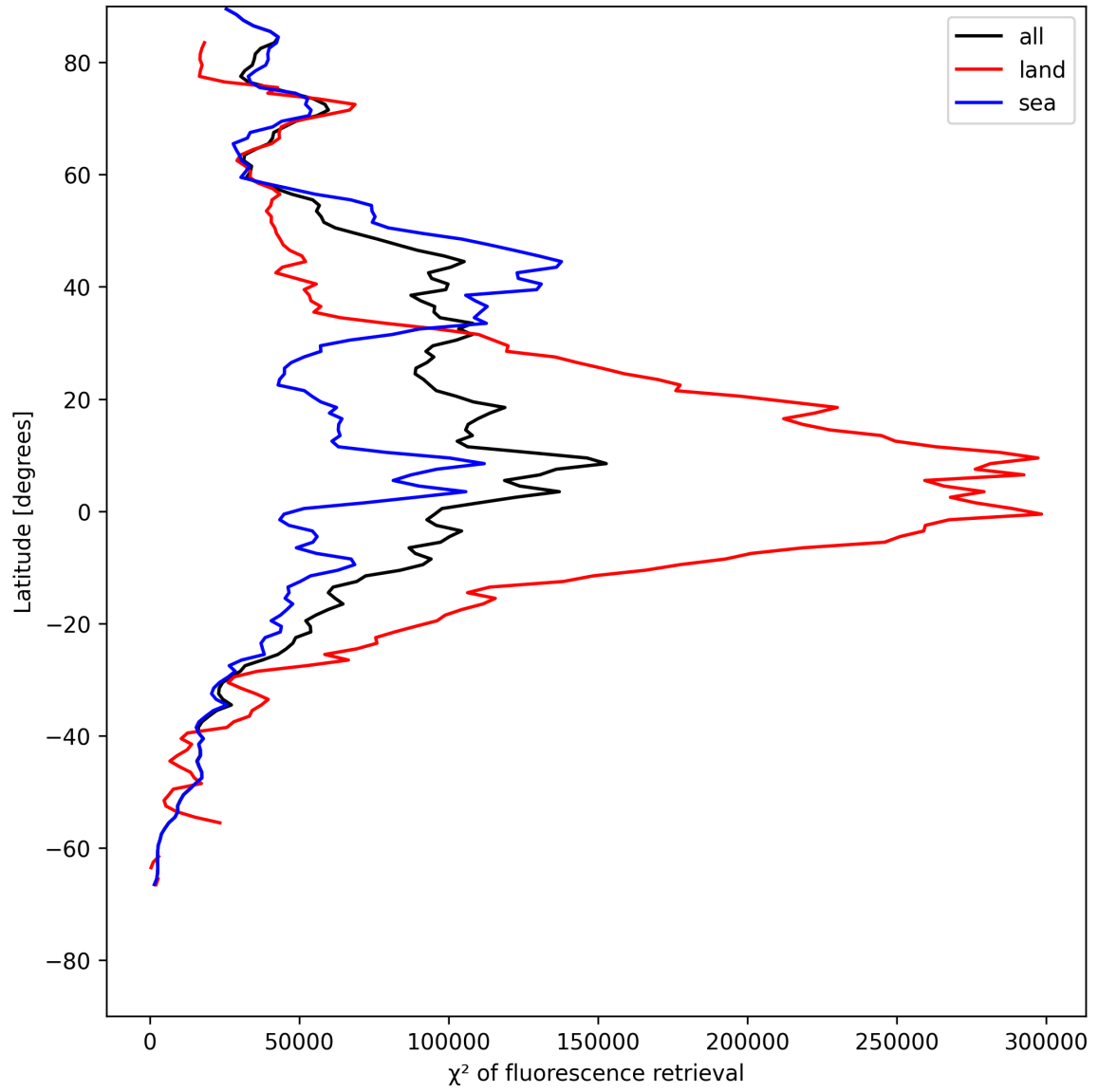
Figure 25: Zonal average of “ \chi^2 of fluorescence retrieval” for 2025-05-22 to 2025-05-24.
