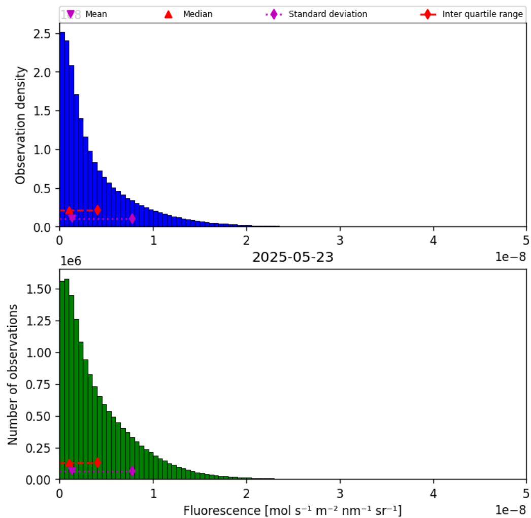
Figure 40: Histogram of “Fluorescence” for 2025-05-22 to 2025-05-24
