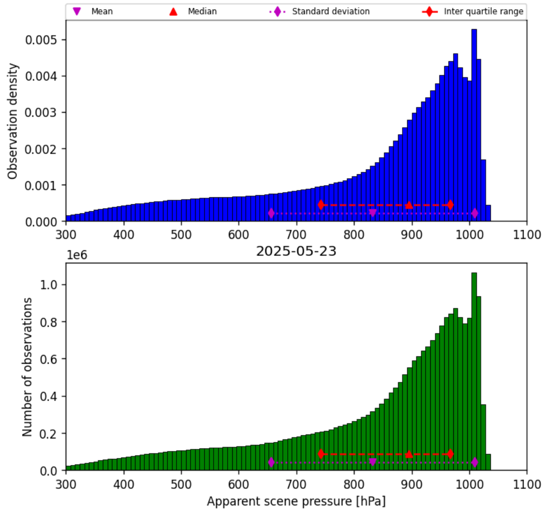
Figure 36: Histogram of “Apparent scene pressure” for 2025-05-22 to 2025-05-24
