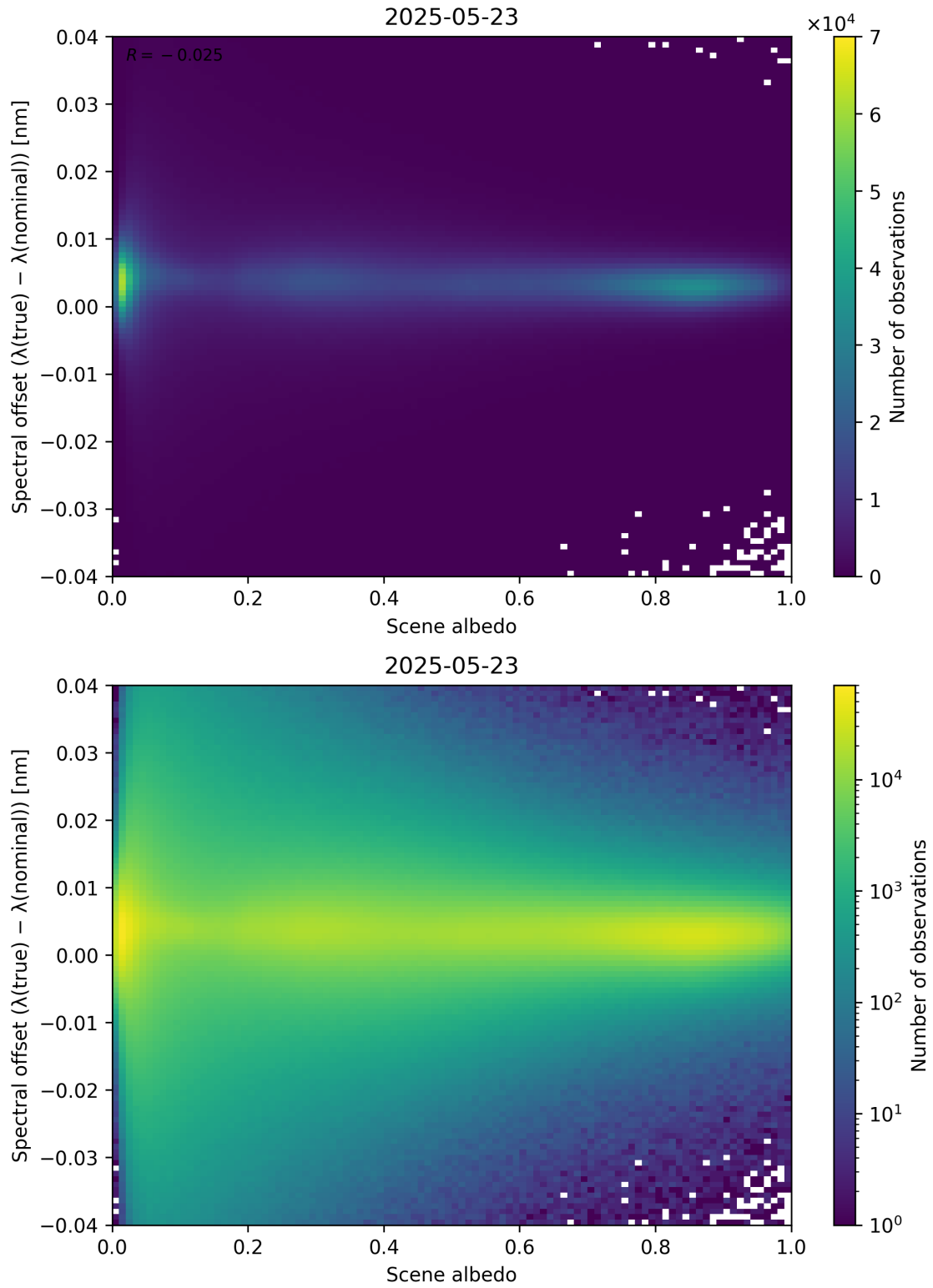
Figure 107: Scatter density plot of “Scene albedo” against “Spectral offset ( \lambda_{\text{true}} - \lambda_{\text{nominal}} )” for 2025-05-22 to 2025-05-24.
