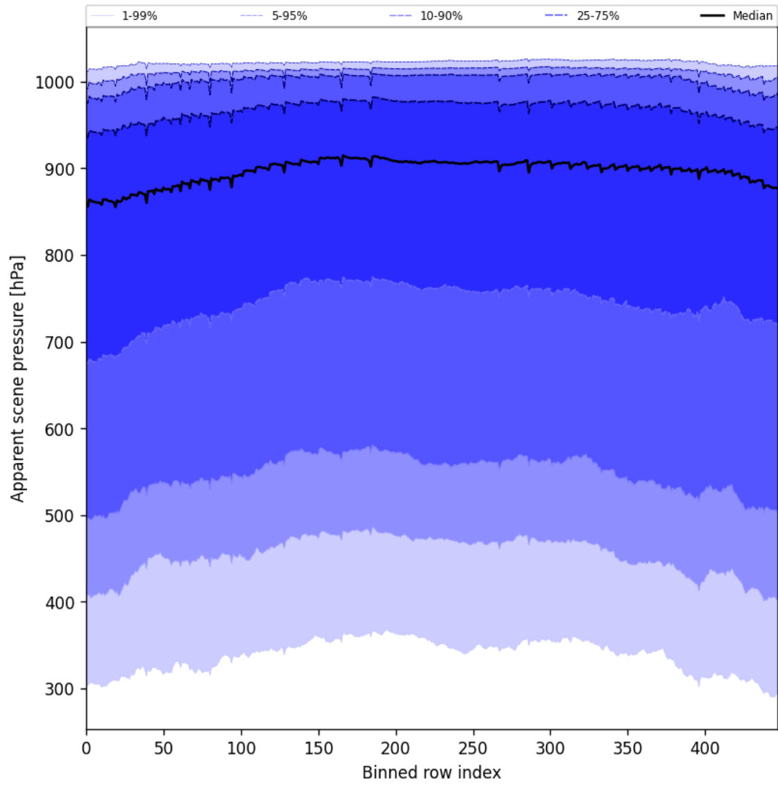
Figure 53: Along track statistics of “Apparent scene pressure” for 2025-05-22 to 2025-05-24
