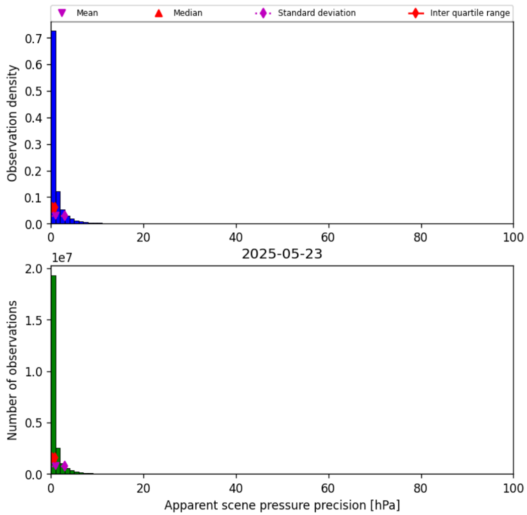
Figure 37: Histogram of “Apparent scene pressure precision” for 2025-05-22 to 2025-05-24
