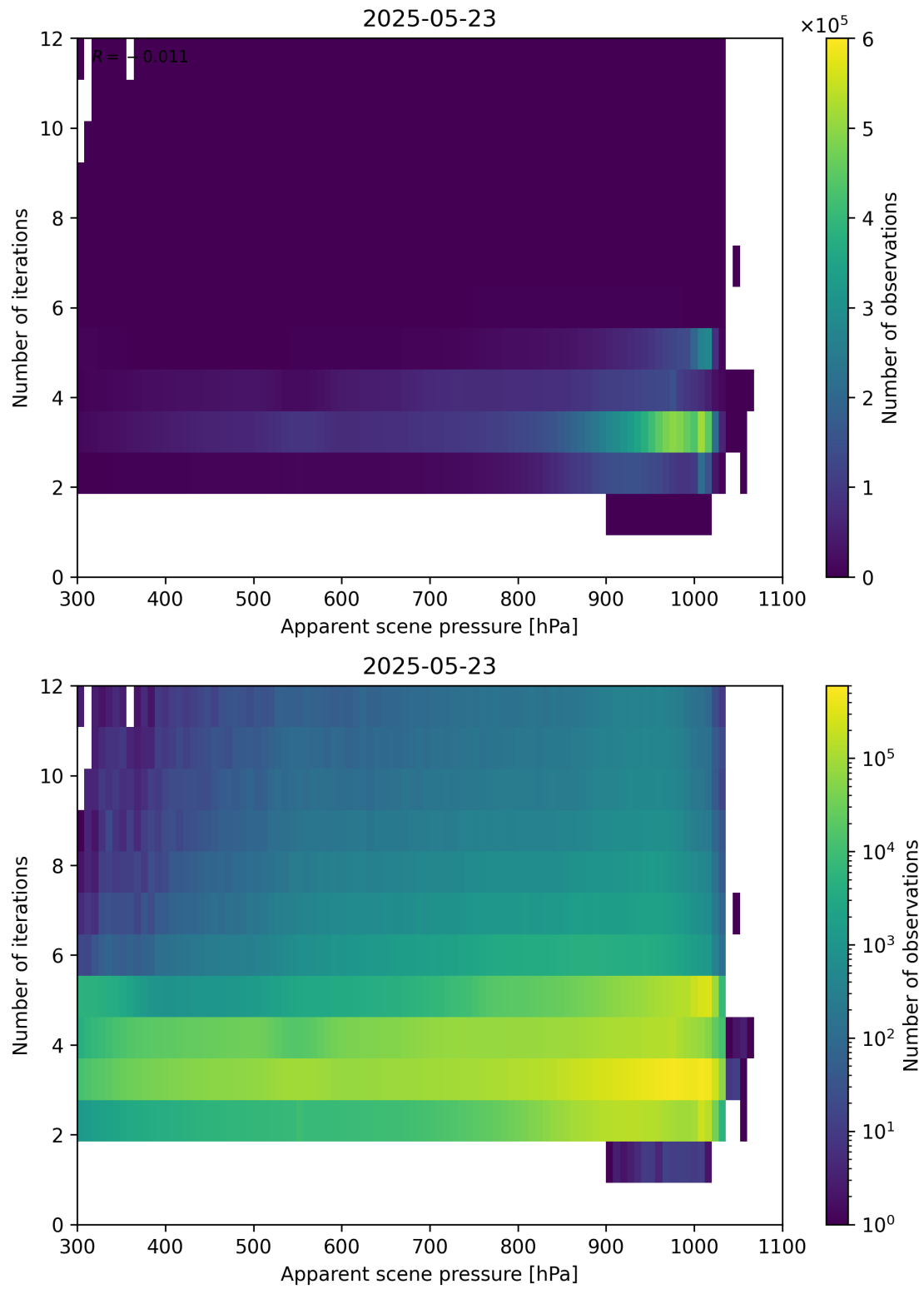
Figure 65: Scatter density plot of “Apparent scene pressure” against “Number of iterations” for 2025-05-22 to 2025-05-24.
