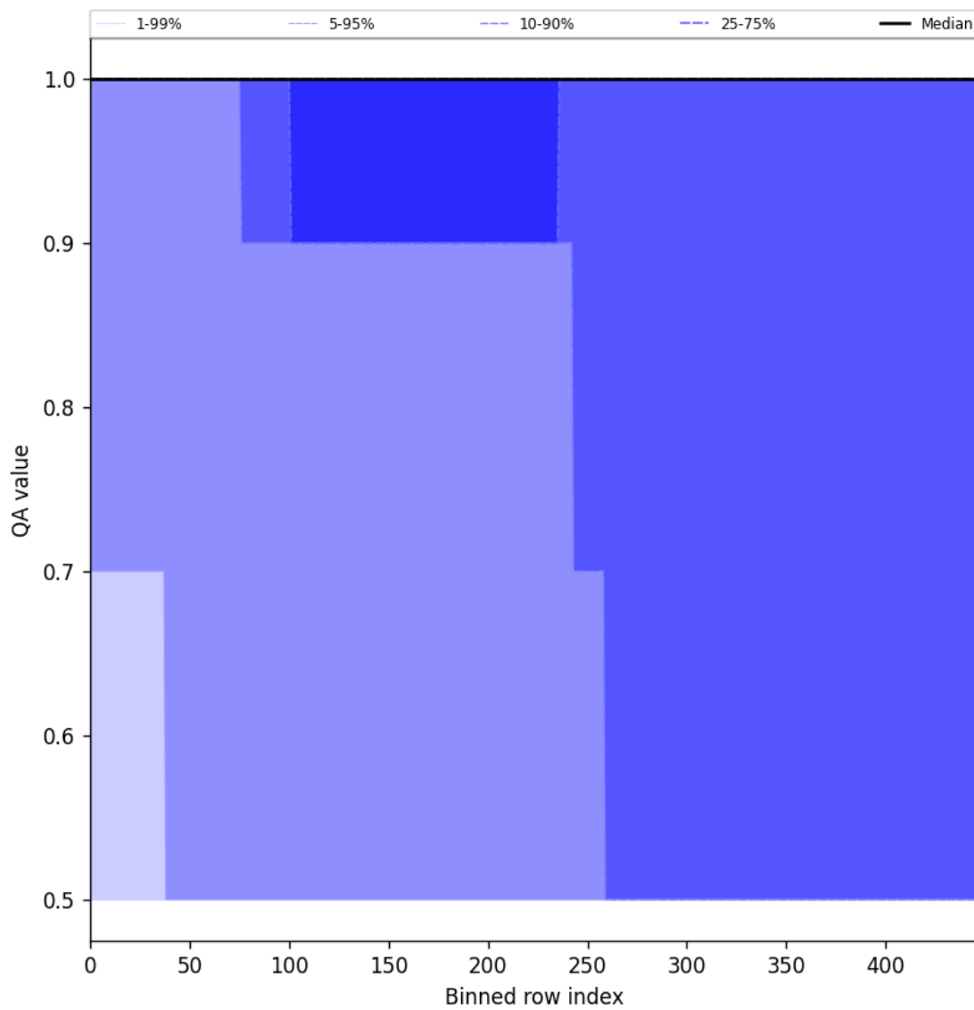
Figure 46: Along track statistics of “QA value” for 2025-05-22 to 2025-05-24
