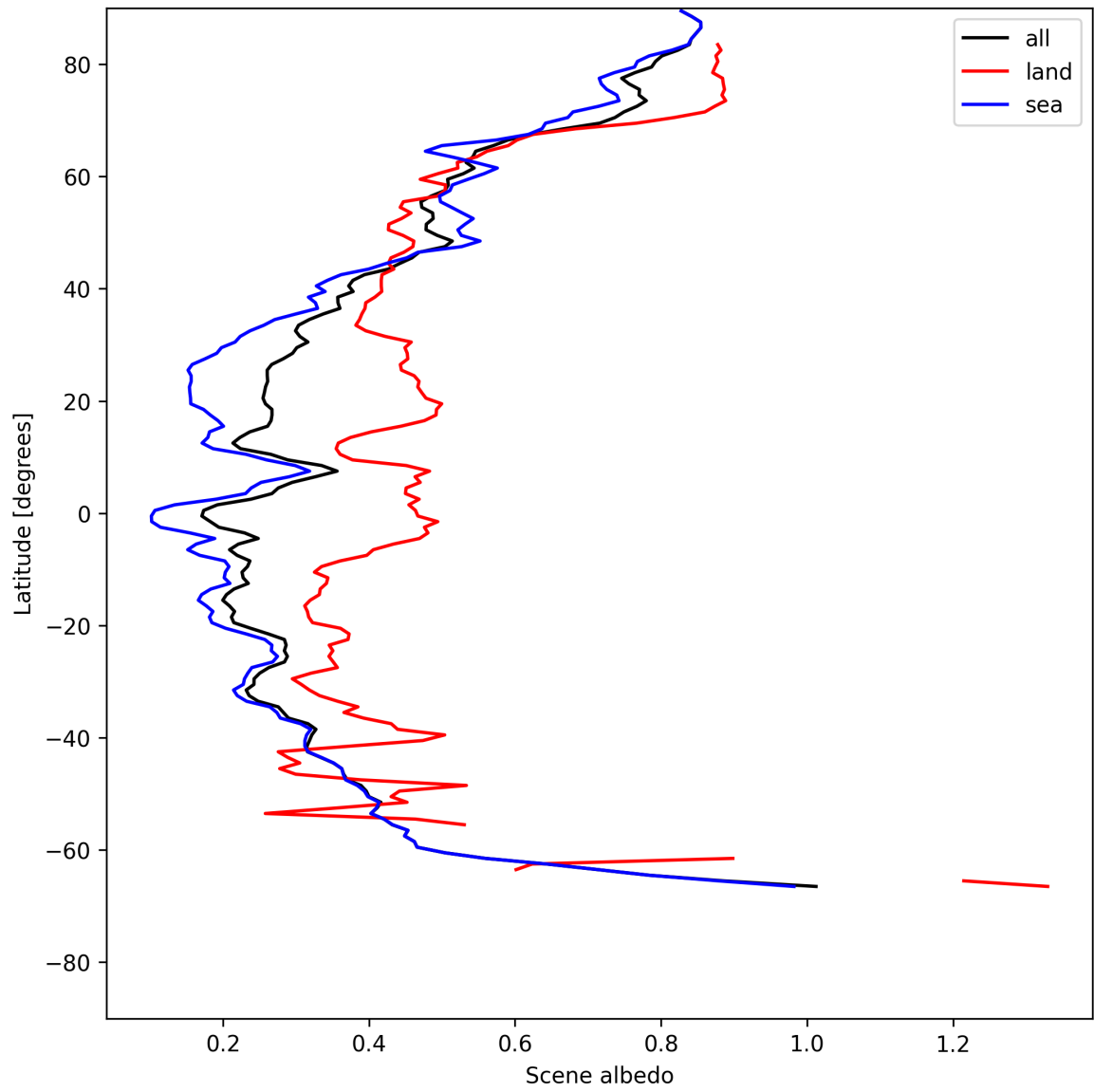
Figure 17: Zonal average of “Scene albedo” for 2025-05-22 to 2025-05-24.
