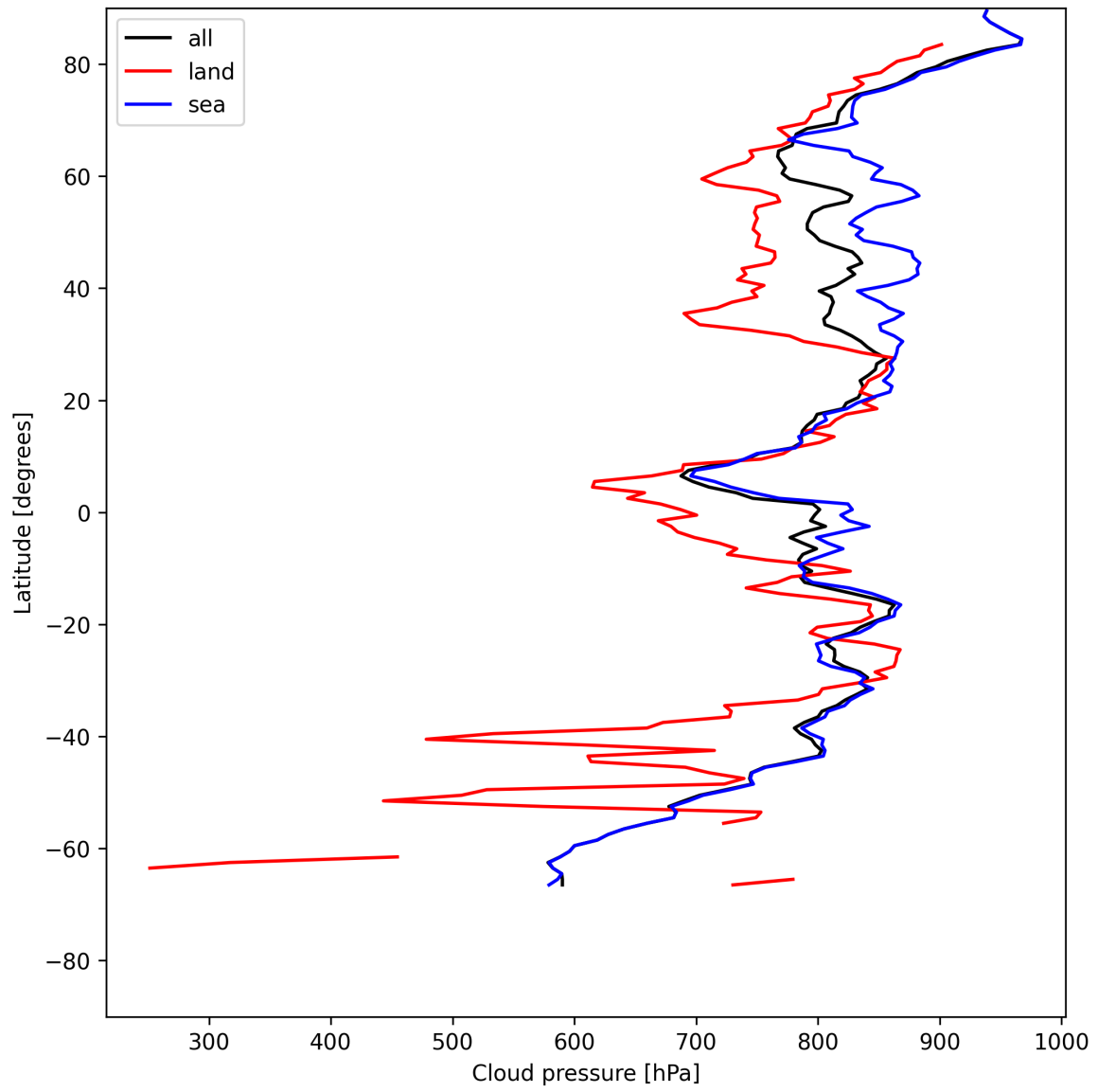
Figure 13: Zonal average of “Cloud pressure” for 2025-05-22 to 2025-05-24.
