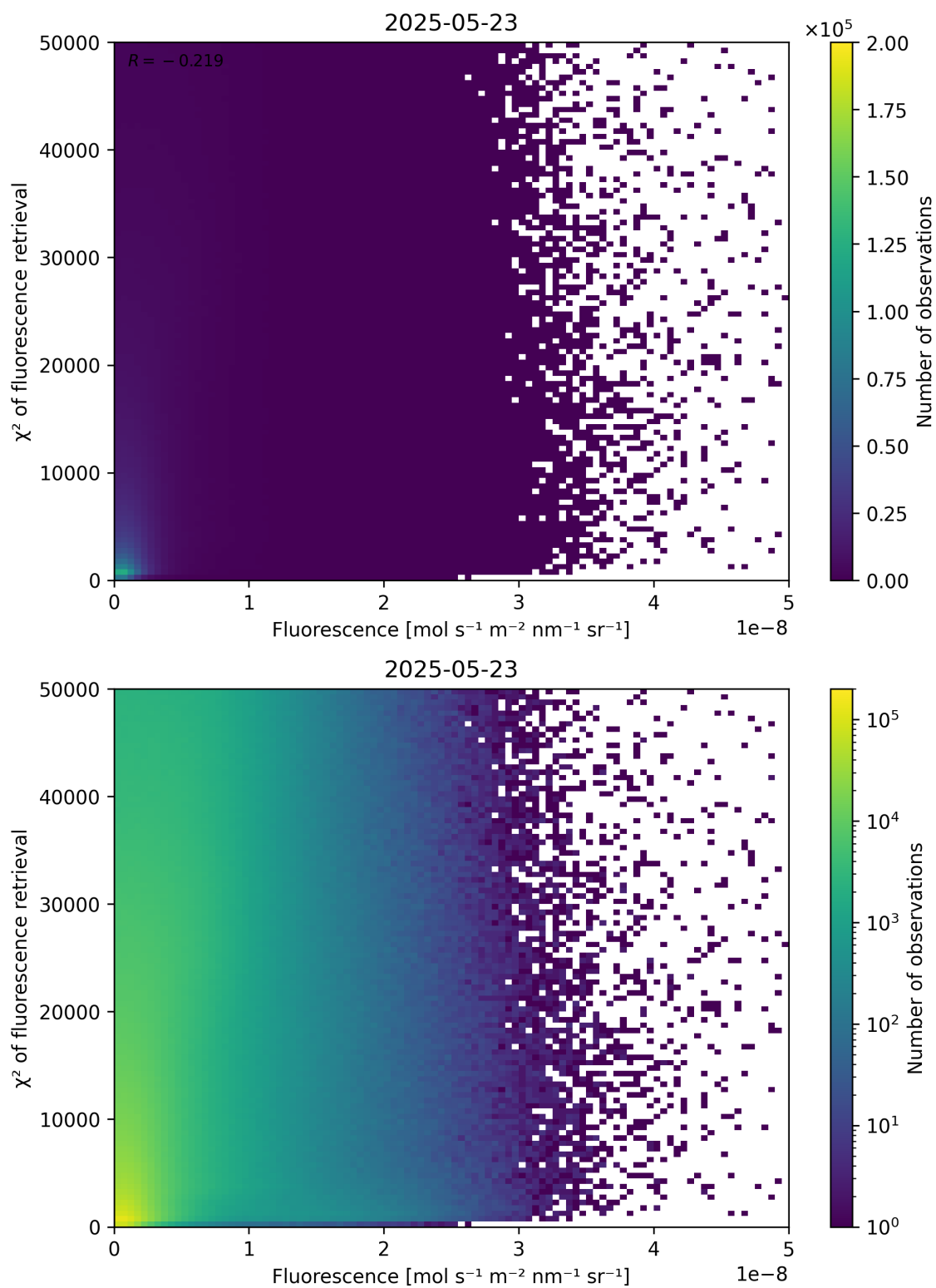
Figure 85: Scatter density plot of “Fluorescence” against “ \chi^2 of fluorescence retrieval” for 2025-05-22 to 2025-05-24.
