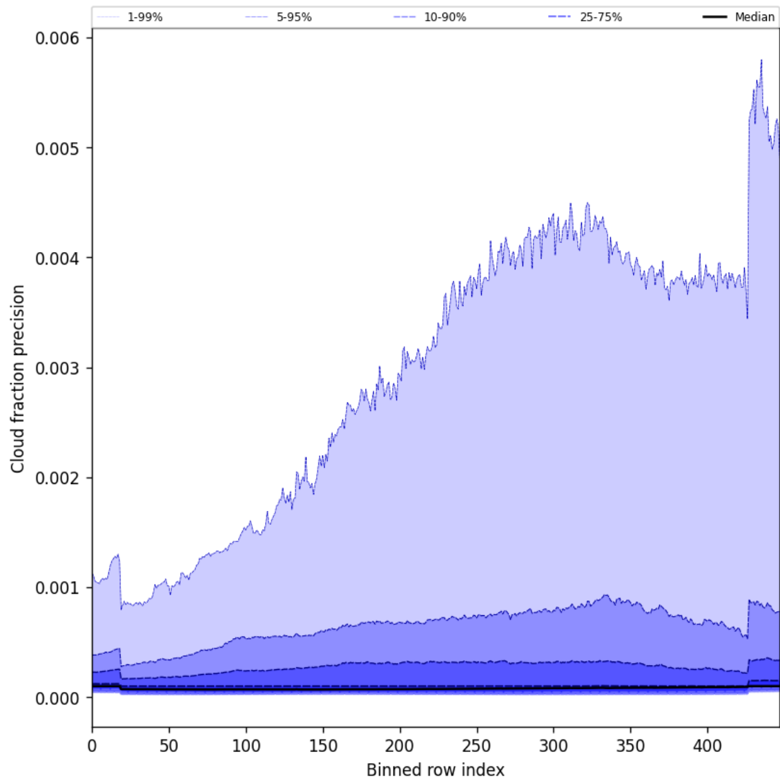
Figure 50: Along track statistics of “Cloud fraction precision” for 2025-05-22 to 2025-05-24
