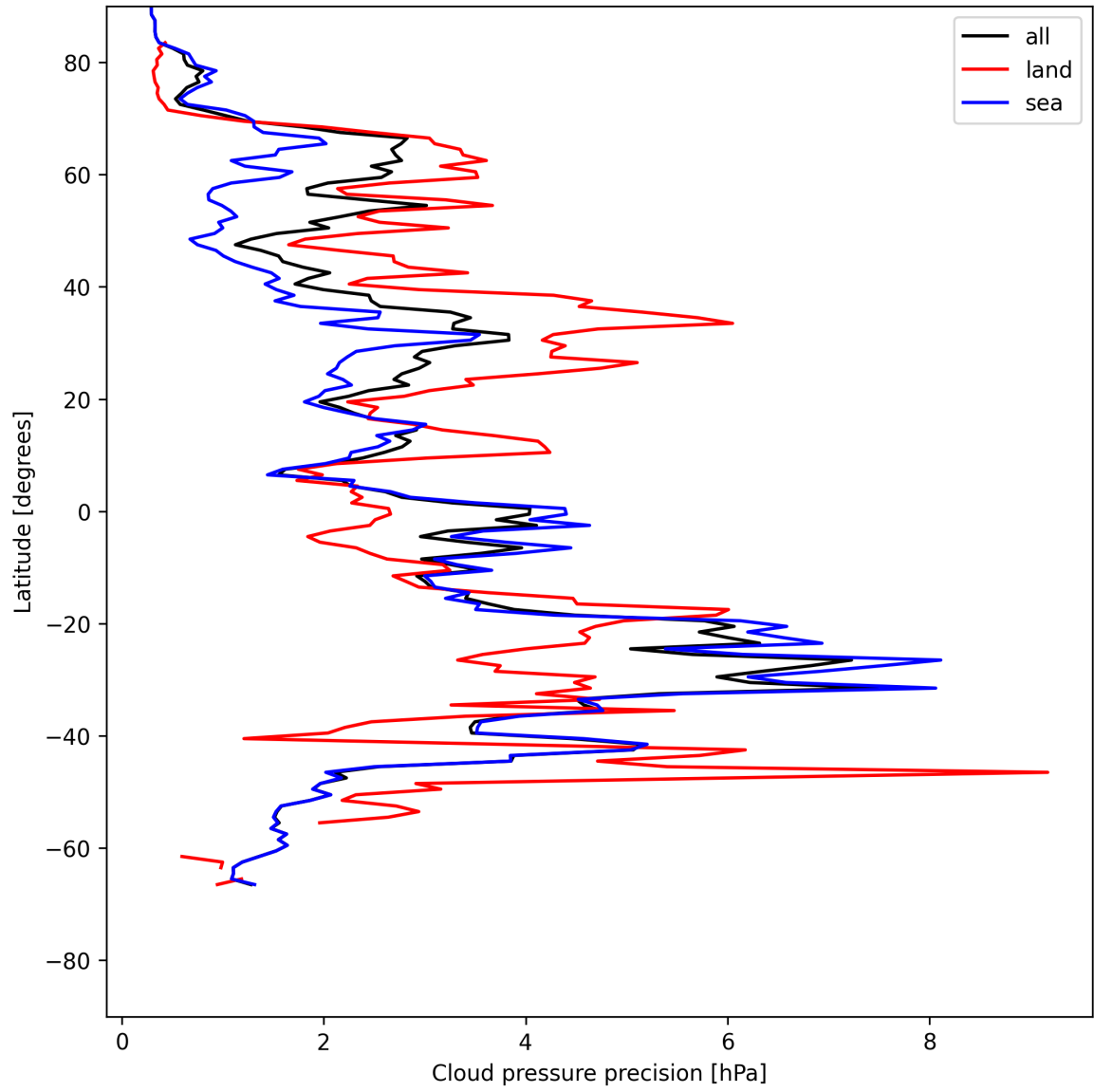
Figure 14: Zonal average of “Cloud pressure precision” for 2025-05-22 to 2025-05-24.
