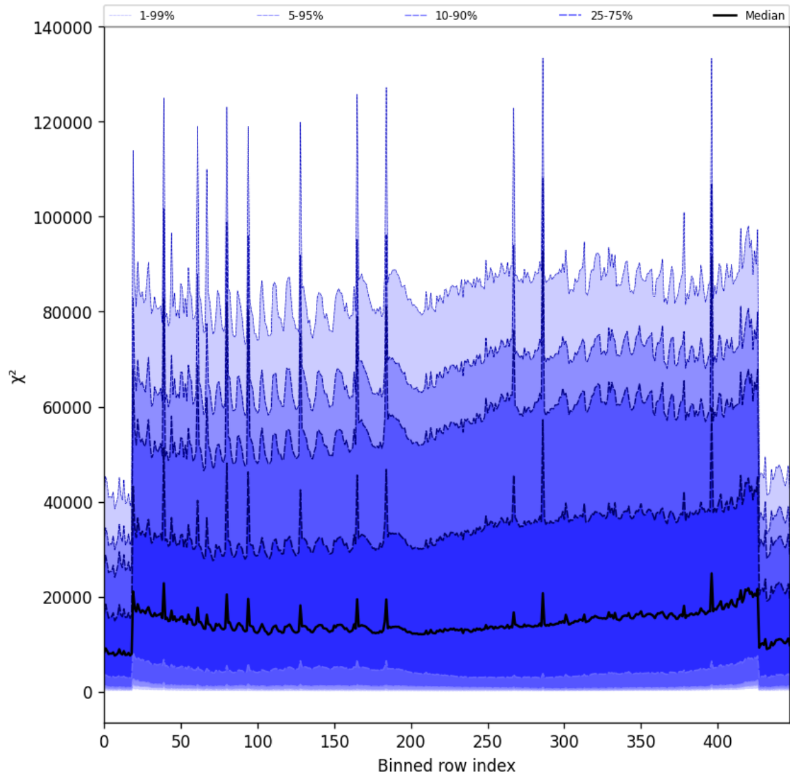
Figure 55: Along track statistics of “ \chi^2 ” for 2025-05-22 to 2025-05-24
