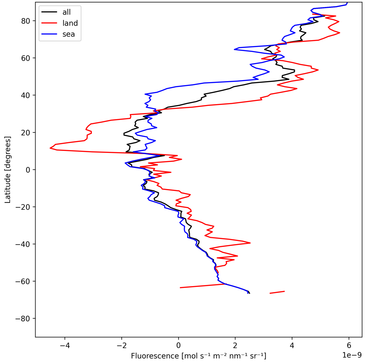
Figure 23: Zonal average of “Fluorescence” for 2025-05-22 to 2025-05-24.
