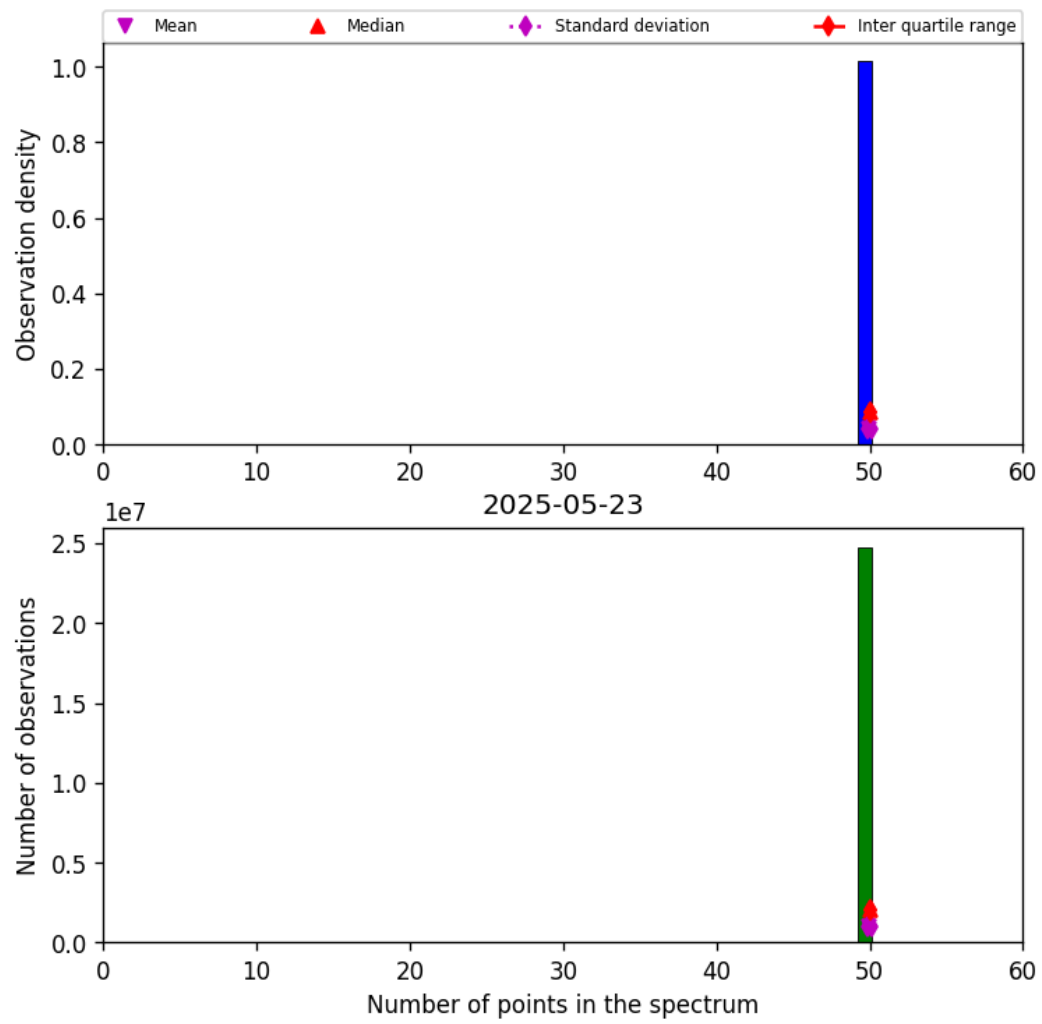
Figure 44: Histogram of “Number of points in the spectrum” for 2025-05-22 to 2025-05-24
