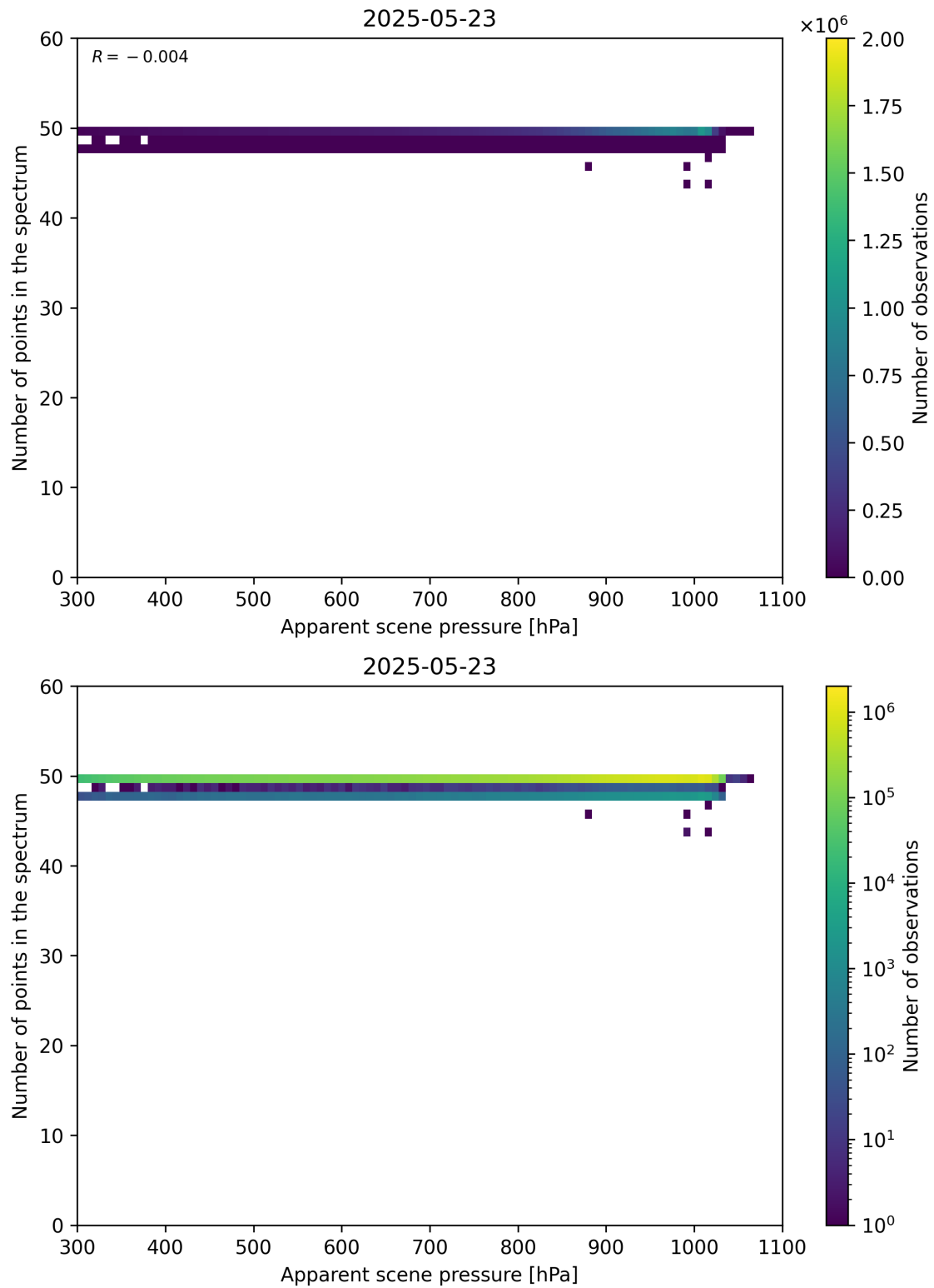
Figure 66: Scatter density plot of “Apparent scene pressure” against “Number of points in the spectrum” for 2025-05-22 to 2025-05-24.
