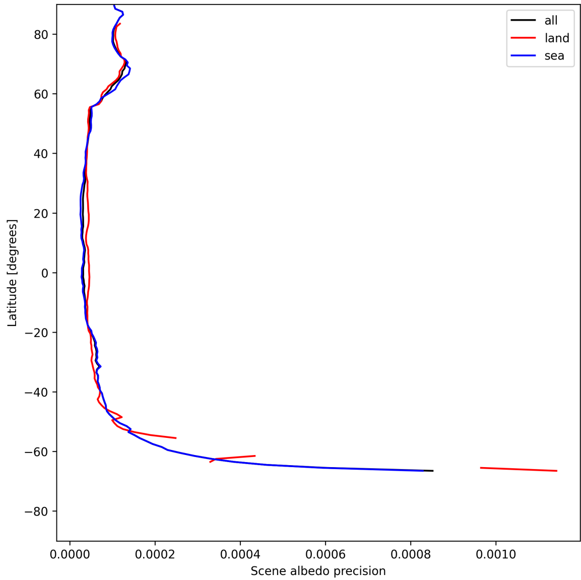
Figure 18: Zonal average of “Scene albedo precision” for 2025-05-22 to 2025-05-24.
