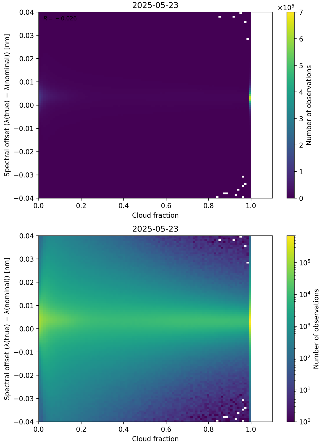
Figure 76: Scatter density plot of “Cloud fraction” against “Spectral offset ( \lambda_{\text{true}} - \lambda_{\text{nominal}} )” for 2025-05-22 to 2025-05-24.
