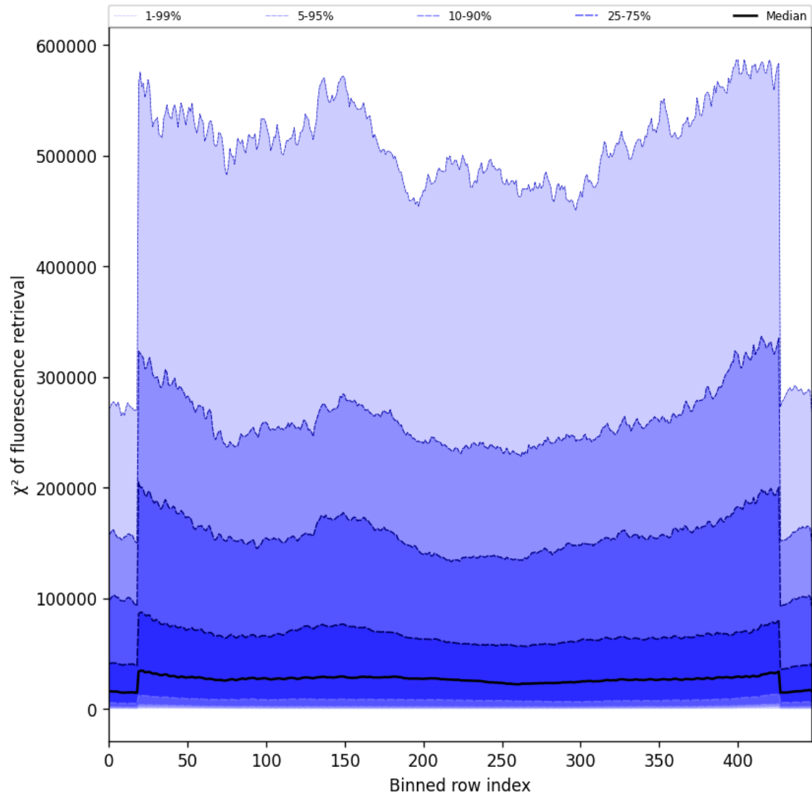
Figure 59: Along track statistics of “ \chi^2 of fluorescence retrieval” for 2025-05-22 to 2025-05-24
