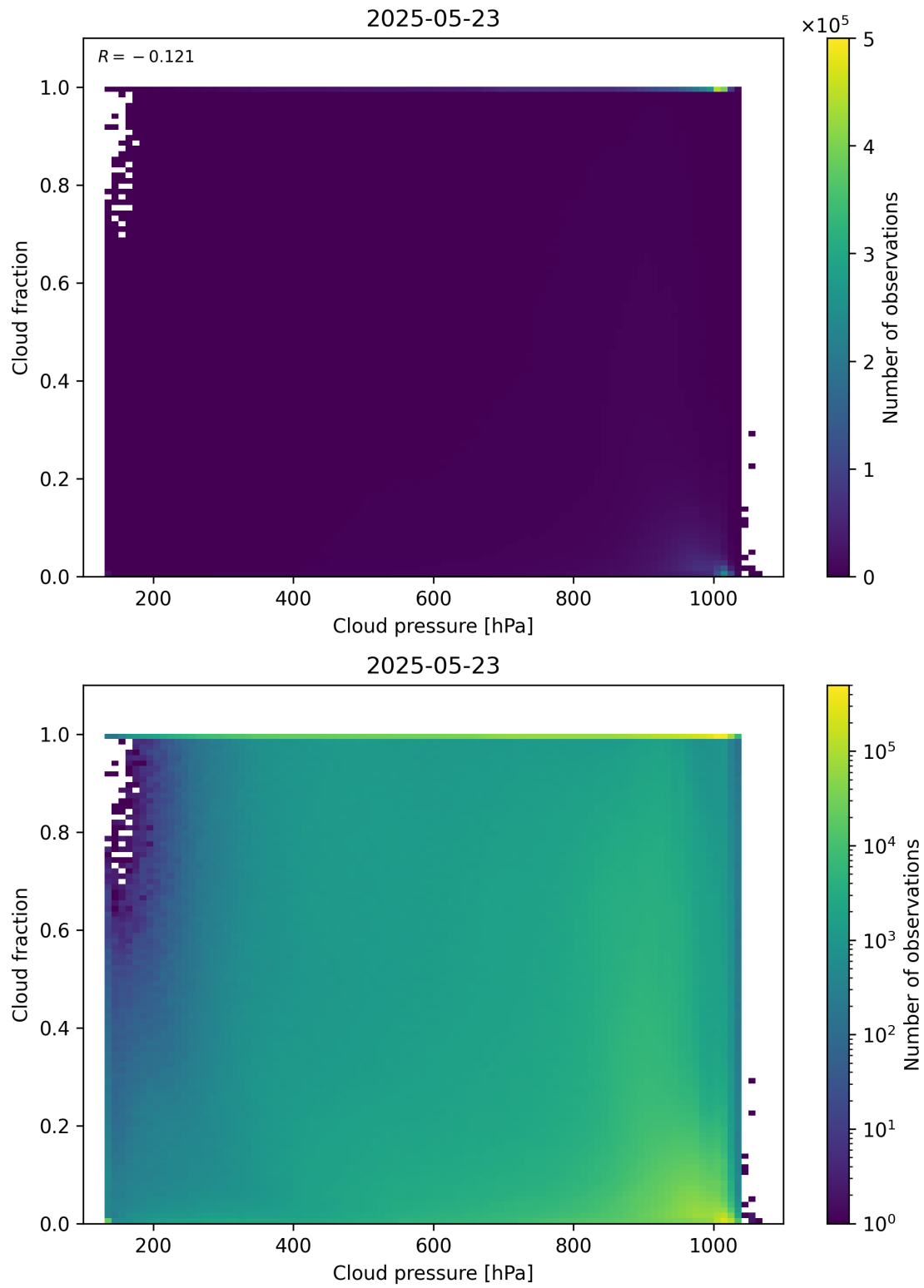
Figure 79: Scatter density plot of “Cloud pressure” against “Cloud fraction” for 2025-05-22 to 2025-05-24.
