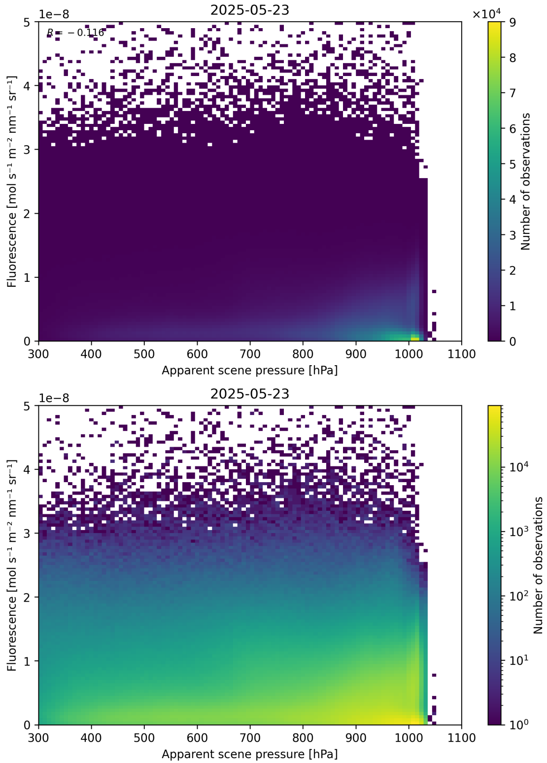
Figure 64: Scatter density plot of “Apparent scene pressure” against “Fluorescence” for 2025-05-22 to 2025-05-24.
