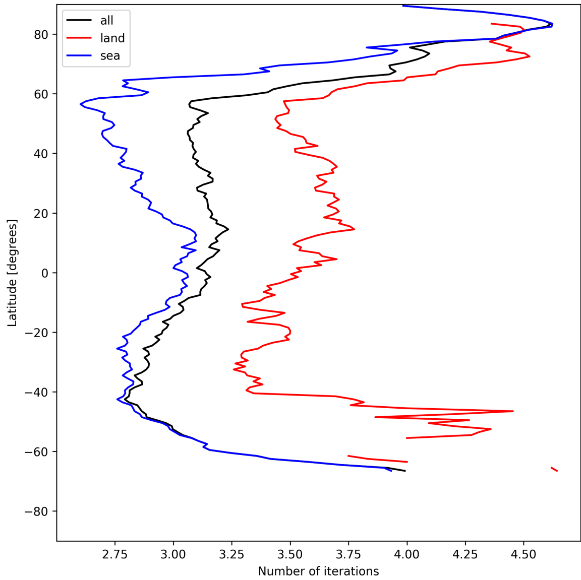
Figure 22: Zonal average of “Number of iterations” for 2025-05-22 to 2025-05-24.
