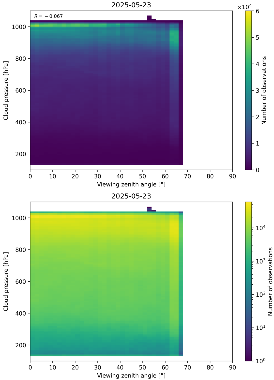
Figure 121: Scatter density plot of “Viewing zenith angle” against “Cloud pressure” for 2025-05-22 to 2025-05-24.
