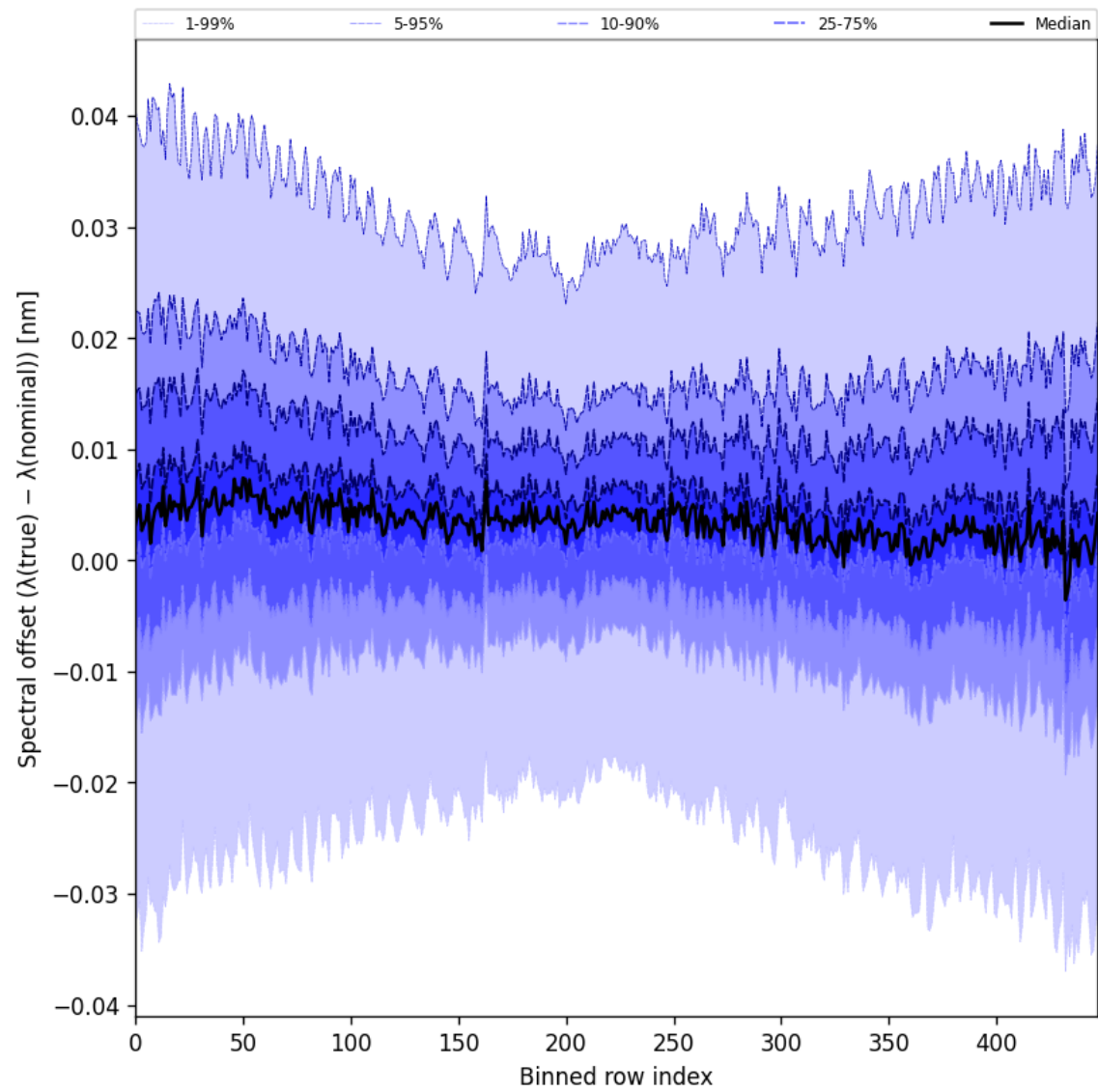
Figure 62: Along track statistics of “Spectral offset ( \lambda_{\text{true}} - \lambda_{\text{nominal}} )” for 2025-05-22 to 2025-05-24
