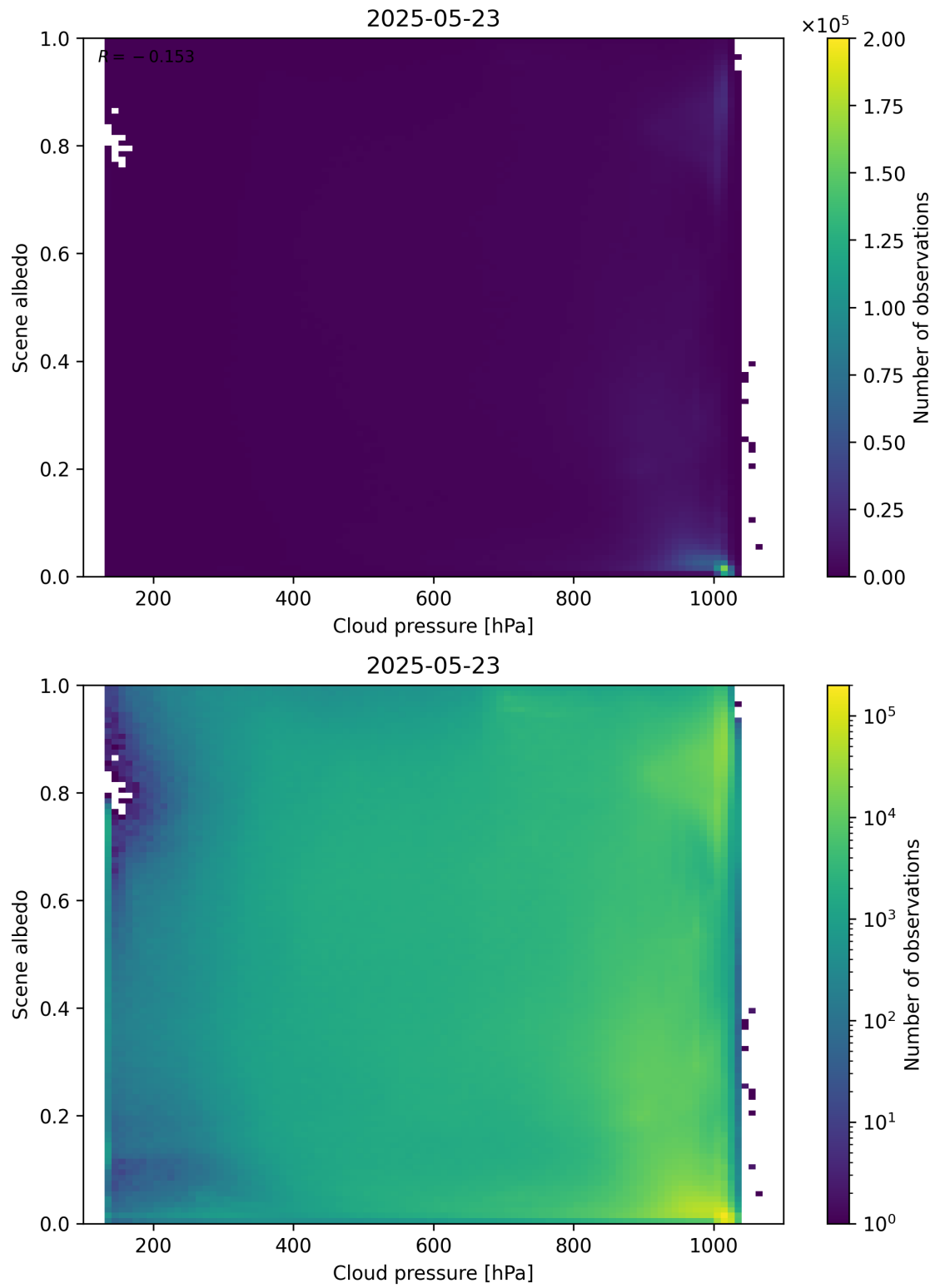
Figure 83: Scatter density plot of “Cloud pressure” against “Scene albedo” for 2025-05-22 to 2025-05-24.
