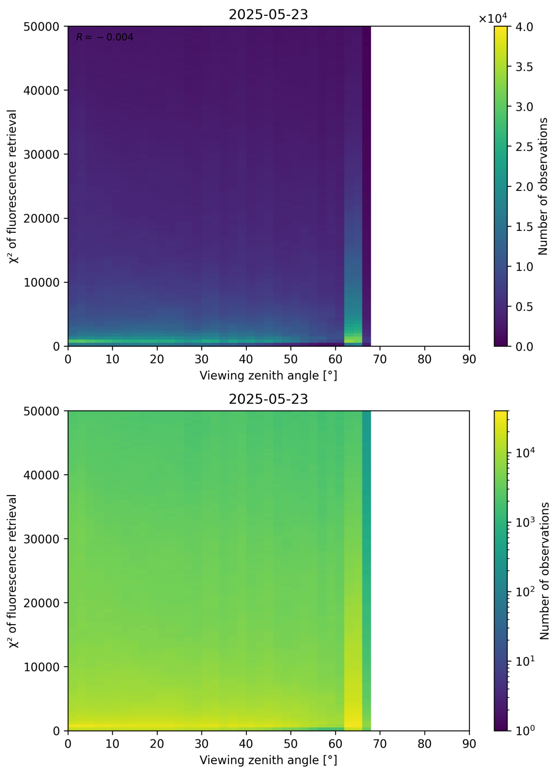
Figure 119: Scatter density plot of “Viewing zenith angle” against “ \chi^2 of fluorescence retrieval” for 2025-05-22 to 2025-05-24.
