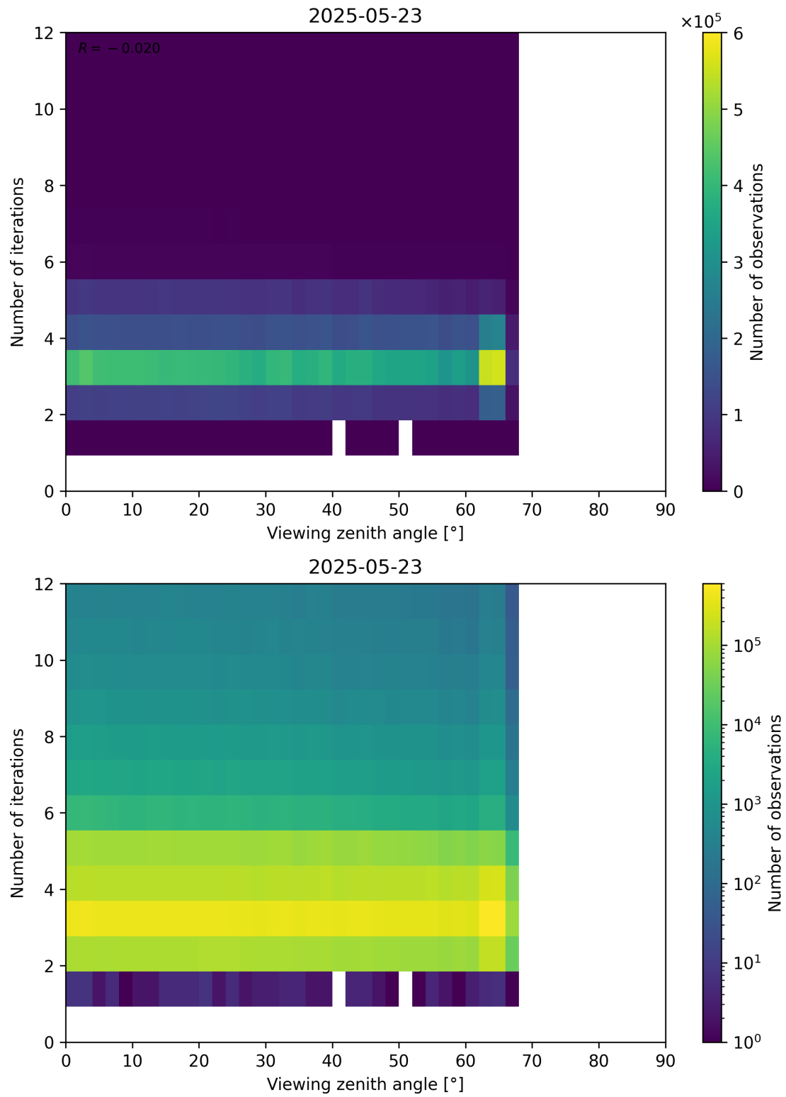
Figure 124: Scatter density plot of “Viewing zenith angle” against “Number of iterations” for 2025-05-22 to 2025-05-24.
