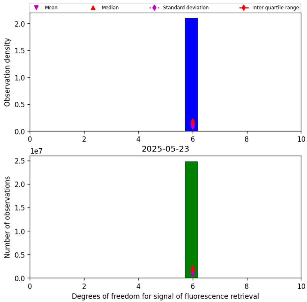
Figure 43: Histogram of “Degrees of freedom for signal of fluorescence retrieval” for 2025-05-22 to 2025-05-24
