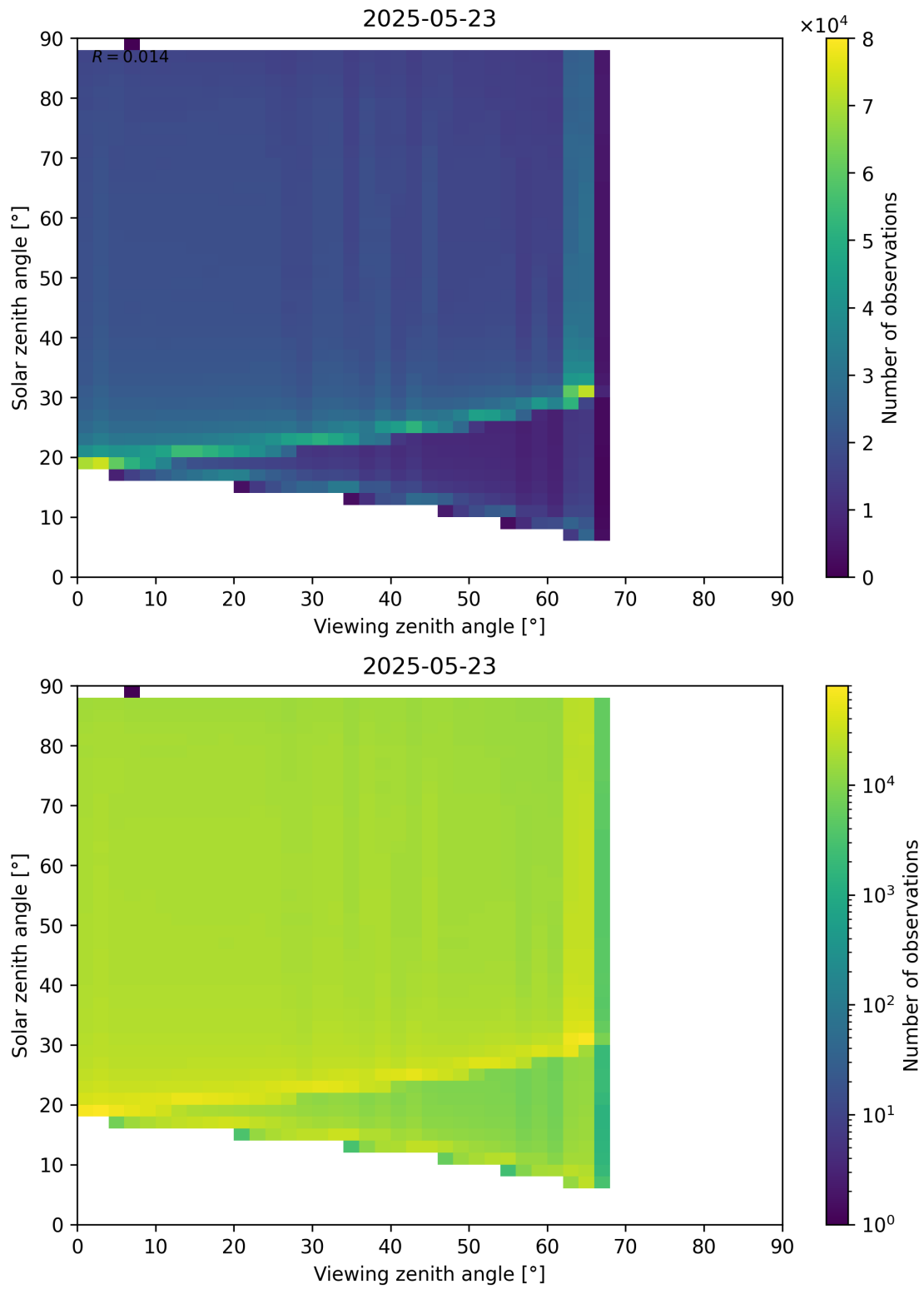
Figure 127: Scatter density plot of “Viewing zenith angle” against “Solar zenith angle” for 2025-05-22 to 2025-05-24.
