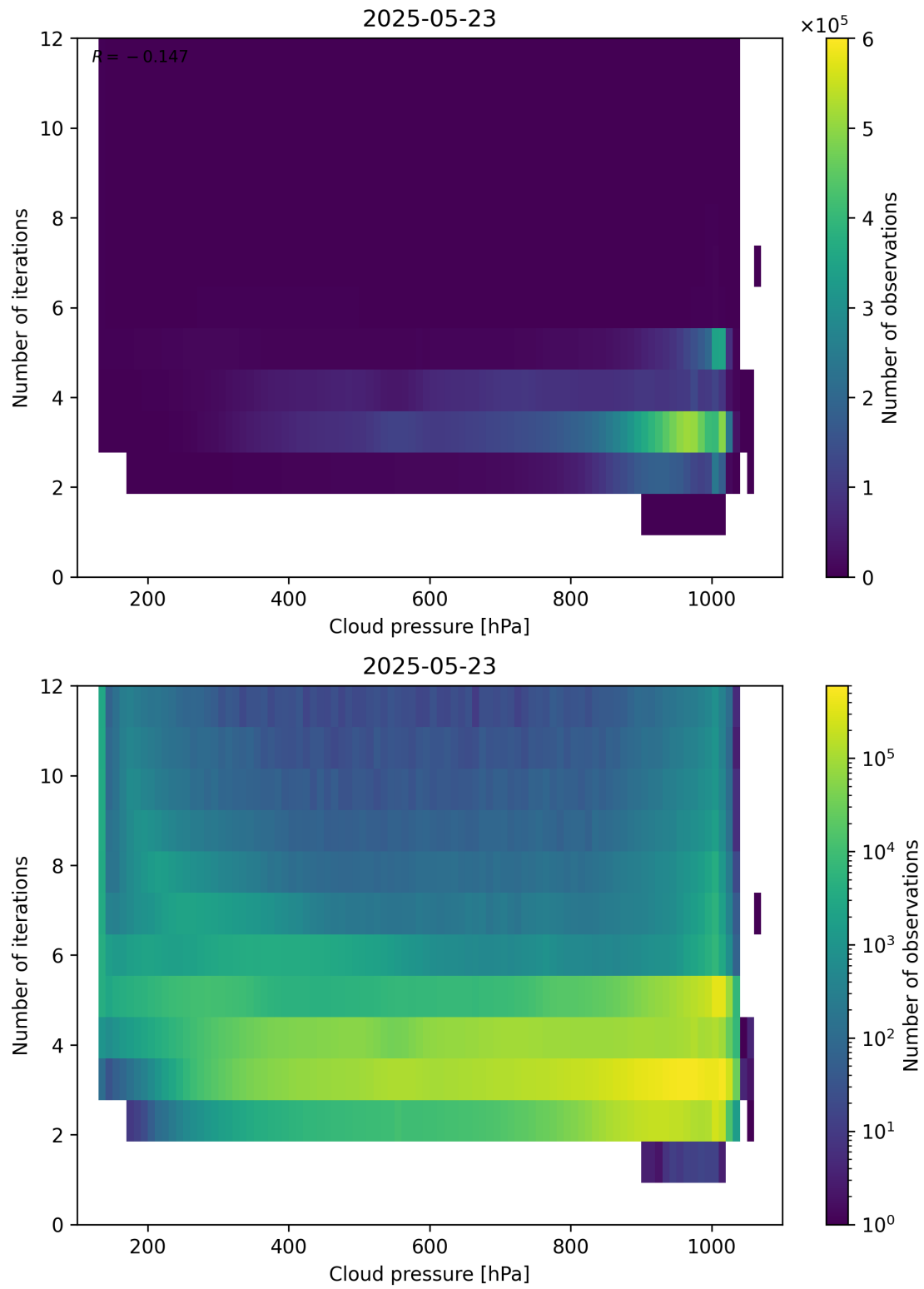
Figure 81: Scatter density plot of “Cloud pressure” against “Number of iterations” for 2025-05-22 to 2025-05-24.
