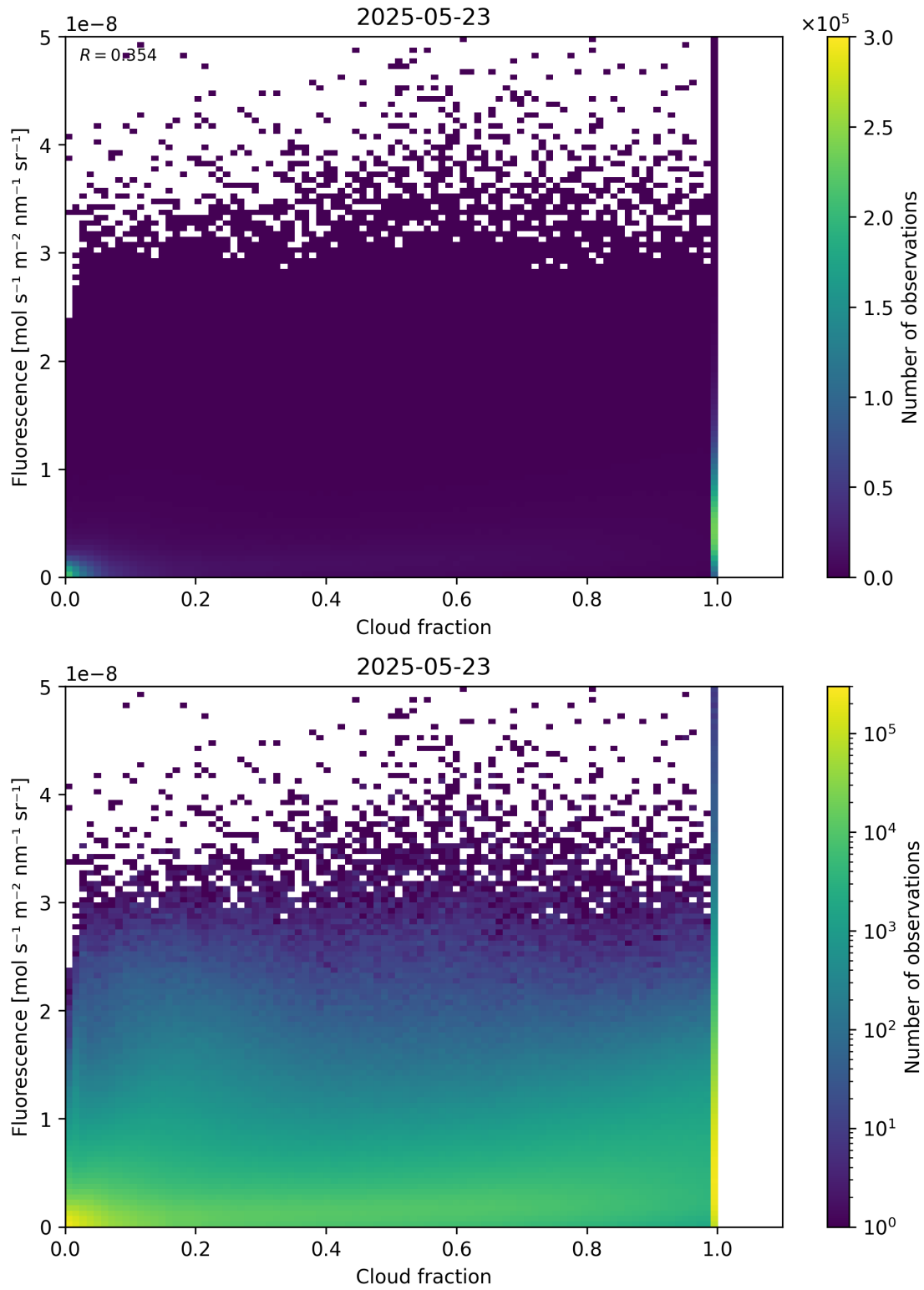
Figure 72: Scatter density plot of “Cloud fraction” against “Fluorescence” for 2025-05-22 to 2025-05-24.
