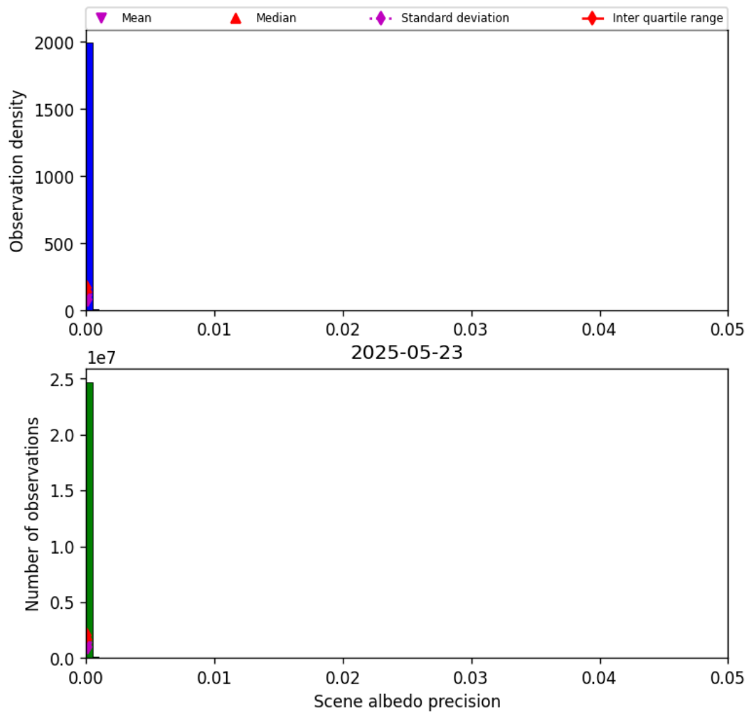
Figure 35: Histogram of “Scene albedo precision” for 2025-05-22 to 2025-05-24
