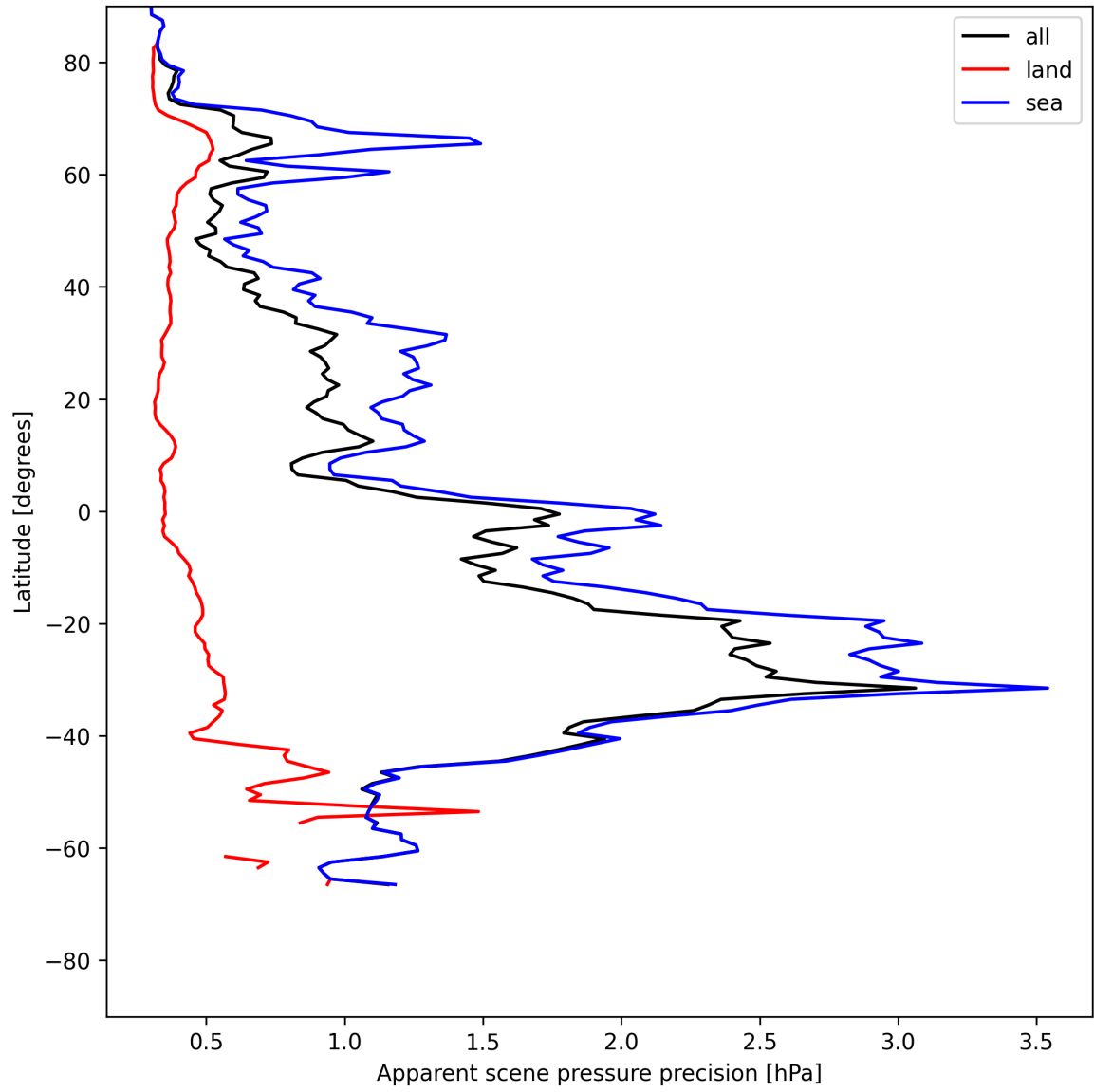
Figure 20: Zonal average of “Apparent scene pressure precision” for 2025-05-22 to 2025-05-24.
