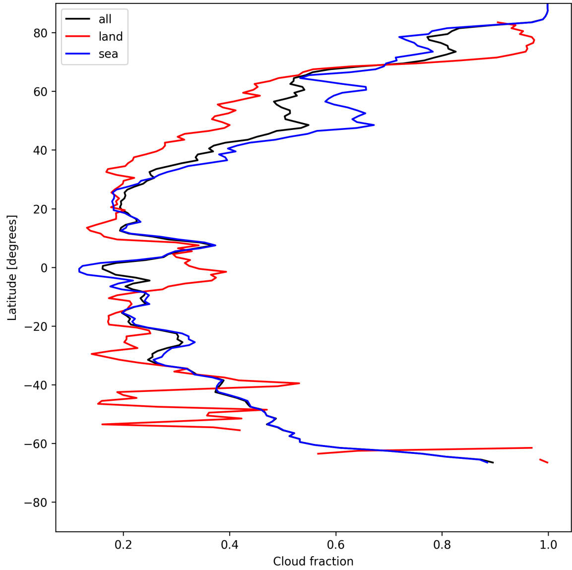
Figure 15: Zonal average of “Cloud fraction” for 2025-05-22 to 2025-05-24.
