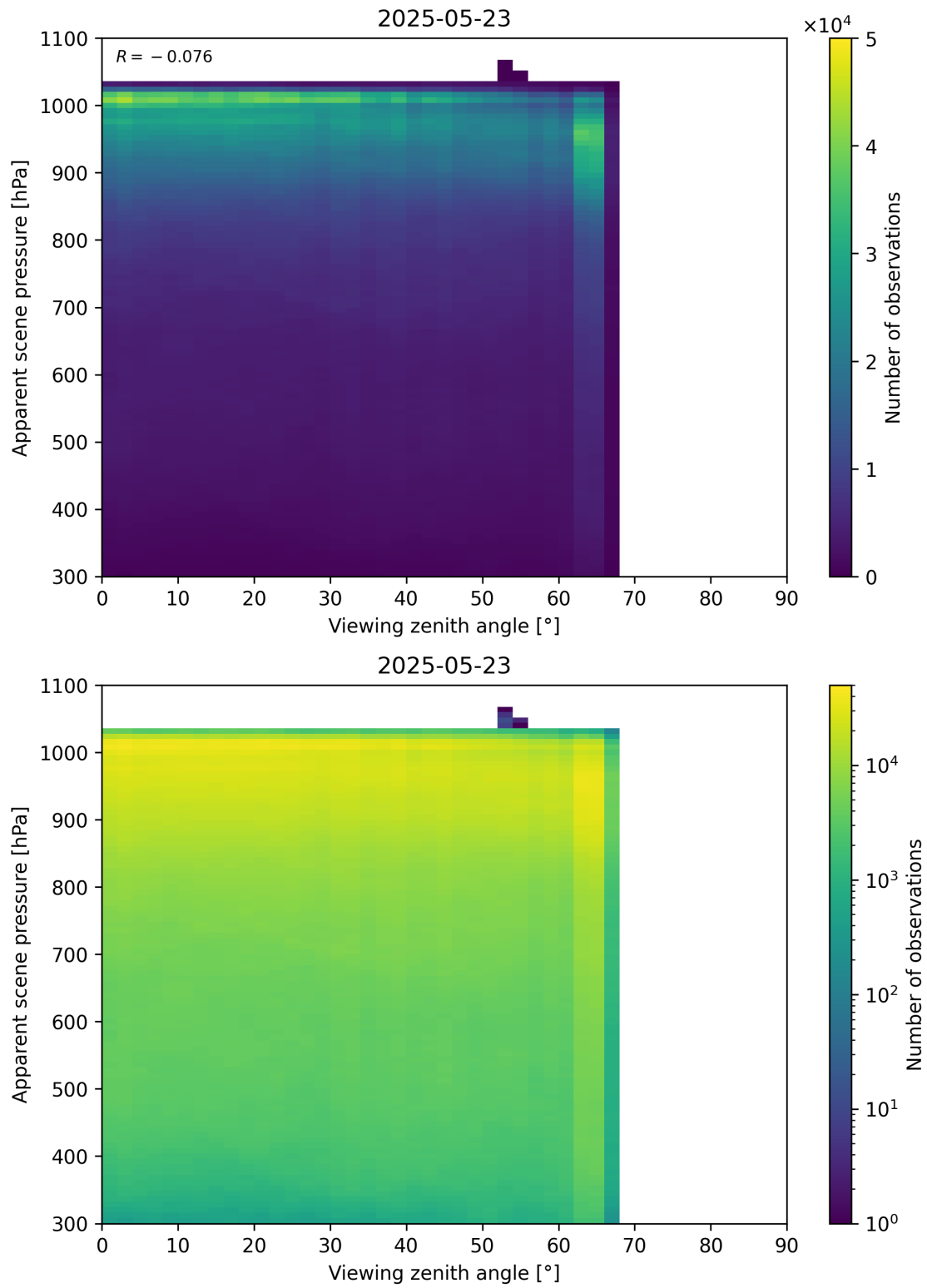
Figure 118: Scatter density plot of “Viewing zenith angle” against “Apparent scene pressure” for 2025-05-22 to 2025-05-24.
