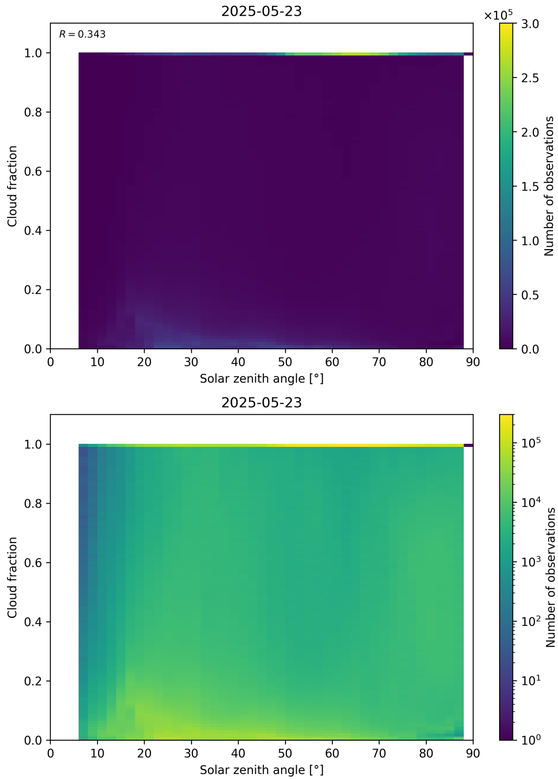
Figure 110: Scatter density plot of “Solar zenith angle” against “Cloud fraction” for 2025-05-22 to 2025-05-24.
