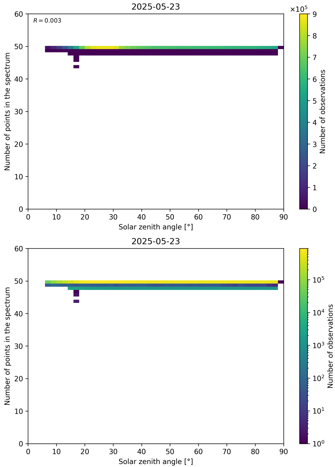
Figure 115: Scatter density plot of “Solar zenith angle” against “Number of points in the spectrum” for 2025-05-22 to 2025-05-24.
