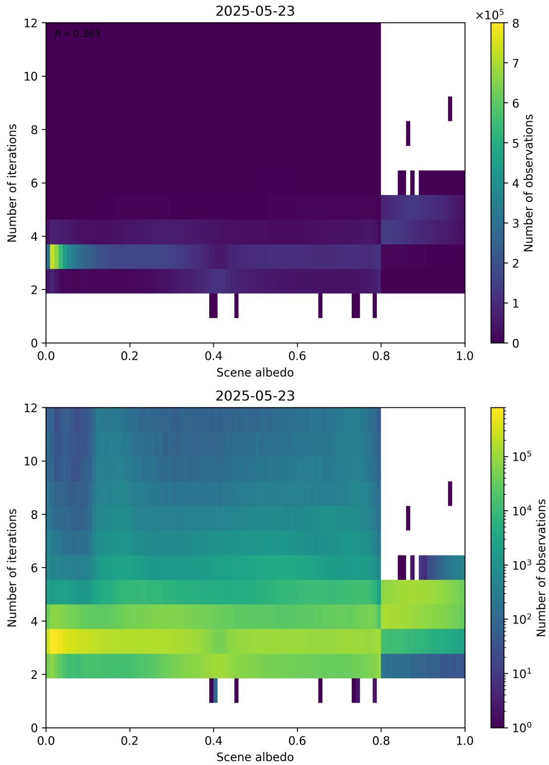
Figure 105: Scatter density plot of “Scene albedo” against “Number of iterations” for 2025-05-22 to 2025-05-24.
