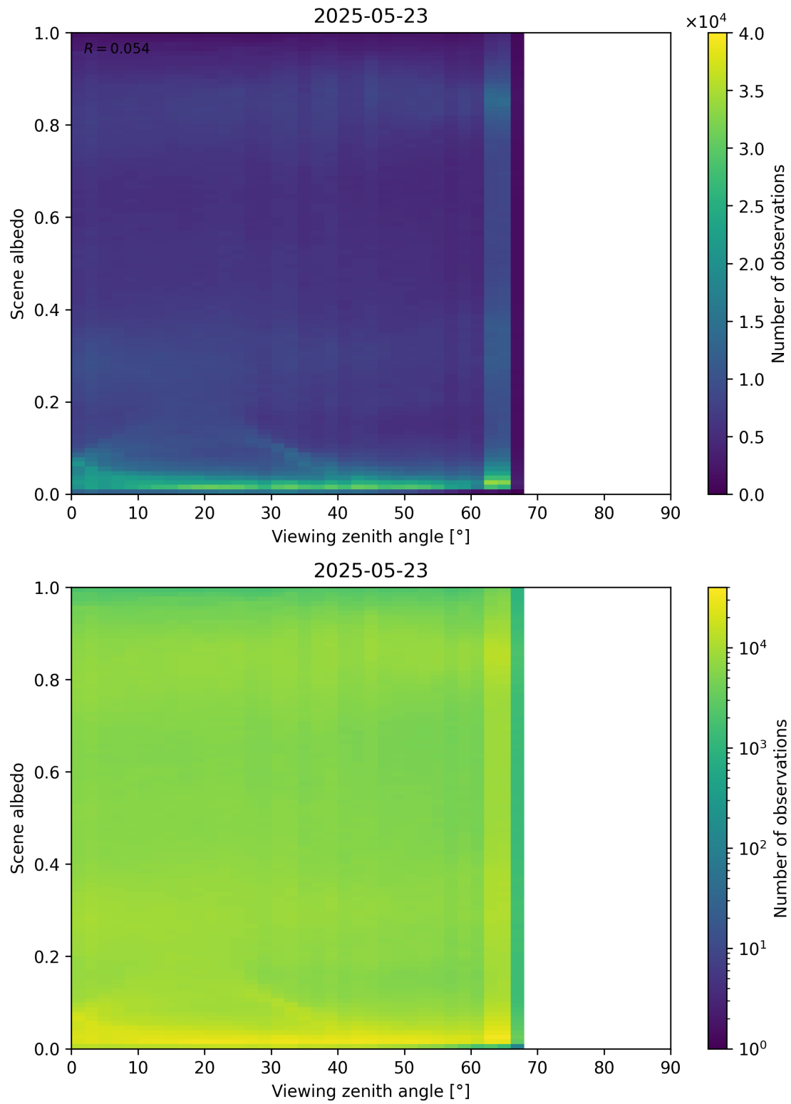
Figure 126: Scatter density plot of “Viewing zenith angle” against “Scene albedo” for 2025-05-22 to 2025-05-24.
