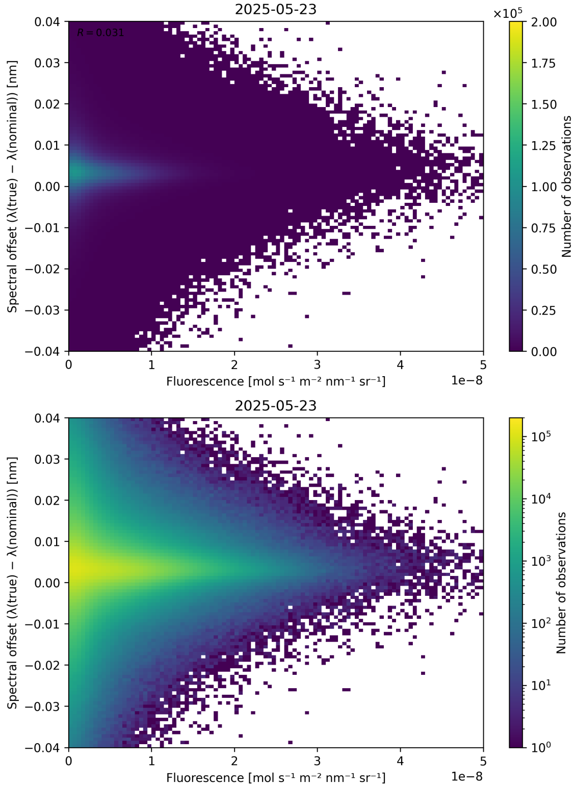
Figure 87: Scatter density plot of “Fluorescence” against “Spectral offset ( \lambda_{\text{true}} - \lambda_{\text{nominal}} )” for 2025-05-22 to 2025-05-24.
