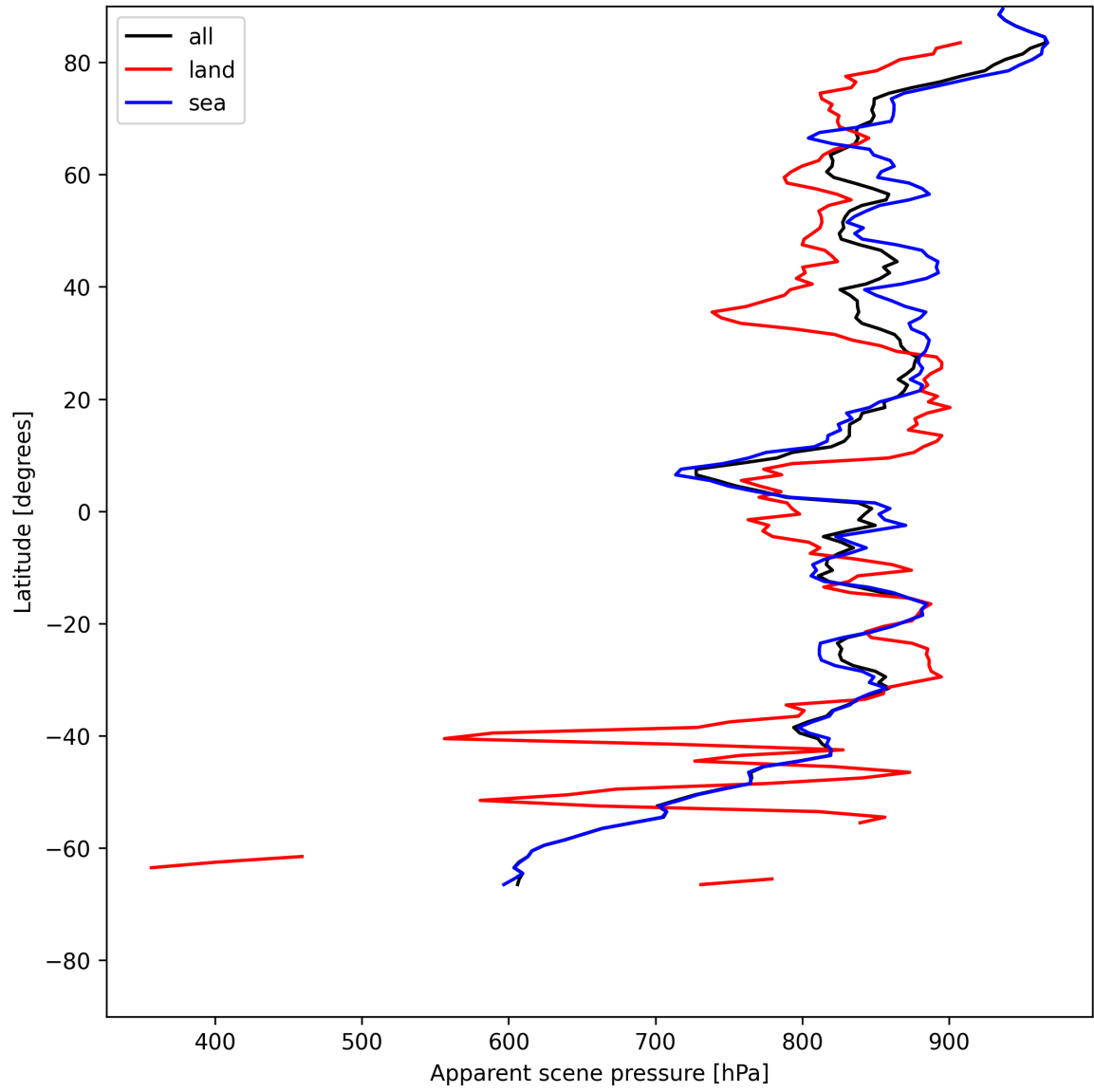
Figure 19: Zonal average of “Apparent scene pressure” for 2025-05-22 to 2025-05-24.
