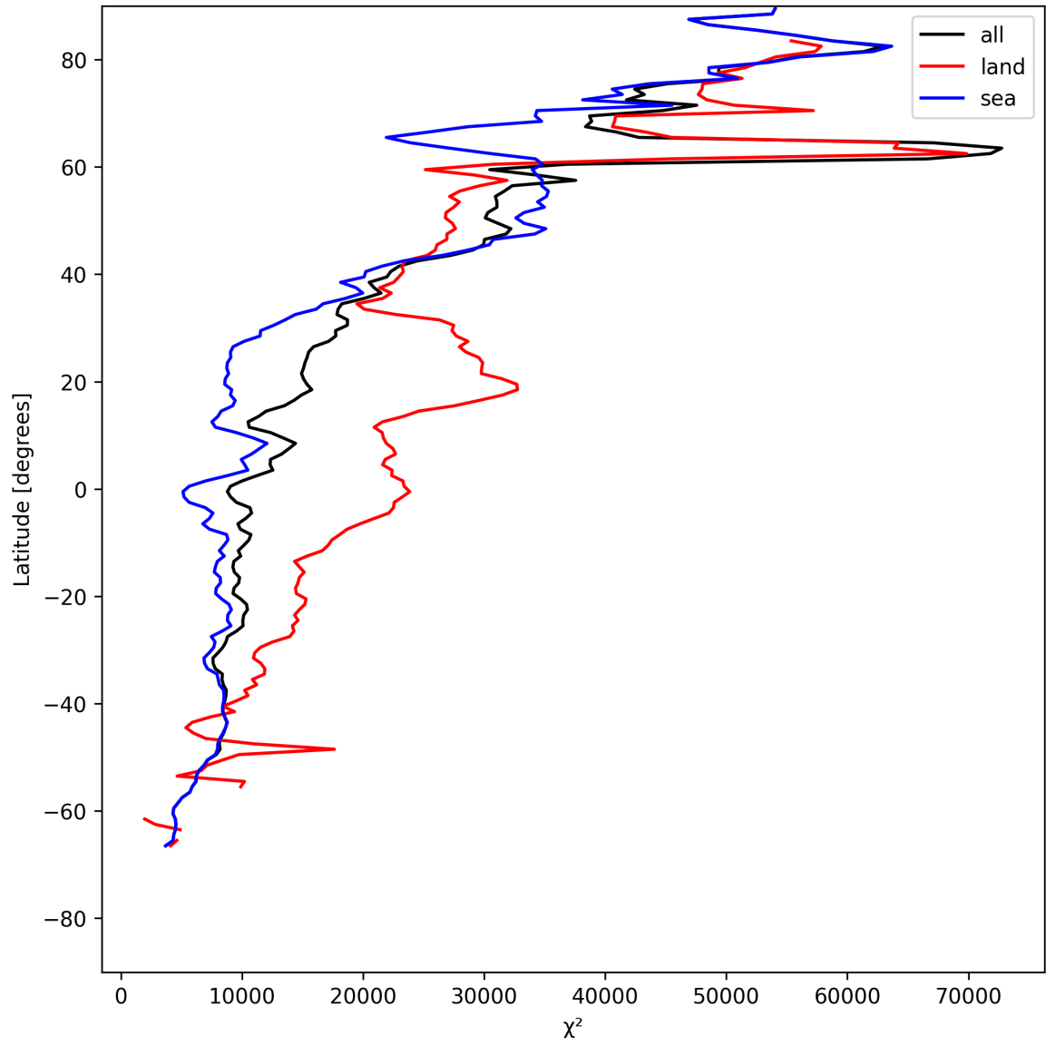
Figure 21: Zonal average of “ \chi^2 ” for 2025-05-22 to 2025-05-24.
