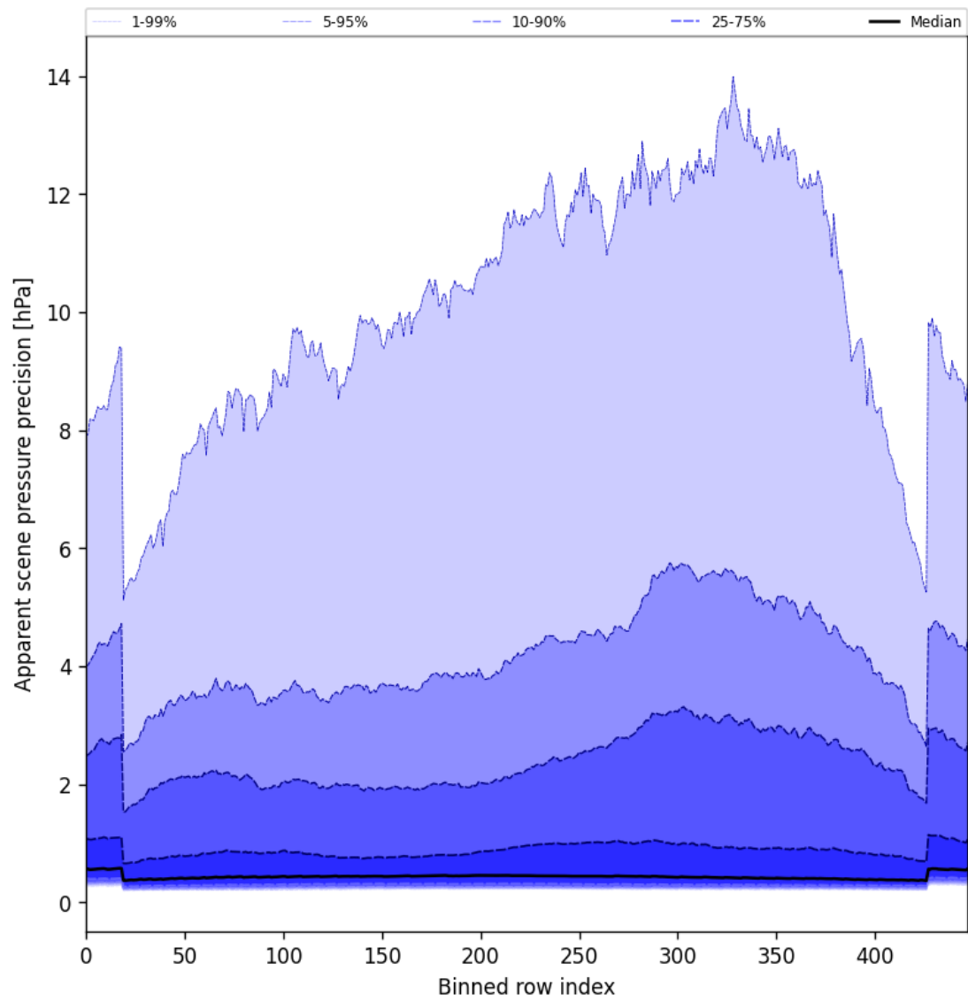
Figure 54: Along track statistics of “Apparent scene pressure precision” for 2025-05-22 to 2025-05-24
