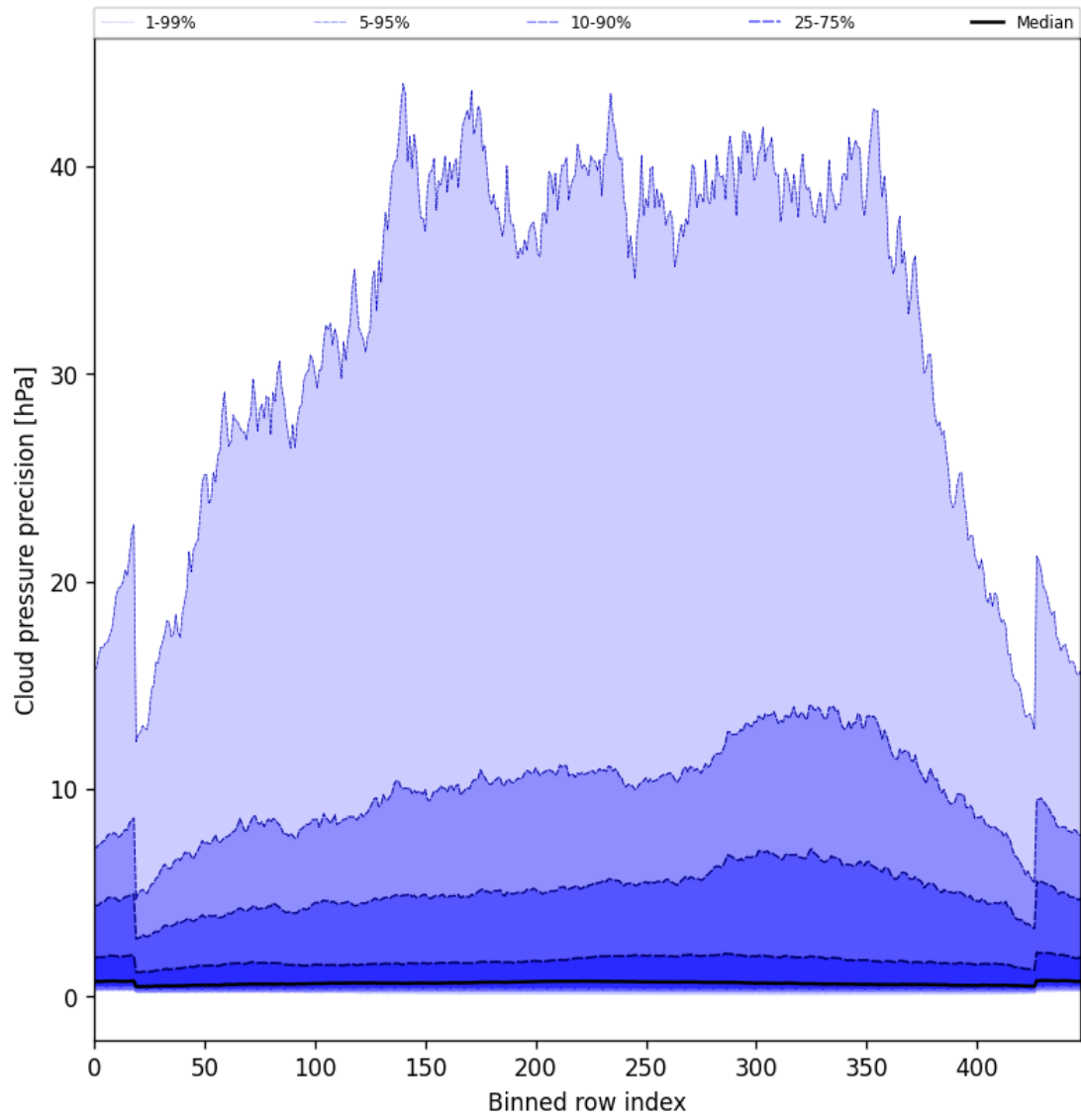
Figure 48: Along track statistics of “Cloud pressure precision” for 2025-05-22 to 2025-05-24
