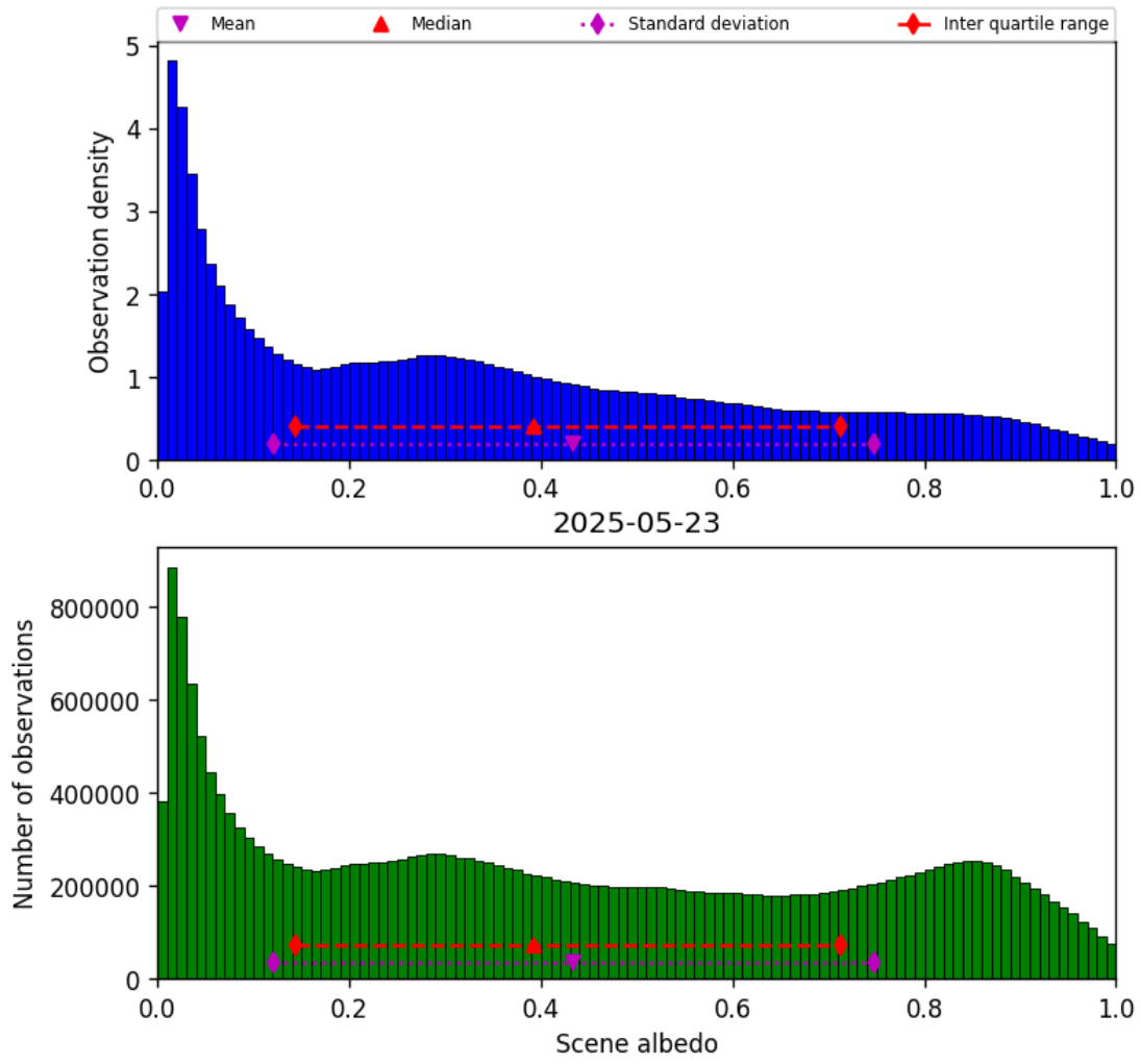
Figure 34: Histogram of “Scene albedo” for 2025-05-22 to 2025-05-24
