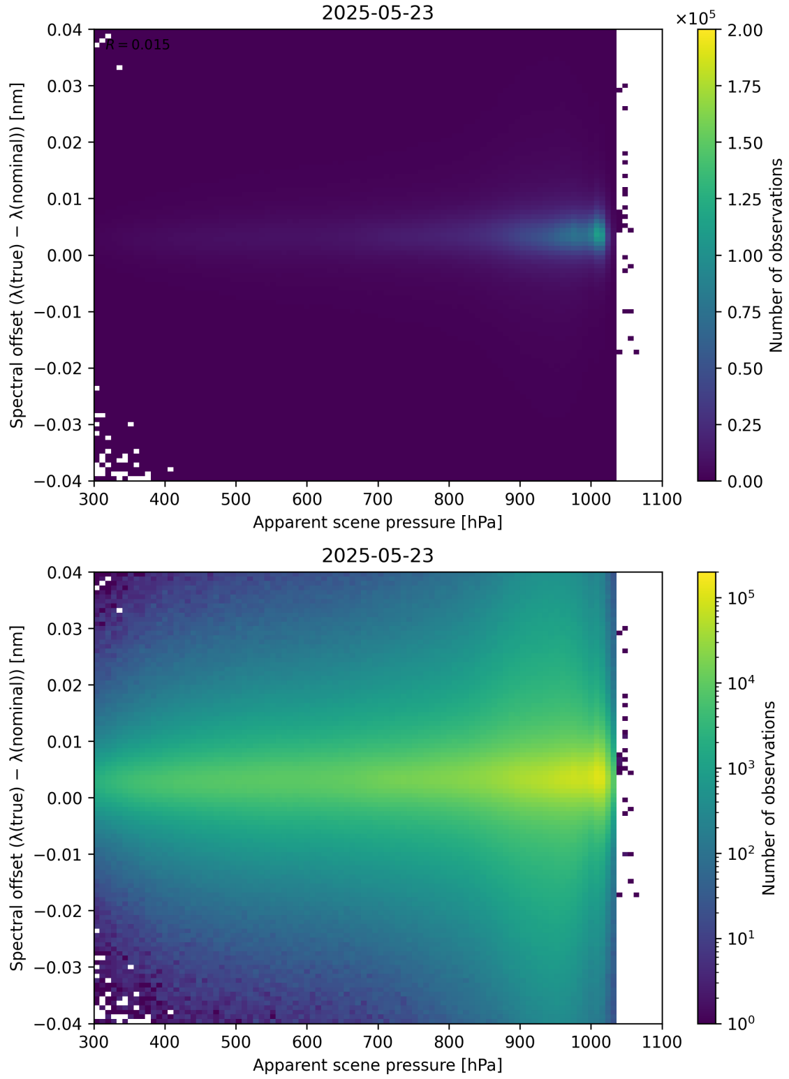
Figure 67: Scatter density plot of “Apparent scene pressure” against “Spectral offset ( \lambda_{\text{true}} - \lambda_{\text{nominal}} )” for 2025-05-22 to 2025-05-24.
