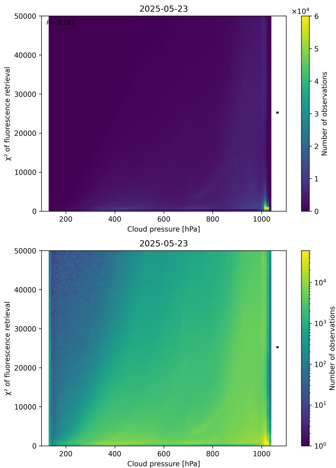
Figure 78: Scatter density plot of “Cloud pressure” against “ \chi^2 of fluorescence retrieval” for 2025-05-22 to 2025-05-24.
