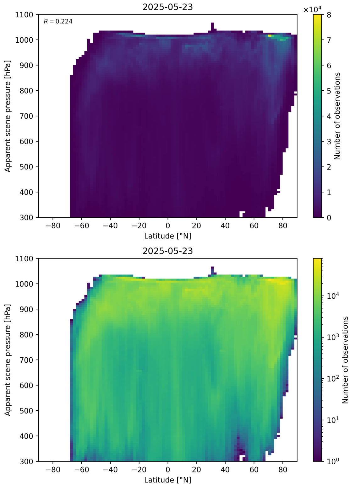
Figure 88: Scatter density plot of “Latitude” against “Apparent scene pressure” for 2025-05-22 to 2025-05-24.
