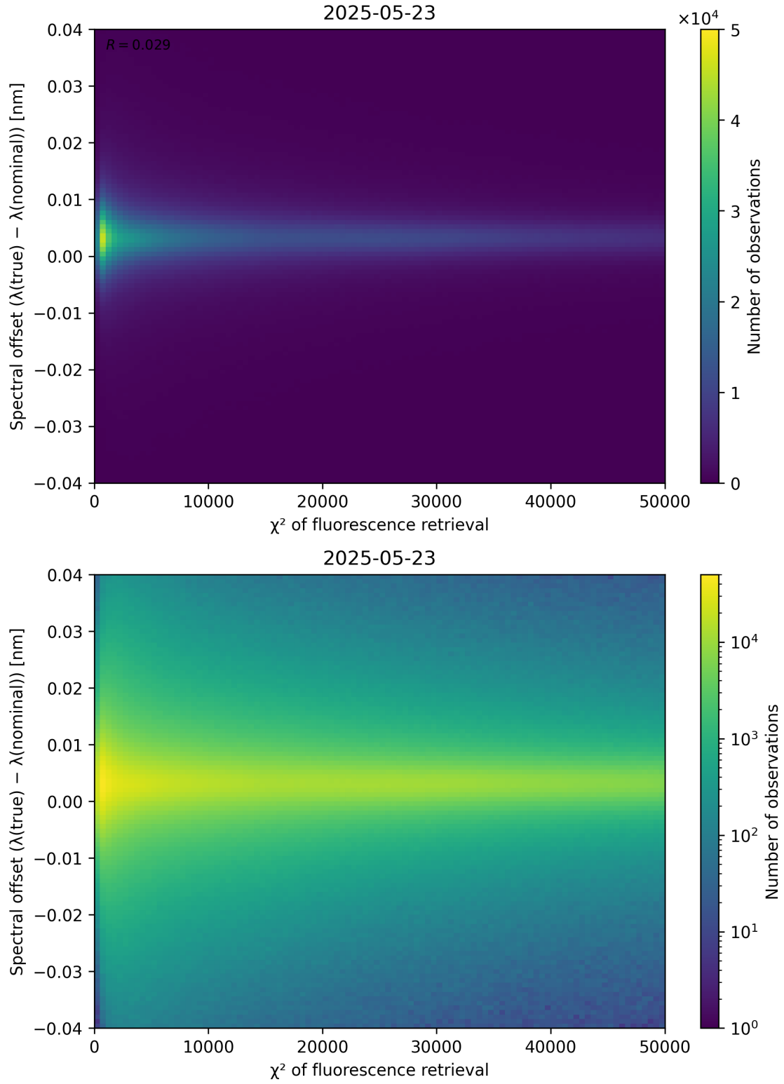
Figure 69: Scatter density plot of “ \chi^2 of fluorescence retrieval” against “Spectral offset ( \lambda_{\text{true}} - \lambda_{\text{nominal}} )” for 2025-05-22 to 2025-05-24.
