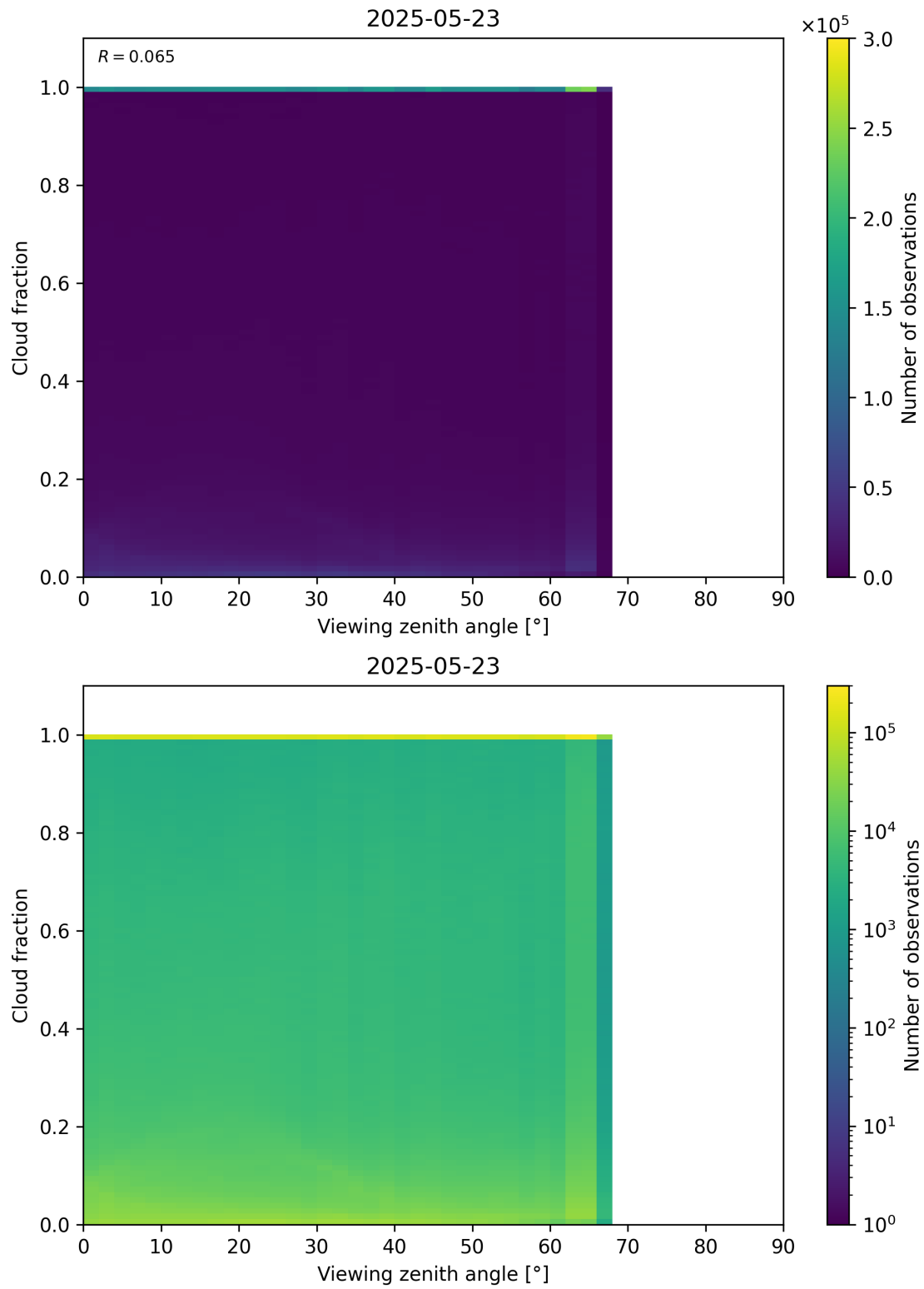
Figure 120: Scatter density plot of “Viewing zenith angle” against “Cloud fraction” for 2025-05-22 to 2025-05-24.
