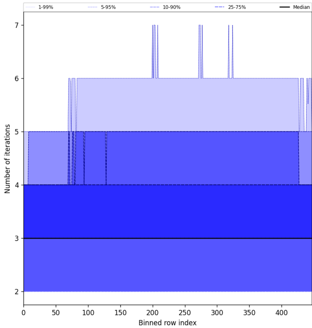
Figure 56: Along track statistics of “Number of iterations” for 2025-05-22 to 2025-05-24
