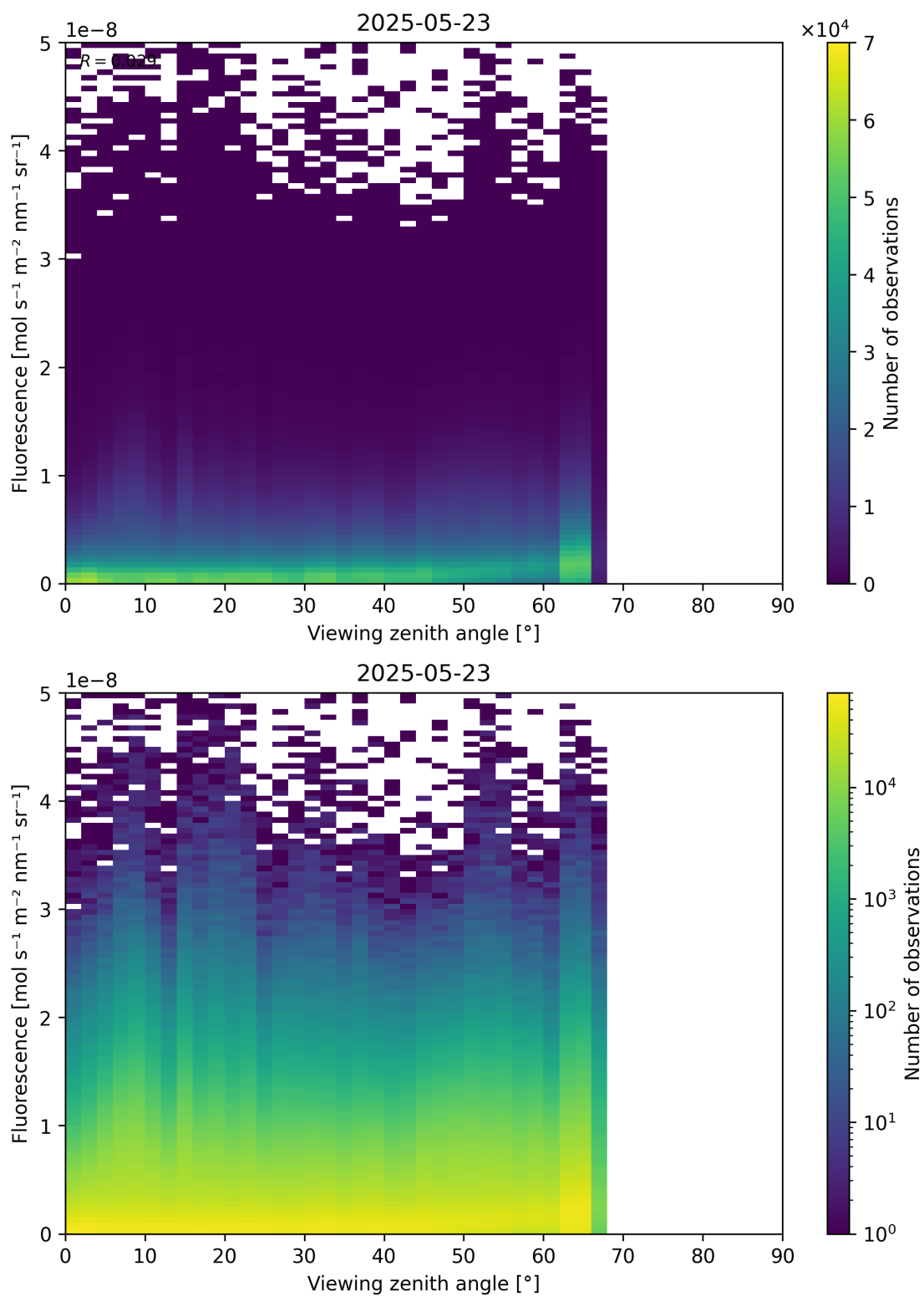
Figure 122: Scatter density plot of "Viewing zenith angle" against "Fluorescence" for 2025-05-22 to 2025-05-24.
