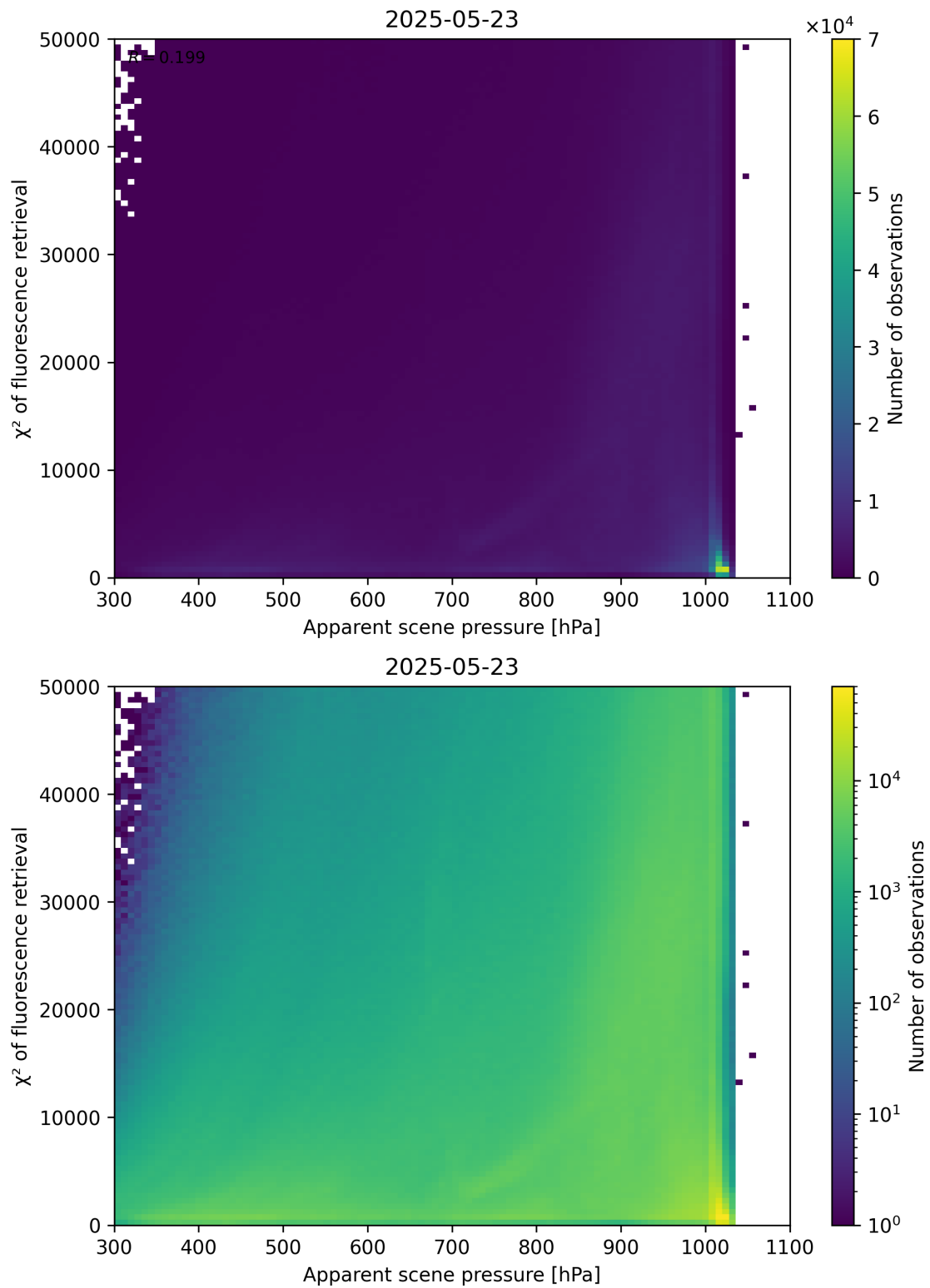
Figure 63: Scatter density plot of “Apparent scene pressure” against “ \chi^2 of fluorescence retrieval” for 2025-05-22 to 2025-05-24.
