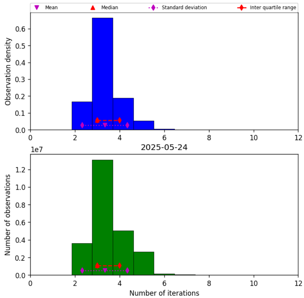
Figure 39: Histogram of “Number of iterations” for 2025-05-23 to 2025-05-25
