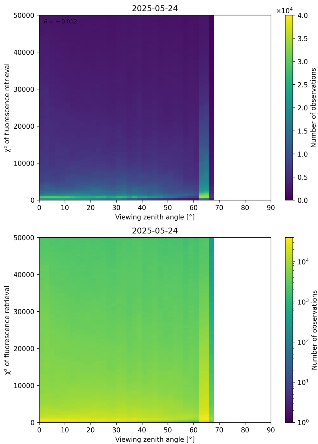
Figure 119: Scatter density plot of “Viewing zenith angle” against “ \chi^2 of fluorescence retrieval” for 2025-05-23 to 2025-05-25.
