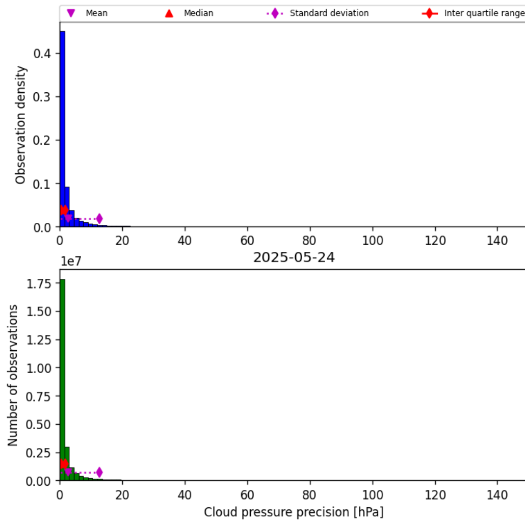
Figure 31: Histogram of “Cloud pressure precision” for 2025-05-23 to 2025-05-25
