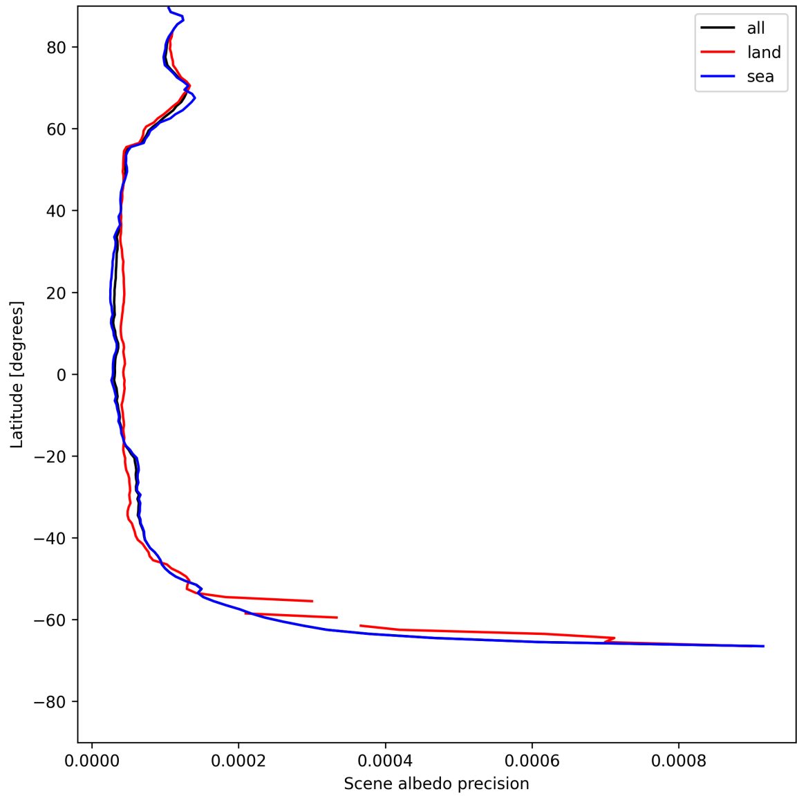
Figure 18: Zonal average of “Scene albedo precision” for 2025-05-23 to 2025-05-25.
