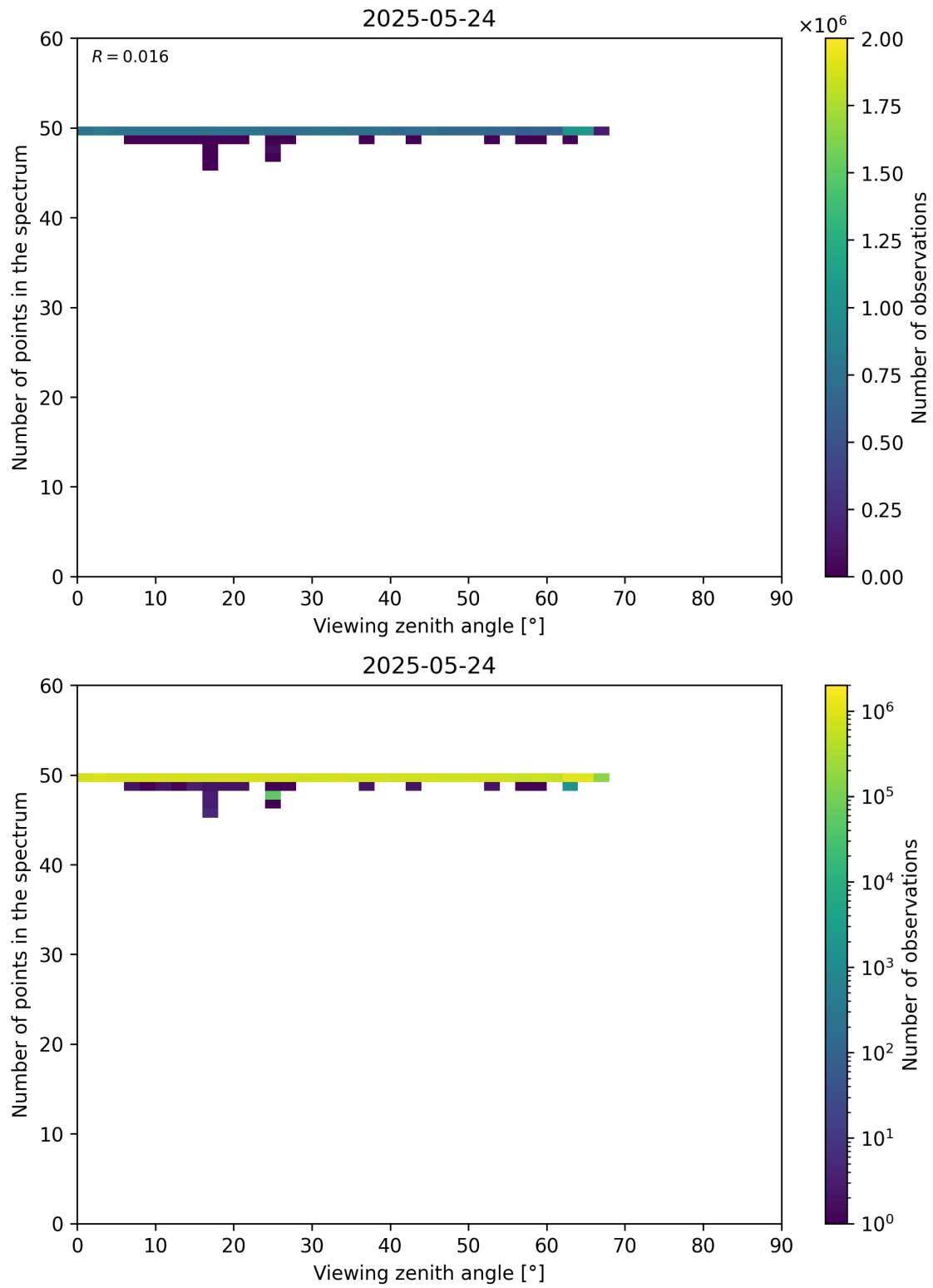
Figure 125: Scatter density plot of “Viewing zenith angle” against “Number of points in the spectrum” for 2025-05-23 to 2025-05-25.
