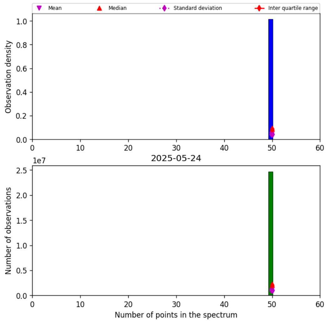
Figure 44: Histogram of “Number of points in the spectrum” for 2025-05-23 to 2025-05-25
