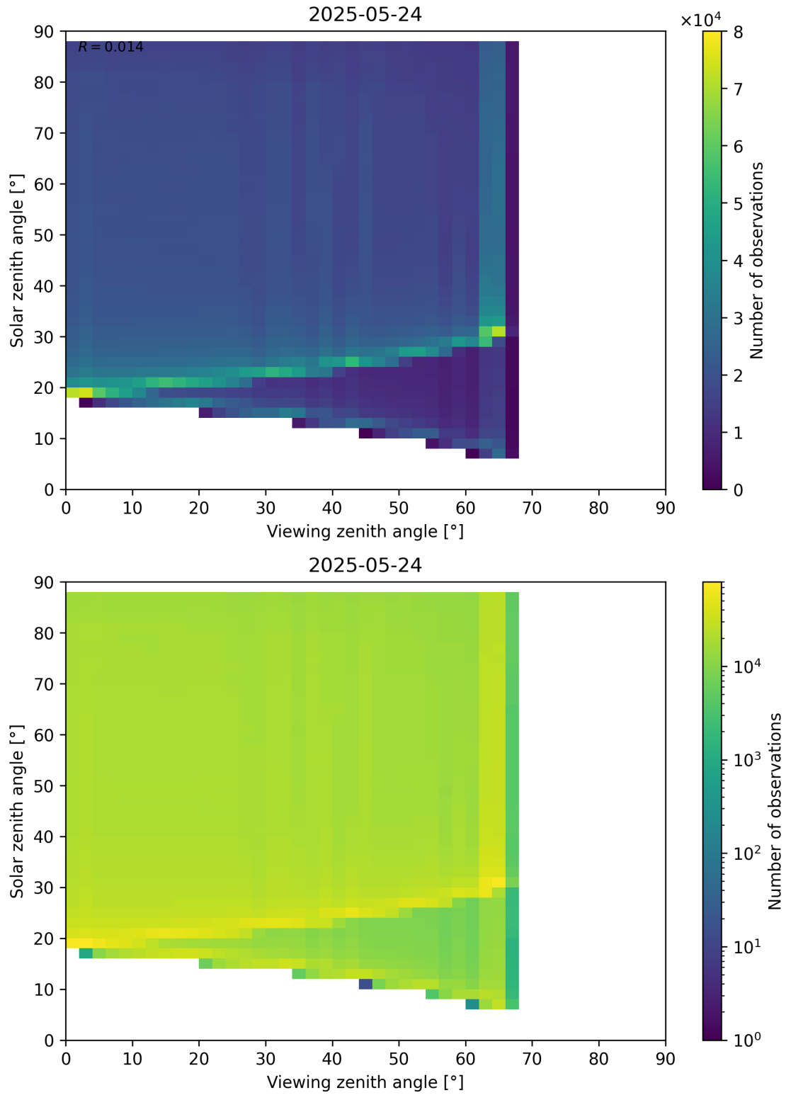
Figure 127: Scatter density plot of “Viewing zenith angle” against “Solar zenith angle” for 2025-05-23 to 2025-05-25.
