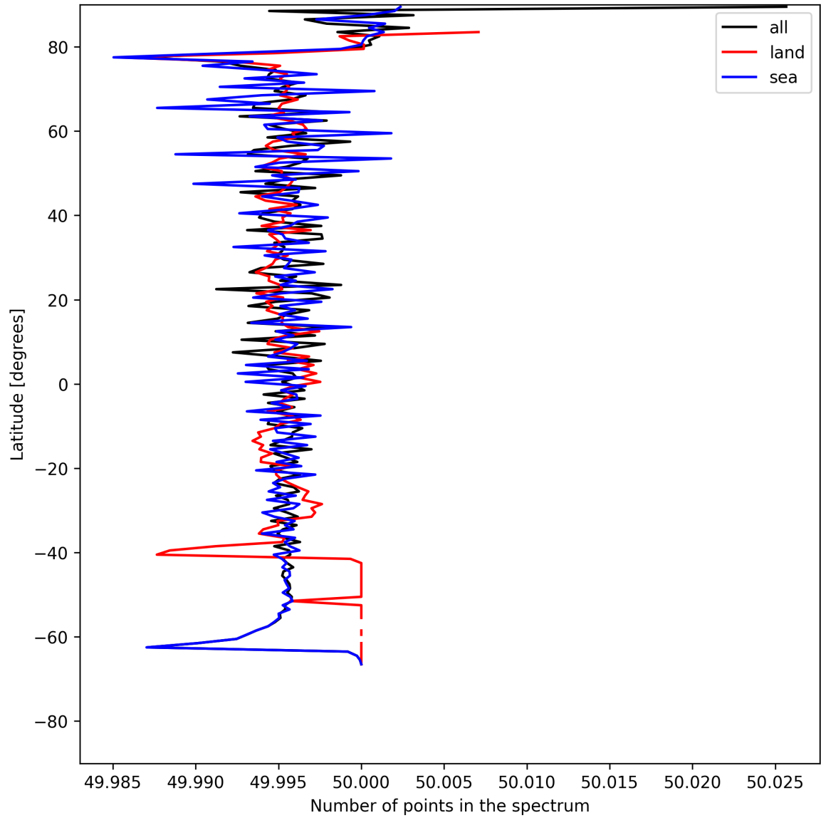
Figure 27: Zonal average of “Number of points in the spectrum” for 2025-05-23 to 2025-05-25.
