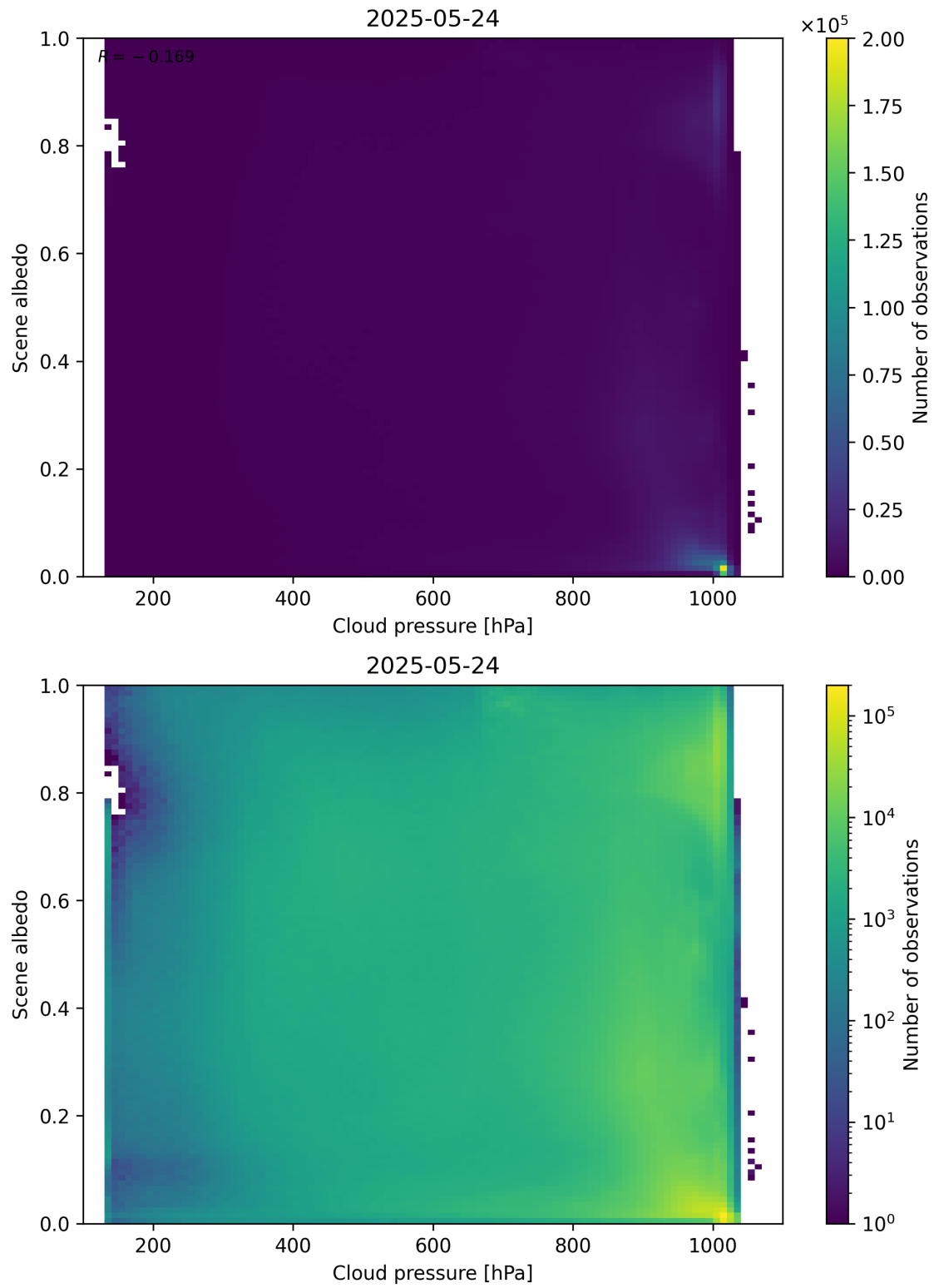
Figure 83: Scatter density plot of “Cloud pressure” against “Scene albedo” for 2025-05-23 to 2025-05-25.
