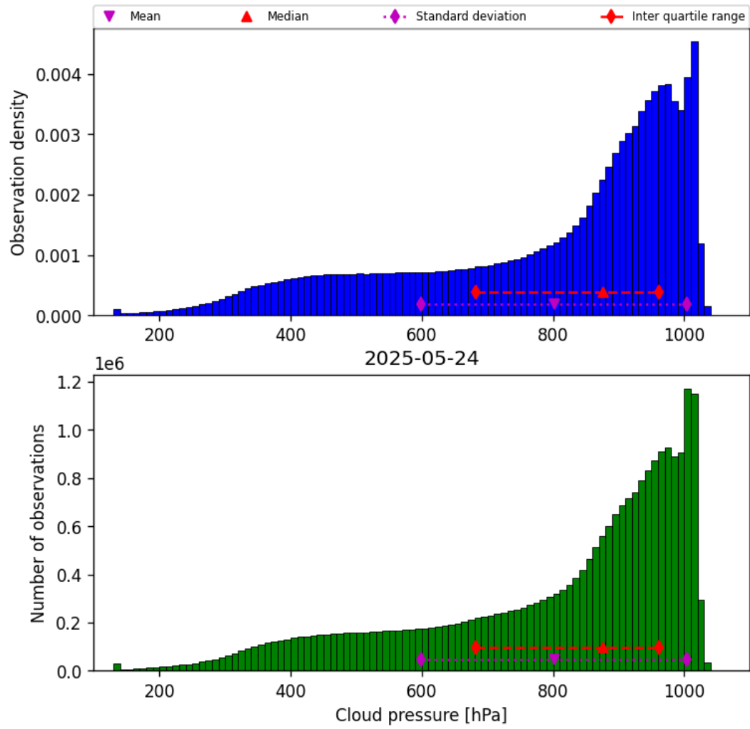
Figure 30: Histogram of “Cloud pressure” for 2025-05-23 to 2025-05-25
