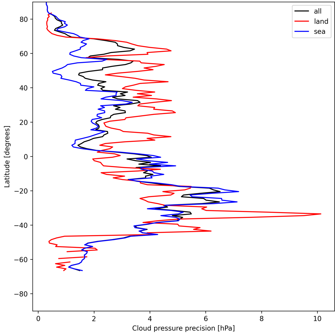
Figure 14: Zonal average of “Cloud pressure precision” for 2025-05-23 to 2025-05-25.
