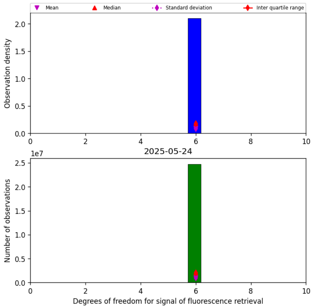
Figure 43: Histogram of “Degrees of freedom for signal of fluorescence retrieval” for 2025-05-23 to 2025-05-25
