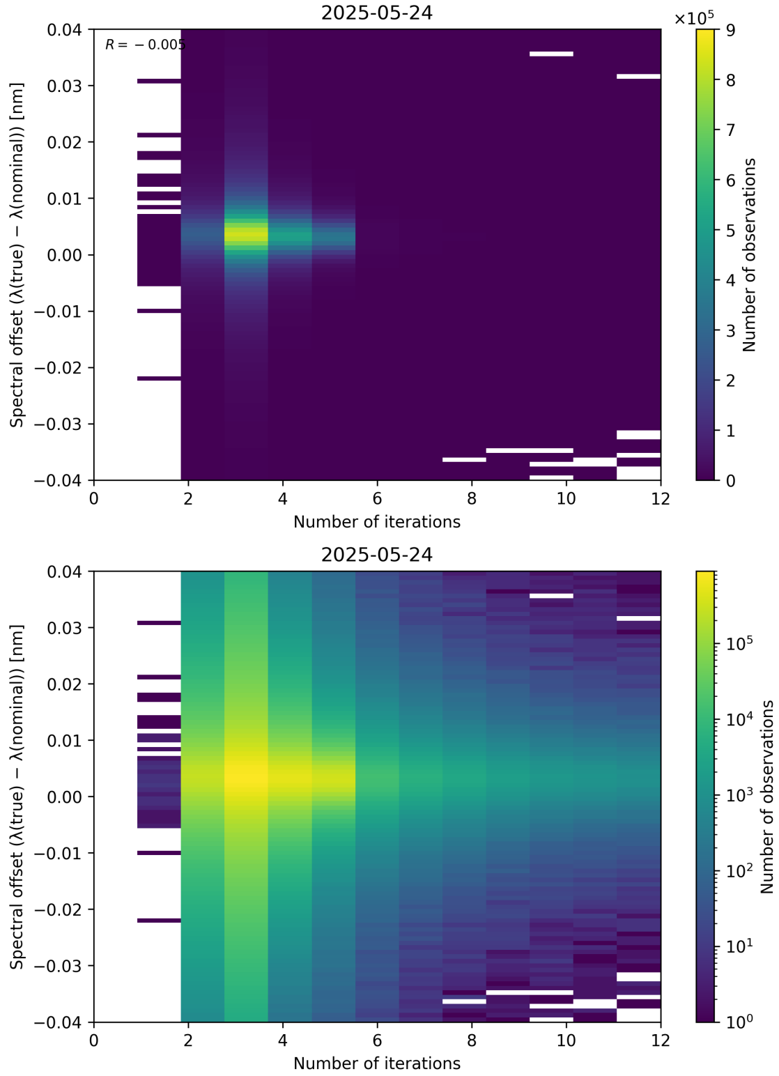
Figure 100: Scatter density plot of “Number of iterations” against “Spectral offset ( \lambda_{\text{true}} - \lambda_{\text{nominal}} )” for 2025-05-23 to 2025-05-25.
