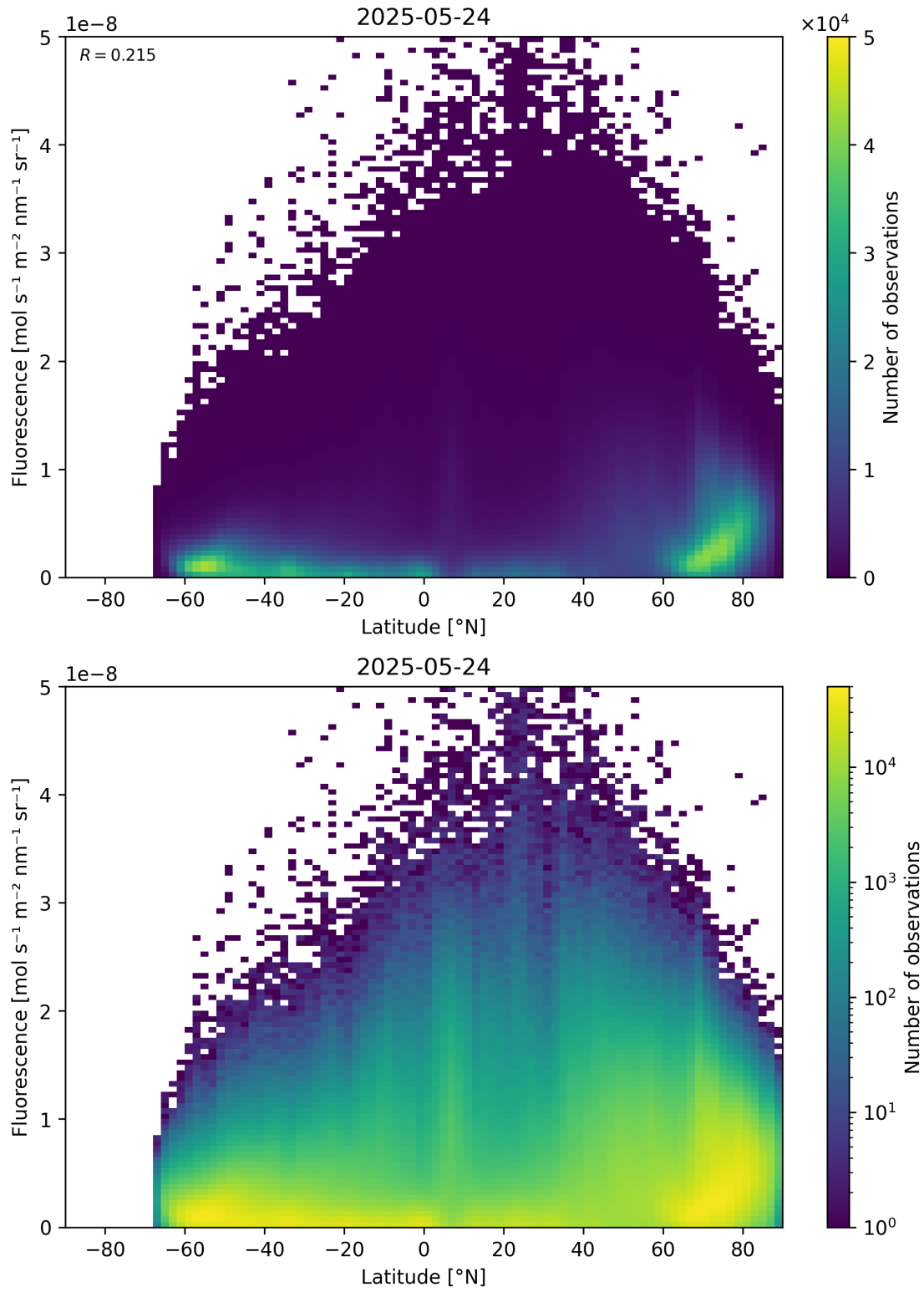
Figure 92: Scatter density plot of “Latitude” against “Fluorescence” for 2025-05-23 to 2025-05-25.
