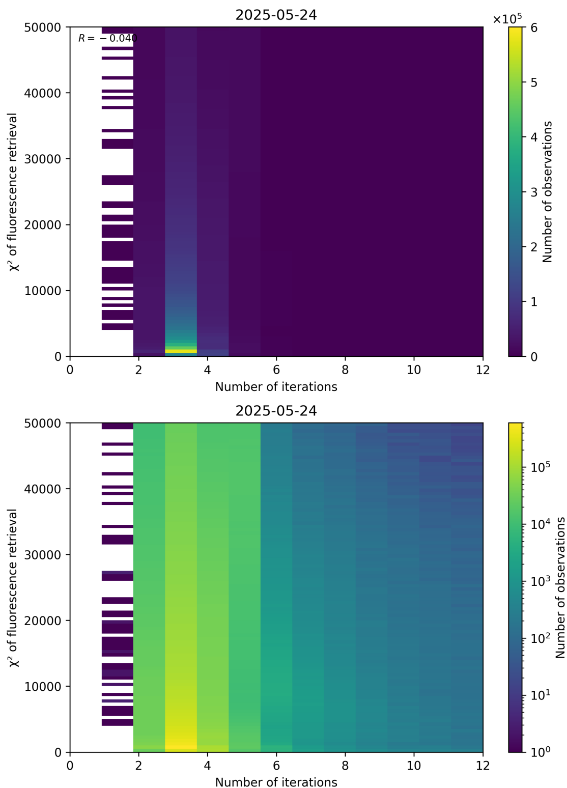
Figure 97: Scatter density plot of “Number of iterations” against “ \chi^2 of fluorescence retrieval” for 2025-05-23 to 2025-05-25.
