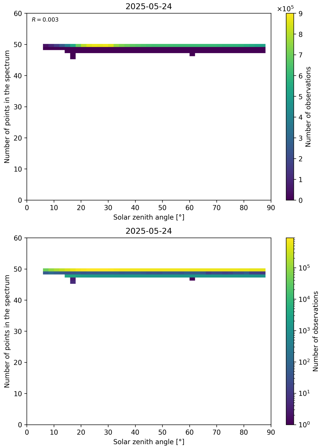
Figure 115: Scatter density plot of “Solar zenith angle” against “Number of points in the spectrum” for 2025-05-23 to 2025-05-25.
