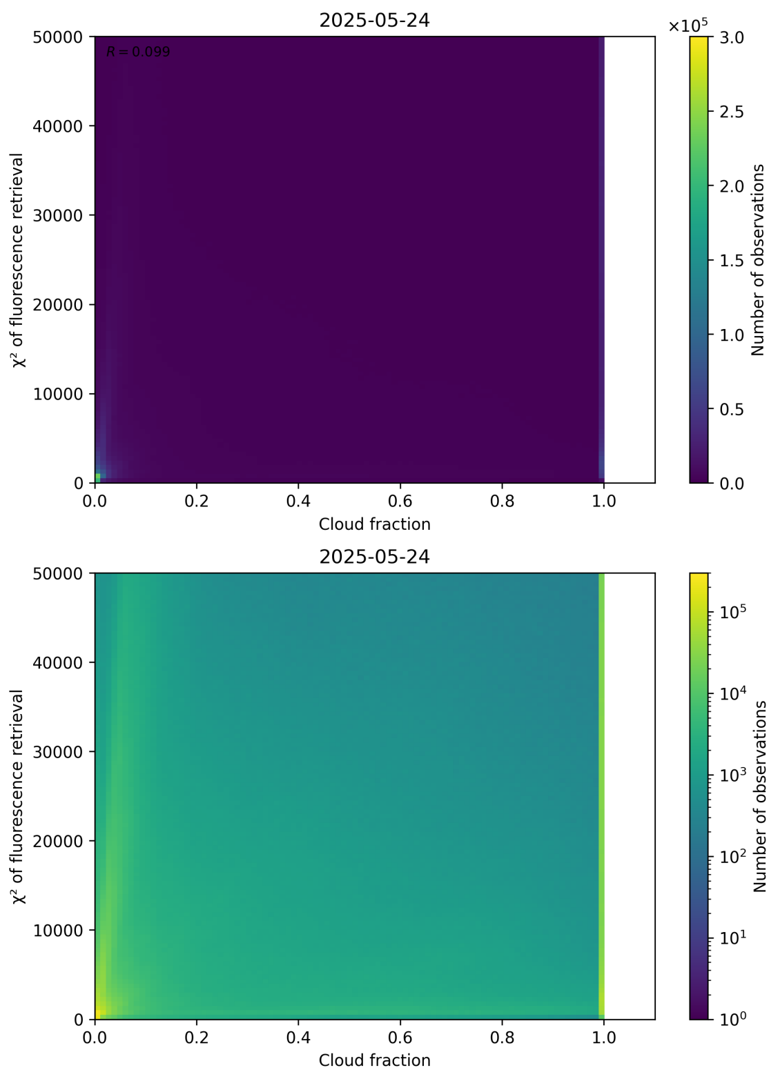
Figure 71: Scatter density plot of “Cloud fraction” against “ \chi^2 of fluorescence retrieval” for 2025-05-23 to 2025-05-25.
