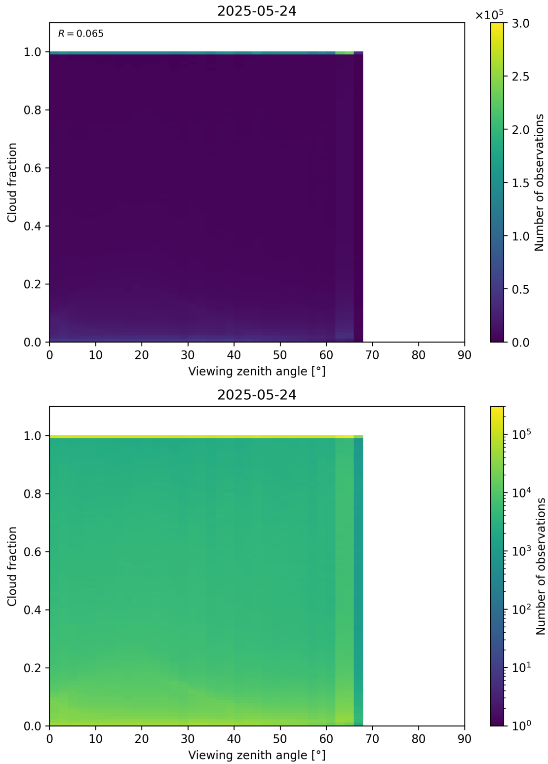
Figure 120: Scatter density plot of “Viewing zenith angle” against “Cloud fraction” for 2025-05-23 to 2025-05-25.
