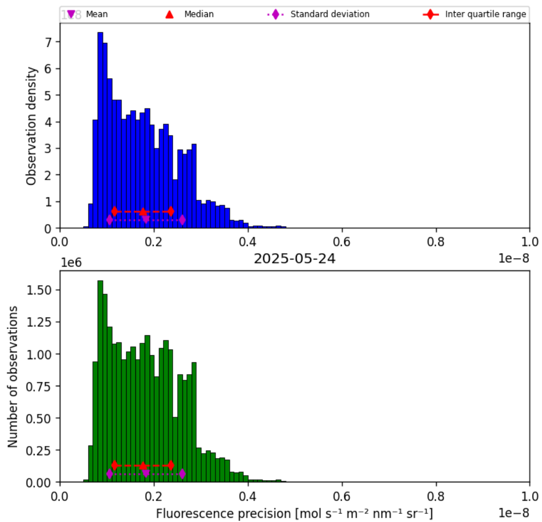
Figure 41: Histogram of “Fluorescence precision” for 2025-05-23 to 2025-05-25
