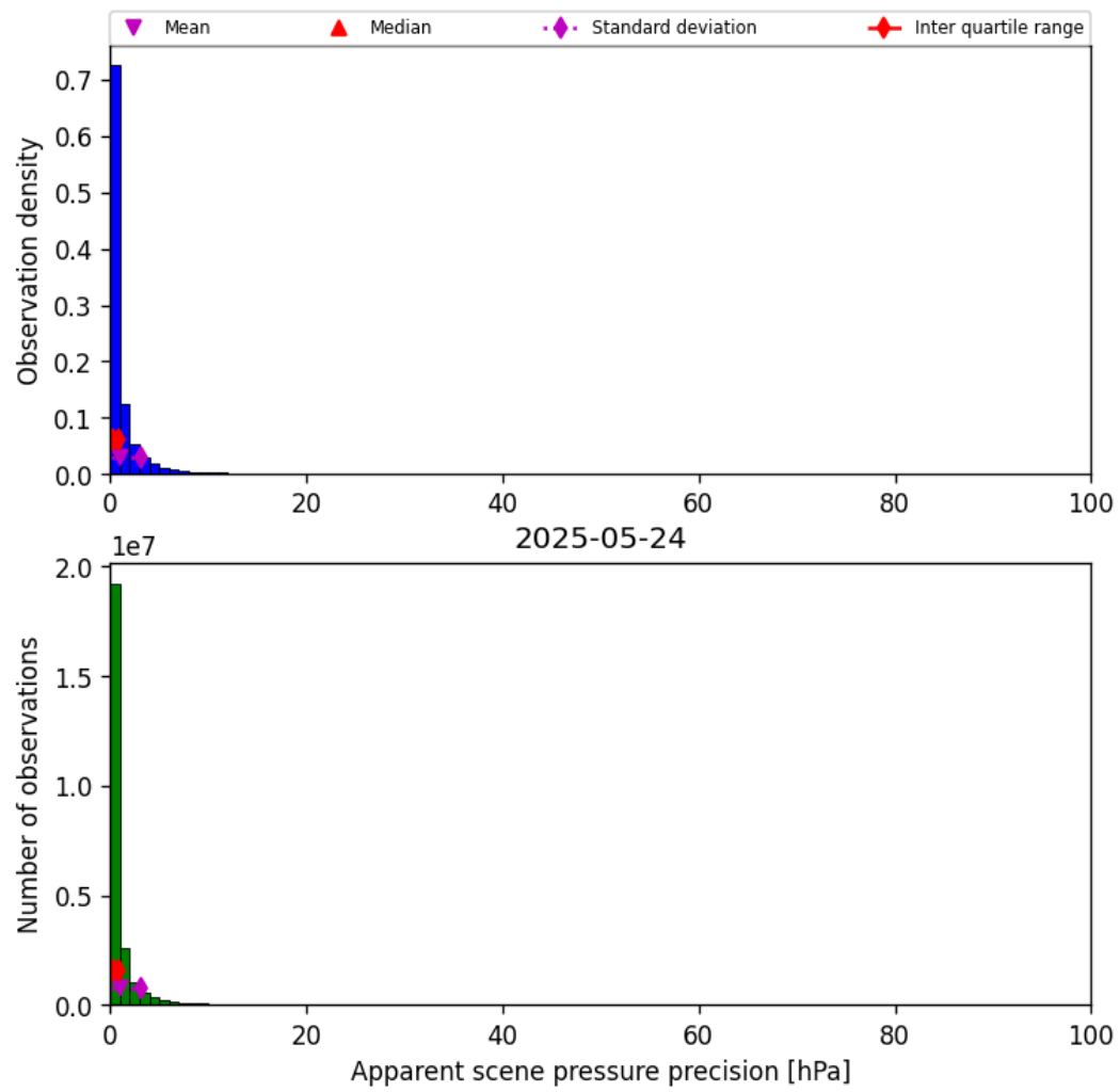
Figure 37: Histogram of “Apparent scene pressure precision” for 2025-05-23 to 2025-05-25
