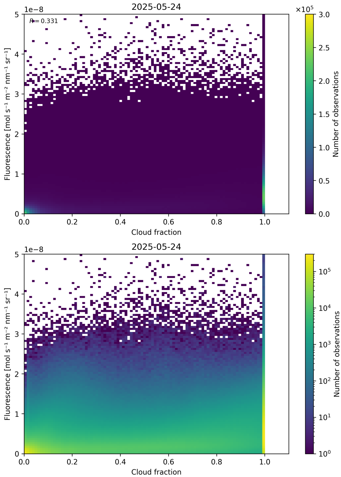
Figure 72: Scatter density plot of “Cloud fraction” against “Fluorescence” for 2025-05-23 to 2025-05-25.
