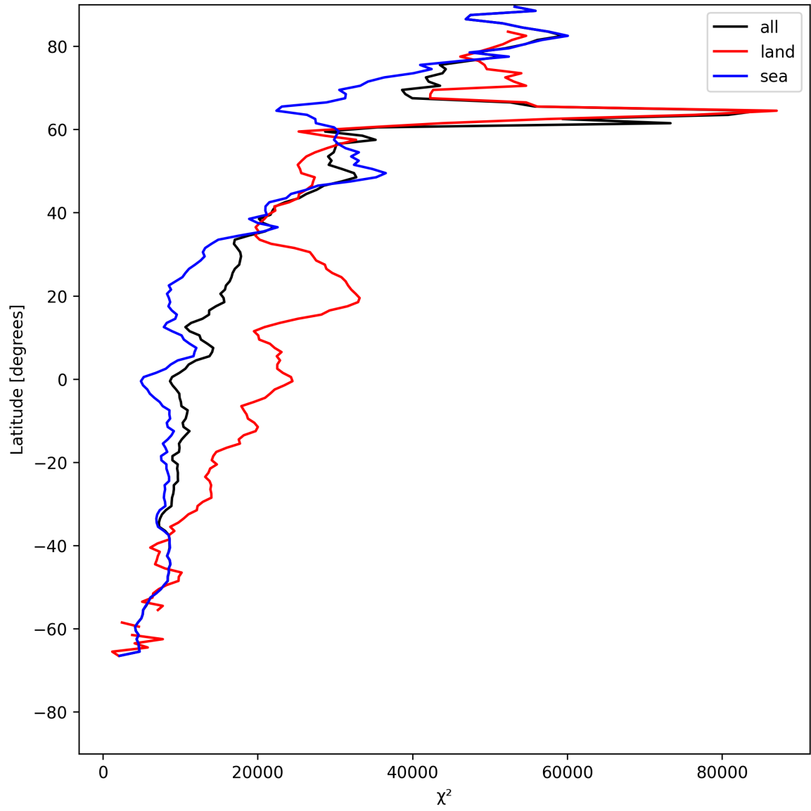
Figure 21: Zonal average of “ \chi^2 ” for 2025-05-23 to 2025-05-25.
