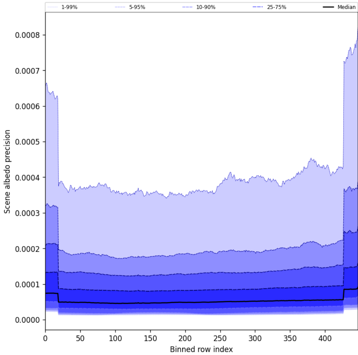
Figure 52: Along track statistics of “Scene albedo precision” for 2025-05-23 to 2025-05-25
