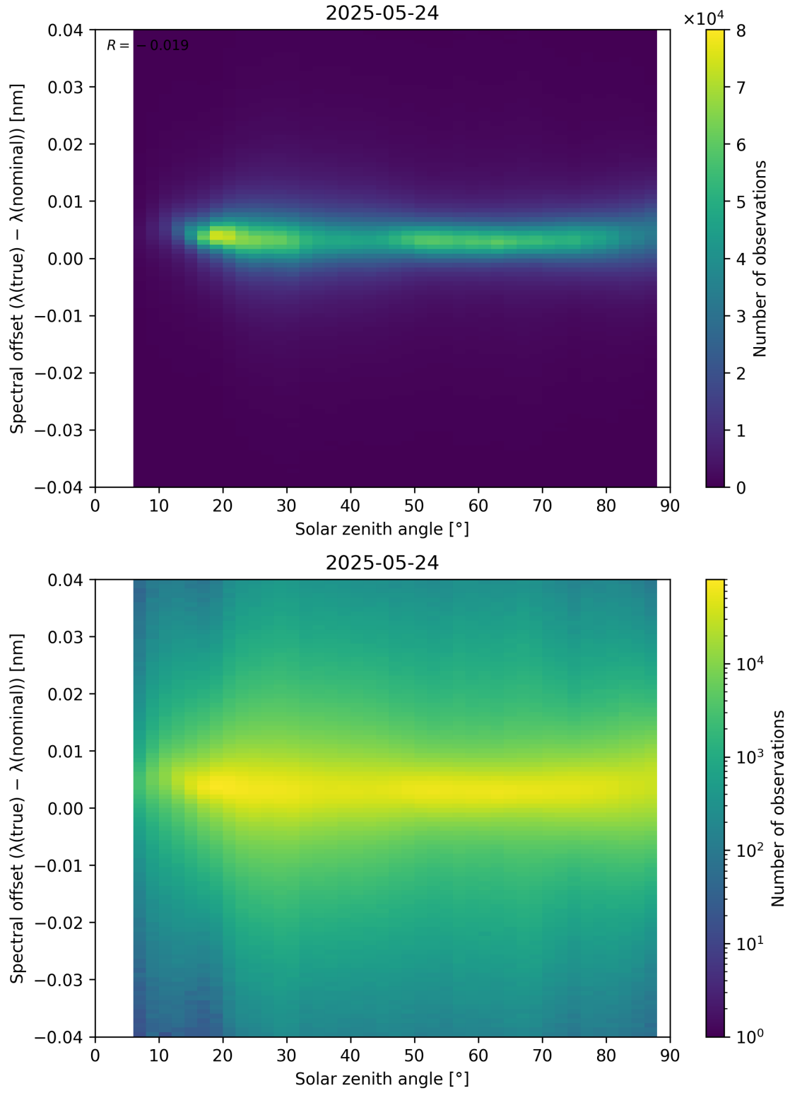
Figure 117: Scatter density plot of “Solar zenith angle” against “Spectral offset ( \lambda_{\text{true}} - \lambda_{\text{nominal}} )” for 2025-05-23 to 2025-05-25.
