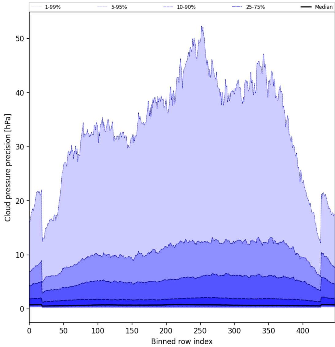
Figure 48: Along track statistics of “Cloud pressure precision” for 2025-05-23 to 2025-05-25
