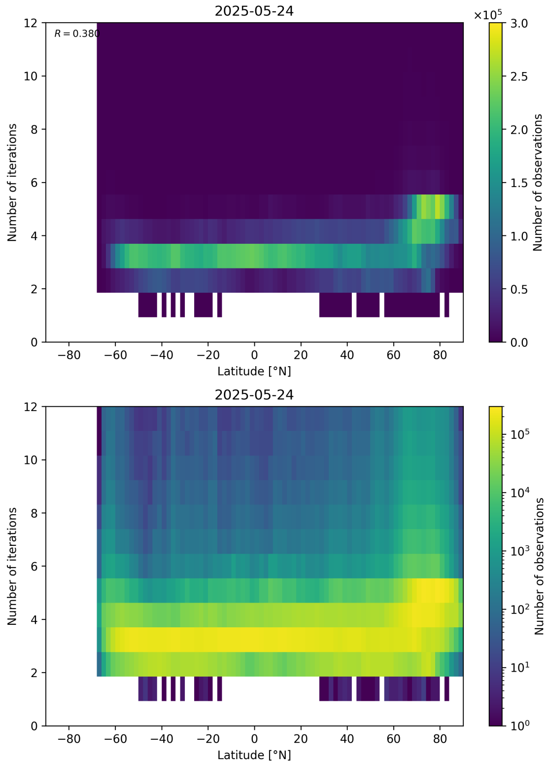
Figure 93: Scatter density plot of “Latitude” against “Number of iterations” for 2025-05-23 to 2025-05-25.
