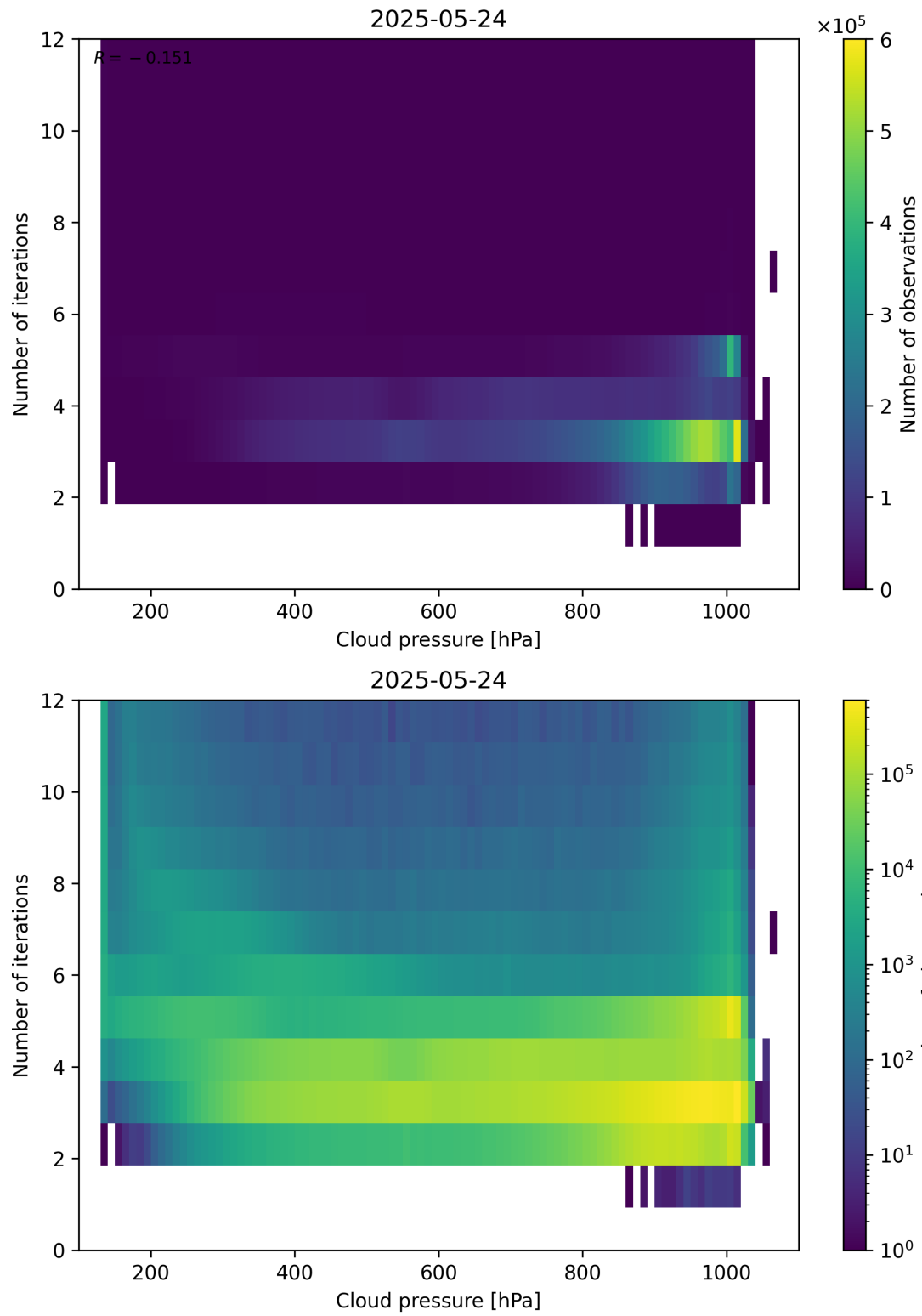
Figure 81: Scatter density plot of “Cloud pressure” against “Number of iterations” for 2025-05-23 to 2025-05-25.
