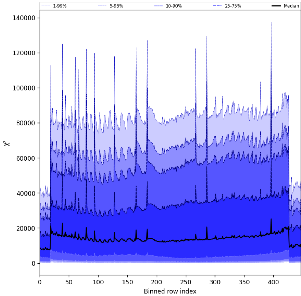
Figure 55: Along track statistics of “ \chi^2 ” for 2025-05-23 to 2025-05-25
