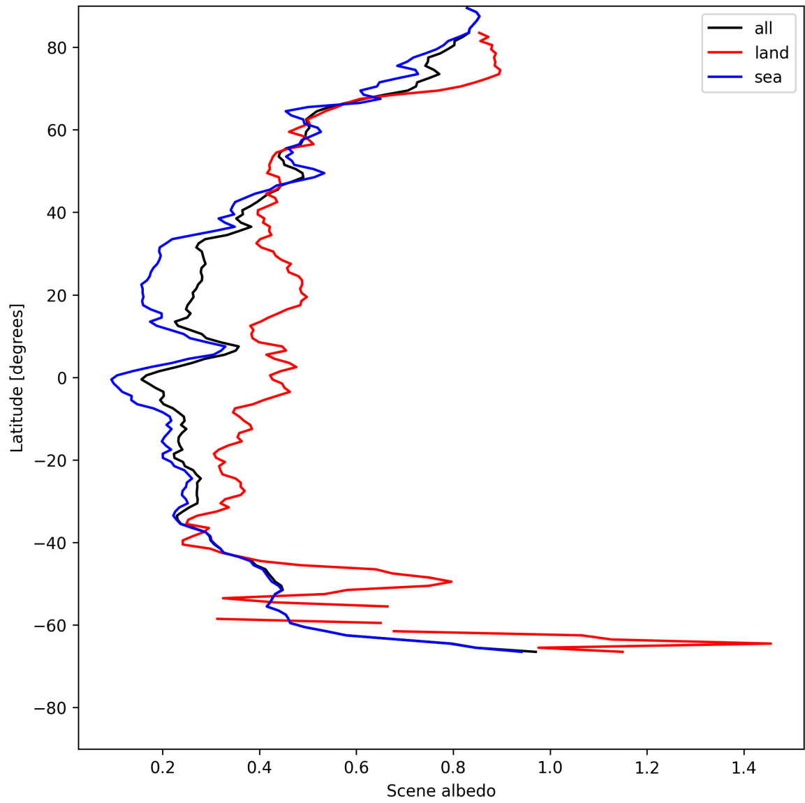
Figure 17: Zonal average of “Scene albedo” for 2025-05-23 to 2025-05-25.
