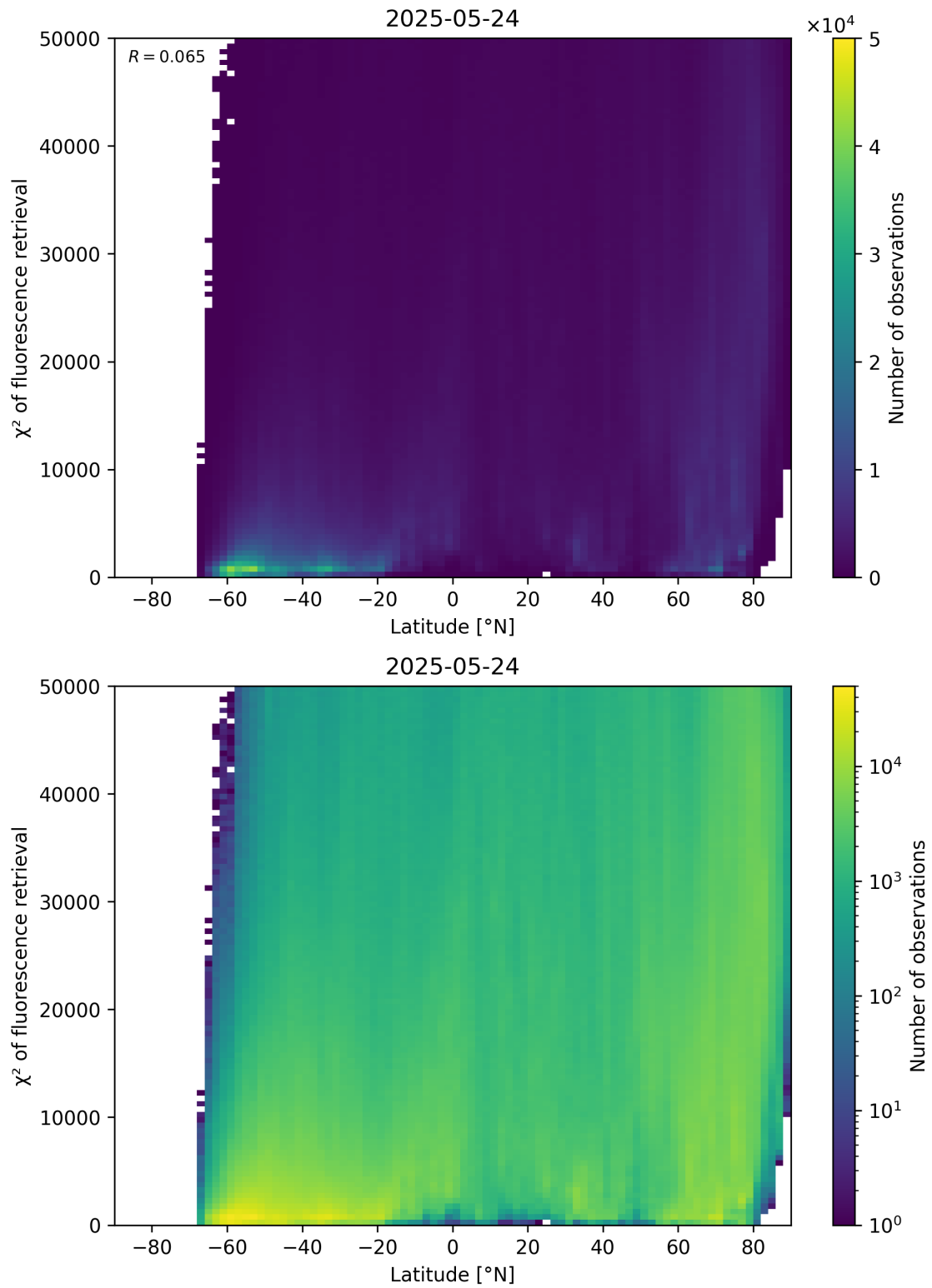
Figure 89: Scatter density plot of “Latitude” against “ \chi^2 of fluorescence retrieval” for 2025-05-23 to 2025-05-25.
