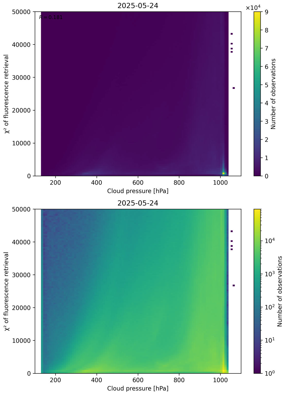
Figure 78: Scatter density plot of “Cloud pressure” against “ \chi^2 of fluorescence retrieval” for 2025-05-23 to 2025-05-25.
