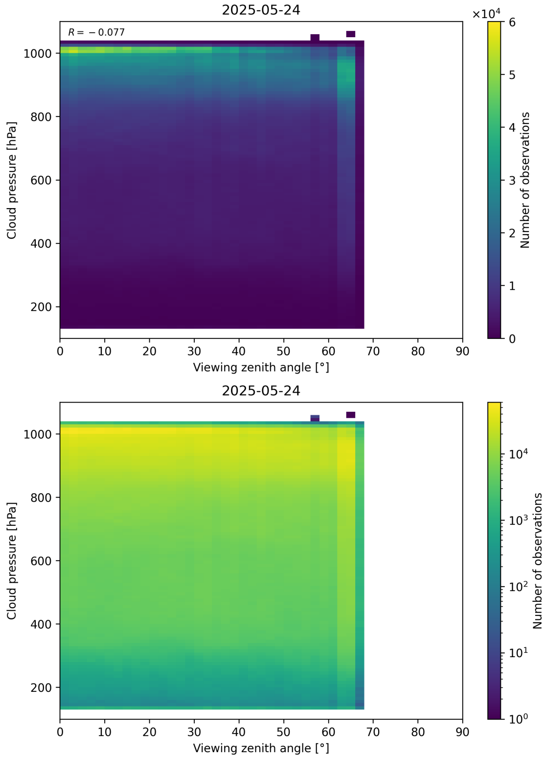
Figure 121: Scatter density plot of “Viewing zenith angle” against “Cloud pressure” for 2025-05-23 to 2025-05-25.
