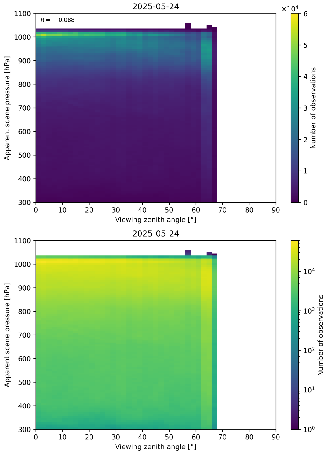
Figure 118: Scatter density plot of “Viewing zenith angle” against “Apparent scene pressure” for 2025-05-23 to 2025-05-25.
