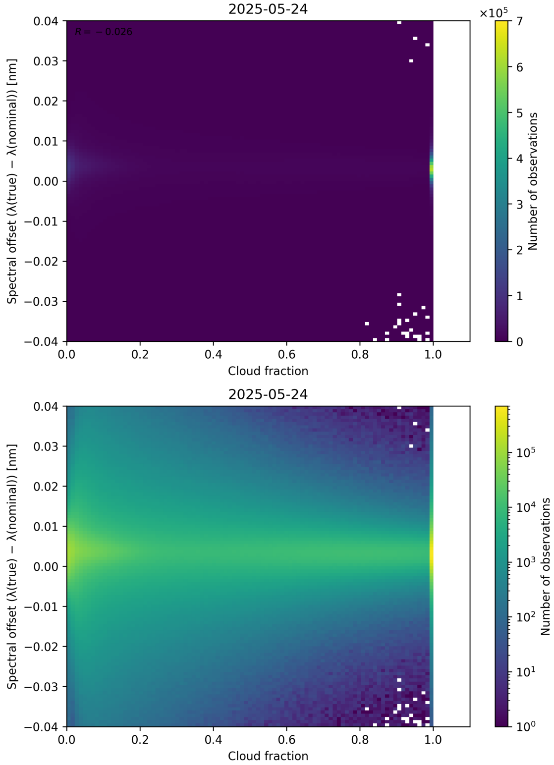
Figure 76: Scatter density plot of “Cloud fraction” against “Spectral offset ( \lambda_{\text{true}} - \lambda_{\text{nominal}} )” for 2025-05-23 to 2025-05-25.
