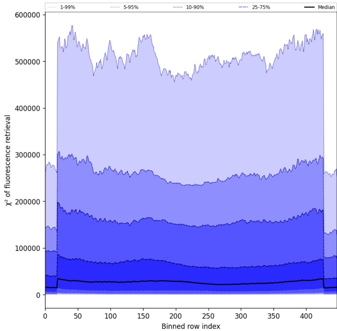
Figure 59: Along track statistics of “ \chi^2 of fluorescence retrieval” for 2025-05-23 to 2025-05-25
