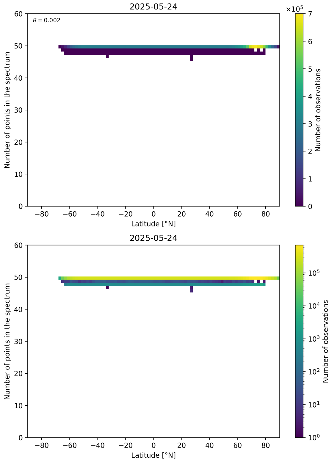
Figure 94: Scatter density plot of “Latitude” against “Number of points in the spectrum” for 2025-05-23 to 2025-05-25.
