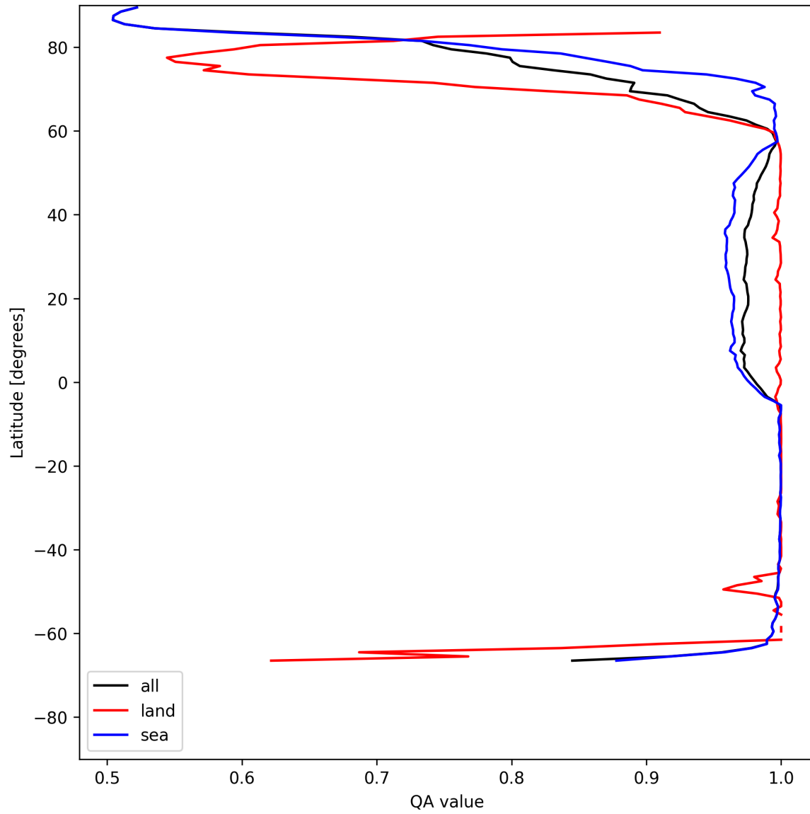
Figure 12: Zonal average of “QA value” for 2025-05-23 to 2025-05-25.
