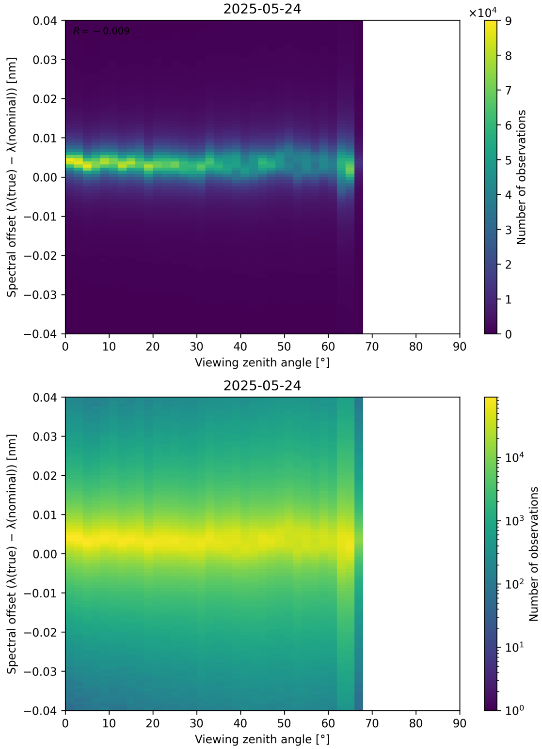
Figure 128: Scatter density plot of “Viewing zenith angle” against “Spectral offset ( \lambda_{\text{true}} - \lambda_{\text{nominal}} )” for 2025-05-23 to 2025-05-25.
