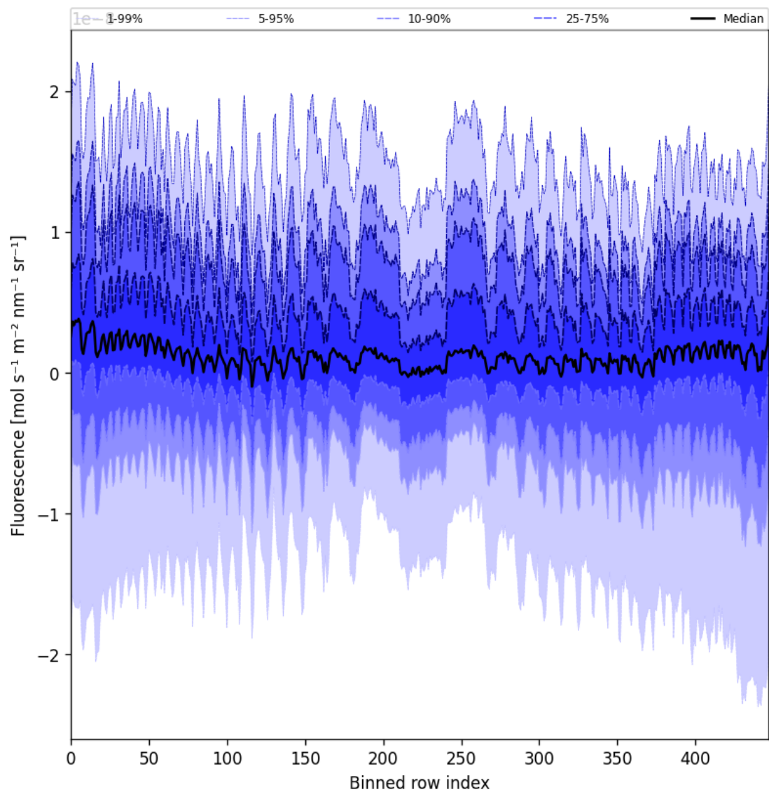
Figure 57: Along track statistics of “Fluorescence” for 2025-05-23 to 2025-05-25
