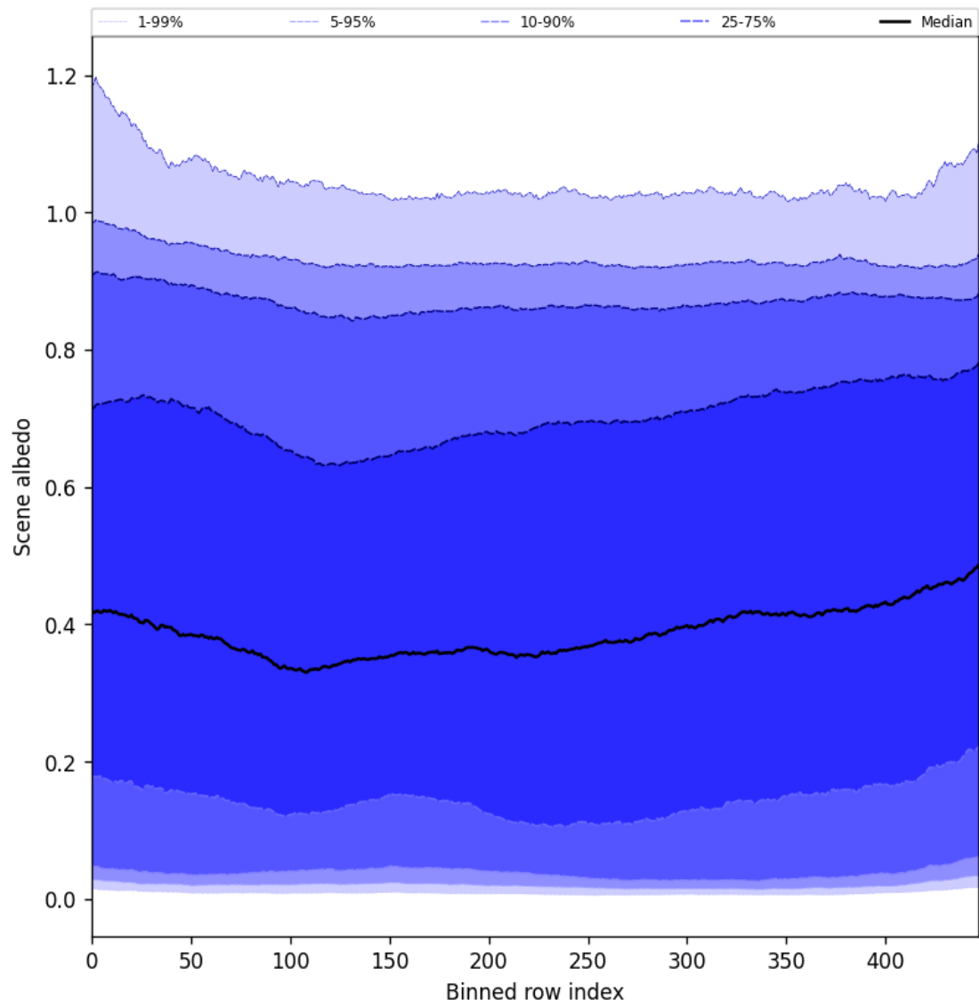
Figure 51: Along track statistics of "Scene albedo" for 2025-05-23 to 2025-05-25
