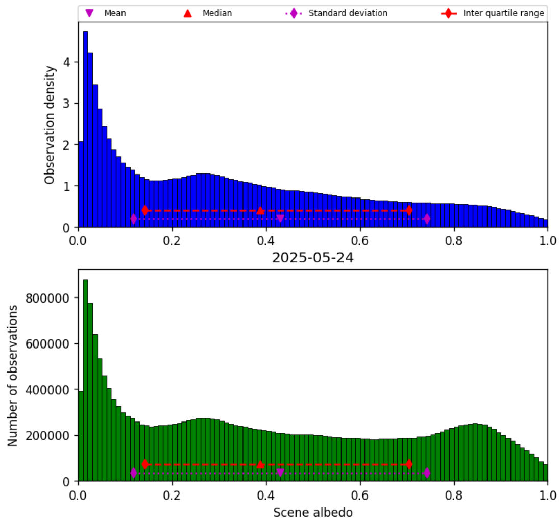
Figure 34: Histogram of “Scene albedo” for 2025-05-23 to 2025-05-25
