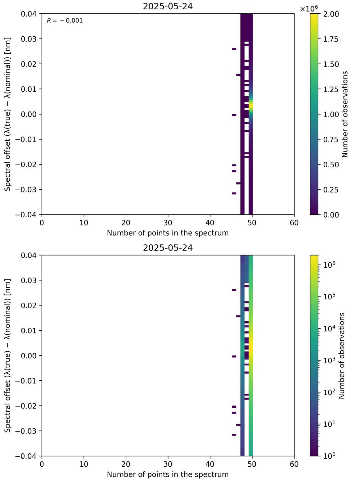
Figure 101: Scatter density plot of “Number of points in the spectrum” against “Spectral offset ( \lambda_{\text{true}} - \lambda_{\text{nominal}} )” for 2025-05-23 to 2025-05-25.
