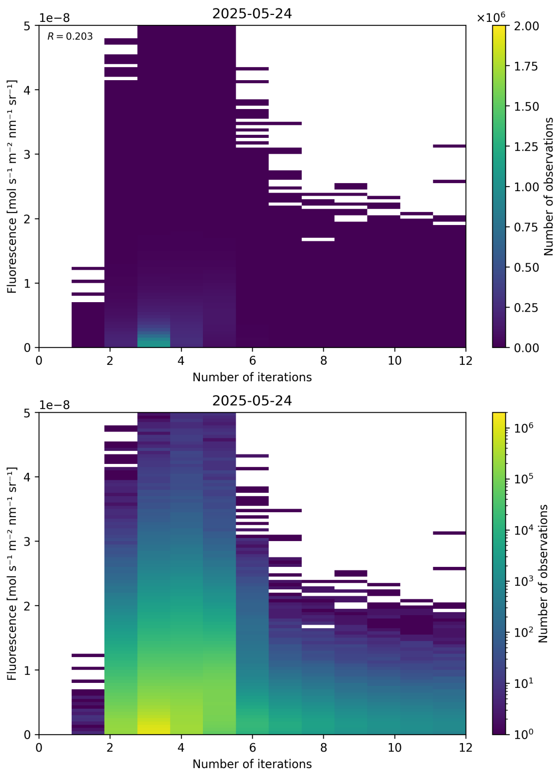
Figure 98: Scatter density plot of “Number of iterations” against “Fluorescence” for 2025-05-23 to 2025-05-25.
