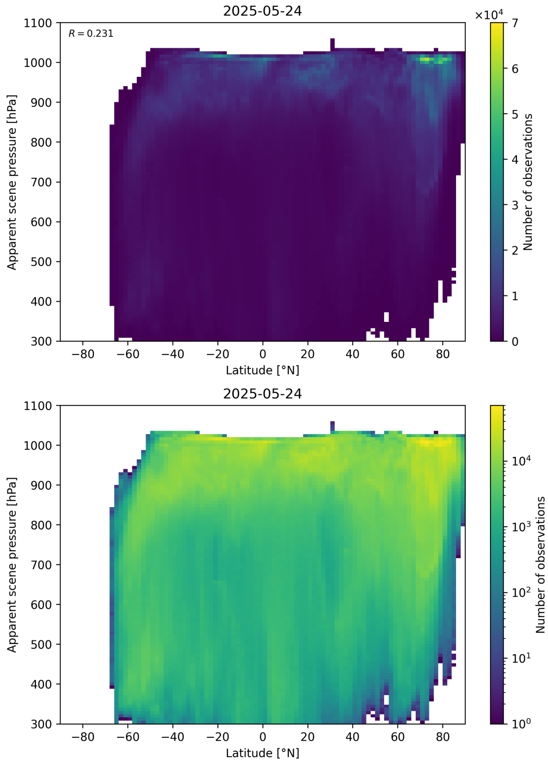
Figure 88: Scatter density plot of “Latitude” against “Apparent scene pressure” for 2025-05-23 to 2025-05-25.
