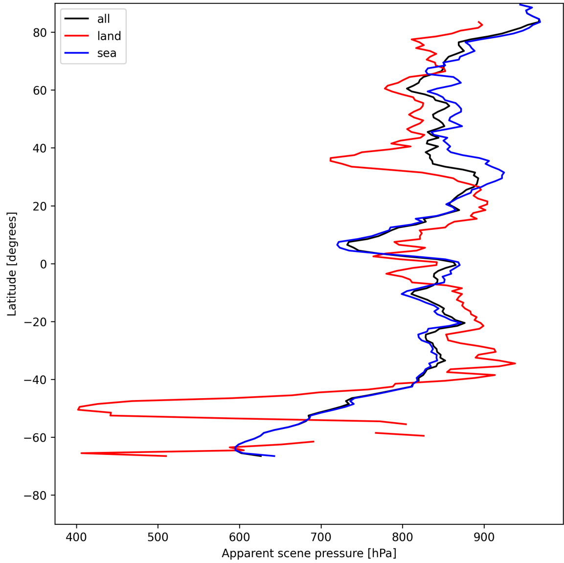
Figure 19: Zonal average of “Apparent scene pressure” for 2025-05-23 to 2025-05-25.
