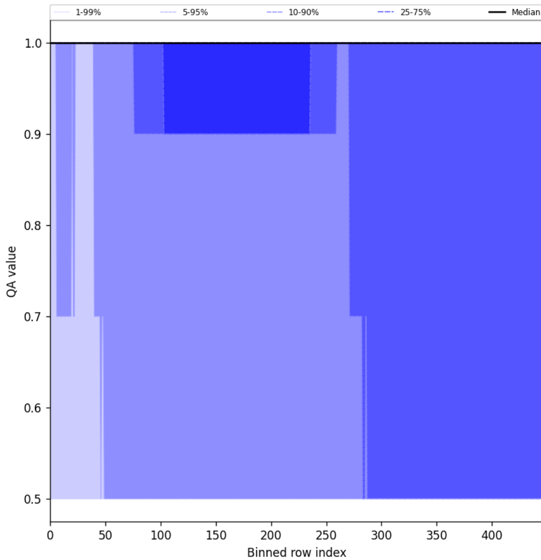
Figure 46: Along track statistics of “QA value” for 2025-05-23 to 2025-05-25
