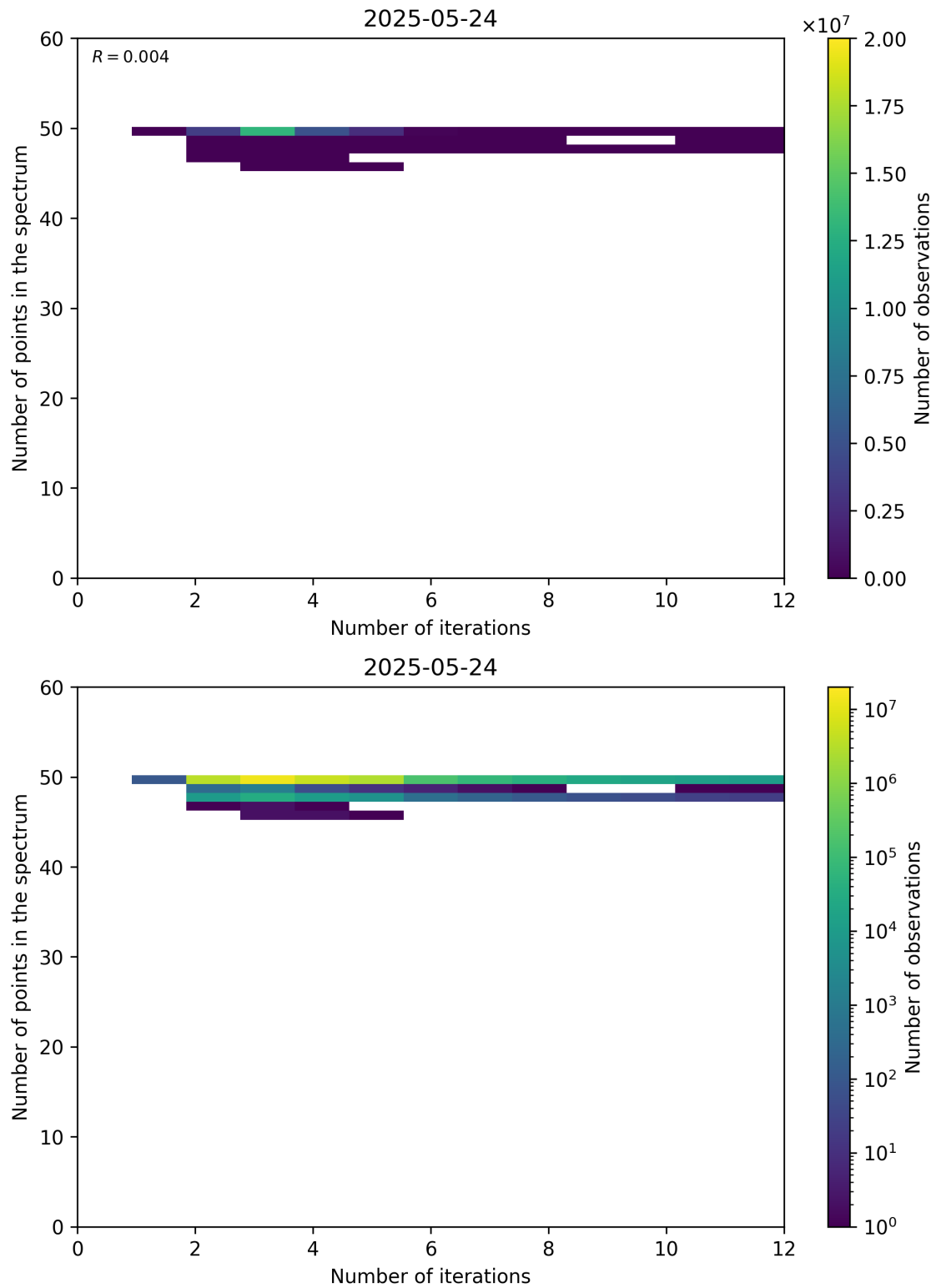
Figure 99: Scatter density plot of “Number of iterations” against “Number of points in the spectrum” for 2025-05-23 to 2025-05-25.
