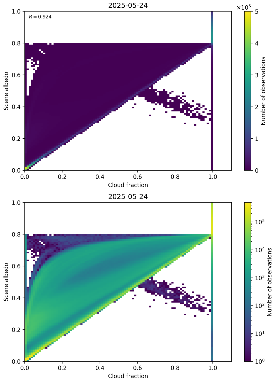
Figure 75: Scatter density plot of “Cloud fraction” against “Scene albedo” for 2025-05-23 to 2025-05-25.
