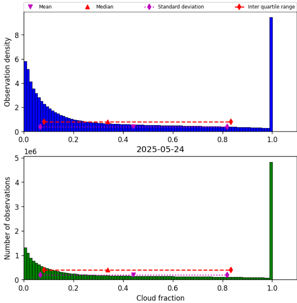
Figure 32: Histogram of "Cloud fraction" for 2025-05-23 to 2025-05-25
