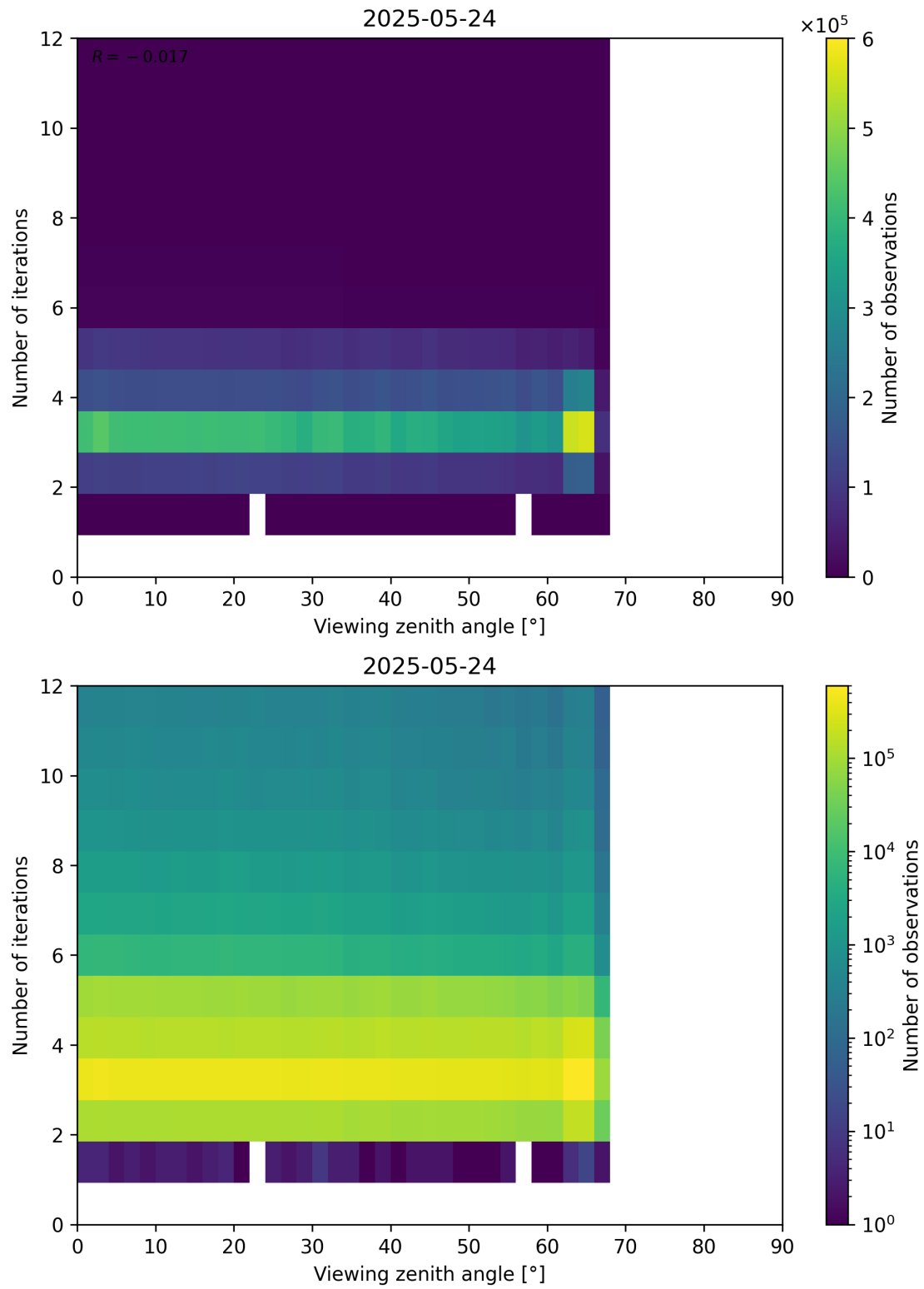
Figure 124: Scatter density plot of “Viewing zenith angle” against “Number of iterations” for 2025-05-23 to 2025-05-25.
