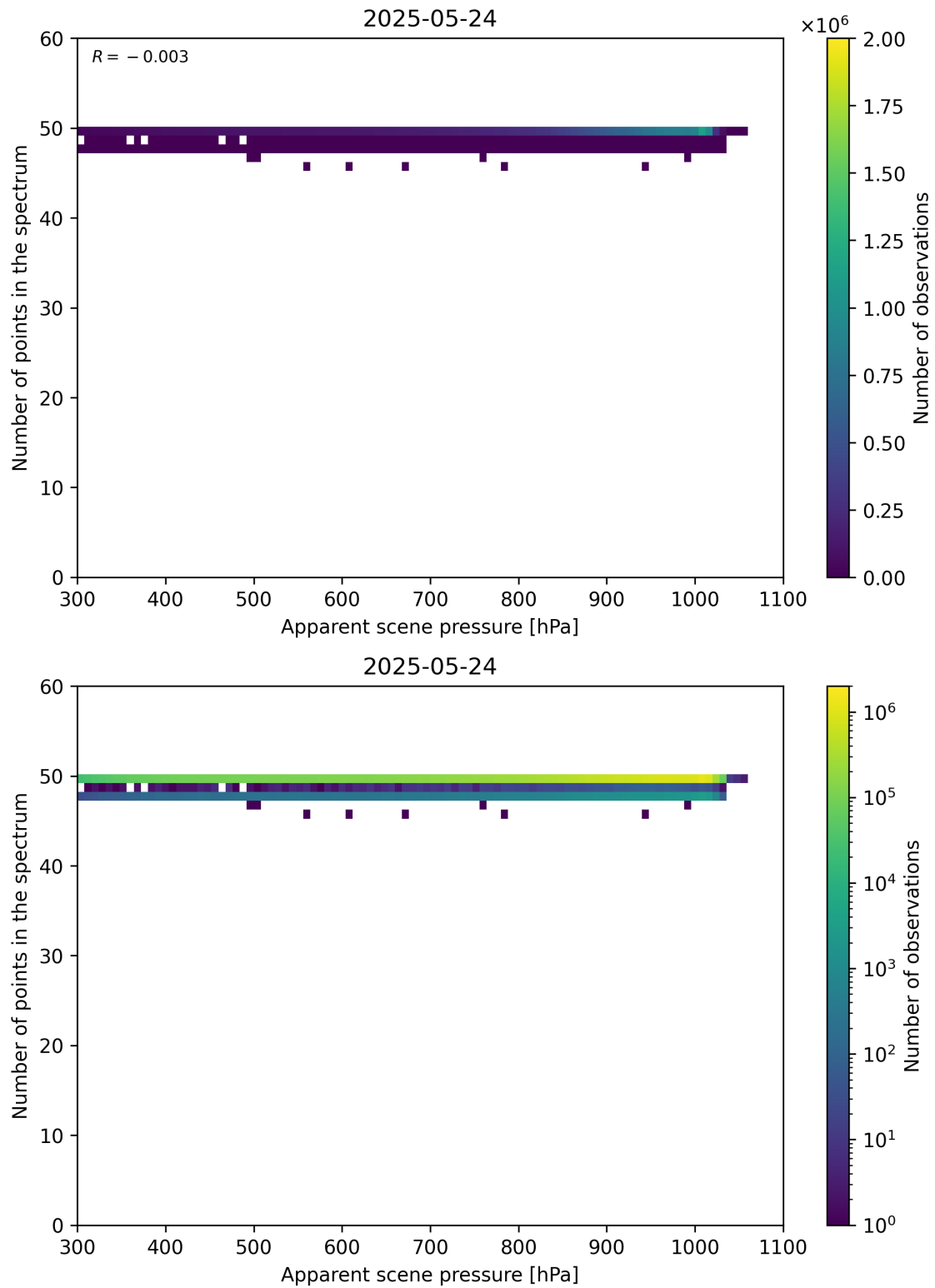
Figure 66: Scatter density plot of “Apparent scene pressure” against “Number of points in the spectrum” for 2025-05-23 to 2025-05-25.
