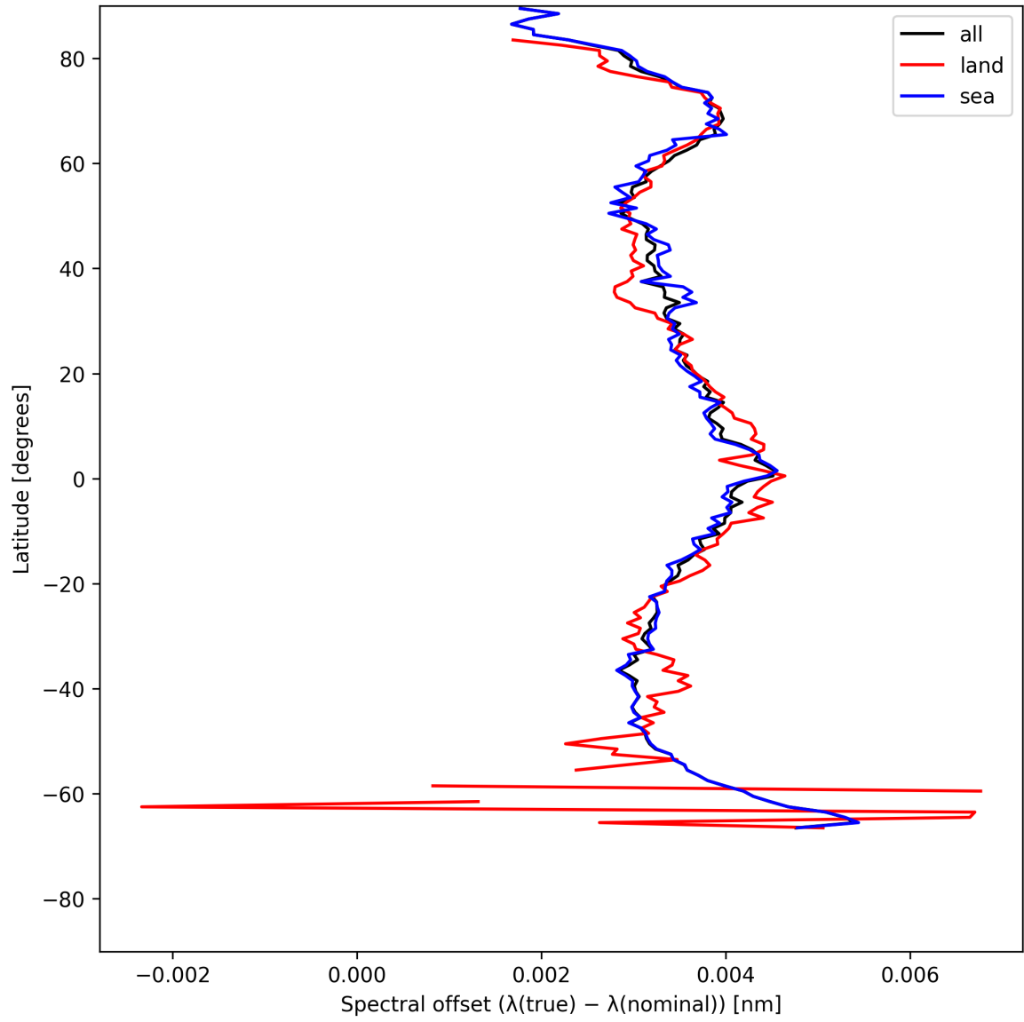
Figure 28: Zonal average of “Spectral offset ( \lambda_{\text{true}} - \lambda_{\text{nominal}} )” for 2025-05-23 to 2025-05-25.
