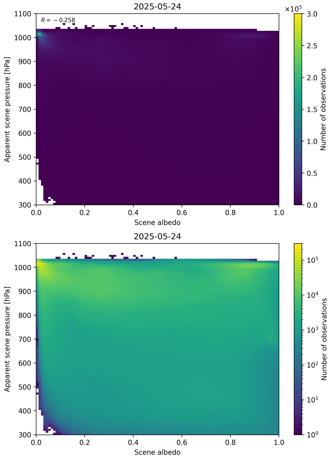
Figure 102: Scatter density plot of “Scene albedo” against “Apparent scene pressure” for 2025-05-23 to 2025-05-25.
