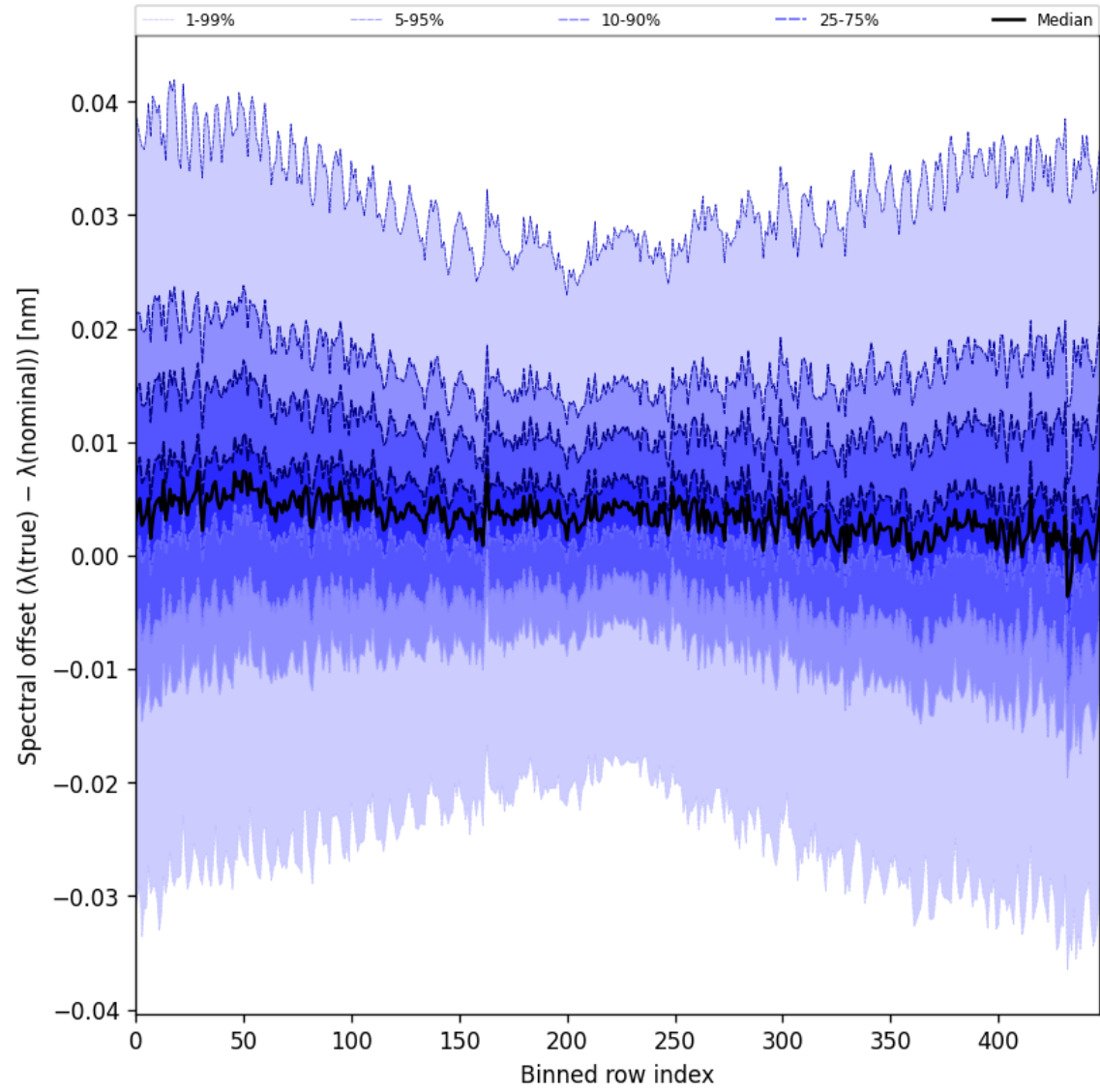
Figure 62: Along track statistics of “Spectral offset ( \lambda_{\text{true}} - \lambda_{\text{nominal}} )” for 2025-05-23 to 2025-05-25
