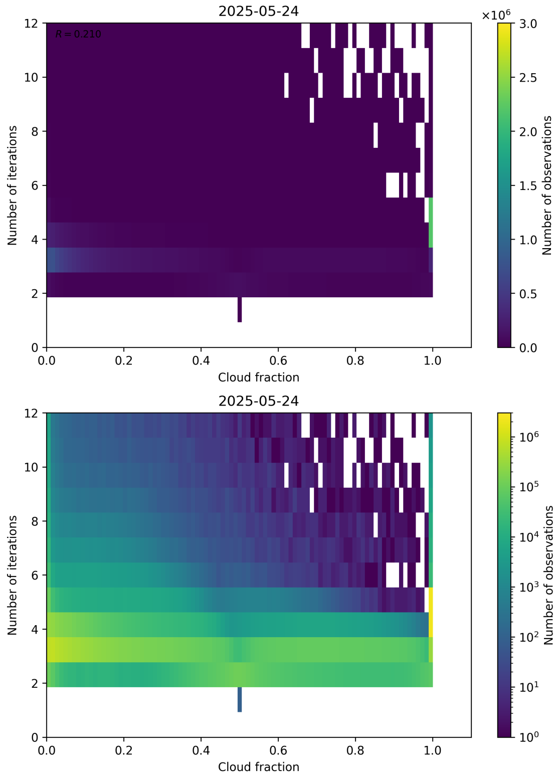
Figure 73: Scatter density plot of “Cloud fraction” against “Number of iterations” for 2025-05-23 to 2025-05-25.
