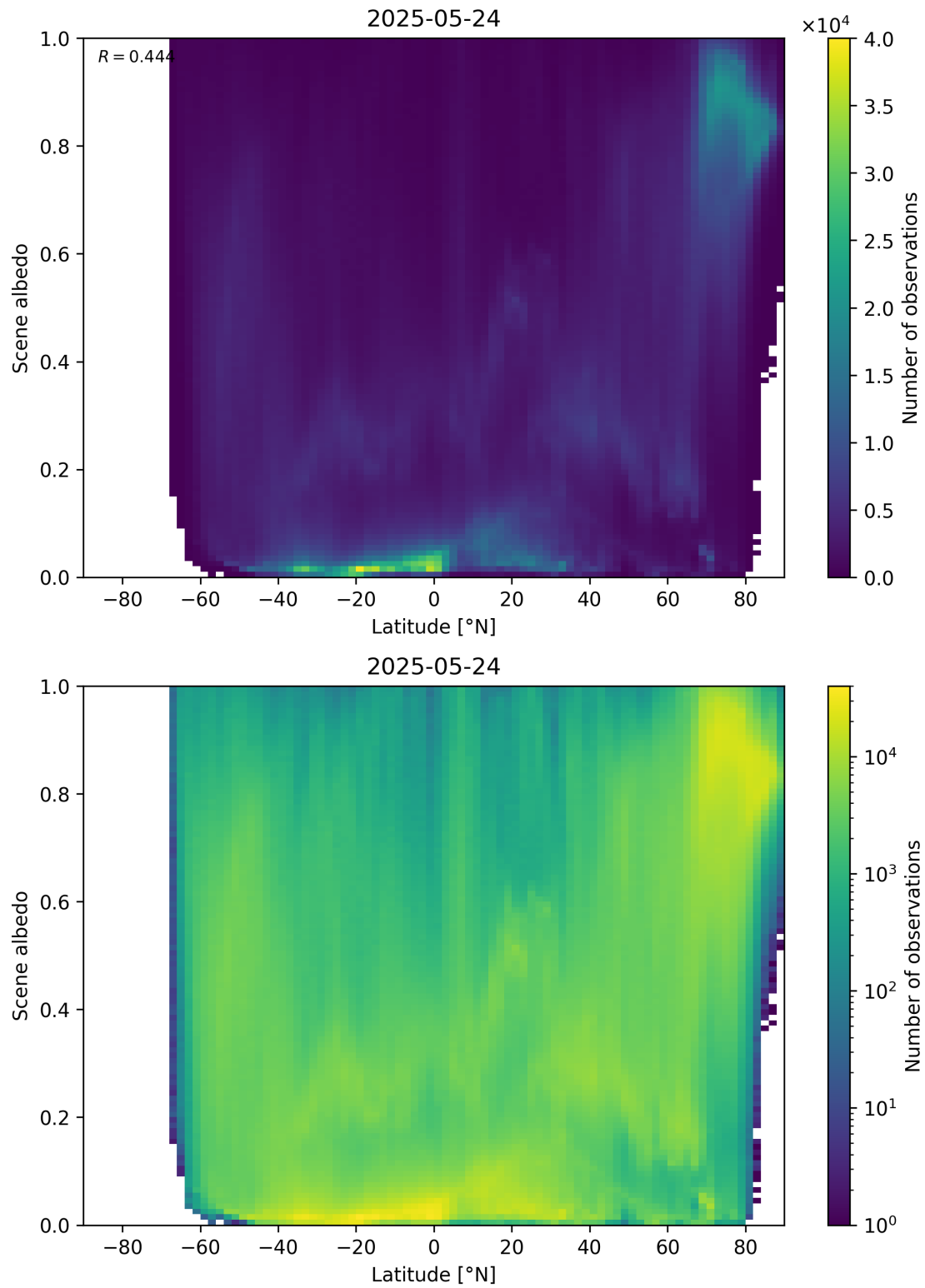
Figure 95: Scatter density plot of “Latitude” against “Scene albedo” for 2025-05-23 to 2025-05-25.
