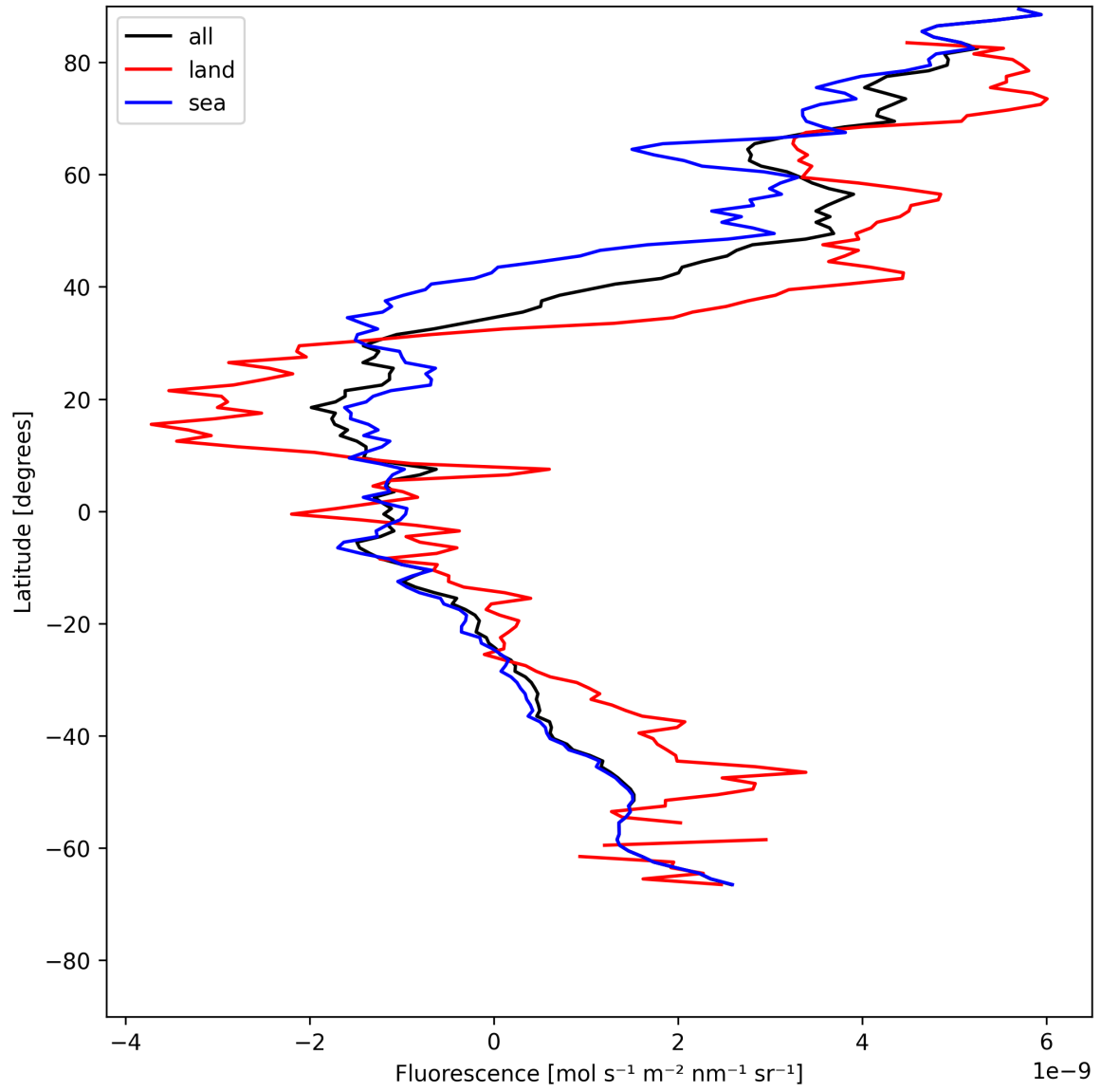
Figure 23: Zonal average of “Fluorescence” for 2025-05-23 to 2025-05-25.
