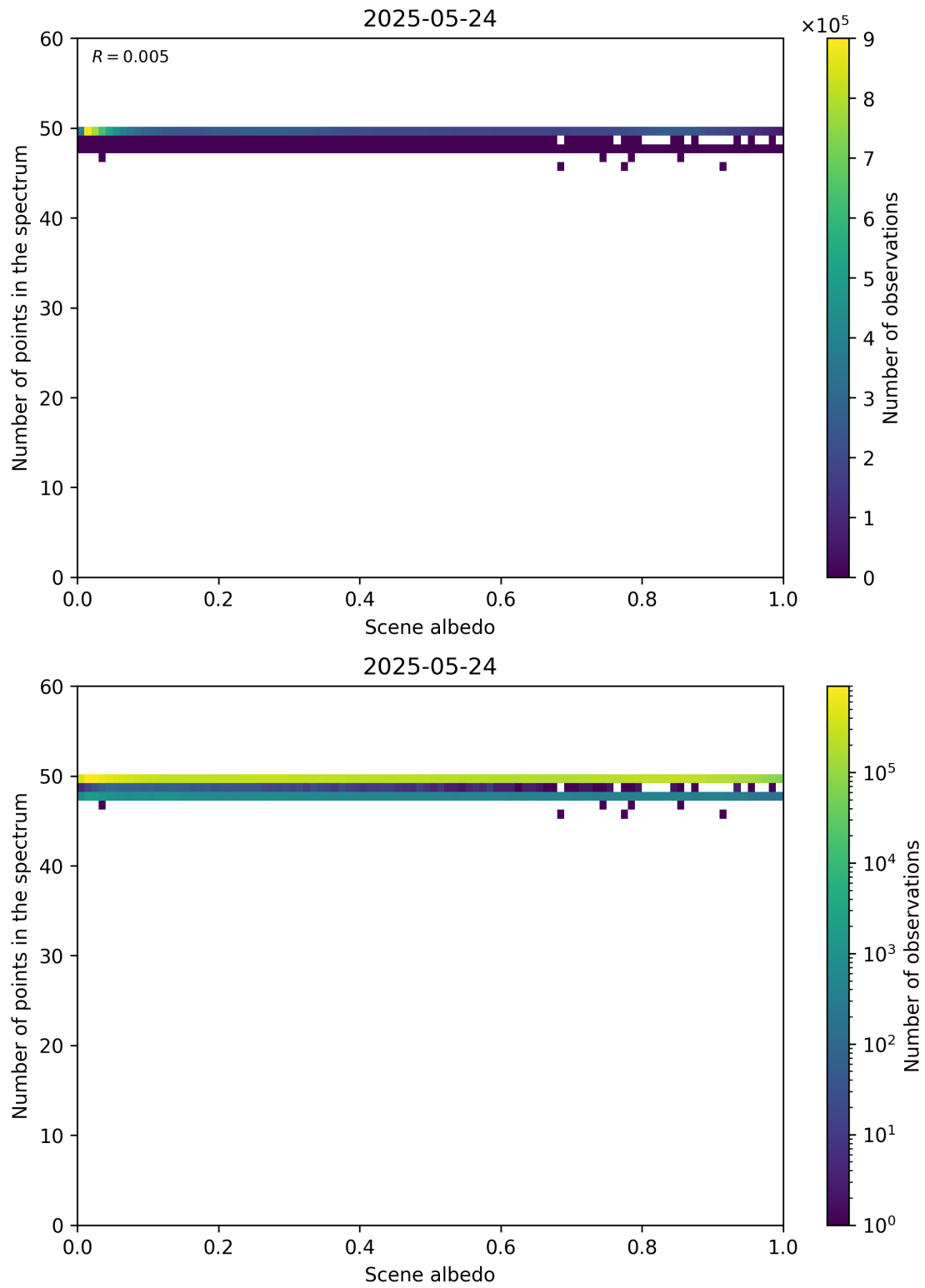
Figure 106: Scatter density plot of “Scene albedo” against “Number of points in the spectrum” for 2025-05-23 to 2025-05-25.
