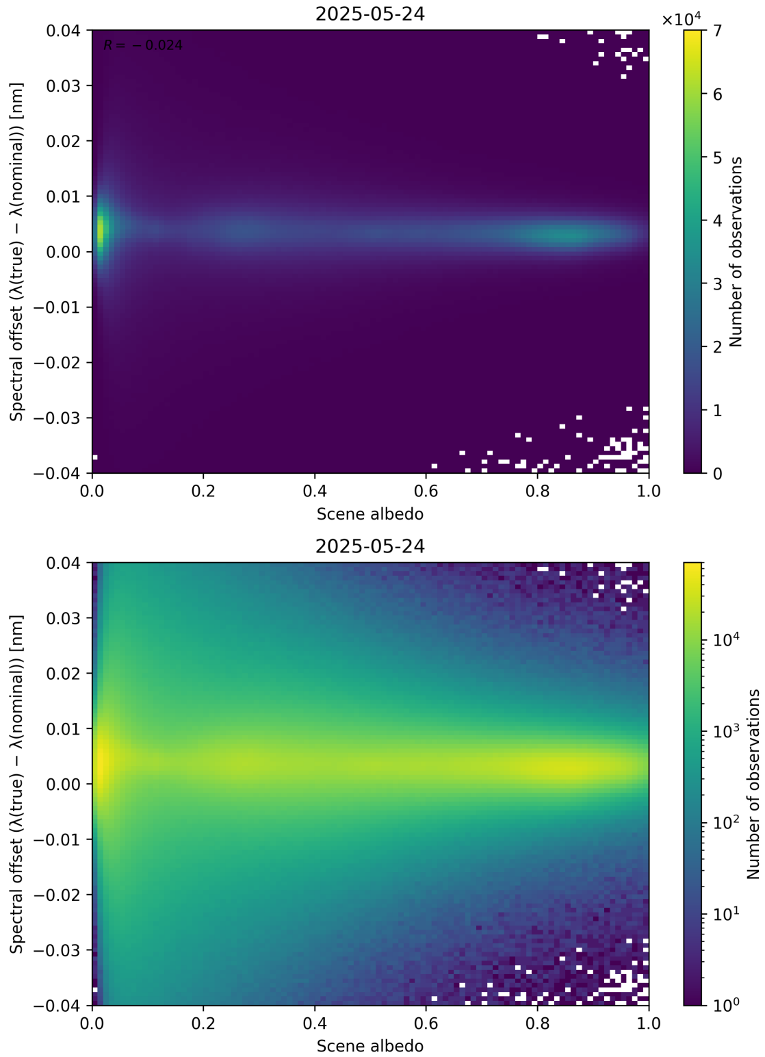
Figure 107: Scatter density plot of “Scene albedo” against “Spectral offset ( \lambda_{\text{true}} - \lambda_{\text{nominal}} )” for 2025-05-23 to 2025-05-25.
