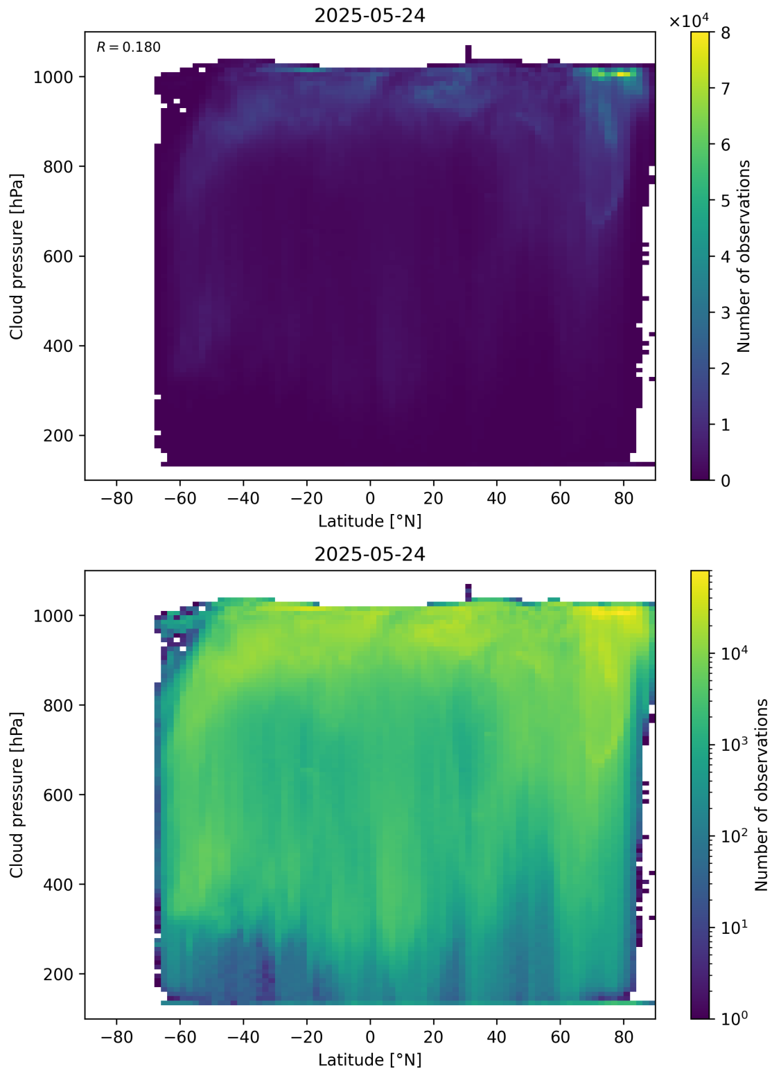
Figure 91: Scatter density plot of “Latitude” against “Cloud pressure” for 2025-05-23 to 2025-05-25.
