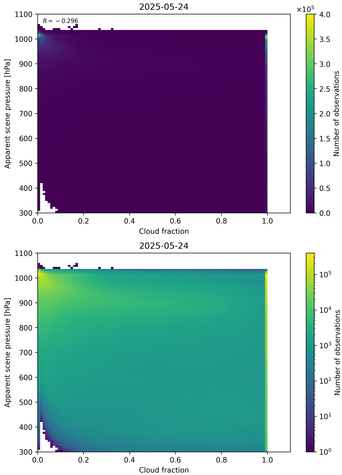
Figure 70: Scatter density plot of “Cloud fraction” against “Apparent scene pressure” for 2025-05-23 to 2025-05-25.
