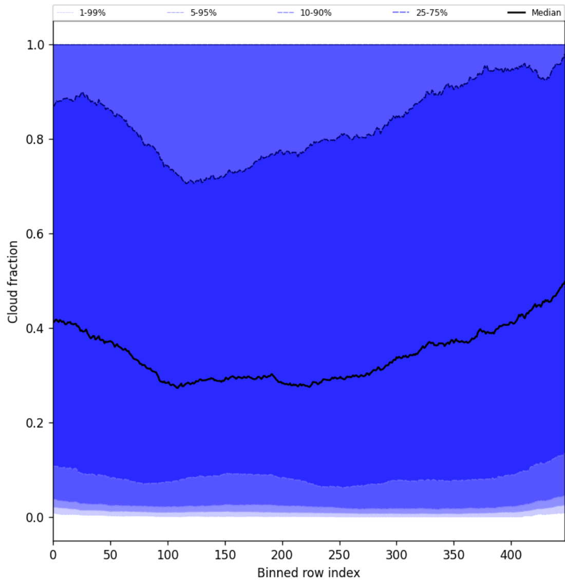
Figure 49: Along track statistics of “Cloud fraction” for 2025-05-23 to 2025-05-25
