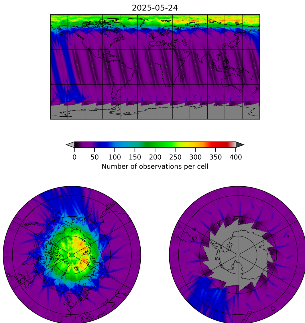
Figure 11: Map of the number of observations for 2025-05-23 to 2025-05-25
