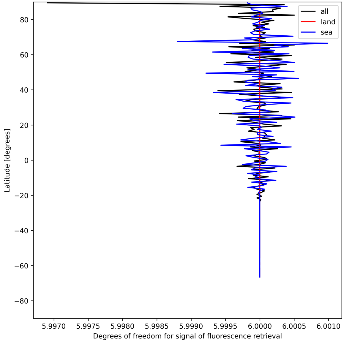
Figure 26: Zonal average of “Degrees of freedom for signal of fluorescence retrieval” for 2025-05-23 to 2025-05-25.
