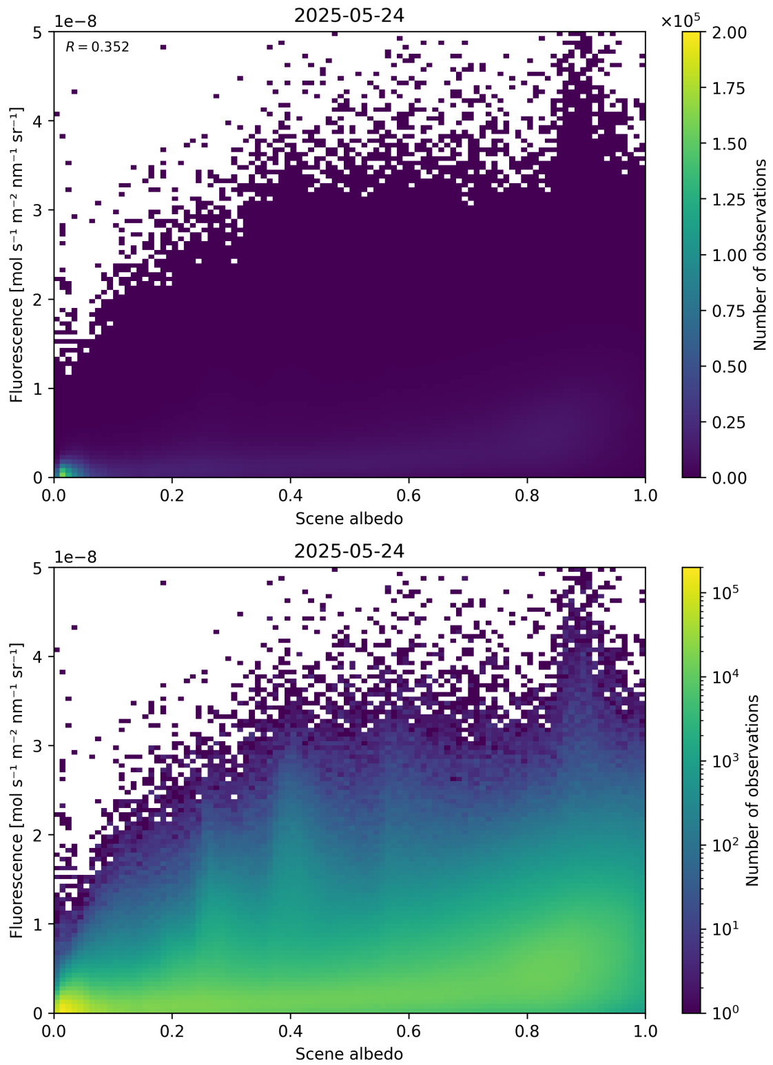
Figure 104: Scatter density plot of “Scene albedo” against “Fluorescence” for 2025-05-23 to 2025-05-25.
