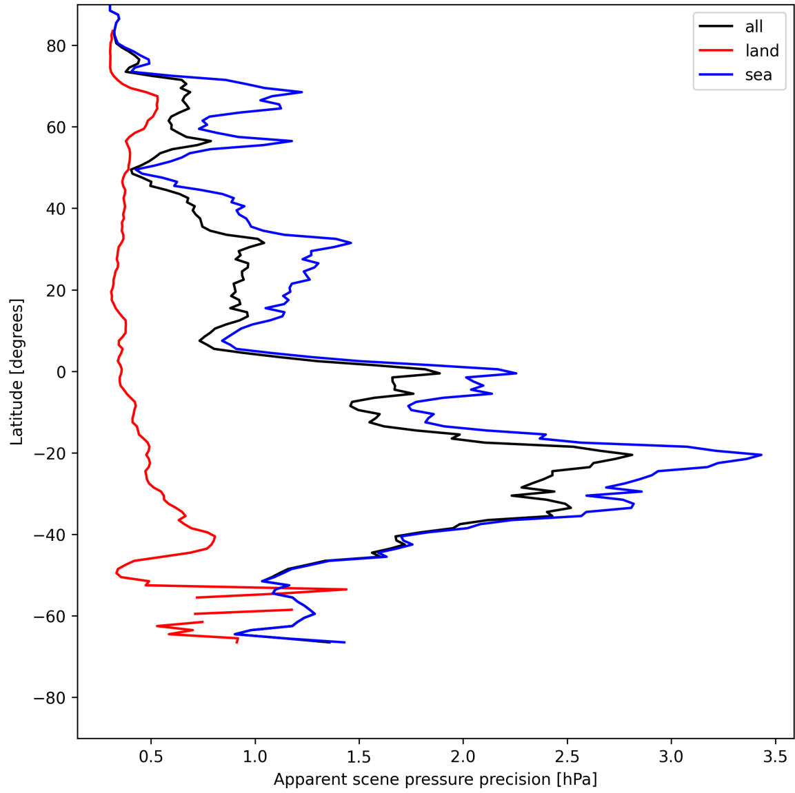
Figure 20: Zonal average of “Apparent scene pressure precision” for 2025-05-23 to 2025-05-25.
