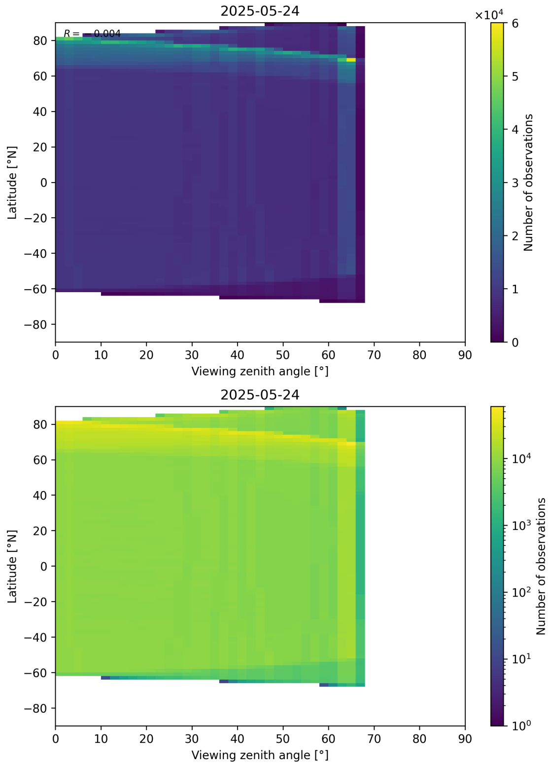
Figure 123: Scatter density plot of “Viewing zenith angle” against “Latitude” for 2025-05-23 to 2025-05-25.
