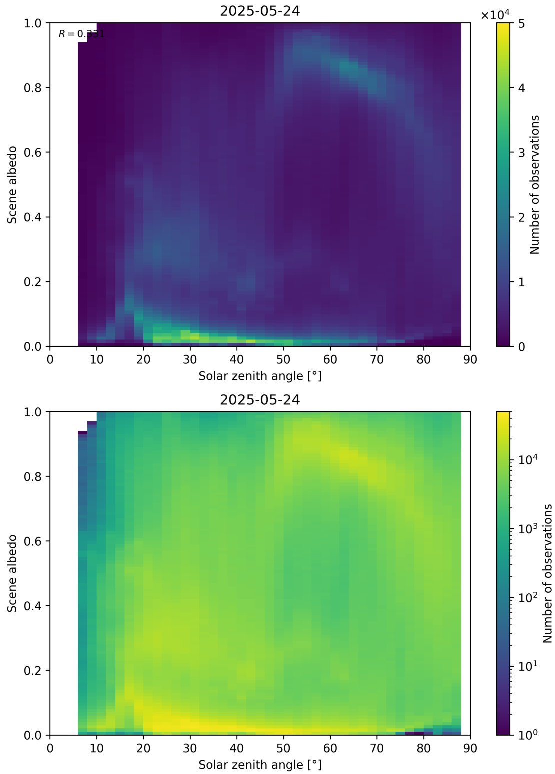
Figure 116: Scatter density plot of “Solar zenith angle” against “Scene albedo” for 2025-05-23 to 2025-05-25.
