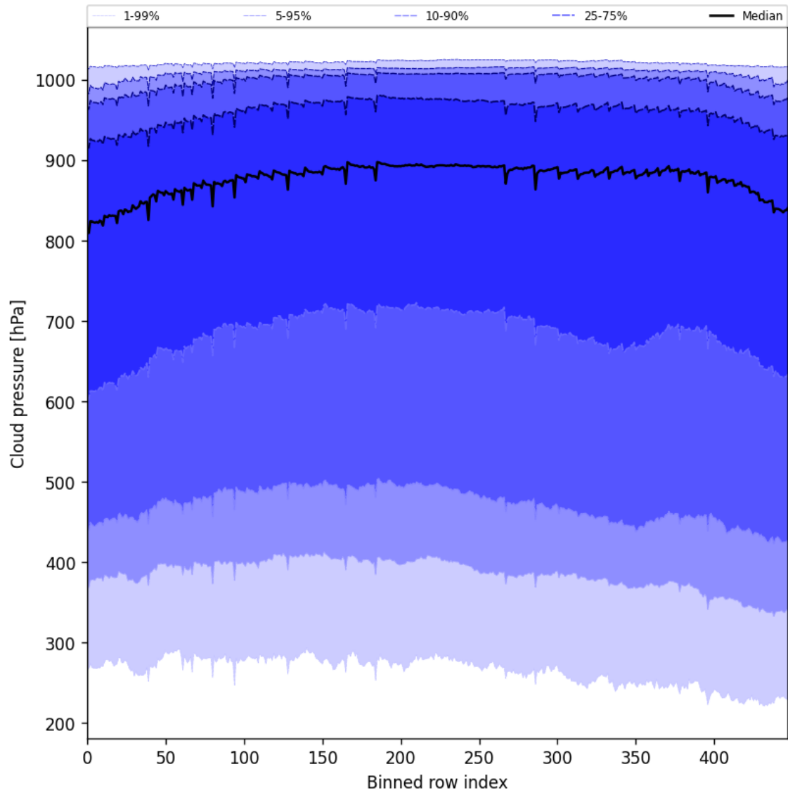
Figure 47: Along track statistics of “Cloud pressure” for 2025-05-23 to 2025-05-25
