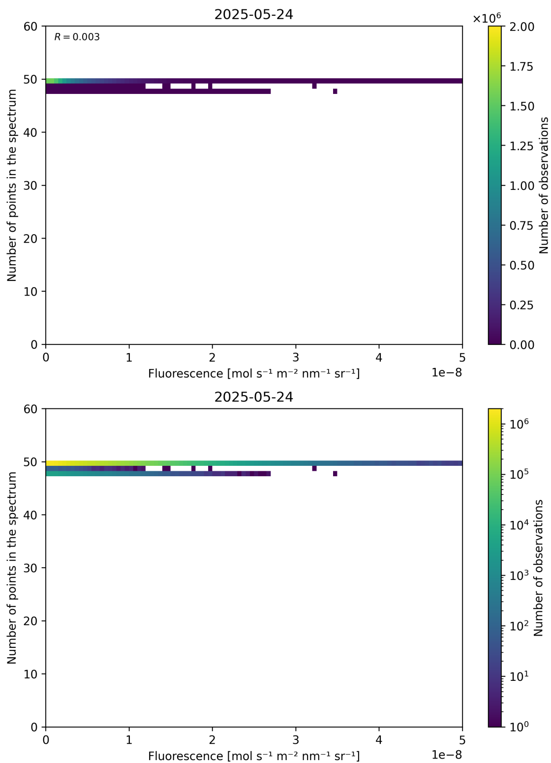
Figure 86: Scatter density plot of “Fluorescence” against “Number of points in the spectrum” for 2025-05-23 to 2025-05-25.
