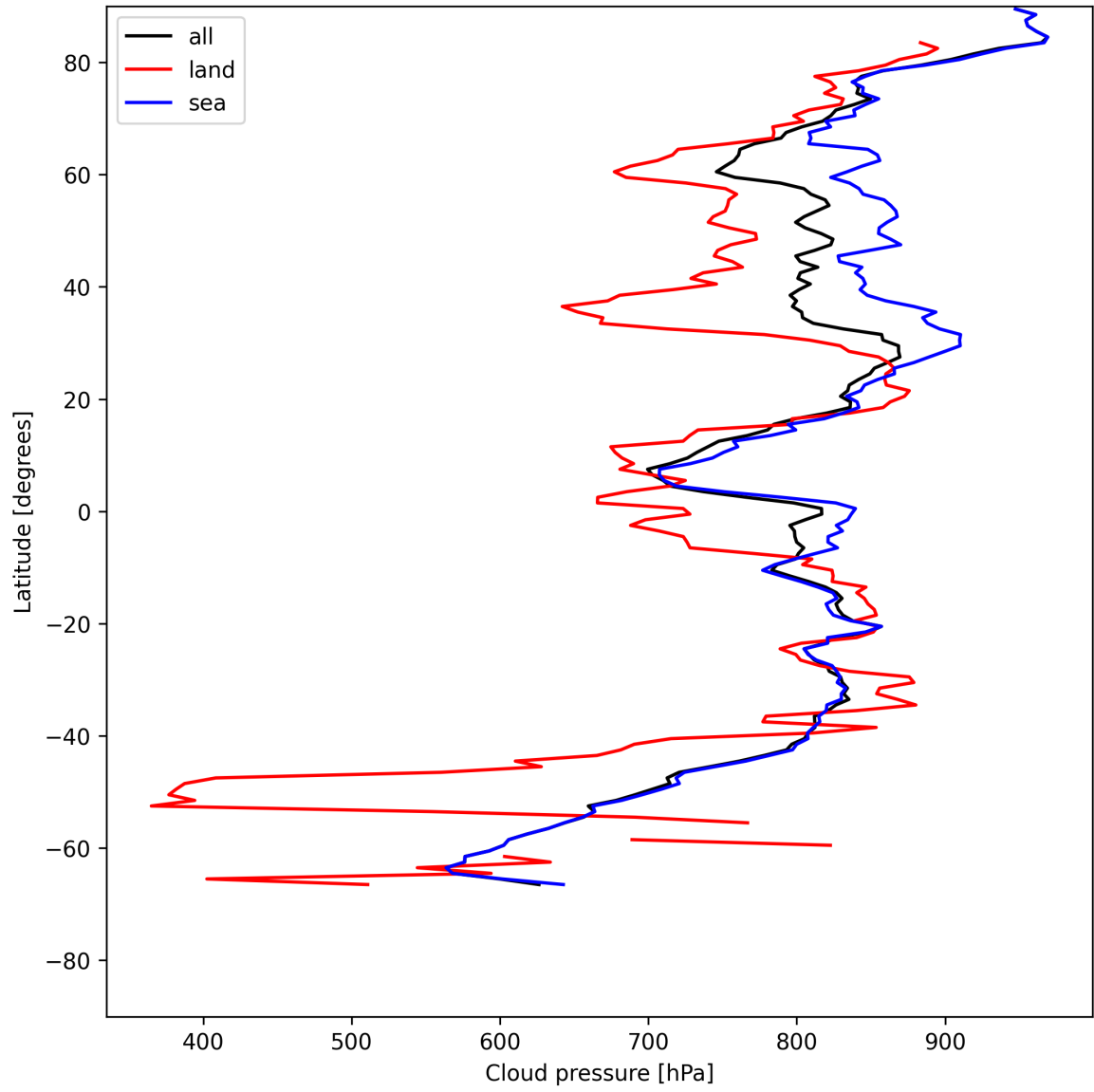
Figure 13: Zonal average of “Cloud pressure” for 2025-05-23 to 2025-05-25.
