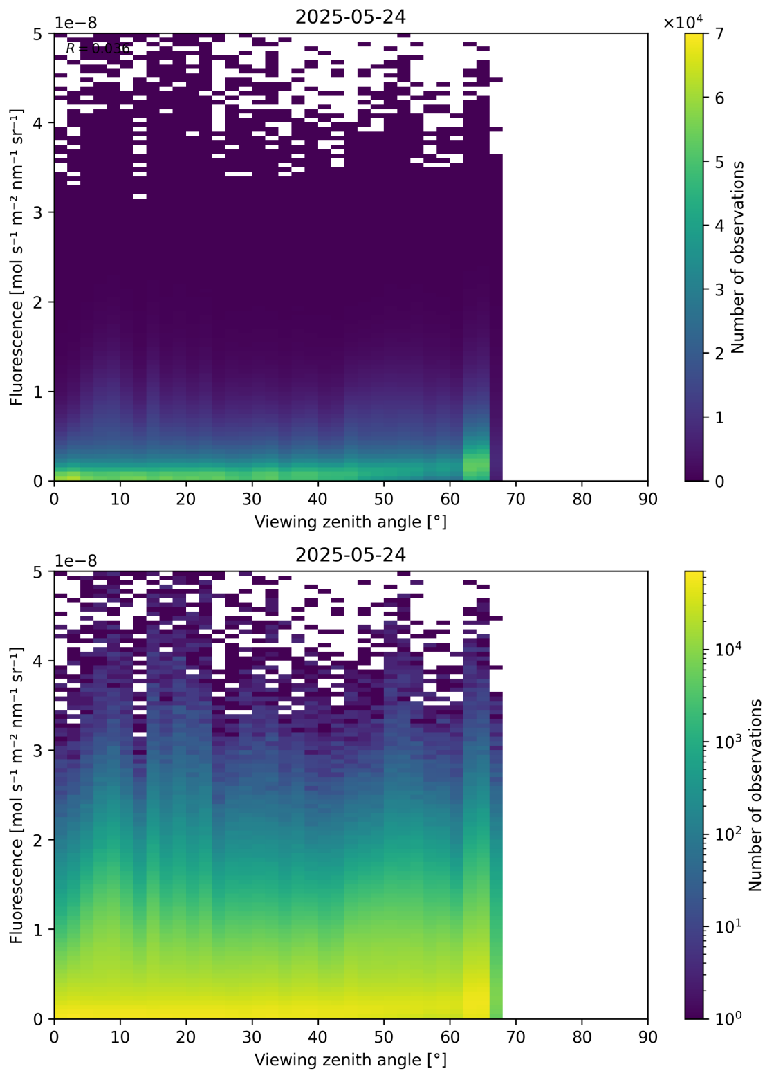
Figure 122: Scatter density plot of “Viewing zenith angle” against “Fluorescence” for 2025-05-23 to 2025-05-25.
