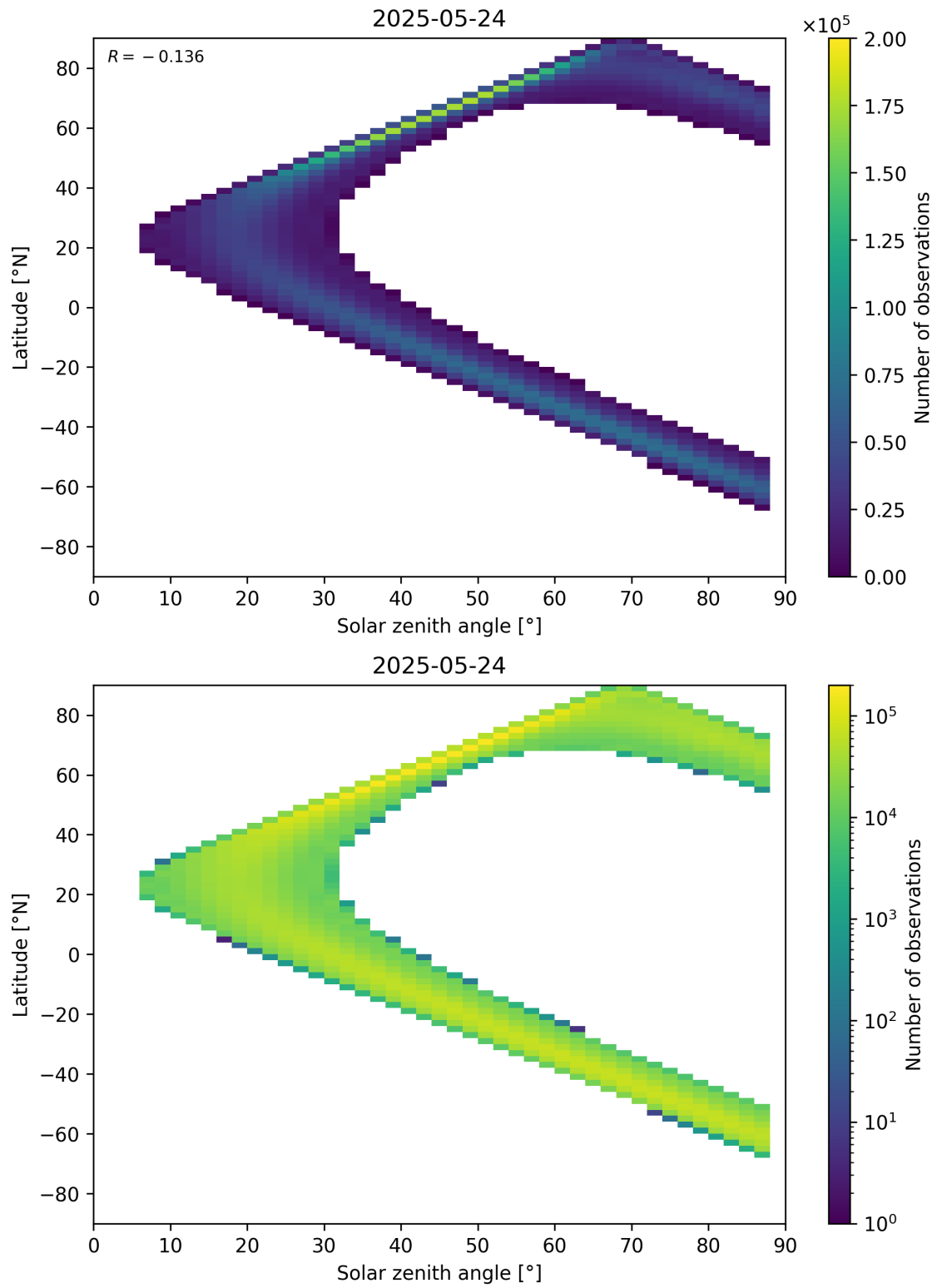
Figure 113: Scatter density plot of “Solar zenith angle” against “Latitude” for 2025-05-23 to 2025-05-25.
