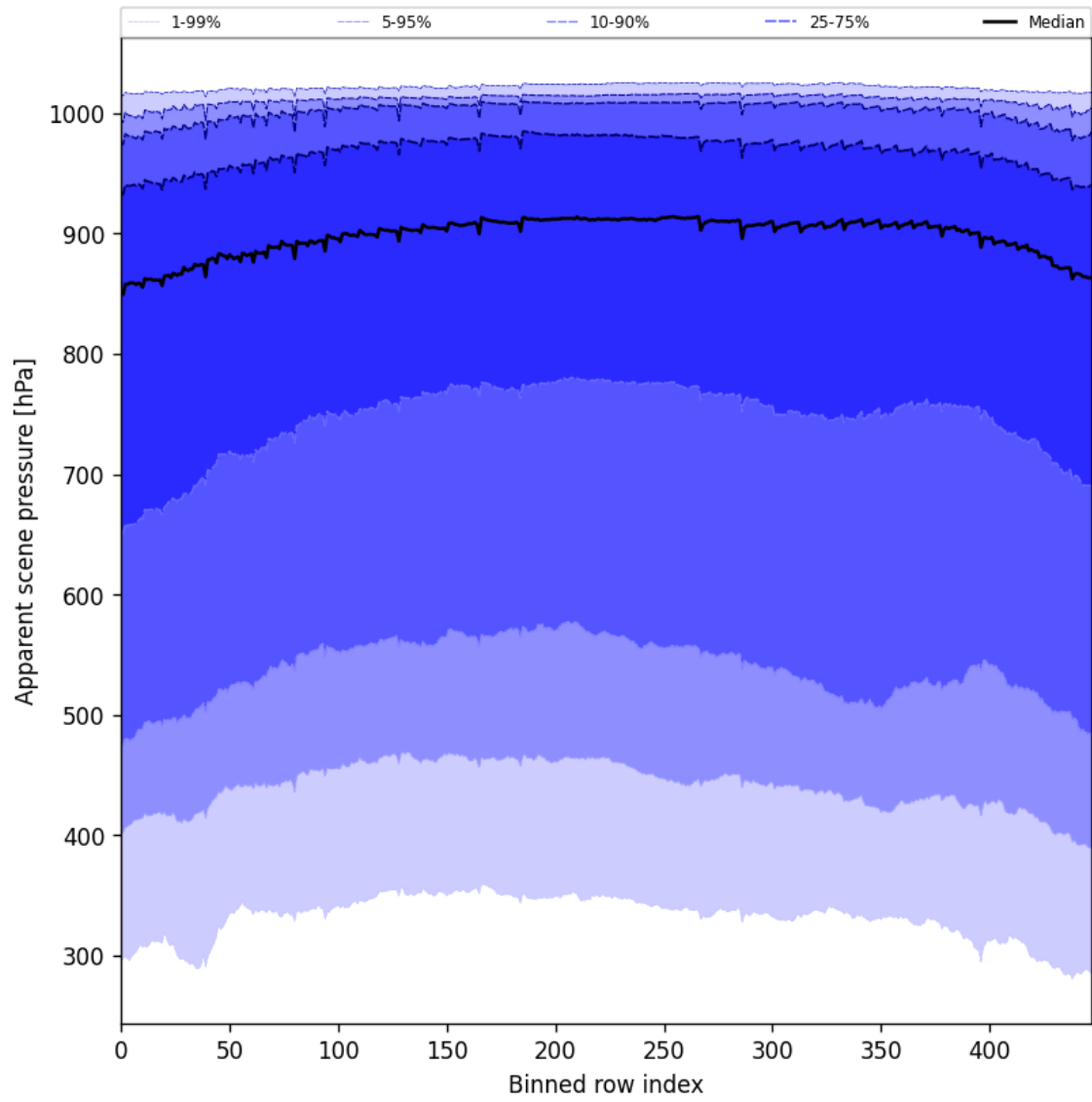
Figure 53: Along track statistics of “Apparent scene pressure” for 2025-05-23 to 2025-05-25
