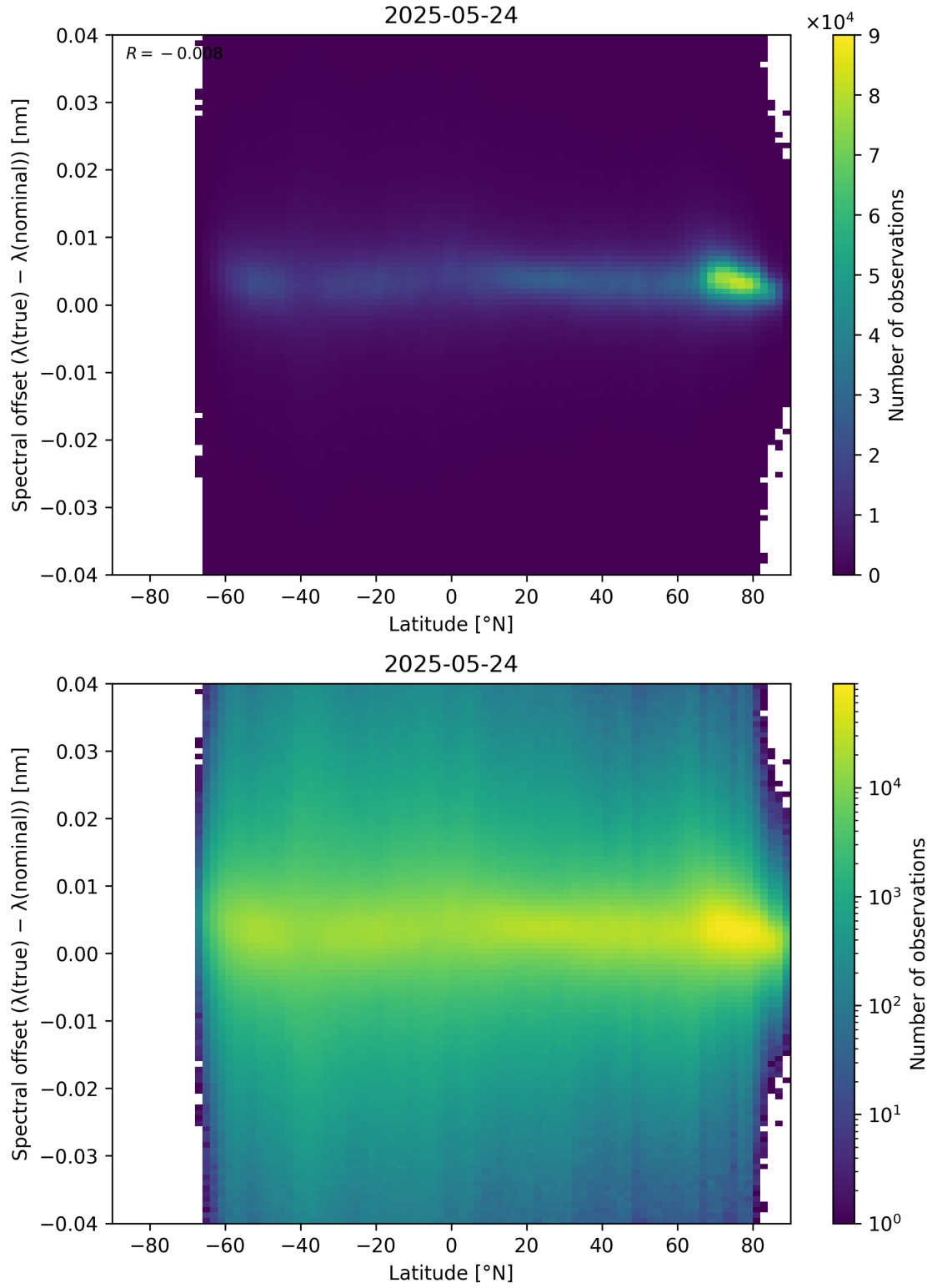
Figure 96: Scatter density plot of “Latitude” against “Spectral offset ( \lambda_{\text{true}} - \lambda_{\text{nominal}} )” for 2025-05-23 to 2025-05-25.
