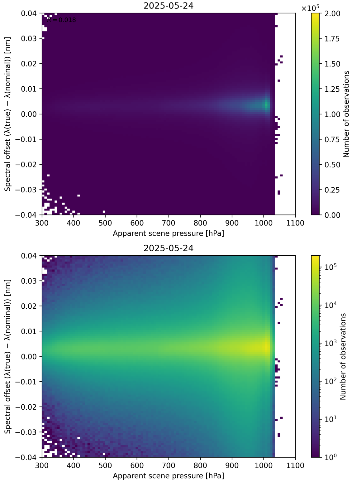
Figure 67: Scatter density plot of “Apparent scene pressure” against “Spectral offset ( \lambda_{\text{true}} - \lambda_{\text{nominal}} )” for 2025-05-23 to 2025-05-25.
