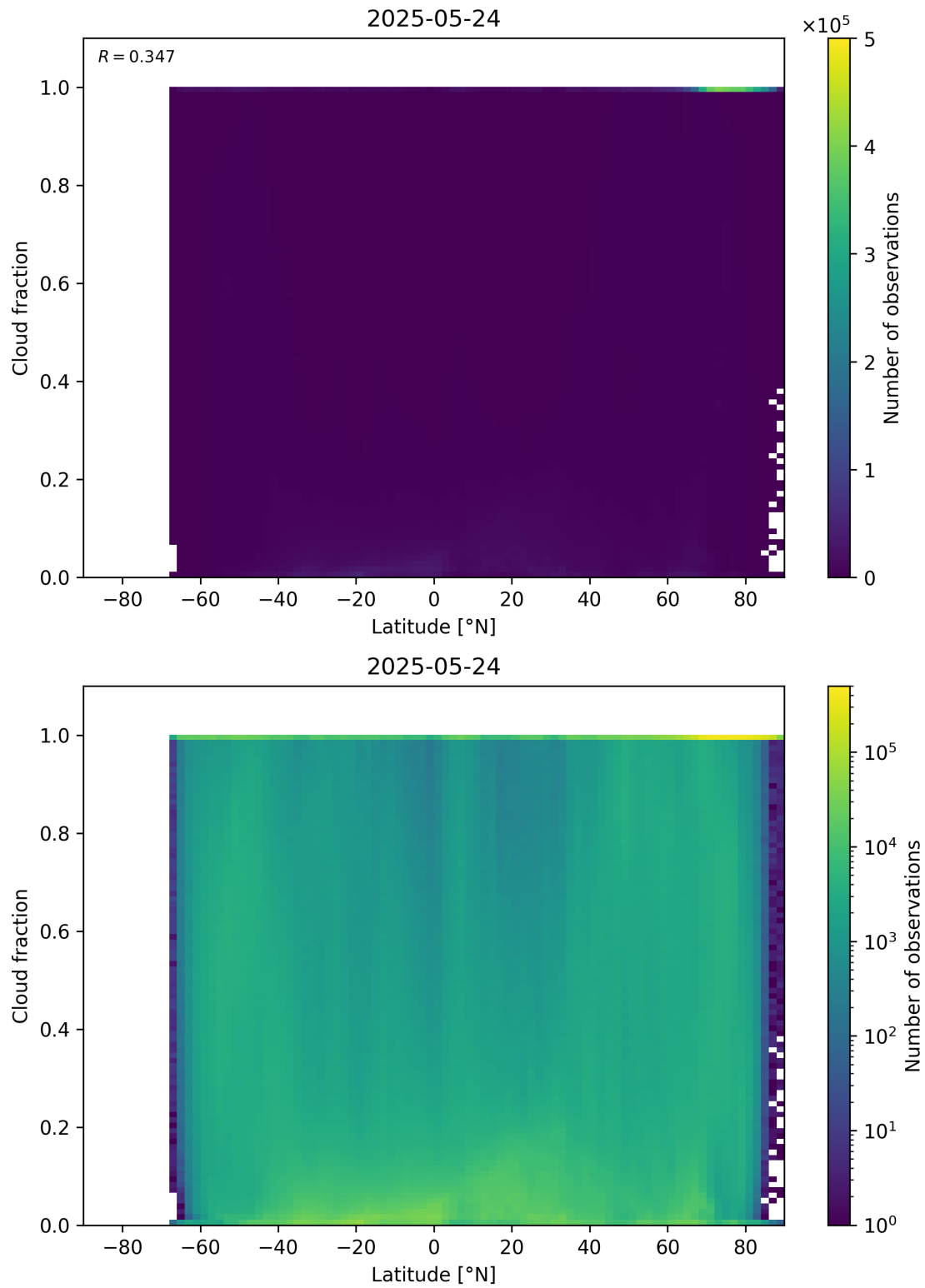
Figure 90: Scatter density plot of “Latitude” against “Cloud fraction” for 2025-05-23 to 2025-05-25.
