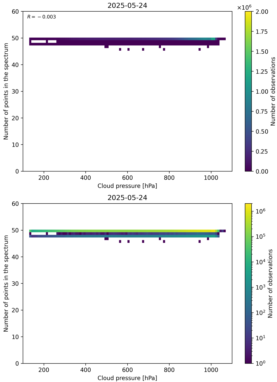
Figure 82: Scatter density plot of “Cloud pressure” against “Number of points in the spectrum” for 2025-05-23 to 2025-05-25.
