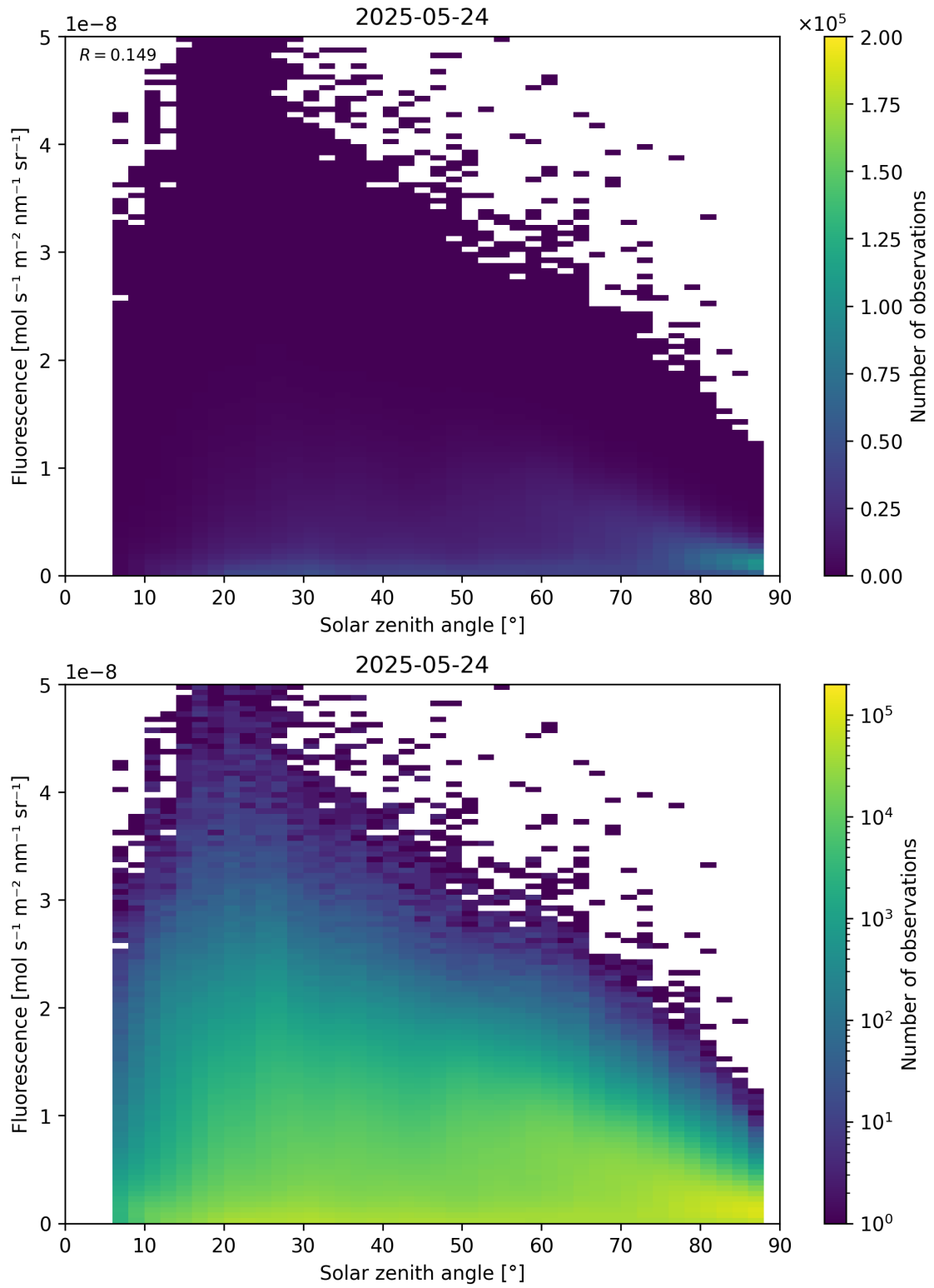
Figure 112: Scatter density plot of “Solar zenith angle” against “Fluorescence” for 2025-05-23 to 2025-05-25.
