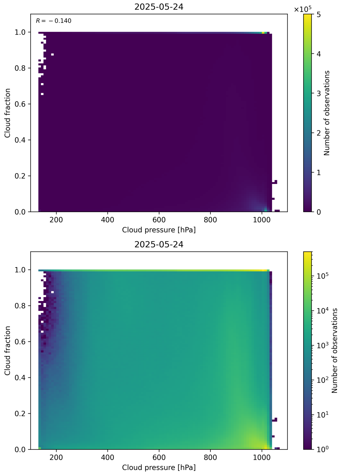
Figure 79: Scatter density plot of “Cloud pressure” against “Cloud fraction” for 2025-05-23 to 2025-05-25.
