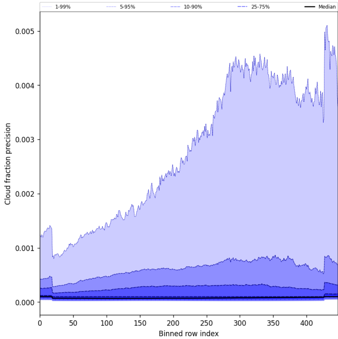
Figure 50: Along track statistics of “Cloud fraction precision” for 2025-05-23 to 2025-05-25
