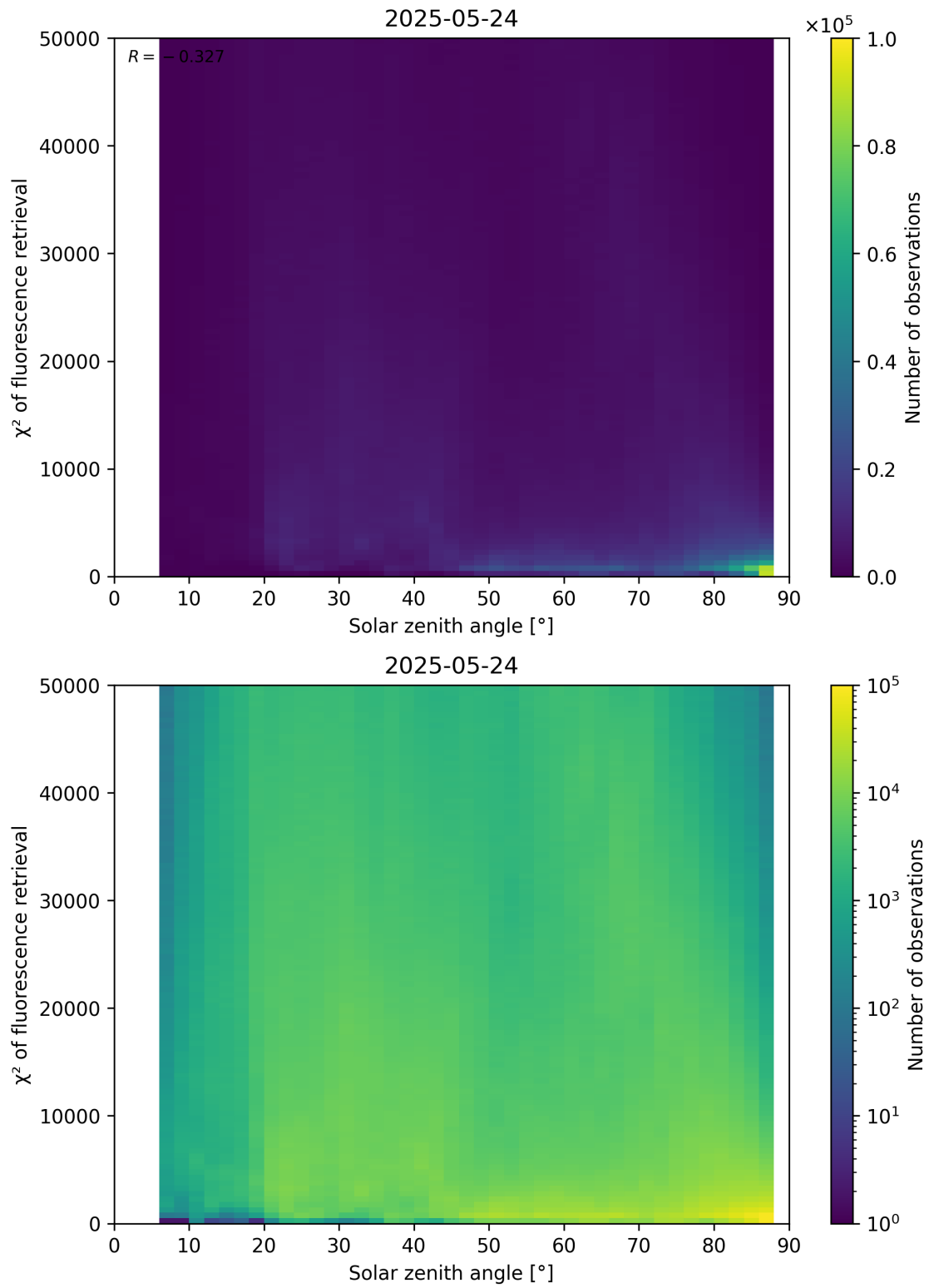
Figure 109: Scatter density plot of “Solar zenith angle” against “ \chi^2 of fluorescence retrieval” for 2025-05-23 to 2025-05-25.
