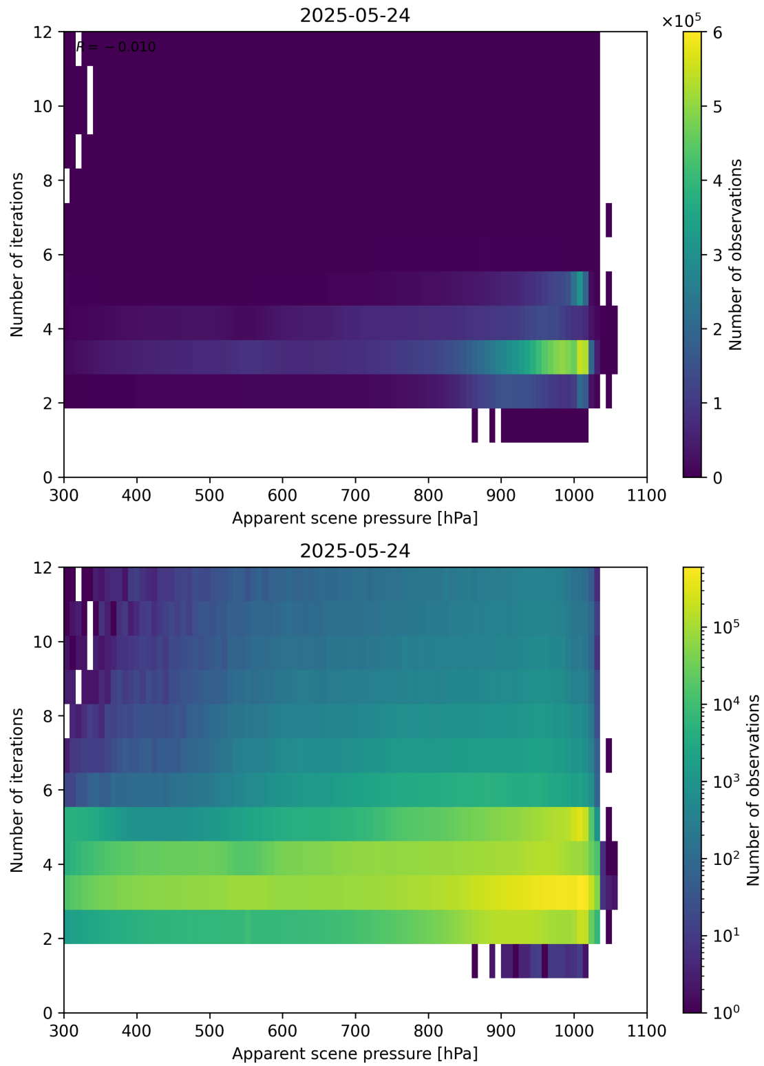
Figure 65: Scatter density plot of “Apparent scene pressure” against “Number of iterations” for 2025-05-23 to 2025-05-25.
