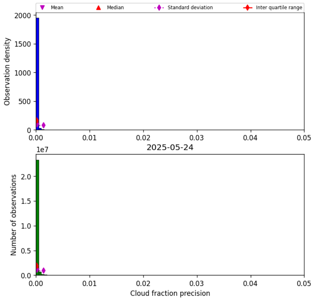
Figure 33: Histogram of “Cloud fraction precision” for 2025-05-23 to 2025-05-25
