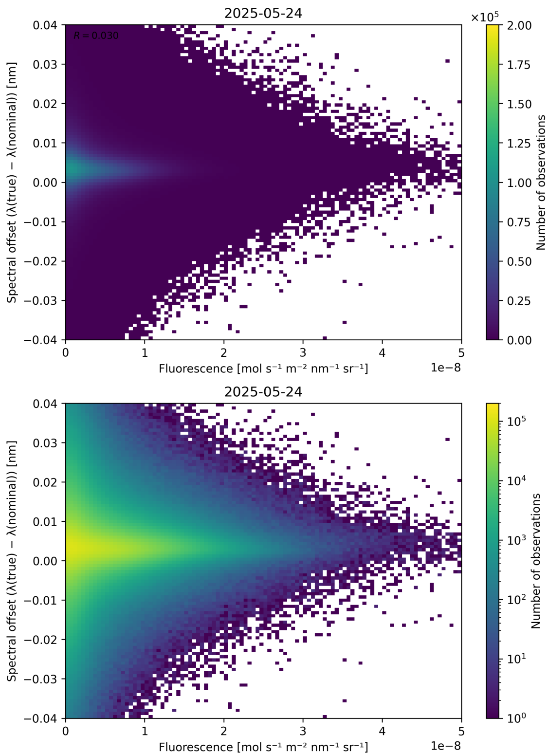
Figure 87: Scatter density plot of “Fluorescence” against “Spectral offset ( \lambda_{\text{true}} - \lambda_{\text{nominal}} )” for 2025-05-23 to 2025-05-25.
