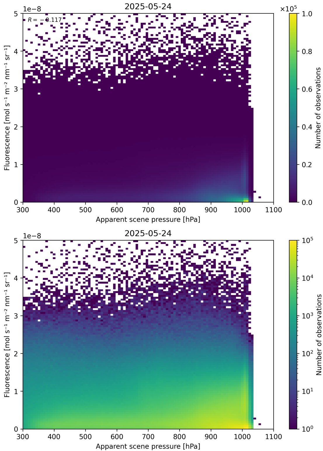
Figure 64: Scatter density plot of “Apparent scene pressure” against “Fluorescence” for 2025-05-23 to 2025-05-25.
