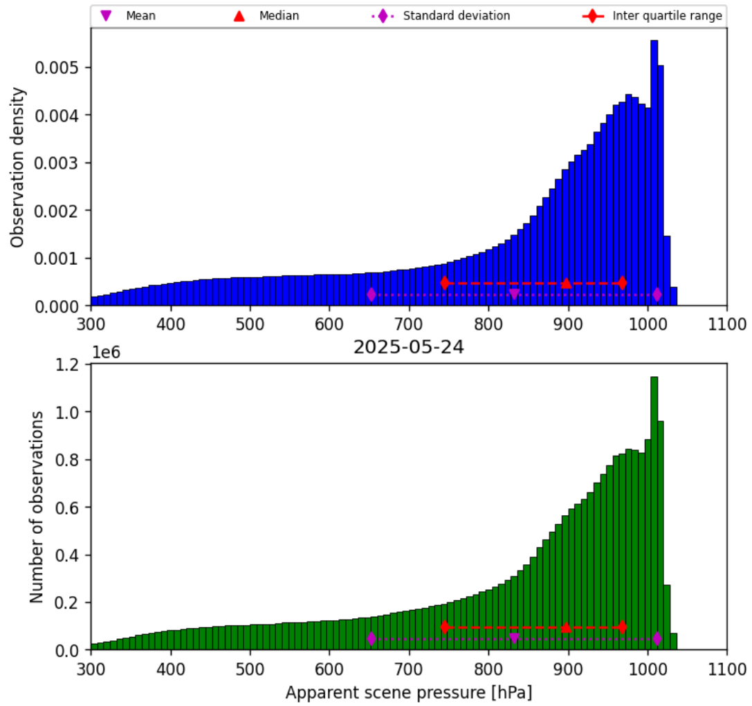
Figure 36: Histogram of “Apparent scene pressure” for 2025-05-23 to 2025-05-25
