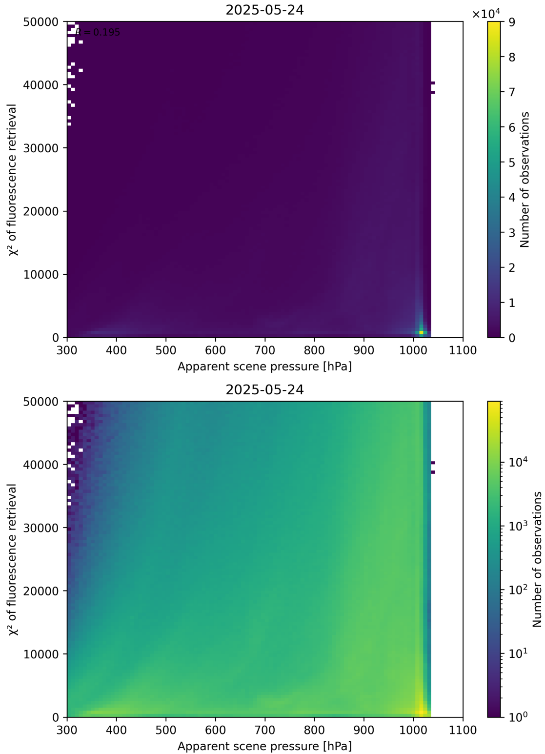
Figure 63: Scatter density plot of “Apparent scene pressure” against “ \chi^2 of fluorescence retrieval” for 2025-05-23 to 2025-05-25.
