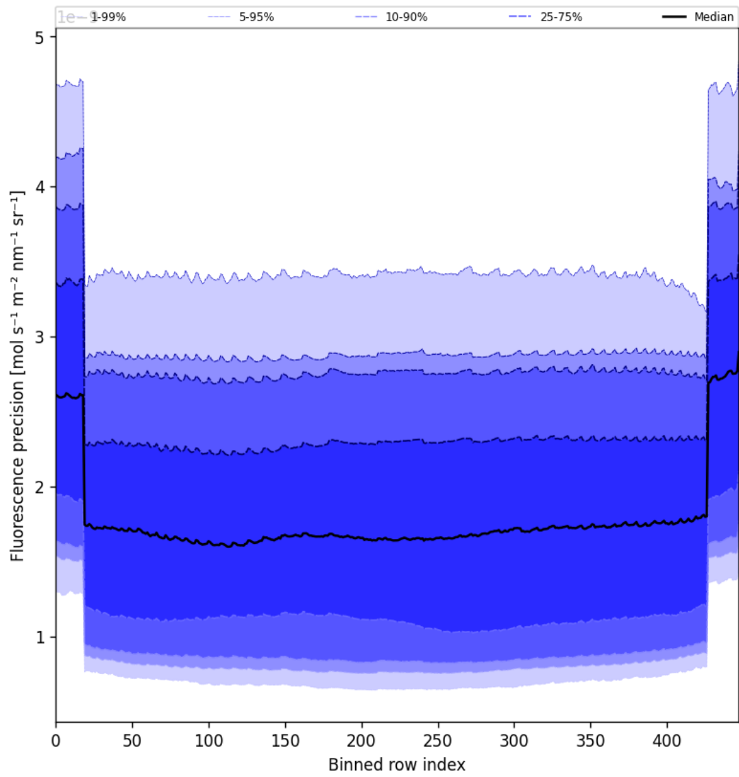
Figure 58: Along track statistics of “Fluorescence precision” for 2025-05-23 to 2025-05-25
