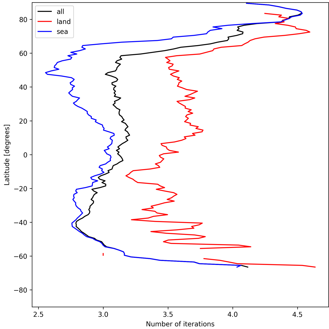
Figure 22: Zonal average of “Number of iterations” for 2025-05-23 to 2025-05-25.
