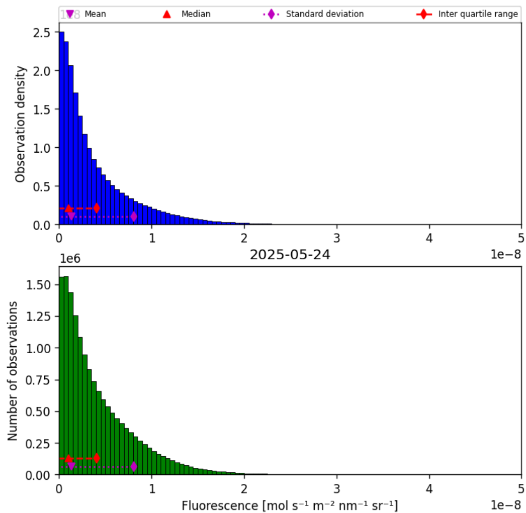
Figure 40: Histogram of “Fluorescence” for 2025-05-23 to 2025-05-25
