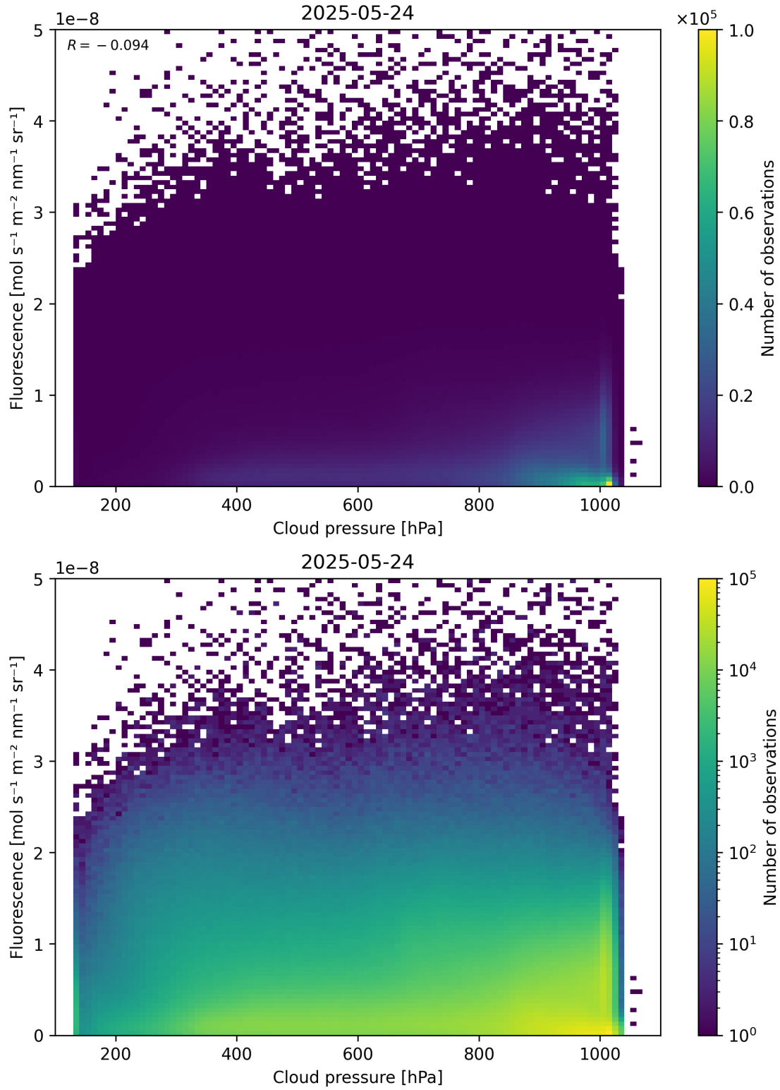
Figure 80: Scatter density plot of “Cloud pressure” against “Fluorescence” for 2025-05-23 to 2025-05-25.
