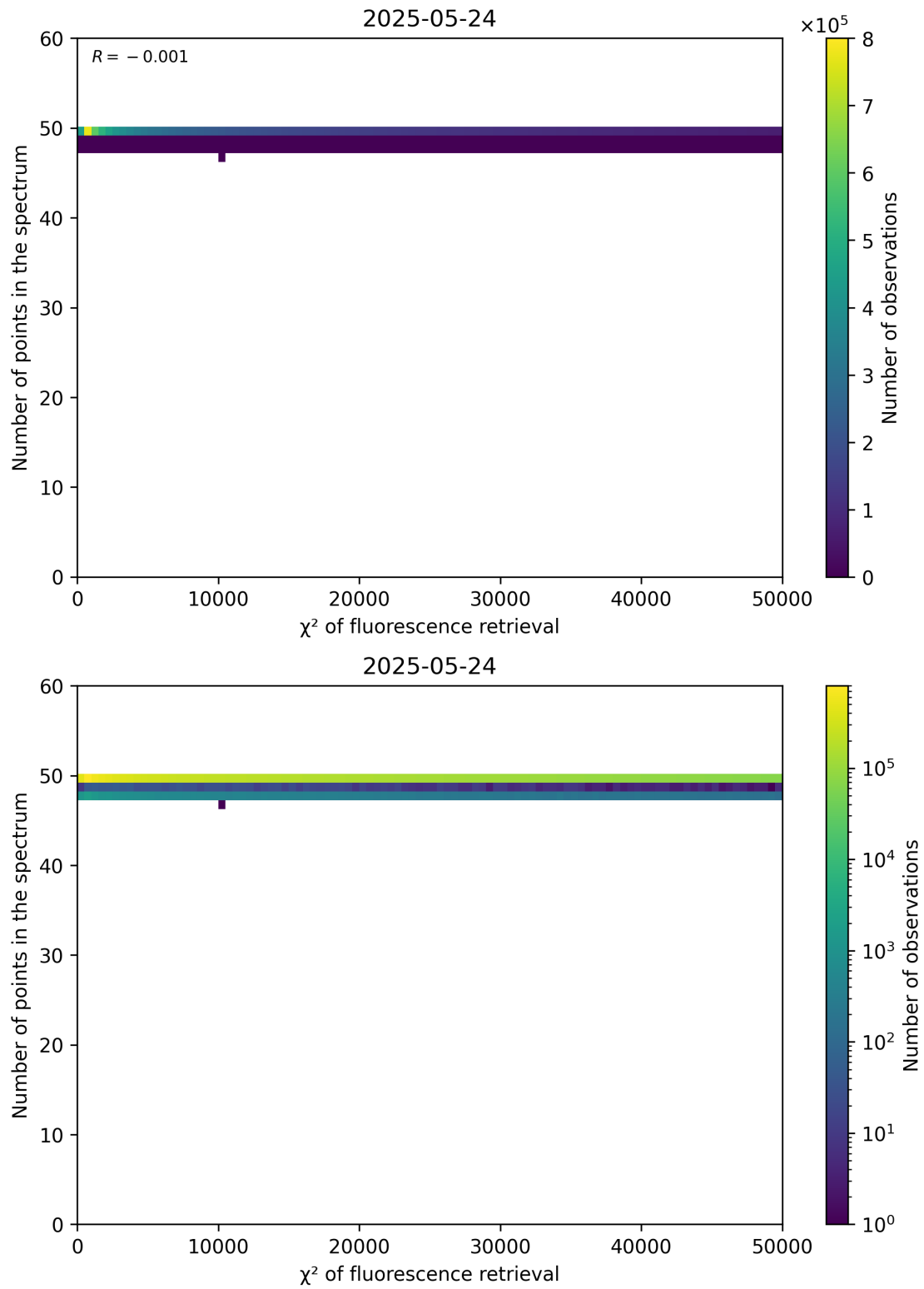
Figure 68: Scatter density plot of “ \chi^2 of fluorescence retrieval” against “Number of points in the spectrum” for 2025-05-23 to 2025-05-25.
