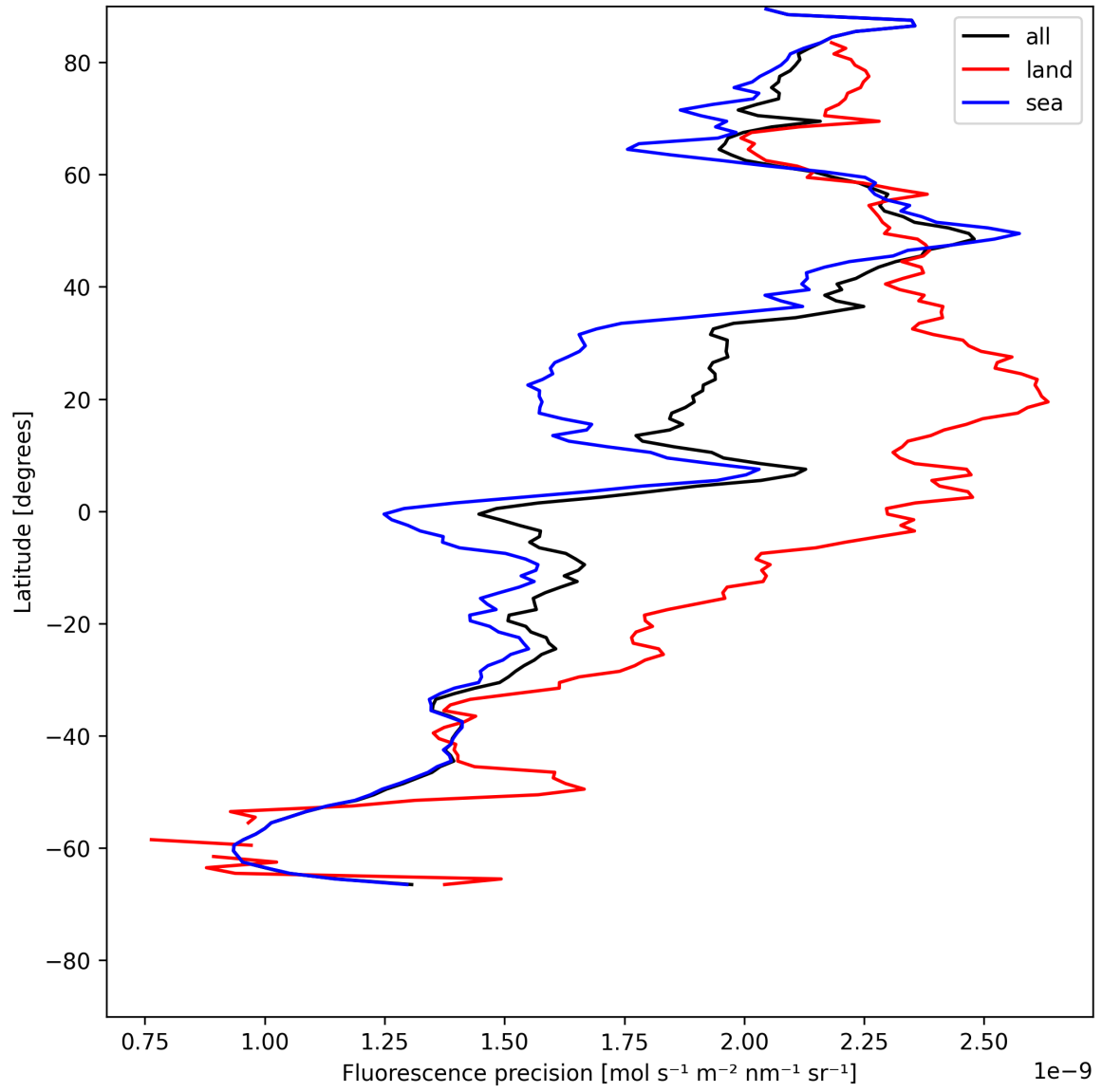
Figure 24: Zonal average of “Fluorescence precision” for 2025-05-23 to 2025-05-25.
