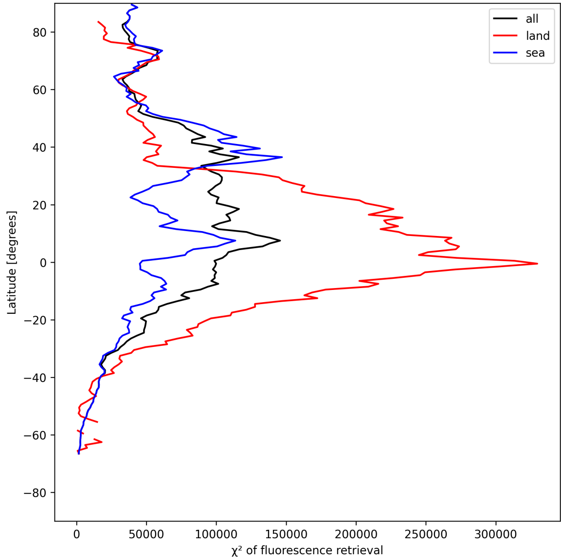
Figure 25: Zonal average of “ \chi^2 of fluorescence retrieval” for 2025-05-23 to 2025-05-25.
