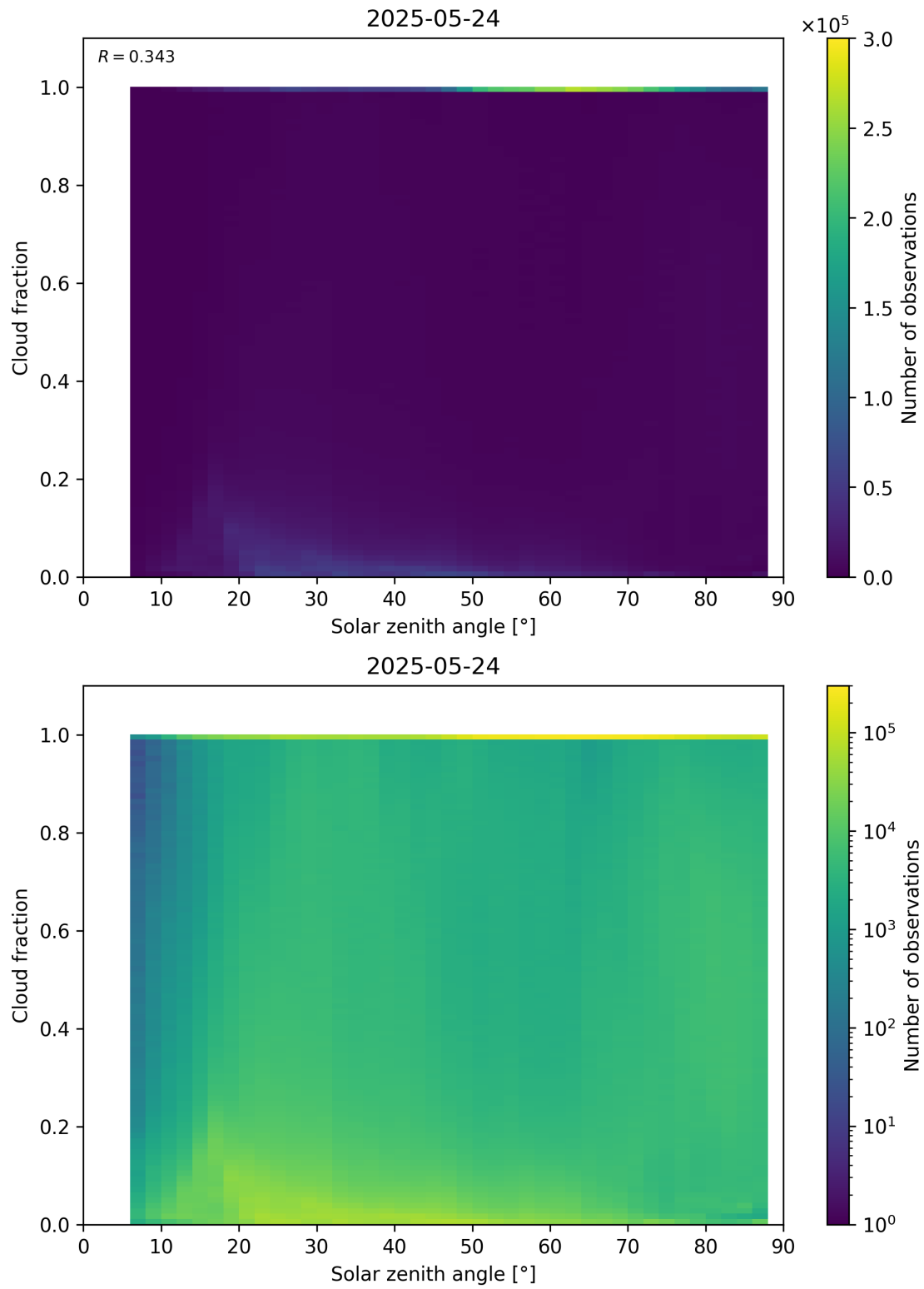
Figure 110: Scatter density plot of “Solar zenith angle” against “Cloud fraction” for 2025-05-23 to 2025-05-25.
