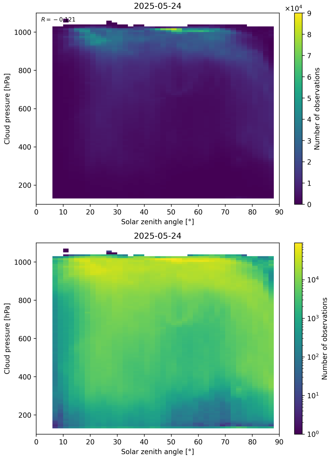
Figure 111: Scatter density plot of “Solar zenith angle” against “Cloud pressure” for 2025-05-23 to 2025-05-25.
