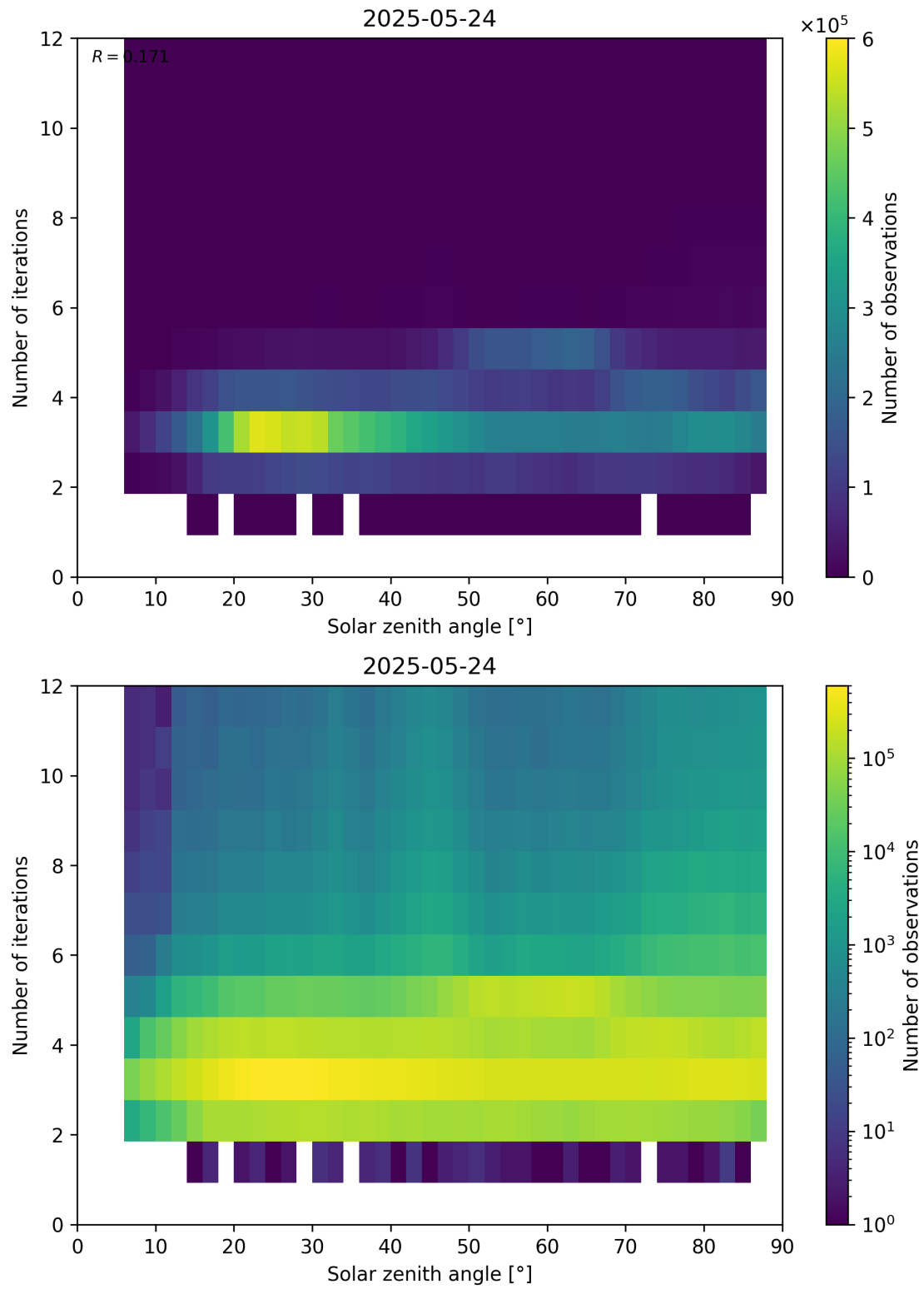
Figure 114: Scatter density plot of “Solar zenith angle” against “Number of iterations” for 2025-05-23 to 2025-05-25.
