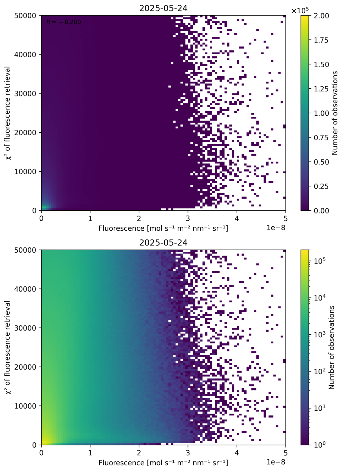
Figure 85: Scatter density plot of “Fluorescence” against “ \chi^2 of fluorescence retrieval” for 2025-05-23 to 2025-05-25.
