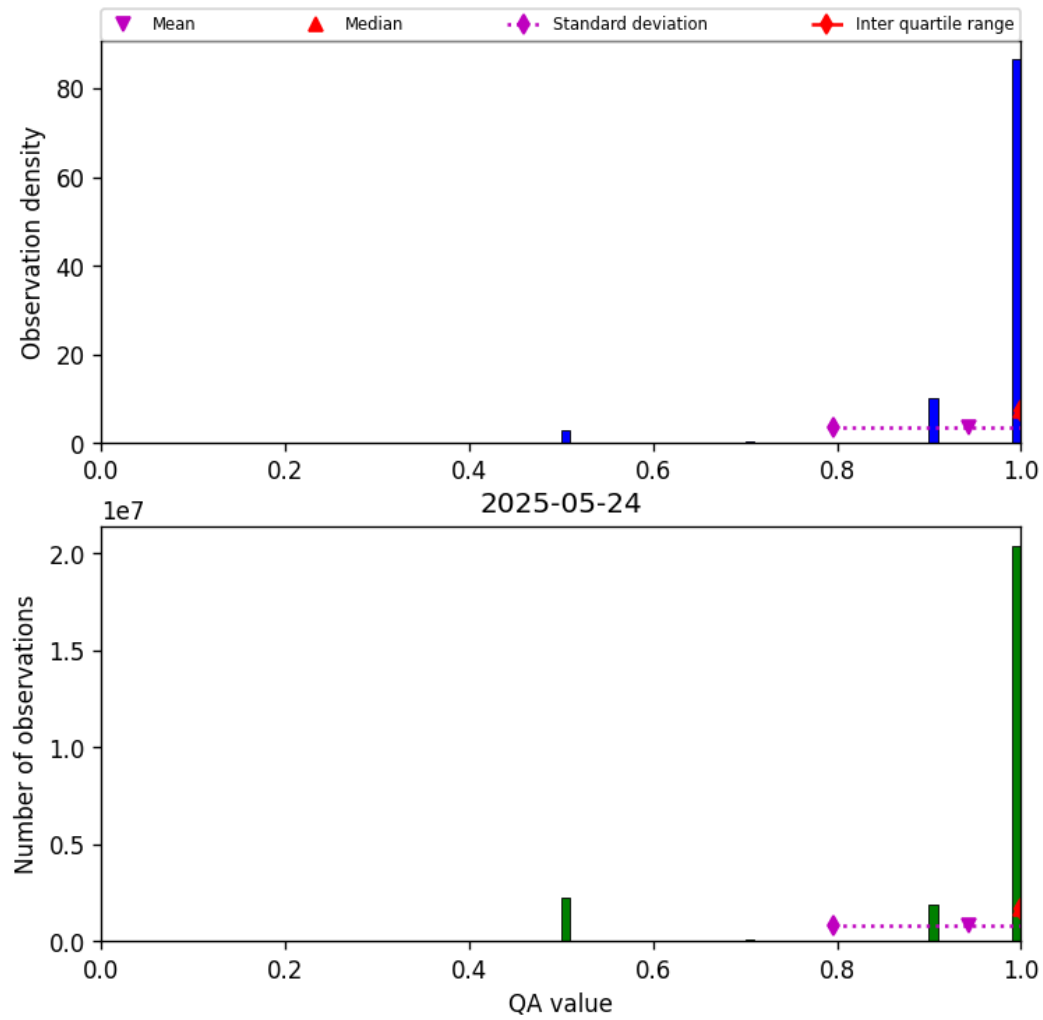
Figure 29: Histogram of “QA value” for 2025-05-23 to 2025-05-25
