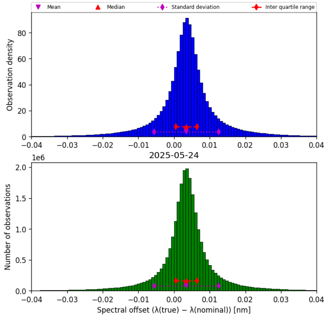
Figure 45: Histogram of “Spectral offset ( \lambda_{\text{true}} - \lambda_{\text{nominal}} )” for 2025-05-23 to 2025-05-25
