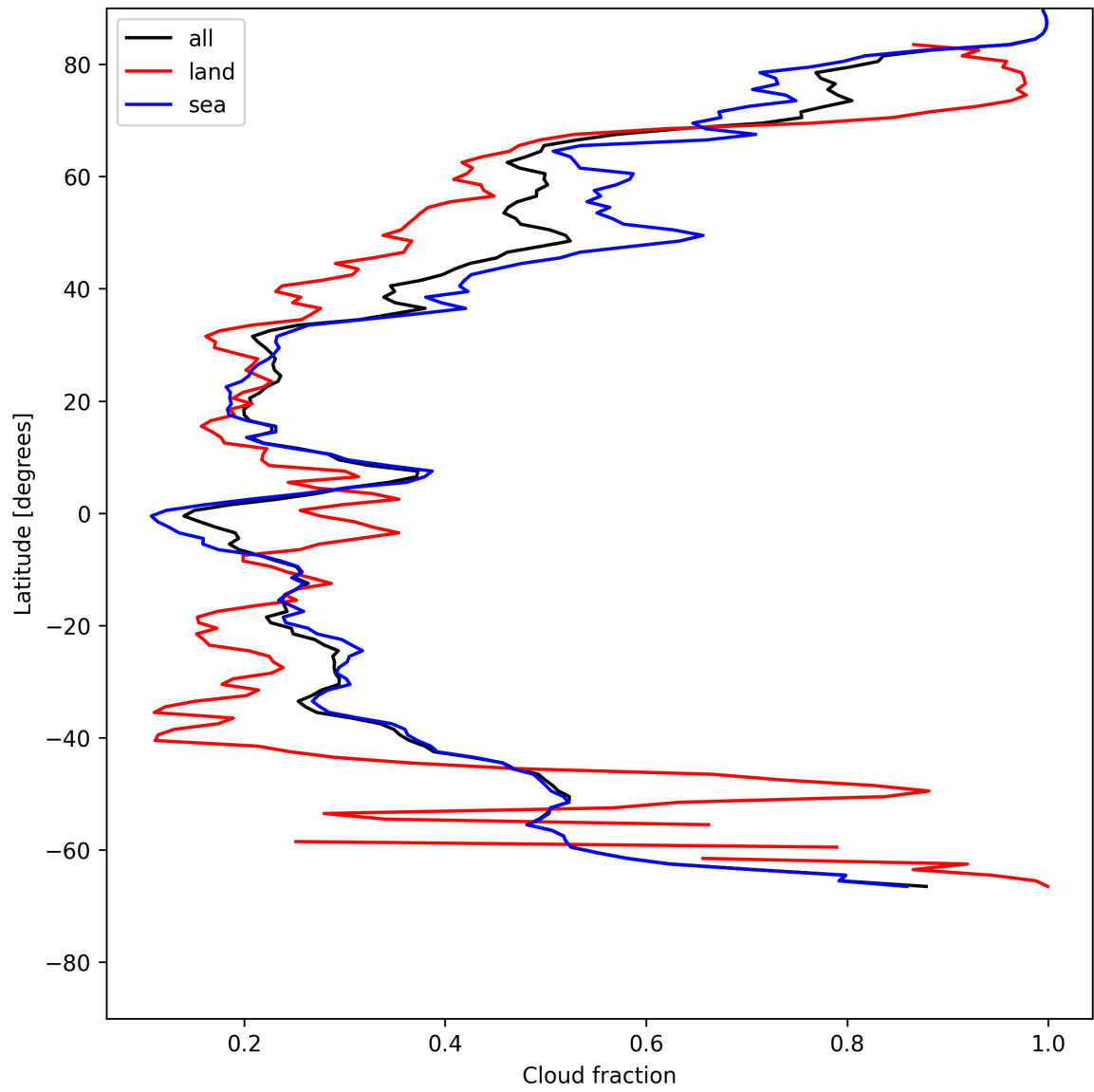
Figure 15: Zonal average of “Cloud fraction” for 2025-05-23 to 2025-05-25.
