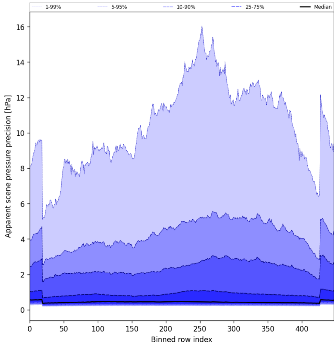
Figure 54: Along track statistics of “Apparent scene pressure precision” for 2025-05-23 to 2025-05-25
