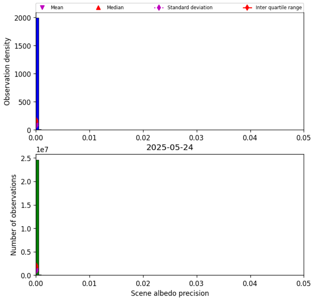
Figure 35: Histogram of “Scene albedo precision” for 2025-05-23 to 2025-05-25
