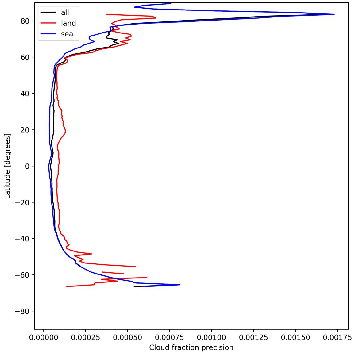
Figure 16: Zonal average of “Cloud fraction precision” for 2025-05-23 to 2025-05-25.
