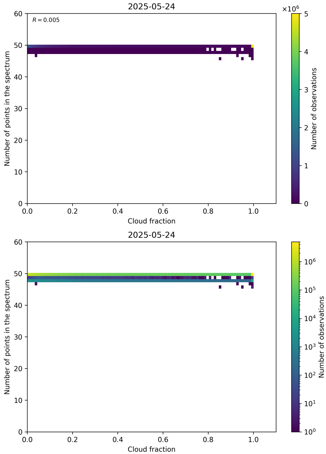
Figure 74: Scatter density plot of “Cloud fraction” against “Number of points in the spectrum” for 2025-05-23 to 2025-05-25.
