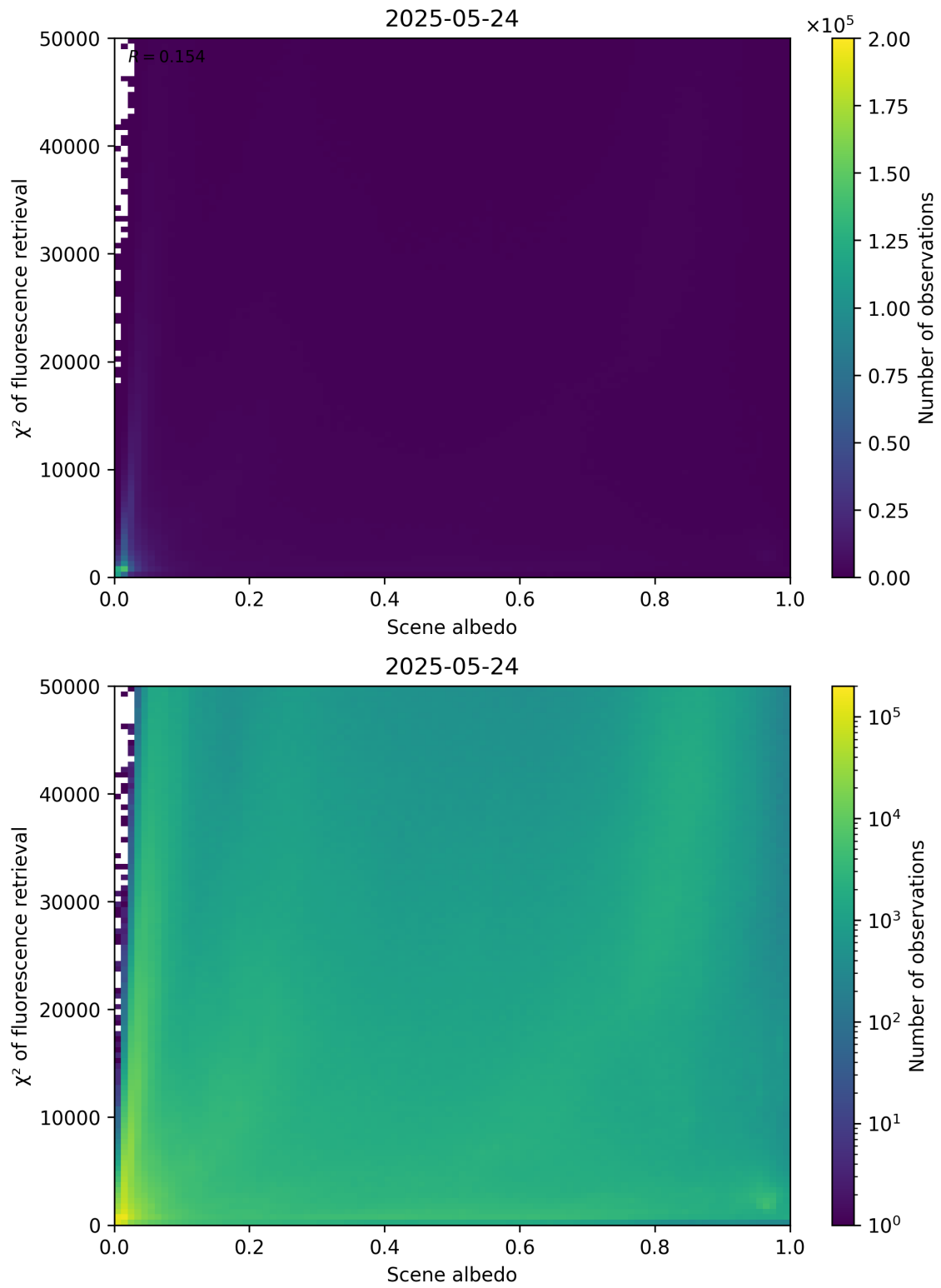
Figure 103: Scatter density plot of “Scene albedo” against “ \chi^2 of fluorescence retrieval” for 2025-05-23 to 2025-05-25.
