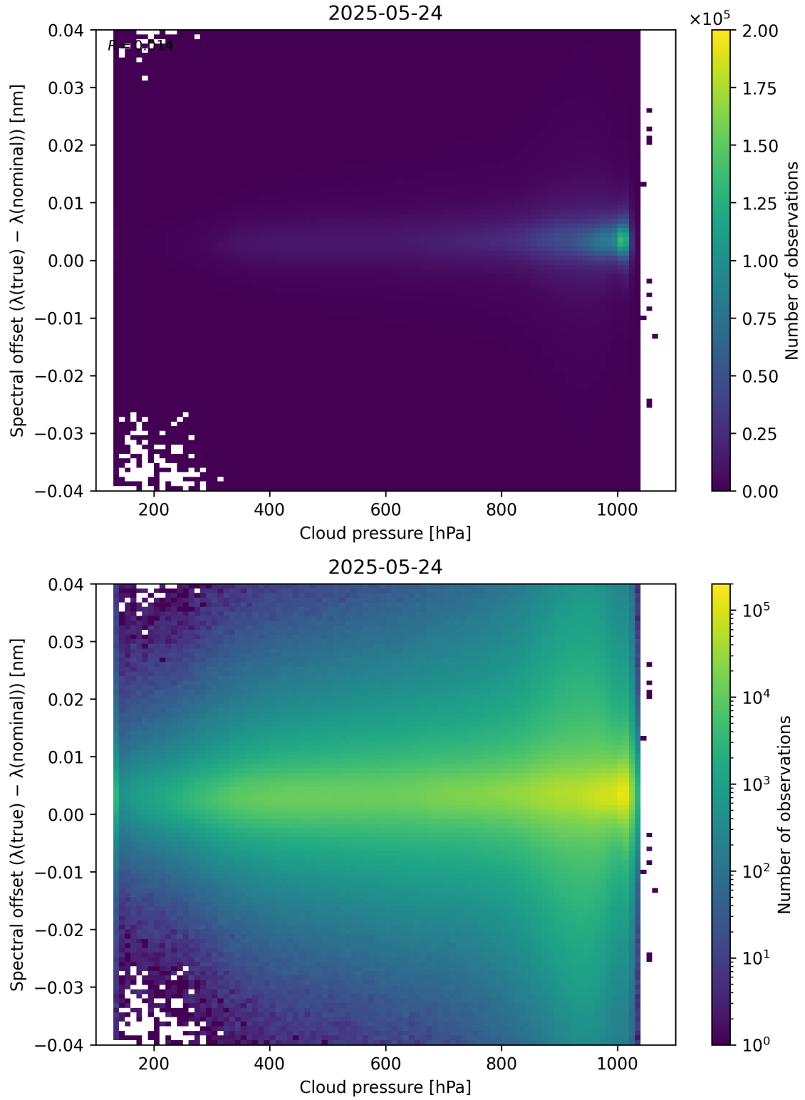
Figure 84: Scatter density plot of “Cloud pressure” against “Spectral offset ( \lambda_{\text{true}} - \lambda_{\text{nominal}} )” for 2025-05-23 to 2025-05-25.
