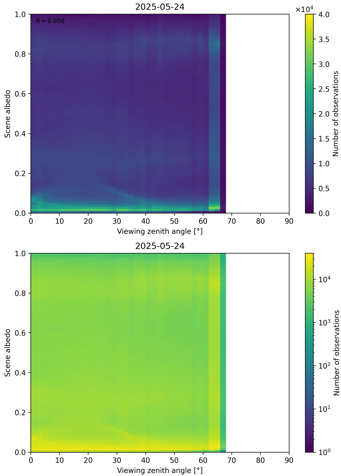
Figure 126: Scatter density plot of “Viewing zenith angle” against “Scene albedo” for 2025-05-23 to 2025-05-25.
