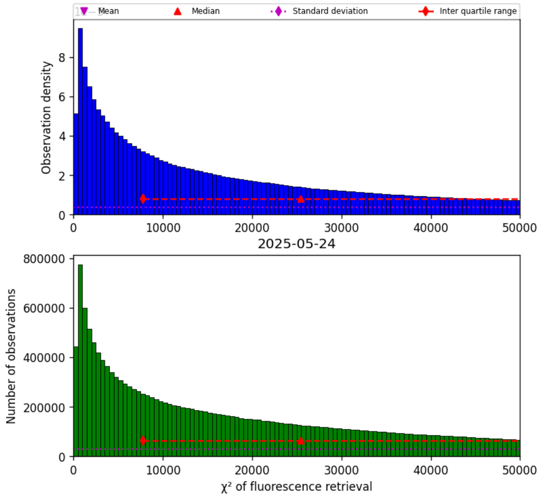
Figure 42: Histogram of “ \chi^2 of fluorescence retrieval” for 2025-05-23 to 2025-05-25
