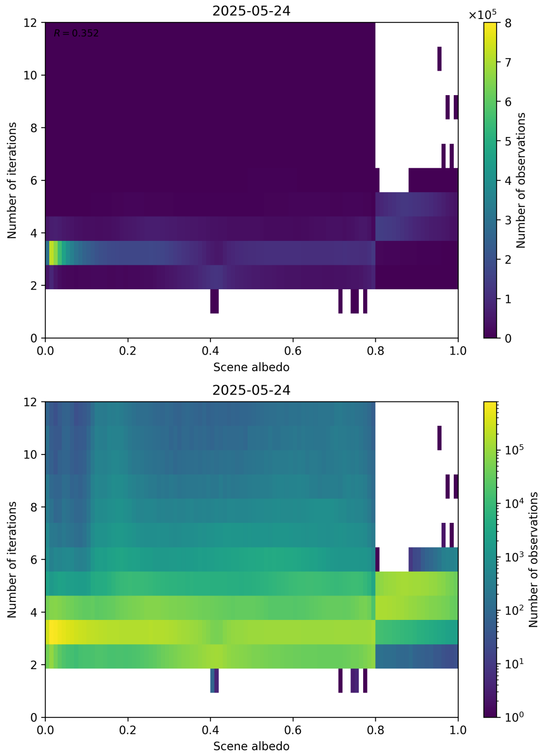
Figure 105: Scatter density plot of “Scene albedo” against “Number of iterations” for 2025-05-23 to 2025-05-25.
