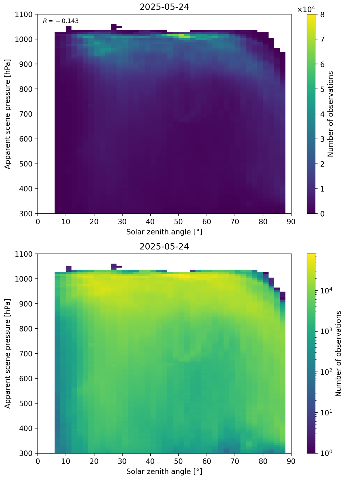
Figure 108: Scatter density plot of “Solar zenith angle” against “Apparent scene pressure” for 2025-05-23 to 2025-05-25.
