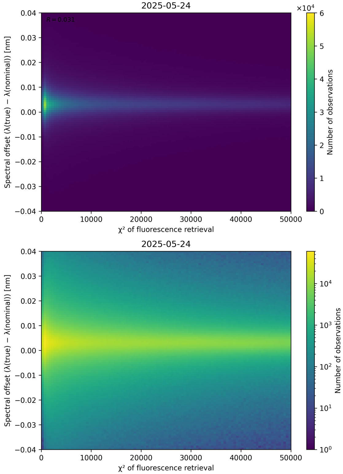
Figure 69: Scatter density plot of “ \chi^2 of fluorescence retrieval” against “Spectral offset ( \lambda_{\text{true}} - \lambda_{\text{nominal}} )” for 2025-05-23 to 2025-05-25.
