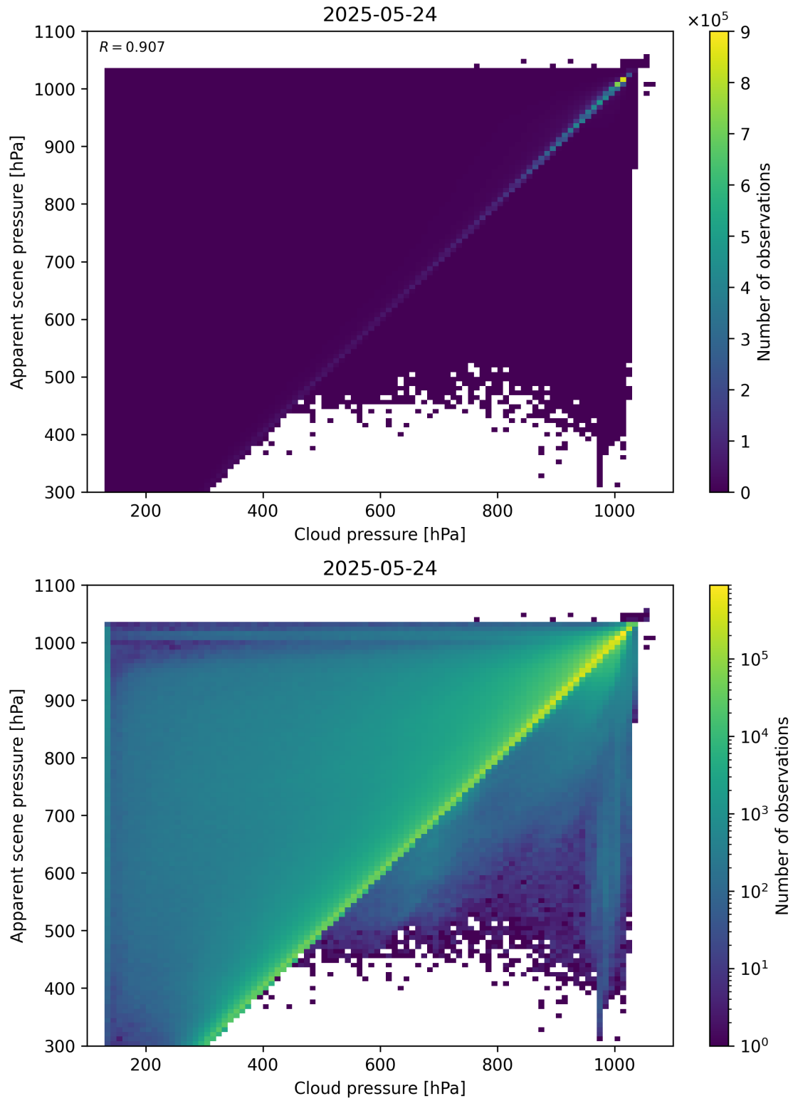
Figure 77: Scatter density plot of “Cloud pressure” against “Apparent scene pressure” for 2025-05-23 to 2025-05-25.
