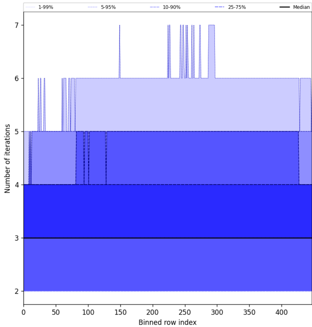
Figure 56: Along track statistics of “Number of iterations” for 2025-05-23 to 2025-05-25
