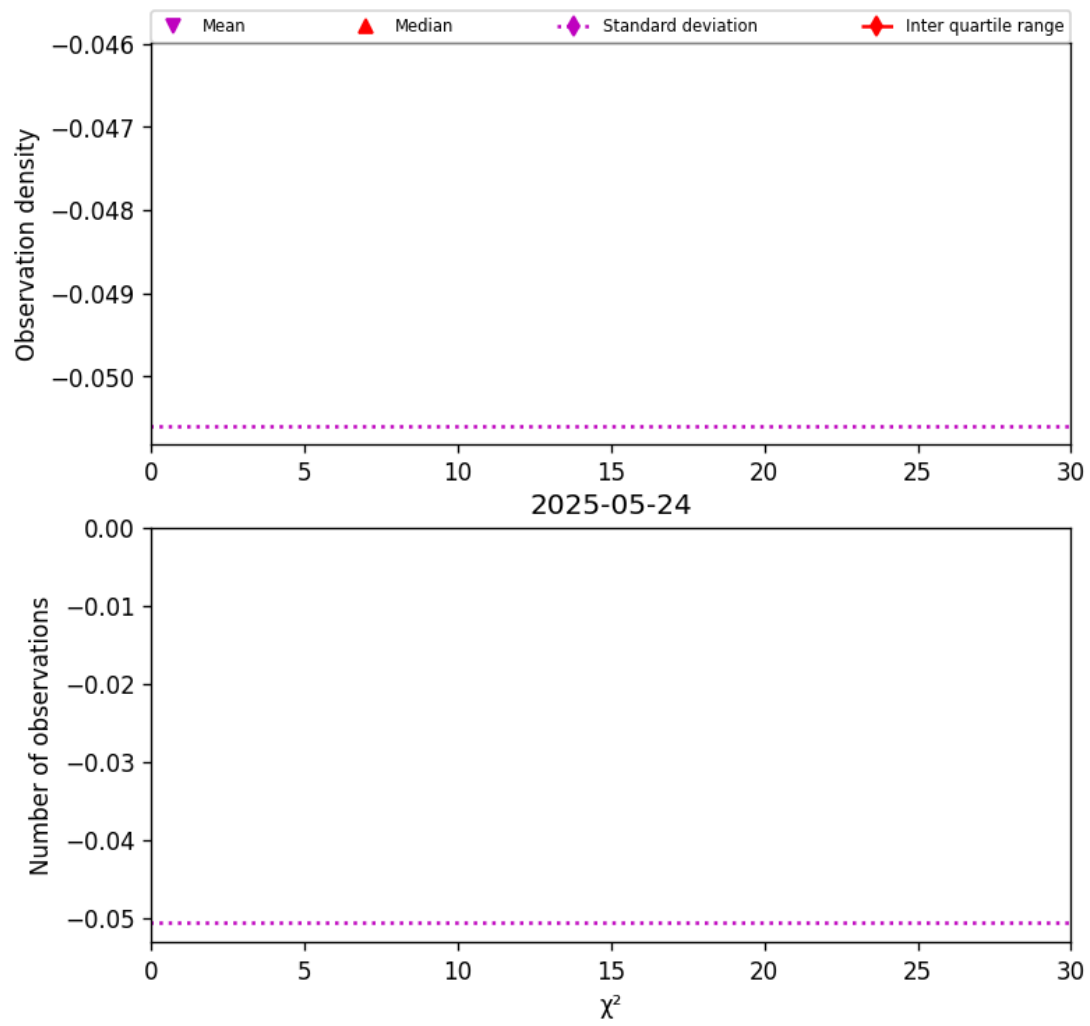
Figure 38: Histogram of “ \chi^2 ” for 2025-05-23 to 2025-05-25
