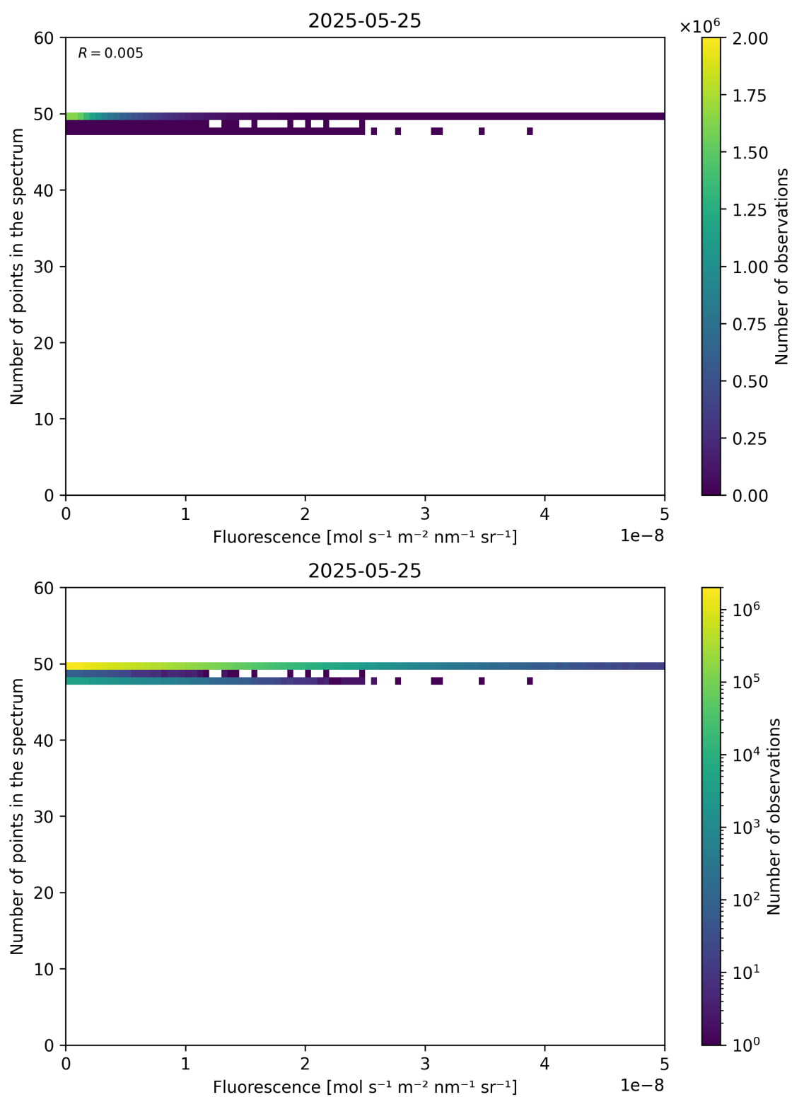
Figure 86: Scatter density plot of “Fluorescence” against “Number of points in the spectrum” for 2025-05-24 to 2025-05-26.
