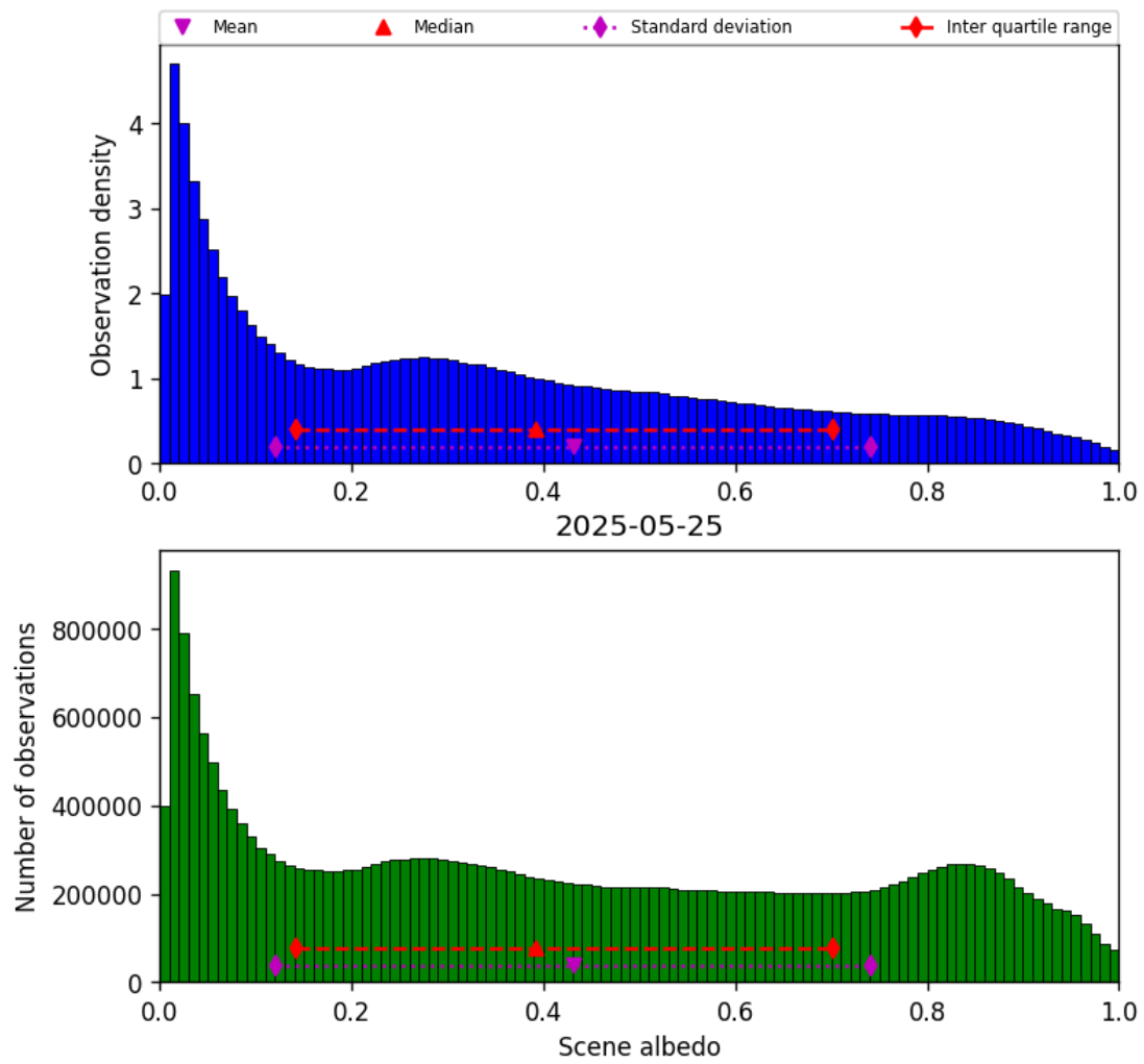
Figure 34: Histogram of “Scene albedo” for 2025-05-24 to 2025-05-26
