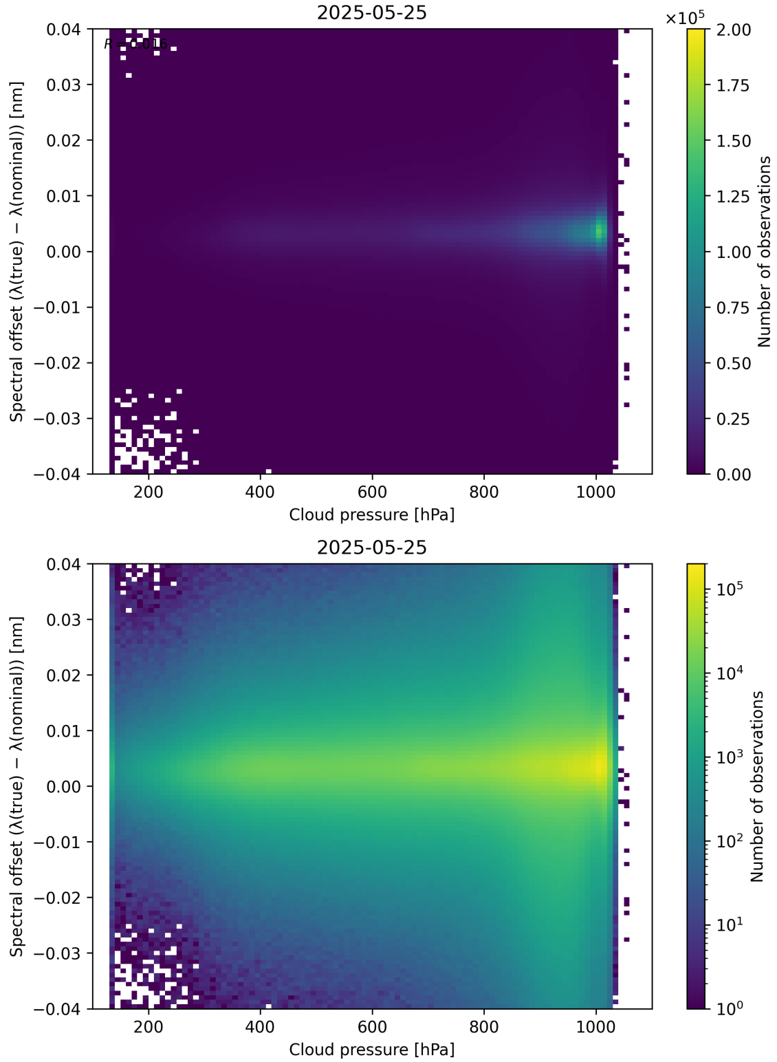
Figure 84: Scatter density plot of “Cloud pressure” against “Spectral offset ( \lambda_{\text{true}} - \lambda_{\text{nominal}} )” for 2025-05-24 to 2025-05-26.
