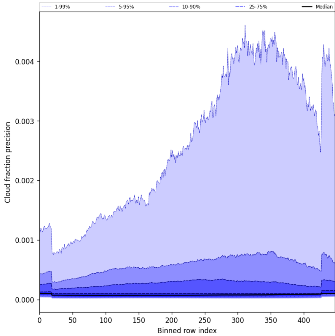
Figure 50: Along track statistics of “Cloud fraction precision” for 2025-05-24 to 2025-05-26
