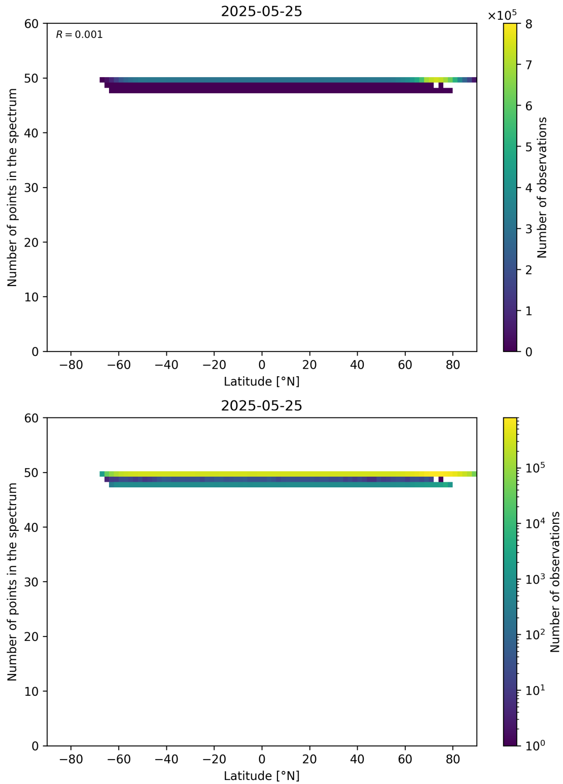
Figure 94: Scatter density plot of “Latitude” against “Number of points in the spectrum” for 2025-05-24 to 2025-05-26.
