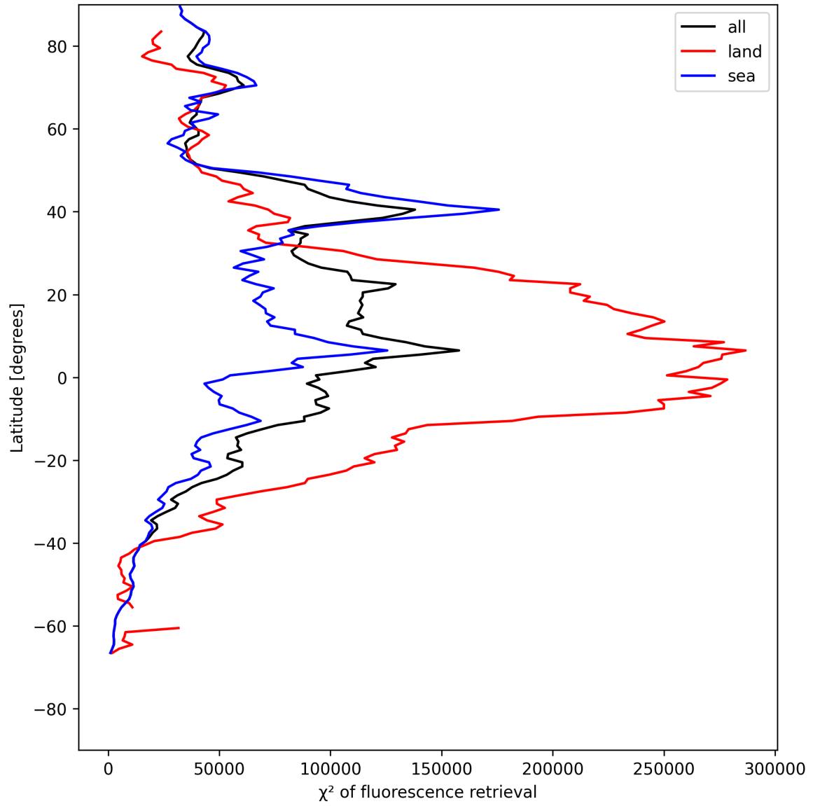
Figure 25: Zonal average of “ \chi^2 of fluorescence retrieval” for 2025-05-24 to 2025-05-26.
