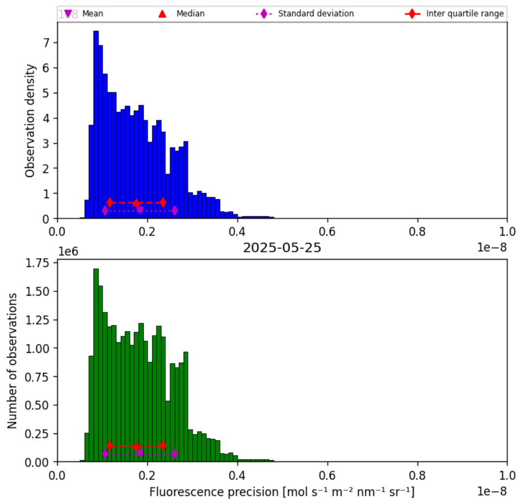
Figure 41: Histogram of “Fluorescence precision” for 2025-05-24 to 2025-05-26
