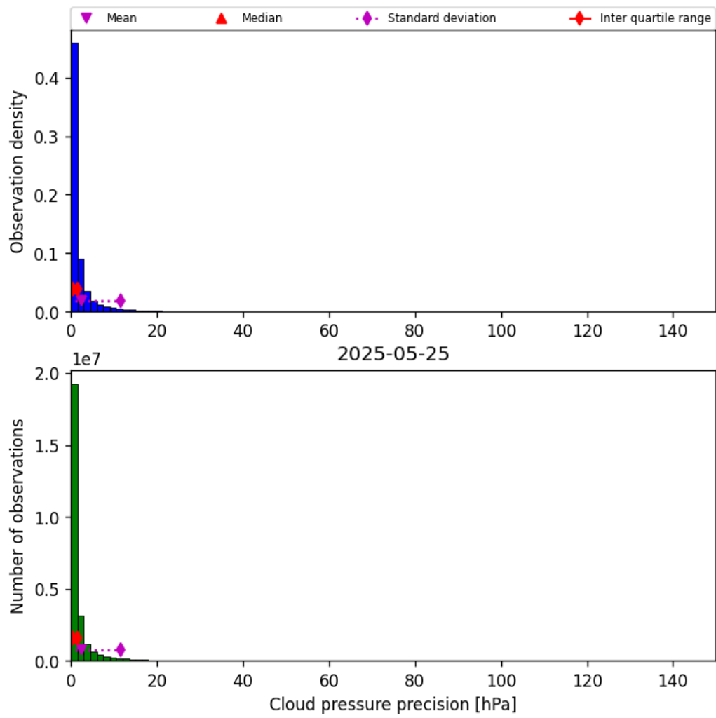
Figure 31: Histogram of “Cloud pressure precision” for 2025-05-24 to 2025-05-26
