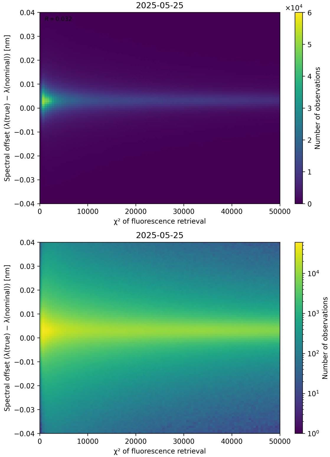
Figure 69: Scatter density plot of “ \chi^2 of fluorescence retrieval” against “Spectral offset ( \lambda_{\text{true}} - \lambda_{\text{nominal}} )” for 2025-05-24 to 2025-05-26.
