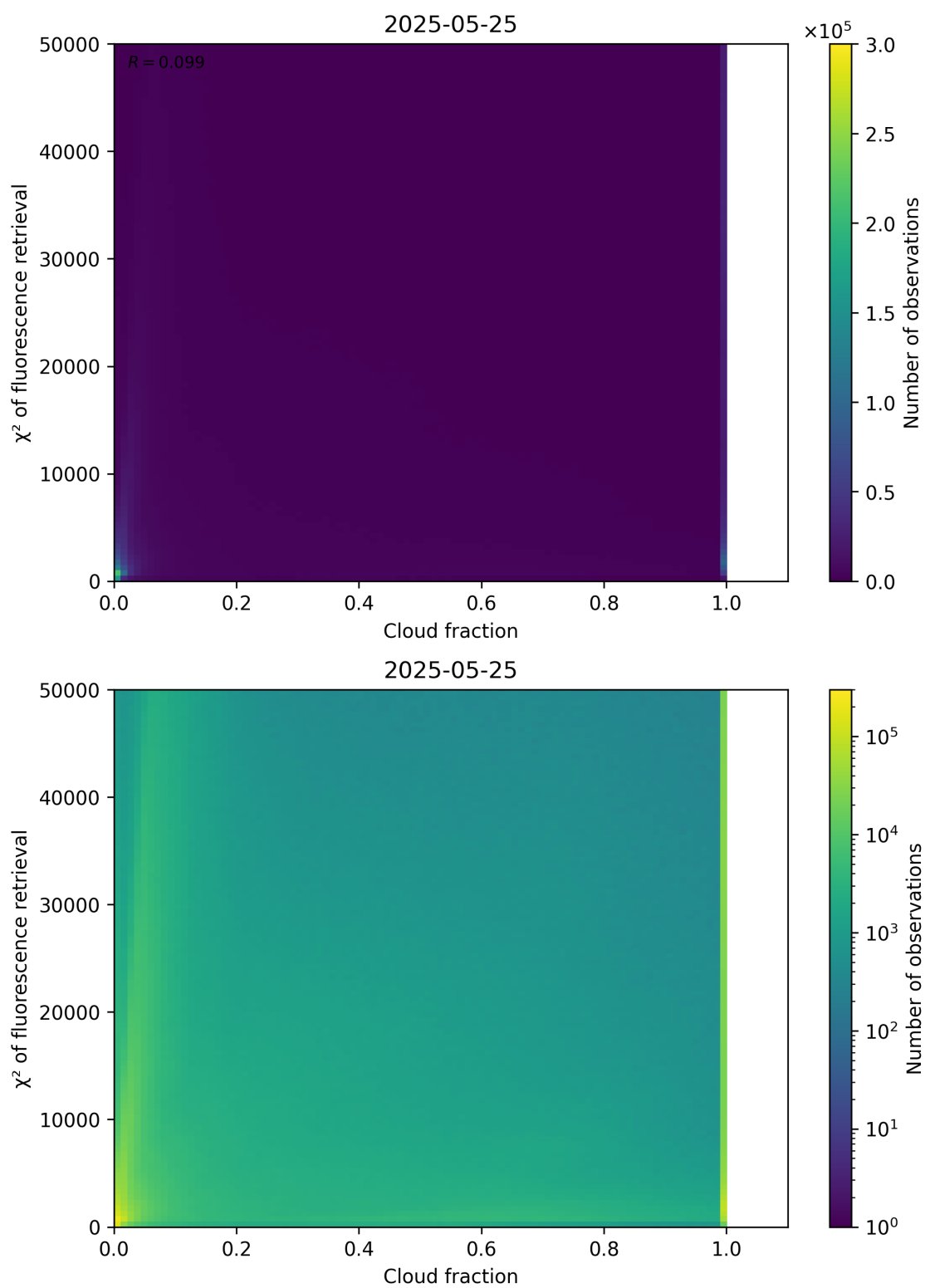
Figure 71: Scatter density plot of “Cloud fraction” against “ \chi^2 of fluorescence retrieval” for 2025-05-24 to 2025-05-26.
