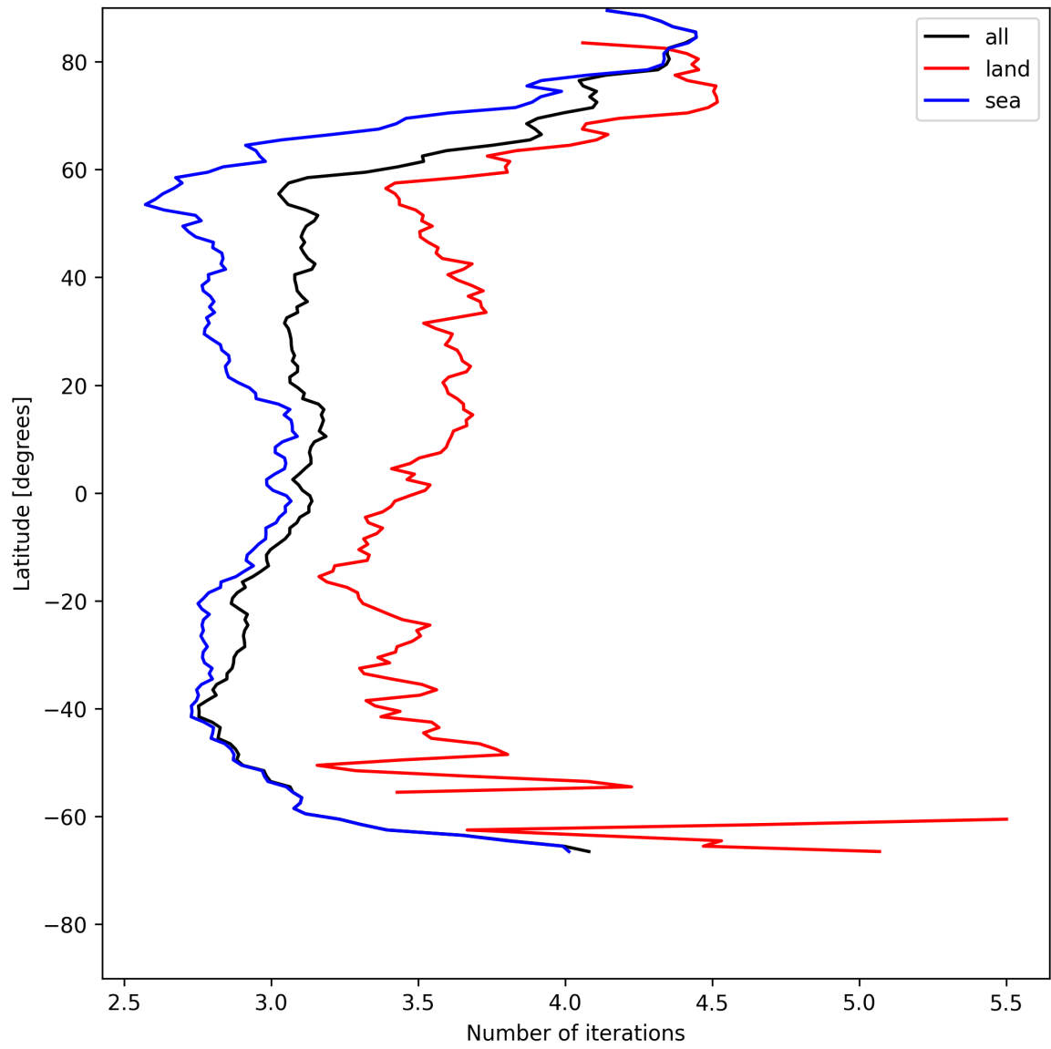
Figure 22: Zonal average of “Number of iterations” for 2025-05-24 to 2025-05-26.
