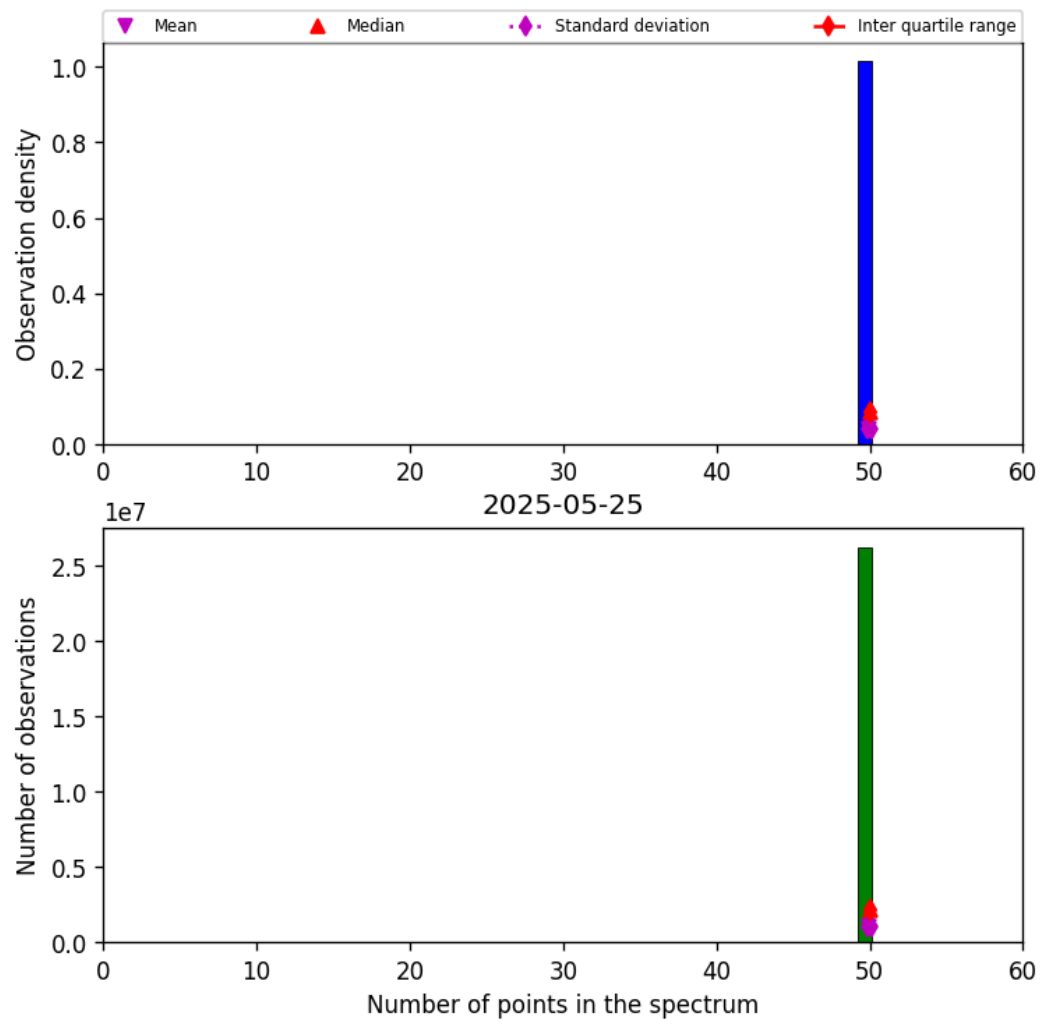
Figure 44: Histogram of “Number of points in the spectrum” for 2025-05-24 to 2025-05-26
