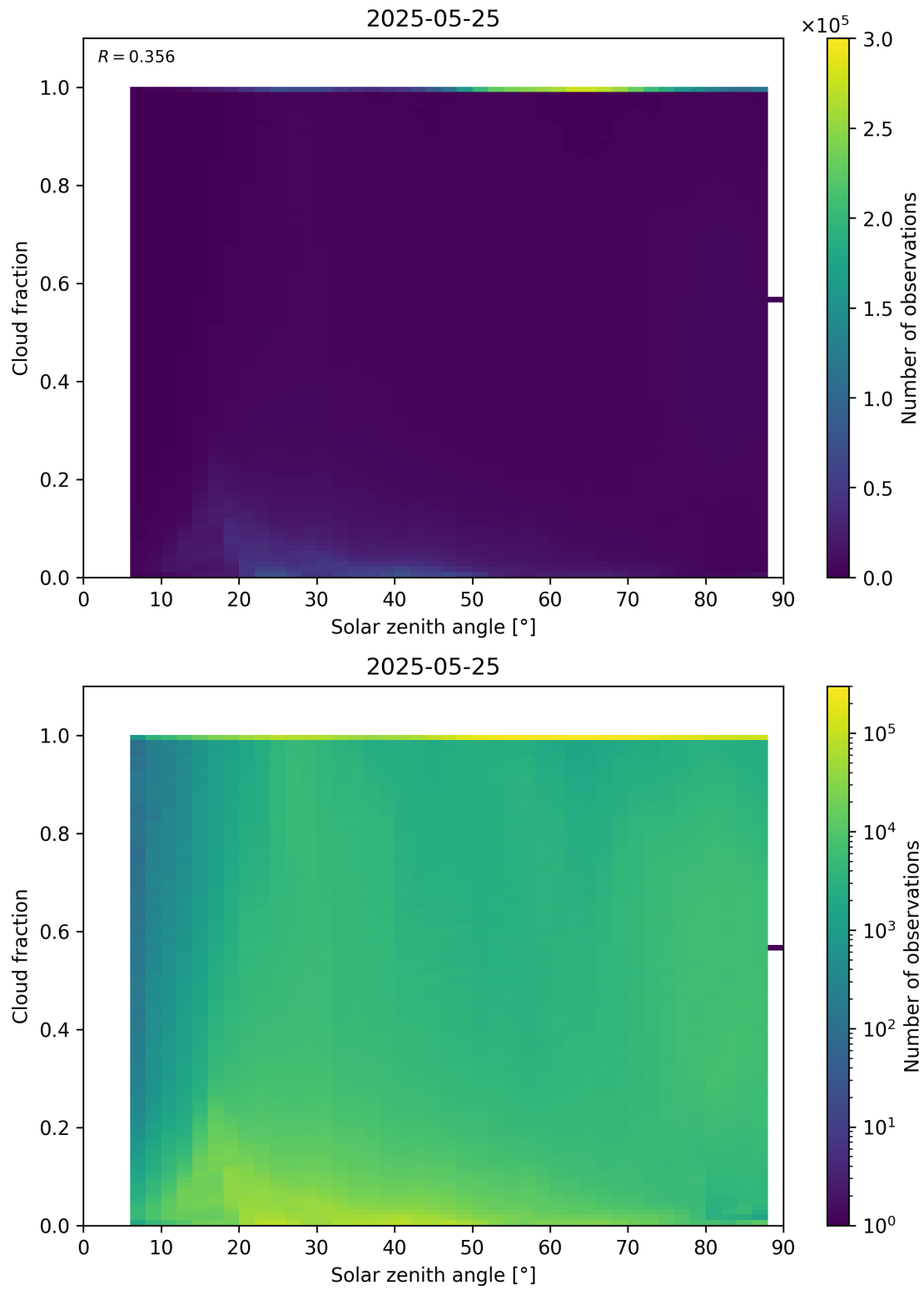
Figure 110: Scatter density plot of “Solar zenith angle” against “Cloud fraction” for 2025-05-24 to 2025-05-26.
