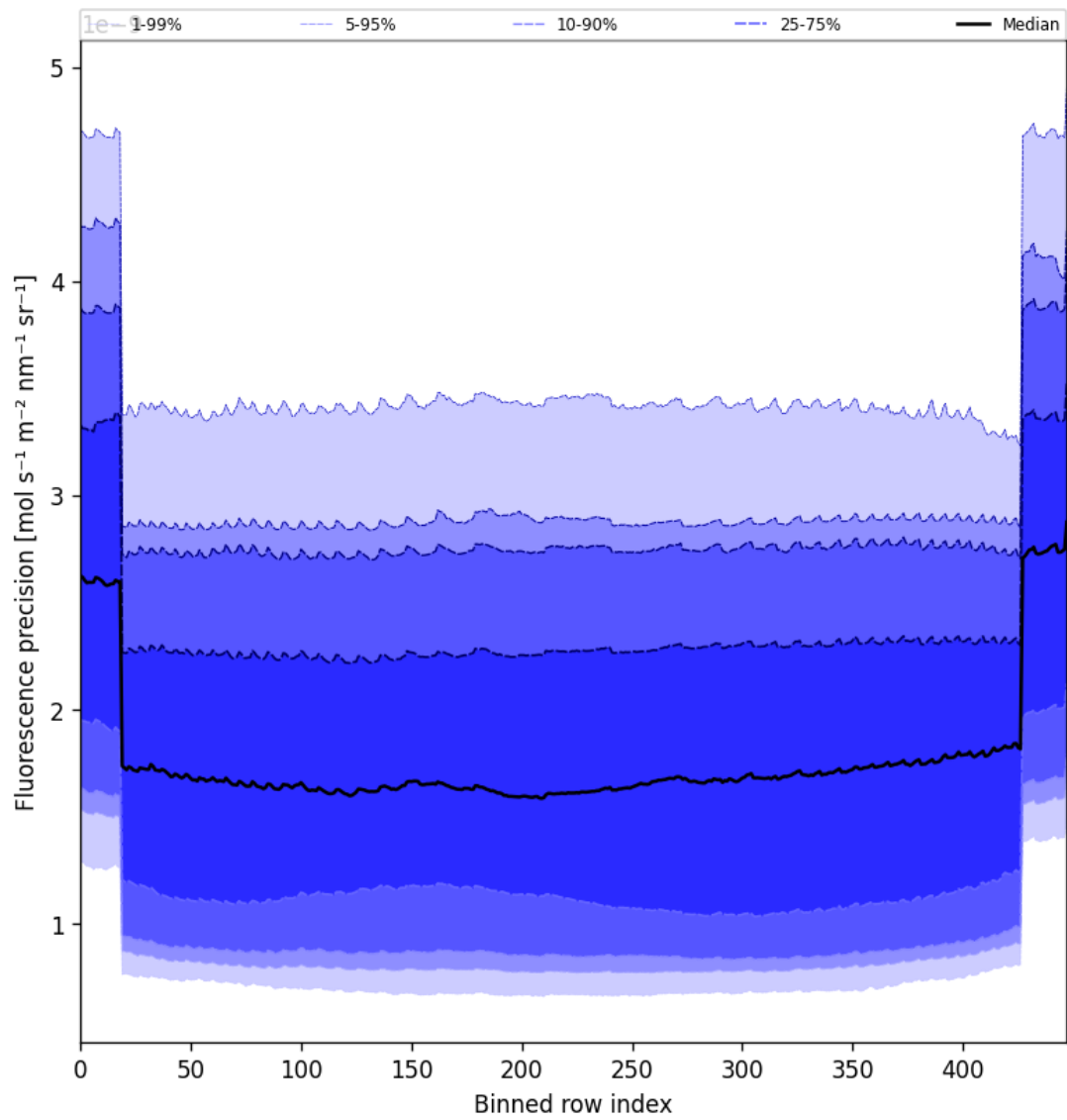
Figure 58: Along track statistics of “Fluorescence precision” for 2025-05-24 to 2025-05-26
