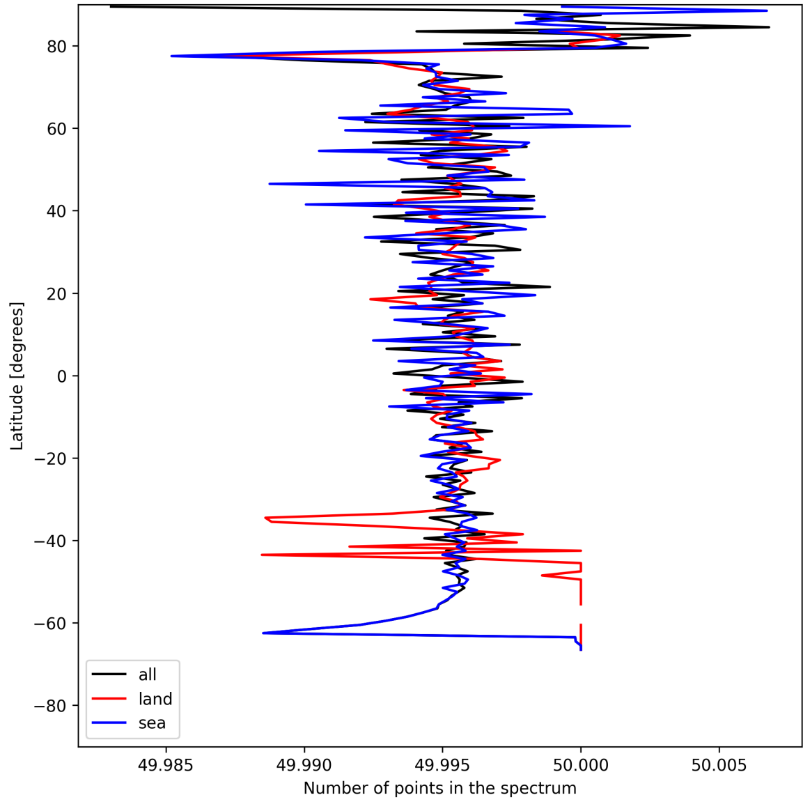
Figure 27: Zonal average of “Number of points in the spectrum” for 2025-05-24 to 2025-05-26.
