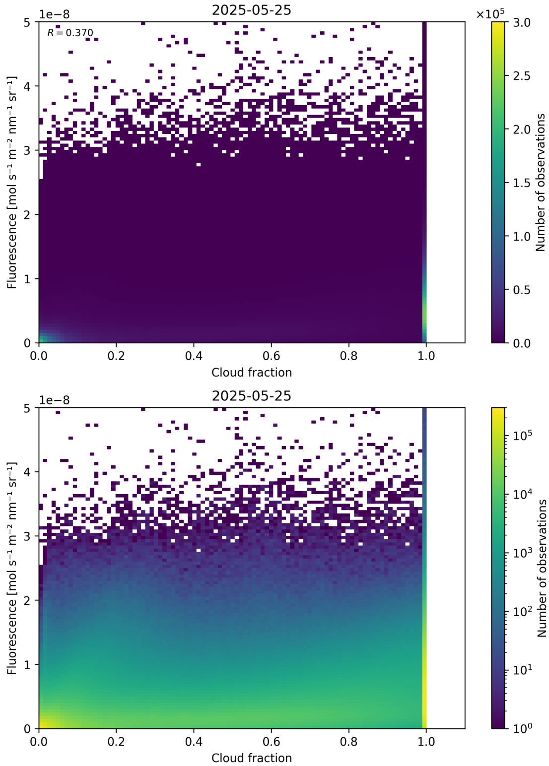
Figure 72: Scatter density plot of “Cloud fraction” against “Fluorescence” for 2025-05-24 to 2025-05-26.
