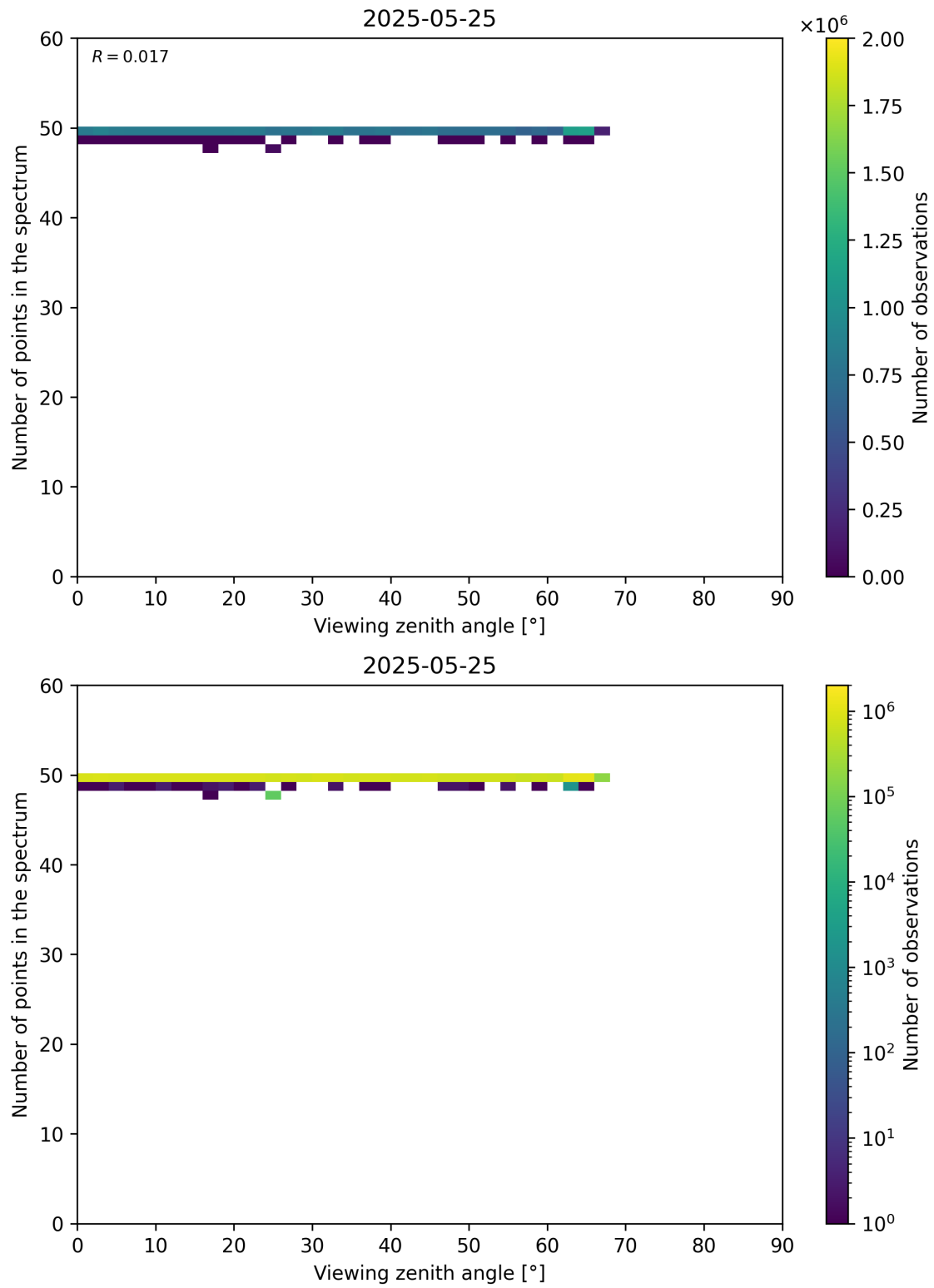
Figure 125: Scatter density plot of “Viewing zenith angle” against “Number of points in the spectrum” for 2025-05-24 to 2025-05-26.
