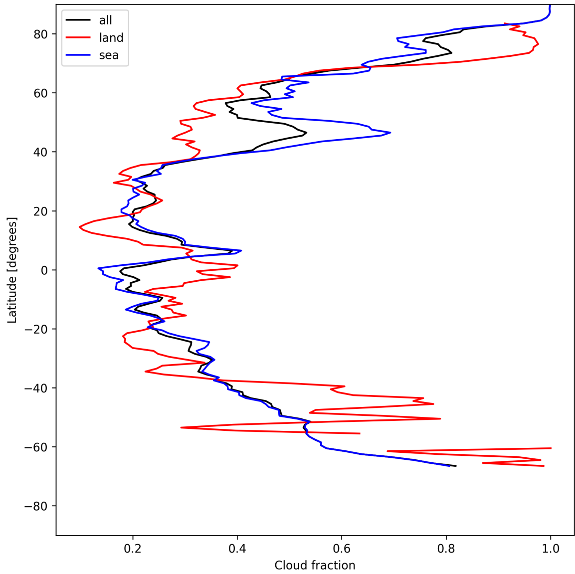
Figure 15: Zonal average of “Cloud fraction” for 2025-05-24 to 2025-05-26.
