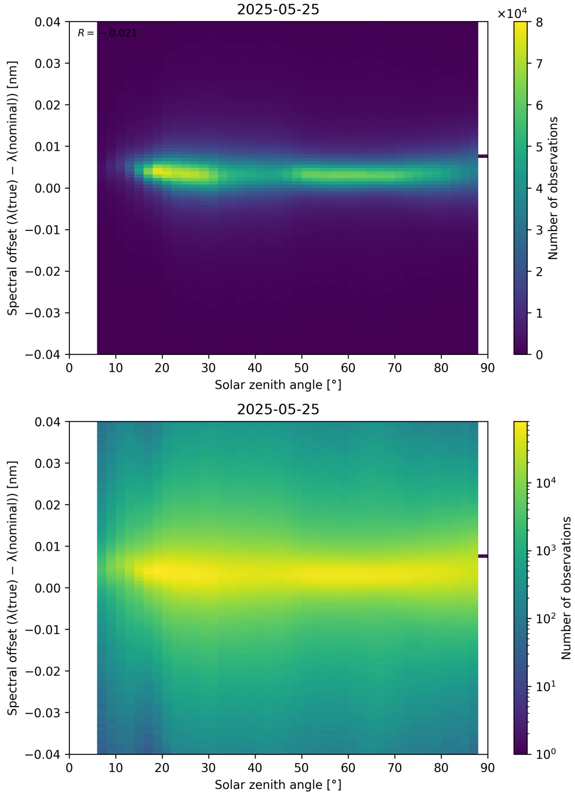
Figure 117: Scatter density plot of “Solar zenith angle” against “Spectral offset ( \lambda_{\text{true}} - \lambda_{\text{nominal}} )” for 2025-05-24 to 2025-05-26.
