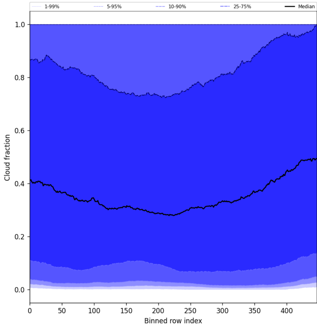
Figure 49: Along track statistics of “Cloud fraction” for 2025-05-24 to 2025-05-26
