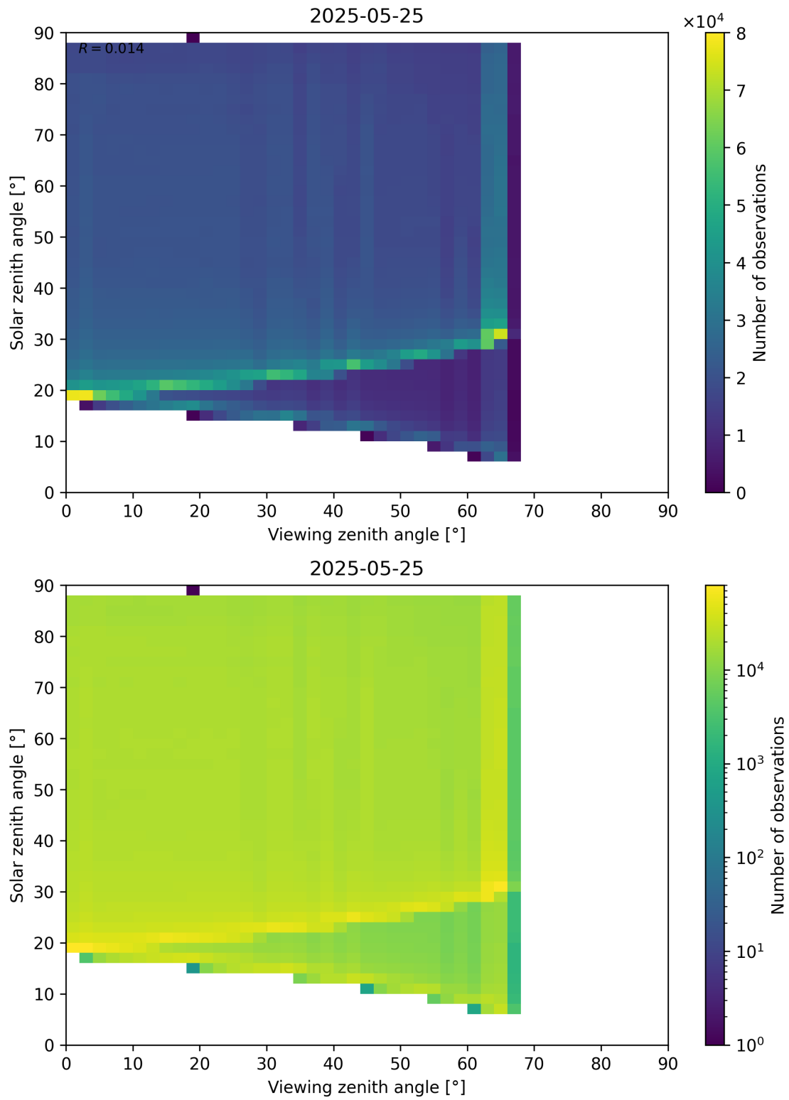
Figure 127: Scatter density plot of “Viewing zenith angle” against “Solar zenith angle” for 2025-05-24 to 2025-05-26.
