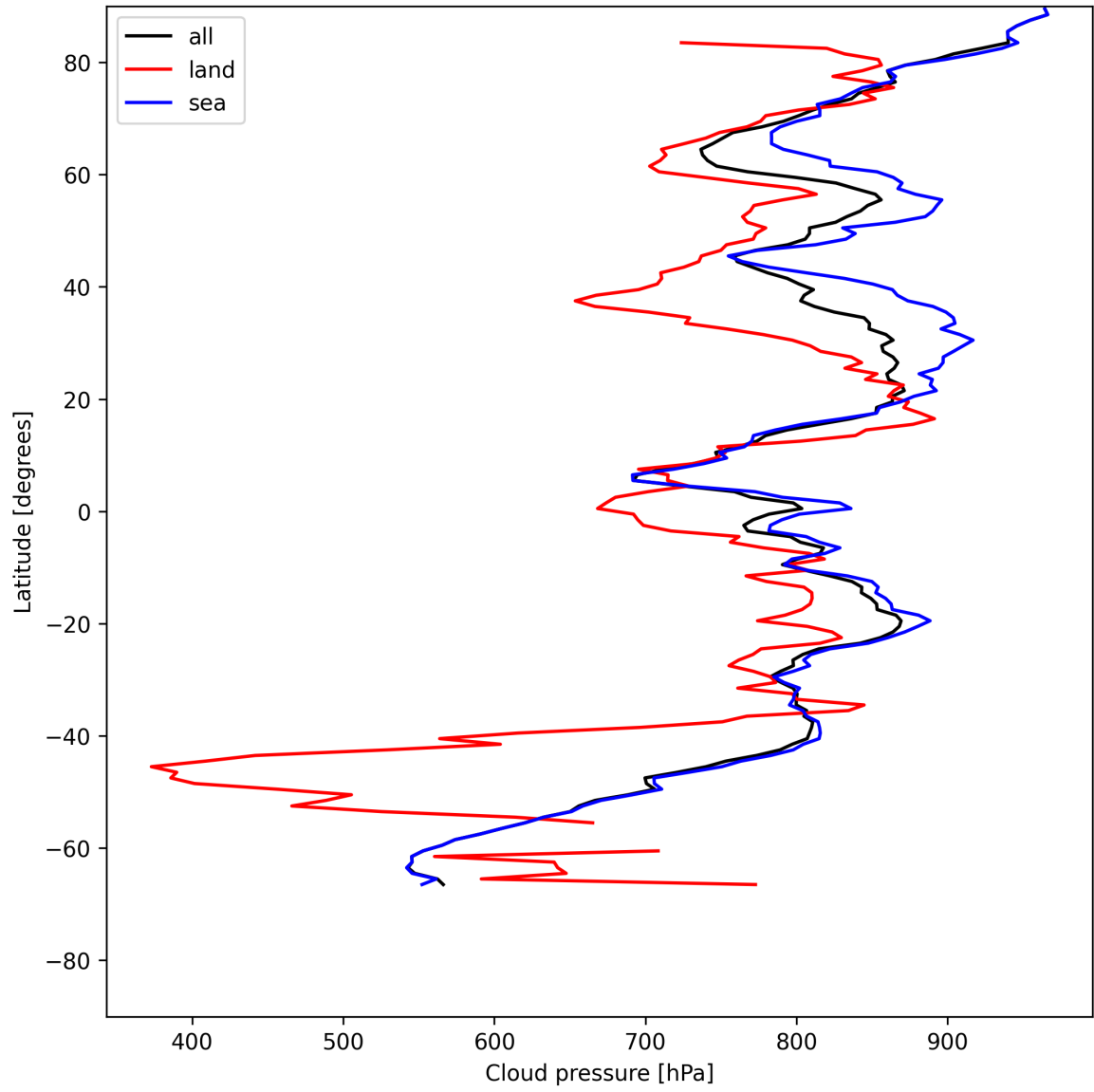
Figure 13: Zonal average of “Cloud pressure” for 2025-05-24 to 2025-05-26.
