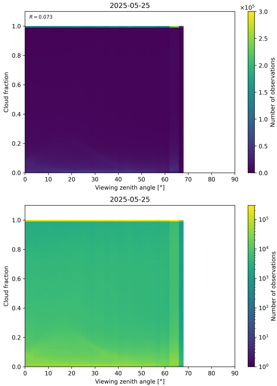
Figure 120: Scatter density plot of “Viewing zenith angle” against “Cloud fraction” for 2025-05-24 to 2025-05-26.
