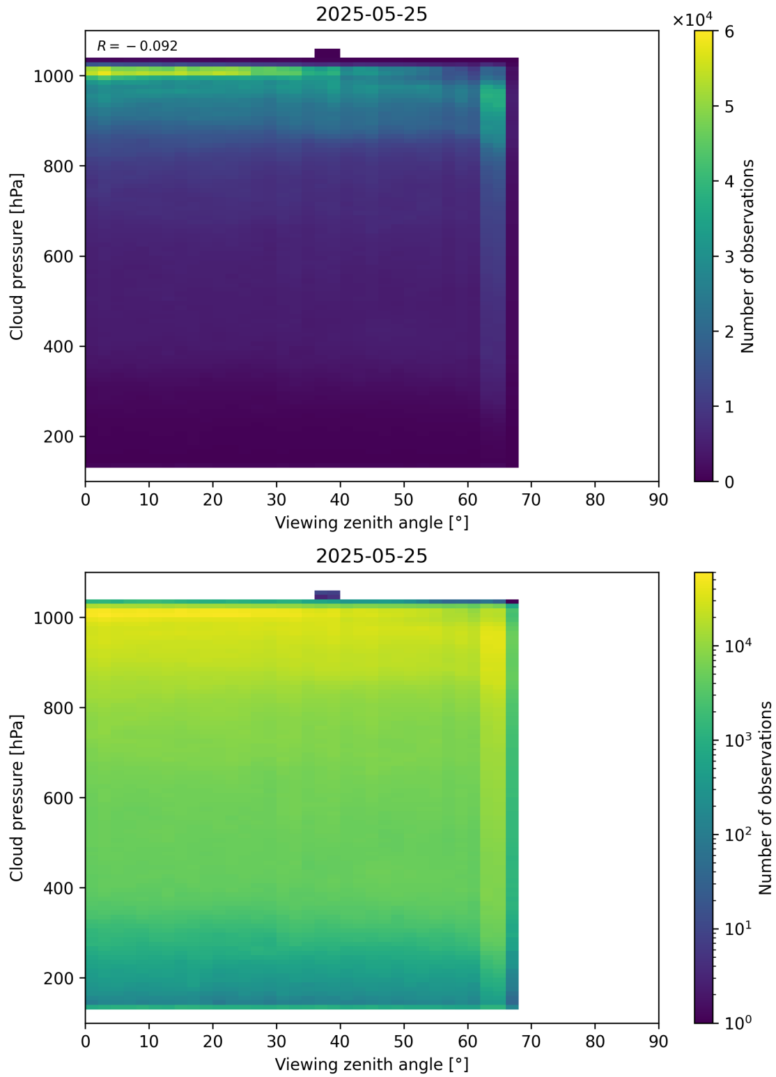
Figure 121: Scatter density plot of “Viewing zenith angle” against “Cloud pressure” for 2025-05-24 to 2025-05-26.
