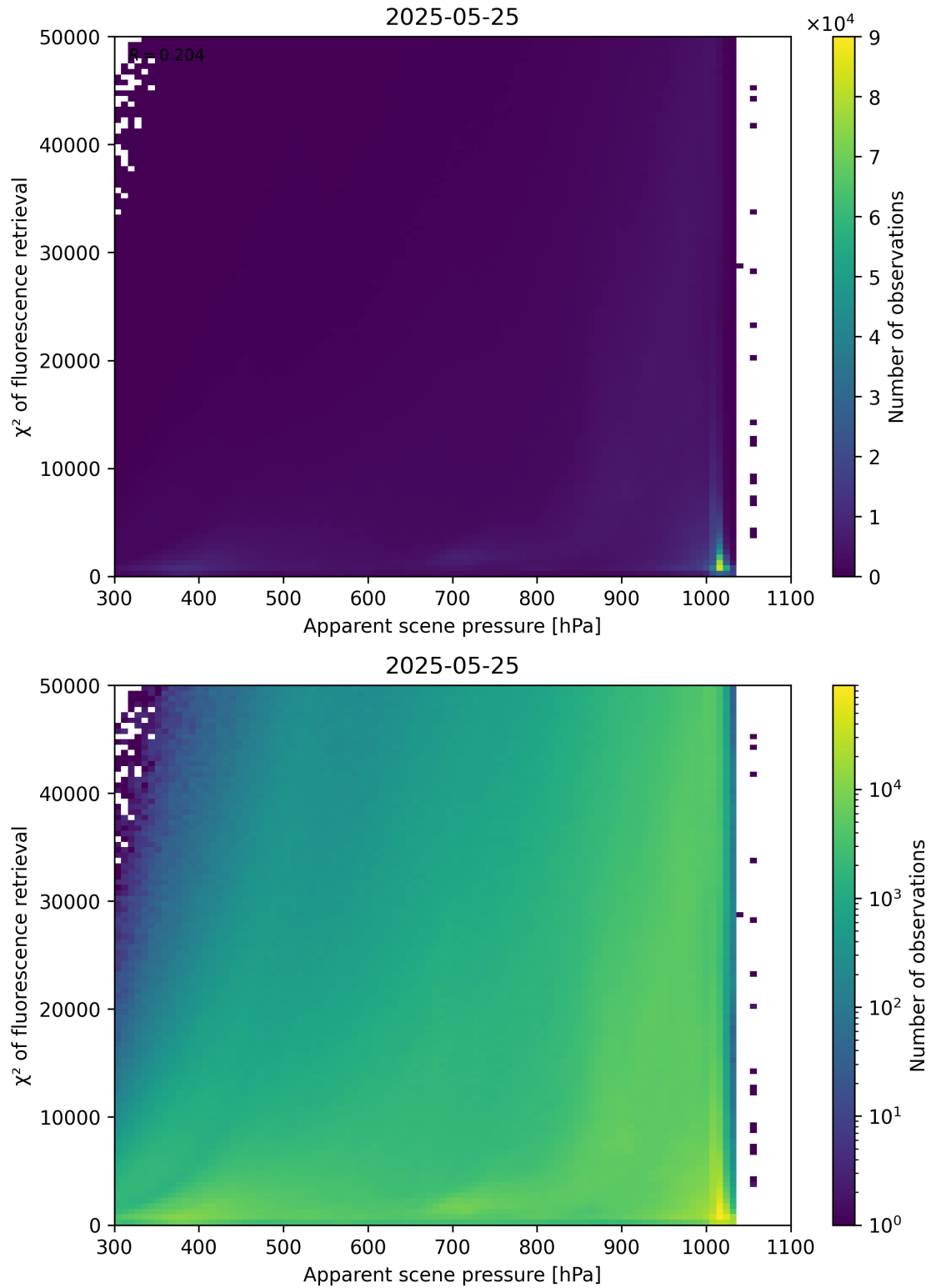
Figure 63: Scatter density plot of “Apparent scene pressure” against “ \chi^2 of fluorescence retrieval” for 2025-05-24 to 2025-05-26.
