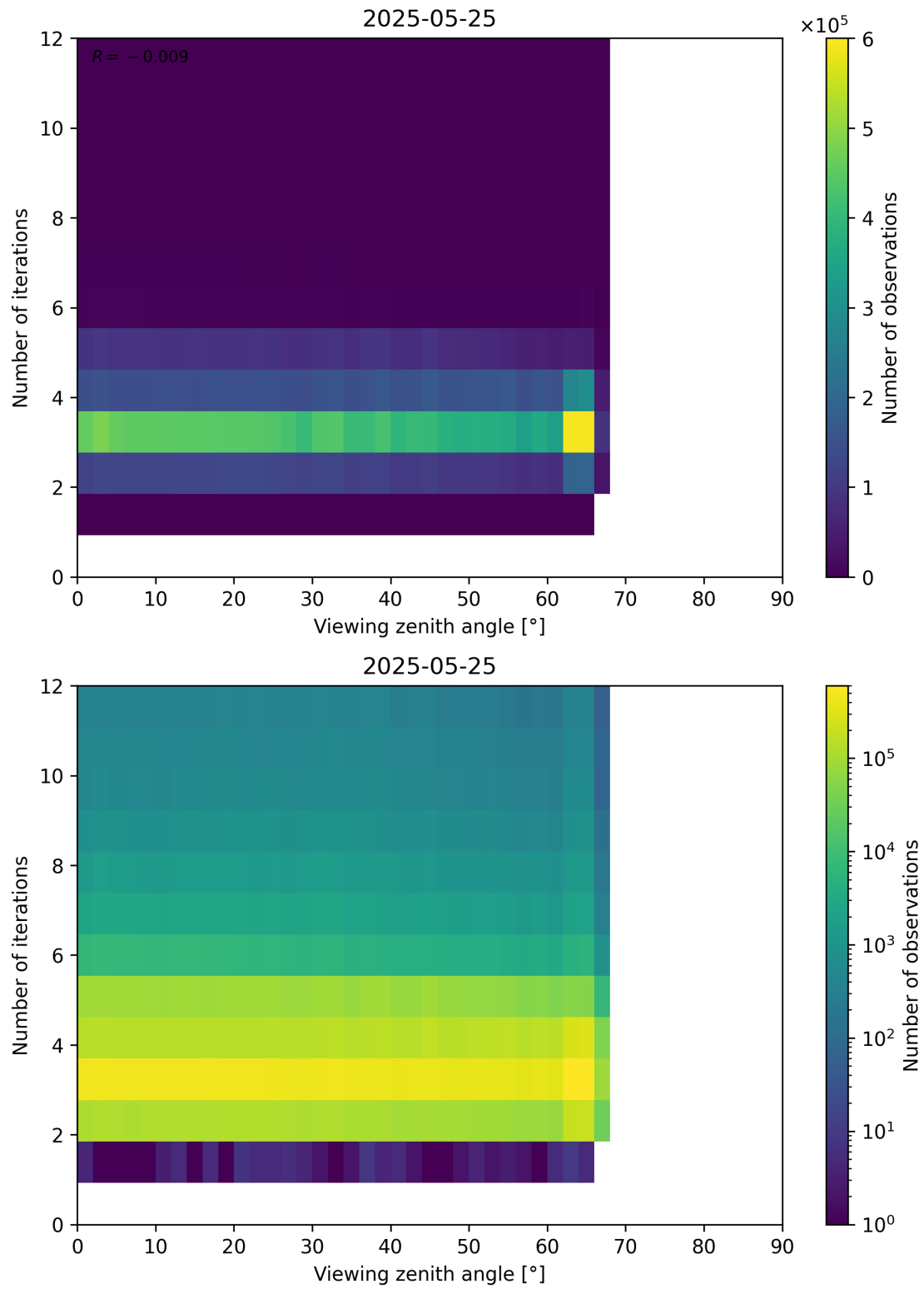
Figure 124: Scatter density plot of “Viewing zenith angle” against “Number of iterations” for 2025-05-24 to 2025-05-26.
