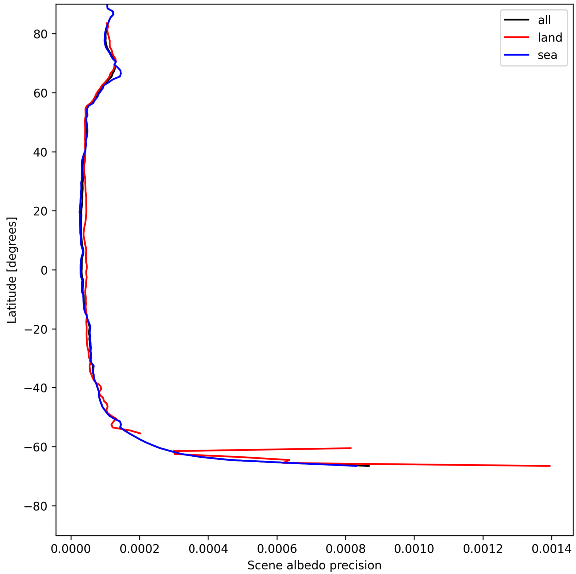
Figure 18: Zonal average of “Scene albedo precision” for 2025-05-24 to 2025-05-26.
