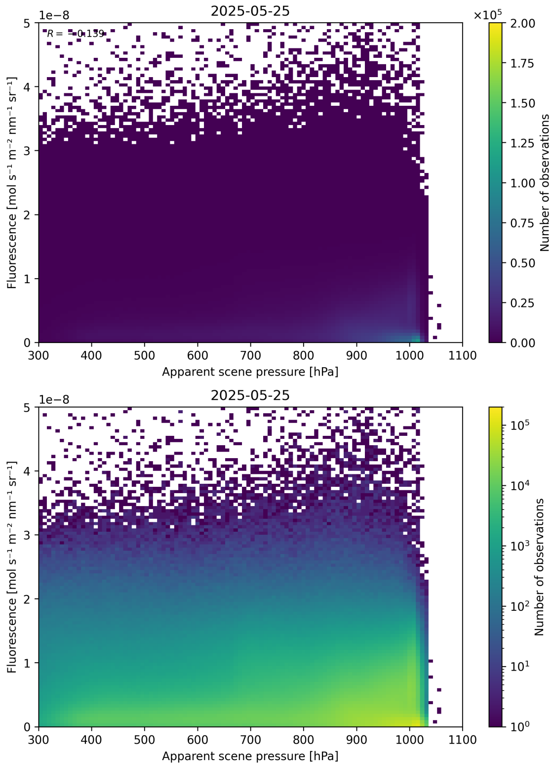
Figure 64: Scatter density plot of “Apparent scene pressure” against “Fluorescence” for 2025-05-24 to 2025-05-26.
