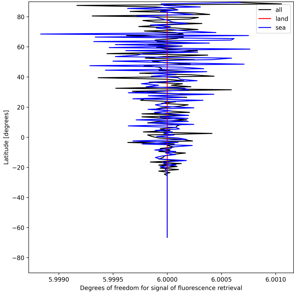
Figure 26: Zonal average of “Degrees of freedom for signal of fluorescence retrieval” for 2025-05-24 to 2025-05-26.
