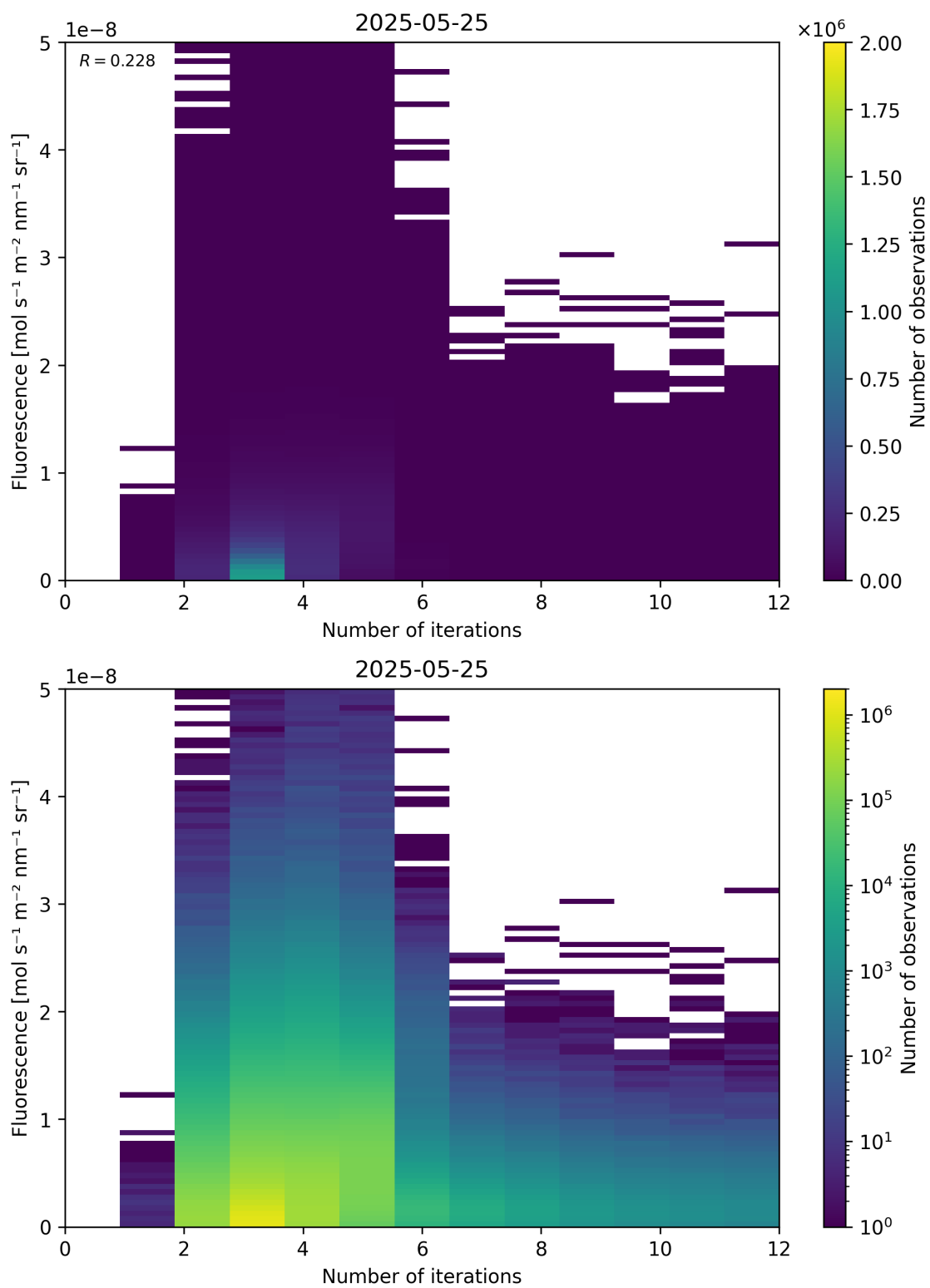
Figure 98: Scatter density plot of “Number of iterations” against “Fluorescence” for 2025-05-24 to 2025-05-26.
