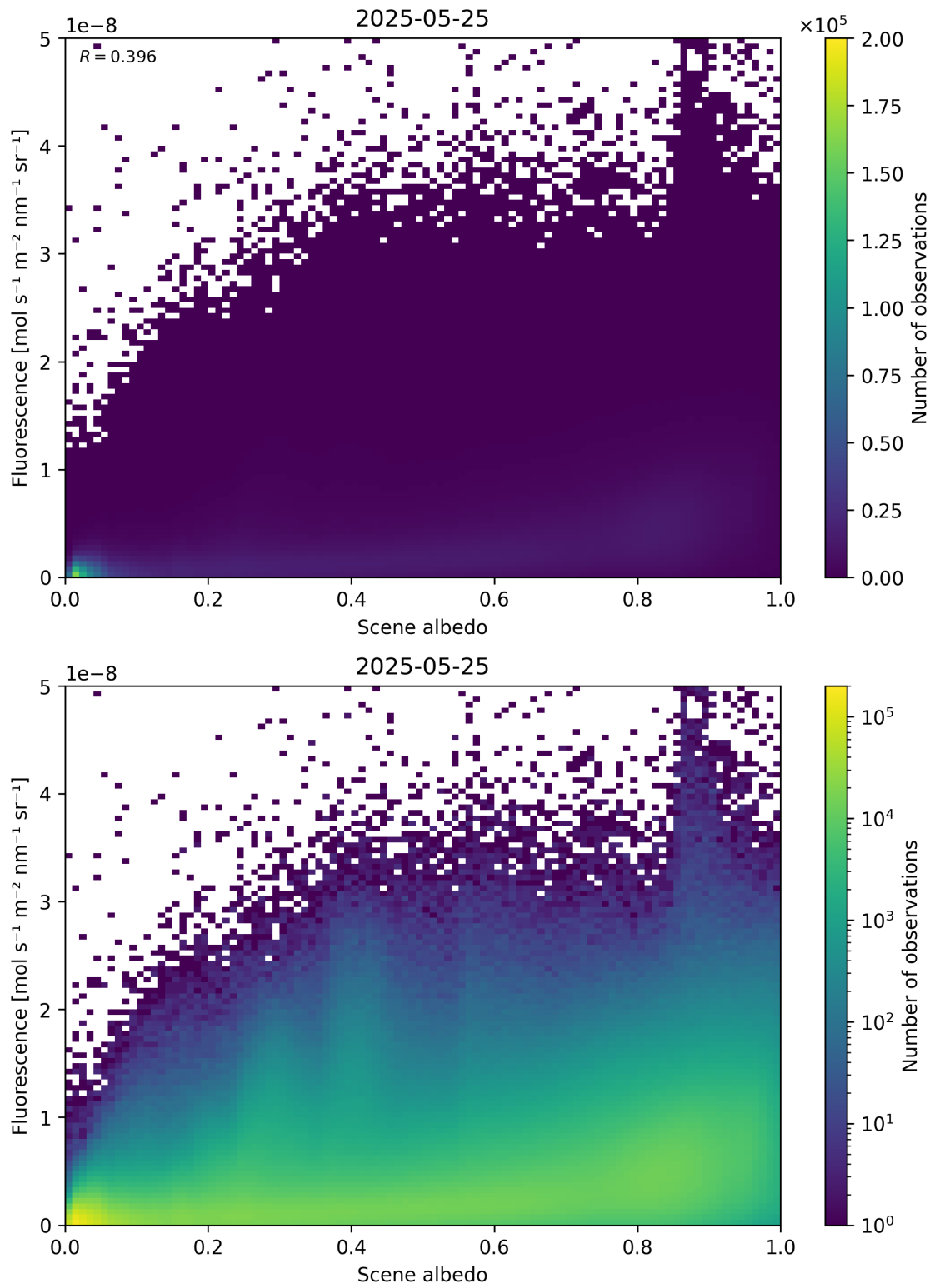
Figure 104: Scatter density plot of “Scene albedo” against “Fluorescence” for 2025-05-24 to 2025-05-26.
