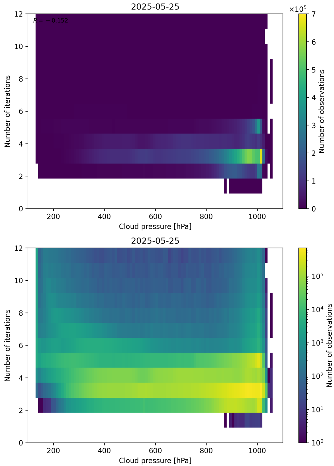
Figure 81: Scatter density plot of “Cloud pressure” against “Number of iterations” for 2025-05-24 to 2025-05-26.
