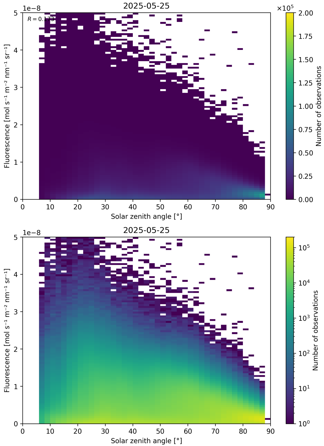
Figure 112: Scatter density plot of “Solar zenith angle” against “Fluorescence” for 2025-05-24 to 2025-05-26.
