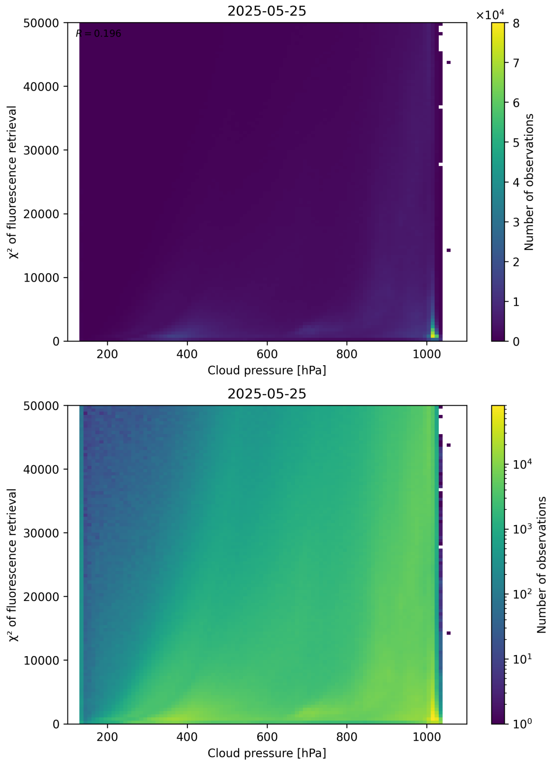
Figure 78: Scatter density plot of “Cloud pressure” against “ \chi^2 of fluorescence retrieval” for 2025-05-24 to 2025-05-26.
