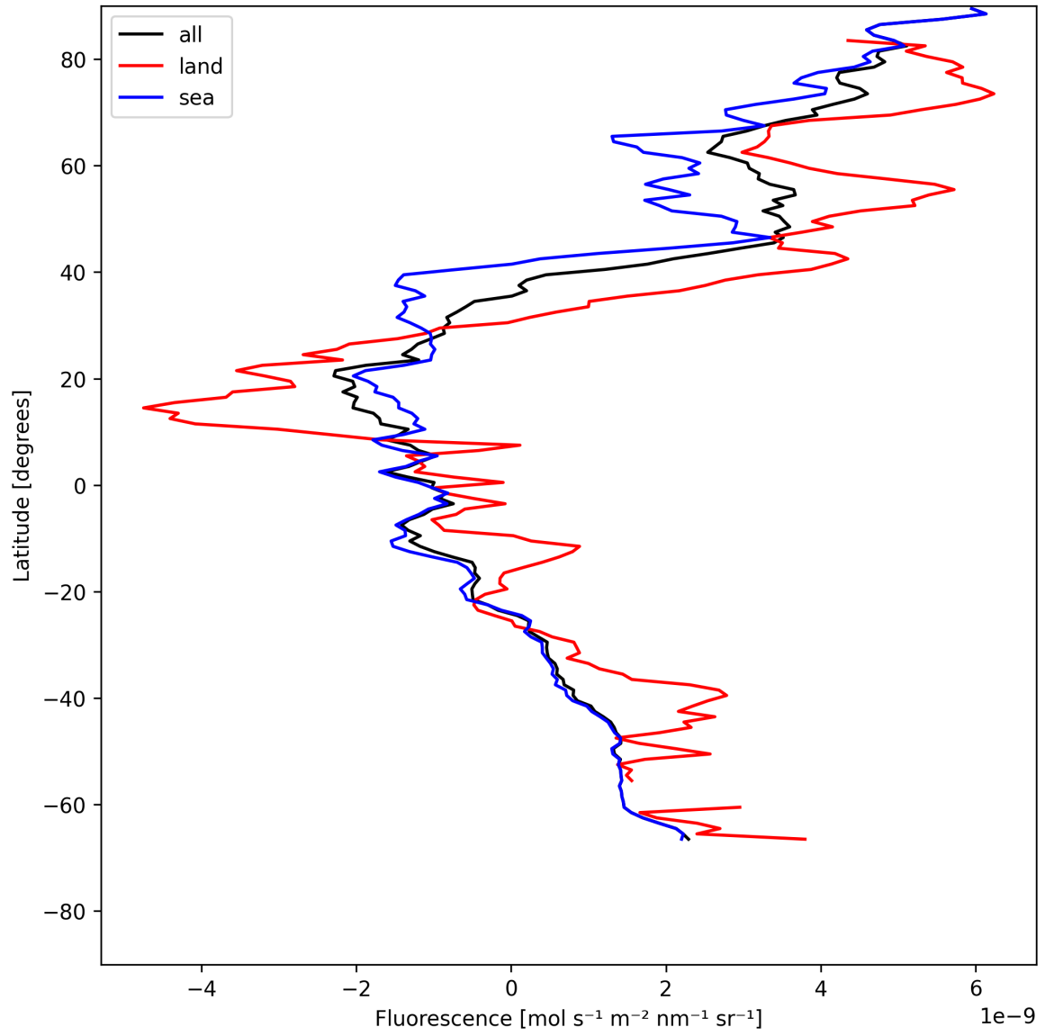
Figure 23: Zonal average of “Fluorescence” for 2025-05-24 to 2025-05-26.
