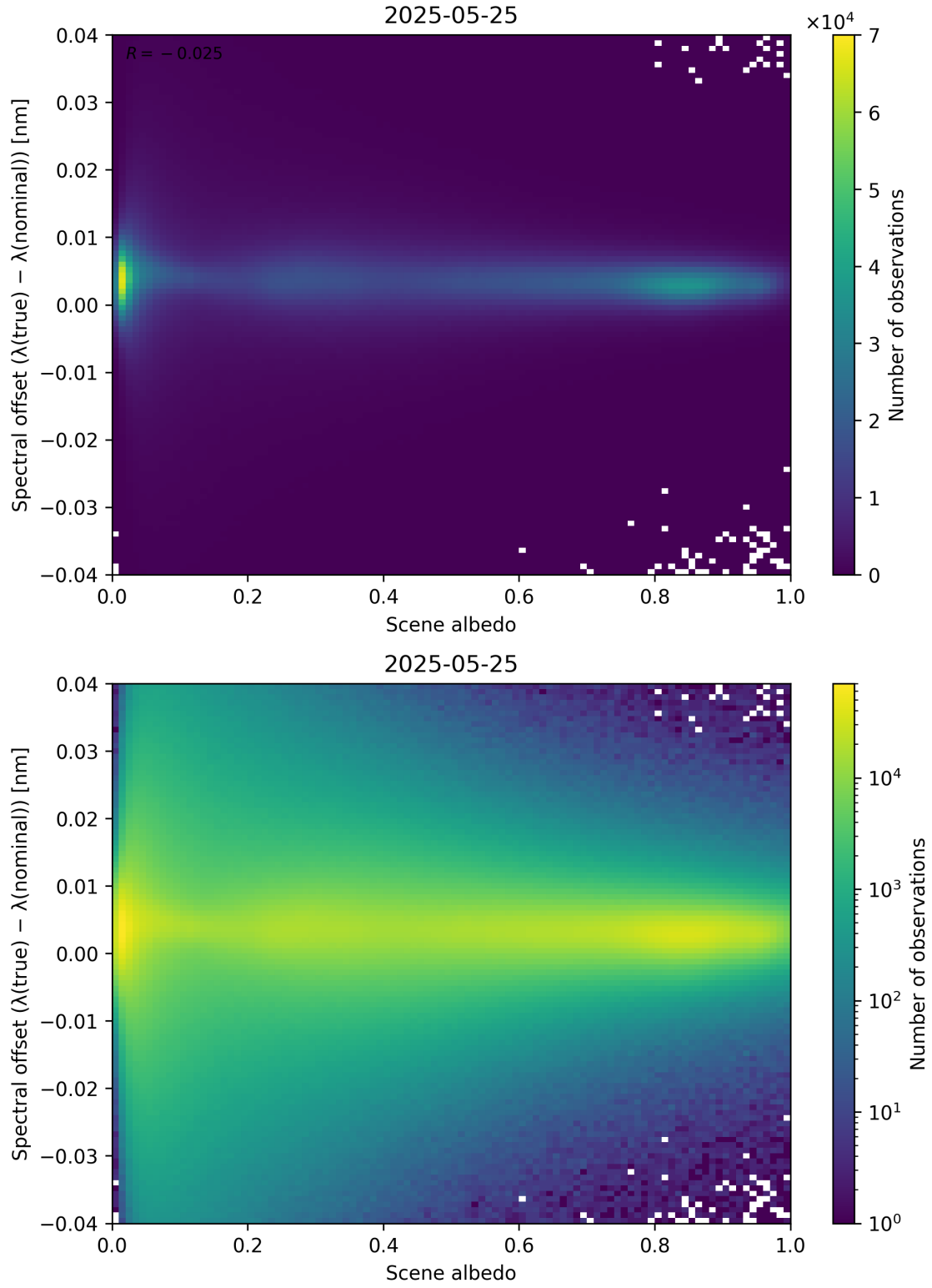
Figure 107: Scatter density plot of “Scene albedo” against “Spectral offset ( \lambda_{\text{true}} - \lambda_{\text{nominal}} )” for 2025-05-24 to 2025-05-26.
