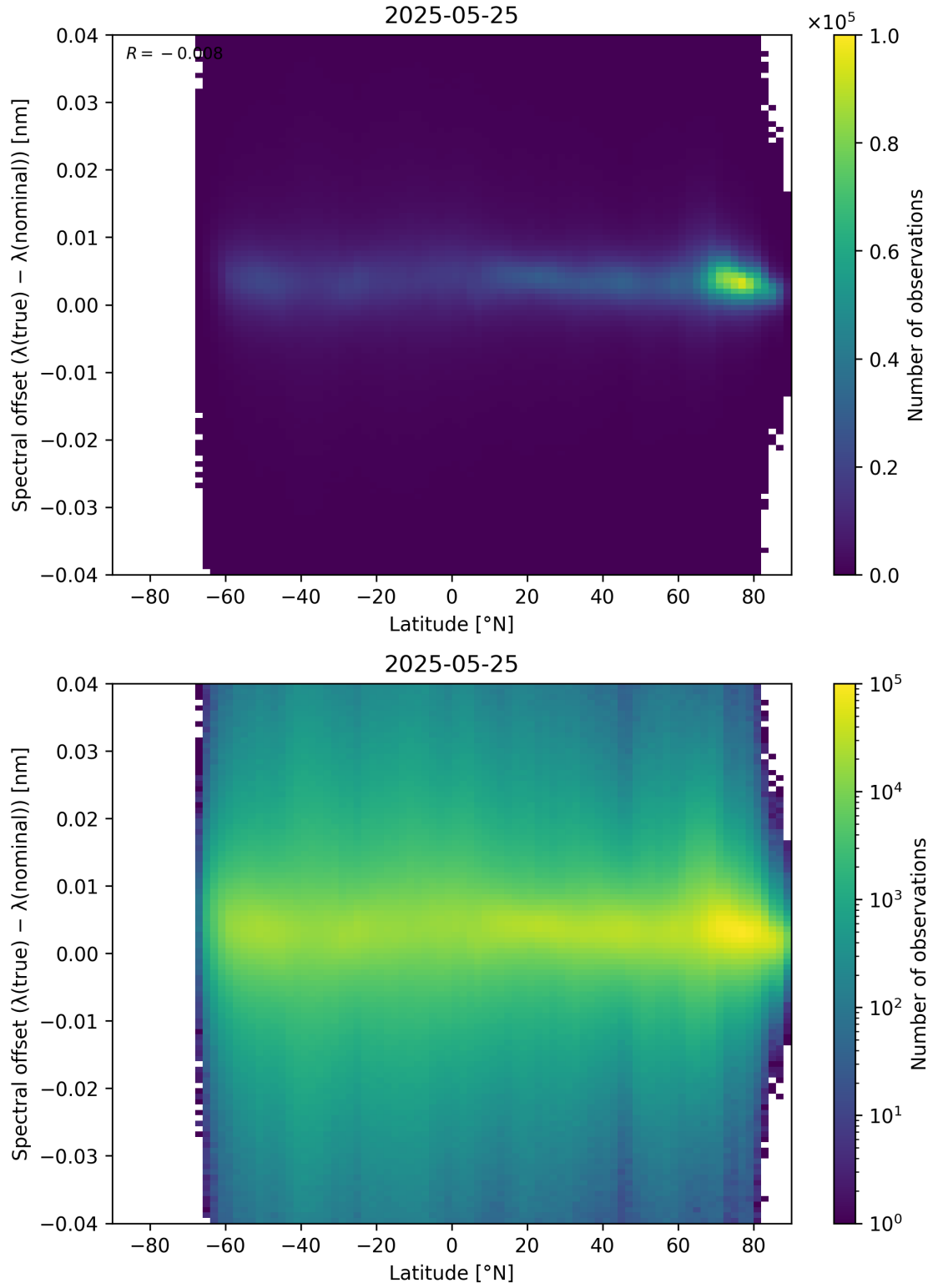
Figure 96: Scatter density plot of “Latitude” against “Spectral offset ( \lambda_{\text{true}} - \lambda_{\text{nominal}} )” for 2025-05-24 to 2025-05-26.
