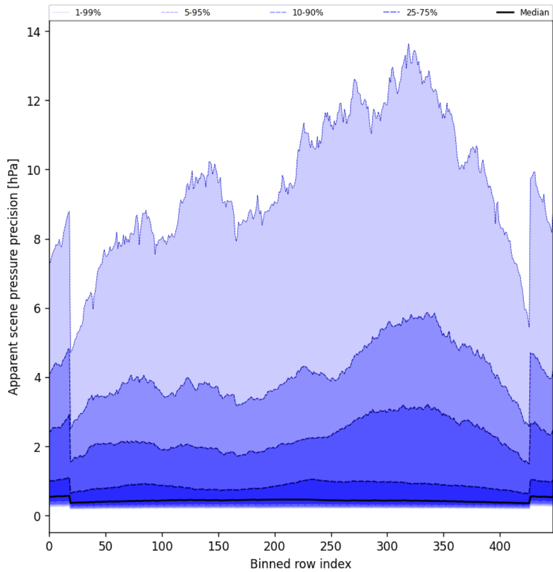
Figure 54: Along track statistics of “Apparent scene pressure precision” for 2025-05-24 to 2025-05-26
