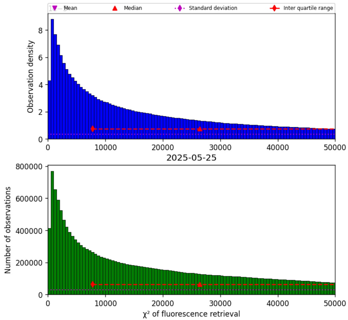
Figure 42: Histogram of “ \chi^2 of fluorescence retrieval” for 2025-05-24 to 2025-05-26
