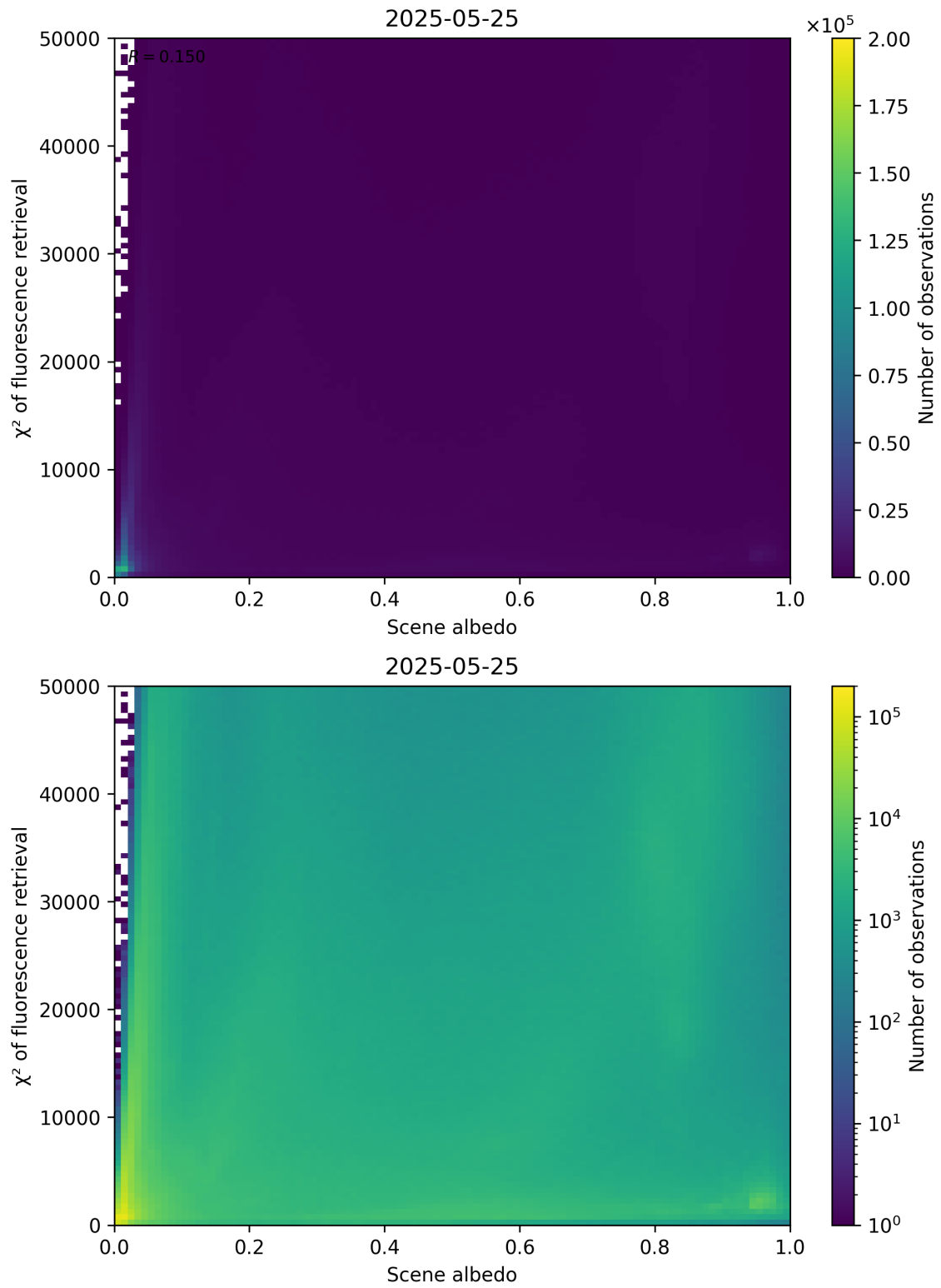
Figure 103: Scatter density plot of “Scene albedo” against “ \chi^2 of fluorescence retrieval” for 2025-05-24 to 2025-05-26.
