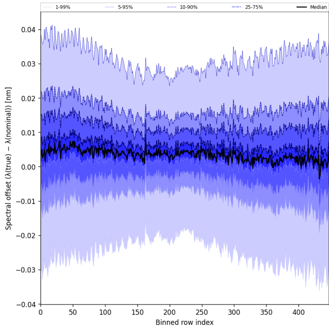
Figure 62: Along track statistics of “Spectral offset ( \lambda_{\text{true}} - \lambda_{\text{nominal}} )” for 2025-05-24 to 2025-05-26
