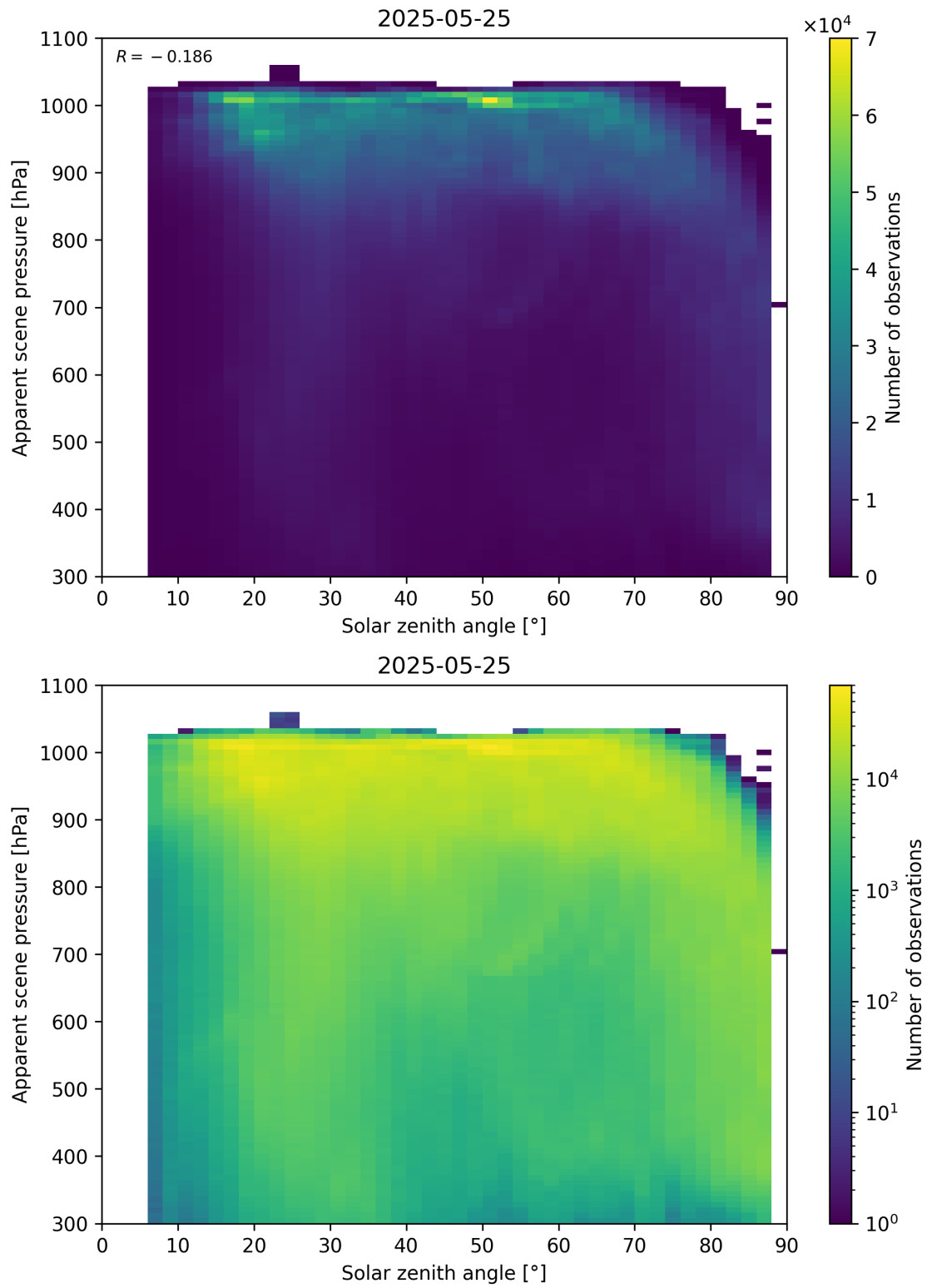
Figure 108: Scatter density plot of “Solar zenith angle” against “Apparent scene pressure” for 2025-05-24 to 2025-05-26.
