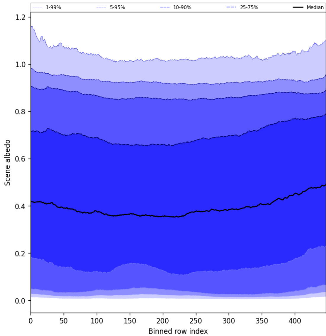
Figure 51: Along track statistics of “Scene albedo” for 2025-05-24 to 2025-05-26
