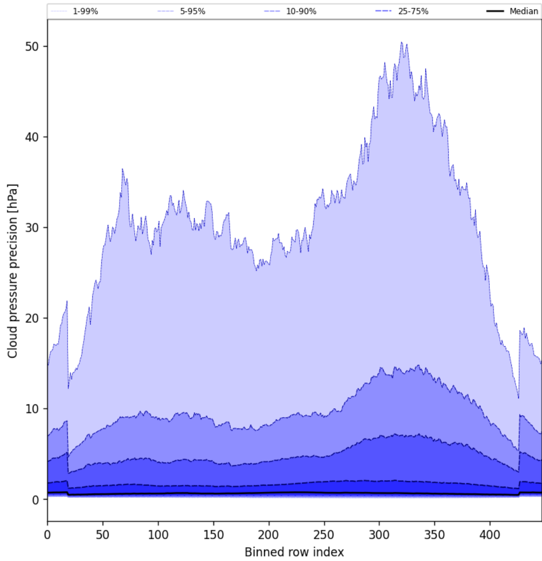
Figure 48: Along track statistics of “Cloud pressure precision” for 2025-05-24 to 2025-05-26
