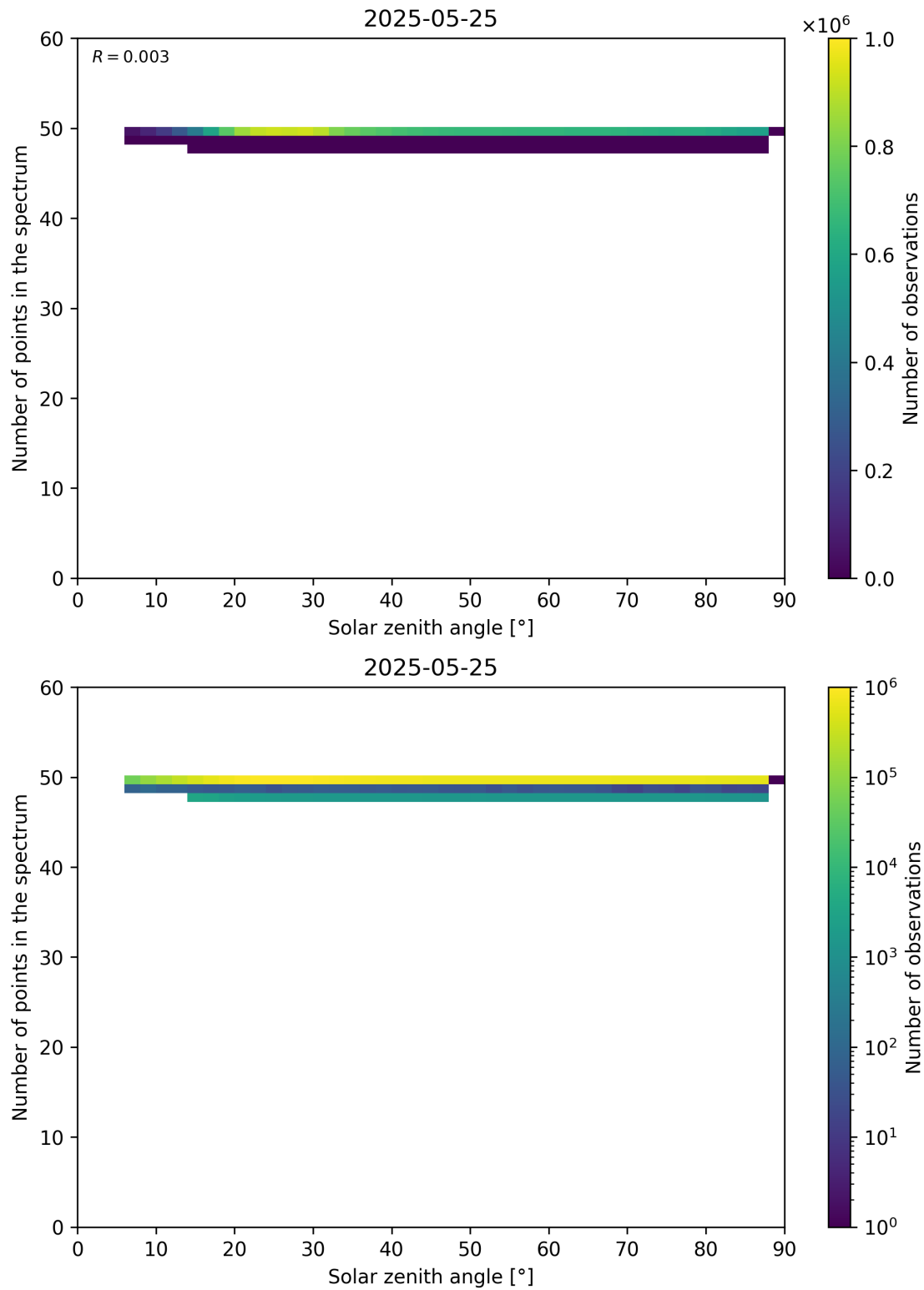
Figure 115: Scatter density plot of “Solar zenith angle” against “Number of points in the spectrum” for 2025-05-24 to 2025-05-26.
