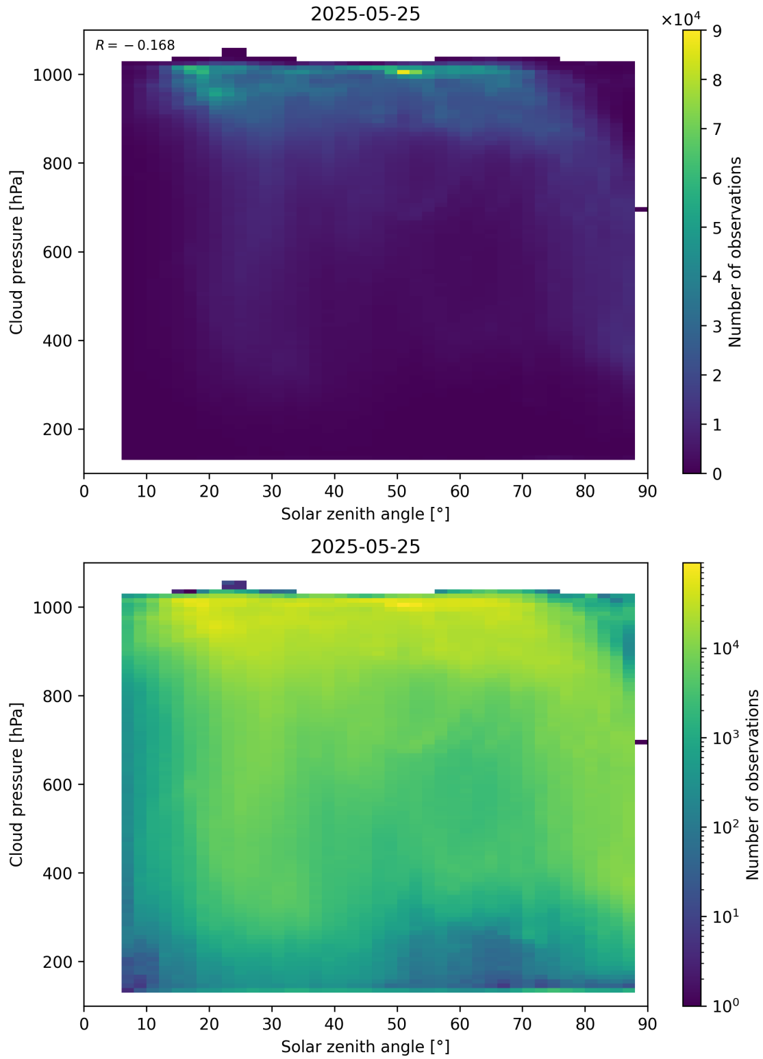
Figure 111: Scatter density plot of “Solar zenith angle” against “Cloud pressure” for 2025-05-24 to 2025-05-26.
