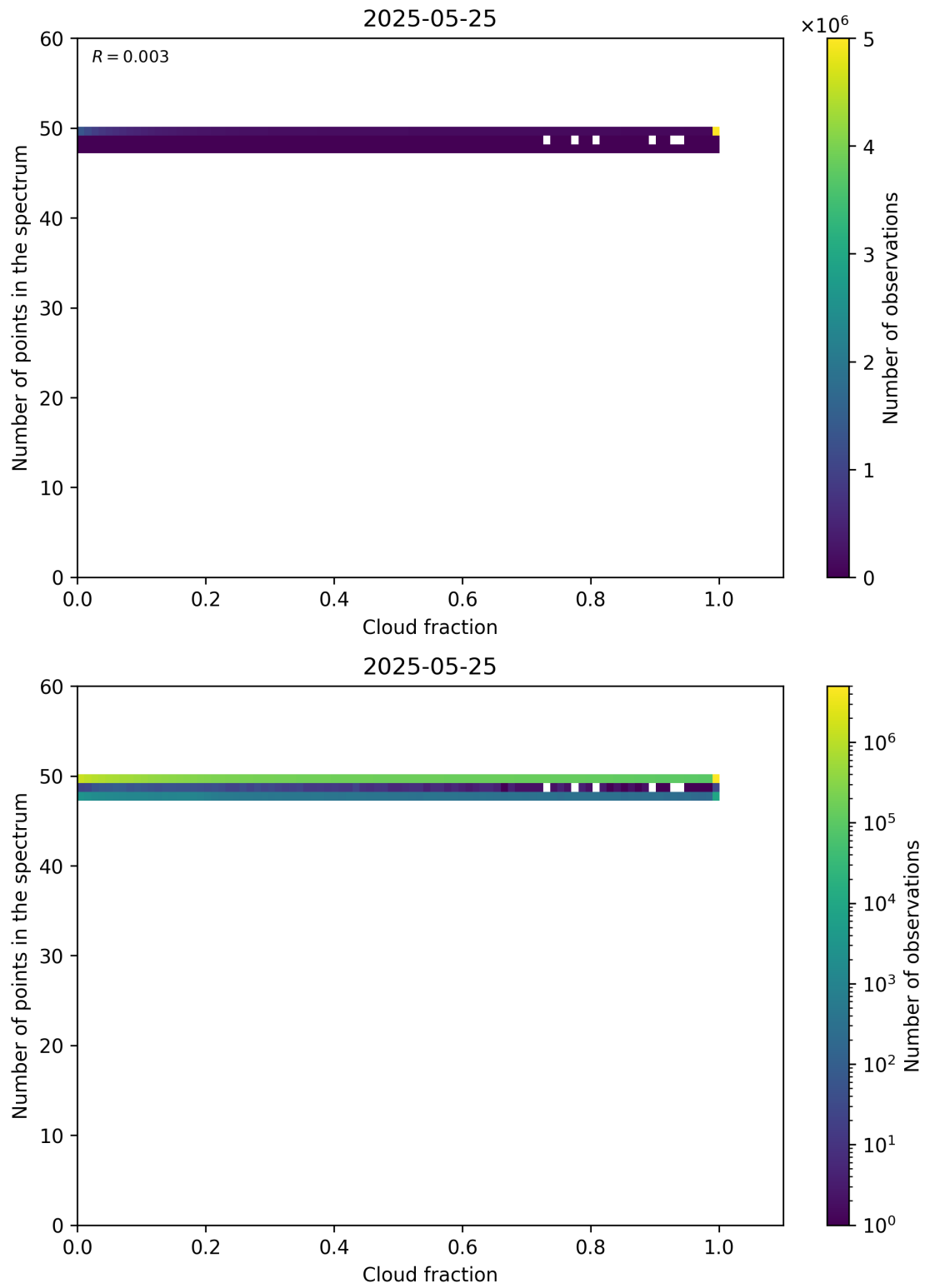
Figure 74: Scatter density plot of “Cloud fraction” against “Number of points in the spectrum” for 2025-05-24 to 2025-05-26.
