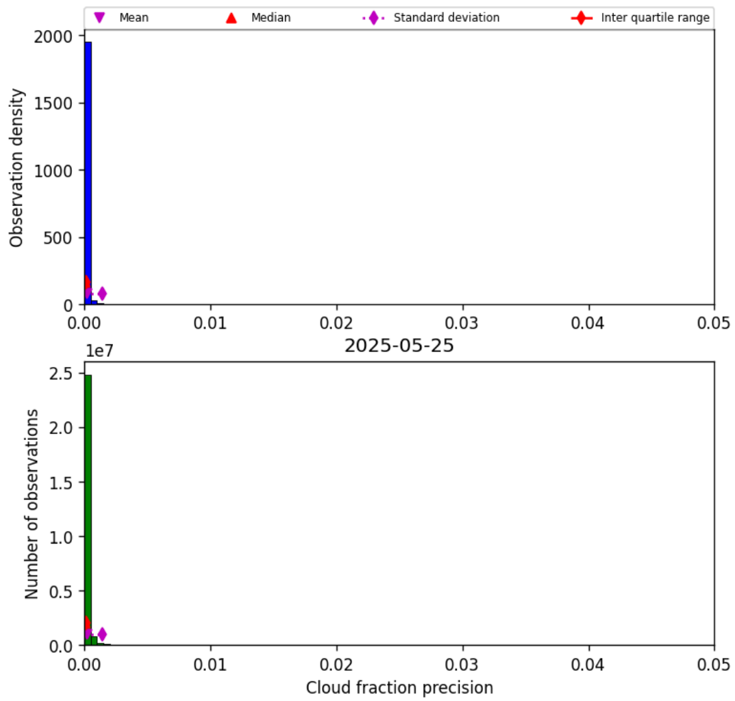
Figure 33: Histogram of “Cloud fraction precision” for 2025-05-24 to 2025-05-26
