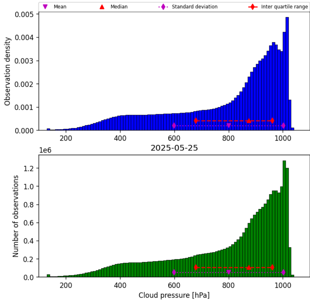
Figure 30: Histogram of “Cloud pressure” for 2025-05-24 to 2025-05-26
