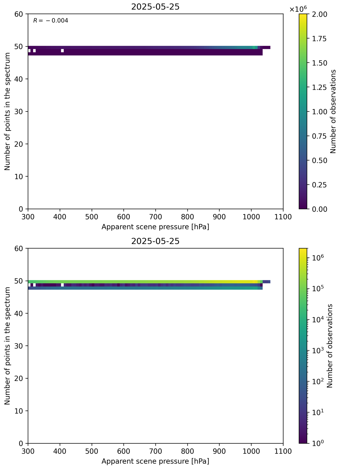
Figure 66: Scatter density plot of “Apparent scene pressure” against “Number of points in the spectrum” for 2025-05-24 to 2025-05-26.
