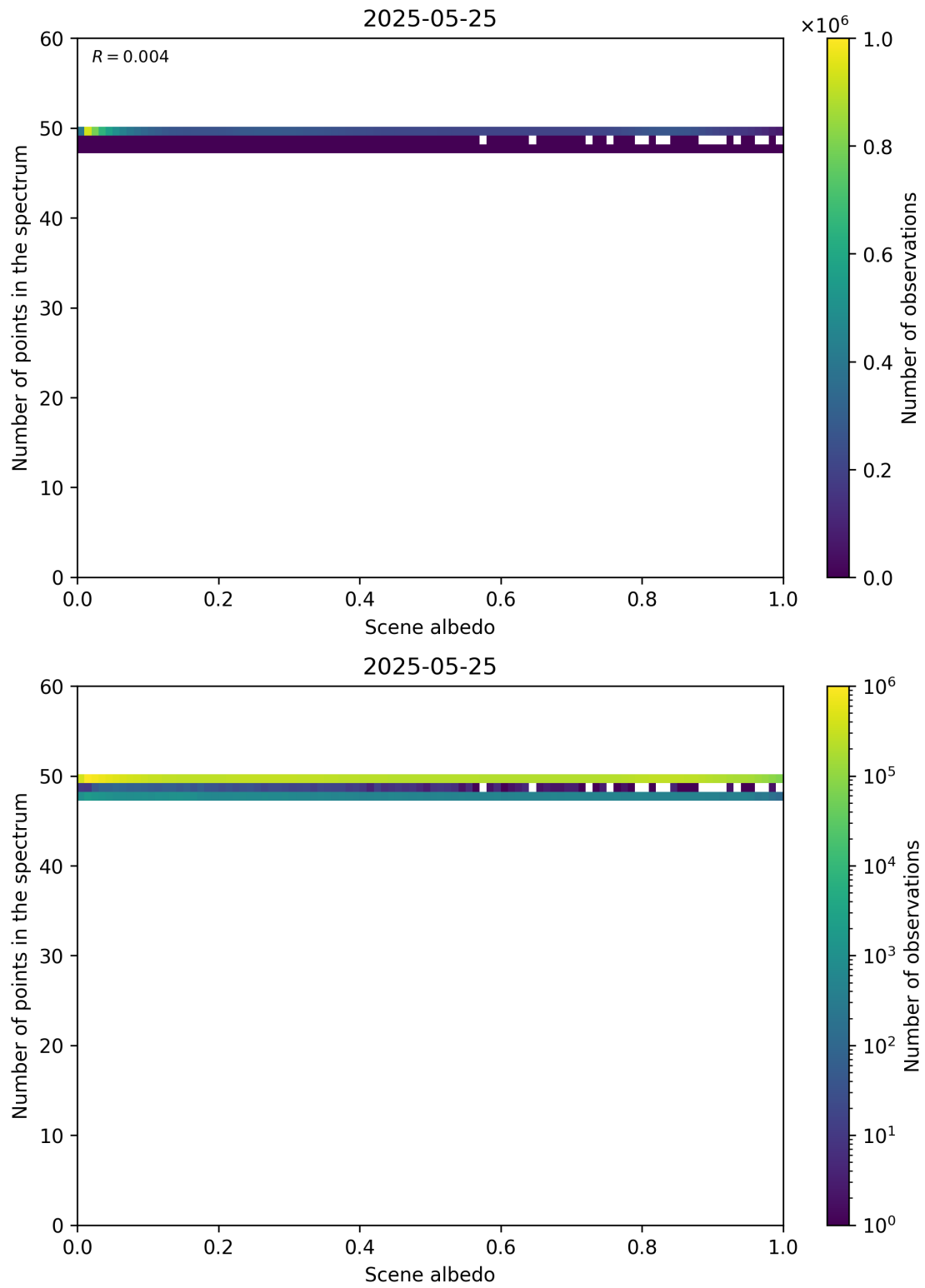
Figure 106: Scatter density plot of “Scene albedo” against “Number of points in the spectrum” for 2025-05-24 to 2025-05-26.
