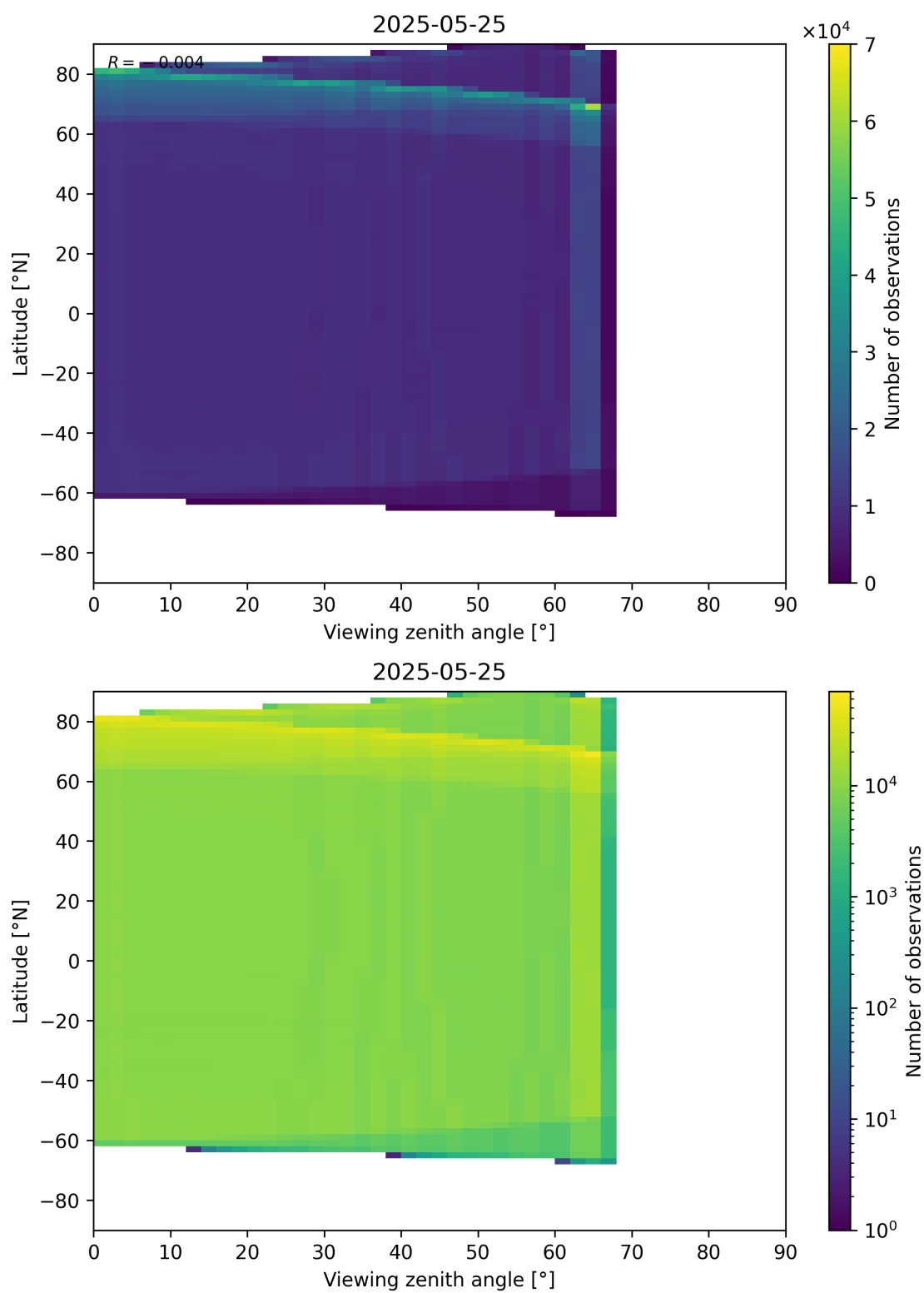
Figure 123: Scatter density plot of “Viewing zenith angle” against “Latitude” for 2025-05-24 to 2025-05-26.
