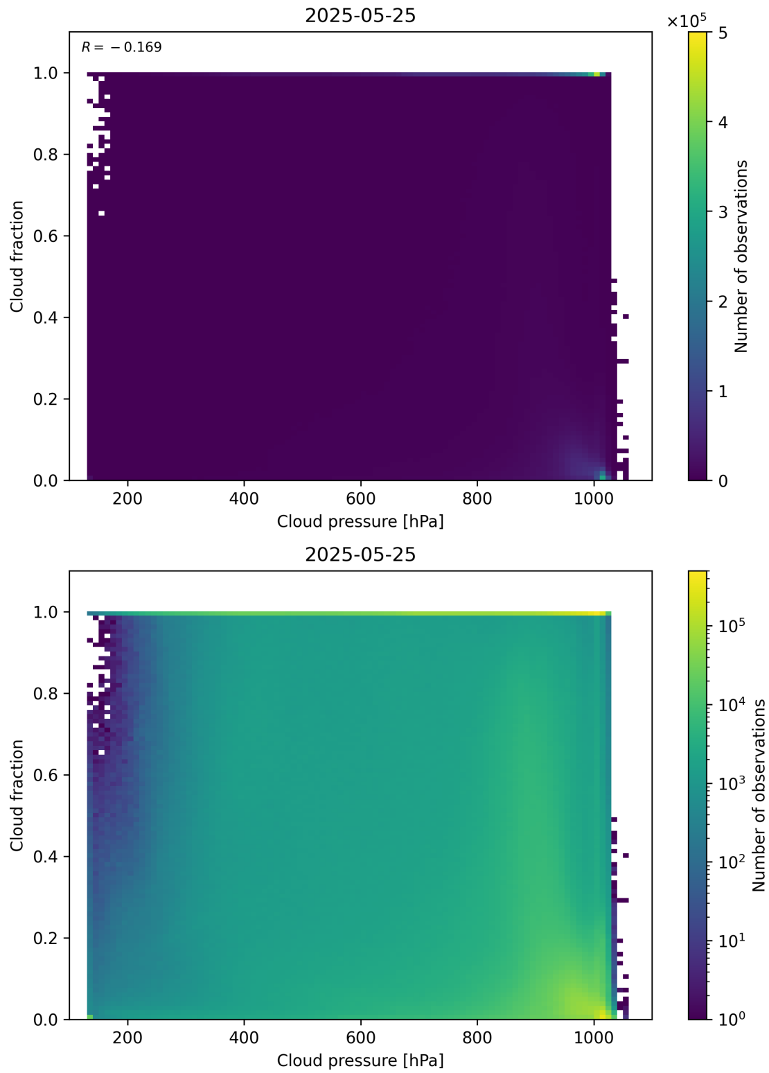
Figure 79: Scatter density plot of “Cloud pressure” against “Cloud fraction” for 2025-05-24 to 2025-05-26.
