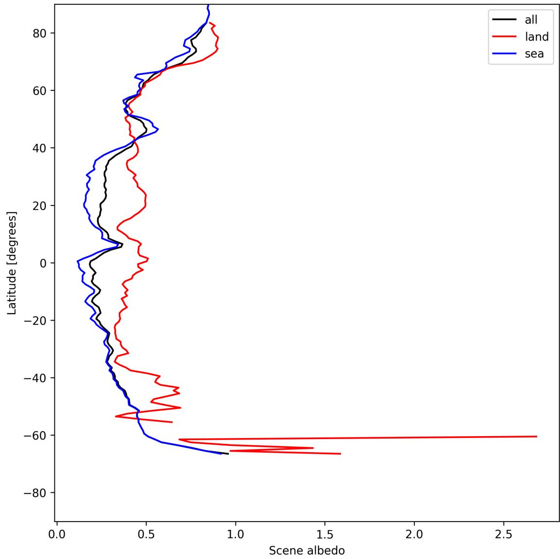
Figure 17: Zonal average of “Scene albedo” for 2025-05-24 to 2025-05-26.
