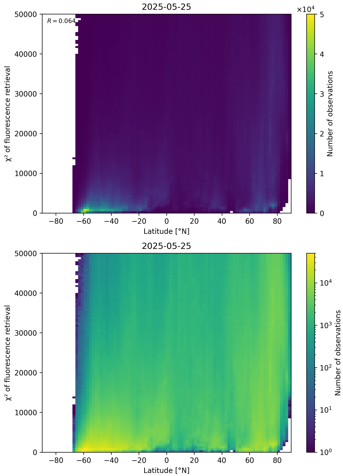
Figure 89: Scatter density plot of “Latitude” against “ \chi^2 of fluorescence retrieval” for 2025-05-24 to 2025-05-26.
