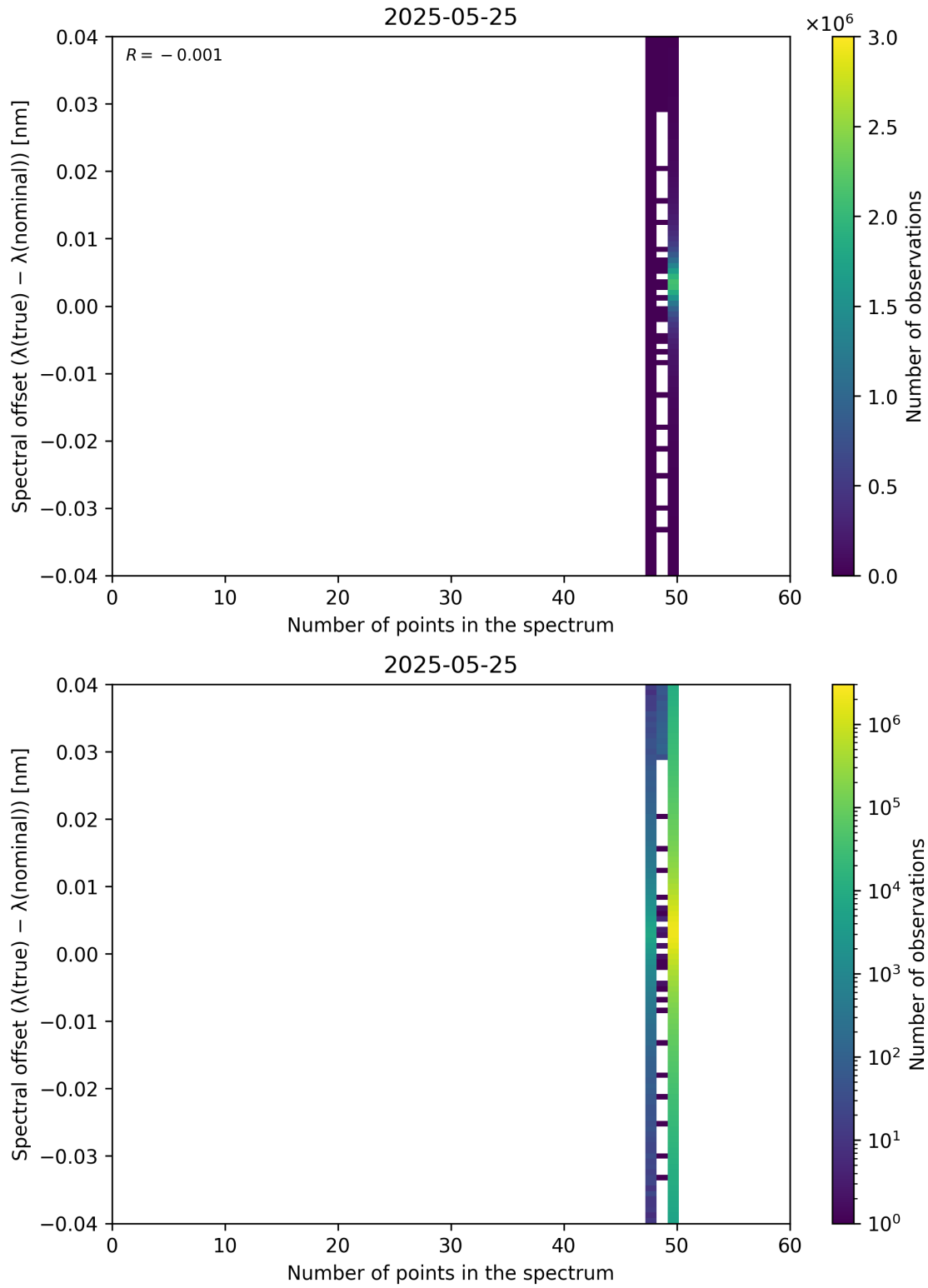
Figure 101: Scatter density plot of “Number of points in the spectrum” against “Spectral offset ( \lambda_{\text{true}} - \lambda_{\text{nominal}} )” for 2025-05-24 to 2025-05-26.
