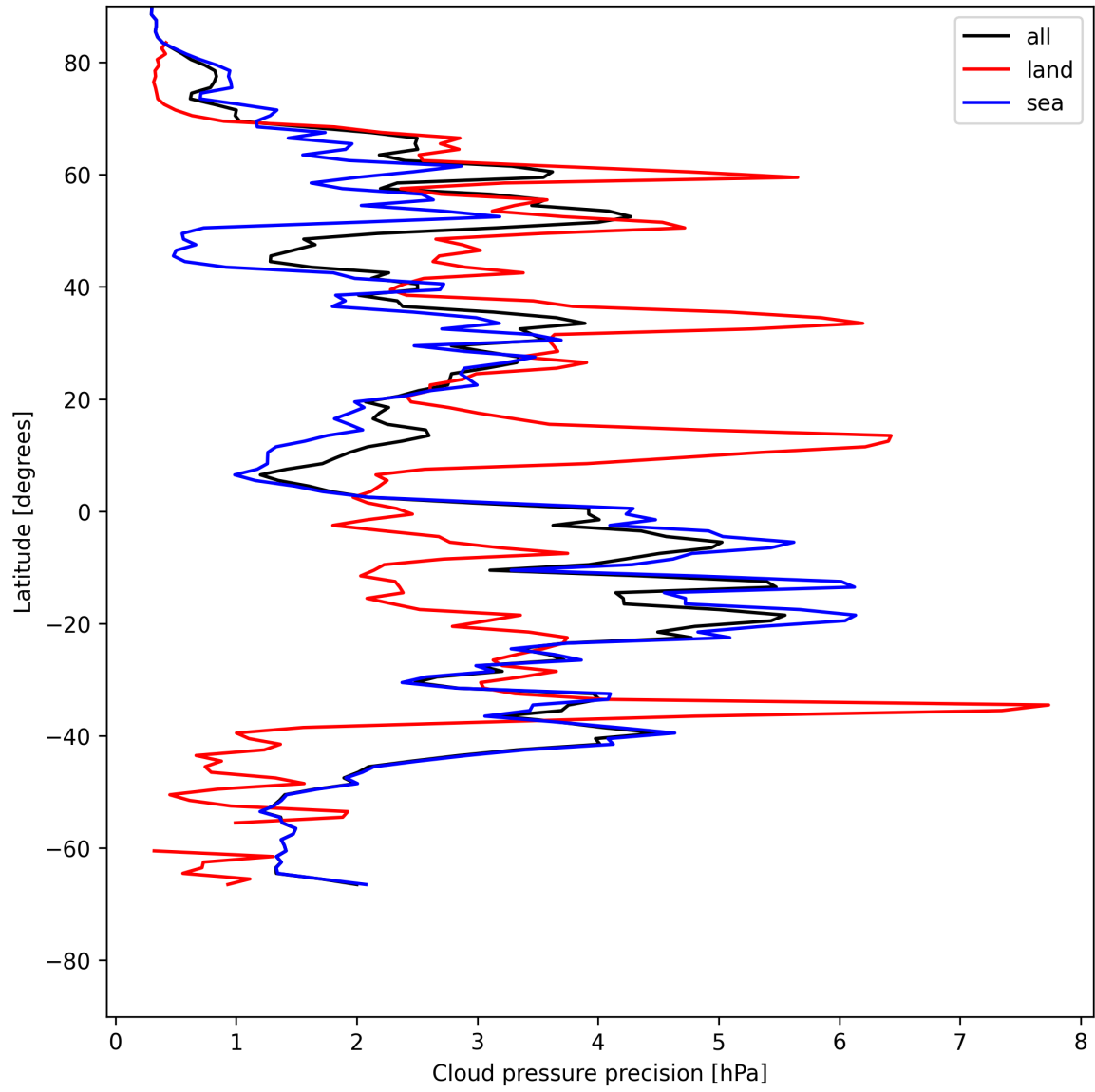
Figure 14: Zonal average of “Cloud pressure precision” for 2025-05-24 to 2025-05-26.
