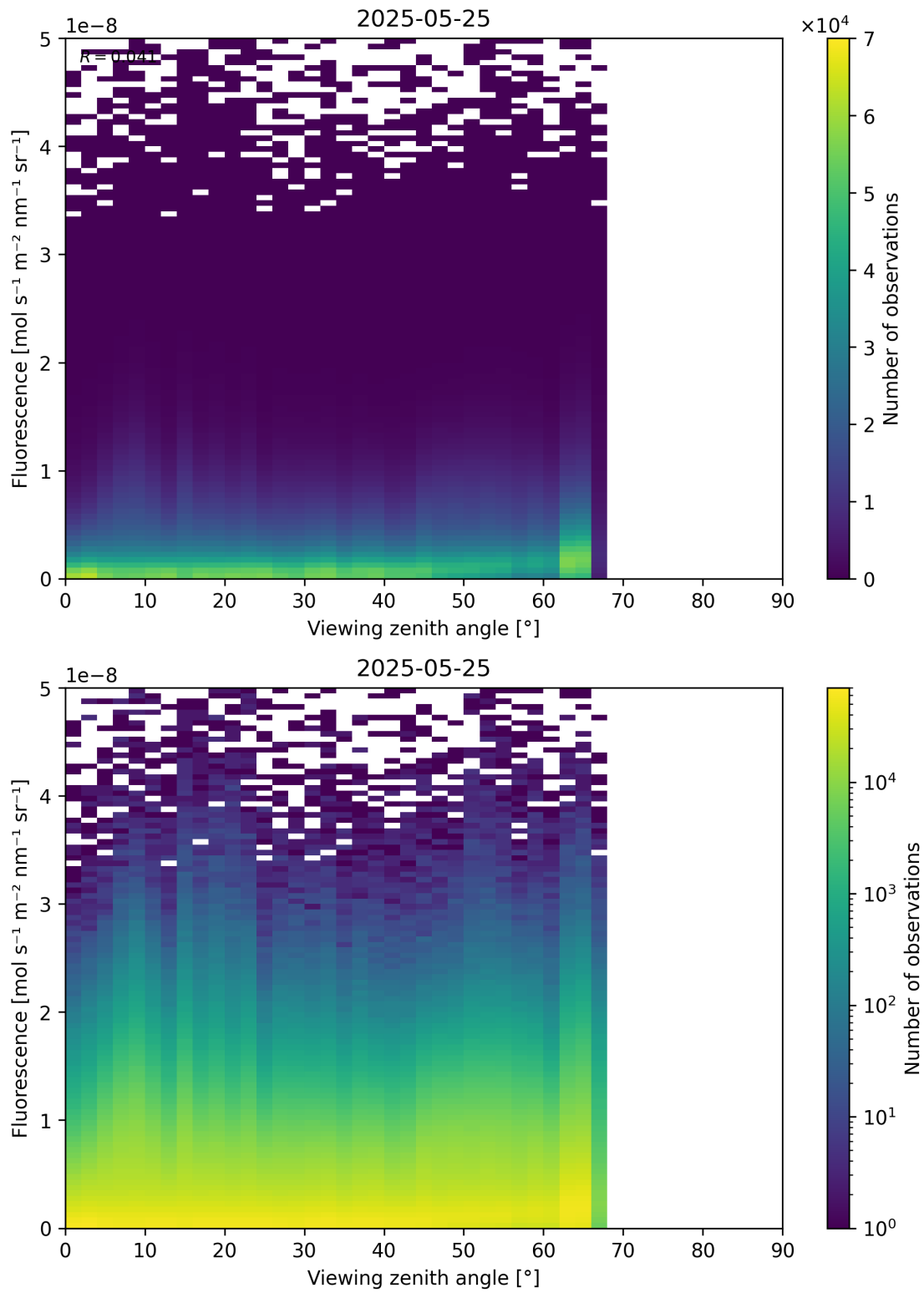
Figure 122: Scatter density plot of “Viewing zenith angle” against “Fluorescence” for 2025-05-24 to 2025-05-26.
