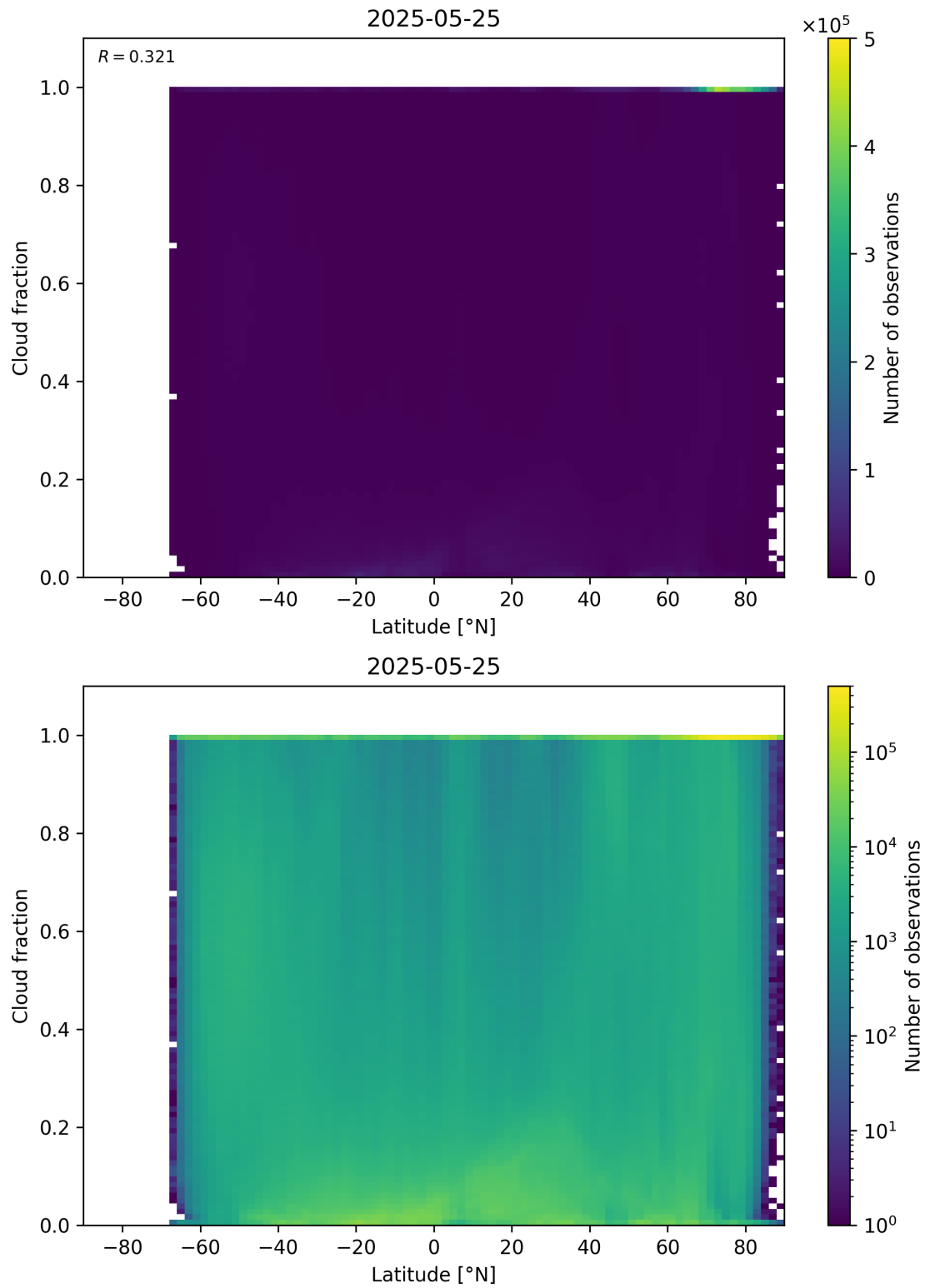
Figure 90: Scatter density plot of “Latitude” against “Cloud fraction” for 2025-05-24 to 2025-05-26.
