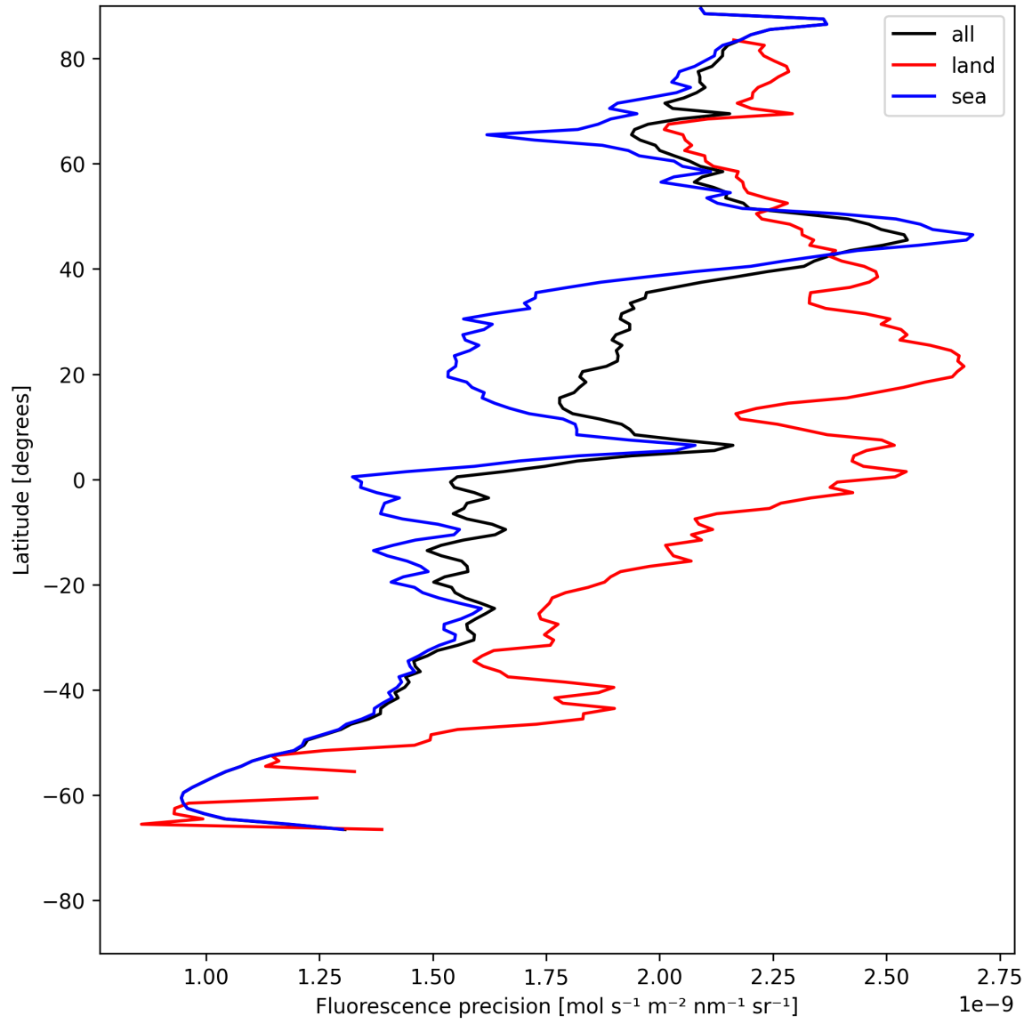
Figure 24: Zonal average of “Fluorescence precision” for 2025-05-24 to 2025-05-26.
