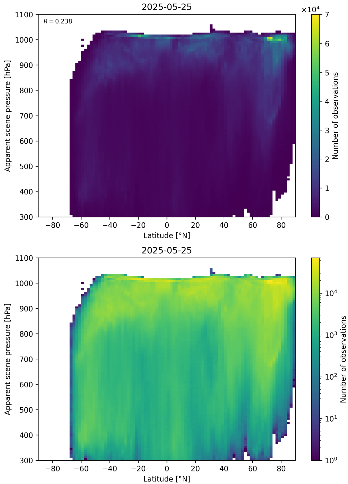
Figure 88: Scatter density plot of “Latitude” against “Apparent scene pressure” for 2025-05-24 to 2025-05-26.
