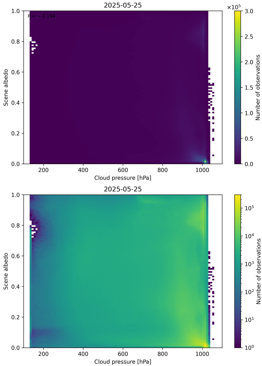
Figure 83: Scatter density plot of “Cloud pressure” against “Scene albedo” for 2025-05-24 to 2025-05-26.
