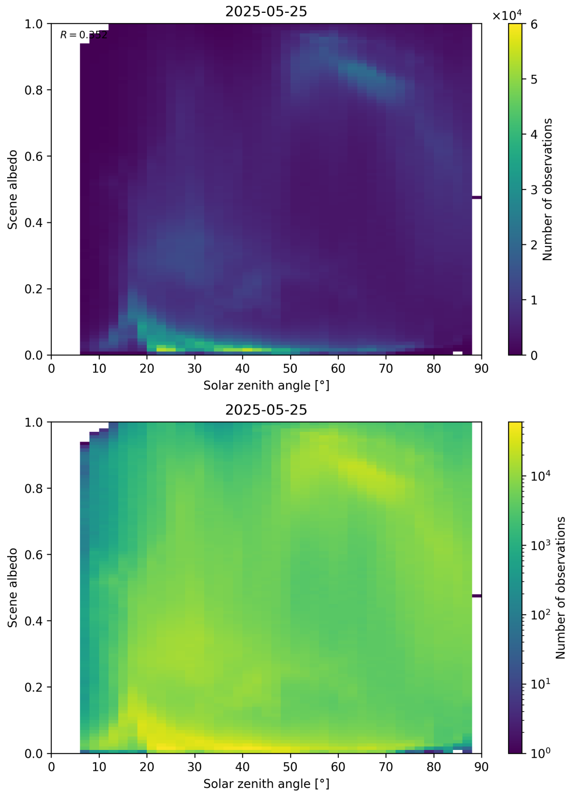
Figure 116: Scatter density plot of “Solar zenith angle” against “Scene albedo” for 2025-05-24 to 2025-05-26.
