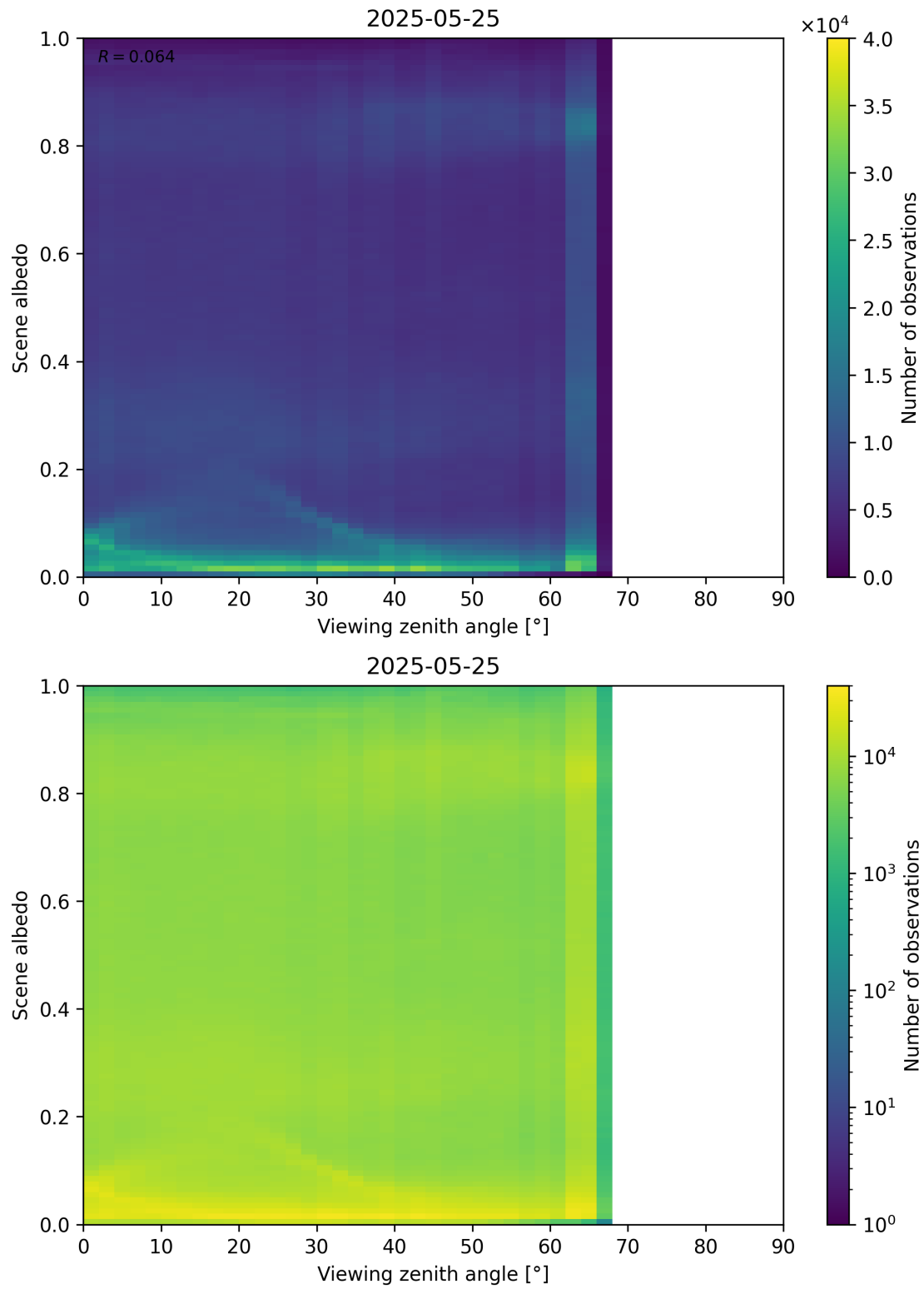
Figure 126: Scatter density plot of “Viewing zenith angle” against “Scene albedo” for 2025-05-24 to 2025-05-26.
