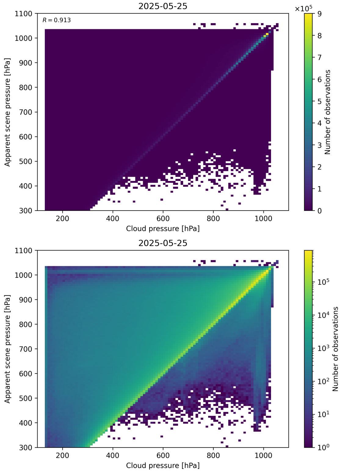
Figure 77: Scatter density plot of “Cloud pressure” against “Apparent scene pressure” for 2025-05-24 to 2025-05-26.
