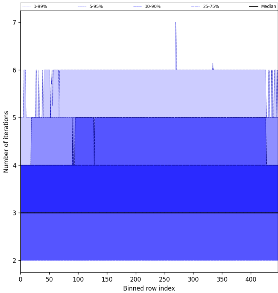
Figure 56: Along track statistics of “Number of iterations” for 2025-05-24 to 2025-05-26
