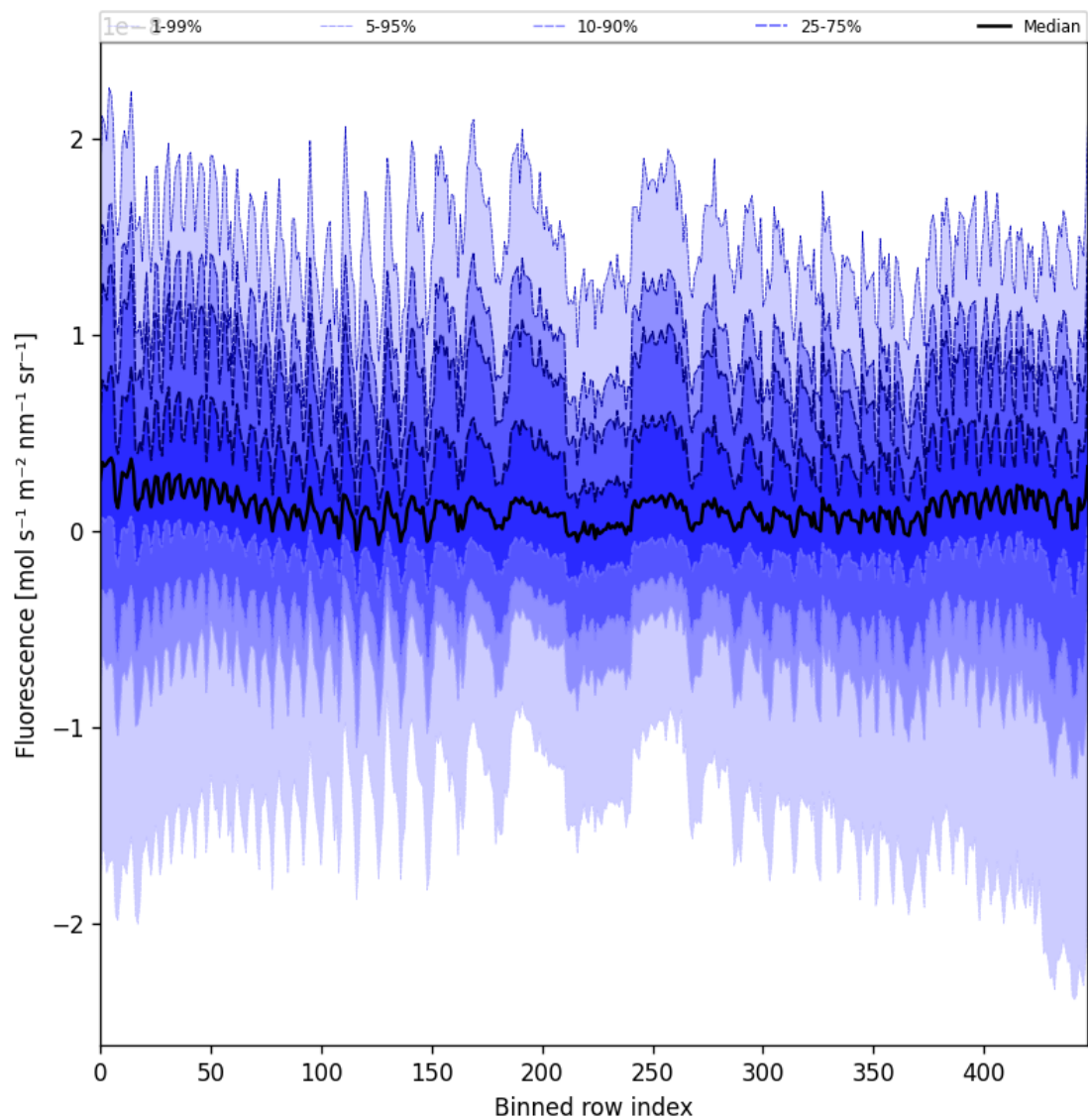
Figure 57: Along track statistics of "Fluorescence" for 2025-05-24 to 2025-05-26
