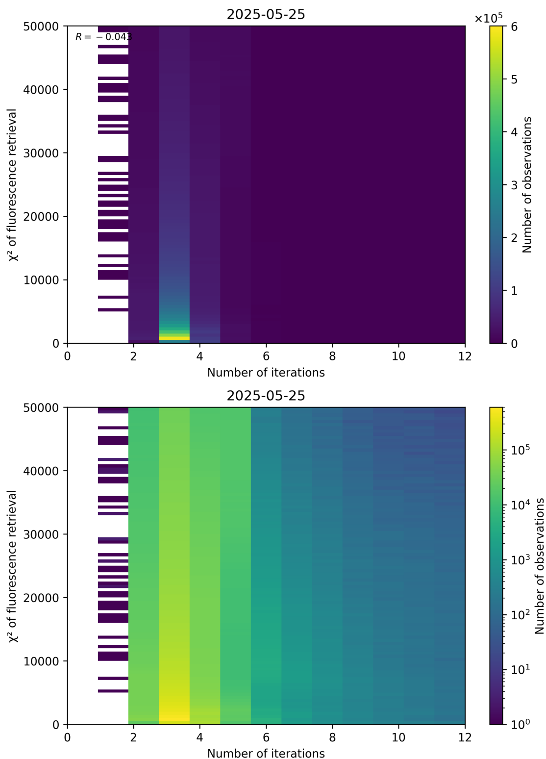
Figure 97: Scatter density plot of “Number of iterations” against “ \chi^2 of fluorescence retrieval” for 2025-05-24 to 2025-05-26.
