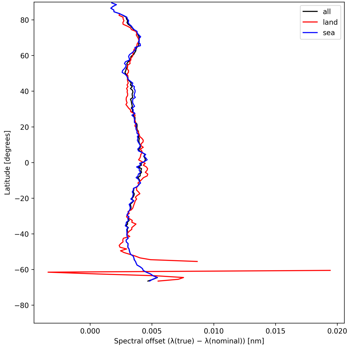
Figure 28: Zonal average of “Spectral offset ( \lambda_{\text{true}} - \lambda_{\text{nominal}} )” for 2025-05-24 to 2025-05-26.
