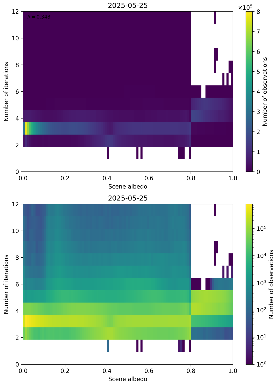
Figure 105: Scatter density plot of “Scene albedo” against “Number of iterations” for 2025-05-24 to 2025-05-26.
