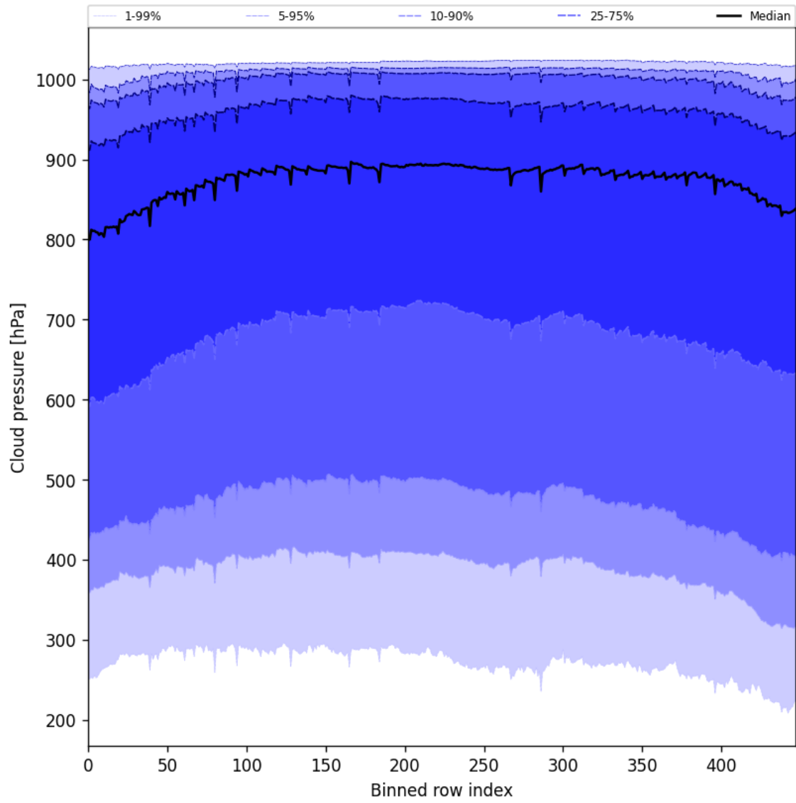
Figure 47: Along track statistics of “Cloud pressure” for 2025-05-24 to 2025-05-26
