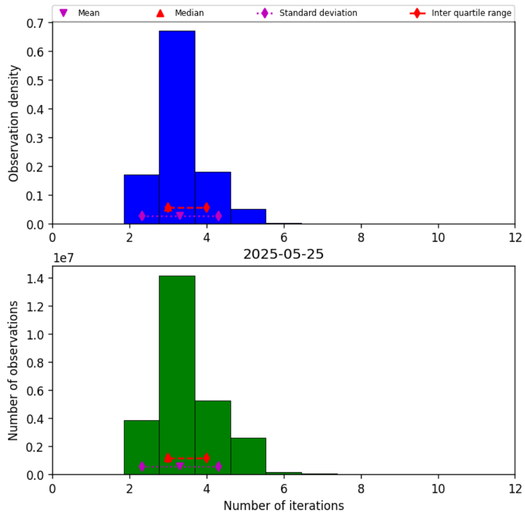
Figure 39: Histogram of “Number of iterations” for 2025-05-24 to 2025-05-26
