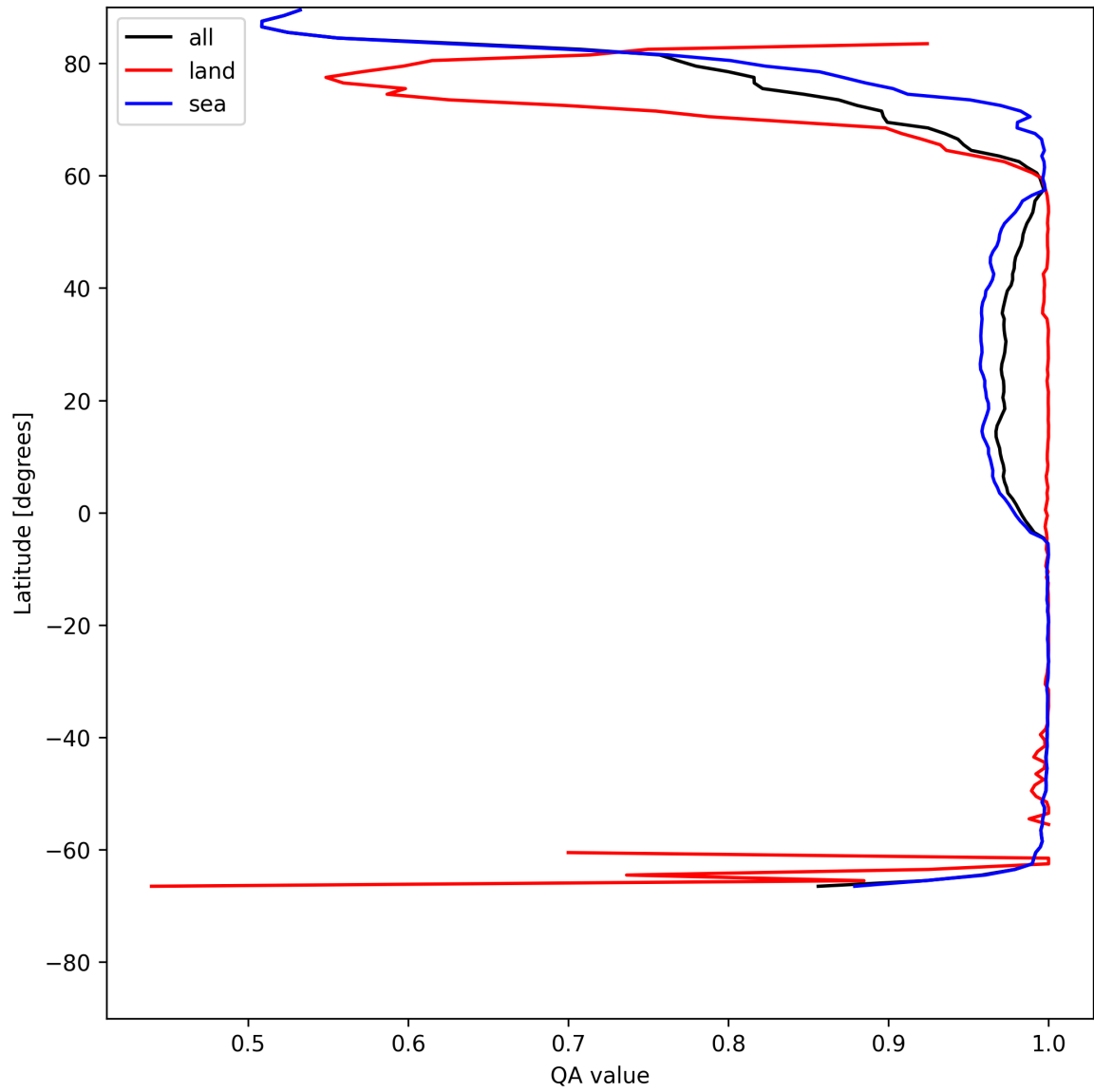
Figure 12: Zonal average of “QA value” for 2025-05-24 to 2025-05-26.
