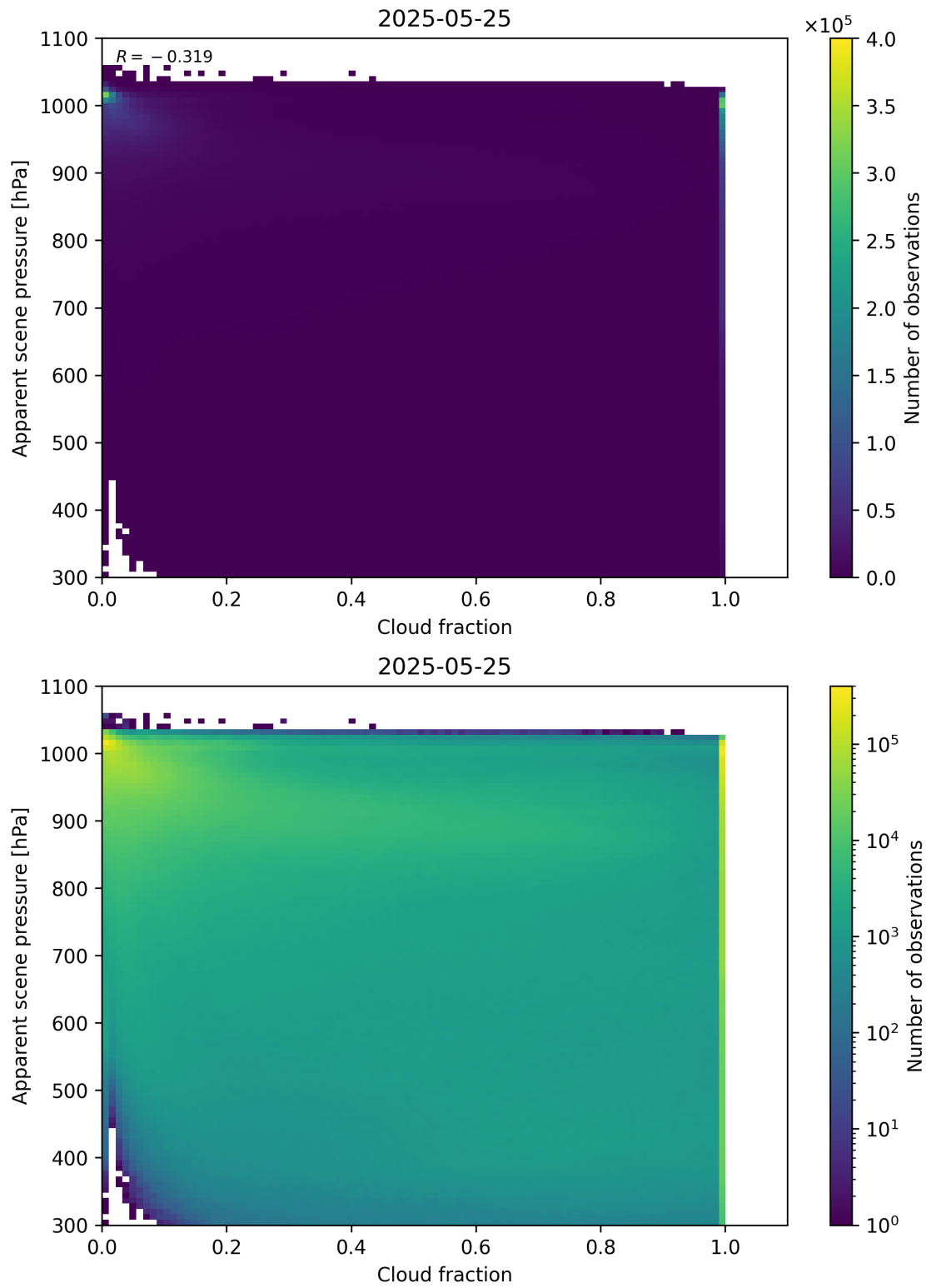
Figure 70: Scatter density plot of “Cloud fraction” against “Apparent scene pressure” for 2025-05-24 to 2025-05-26.
