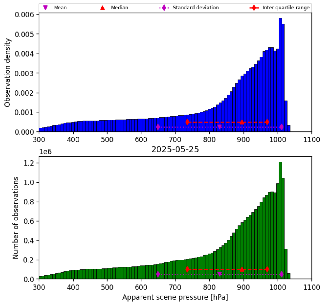
Figure 36: Histogram of “Apparent scene pressure” for 2025-05-24 to 2025-05-26
