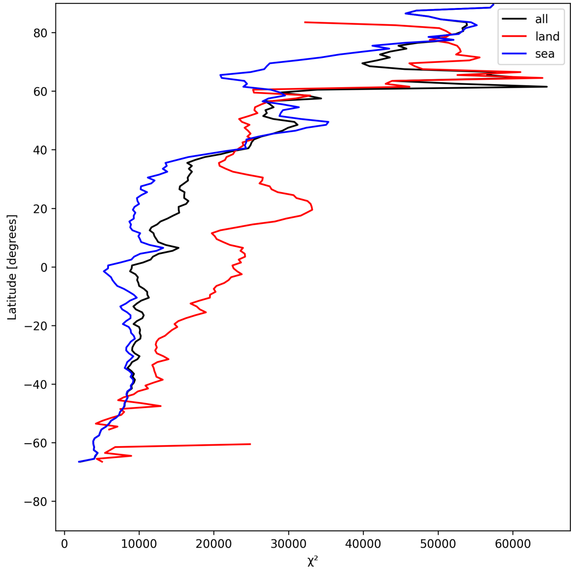
Figure 21: Zonal average of “ \chi^2 ” for 2025-05-24 to 2025-05-26.
