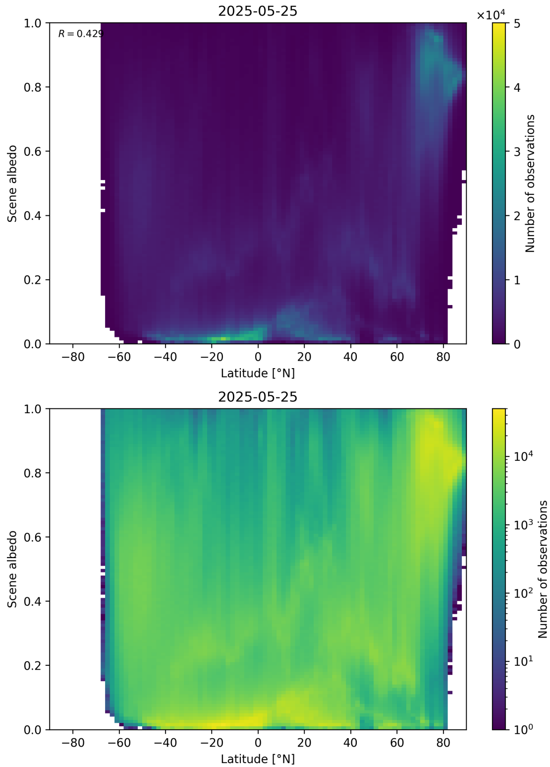
Figure 95: Scatter density plot of “Latitude” against “Scene albedo” for 2025-05-24 to 2025-05-26.
