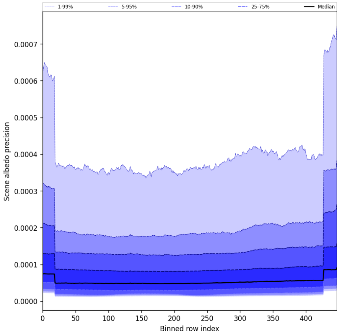
Figure 52: Along track statistics of “Scene albedo precision” for 2025-05-24 to 2025-05-26
