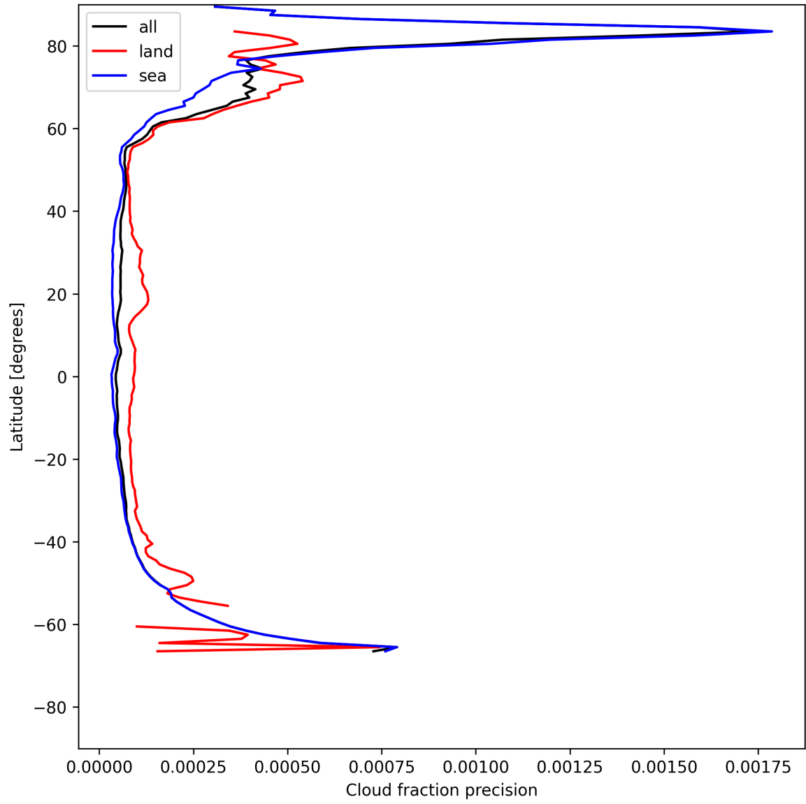
Figure 16: Zonal average of “Cloud fraction precision” for 2025-05-24 to 2025-05-26.
