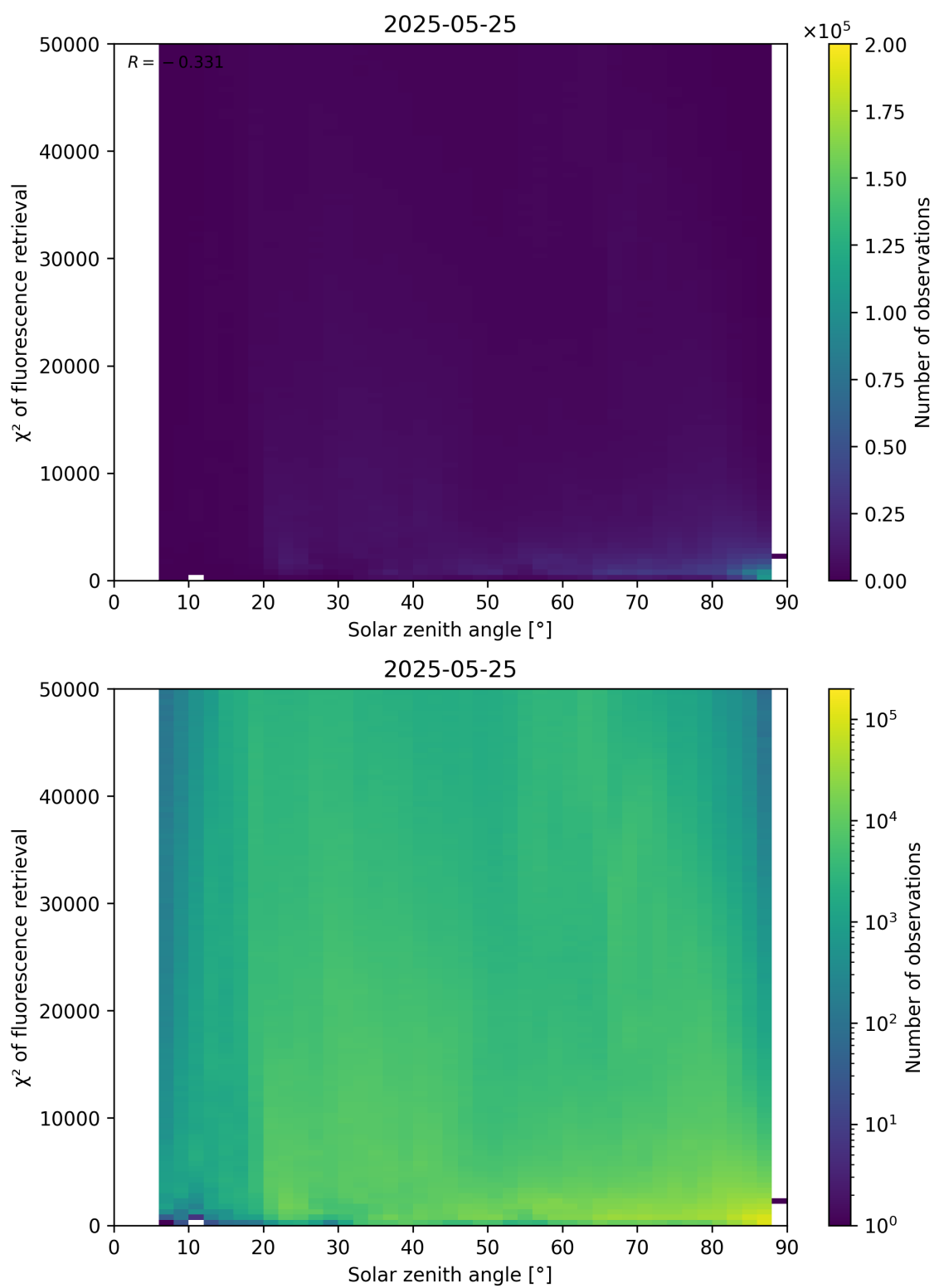
Figure 109: Scatter density plot of “Solar zenith angle” against “ \chi^2 of fluorescence retrieval” for 2025-05-24 to 2025-05-26.
