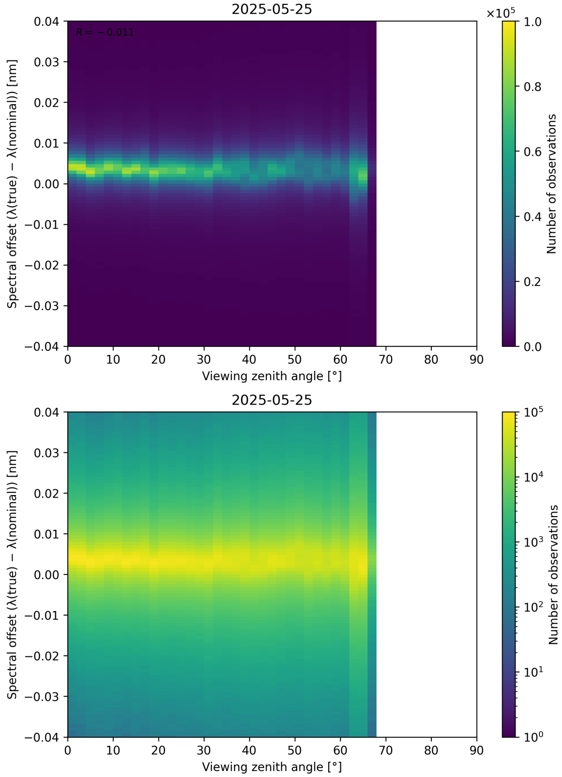
Figure 128: Scatter density plot of “Viewing zenith angle” against “Spectral offset ( \lambda_{\text{true}} - \lambda_{\text{nominal}} )” for 2025-05-24 to 2025-05-26.
