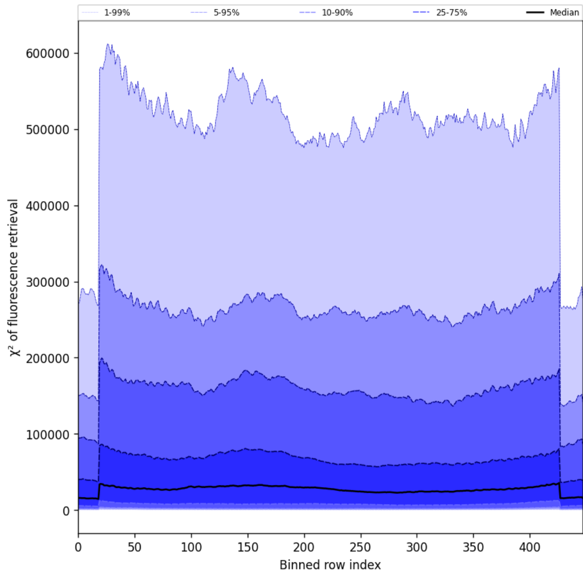
Figure 59: Along track statistics of “ \chi^2 of fluorescence retrieval” for 2025-05-24 to 2025-05-26
