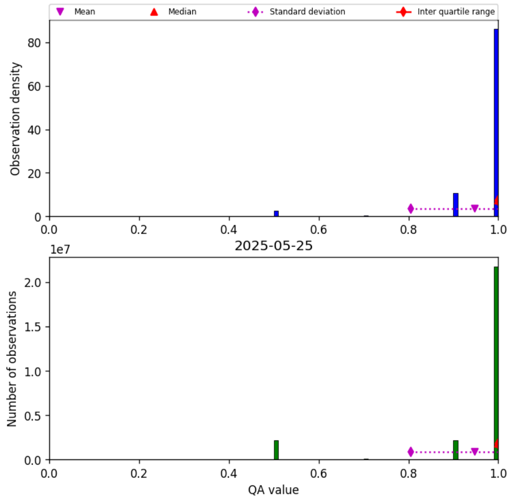
Figure 29: Histogram of “QA value” for 2025-05-24 to 2025-05-26
