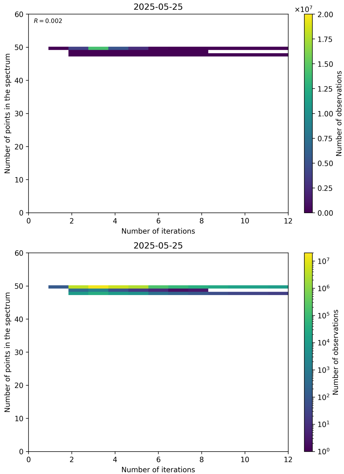
Figure 99: Scatter density plot of “Number of iterations” against “Number of points in the spectrum” for 2025-05-24 to 2025-05-26.
