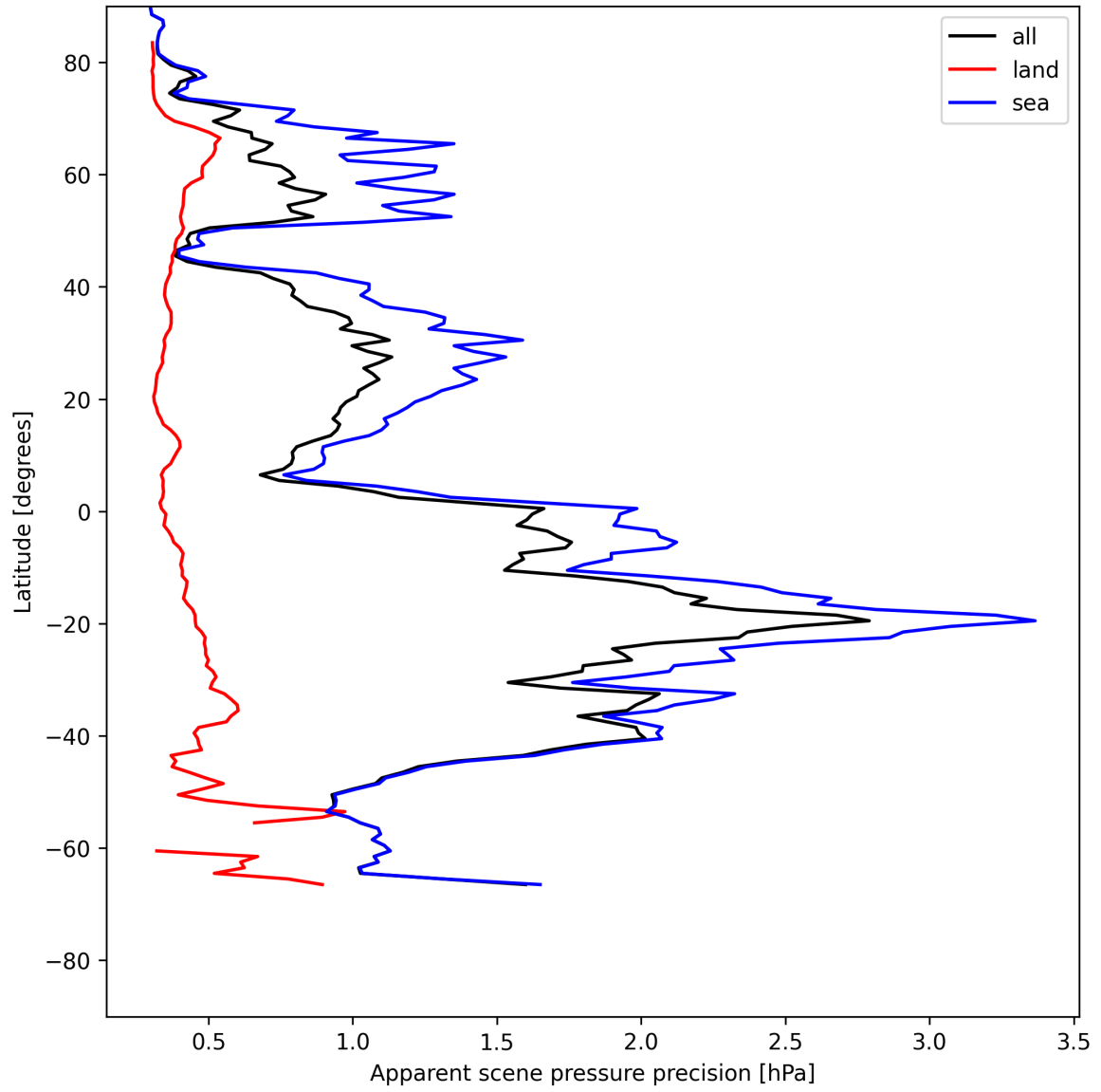
Figure 20: Zonal average of “Apparent scene pressure precision” for 2025-05-24 to 2025-05-26.
