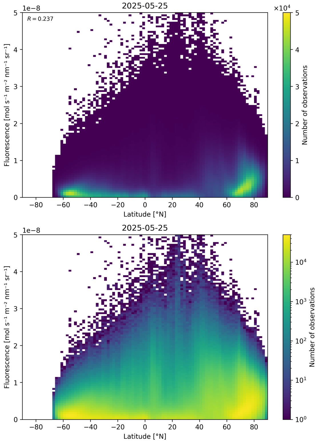
Figure 92: Scatter density plot of “Latitude” against “Fluorescence” for 2025-05-24 to 2025-05-26.
