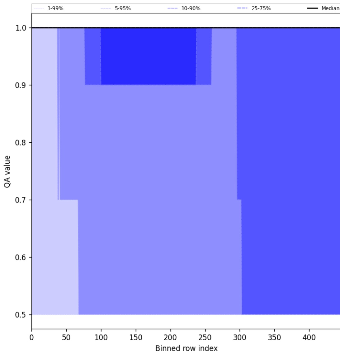
Figure 46: Along track statistics of “QA value” for 2025-05-24 to 2025-05-26
