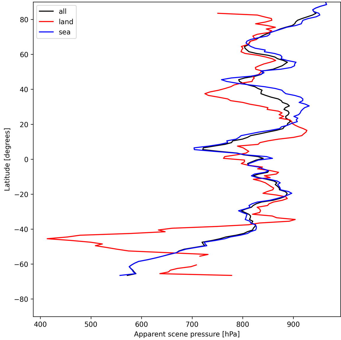
Figure 19: Zonal average of “Apparent scene pressure” for 2025-05-24 to 2025-05-26.
