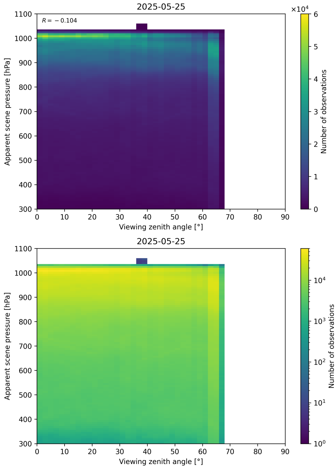
Figure 118: Scatter density plot of “Viewing zenith angle” against “Apparent scene pressure” for 2025-05-24 to 2025-05-26.
