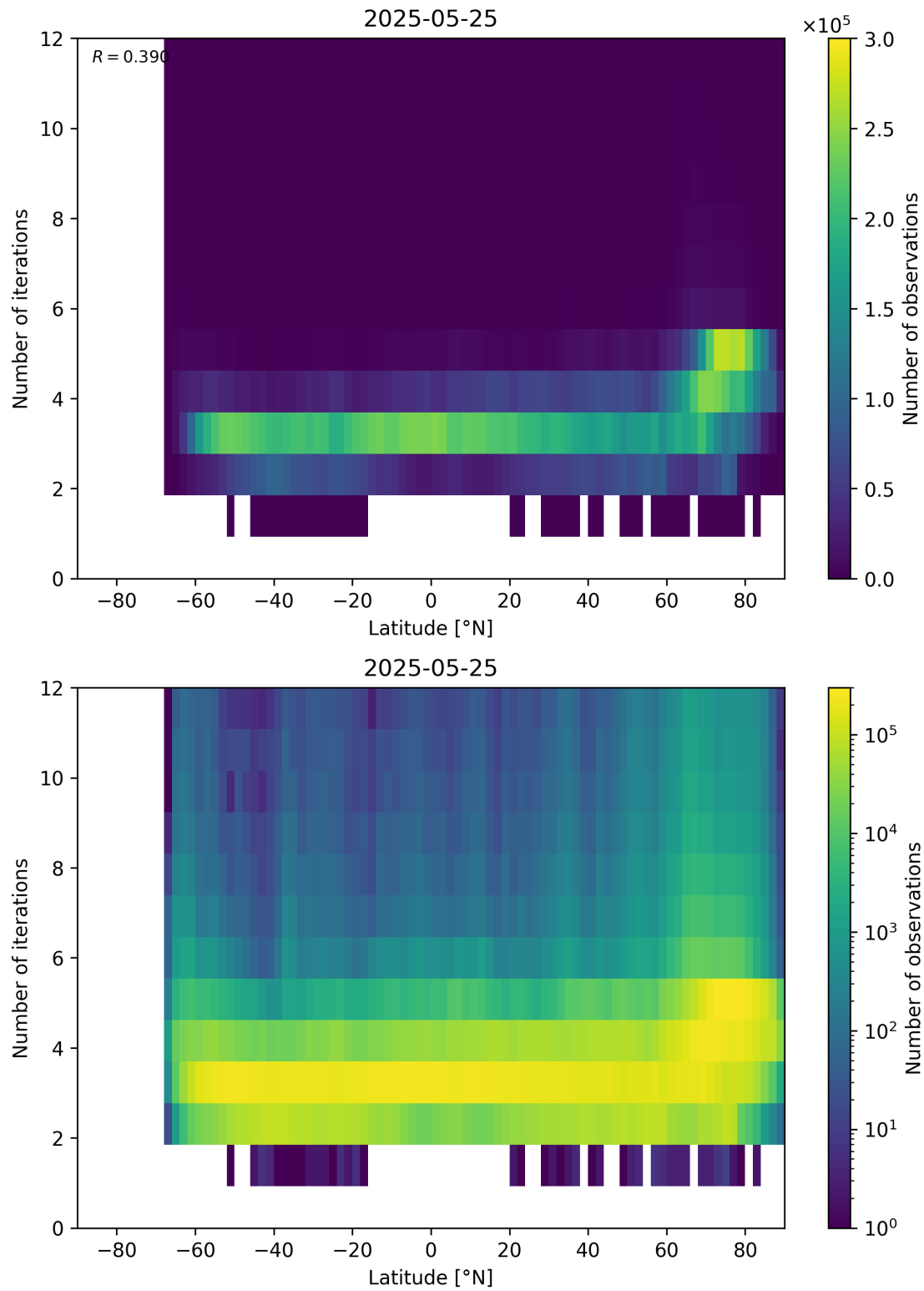
Figure 93: Scatter density plot of “Latitude” against “Number of iterations” for 2025-05-24 to 2025-05-26.
