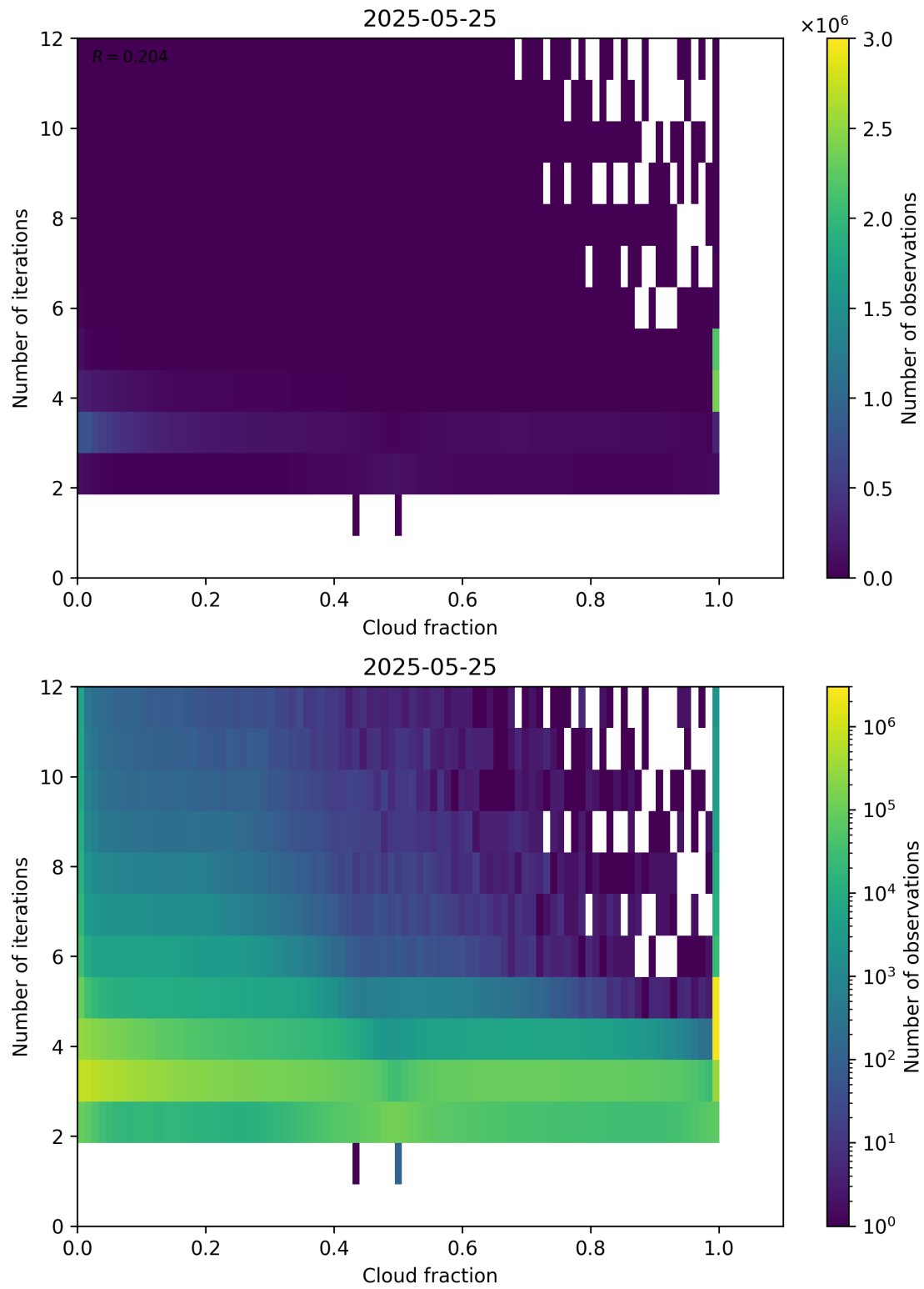
Figure 73: Scatter density plot of “Cloud fraction” against “Number of iterations” for 2025-05-24 to 2025-05-26.
