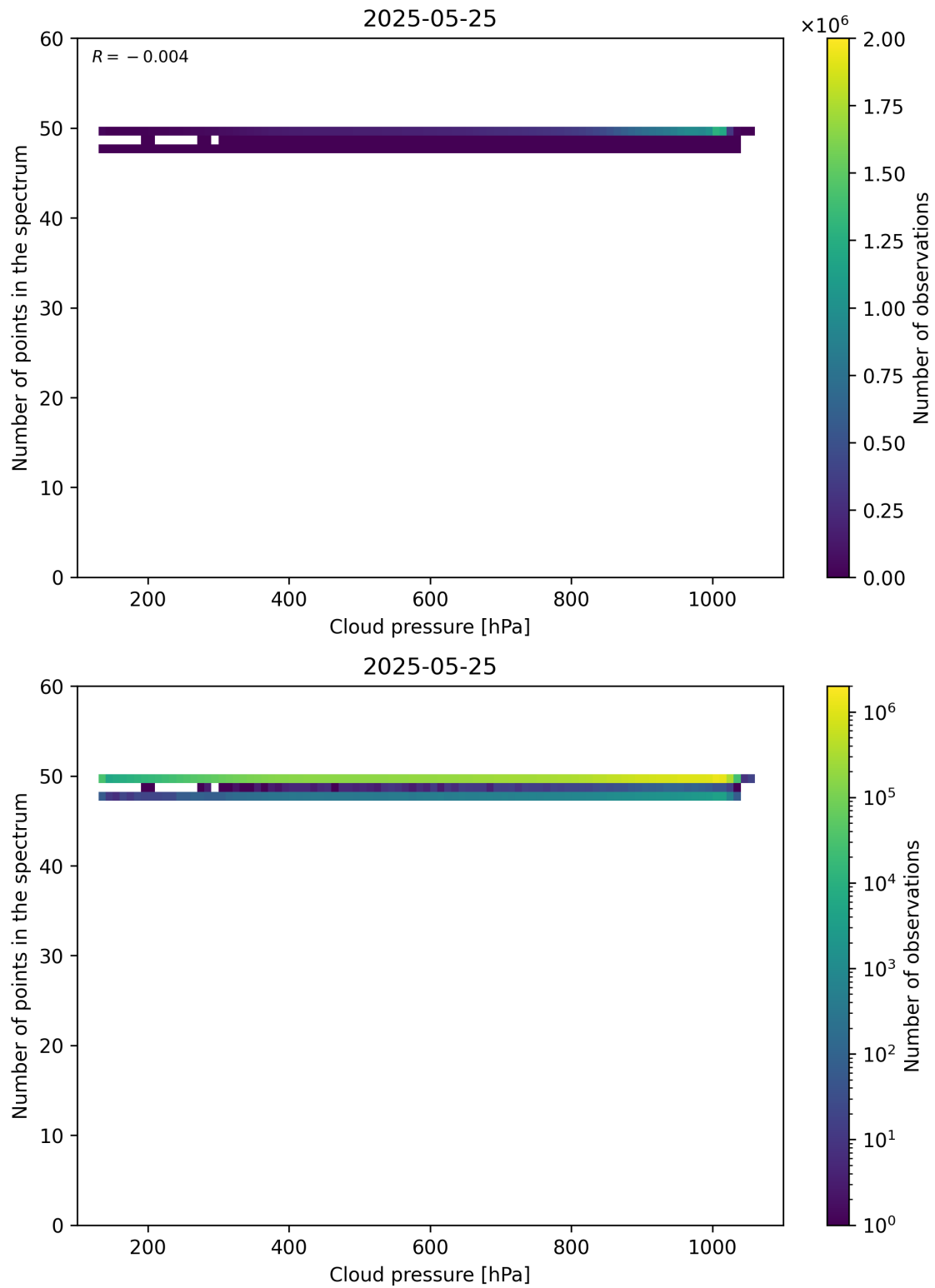
Figure 82: Scatter density plot of “Cloud pressure” against “Number of points in the spectrum” for 2025-05-24 to 2025-05-26.
