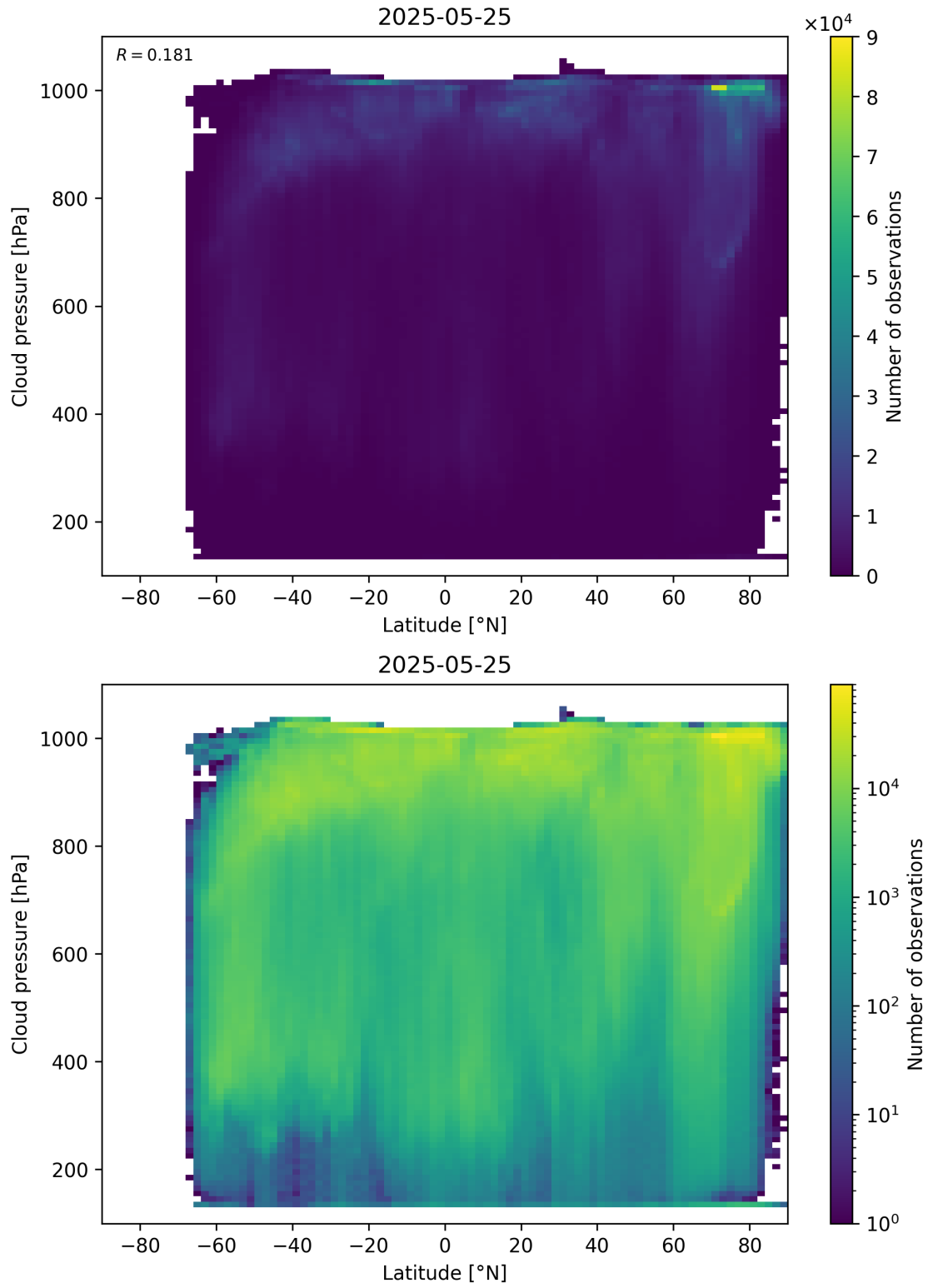
Figure 91: Scatter density plot of “Latitude” against “Cloud pressure” for 2025-05-24 to 2025-05-26.
