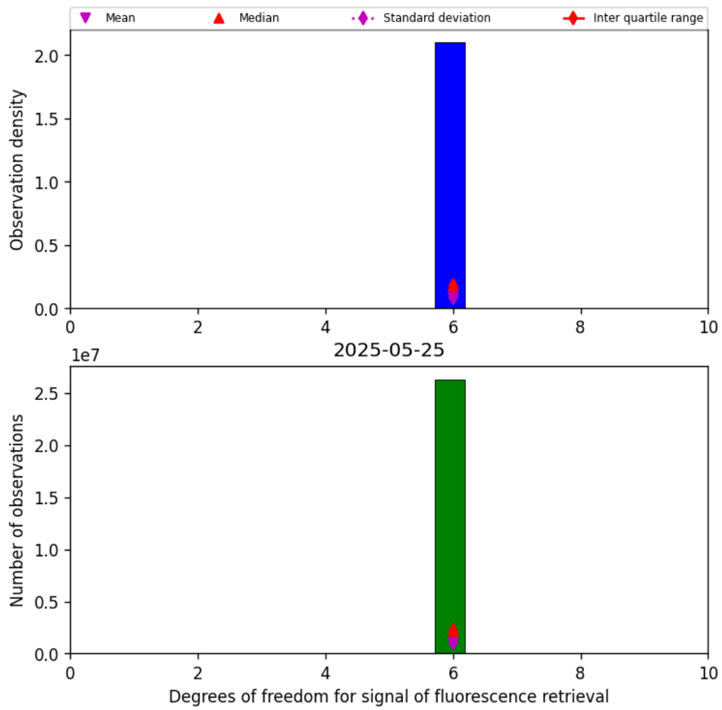
Figure 43: Histogram of "Degrees of freedom for signal of fluorescence retrieval" for 2025-05-24 to 2025-05-26
