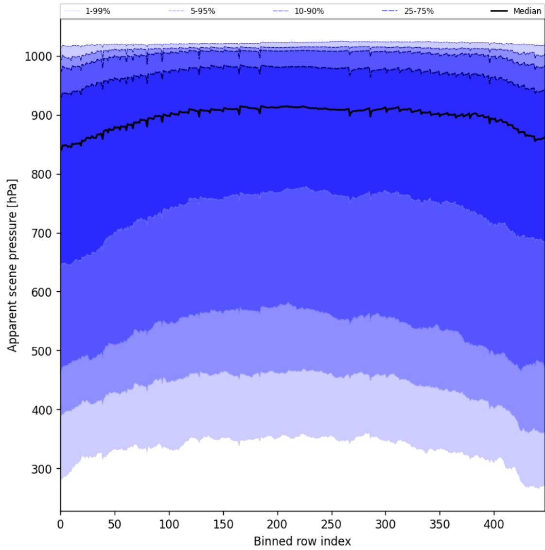
Figure 53: Along track statistics of “Apparent scene pressure” for 2025-05-24 to 2025-05-26
