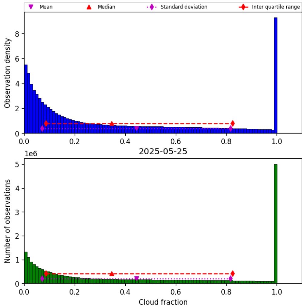
Figure 32: Histogram of “Cloud fraction” for 2025-05-24 to 2025-05-26
