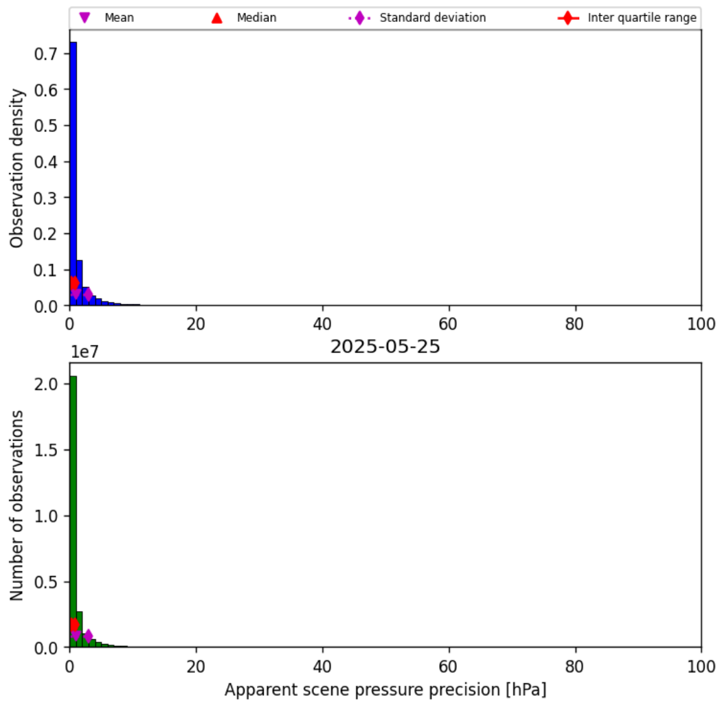
Figure 37: Histogram of “Apparent scene pressure precision” for 2025-05-24 to 2025-05-26
