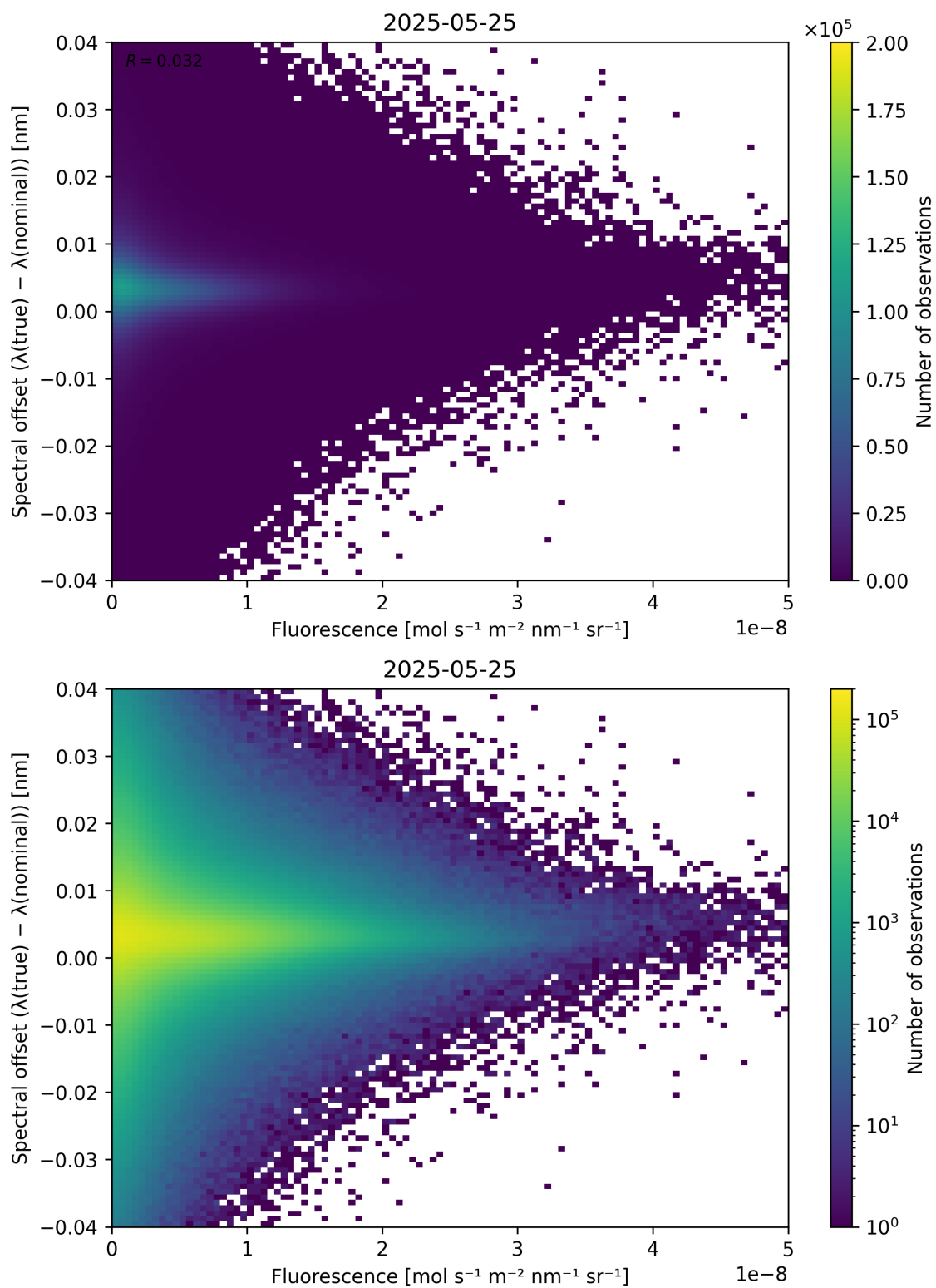
Figure 87: Scatter density plot of “Fluorescence” against “Spectral offset ( \lambda_{\text{true}} - \lambda_{\text{nominal}} )” for 2025-05-24 to 2025-05-26.
