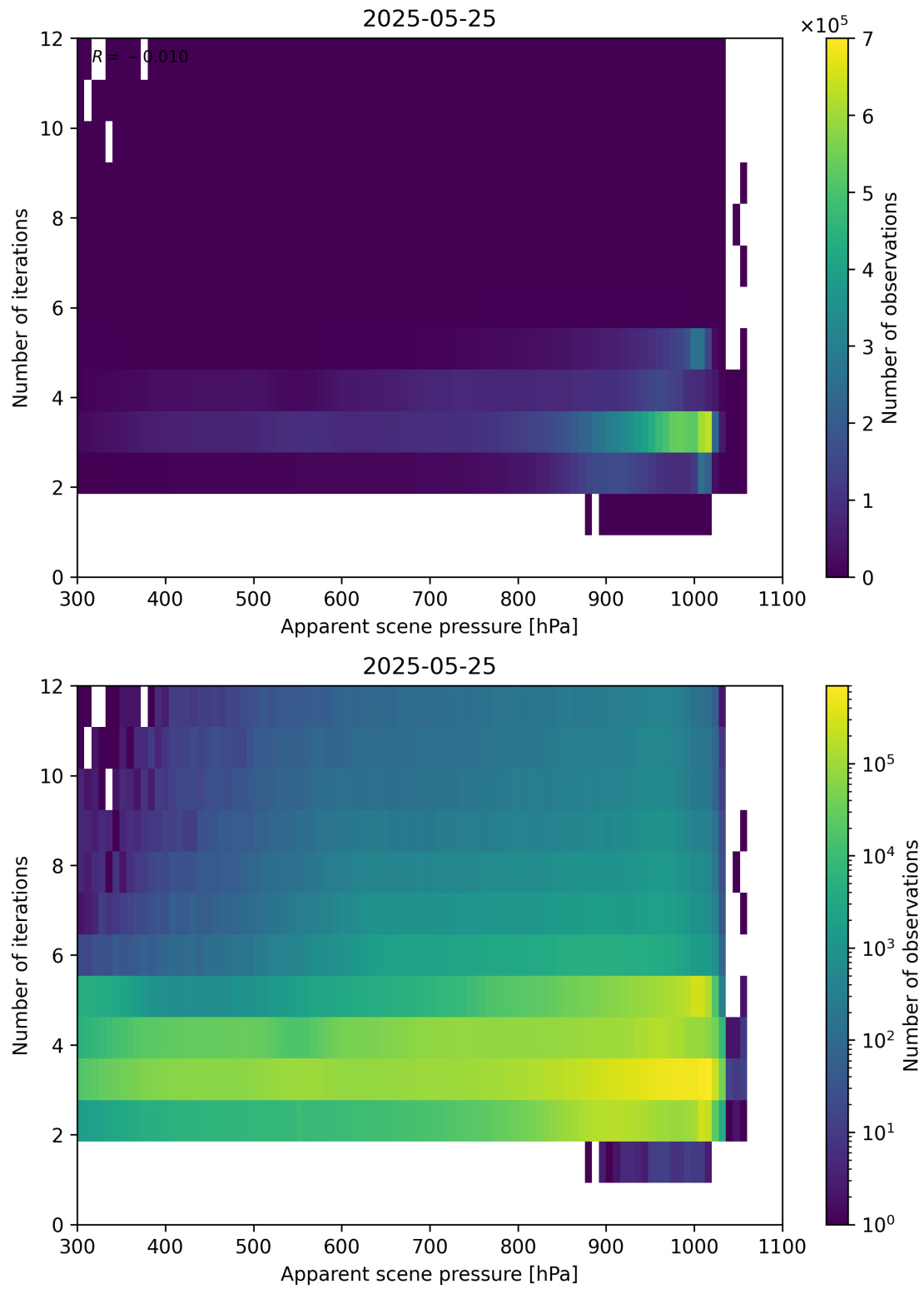
Figure 65: Scatter density plot of “Apparent scene pressure” against “Number of iterations” for 2025-05-24 to 2025-05-26.
