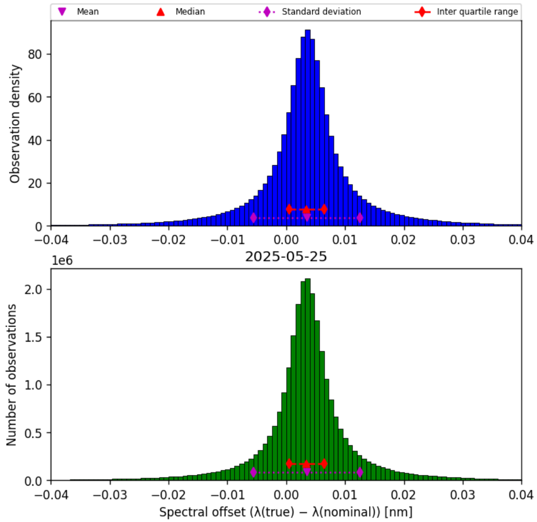
Figure 45: Histogram of “Spectral offset ( \lambda_{\text{true}} - \lambda_{\text{nominal}} )” for 2025-05-24 to 2025-05-26
