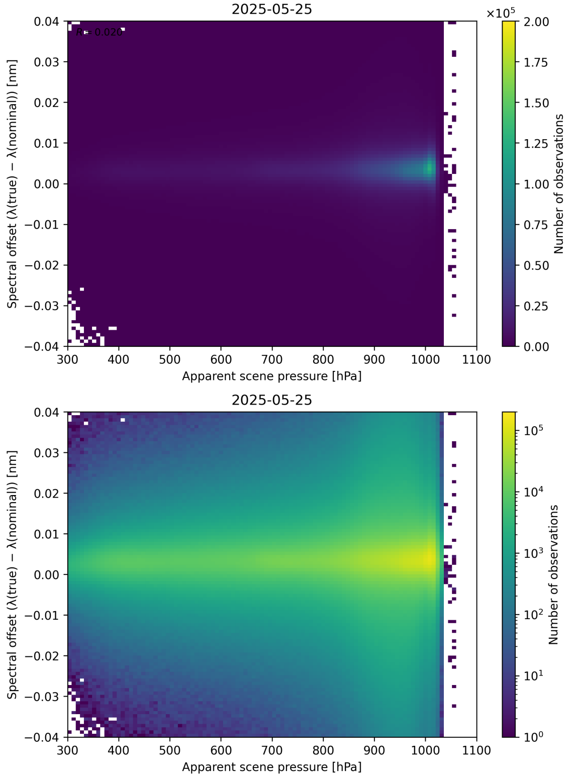
Figure 67: Scatter density plot of “Apparent scene pressure” against “Spectral offset ( \lambda_{\text{true}} - \lambda_{\text{nominal}} )” for 2025-05-24 to 2025-05-26.
