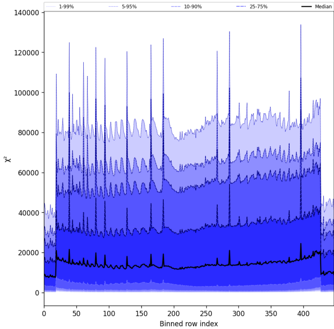
Figure 55: Along track statistics of “ \chi^2 ” for 2025-05-24 to 2025-05-26
