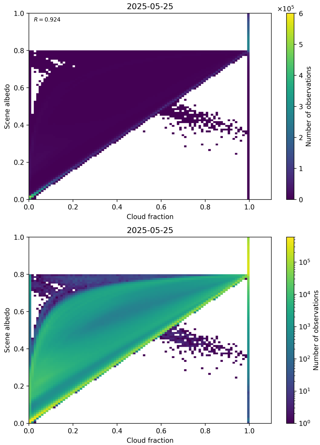
Figure 75: Scatter density plot of “Cloud fraction” against “Scene albedo” for 2025-05-24 to 2025-05-26.
