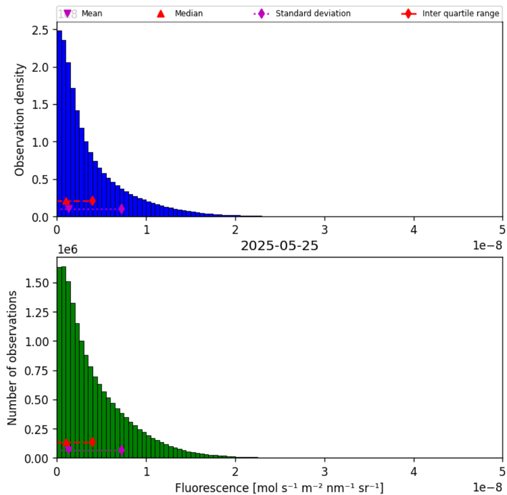
Figure 40: Histogram of “Fluorescence” for 2025-05-24 to 2025-05-26
