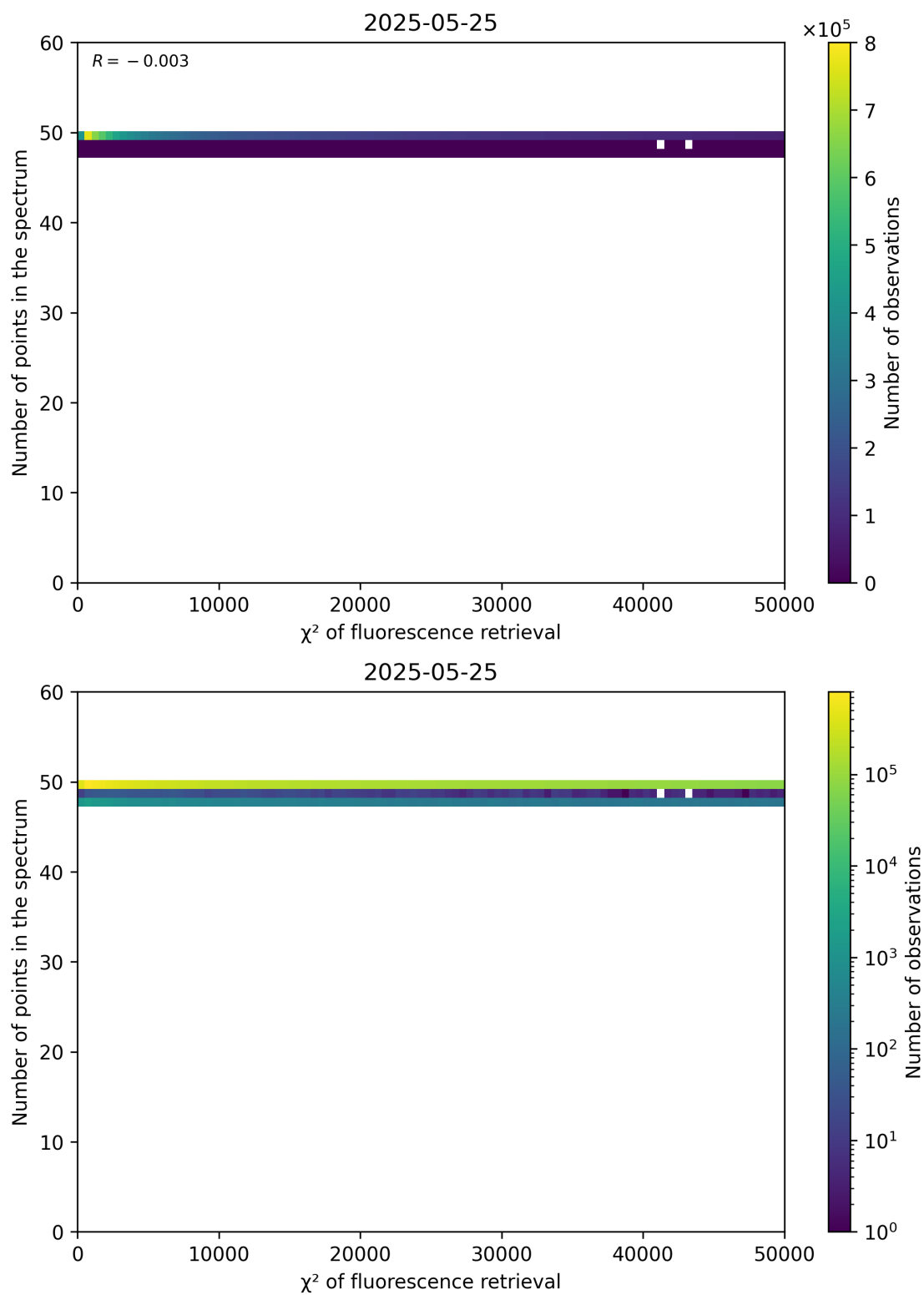
Figure 68: Scatter density plot of " \chi^2 of fluorescence retrieval" against "Number of points in the spectrum" for 2025-05-24 to 2025-05-26.
