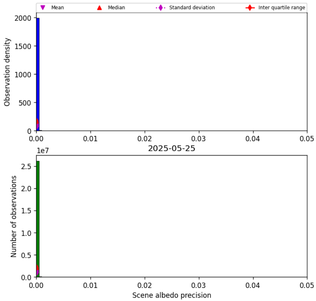
Figure 35: Histogram of “Scene albedo precision” for 2025-05-24 to 2025-05-26
