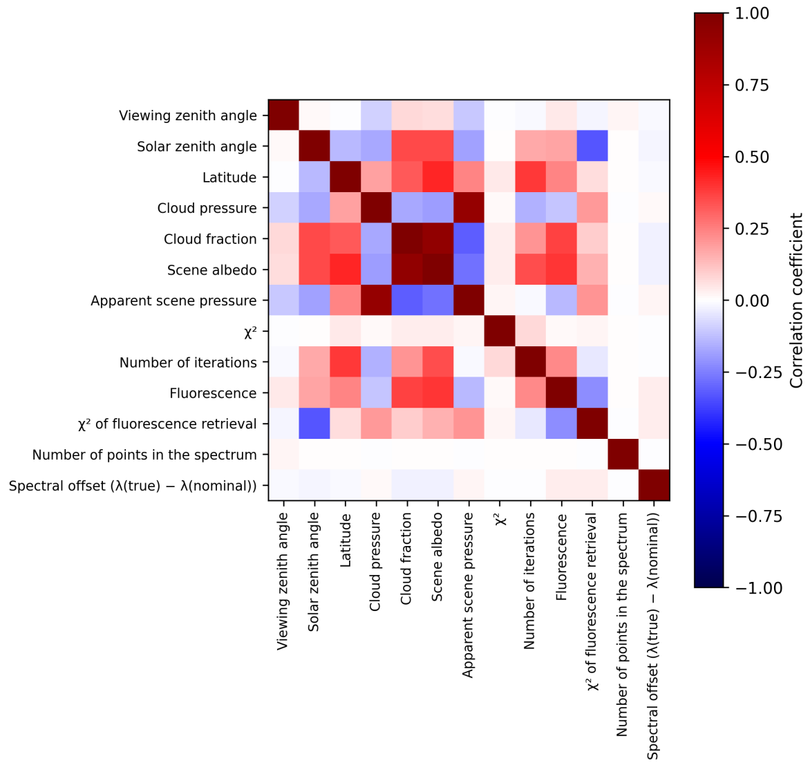
Figure 2: Map of correlation matrix for 2025-05-24 to 2025-05-26.
