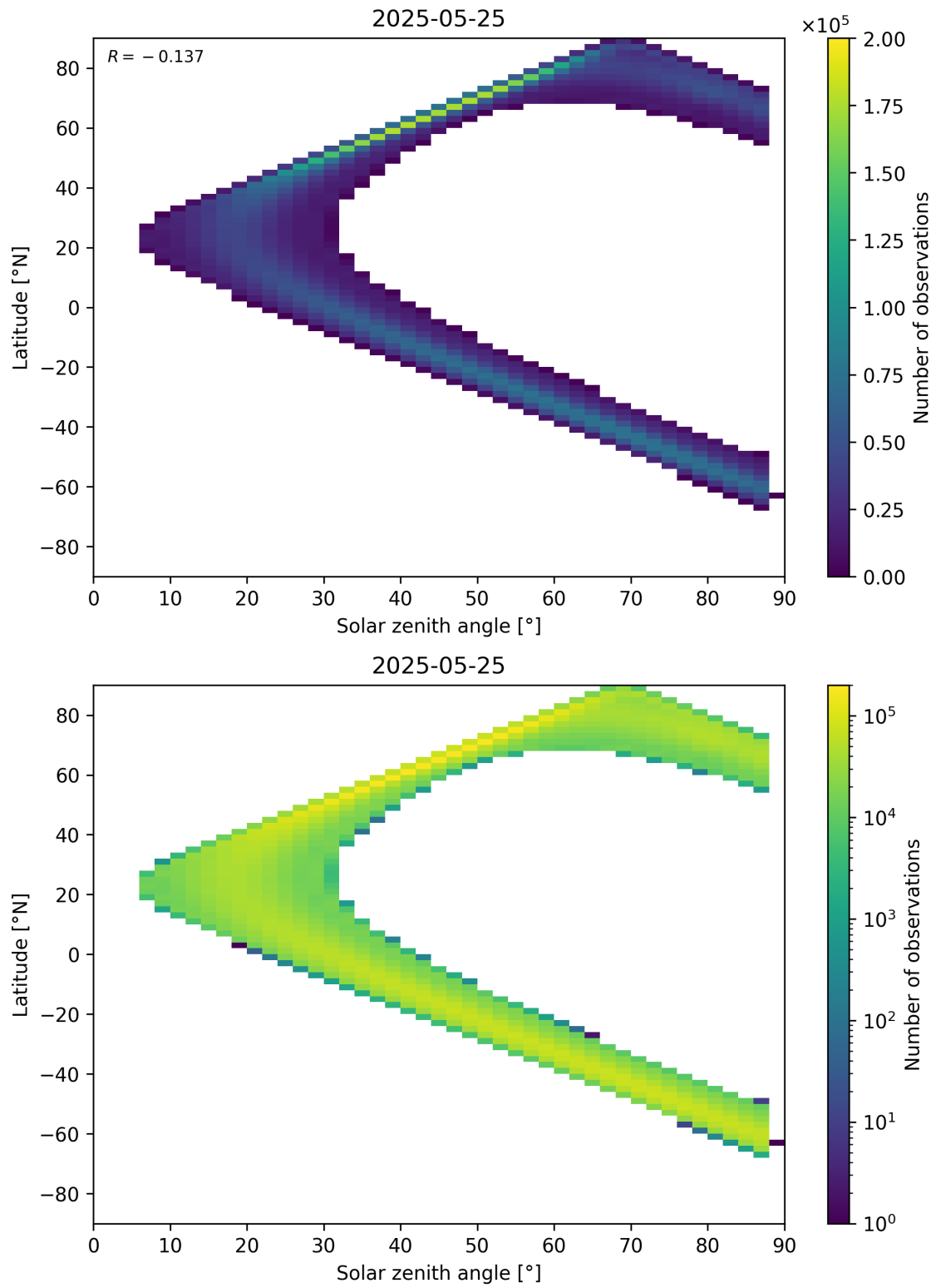
Figure 113: Scatter density plot of “Solar zenith angle” against “Latitude” for 2025-05-24 to 2025-05-26.
