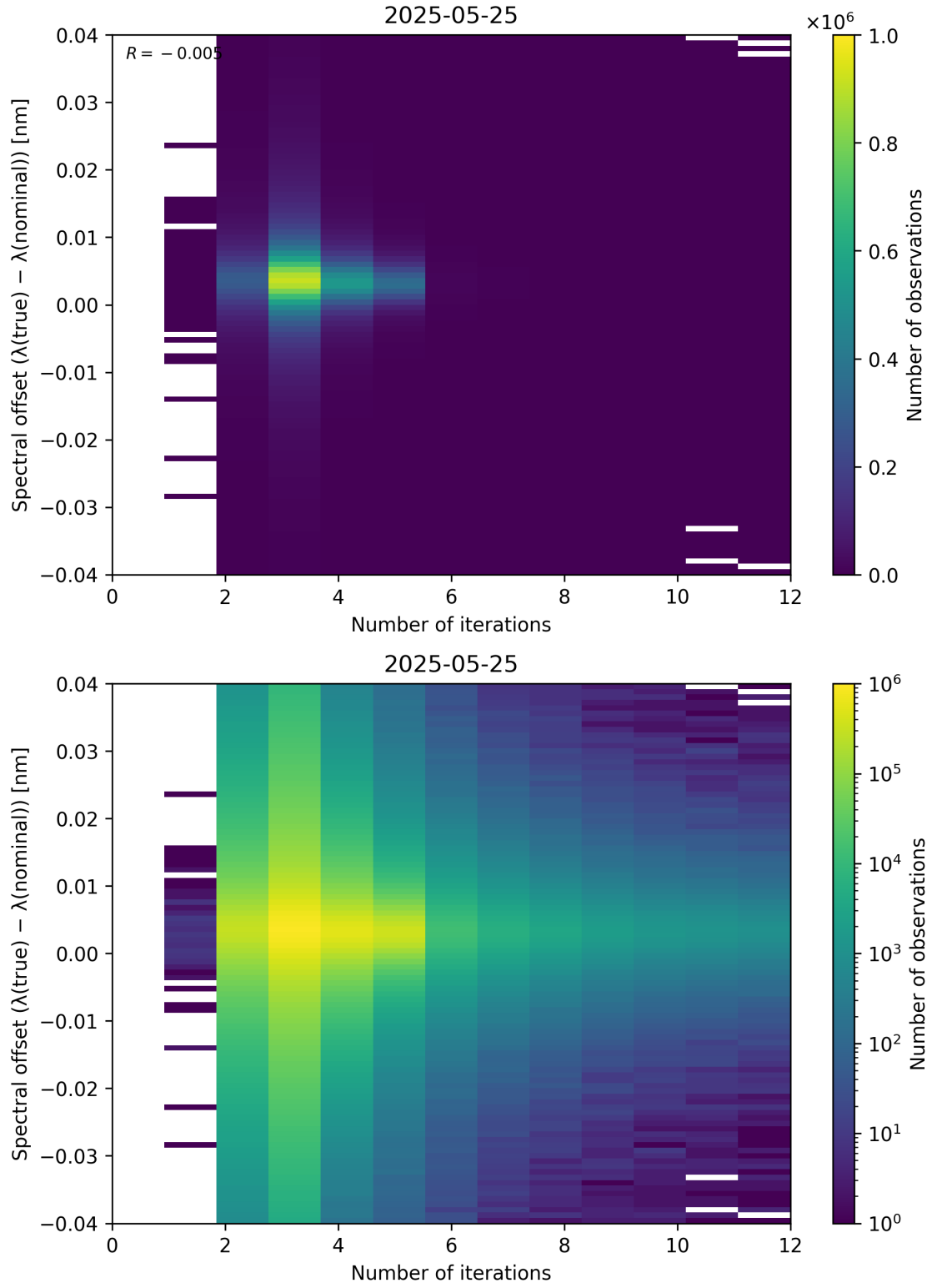
Figure 100: Scatter density plot of “Number of iterations” against “Spectral offset ( \lambda_{\text{true}} - \lambda_{\text{nominal}} )” for 2025-05-24 to 2025-05-26.
