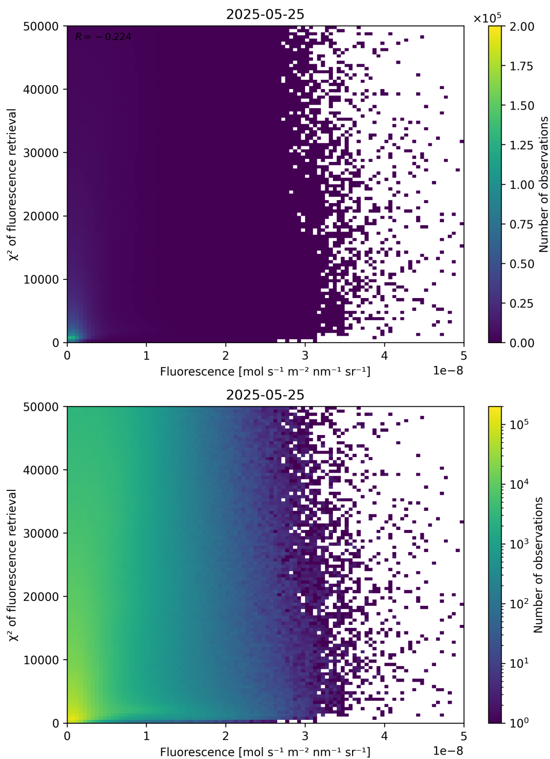
Figure 85: Scatter density plot of “Fluorescence” against “ \chi^2 of fluorescence retrieval” for 2025-05-24 to 2025-05-26.
