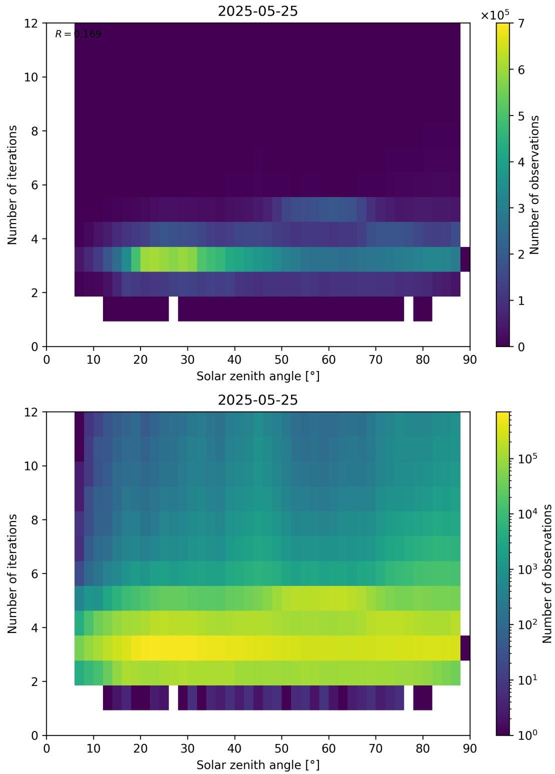
Figure 114: Scatter density plot of “Solar zenith angle” against “Number of iterations” for 2025-05-24 to 2025-05-26.
