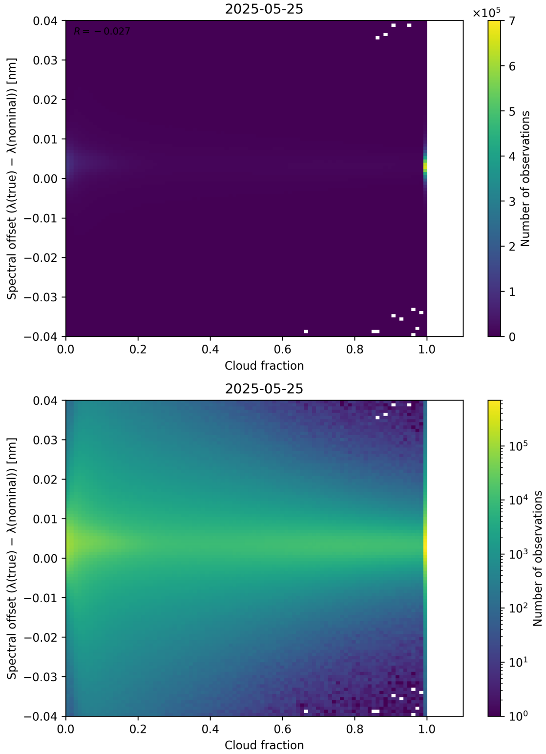
Figure 76: Scatter density plot of “Cloud fraction” against “Spectral offset ( \lambda_{\text{true}} - \lambda_{\text{nominal}} )” for 2025-05-24 to 2025-05-26.
