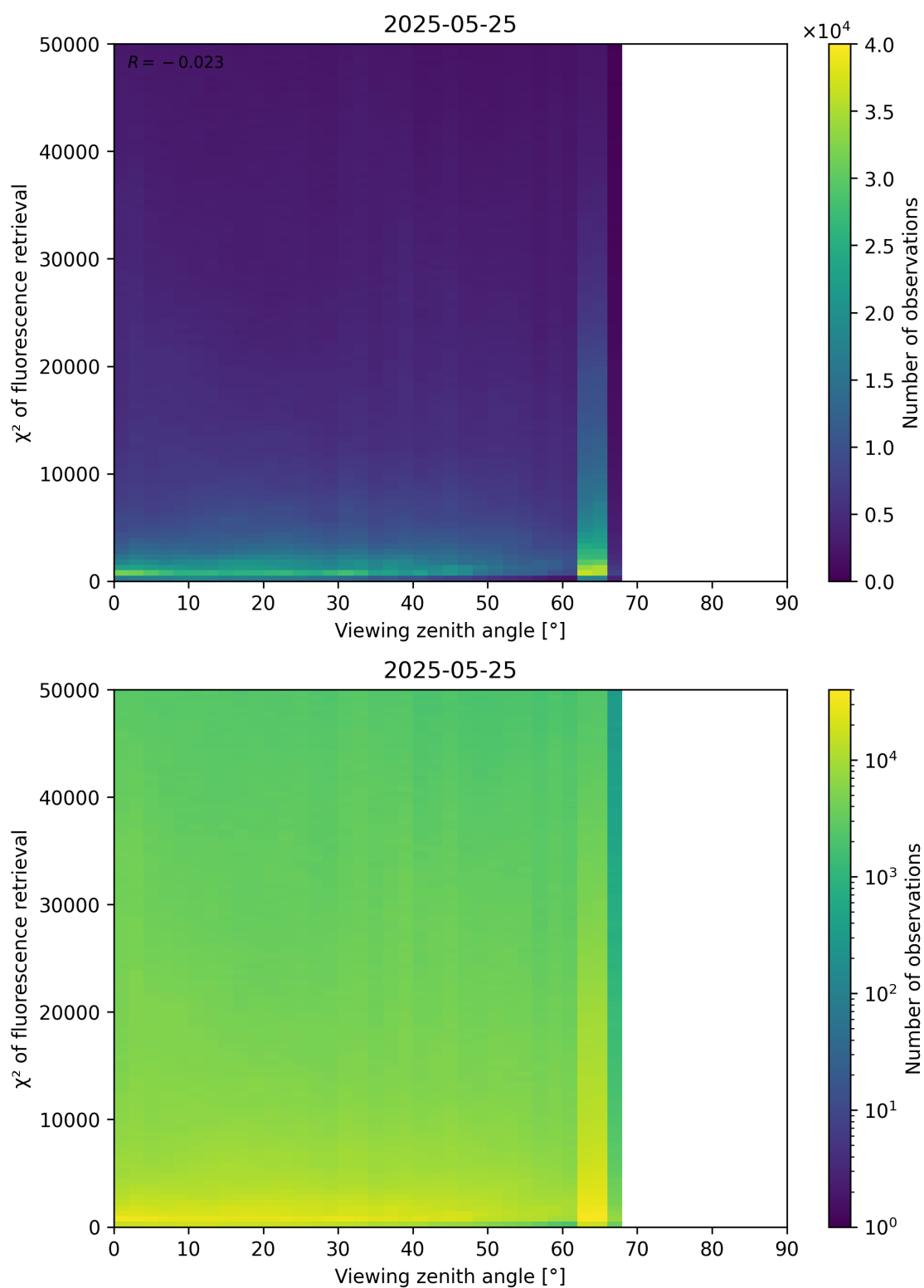
Figure 119: Scatter density plot of “Viewing zenith angle” against “ \chi^2 of fluorescence retrieval” for 2025-05-24 to 2025-05-26.
