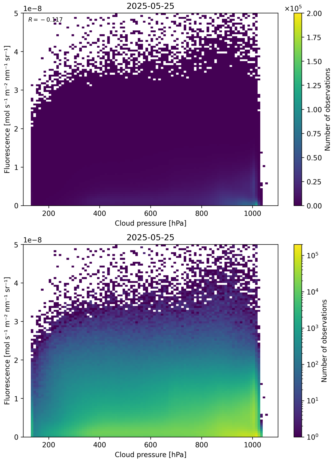
Figure 80: Scatter density plot of “Cloud pressure” against “Fluorescence” for 2025-05-24 to 2025-05-26.
