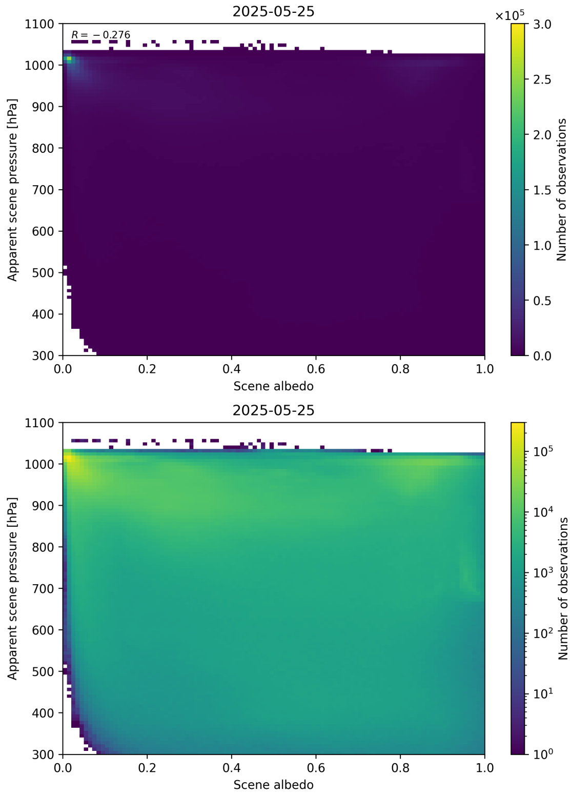
Figure 102: Scatter density plot of “Scene albedo” against “Apparent scene pressure” for 2025-05-24 to 2025-05-26.
