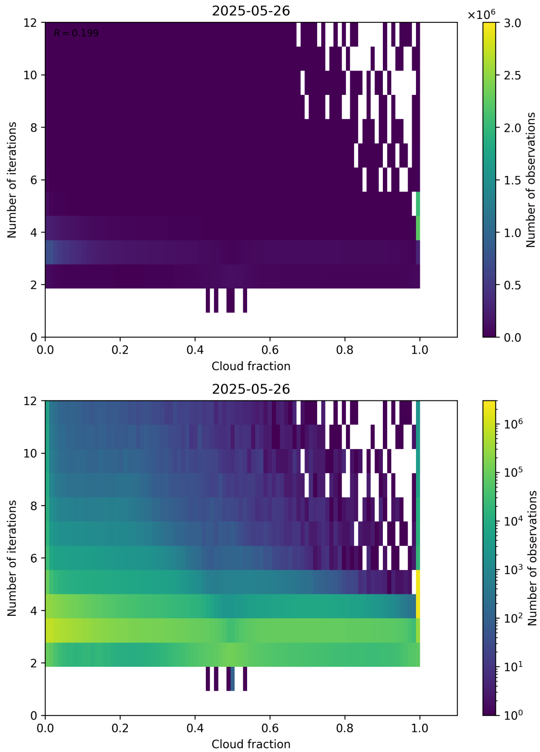
Figure 73: Scatter density plot of “Cloud fraction” against “Number of iterations” for 2025-05-26 to 2025-05-27.
