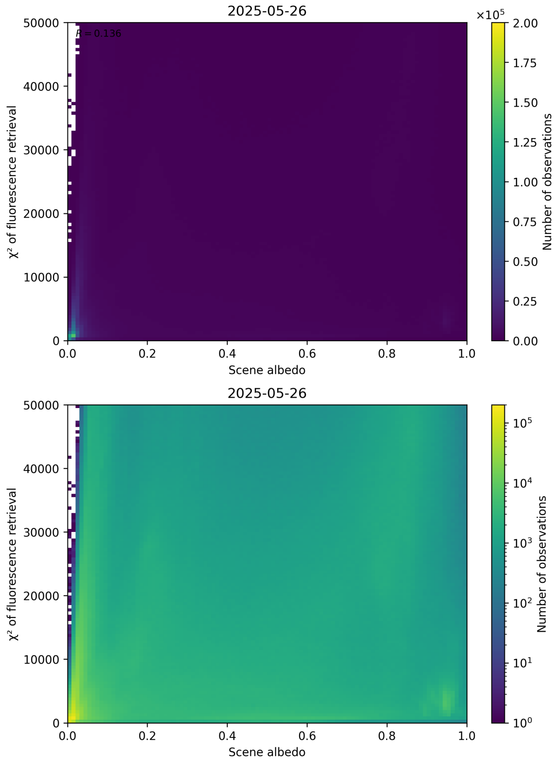
Figure 103: Scatter density plot of “Scene albedo” against “ \chi^2 of fluorescence retrieval” for 2025-05-26 to 2025-05-27.
