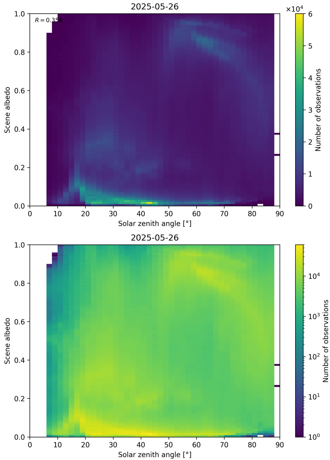
Figure 116: Scatter density plot of “Solar zenith angle” against “Scene albedo” for 2025-05-26 to 2025-05-27.
