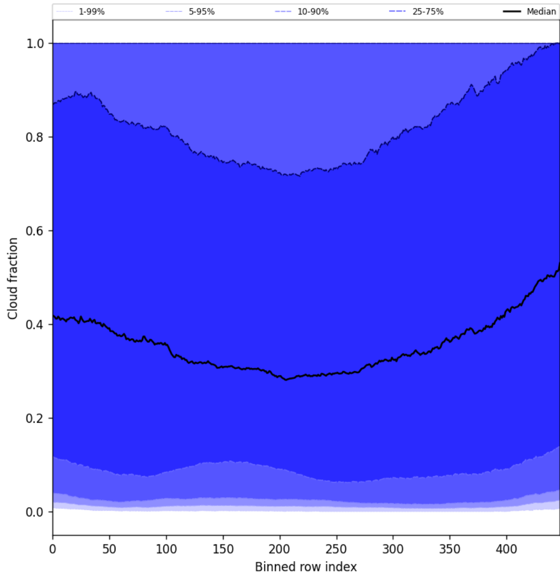
Figure 49: Along track statistics of “Cloud fraction” for 2025-05-26 to 2025-05-27
