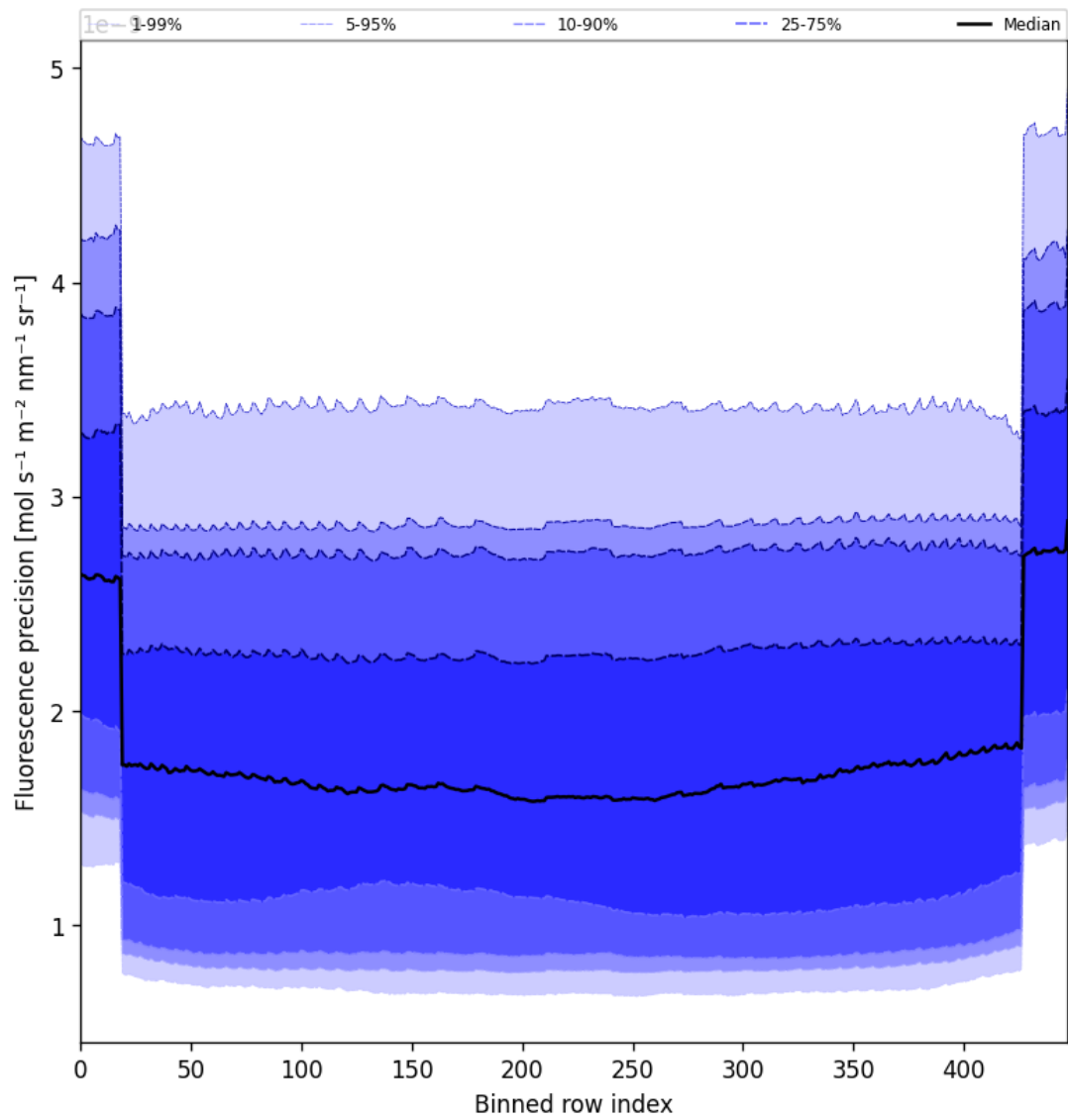
Figure 58: Along track statistics of “Fluorescence precision” for 2025-05-26 to 2025-05-27
