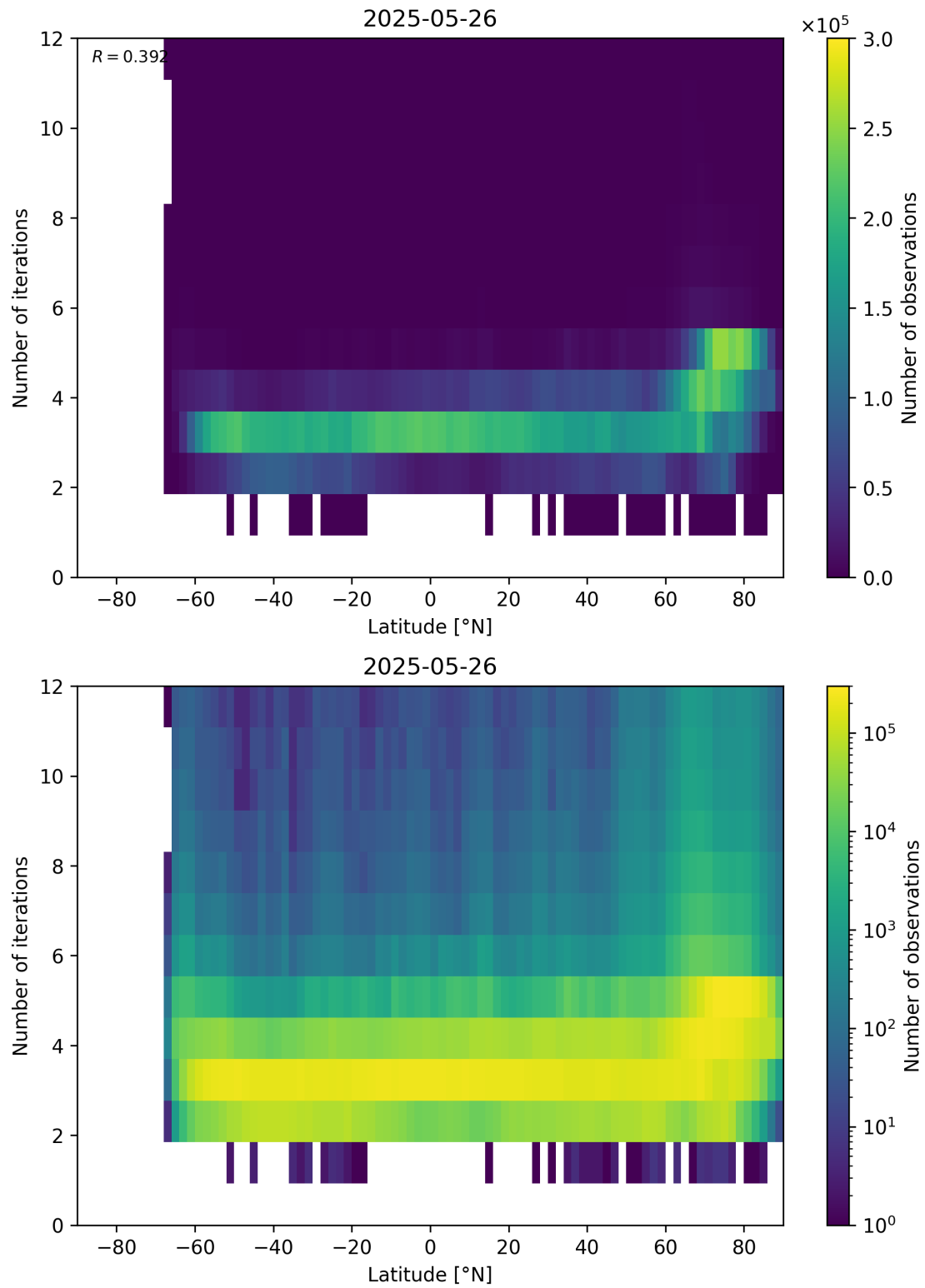
Figure 93: Scatter density plot of “Latitude” against “Number of iterations” for 2025-05-26 to 2025-05-27.
