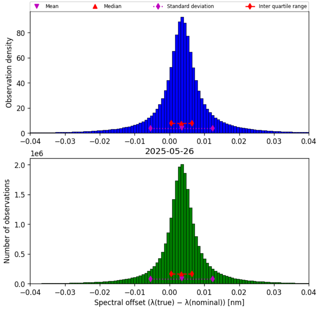
Figure 45: Histogram of “Spectral offset ( \lambda_{\text{true}} - \lambda_{\text{nominal}} )” for 2025-05-26 to 2025-05-27
