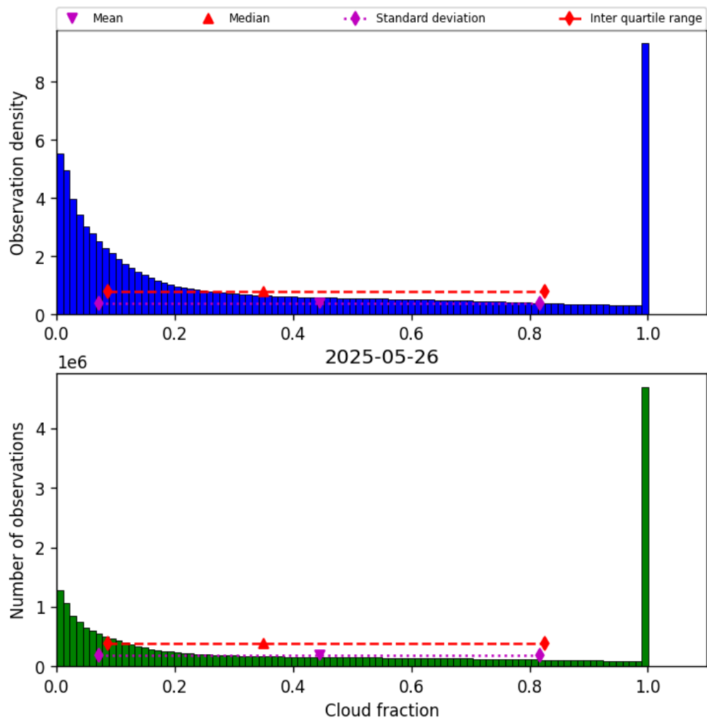
Figure 32: Histogram of “Cloud fraction” for 2025-05-26 to 2025-05-27
