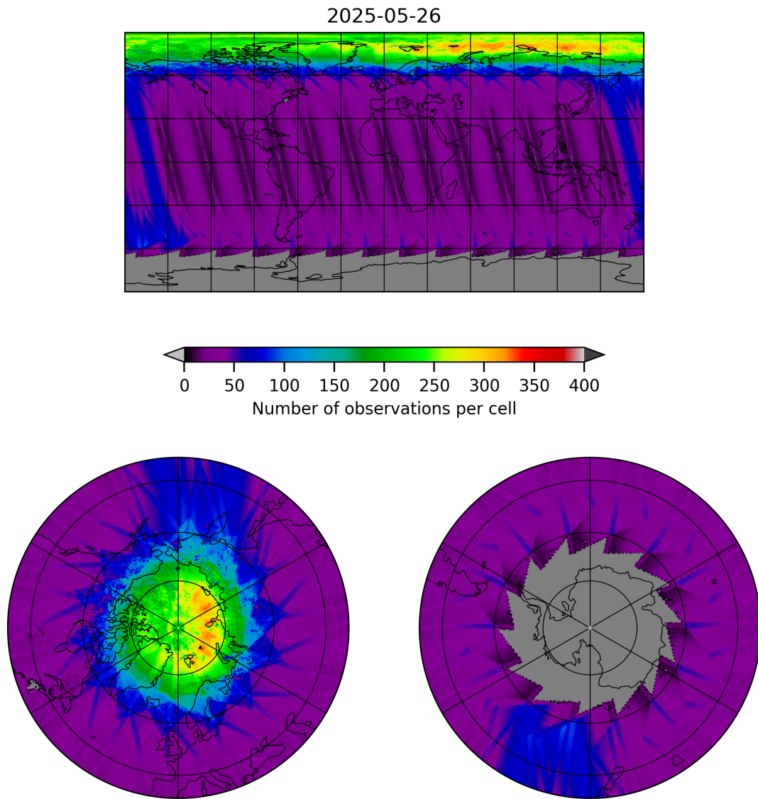
Figure 11: Map of the number of observations for 2025-05-26 to 2025-05-27
