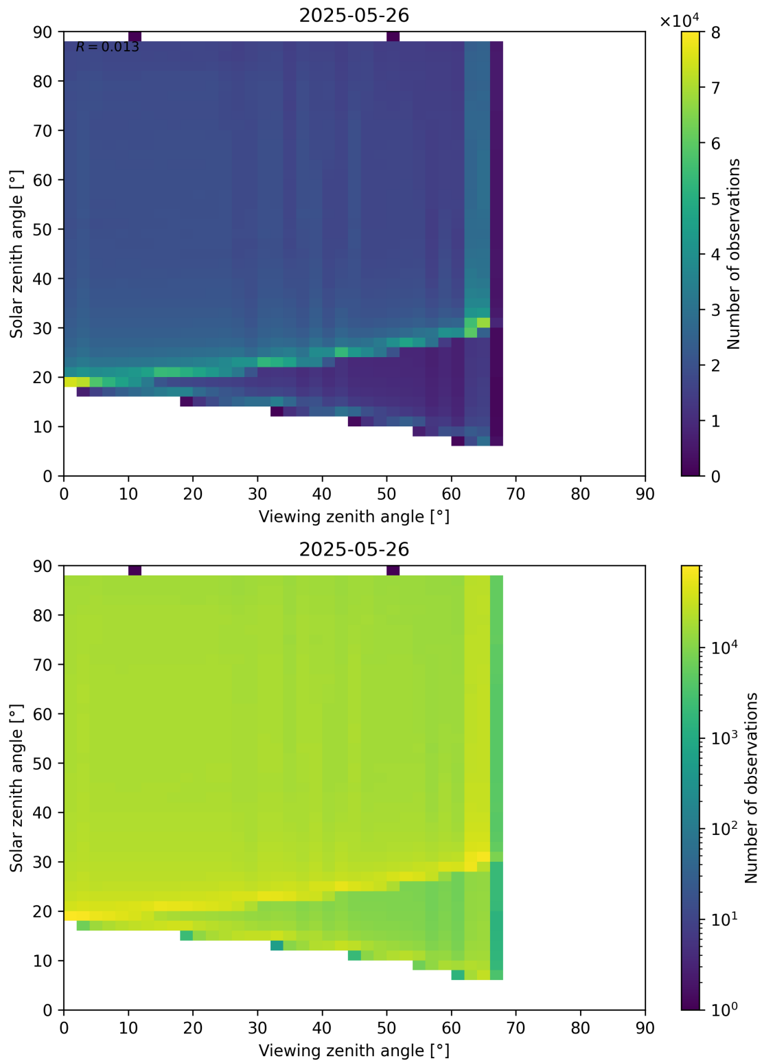
Figure 127: Scatter density plot of “Viewing zenith angle” against “Solar zenith angle” for 2025-05-26 to 2025-05-27.
