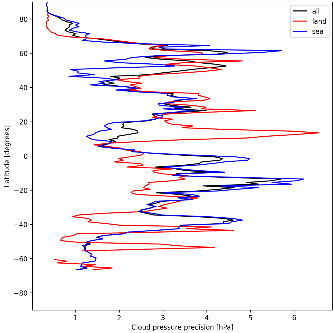
Figure 14: Zonal average of “Cloud pressure precision” for 2025-05-26 to 2025-05-27.
