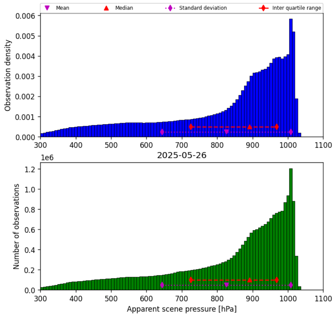
Figure 36: Histogram of “Apparent scene pressure” for 2025-05-26 to 2025-05-27
