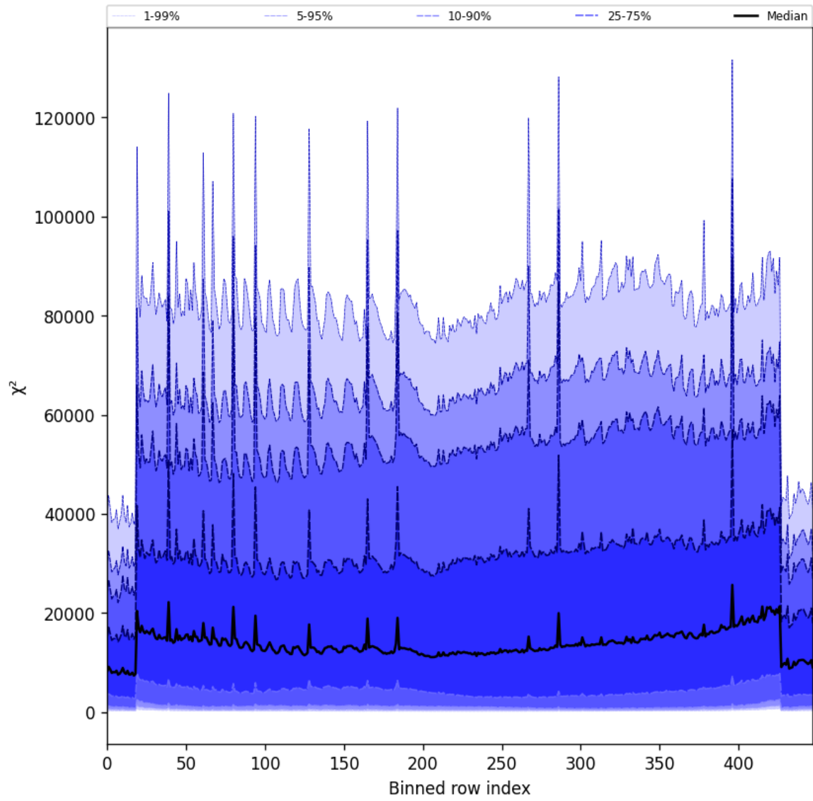
Figure 55: Along track statistics of “ \chi^2 ” for 2025-05-26 to 2025-05-27
