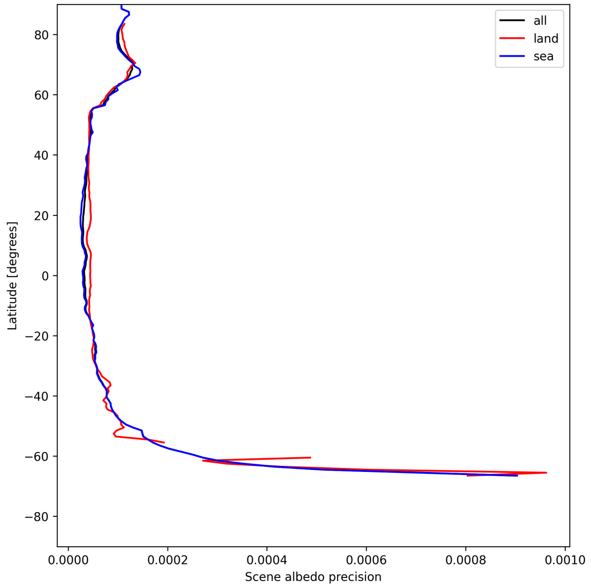
Figure 18: Zonal average of “Scene albedo precision” for 2025-05-26 to 2025-05-27.
