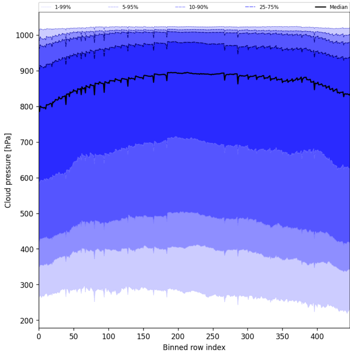
Figure 47: Along track statistics of “Cloud pressure” for 2025-05-26 to 2025-05-27
