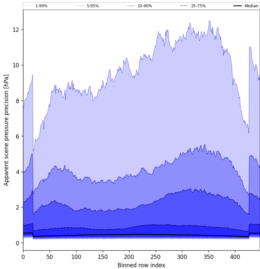
Figure 54: Along track statistics of “Apparent scene pressure precision” for 2025-05-26 to 2025-05-27
