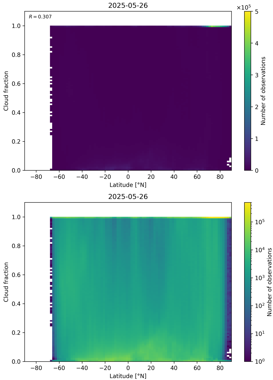
Figure 90: Scatter density plot of “Latitude” against “Cloud fraction” for 2025-05-26 to 2025-05-27.
