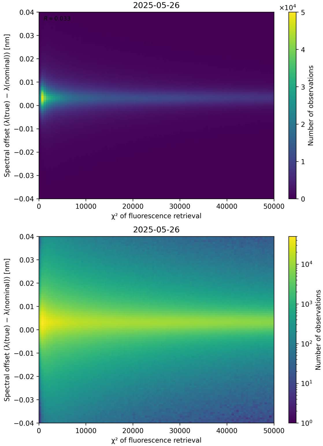
Figure 69: Scatter density plot of “ \chi^2 of fluorescence retrieval” against “Spectral offset ( \lambda_{\text{true}} - \lambda_{\text{nominal}} )” for 2025-05-26 to 2025-05-27.
