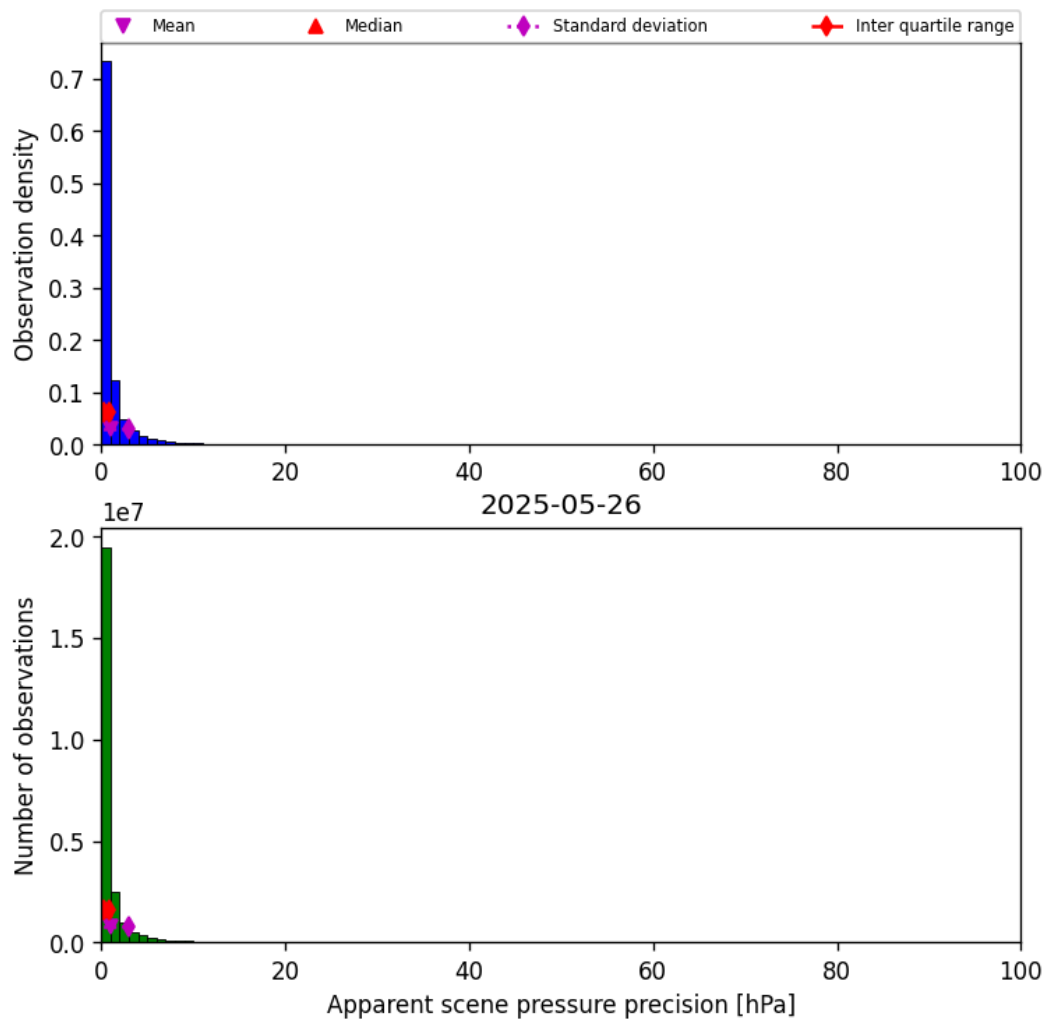
Figure 37: Histogram of “Apparent scene pressure precision” for 2025-05-26 to 2025-05-27
