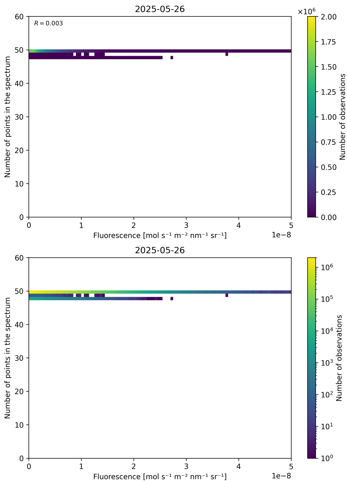
Figure 86: Scatter density plot of “Fluorescence” against “Number of points in the spectrum” for 2025-05-26 to 2025-05-27.
