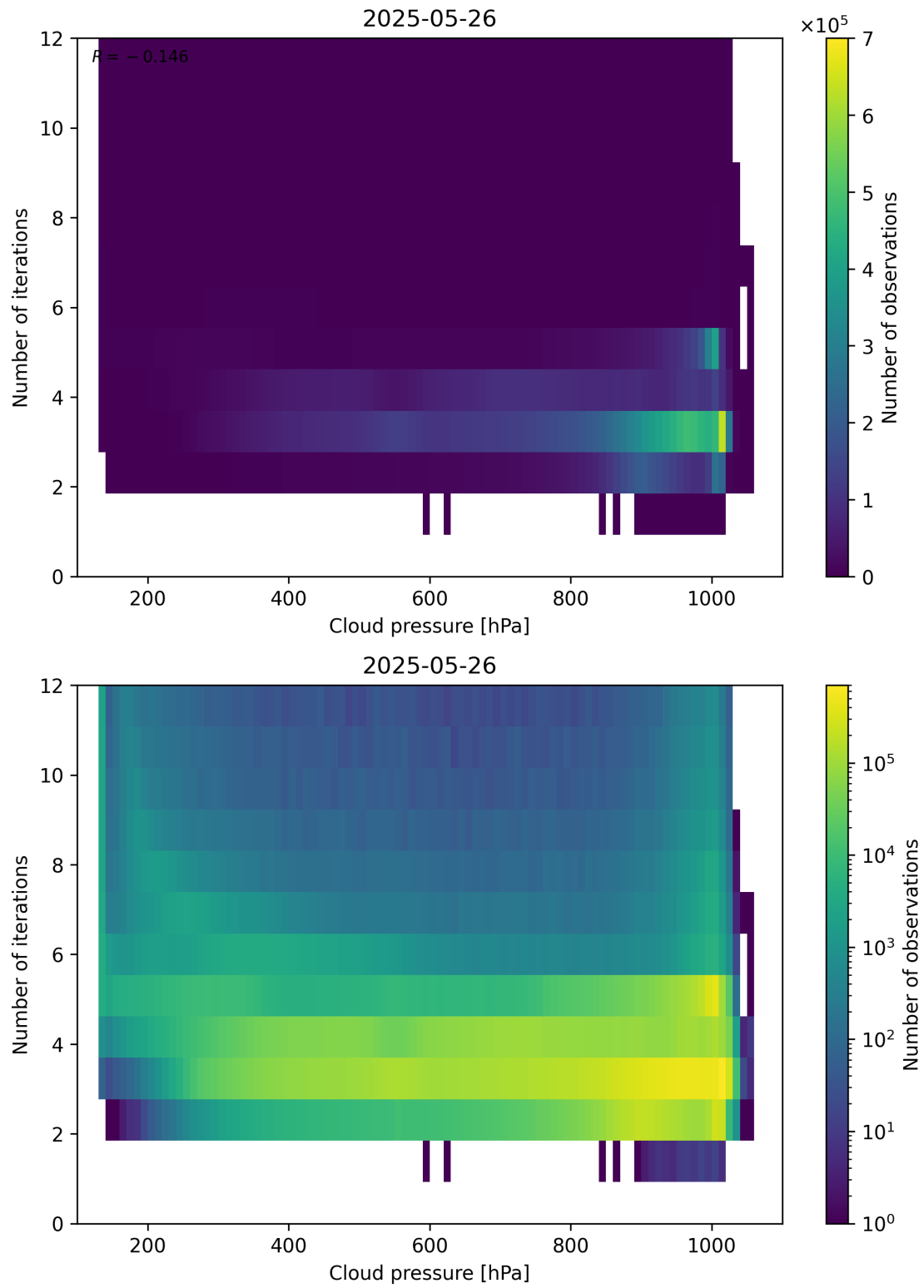
Figure 81: Scatter density plot of “Cloud pressure” against “Number of iterations” for 2025-05-26 to 2025-05-27.
