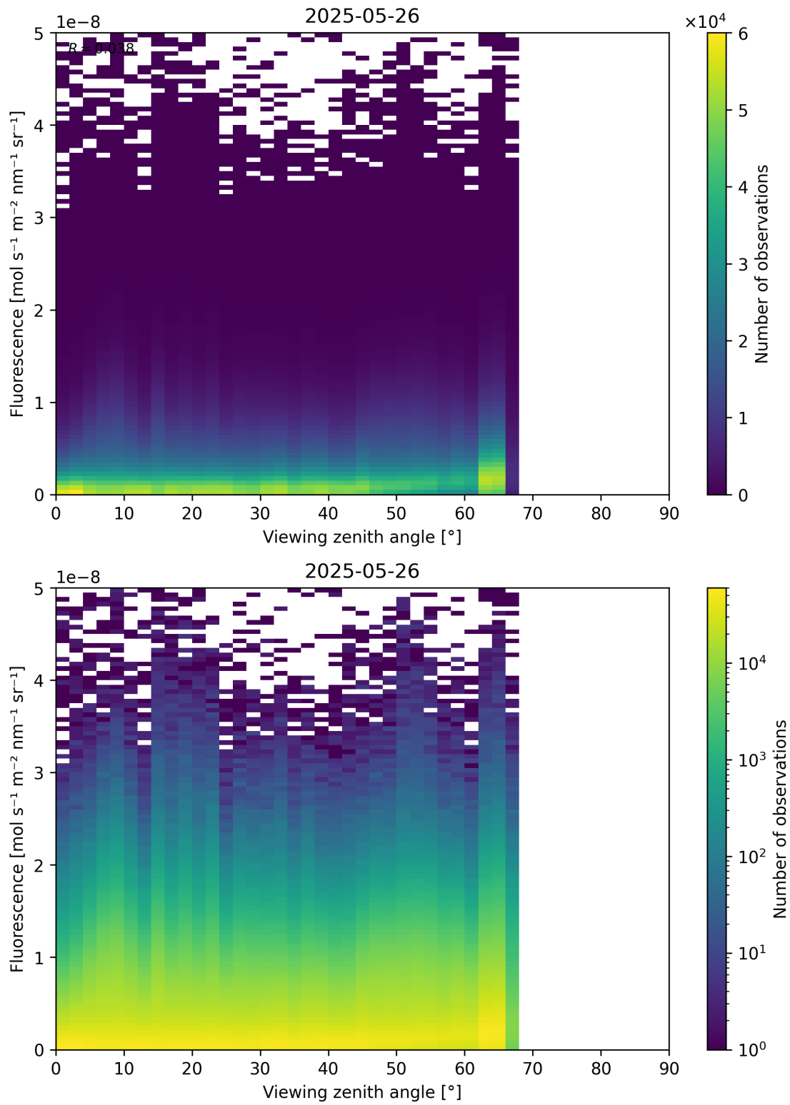
Figure 122: Scatter density plot of “Viewing zenith angle” against “Fluorescence” for 2025-05-26 to 2025-05-27.
