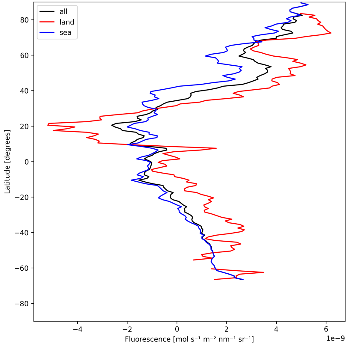
Figure 23: Zonal average of “Fluorescence” for 2025-05-26 to 2025-05-27.
