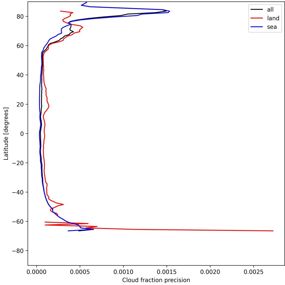
Figure 16: Zonal average of “Cloud fraction precision” for 2025-05-26 to 2025-05-27.
