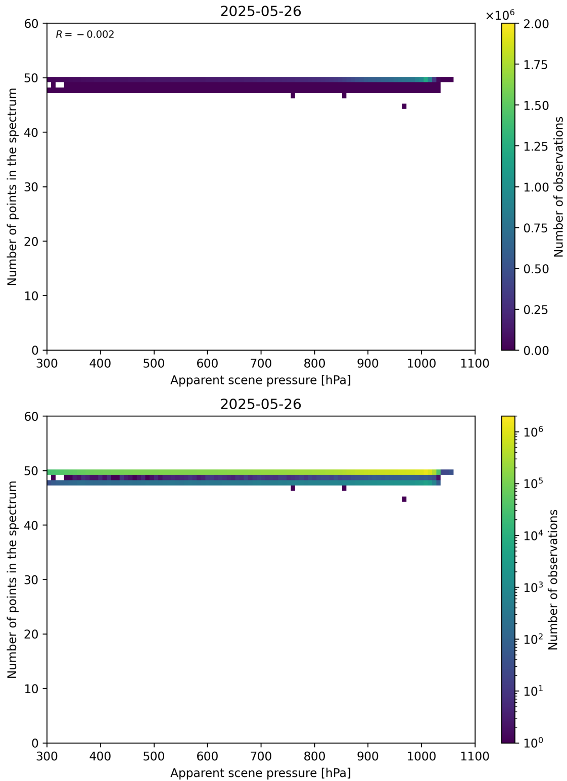
Figure 66: Scatter density plot of “Apparent scene pressure” against “Number of points in the spectrum” for 2025-05-26 to 2025-05-27.
