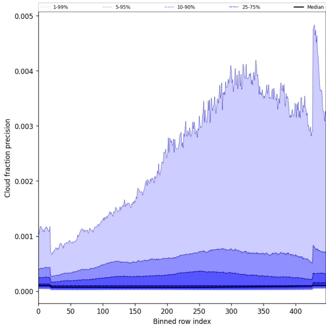
Figure 50: Along track statistics of “Cloud fraction precision” for 2025-05-26 to 2025-05-27
