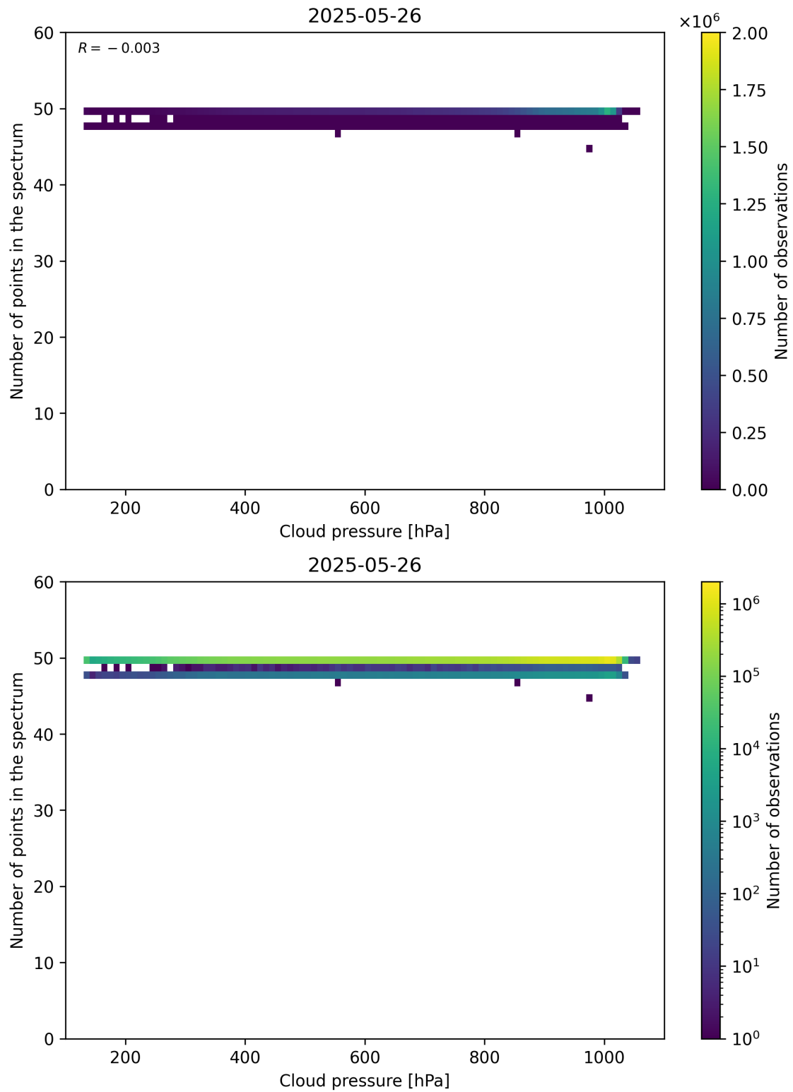
Figure 82: Scatter density plot of “Cloud pressure” against “Number of points in the spectrum” for 2025-05-26 to 2025-05-27.
