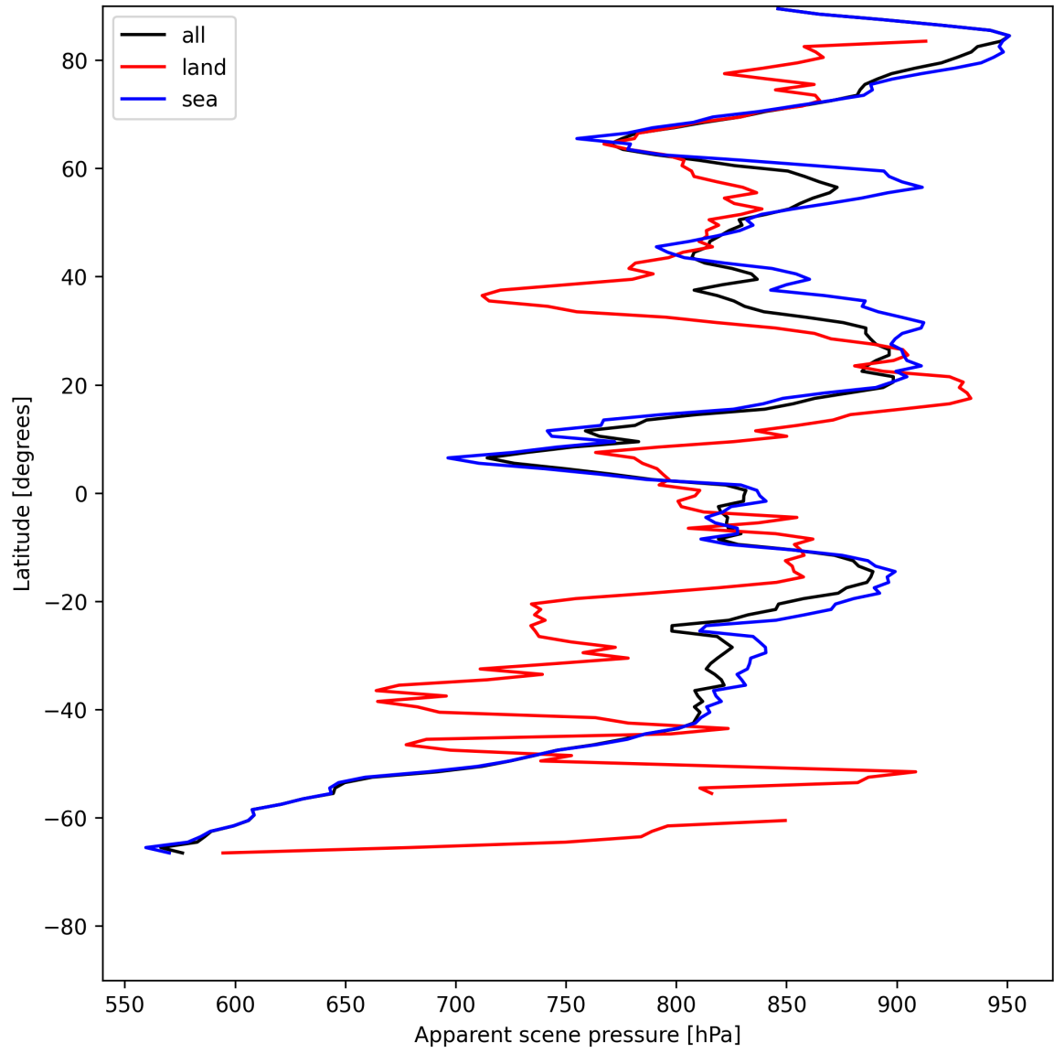
Figure 19: Zonal average of “Apparent scene pressure” for 2025-05-26 to 2025-05-27.
