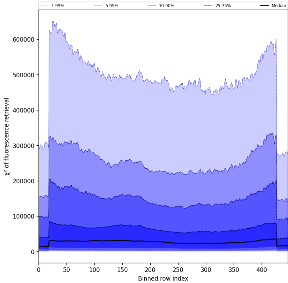
Figure 59: Along track statistics of “ \chi^2 of fluorescence retrieval” for 2025-05-26 to 2025-05-27
