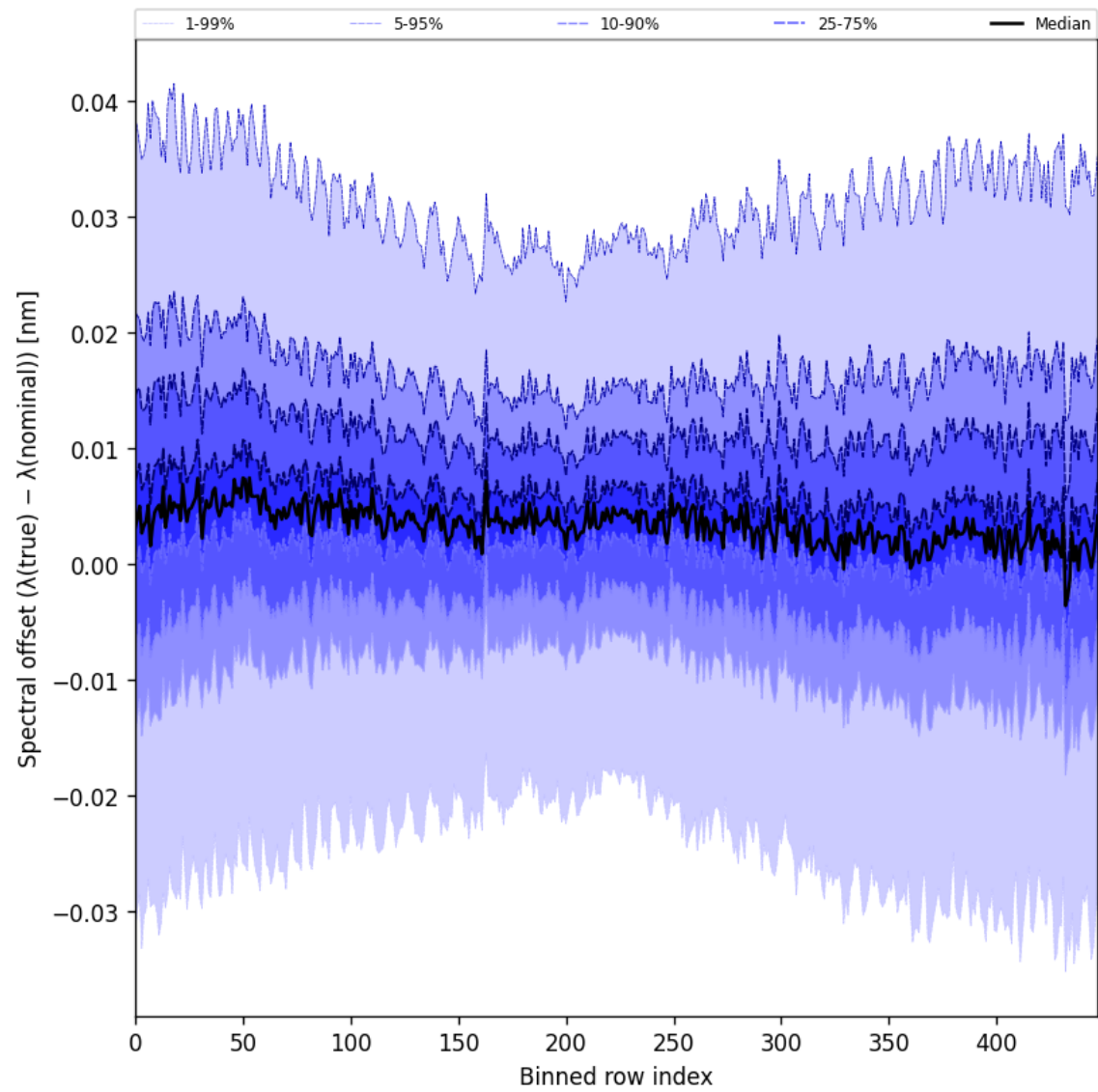
Figure 62: Along track statistics of “Spectral offset ( \lambda_{\text{true}} - \lambda_{\text{nominal}} )” for 2025-05-26 to 2025-05-27
