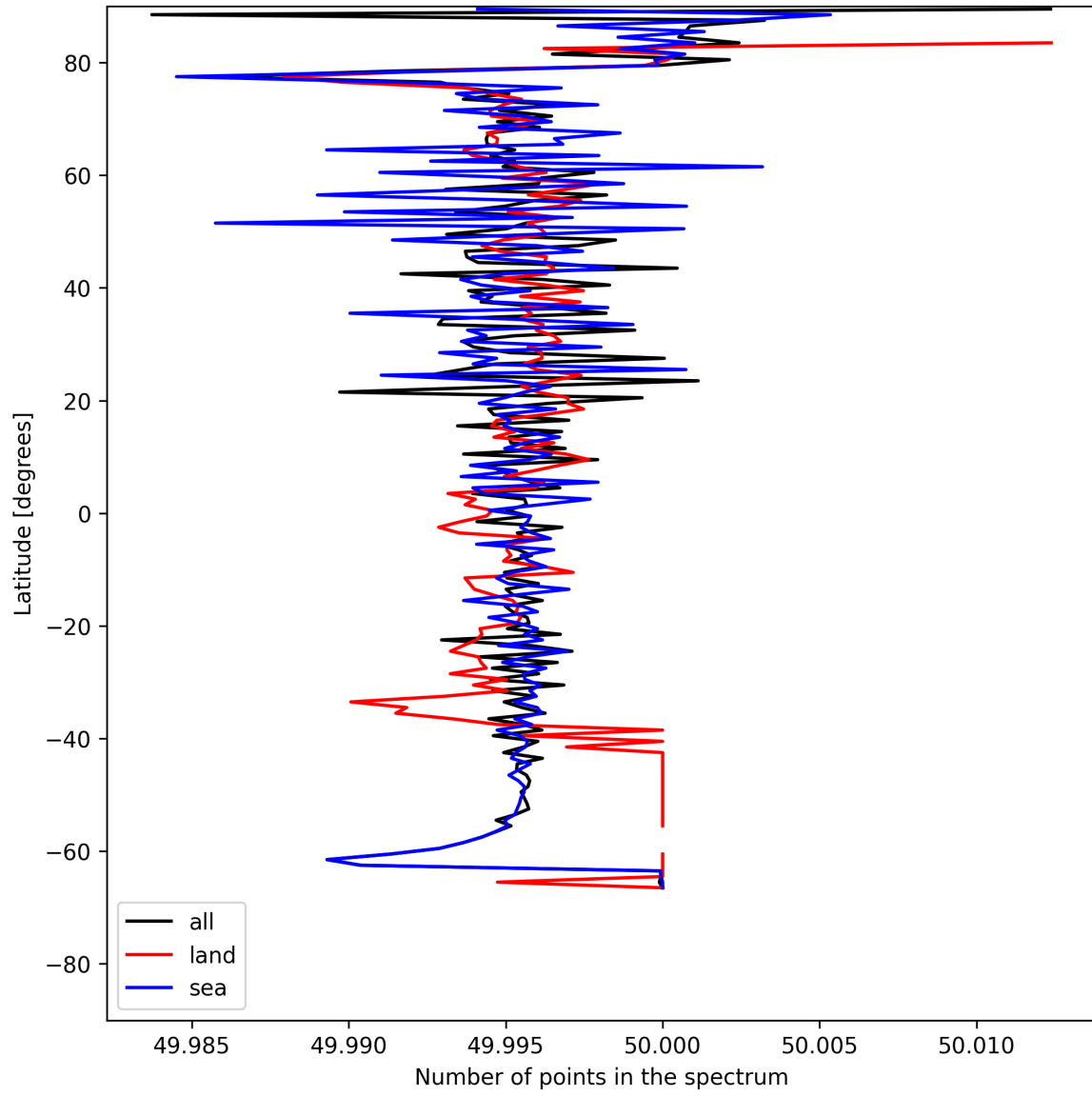
Figure 27: Zonal average of “Number of points in the spectrum” for 2025-05-26 to 2025-05-27.
