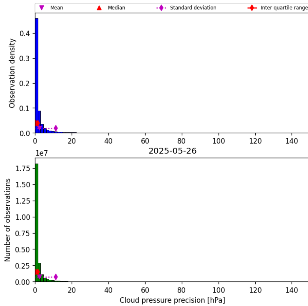
Figure 31: Histogram of "Cloud pressure precision" for 2025-05-26 to 2025-05-27
