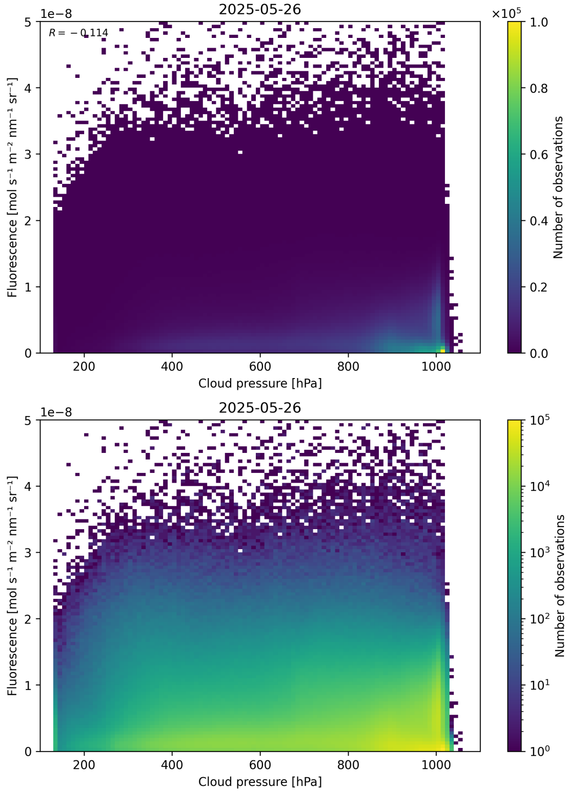
Figure 80: Scatter density plot of “Cloud pressure” against “Fluorescence” for 2025-05-26 to 2025-05-27.
