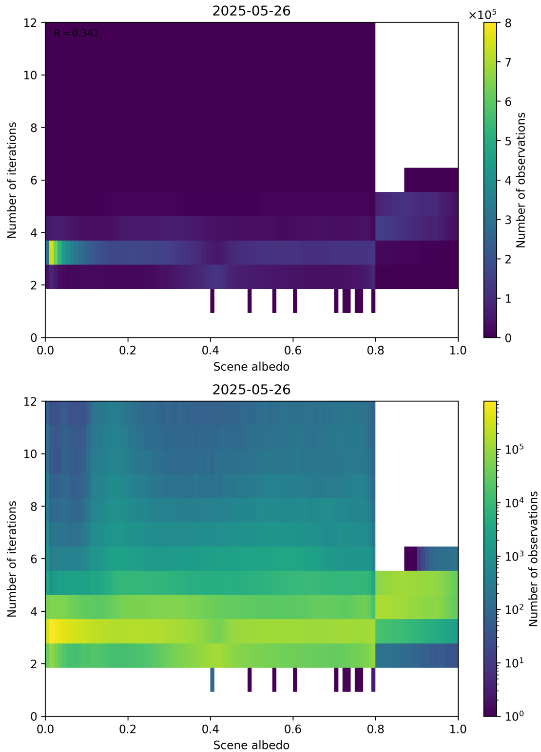
Figure 105: Scatter density plot of “Scene albedo” against “Number of iterations” for 2025-05-26 to 2025-05-27.
