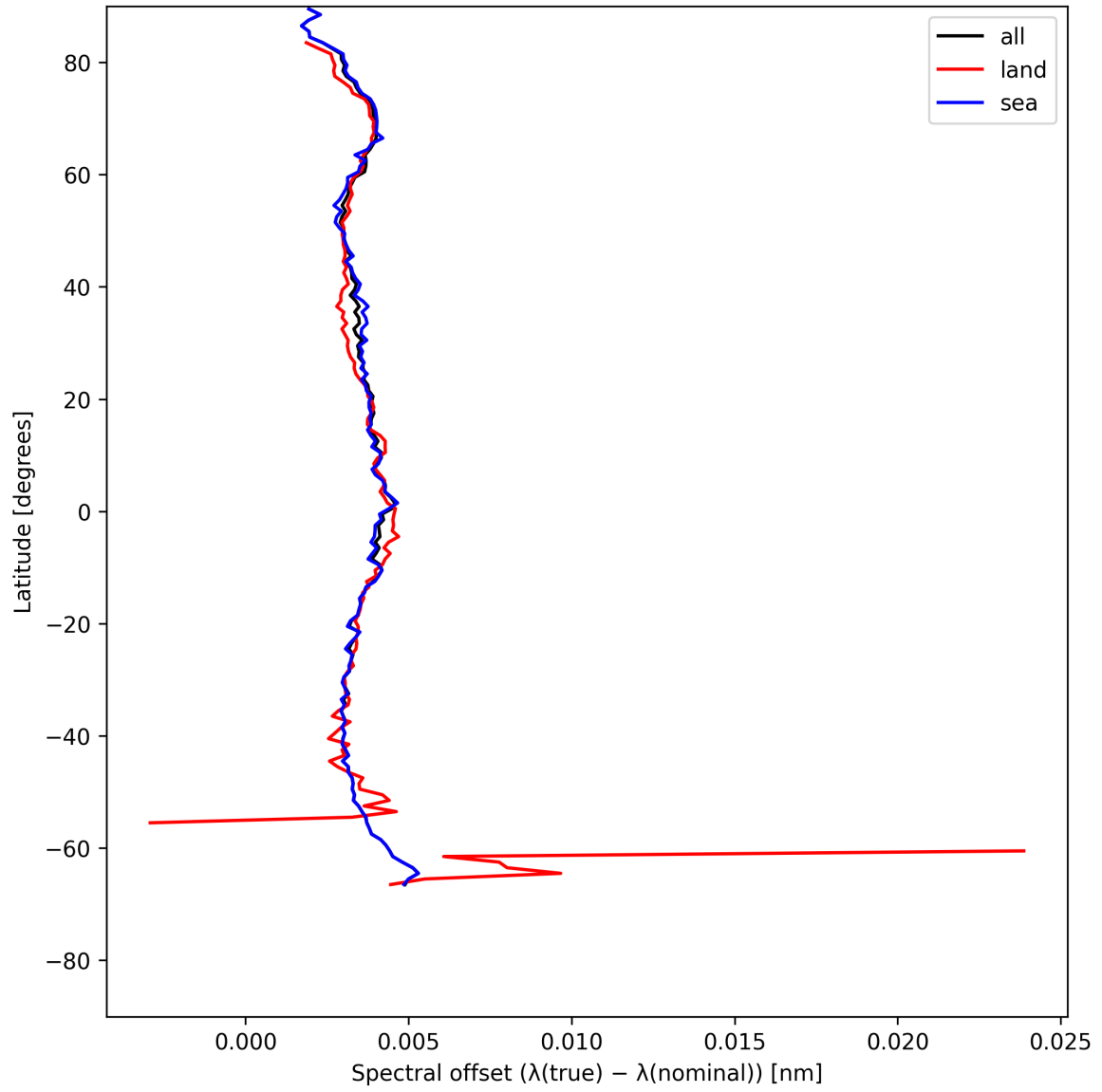
Figure 28: Zonal average of “Spectral offset ( \lambda_{\text{true}} - \lambda_{\text{nominal}} )” for 2025-05-26 to 2025-05-27.
