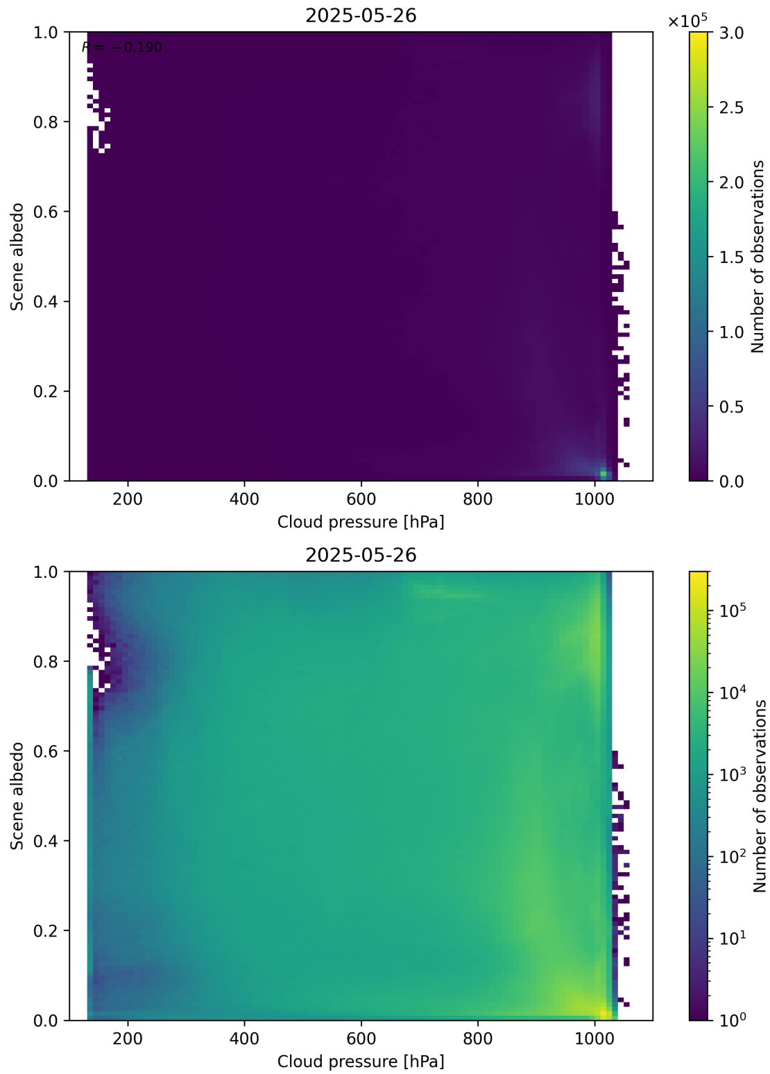
Figure 83: Scatter density plot of “Cloud pressure” against “Scene albedo” for 2025-05-26 to 2025-05-27.
