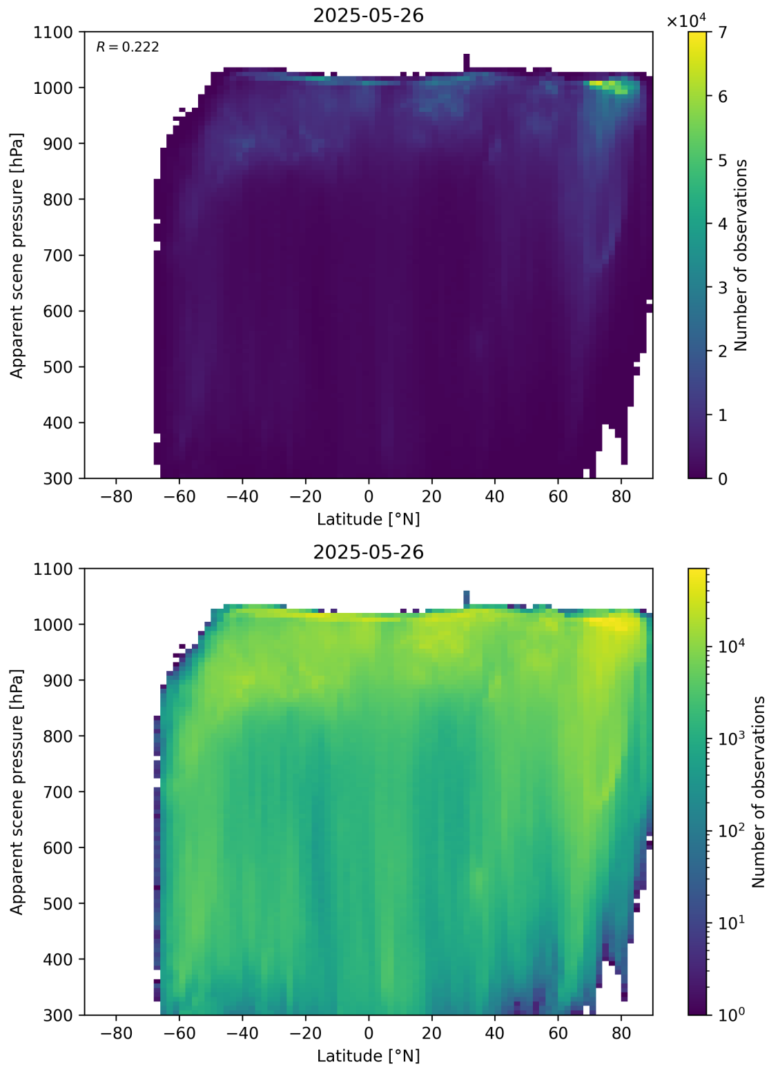
Figure 88: Scatter density plot of “Latitude” against “Apparent scene pressure” for 2025-05-26 to 2025-05-27.
