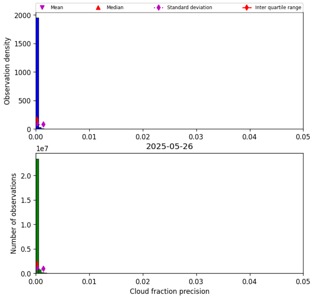
Figure 33: Histogram of “Cloud fraction precision” for 2025-05-26 to 2025-05-27
