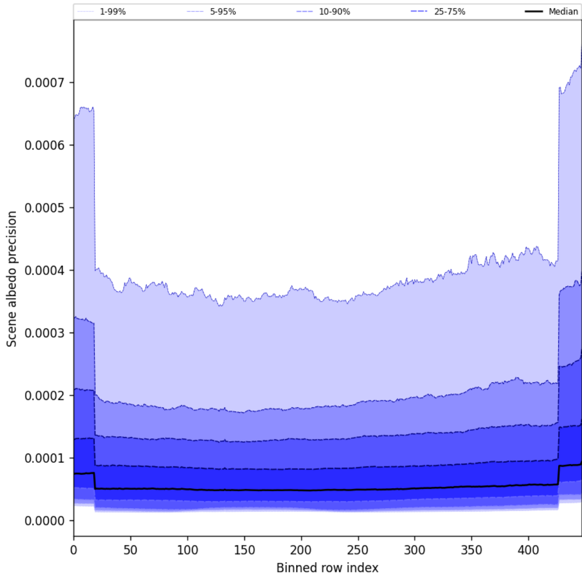
Figure 52: Along track statistics of “Scene albedo precision” for 2025-05-26 to 2025-05-27
