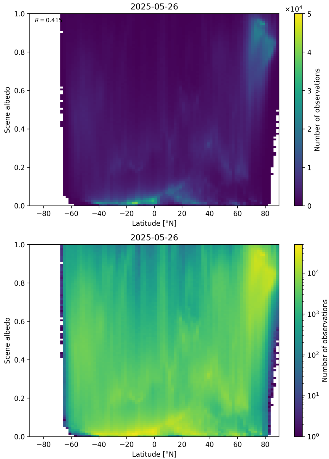
Figure 95: Scatter density plot of “Latitude” against “Scene albedo” for 2025-05-26 to 2025-05-27.
