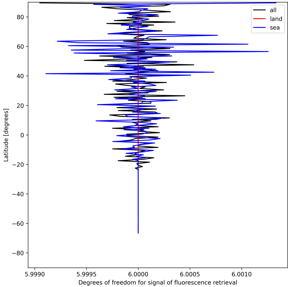
Figure 26: Zonal average of “Degrees of freedom for signal of fluorescence retrieval” for 2025-05-26 to 2025-05-27.
