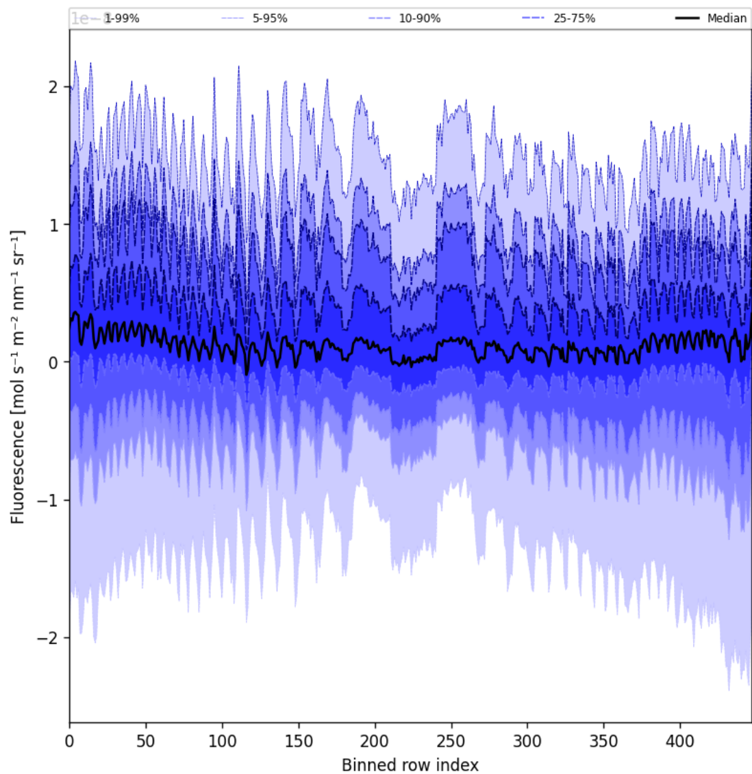
Figure 57: Along track statistics of “Fluorescence” for 2025-05-26 to 2025-05-27
