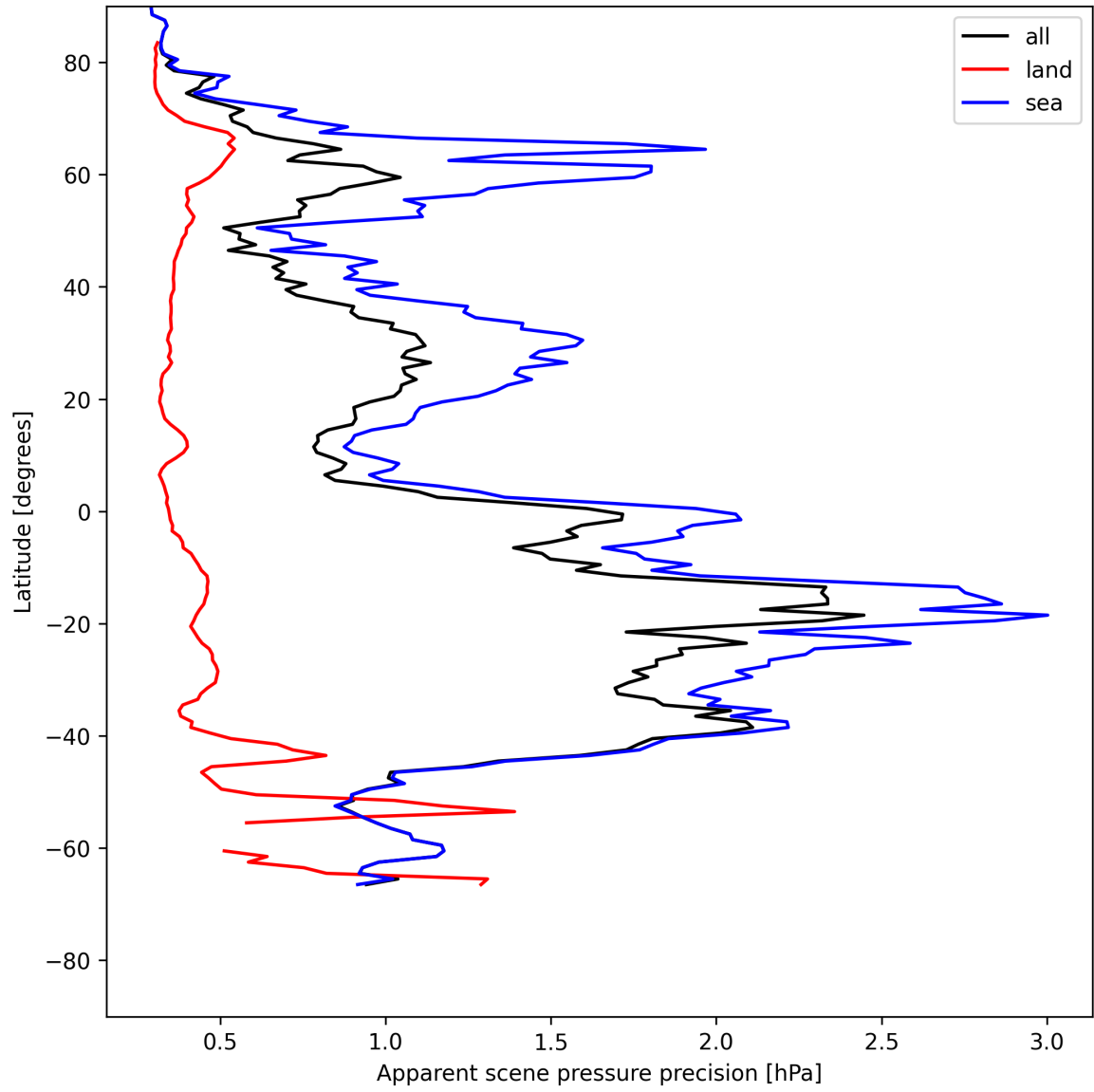
Figure 20: Zonal average of “Apparent scene pressure precision” for 2025-05-26 to 2025-05-27.
