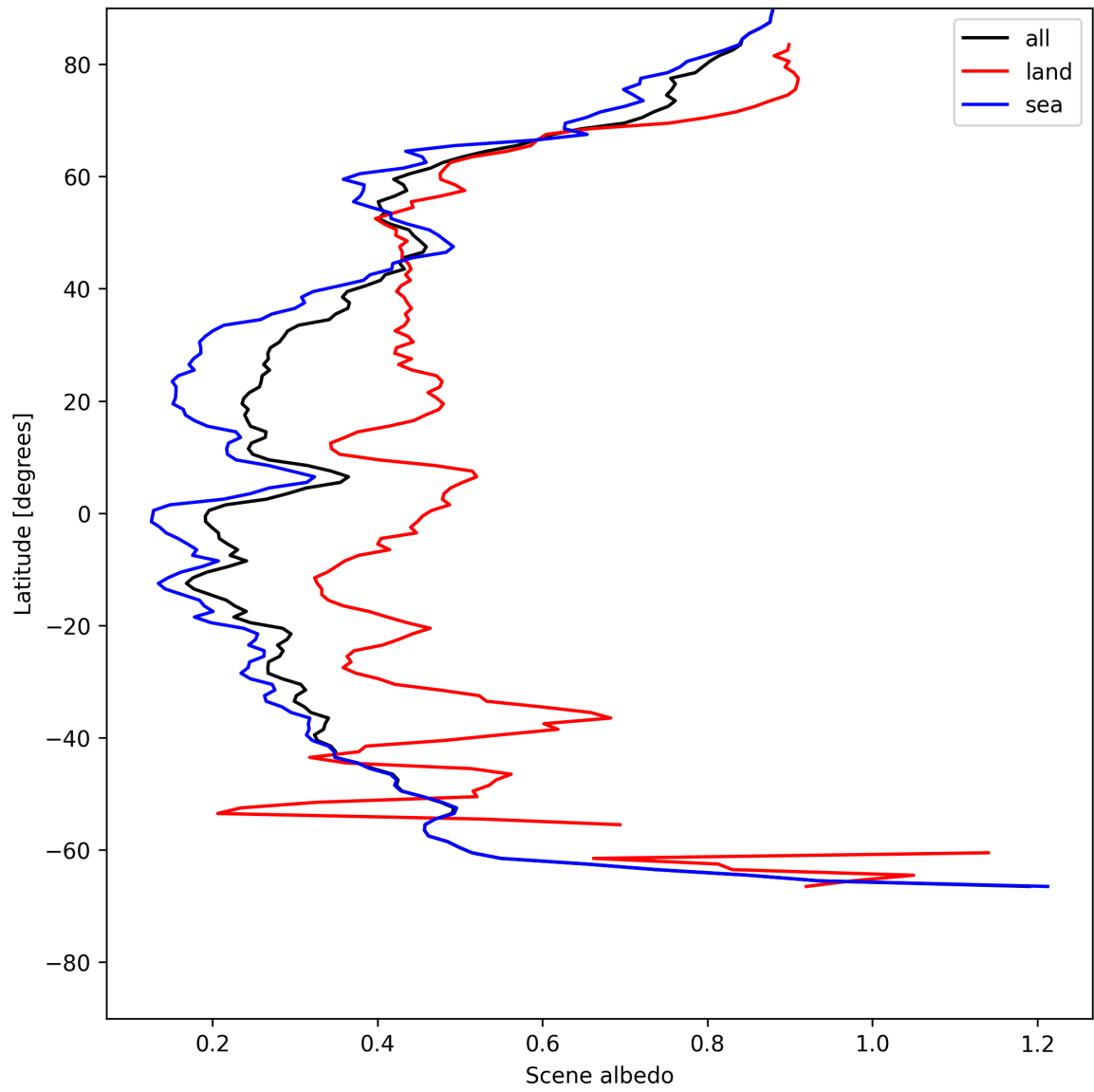
Figure 17: Zonal average of “Scene albedo” for 2025-05-26 to 2025-05-27.
