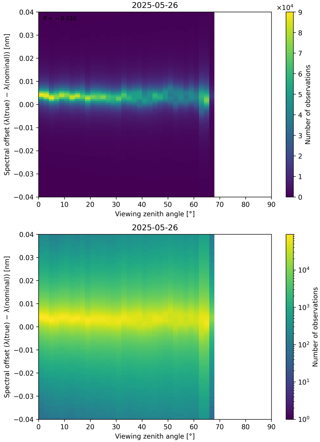
Figure 128: Scatter density plot of “Viewing zenith angle” against “Spectral offset ( \lambda_{\text{true}} - \lambda_{\text{nominal}} )” for 2025-05-26 to 2025-05-27.
