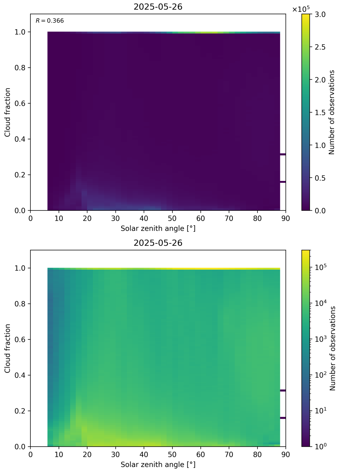
Figure 110: Scatter density plot of “Solar zenith angle” against “Cloud fraction” for 2025-05-26 to 2025-05-27.
