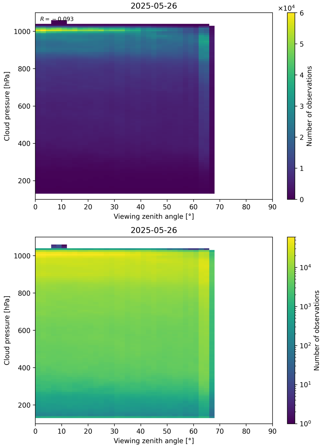
Figure 121: Scatter density plot of “Viewing zenith angle” against “Cloud pressure” for 2025-05-26 to 2025-05-27.
