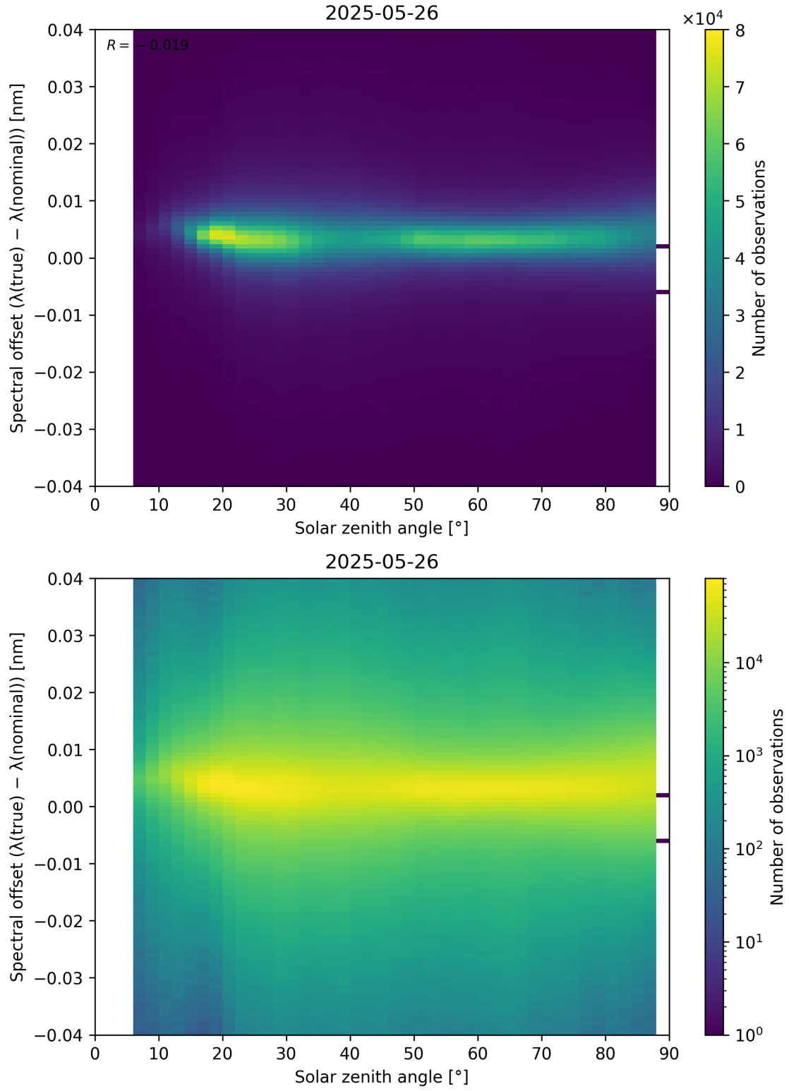
Figure 117: Scatter density plot of “Solar zenith angle” against “Spectral offset ( \lambda_{\text{true}} - \lambda_{\text{nominal}} )” for 2025-05-26 to 2025-05-27.
