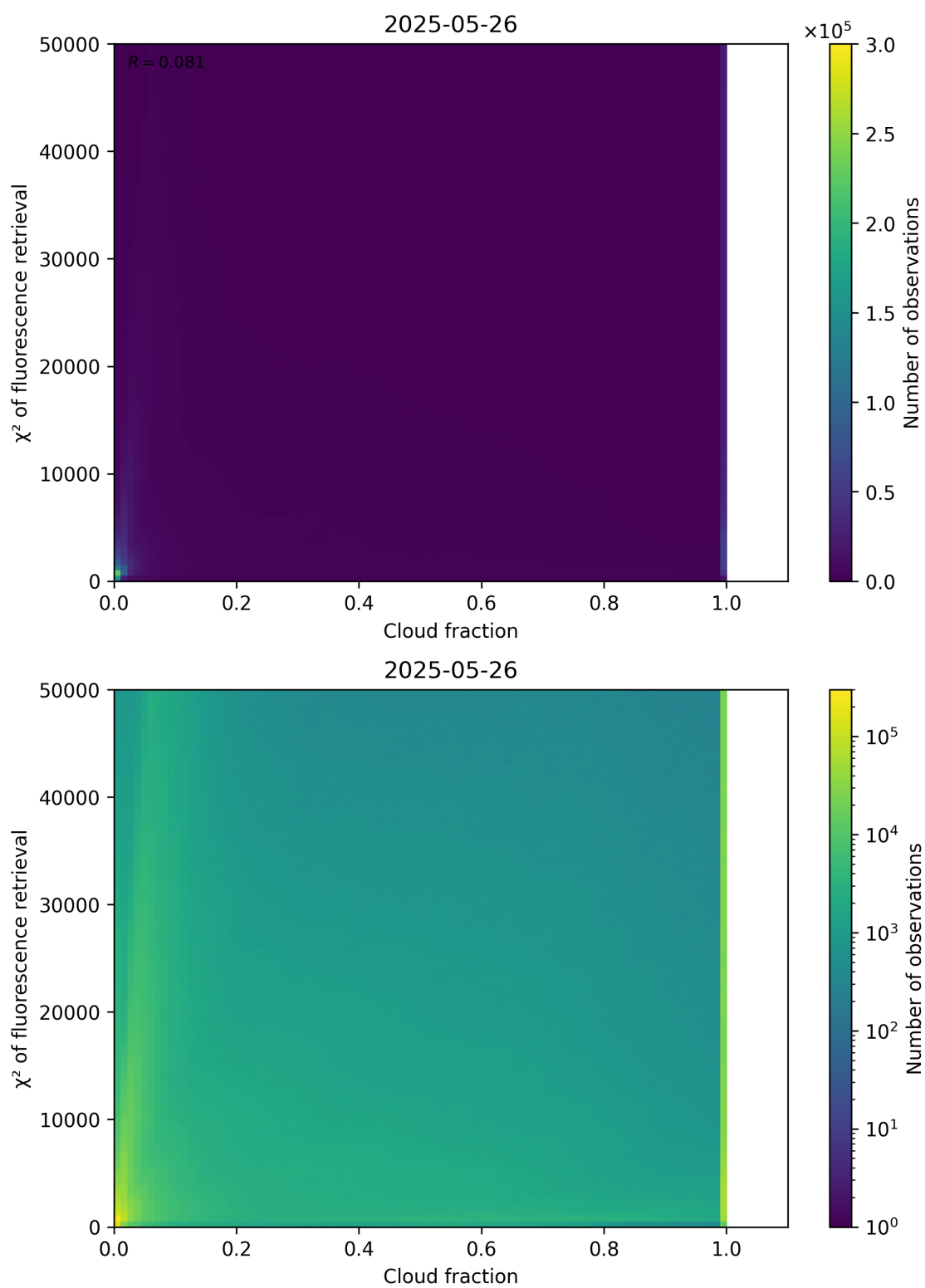
Figure 71: Scatter density plot of “Cloud fraction” against “ \chi^2 of fluorescence retrieval” for 2025-05-26 to 2025-05-27.
