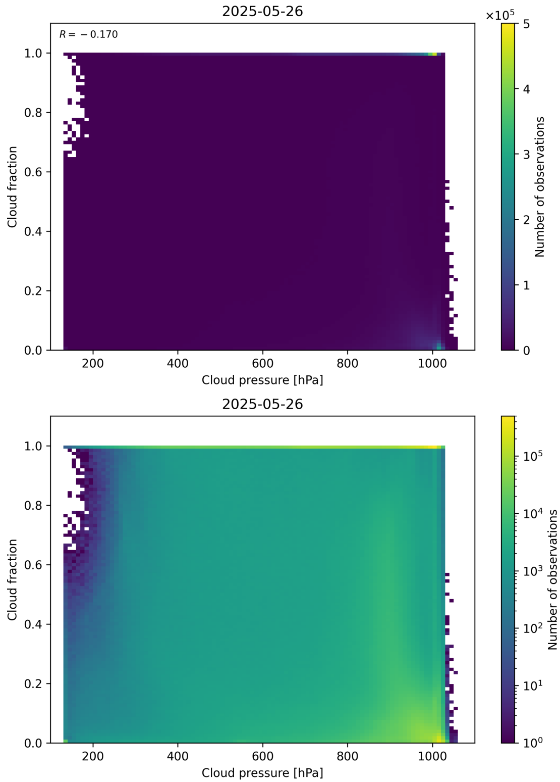
Figure 79: Scatter density plot of “Cloud pressure” against “Cloud fraction” for 2025-05-26 to 2025-05-27.
