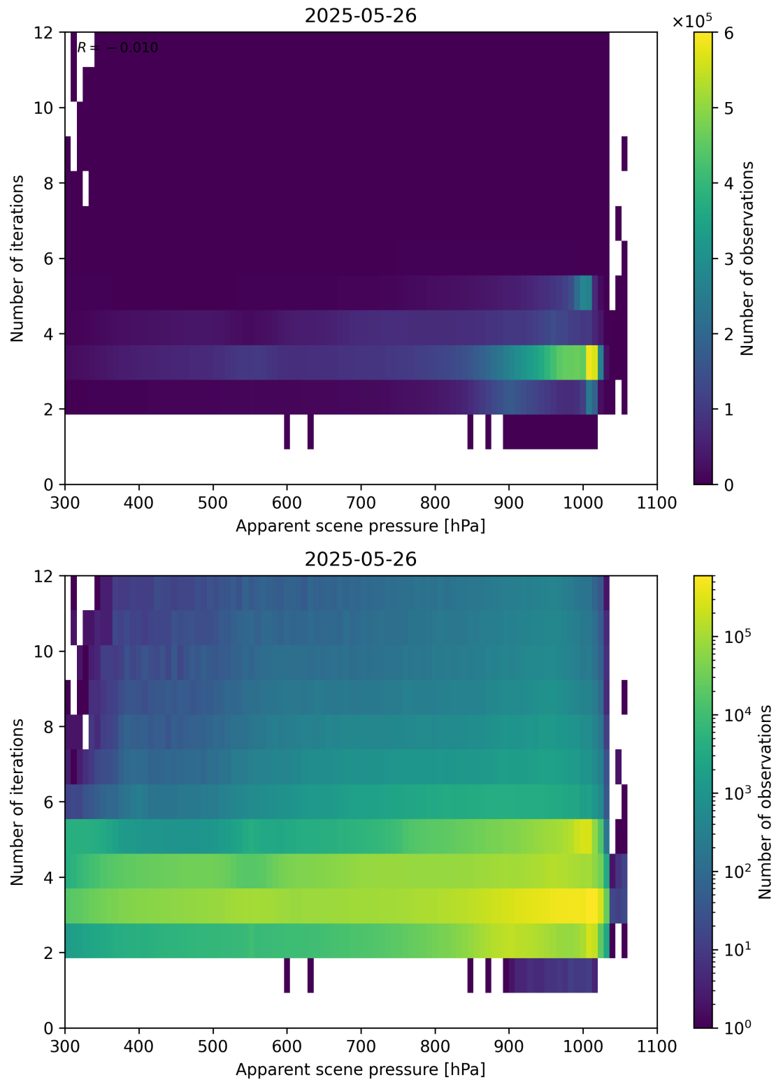
Figure 65: Scatter density plot of “Apparent scene pressure” against “Number of iterations” for 2025-05-26 to 2025-05-27.
