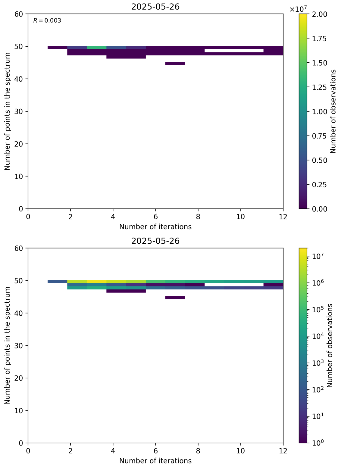
Figure 99: Scatter density plot of “Number of iterations” against “Number of points in the spectrum” for 2025-05-26 to 2025-05-27.
