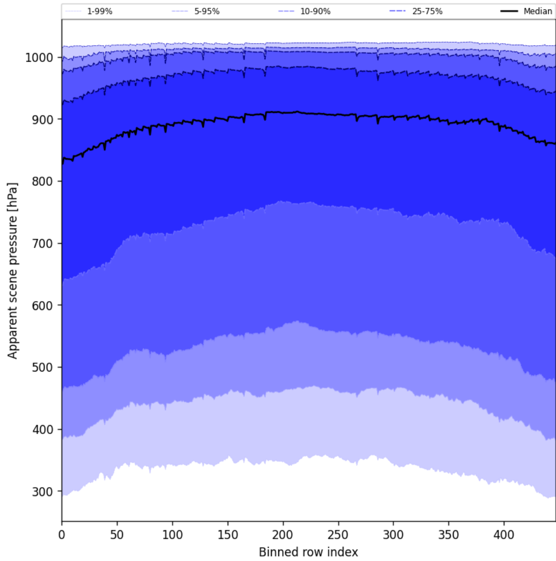
Figure 53: Along track statistics of “Apparent scene pressure” for 2025-05-26 to 2025-05-27
