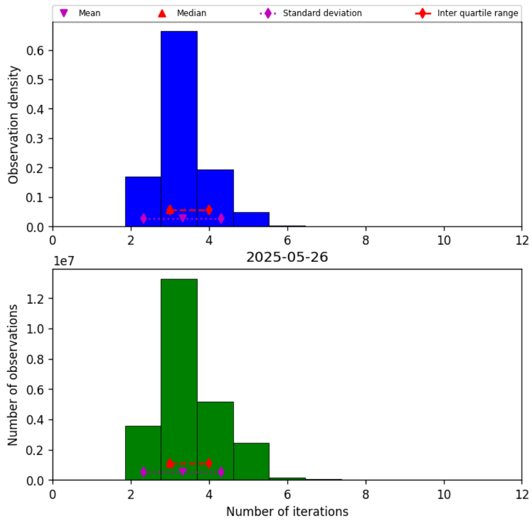
Figure 39: Histogram of “Number of iterations” for 2025-05-26 to 2025-05-27
