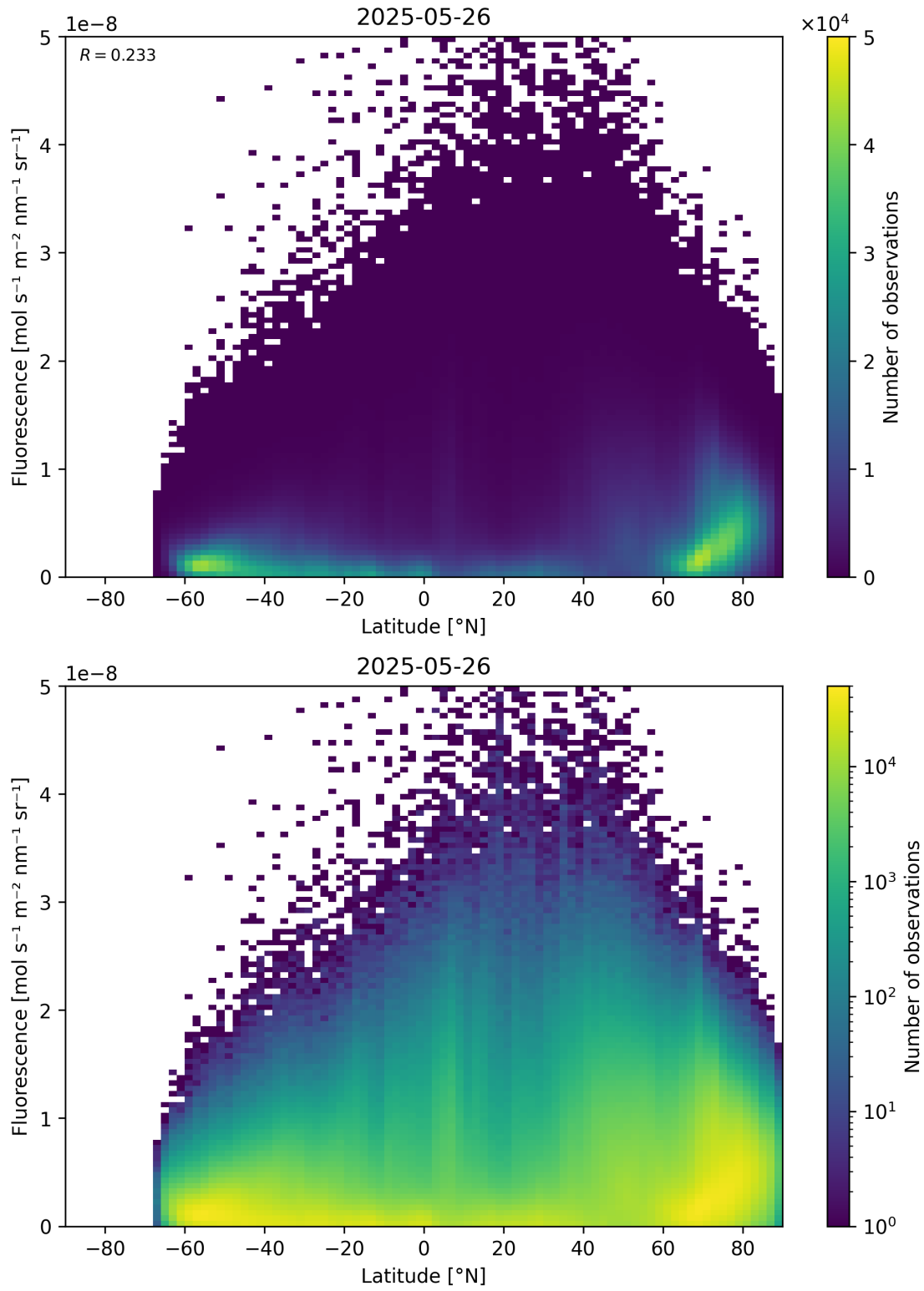
Figure 92: Scatter density plot of “Latitude” against “Fluorescence” for 2025-05-26 to 2025-05-27.
