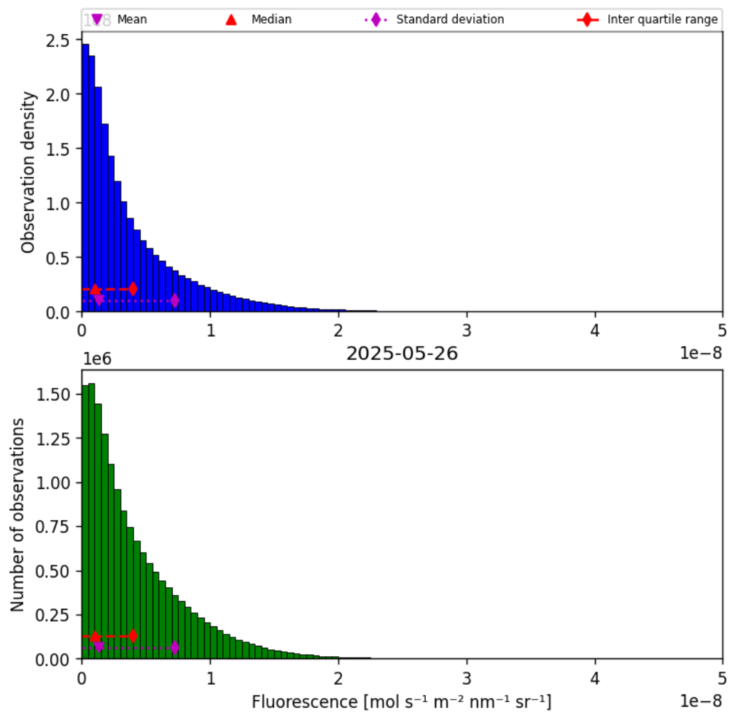
Figure 40: Histogram of “Fluorescence” for 2025-05-26 to 2025-05-27
