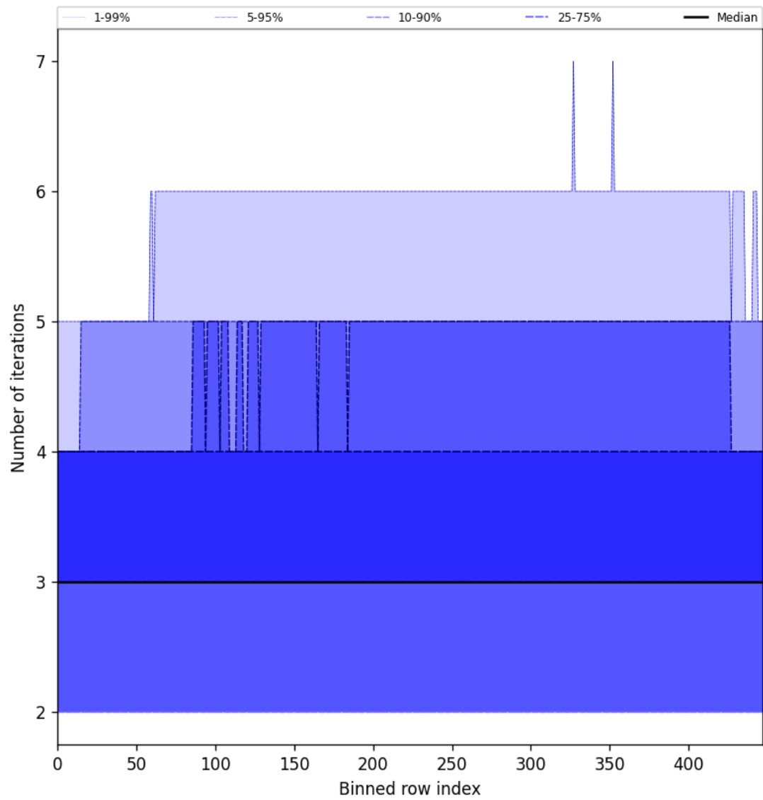
Figure 56: Along track statistics of “Number of iterations” for 2025-05-26 to 2025-05-27
