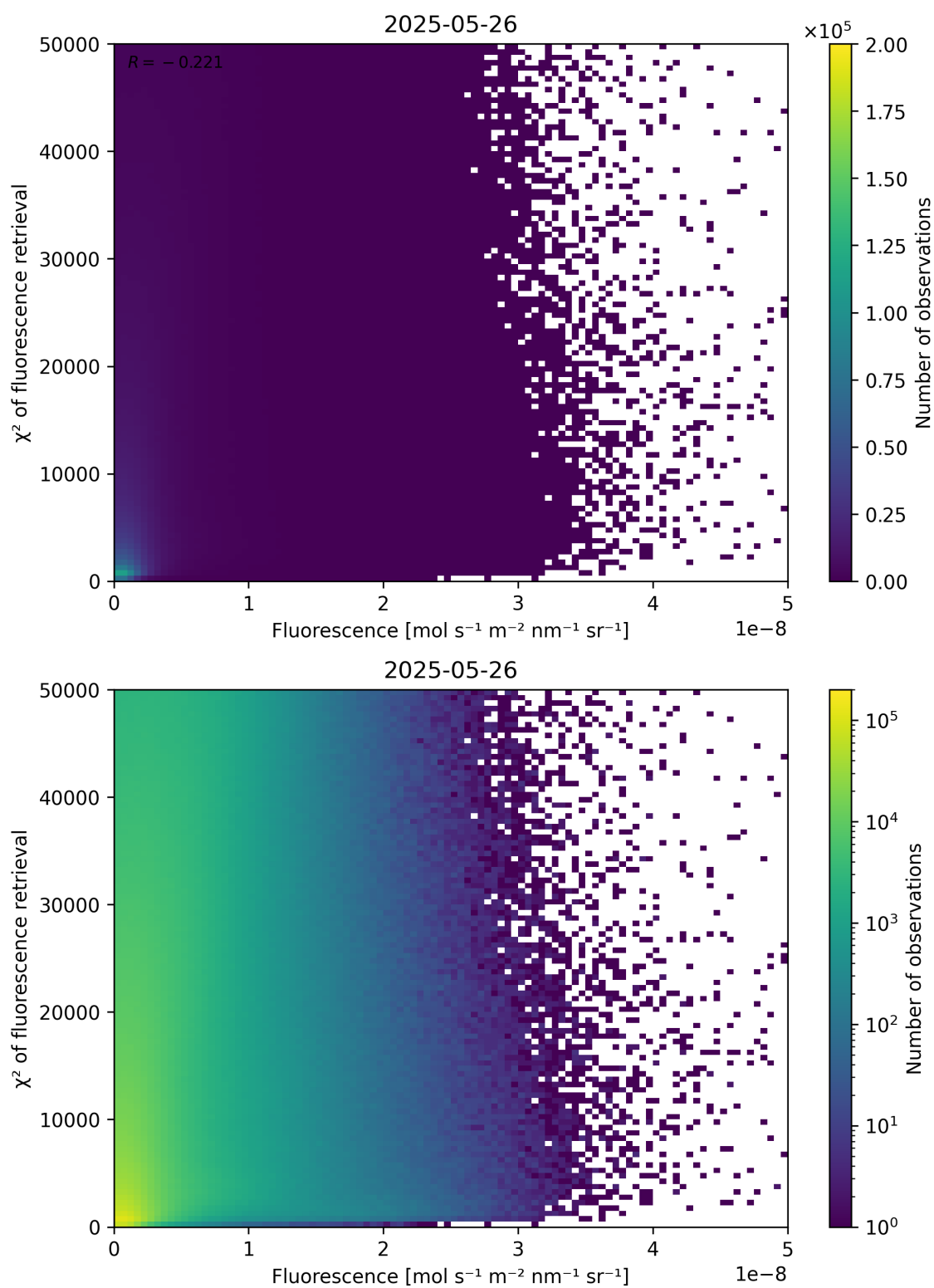
Figure 85: Scatter density plot of “Fluorescence” against “ \chi^2 of fluorescence retrieval” for 2025-05-26 to 2025-05-27.
