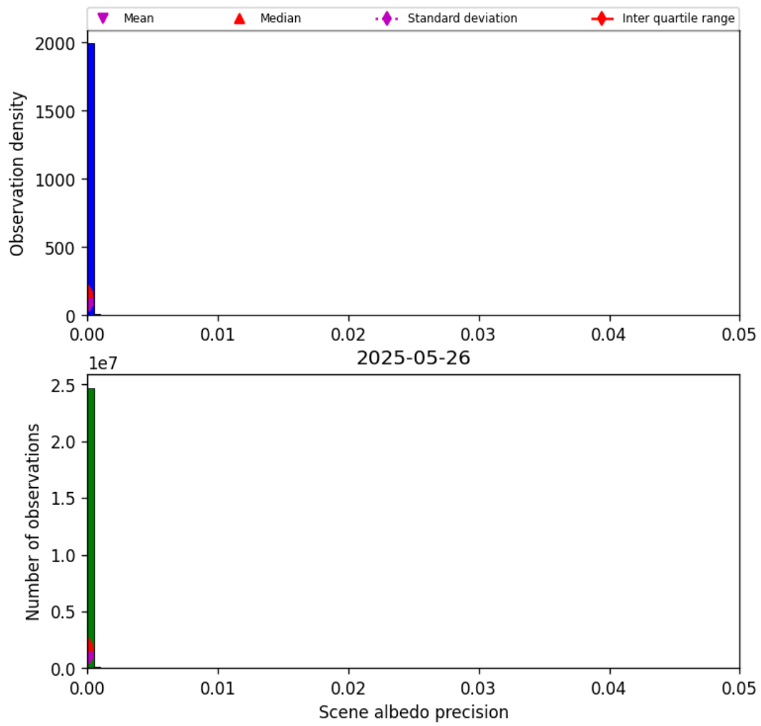
Figure 35: Histogram of “Scene albedo precision” for 2025-05-26 to 2025-05-27
