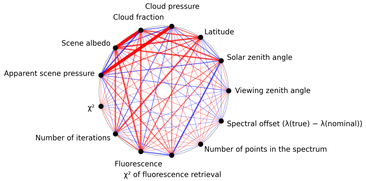
Figure 1: Map of correlation graph for 2025-05-26 to 2025-05-27.
