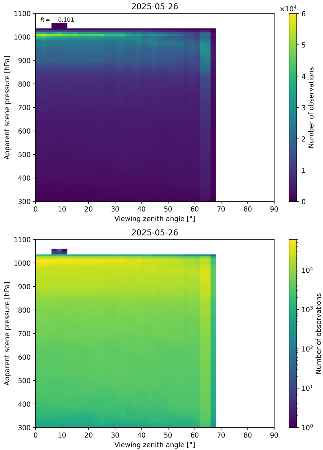
Figure 118: Scatter density plot of “Viewing zenith angle” against “Apparent scene pressure” for 2025-05-26 to 2025-05-27.
