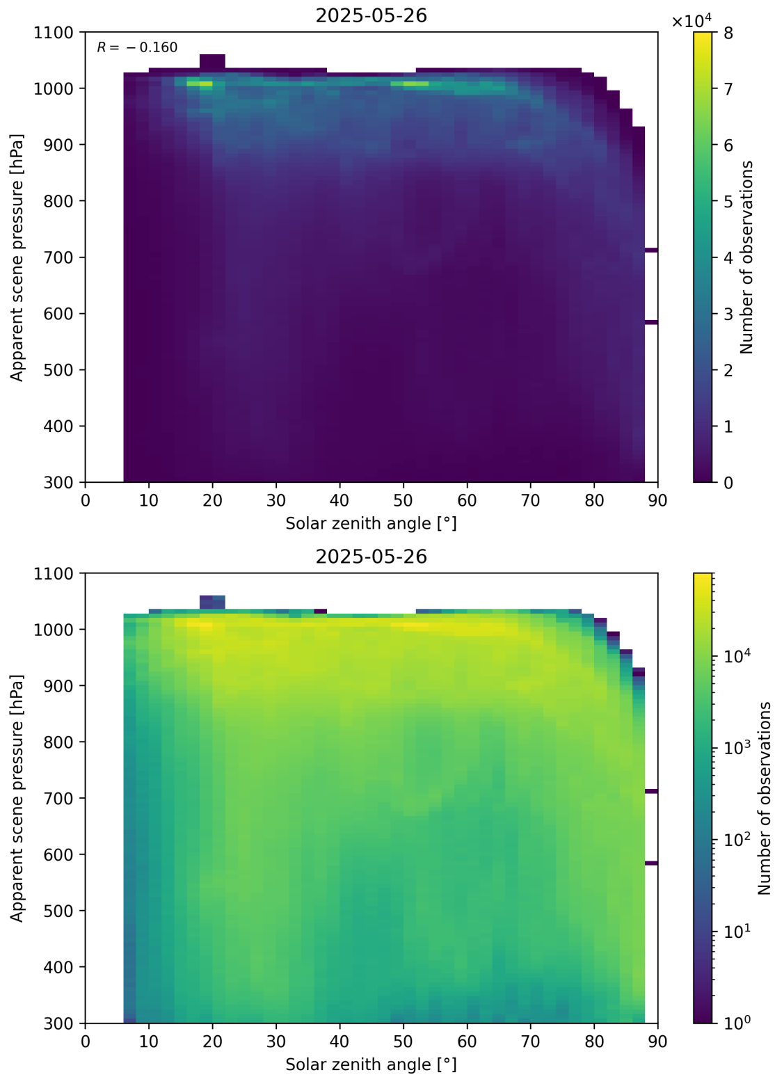
Figure 108: Scatter density plot of “Solar zenith angle” against “Apparent scene pressure” for 2025-05-26 to 2025-05-27.
