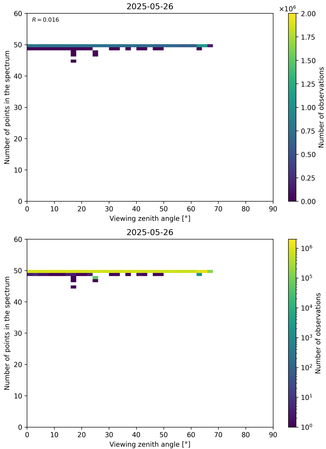
Figure 125: Scatter density plot of “Viewing zenith angle” against “Number of points in the spectrum” for 2025-05-26 to 2025-05-27.
