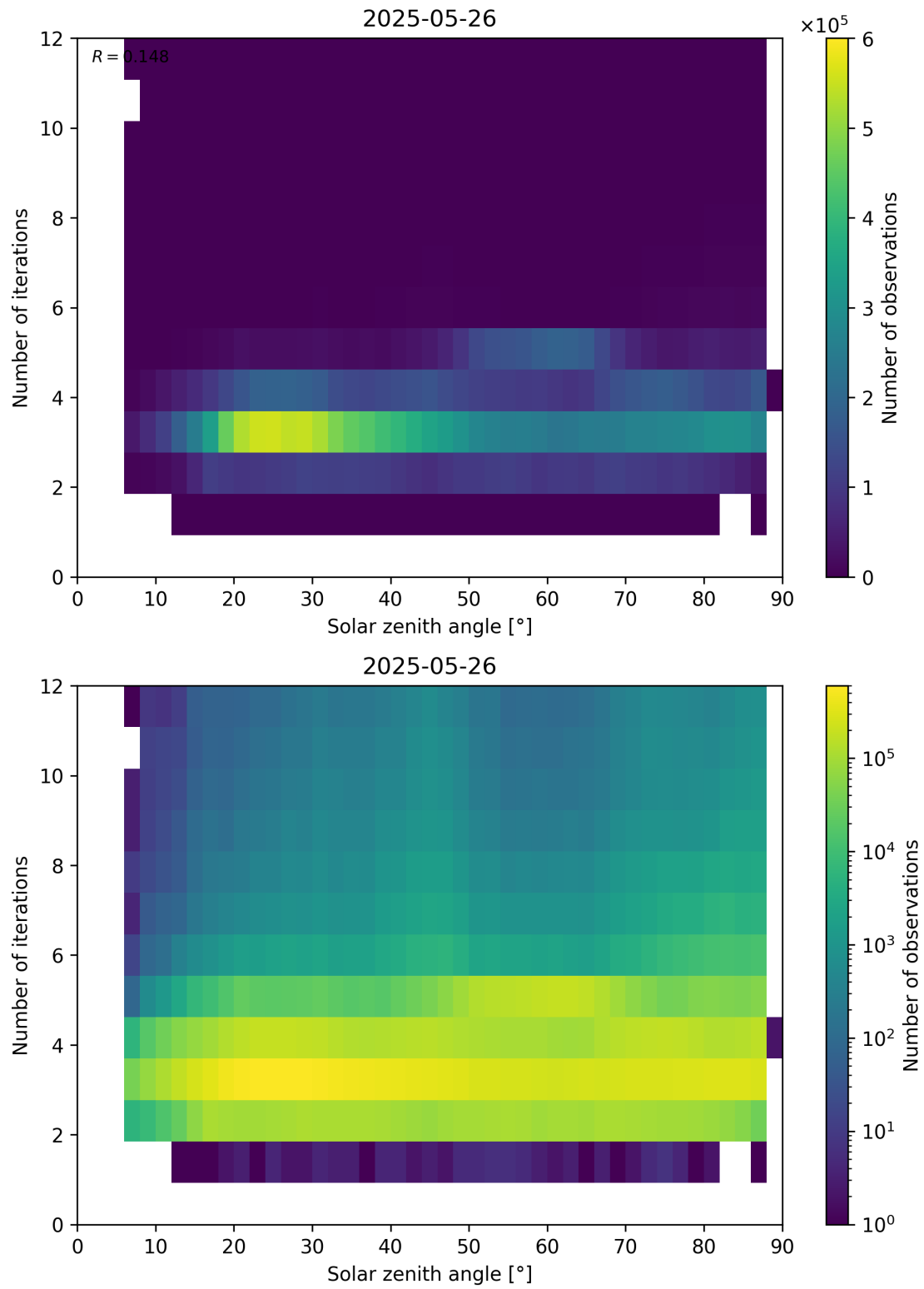
Figure 114: Scatter density plot of “Solar zenith angle” against “Number of iterations” for 2025-05-26 to 2025-05-27.
