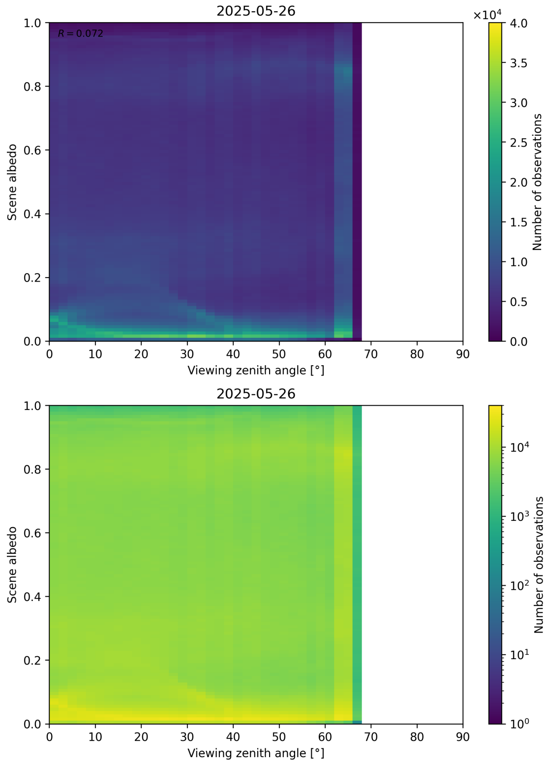
Figure 126: Scatter density plot of “Viewing zenith angle” against “Scene albedo” for 2025-05-26 to 2025-05-27.
