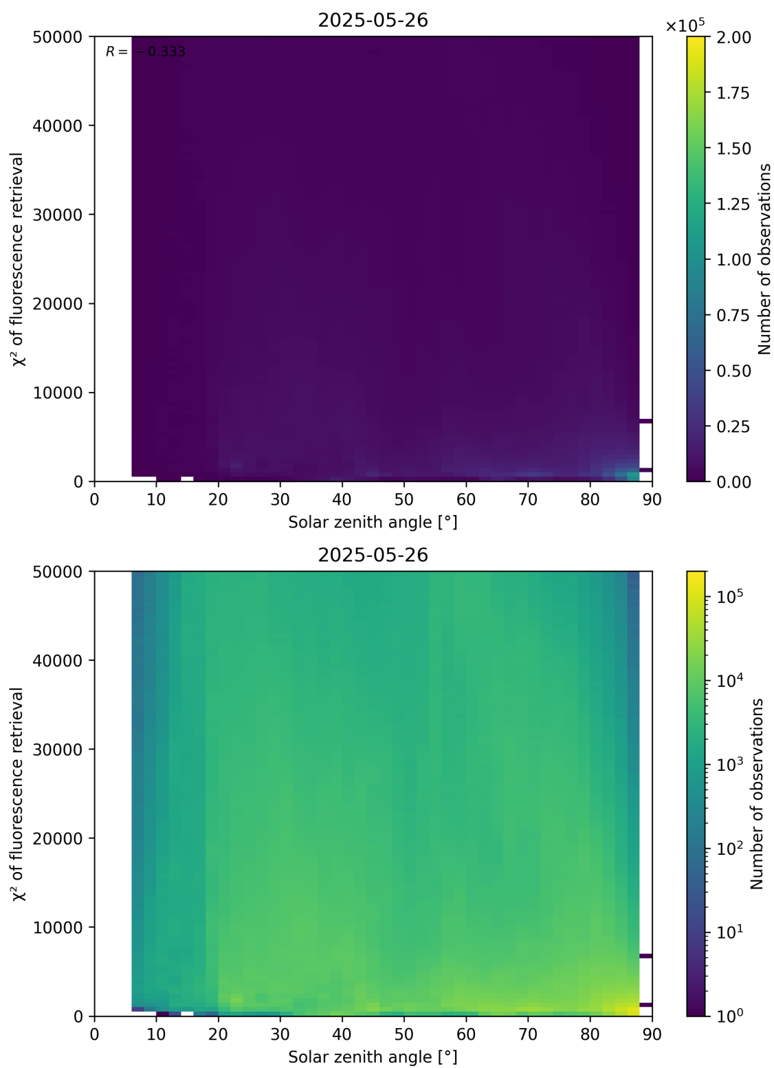
Figure 109: Scatter density plot of “Solar zenith angle” against “ \chi^2 of fluorescence retrieval” for 2025-05-26 to 2025-05-27.
