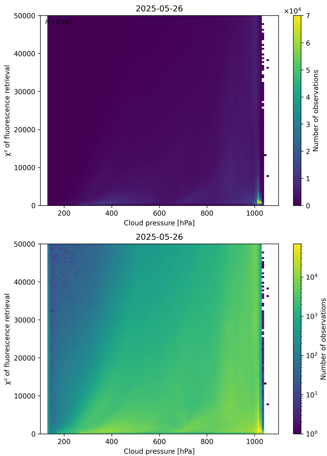
Figure 78: Scatter density plot of “Cloud pressure” against “ \chi^2 of fluorescence retrieval” for 2025-05-26 to 2025-05-27.
