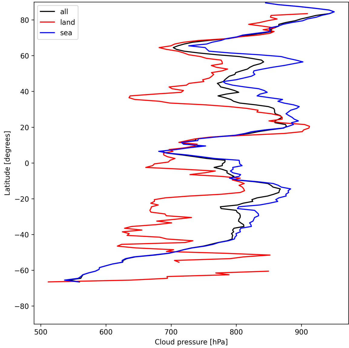
Figure 13: Zonal average of “Cloud pressure” for 2025-05-26 to 2025-05-27.
