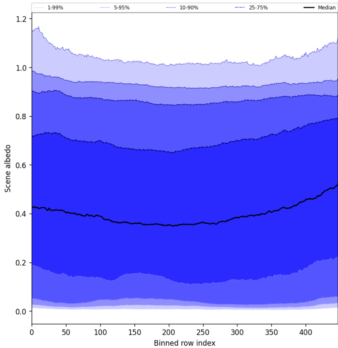
Figure 51: Along track statistics of “Scene albedo” for 2025-05-26 to 2025-05-27
