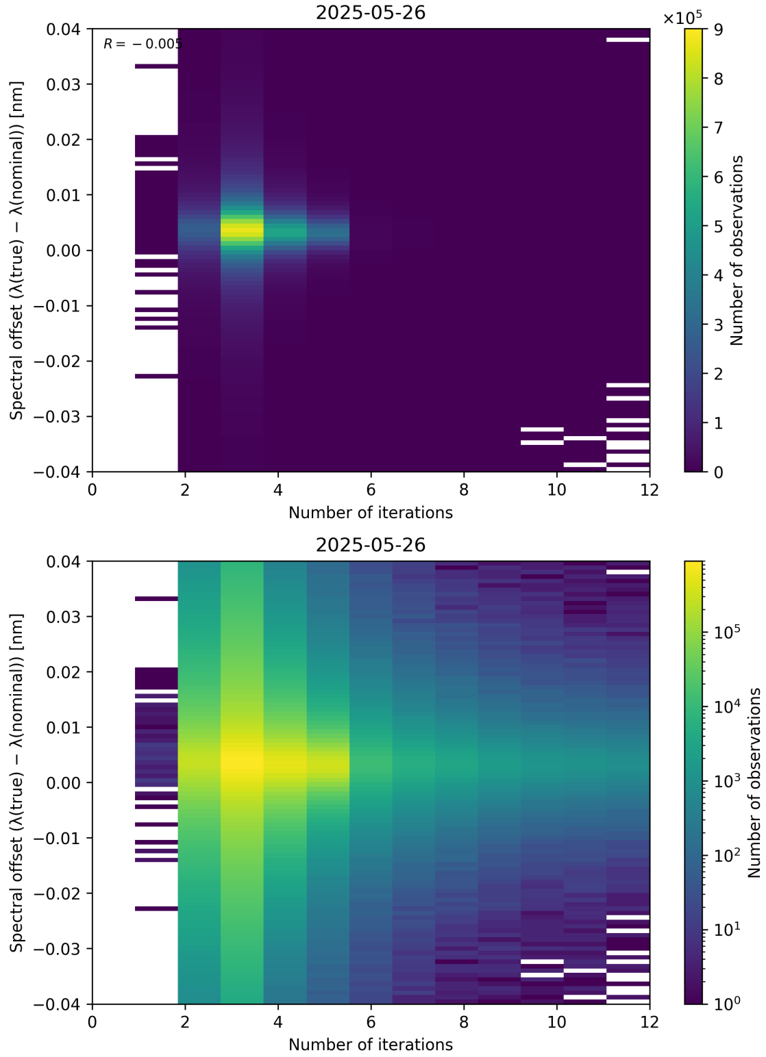
Figure 100: Scatter density plot of “Number of iterations” against “Spectral offset ( \lambda_{\text{true}} - \lambda_{\text{nominal}} )” for 2025-05-26 to 2025-05-27.
