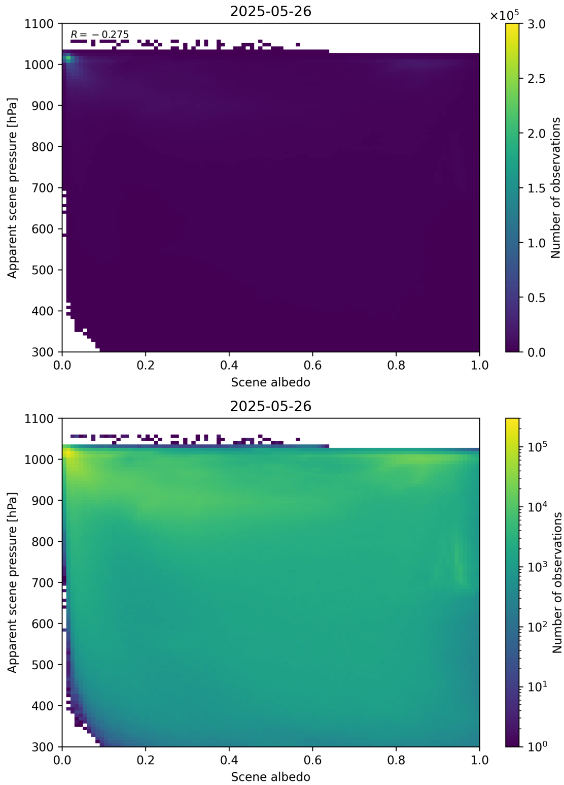
Figure 102: Scatter density plot of “Scene albedo” against “Apparent scene pressure” for 2025-05-26 to 2025-05-27.
