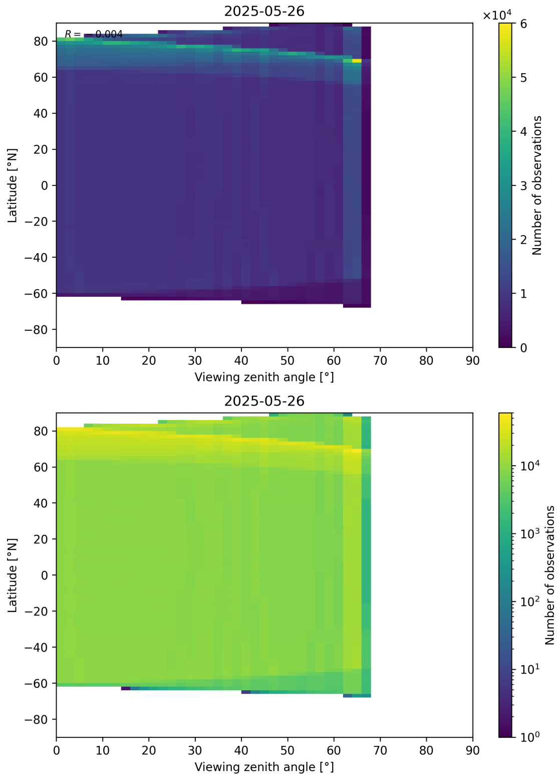
Figure 123: Scatter density plot of “Viewing zenith angle” against “Latitude” for 2025-05-26 to 2025-05-27.
