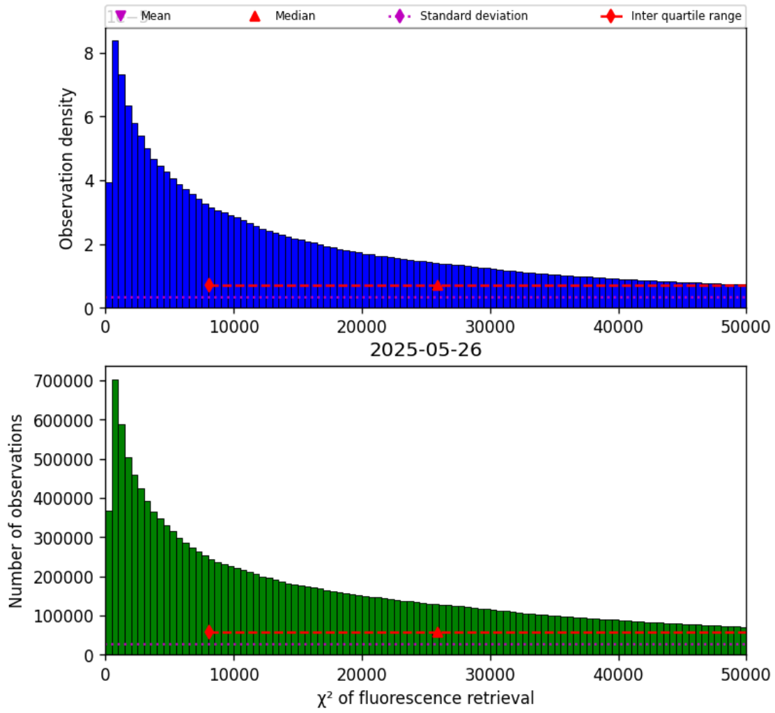
Figure 42: Histogram of “ \chi^2 of fluorescence retrieval” for 2025-05-26 to 2025-05-27
