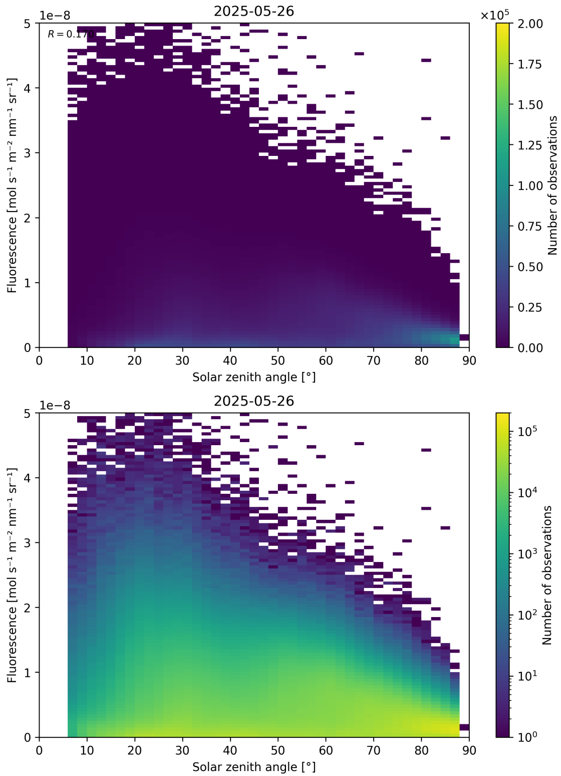
Figure 112: Scatter density plot of “Solar zenith angle” against “Fluorescence” for 2025-05-26 to 2025-05-27.
