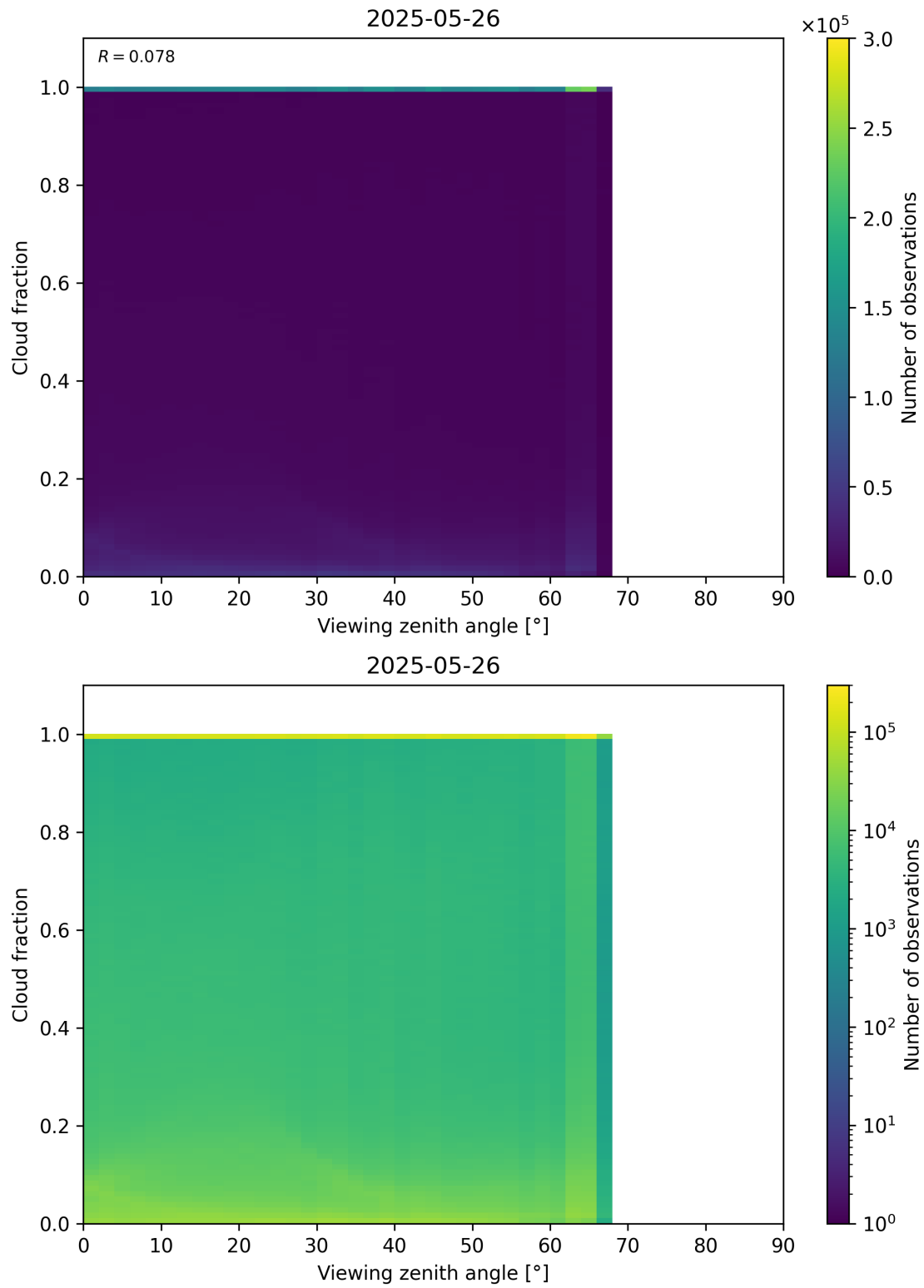
Figure 120: Scatter density plot of “Viewing zenith angle” against “Cloud fraction” for 2025-05-26 to 2025-05-27.
