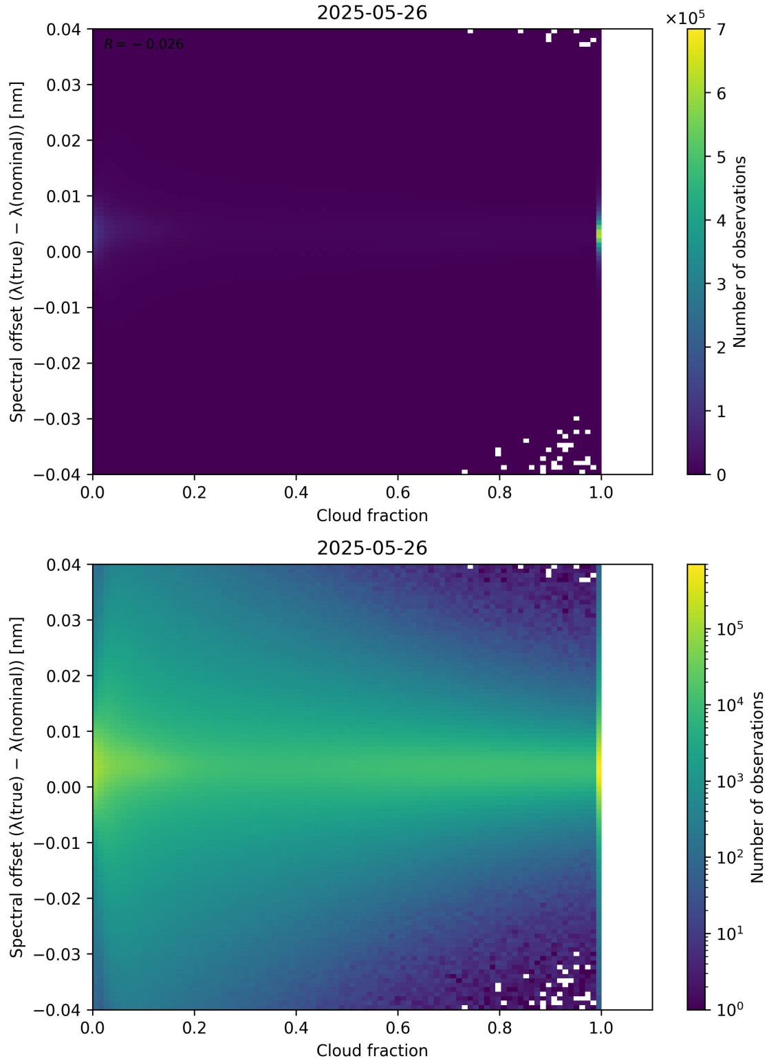
Figure 76: Scatter density plot of “Cloud fraction” against “Spectral offset ( \lambda_{\text{true}} - \lambda_{\text{nominal}} )” for 2025-05-26 to 2025-05-27.
