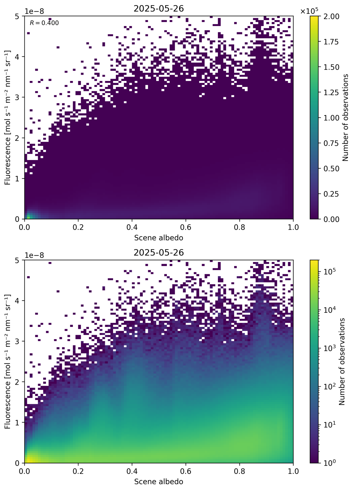
Figure 104: Scatter density plot of “Scene albedo” against “Fluorescence” for 2025-05-26 to 2025-05-27.
