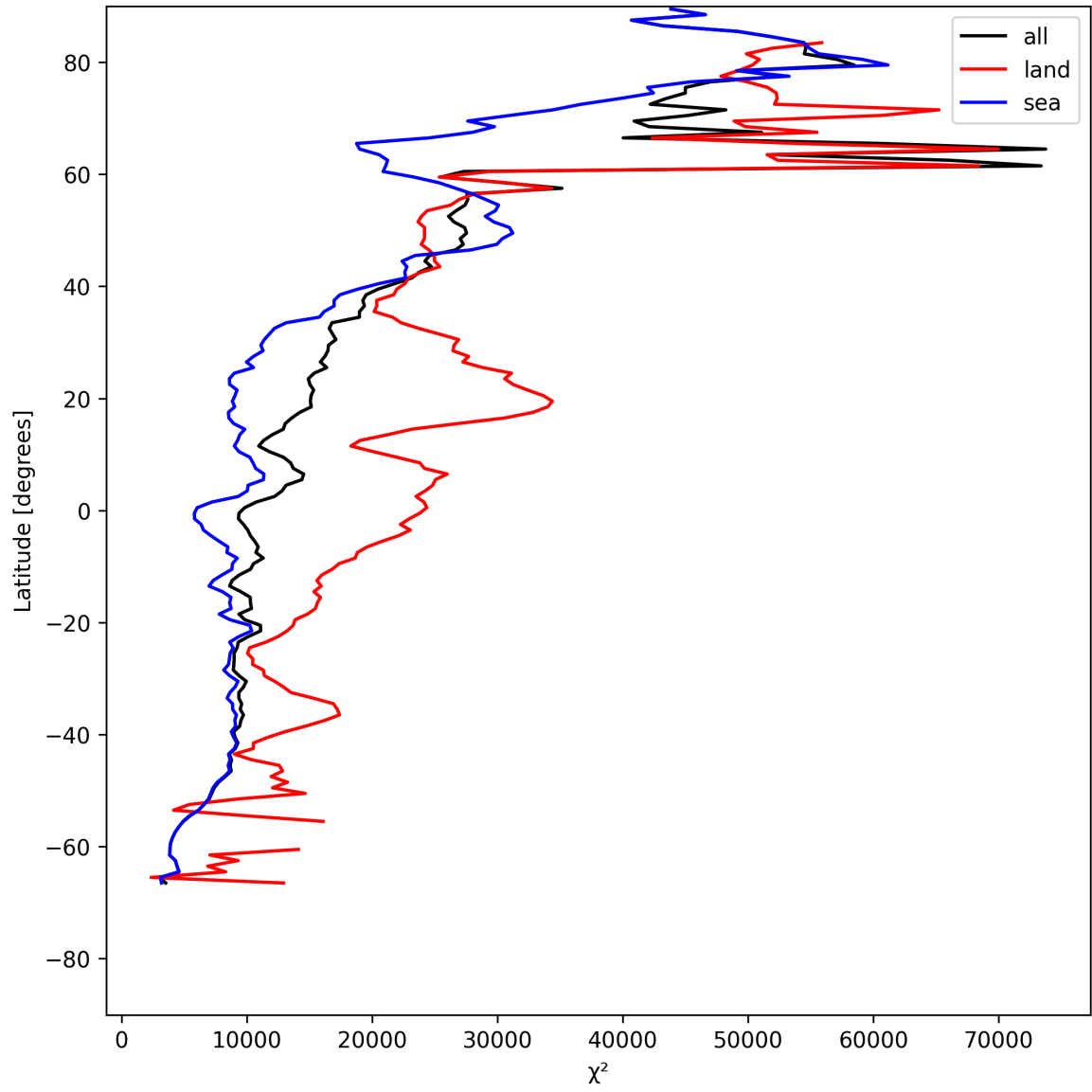
Figure 21: Zonal average of “ \chi^2 ” for 2025-05-26 to 2025-05-27.
