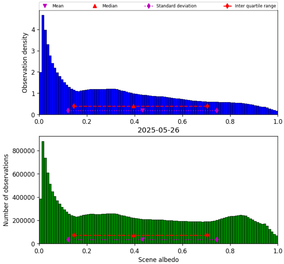
Figure 34: Histogram of “Scene albedo” for 2025-05-26 to 2025-05-27
