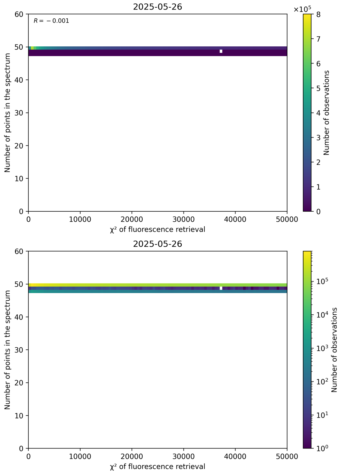
Figure 68: Scatter density plot of “ \chi^2 of fluorescence retrieval” against “Number of points in the spectrum” for 2025-05-26 to 2025-05-27.
