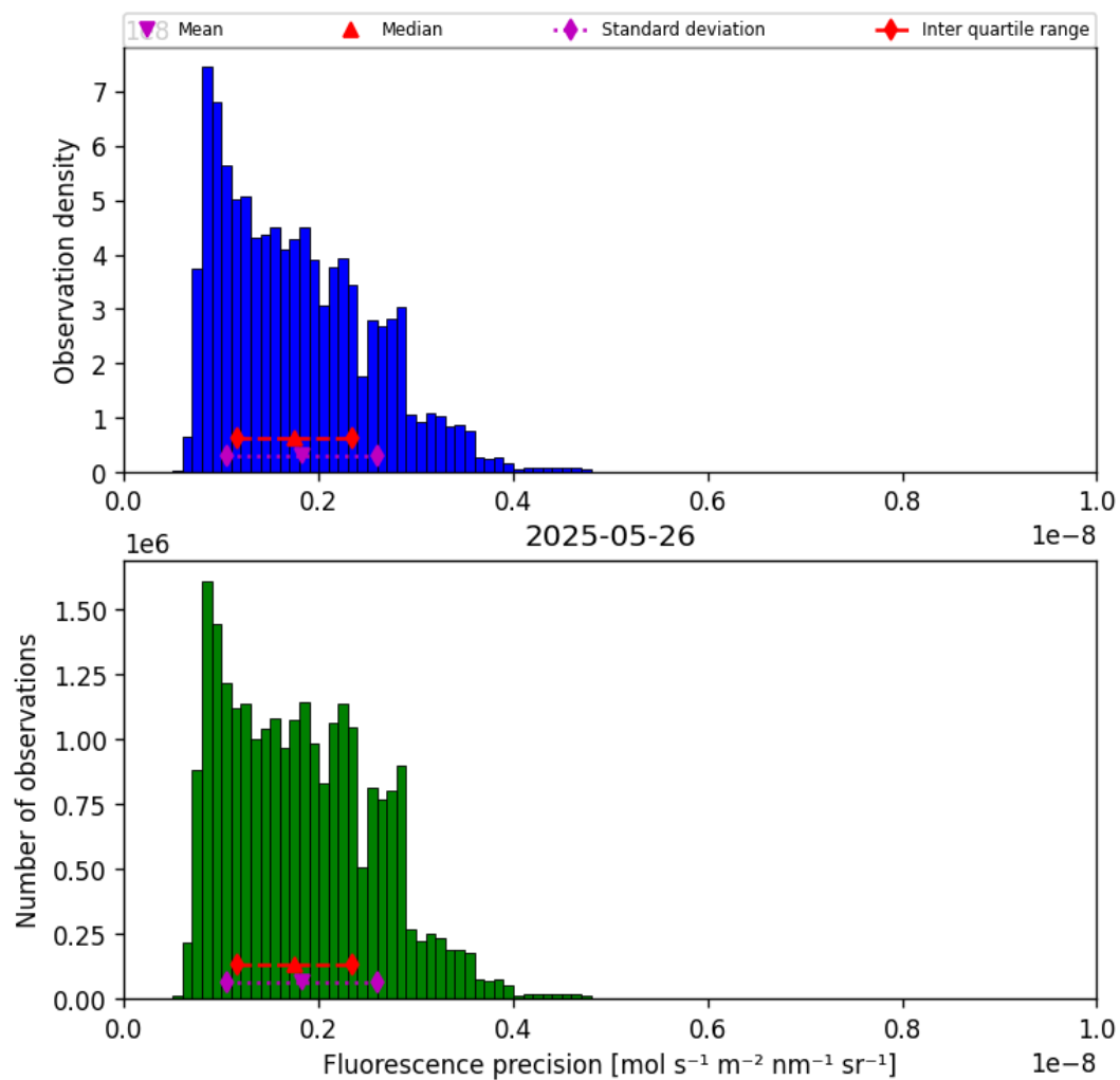
Figure 41: Histogram of “Fluorescence precision” for 2025-05-26 to 2025-05-27
