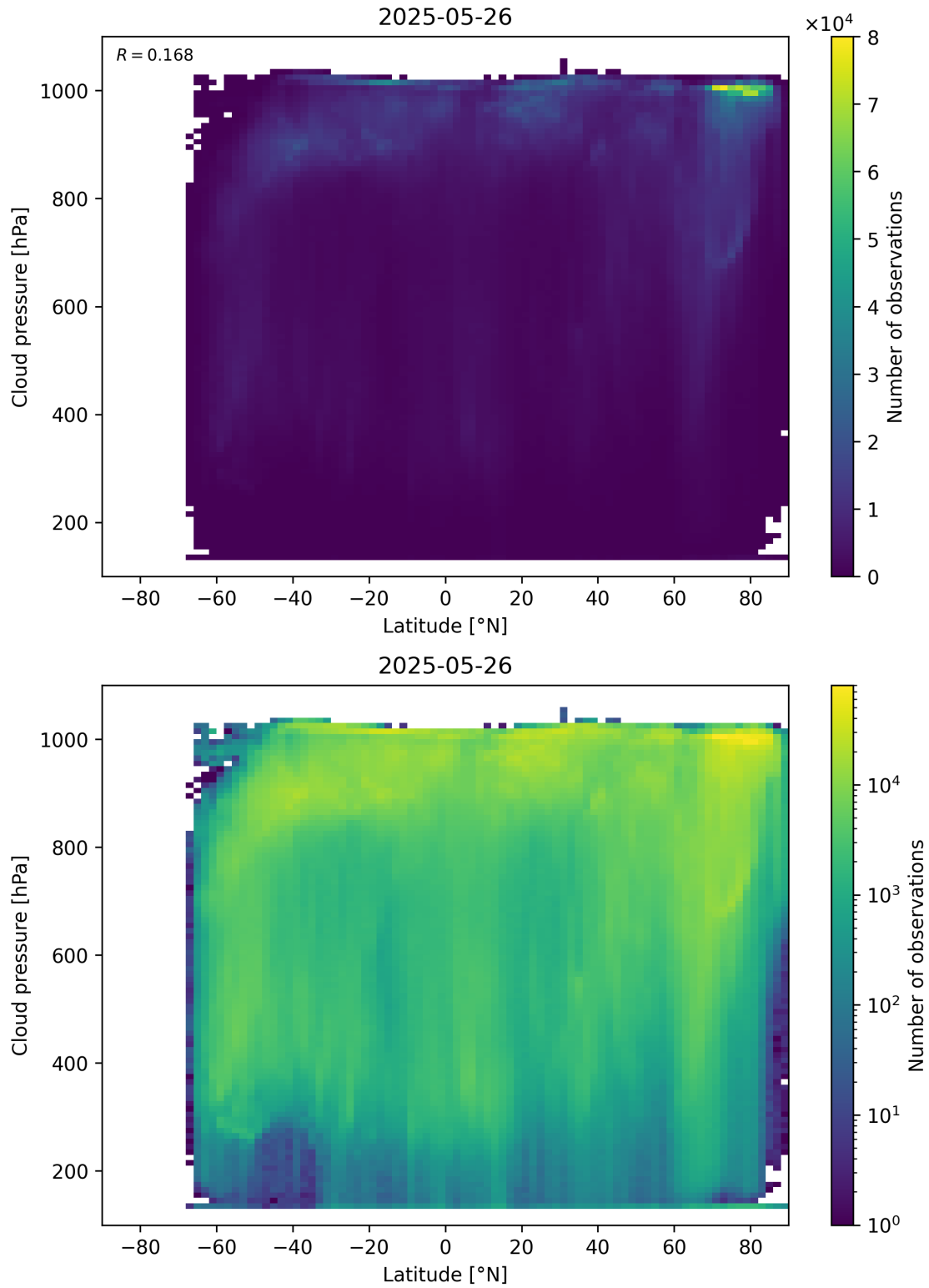
Figure 91: Scatter density plot of “Latitude” against “Cloud pressure” for 2025-05-26 to 2025-05-27.
