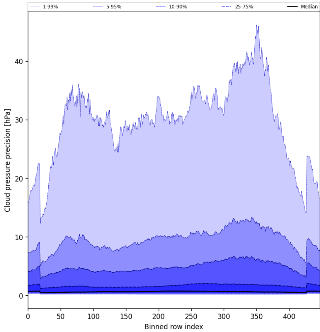
Figure 48: Along track statistics of “Cloud pressure precision” for 2025-05-26 to 2025-05-27
