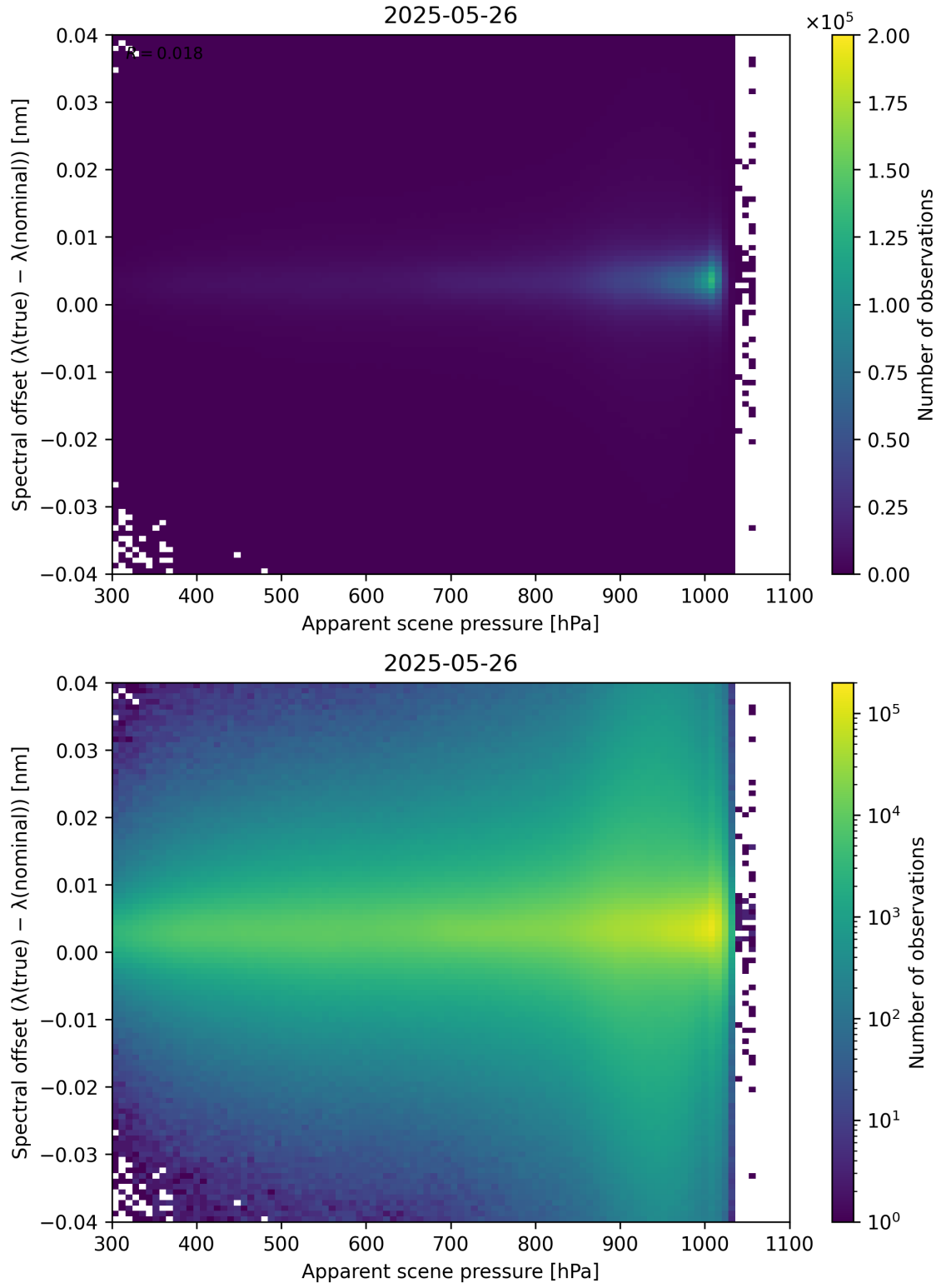
Figure 67: Scatter density plot of “Apparent scene pressure” against “Spectral offset ( \lambda_{\text{true}} - \lambda_{\text{nominal}} )” for 2025-05-26 to 2025-05-27.
