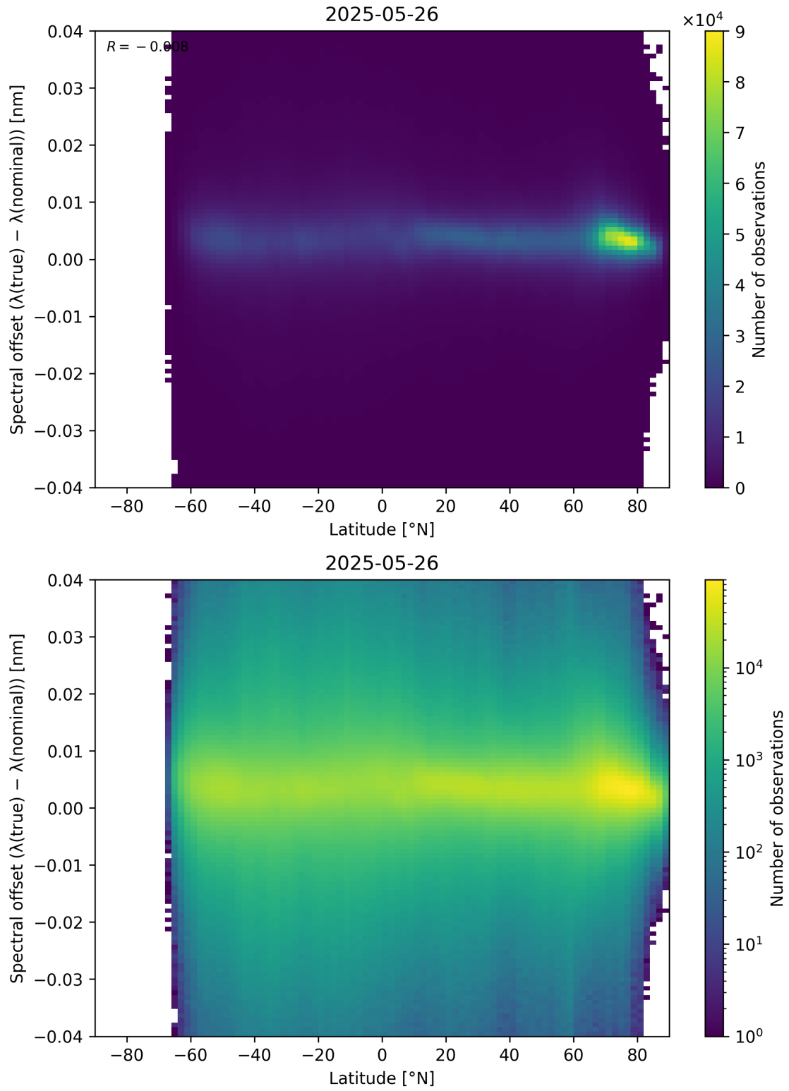
Figure 96: Scatter density plot of “Latitude” against “Spectral offset ( \lambda_{\text{true}} - \lambda_{\text{nominal}} )” for 2025-05-26 to 2025-05-27.
