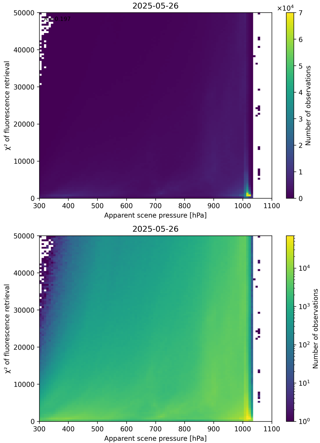
Figure 63: Scatter density plot of “Apparent scene pressure” against “ \chi^2 of fluorescence retrieval” for 2025-05-26 to 2025-05-27.
