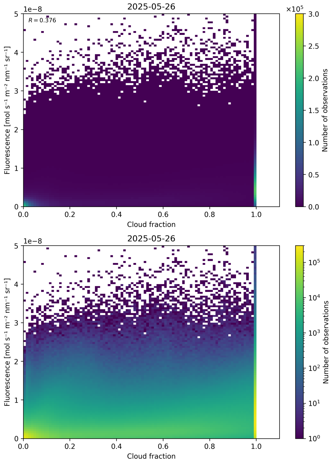
Figure 72: Scatter density plot of “Cloud fraction” against “Fluorescence” for 2025-05-26 to 2025-05-27.
