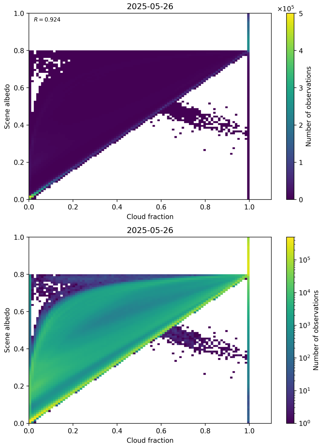
Figure 75: Scatter density plot of “Cloud fraction” against “Scene albedo” for 2025-05-26 to 2025-05-27.
