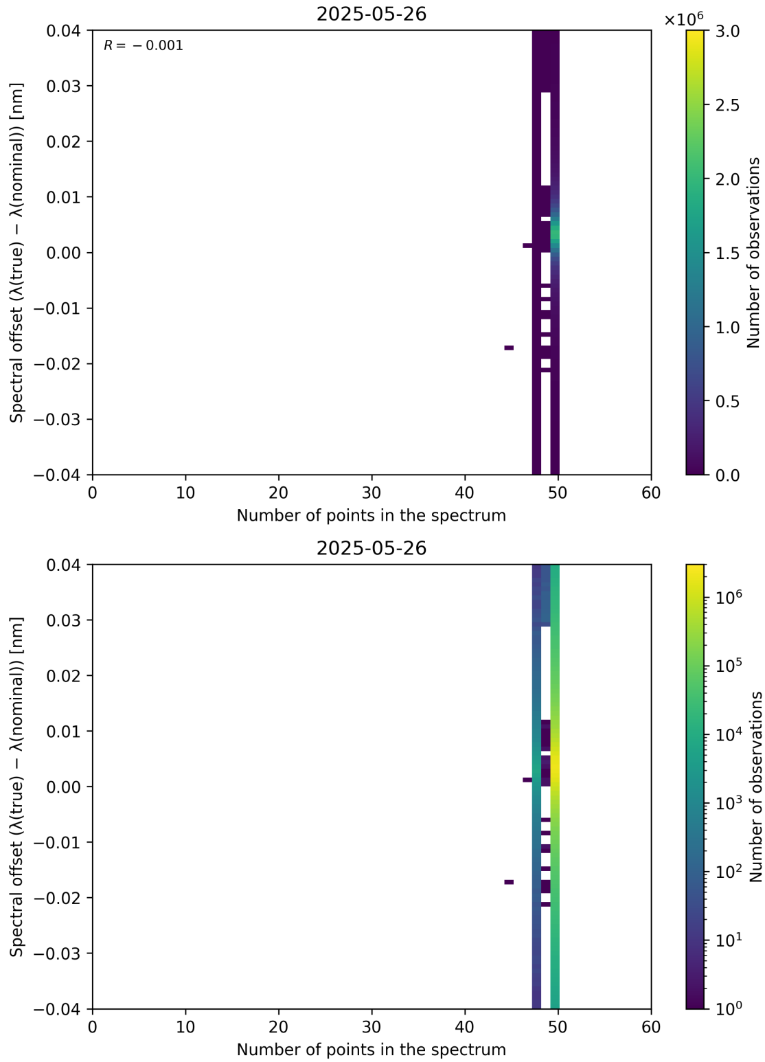
Figure 101: Scatter density plot of “Number of points in the spectrum” against “Spectral offset ( \lambda_{\text{true}} - \lambda_{\text{nominal}} )” for 2025-05-26 to 2025-05-27.
