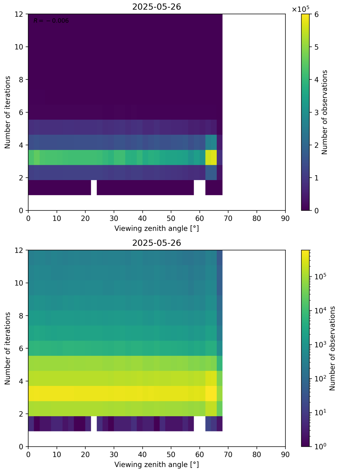
Figure 124: Scatter density plot of “Viewing zenith angle” against “Number of iterations” for 2025-05-26 to 2025-05-27.
