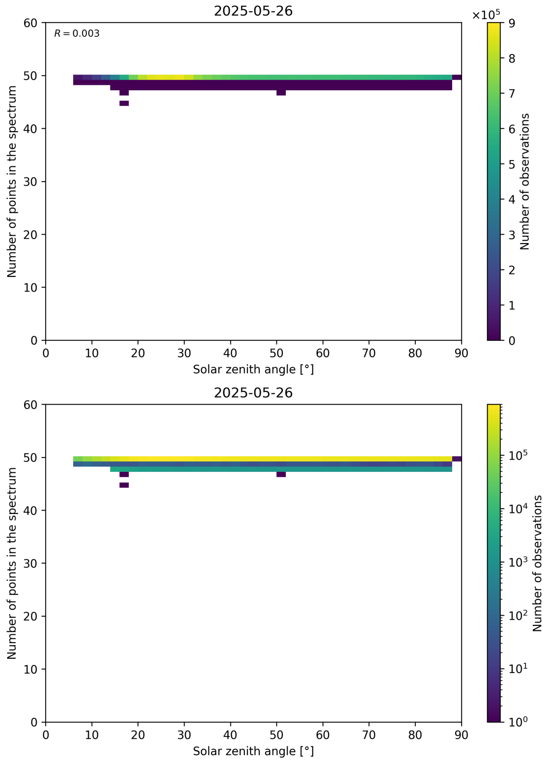
Figure 115: Scatter density plot of “Solar zenith angle” against “Number of points in the spectrum” for 2025-05-26 to 2025-05-27.
