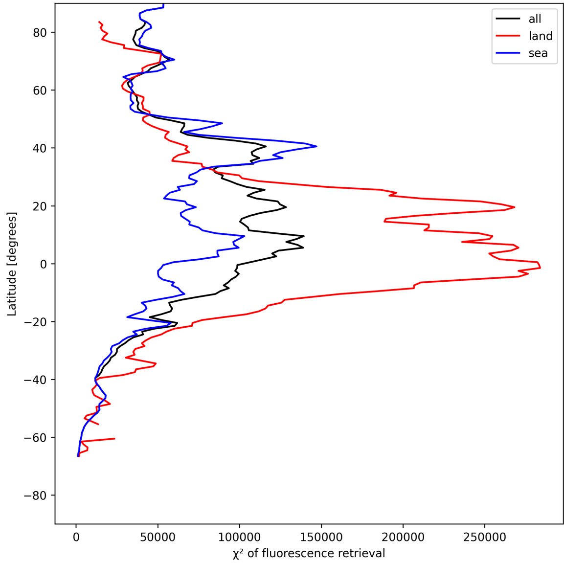
Figure 25: Zonal average of “ \chi^2 of fluorescence retrieval” for 2025-05-26 to 2025-05-27.
