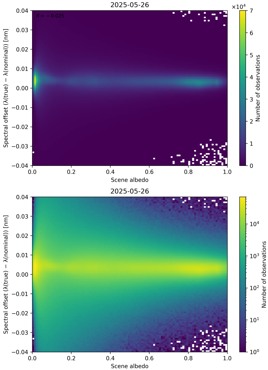
Figure 107: Scatter density plot of “Scene albedo” against “Spectral offset ( \lambda_{\text{true}} - \lambda_{\text{nominal}} )” for 2025-05-26 to 2025-05-27.
