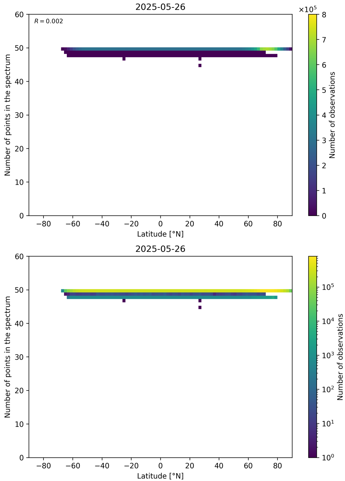
Figure 94: Scatter density plot of “Latitude” against “Number of points in the spectrum” for 2025-05-26 to 2025-05-27.
