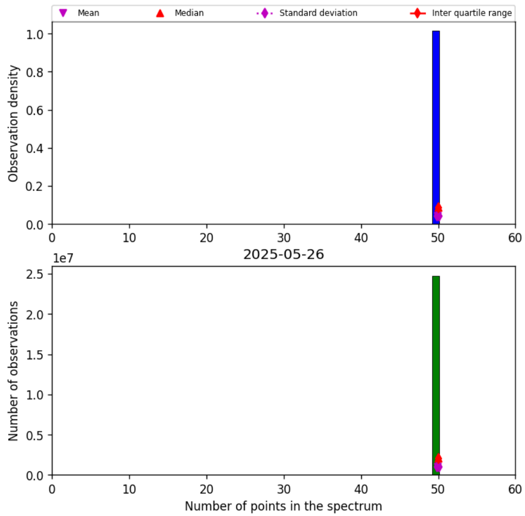
Figure 44: Histogram of “Number of points in the spectrum” for 2025-05-26 to 2025-05-27
