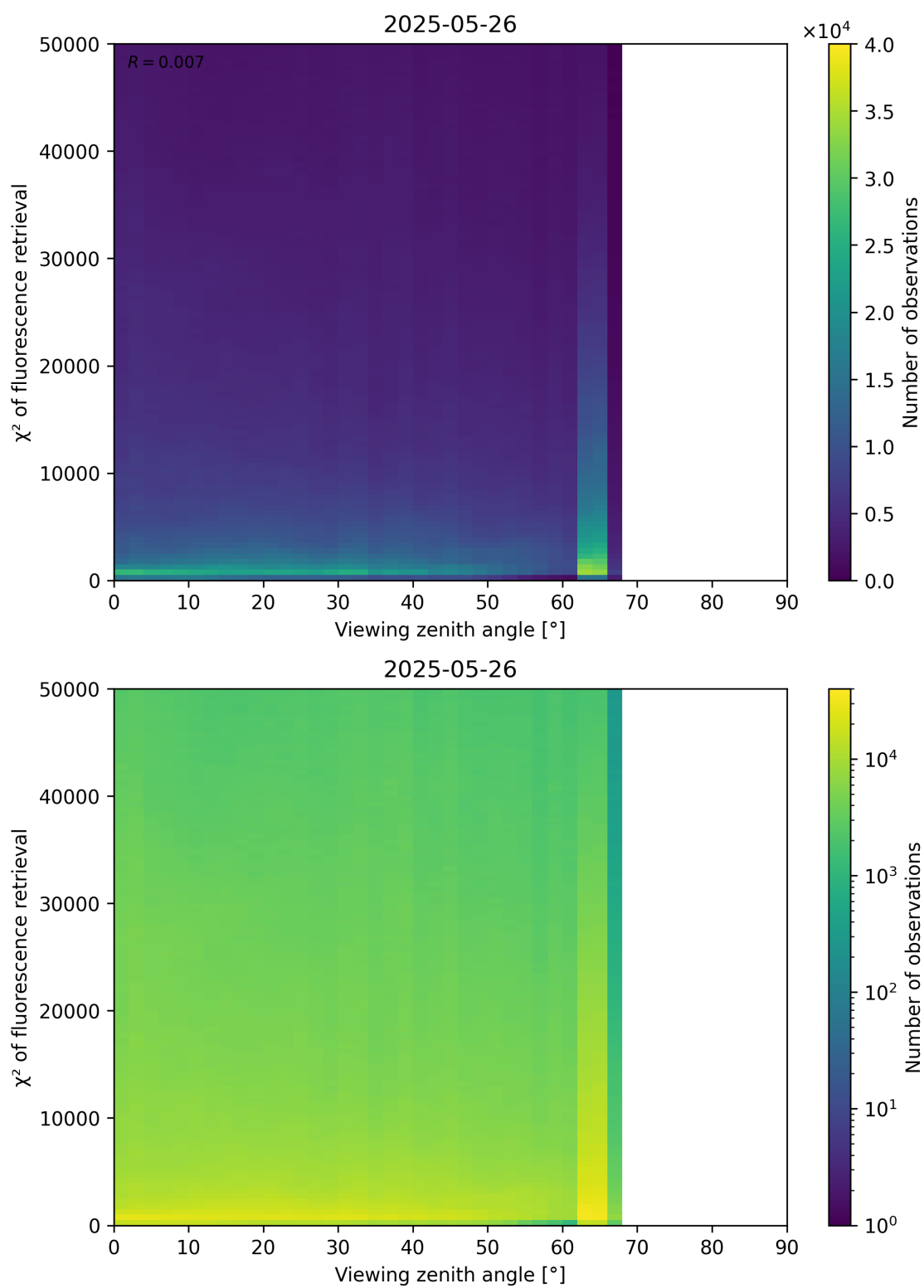
Figure 119: Scatter density plot of “Viewing zenith angle” against “ \chi^2 of fluorescence retrieval” for 2025-05-26 to 2025-05-27.
