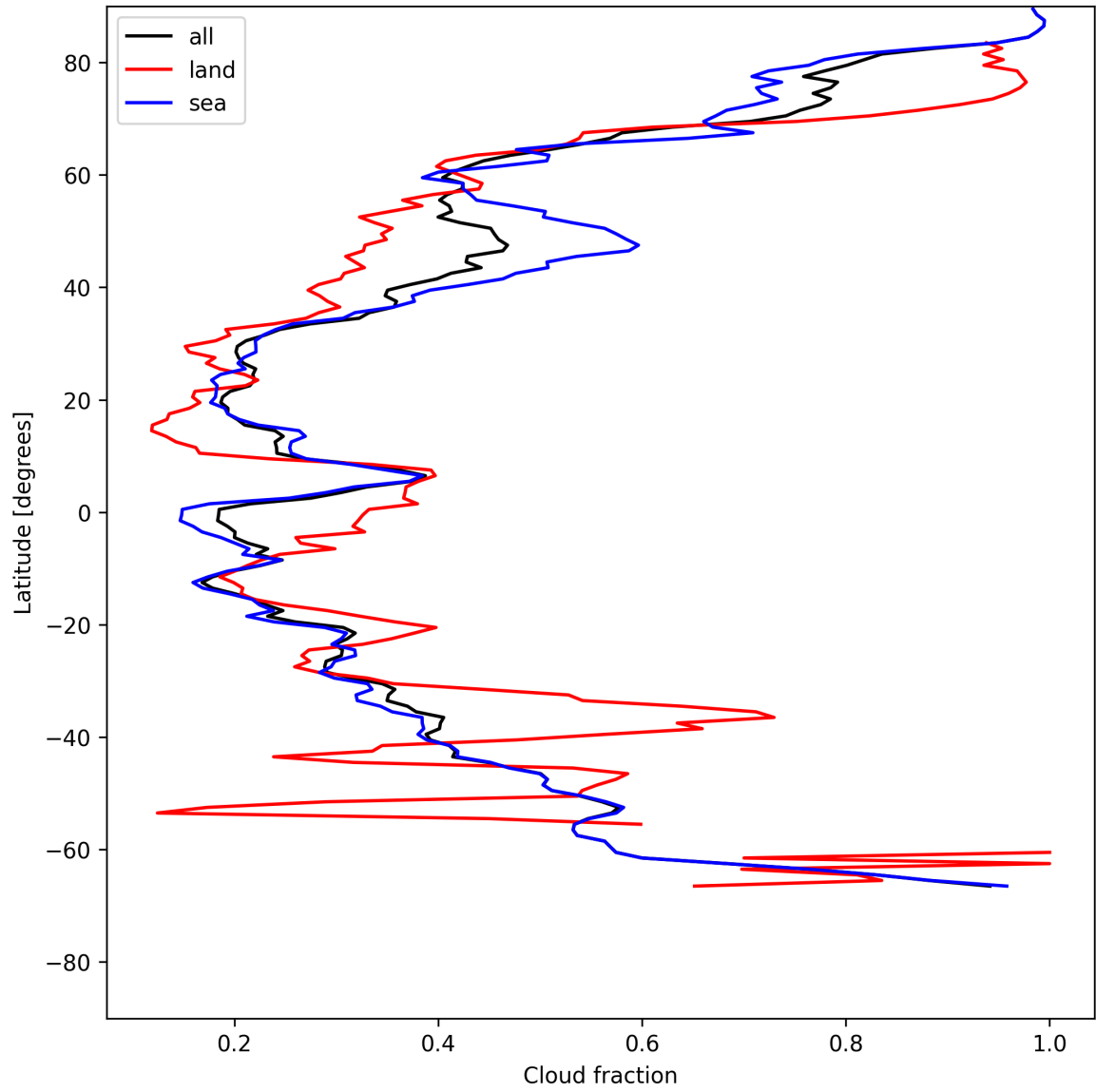
Figure 15: Zonal average of “Cloud fraction” for 2025-05-26 to 2025-05-27.
