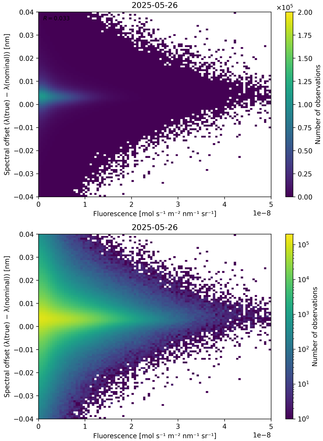
Figure 87: Scatter density plot of “Fluorescence” against “Spectral offset ( \lambda_{\text{true}} - \lambda_{\text{nominal}} )” for 2025-05-26 to 2025-05-27.
