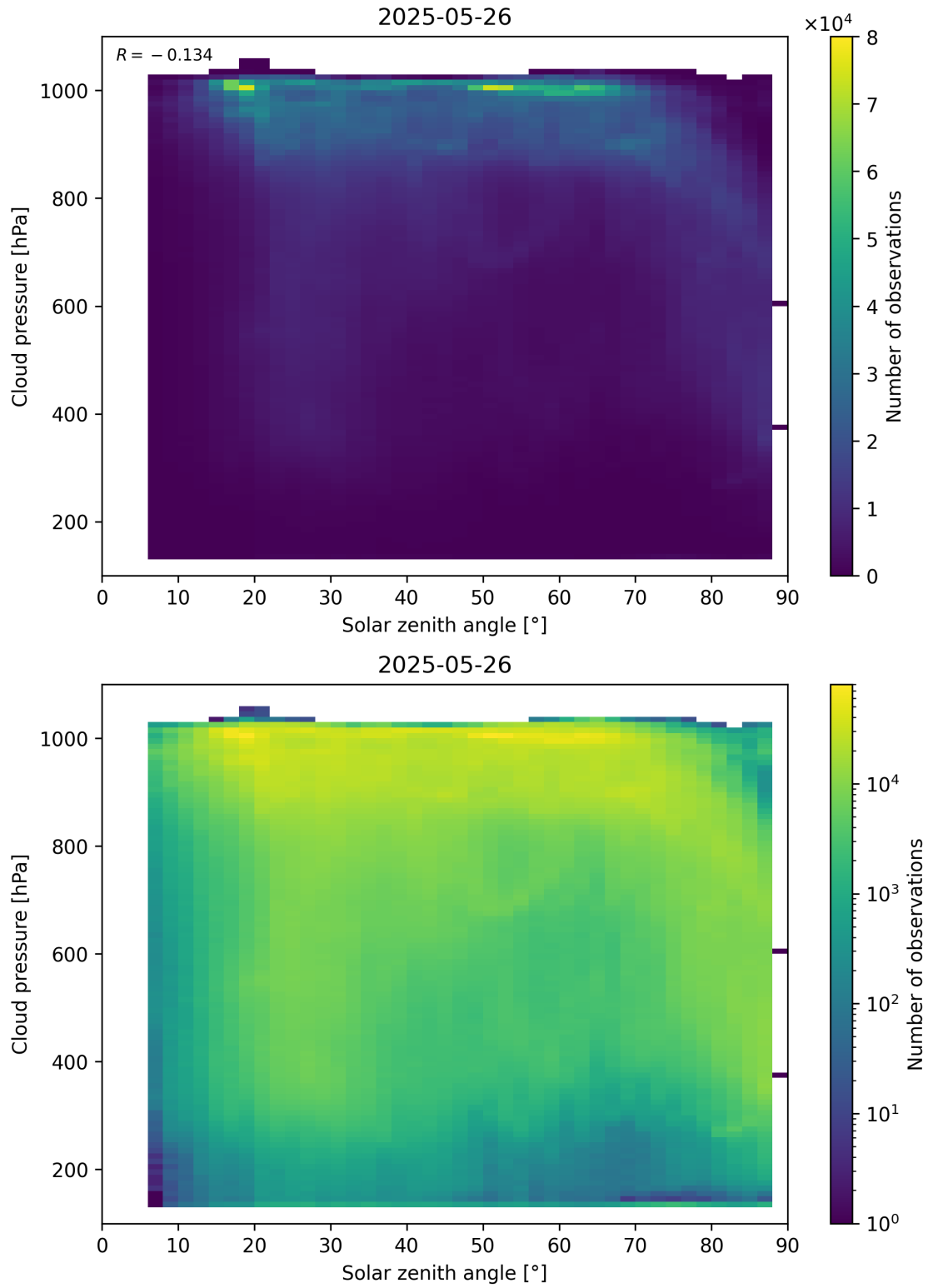
Figure 111: Scatter density plot of “Solar zenith angle” against “Cloud pressure” for 2025-05-26 to 2025-05-27.
