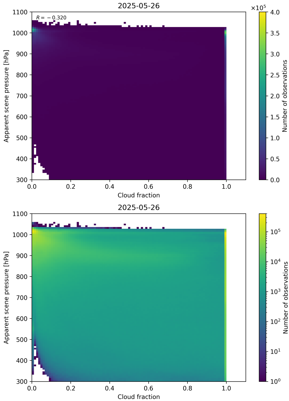
Figure 70: Scatter density plot of “Cloud fraction” against “Apparent scene pressure” for 2025-05-26 to 2025-05-27.
