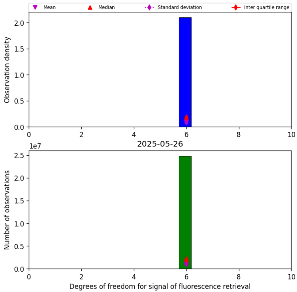
Figure 43: Histogram of “Degrees of freedom for signal of fluorescence retrieval” for 2025-05-26 to 2025-05-27
