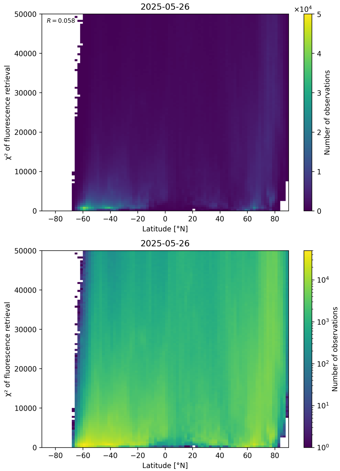
Figure 89: Scatter density plot of “Latitude” against “ \chi^2 of fluorescence retrieval” for 2025-05-26 to 2025-05-27.
