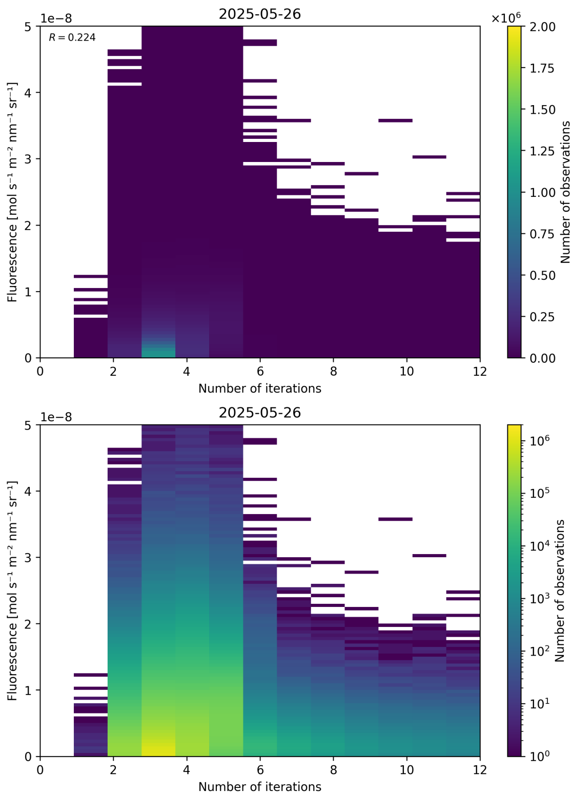
Figure 98: Scatter density plot of “Number of iterations” against “Fluorescence” for 2025-05-26 to 2025-05-27.
