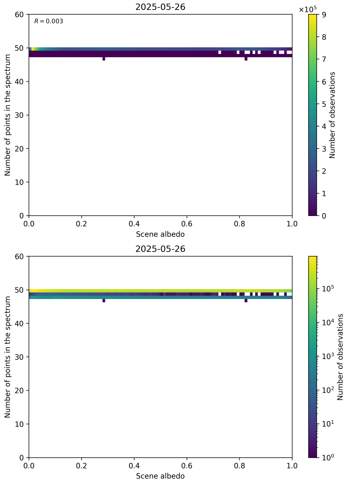
Figure 106: Scatter density plot of “Scene albedo” against “Number of points in the spectrum” for 2025-05-26 to 2025-05-27.
