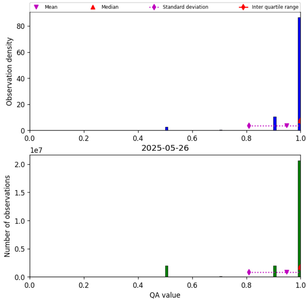
Figure 29: Histogram of “QA value” for 2025-05-26 to 2025-05-27
