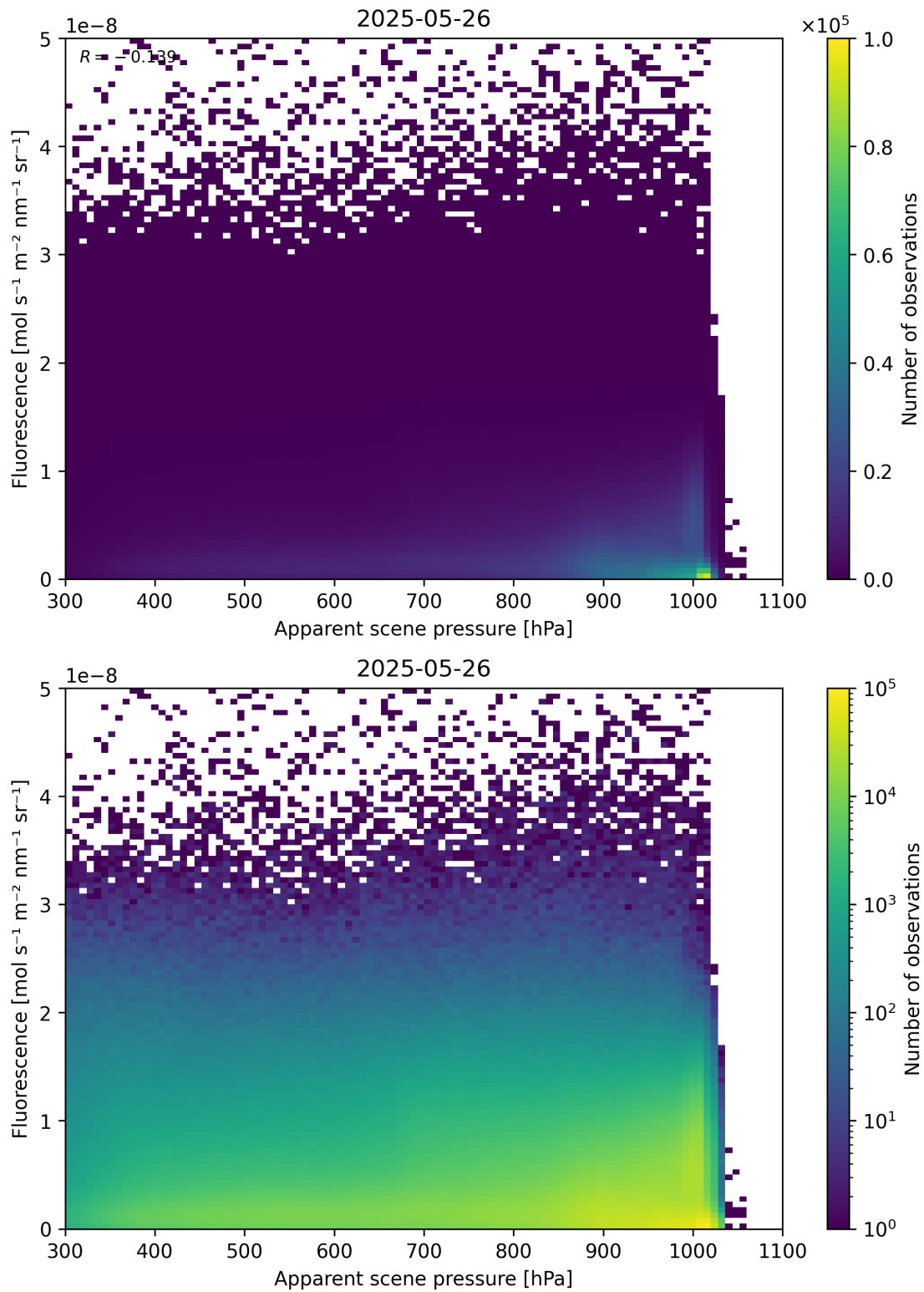
Figure 64: Scatter density plot of “Apparent scene pressure” against “Fluorescence” for 2025-05-26 to 2025-05-27.
