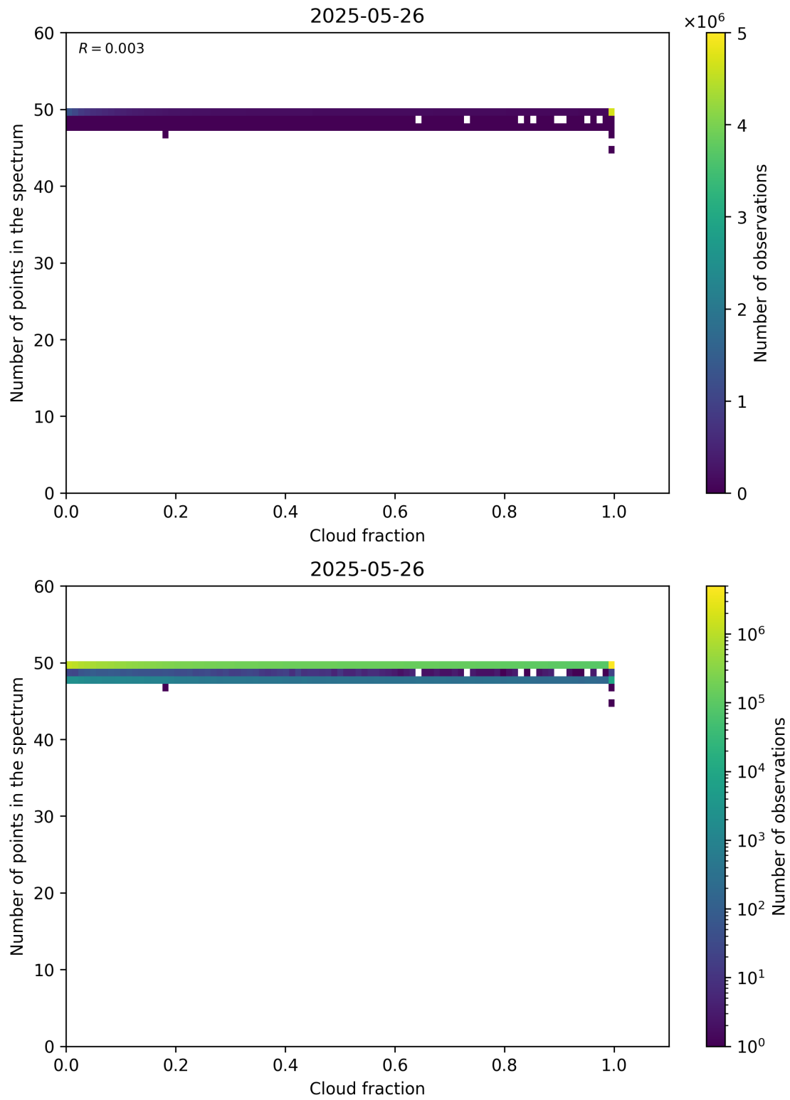
Figure 74: Scatter density plot of “Cloud fraction” against “Number of points in the spectrum” for 2025-05-26 to 2025-05-27.
