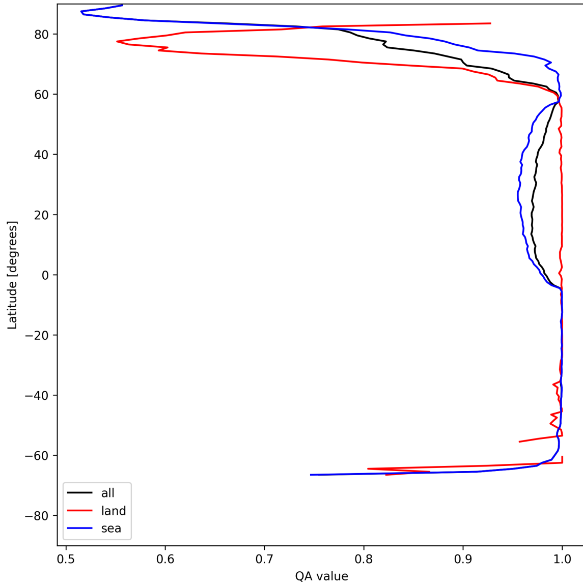
Figure 12: Zonal average of “QA value” for 2025-05-26 to 2025-05-27.
