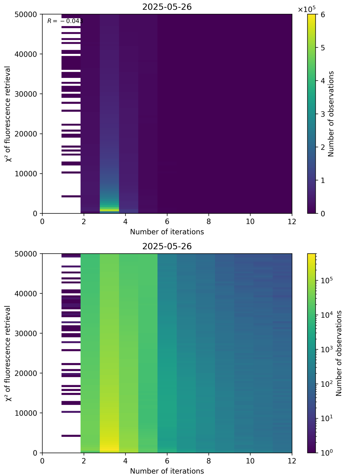
Figure 97: Scatter density plot of “Number of iterations” against “ \chi^2 of fluorescence retrieval” for 2025-05-26 to 2025-05-27.
