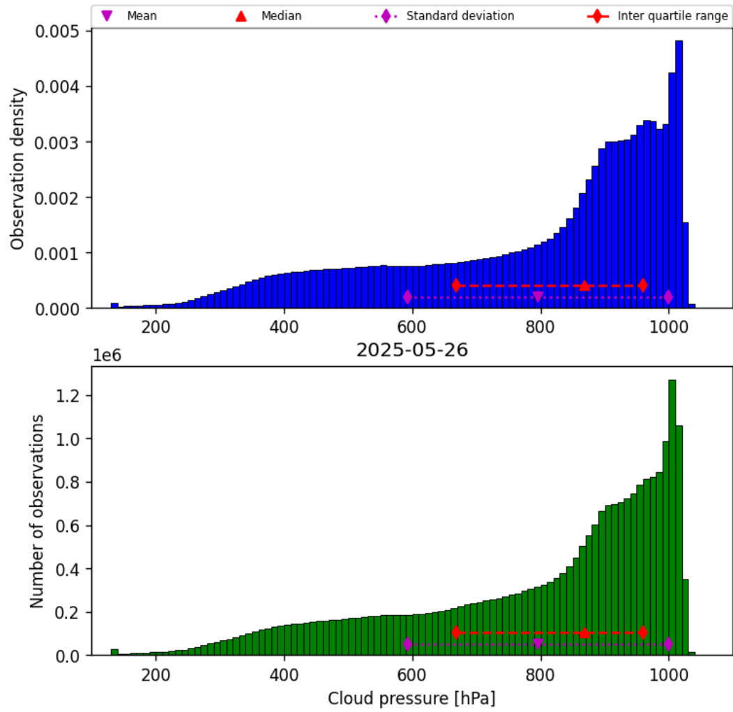
Figure 30: Histogram of “Cloud pressure” for 2025-05-26 to 2025-05-27
