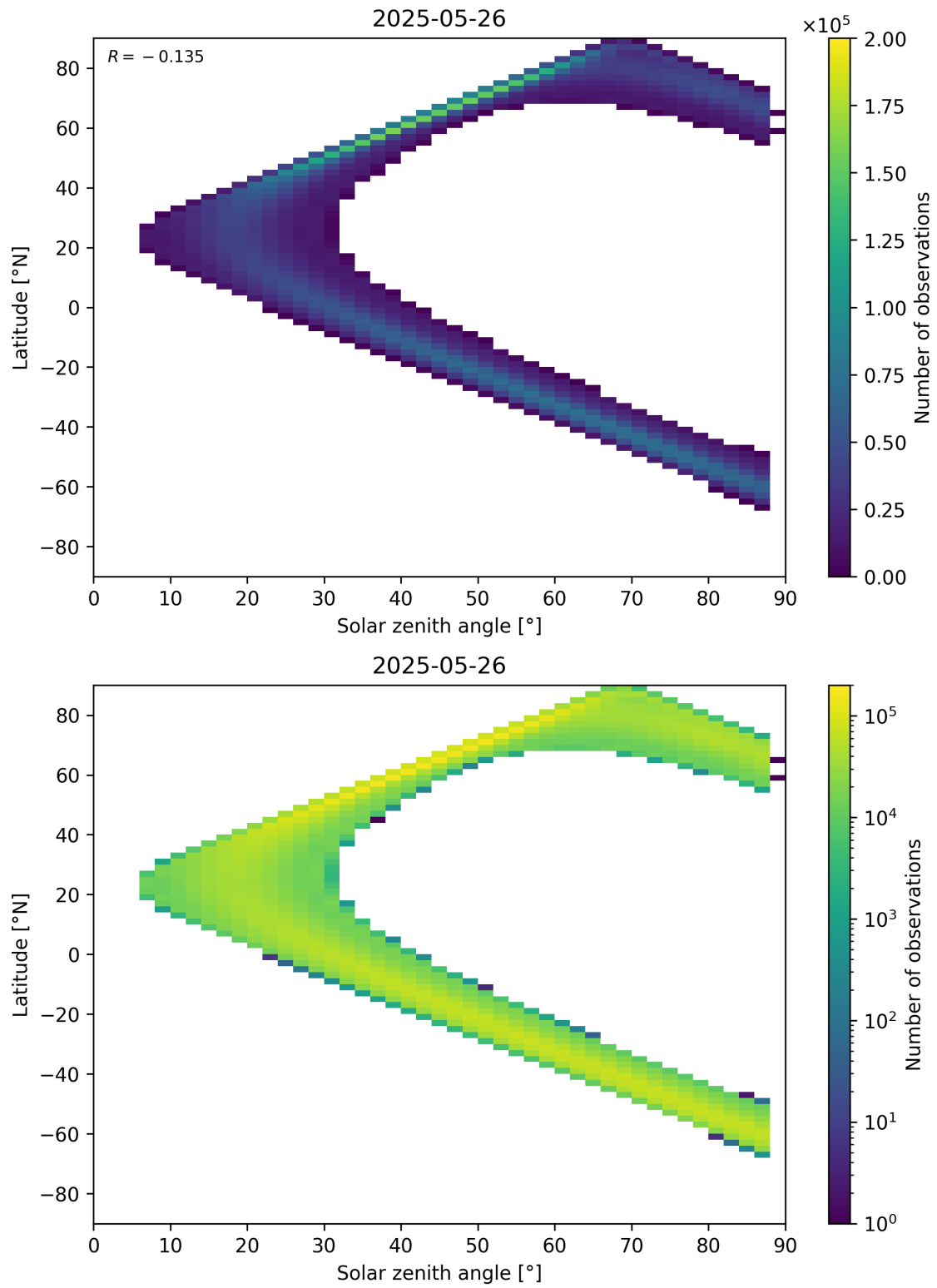
Figure 113: Scatter density plot of “Solar zenith angle” against “Latitude” for 2025-05-26 to 2025-05-27.
