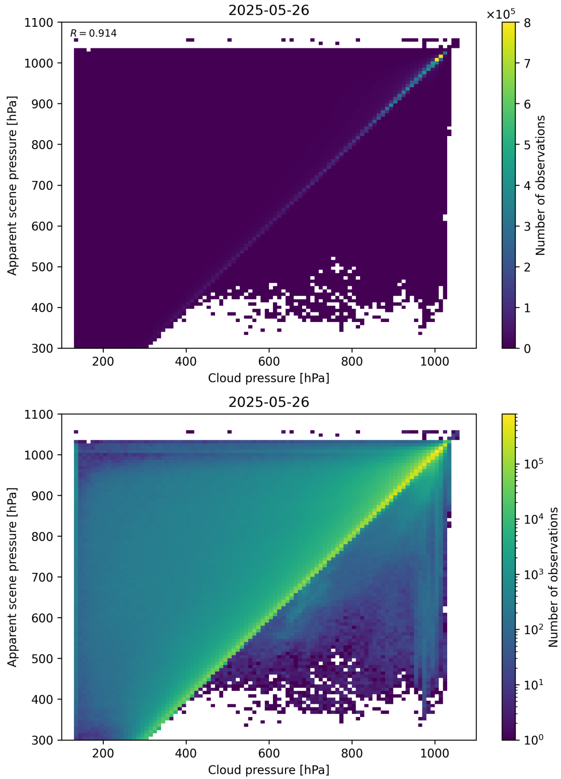
Figure 77: Scatter density plot of “Cloud pressure” against “Apparent scene pressure” for 2025-05-26 to 2025-05-27.
