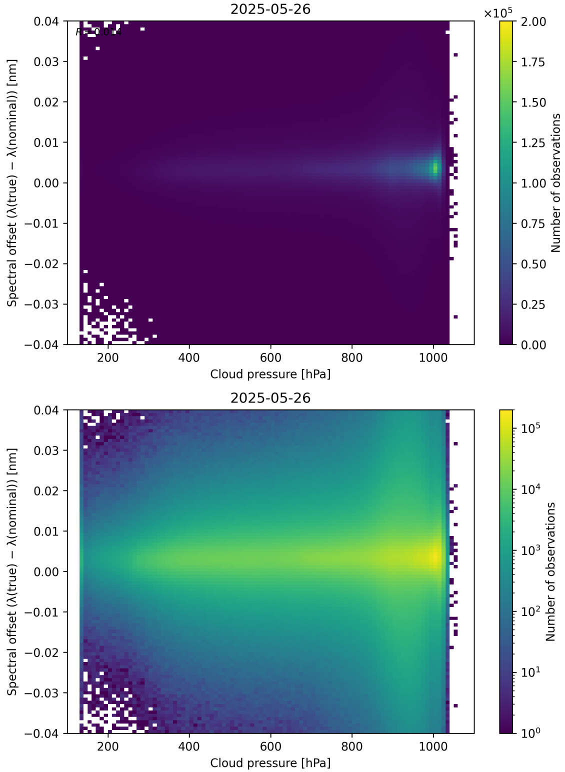
Figure 84: Scatter density plot of “Cloud pressure” against “Spectral offset ( \lambda_{\text{true}} - \lambda_{\text{nominal}} )” for 2025-05-26 to 2025-05-27.
