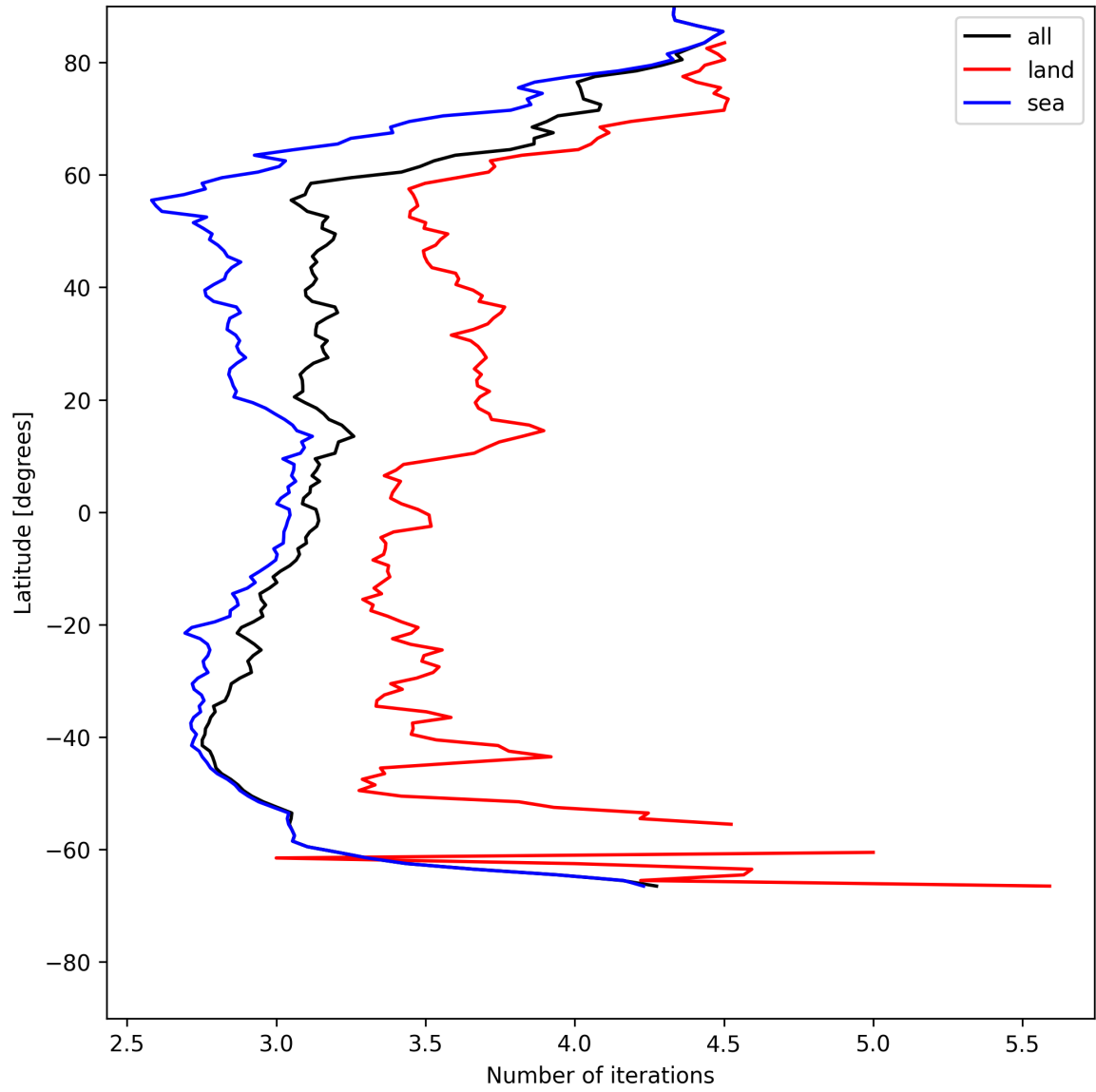
Figure 22: Zonal average of “Number of iterations” for 2025-05-26 to 2025-05-27.
