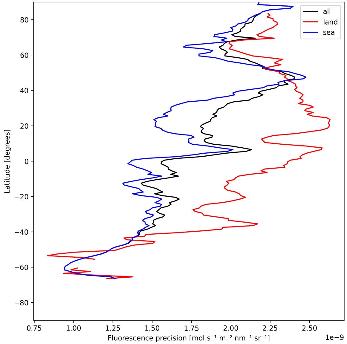
Figure 24: Zonal average of “Fluorescence precision” for 2025-05-26 to 2025-05-27.
