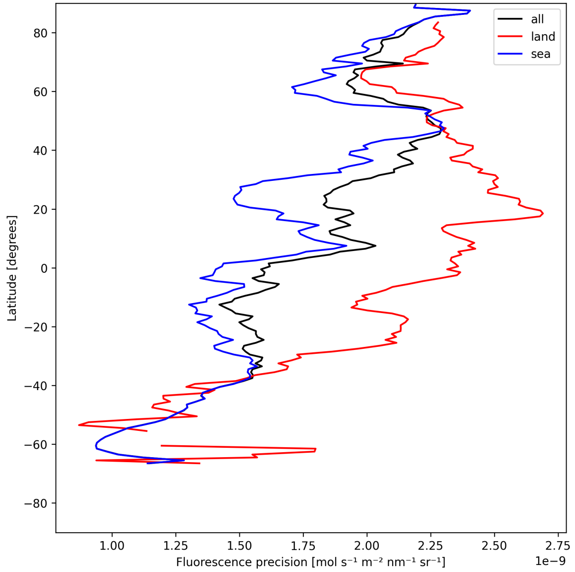
Figure 24: Zonal average of “Fluorescence precision” for 2025-05-26 to 2025-05-28.
