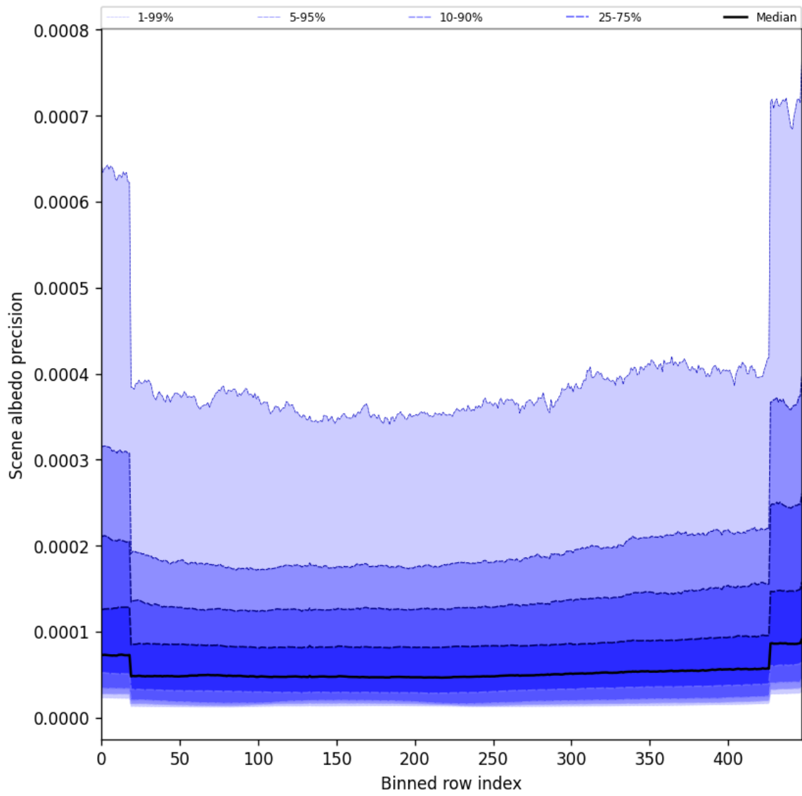
Figure 52: Along track statistics of “Scene albedo precision” for 2025-05-26 to 2025-05-28
