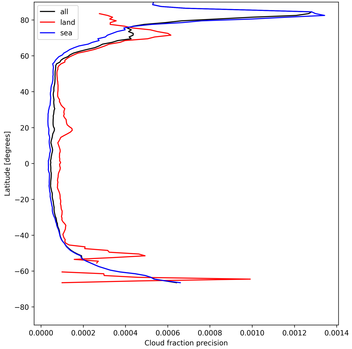
Figure 16: Zonal average of “Cloud fraction precision” for 2025-05-26 to 2025-05-28.
