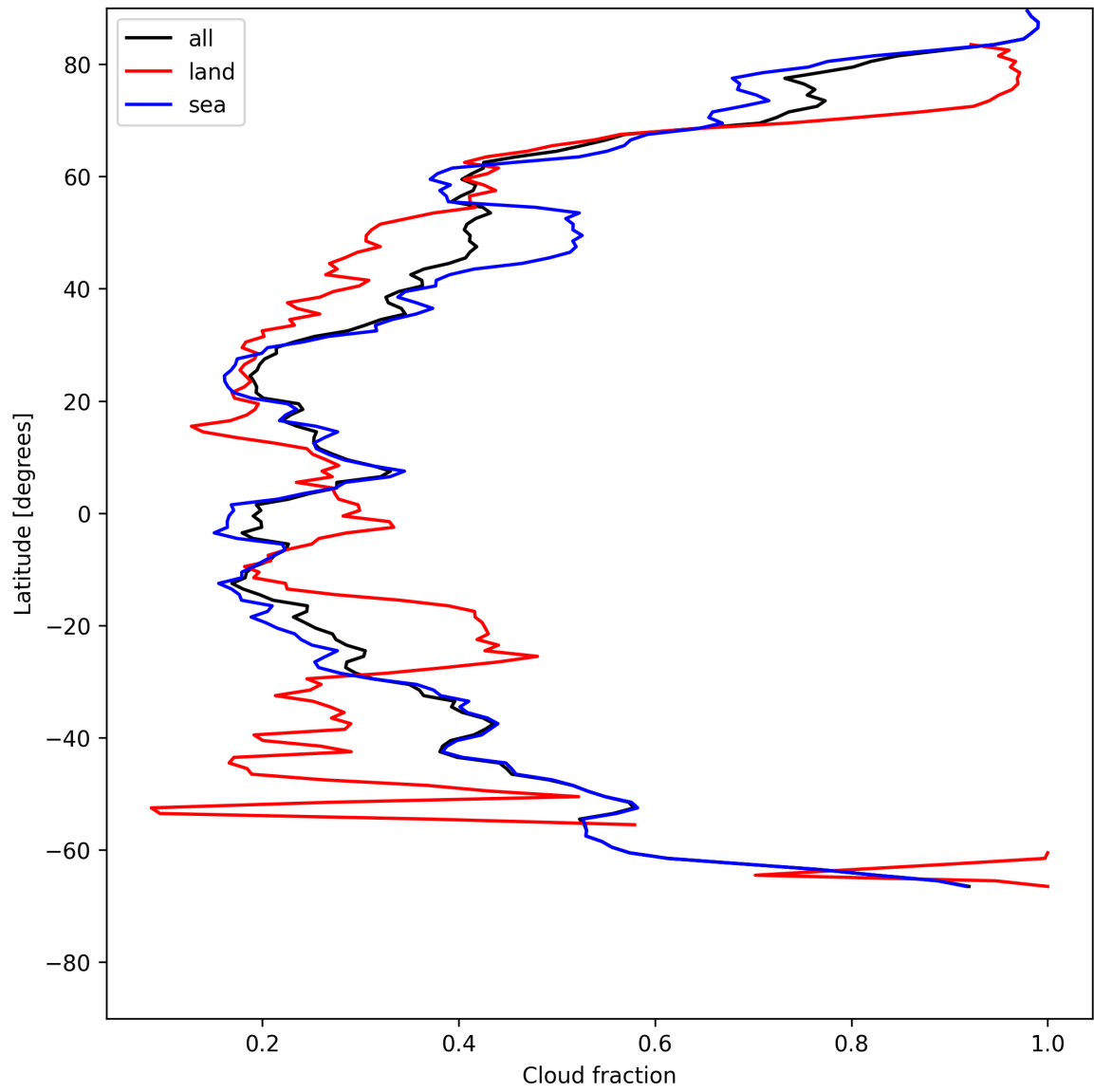
Figure 15: Zonal average of “Cloud fraction” for 2025-05-26 to 2025-05-28.
