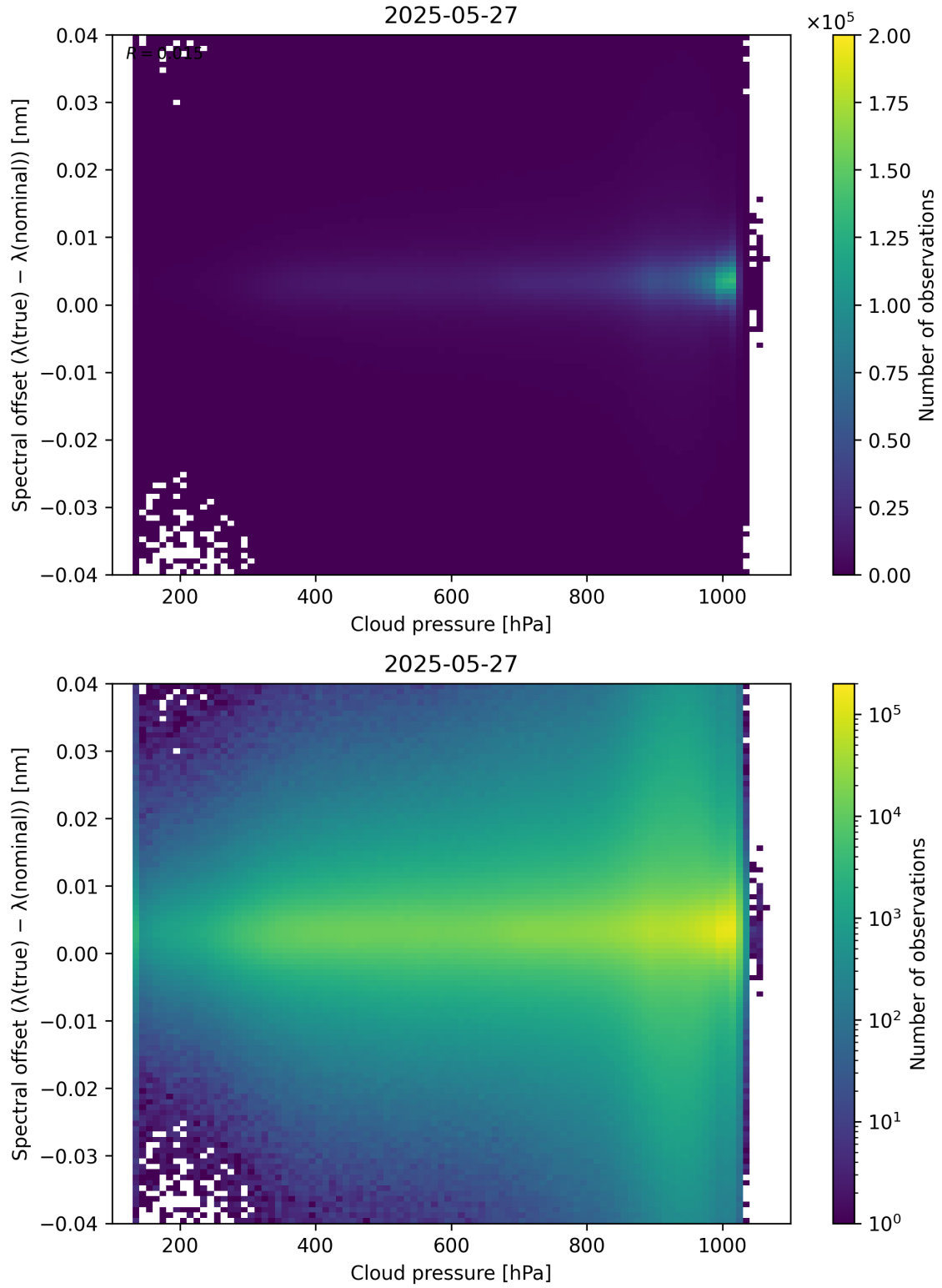
Figure 84: Scatter density plot of “Cloud pressure” against “Spectral offset ( \lambda_{\text{true}} - \lambda_{\text{nominal}} )” for 2025-05-26 to 2025-05-28.
