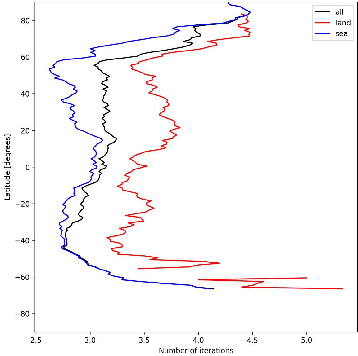
Figure 22: Zonal average of “Number of iterations” for 2025-05-26 to 2025-05-28.
