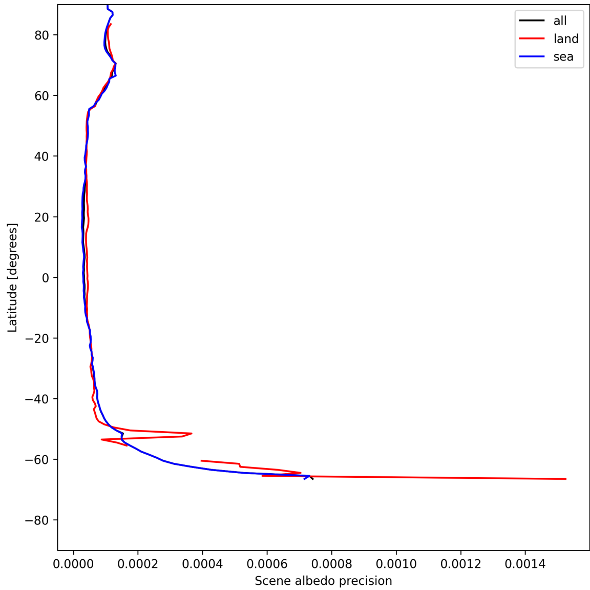
Figure 18: Zonal average of “Scene albedo precision” for 2025-05-26 to 2025-05-28.
