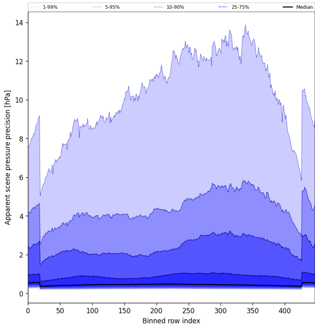
Figure 54: Along track statistics of “Apparent scene pressure precision” for 2025-05-26 to 2025-05-28
