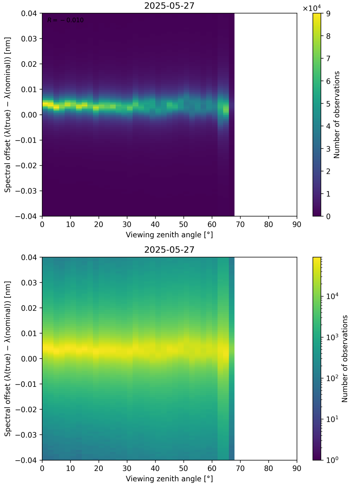
Figure 128: Scatter density plot of “Viewing zenith angle” against “Spectral offset ( \lambda_{\text{true}} - \lambda_{\text{nominal}} )” for 2025-05-26 to 2025-05-28.
