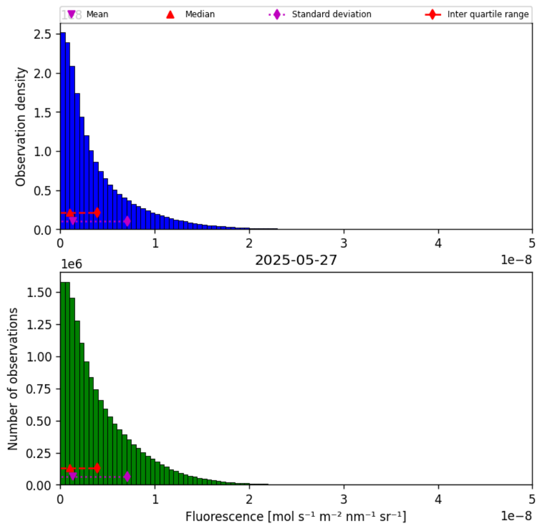
Figure 40: Histogram of “Fluorescence” for 2025-05-26 to 2025-05-28
