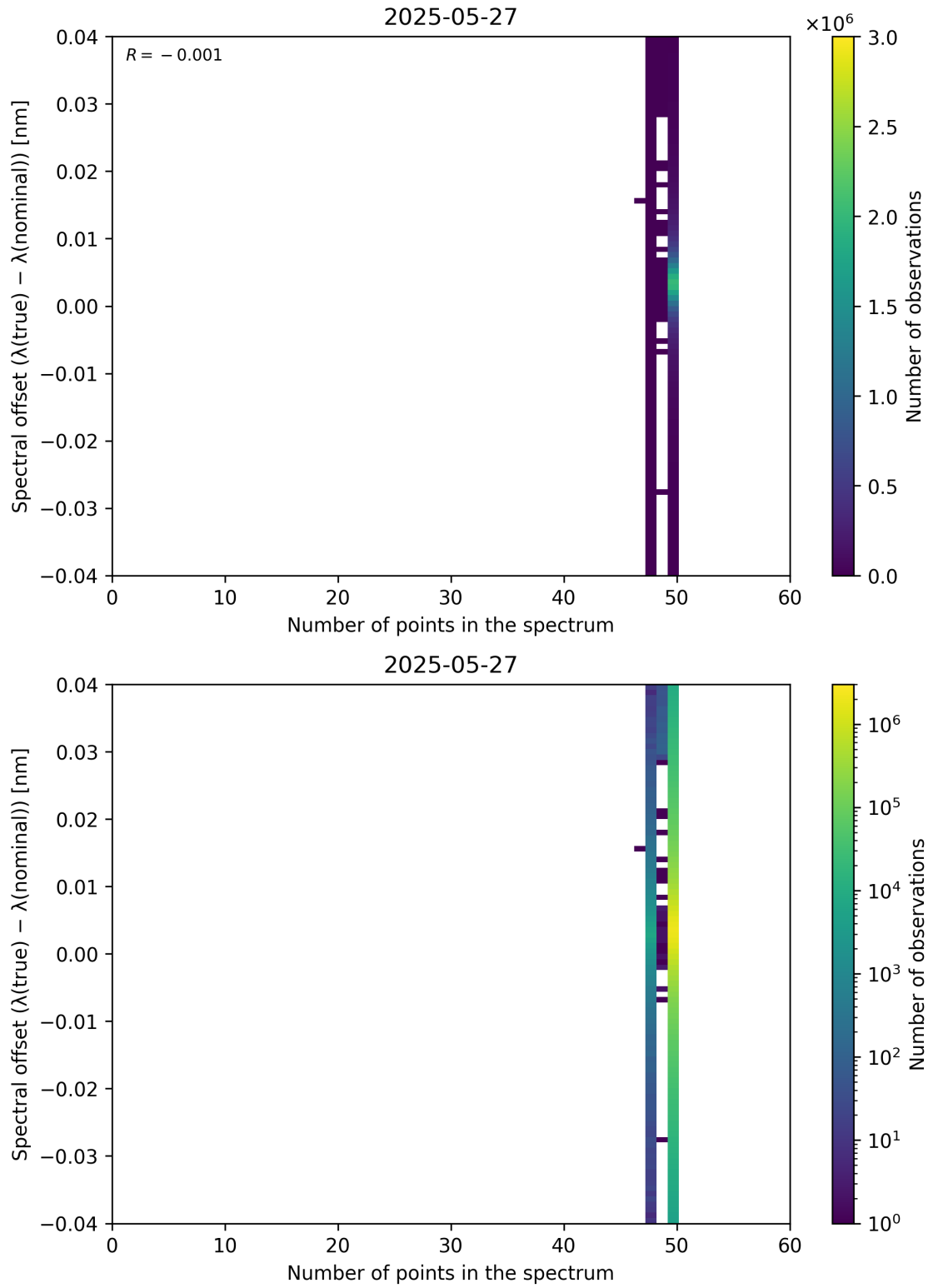
Figure 101: Scatter density plot of “Number of points in the spectrum” against “Spectral offset ( \lambda_{\text{true}} - \lambda_{\text{nominal}} )” for 2025-05-26 to 2025-05-28.
