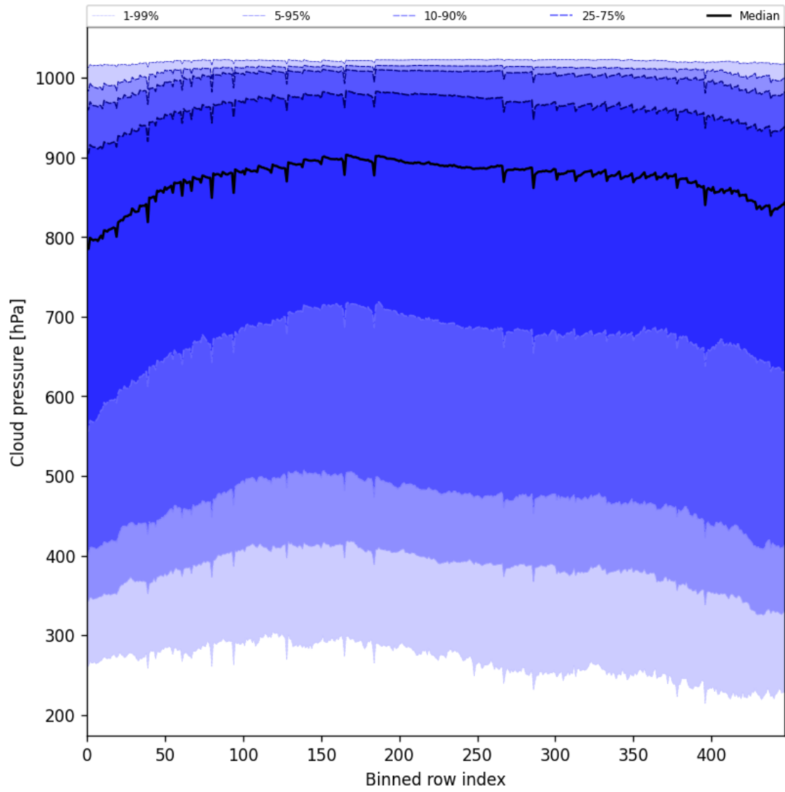
Figure 47: Along track statistics of “Cloud pressure” for 2025-05-26 to 2025-05-28
