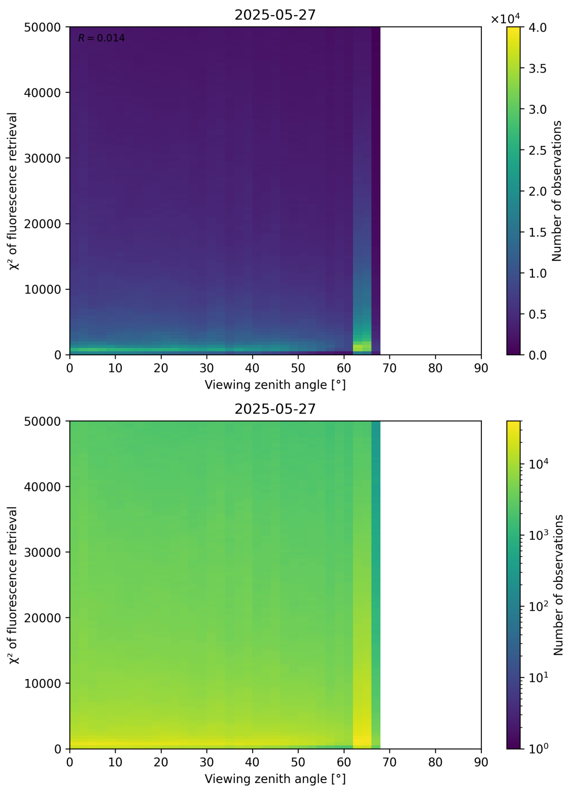
Figure 119: Scatter density plot of “Viewing zenith angle” against “ \chi^2 of fluorescence retrieval” for 2025-05-26 to 2025-05-28.
