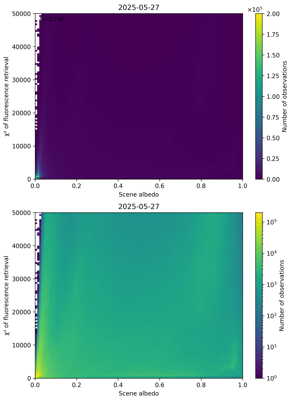
Figure 103: Scatter density plot of “Scene albedo” against “ \chi^2 of fluorescence retrieval” for 2025-05-26 to 2025-05-28.
