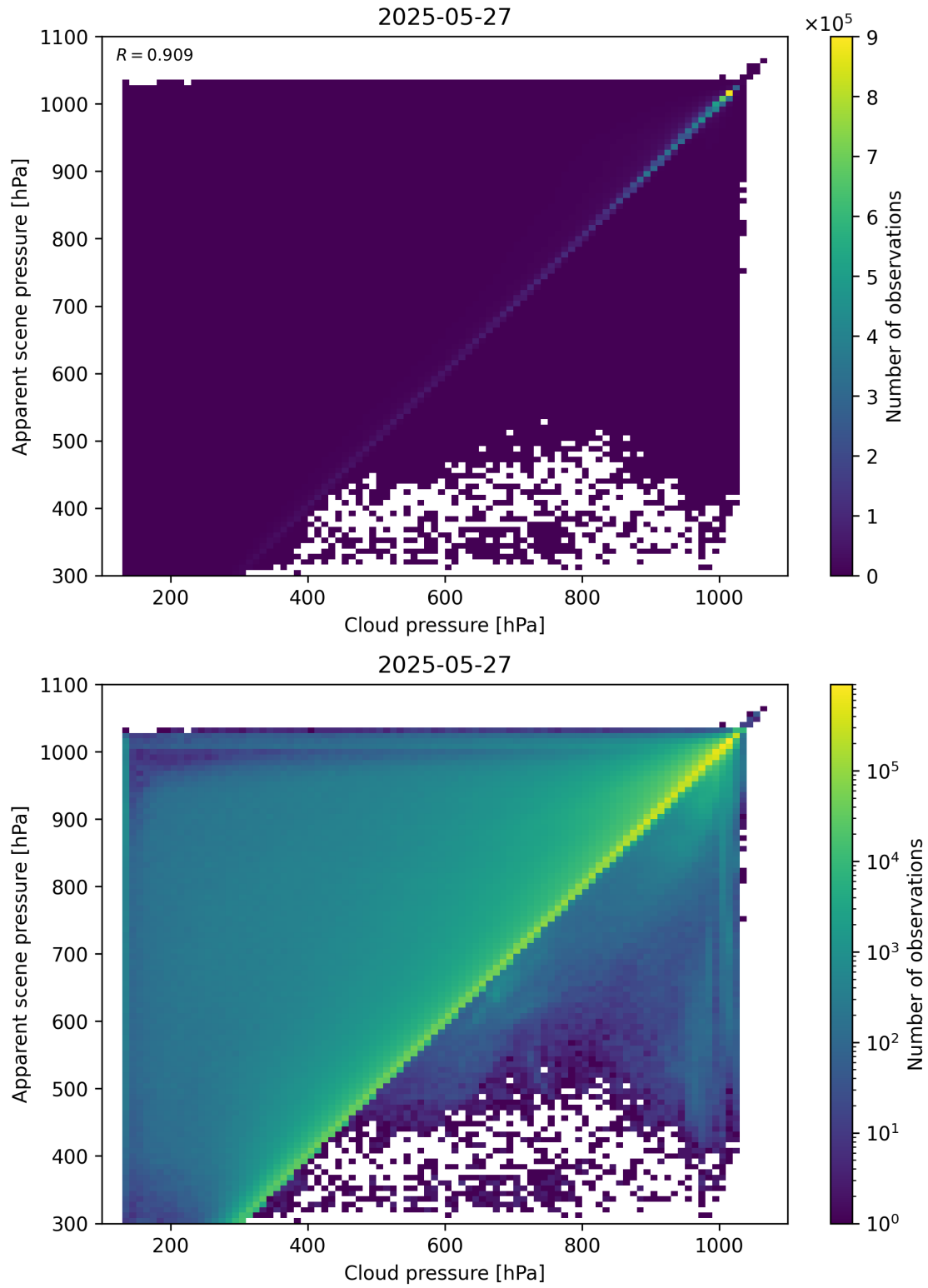
Figure 77: Scatter density plot of “Cloud pressure” against “Apparent scene pressure” for 2025-05-26 to 2025-05-28.
