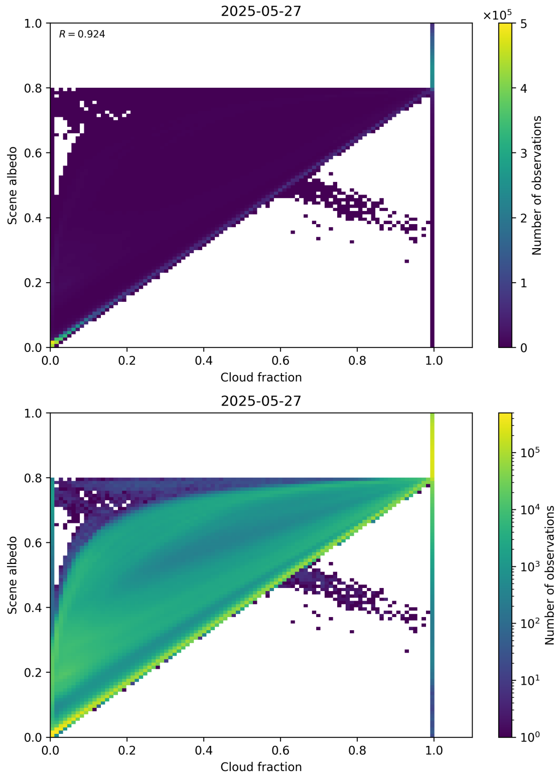
Figure 75: Scatter density plot of “Cloud fraction” against “Scene albedo” for 2025-05-26 to 2025-05-28.
