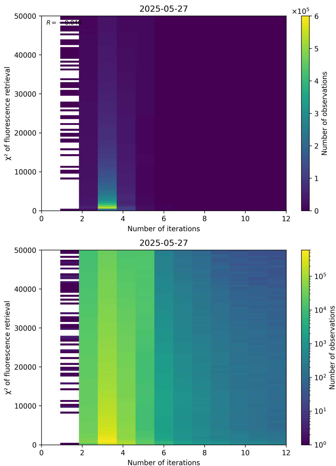
Figure 97: Scatter density plot of “Number of iterations” against “ \chi^2 of fluorescence retrieval” for 2025-05-26 to 2025-05-28.
