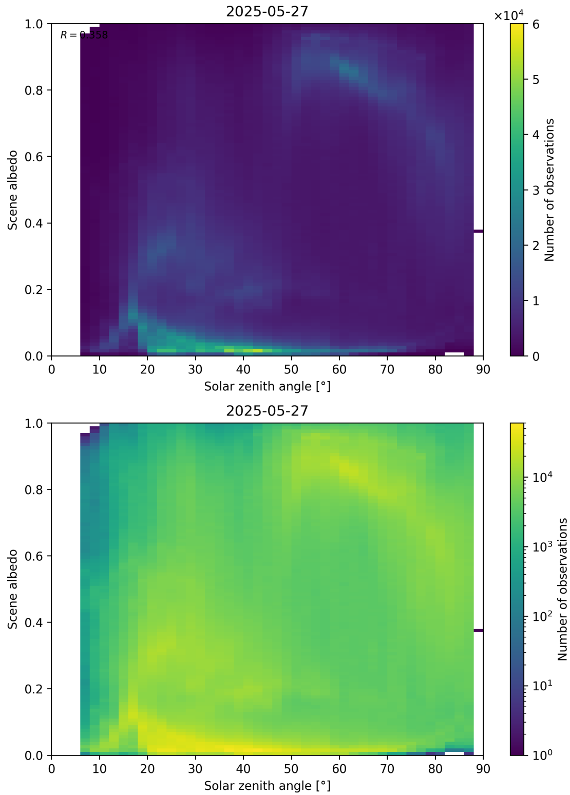
Figure 116: Scatter density plot of “Solar zenith angle” against “Scene albedo” for 2025-05-26 to 2025-05-28.
