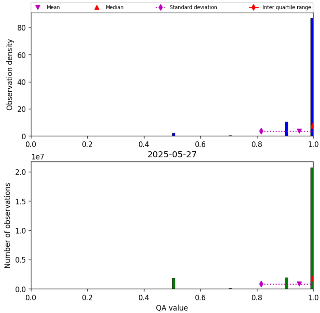
Figure 29: Histogram of “QA value” for 2025-05-26 to 2025-05-28
