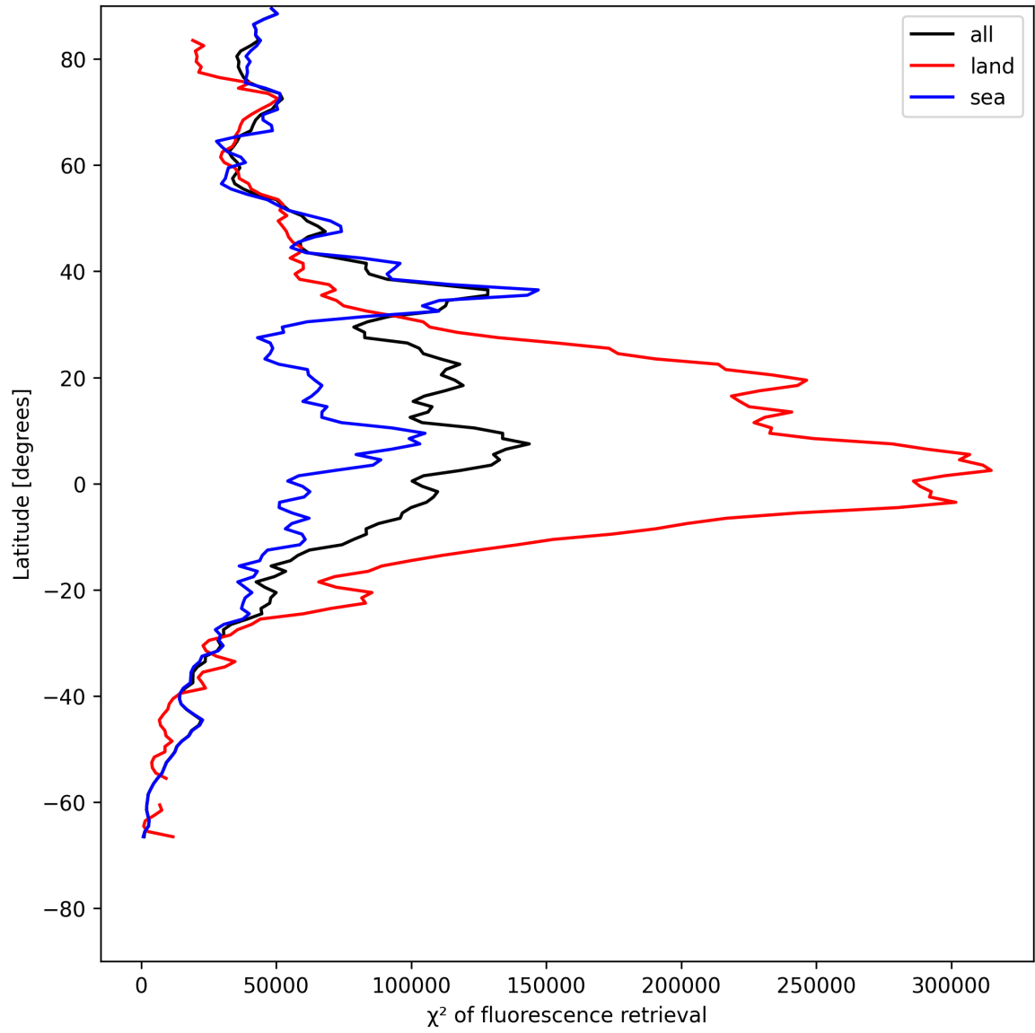
Figure 25: Zonal average of “ \chi^2 of fluorescence retrieval” for 2025-05-26 to 2025-05-28.
