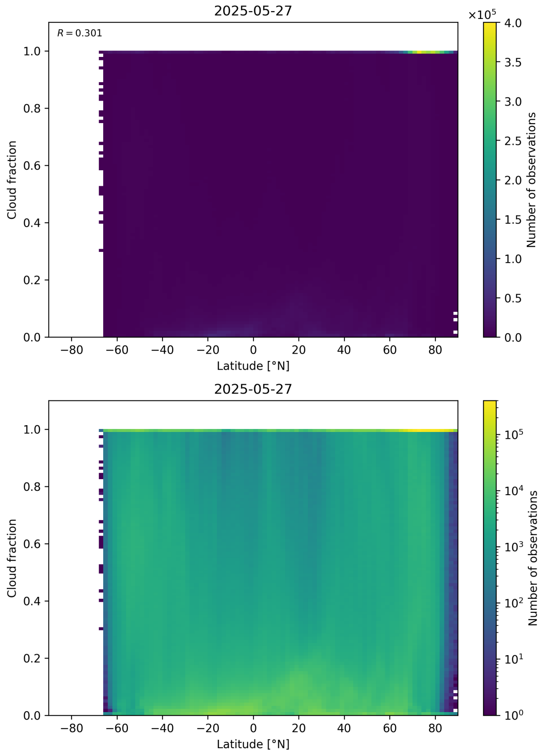
Figure 90: Scatter density plot of “Latitude” against “Cloud fraction” for 2025-05-26 to 2025-05-28.
