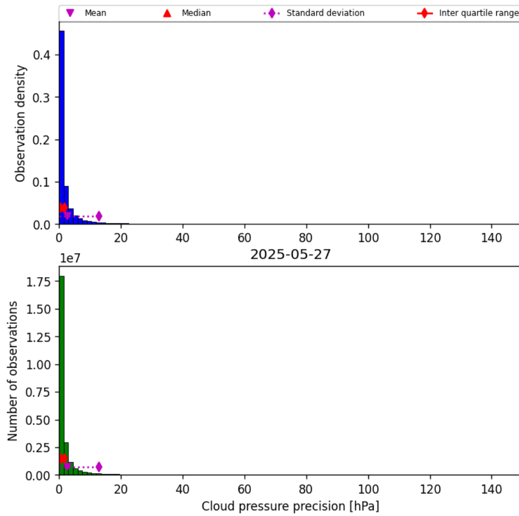
Figure 31: Histogram of “Cloud pressure precision” for 2025-05-26 to 2025-05-28
