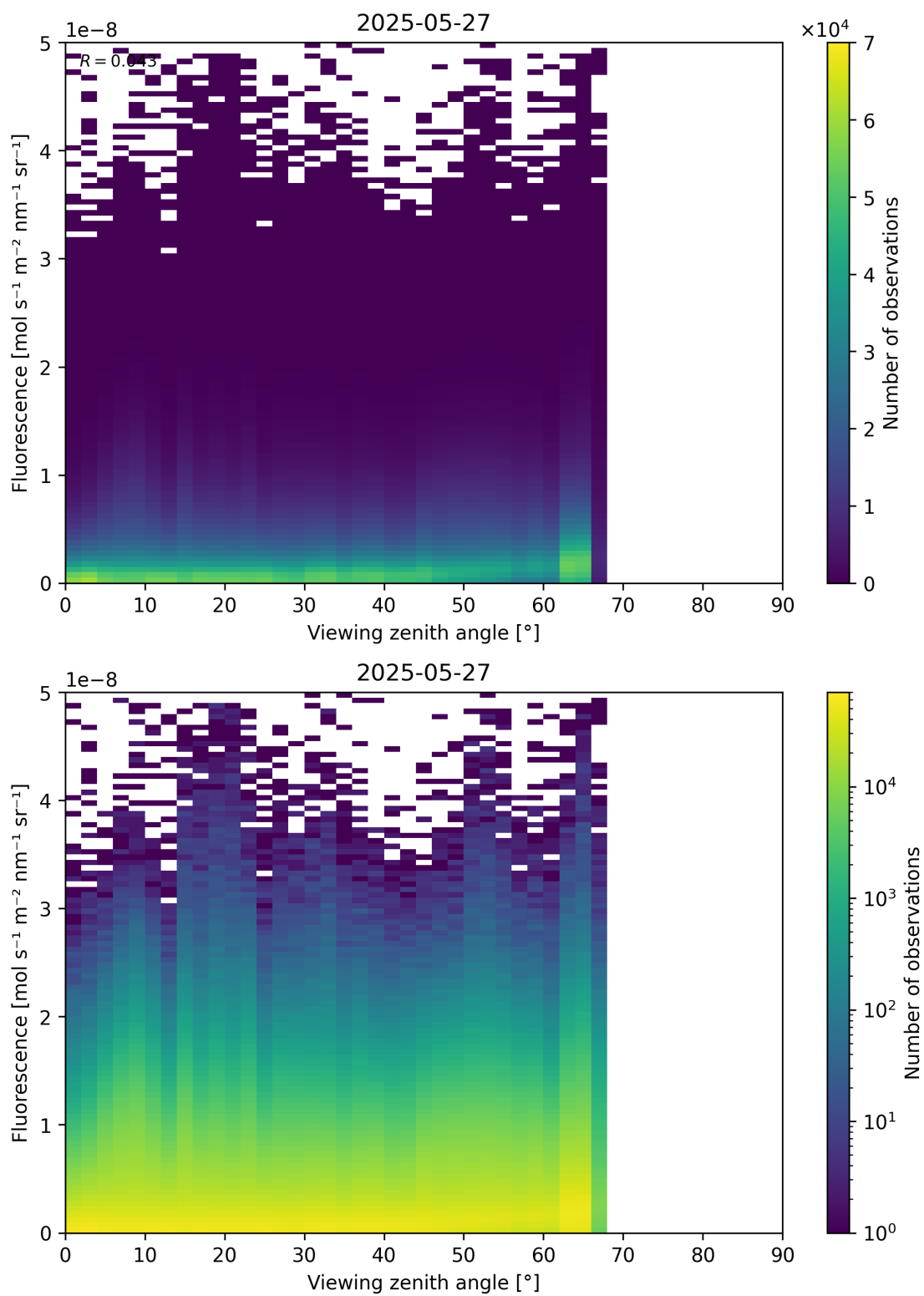
Figure 122: Scatter density plot of “Viewing zenith angle” against “Fluorescence” for 2025-05-26 to 2025-05-28.
