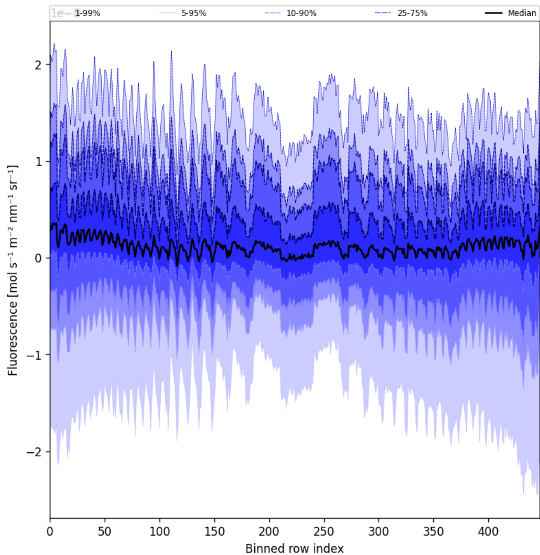
Figure 57: Along track statistics of “Fluorescence” for 2025-05-26 to 2025-05-28
