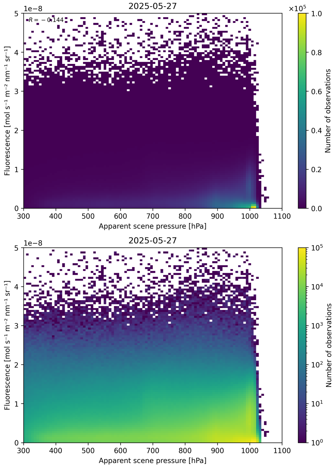
Figure 64: Scatter density plot of “Apparent scene pressure” against “Fluorescence” for 2025-05-26 to 2025-05-28.
