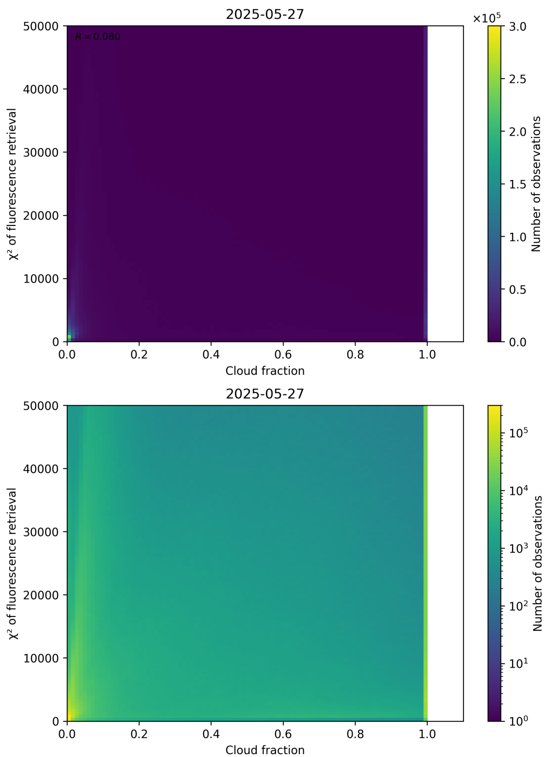
Figure 71: Scatter density plot of “Cloud fraction” against “ \chi^2 of fluorescence retrieval” for 2025-05-26 to 2025-05-28.
