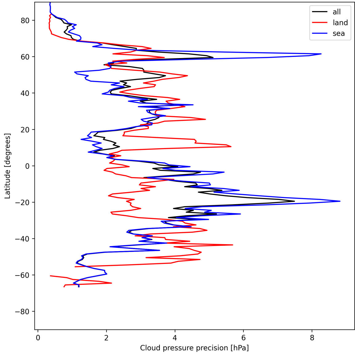
Figure 14: Zonal average of “Cloud pressure precision” for 2025-05-26 to 2025-05-28.
