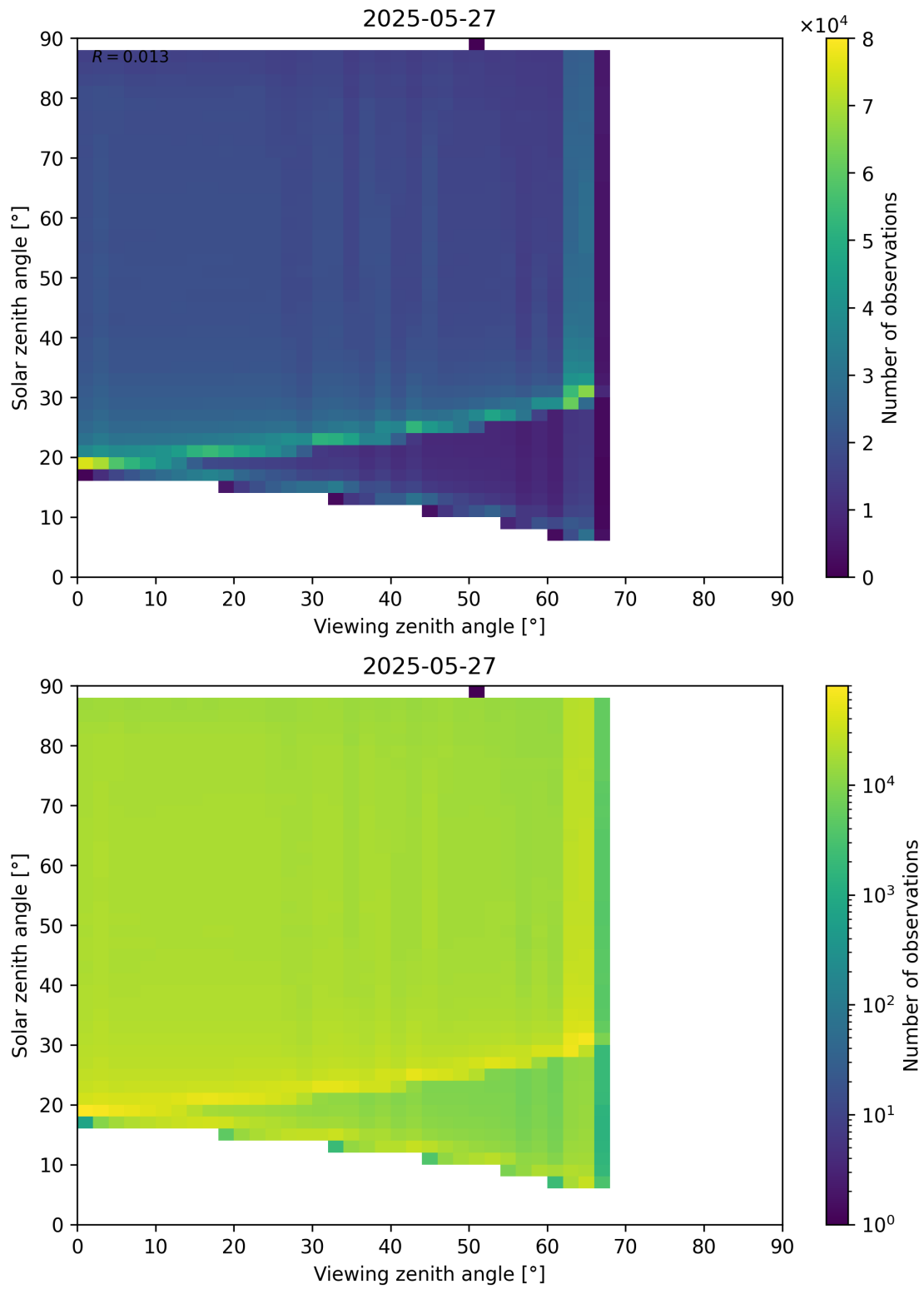
Figure 127: Scatter density plot of “Viewing zenith angle” against “Solar zenith angle” for 2025-05-26 to 2025-05-28.
