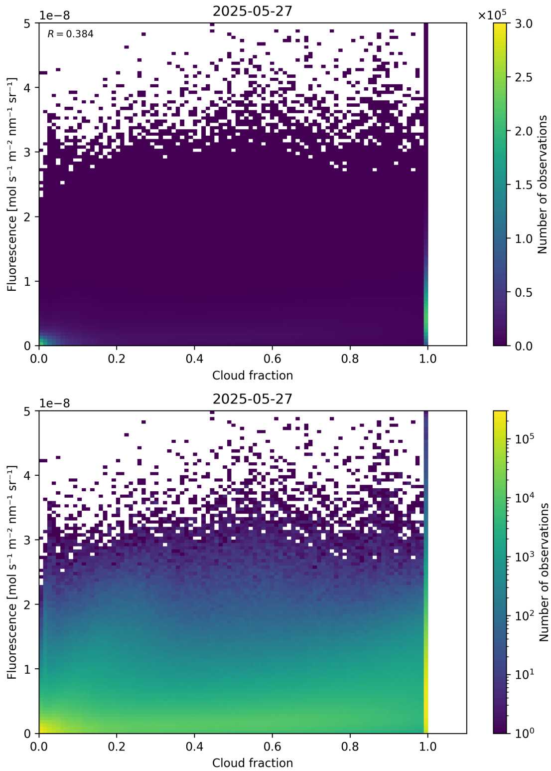
Figure 72: Scatter density plot of “Cloud fraction” against “Fluorescence” for 2025-05-26 to 2025-05-28.
