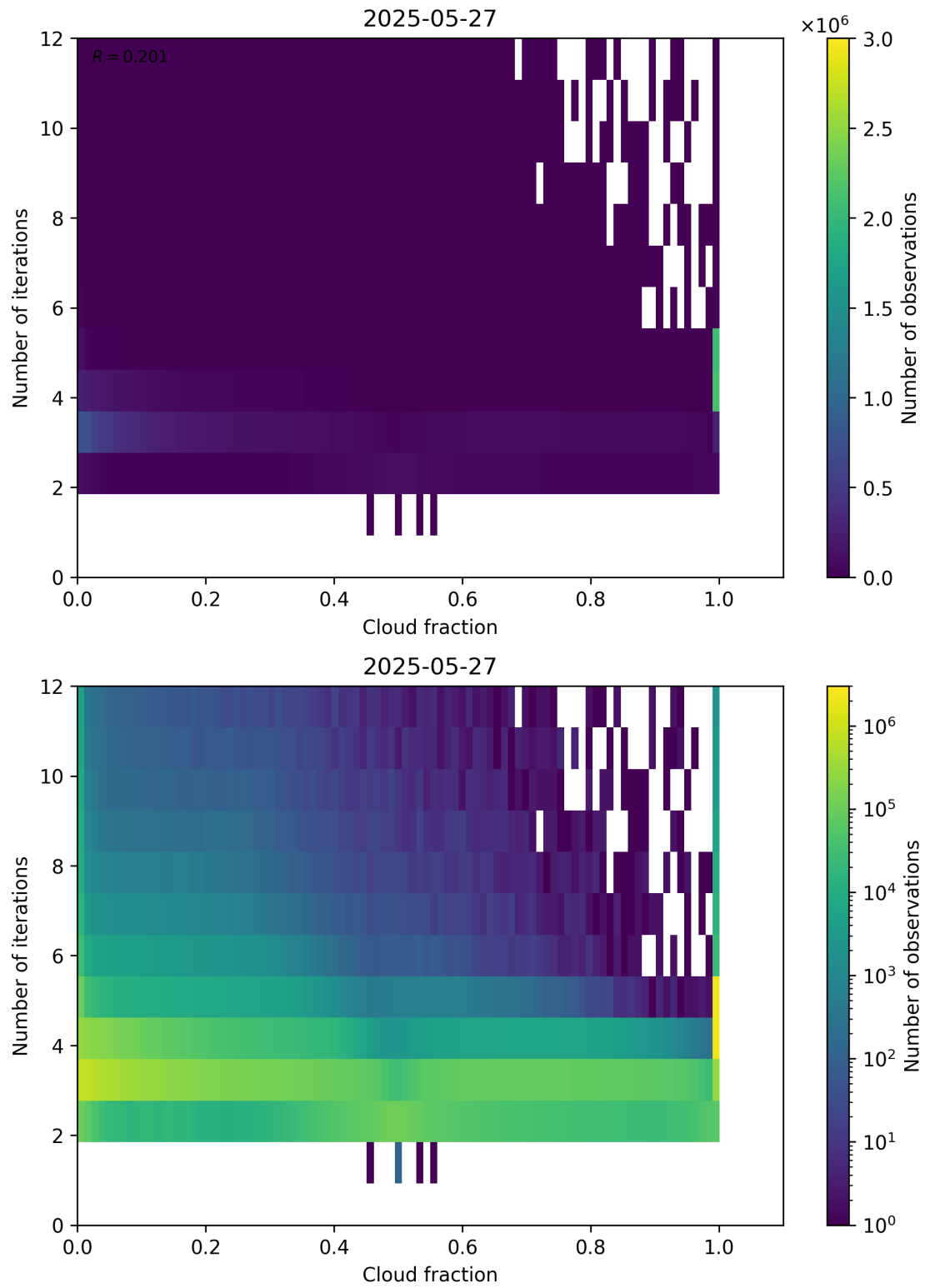
Figure 73: Scatter density plot of “Cloud fraction” against “Number of iterations” for 2025-05-26 to 2025-05-28.
