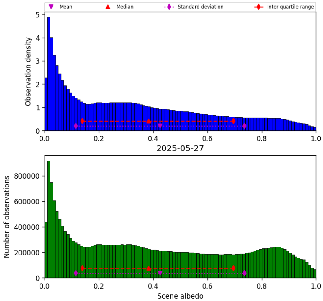
Figure 34: Histogram of “Scene albedo” for 2025-05-26 to 2025-05-28
