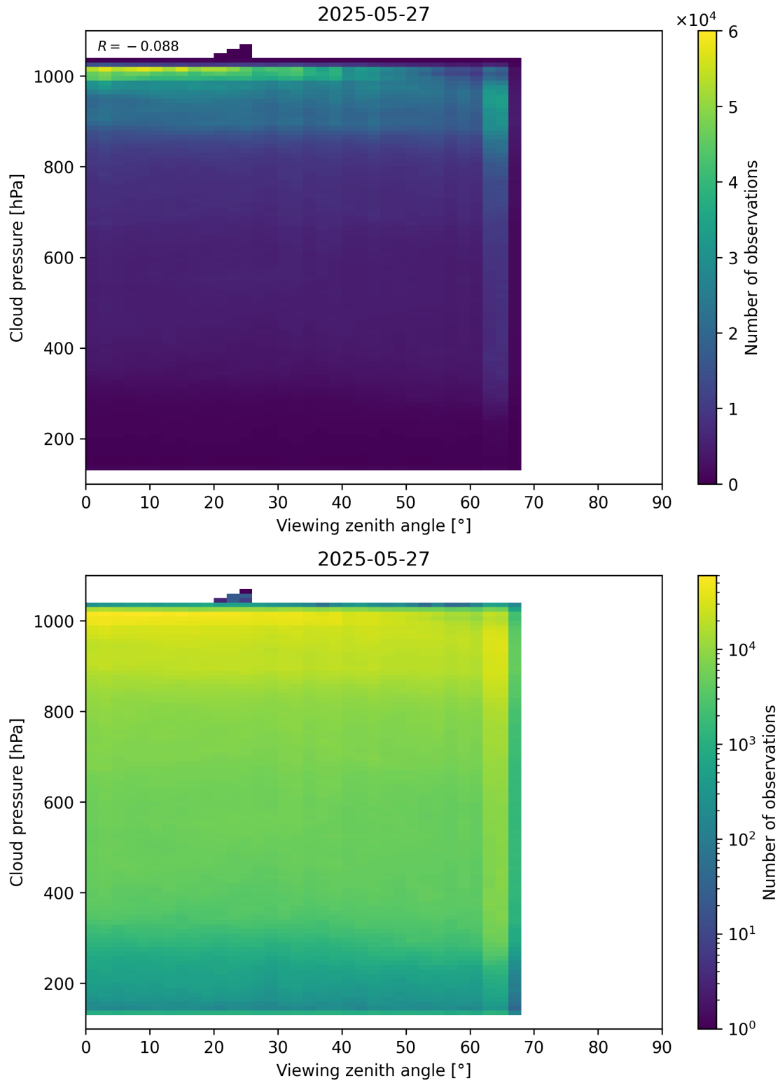
Figure 121: Scatter density plot of “Viewing zenith angle” against “Cloud pressure” for 2025-05-26 to 2025-05-28.
