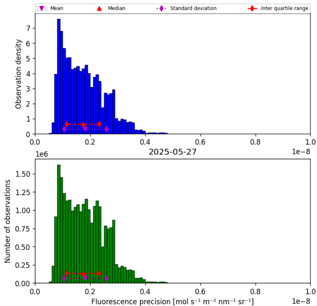
Figure 41: Histogram of “Fluorescence precision” for 2025-05-26 to 2025-05-28
