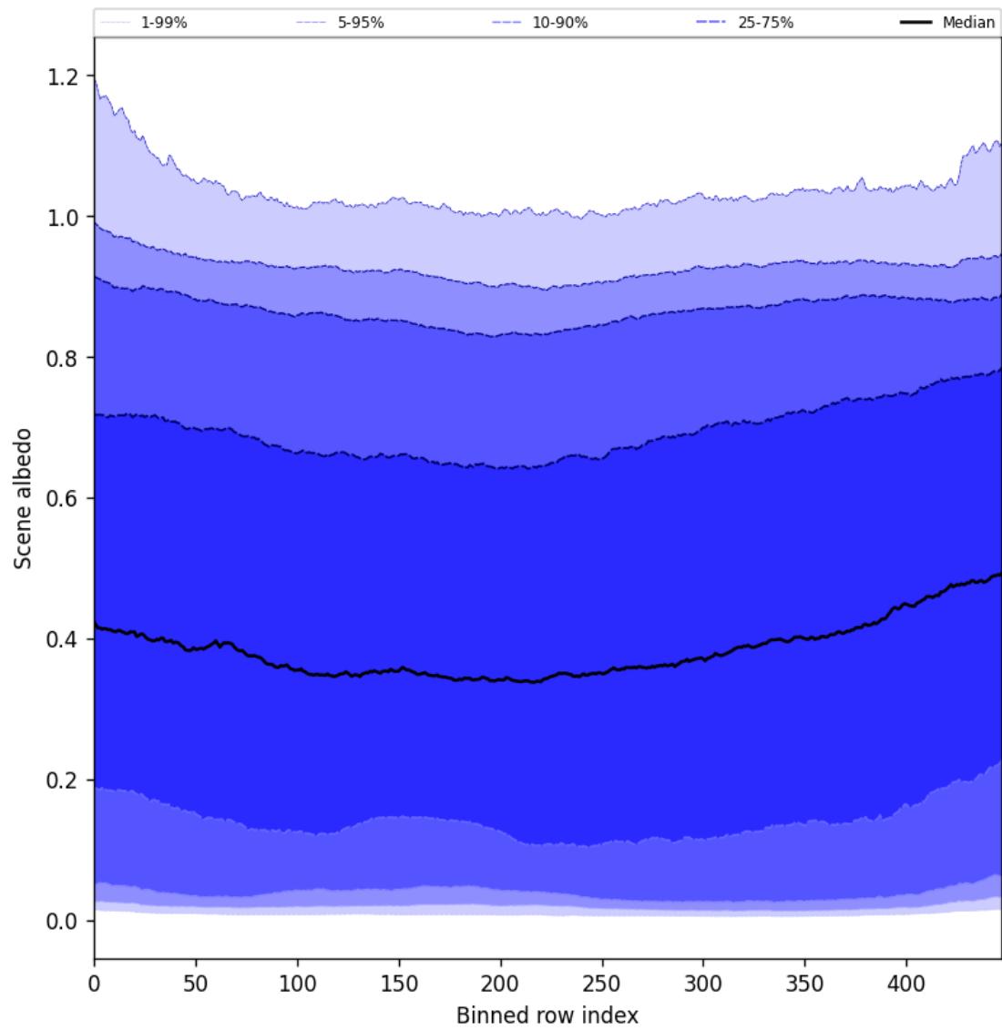
Figure 51: Along track statistics of “Scene albedo” for 2025-05-26 to 2025-05-28
