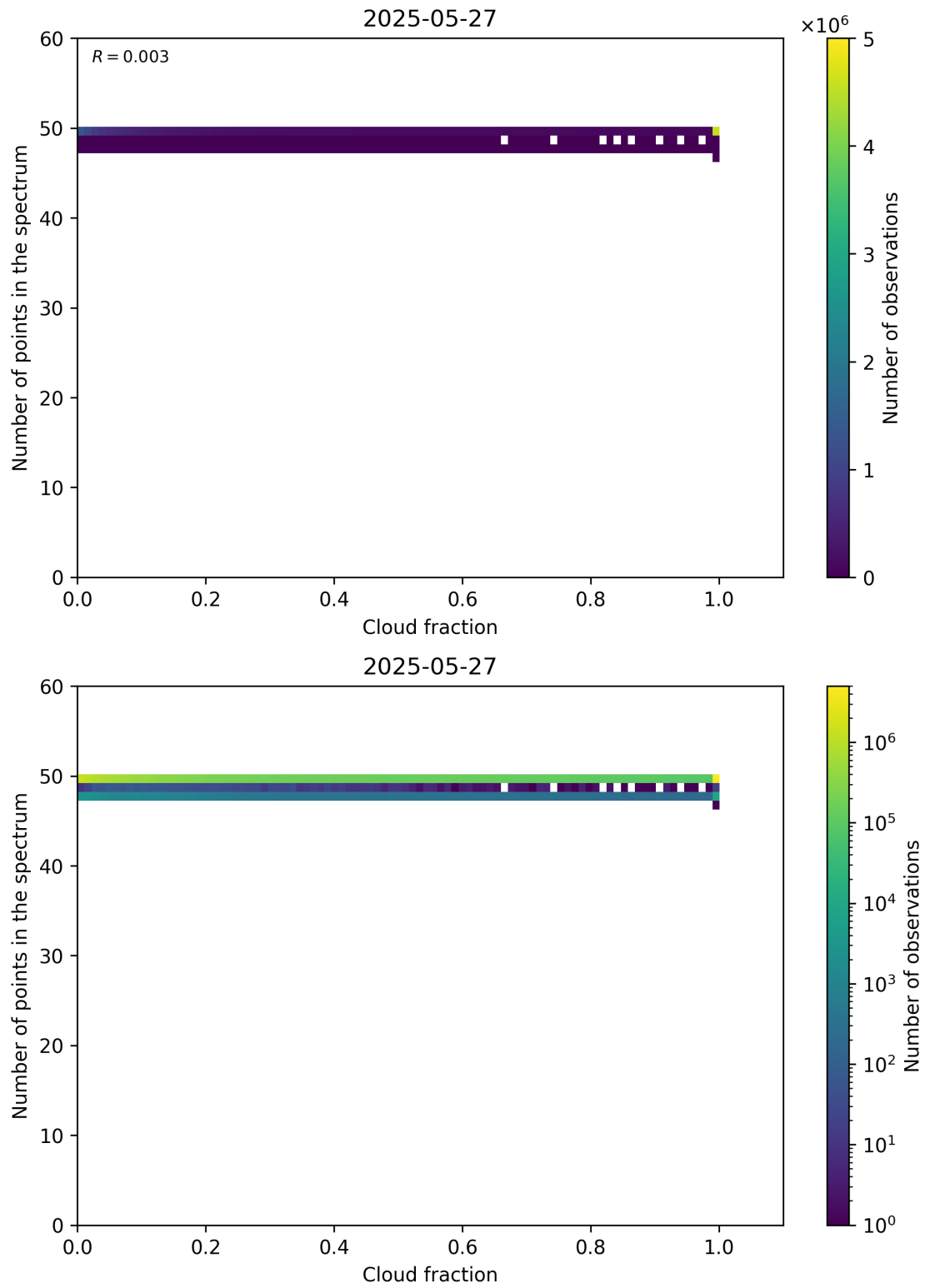
Figure 74: Scatter density plot of “Cloud fraction” against “Number of points in the spectrum” for 2025-05-26 to 2025-05-28.
