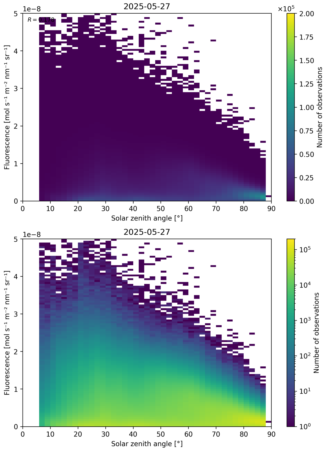
Figure 112: Scatter density plot of “Solar zenith angle” against “Fluorescence” for 2025-05-26 to 2025-05-28.
