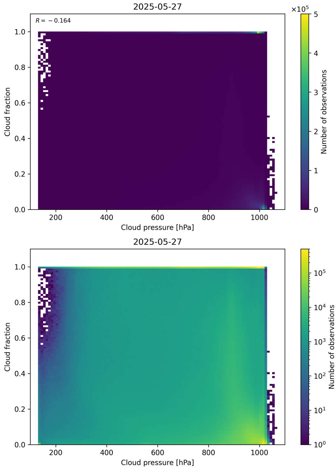
Figure 79: Scatter density plot of “Cloud pressure” against “Cloud fraction” for 2025-05-26 to 2025-05-28.
