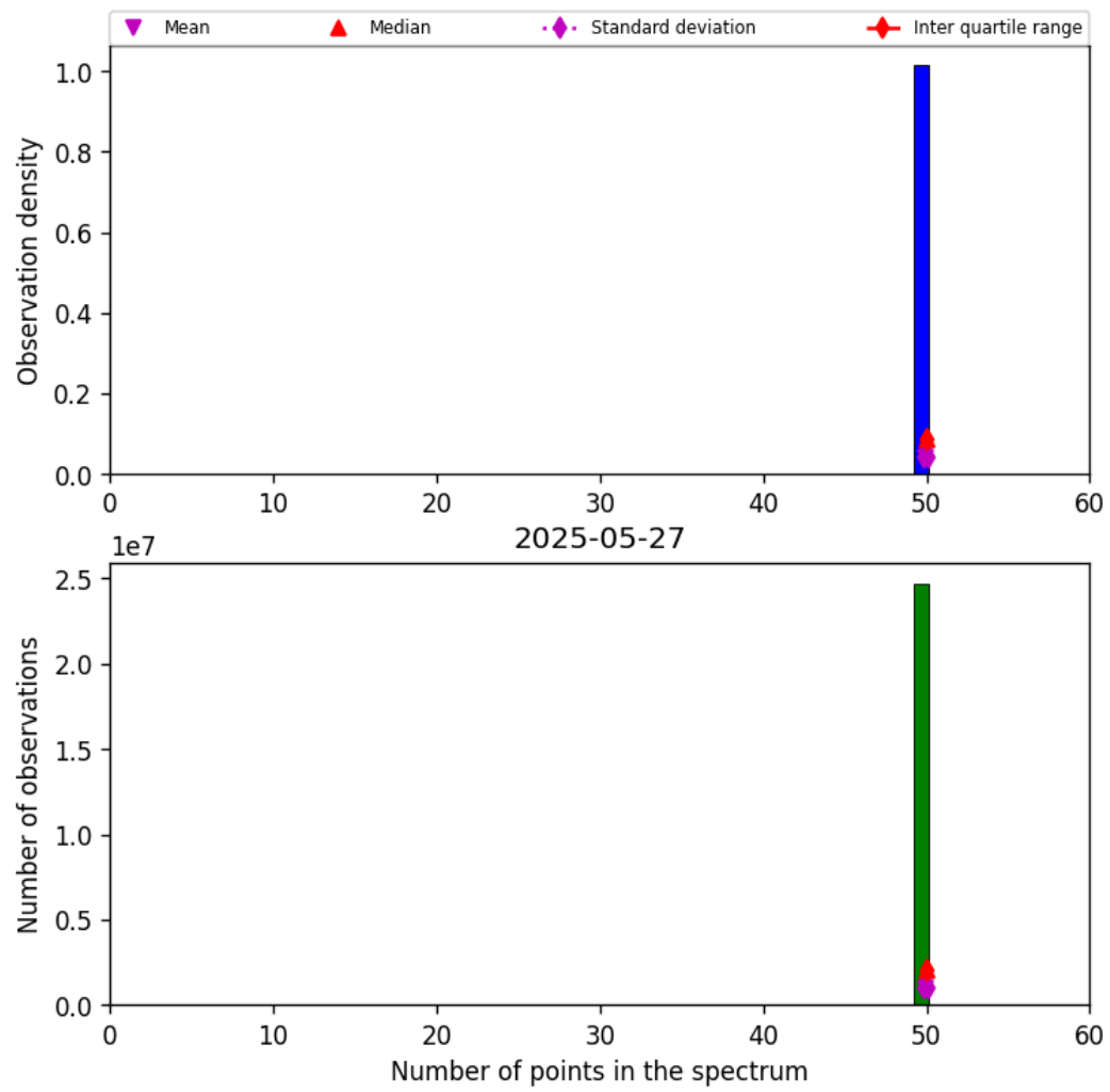
Figure 44: Histogram of “Number of points in the spectrum” for 2025-05-26 to 2025-05-28
