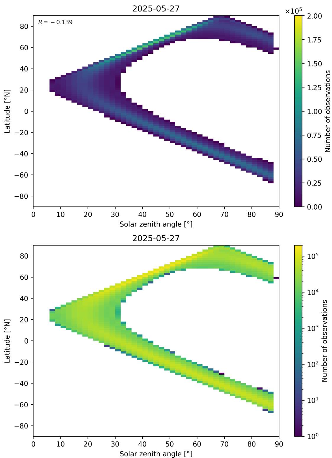
Figure 113: Scatter density plot of “Solar zenith angle” against “Latitude” for 2025-05-26 to 2025-05-28.
