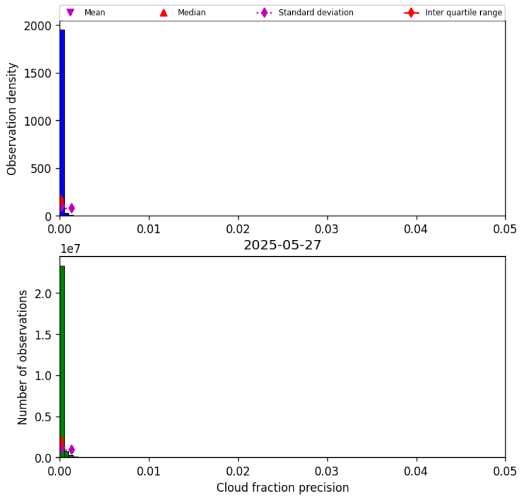
Figure 33: Histogram of “Cloud fraction precision” for 2025-05-26 to 2025-05-28
