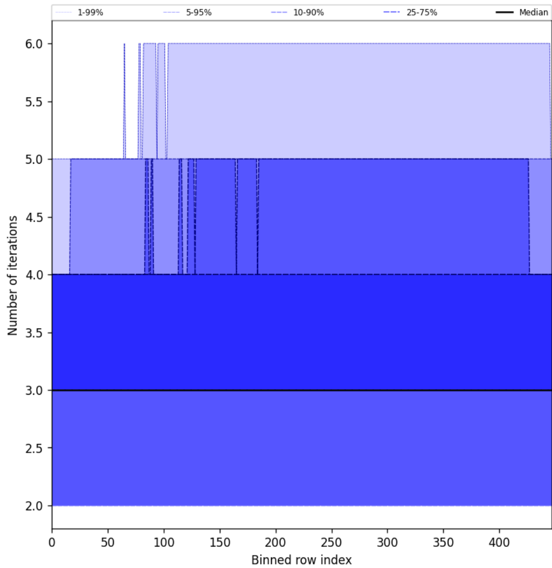
Figure 56: Along track statistics of “Number of iterations” for 2025-05-26 to 2025-05-28
