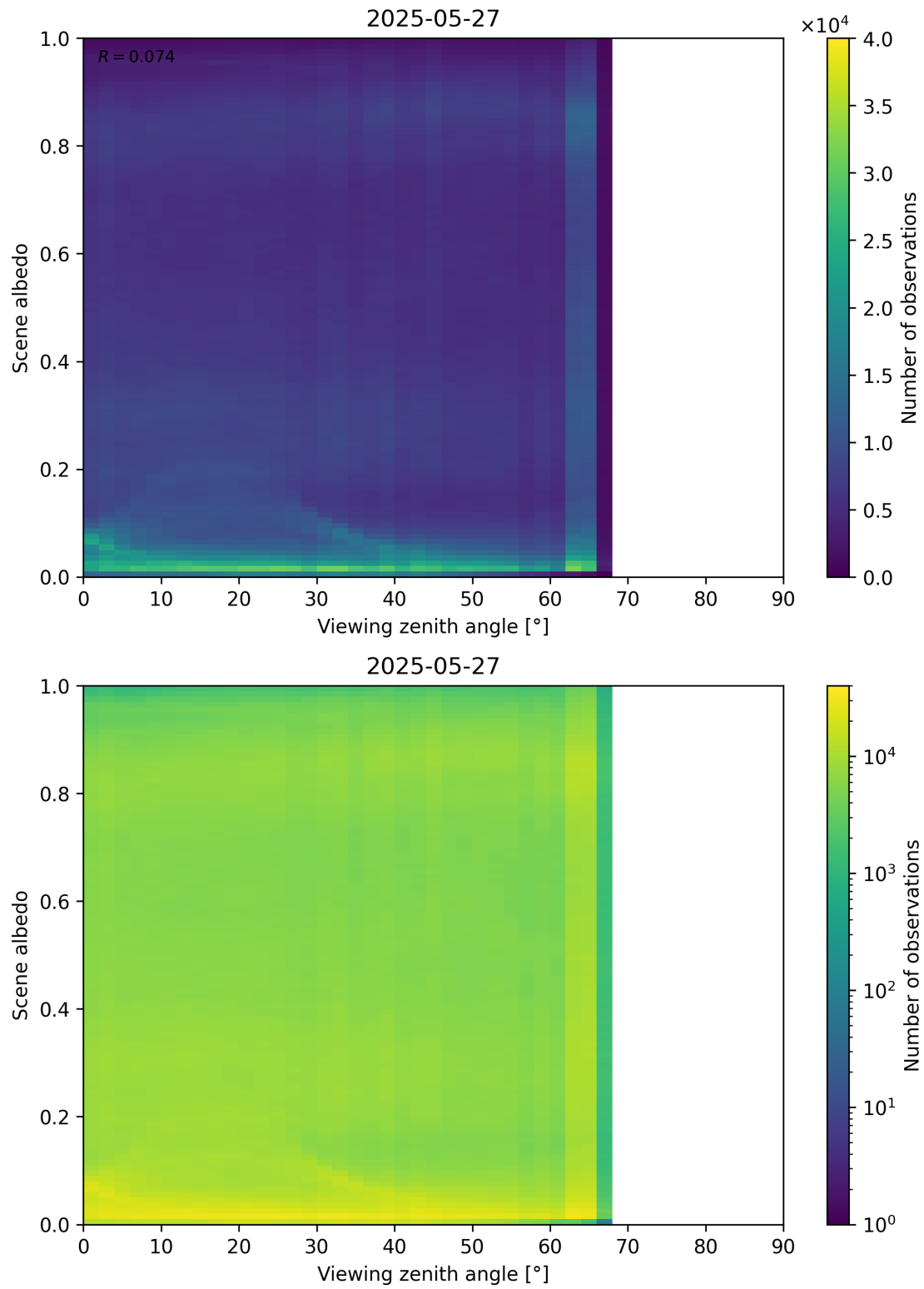
Figure 126: Scatter density plot of “Viewing zenith angle” against “Scene albedo” for 2025-05-26 to 2025-05-28.
