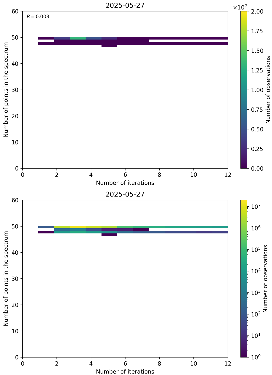
Figure 99: Scatter density plot of “Number of iterations” against “Number of points in the spectrum” for 2025-05-26 to 2025-05-28.
