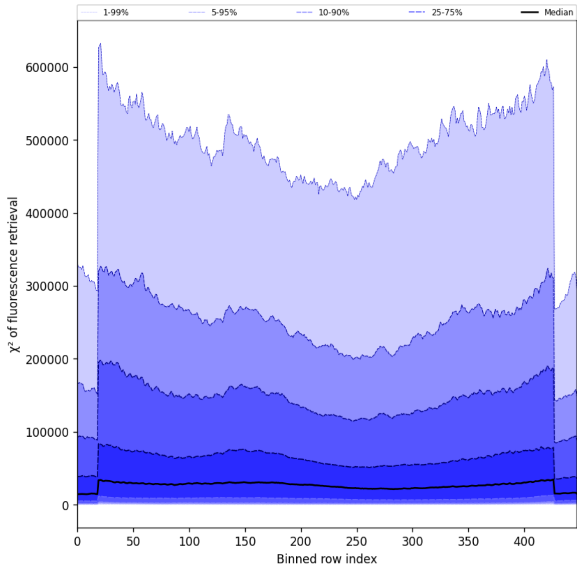
Figure 59: Along track statistics of “ \chi^2 of fluorescence retrieval” for 2025-05-26 to 2025-05-28
