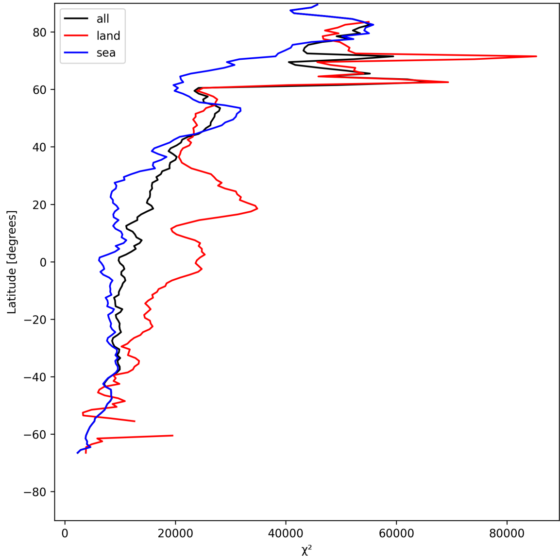
Figure 21: Zonal average of “ \chi^2 ” for 2025-05-26 to 2025-05-28.
