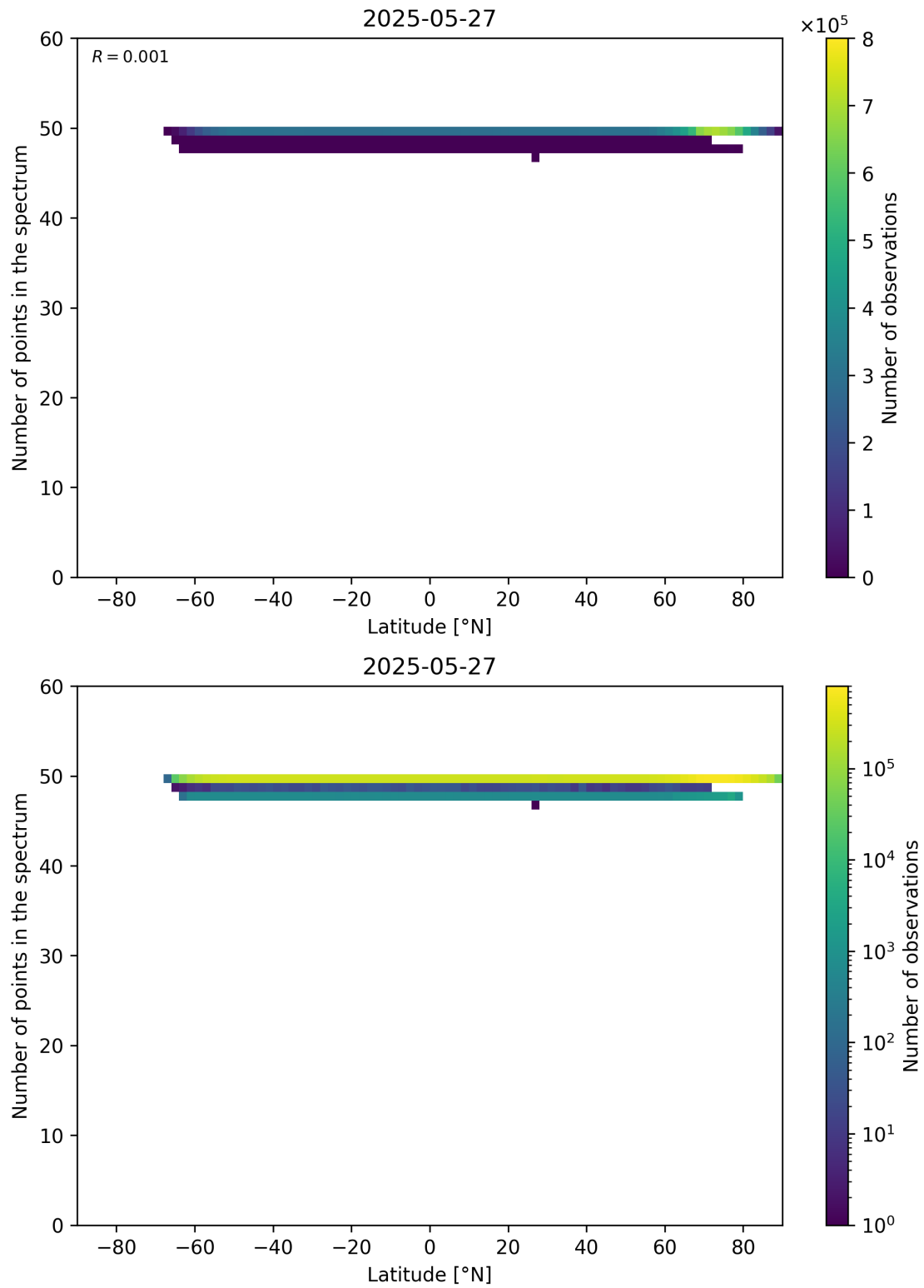
Figure 94: Scatter density plot of “Latitude” against “Number of points in the spectrum” for 2025-05-26 to 2025-05-28.
