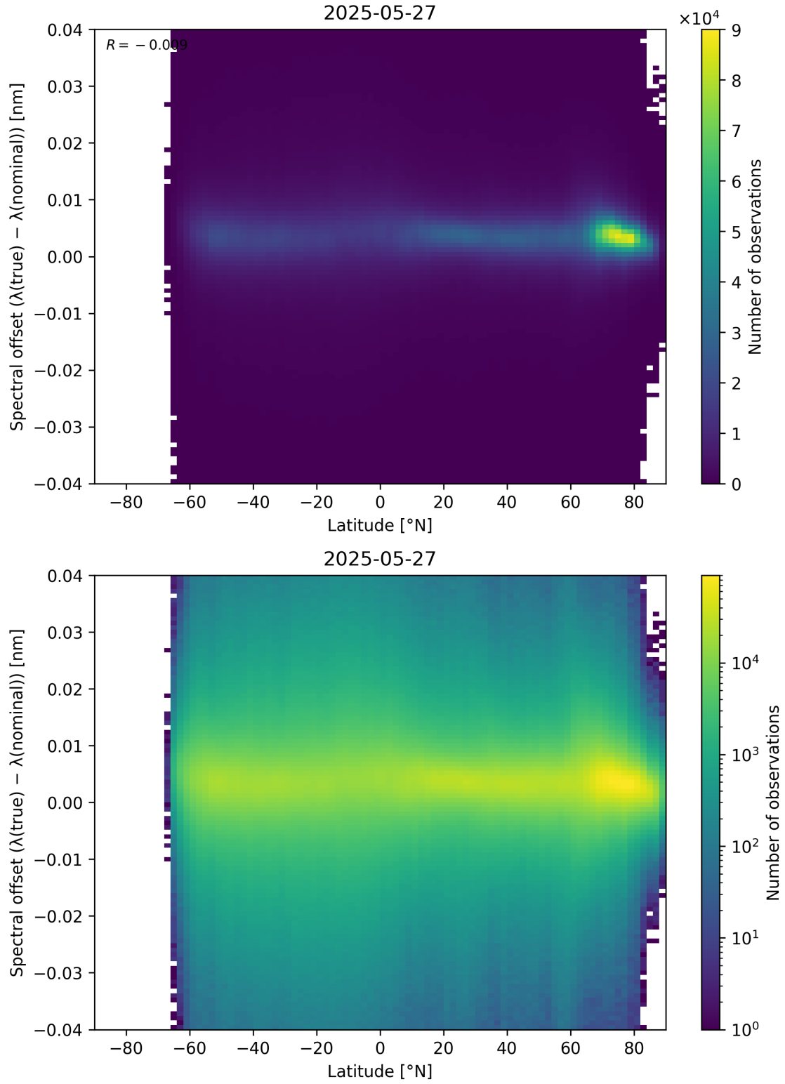
Figure 96: Scatter density plot of “Latitude” against “Spectral offset ( \lambda_{\text{true}} - \lambda_{\text{nominal}} )” for 2025-05-26 to 2025-05-28.
