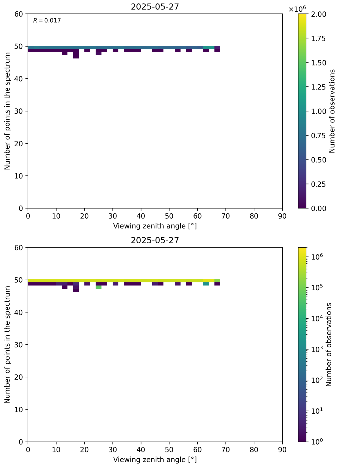
Figure 125: Scatter density plot of “Viewing zenith angle” against “Number of points in the spectrum” for 2025-05-26 to 2025-05-28.
