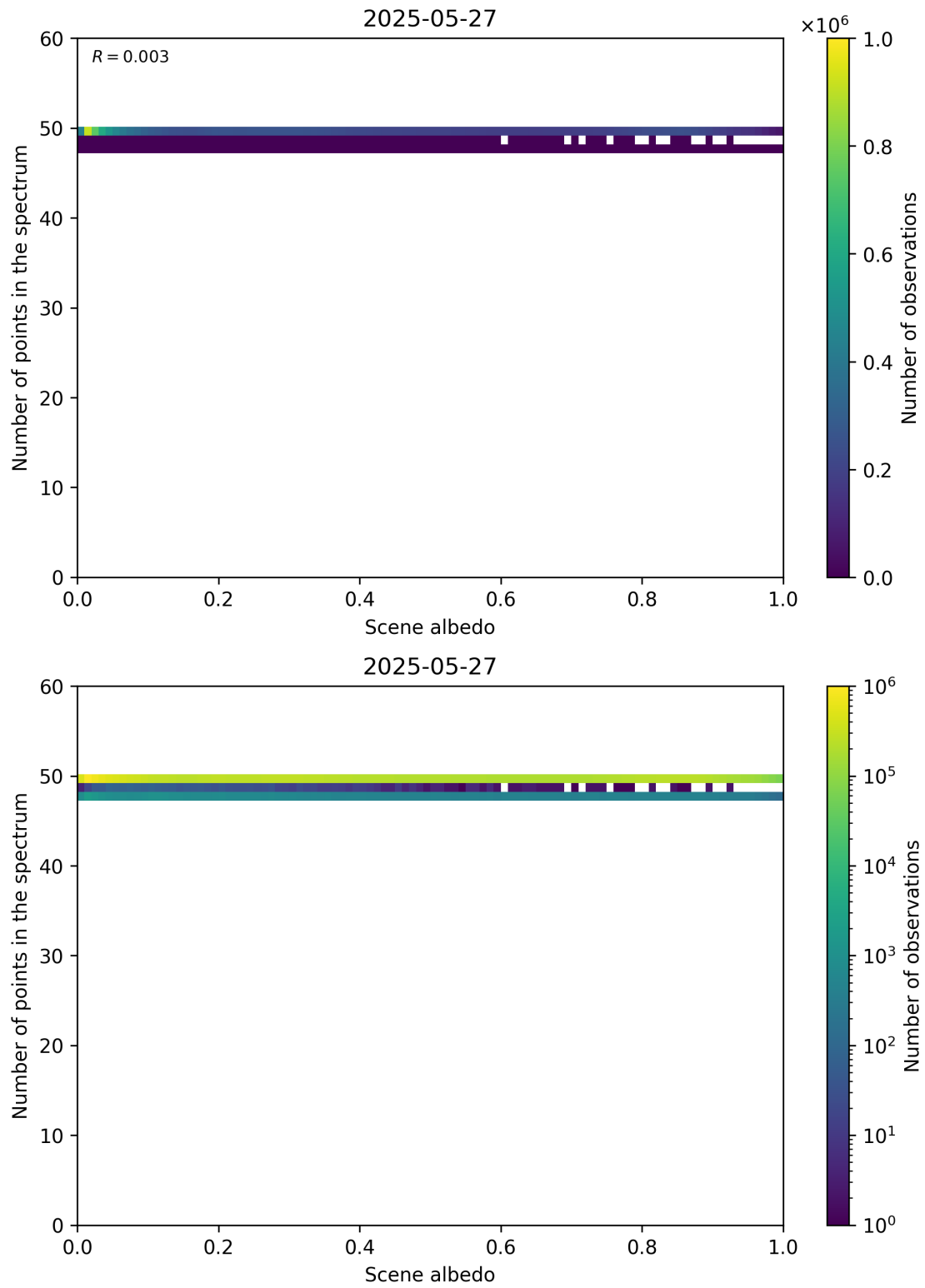
Figure 106: Scatter density plot of “Scene albedo” against “Number of points in the spectrum” for 2025-05-26 to 2025-05-28.
