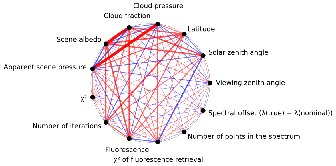
Figure 1: Map of correlation graph for 2025-05-26 to 2025-05-28.
