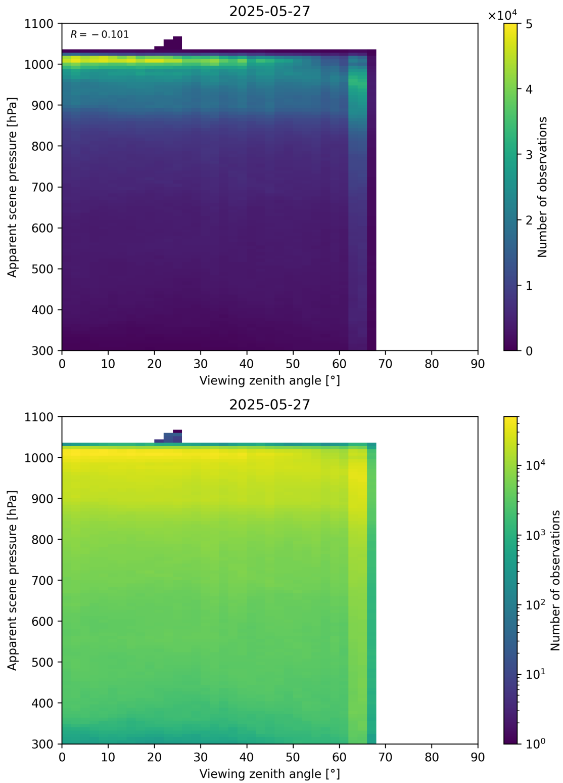
Figure 118: Scatter density plot of “Viewing zenith angle” against “Apparent scene pressure” for 2025-05-26 to 2025-05-28.
