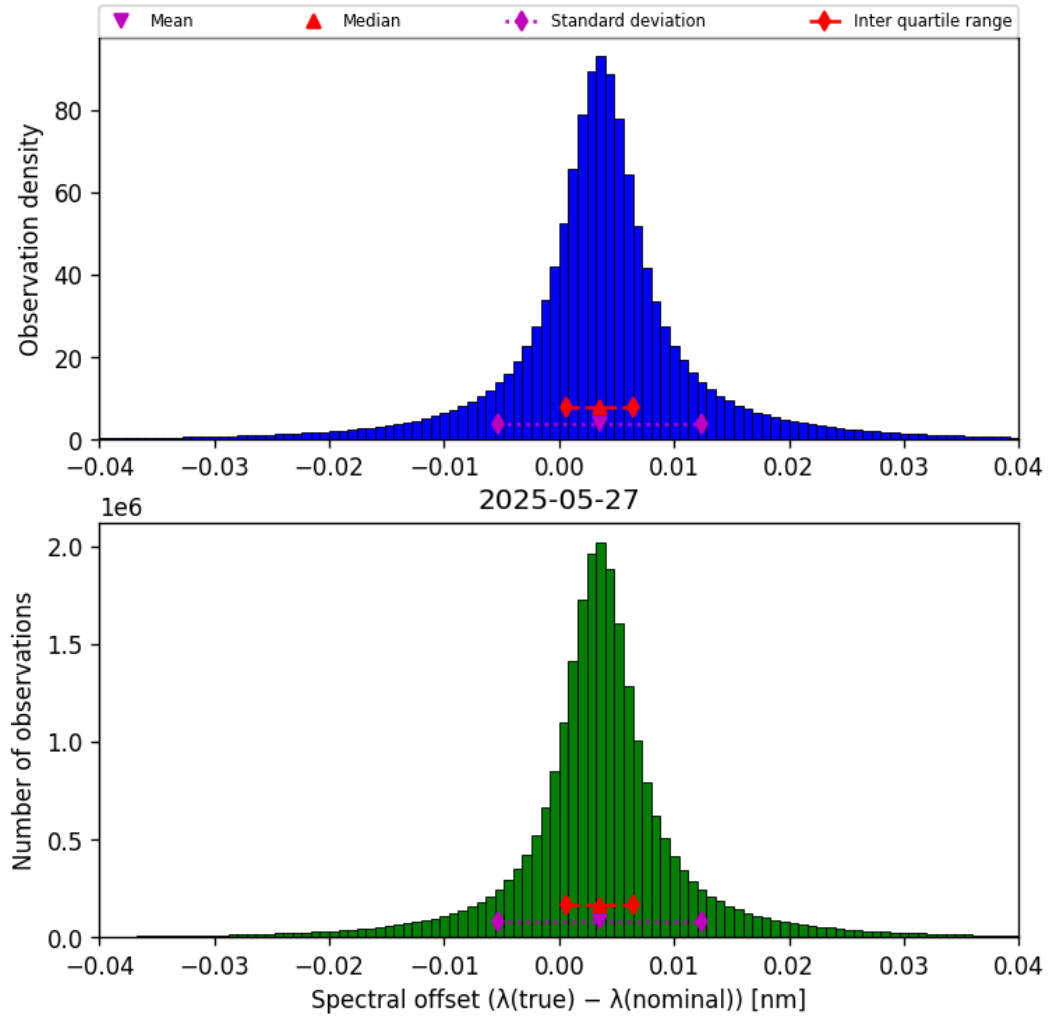
Figure 45: Histogram of “Spectral offset ( \lambda_{\text{true}} - \lambda_{\text{nominal}} )” for 2025-05-26 to 2025-05-28
