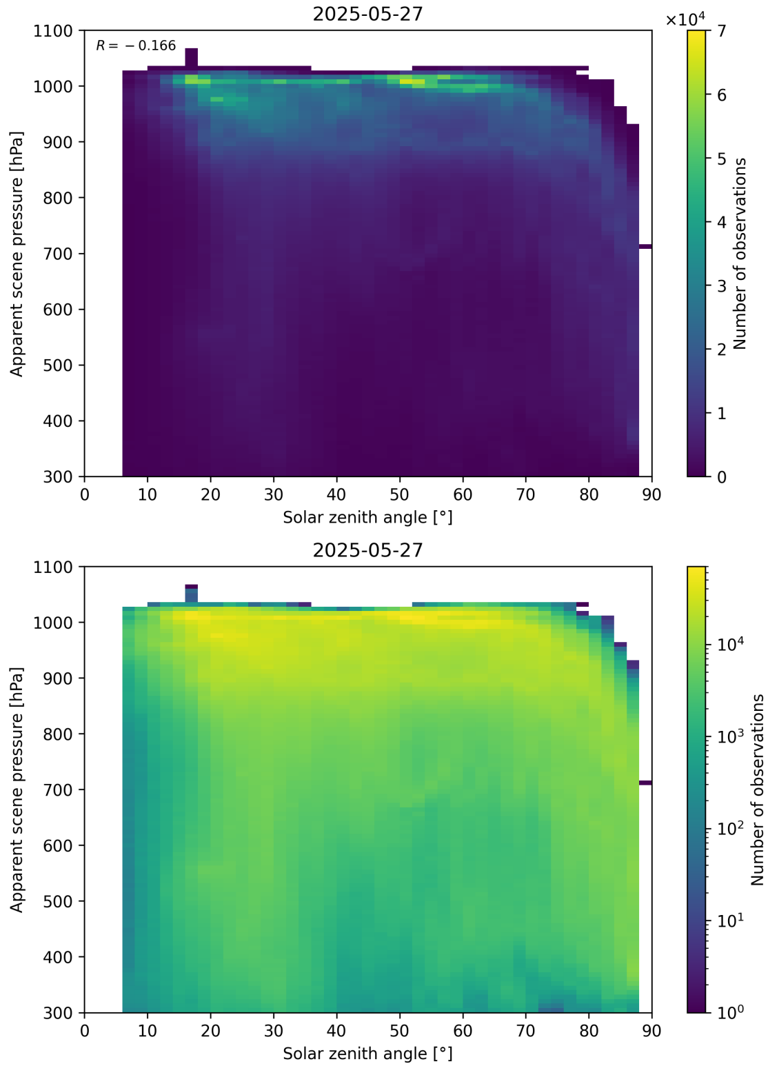
Figure 108: Scatter density plot of “Solar zenith angle” against “Apparent scene pressure” for 2025-05-26 to 2025-05-28.
