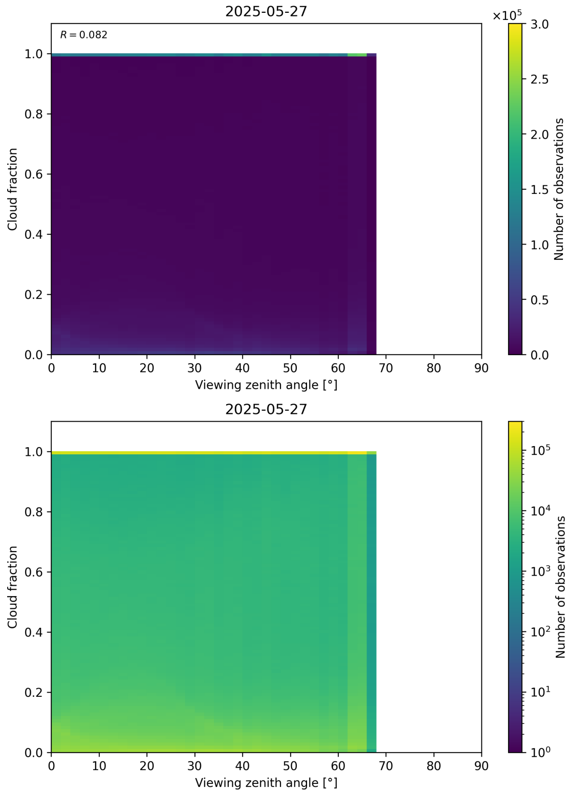
Figure 120: Scatter density plot of “Viewing zenith angle” against “Cloud fraction” for 2025-05-26 to 2025-05-28.
