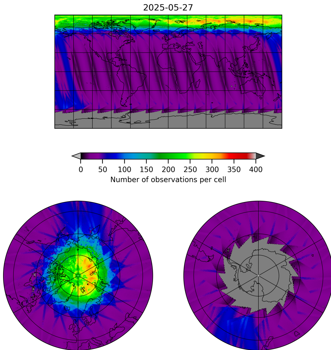
Figure 11: Map of the number of observations for 2025-05-26 to 2025-05-28
