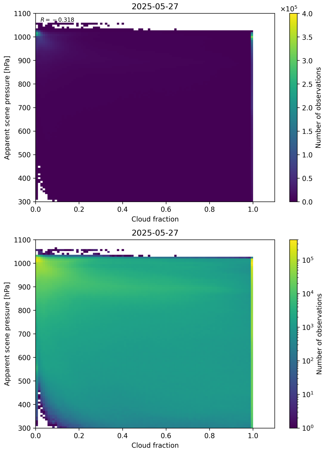
Figure 70: Scatter density plot of “Cloud fraction” against “Apparent scene pressure” for 2025-05-26 to 2025-05-28.
