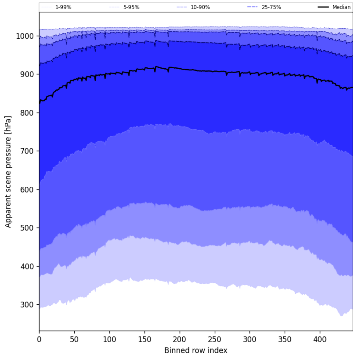
Figure 53: Along track statistics of “Apparent scene pressure” for 2025-05-26 to 2025-05-28
