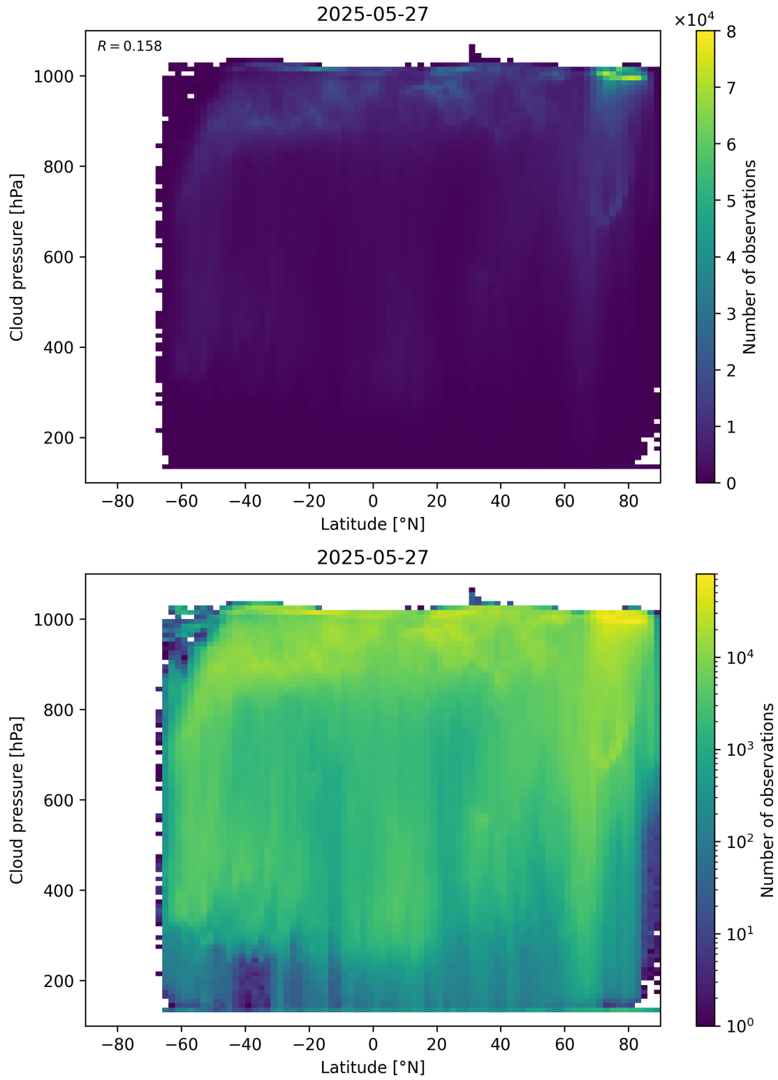
Figure 91: Scatter density plot of “Latitude” against “Cloud pressure” for 2025-05-26 to 2025-05-28.
