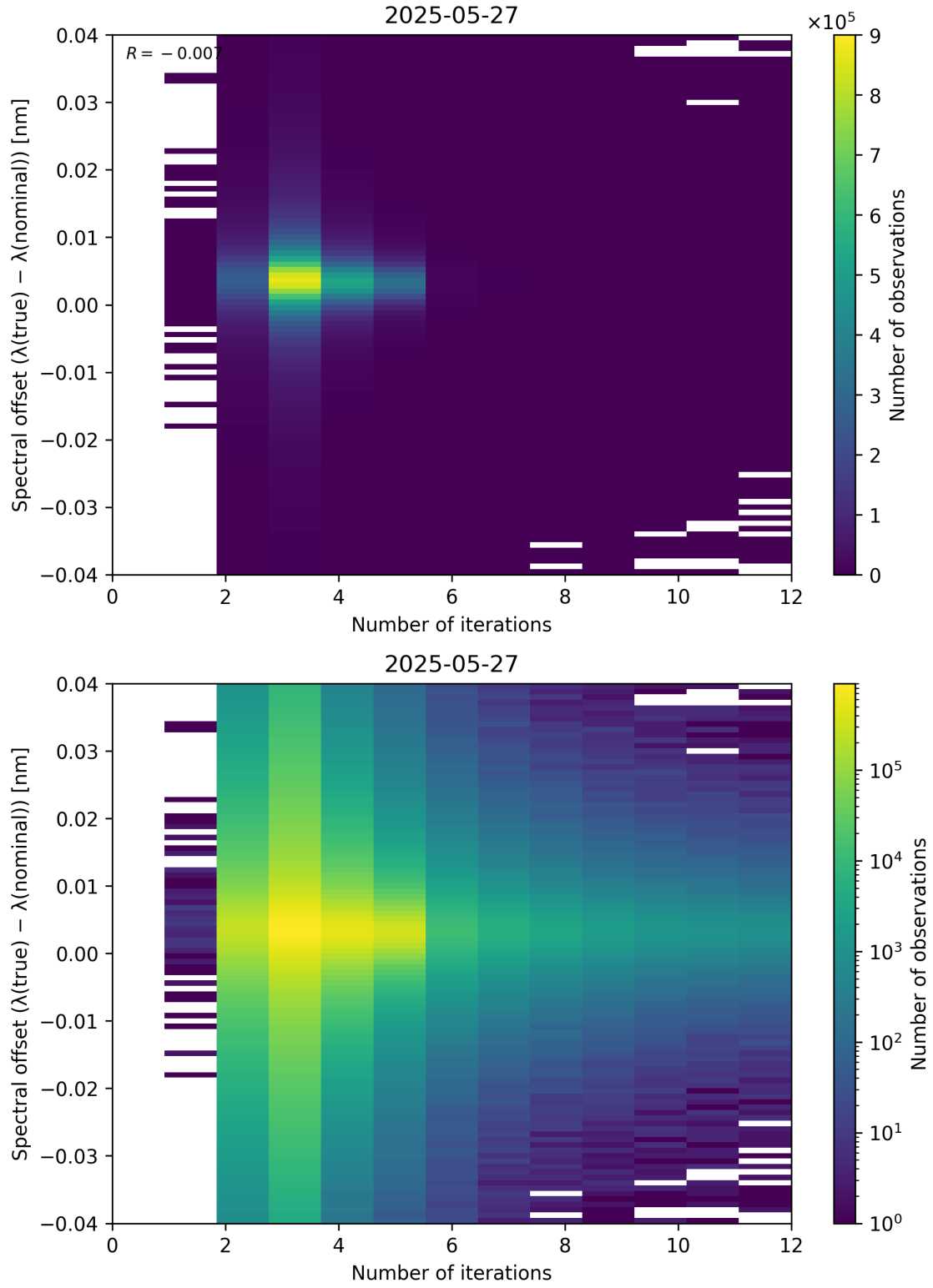
Figure 100: Scatter density plot of “Number of iterations” against “Spectral offset ( \lambda_{\text{true}} - \lambda_{\text{nominal}} )” for 2025-05-26 to 2025-05-28.
