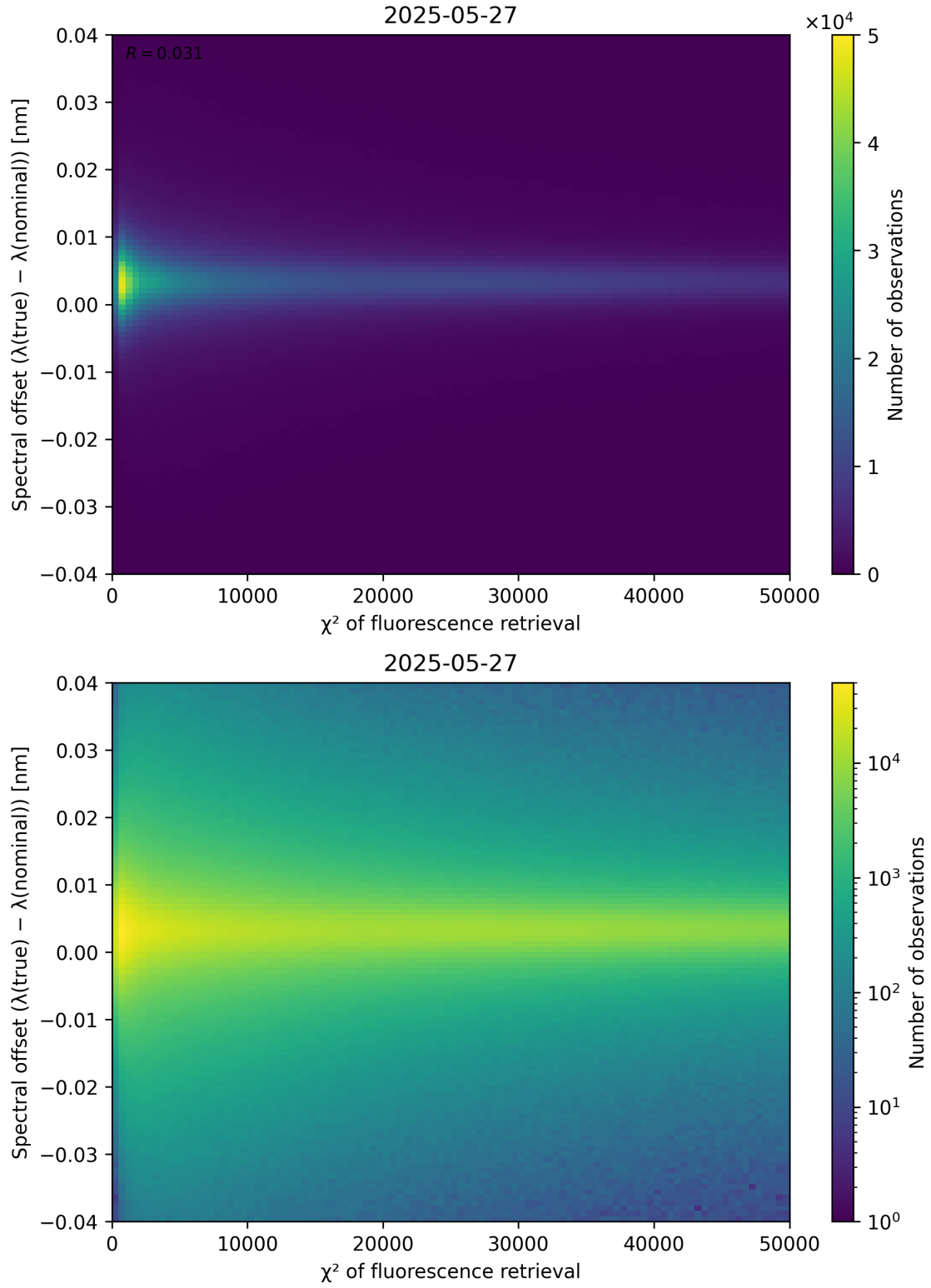
Figure 69: Scatter density plot of “ \chi^2 of fluorescence retrieval” against “Spectral offset ( \lambda_{\text{true}} - \lambda_{\text{nominal}} )” for 2025-05-26 to 2025-05-28.
