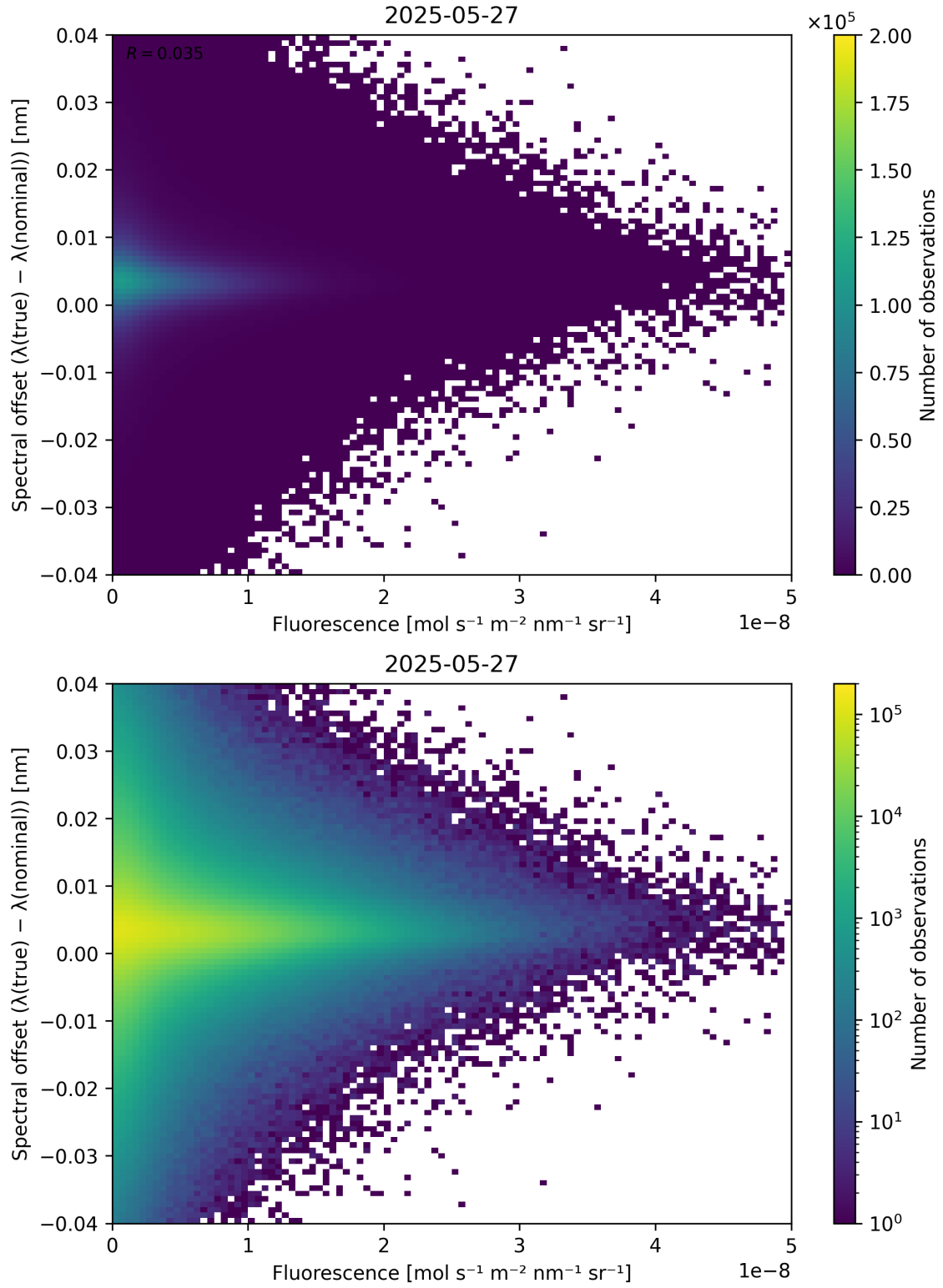
Figure 87: Scatter density plot of “Fluorescence” against “Spectral offset ( \lambda_{\text{true}} - \lambda_{\text{nominal}} )” for 2025-05-26 to 2025-05-28.
