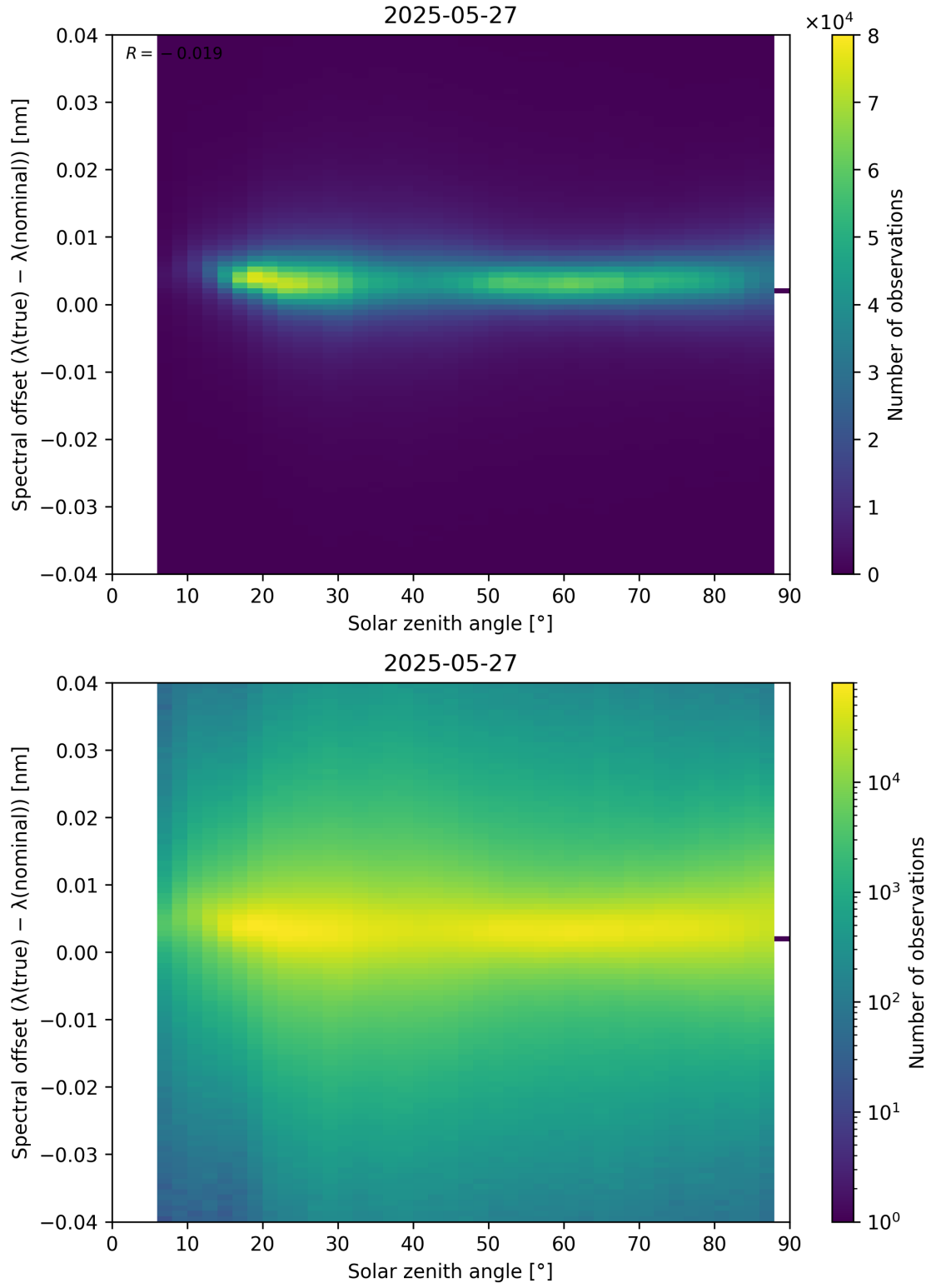
Figure 117: Scatter density plot of “Solar zenith angle” against “Spectral offset ( \lambda_{\text{true}} - \lambda_{\text{nominal}} )” for 2025-05-26 to 2025-05-28.
