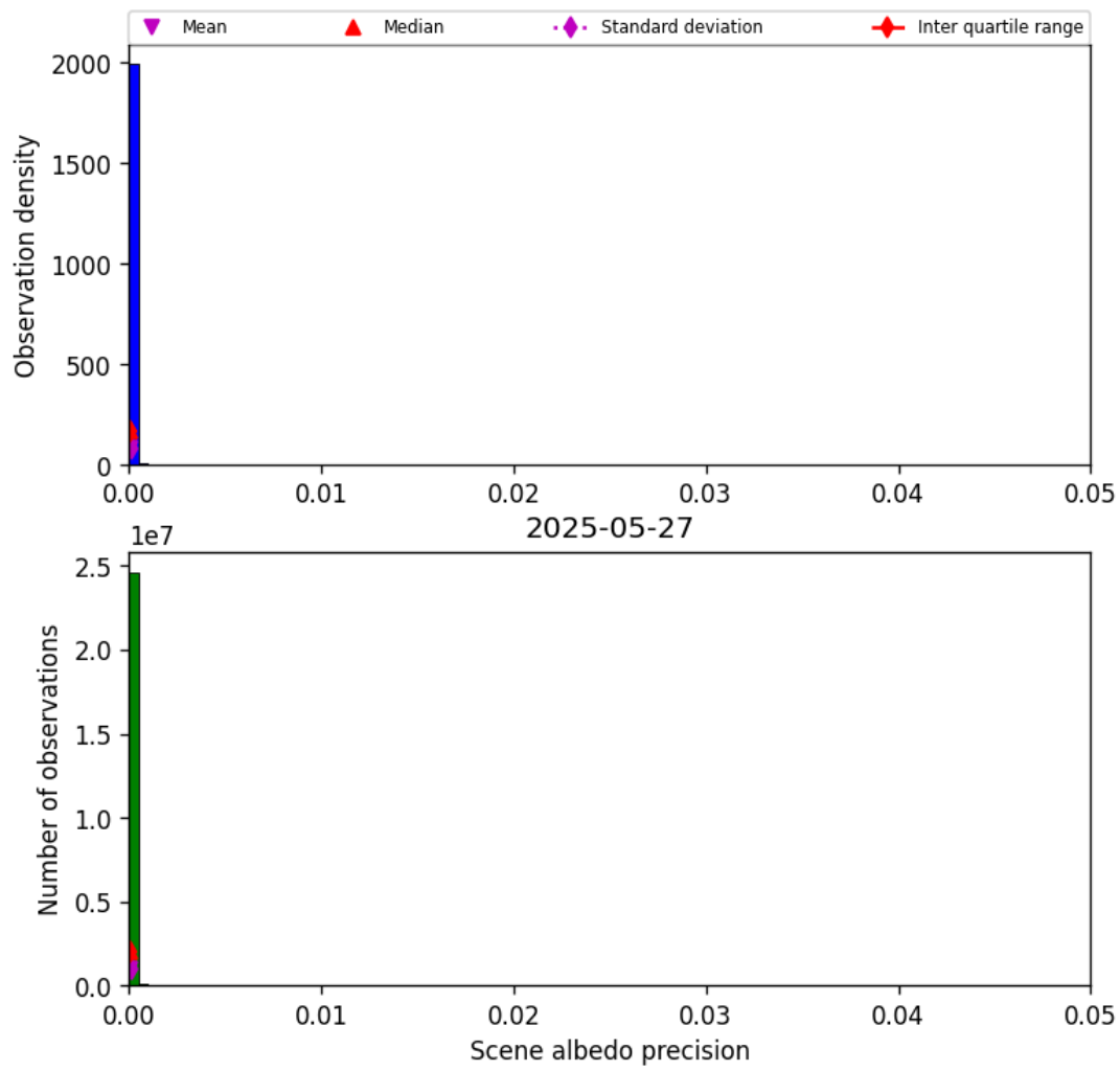
Figure 35: Histogram of “Scene albedo precision” for 2025-05-26 to 2025-05-28
