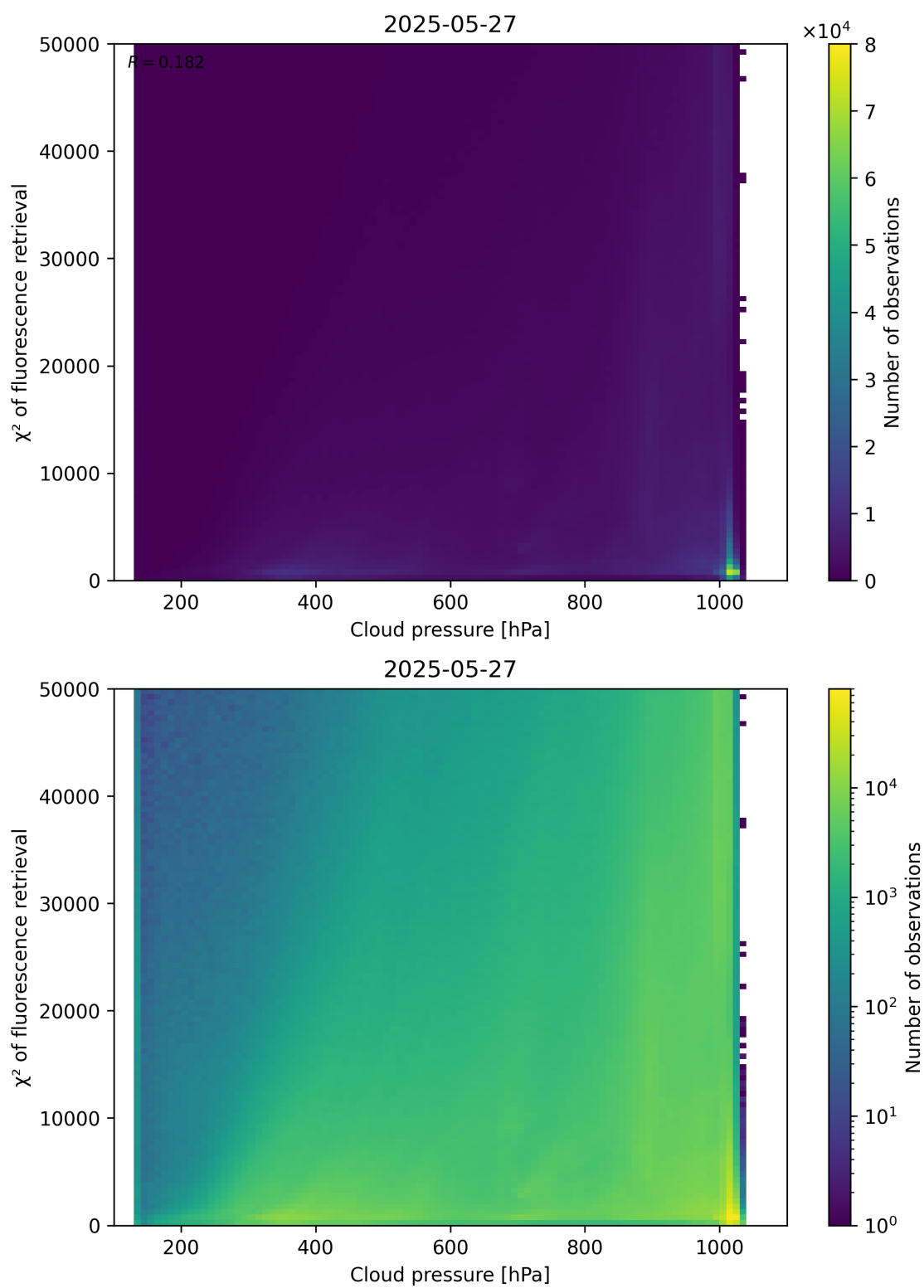
Figure 78: Scatter density plot of “Cloud pressure” against “ \chi^2 of fluorescence retrieval” for 2025-05-26 to 2025-05-28.
