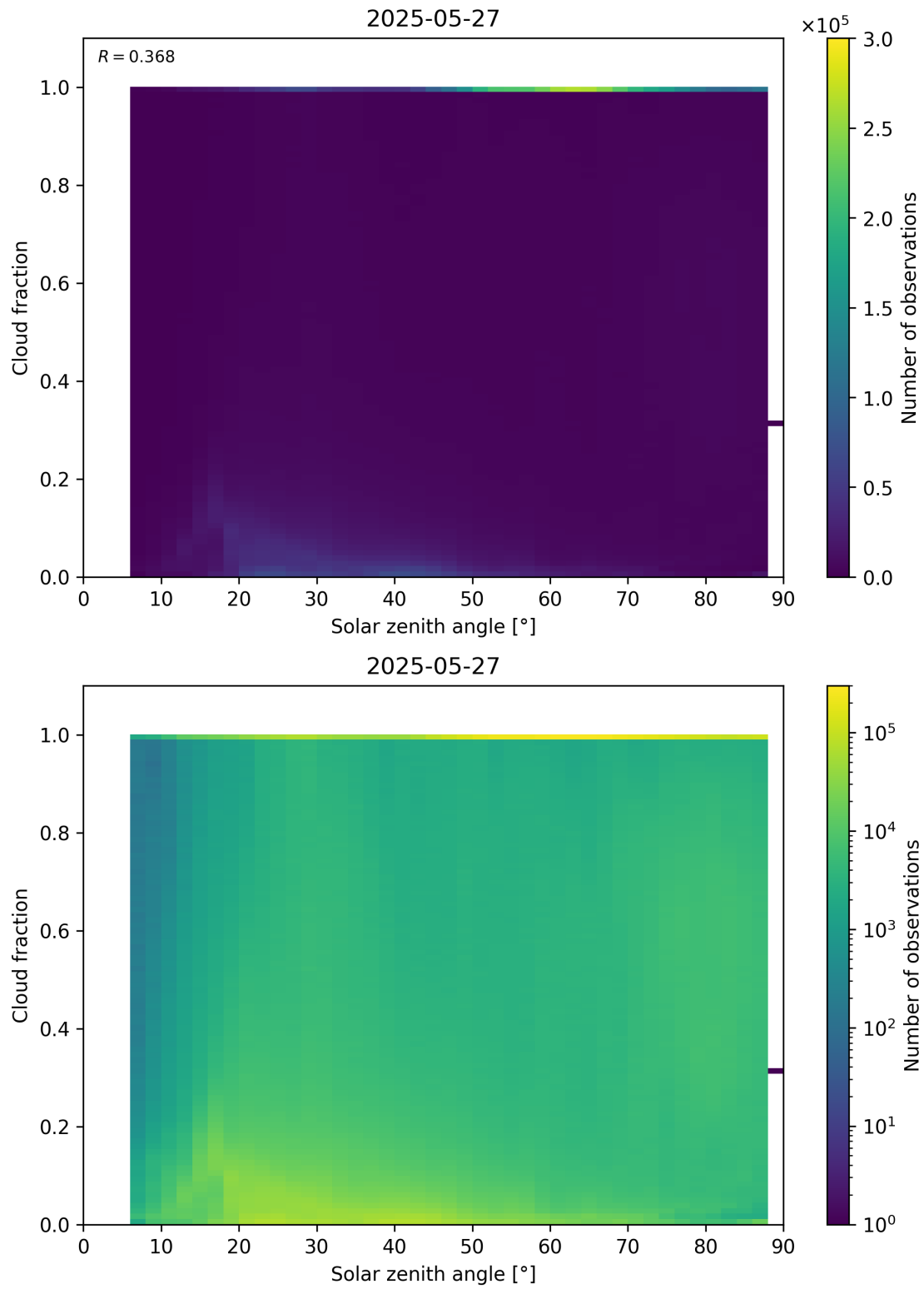
Figure 110: Scatter density plot of “Solar zenith angle” against “Cloud fraction” for 2025-05-26 to 2025-05-28.
