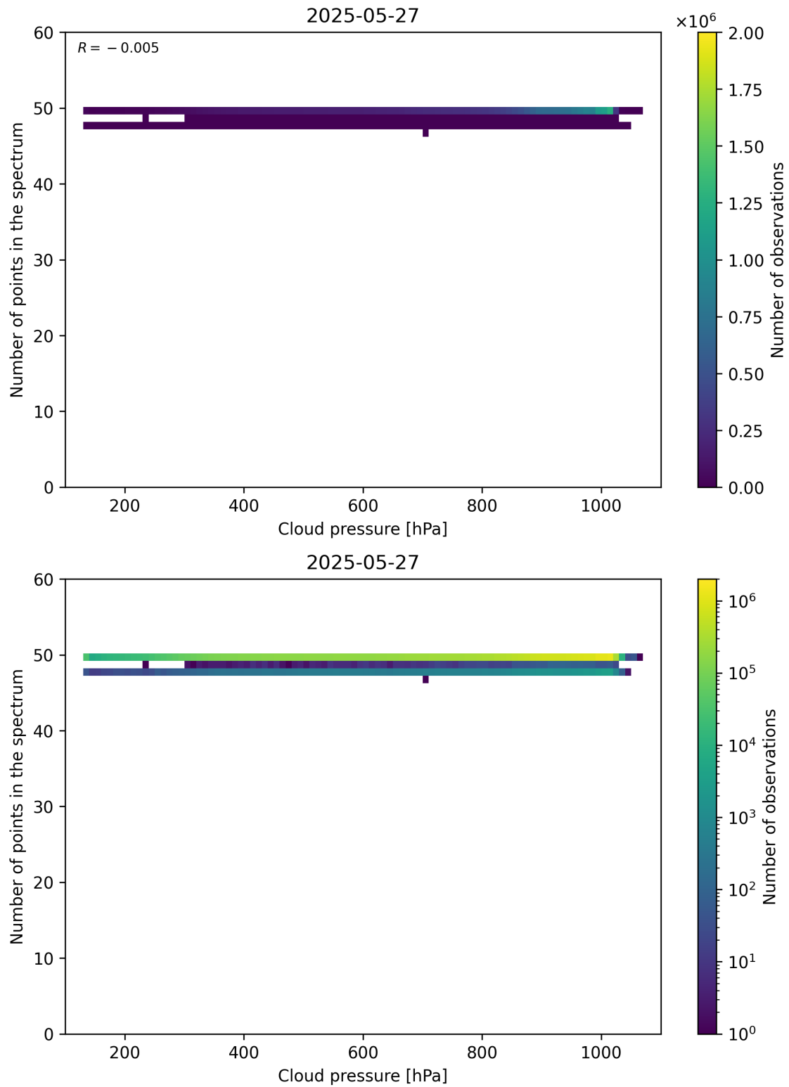
Figure 82: Scatter density plot of “Cloud pressure” against “Number of points in the spectrum” for 2025-05-26 to 2025-05-28.
