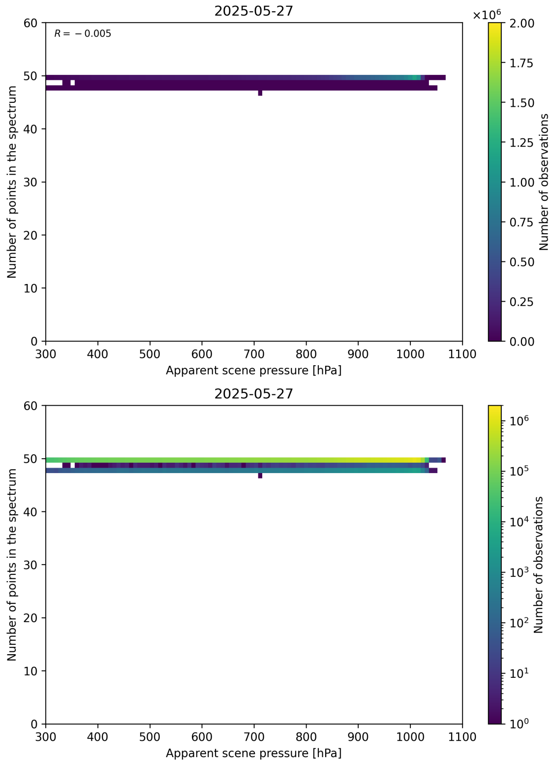
Figure 66: Scatter density plot of “Apparent scene pressure” against “Number of points in the spectrum” for 2025-05-26 to 2025-05-28.
