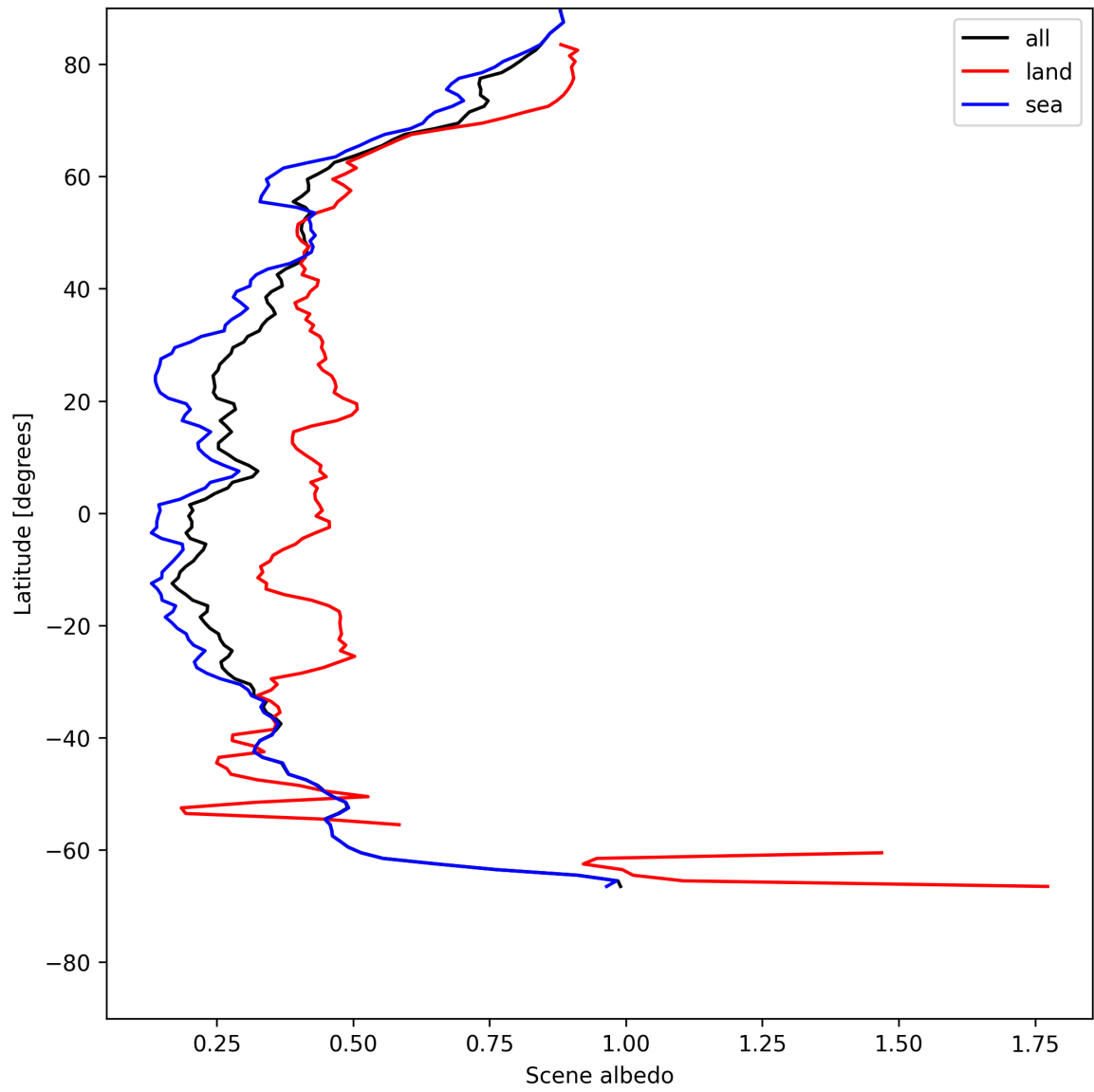
Figure 17: Zonal average of “Scene albedo” for 2025-05-26 to 2025-05-28.
