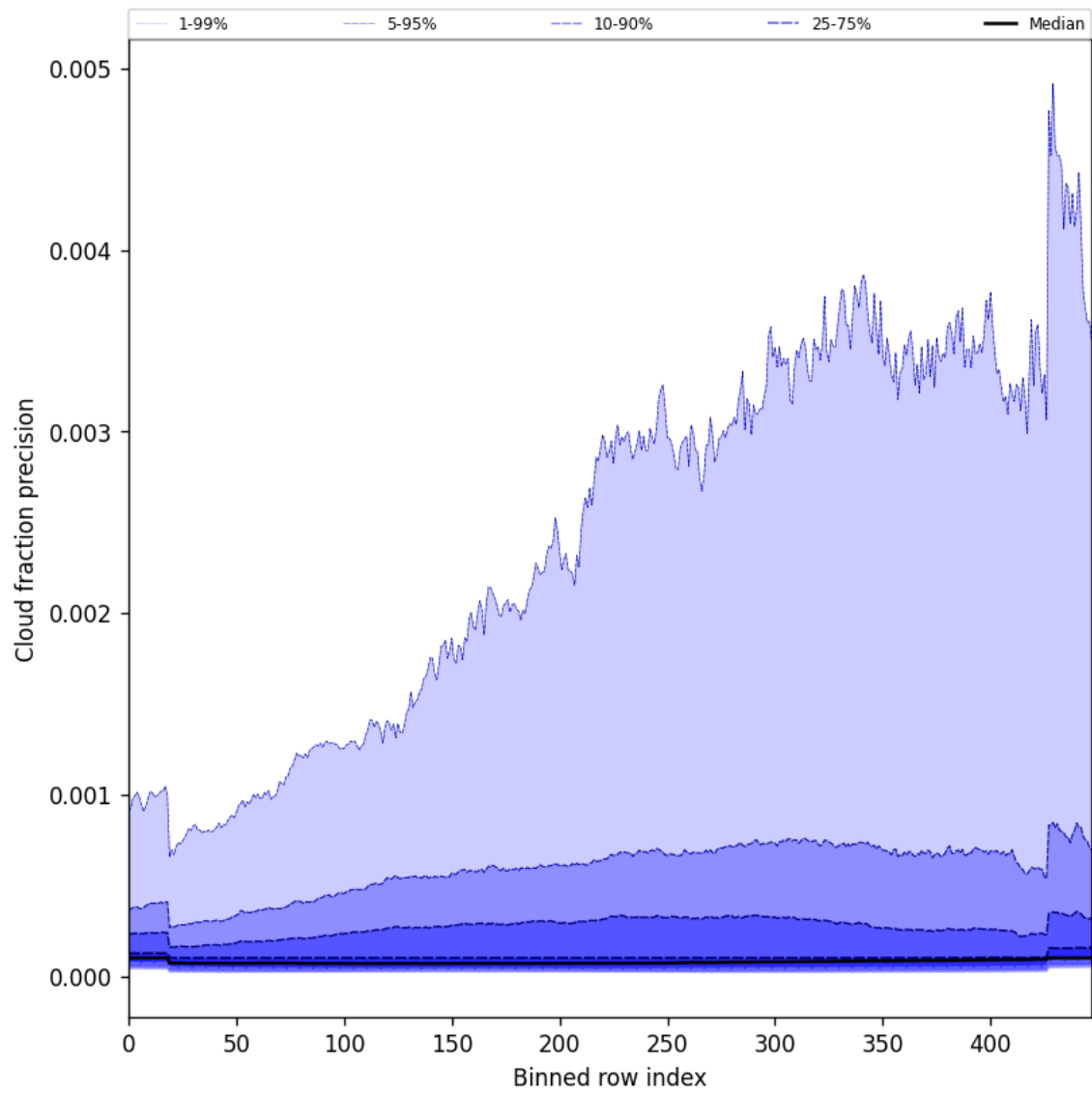
Figure 50: Along track statistics of “Cloud fraction precision” for 2025-05-26 to 2025-05-28
