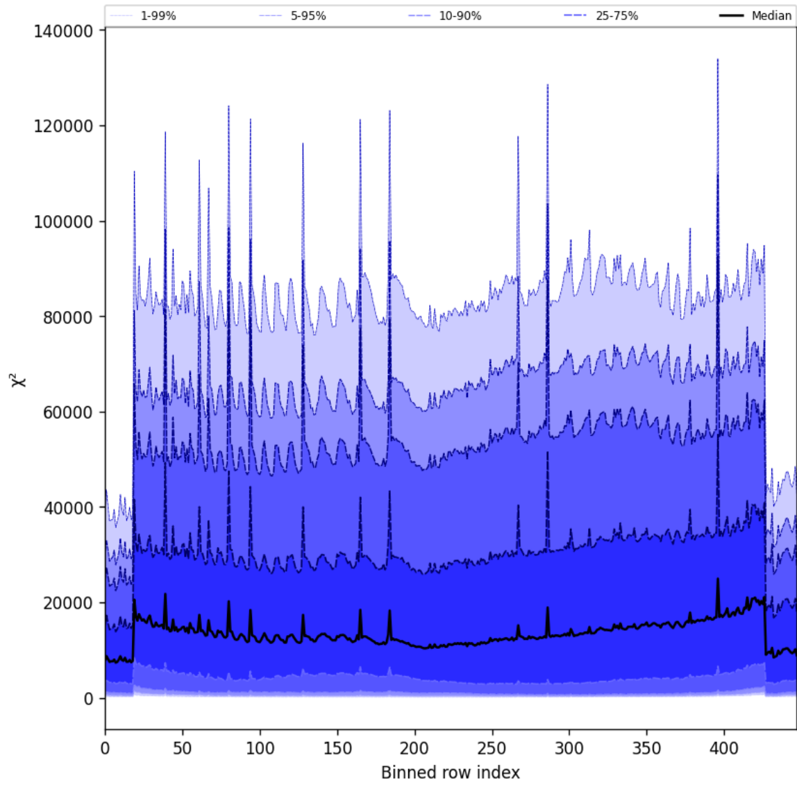
Figure 55: Along track statistics of “ \chi^2 ” for 2025-05-26 to 2025-05-28
