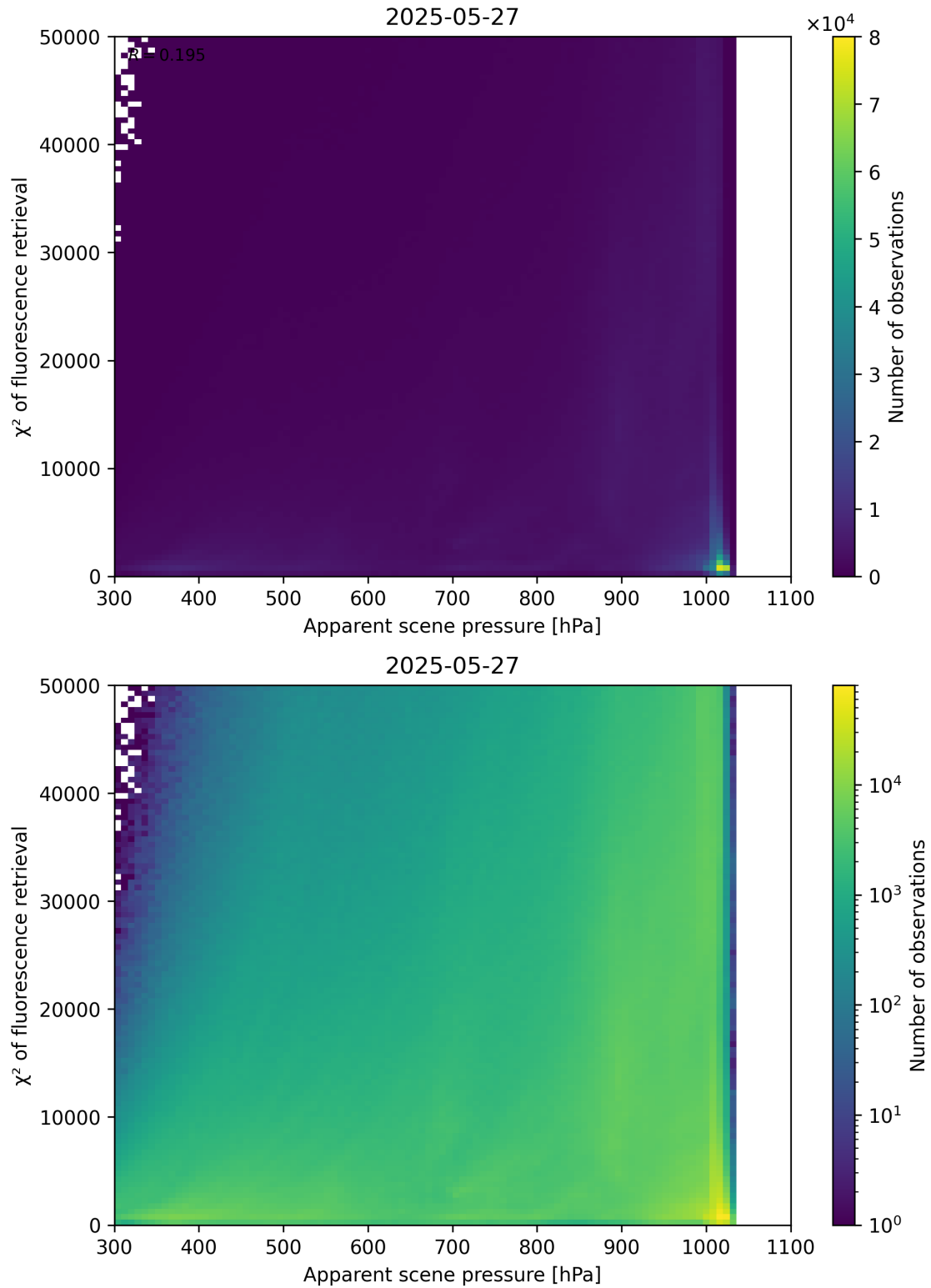
Figure 63: Scatter density plot of “Apparent scene pressure” against “ \chi^2 of fluorescence retrieval” for 2025-05-26 to 2025-05-28.
