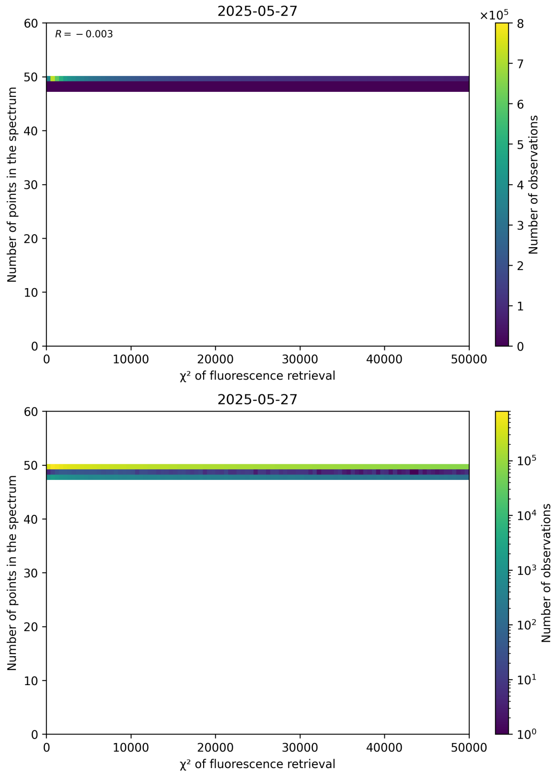
Figure 68: Scatter density plot of “ \chi^2 of fluorescence retrieval” against “Number of points in the spectrum” for 2025-05-26 to 2025-05-28.
