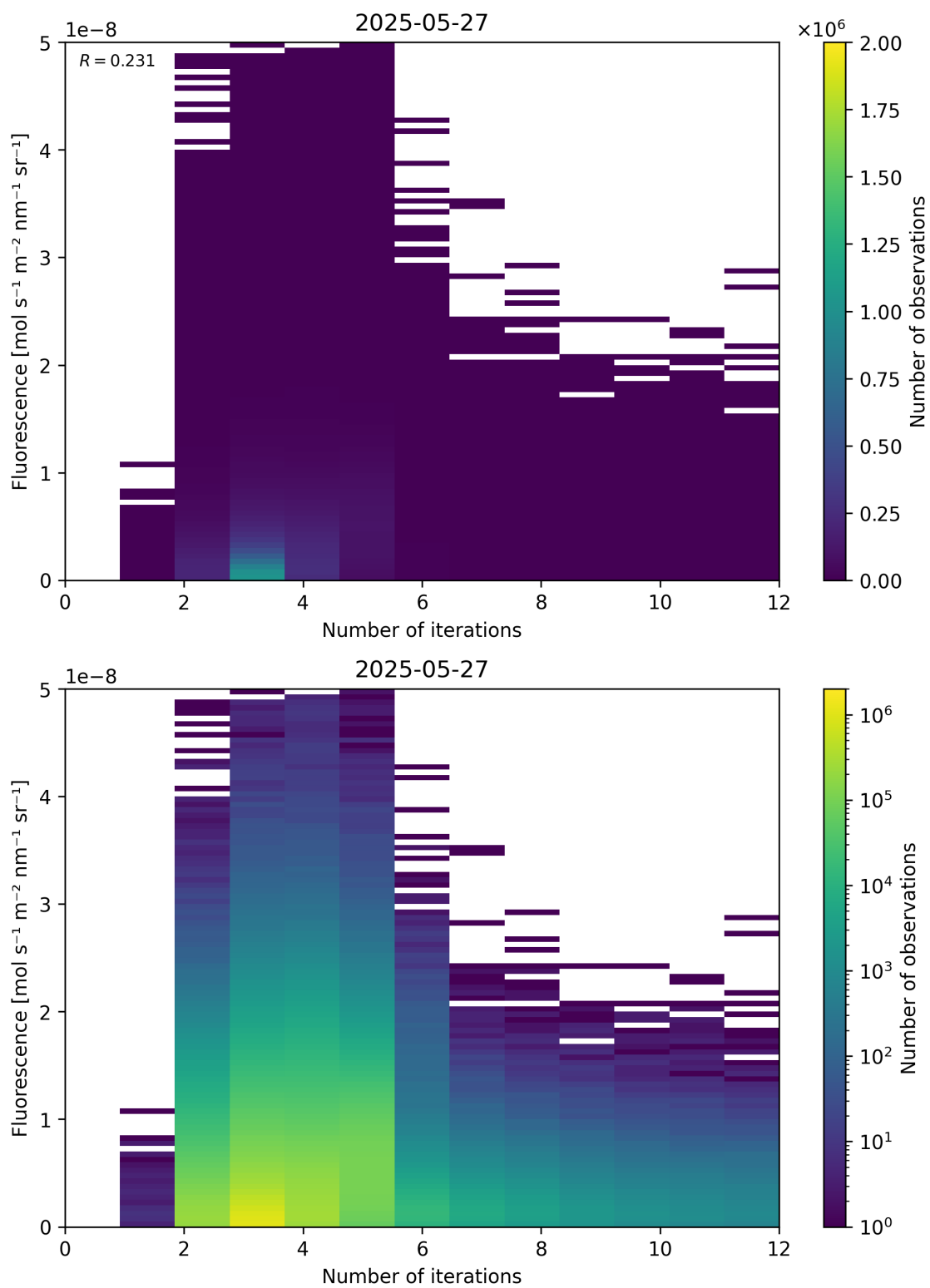
Figure 98: Scatter density plot of “Number of iterations” against “Fluorescence” for 2025-05-26 to 2025-05-28.
