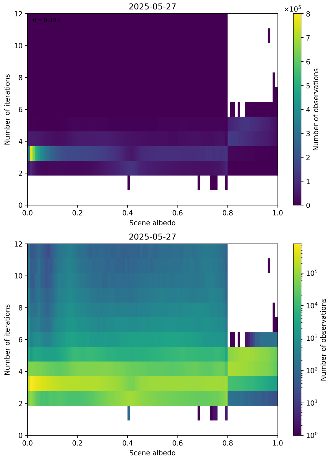
Figure 105: Scatter density plot of “Scene albedo” against “Number of iterations” for 2025-05-26 to 2025-05-28.
