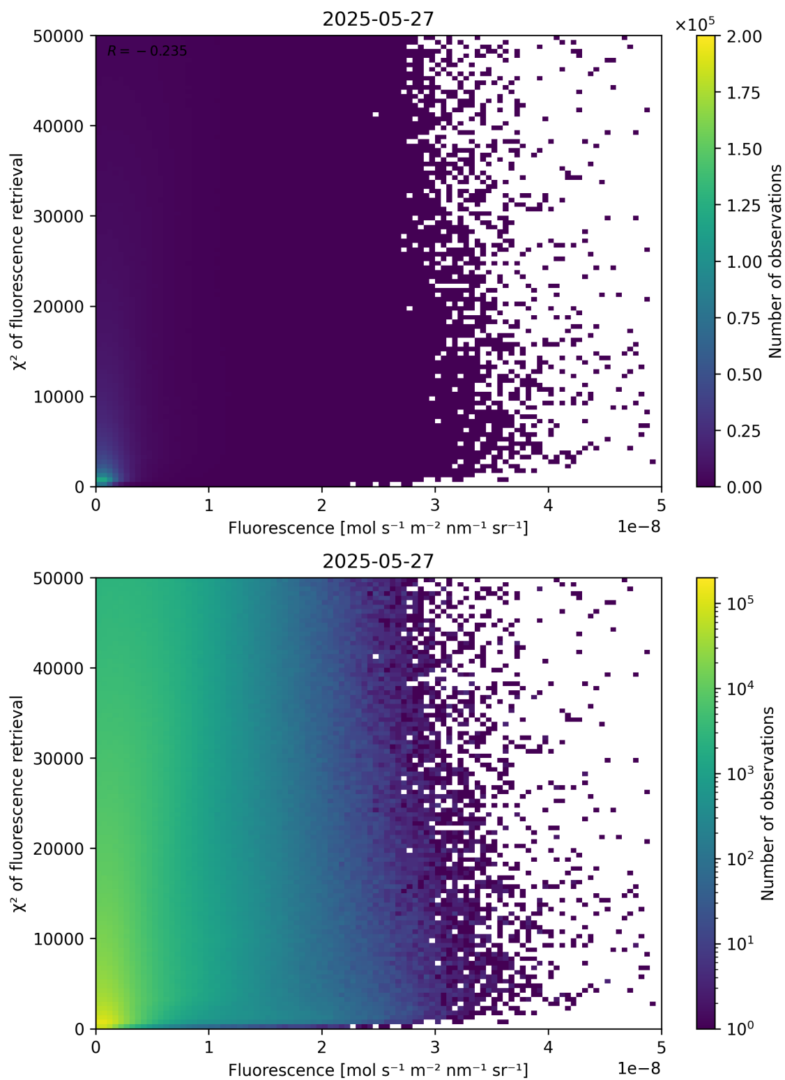
Figure 85: Scatter density plot of “Fluorescence” against “ \chi^2 of fluorescence retrieval” for 2025-05-26 to 2025-05-28.
