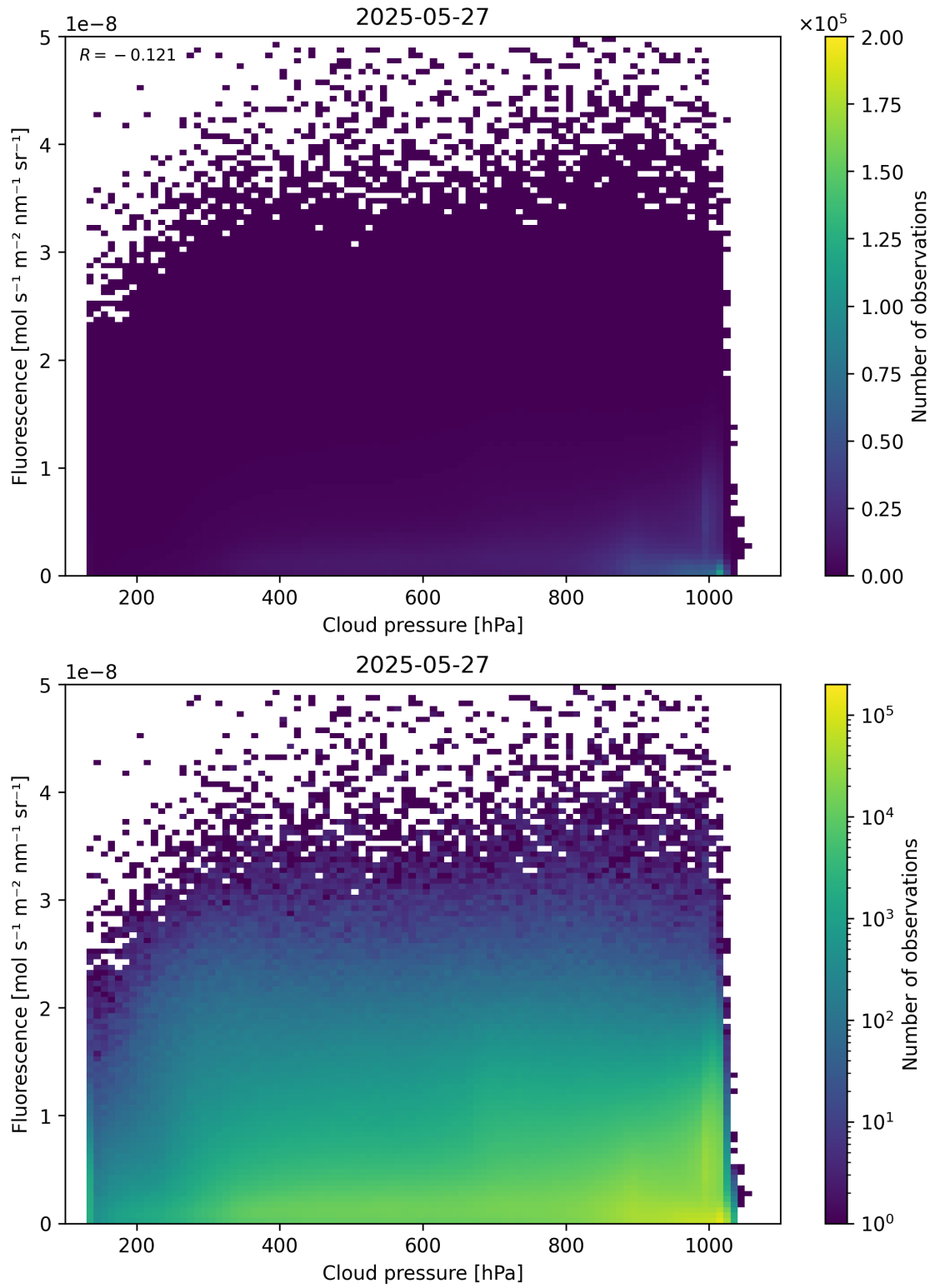
Figure 80: Scatter density plot of “Cloud pressure” against “Fluorescence” for 2025-05-26 to 2025-05-28.
