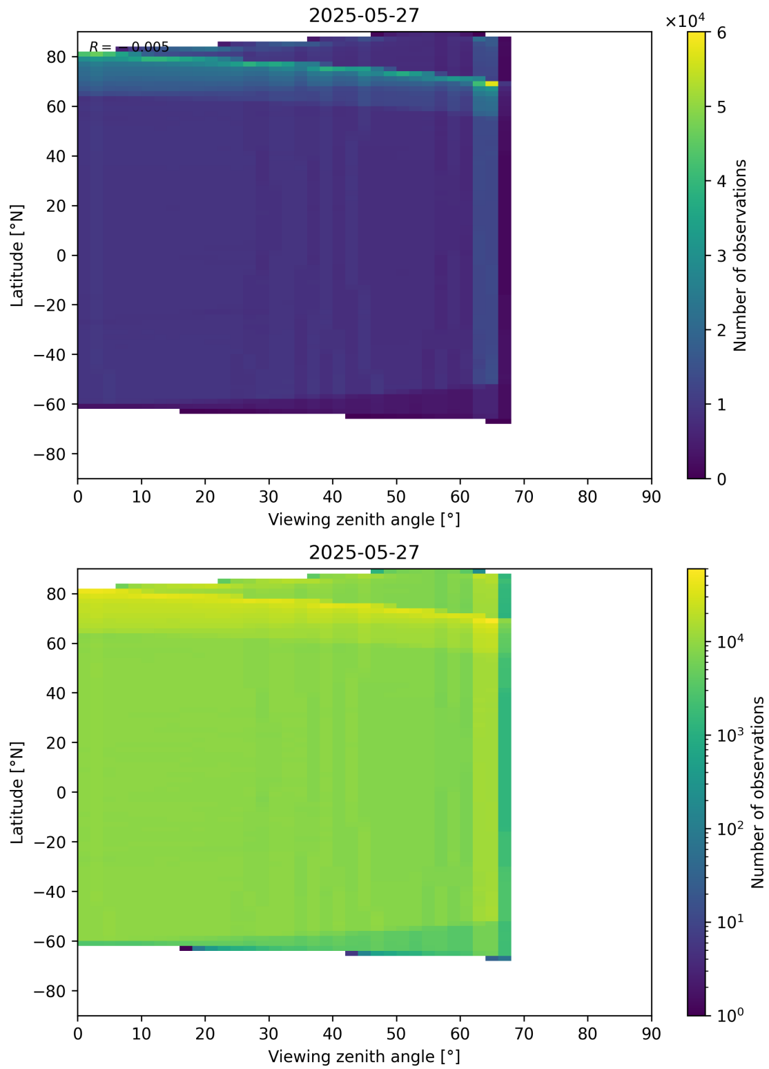
Figure 123: Scatter density plot of “Viewing zenith angle” against “Latitude” for 2025-05-26 to 2025-05-28.
