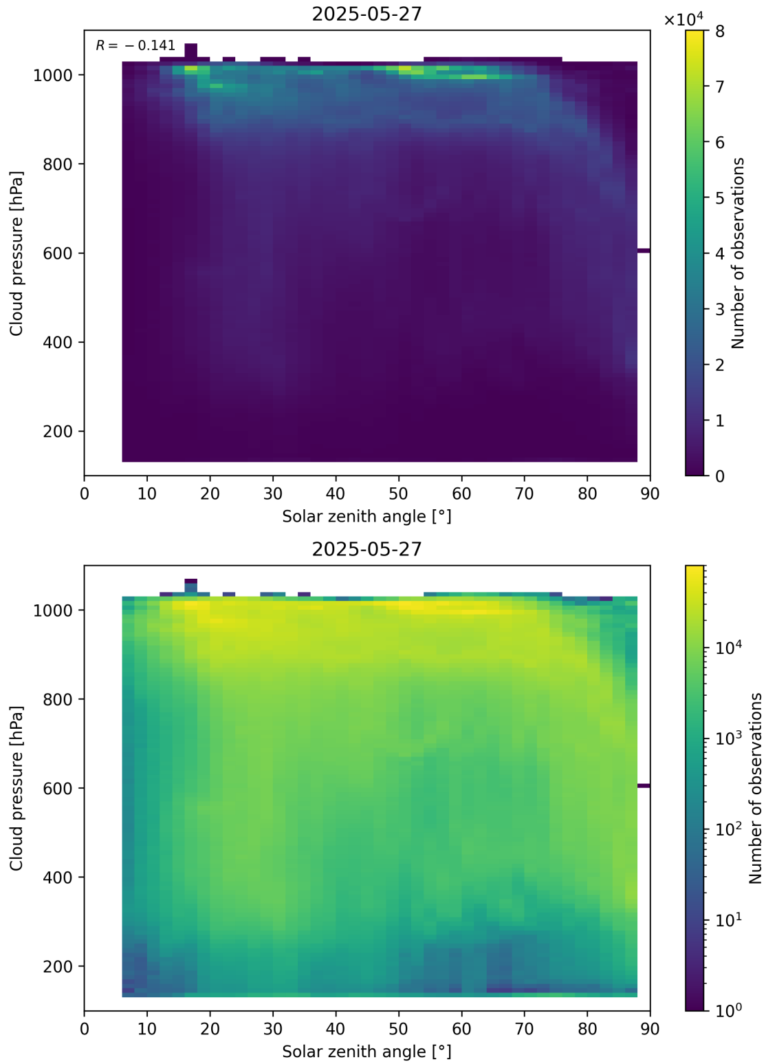
Figure 111: Scatter density plot of “Solar zenith angle” against “Cloud pressure” for 2025-05-26 to 2025-05-28.
