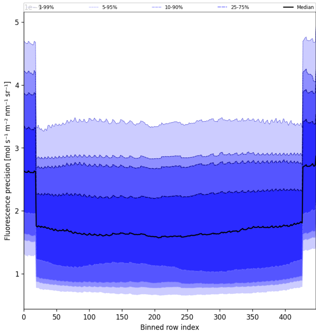
Figure 58: Along track statistics of “Fluorescence precision” for 2025-05-26 to 2025-05-28
