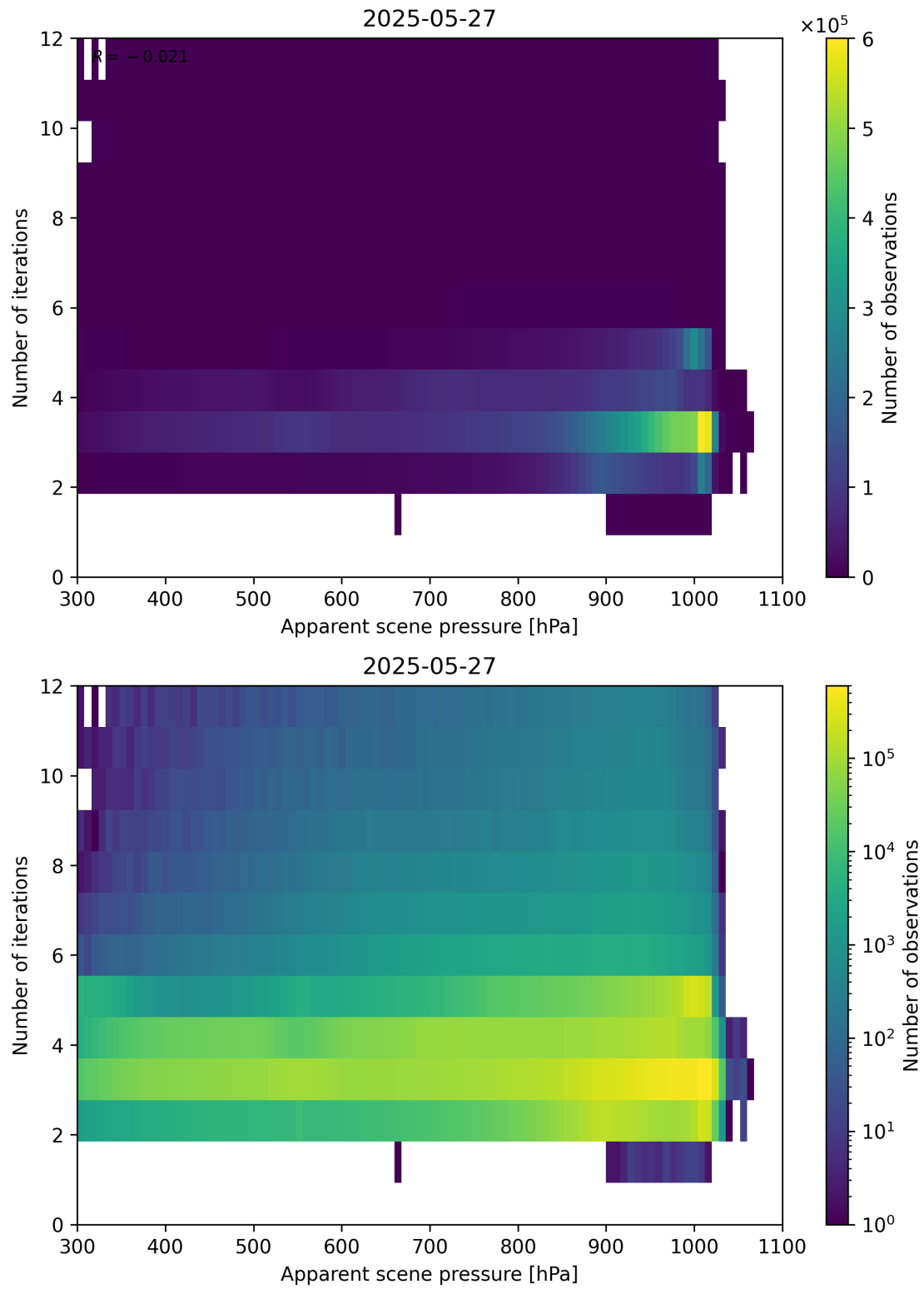
Figure 65: Scatter density plot of “Apparent scene pressure” against “Number of iterations” for 2025-05-26 to 2025-05-28.
