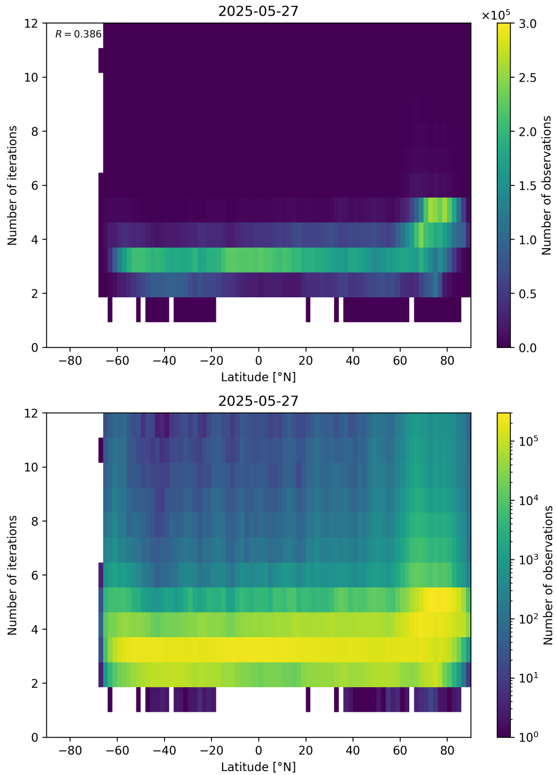
Figure 93: Scatter density plot of “Latitude” against “Number of iterations” for 2025-05-26 to 2025-05-28.
