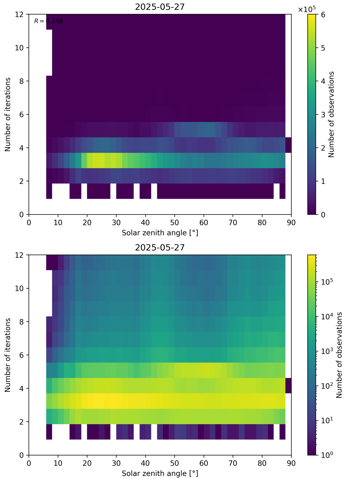
Figure 114: Scatter density plot of “Solar zenith angle” against “Number of iterations” for 2025-05-26 to 2025-05-28.
