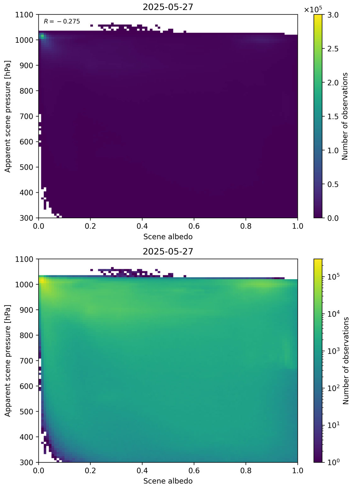
Figure 102: Scatter density plot of “Scene albedo” against “Apparent scene pressure” for 2025-05-26 to 2025-05-28.
