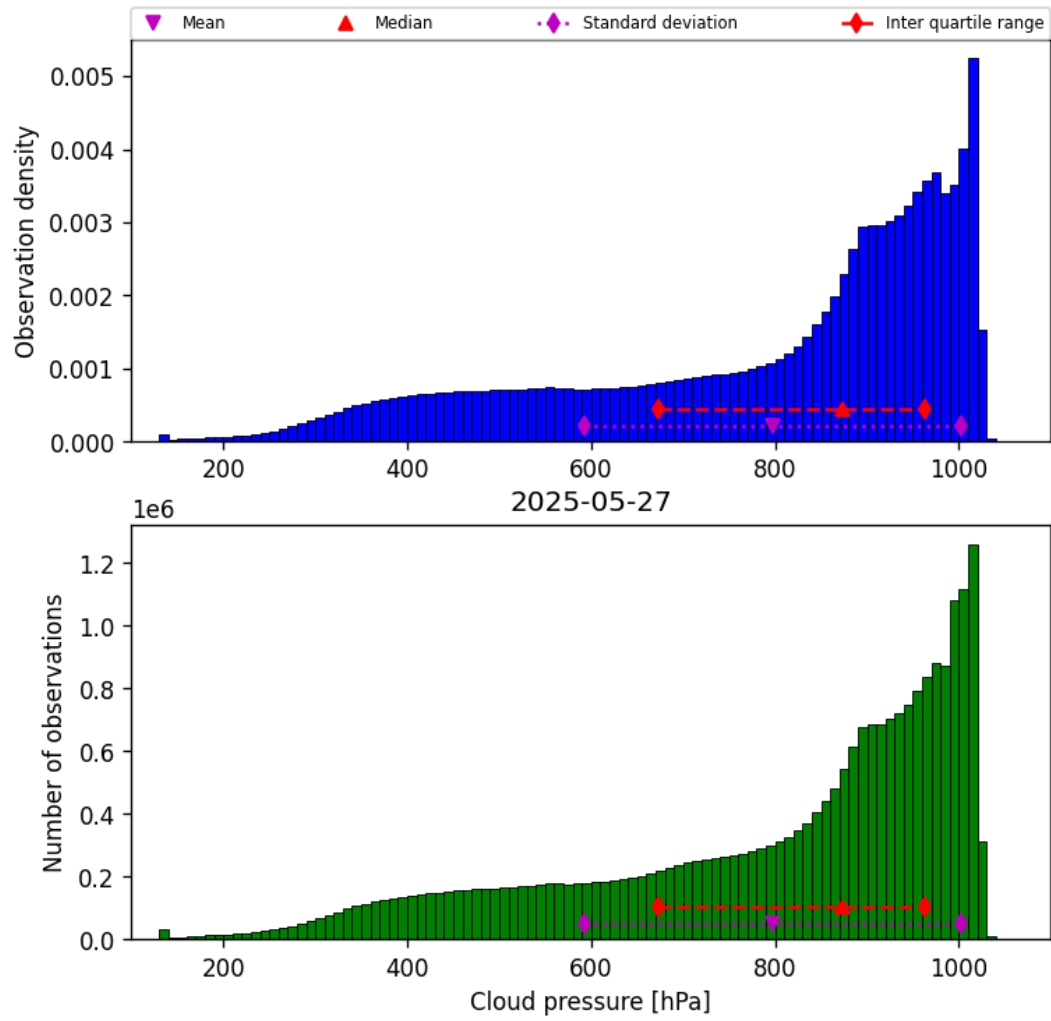
Figure 30: Histogram of “Cloud pressure” for 2025-05-26 to 2025-05-28
