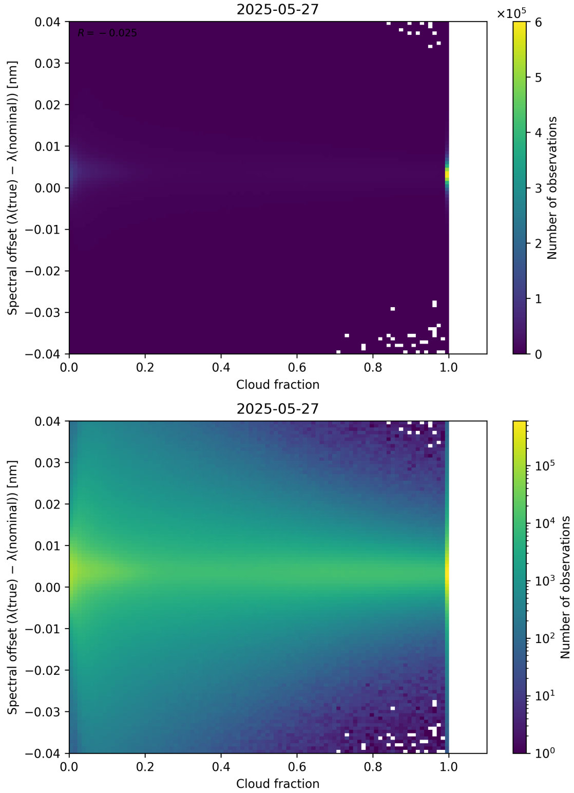
Figure 76: Scatter density plot of “Cloud fraction” against “Spectral offset ( \lambda_{\text{true}} - \lambda_{\text{nominal}} )” for 2025-05-26 to 2025-05-28.
