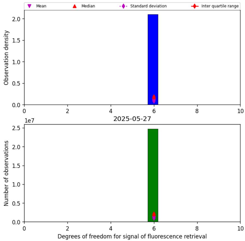
Figure 43: Histogram of "Degrees of freedom for signal of fluorescence retrieval" for 2025-05-26 to 2025-05-28
