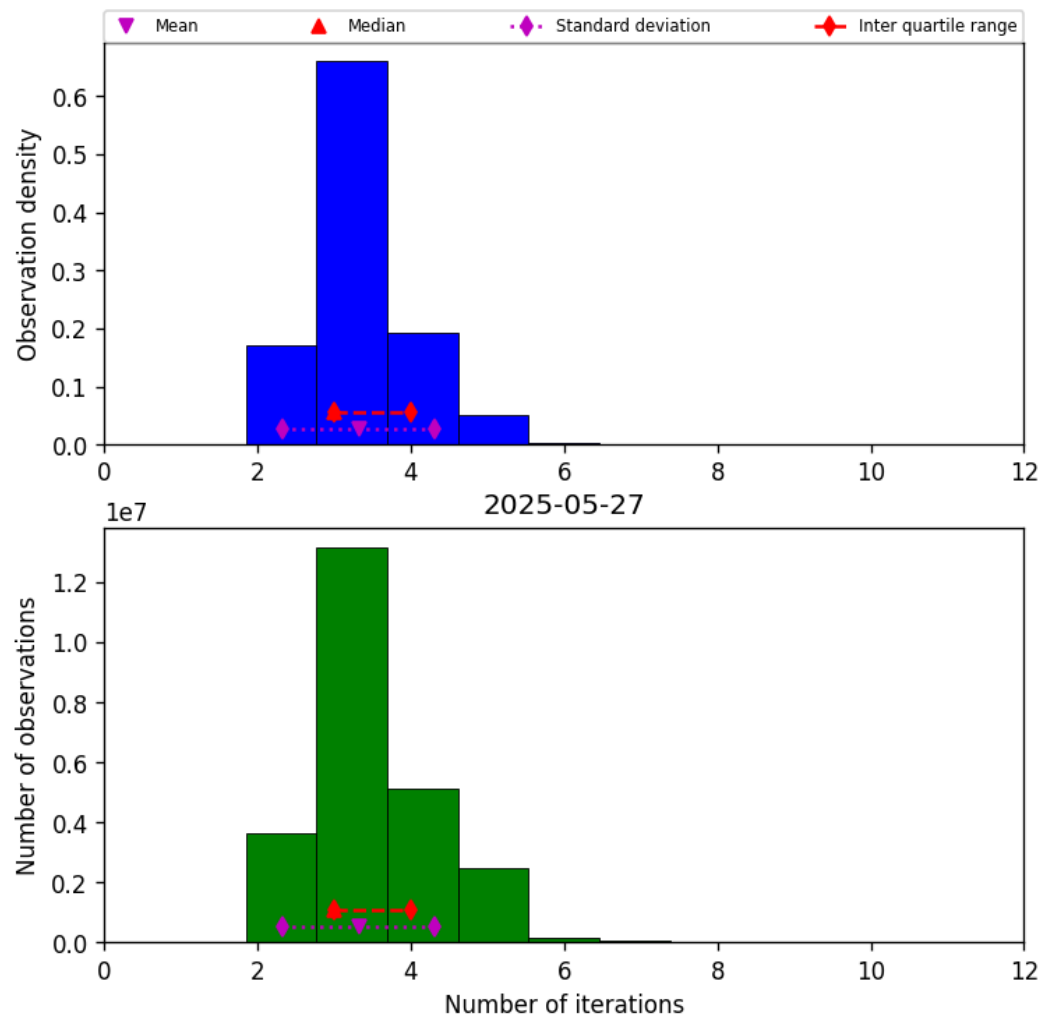
Figure 39: Histogram of “Number of iterations” for 2025-05-26 to 2025-05-28
