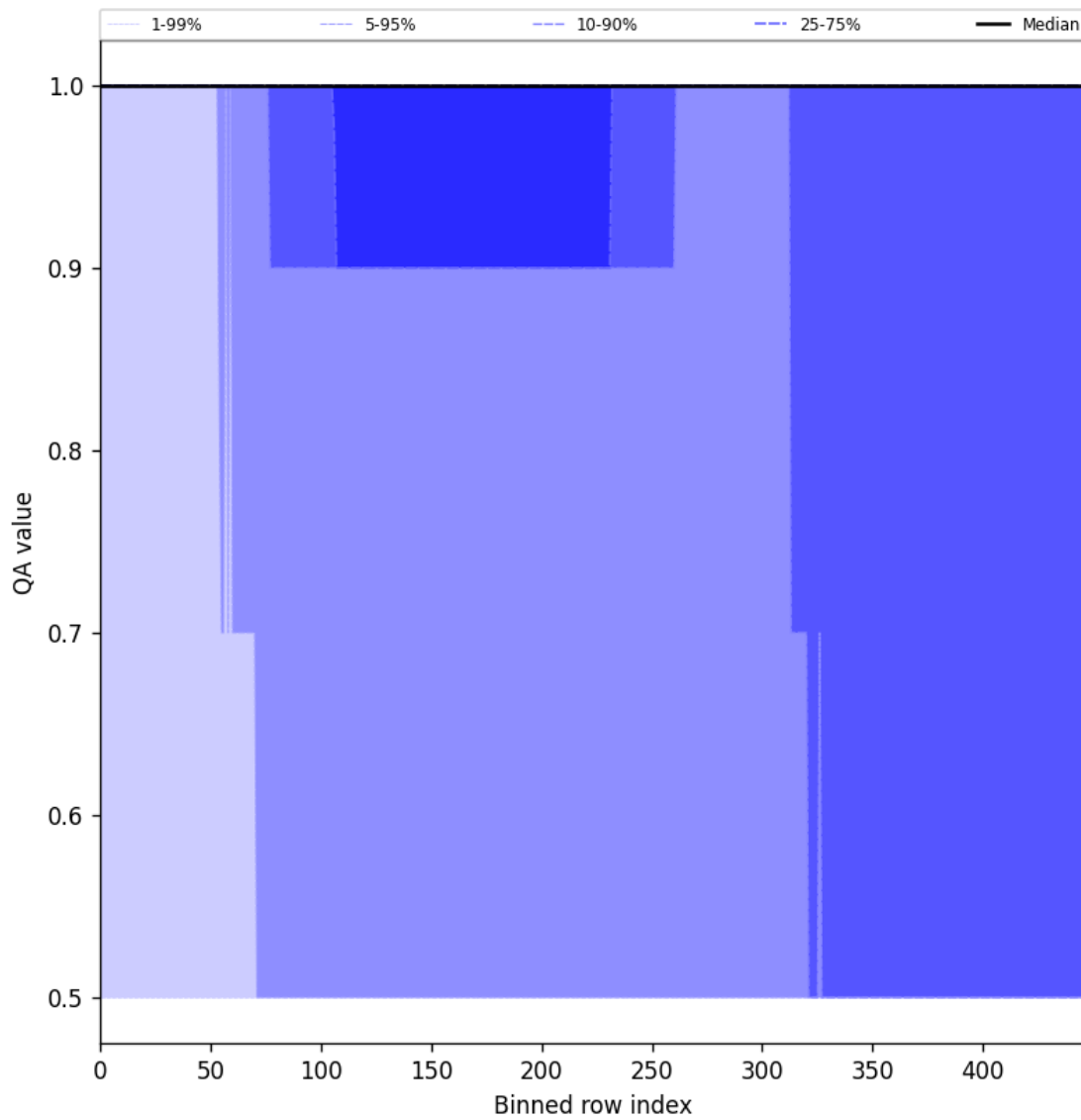
Figure 46: Along track statistics of “QA value” for 2025-05-26 to 2025-05-28
