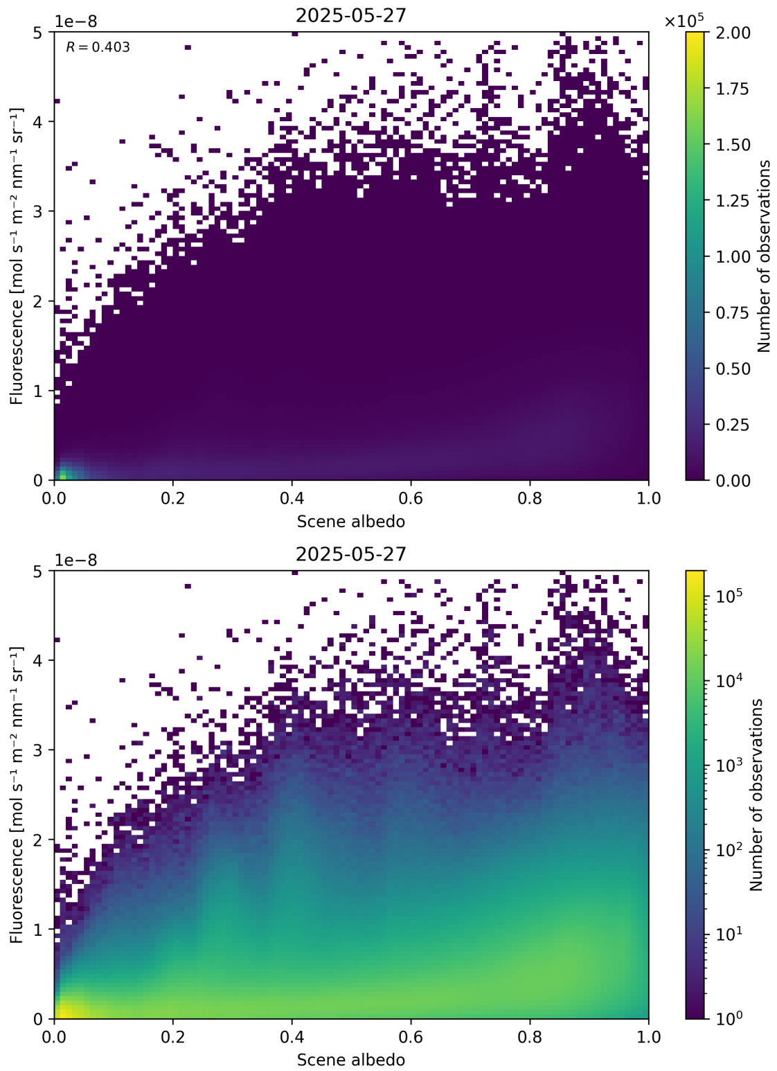
Figure 104: Scatter density plot of “Scene albedo” against “Fluorescence” for 2025-05-26 to 2025-05-28.
