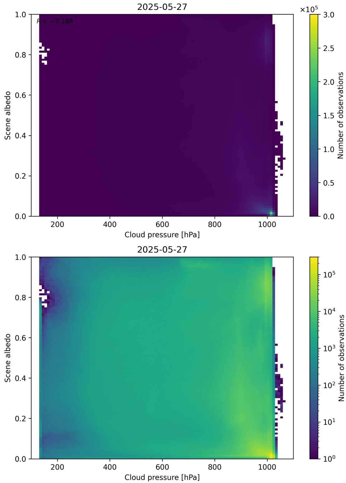
Figure 83: Scatter density plot of “Cloud pressure” against “Scene albedo” for 2025-05-26 to 2025-05-28.
