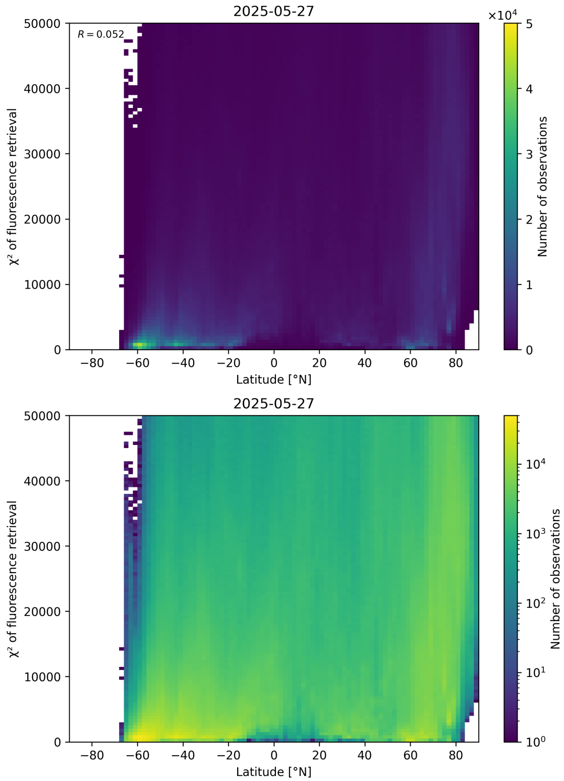
Figure 89: Scatter density plot of “Latitude” against “ \chi^2 of fluorescence retrieval” for 2025-05-26 to 2025-05-28.
