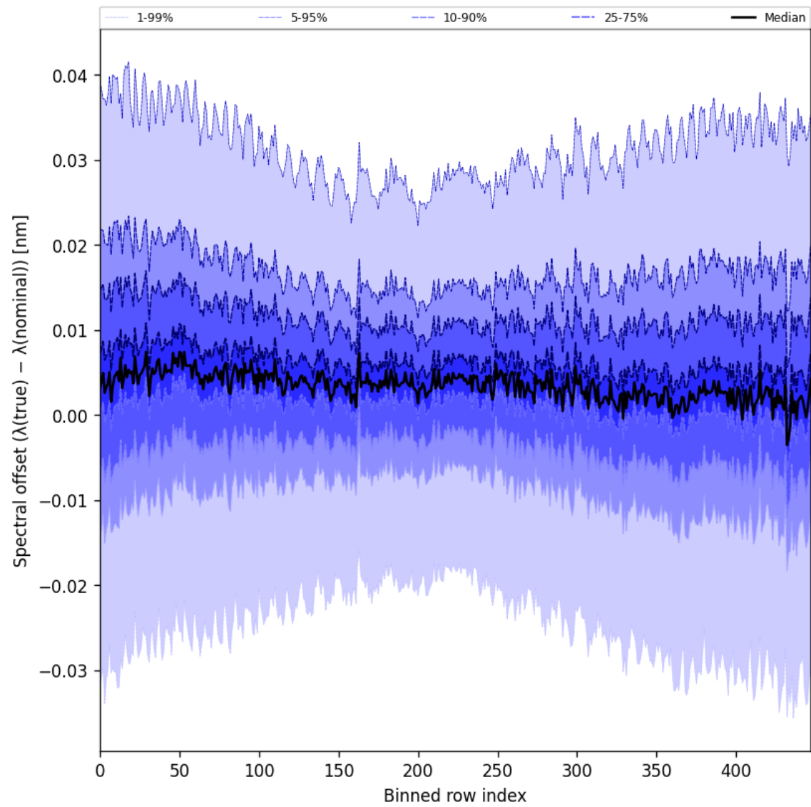
Figure 62: Along track statistics of “Spectral offset ( \lambda_{\text{true}} - \lambda_{\text{nominal}} )” for 2025-05-26 to 2025-05-28
