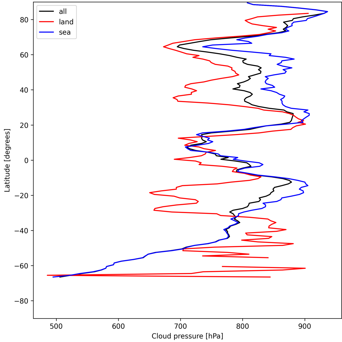
Figure 13: Zonal average of “Cloud pressure” for 2025-05-26 to 2025-05-28.
