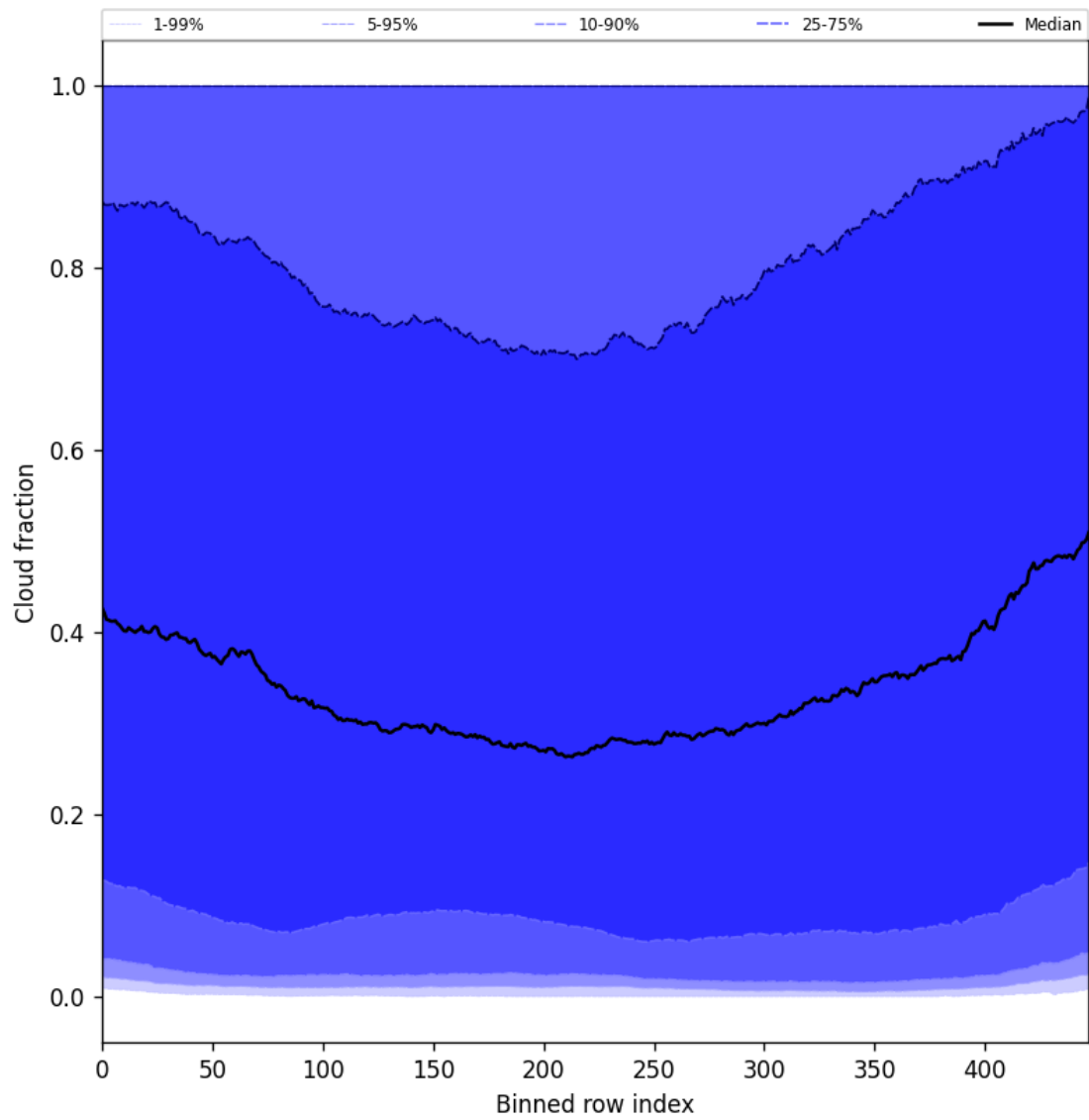
Figure 49: Along track statistics of “Cloud fraction” for 2025-05-26 to 2025-05-28
