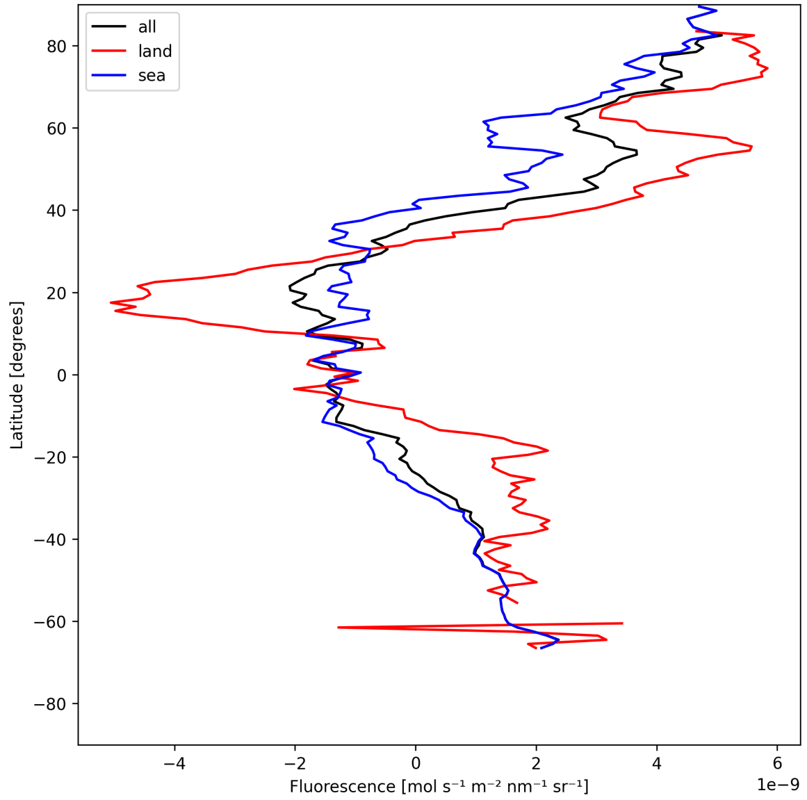
Figure 23: Zonal average of “Fluorescence” for 2025-05-26 to 2025-05-28.
