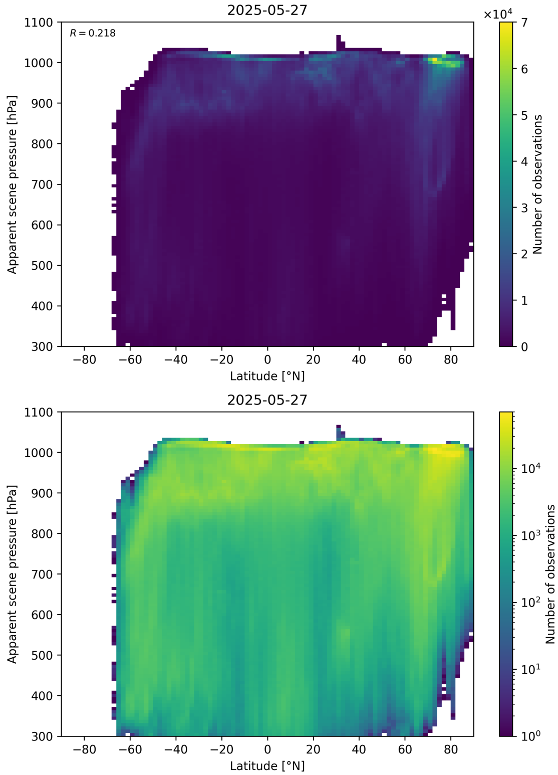
Figure 88: Scatter density plot of “Latitude” against “Apparent scene pressure” for 2025-05-26 to 2025-05-28.
