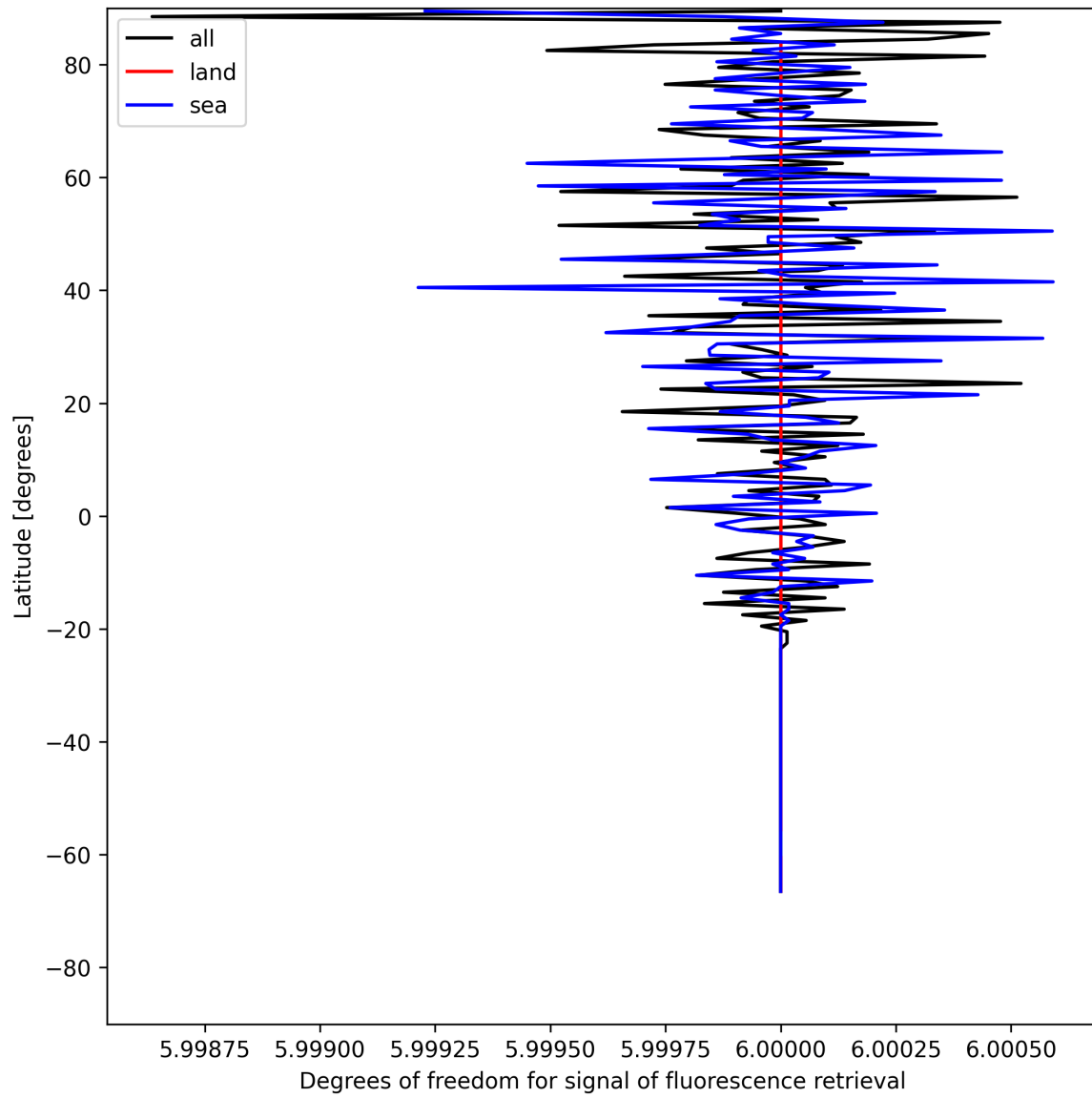
Figure 26: Zonal average of “Degrees of freedom for signal of fluorescence retrieval” for 2025-05-26 to 2025-05-28.
