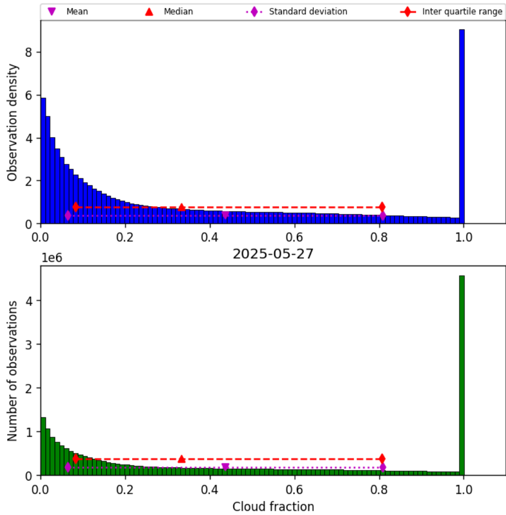
Figure 32: Histogram of “Cloud fraction” for 2025-05-26 to 2025-05-28
