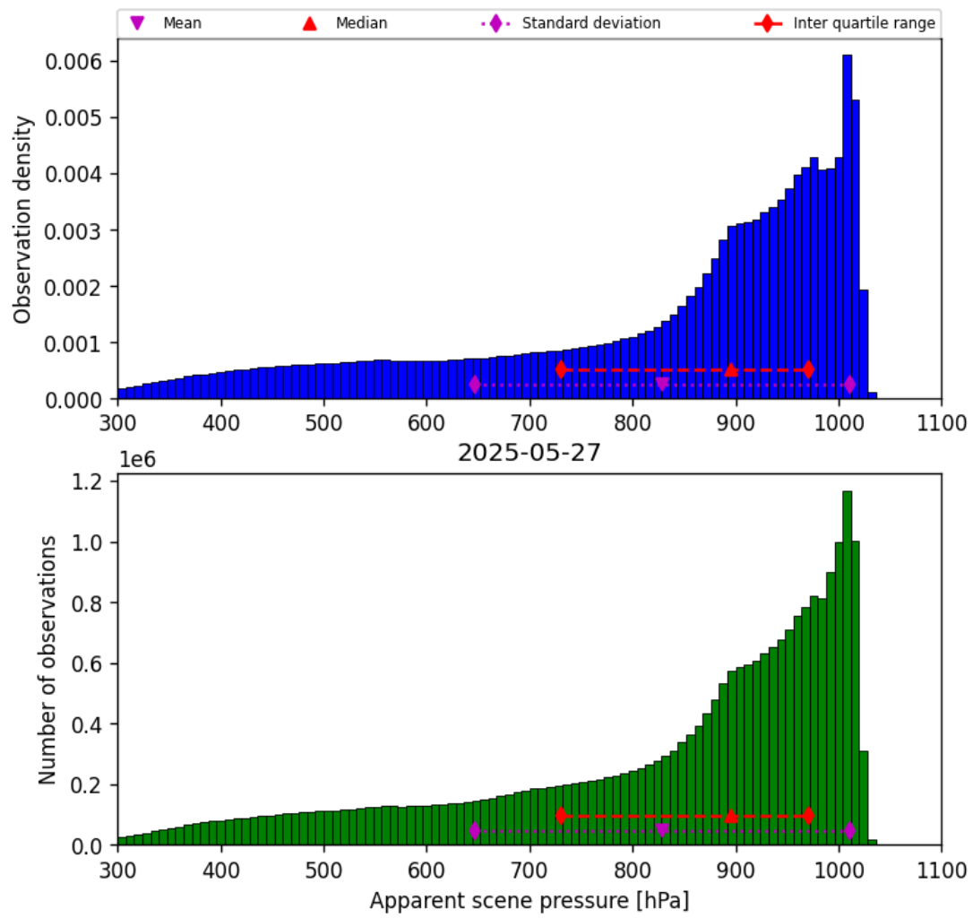
Figure 36: Histogram of “Apparent scene pressure” for 2025-05-26 to 2025-05-28
