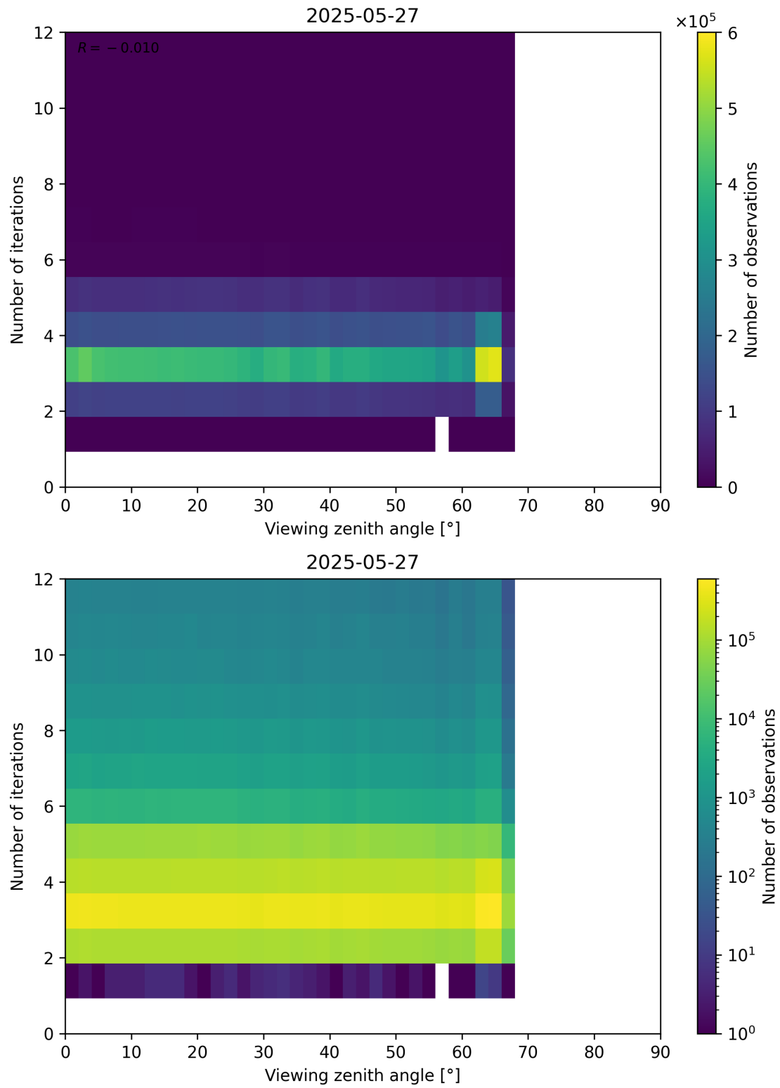
Figure 124: Scatter density plot of “Viewing zenith angle” against “Number of iterations” for 2025-05-26 to 2025-05-28.
