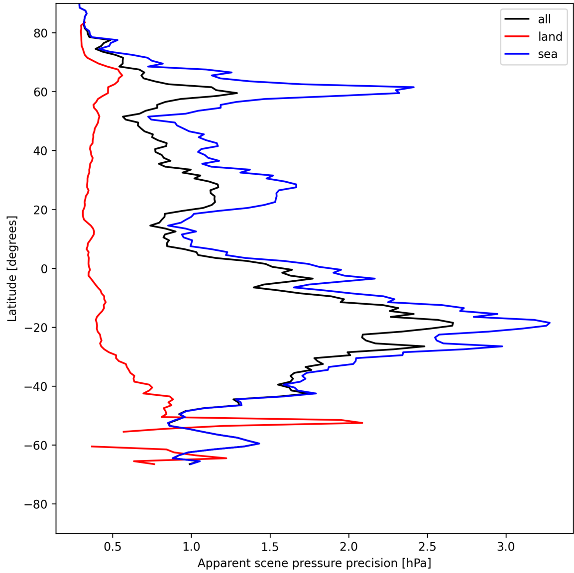
Figure 20: Zonal average of “Apparent scene pressure precision” for 2025-05-26 to 2025-05-28.
