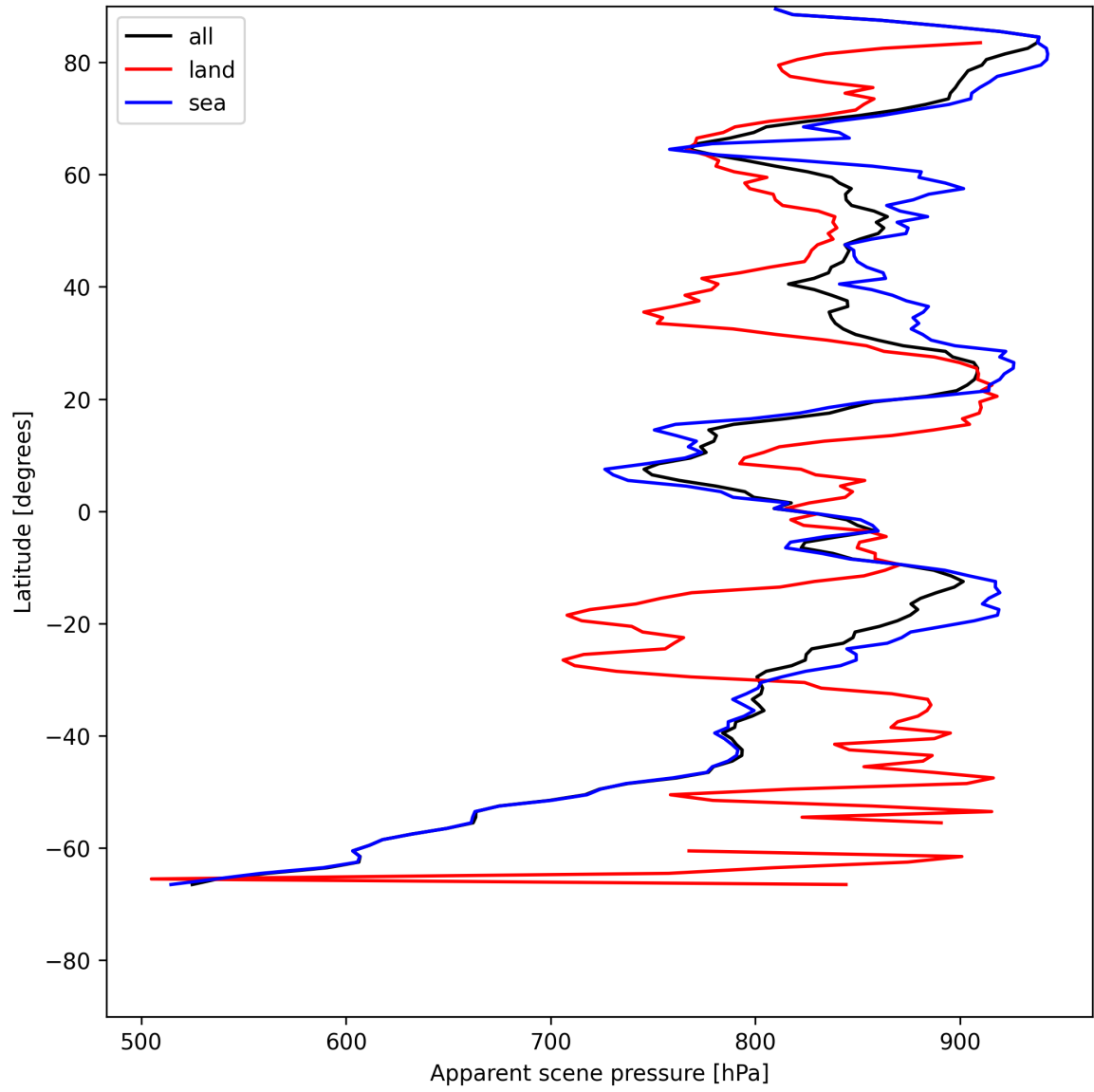
Figure 19: Zonal average of “Apparent scene pressure” for 2025-05-26 to 2025-05-28.
