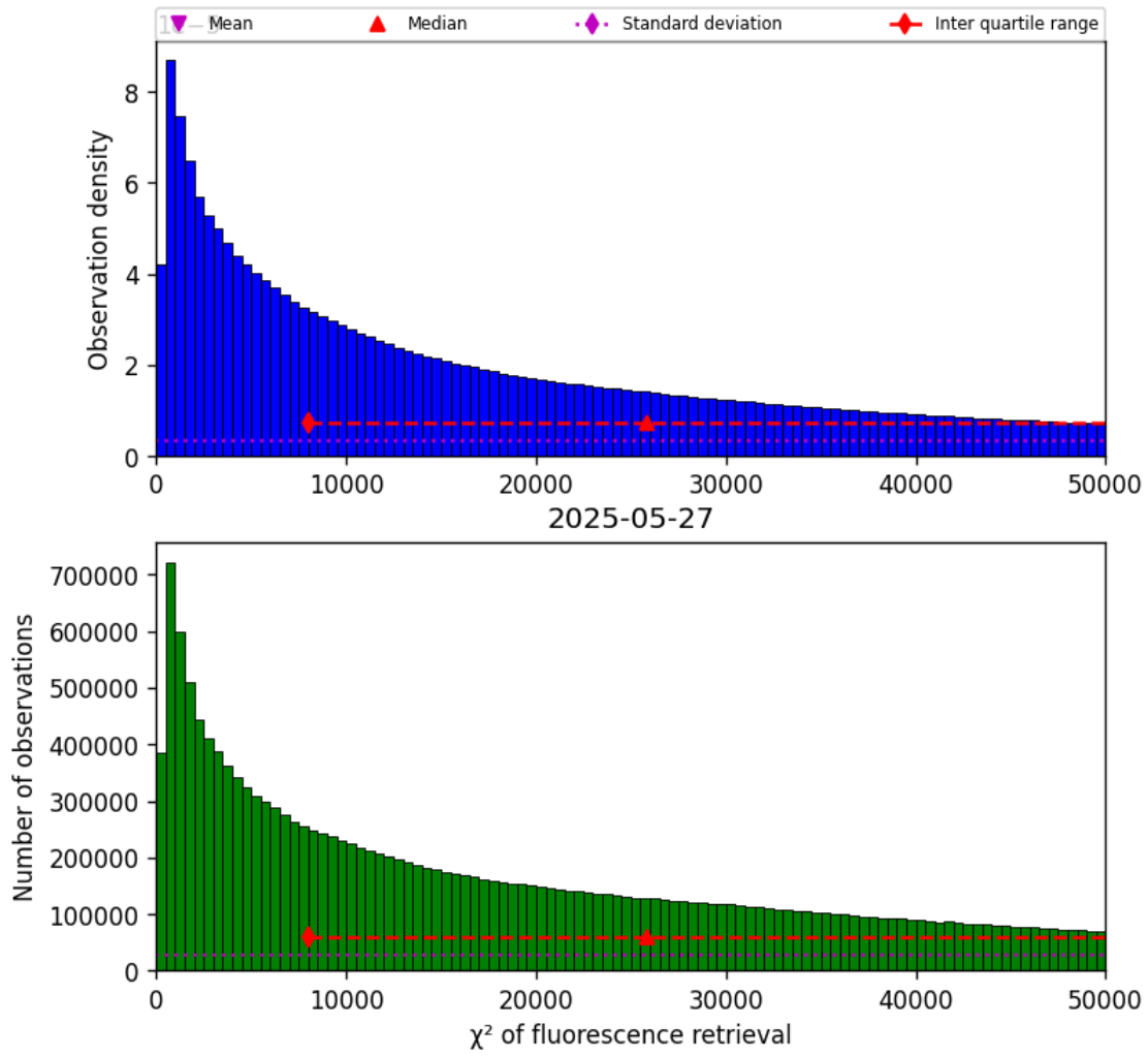
Figure 42: Histogram of “ \chi^2 of fluorescence retrieval” for 2025-05-26 to 2025-05-28
