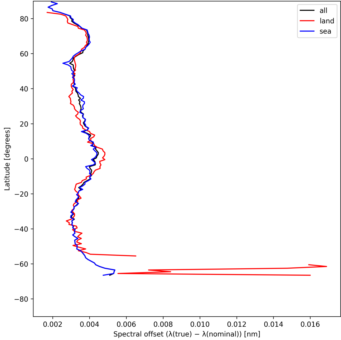
Figure 28: Zonal average of “Spectral offset ( \lambda_{\text{true}} - \lambda_{\text{nominal}} )” for 2025-05-26 to 2025-05-28.
