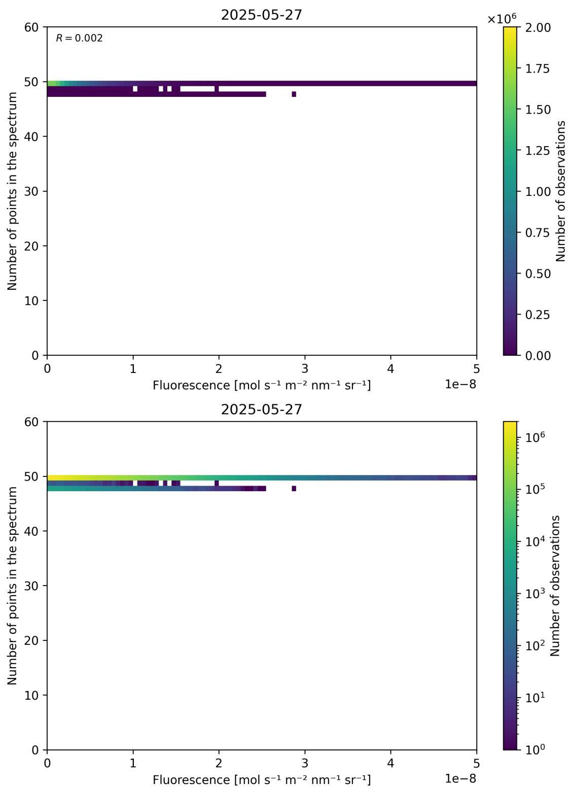
Figure 86: Scatter density plot of “Fluorescence” against “Number of points in the spectrum” for 2025-05-26 to 2025-05-28.
