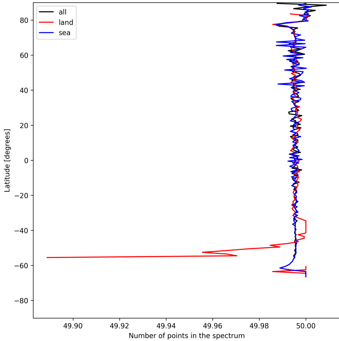
Figure 27: Zonal average of “Number of points in the spectrum” for 2025-05-26 to 2025-05-28.
