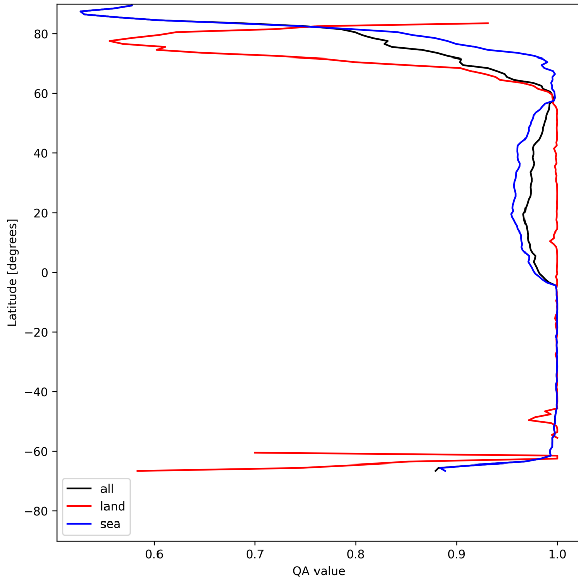
Figure 12: Zonal average of “QA value” for 2025-05-26 to 2025-05-28.
