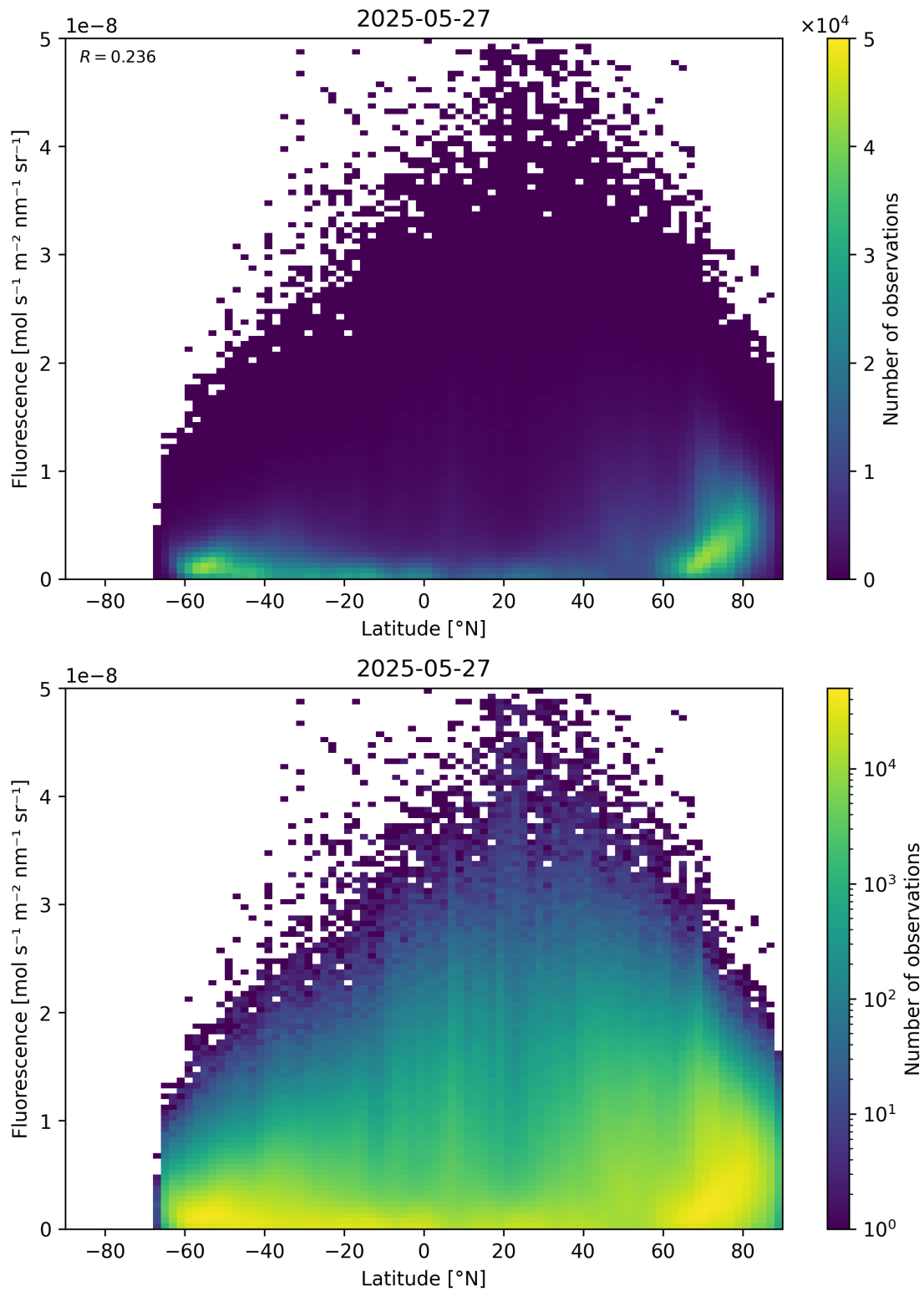
Figure 92: Scatter density plot of “Latitude” against “Fluorescence” for 2025-05-26 to 2025-05-28.
