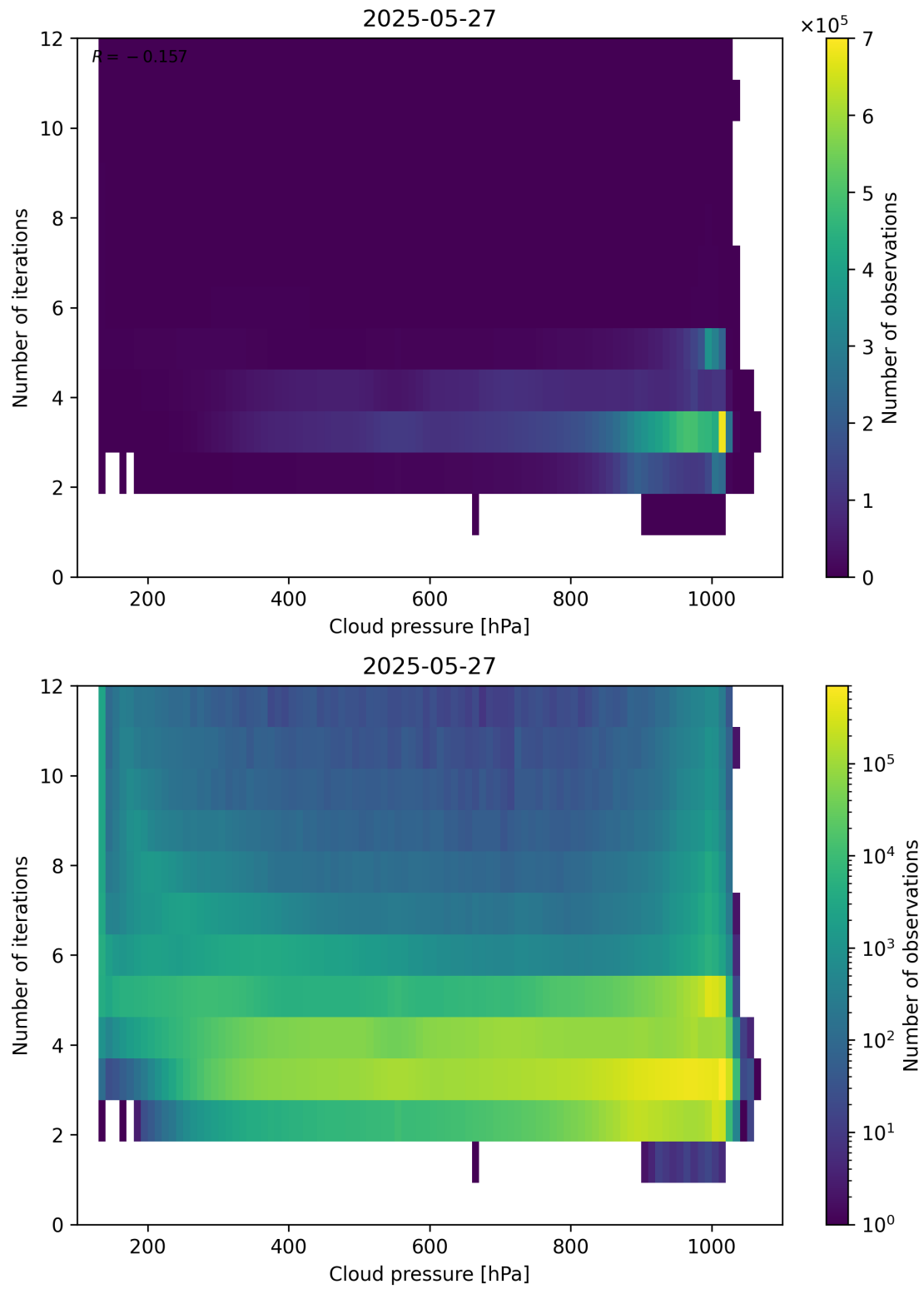
Figure 81: Scatter density plot of “Cloud pressure” against “Number of iterations” for 2025-05-26 to 2025-05-28.
