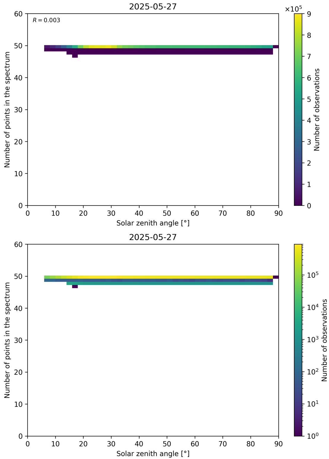
Figure 115: Scatter density plot of “Solar zenith angle” against “Number of points in the spectrum” for 2025-05-26 to 2025-05-28.
