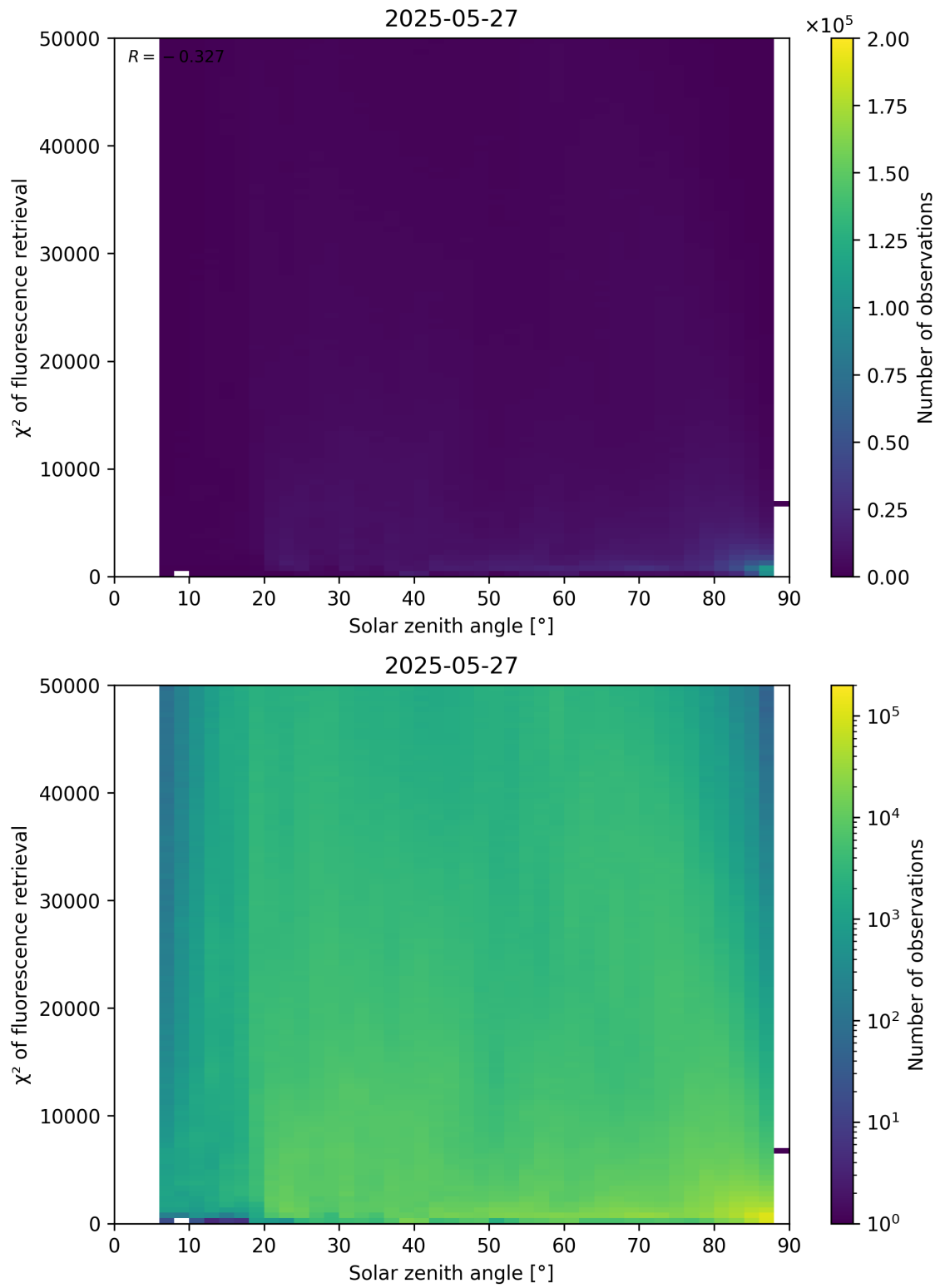
Figure 109: Scatter density plot of “Solar zenith angle” against “ \chi^2 of fluorescence retrieval” for 2025-05-26 to 2025-05-28.
