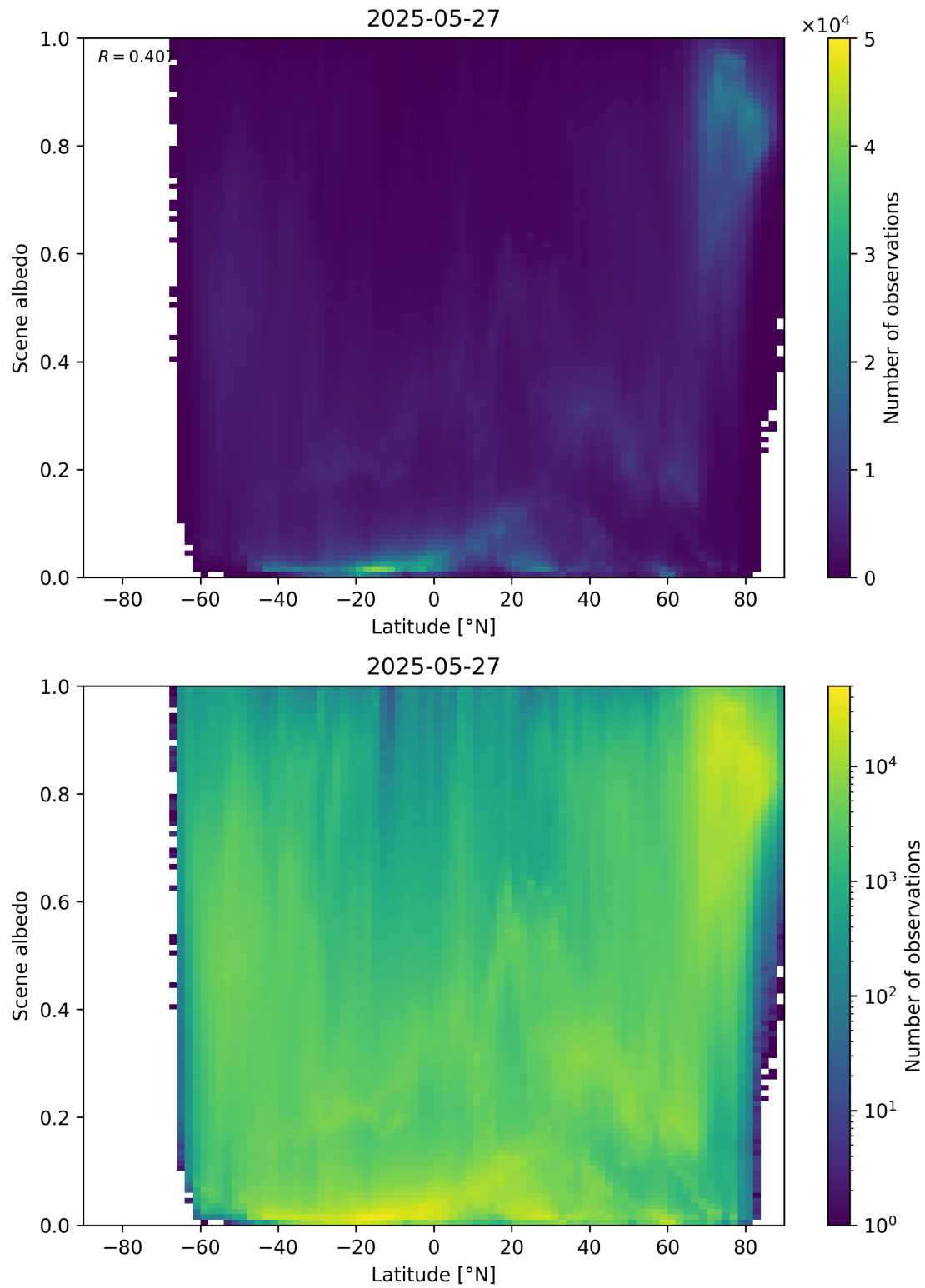
Figure 95: Scatter density plot of “Latitude” against “Scene albedo” for 2025-05-26 to 2025-05-28.
