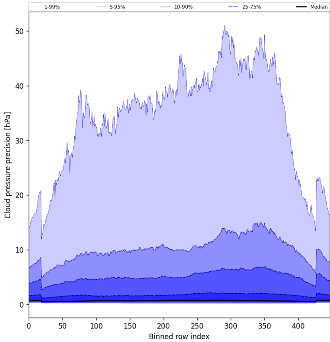
Figure 48: Along track statistics of “Cloud pressure precision” for 2025-05-26 to 2025-05-28
