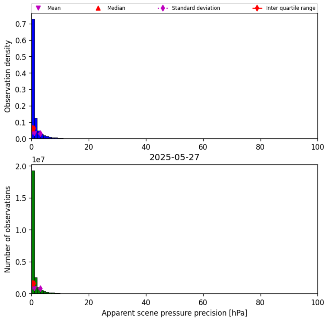
Figure 37: Histogram of “Apparent scene pressure precision” for 2025-05-26 to 2025-05-28
