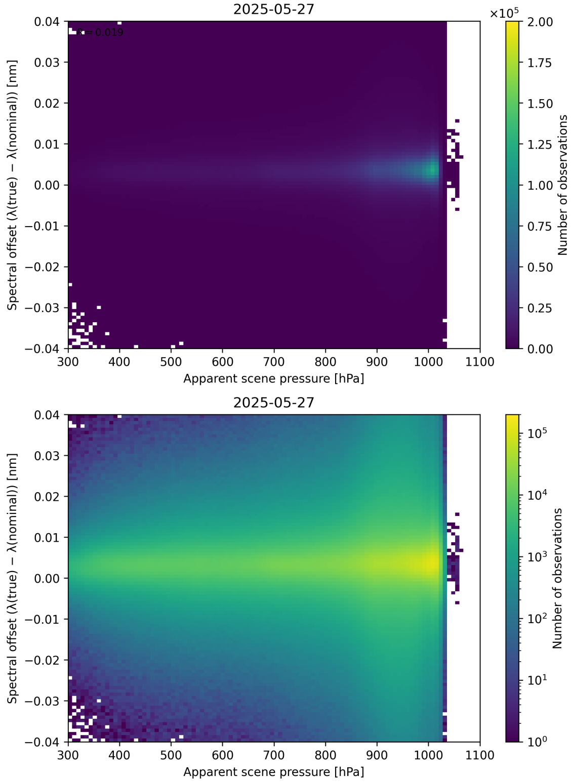
Figure 67: Scatter density plot of “Apparent scene pressure” against “Spectral offset ( \lambda_{\text{true}} - \lambda_{\text{nominal}} )” for 2025-05-26 to 2025-05-28.
