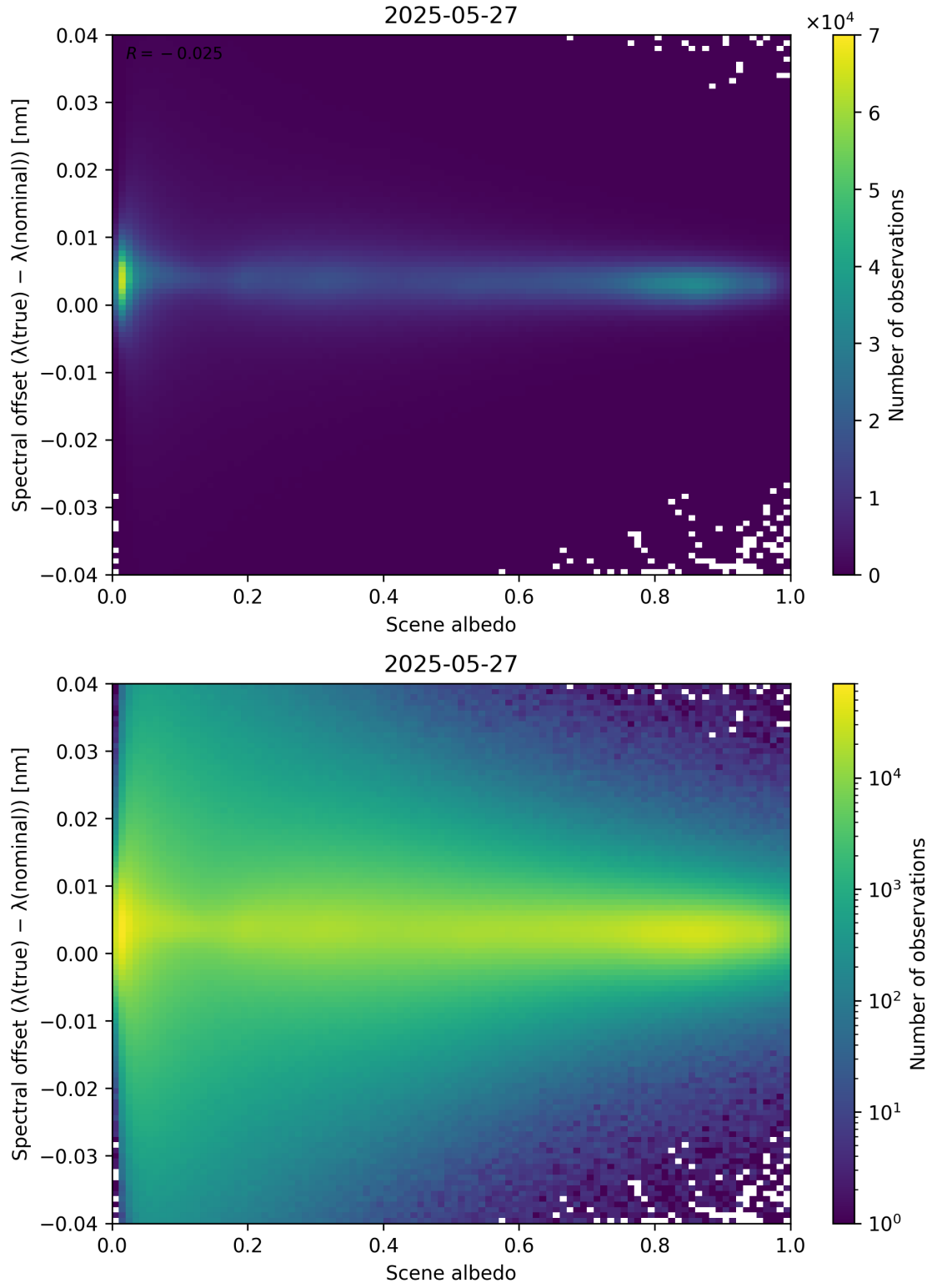
Figure 107: Scatter density plot of “Scene albedo” against “Spectral offset ( \lambda_{\text{true}} - \lambda_{\text{nominal}} )” for 2025-05-26 to 2025-05-28.
