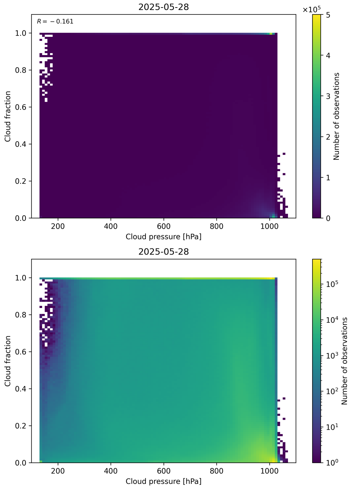
Figure 79: Scatter density plot of “Cloud pressure” against “Cloud fraction” for 2025-05-27 to 2025-05-29.
