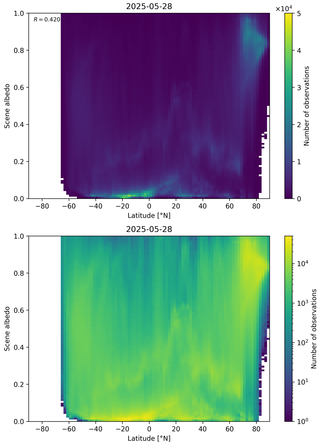
Figure 95: Scatter density plot of “Latitude” against “Scene albedo” for 2025-05-27 to 2025-05-29.
