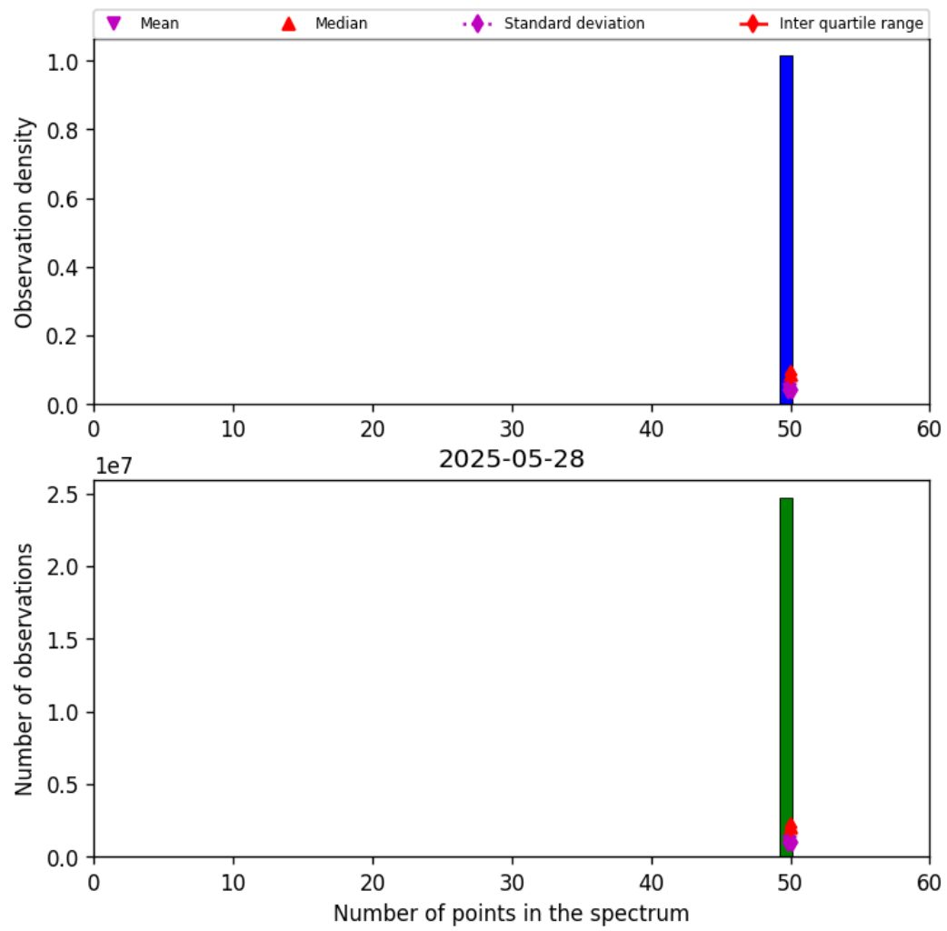
Figure 44: Histogram of “Number of points in the spectrum” for 2025-05-27 to 2025-05-29
