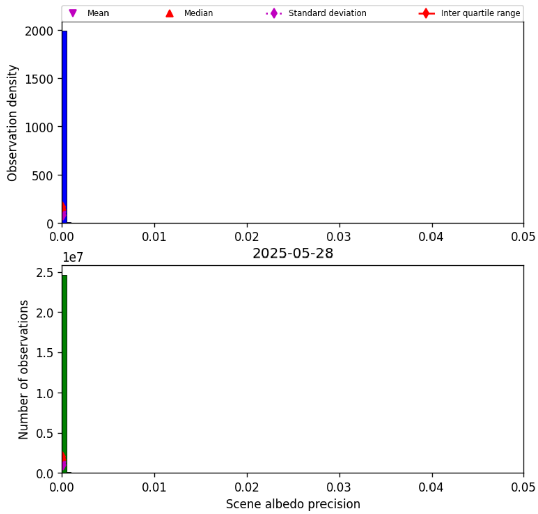
Figure 35: Histogram of “Scene albedo precision” for 2025-05-27 to 2025-05-29
