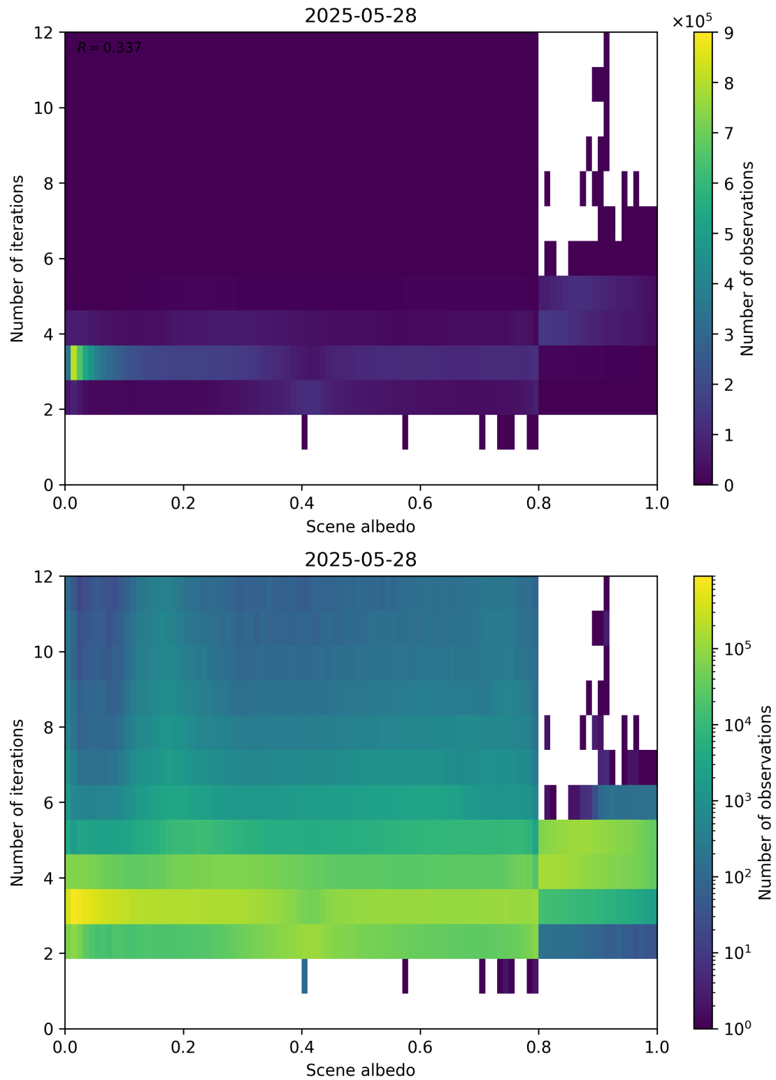
Figure 105: Scatter density plot of “Scene albedo” against “Number of iterations” for 2025-05-27 to 2025-05-29.
