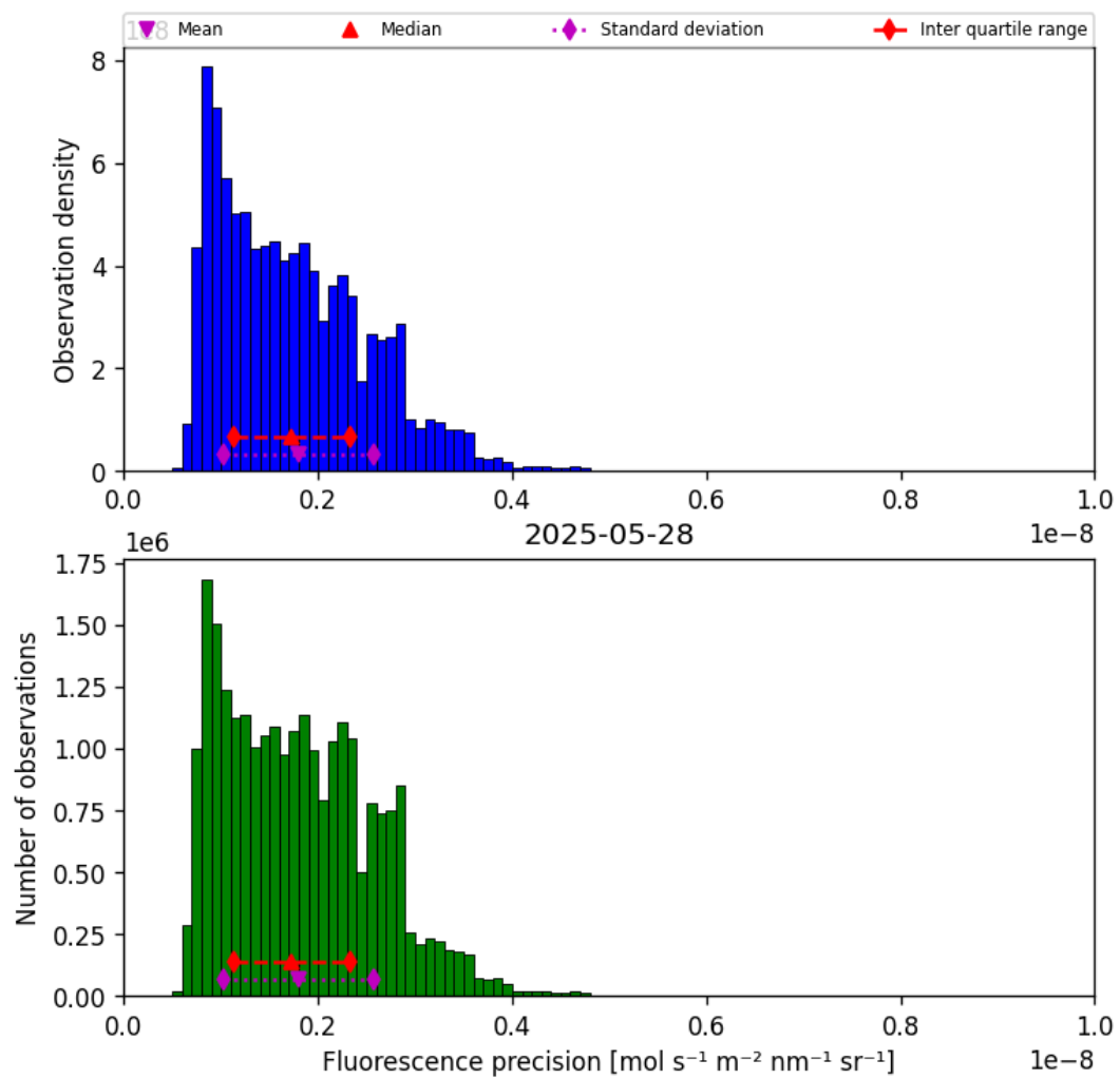
Figure 41: Histogram of “Fluorescence precision” for 2025-05-27 to 2025-05-29
