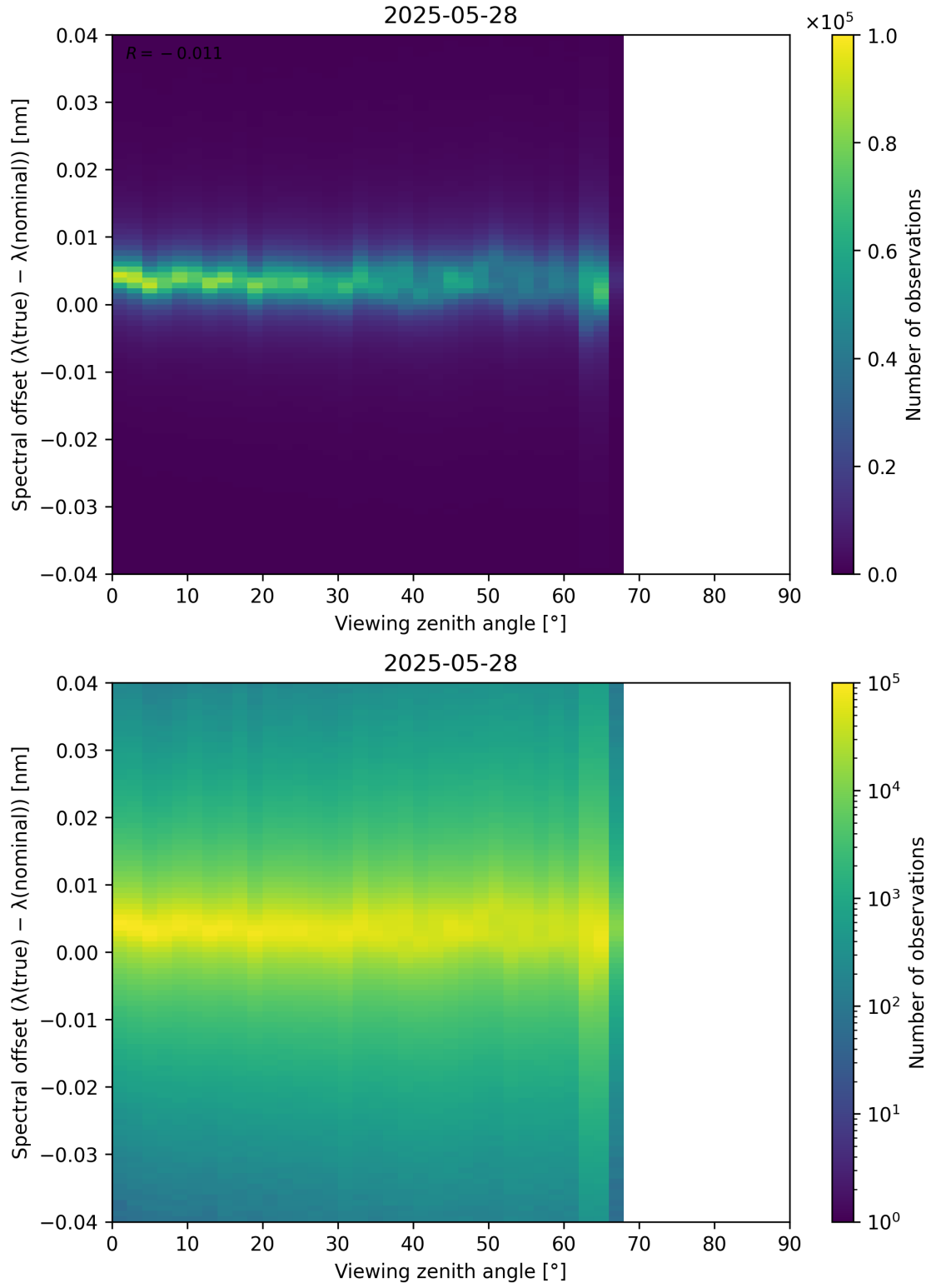
Figure 128: Scatter density plot of “Viewing zenith angle” against “Spectral offset ( \lambda_{\text{true}} - \lambda_{\text{nominal}} )” for 2025-05-27 to 2025-05-29.
