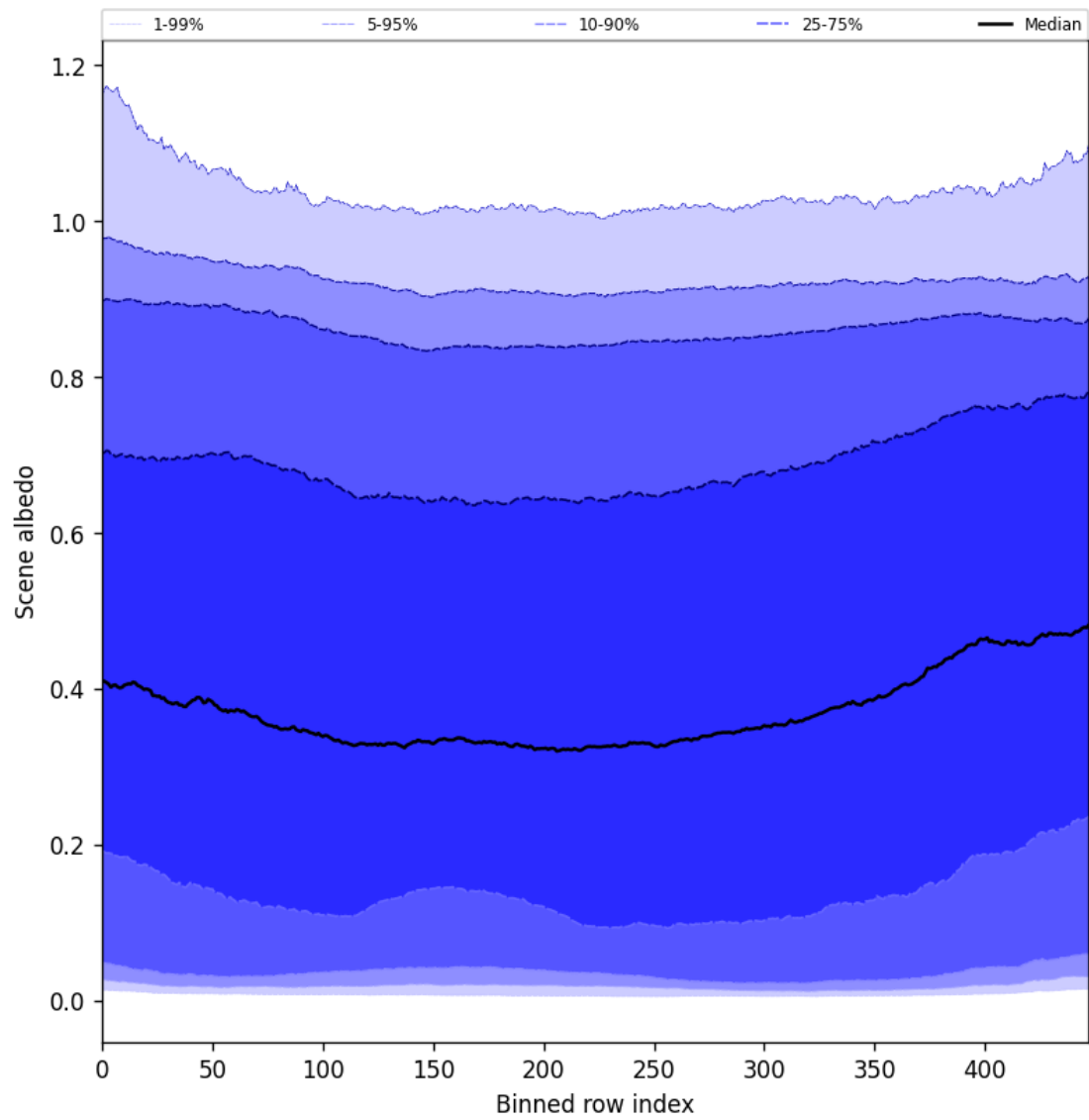
Figure 51: Along track statistics of “Scene albedo” for 2025-05-27 to 2025-05-29
