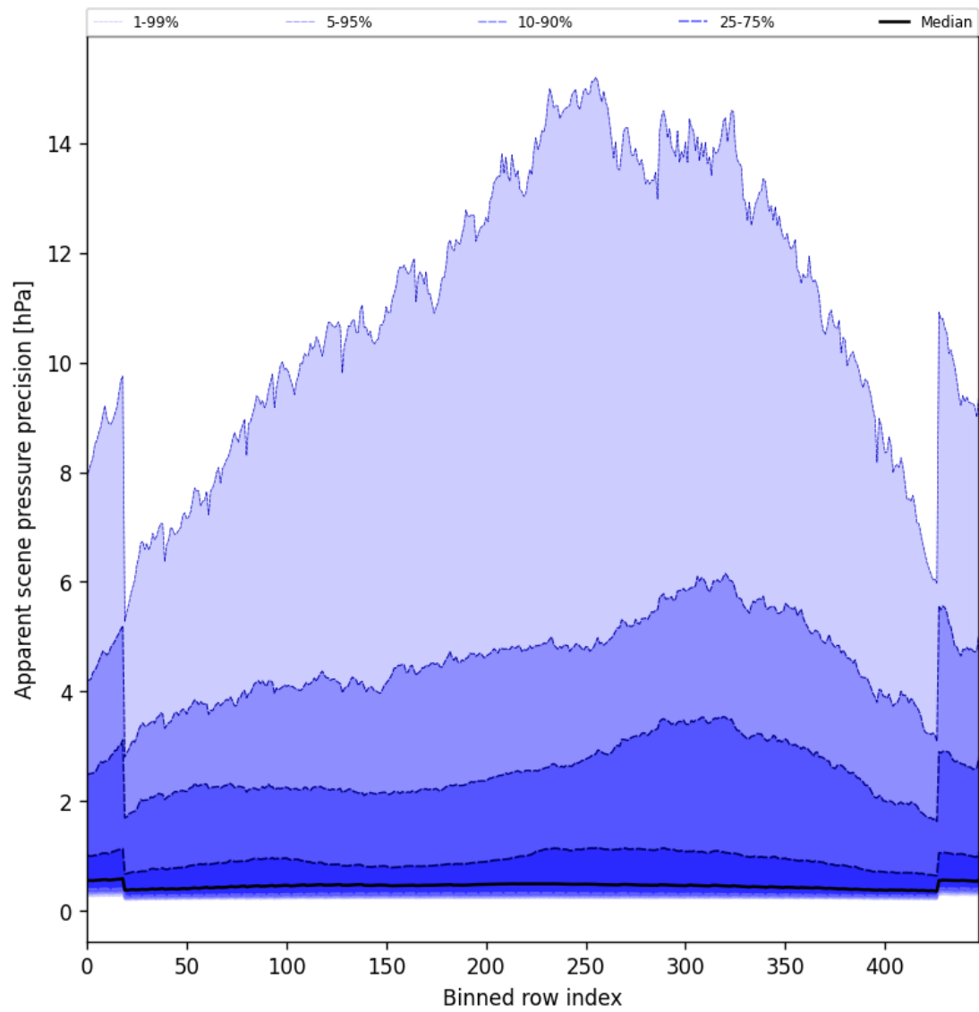
Figure 54: Along track statistics of “Apparent scene pressure precision” for 2025-05-27 to 2025-05-29
