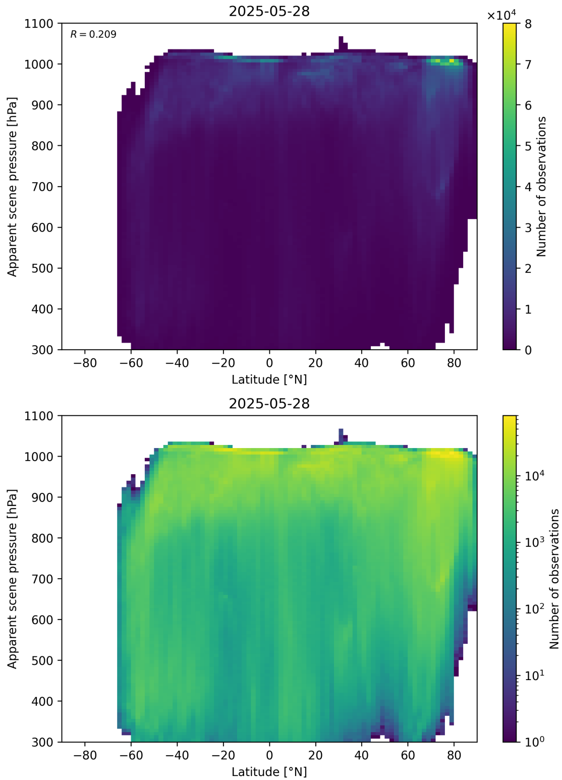
Figure 88: Scatter density plot of “Latitude” against “Apparent scene pressure” for 2025-05-27 to 2025-05-29.
