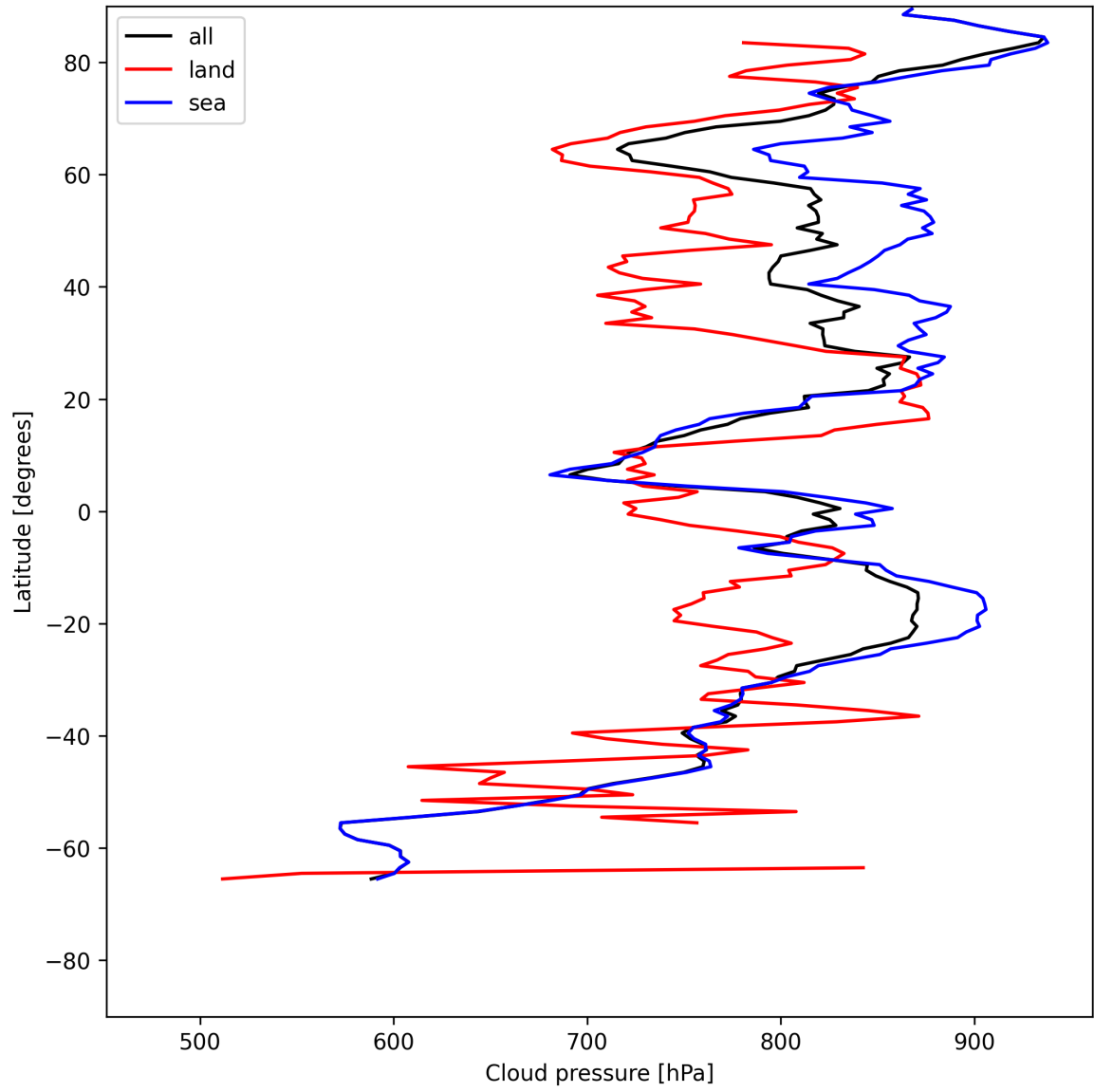
Figure 13: Zonal average of “Cloud pressure” for 2025-05-27 to 2025-05-29.
