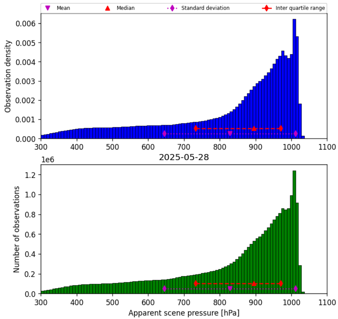
Figure 36: Histogram of “Apparent scene pressure” for 2025-05-27 to 2025-05-29
