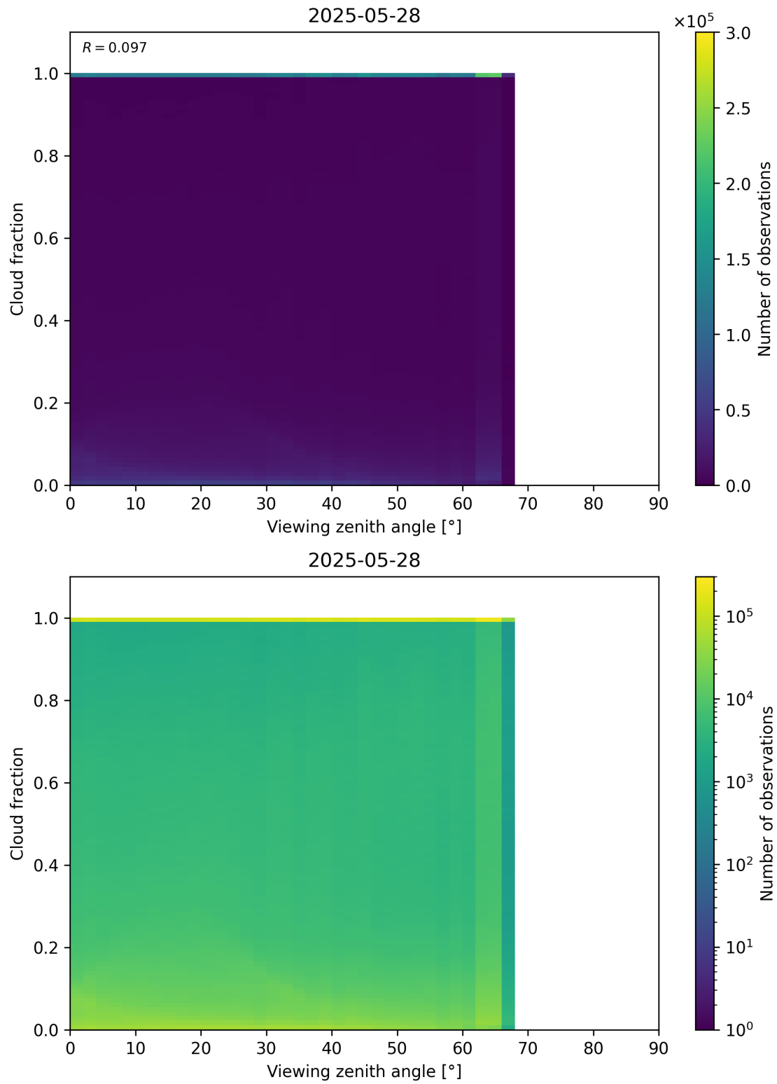
Figure 120: Scatter density plot of “Viewing zenith angle” against “Cloud fraction” for 2025-05-27 to 2025-05-29.
