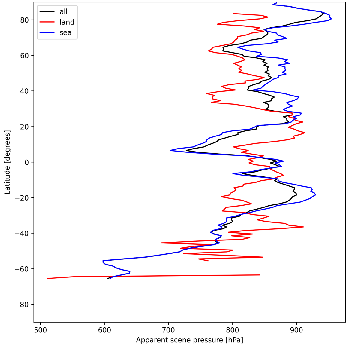
Figure 19: Zonal average of “Apparent scene pressure” for 2025-05-27 to 2025-05-29.
