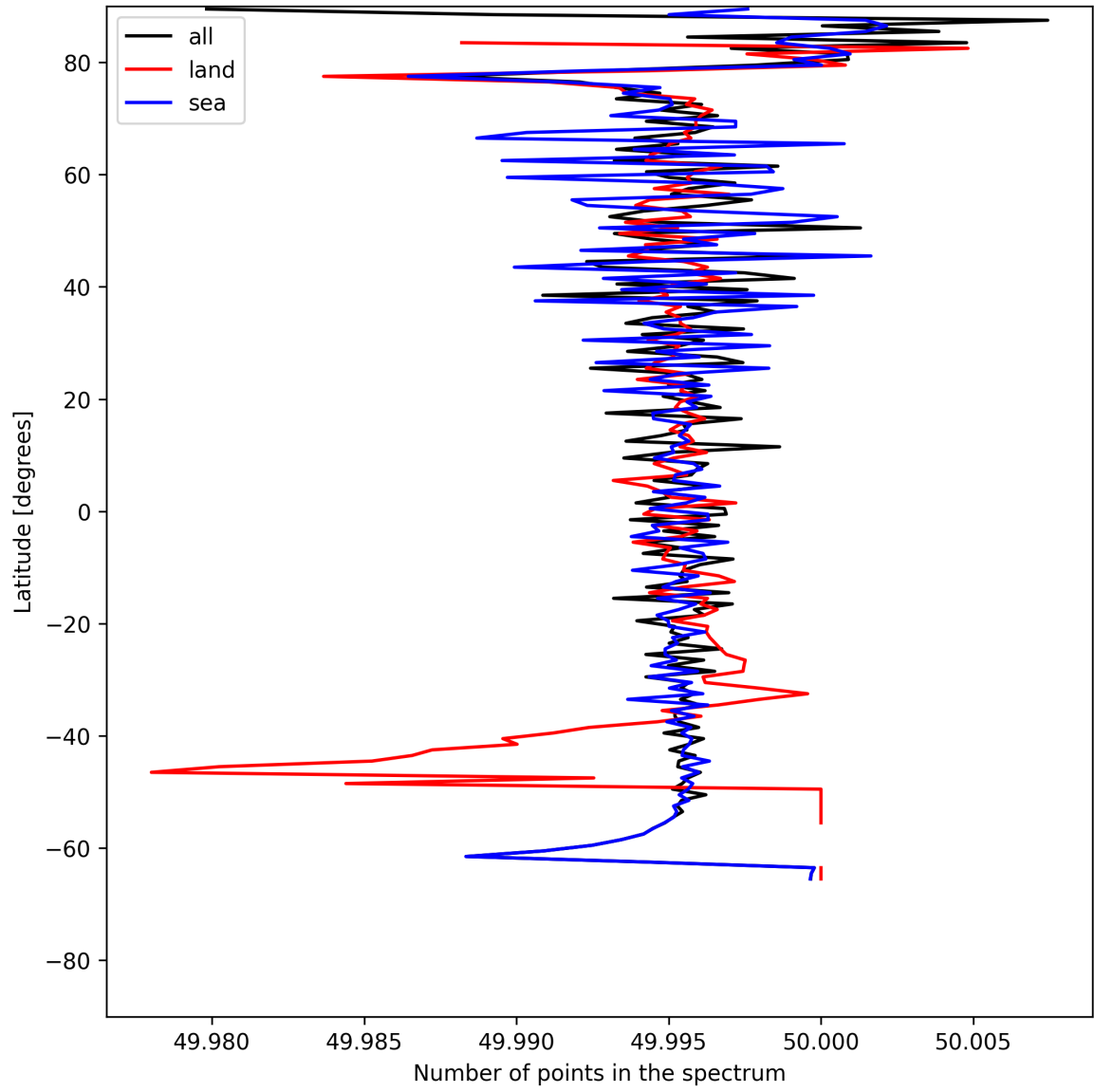
Figure 27: Zonal average of “Number of points in the spectrum” for 2025-05-27 to 2025-05-29.
