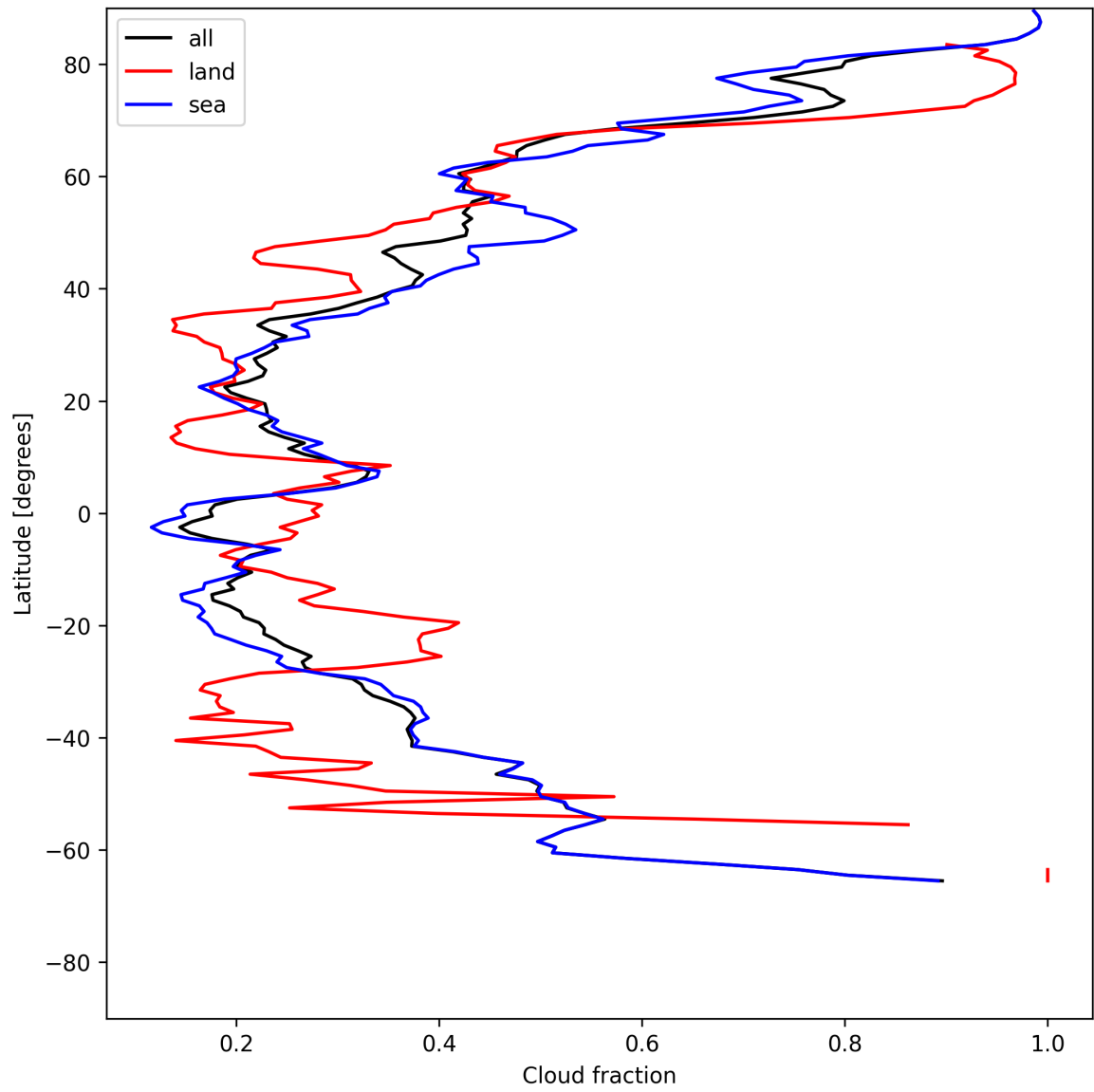
Figure 15: Zonal average of “Cloud fraction” for 2025-05-27 to 2025-05-29.
