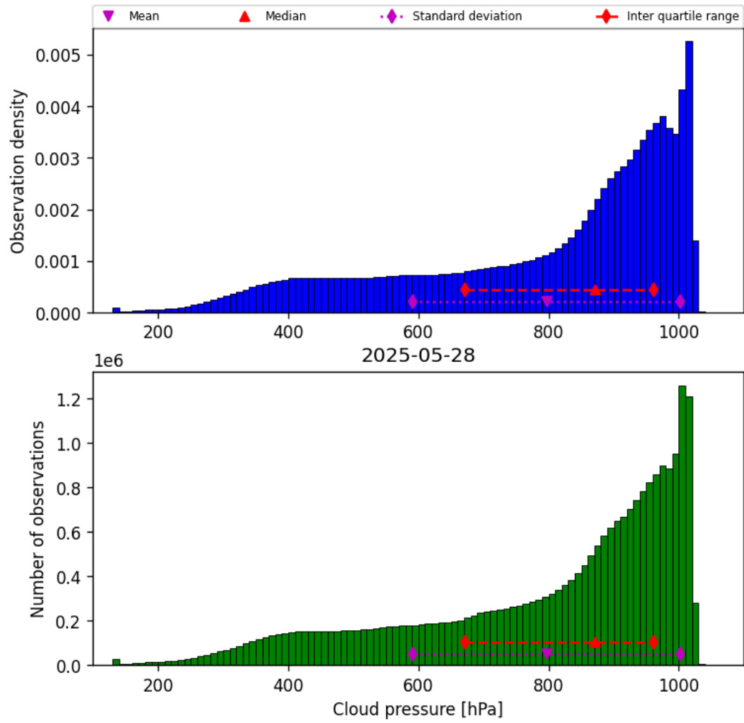
Figure 30: Histogram of “Cloud pressure” for 2025-05-27 to 2025-05-29
