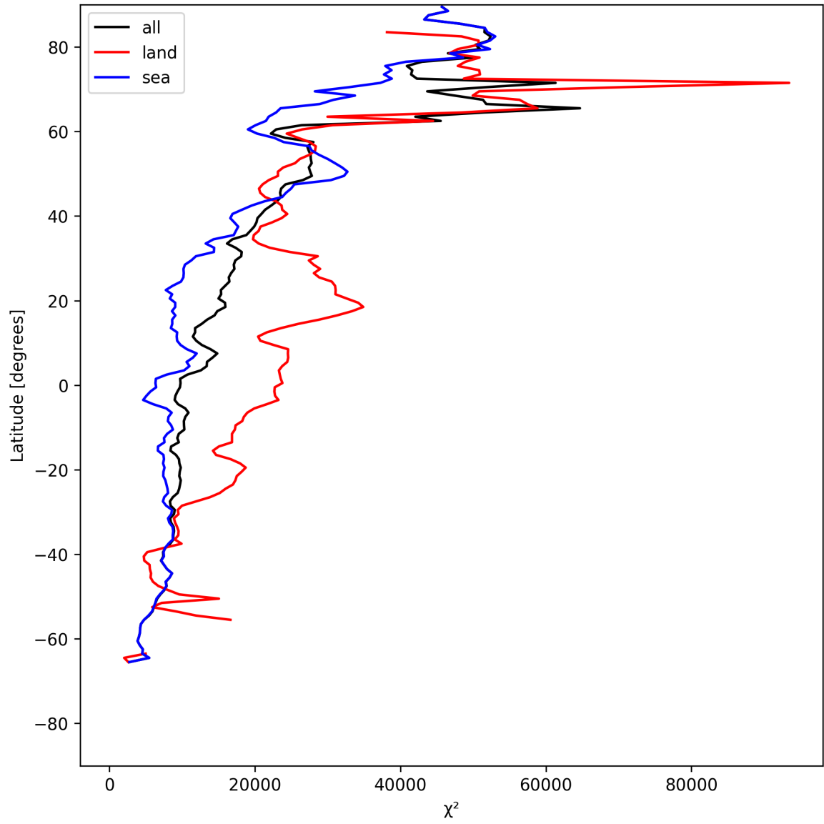
Figure 21: Zonal average of “ \chi^2 ” for 2025-05-27 to 2025-05-29.
