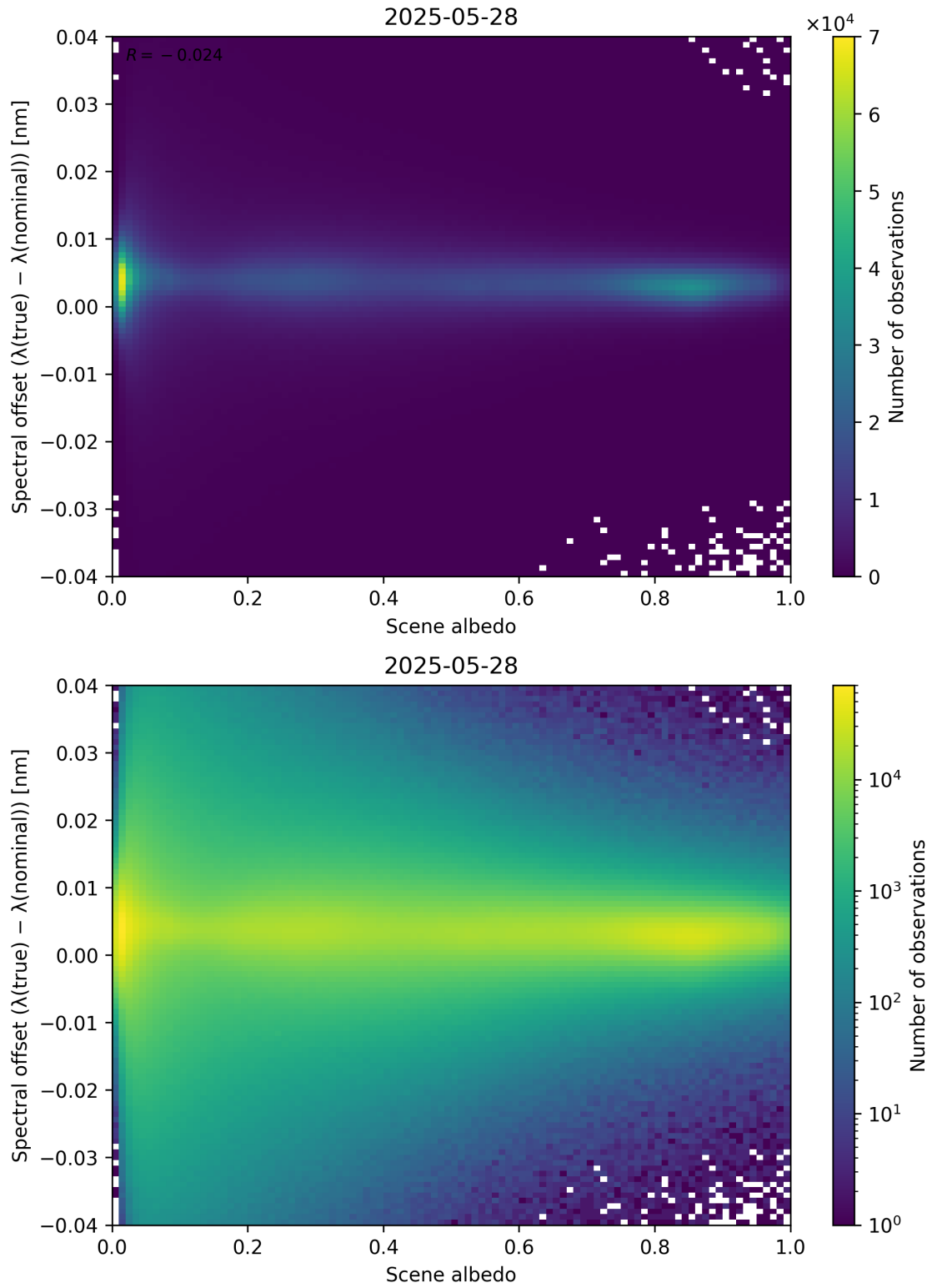
Figure 107: Scatter density plot of “Scene albedo” against “Spectral offset ( \lambda_{\text{true}} - \lambda_{\text{nominal}} )” for 2025-05-27 to 2025-05-29.
