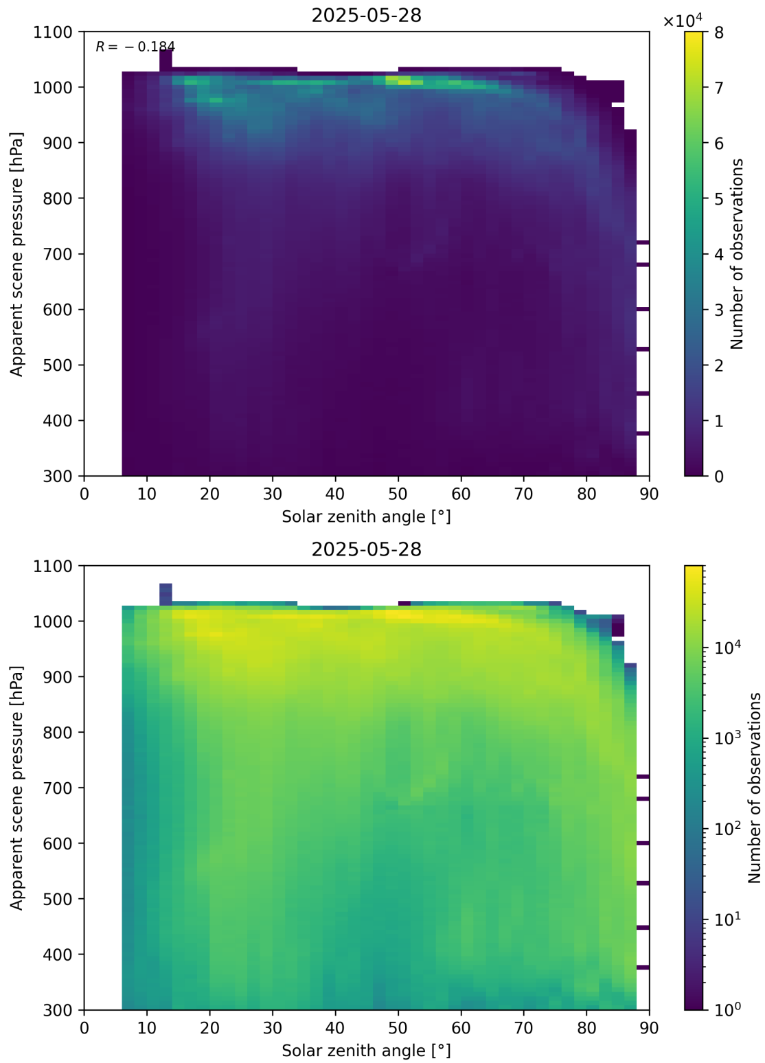
Figure 108: Scatter density plot of “Solar zenith angle” against “Apparent scene pressure” for 2025-05-27 to 2025-05-29.
