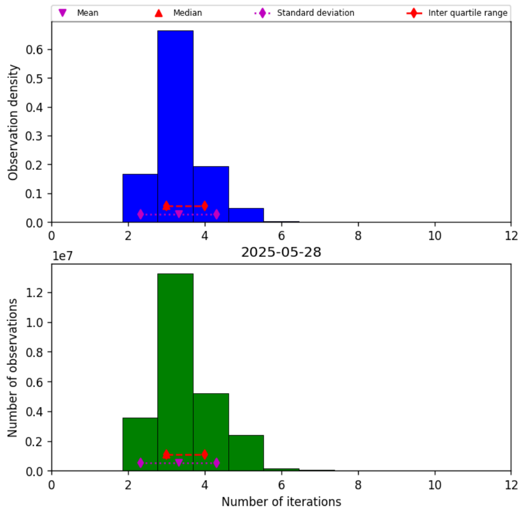
Figure 39: Histogram of “Number of iterations” for 2025-05-27 to 2025-05-29
