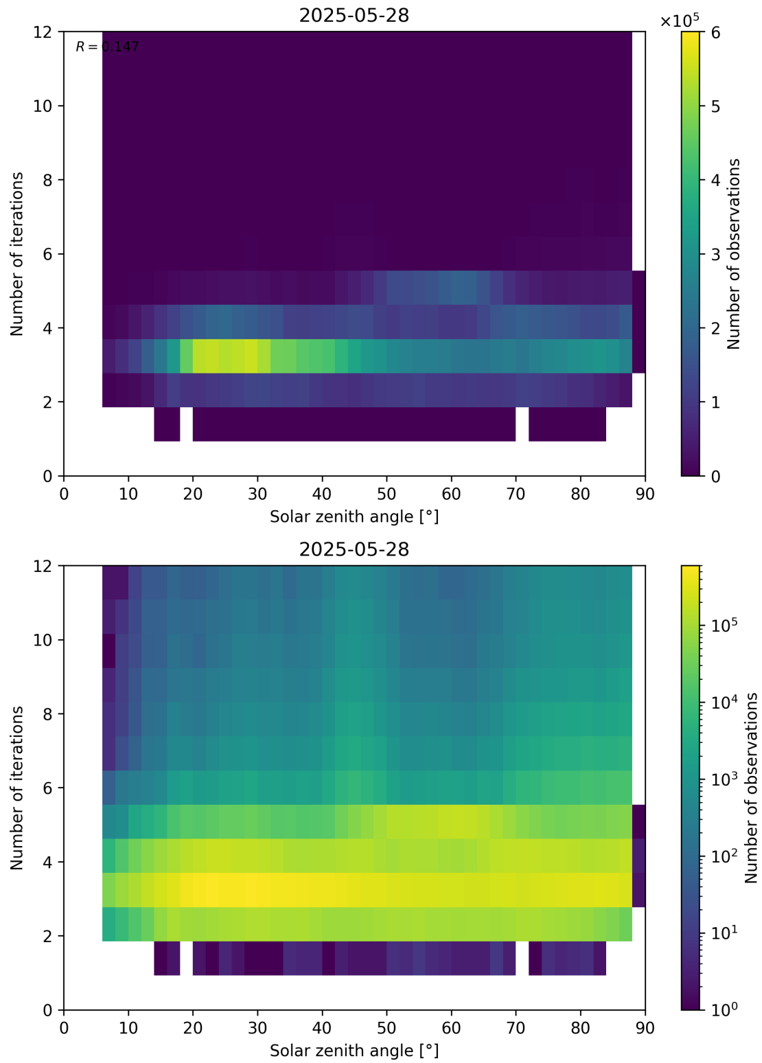
Figure 114: Scatter density plot of “Solar zenith angle” against “Number of iterations” for 2025-05-27 to 2025-05-29.
