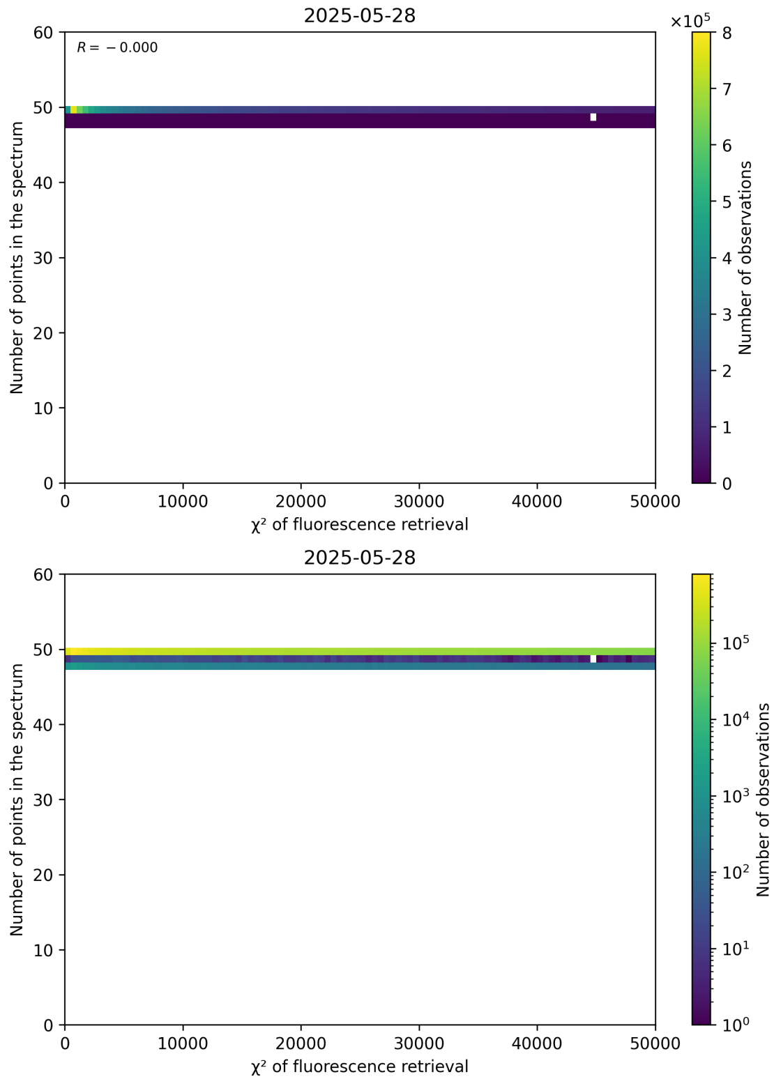
Figure 68: Scatter density plot of “ \chi^2 of fluorescence retrieval” against “Number of points in the spectrum” for 2025-05-27 to 2025-05-29.
