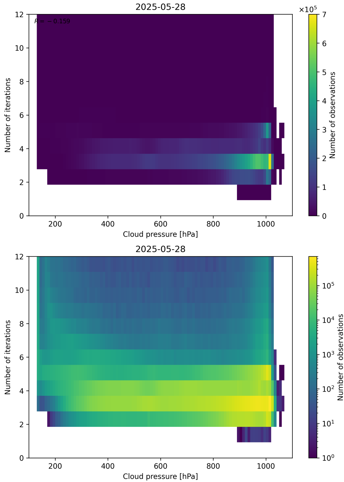
Figure 81: Scatter density plot of “Cloud pressure” against “Number of iterations” for 2025-05-27 to 2025-05-29.
