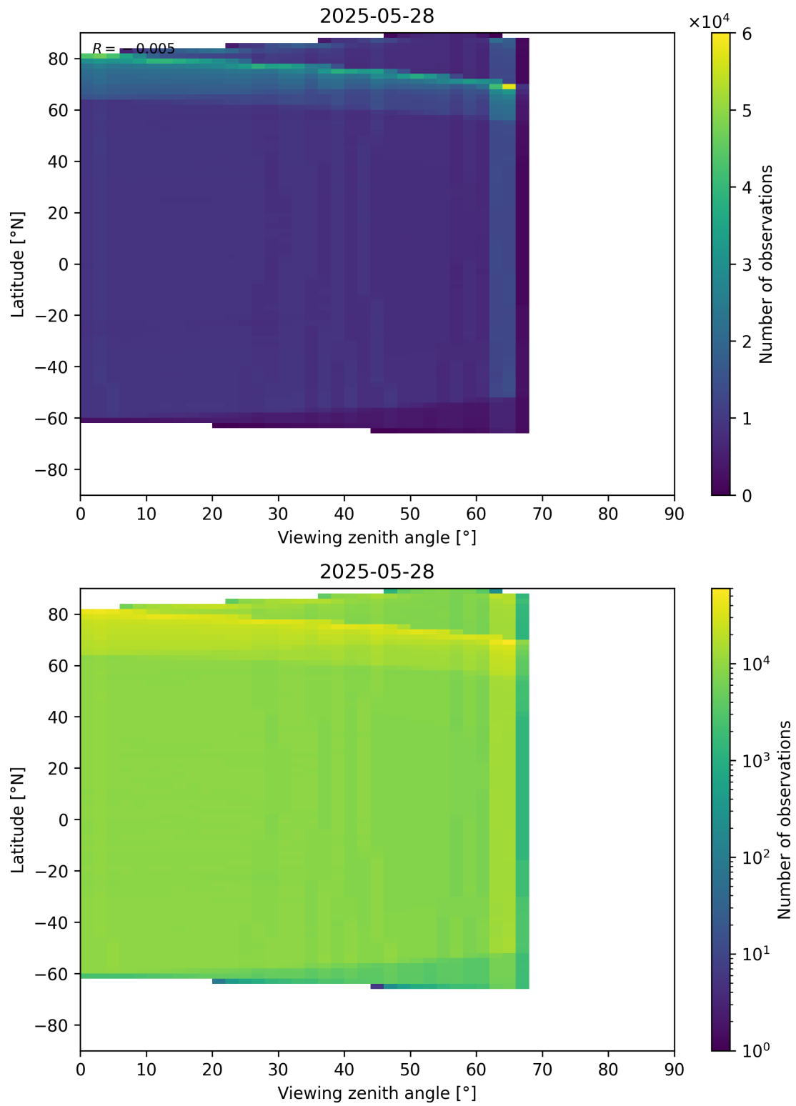
Figure 123: Scatter density plot of “Viewing zenith angle” against “Latitude” for 2025-05-27 to 2025-05-29.
