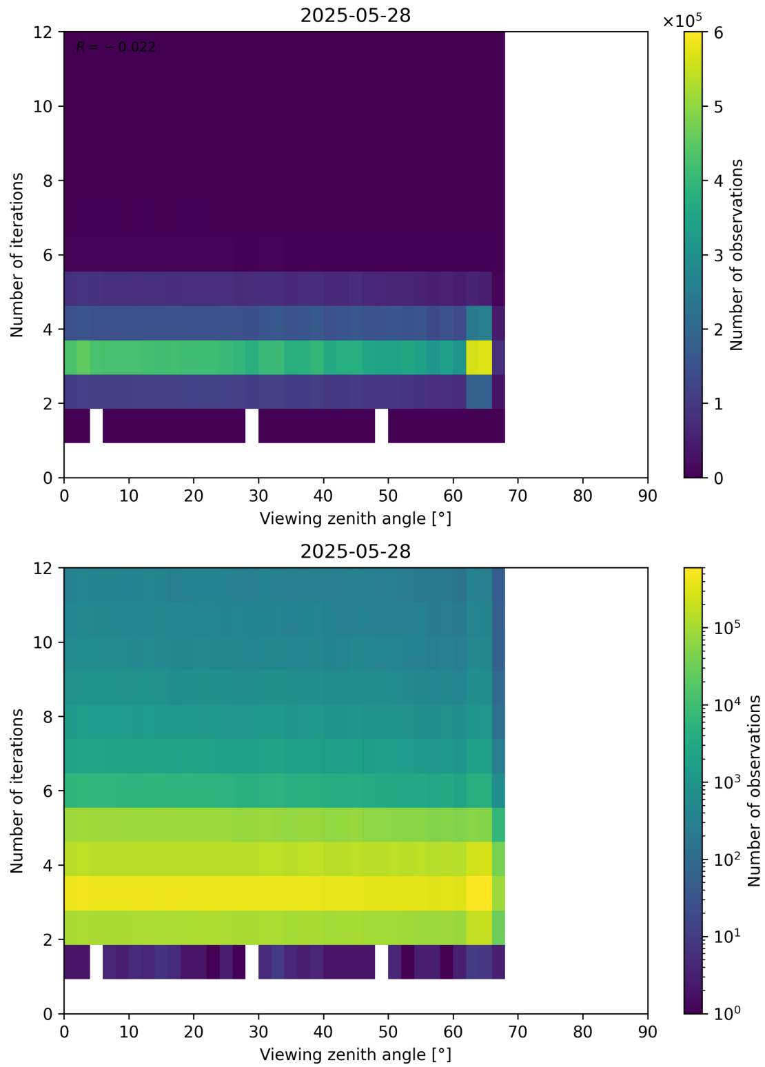
Figure 124: Scatter density plot of “Viewing zenith angle” against “Number of iterations” for 2025-05-27 to 2025-05-29.
