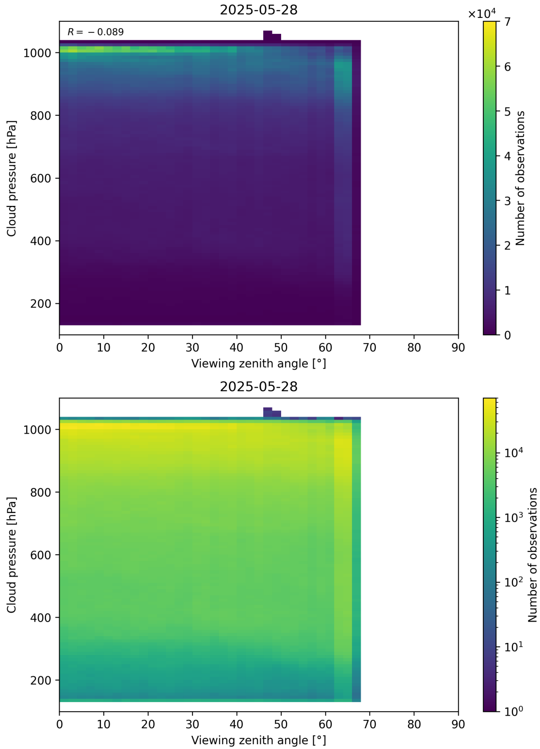
Figure 121: Scatter density plot of “Viewing zenith angle” against “Cloud pressure” for 2025-05-27 to 2025-05-29.
