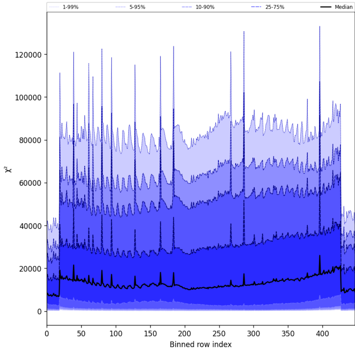
Figure 55: Along track statistics of “ \chi^2 ” for 2025-05-27 to 2025-05-29
