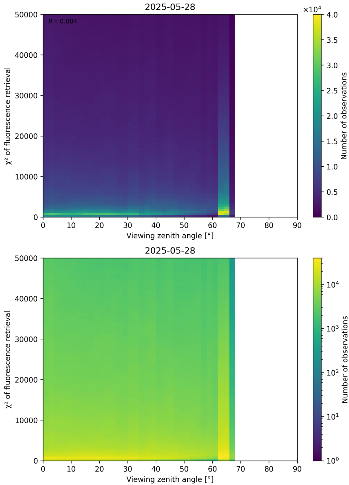
Figure 119: Scatter density plot of “Viewing zenith angle” against “ \chi^2 of fluorescence retrieval” for 2025-05-27 to 2025-05-29.
