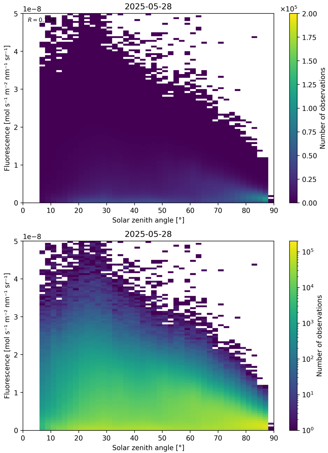
Figure 112: Scatter density plot of “Solar zenith angle” against “Fluorescence” for 2025-05-27 to 2025-05-29.
