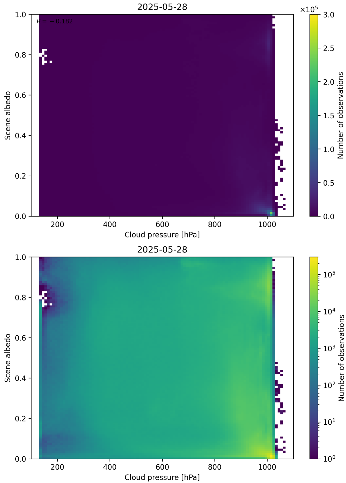
Figure 83: Scatter density plot of “Cloud pressure” against “Scene albedo” for 2025-05-27 to 2025-05-29.
