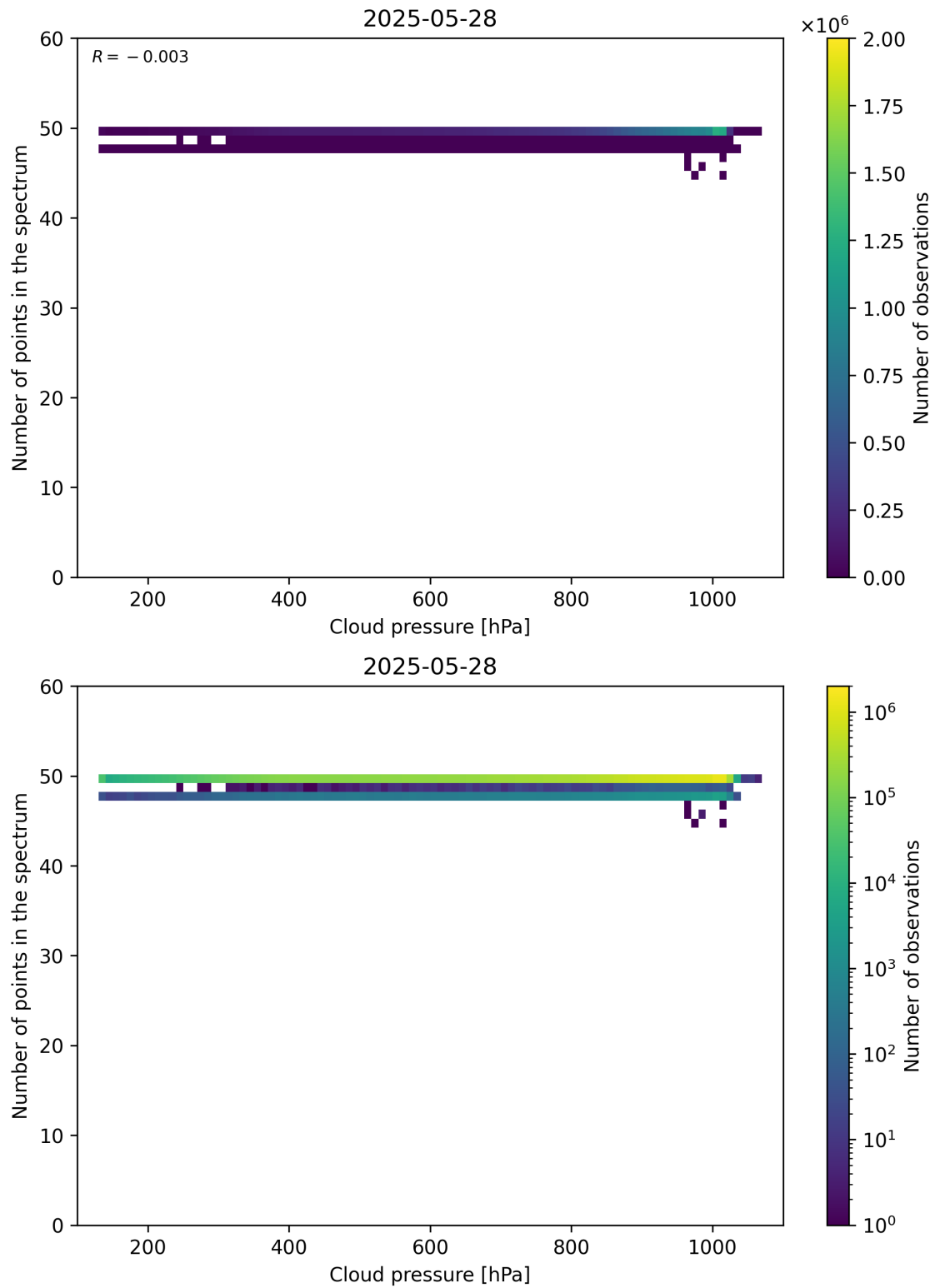
Figure 82: Scatter density plot of “Cloud pressure” against “Number of points in the spectrum” for 2025-05-27 to 2025-05-29.
