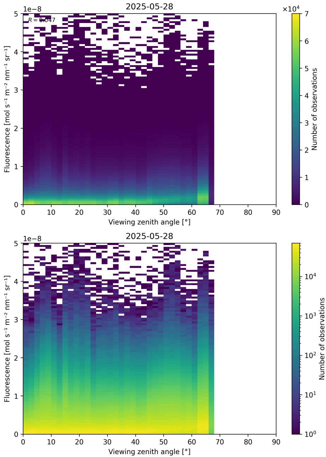
Figure 122: Scatter density plot of “Viewing zenith angle” against “Fluorescence” for 2025-05-27 to 2025-05-29.
