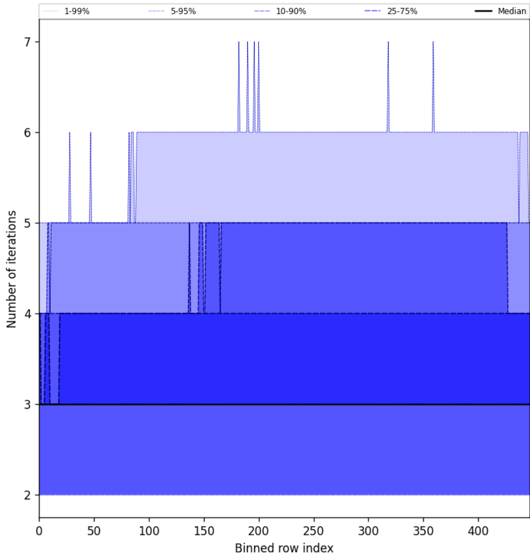
Figure 56: Along track statistics of “Number of iterations” for 2025-05-27 to 2025-05-29
