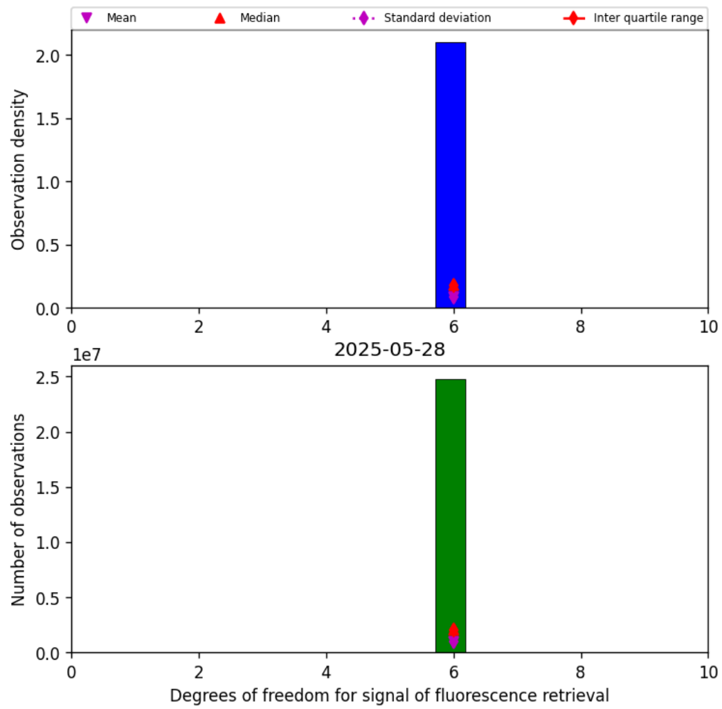
Figure 43: Histogram of “Degrees of freedom for signal of fluorescence retrieval” for 2025-05-27 to 2025-05-29
