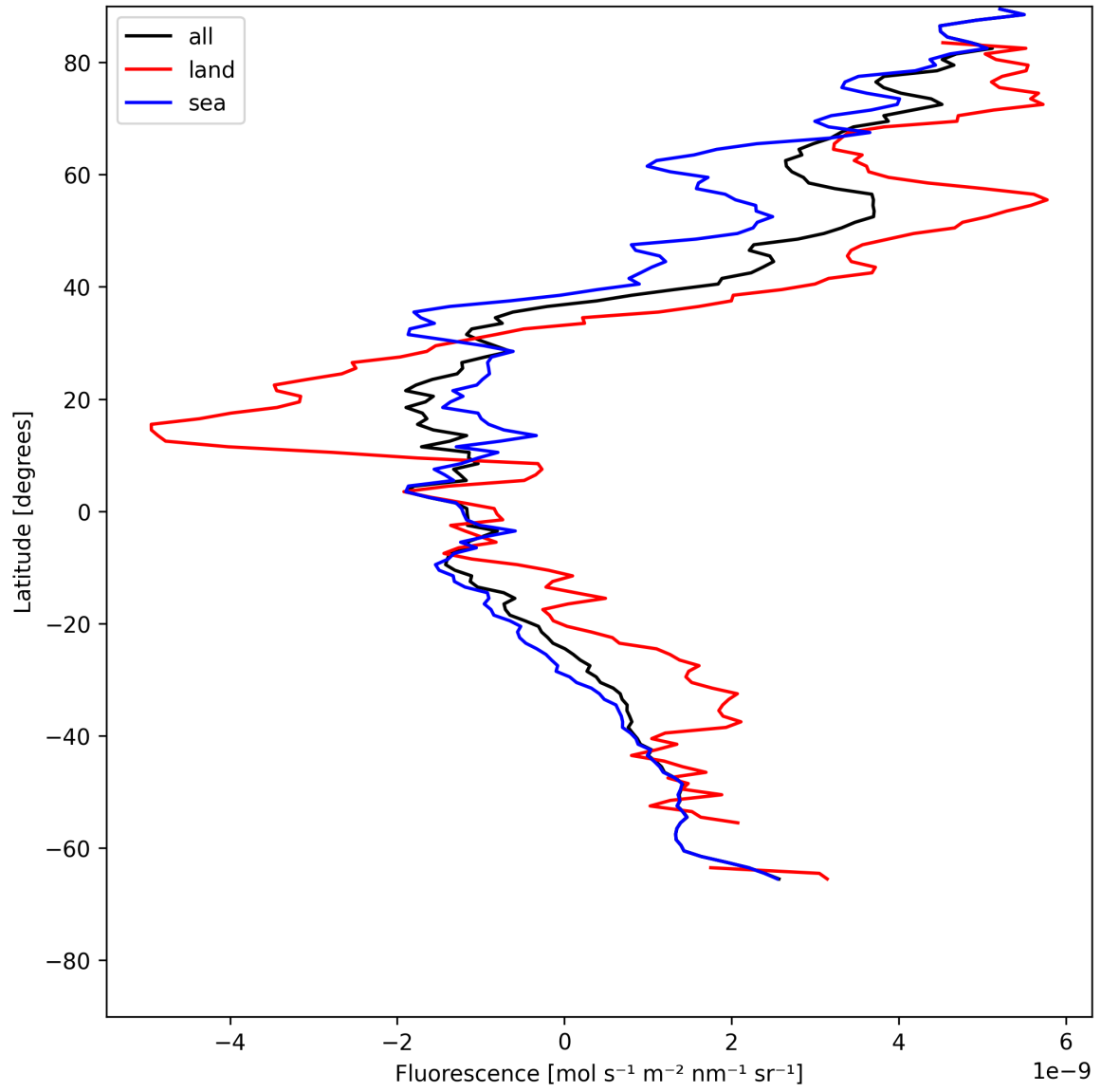
Figure 23: Zonal average of “Fluorescence” for 2025-05-27 to 2025-05-29.
