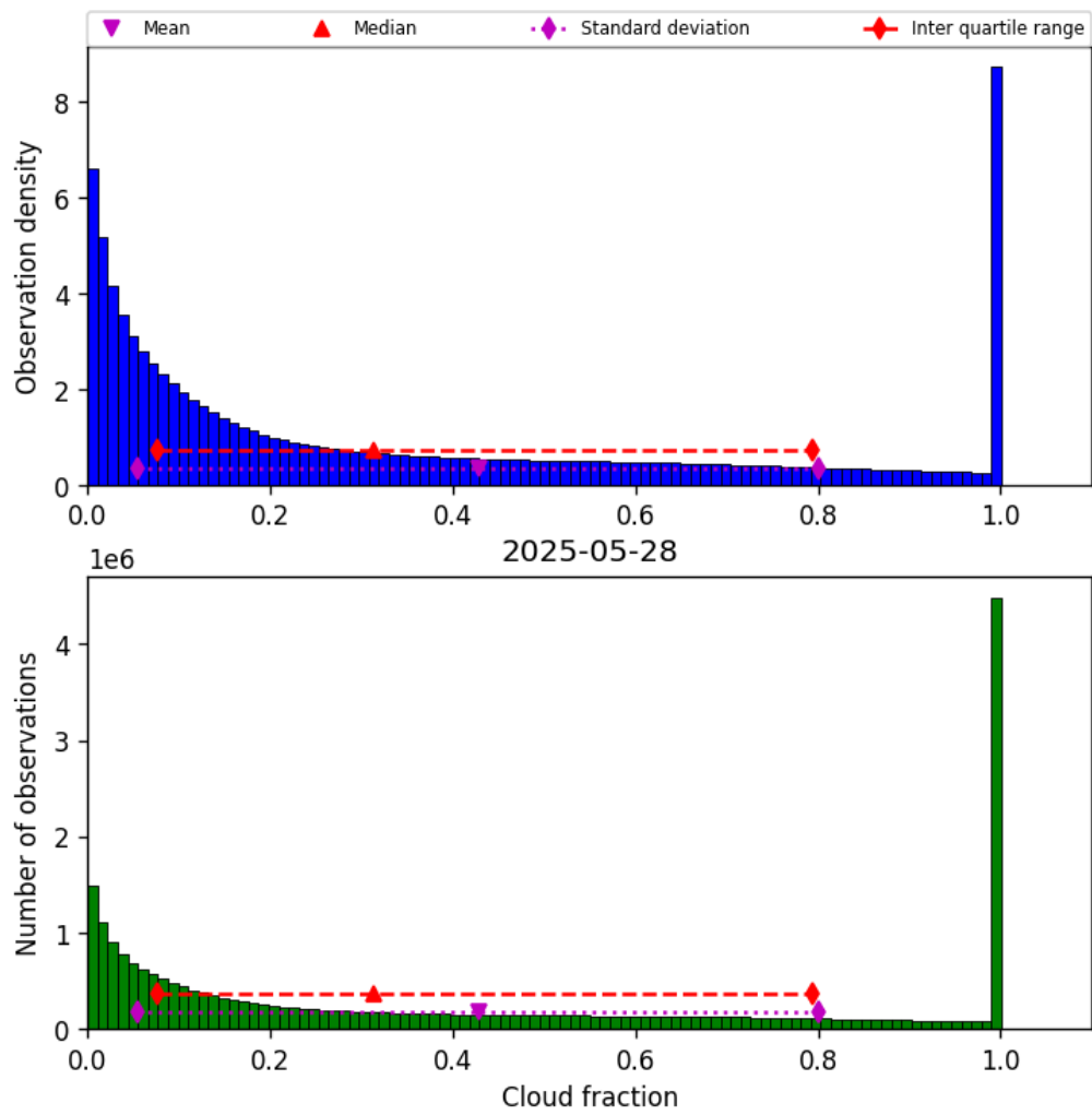
Figure 32: Histogram of “Cloud fraction” for 2025-05-27 to 2025-05-29
