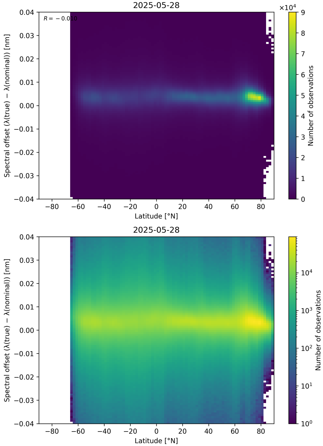
Figure 96: Scatter density plot of “Latitude” against “Spectral offset ( \lambda_{\text{true}} - \lambda_{\text{nominal}} )” for 2025-05-27 to 2025-05-29.
