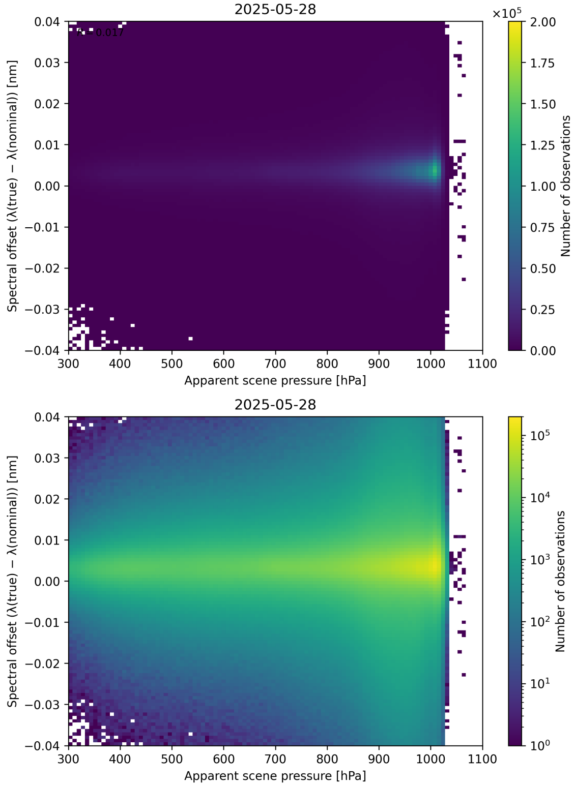
Figure 67: Scatter density plot of “Apparent scene pressure” against “Spectral offset ( \lambda_{\text{true}} - \lambda_{\text{nominal}} )” for 2025-05-27 to 2025-05-29.
