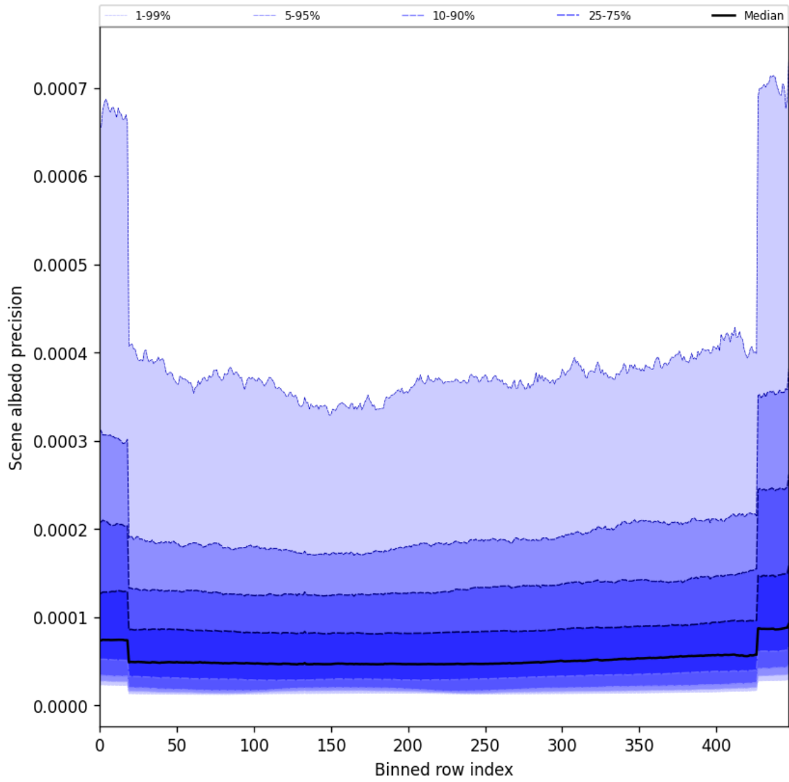
Figure 52: Along track statistics of “Scene albedo precision” for 2025-05-27 to 2025-05-29
