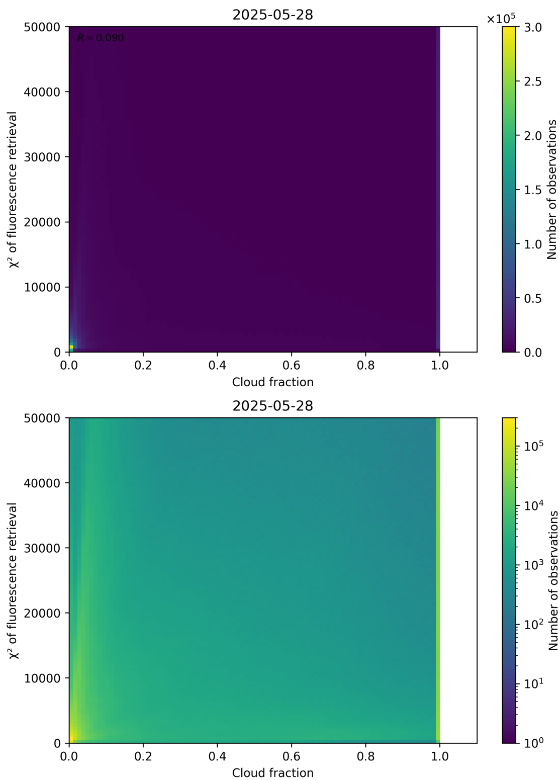
Figure 71: Scatter density plot of “Cloud fraction” against “ \chi^2 of fluorescence retrieval” for 2025-05-27 to 2025-05-29.
