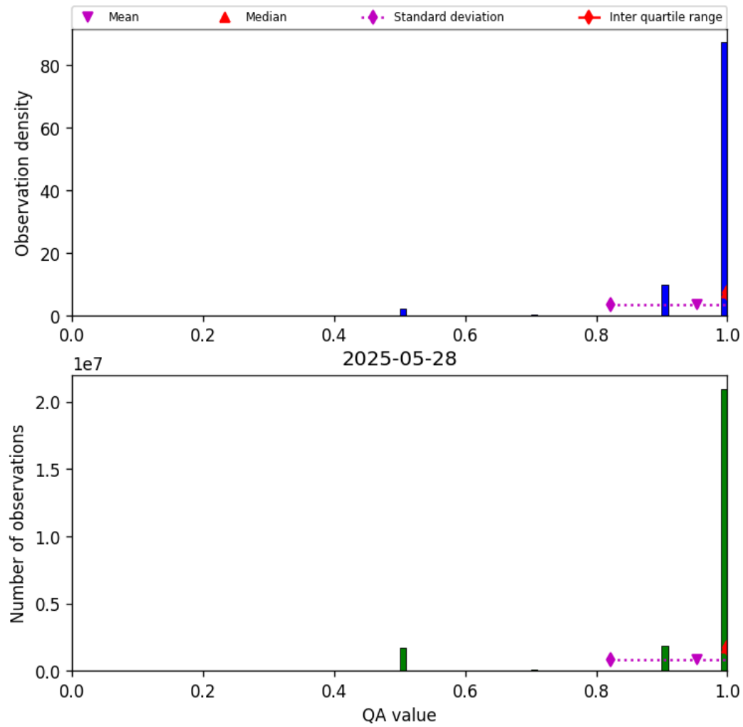
Figure 29: Histogram of “QA value” for 2025-05-27 to 2025-05-29
