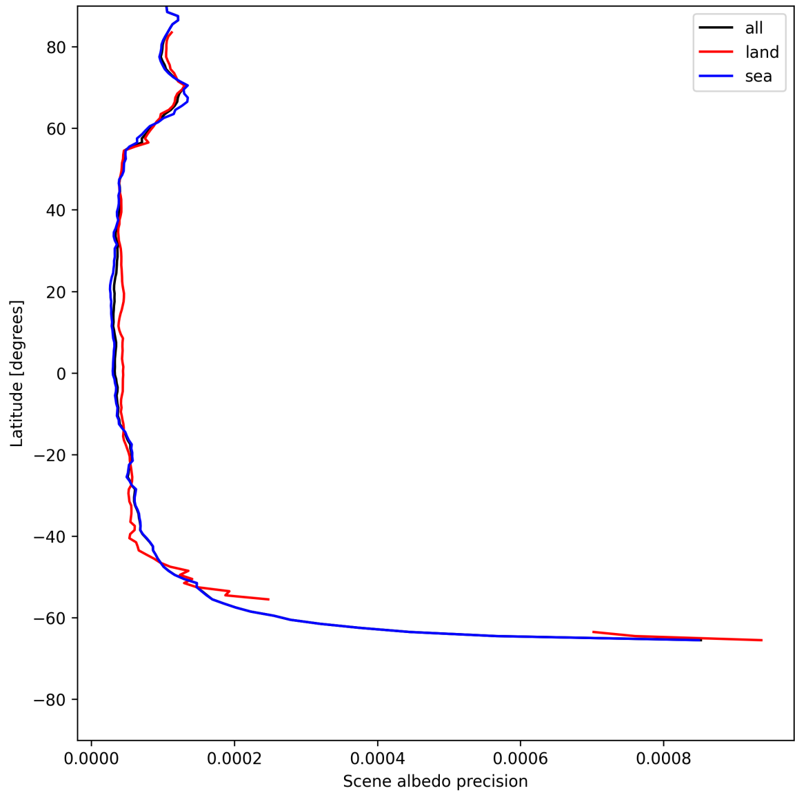
Figure 18: Zonal average of “Scene albedo precision” for 2025-05-27 to 2025-05-29.
