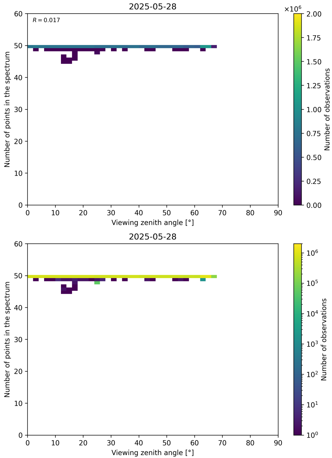
Figure 125: Scatter density plot of “Viewing zenith angle” against “Number of points in the spectrum” for 2025-05-27 to 2025-05-29.
