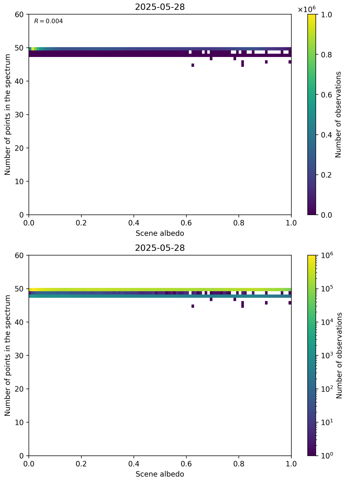
Figure 106: Scatter density plot of “Scene albedo” against “Number of points in the spectrum” for 2025-05-27 to 2025-05-29.
