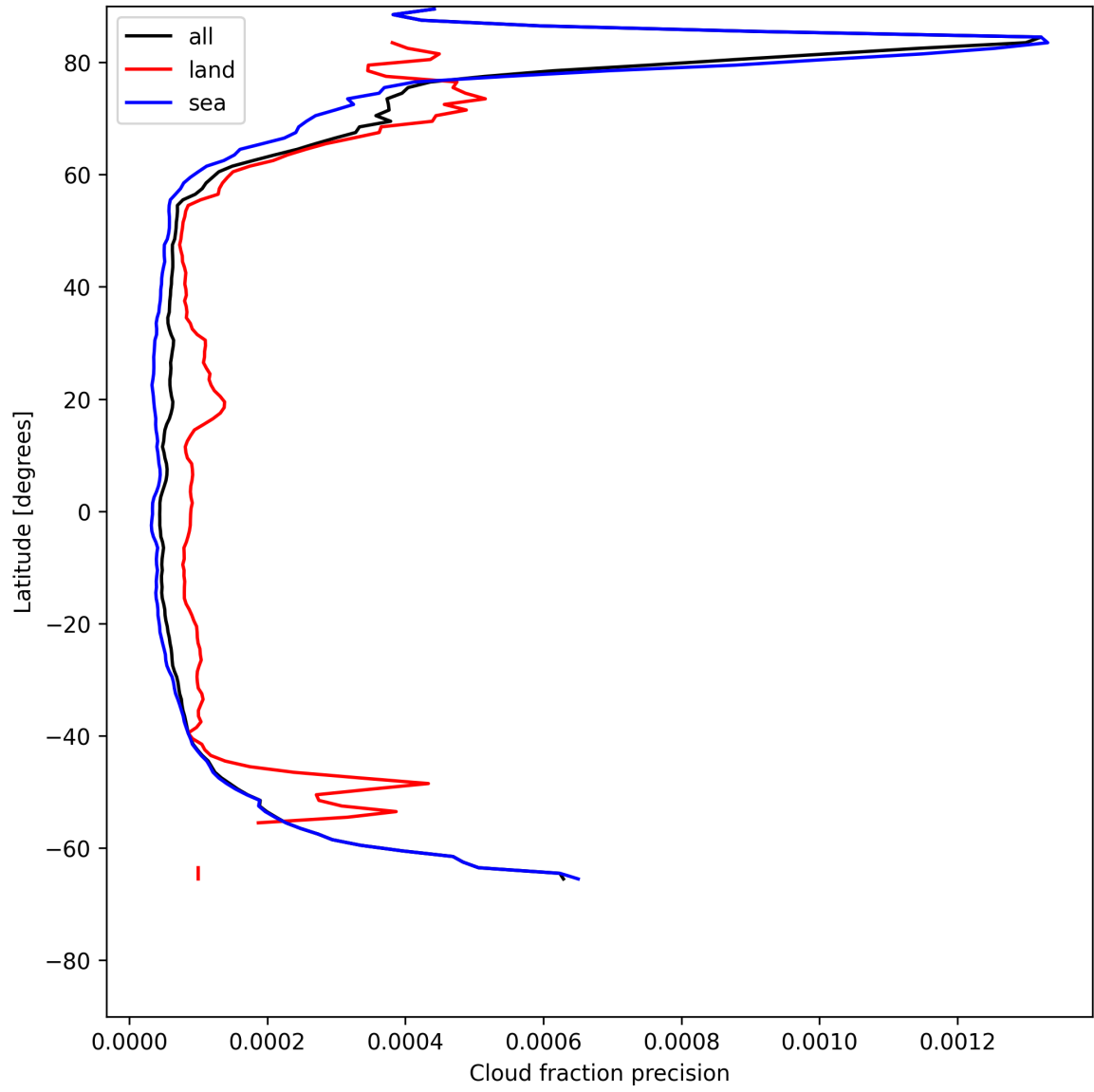
Figure 16: Zonal average of “Cloud fraction precision” for 2025-05-27 to 2025-05-29.
