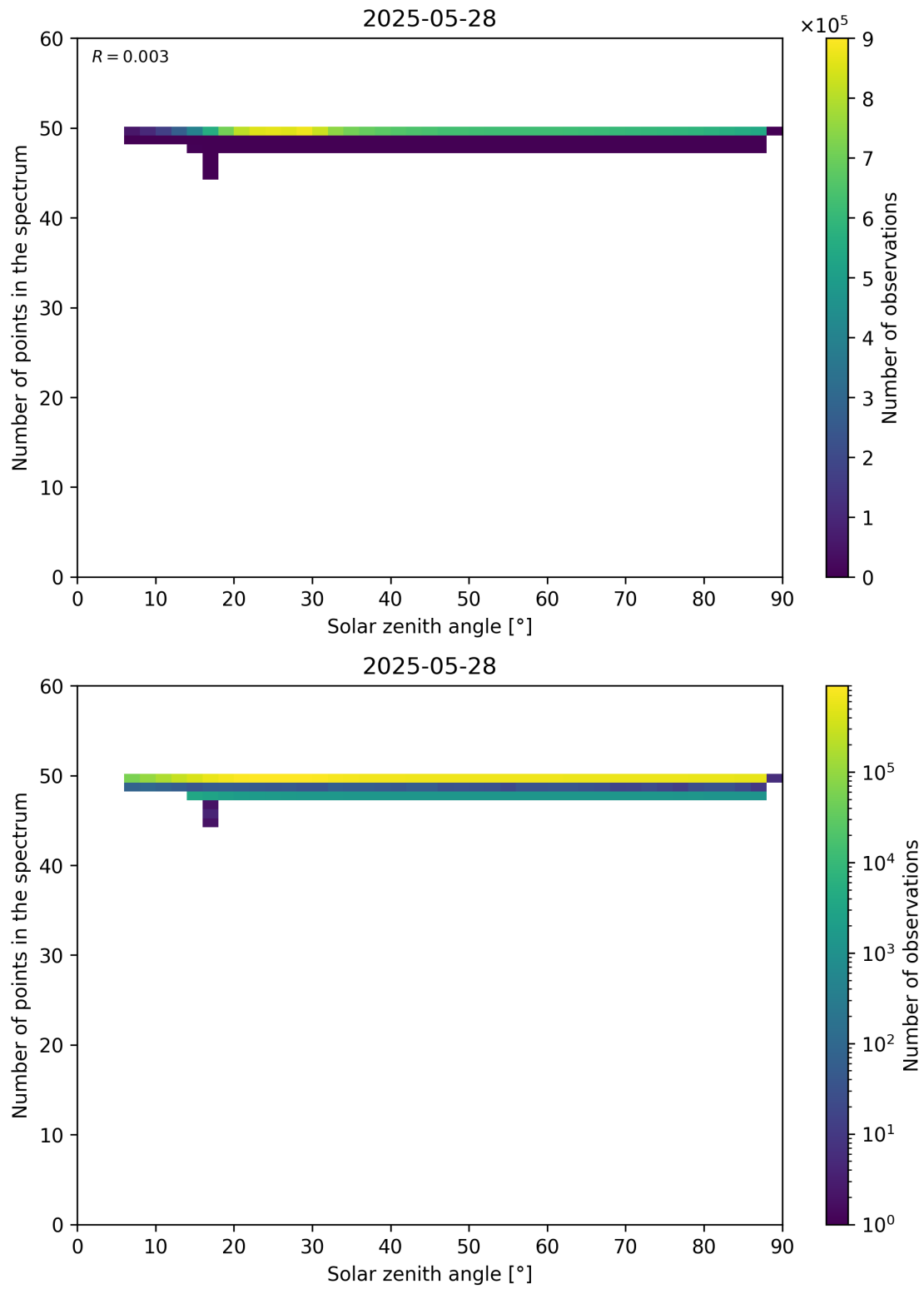
Figure 115: Scatter density plot of “Solar zenith angle” against “Number of points in the spectrum” for 2025-05-27 to 2025-05-29.
