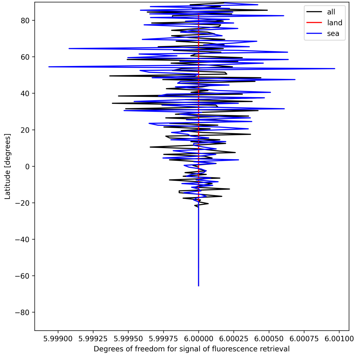
Figure 26: Zonal average of “Degrees of freedom for signal of fluorescence retrieval” for 2025-05-27 to 2025-05-29.
