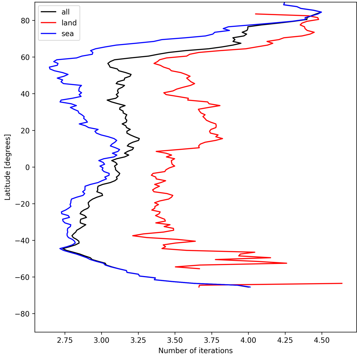
Figure 22: Zonal average of “Number of iterations” for 2025-05-27 to 2025-05-29.
