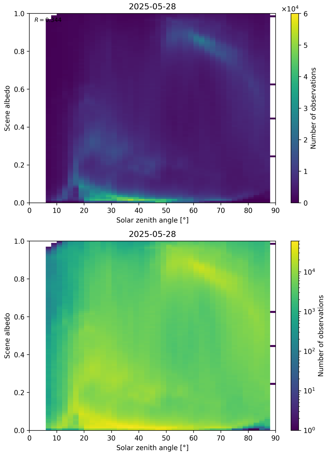
Figure 116: Scatter density plot of “Solar zenith angle” against “Scene albedo” for 2025-05-27 to 2025-05-29.
