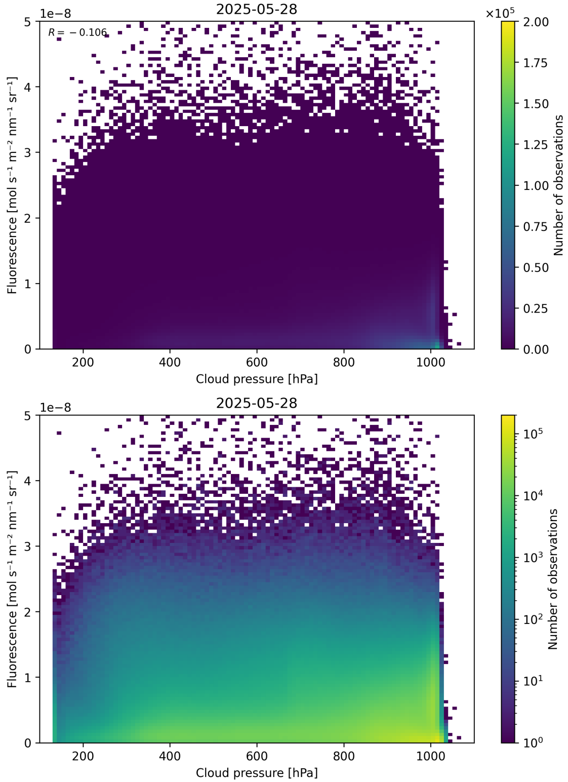
Figure 80: Scatter density plot of “Cloud pressure” against “Fluorescence” for 2025-05-27 to 2025-05-29.
