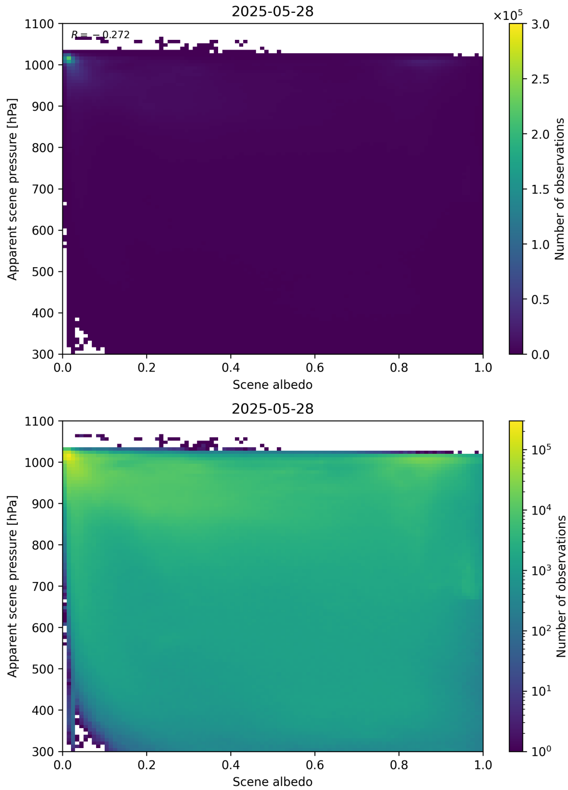
Figure 102: Scatter density plot of “Scene albedo” against “Apparent scene pressure” for 2025-05-27 to 2025-05-29.
