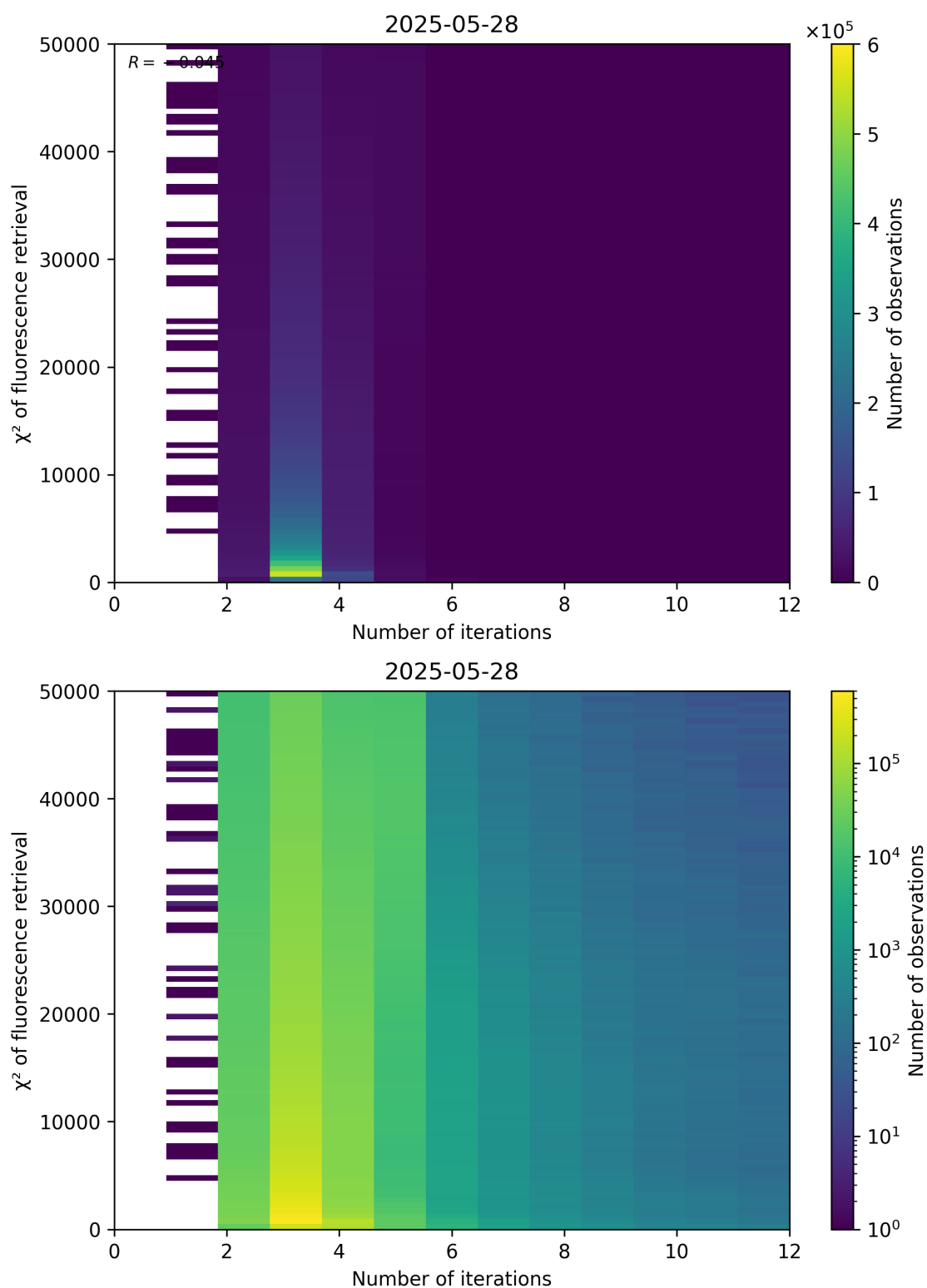
Figure 97: Scatter density plot of “Number of iterations” against “ \chi^2 of fluorescence retrieval” for 2025-05-27 to 2025-05-29.
