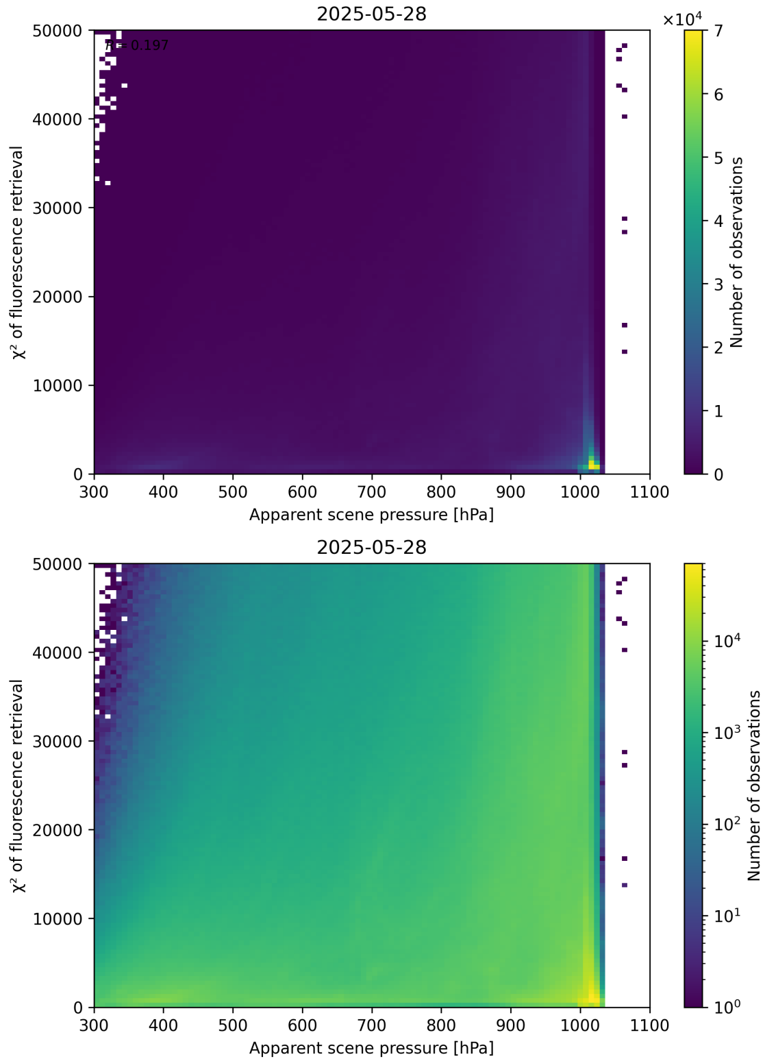
Figure 63: Scatter density plot of “Apparent scene pressure” against “ \chi^2 of fluorescence retrieval” for 2025-05-27 to 2025-05-29.
