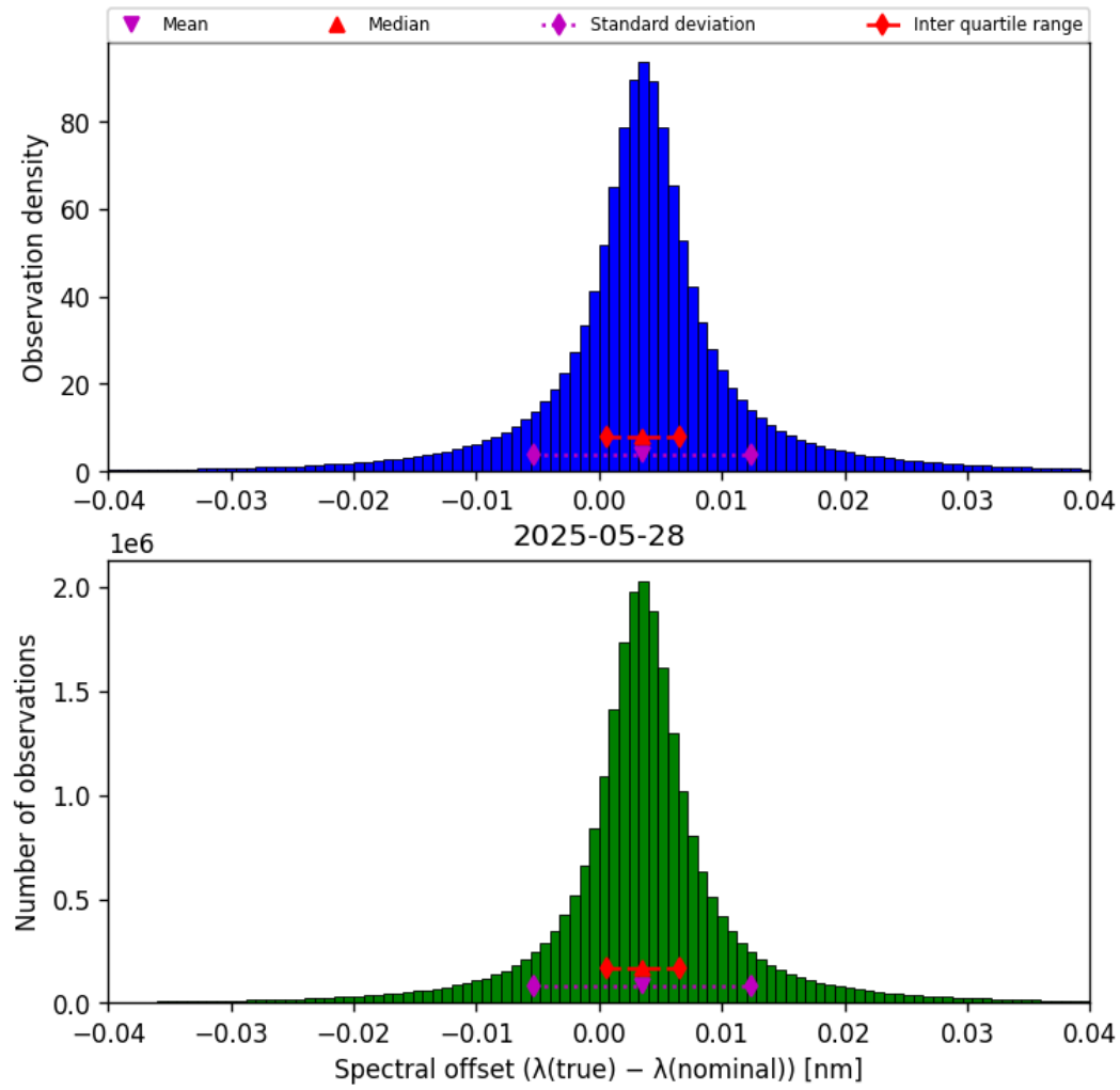
Figure 45: Histogram of “Spectral offset ( \lambda_{\text{true}} - \lambda_{\text{nominal}} )” for 2025-05-27 to 2025-05-29
