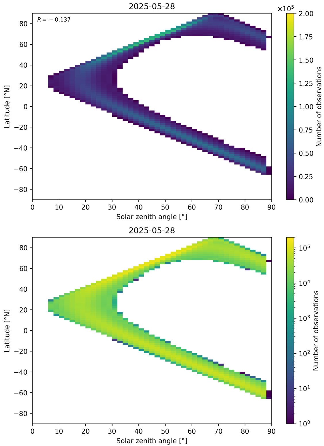
Figure 113: Scatter density plot of “Solar zenith angle” against “Latitude” for 2025-05-27 to 2025-05-29.
