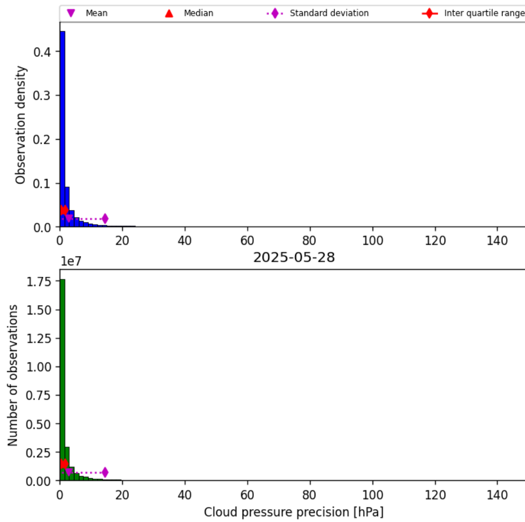
Figure 31: Histogram of “Cloud pressure precision” for 2025-05-27 to 2025-05-29
