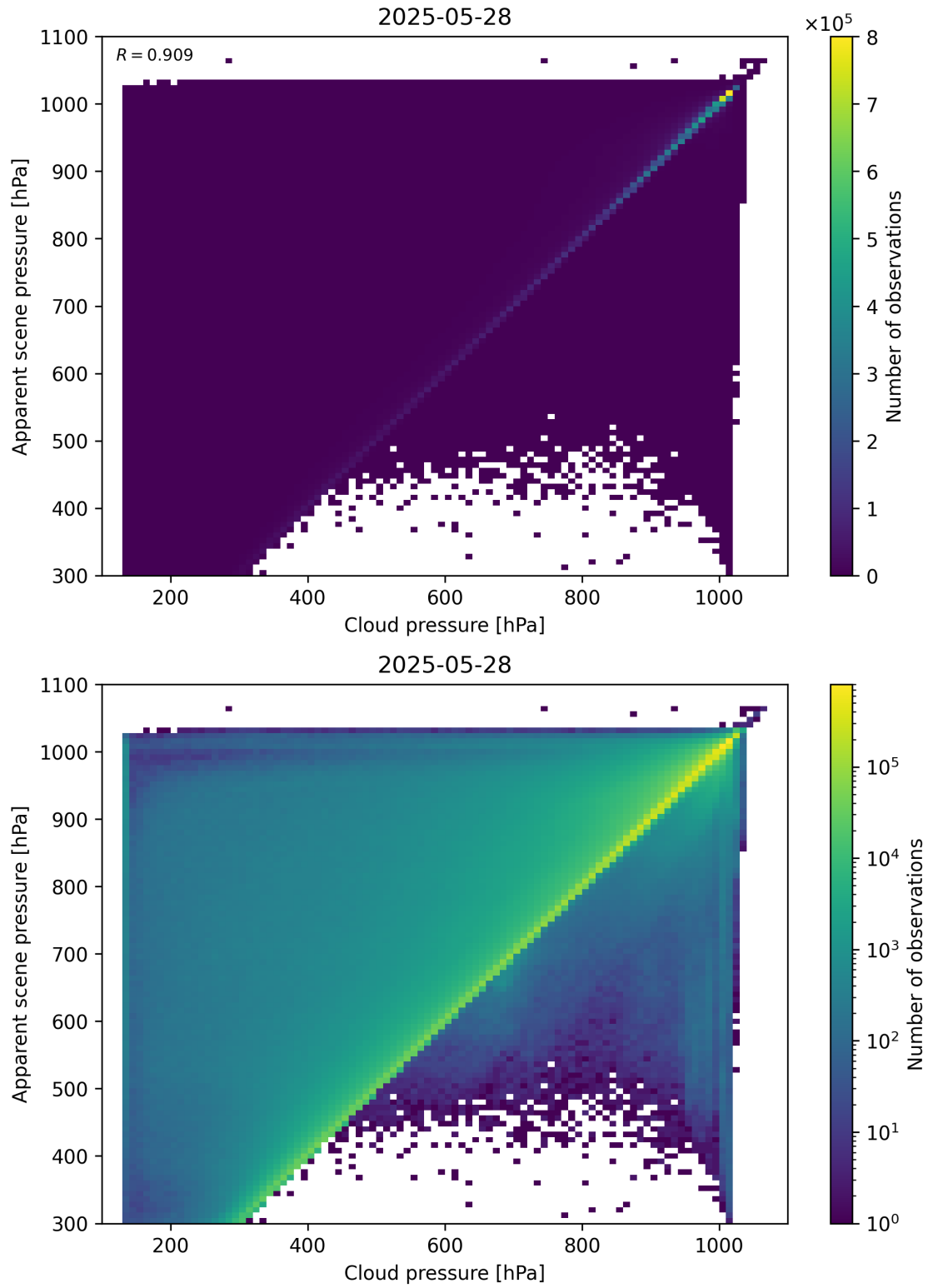
Figure 77: Scatter density plot of “Cloud pressure” against “Apparent scene pressure” for 2025-05-27 to 2025-05-29.
