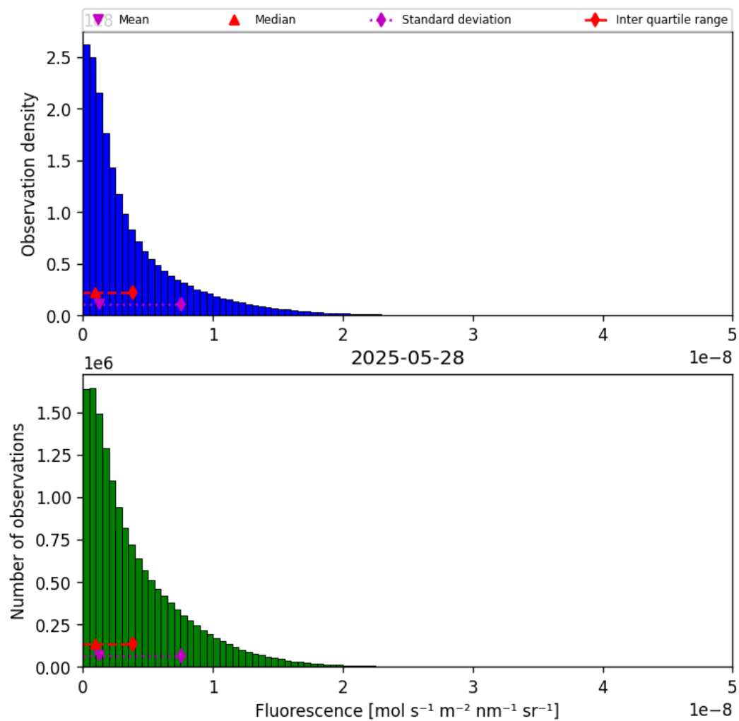
Figure 40: Histogram of “Fluorescence” for 2025-05-27 to 2025-05-29
