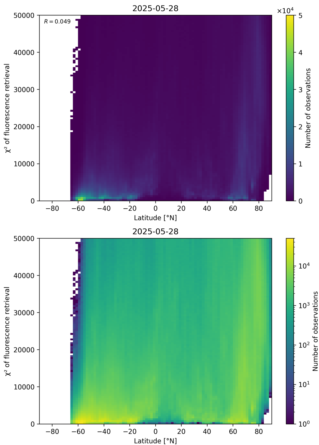
Figure 89: Scatter density plot of “Latitude” against “ \chi^2 of fluorescence retrieval” for 2025-05-27 to 2025-05-29.
