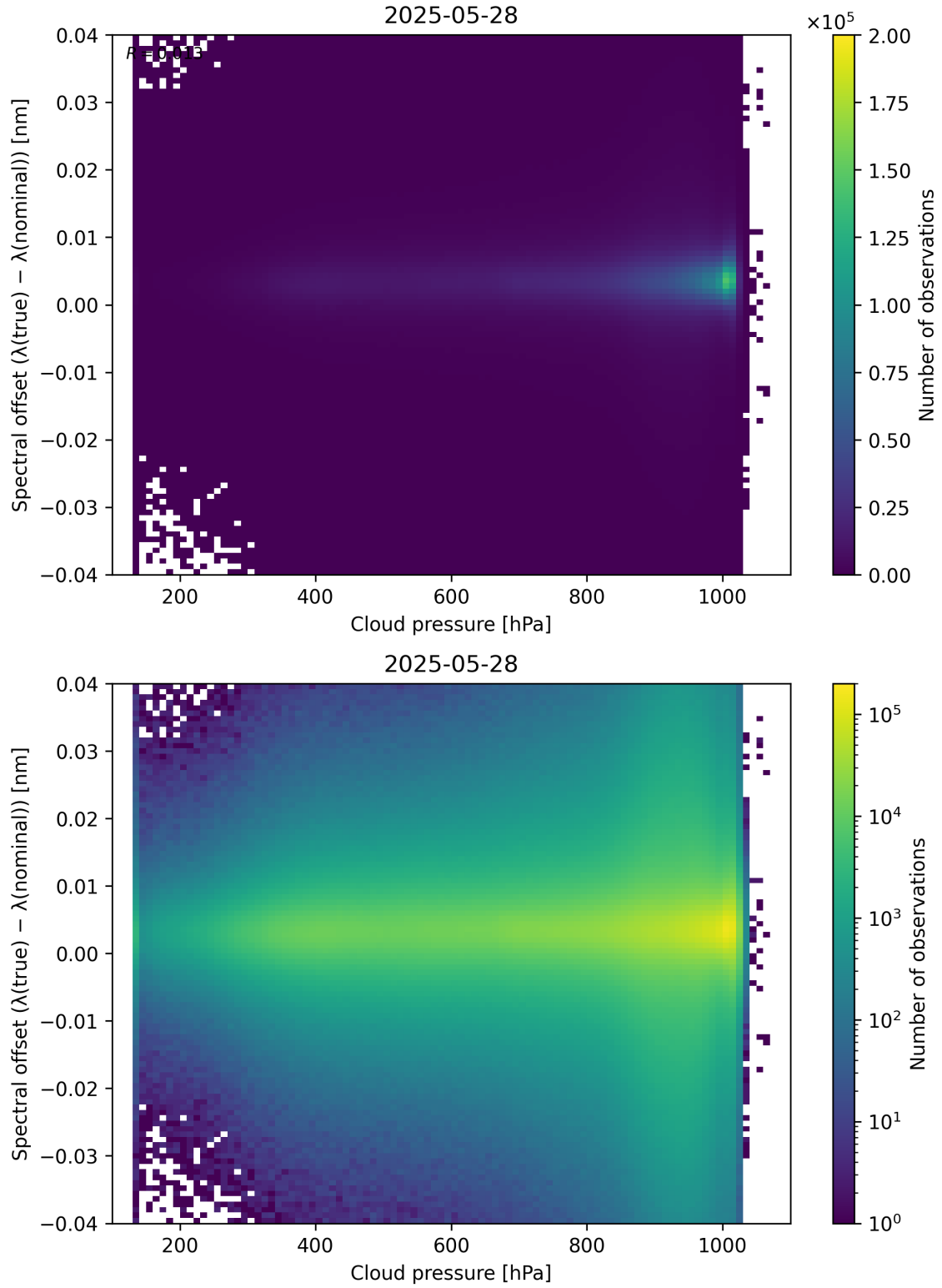
Figure 84: Scatter density plot of “Cloud pressure” against “Spectral offset ( \lambda_{\text{true}} - \lambda_{\text{nominal}} )” for 2025-05-27 to 2025-05-29.
