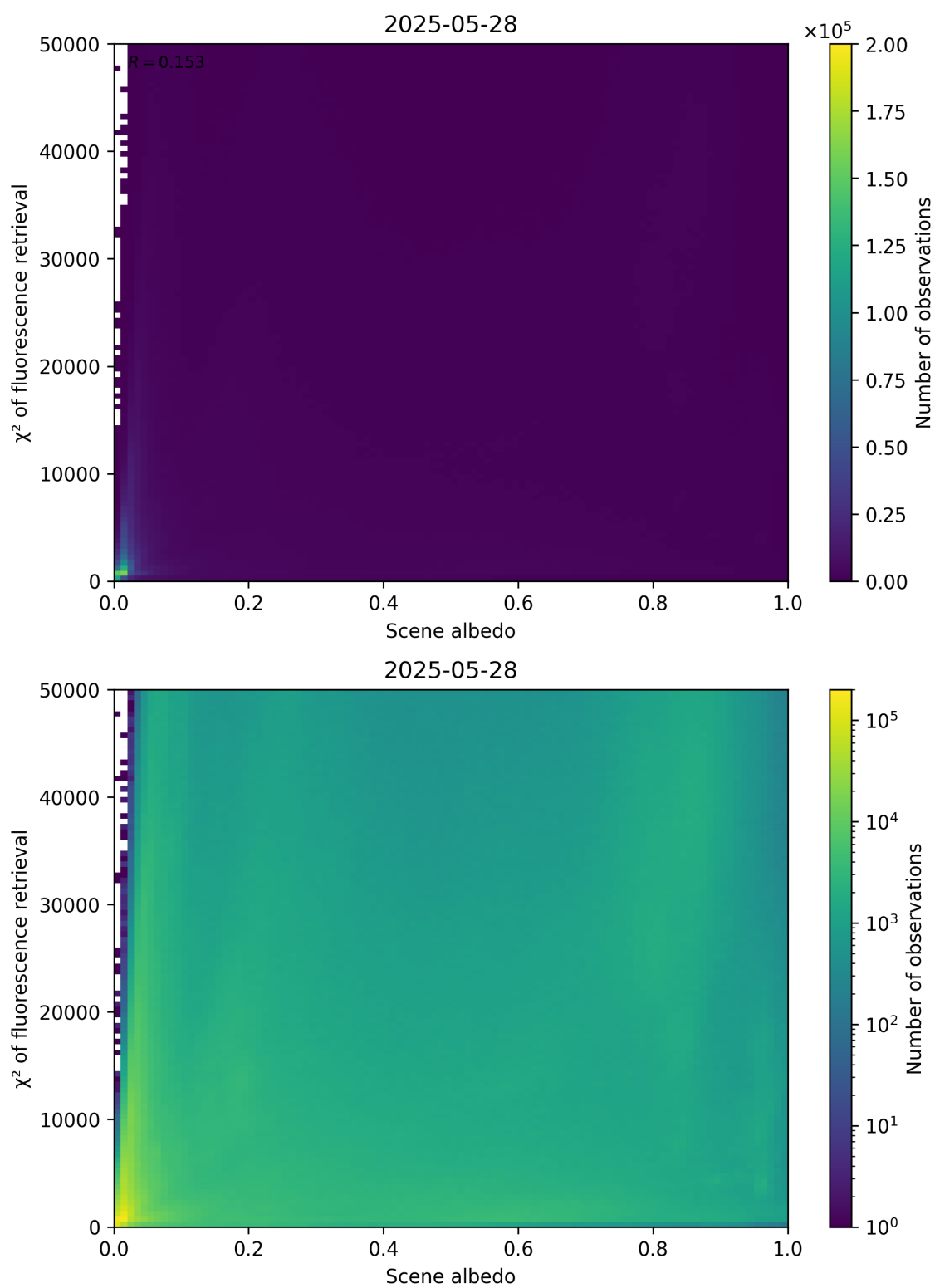
Figure 103: Scatter density plot of “Scene albedo” against “ \chi^2 of fluorescence retrieval” for 2025-05-27 to 2025-05-29.
