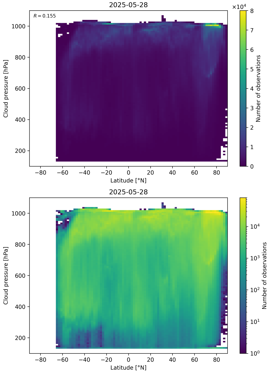
Figure 91: Scatter density plot of “Latitude” against “Cloud pressure” for 2025-05-27 to 2025-05-29.
