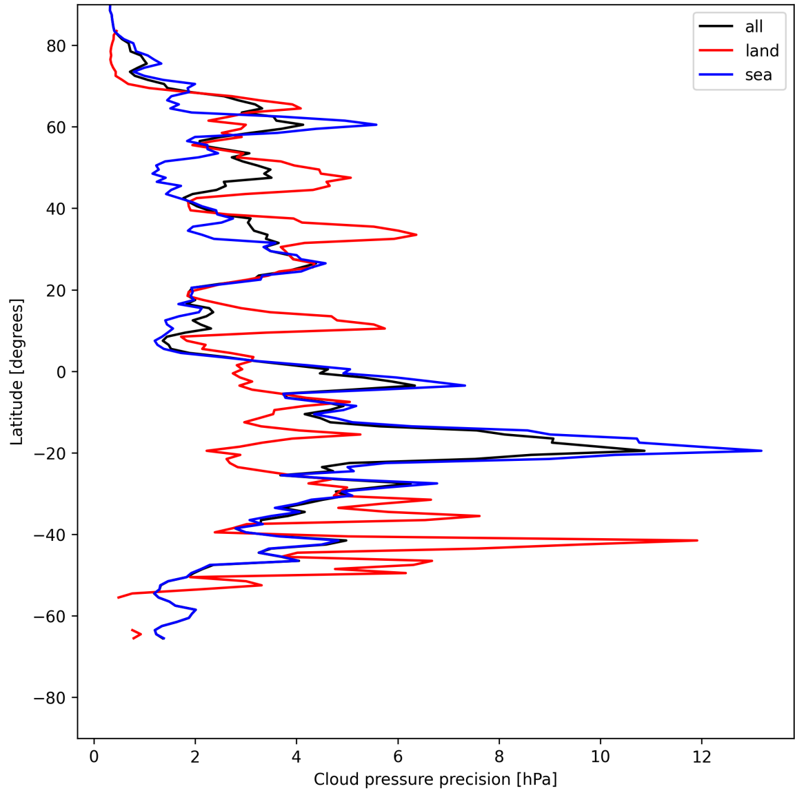
Figure 14: Zonal average of "Cloud pressure precision" for 2025-05-27 to 2025-05-29.
