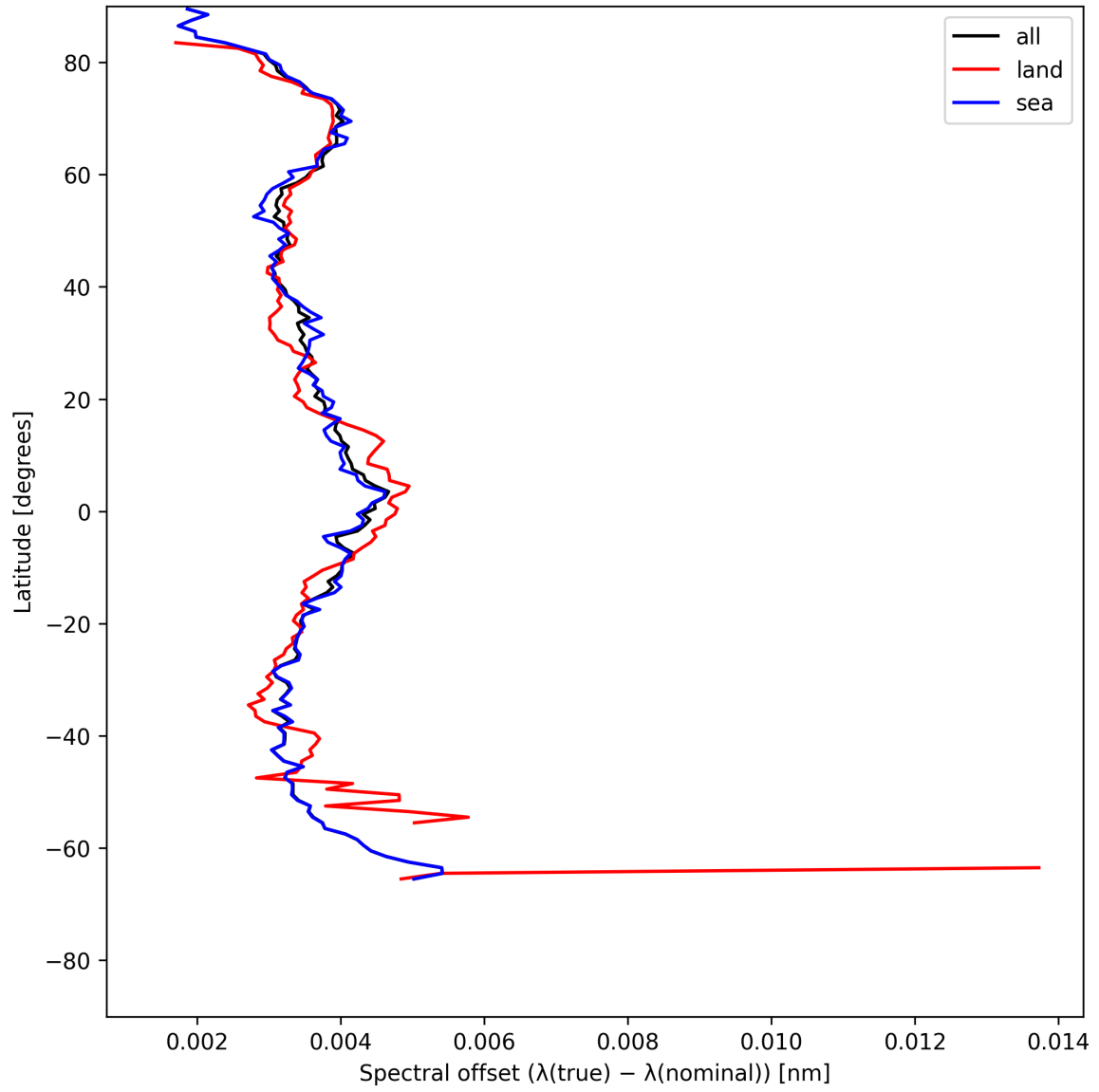
Figure 28: Zonal average of “Spectral offset ( \lambda_{\text{true}} - \lambda_{\text{nominal}} )” for 2025-05-27 to 2025-05-29.
