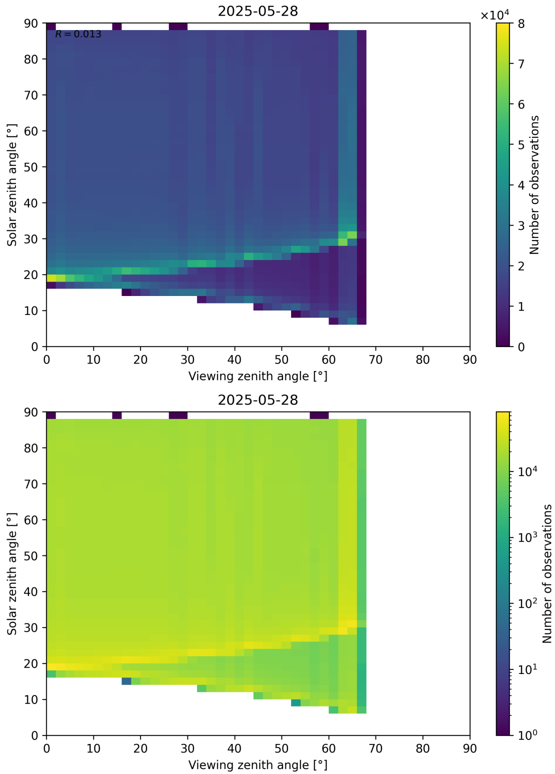
Figure 127: Scatter density plot of “Viewing zenith angle” against “Solar zenith angle” for 2025-05-27 to 2025-05-29.
