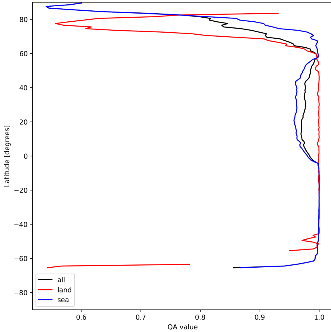
Figure 12: Zonal average of “QA value” for 2025-05-27 to 2025-05-29.
