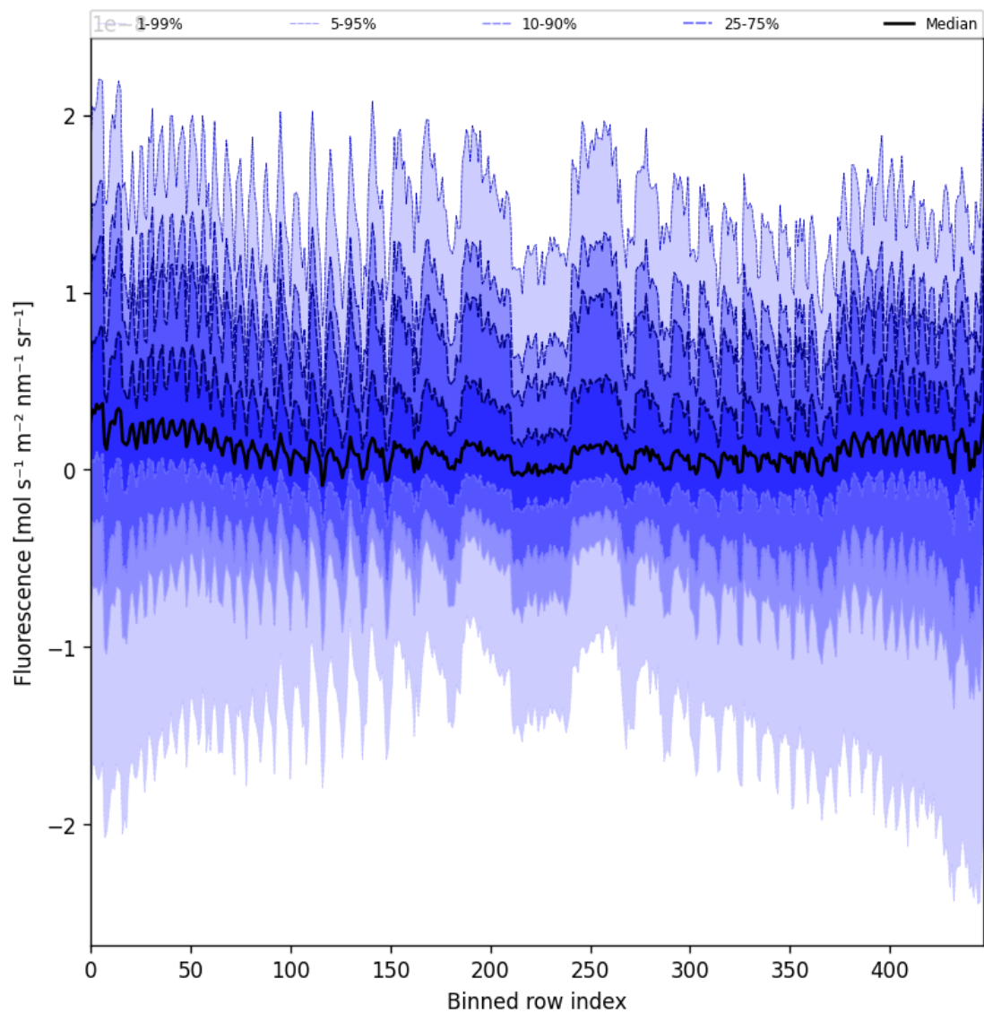
Figure 57: Along track statistics of “Fluorescence” for 2025-05-27 to 2025-05-29
