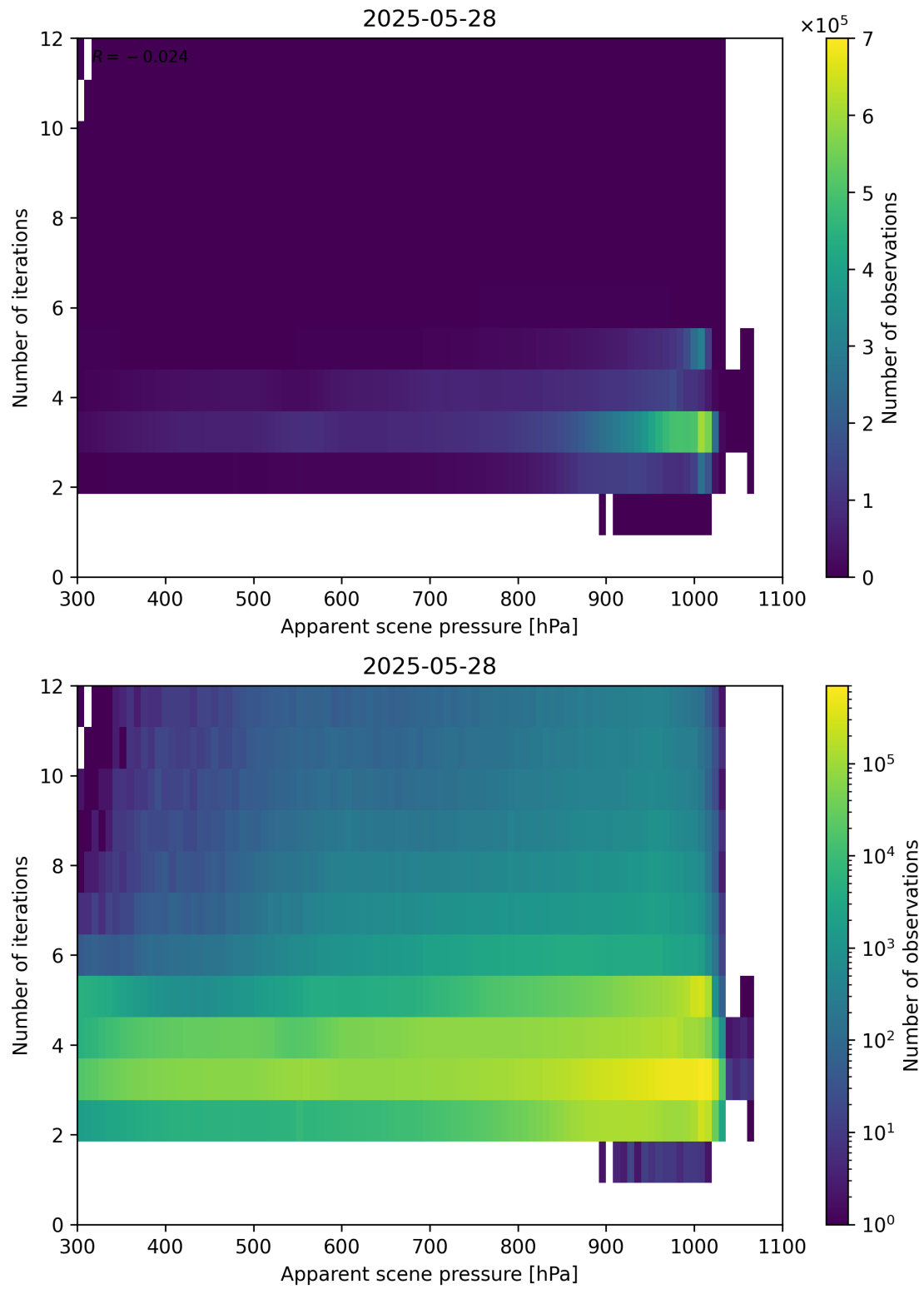
Figure 65: Scatter density plot of “Apparent scene pressure” against “Number of iterations” for 2025-05-27 to 2025-05-29.
