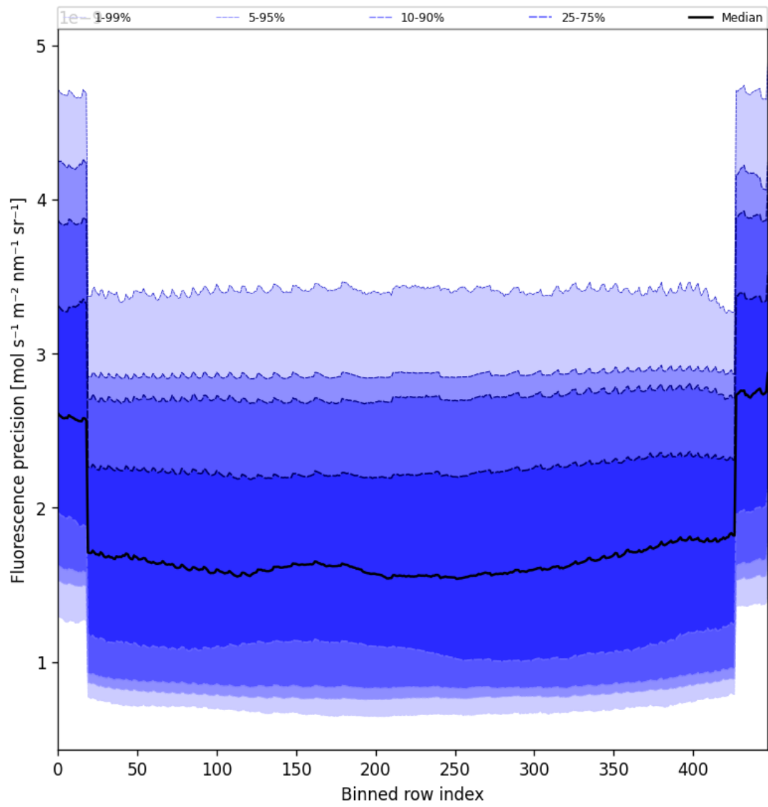
Figure 58: Along track statistics of “Fluorescence precision” for 2025-05-27 to 2025-05-29
