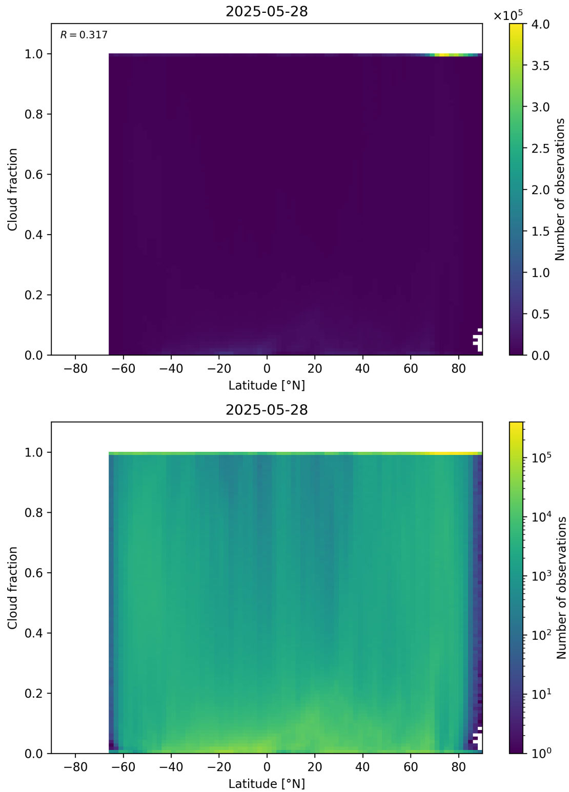
Figure 90: Scatter density plot of “Latitude” against “Cloud fraction” for 2025-05-27 to 2025-05-29.
