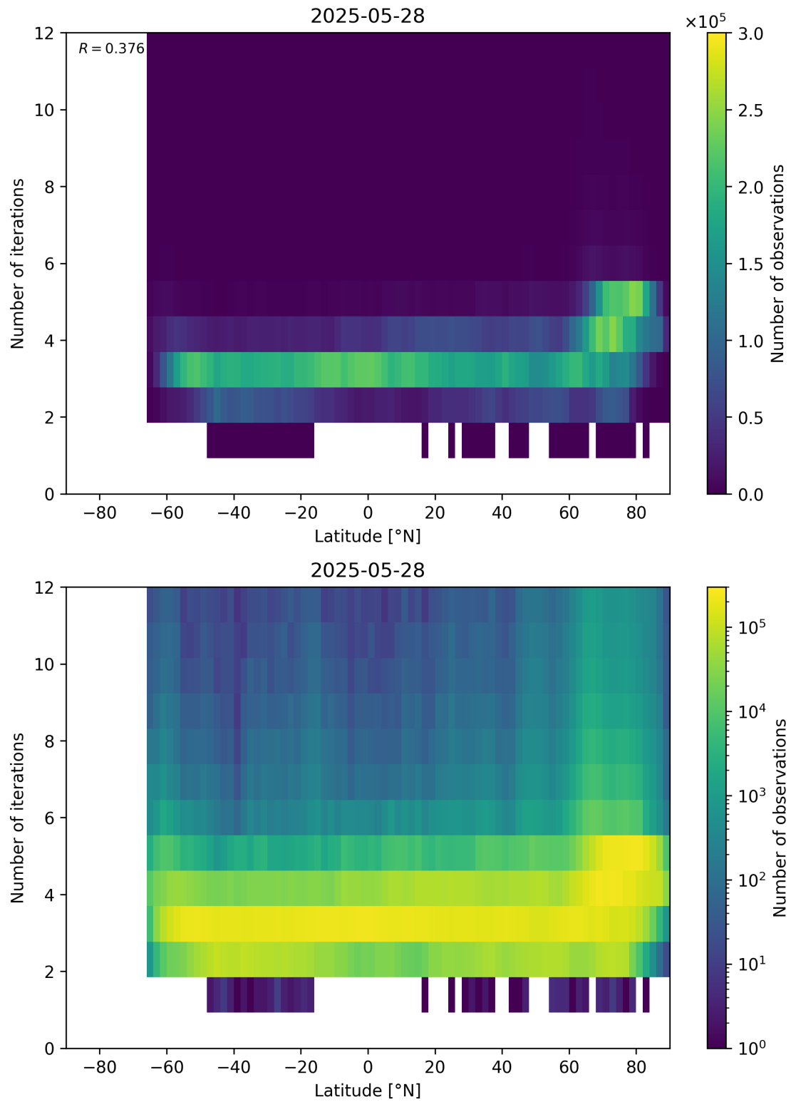
Figure 93: Scatter density plot of “Latitude” against “Number of iterations” for 2025-05-27 to 2025-05-29.
