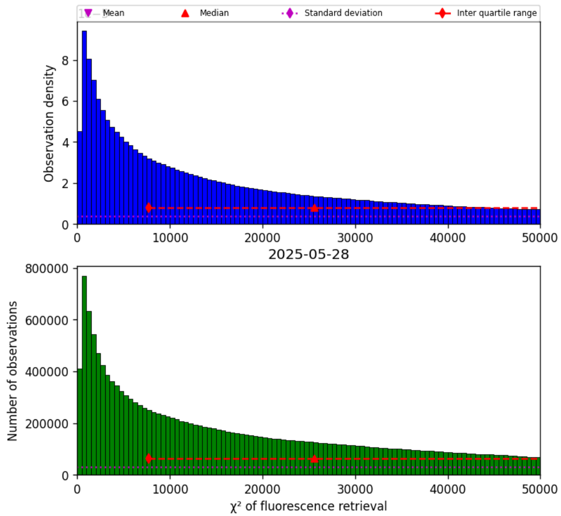
Figure 42: Histogram of “ \chi^2 of fluorescence retrieval” for 2025-05-27 to 2025-05-29
