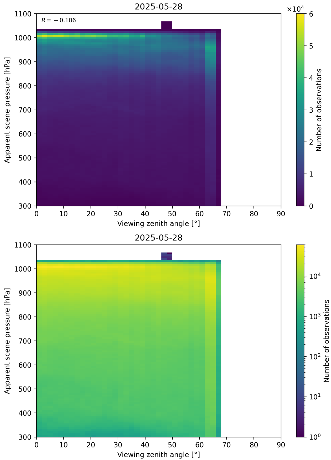
Figure 118: Scatter density plot of “Viewing zenith angle” against “Apparent scene pressure” for 2025-05-27 to 2025-05-29.
