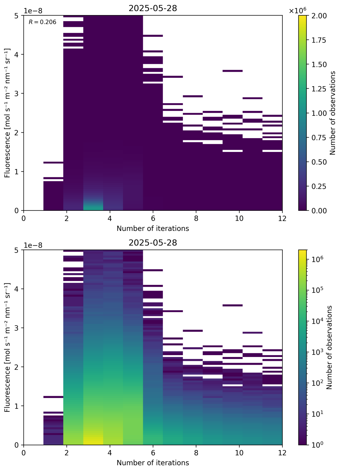
Figure 98: Scatter density plot of “Number of iterations” against “Fluorescence” for 2025-05-27 to 2025-05-29.
