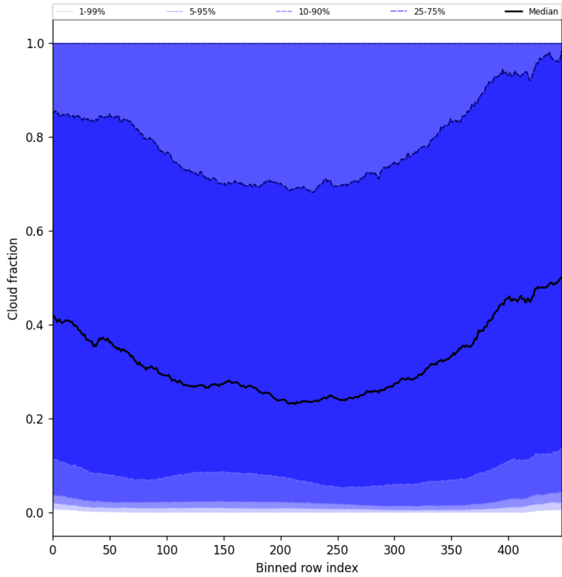
Figure 49: Along track statistics of “Cloud fraction” for 2025-05-27 to 2025-05-29
