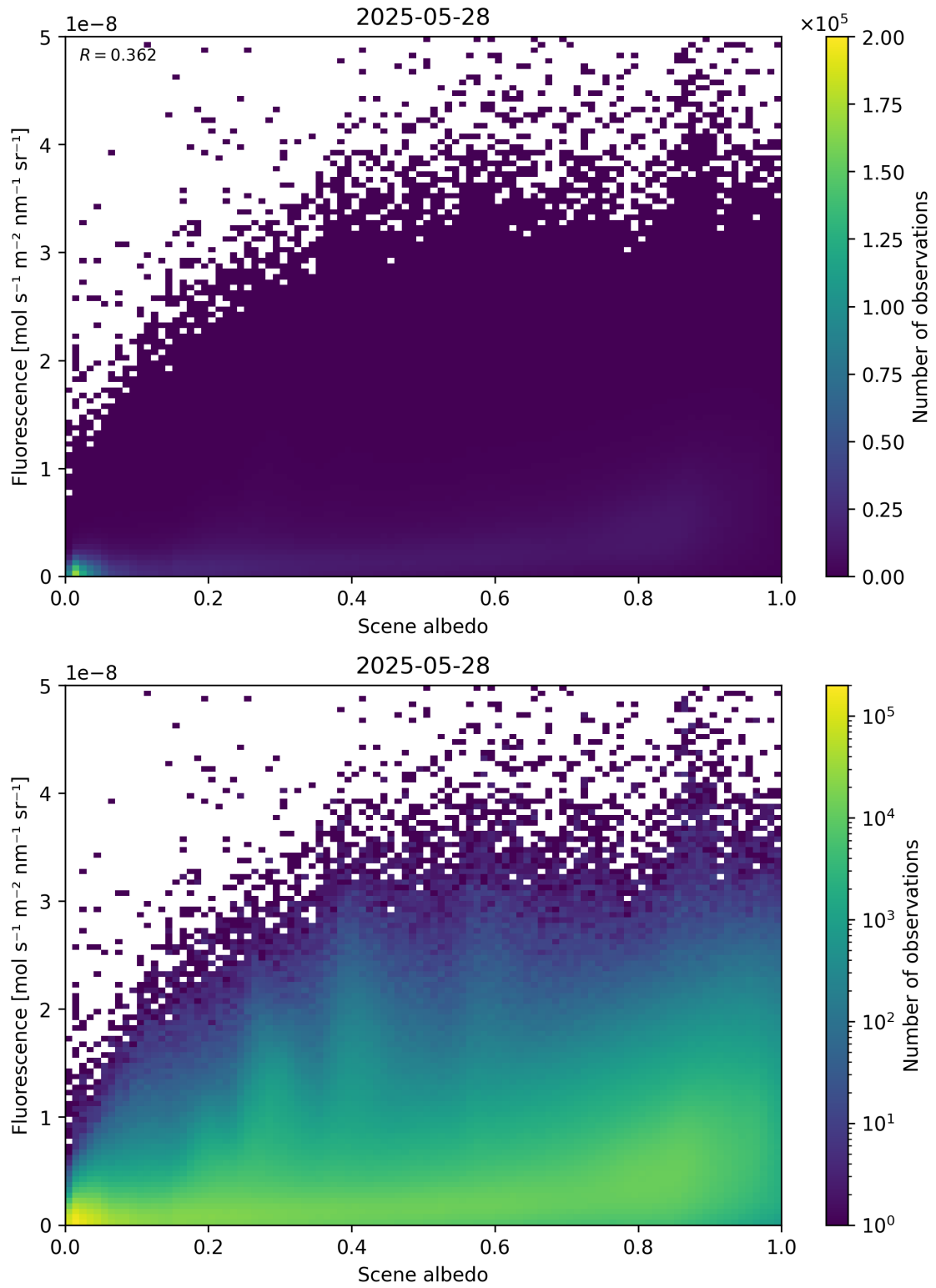
Figure 104: Scatter density plot of “Scene albedo” against “Fluorescence” for 2025-05-27 to 2025-05-29.
