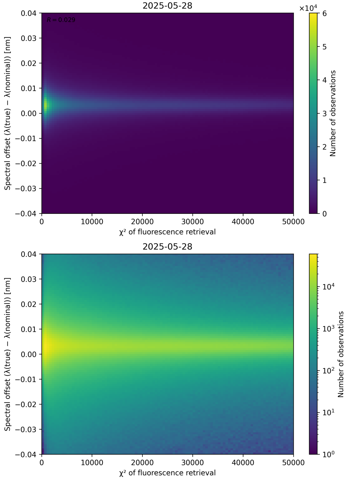
Figure 69: Scatter density plot of “ \chi^2 of fluorescence retrieval” against “Spectral offset ( \lambda_{\text{true}} - \lambda_{\text{nominal}} )” for 2025-05-27 to 2025-05-29.
