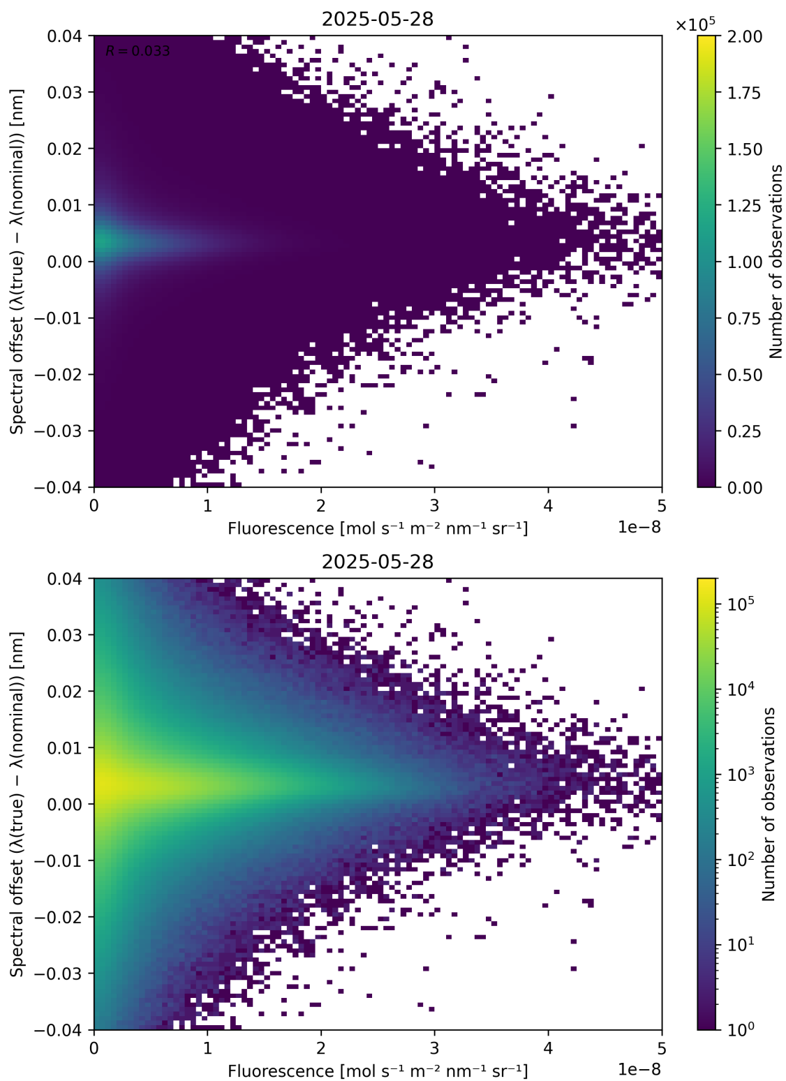
Figure 87: Scatter density plot of “Fluorescence” against “Spectral offset ( \lambda_{\text{true}} - \lambda_{\text{nominal}} )” for 2025-05-27 to 2025-05-29.
