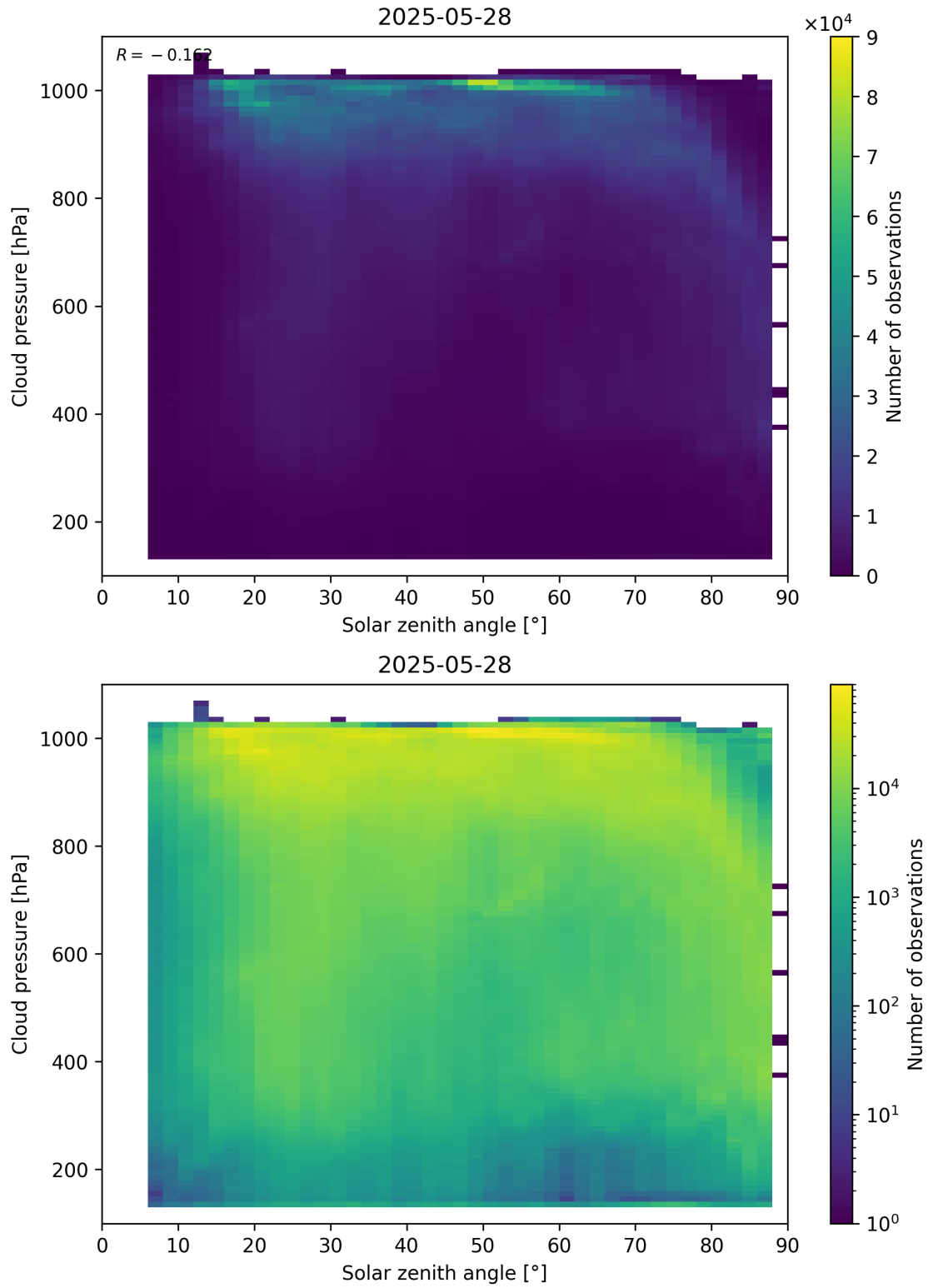
Figure 111: Scatter density plot of “Solar zenith angle” against “Cloud pressure” for 2025-05-27 to 2025-05-29.
