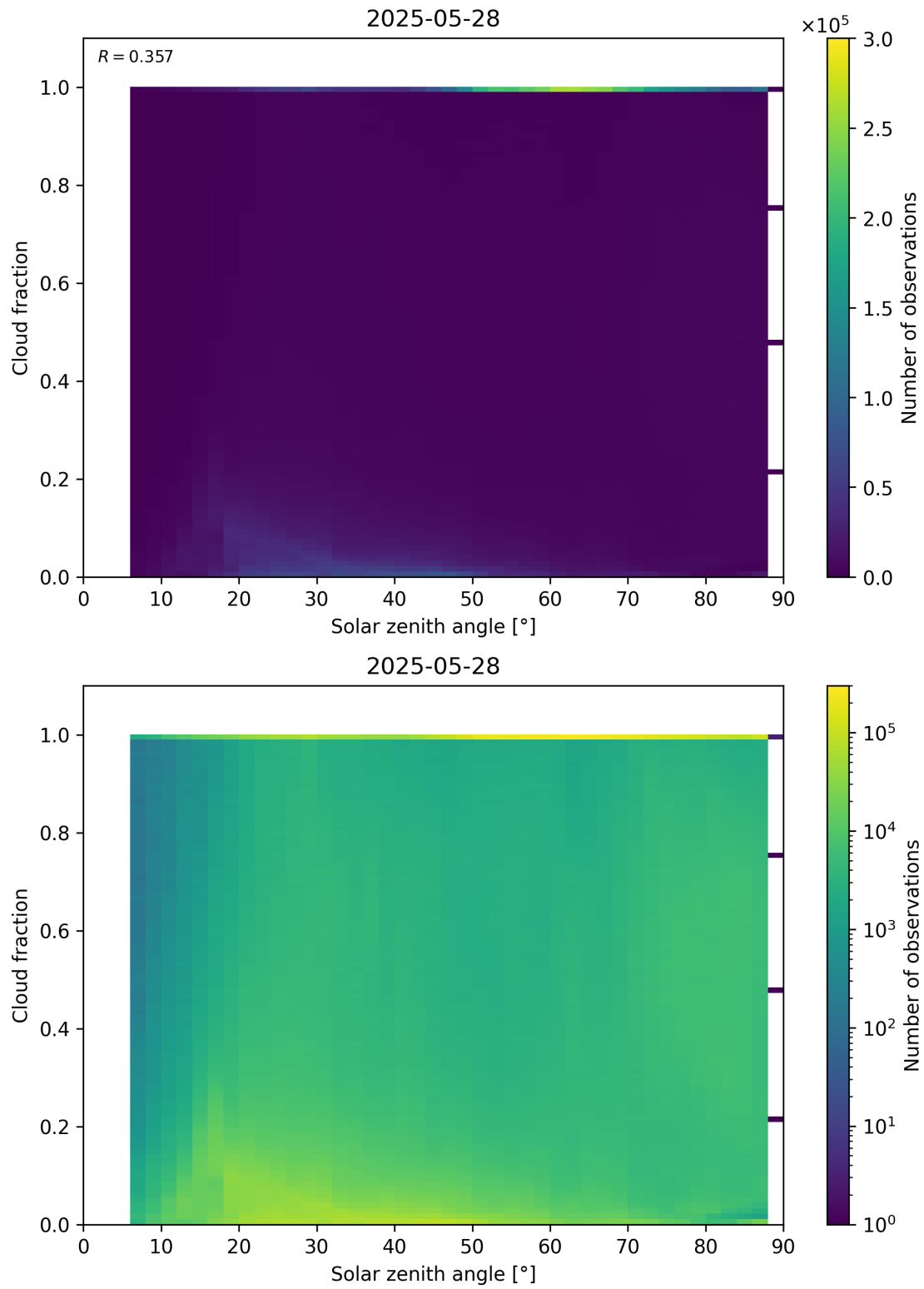
Figure 110: Scatter density plot of “Solar zenith angle” against “Cloud fraction” for 2025-05-27 to 2025-05-29.
