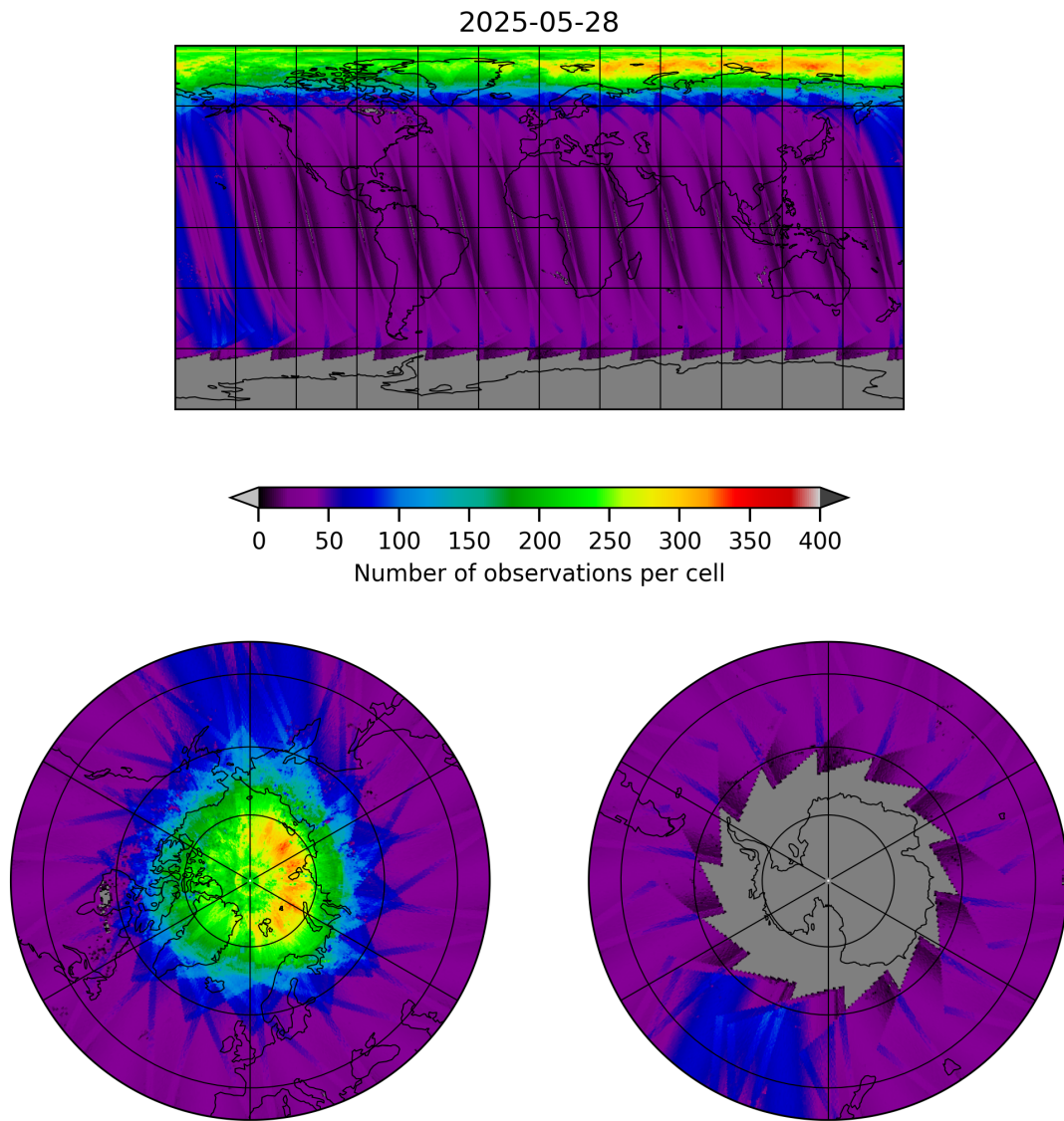
Figure 11: Map of the number of observations for 2025-05-27 to 2025-05-29
