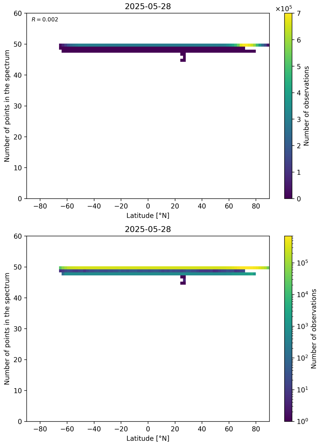
Figure 94: Scatter density plot of “Latitude” against “Number of points in the spectrum” for 2025-05-27 to 2025-05-29.
