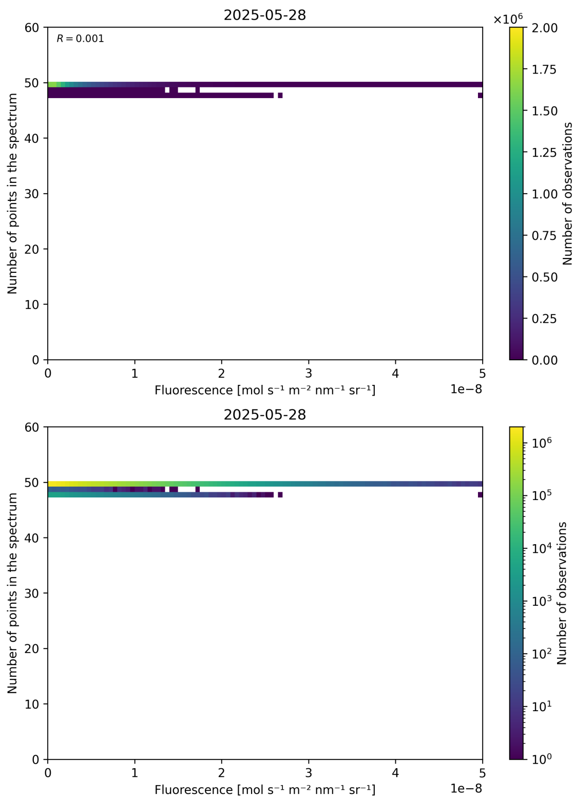
Figure 86: Scatter density plot of “Fluorescence” against “Number of points in the spectrum” for 2025-05-27 to 2025-05-29.
