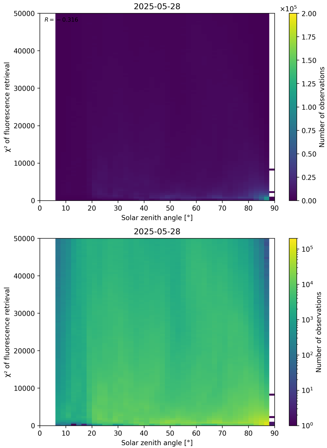
Figure 109: Scatter density plot of “Solar zenith angle” against “ \chi^2 of fluorescence retrieval” for 2025-05-27 to 2025-05-29.
