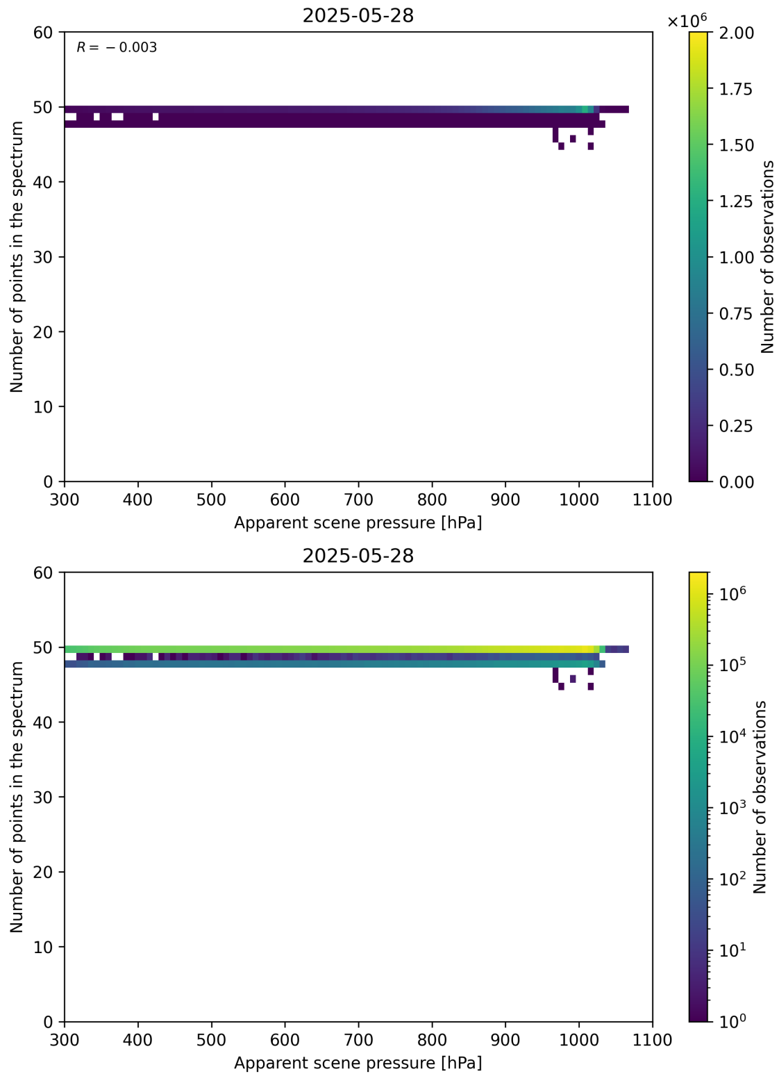
Figure 66: Scatter density plot of “Apparent scene pressure” against “Number of points in the spectrum” for 2025-05-27 to 2025-05-29.
