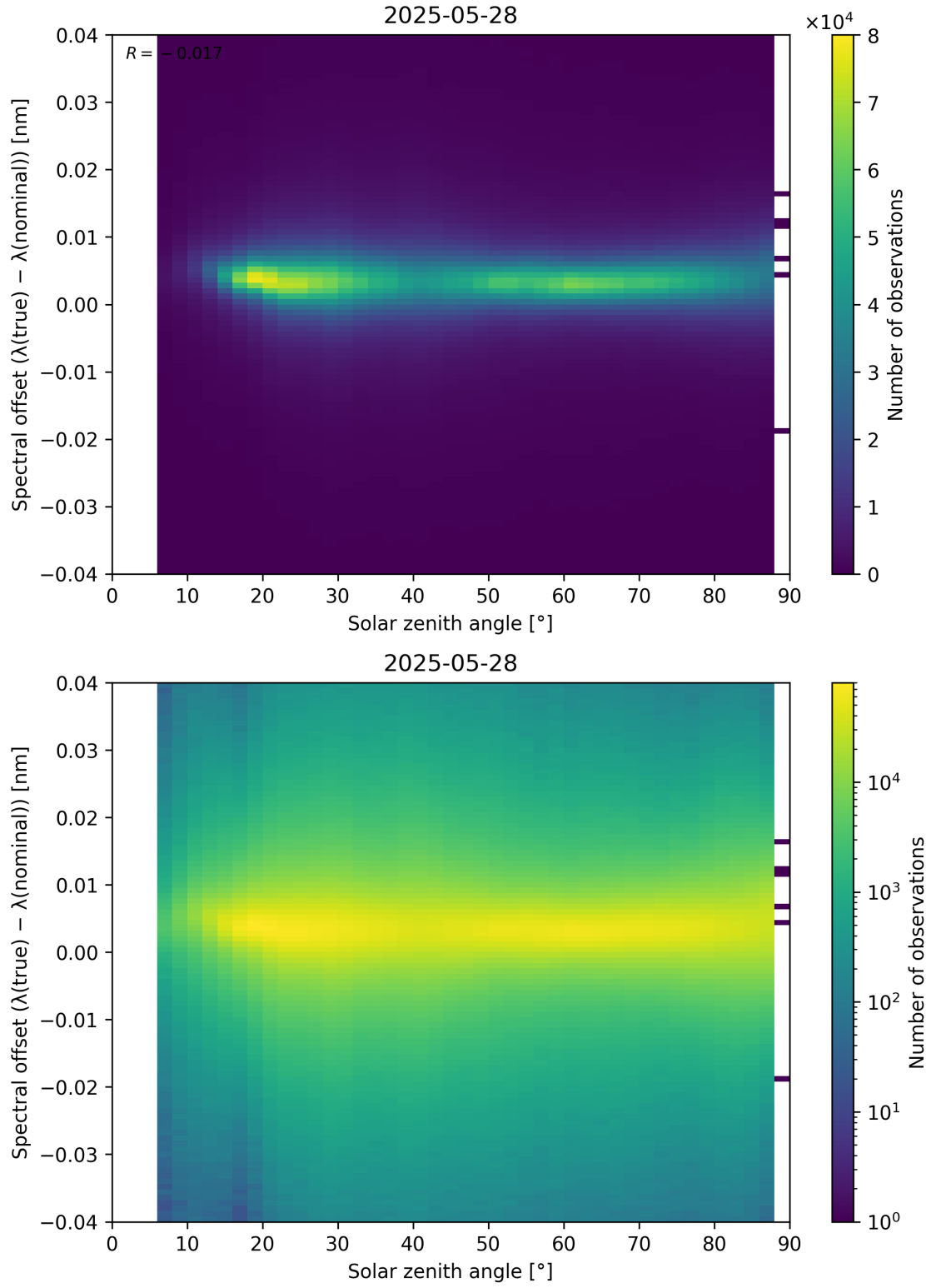
Figure 117: Scatter density plot of “Solar zenith angle” against “Spectral offset ( \lambda_{\text{true}} - \lambda_{\text{nominal}} )” for 2025-05-27 to 2025-05-29.
