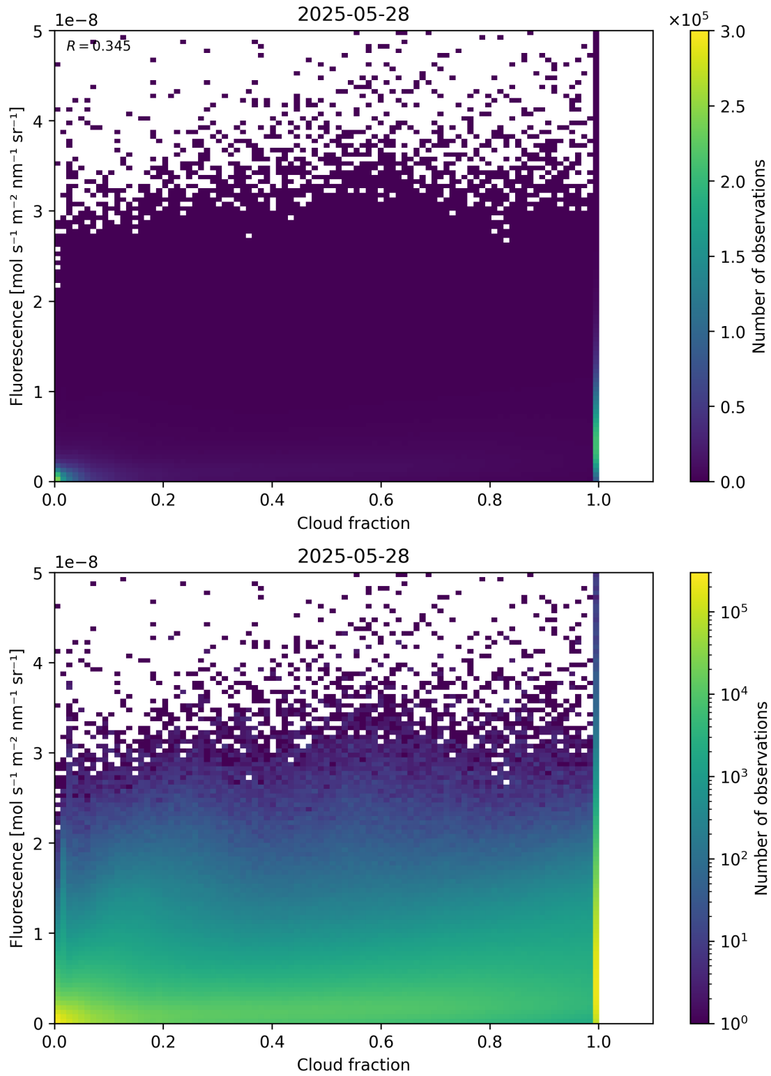
Figure 72: Scatter density plot of “Cloud fraction” against “Fluorescence” for 2025-05-27 to 2025-05-29.
