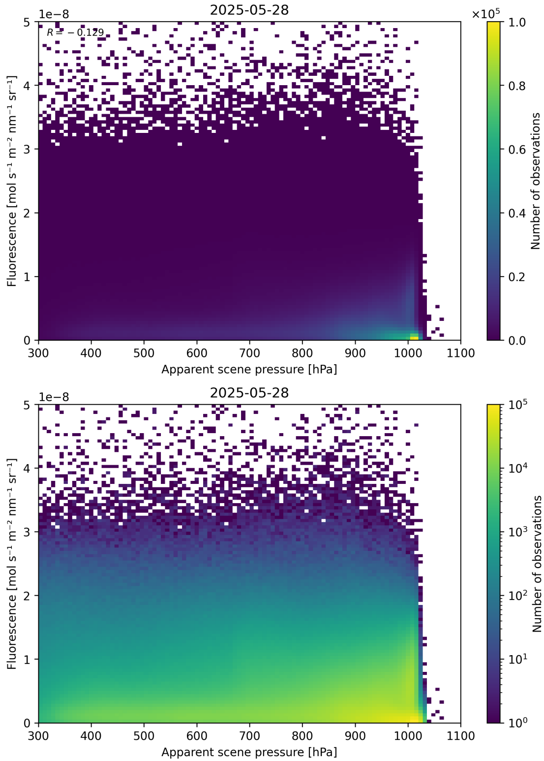
Figure 64: Scatter density plot of “Apparent scene pressure” against “Fluorescence” for 2025-05-27 to 2025-05-29.
