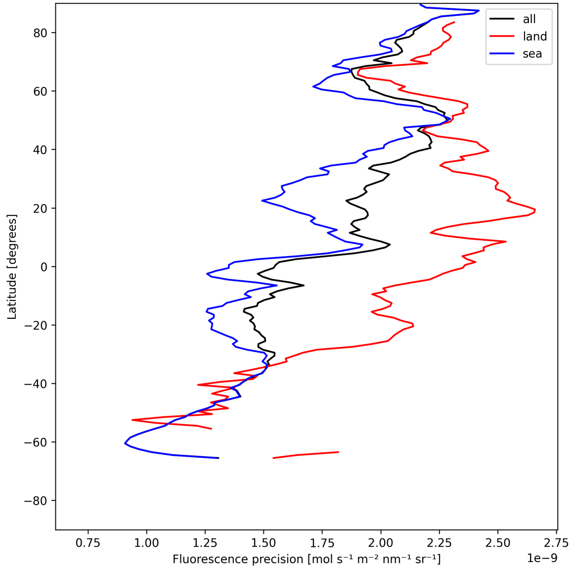
Figure 24: Zonal average of “Fluorescence precision” for 2025-05-27 to 2025-05-29.
