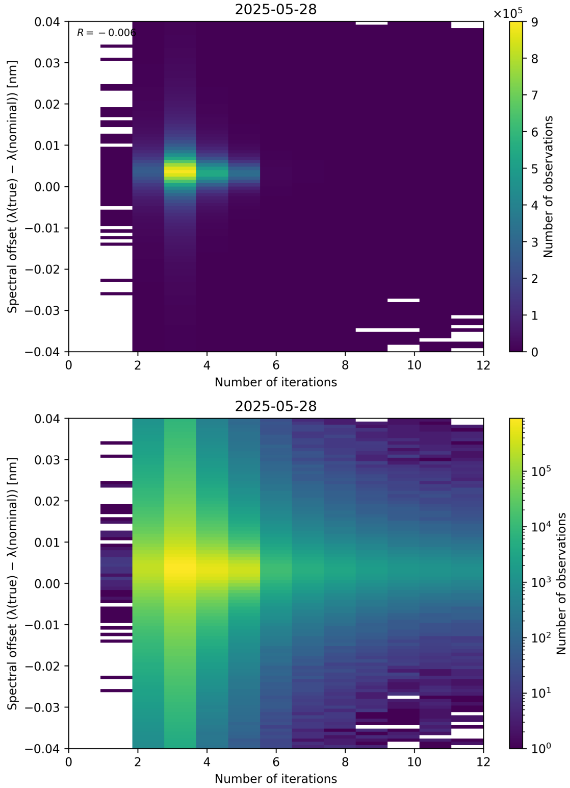
Figure 100: Scatter density plot of “Number of iterations” against “Spectral offset ( \lambda_{\text{true}} - \lambda_{\text{nominal}} )” for 2025-05-27 to 2025-05-29.
