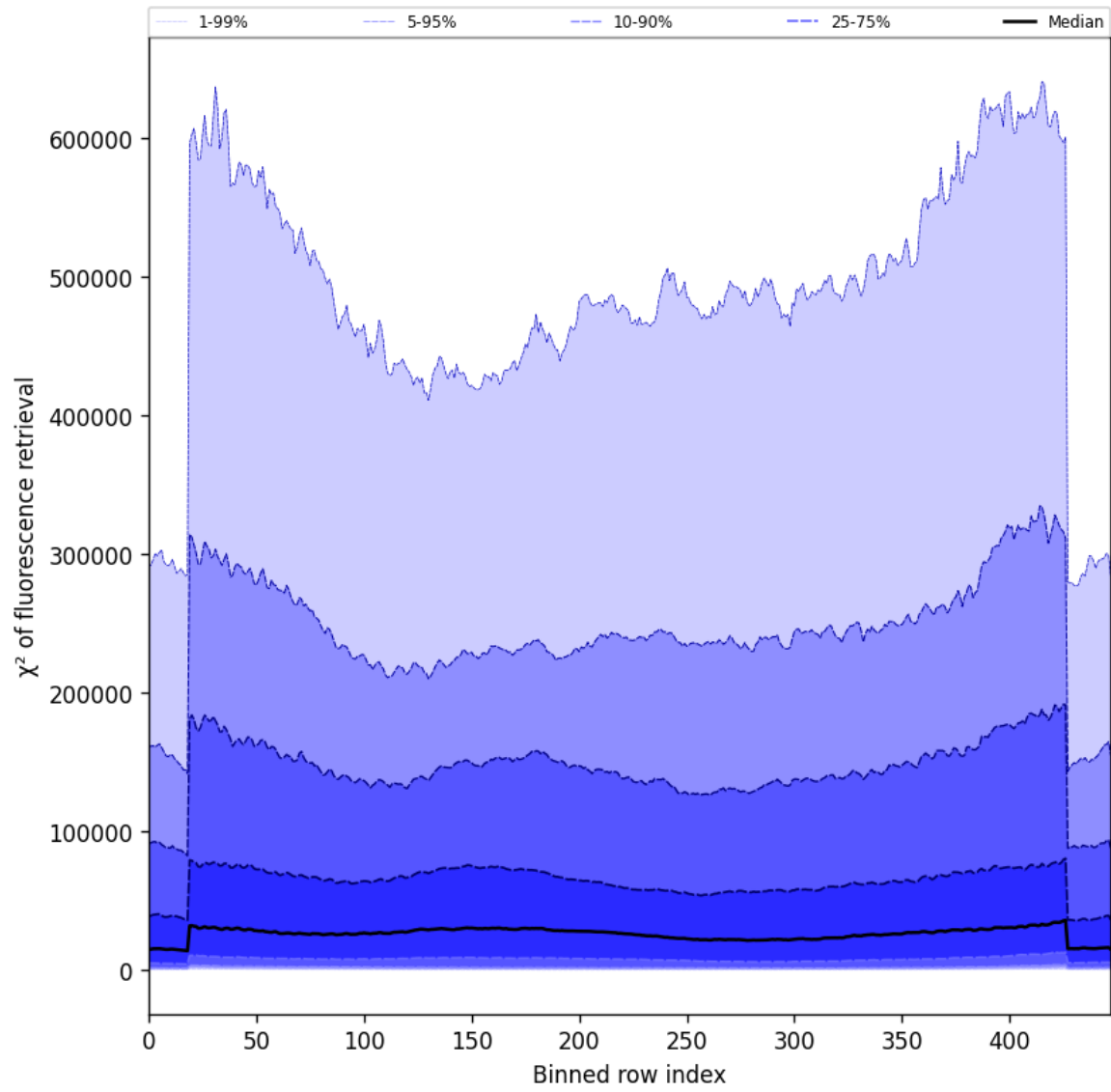
Figure 59: Along track statistics of “ \chi^2 of fluorescence retrieval” for 2025-05-27 to 2025-05-29
