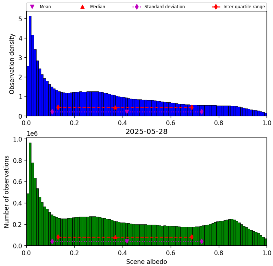
Figure 34: Histogram of “Scene albedo” for 2025-05-27 to 2025-05-29
