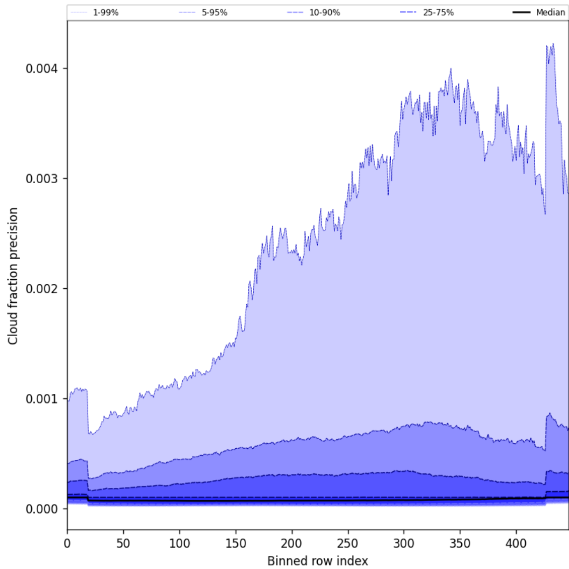
Figure 50: Along track statistics of “Cloud fraction precision” for 2025-05-27 to 2025-05-29
