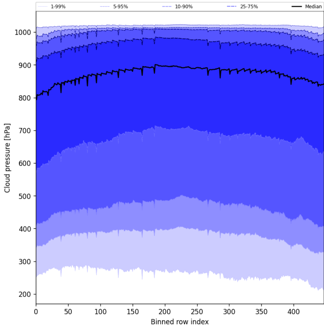
Figure 47: Along track statistics of “Cloud pressure” for 2025-05-27 to 2025-05-29
