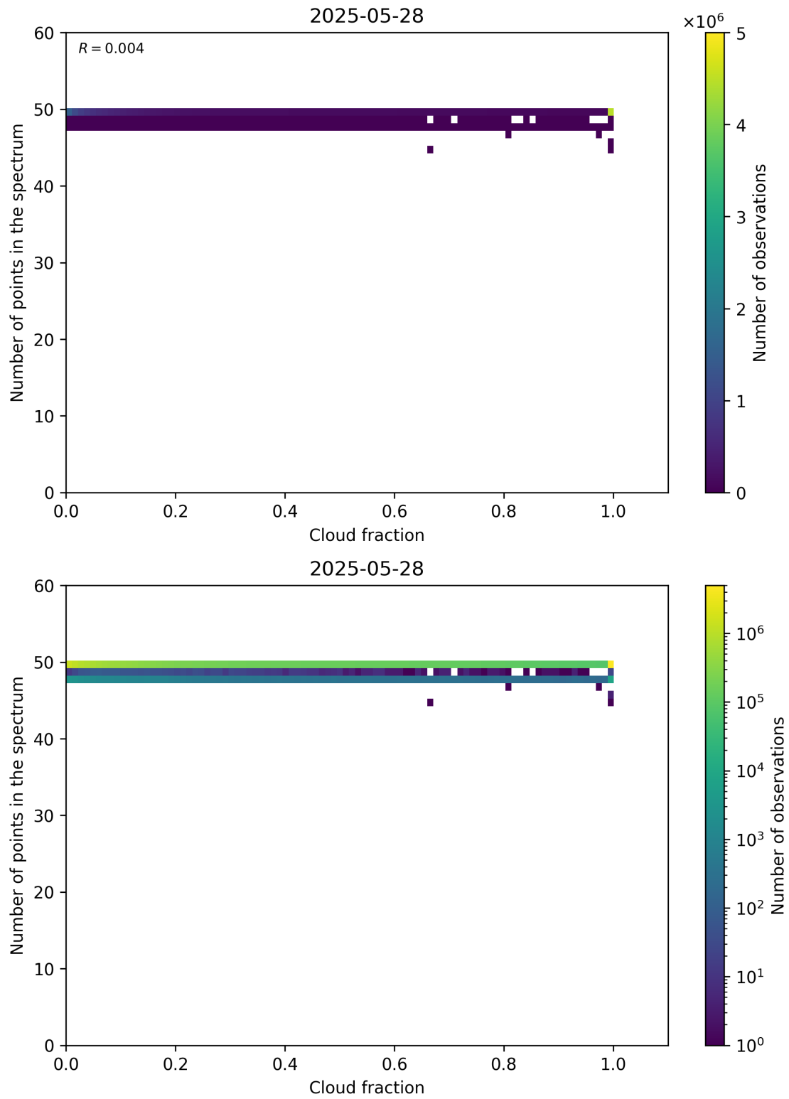
Figure 74: Scatter density plot of “Cloud fraction” against “Number of points in the spectrum” for 2025-05-27 to 2025-05-29.
