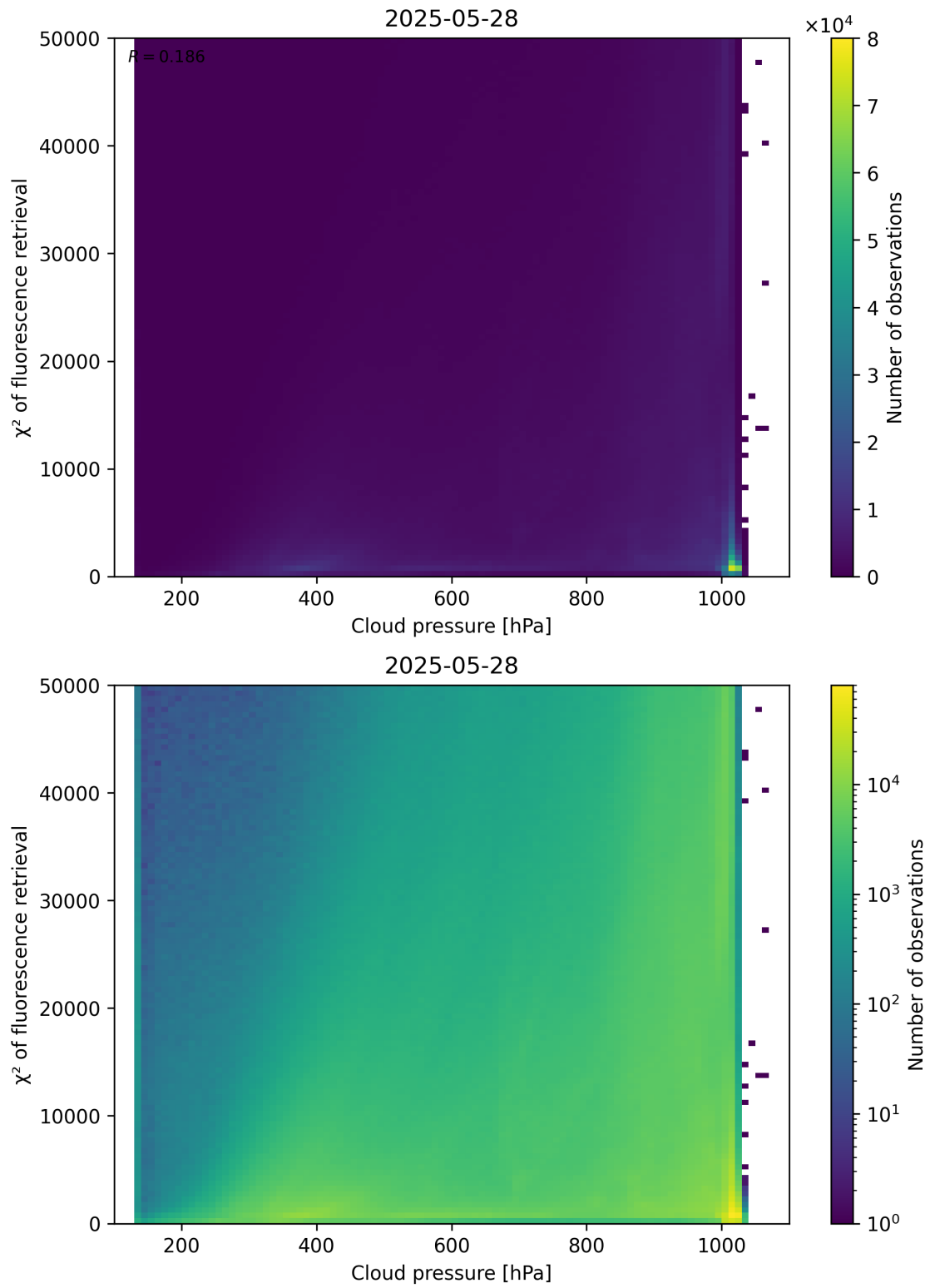
Figure 78: Scatter density plot of “Cloud pressure” against “ \chi^2 of fluorescence retrieval” for 2025-05-27 to 2025-05-29.
