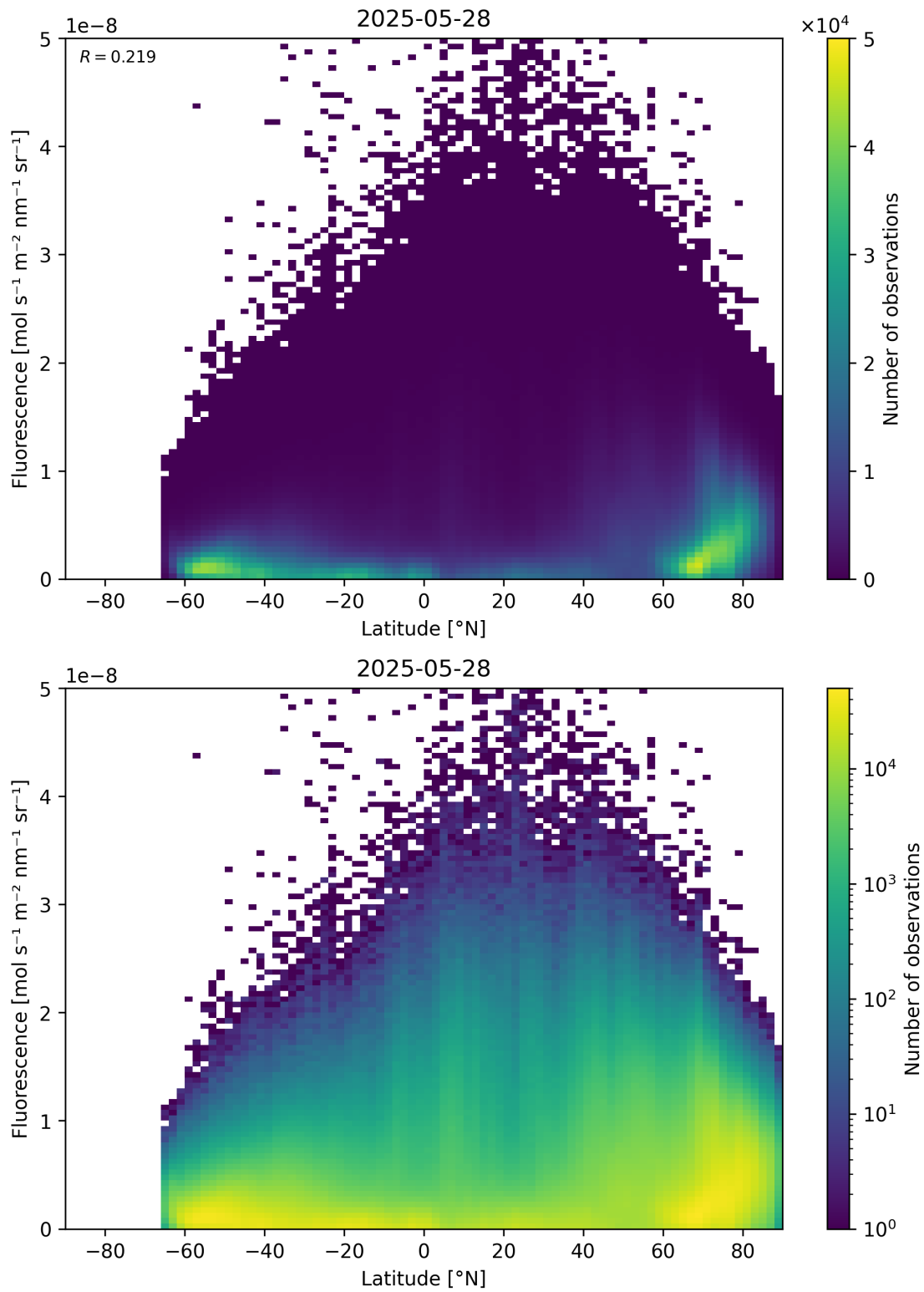
Figure 92: Scatter density plot of “Latitude” against “Fluorescence” for 2025-05-27 to 2025-05-29.
