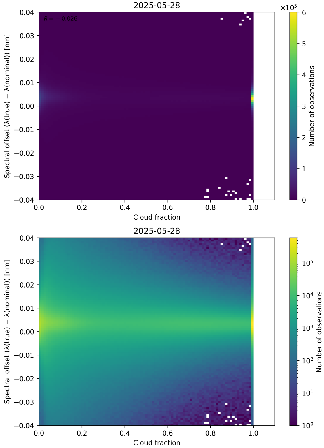
Figure 76: Scatter density plot of “Cloud fraction” against “Spectral offset ( \lambda_{\text{true}} - \lambda_{\text{nominal}} )” for 2025-05-27 to 2025-05-29.
