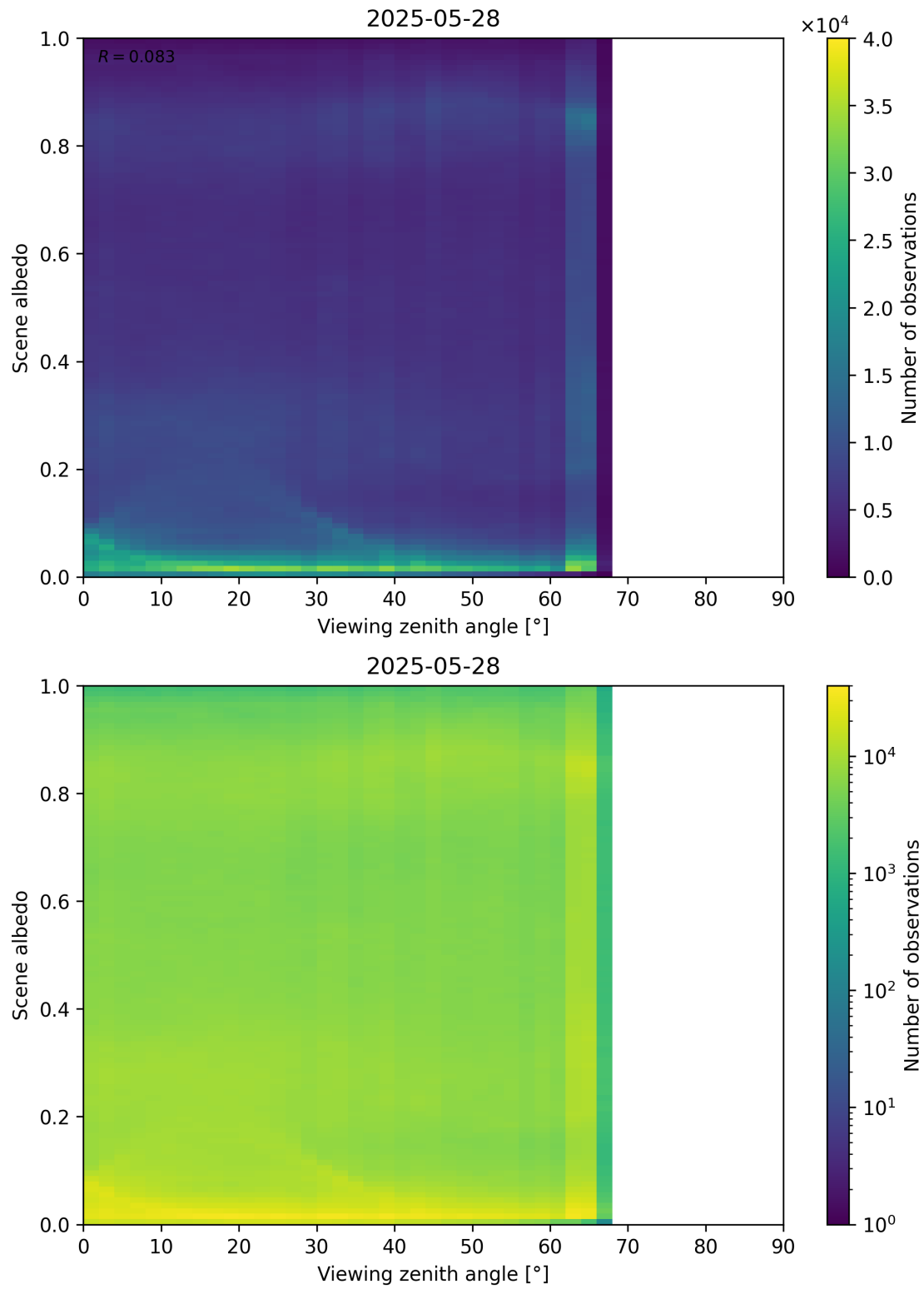
Figure 126: Scatter density plot of “Viewing zenith angle” against “Scene albedo” for 2025-05-27 to 2025-05-29.
