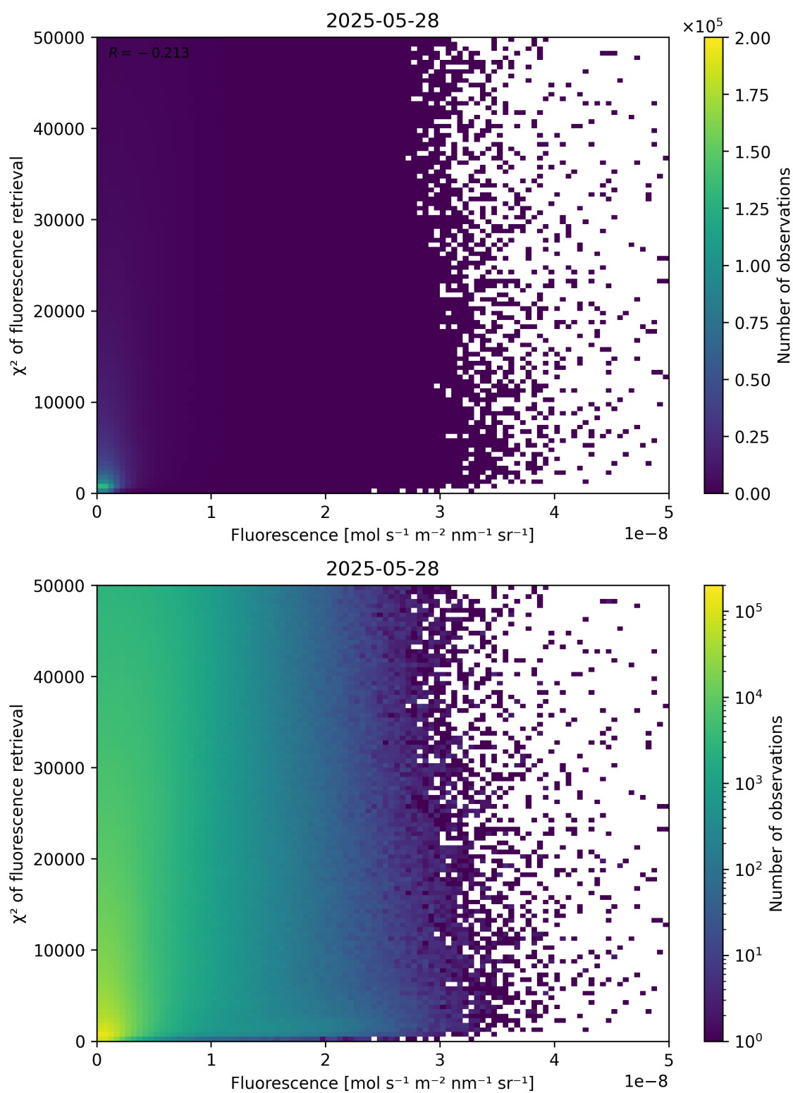
Figure 85: Scatter density plot of “Fluorescence” against “ \chi^2 of fluorescence retrieval” for 2025-05-27 to 2025-05-29.
