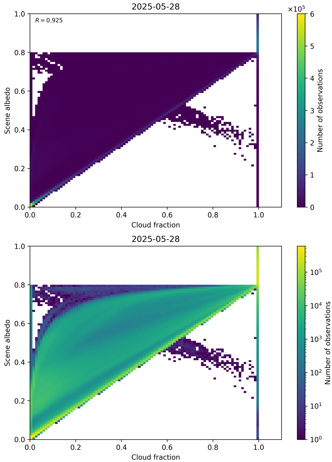
Figure 75: Scatter density plot of “Cloud fraction” against “Scene albedo” for 2025-05-27 to 2025-05-29.
