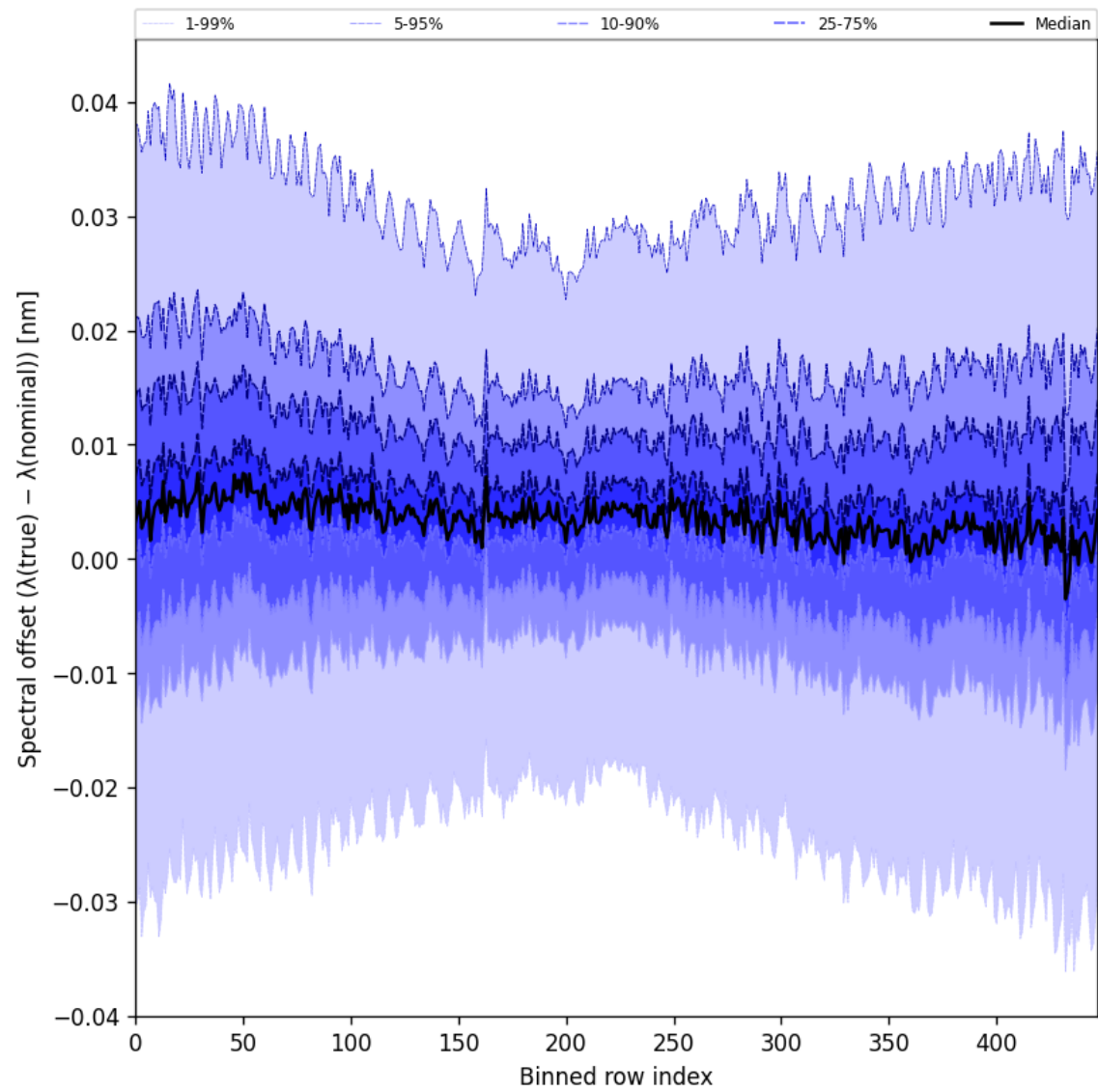
Figure 62: Along track statistics of “Spectral offset ( \lambda_{\text{true}} - \lambda_{\text{nominal}} )” for 2025-05-27 to 2025-05-29
