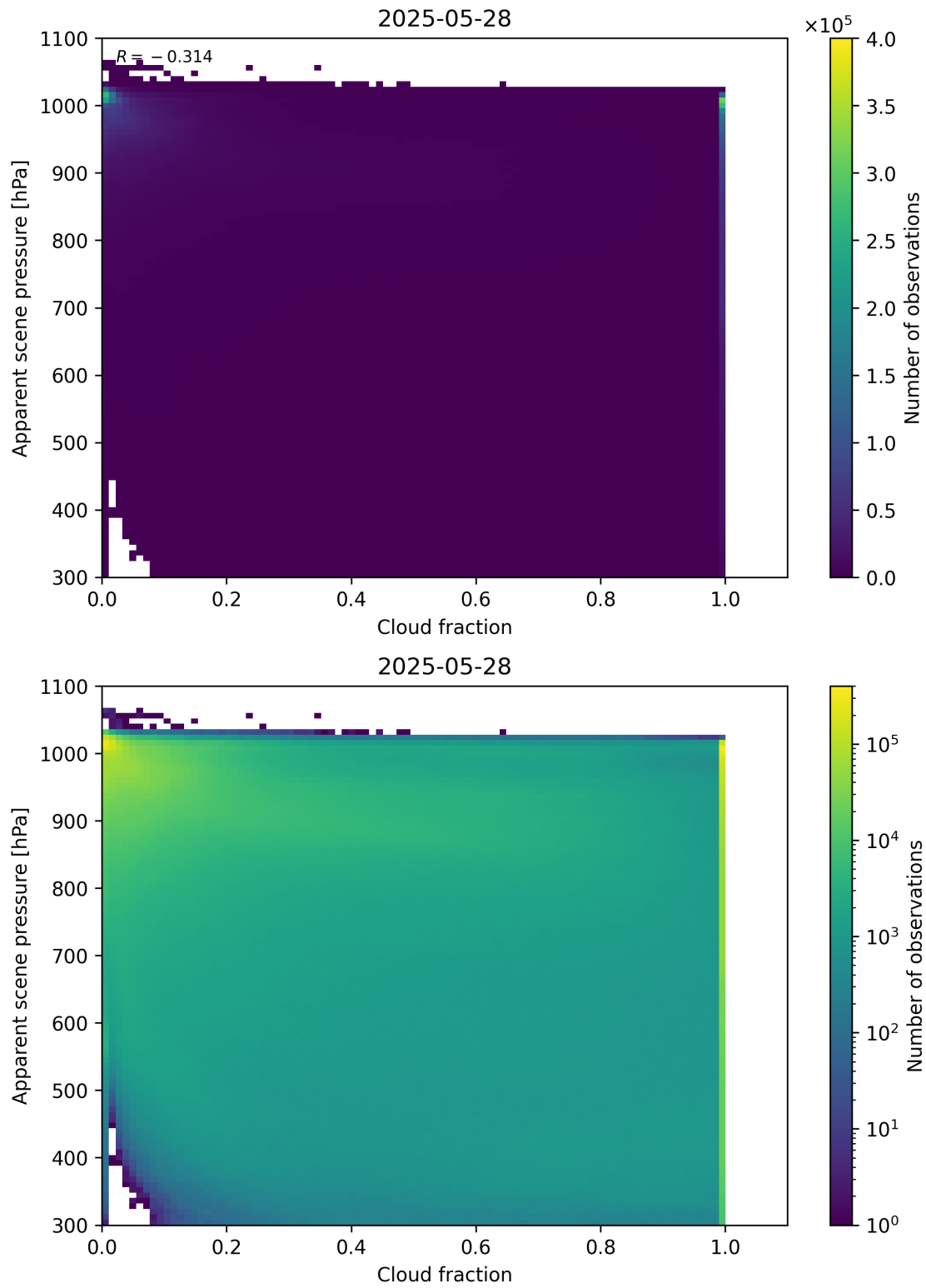
Figure 70: Scatter density plot of “Cloud fraction” against “Apparent scene pressure” for 2025-05-27 to 2025-05-29.
