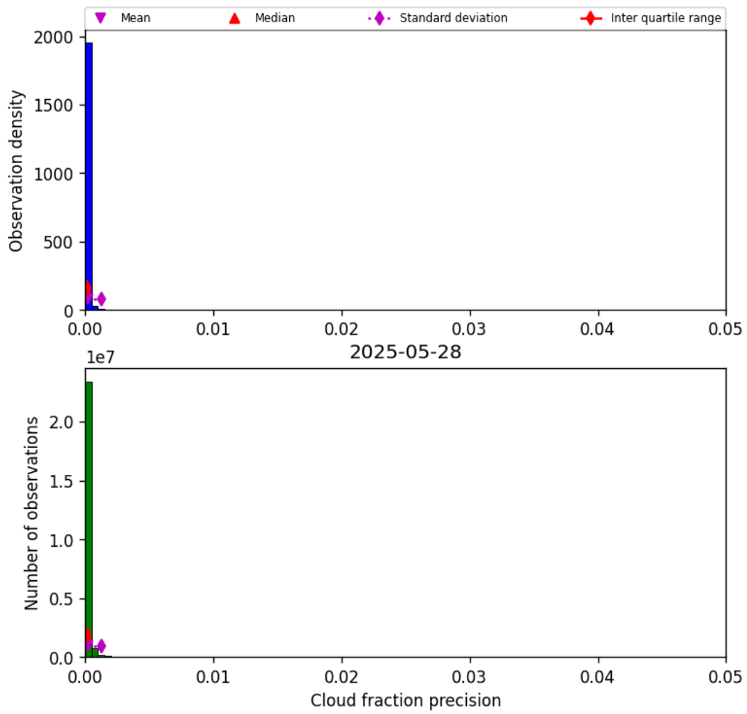
Figure 33: Histogram of “Cloud fraction precision” for 2025-05-27 to 2025-05-29
