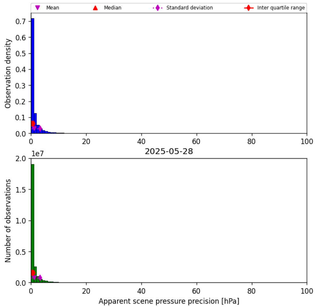
Figure 37: Histogram of "Apparent scene pressure precision" for 2025-05-27 to 2025-05-29
