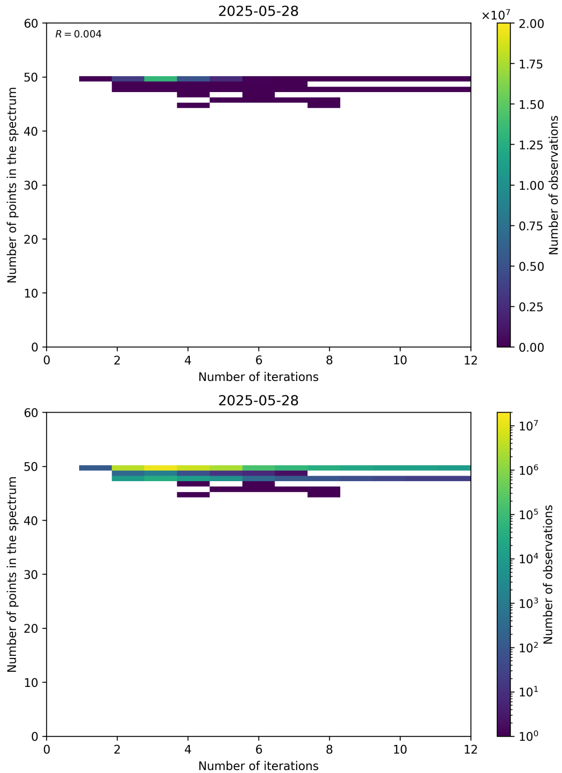
Figure 99: Scatter density plot of “Number of iterations” against “Number of points in the spectrum” for 2025-05-27 to 2025-05-29.
