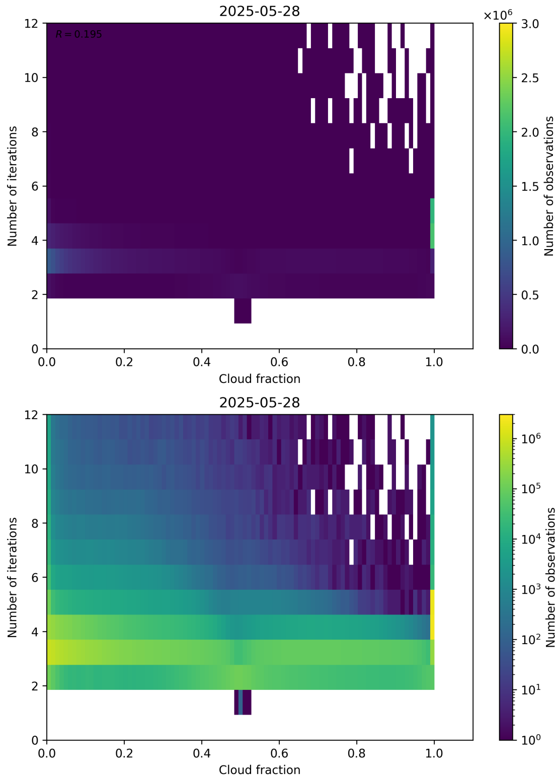
Figure 73: Scatter density plot of “Cloud fraction” against “Number of iterations” for 2025-05-27 to 2025-05-29.
