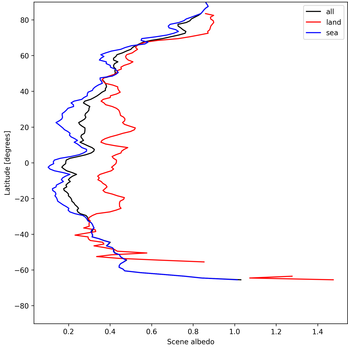
Figure 17: Zonal average of “Scene albedo” for 2025-05-27 to 2025-05-29.
