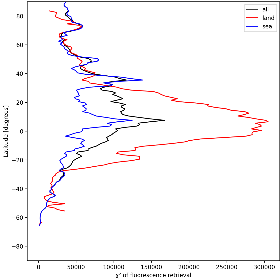
Figure 25: Zonal average of “ \chi^2 of fluorescence retrieval” for 2025-05-27 to 2025-05-29.
