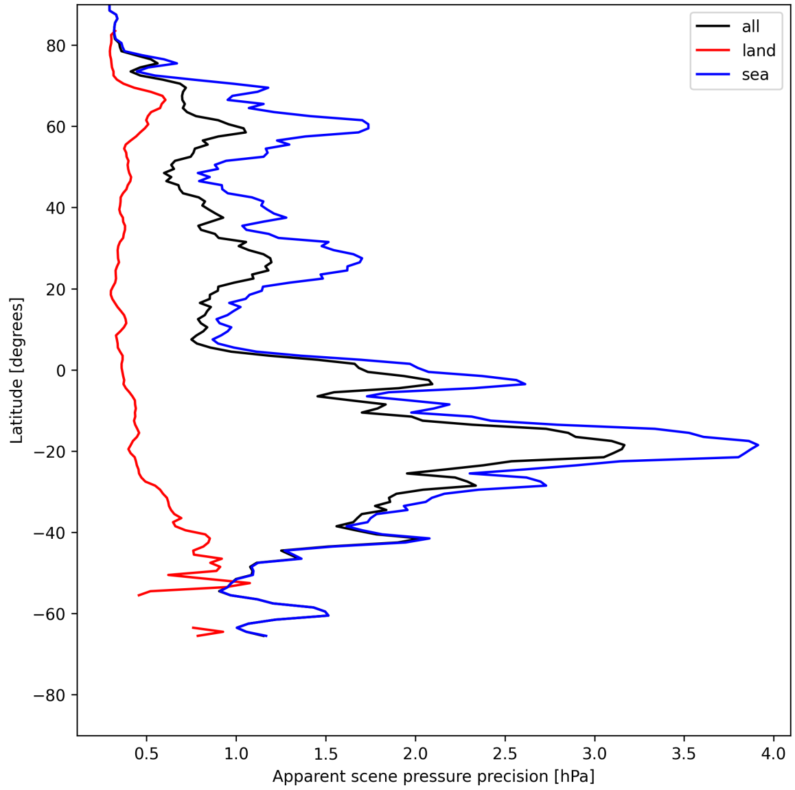
Figure 20: Zonal average of “Apparent scene pressure precision” for 2025-05-27 to 2025-05-29.
