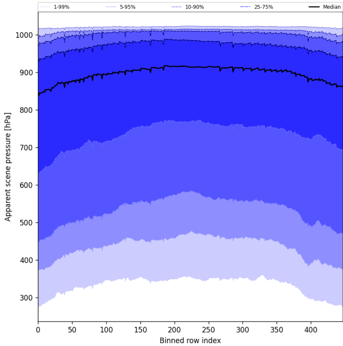
Figure 53: Along track statistics of “Apparent scene pressure” for 2025-05-27 to 2025-05-29
