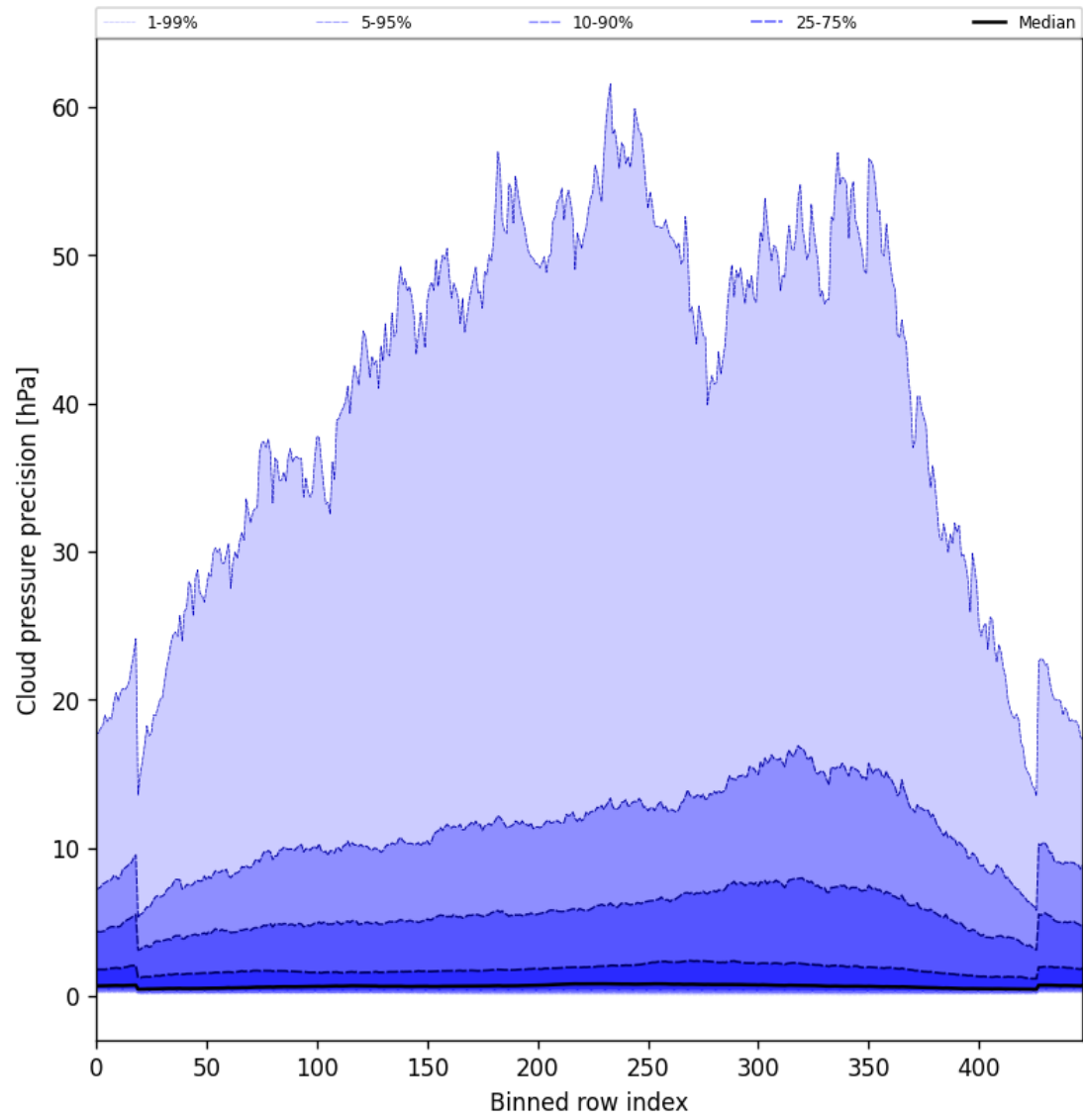
Figure 48: Along track statistics of “Cloud pressure precision” for 2025-05-27 to 2025-05-29
