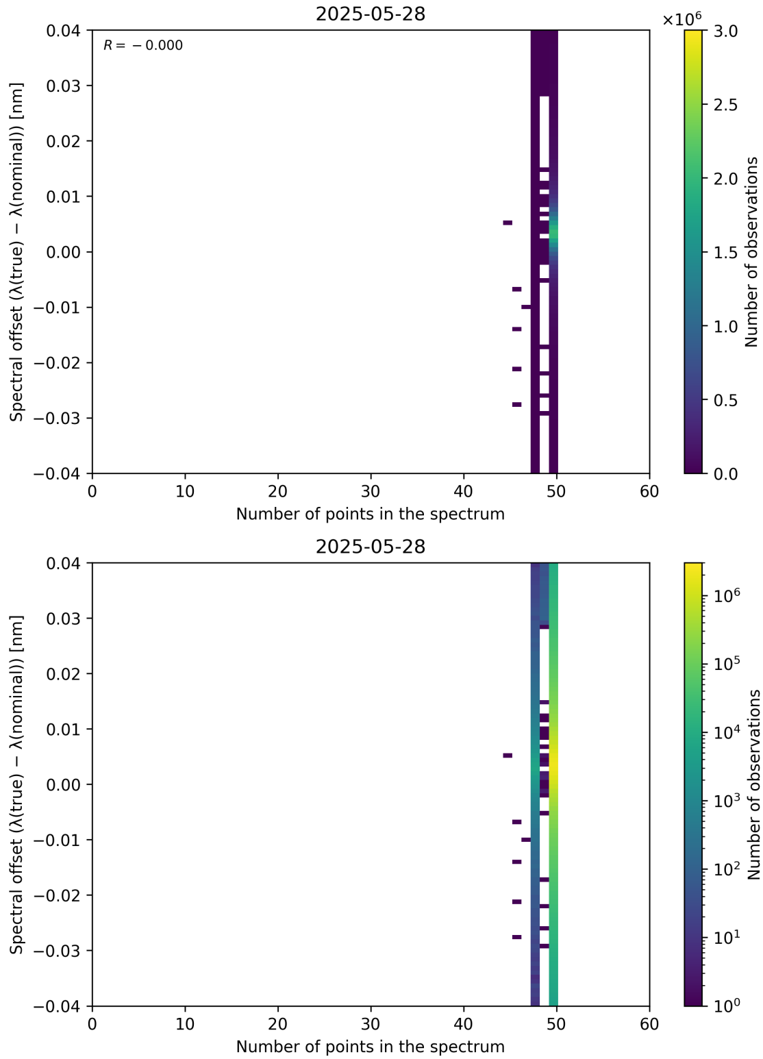
Figure 101: Scatter density plot of “Number of points in the spectrum” against “Spectral offset ( \lambda_{\text{true}} - \lambda_{\text{nominal}} )” for 2025-05-27 to 2025-05-29.
