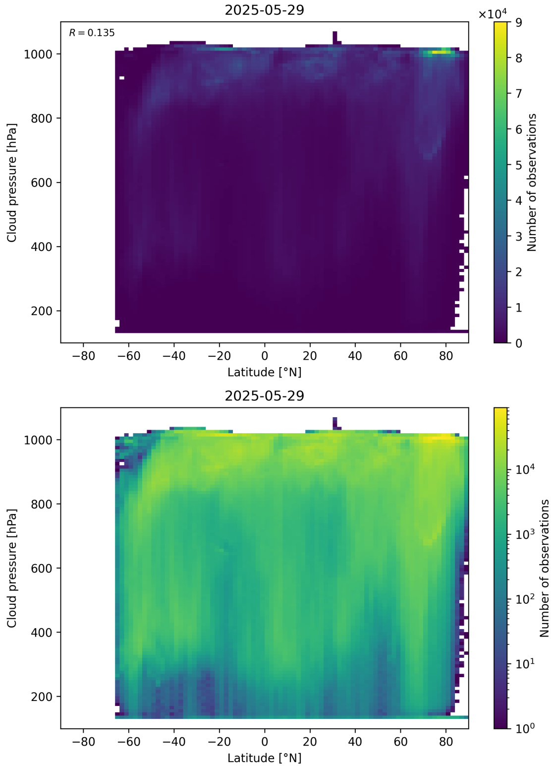
Figure 91: Scatter density plot of “Latitude” against “Cloud pressure” for 2025-05-28 to 2025-05-30.
