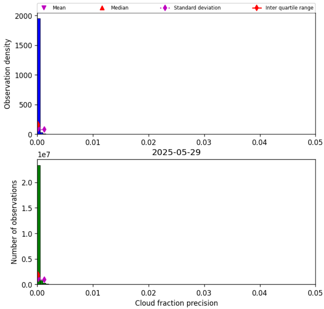
Figure 33: Histogram of “Cloud fraction precision” for 2025-05-28 to 2025-05-30
