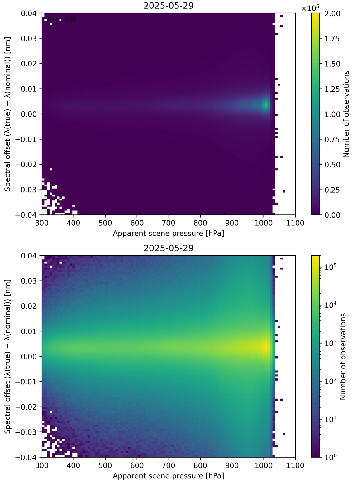
Figure 67: Scatter density plot of “Apparent scene pressure” against “Spectral offset ( \lambda_{\text{true}} - \lambda_{\text{nominal}} )” for 2025-05-28 to 2025-05-30.
