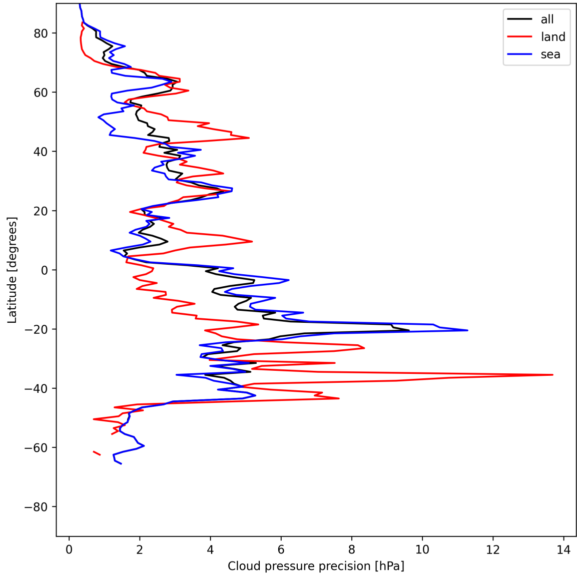
Figure 14: Zonal average of “Cloud pressure precision” for 2025-05-28 to 2025-05-30.
