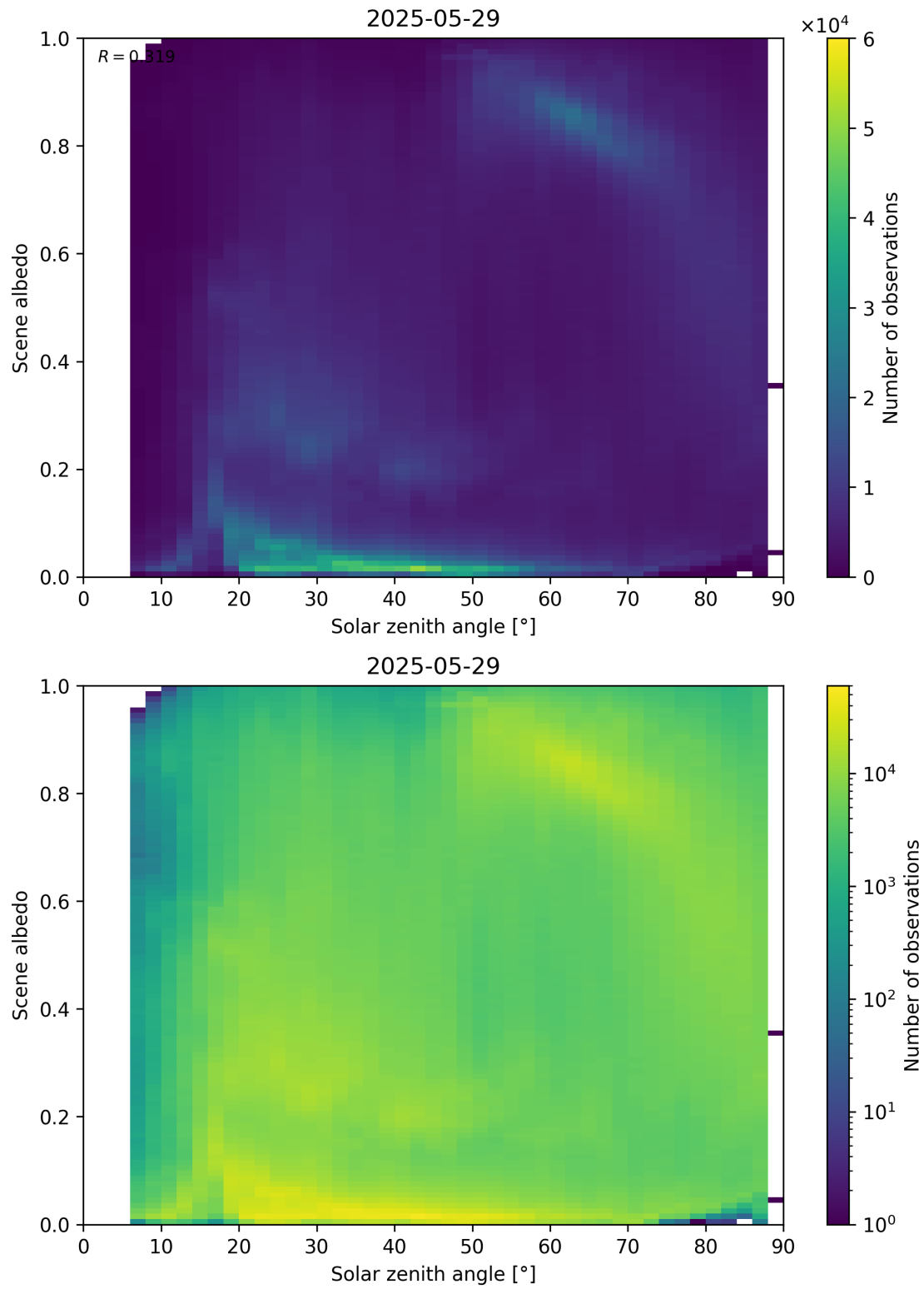
Figure 116: Scatter density plot of “Solar zenith angle” against “Scene albedo” for 2025-05-28 to 2025-05-30.
