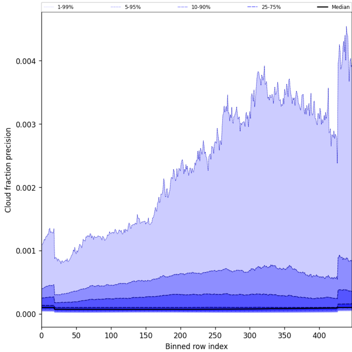
Figure 50: Along track statistics of “Cloud fraction precision” for 2025-05-28 to 2025-05-30
