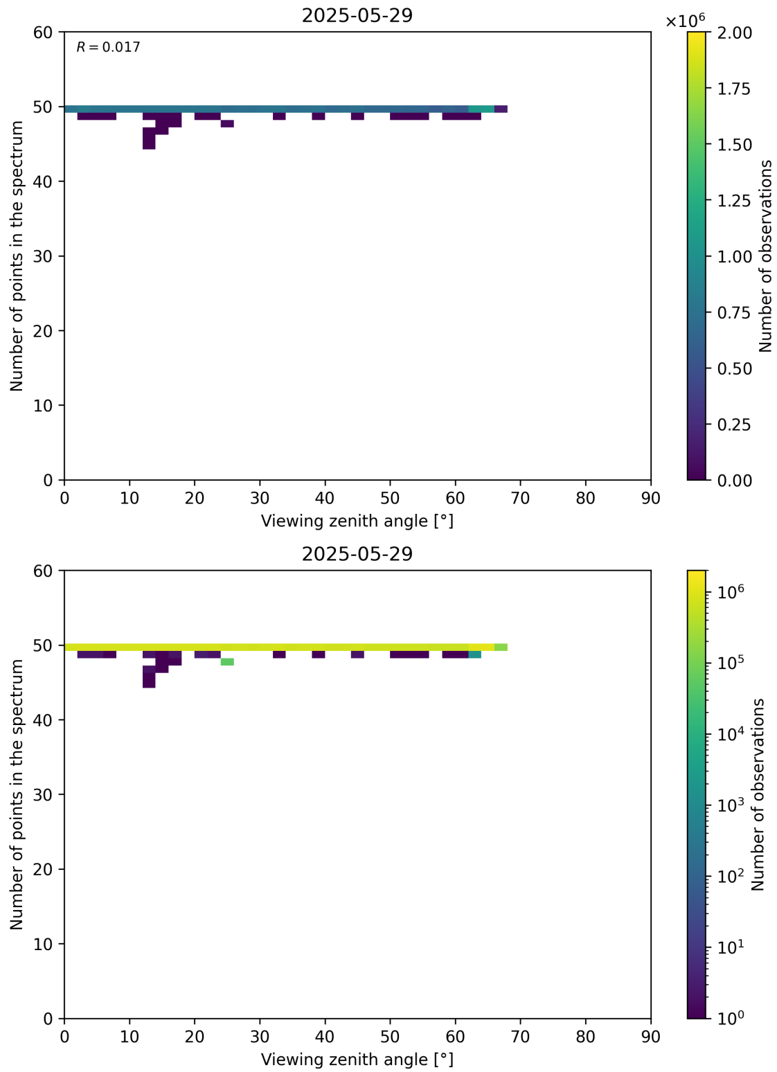
Figure 125: Scatter density plot of “Viewing zenith angle” against “Number of points in the spectrum” for 2025-05-28 to 2025-05-30.
