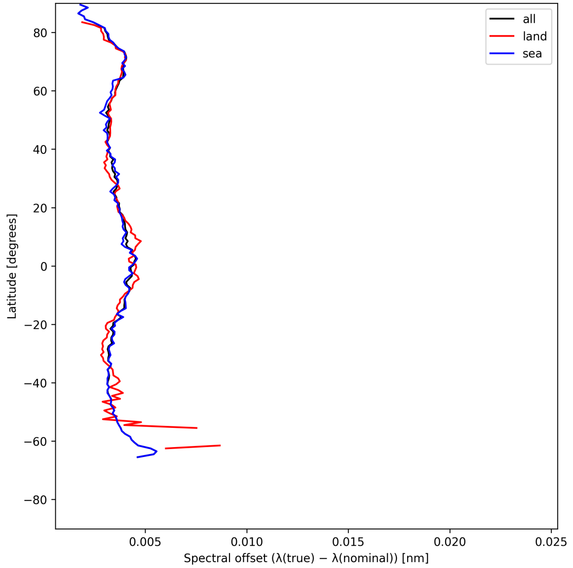
Figure 28: Zonal average of “Spectral offset ( \lambda_{\text{true}} - \lambda_{\text{nominal}} )” for 2025-05-28 to 2025-05-30.
