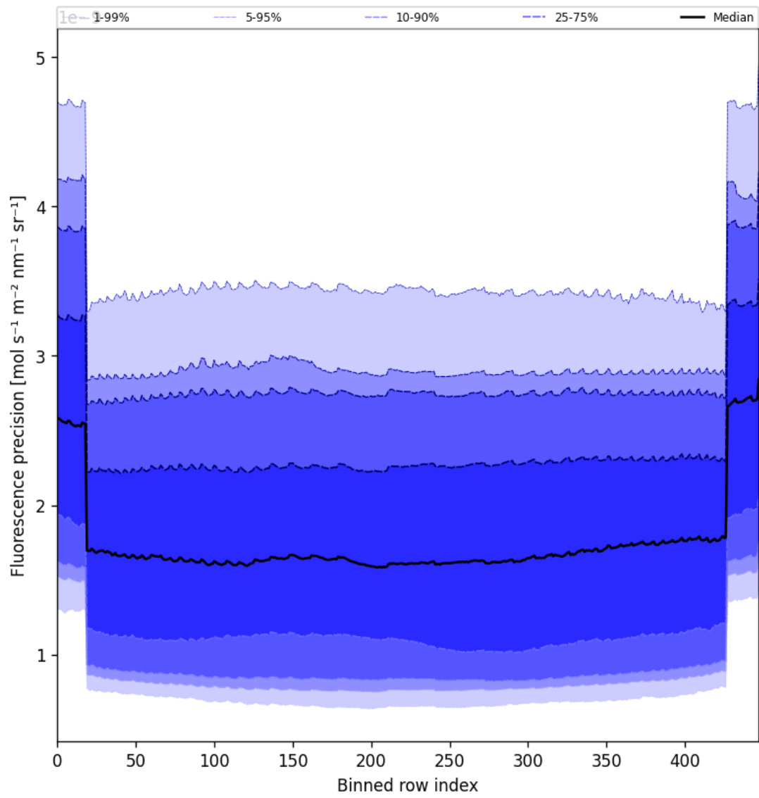
Figure 58: Along track statistics of “Fluorescence precision” for 2025-05-28 to 2025-05-30
