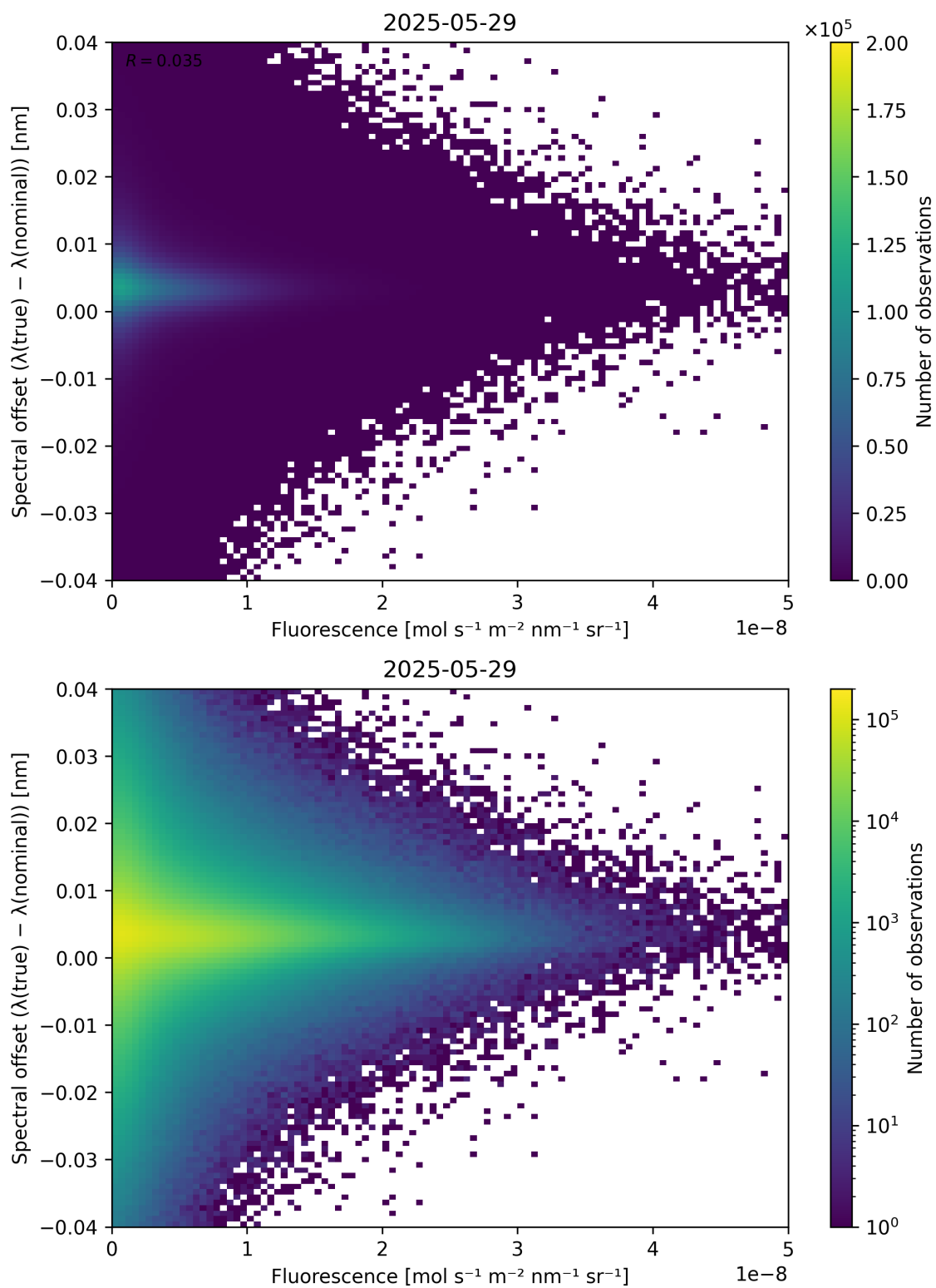
Figure 87: Scatter density plot of “Fluorescence” against “Spectral offset ( \lambda_{\text{true}} - \lambda_{\text{nominal}} )” for 2025-05-28 to 2025-05-30.
