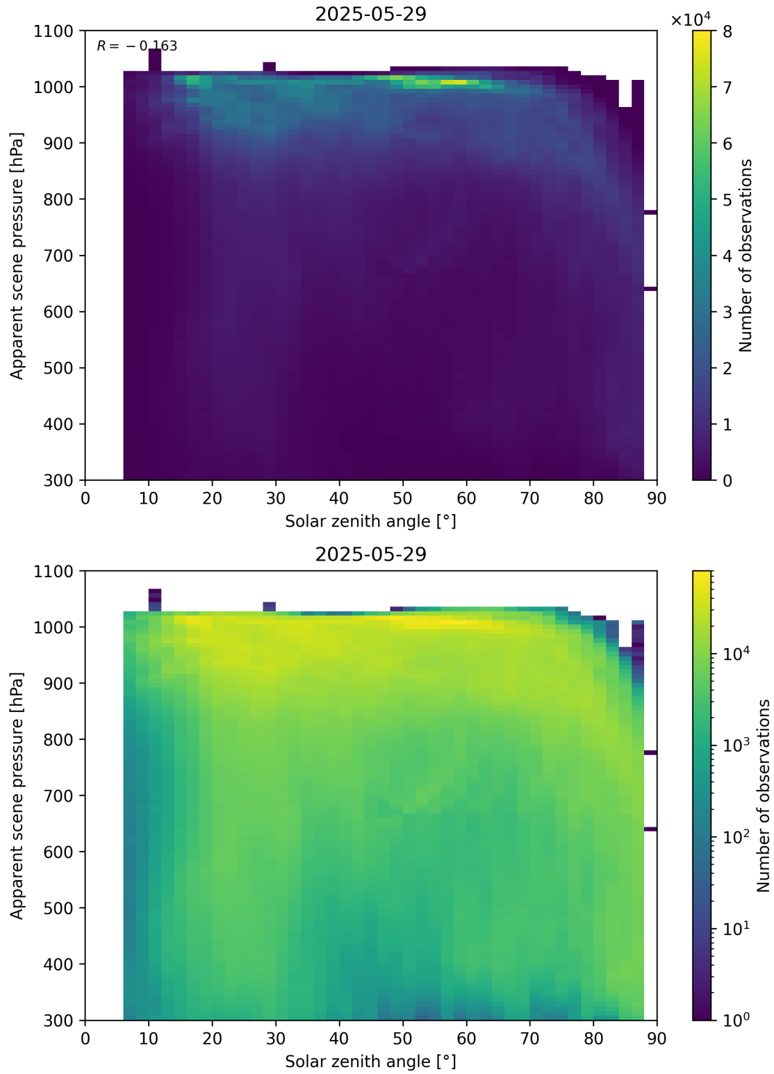
Figure 108: Scatter density plot of “Solar zenith angle” against “Apparent scene pressure” for 2025-05-28 to 2025-05-30.
