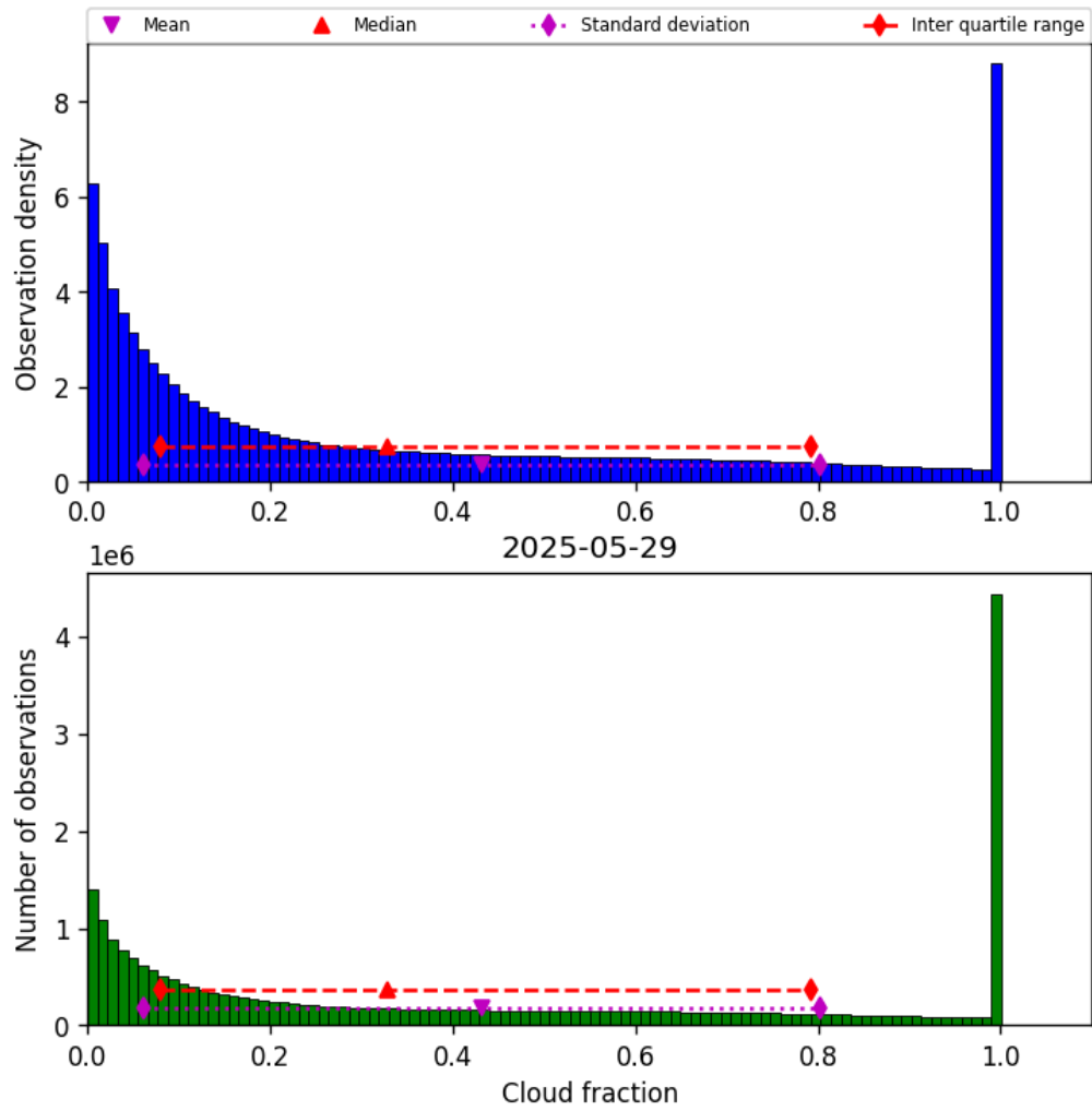
Figure 32: Histogram of “Cloud fraction” for 2025-05-28 to 2025-05-30
