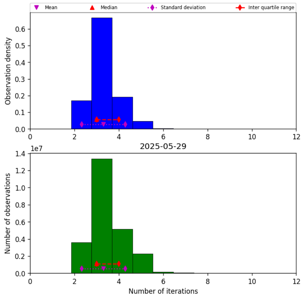
Figure 39: Histogram of “Number of iterations” for 2025-05-28 to 2025-05-30
