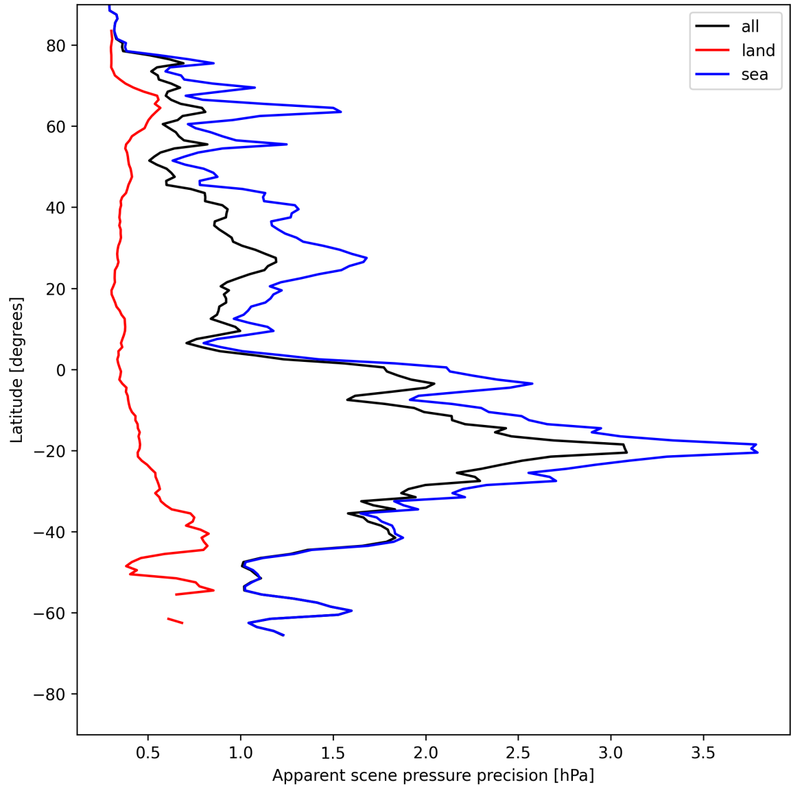
Figure 20: Zonal average of “Apparent scene pressure precision” for 2025-05-28 to 2025-05-30.
