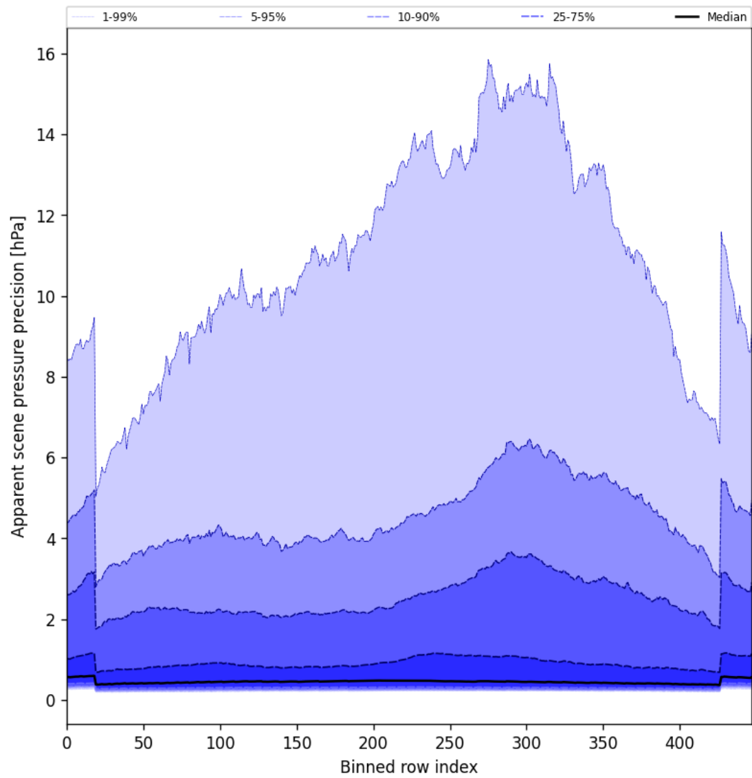
Figure 54: Along track statistics of “Apparent scene pressure precision” for 2025-05-28 to 2025-05-30
