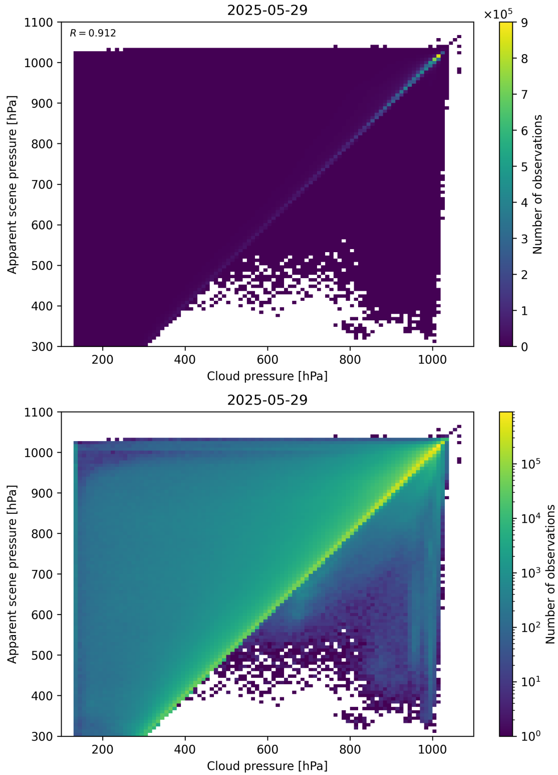
Figure 77: Scatter density plot of “Cloud pressure” against “Apparent scene pressure” for 2025-05-28 to 2025-05-30.
