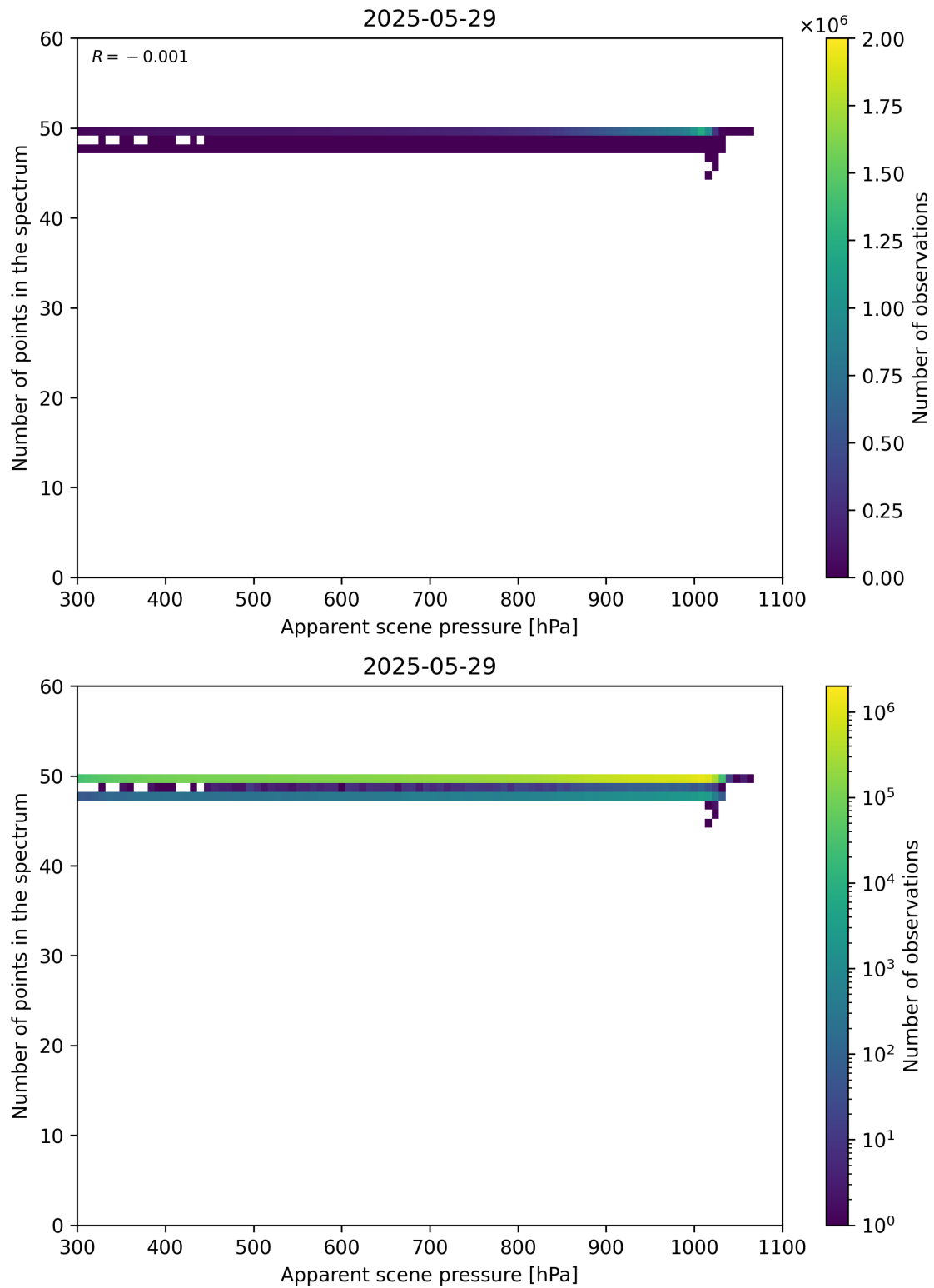
Figure 66: Scatter density plot of “Apparent scene pressure” against “Number of points in the spectrum” for 2025-05-28 to 2025-05-30.
