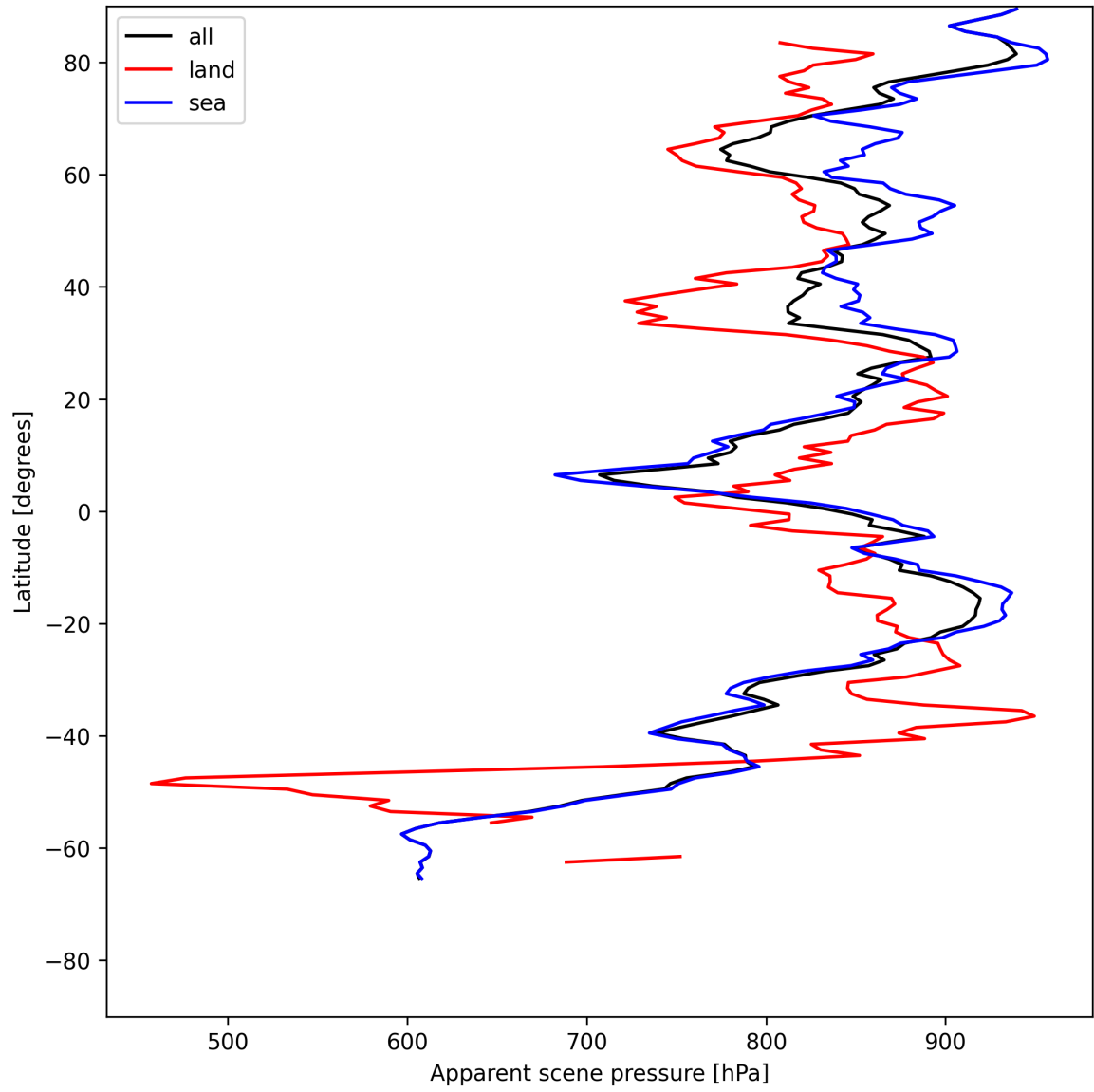
Figure 19: Zonal average of “Apparent scene pressure” for 2025-05-28 to 2025-05-30.
