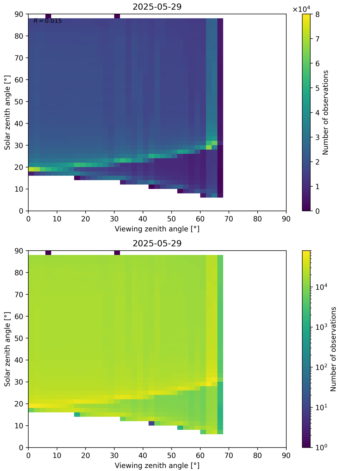
Figure 127: Scatter density plot of “Viewing zenith angle” against “Solar zenith angle” for 2025-05-28 to 2025-05-30.
