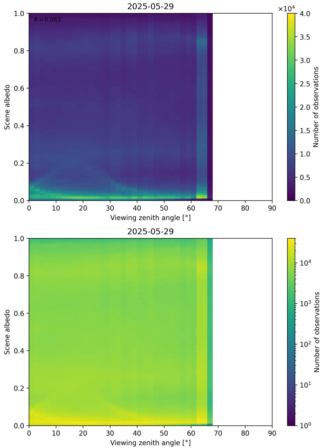
Figure 126: Scatter density plot of “Viewing zenith angle” against “Scene albedo” for 2025-05-28 to 2025-05-30.
