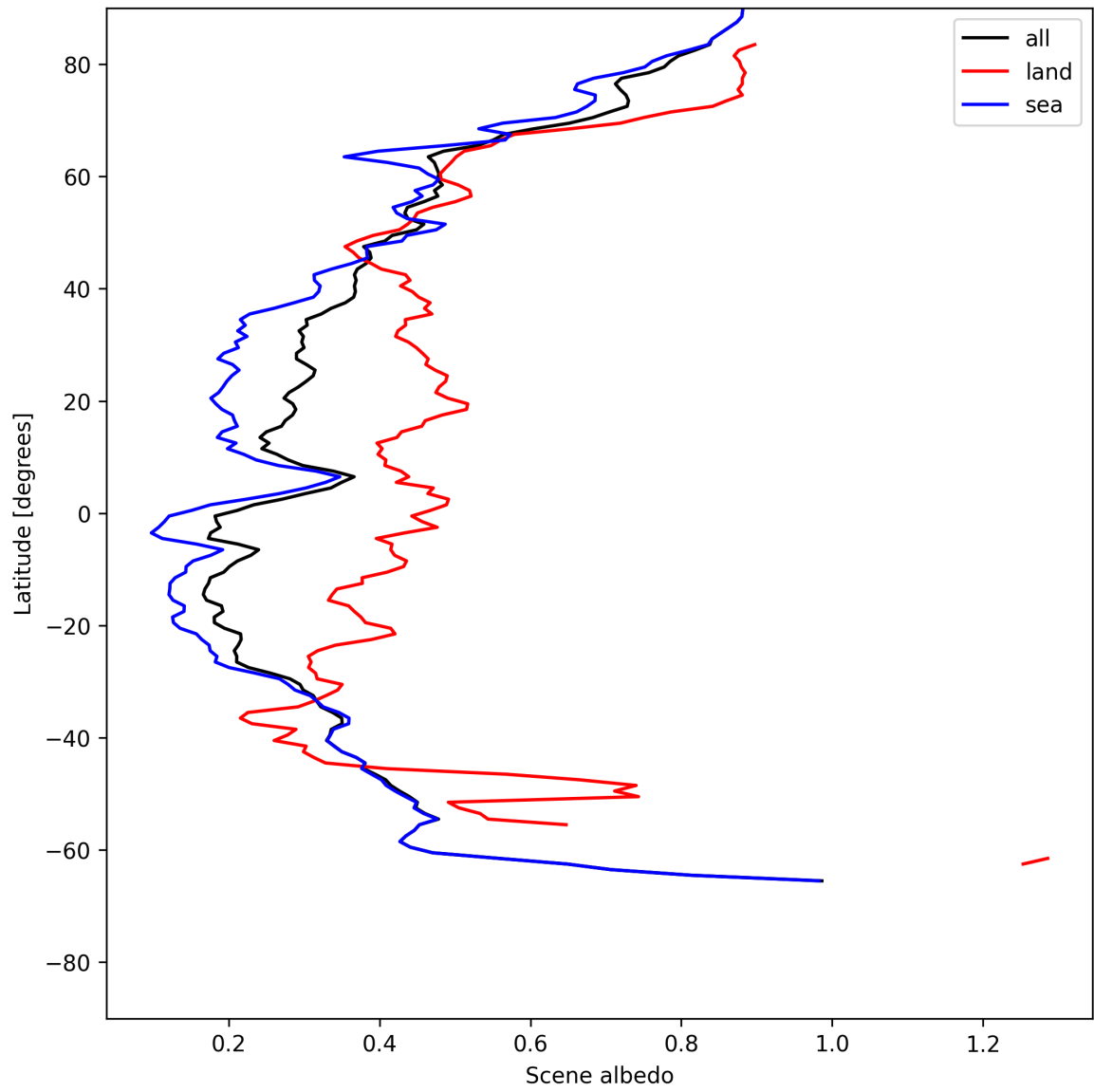
Figure 17: Zonal average of “Scene albedo” for 2025-05-28 to 2025-05-30.
