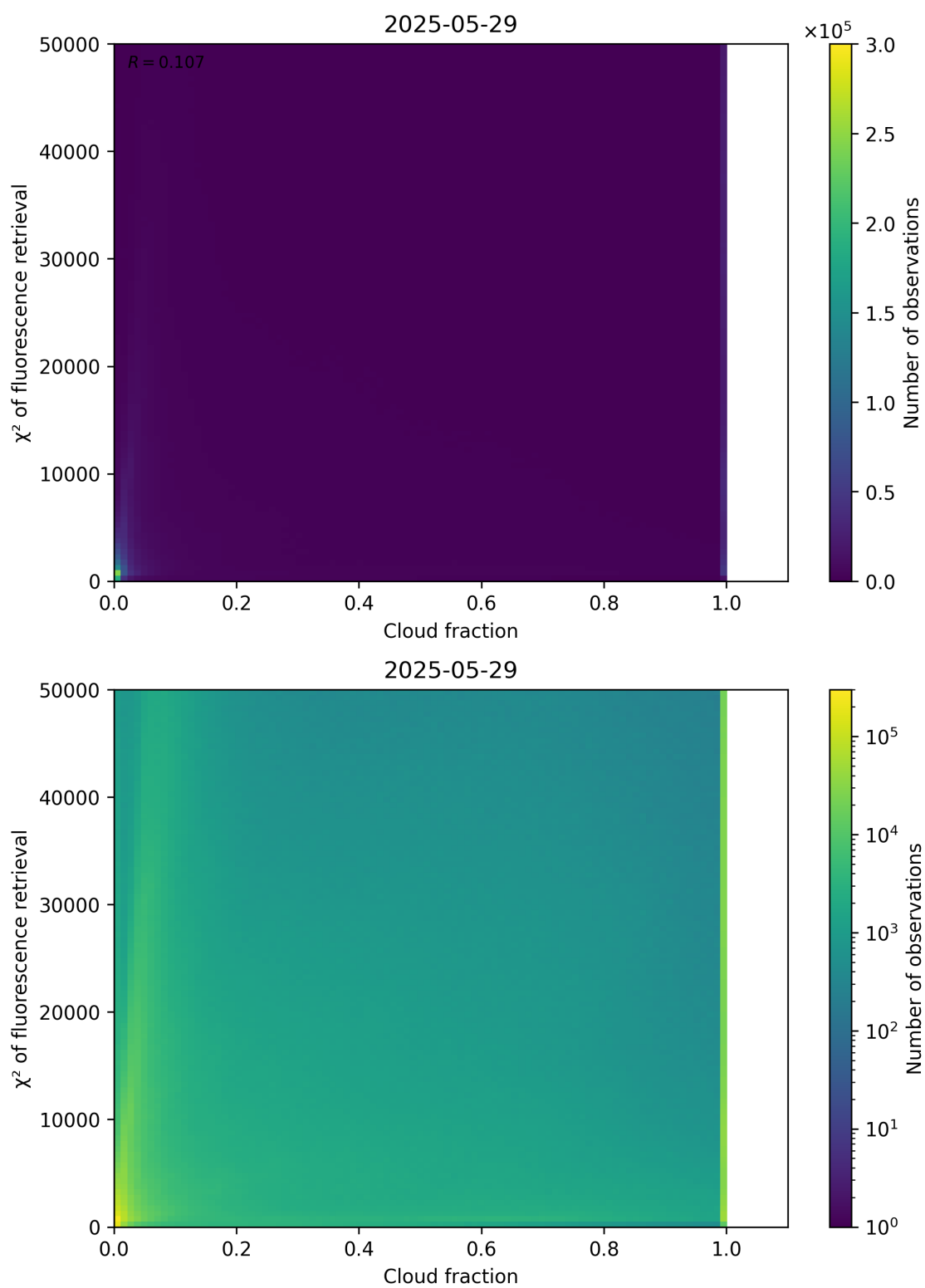
Figure 71: Scatter density plot of “Cloud fraction” against “ \chi^2 of fluorescence retrieval” for 2025-05-28 to 2025-05-30.
