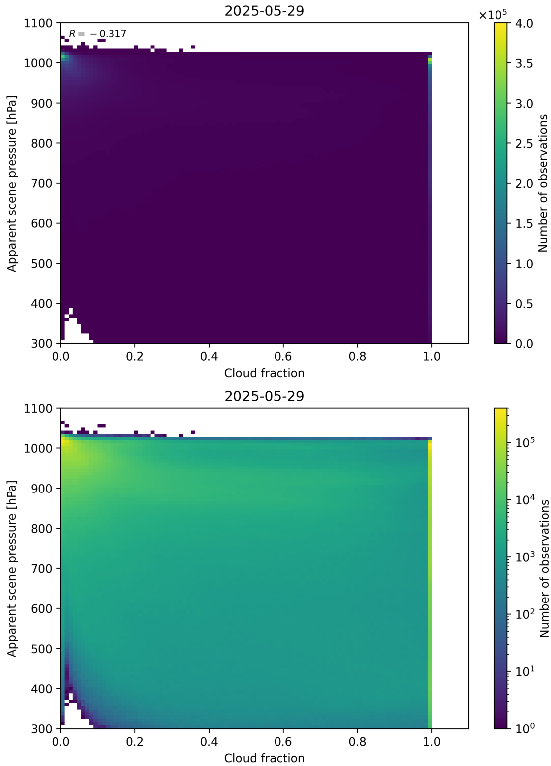
Figure 70: Scatter density plot of “Cloud fraction” against “Apparent scene pressure” for 2025-05-28 to 2025-05-30.
