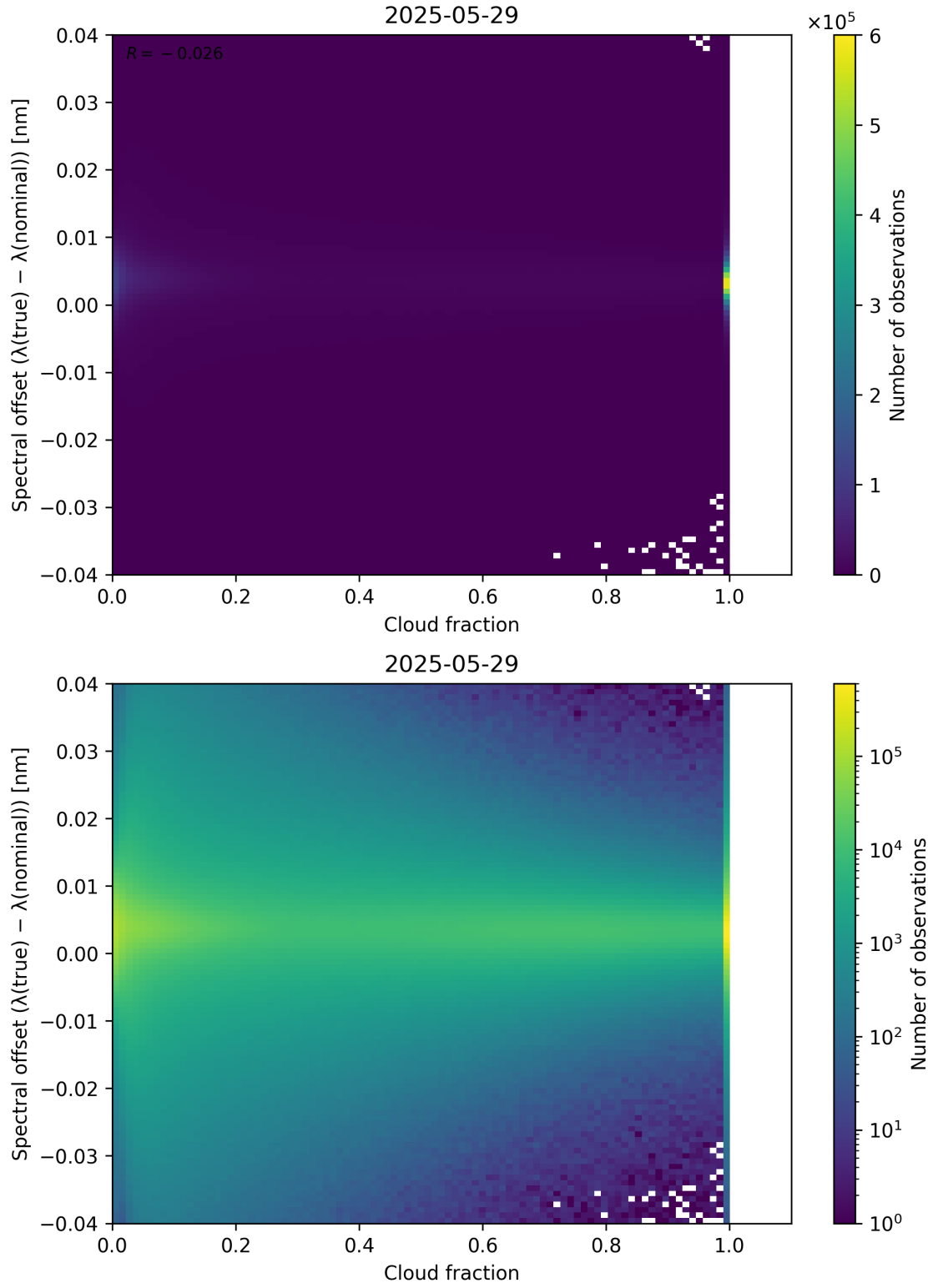
Figure 76: Scatter density plot of “Cloud fraction” against “Spectral offset ( \lambda_{\text{true}} - \lambda_{\text{nominal}} )” for 2025-05-28 to 2025-05-30.
