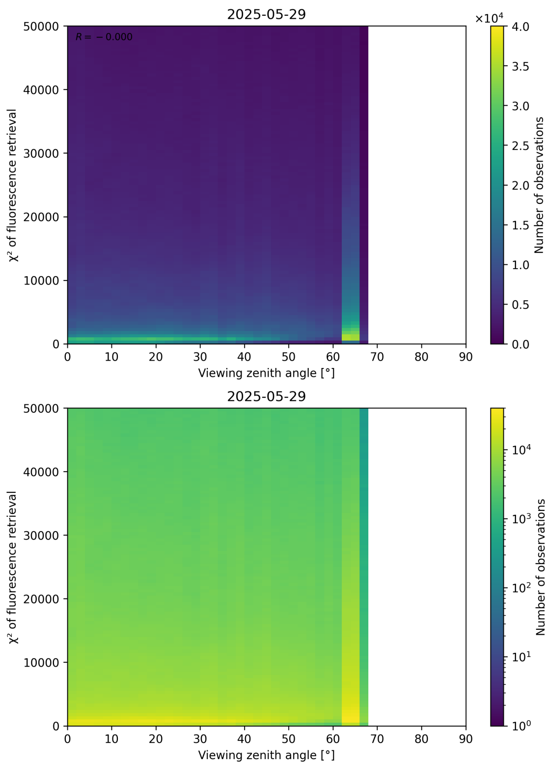
Figure 119: Scatter density plot of “Viewing zenith angle” against “ \chi^2 of fluorescence retrieval” for 2025-05-28 to 2025-05-30.
