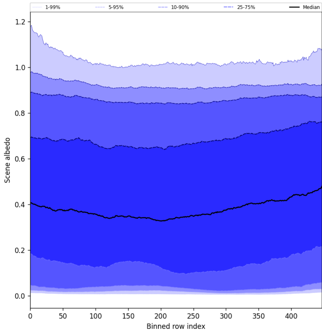
Figure 51: Along track statistics of “Scene albedo” for 2025-05-28 to 2025-05-30
