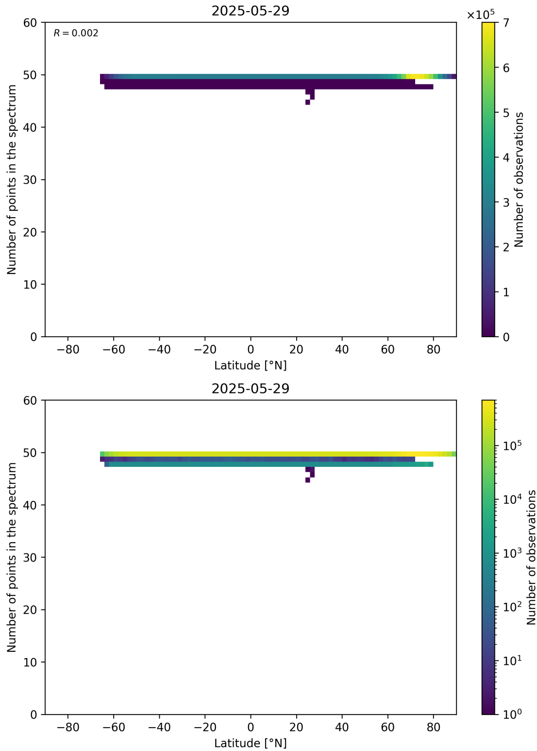
Figure 94: Scatter density plot of “Latitude” against “Number of points in the spectrum” for 2025-05-28 to 2025-05-30.
