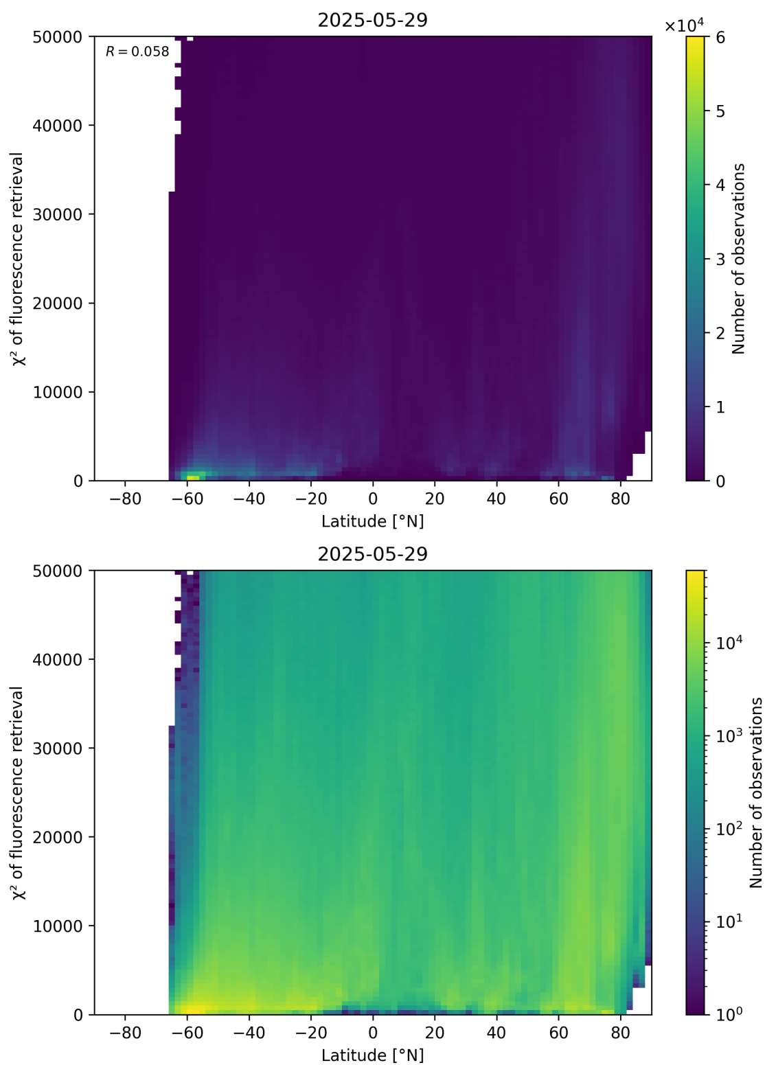
Figure 89: Scatter density plot of “Latitude” against “ \chi^2 of fluorescence retrieval” for 2025-05-28 to 2025-05-30.
