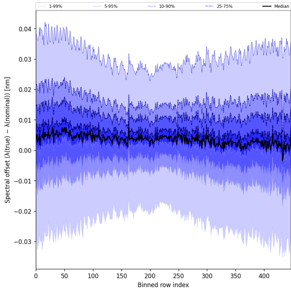
Figure 62: Along track statistics of “Spectral offset ( \lambda_{\text{true}} - \lambda_{\text{nominal}} )” for 2025-05-28 to 2025-05-30
