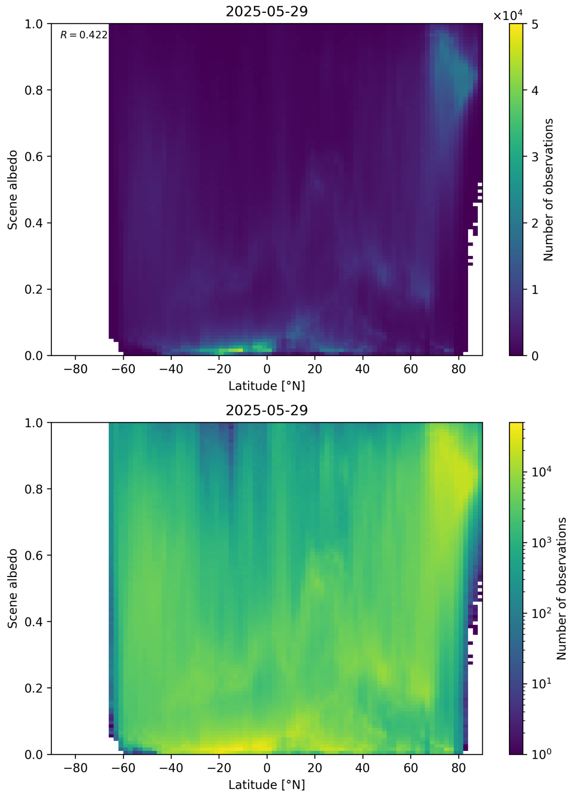
Figure 95: Scatter density plot of “Latitude” against “Scene albedo” for 2025-05-28 to 2025-05-30.
