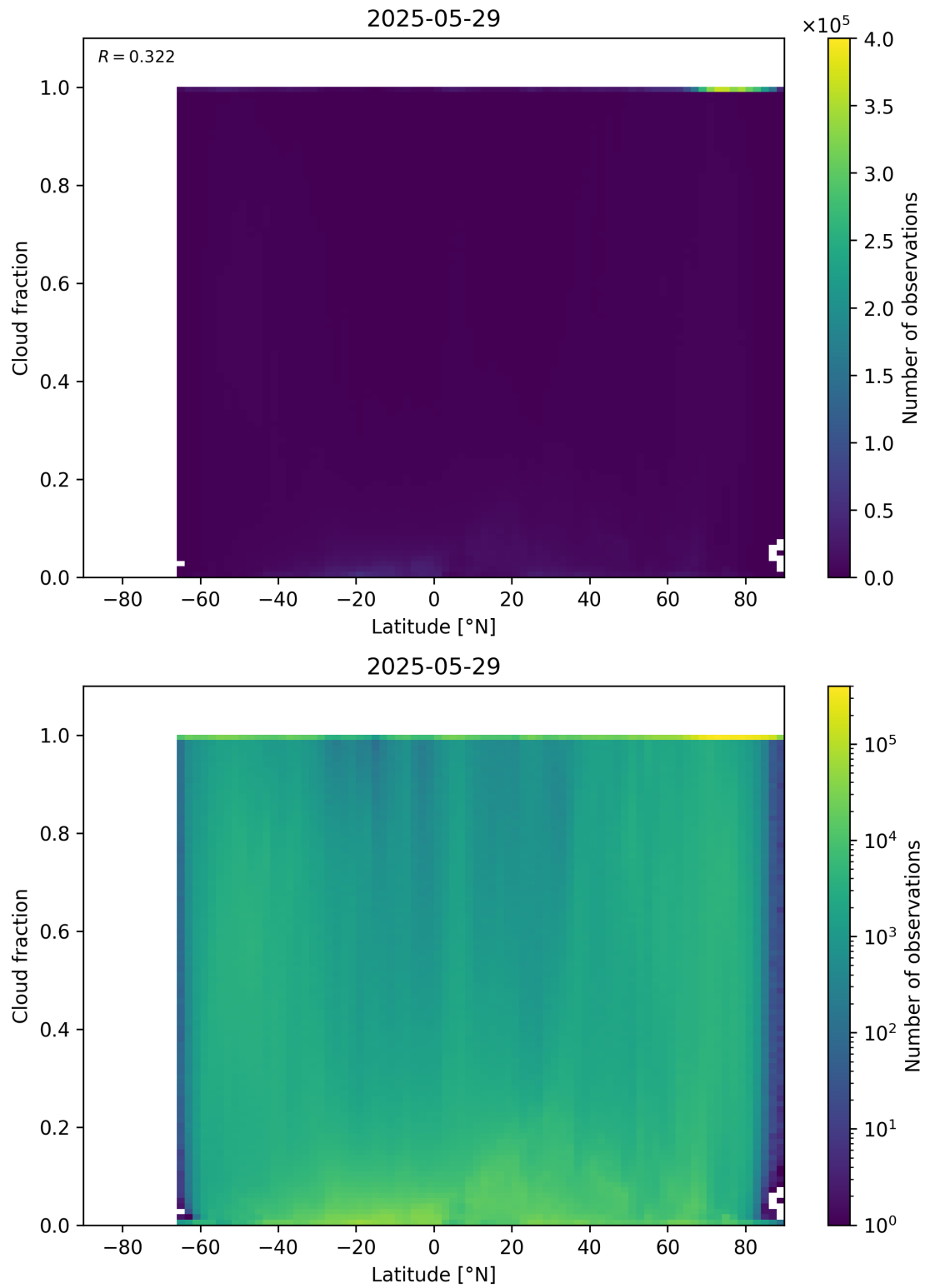
Figure 90: Scatter density plot of “Latitude” against “Cloud fraction” for 2025-05-28 to 2025-05-30.
