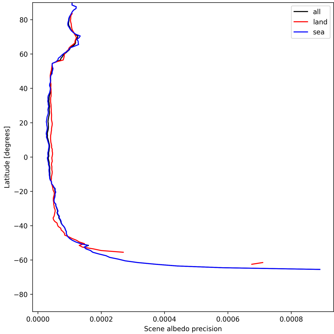
Figure 18: Zonal average of “Scene albedo precision” for 2025-05-28 to 2025-05-30.
