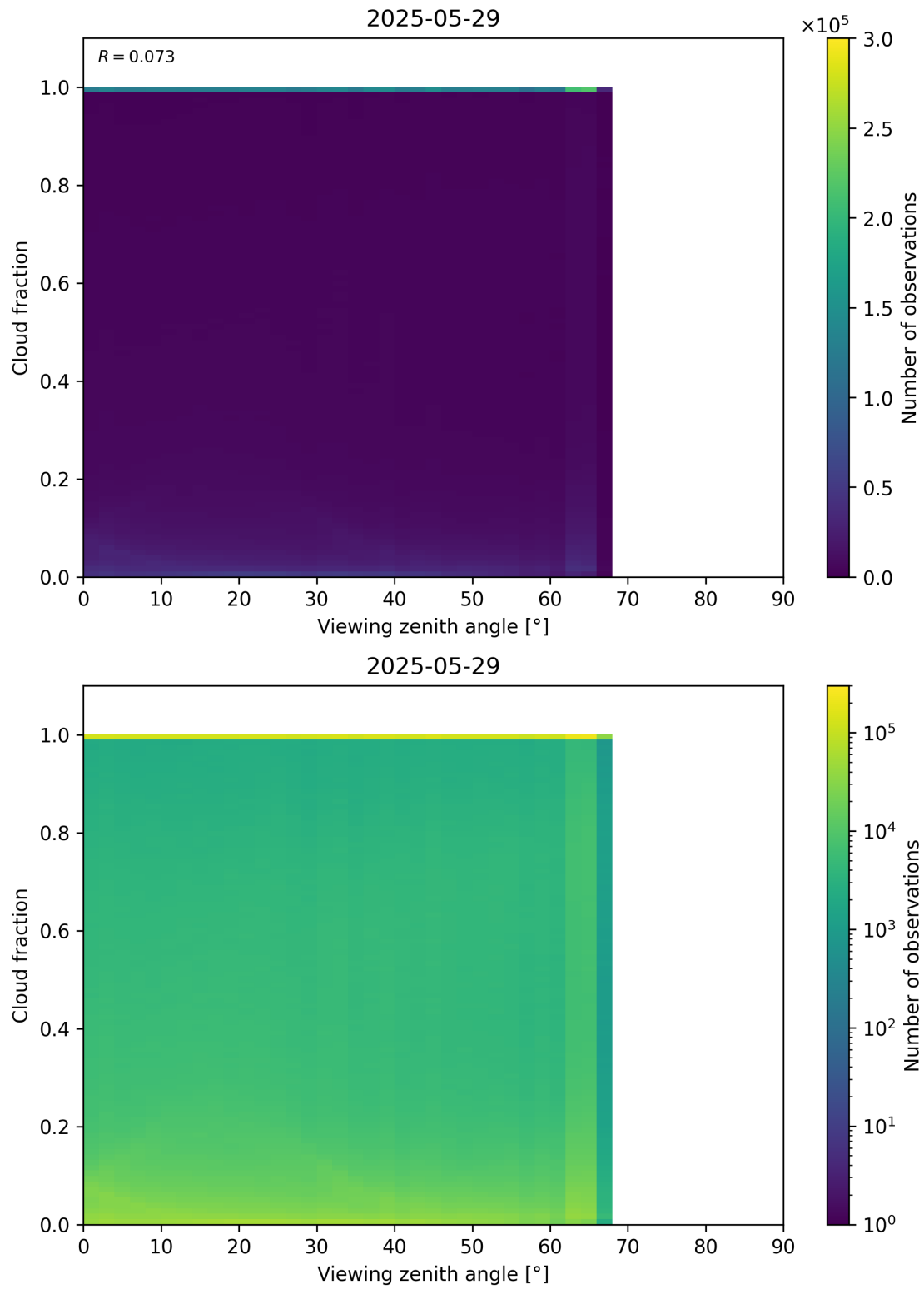
Figure 120: Scatter density plot of “Viewing zenith angle” against “Cloud fraction” for 2025-05-28 to 2025-05-30.
