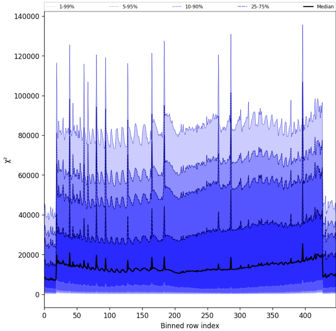
Figure 55: Along track statistics of “ \chi^2 ” for 2025-05-28 to 2025-05-30
