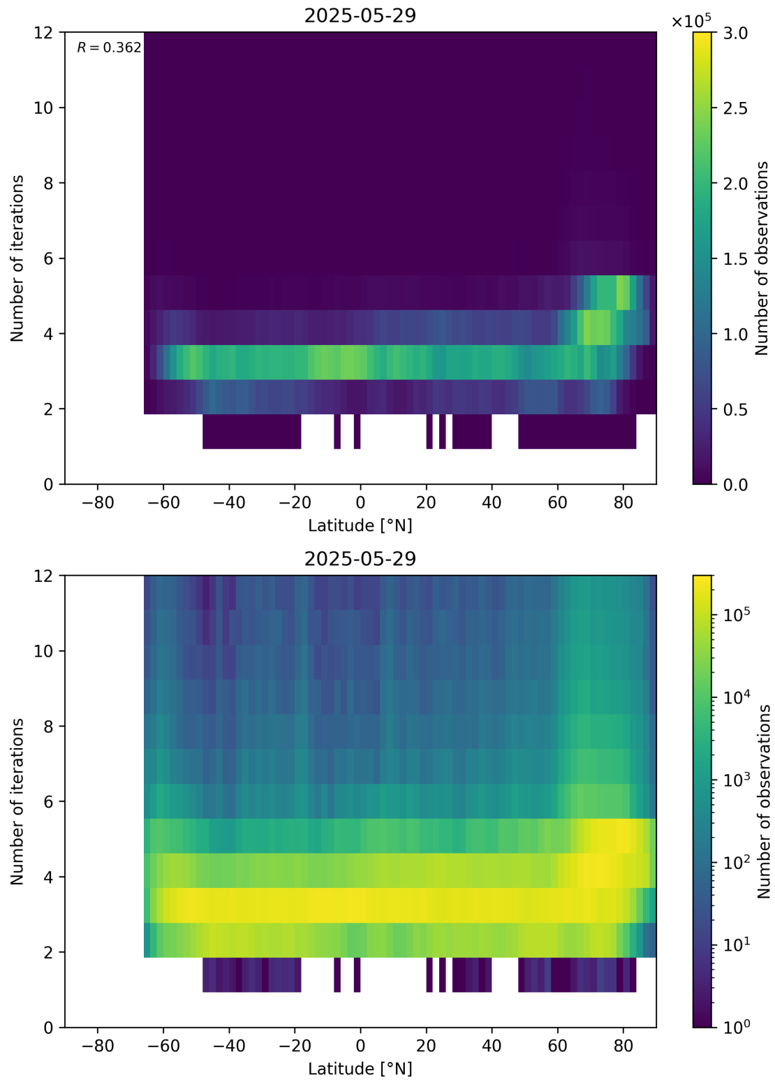
Figure 93: Scatter density plot of “Latitude” against “Number of iterations” for 2025-05-28 to 2025-05-30.
