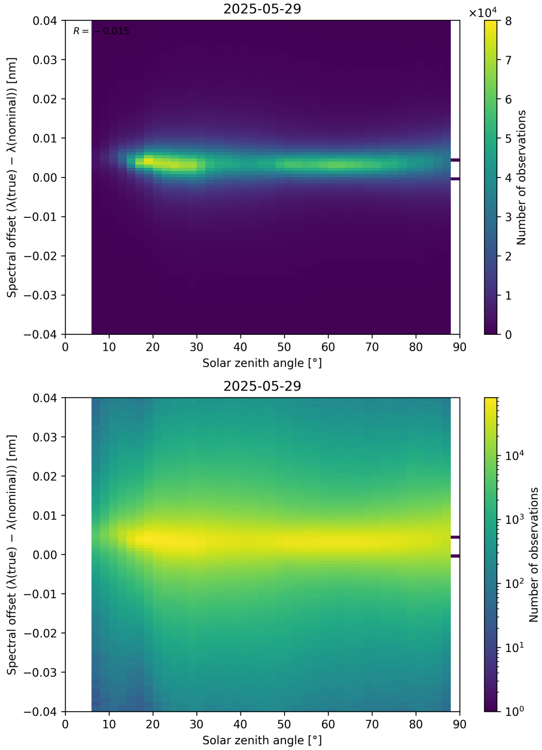
Figure 117: Scatter density plot of “Solar zenith angle” against “Spectral offset ( \lambda_{\text{true}} - \lambda_{\text{nominal}} )” for 2025-05-28 to 2025-05-30.
