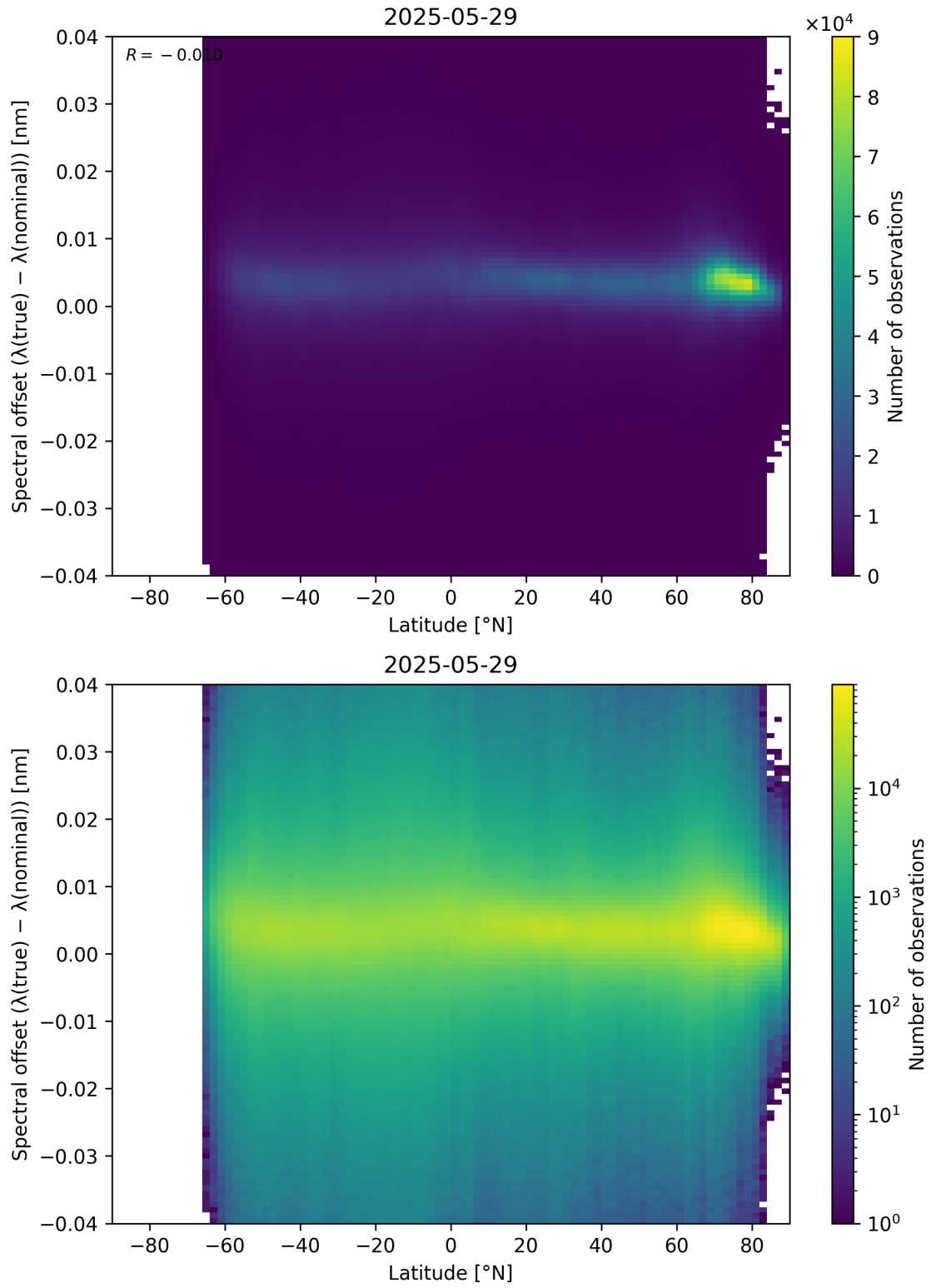
Figure 96: Scatter density plot of “Latitude” against “Spectral offset ( \lambda_{\text{true}} - \lambda_{\text{nominal}} )” for 2025-05-28 to 2025-05-30.
