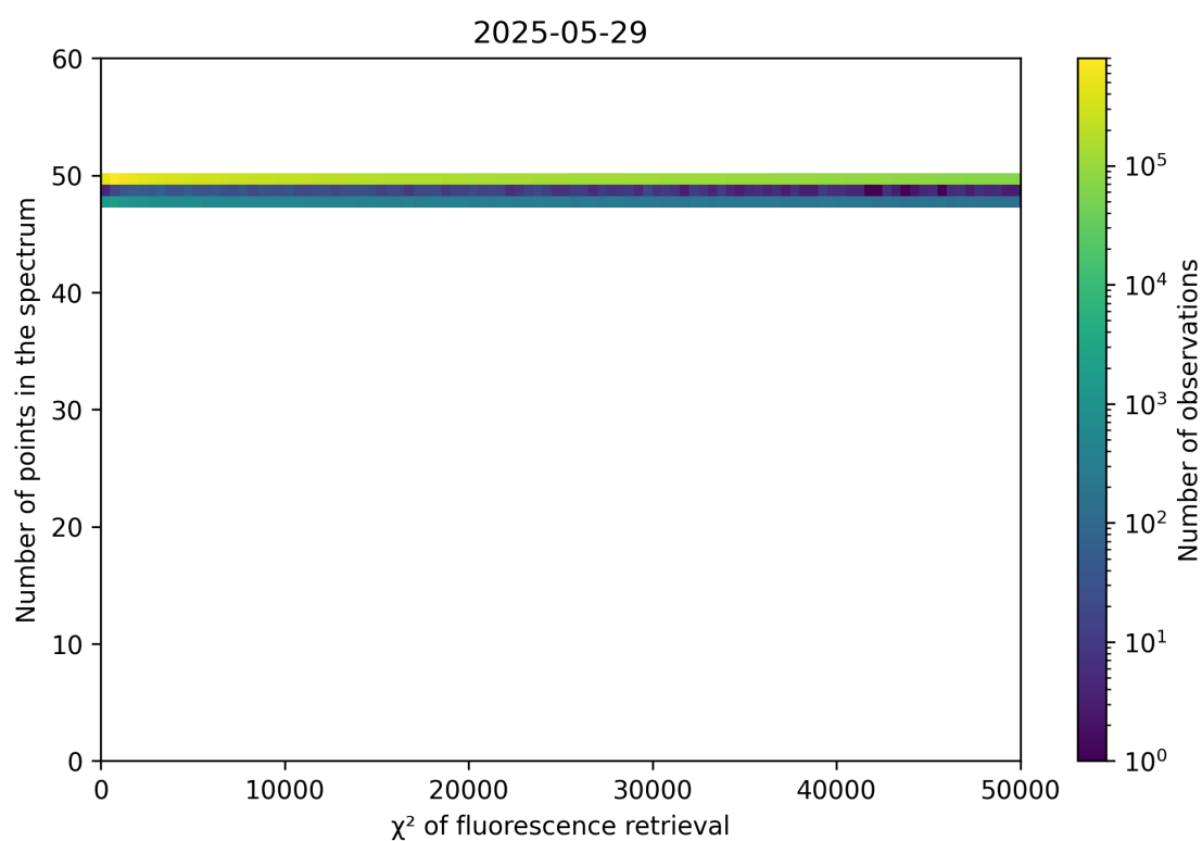
Figure 68: Scatter density plot of “ \chi^2 of fluorescence retrieval” against “Number of points in the spectrum” for 2025-05-28 to 2025-05-30.
