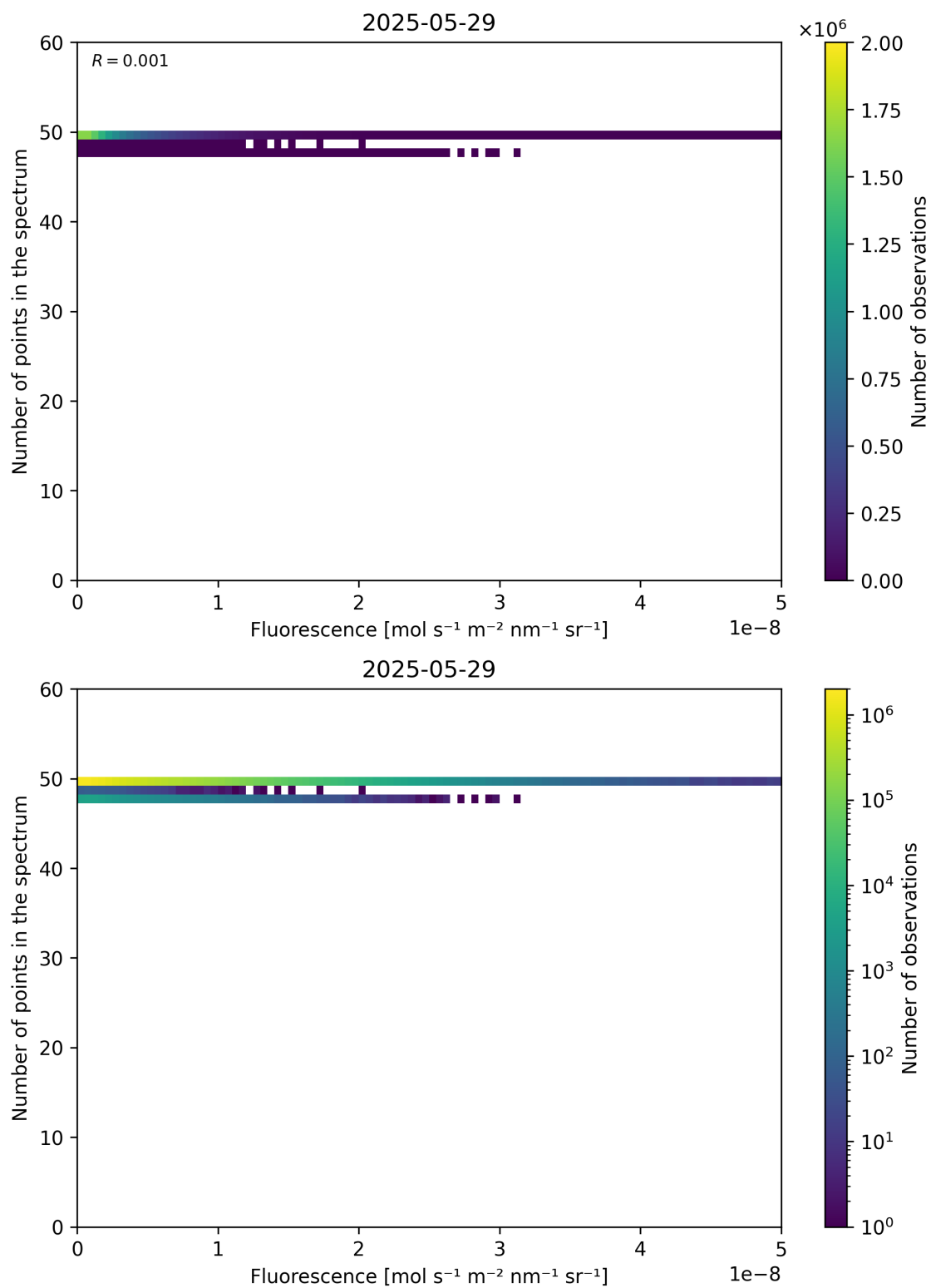
Figure 86: Scatter density plot of “Fluorescence” against “Number of points in the spectrum” for 2025-05-28 to 2025-05-30.
