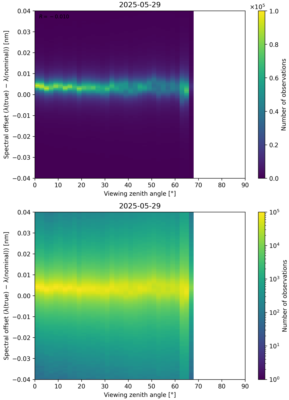
Figure 128: Scatter density plot of “Viewing zenith angle” against “Spectral offset ( \lambda_{\text{true}} - \lambda_{\text{nominal}} )” for 2025-05-28 to 2025-05-30.
