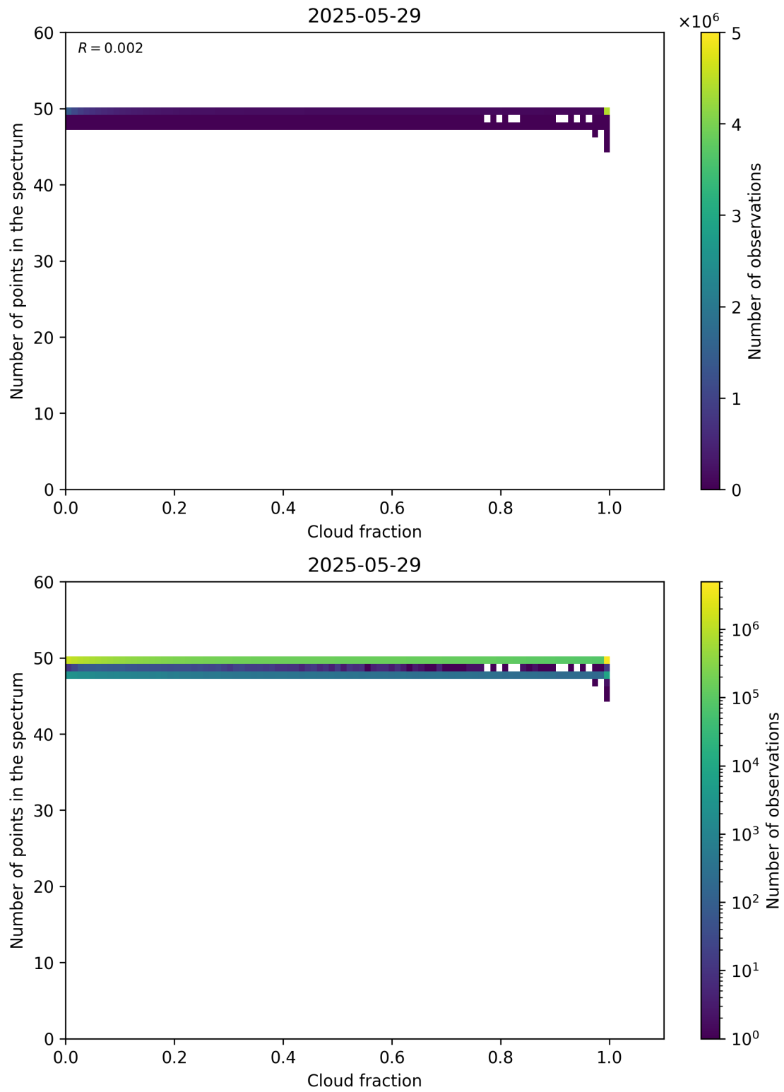
Figure 74: Scatter density plot of “Cloud fraction” against “Number of points in the spectrum” for 2025-05-28 to 2025-05-30.
