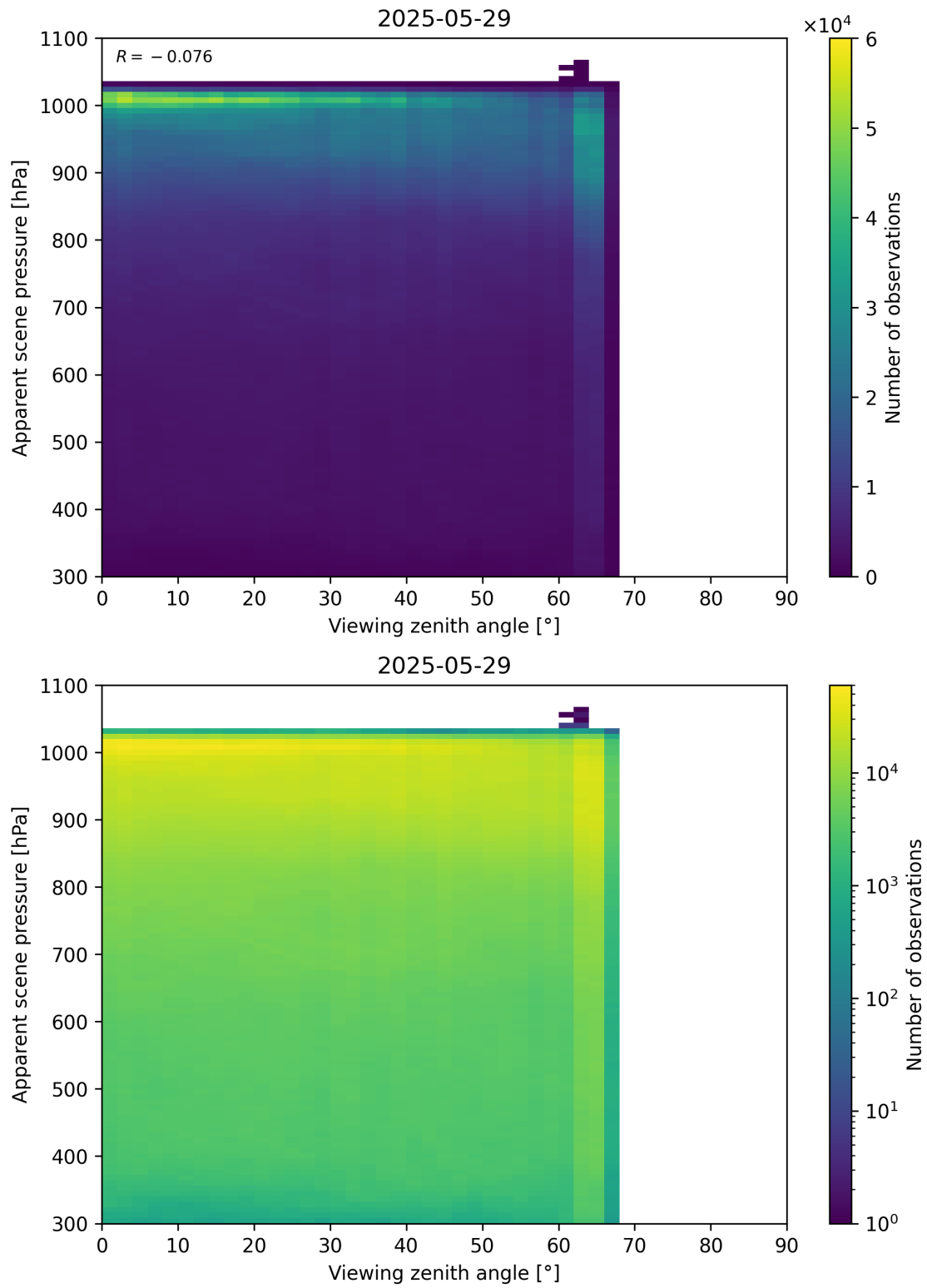
Figure 118: Scatter density plot of “Viewing zenith angle” against “Apparent scene pressure” for 2025-05-28 to 2025-05-30.
