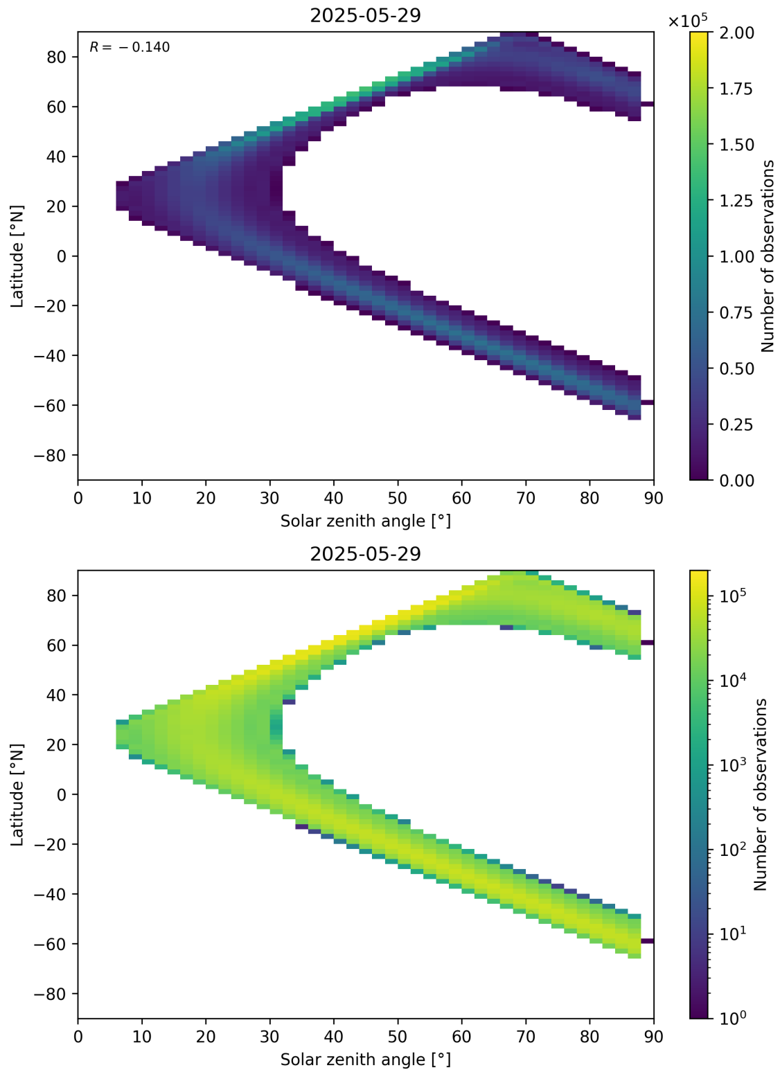
Figure 113: Scatter density plot of “Solar zenith angle” against “Latitude” for 2025-05-28 to 2025-05-30.
