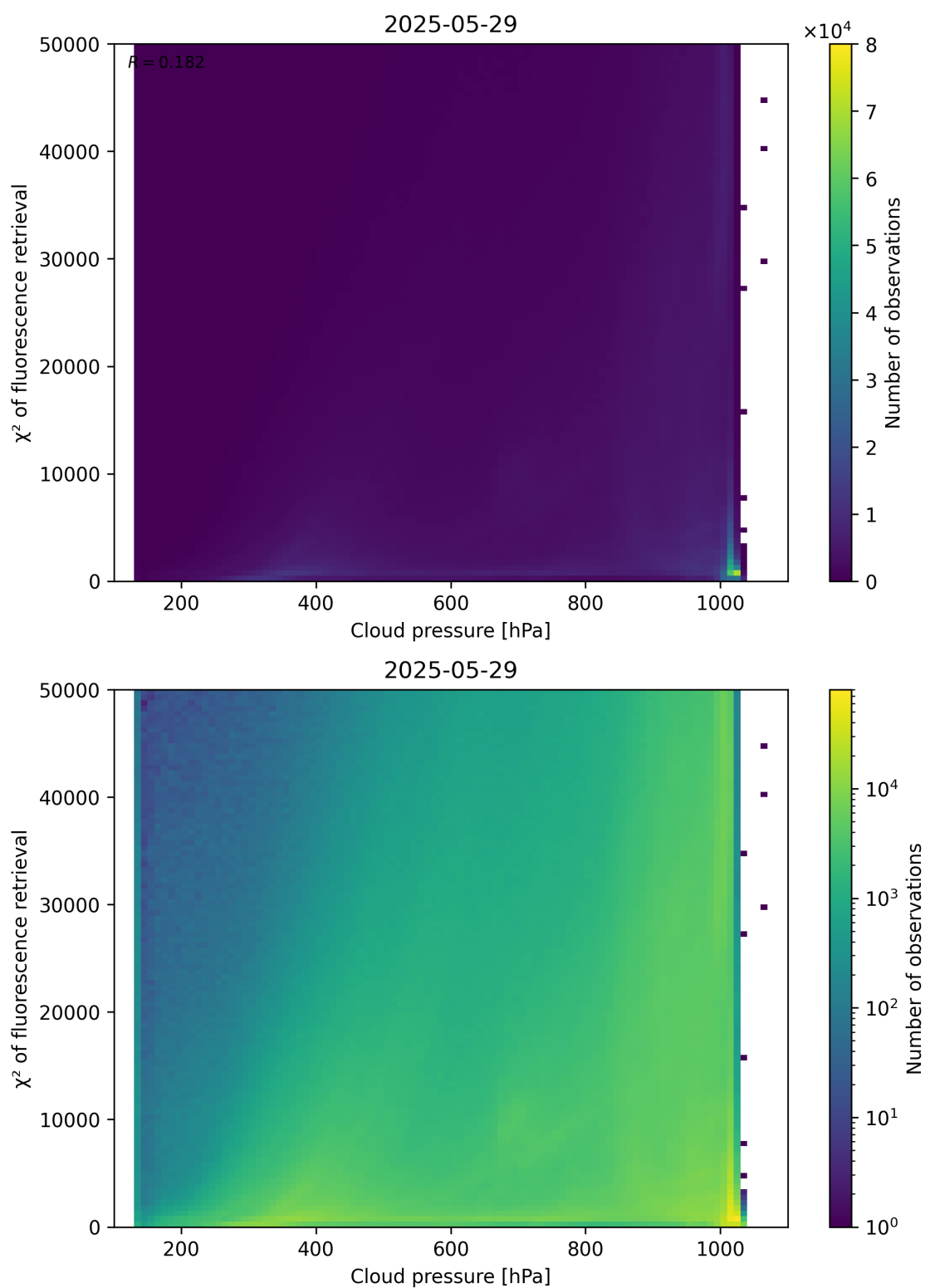
Figure 78: Scatter density plot of “Cloud pressure” against “ \chi^2 of fluorescence retrieval” for 2025-05-28 to 2025-05-30.
