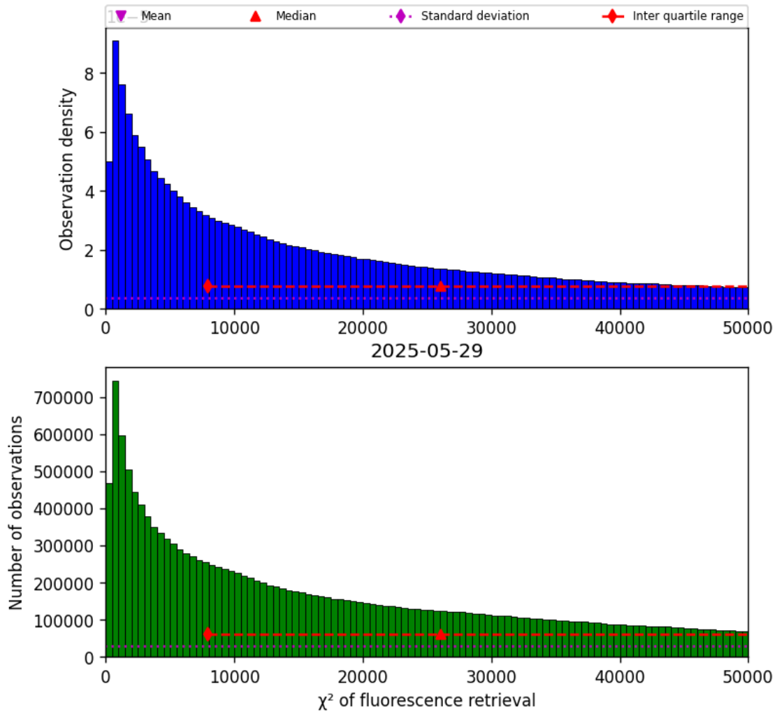
Figure 42: Histogram of “ \chi^2 of fluorescence retrieval” for 2025-05-28 to 2025-05-30
