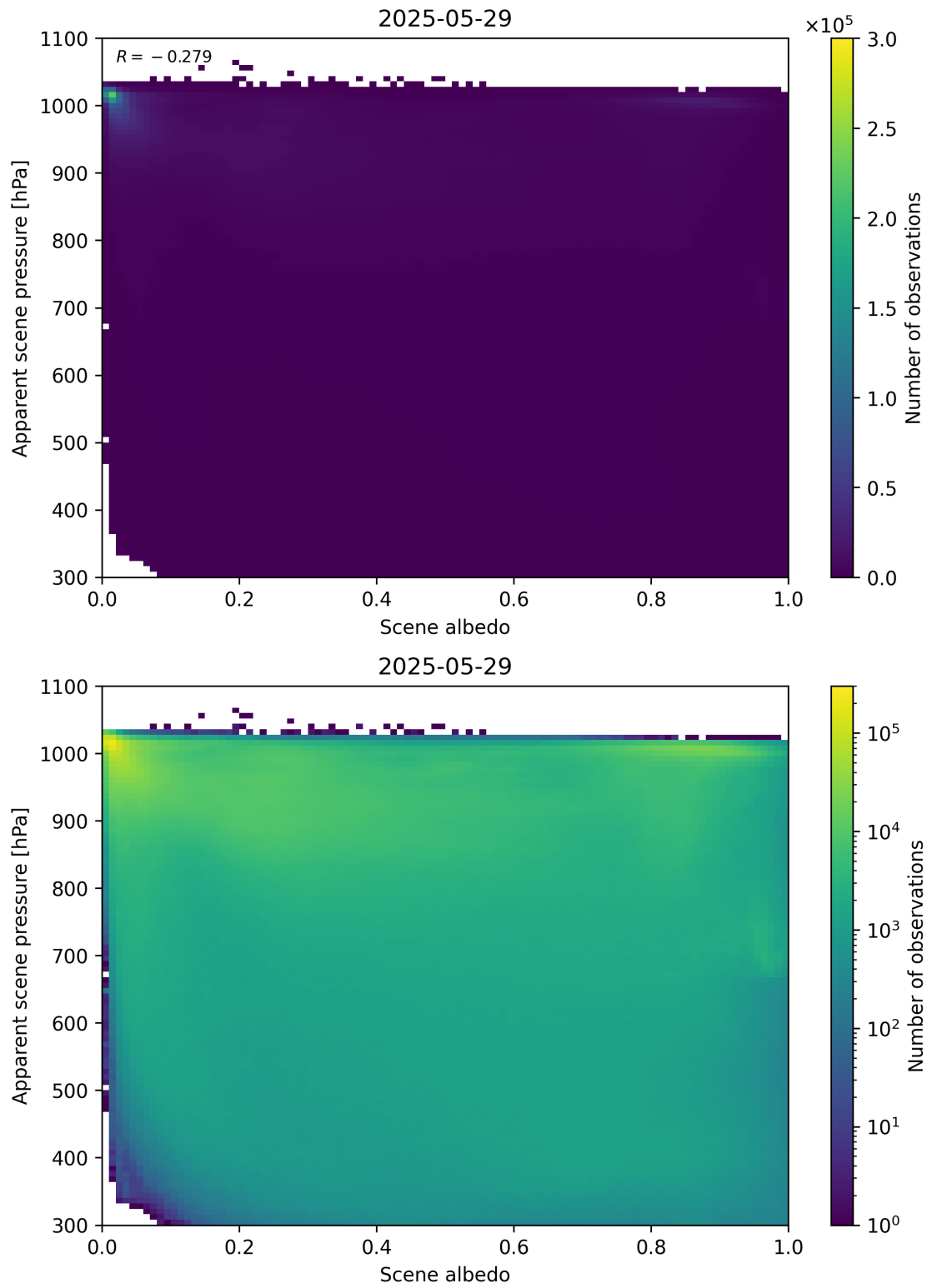
Figure 102: Scatter density plot of “Scene albedo” against “Apparent scene pressure” for 2025-05-28 to 2025-05-30.
