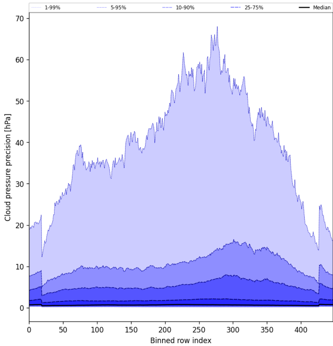
Figure 48: Along track statistics of “Cloud pressure precision” for 2025-05-28 to 2025-05-30
