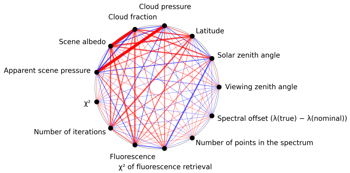
Figure 1: Map of correlation graph for 2025-05-28 to 2025-05-30.
