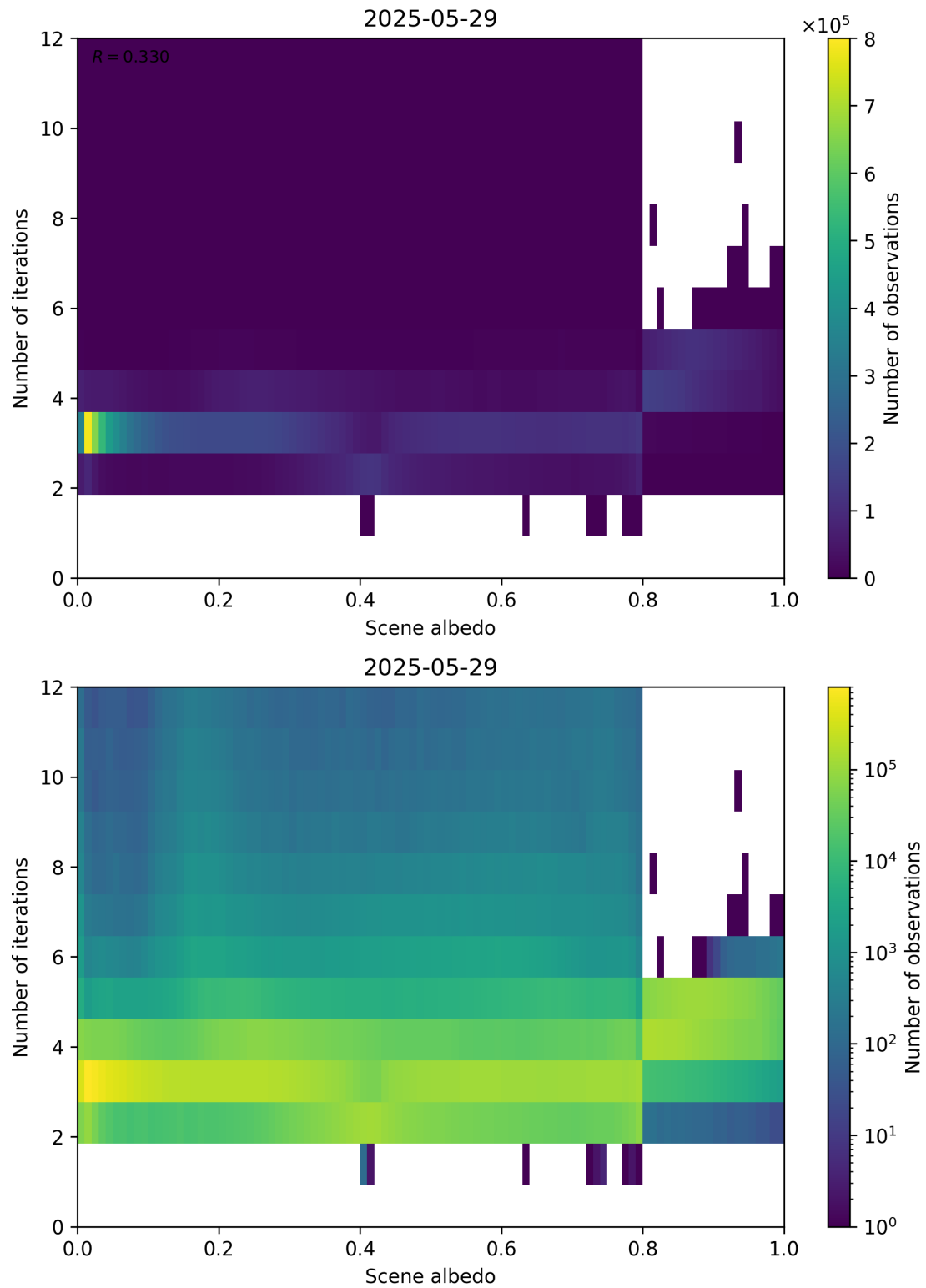
Figure 105: Scatter density plot of “Scene albedo” against “Number of iterations” for 2025-05-28 to 2025-05-30.
