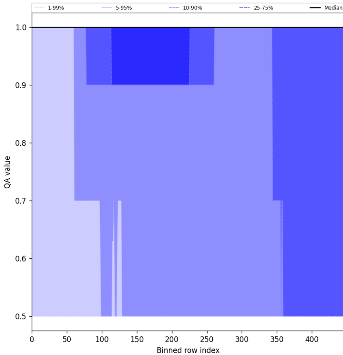
Figure 46: Along track statistics of “QA value” for 2025-05-28 to 2025-05-30
