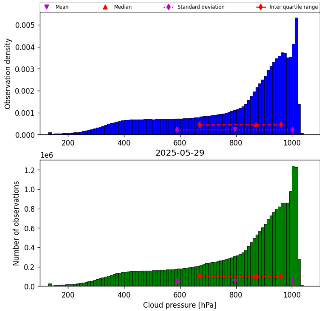
Figure 30: Histogram of “Cloud pressure” for 2025-05-28 to 2025-05-30
