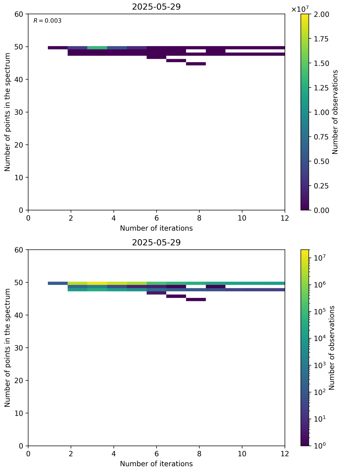
Figure 99: Scatter density plot of “Number of iterations” against “Number of points in the spectrum” for 2025-05-28 to 2025-05-30.
