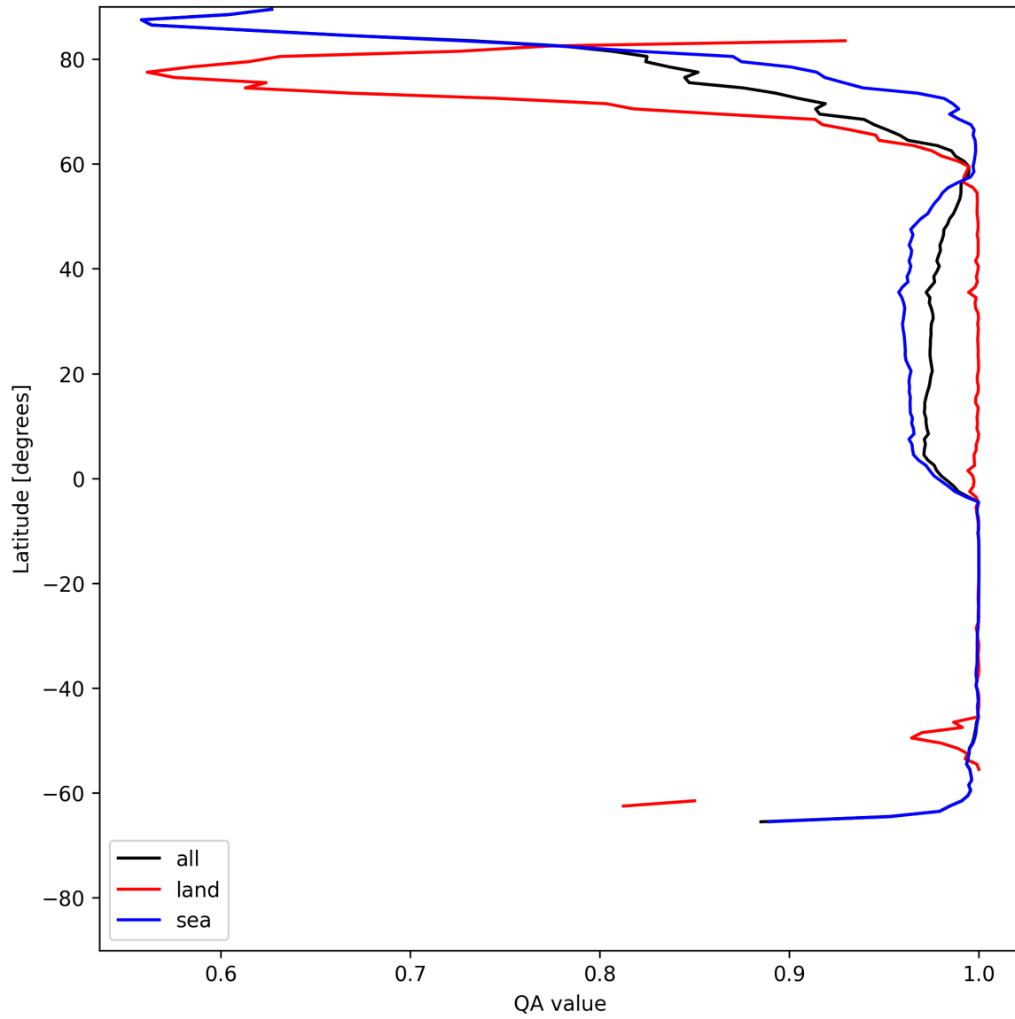
Figure 12: Zonal average of “QA value” for 2025-05-28 to 2025-05-30.
