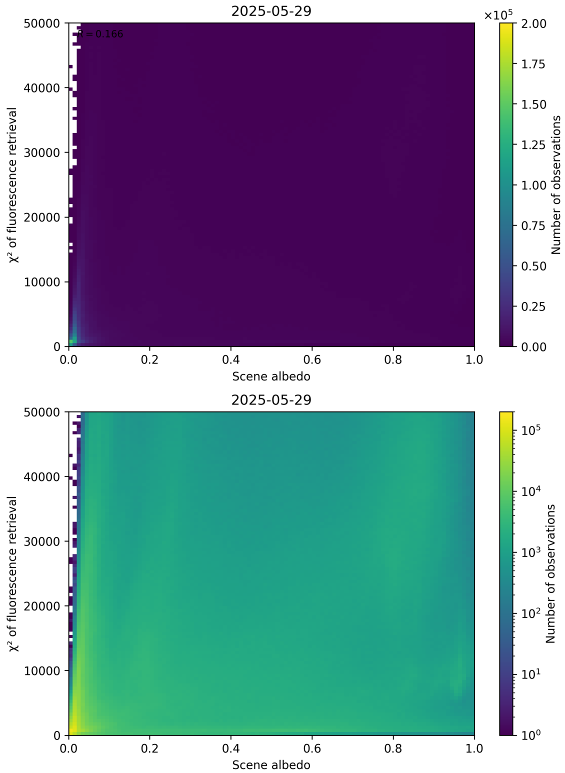
Figure 103: Scatter density plot of “Scene albedo” against “ \chi^2 of fluorescence retrieval” for 2025-05-28 to 2025-05-30.
