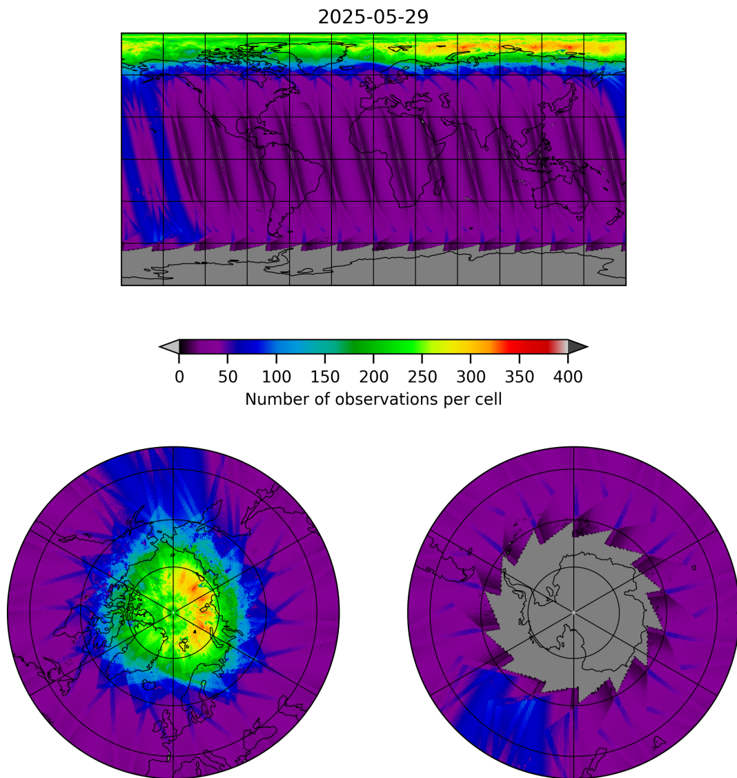
Figure 11: Map of the number of observations for 2025-05-28 to 2025-05-30
