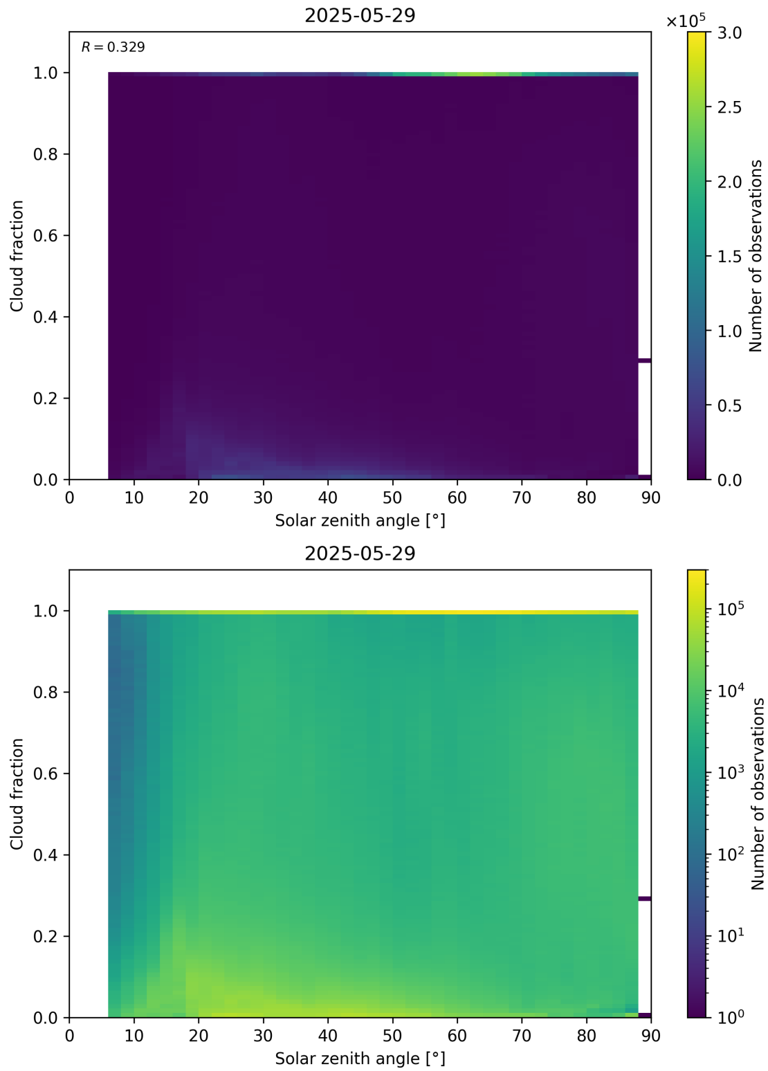
Figure 110: Scatter density plot of “Solar zenith angle” against “Cloud fraction” for 2025-05-28 to 2025-05-30.
