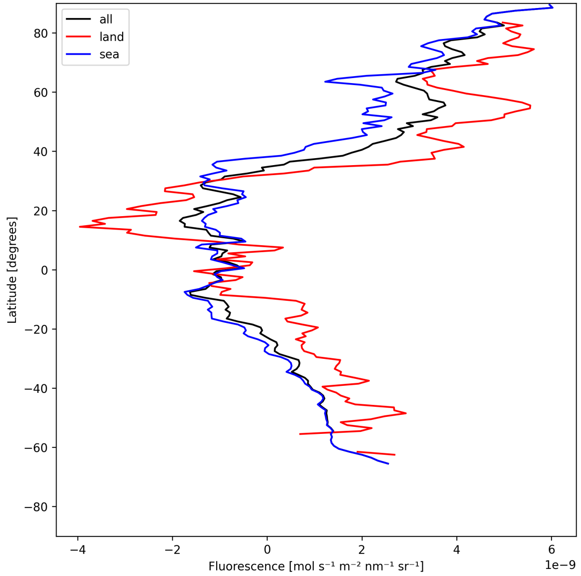
Figure 23: Zonal average of “Fluorescence” for 2025-05-28 to 2025-05-30.
