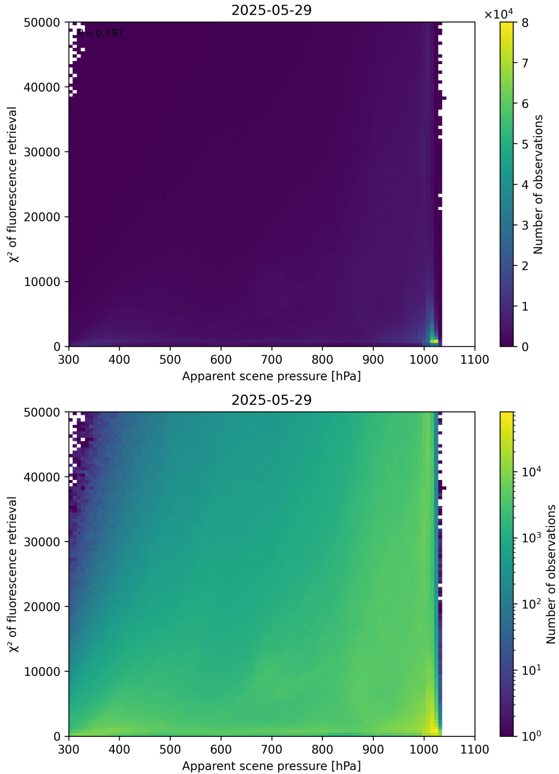
Figure 63: Scatter density plot of “Apparent scene pressure” against “ \chi^2 of fluorescence retrieval” for 2025-05-28 to 2025-05-30.
