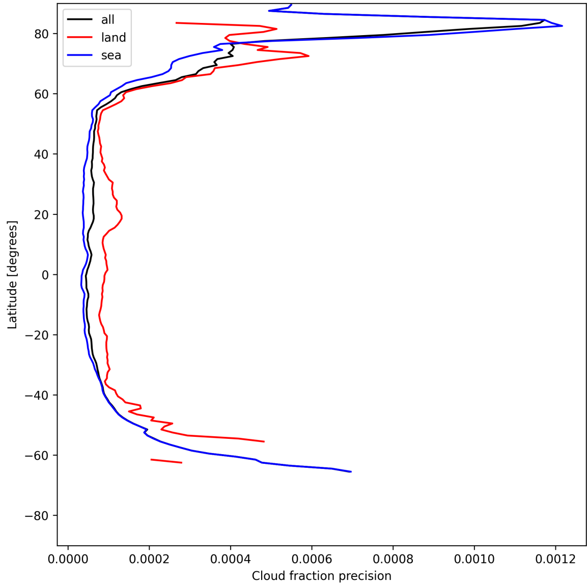
Figure 16: Zonal average of “Cloud fraction precision” for 2025-05-28 to 2025-05-30.
