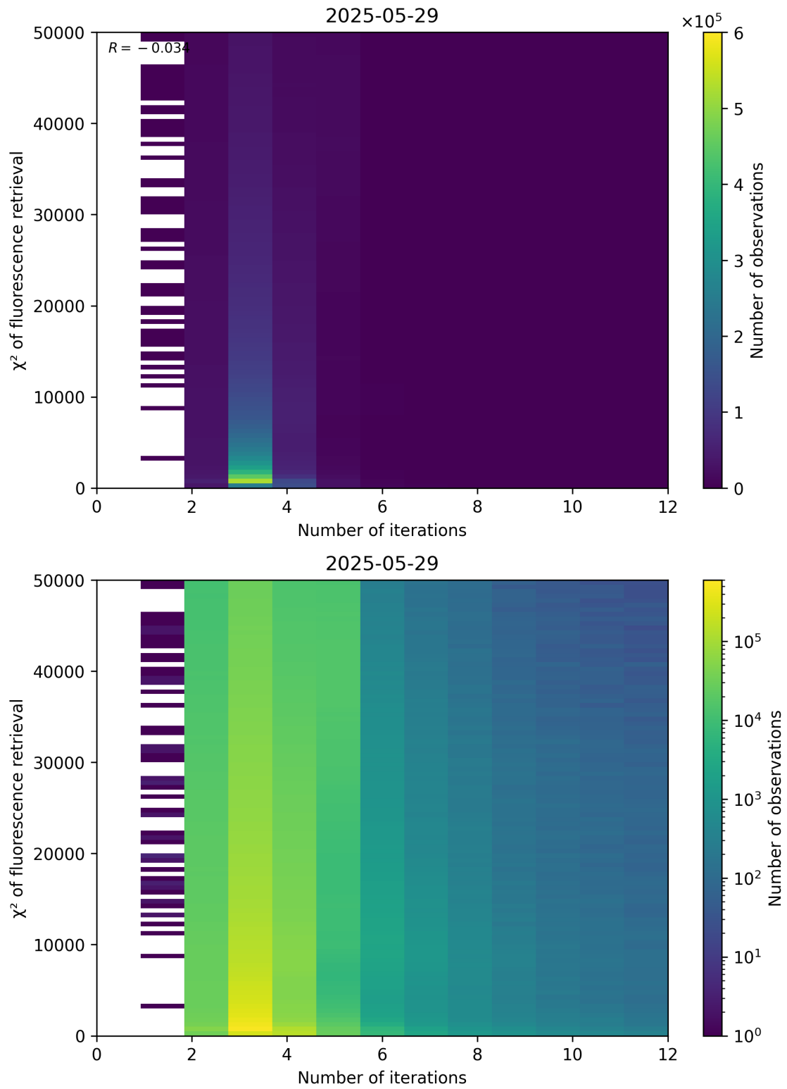
Figure 97: Scatter density plot of “Number of iterations” against “ \chi^2 of fluorescence retrieval” for 2025-05-28 to 2025-05-30.
