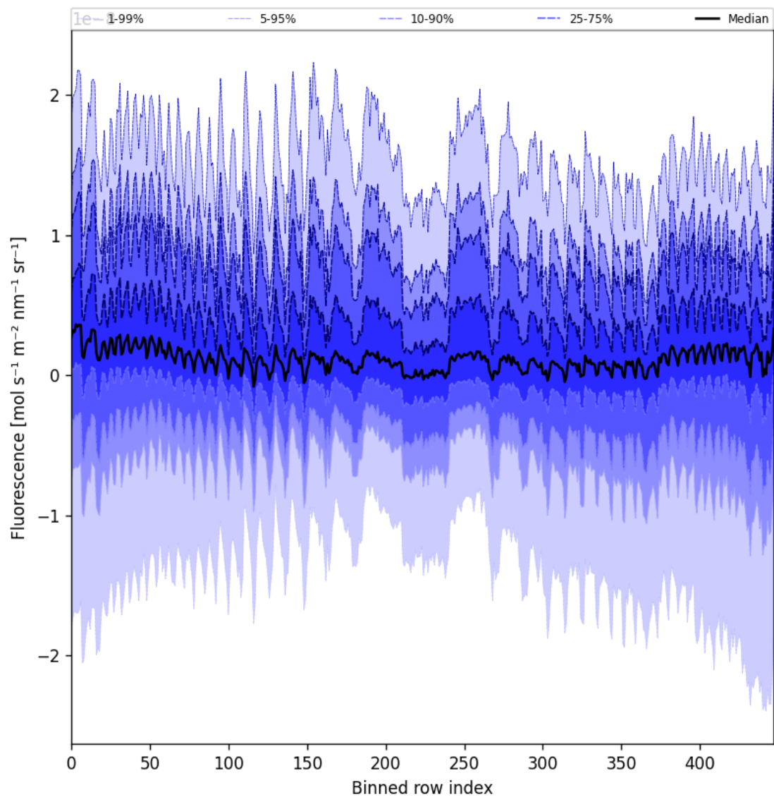
Figure 57: Along track statistics of “Fluorescence” for 2025-05-28 to 2025-05-30
