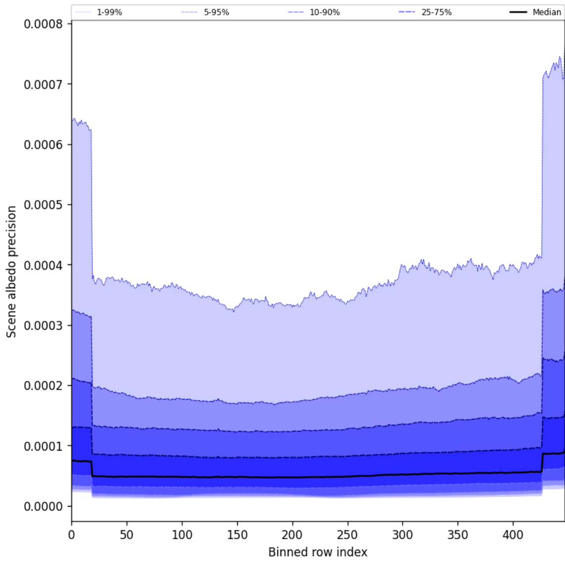
Figure 52: Along track statistics of “Scene albedo precision” for 2025-05-28 to 2025-05-30
