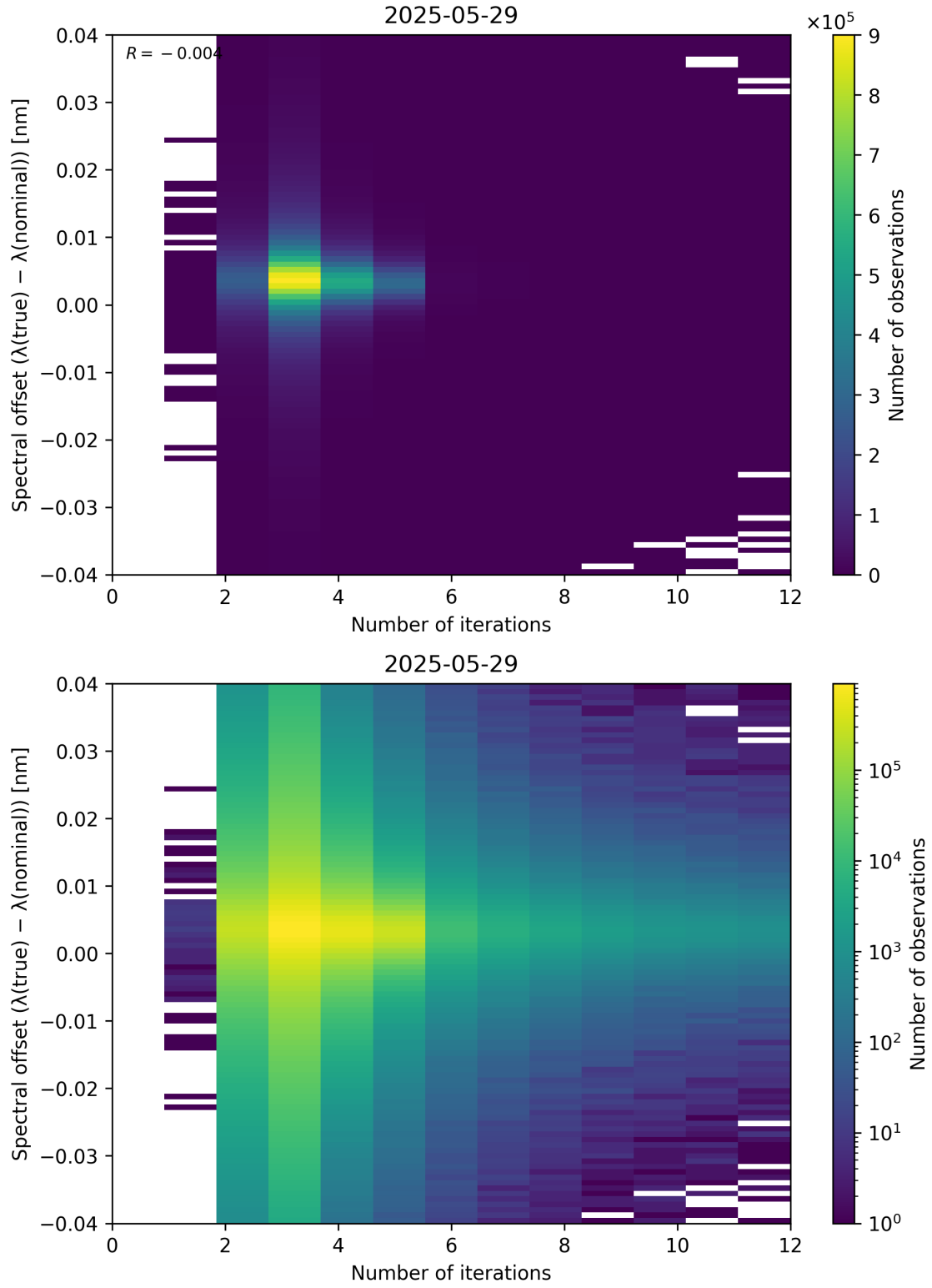
Figure 100: Scatter density plot of “Number of iterations” against “Spectral offset ( \lambda_{\text{true}} - \lambda_{\text{nominal}} )” for 2025-05-28 to 2025-05-30.
