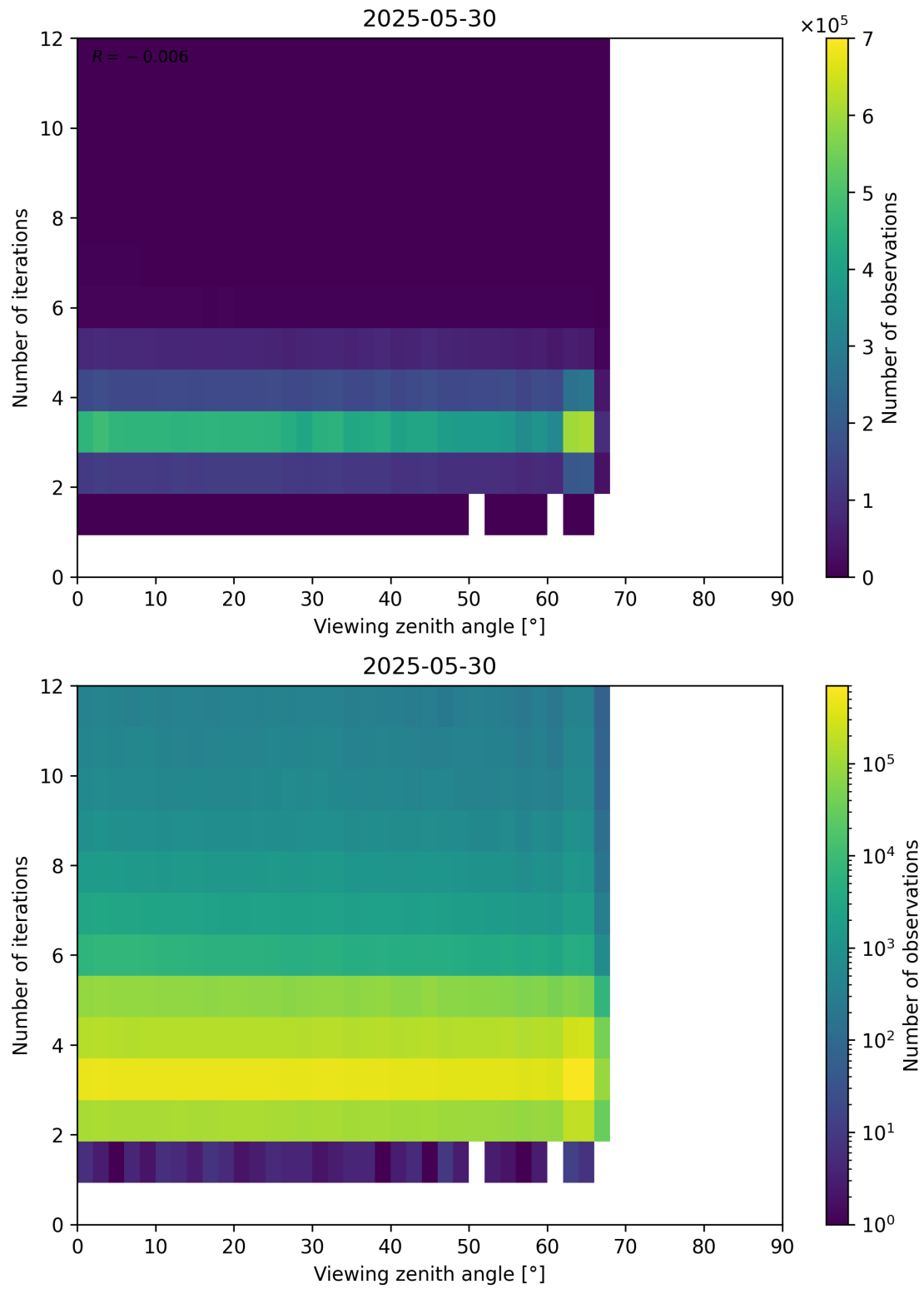
Figure 124: Scatter density plot of “Viewing zenith angle” against “Number of iterations” for 2025-05-29 to 2025-05-31.
