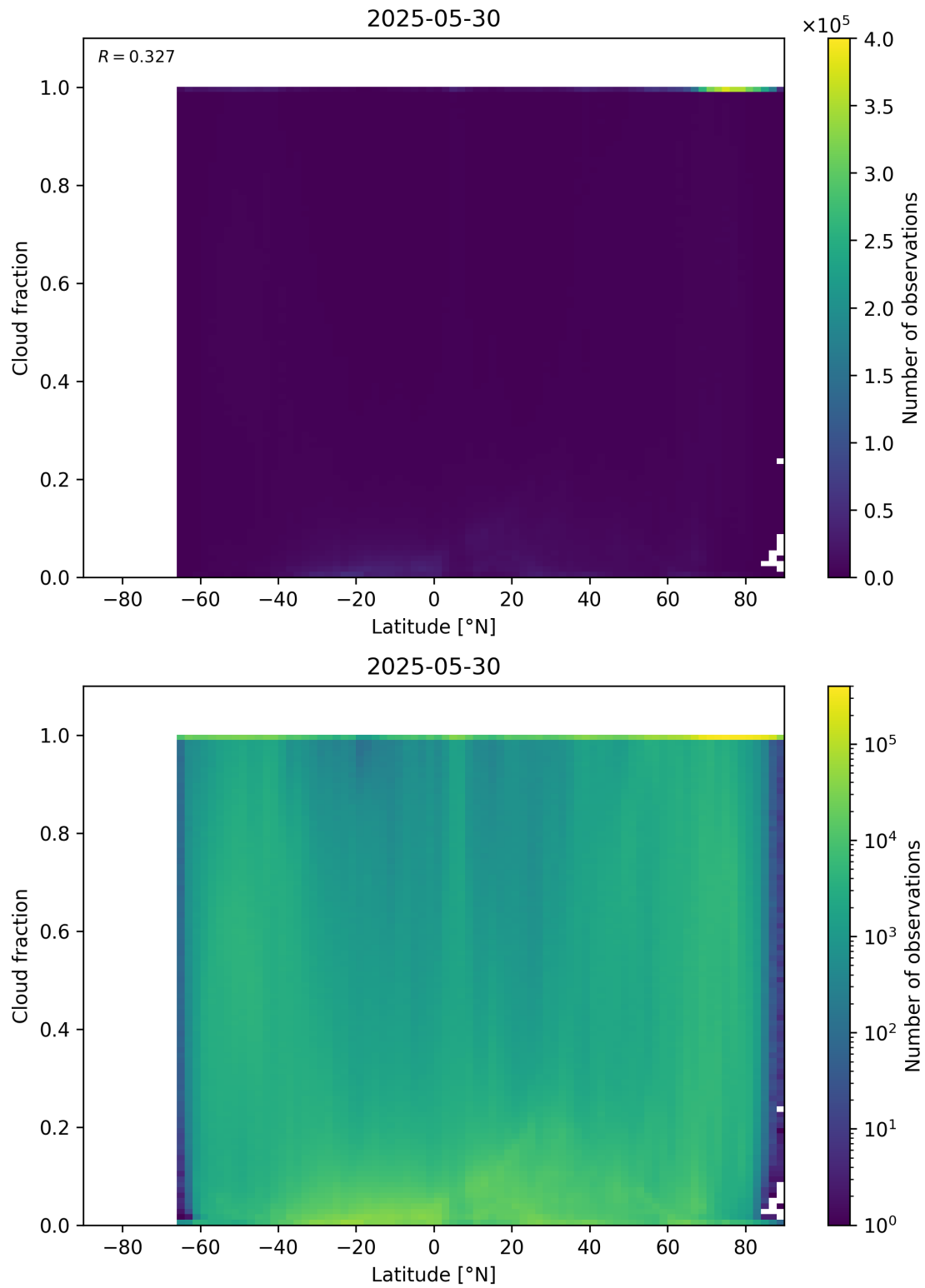
Figure 90: Scatter density plot of “Latitude” against “Cloud fraction” for 2025-05-29 to 2025-05-31.
