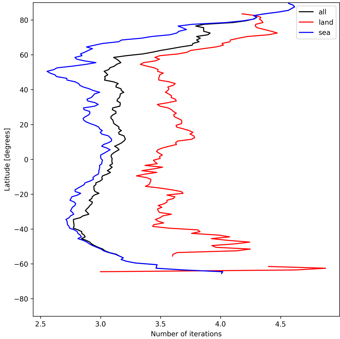
Figure 22: Zonal average of “Number of iterations” for 2025-05-29 to 2025-05-31.
