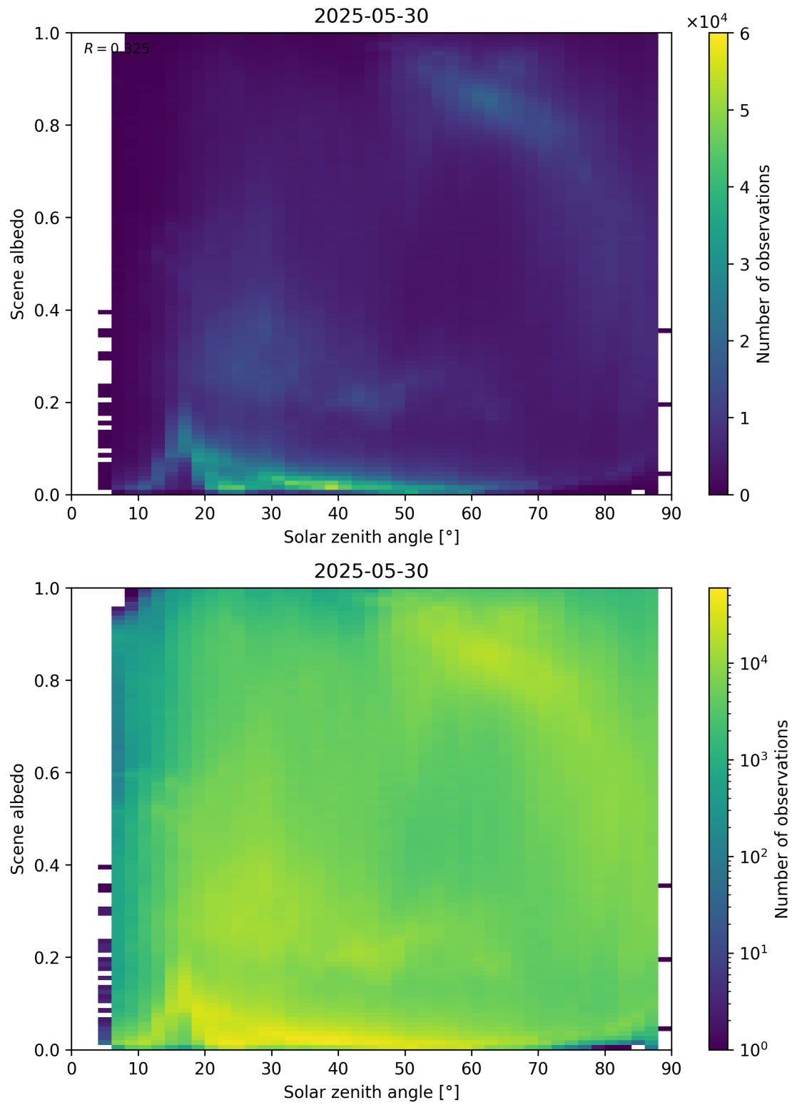
Figure 116: Scatter density plot of “Solar zenith angle” against “Scene albedo” for 2025-05-29 to 2025-05-31.
