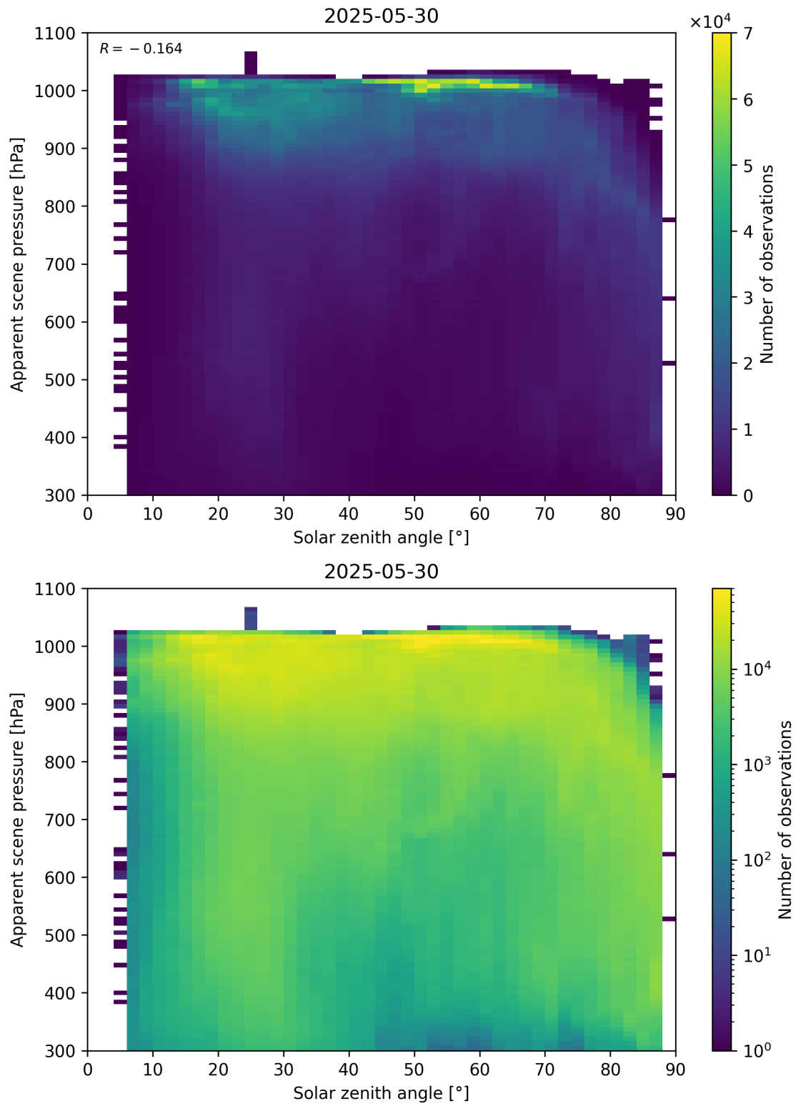
Figure 108: Scatter density plot of “Solar zenith angle” against “Apparent scene pressure” for 2025-05-29 to 2025-05-31.
