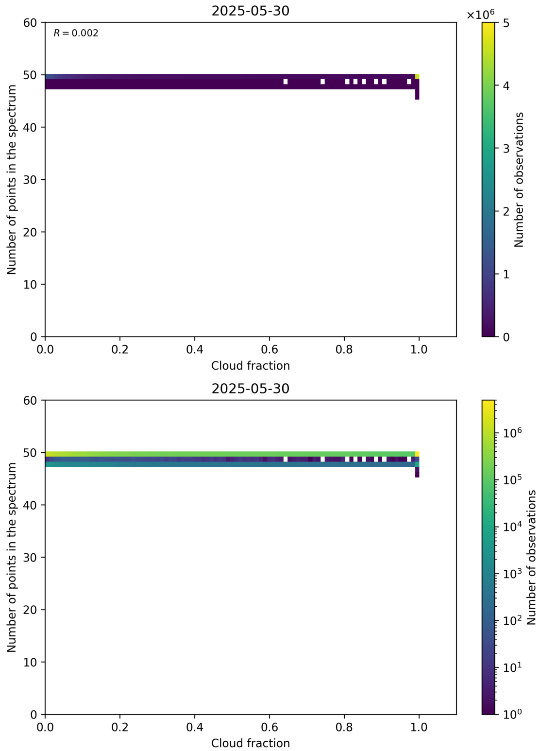
Figure 74: Scatter density plot of “Cloud fraction” against “Number of points in the spectrum” for 2025-05-29 to 2025-05-31.
