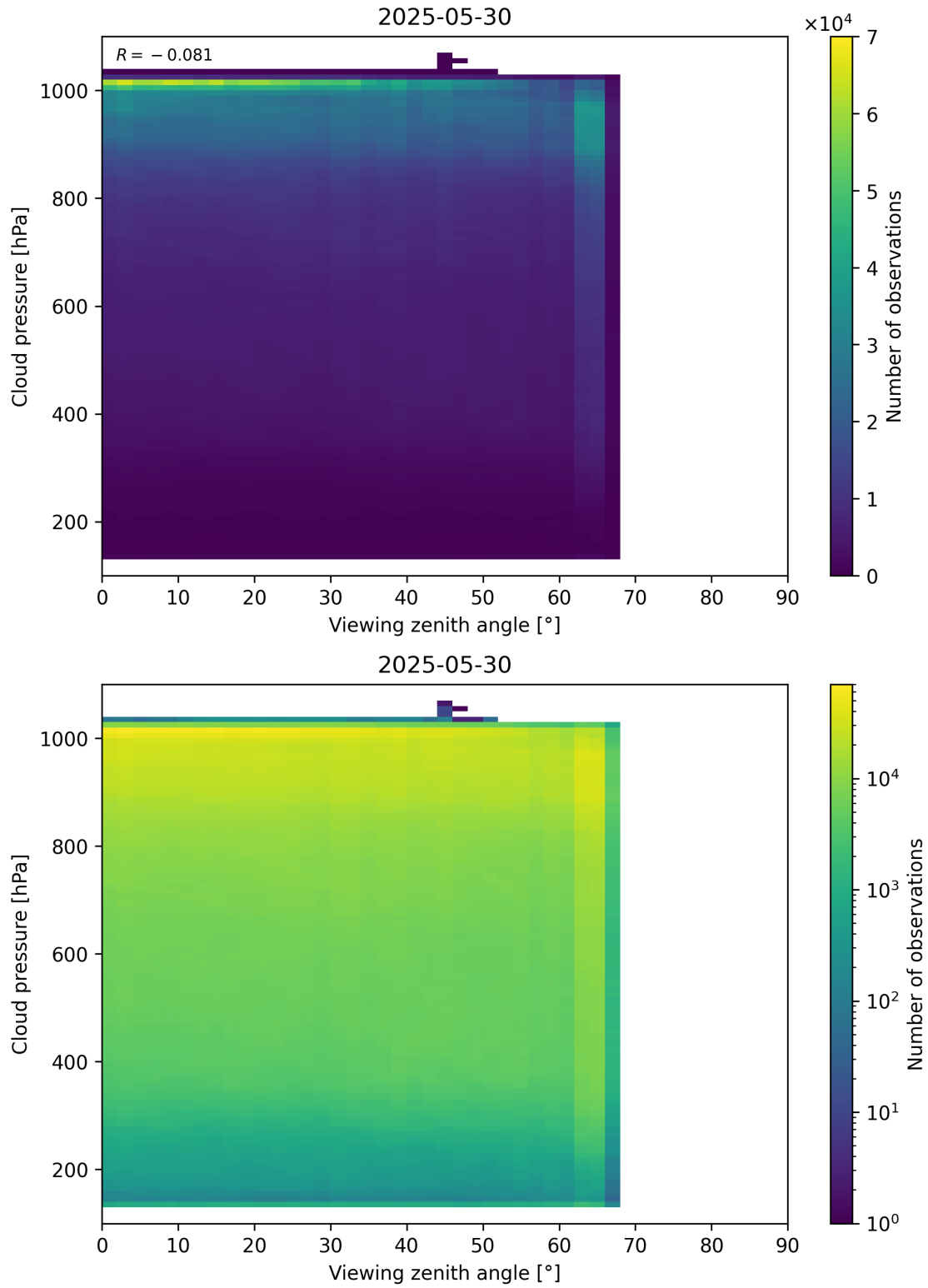
Figure 121: Scatter density plot of “Viewing zenith angle” against “Cloud pressure” for 2025-05-29 to 2025-05-31.
