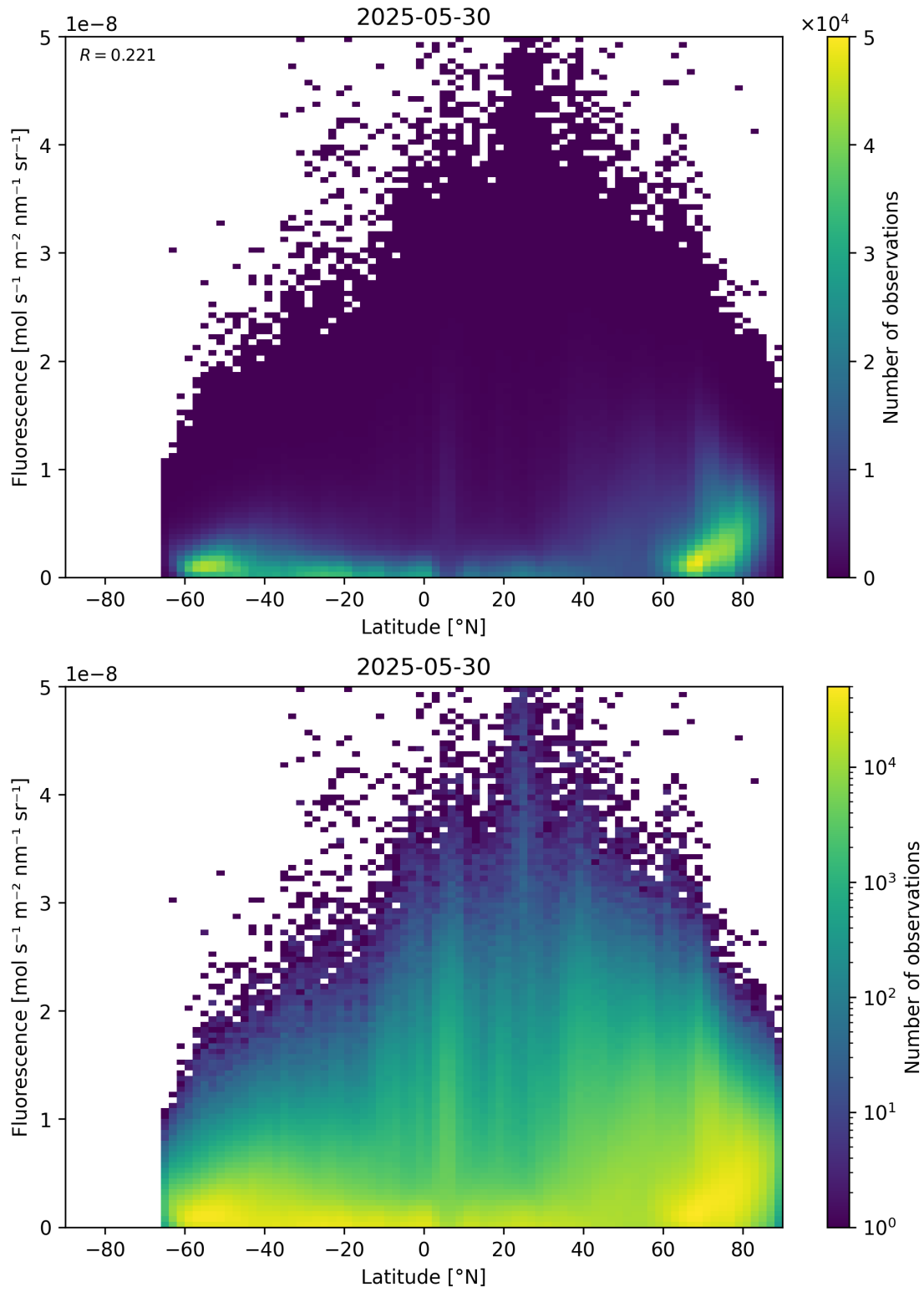
Figure 92: Scatter density plot of “Latitude” against “Fluorescence” for 2025-05-29 to 2025-05-31.
