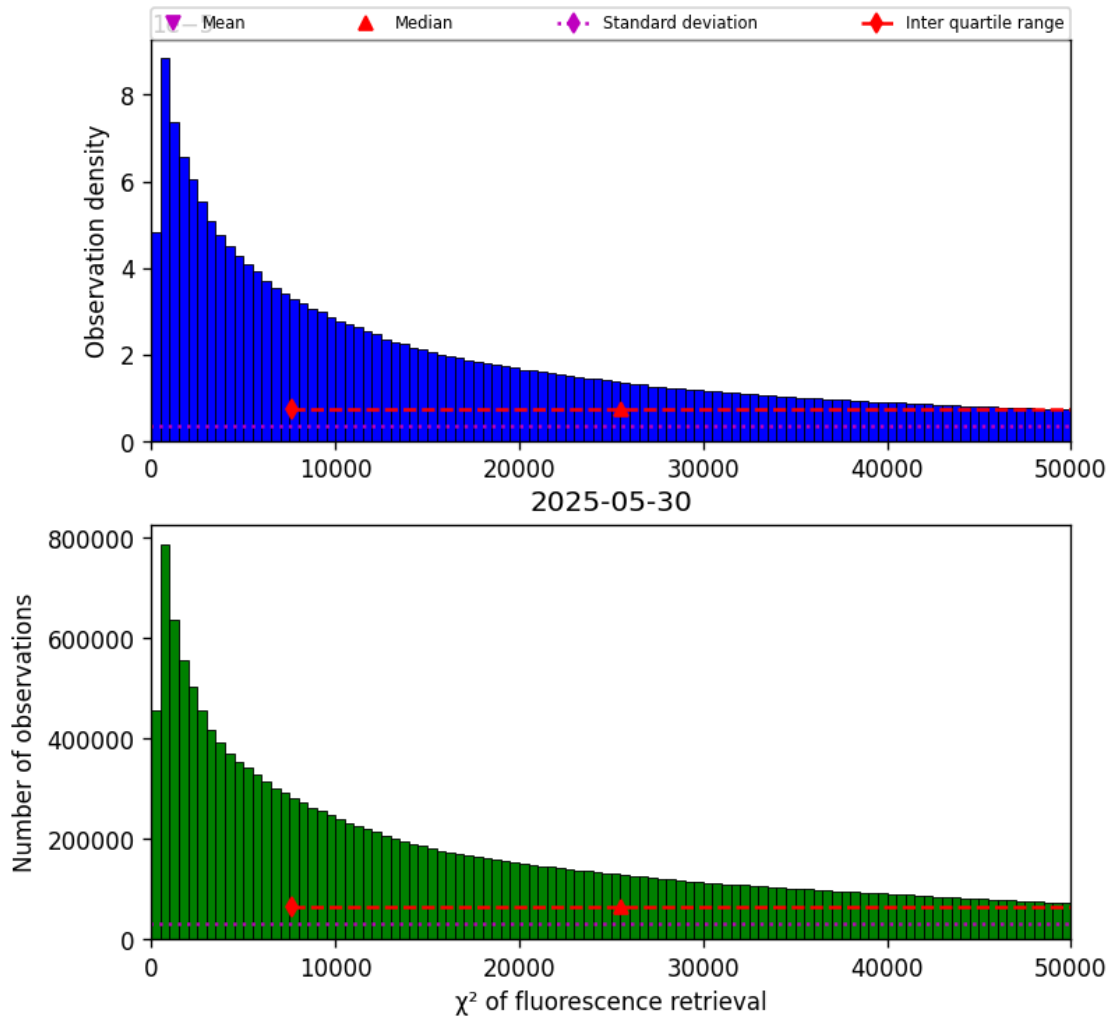
Figure 42: Histogram of “ \chi^2 of fluorescence retrieval” for 2025-05-29 to 2025-05-31
