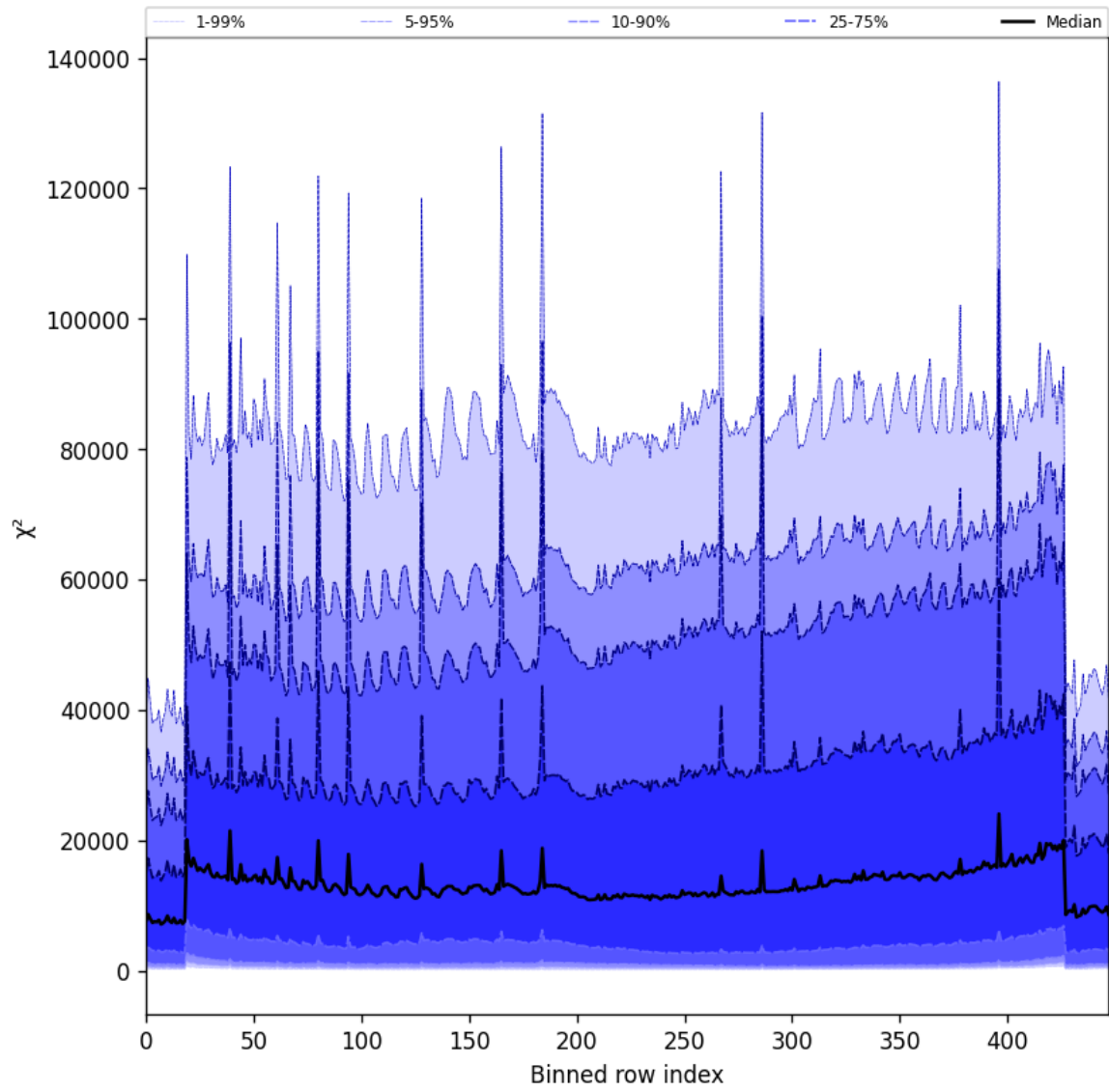
Figure 55: Along track statistics of “ \chi^2 ” for 2025-05-29 to 2025-05-31
