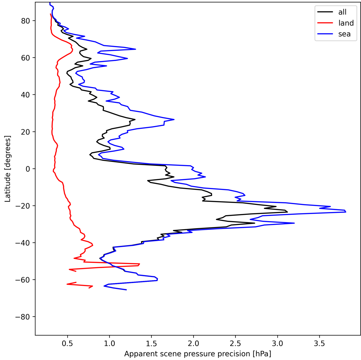
Figure 20: Zonal average of “Apparent scene pressure precision” for 2025-05-29 to 2025-05-31.
