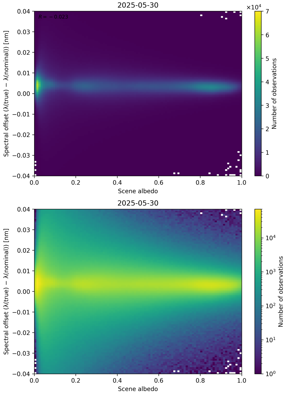
Figure 107: Scatter density plot of “Scene albedo” against “Spectral offset ( \lambda_{\text{true}} - \lambda_{\text{nominal}} )” for 2025-05-29 to 2025-05-31.
