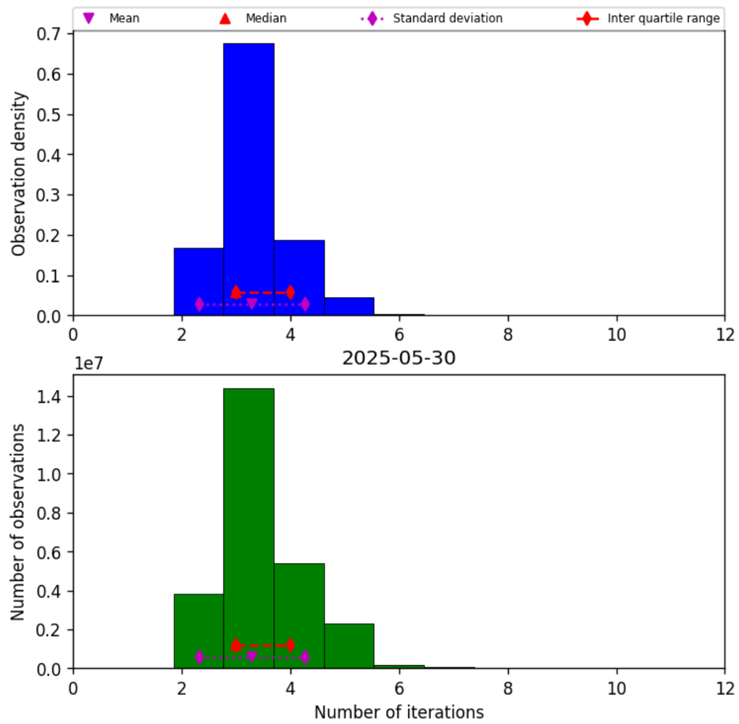
Figure 39: Histogram of “Number of iterations” for 2025-05-29 to 2025-05-31
