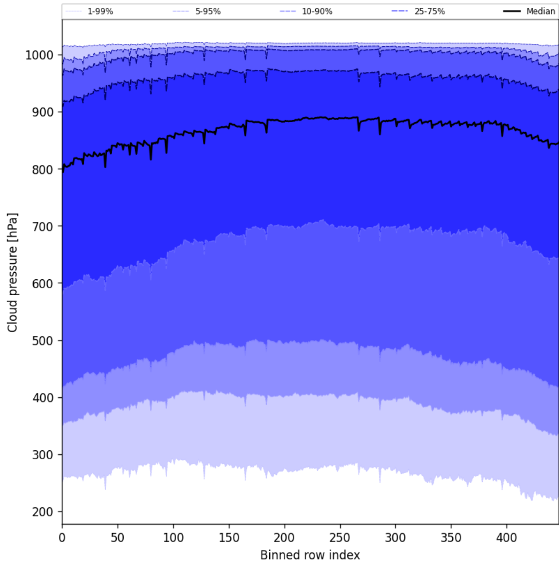
Figure 47: Along track statistics of “Cloud pressure” for 2025-05-29 to 2025-05-31
