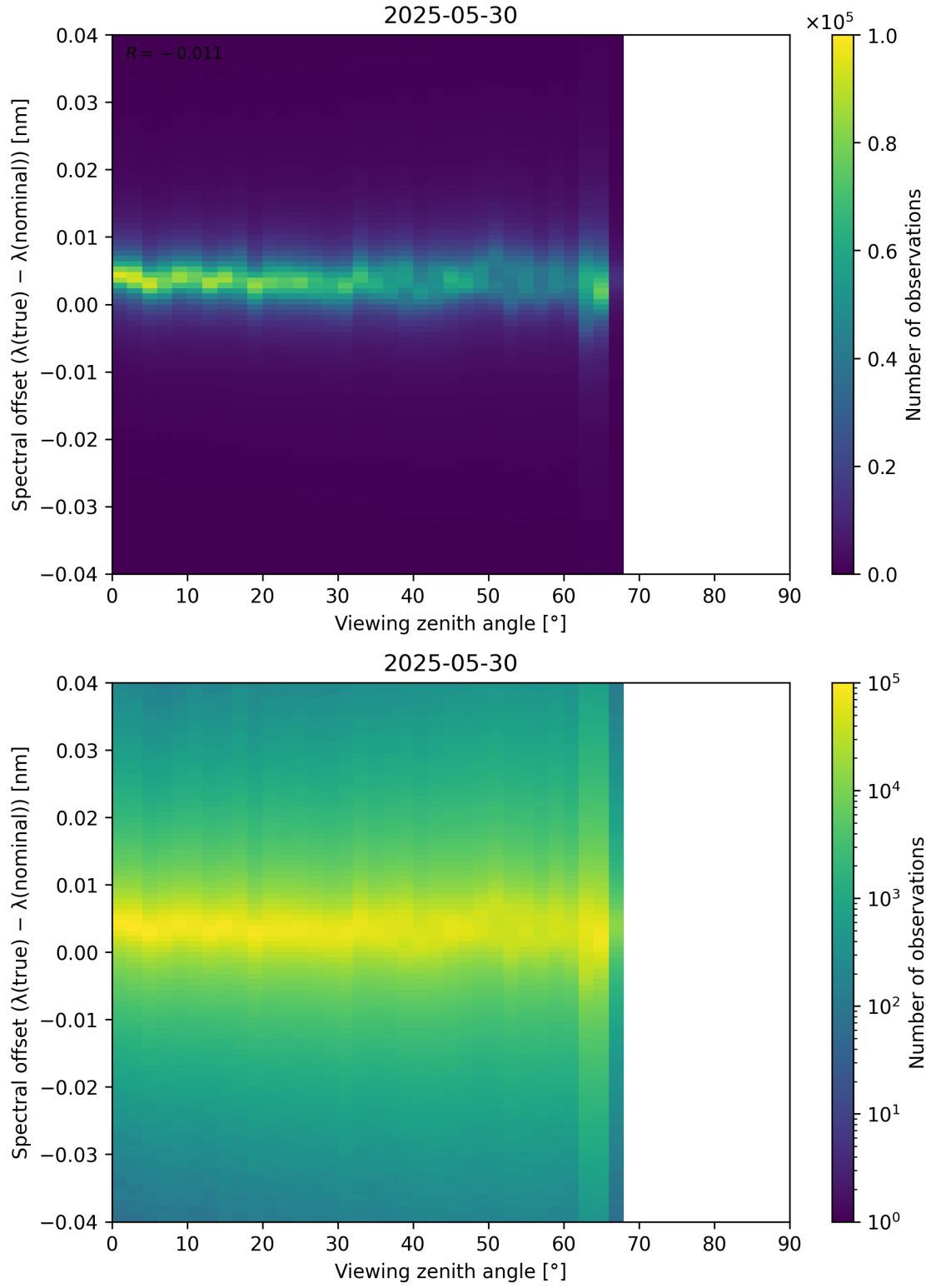
Figure 128: Scatter density plot of “Viewing zenith angle” against “Spectral offset ( \lambda_{\text{true}} - \lambda_{\text{nominal}} )” for 2025-05-29 to 2025-05-31.
