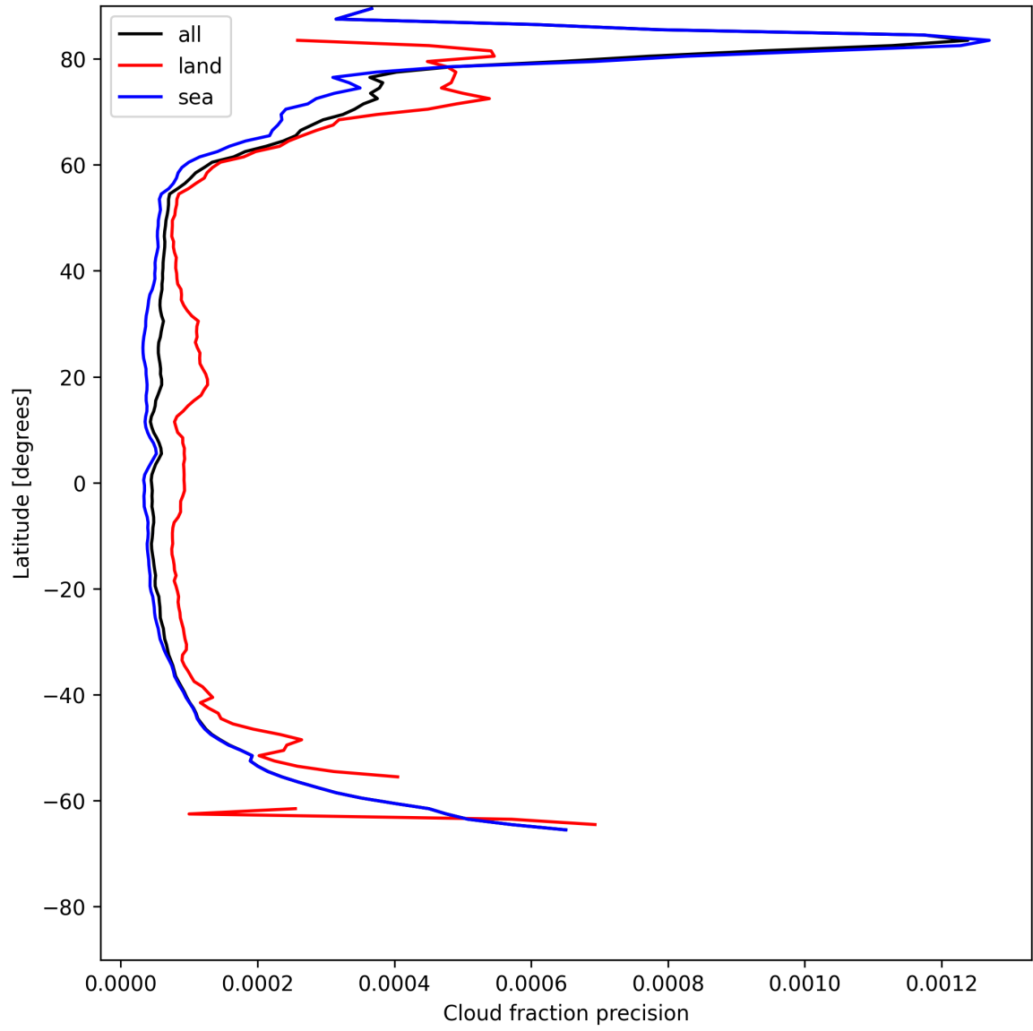
Figure 16: Zonal average of “Cloud fraction precision” for 2025-05-29 to 2025-05-31.
