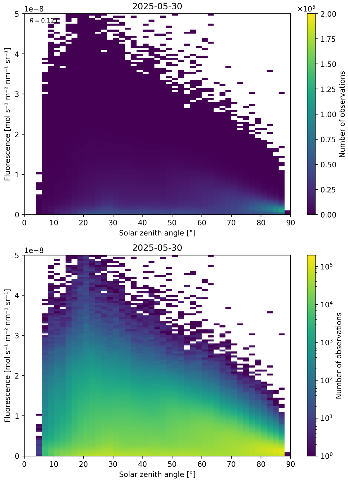
Figure 112: Scatter density plot of “Solar zenith angle” against “Fluorescence” for 2025-05-29 to 2025-05-31.
