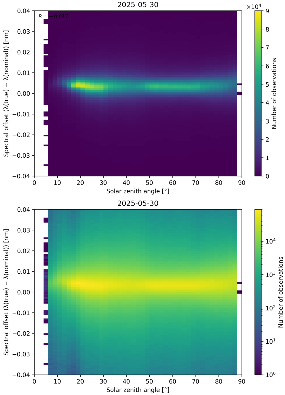
Figure 117: Scatter density plot of “Solar zenith angle” against “Spectral offset ( \lambda_{\text{true}} - \lambda_{\text{nominal}} )” for 2025-05-29 to 2025-05-31.
