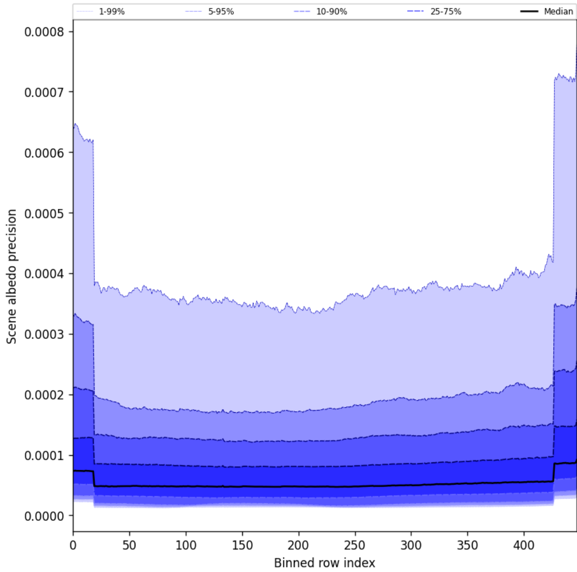
Figure 52: Along track statistics of “Scene albedo precision” for 2025-05-29 to 2025-05-31
