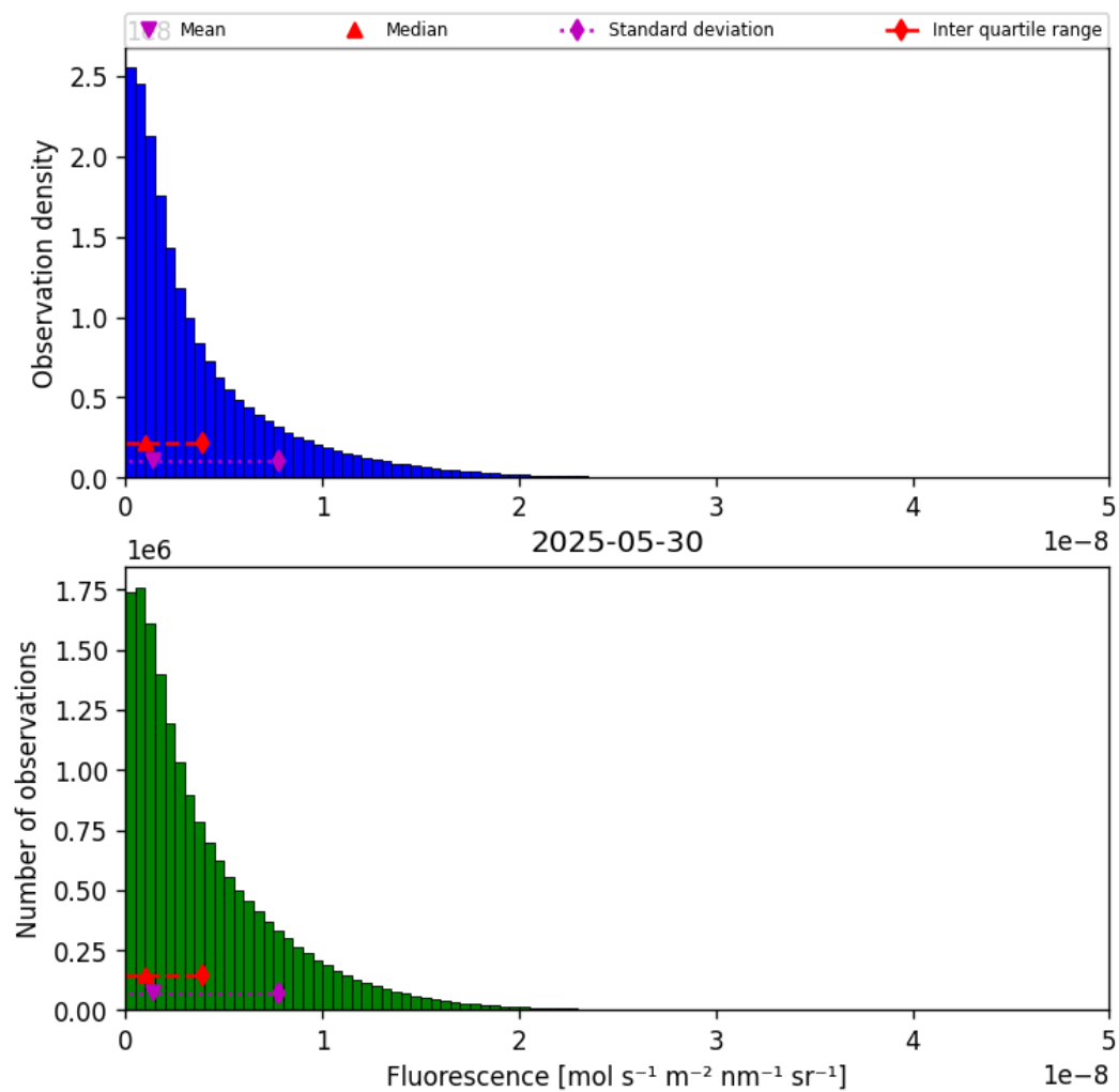
Figure 40: Histogram of “Fluorescence” for 2025-05-29 to 2025-05-31
