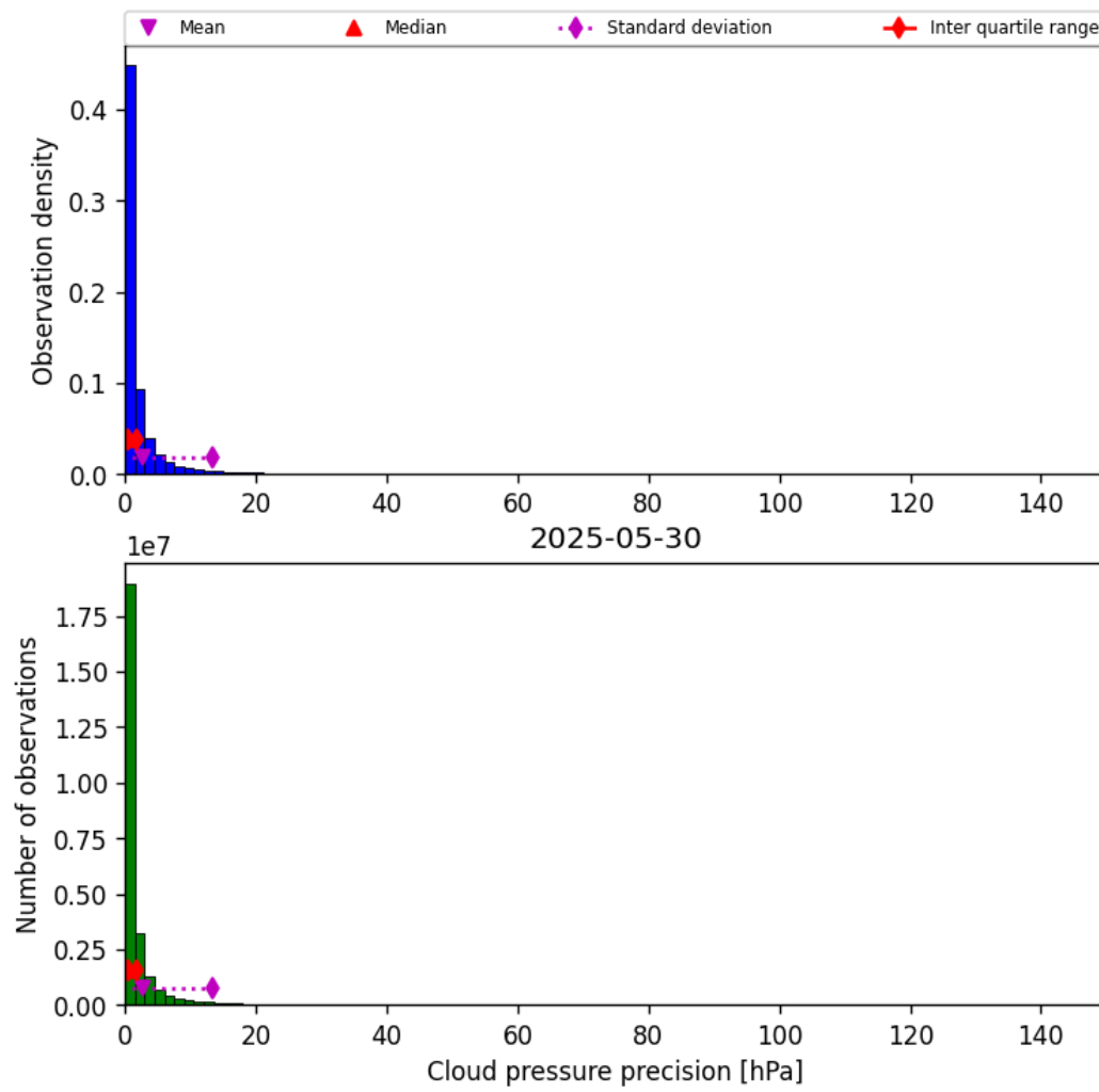
Figure 31: Histogram of “Cloud pressure precision” for 2025-05-29 to 2025-05-31
