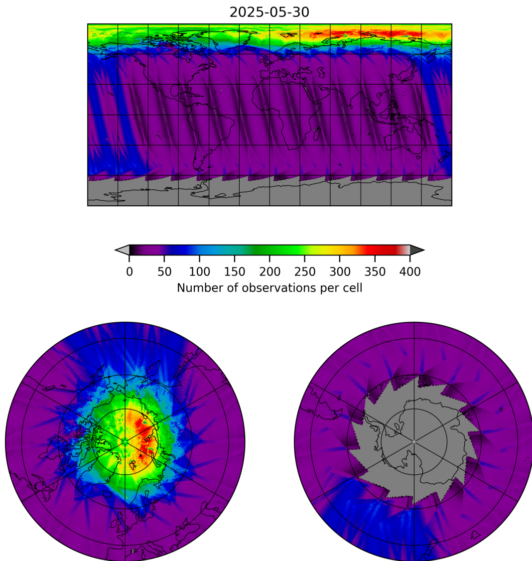
Figure 11: Map of the number of observations for 2025-05-29 to 2025-05-31
