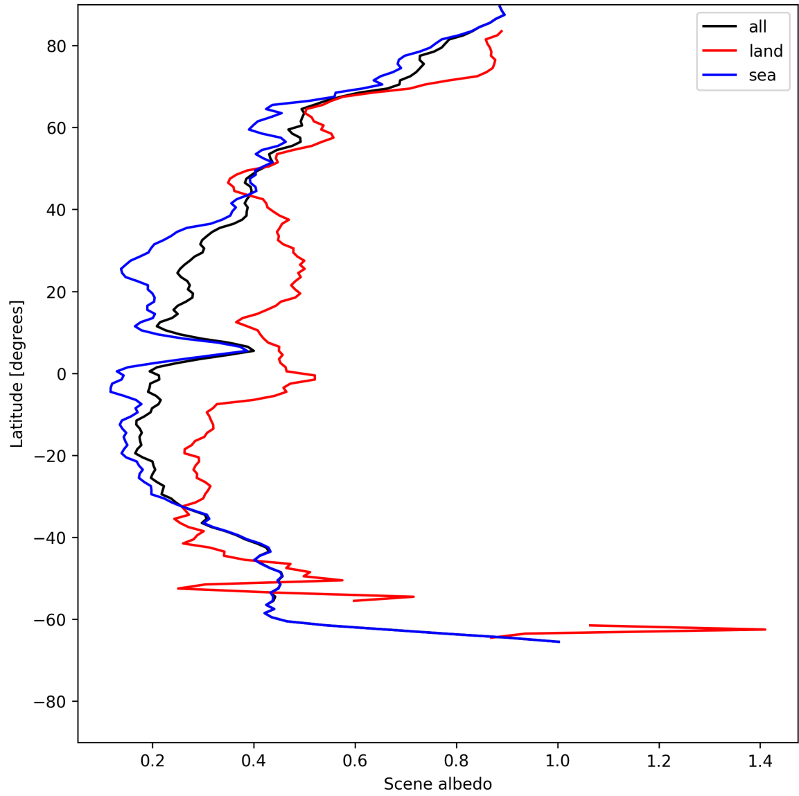
Figure 17: Zonal average of “Scene albedo” for 2025-05-29 to 2025-05-31.
