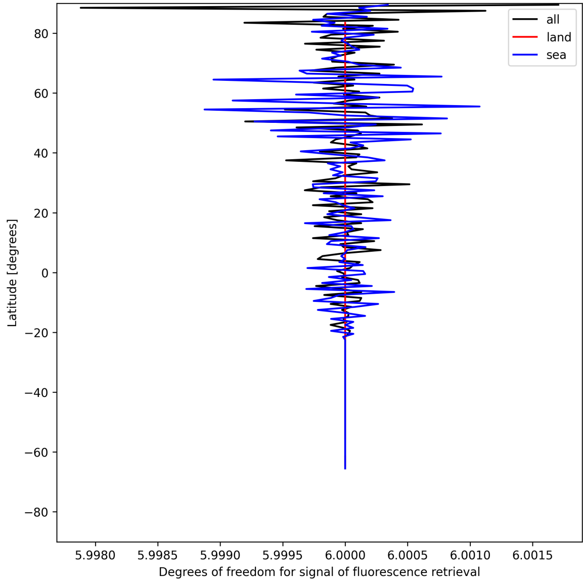
Figure 26: Zonal average of “Degrees of freedom for signal of fluorescence retrieval” for 2025-05-29 to 2025-05-31.
