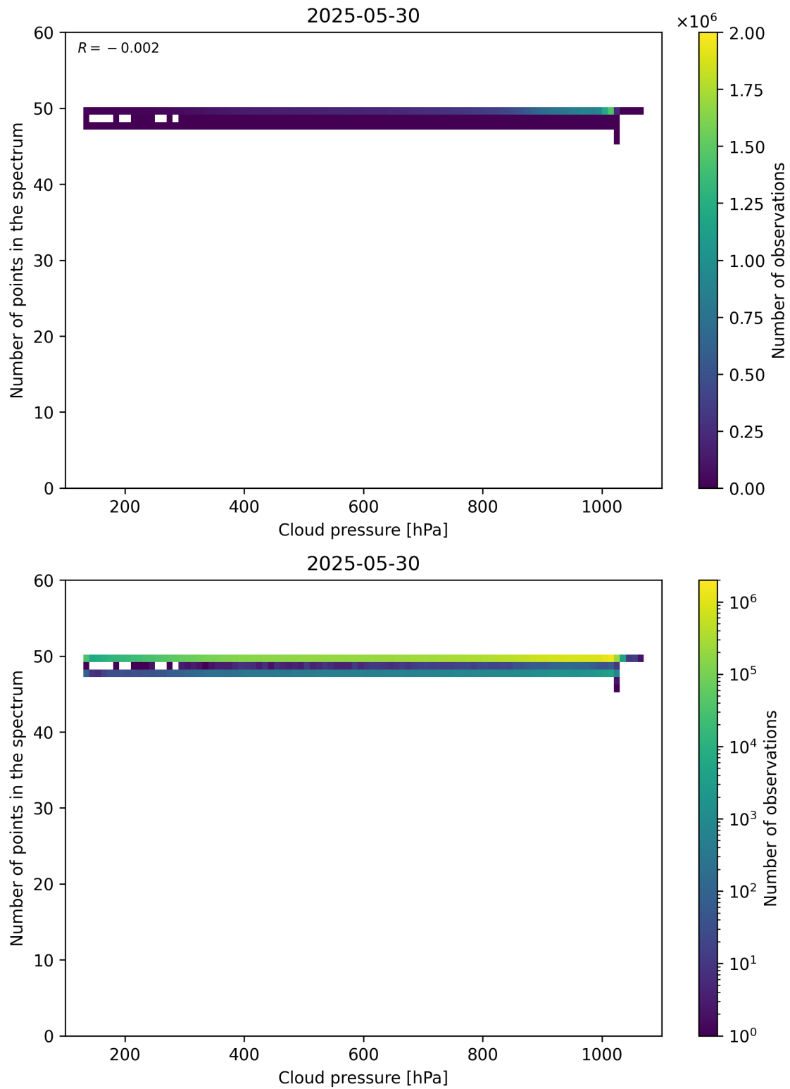
Figure 82: Scatter density plot of “Cloud pressure” against “Number of points in the spectrum” for 2025-05-29 to 2025-05-31.
