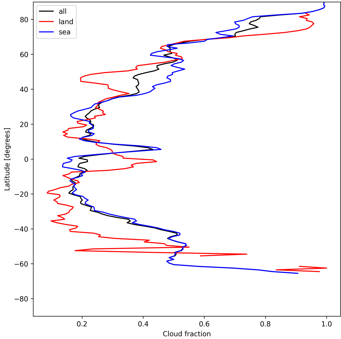
Figure 15: Zonal average of “Cloud fraction” for 2025-05-29 to 2025-05-31.
