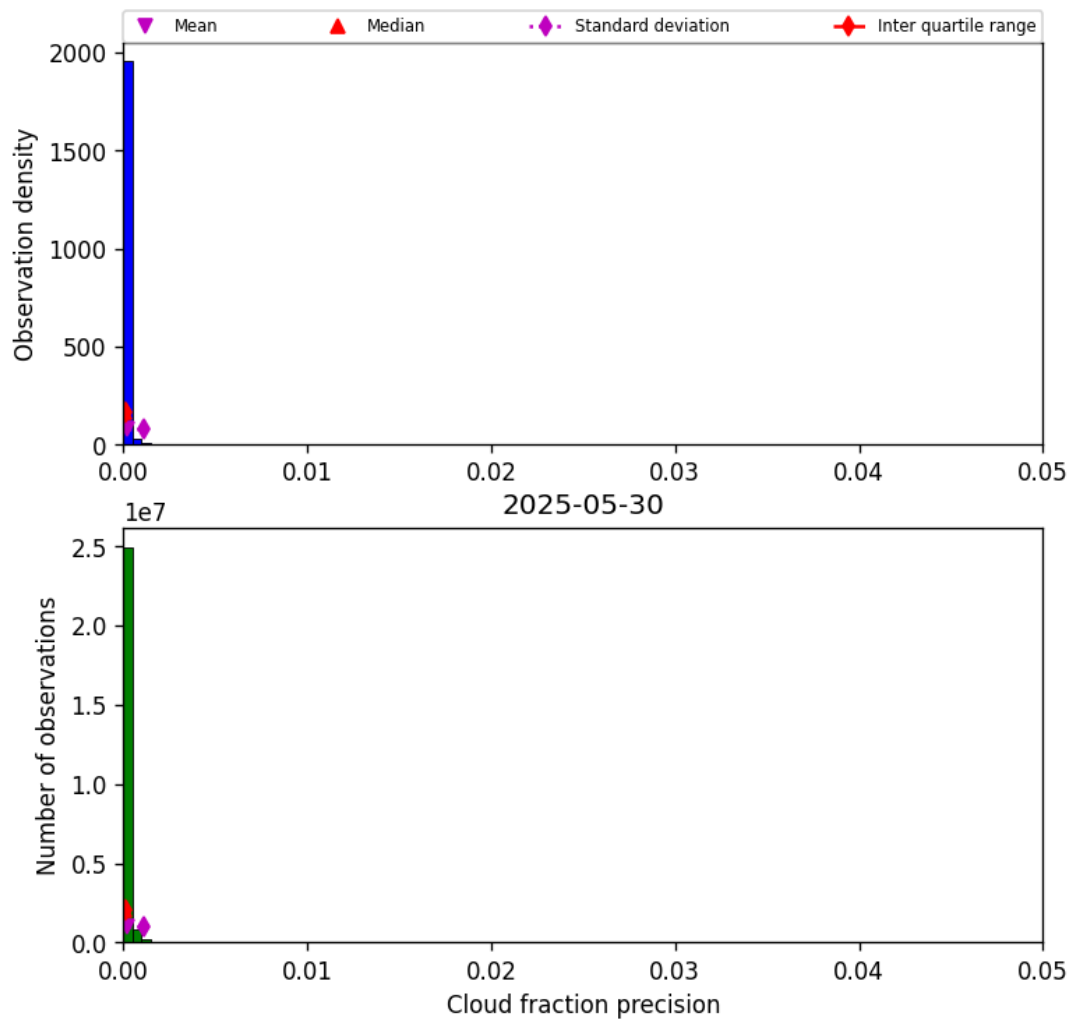
Figure 33: Histogram of “Cloud fraction precision” for 2025-05-29 to 2025-05-31
