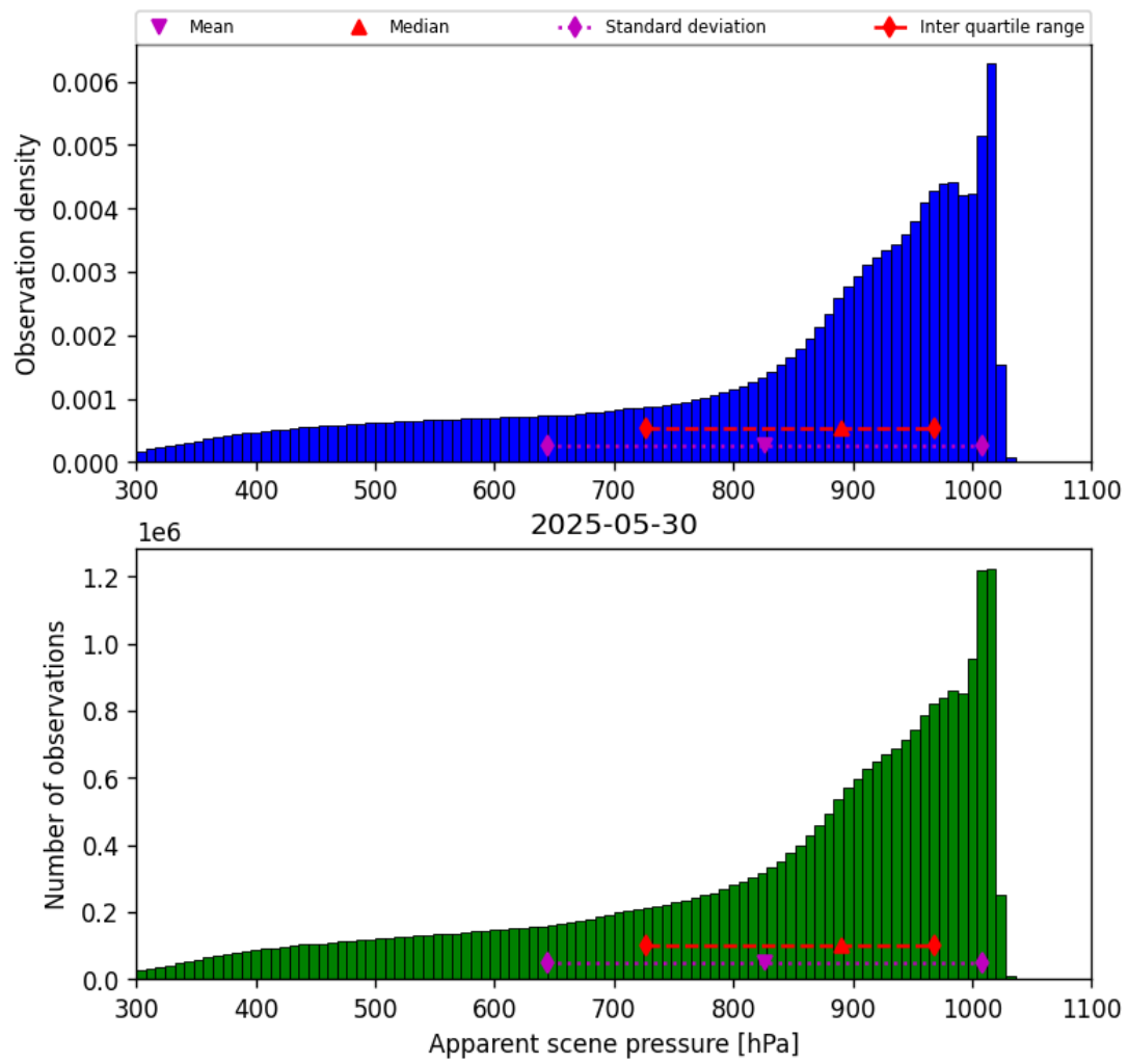
Figure 36: Histogram of “Apparent scene pressure” for 2025-05-29 to 2025-05-31
