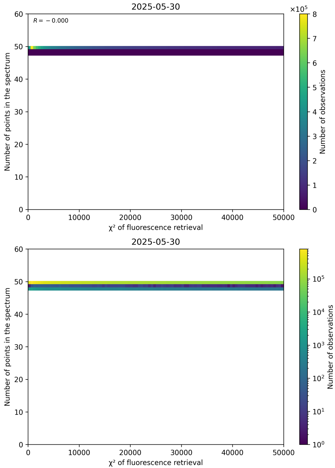
Figure 68: Scatter density plot of " \chi^2 of fluorescence retrieval" against "Number of points in the spectrum" for 2025-05-29 to 2025-05-31.
