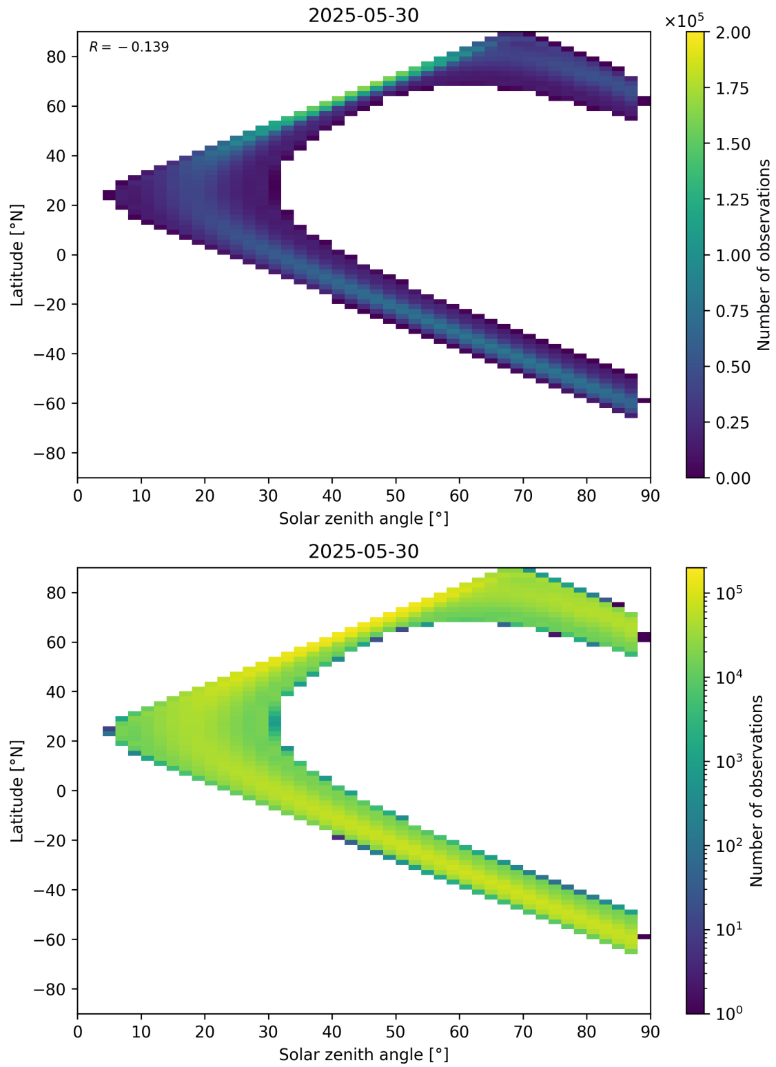
Figure 113: Scatter density plot of “Solar zenith angle” against “Latitude” for 2025-05-29 to 2025-05-31.
