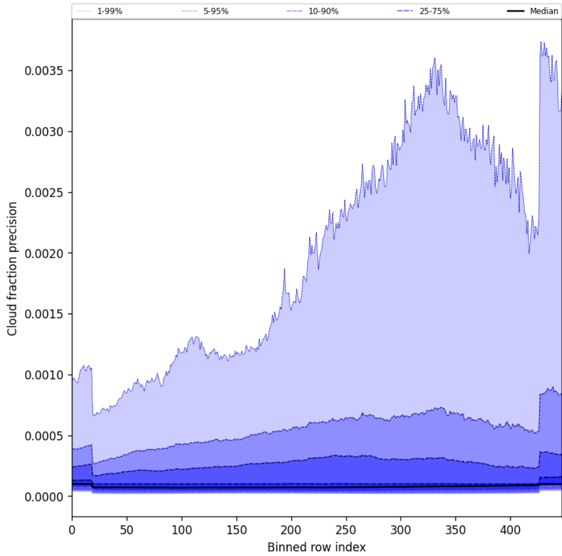
Figure 50: Along track statistics of “Cloud fraction precision” for 2025-05-29 to 2025-05-31
