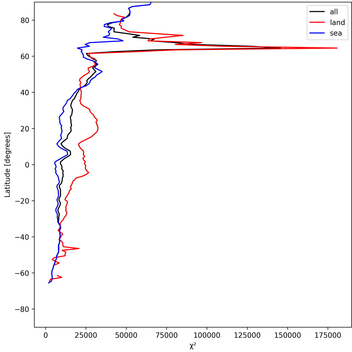
Figure 21: Zonal average of “ \chi^2 ” for 2025-05-29 to 2025-05-31.
