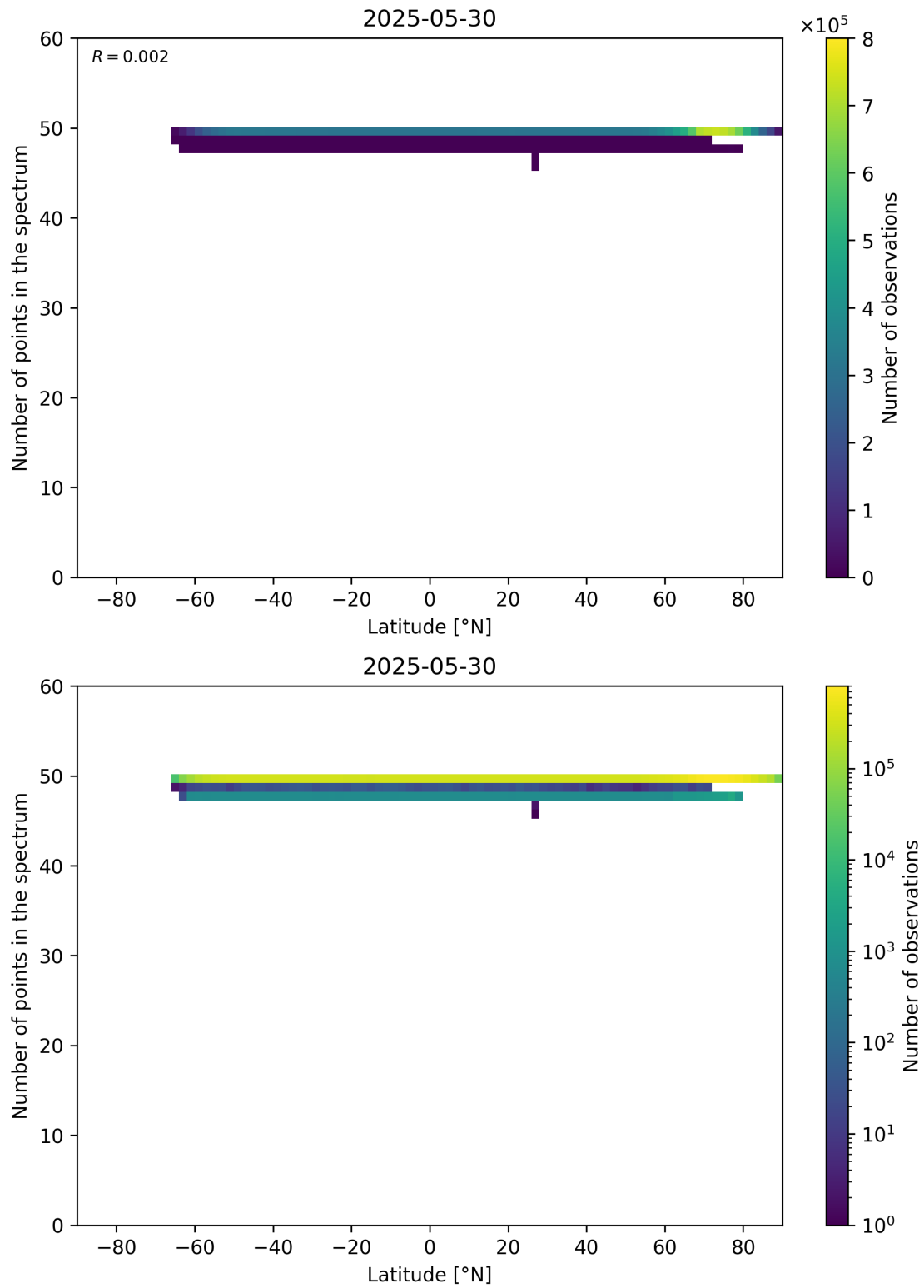
Figure 94: Scatter density plot of “Latitude” against “Number of points in the spectrum” for 2025-05-29 to 2025-05-31.
