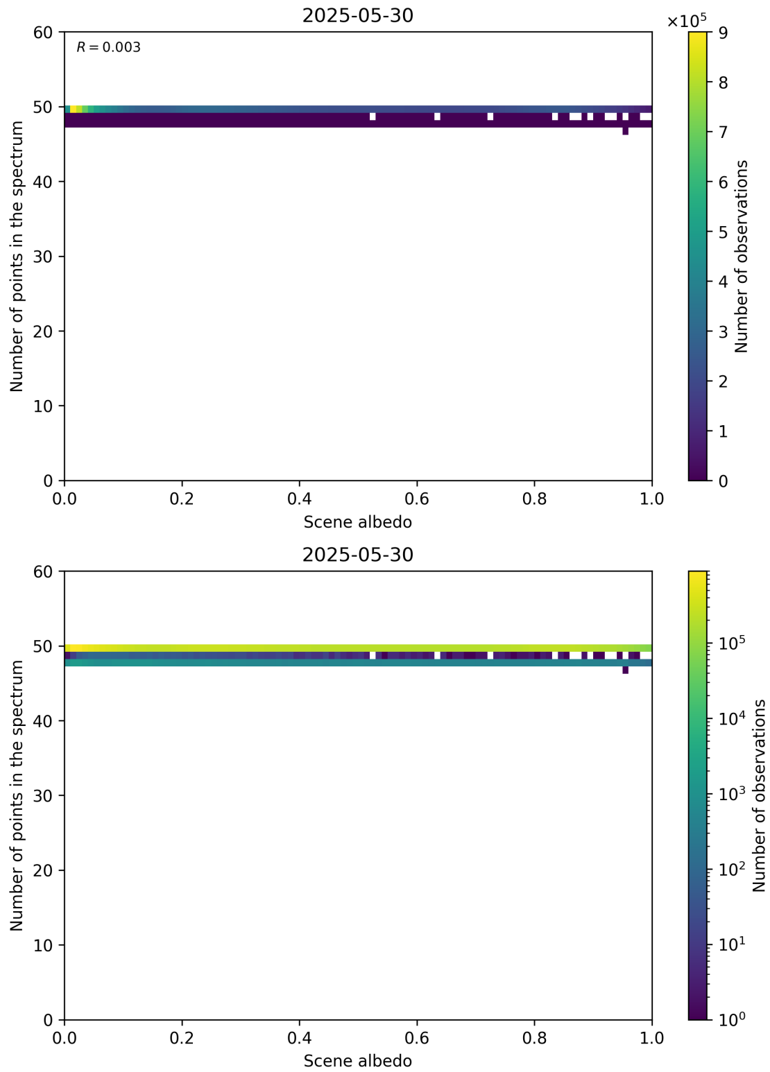
Figure 106: Scatter density plot of “Scene albedo” against “Number of points in the spectrum” for 2025-05-29 to 2025-05-31.
