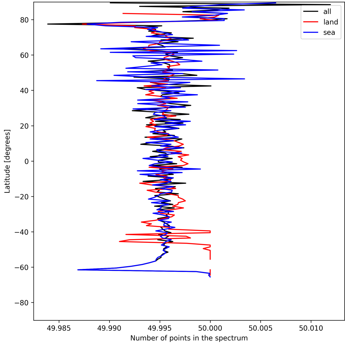
Figure 27: Zonal average of “Number of points in the spectrum” for 2025-05-29 to 2025-05-31.
