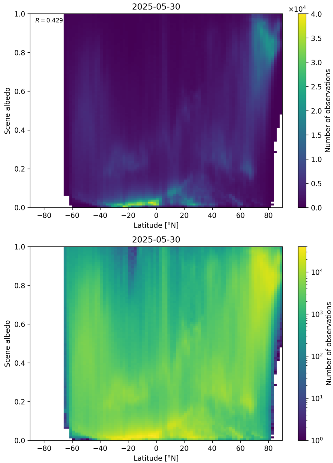
Figure 95: Scatter density plot of “Latitude” against “Scene albedo” for 2025-05-29 to 2025-05-31.
