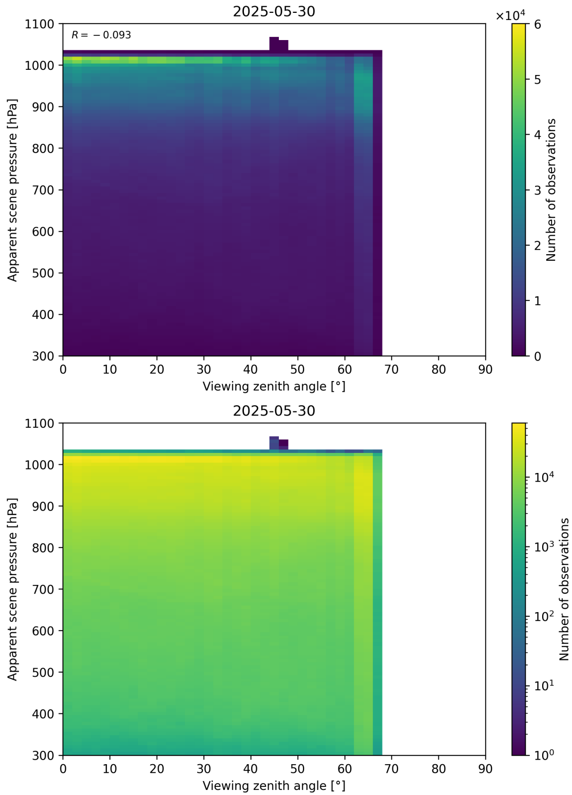
Figure 118: Scatter density plot of “Viewing zenith angle” against “Apparent scene pressure” for 2025-05-29 to 2025-05-31.
