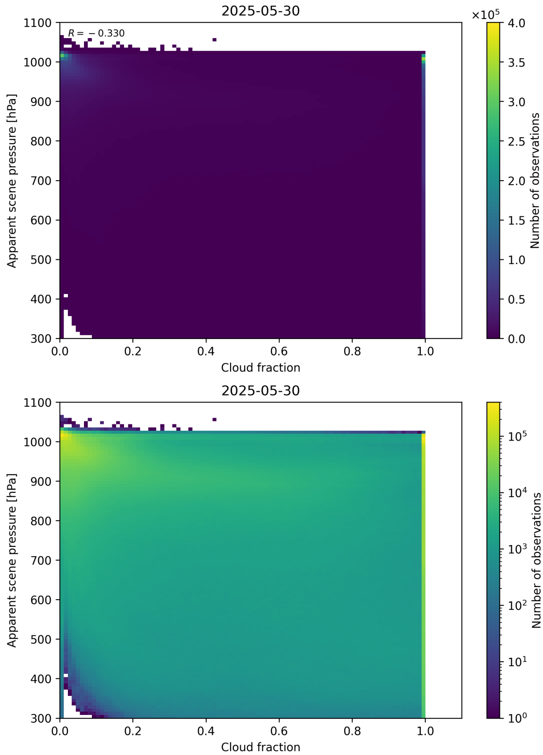
Figure 70: Scatter density plot of “Cloud fraction” against “Apparent scene pressure” for 2025-05-29 to 2025-05-31.
