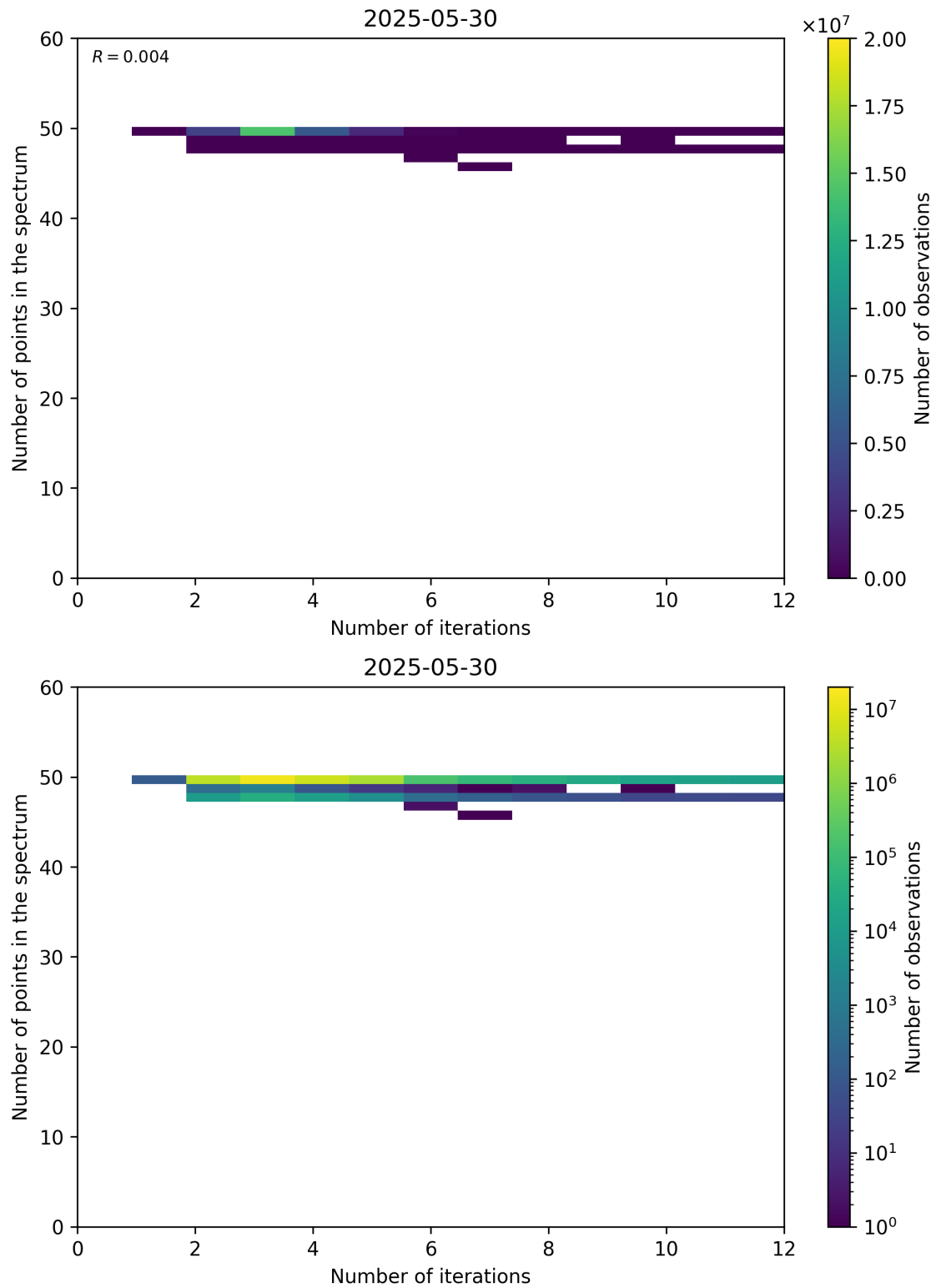
Figure 99: Scatter density plot of “Number of iterations” against “Number of points in the spectrum” for 2025-05-29 to 2025-05-31.
