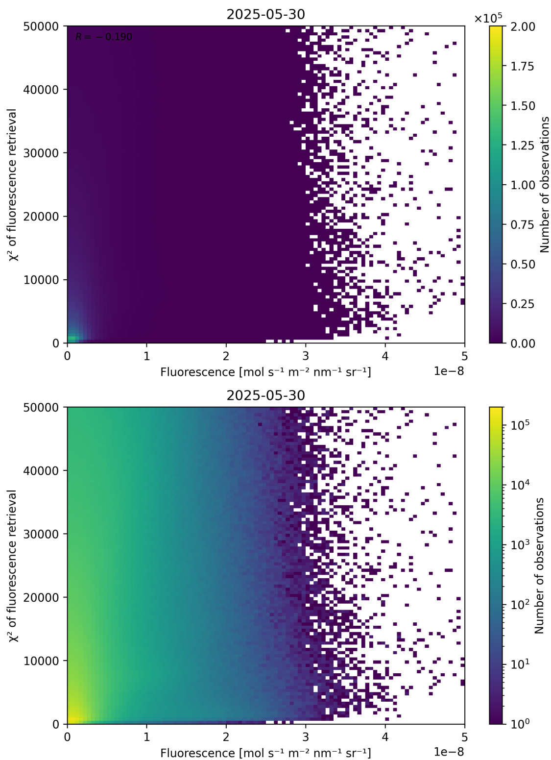
Figure 85: Scatter density plot of “Fluorescence” against “ \chi^2 of fluorescence retrieval” for 2025-05-29 to 2025-05-31.
