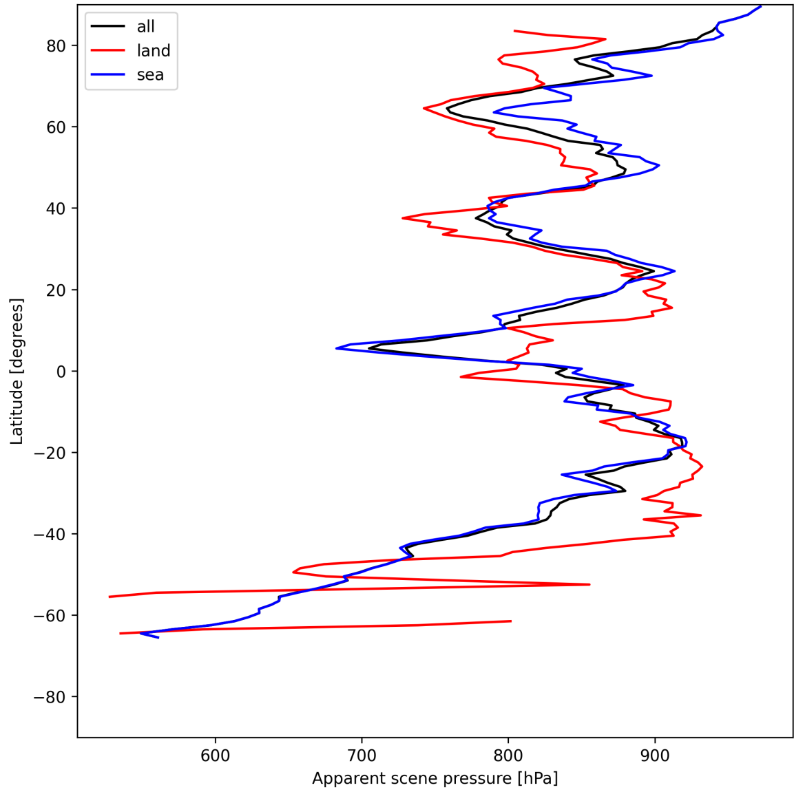
Figure 19: Zonal average of “Apparent scene pressure” for 2025-05-29 to 2025-05-31.
