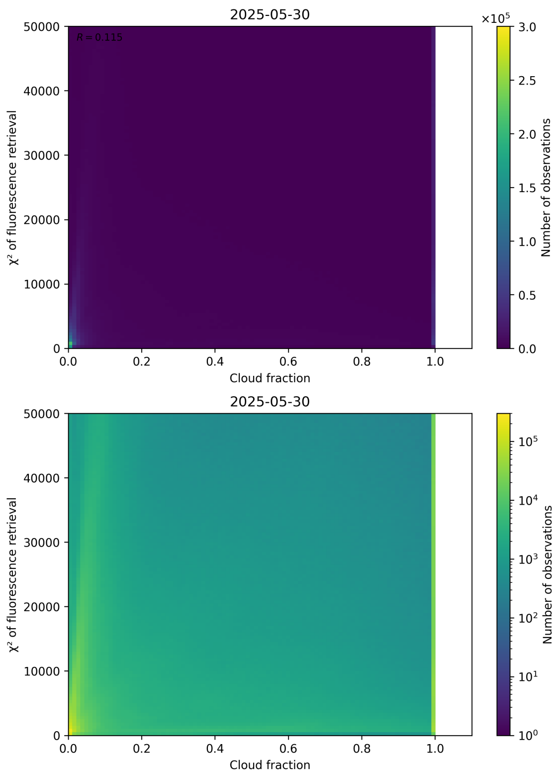
Figure 71: Scatter density plot of “Cloud fraction” against “ \chi^2 of fluorescence retrieval” for 2025-05-29 to 2025-05-31.
