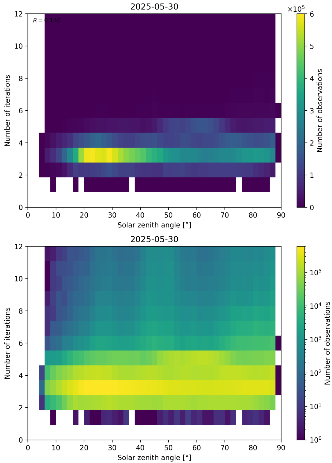
Figure 114: Scatter density plot of “Solar zenith angle” against “Number of iterations” for 2025-05-29 to 2025-05-31.
