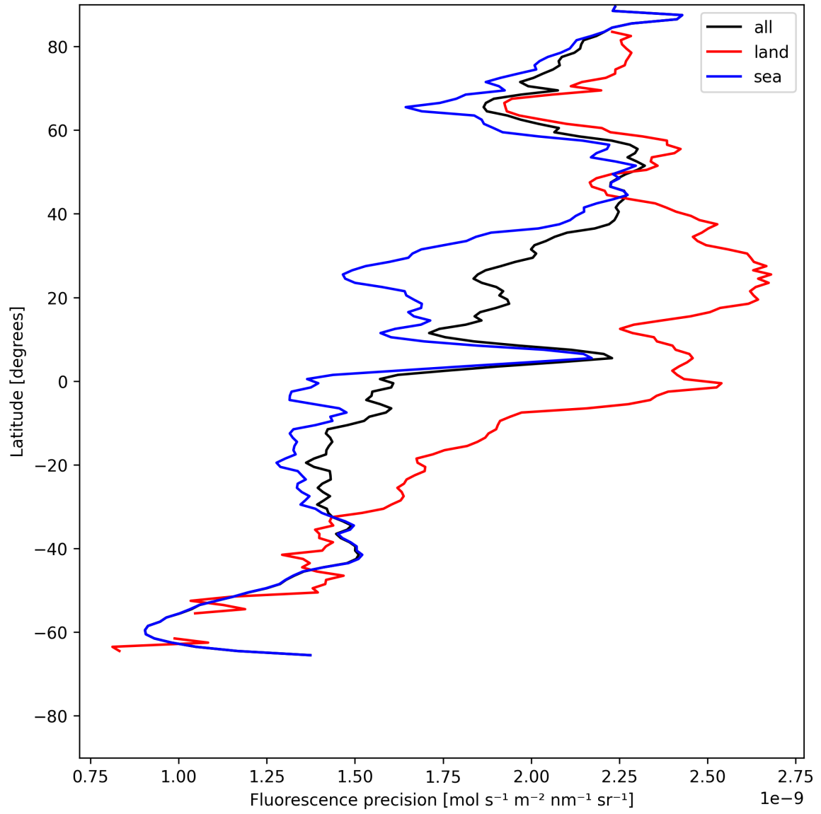
Figure 24: Zonal average of “Fluorescence precision” for 2025-05-29 to 2025-05-31.
