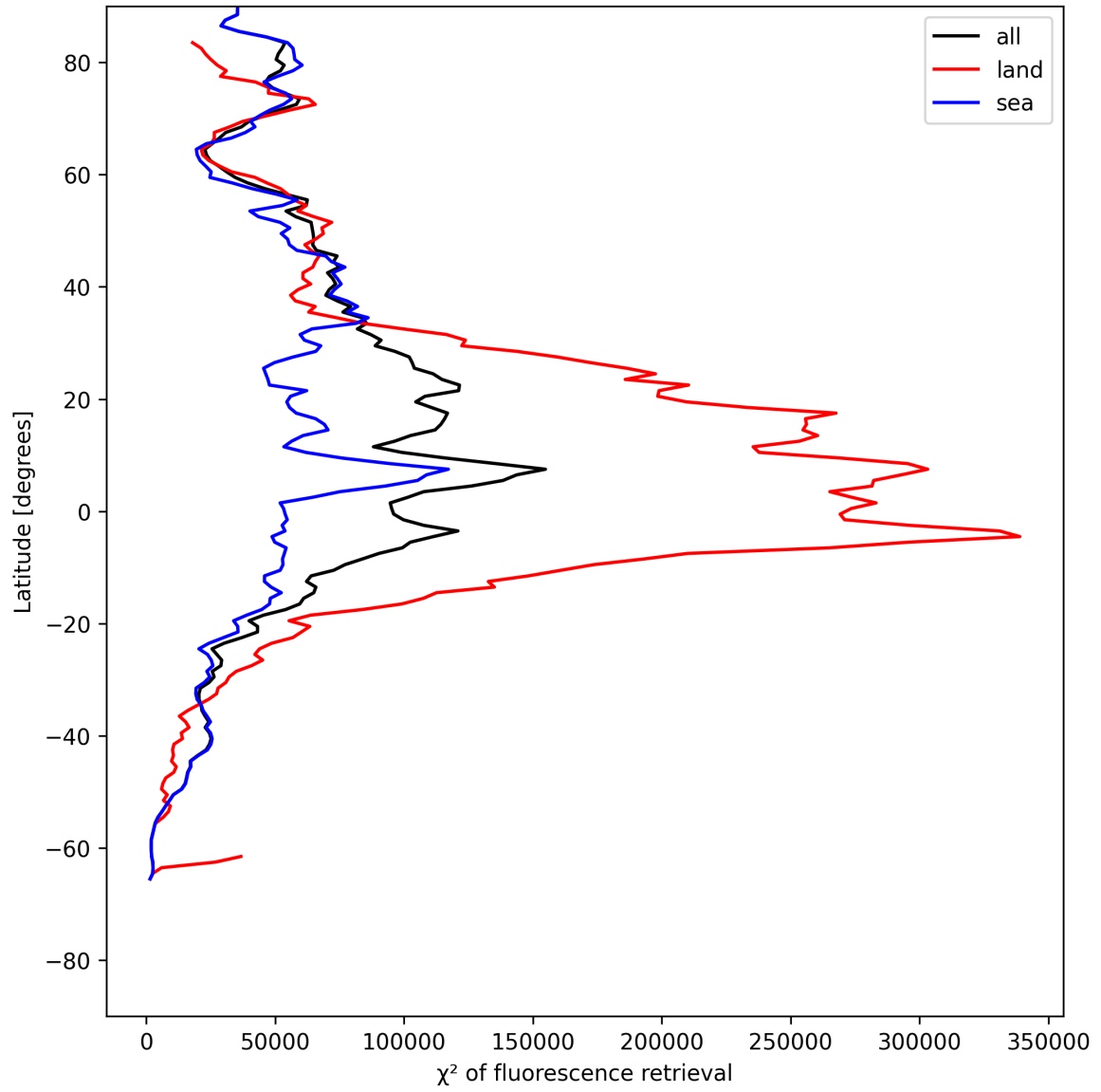
Figure 25: Zonal average of “ \chi^2 of fluorescence retrieval” for 2025-05-29 to 2025-05-31.
