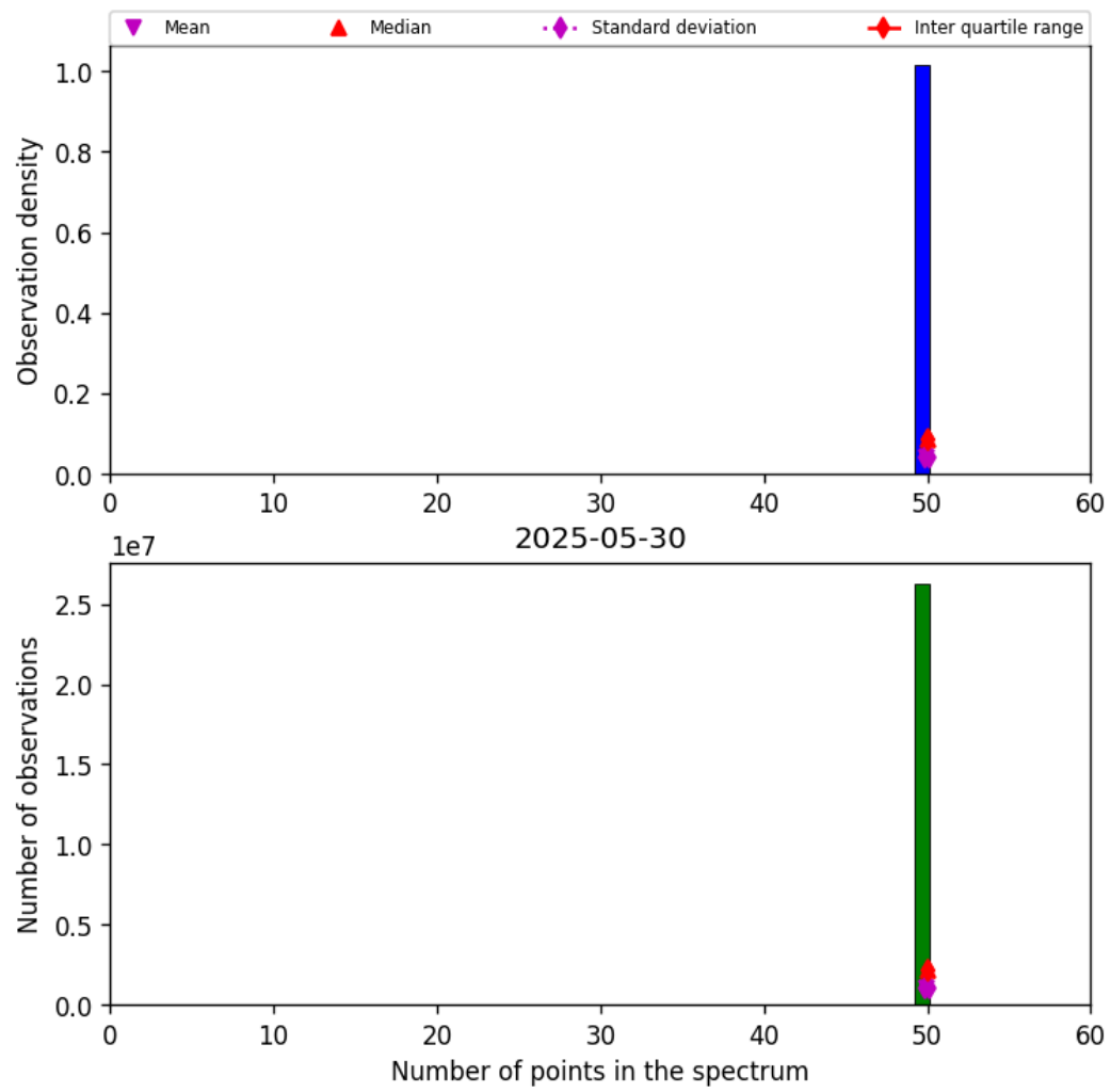
Figure 44: Histogram of “Number of points in the spectrum” for 2025-05-29 to 2025-05-31
