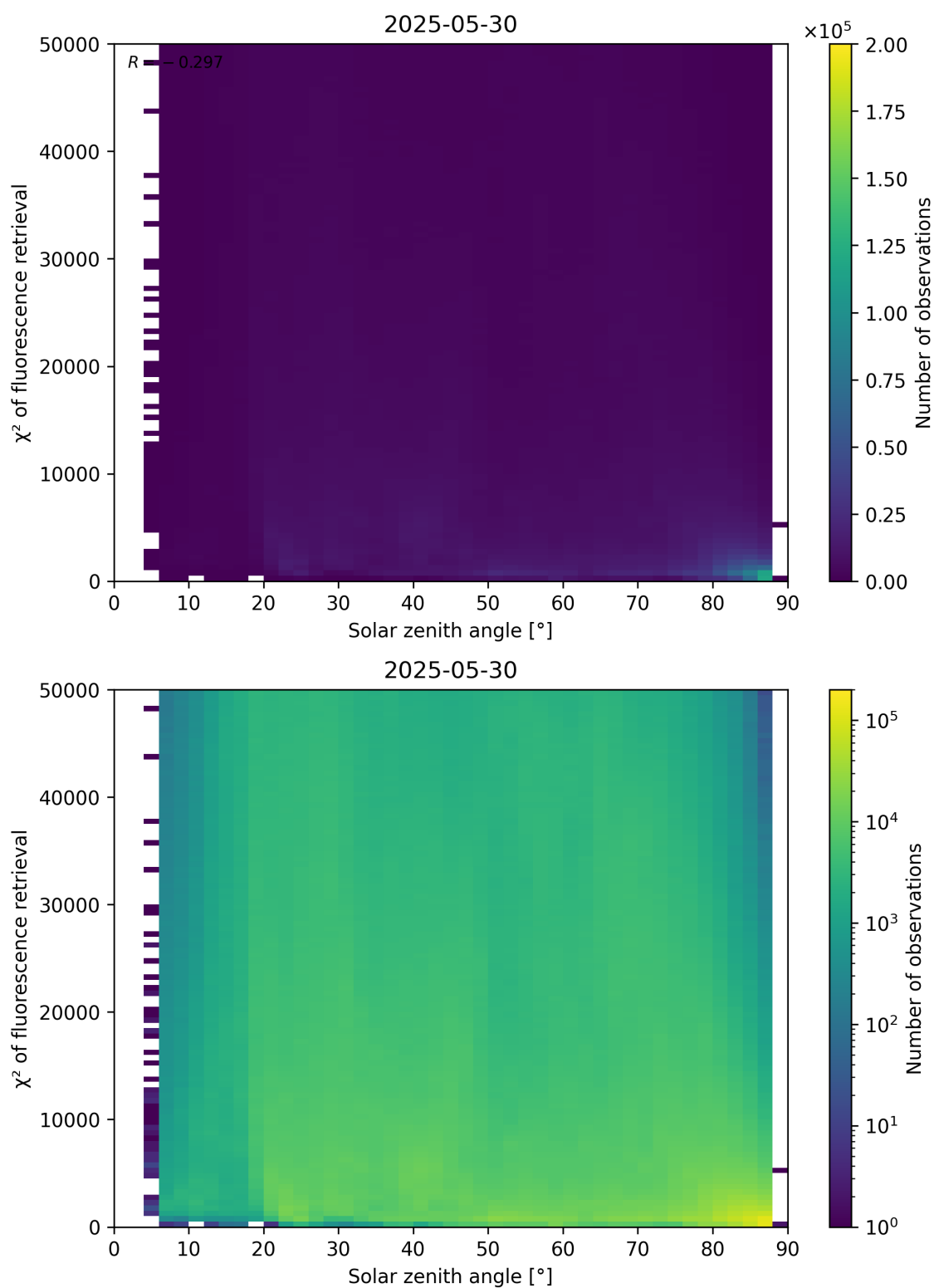
Figure 109: Scatter density plot of “Solar zenith angle” against “ \chi^2 of fluorescence retrieval” for 2025-05-29 to 2025-05-31.
