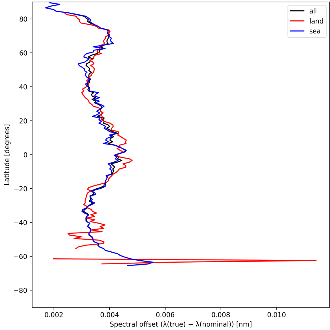
Figure 28: Zonal average of “Spectral offset ( \lambda_{\text{true}} - \lambda_{\text{nominal}} )” for 2025-05-29 to 2025-05-31.
