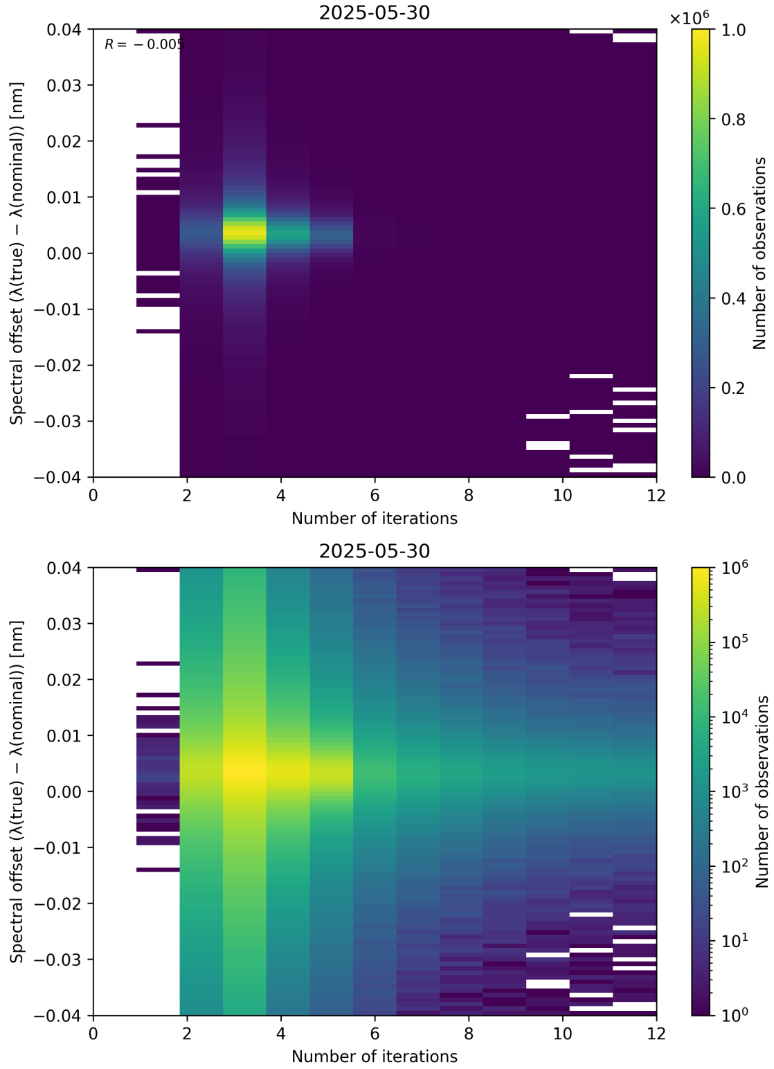
Figure 100: Scatter density plot of “Number of iterations” against “Spectral offset ( \lambda_{\text{true}} - \lambda_{\text{nominal}} )” for 2025-05-29 to 2025-05-31.
