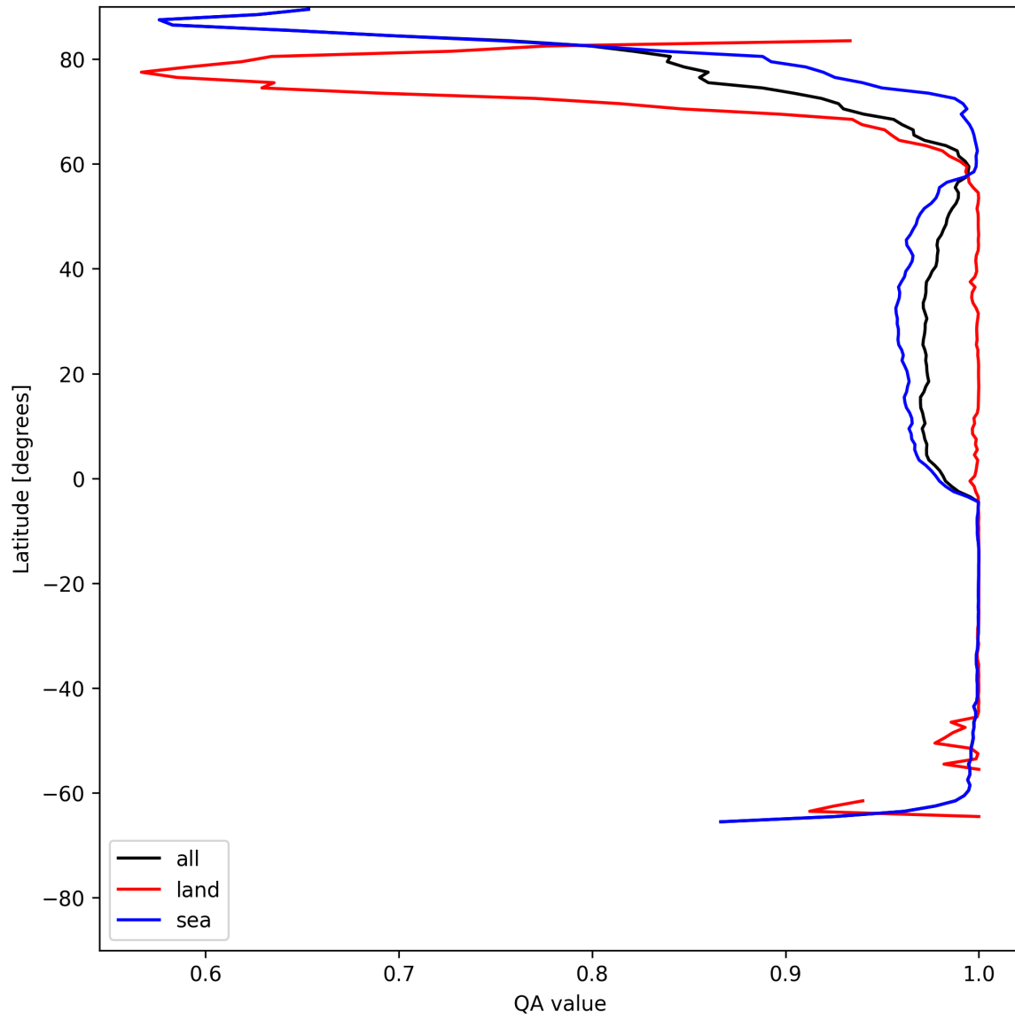
Figure 12: Zonal average of “QA value” for 2025-05-29 to 2025-05-31.
