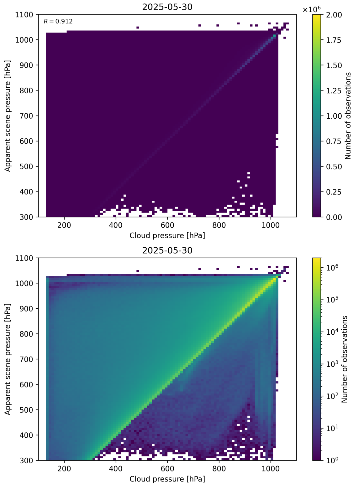
Figure 77: Scatter density plot of “Cloud pressure” against “Apparent scene pressure” for 2025-05-29 to 2025-05-31.
