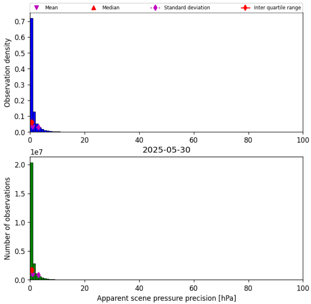
Figure 37: Histogram of “Apparent scene pressure precision” for 2025-05-29 to 2025-05-31
