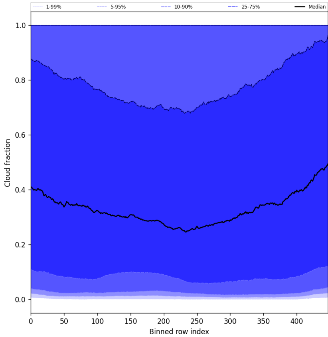
Figure 49: Along track statistics of “Cloud fraction” for 2025-05-29 to 2025-05-31
