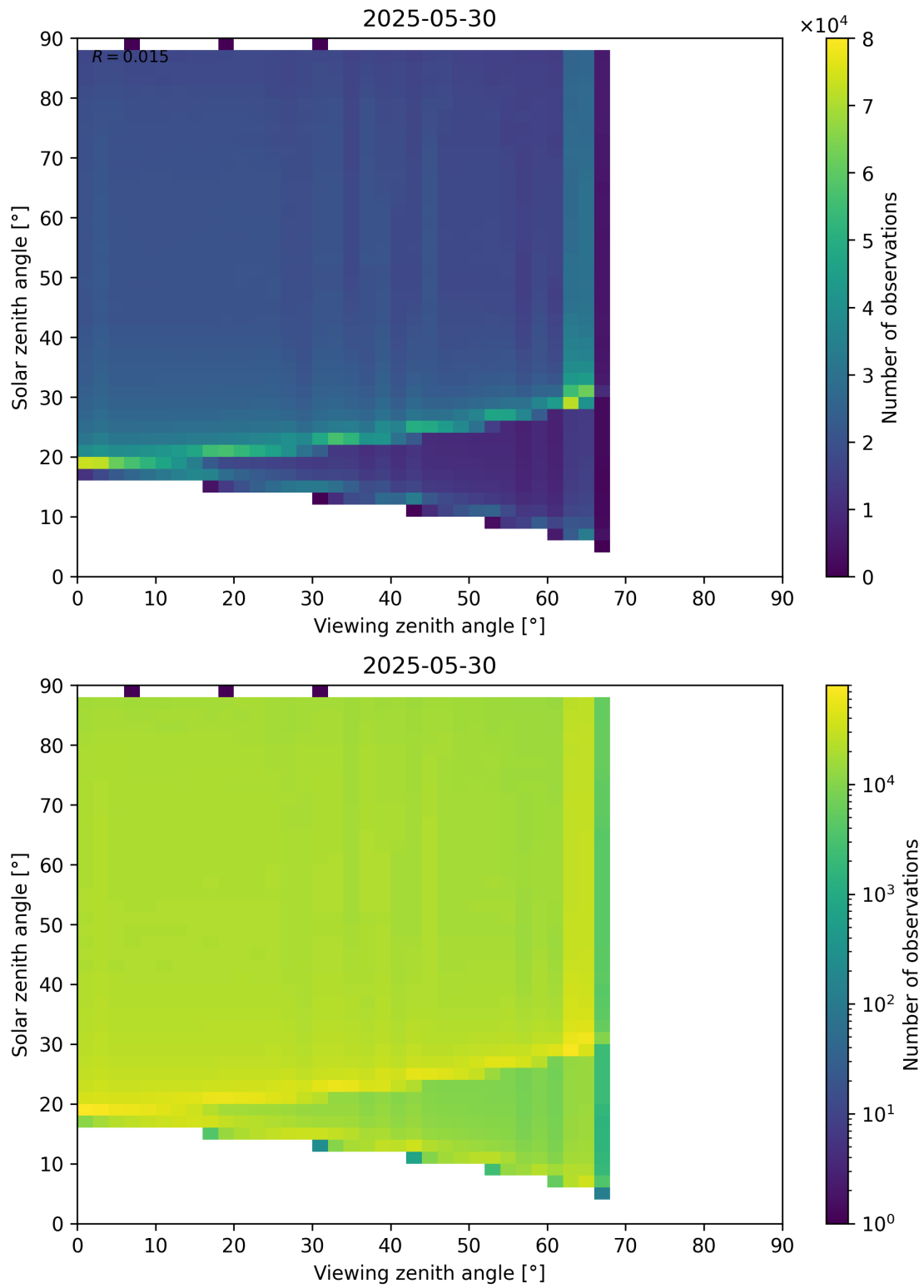
Figure 127: Scatter density plot of “Viewing zenith angle” against “Solar zenith angle” for 2025-05-29 to 2025-05-31.
