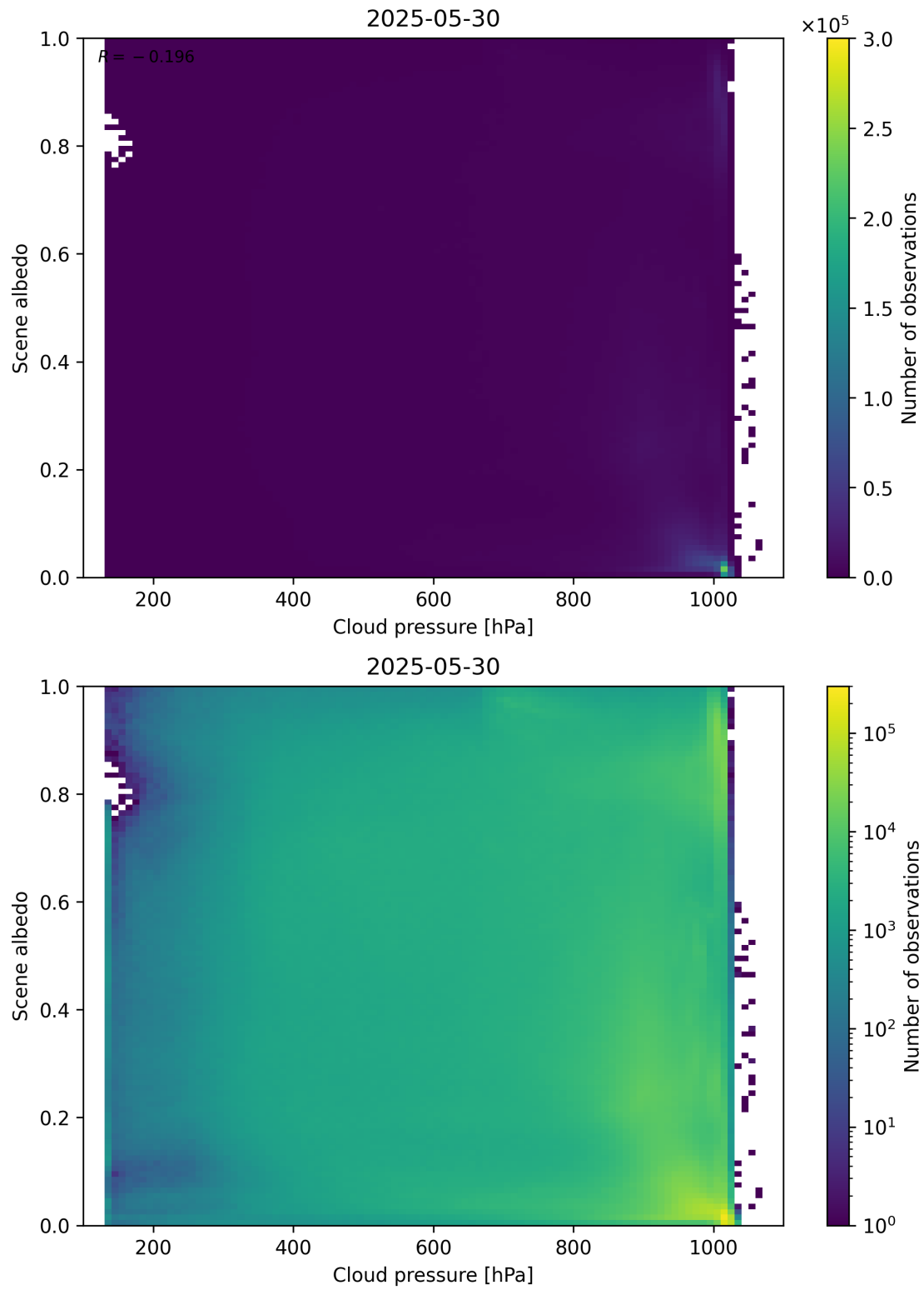
Figure 83: Scatter density plot of “Cloud pressure” against “Scene albedo” for 2025-05-29 to 2025-05-31.
