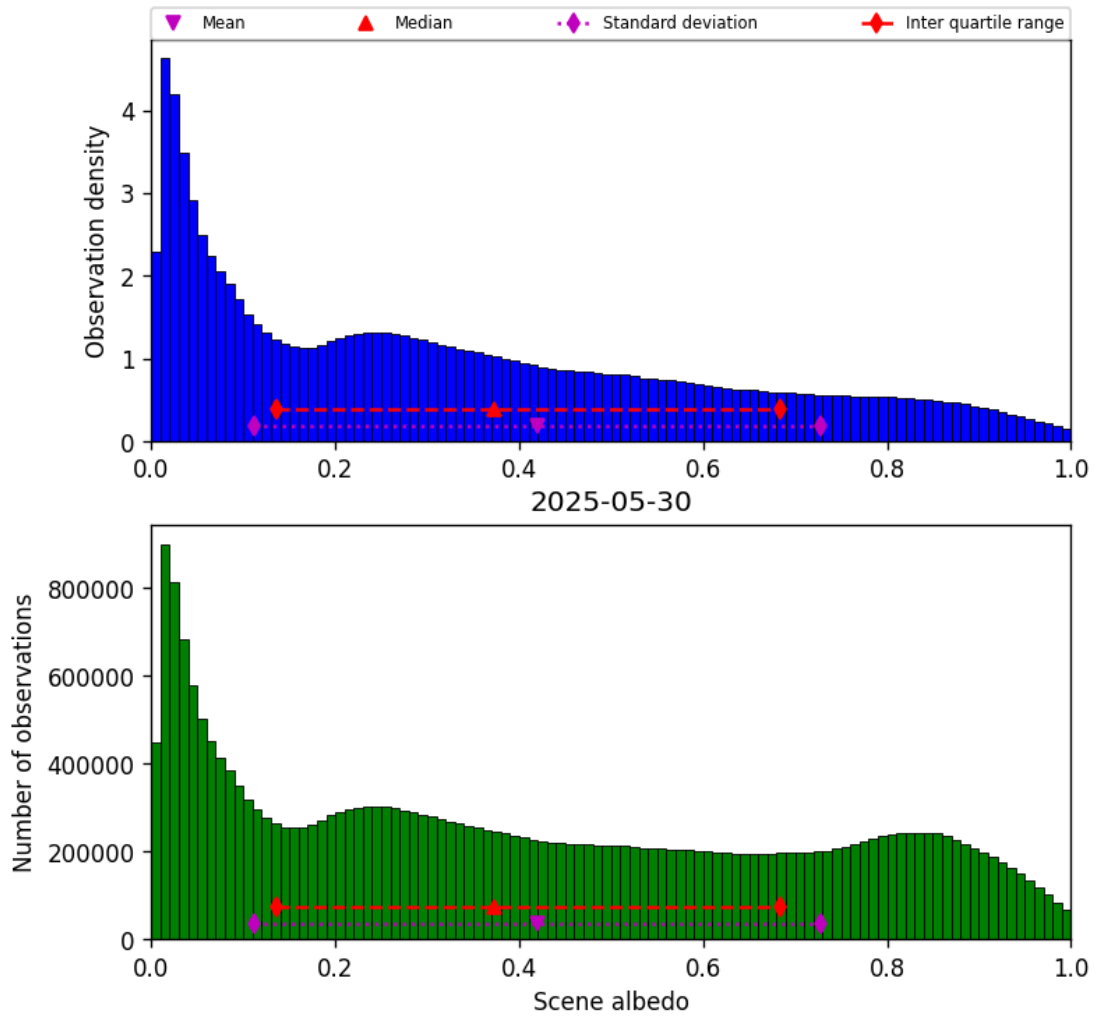
Figure 34: Histogram of “Scene albedo” for 2025-05-29 to 2025-05-31
