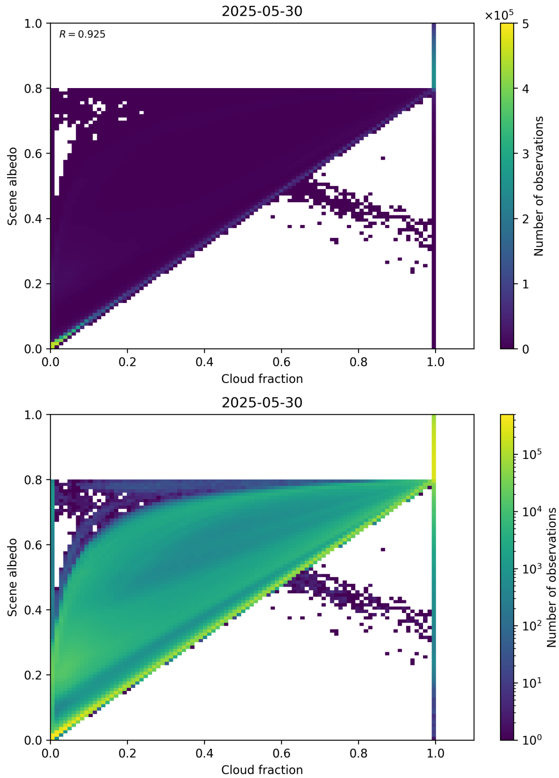
Figure 75: Scatter density plot of “Cloud fraction” against “Scene albedo” for 2025-05-29 to 2025-05-31.
