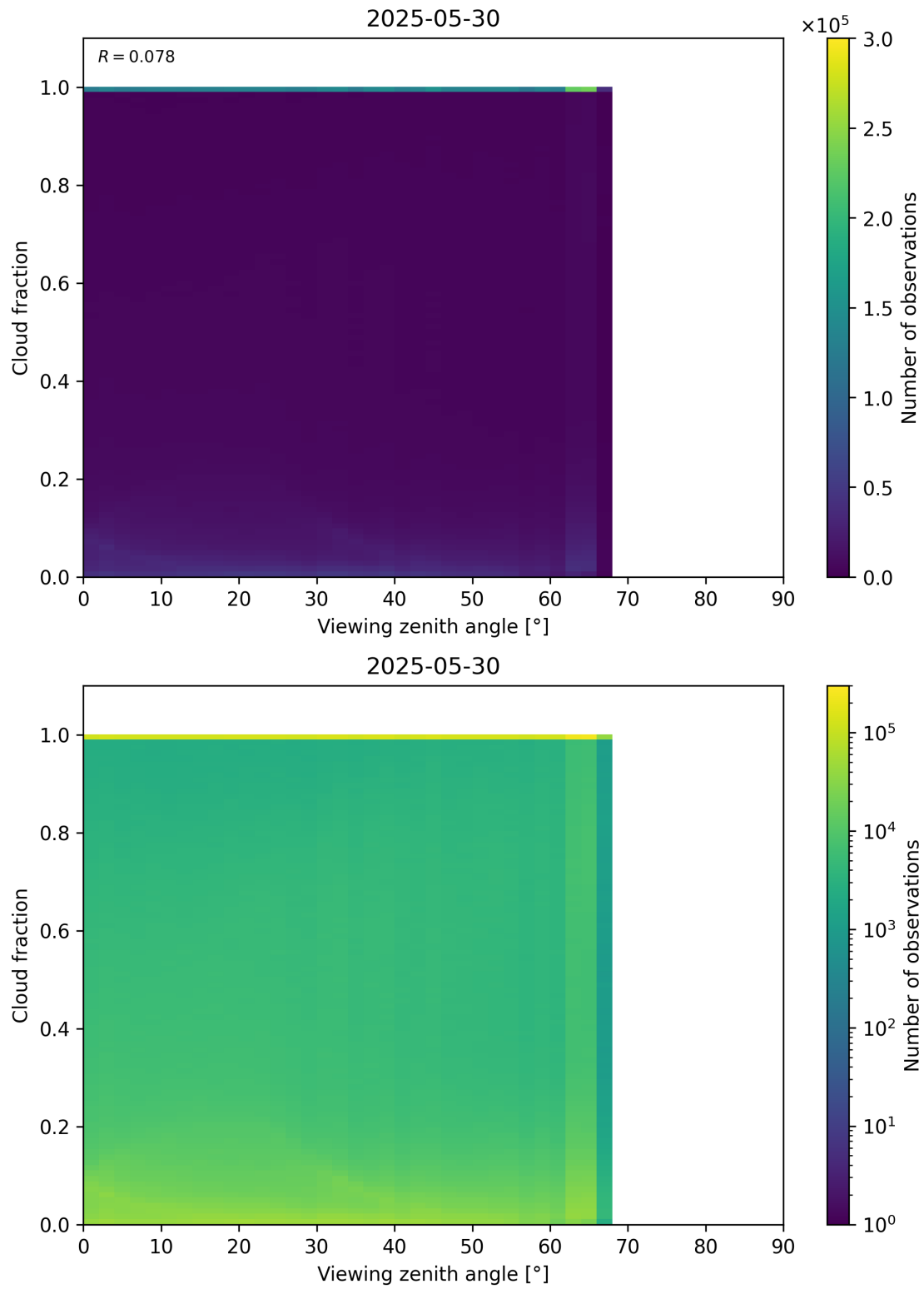
Figure 120: Scatter density plot of “Viewing zenith angle” against “Cloud fraction” for 2025-05-29 to 2025-05-31.
