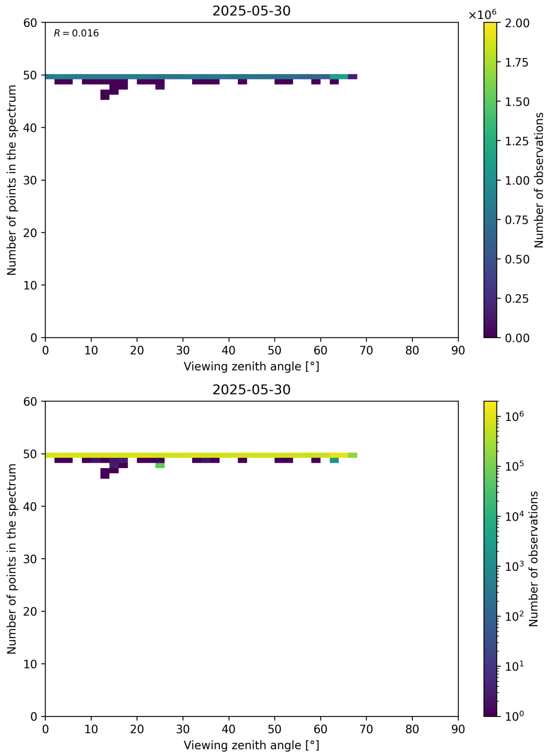
Figure 125: Scatter density plot of “Viewing zenith angle” against “Number of points in the spectrum” for 2025-05-29 to 2025-05-31.
