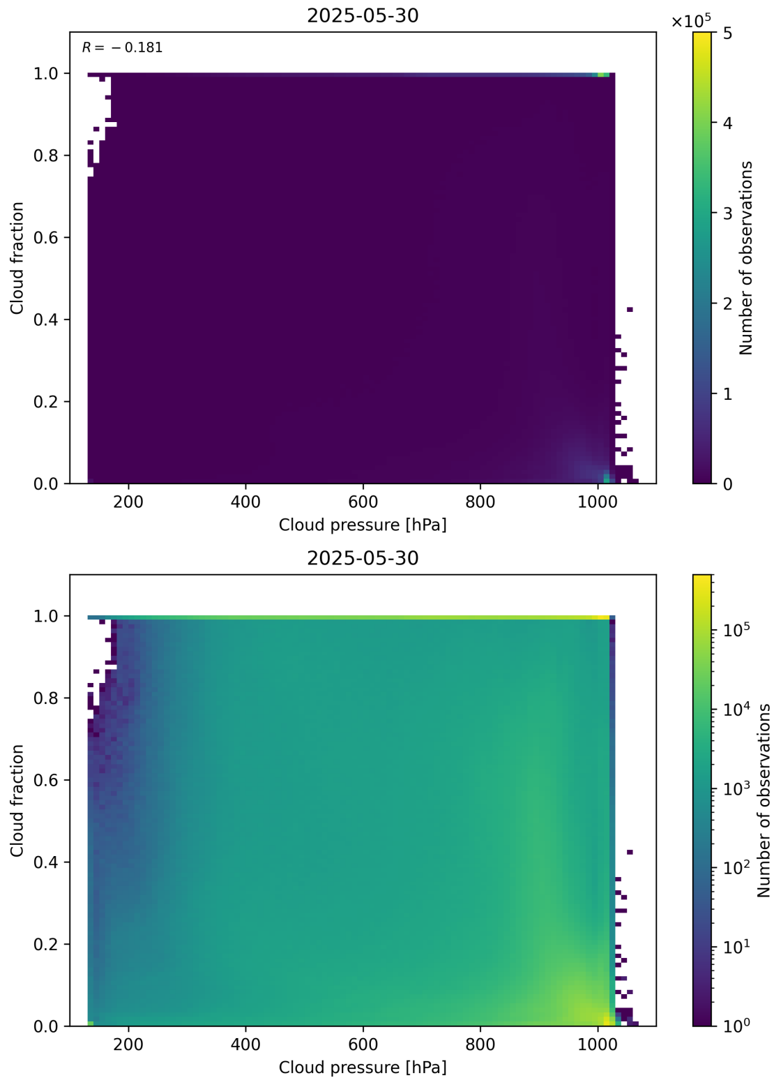
Figure 79: Scatter density plot of “Cloud pressure” against “Cloud fraction” for 2025-05-29 to 2025-05-31.
