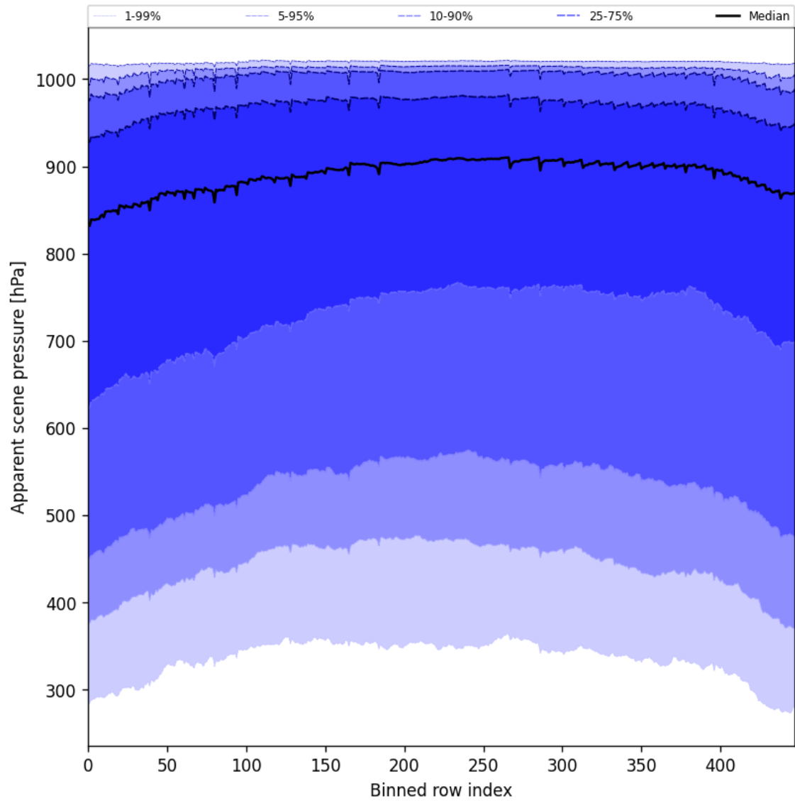
Figure 53: Along track statistics of “Apparent scene pressure” for 2025-05-29 to 2025-05-31
