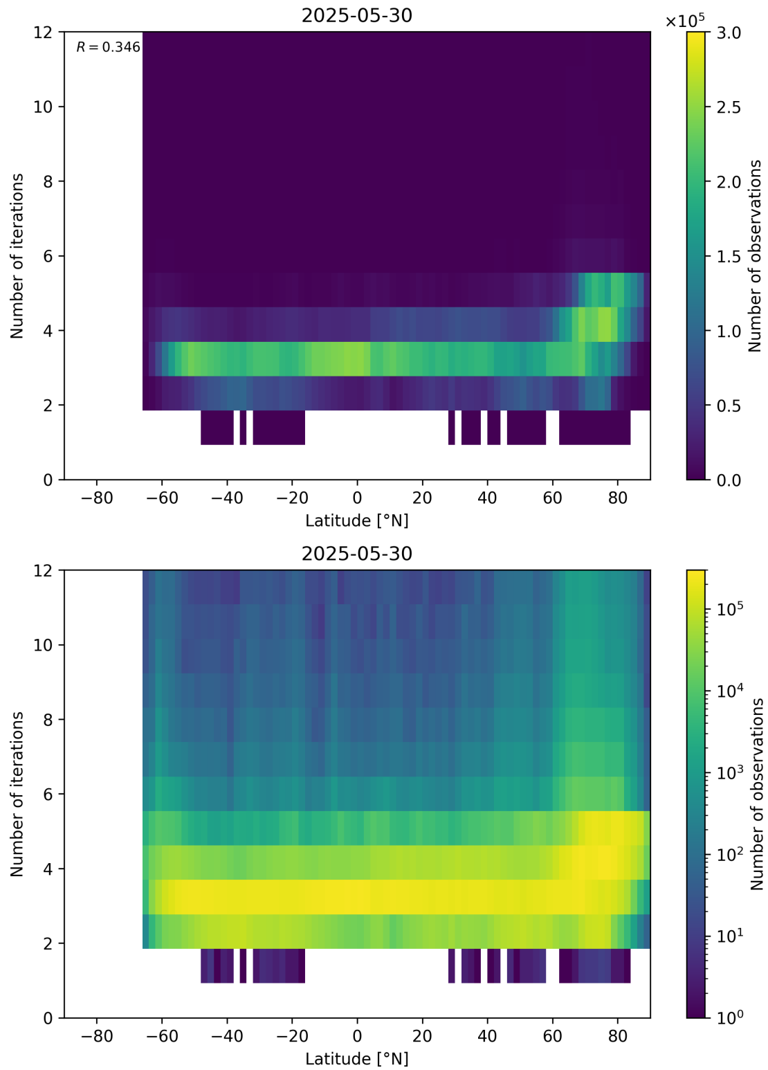
Figure 93: Scatter density plot of “Latitude” against “Number of iterations” for 2025-05-29 to 2025-05-31.
