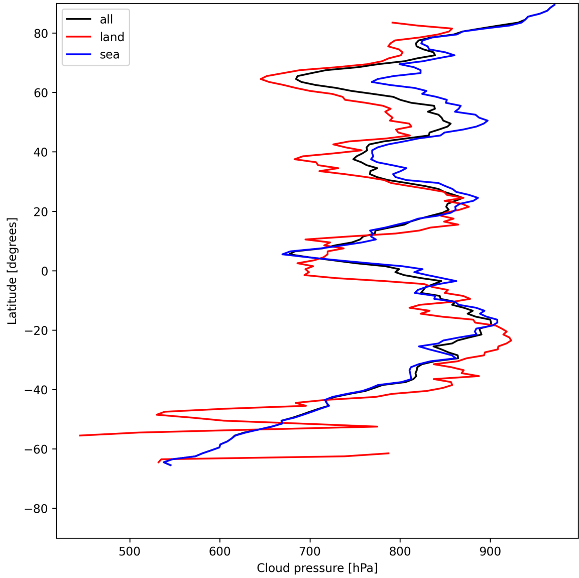
Figure 13: Zonal average of “Cloud pressure” for 2025-05-29 to 2025-05-31.
