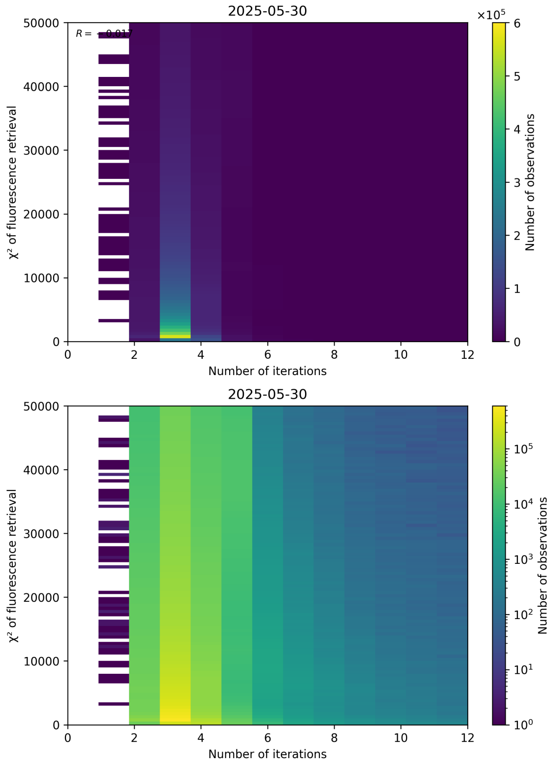
Figure 97: Scatter density plot of “Number of iterations” against “ \chi^2 of fluorescence retrieval” for 2025-05-29 to 2025-05-31.
