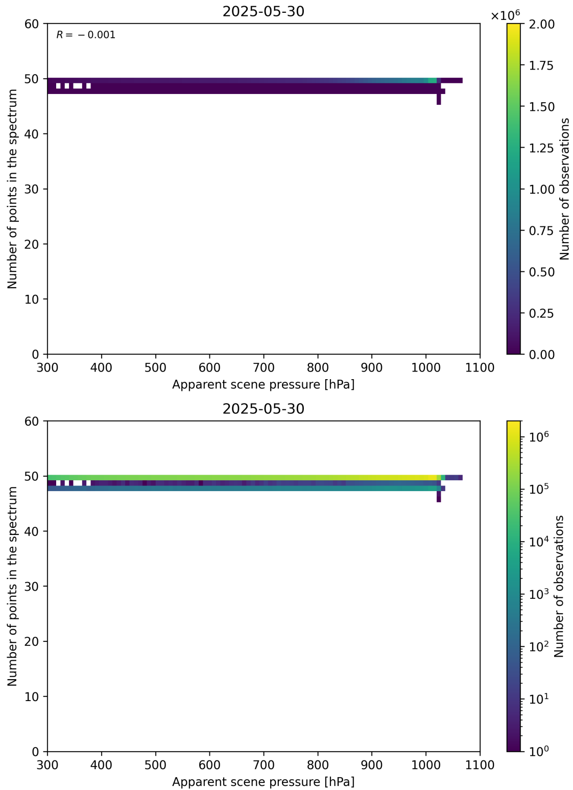
Figure 66: Scatter density plot of “Apparent scene pressure” against “Number of points in the spectrum” for 2025-05-29 to 2025-05-31.
