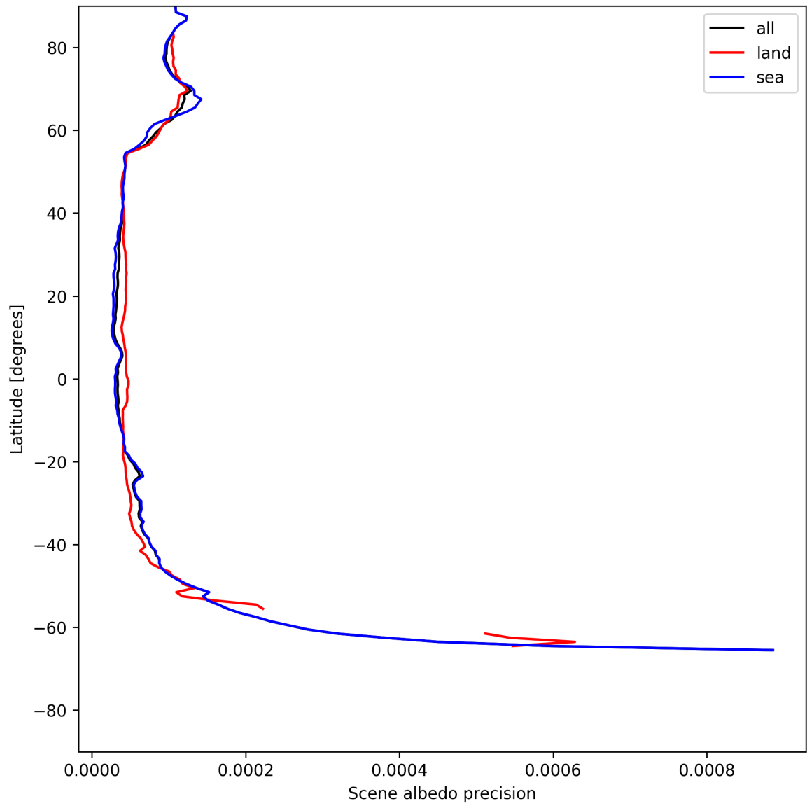
Figure 18: Zonal average of “Scene albedo precision” for 2025-05-29 to 2025-05-31.
