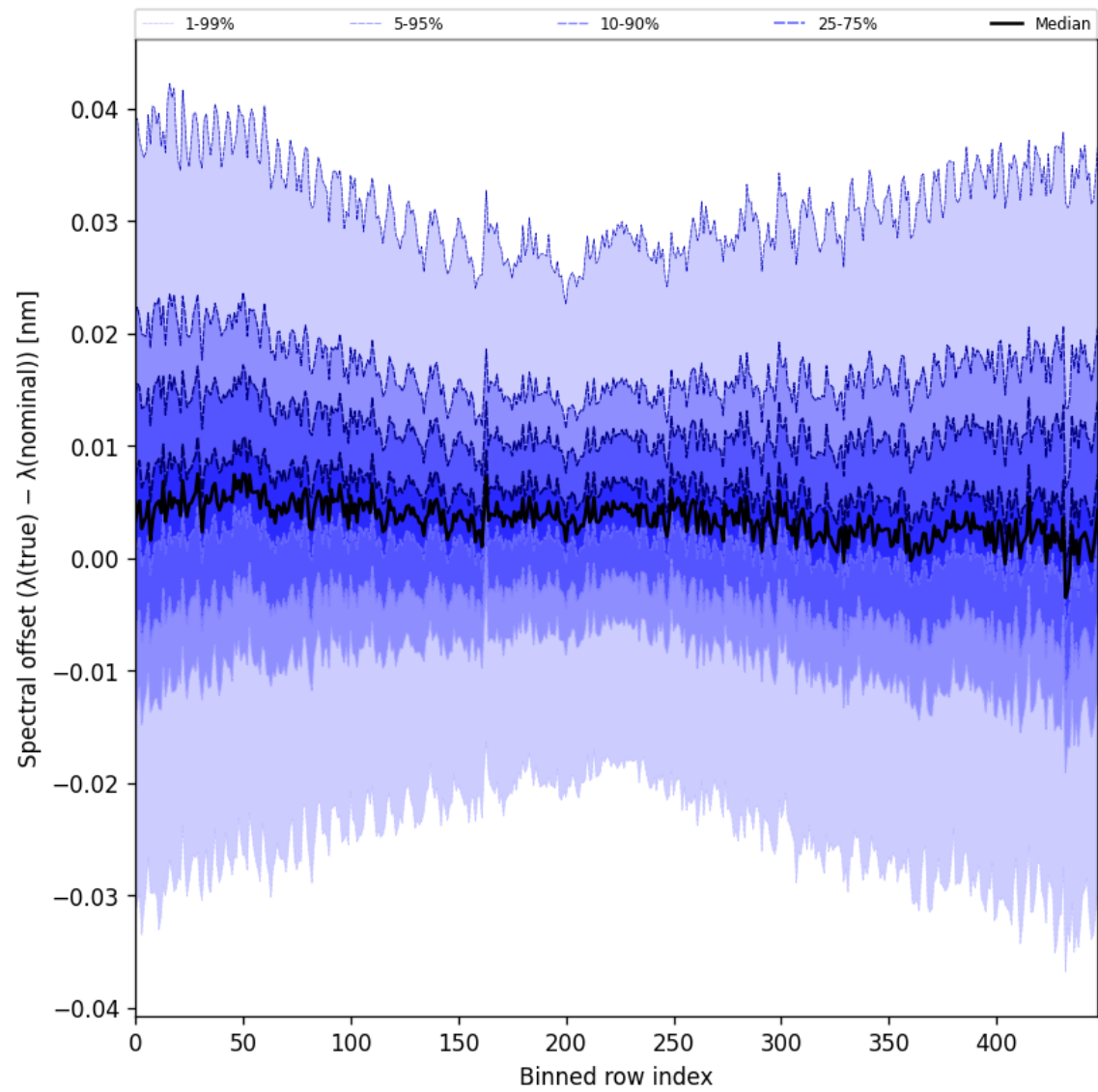
Figure 62: Along track statistics of “Spectral offset ( \lambda_{\text{true}} - \lambda_{\text{nominal}} )” for 2025-05-29 to 2025-05-31
