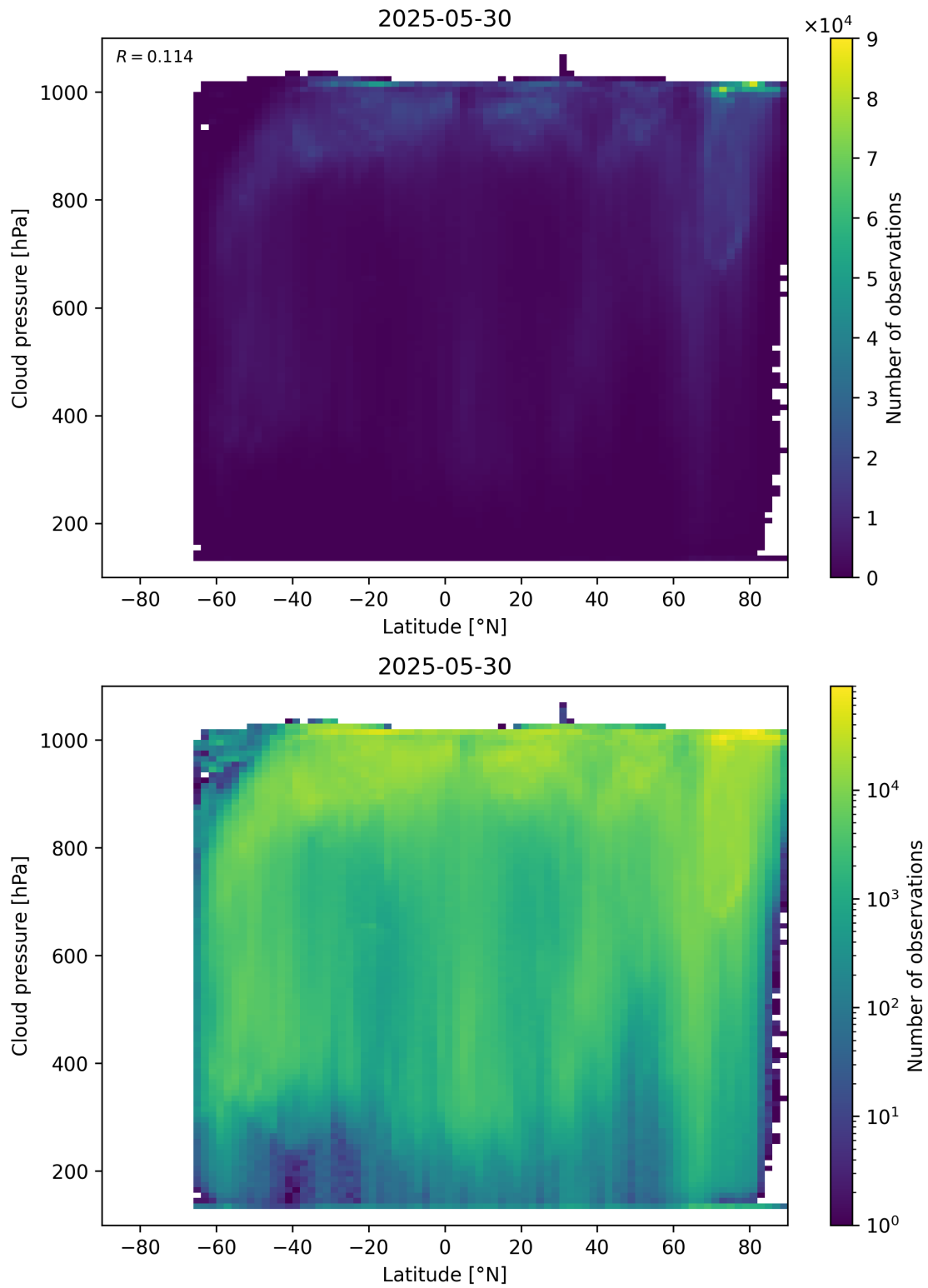
Figure 91: Scatter density plot of “Latitude” against “Cloud pressure” for 2025-05-29 to 2025-05-31.
