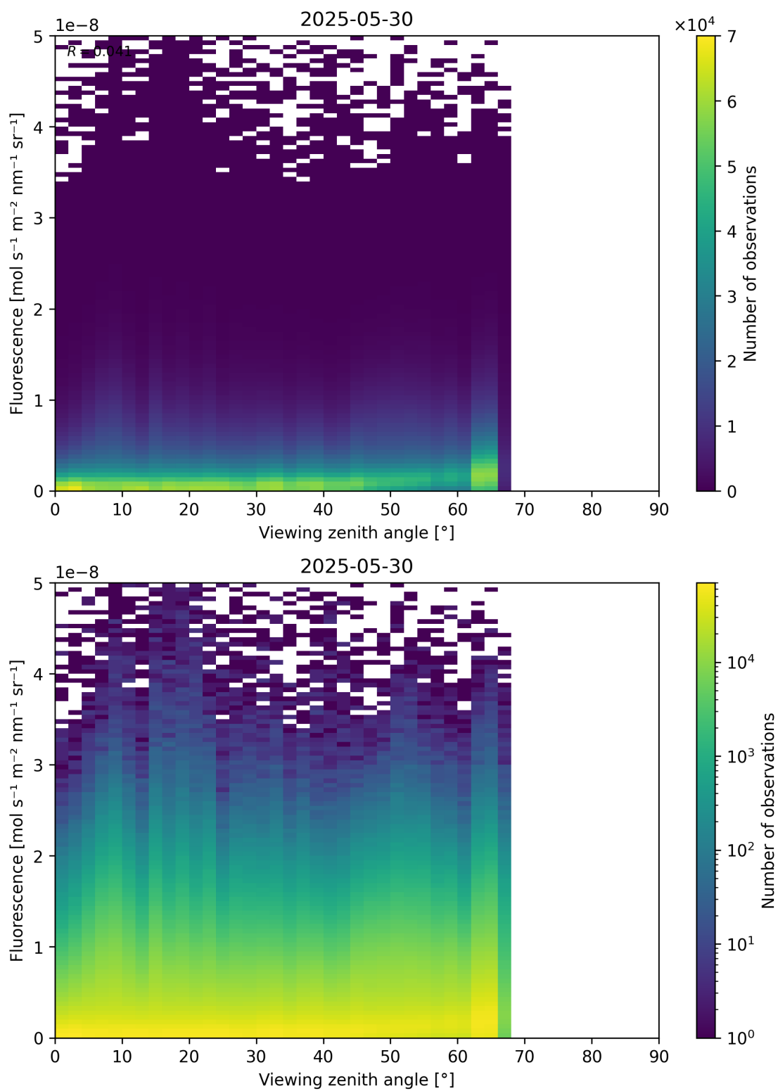
Figure 122: Scatter density plot of “Viewing zenith angle” against “Fluorescence” for 2025-05-29 to 2025-05-31.
