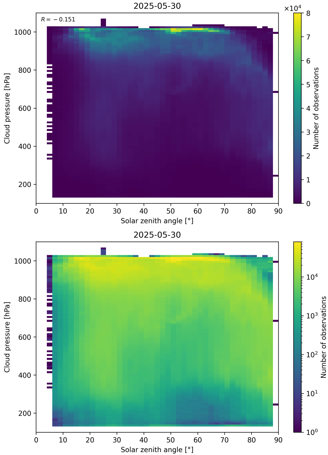
Figure 111: Scatter density plot of “Solar zenith angle” against “Cloud pressure” for 2025-05-29 to 2025-05-31.
