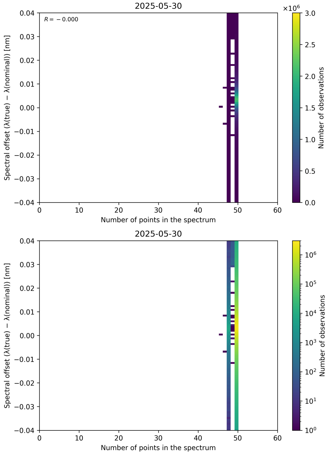
Figure 101: Scatter density plot of “Number of points in the spectrum” against “Spectral offset ( \lambda_{\text{true}} - \lambda_{\text{nominal}} )” for 2025-05-29 to 2025-05-31.
