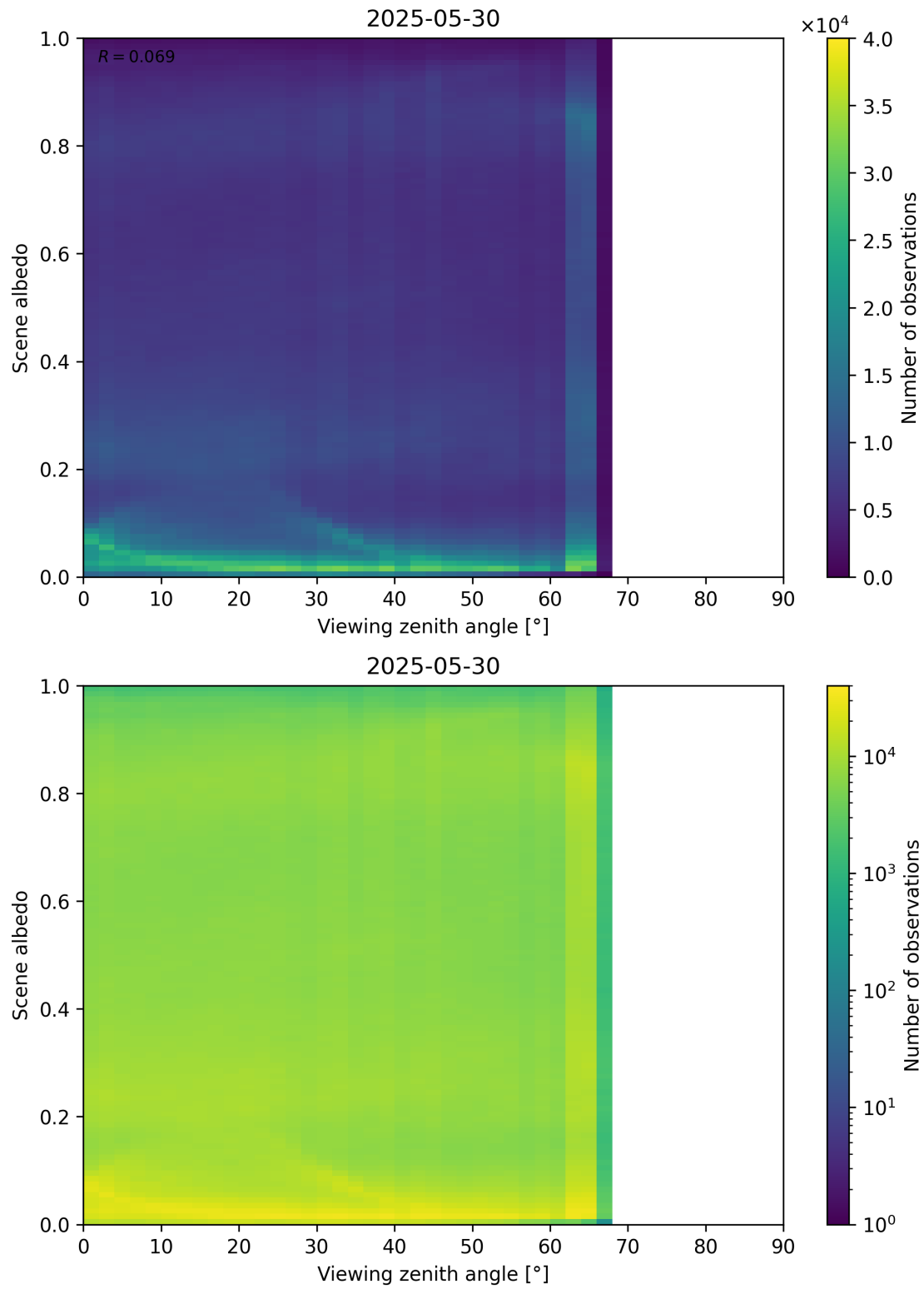
Figure 126: Scatter density plot of “Viewing zenith angle” against “Scene albedo” for 2025-05-29 to 2025-05-31.
