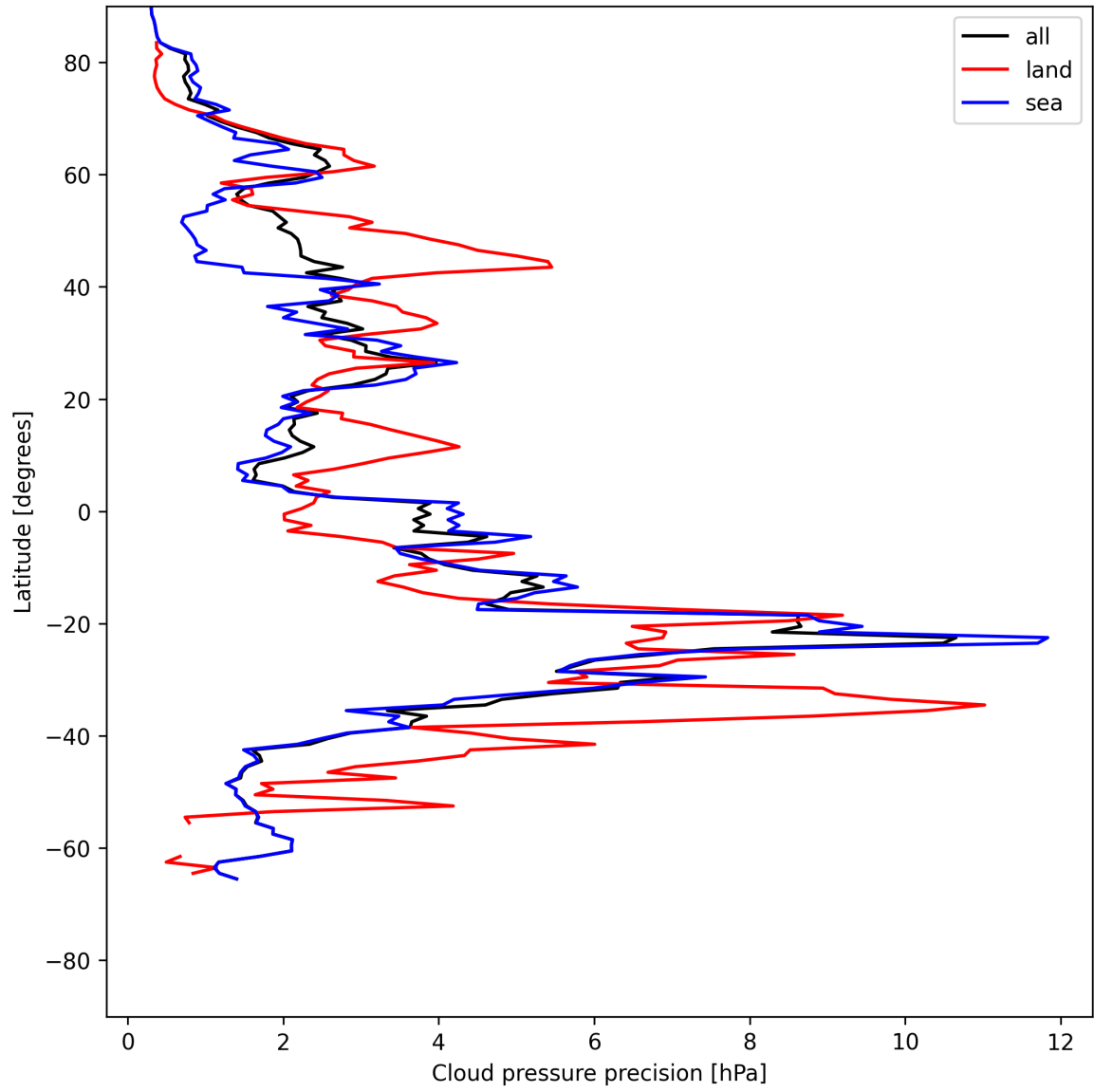
Figure 14: Zonal average of “Cloud pressure precision” for 2025-05-29 to 2025-05-31.
