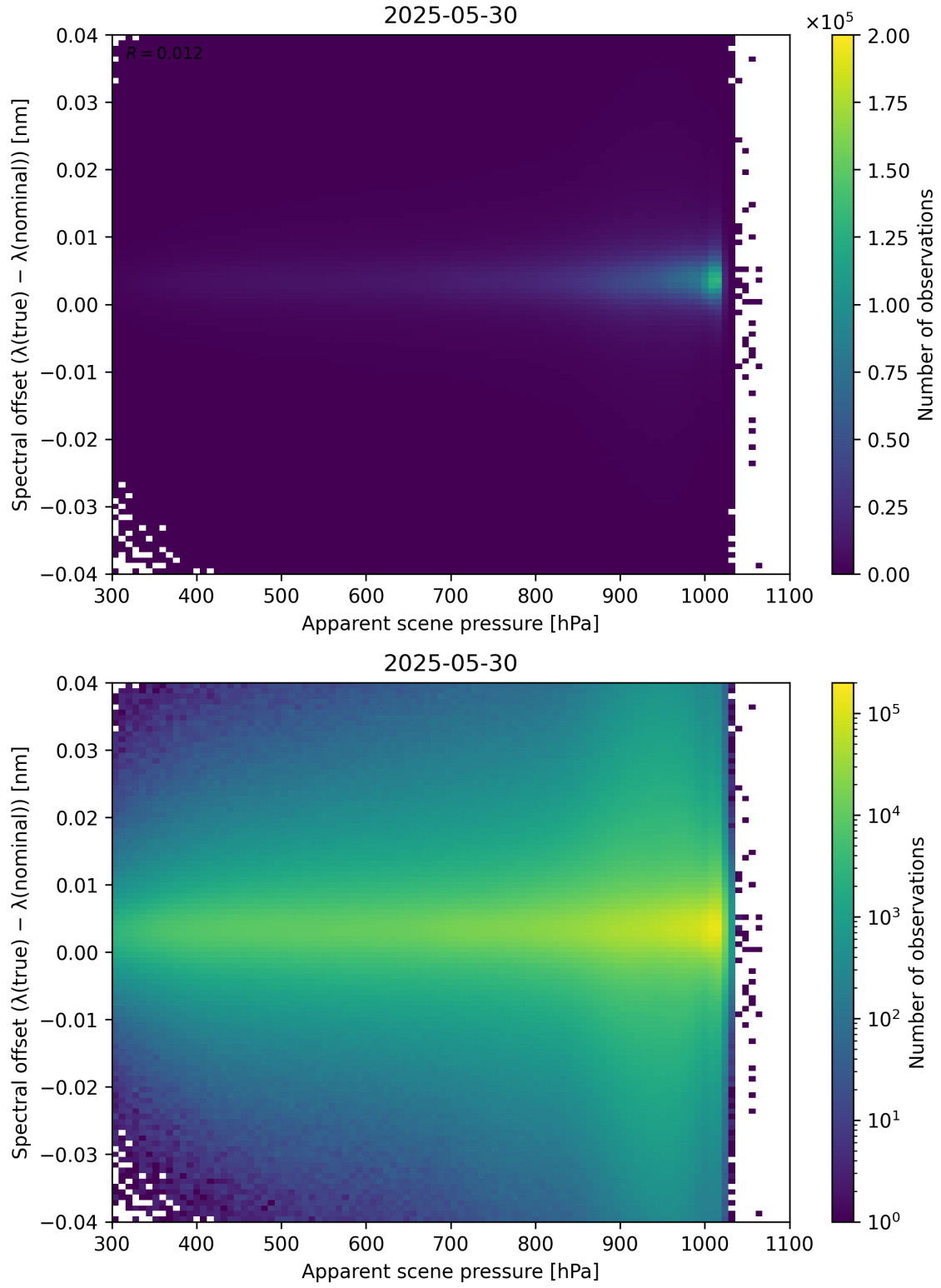
Figure 67: Scatter density plot of “Apparent scene pressure” against “Spectral offset ( \lambda_{\text{true}} - \lambda_{\text{nominal}} )” for 2025-05-29 to 2025-05-31.
