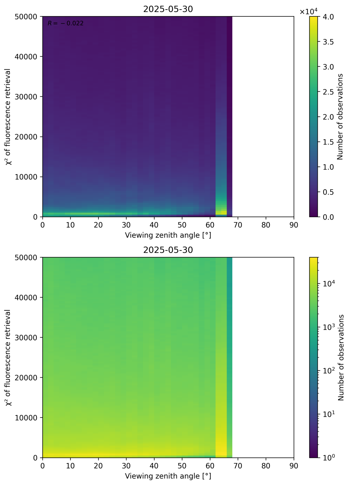
Figure 119: Scatter density plot of “Viewing zenith angle” against “ \chi^2 of fluorescence retrieval” for 2025-05-29 to 2025-05-31.
