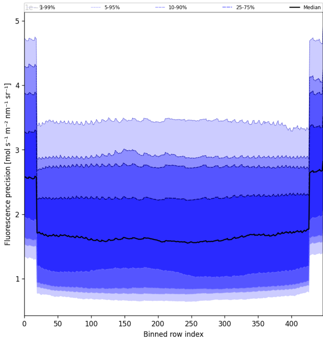
Figure 58: Along track statistics of “Fluorescence precision” for 2025-05-29 to 2025-05-31
