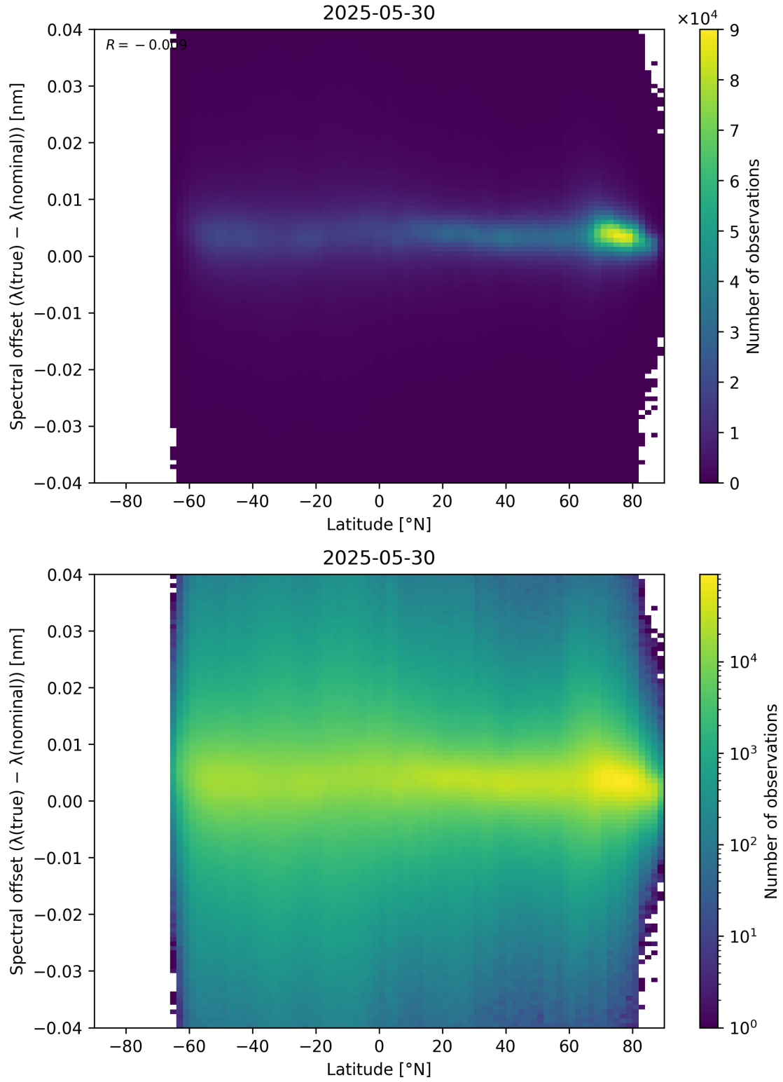
Figure 96: Scatter density plot of “Latitude” against “Spectral offset ( \lambda_{\text{true}} - \lambda_{\text{nominal}} )” for 2025-05-29 to 2025-05-31.
