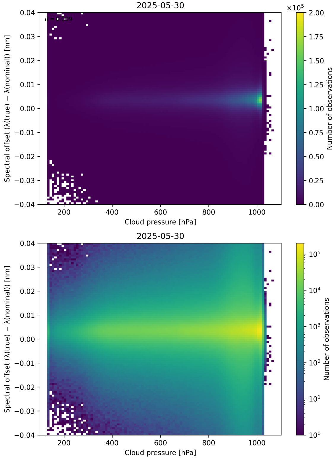
Figure 84: Scatter density plot of “Cloud pressure” against “Spectral offset ( \lambda_{\text{true}} - \lambda_{\text{nominal}} )” for 2025-05-29 to 2025-05-31.
