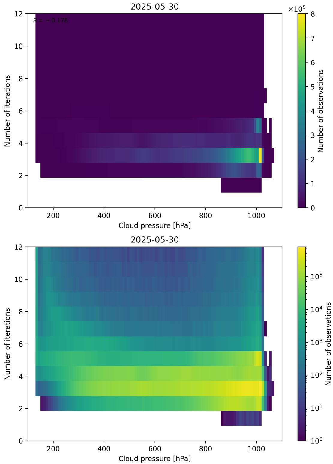
Figure 81: Scatter density plot of “Cloud pressure” against “Number of iterations” for 2025-05-29 to 2025-05-31.
