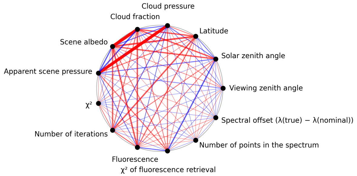
Figure 1: Map of correlation graph for 2025-05-29 to 2025-05-31.
