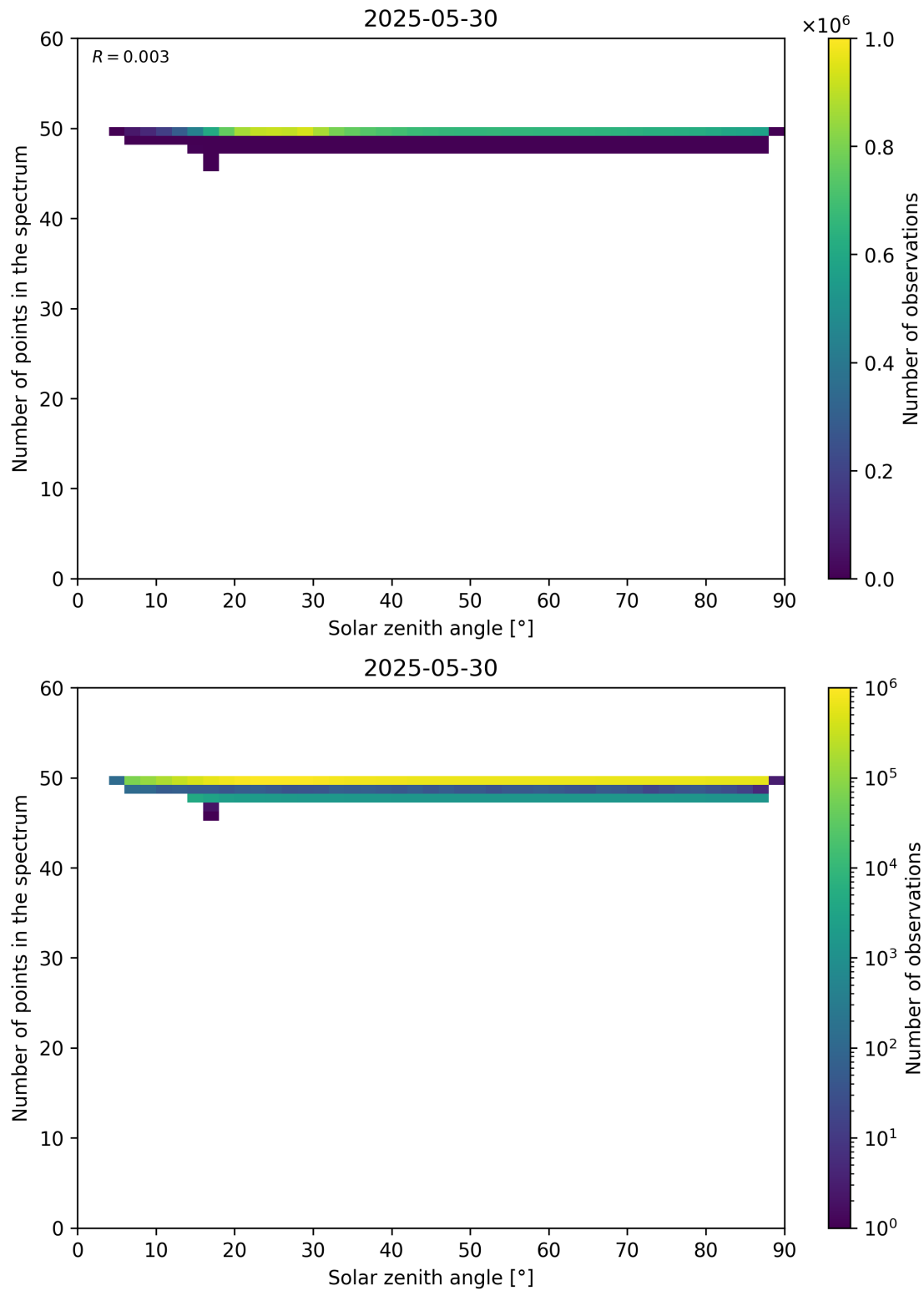
Figure 115: Scatter density plot of “Solar zenith angle” against “Number of points in the spectrum” for 2025-05-29 to 2025-05-31.
