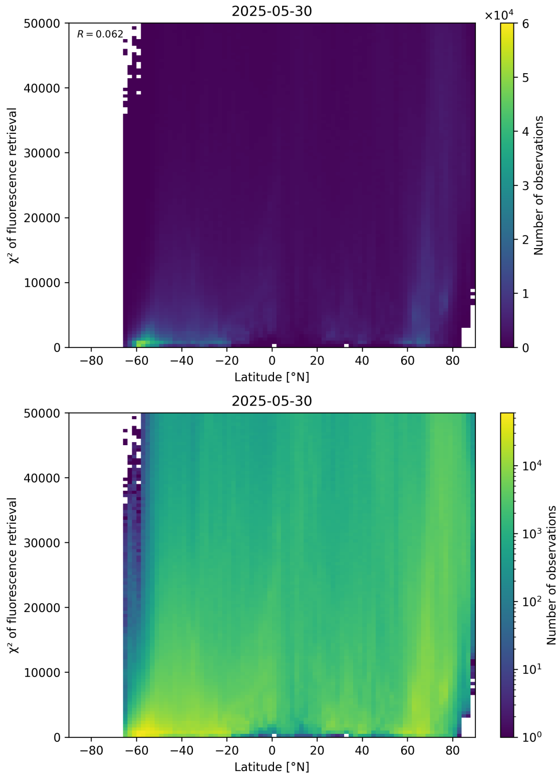
Figure 89: Scatter density plot of “Latitude” against “ \chi^2 of fluorescence retrieval” for 2025-05-29 to 2025-05-31.
