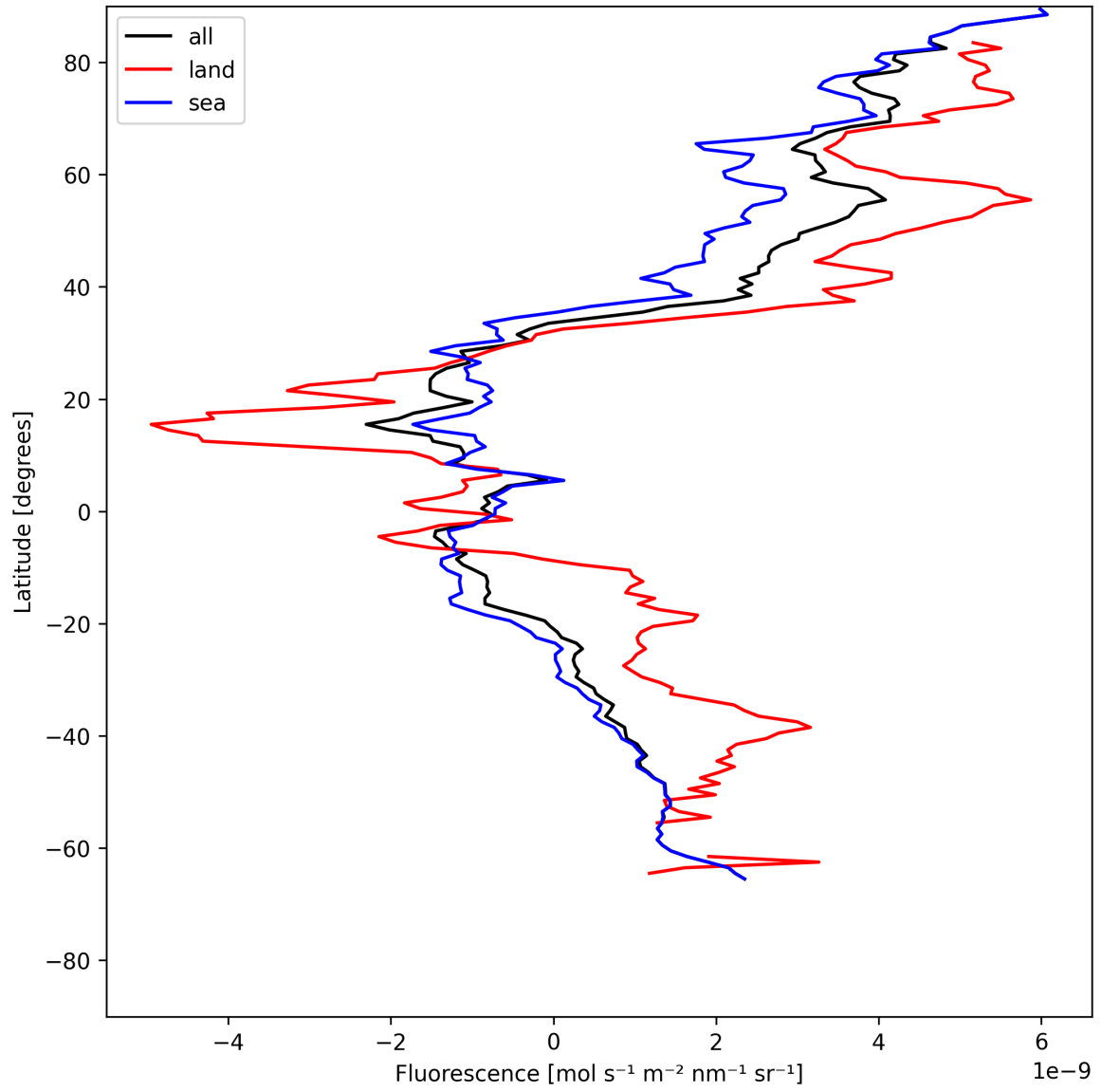
Figure 23: Zonal average of “Fluorescence” for 2025-05-29 to 2025-05-31.
