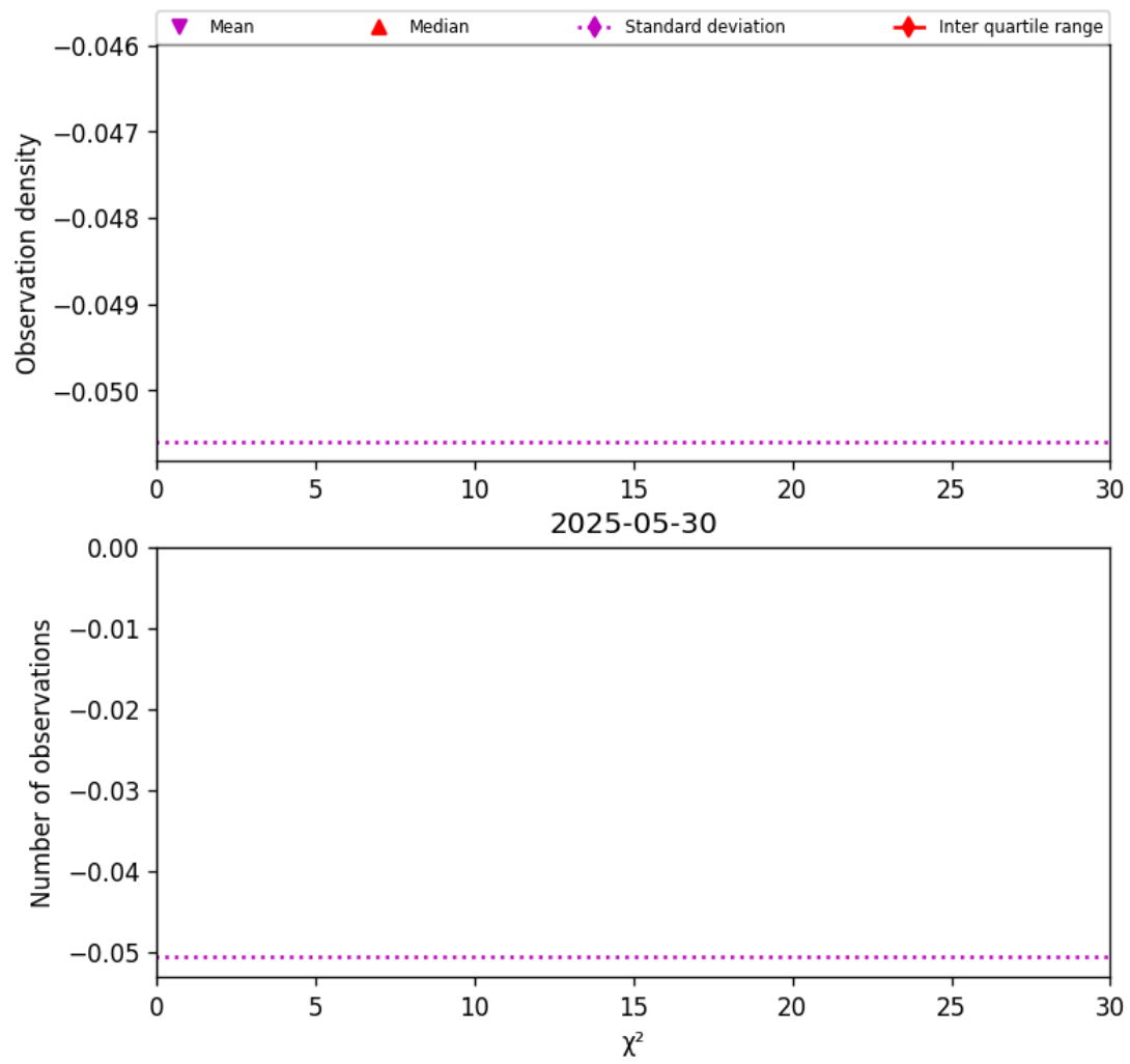
Figure 38: Histogram of “ \chi^2 ” for 2025-05-29 to 2025-05-31
