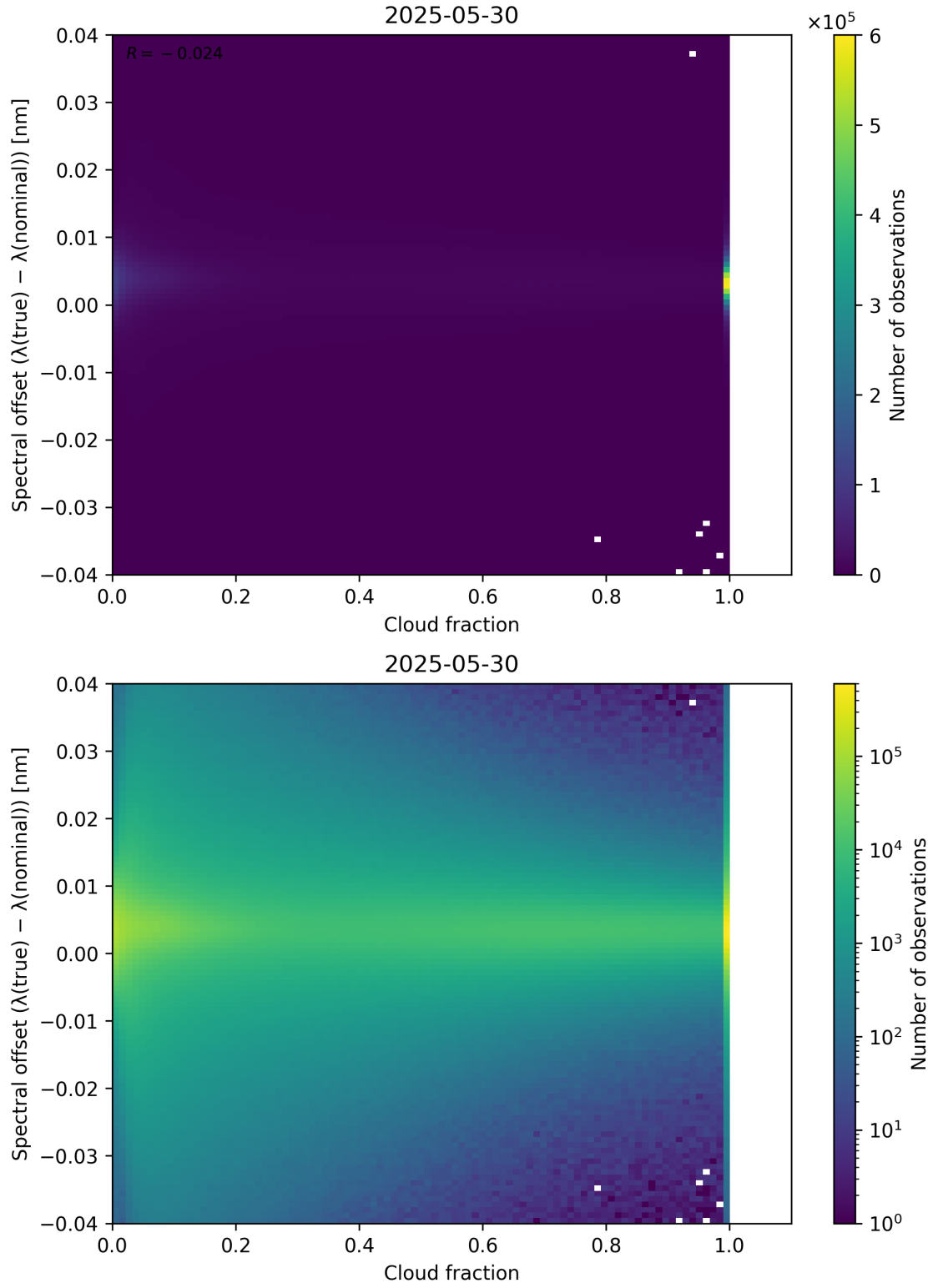
Figure 76: Scatter density plot of “Cloud fraction” against “Spectral offset ( \lambda_{\text{true}} - \lambda_{\text{nominal}} )” for 2025-05-29 to 2025-05-31.
