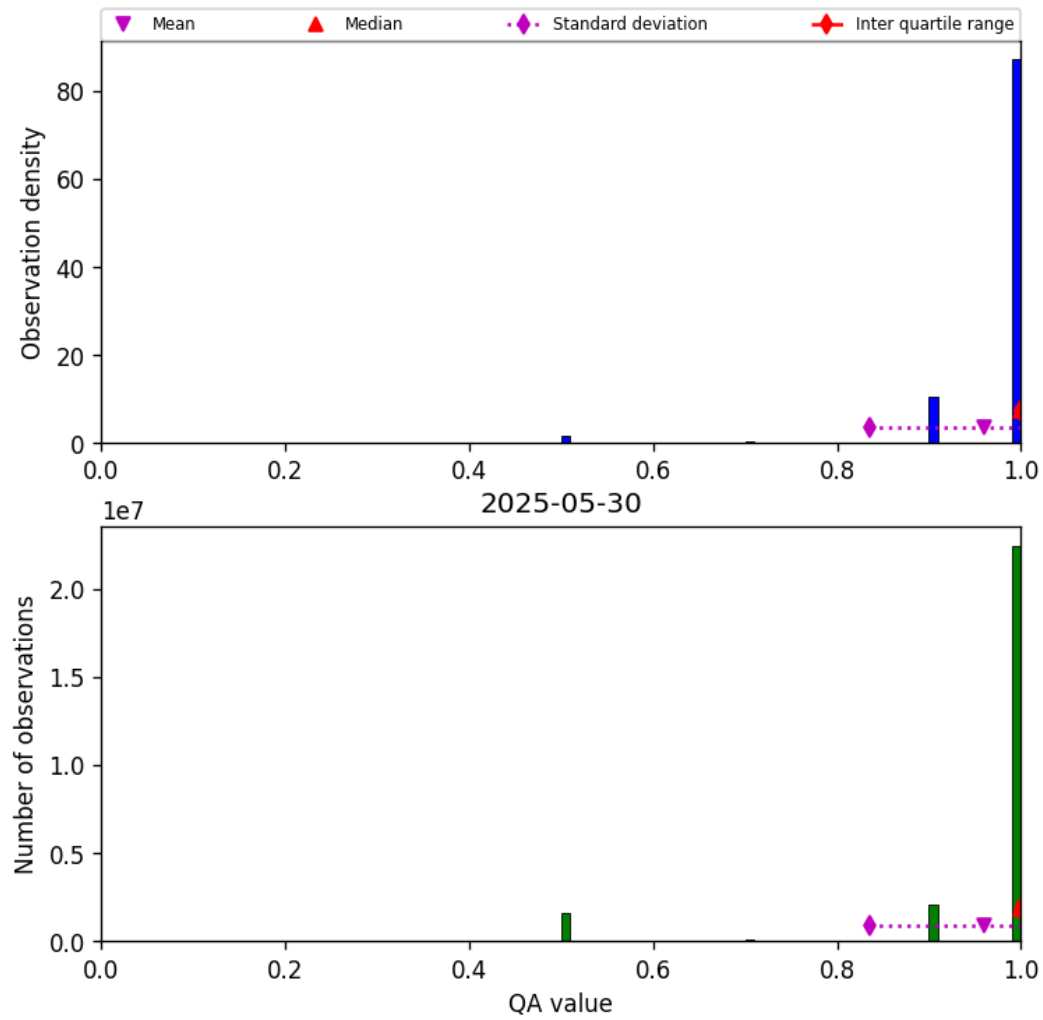
Figure 29: Histogram of “QA value” for 2025-05-29 to 2025-05-31
