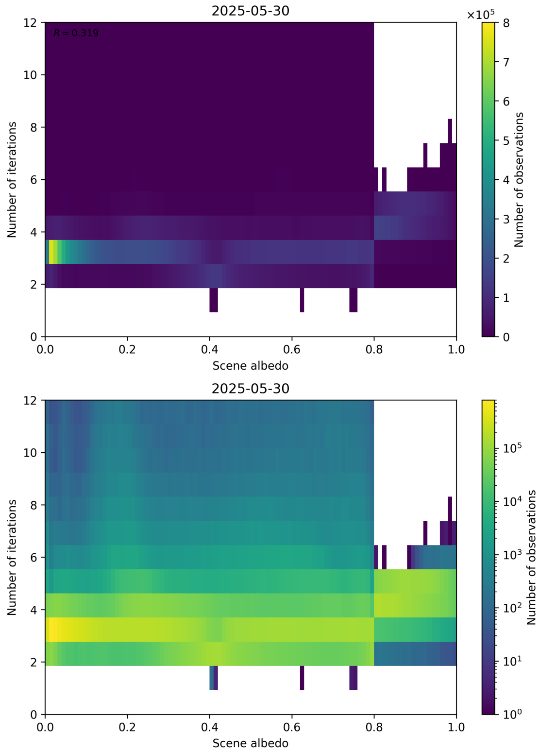
Figure 105: Scatter density plot of “Scene albedo” against “Number of iterations” for 2025-05-29 to 2025-05-31.
