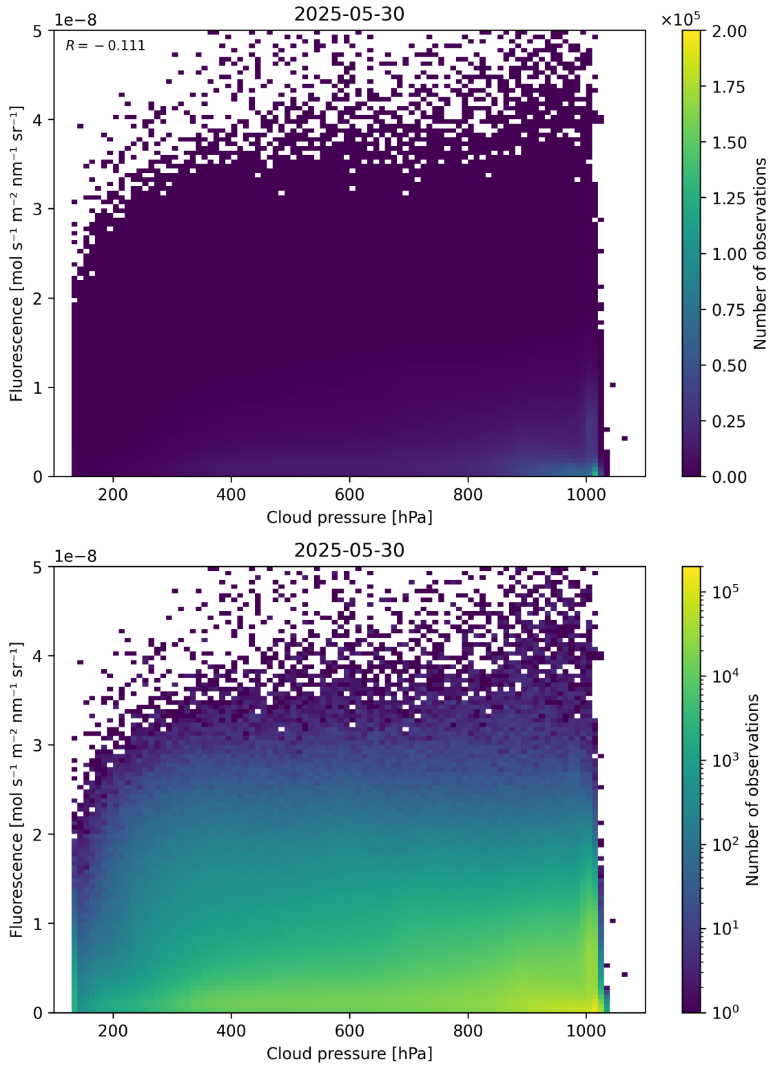
Figure 80: Scatter density plot of “Cloud pressure” against “Fluorescence” for 2025-05-29 to 2025-05-31.
