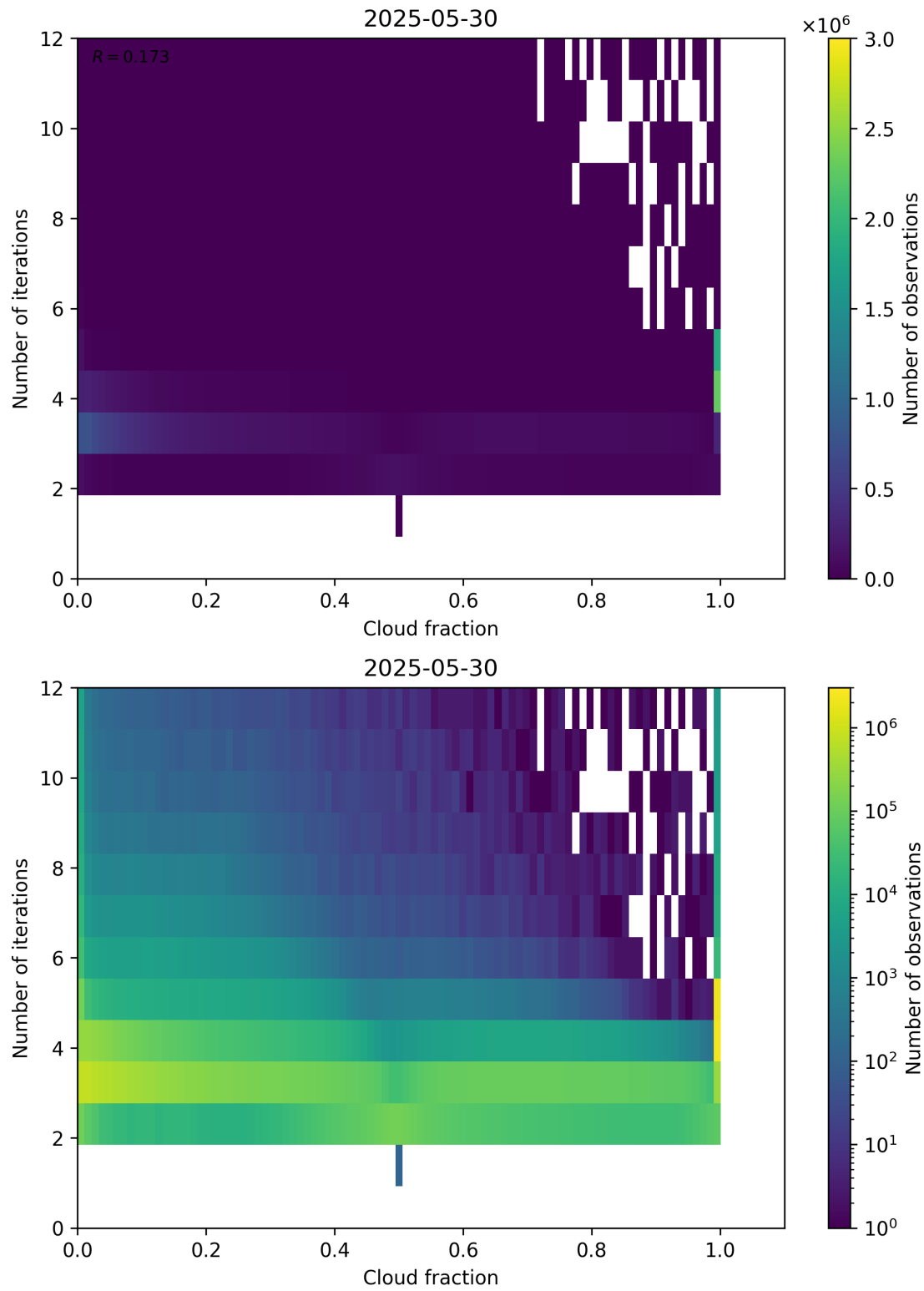
Figure 73: Scatter density plot of “Cloud fraction” against “Number of iterations” for 2025-05-29 to 2025-05-31.
