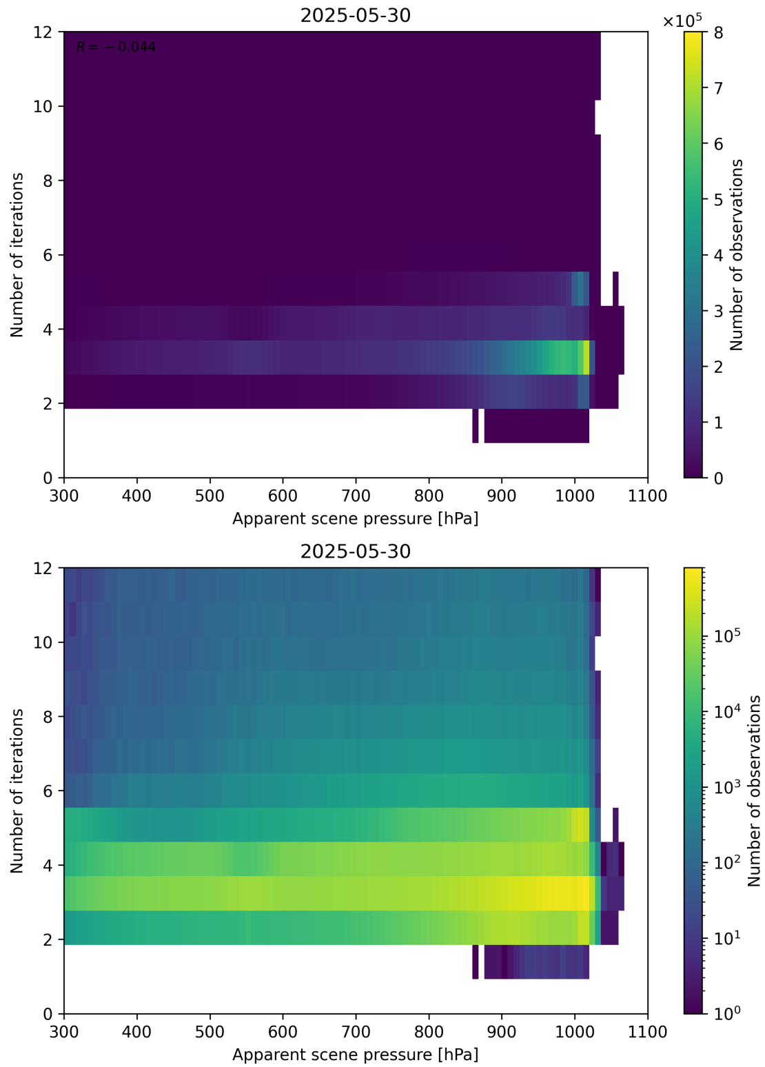
Figure 65: Scatter density plot of “Apparent scene pressure” against “Number of iterations” for 2025-05-29 to 2025-05-31.
