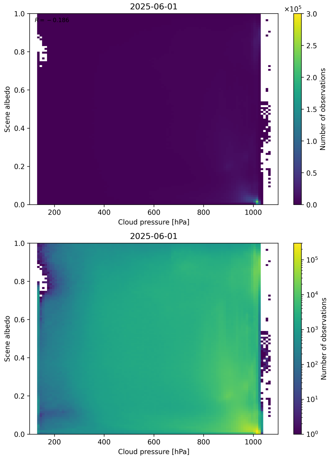
Figure 83: Scatter density plot of “Cloud pressure” against “Scene albedo” for 2025-06-01 to 2025-06-02.
