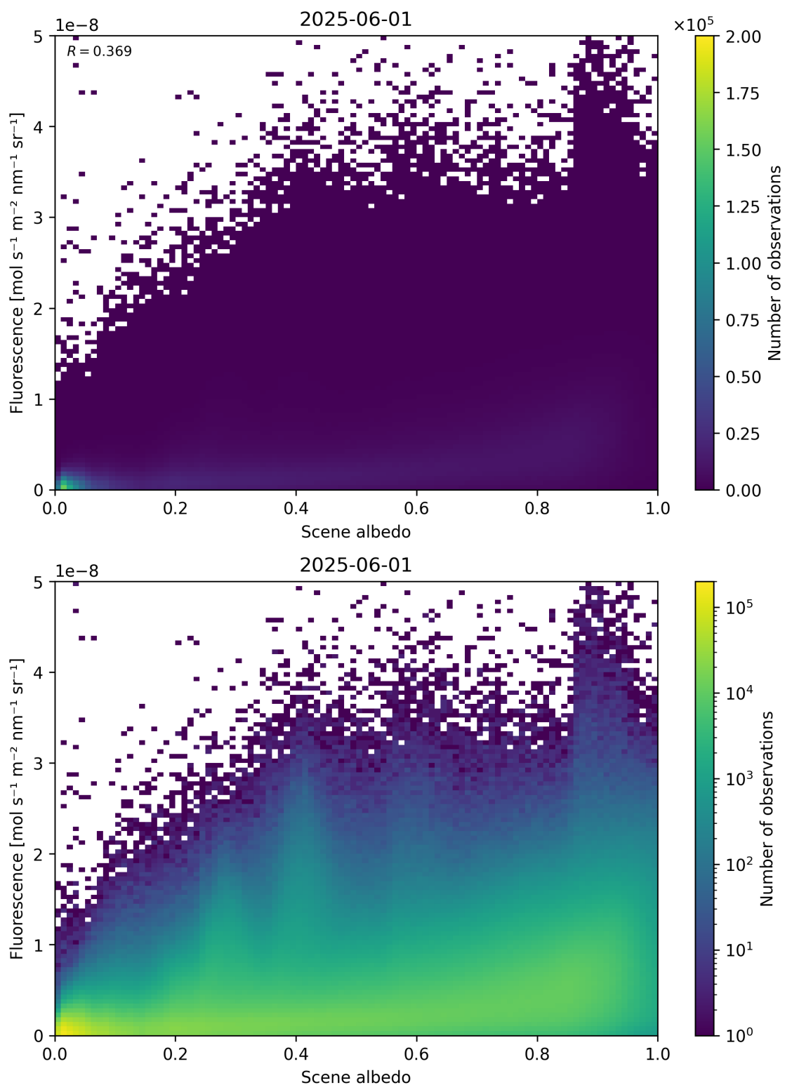
Figure 104: Scatter density plot of “Scene albedo” against “Fluorescence” for 2025-06-01 to 2025-06-02.
