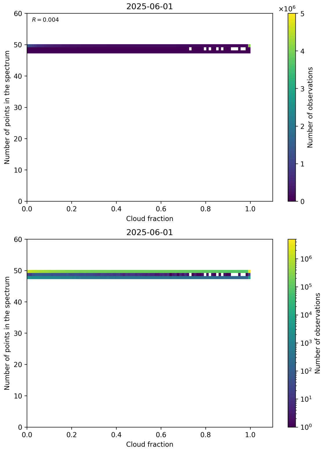
Figure 74: Scatter density plot of “Cloud fraction” against “Number of points in the spectrum” for 2025-06-01 to 2025-06-02.
