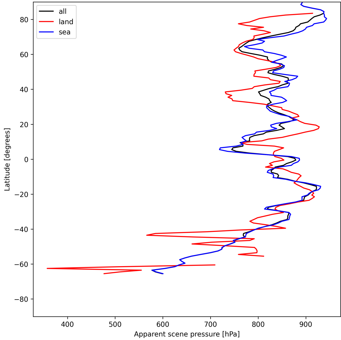
Figure 19: Zonal average of “Apparent scene pressure” for 2025-06-01 to 2025-06-02.
