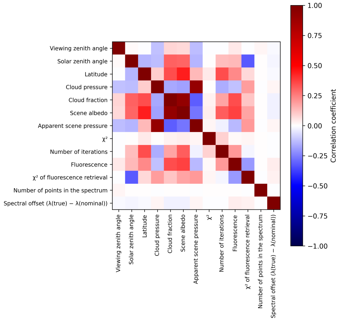
Figure 2: Map of correlation matrix for 2025-06-01 to 2025-06-02.
