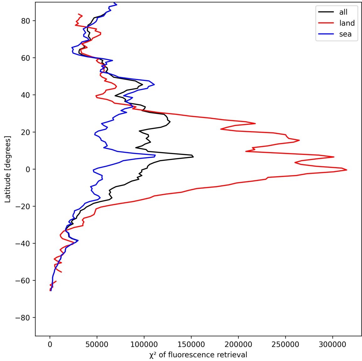
Figure 25: Zonal average of “ \chi^2 of fluorescence retrieval” for 2025-06-01 to 2025-06-02.
