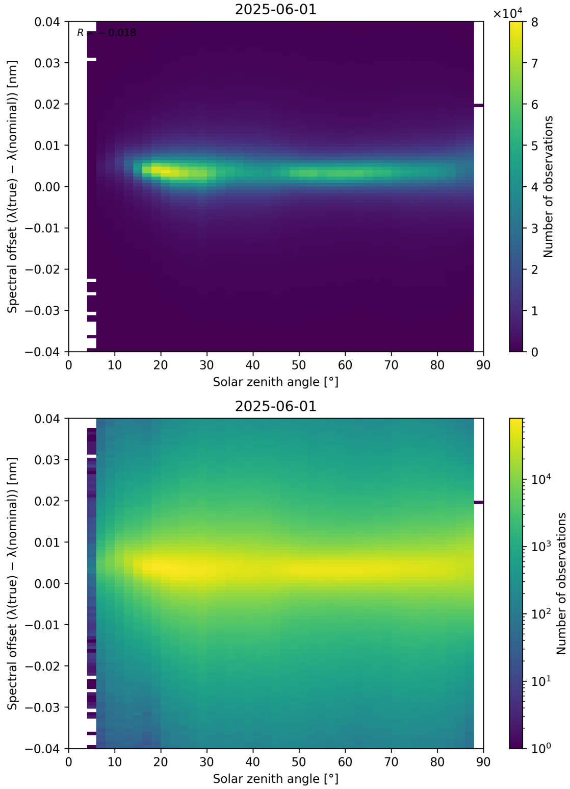
Figure 117: Scatter density plot of “Solar zenith angle” against “Spectral offset ( \lambda_{\text{true}} - \lambda_{\text{nominal}} )” for 2025-06-01 to 2025-06-02.
