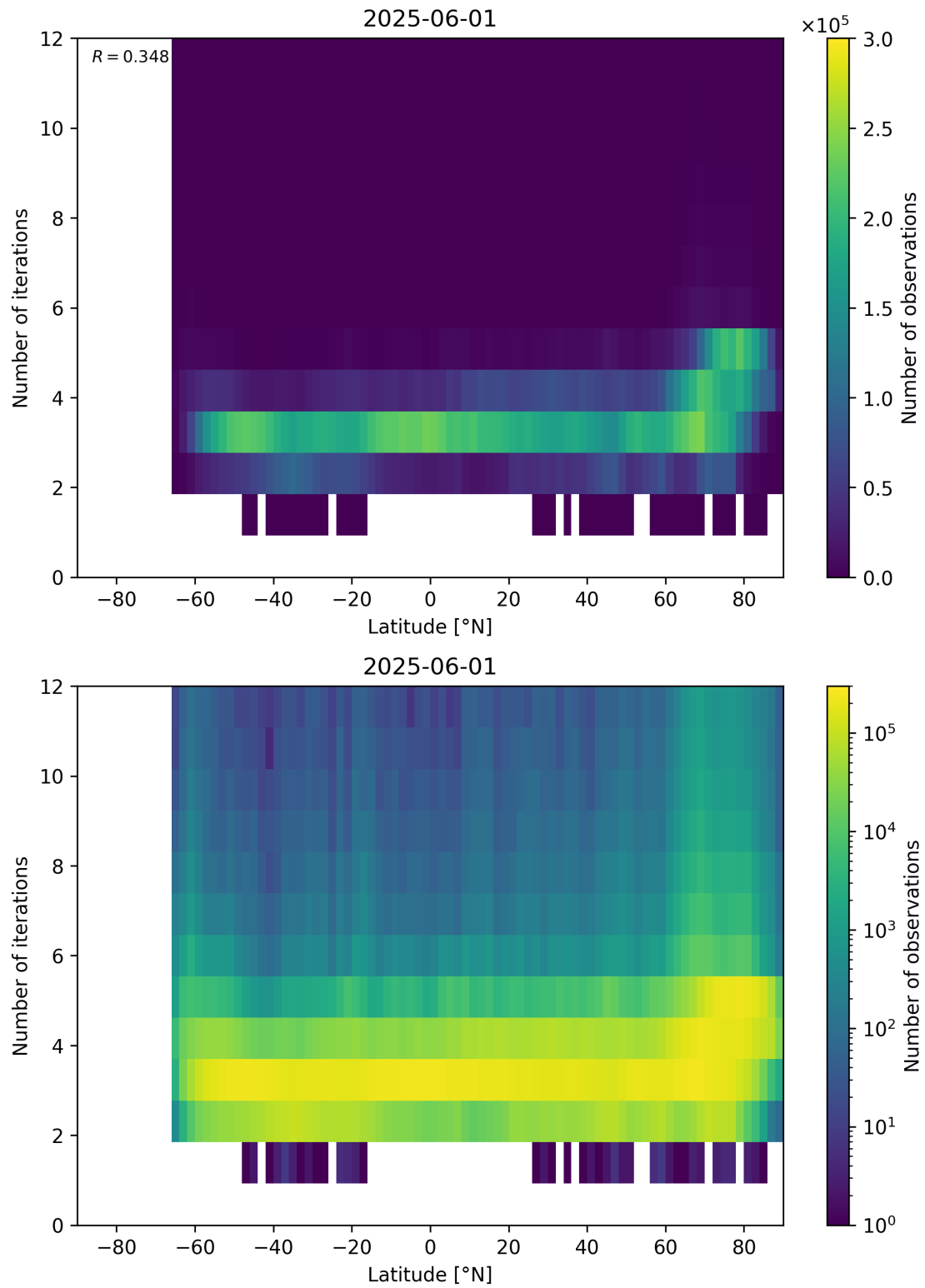
Figure 93: Scatter density plot of “Latitude” against “Number of iterations” for 2025-06-01 to 2025-06-02.
