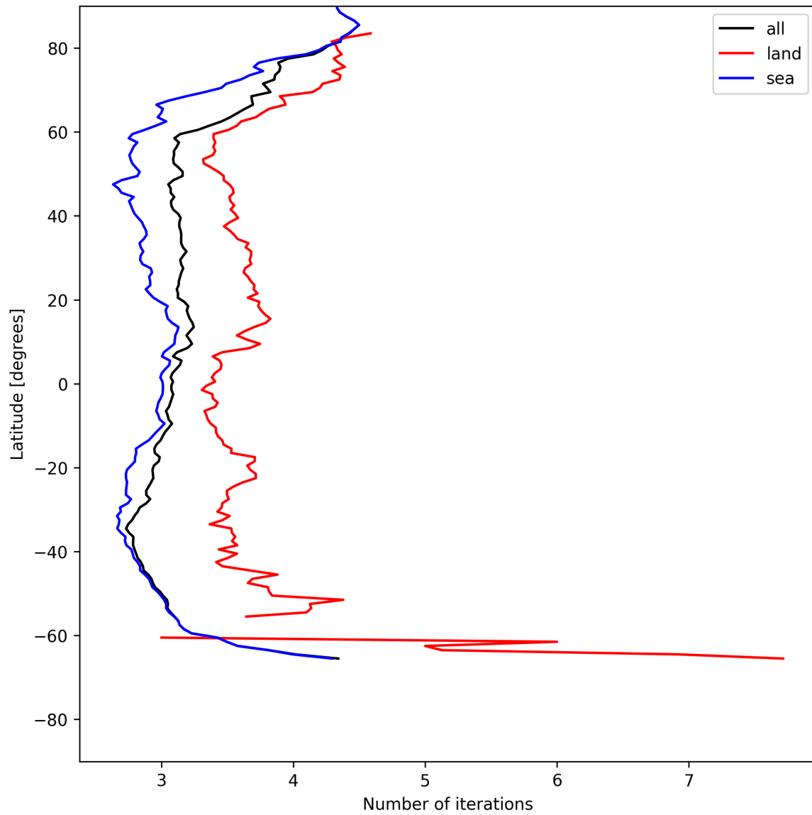
Figure 22: Zonal average of “Number of iterations” for 2025-06-01 to 2025-06-02.
