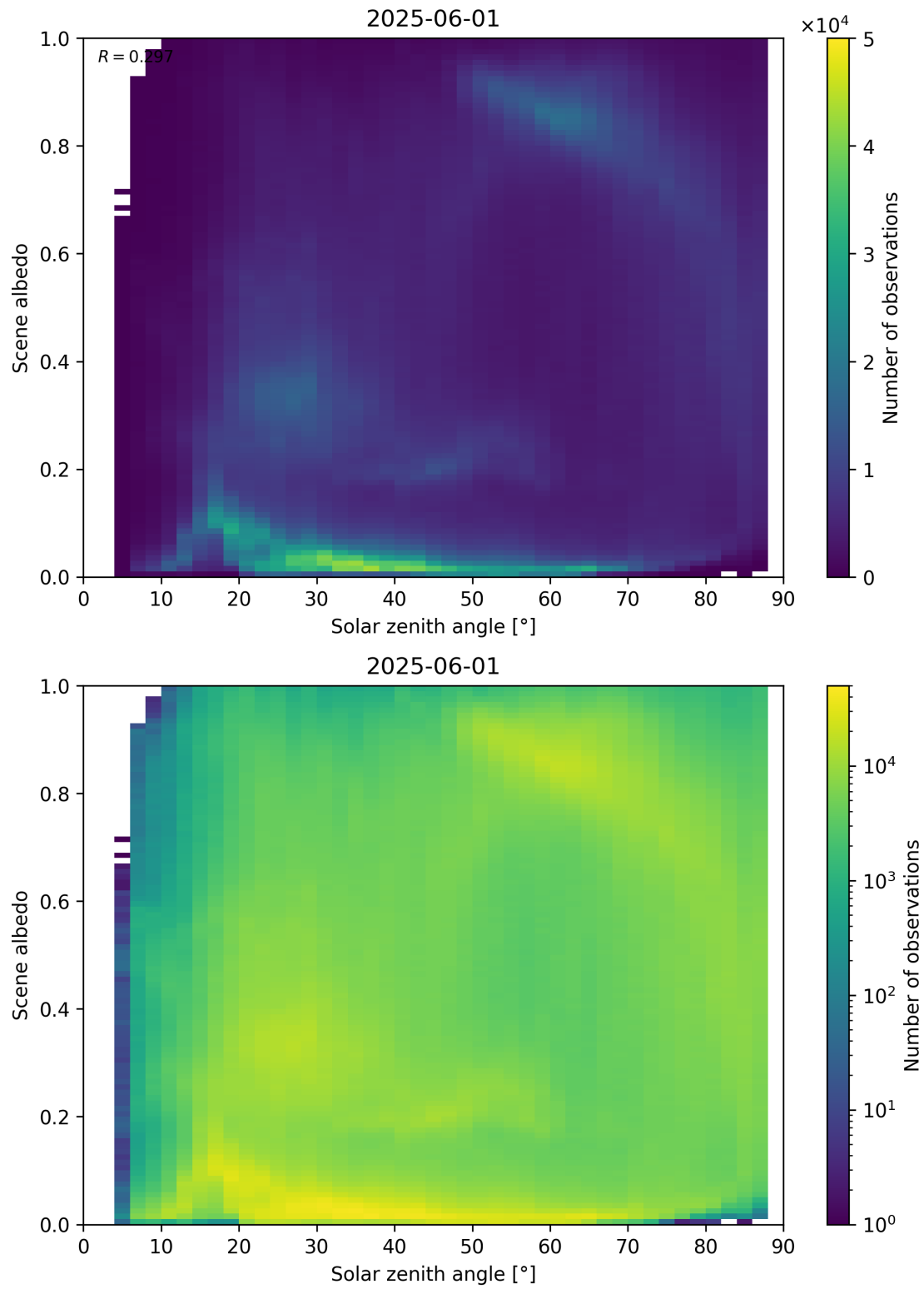
Figure 116: Scatter density plot of “Solar zenith angle” against “Scene albedo” for 2025-06-01 to 2025-06-02.
