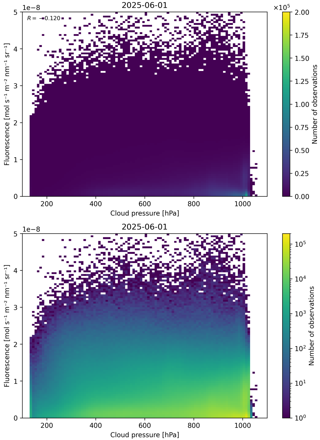
Figure 80: Scatter density plot of “Cloud pressure” against “Fluorescence” for 2025-06-01 to 2025-06-02.
