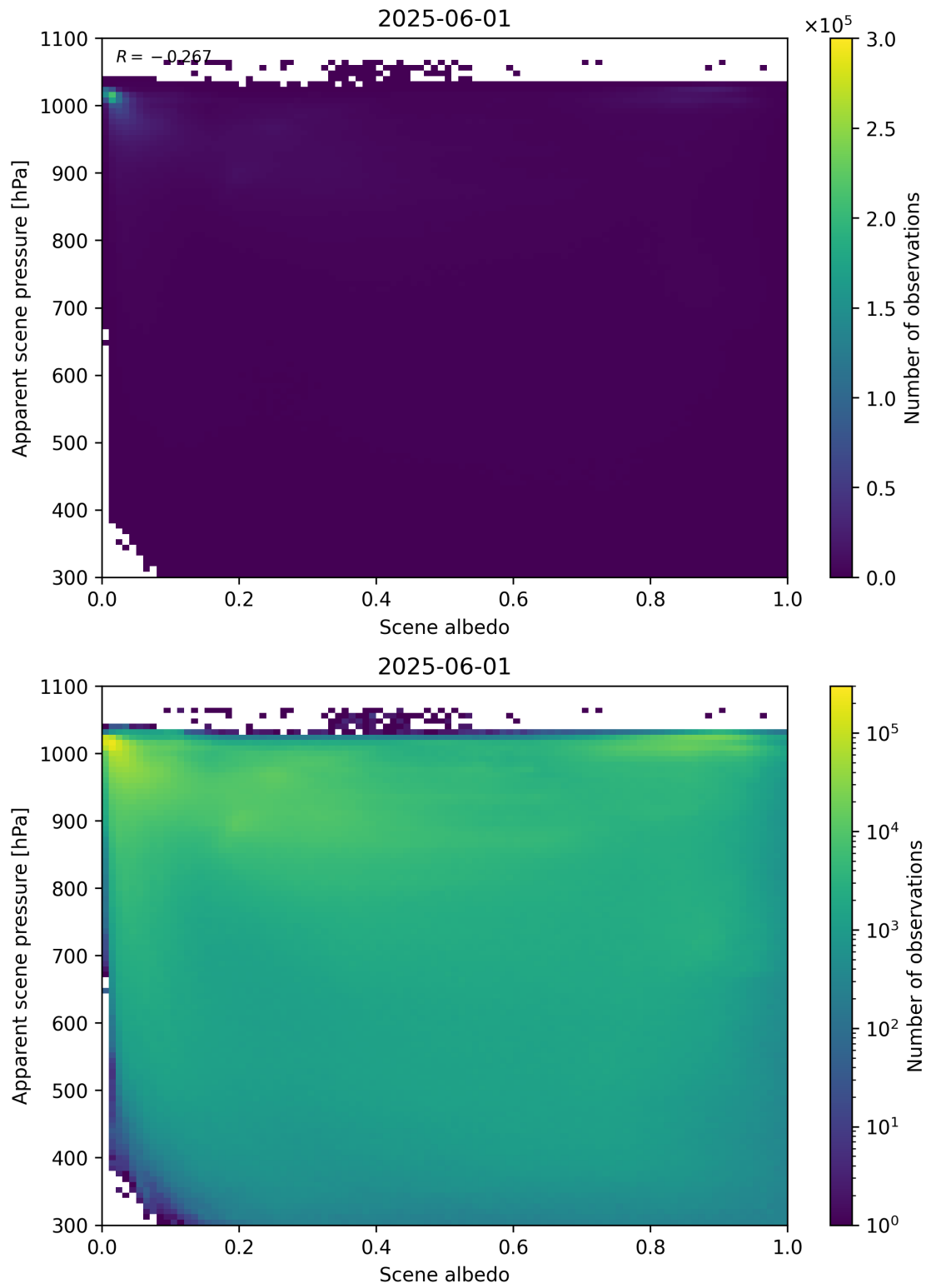
Figure 102: Scatter density plot of “Scene albedo” against “Apparent scene pressure” for 2025-06-01 to 2025-06-02.
