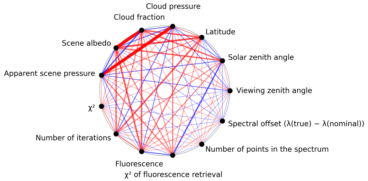
Figure 1: Map of correlation graph for 2025-06-01 to 2025-06-02.
