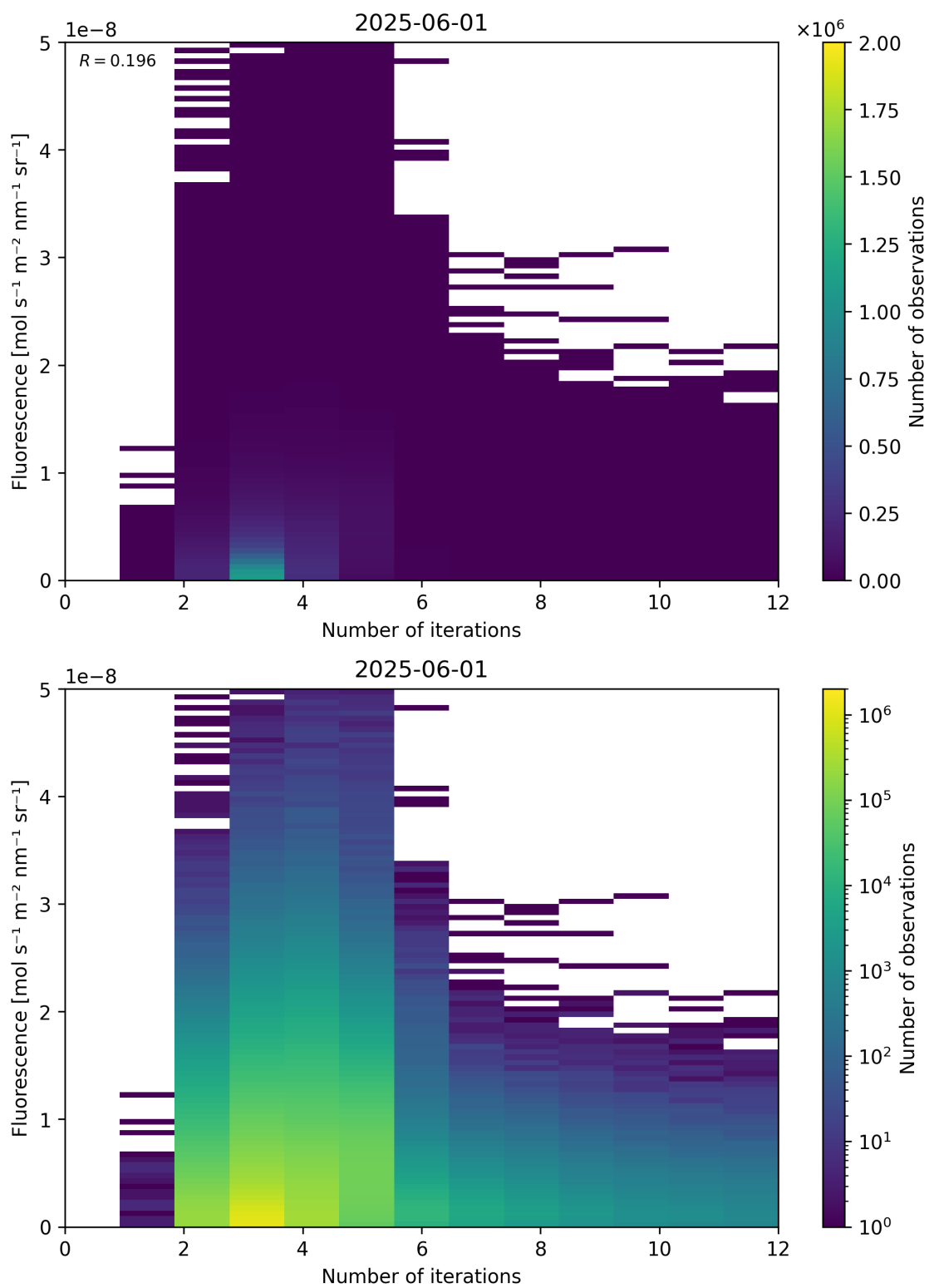
Figure 98: Scatter density plot of “Number of iterations” against “Fluorescence” for 2025-06-01 to 2025-06-02.
