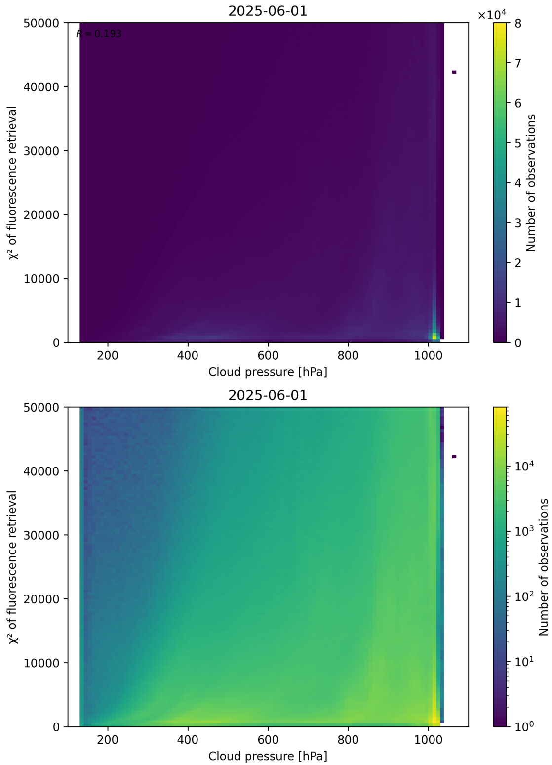
Figure 78: Scatter density plot of “Cloud pressure” against “ \chi^2 of fluorescence retrieval” for 2025-06-01 to 2025-06-02.
