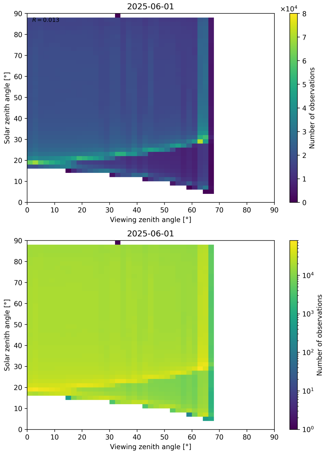
Figure 127: Scatter density plot of “Viewing zenith angle” against “Solar zenith angle” for 2025-06-01 to 2025-06-02.
