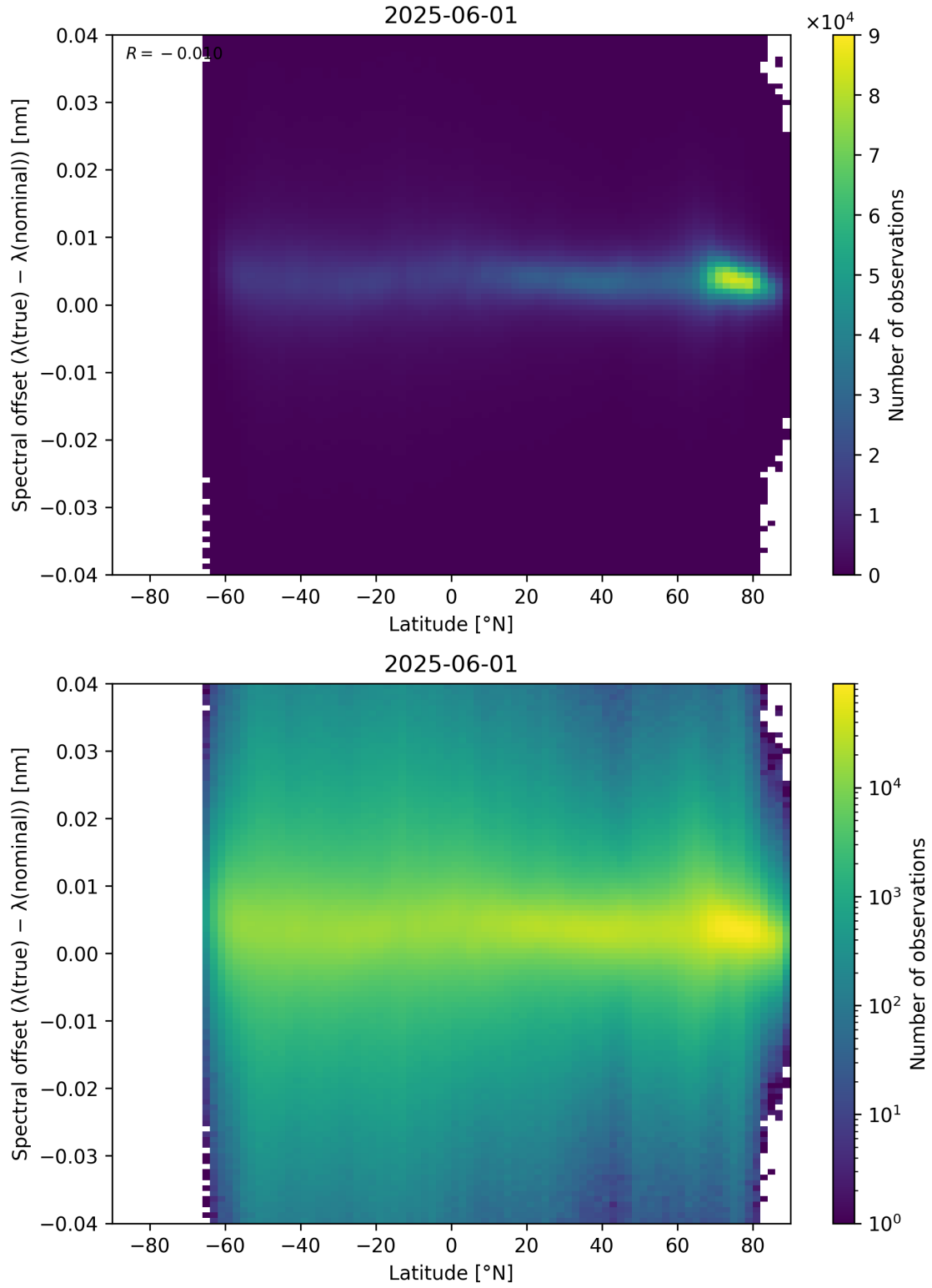
Figure 96: Scatter density plot of “Latitude” against “Spectral offset ( \lambda_{\text{true}} - \lambda_{\text{nominal}} )” for 2025-06-01 to 2025-06-02.
