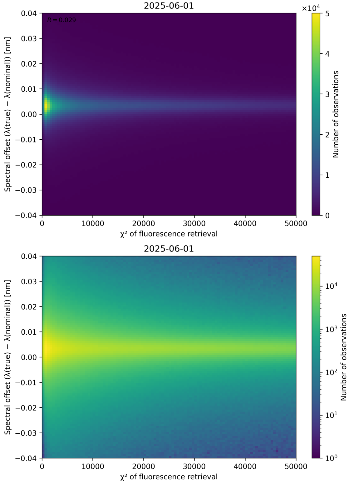
Figure 69: Scatter density plot of “ \chi^2 of fluorescence retrieval” against “Spectral offset ( \lambda_{\text{true}} - \lambda_{\text{nominal}} )” for 2025-06-01 to 2025-06-02.
