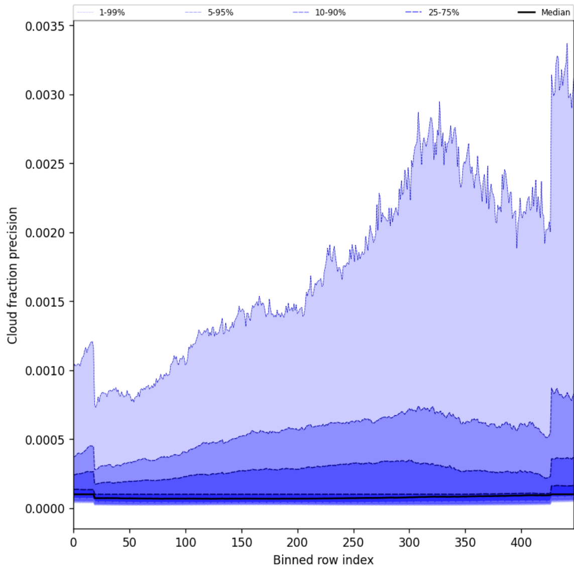
Figure 50: Along track statistics of “Cloud fraction precision” for 2025-06-01 to 2025-06-02
