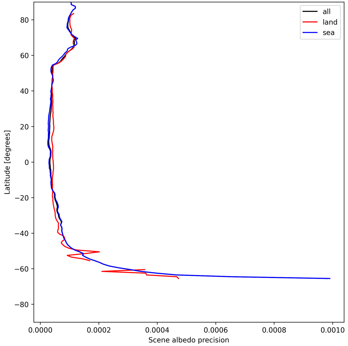
Figure 18: Zonal average of “Scene albedo precision” for 2025-06-01 to 2025-06-02.
