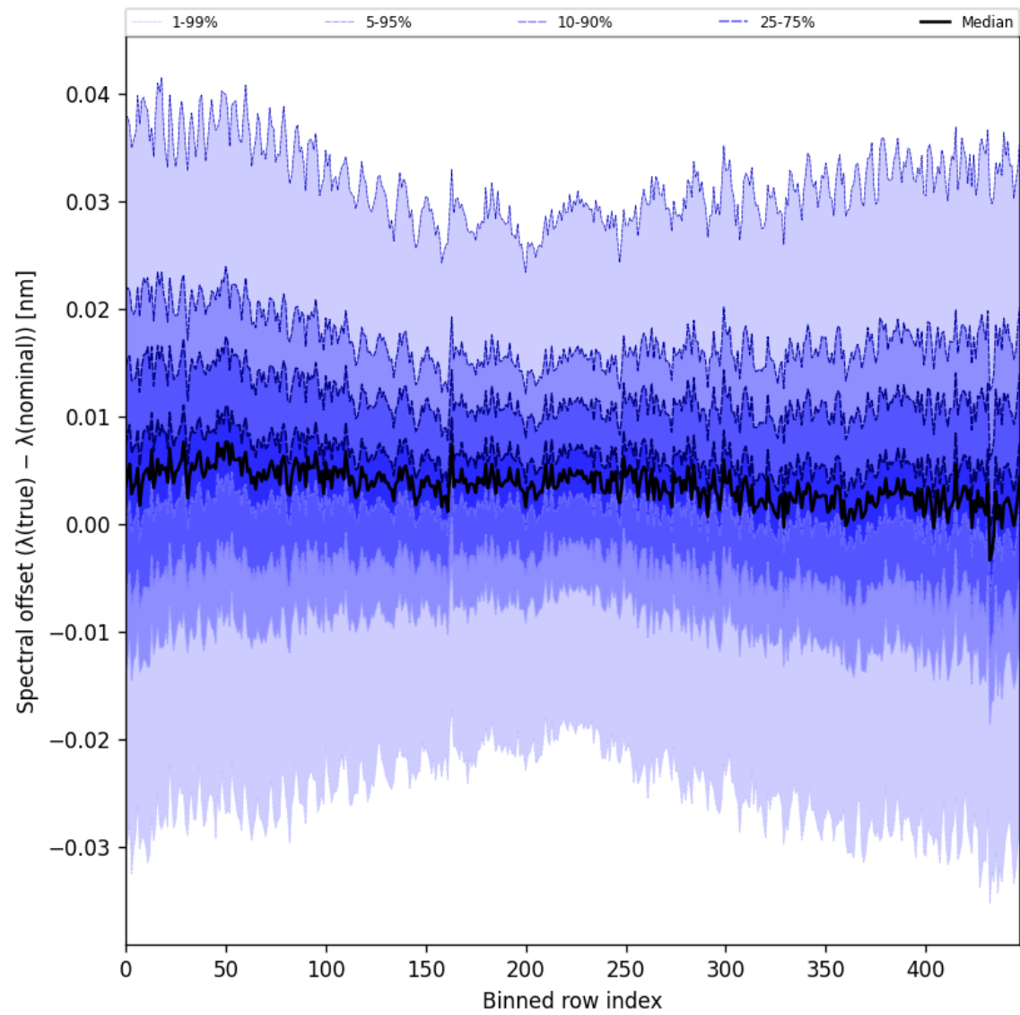
Figure 62: Along track statistics of “Spectral offset ( \lambda_{\text{true}} - \lambda_{\text{nominal}} )” for 2025-06-01 to 2025-06-02
