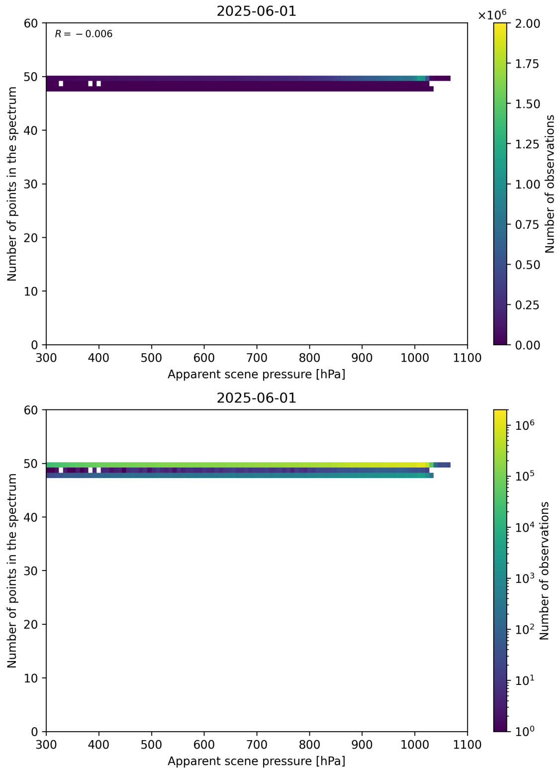
Figure 66: Scatter density plot of “Apparent scene pressure” against “Number of points in the spectrum” for 2025-06-01 to 2025-06-02.
