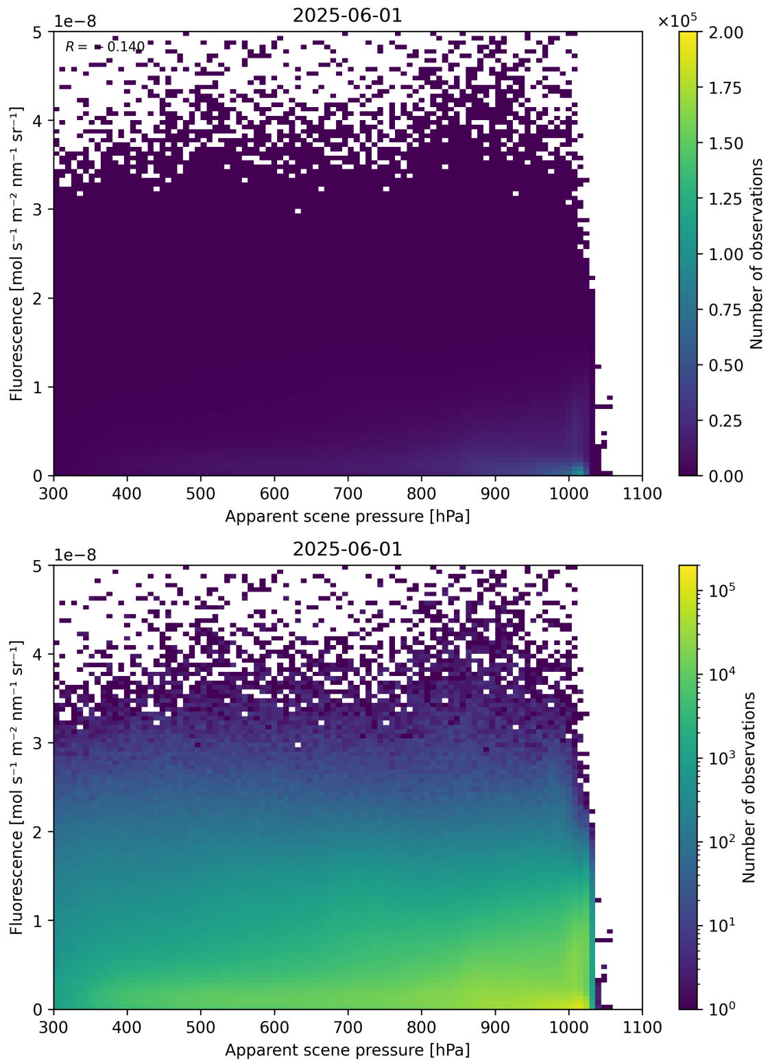
Figure 64: Scatter density plot of “Apparent scene pressure” against “Fluorescence” for 2025-06-01 to 2025-06-02.
