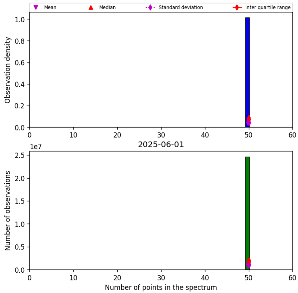
Figure 44: Histogram of “Number of points in the spectrum” for 2025-06-01 to 2025-06-02
