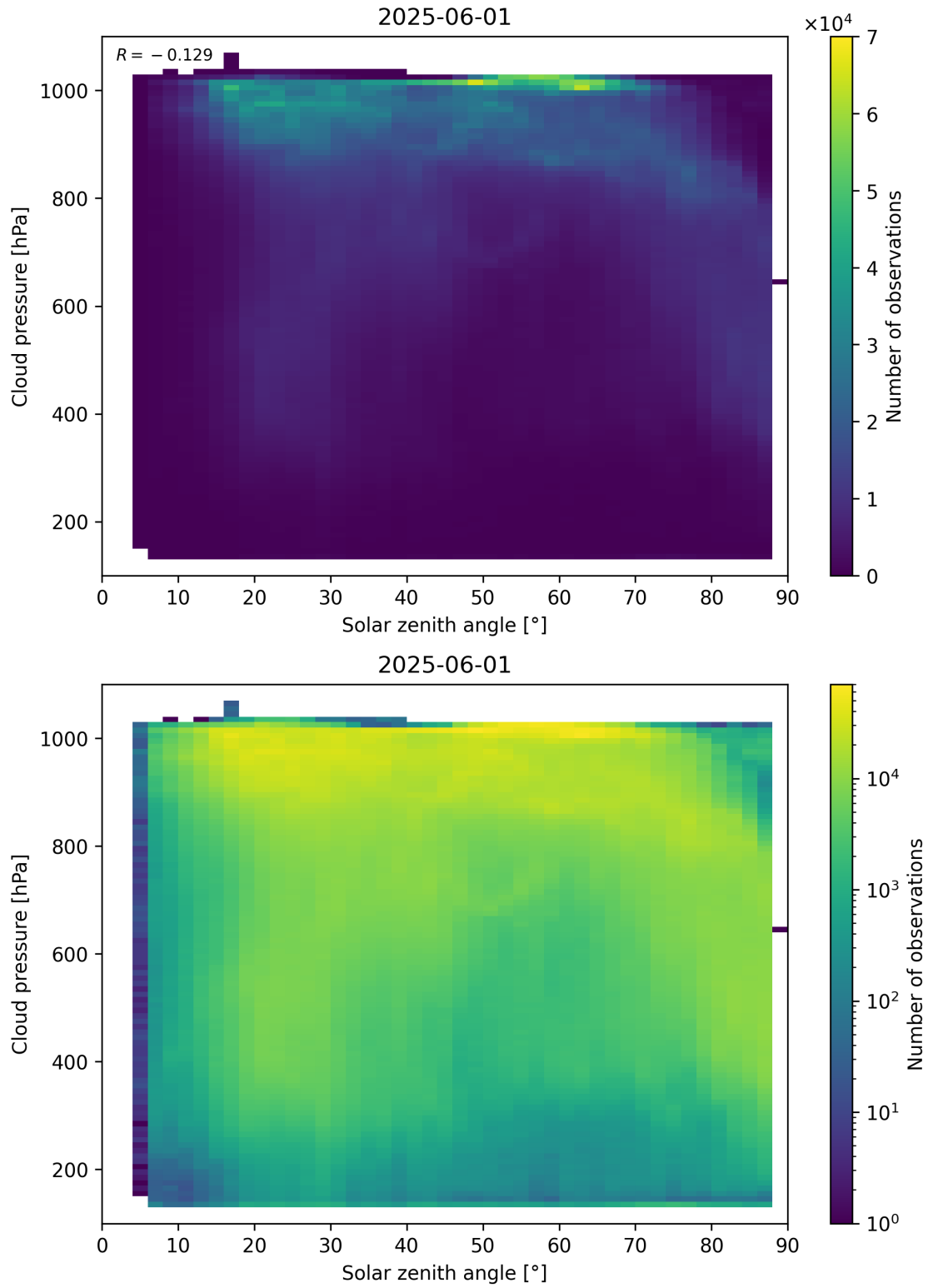
Figure 111: Scatter density plot of “Solar zenith angle” against “Cloud pressure” for 2025-06-01 to 2025-06-02.
