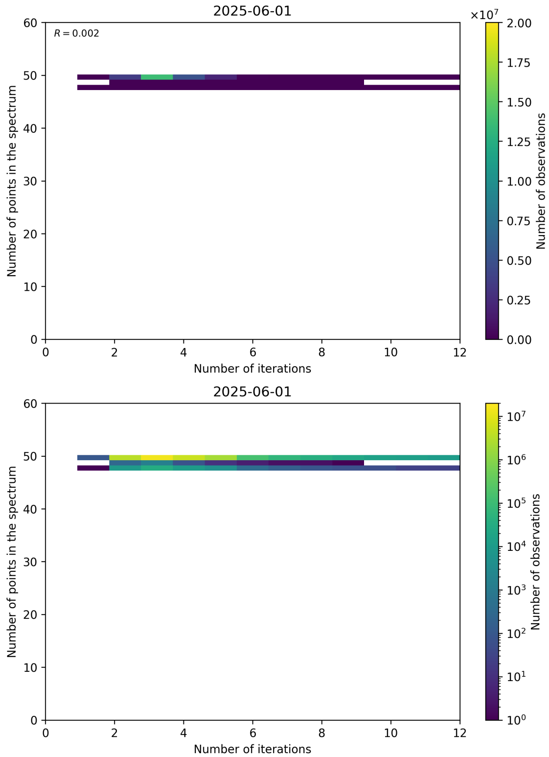
Figure 99: Scatter density plot of “Number of iterations” against “Number of points in the spectrum” for 2025-06-01 to 2025-06-02.
