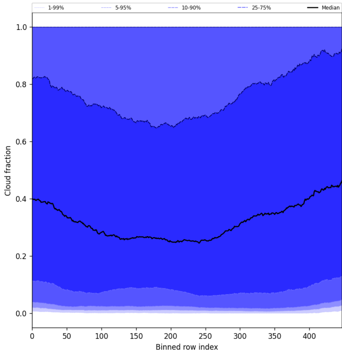
Figure 49: Along track statistics of “Cloud fraction” for 2025-06-01 to 2025-06-02
