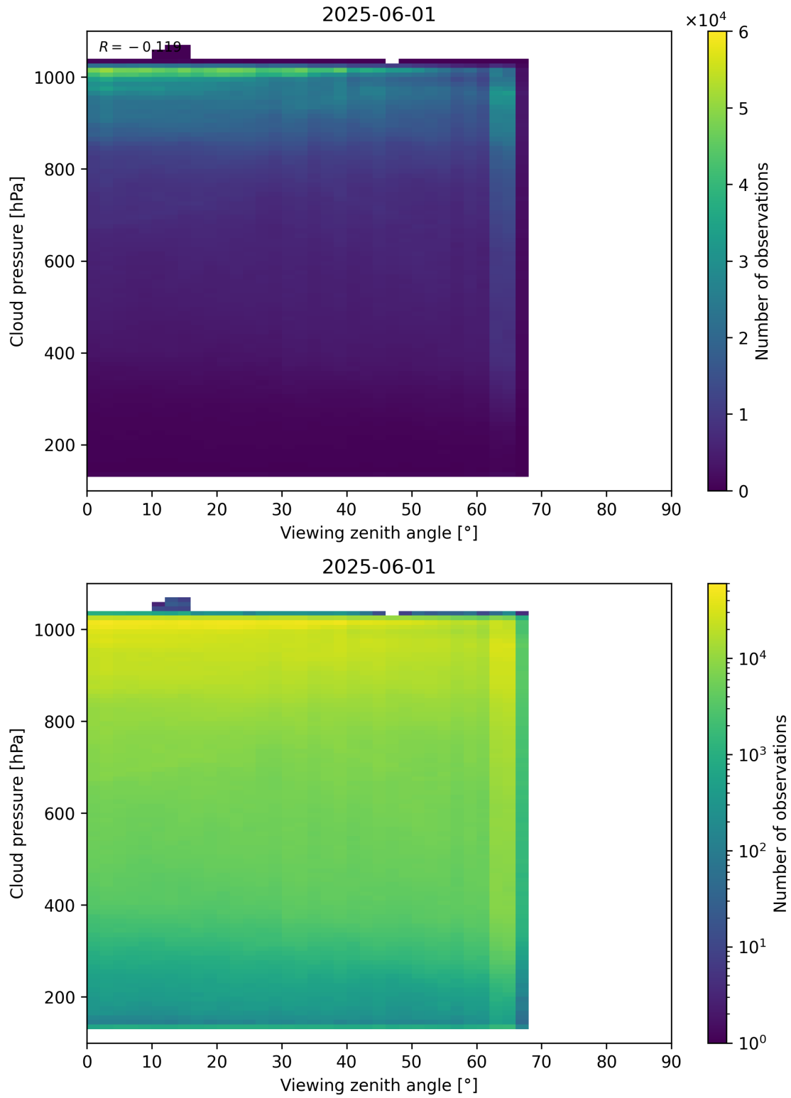
Figure 121: Scatter density plot of “Viewing zenith angle” against “Cloud pressure” for 2025-06-01 to 2025-06-02.
