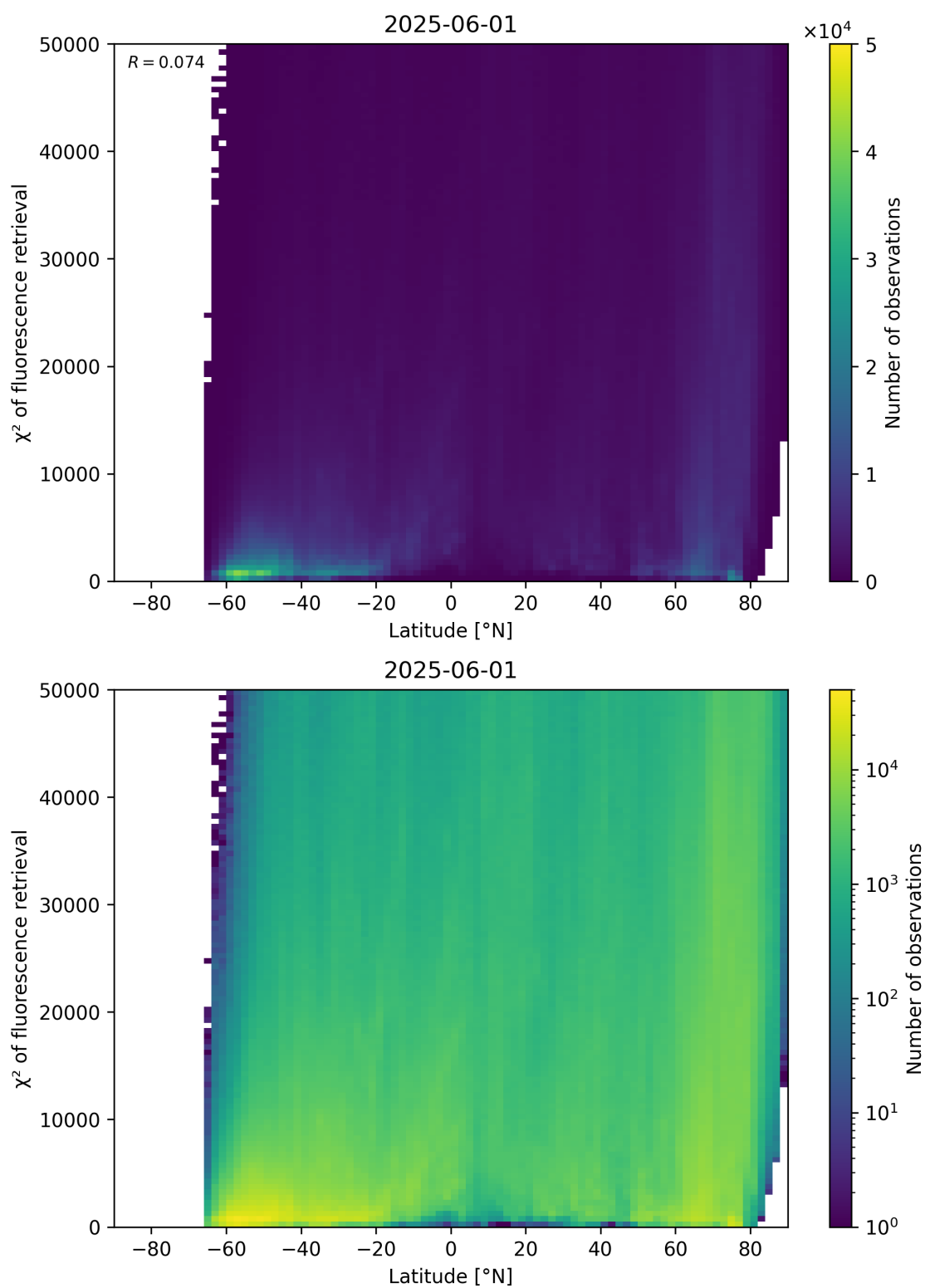
Figure 89: Scatter density plot of “Latitude” against “ \chi^2 of fluorescence retrieval” for 2025-06-01 to 2025-06-02.
