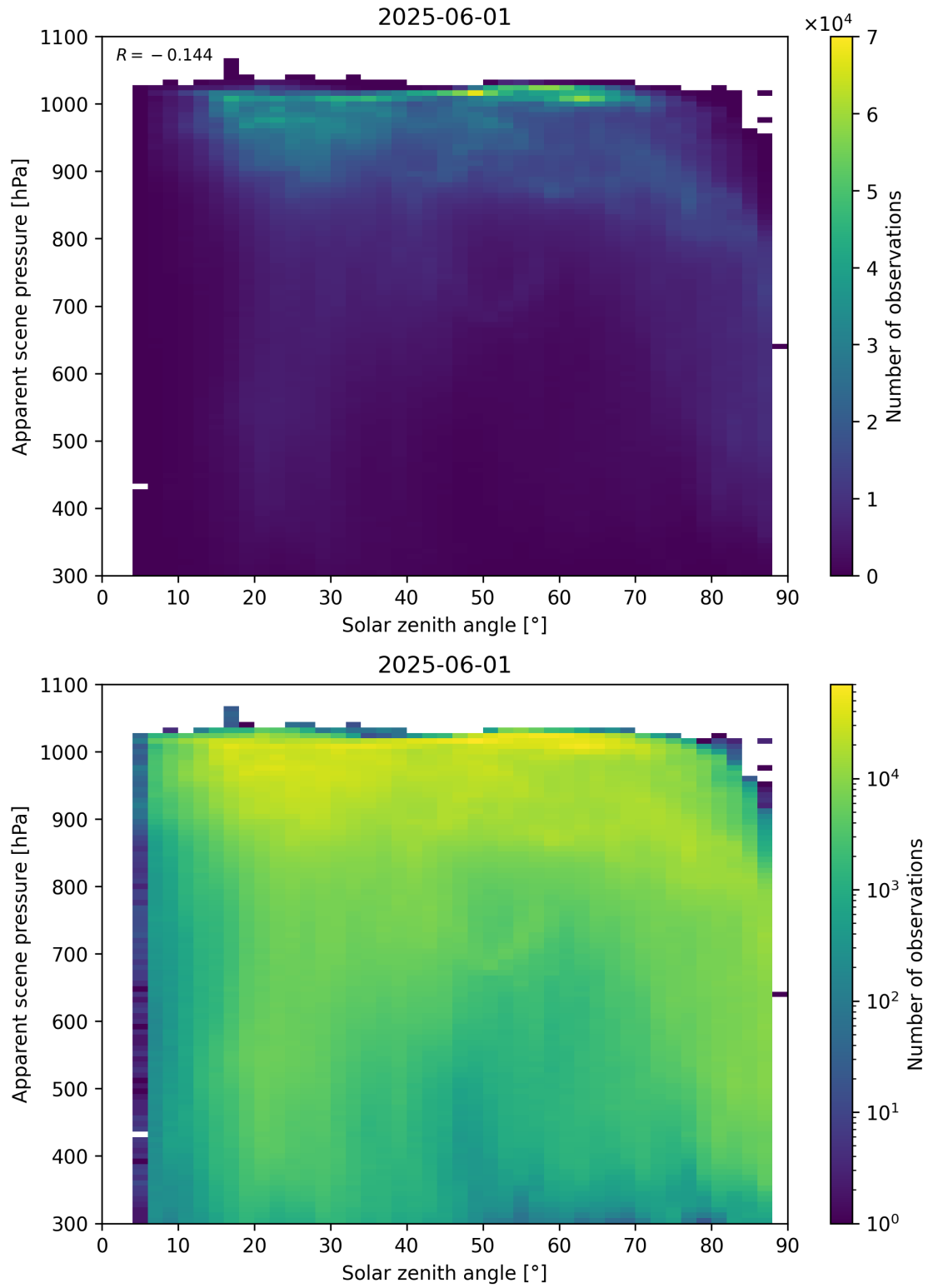
Figure 108: Scatter density plot of “Solar zenith angle” against “Apparent scene pressure” for 2025-06-01 to 2025-06-02.
