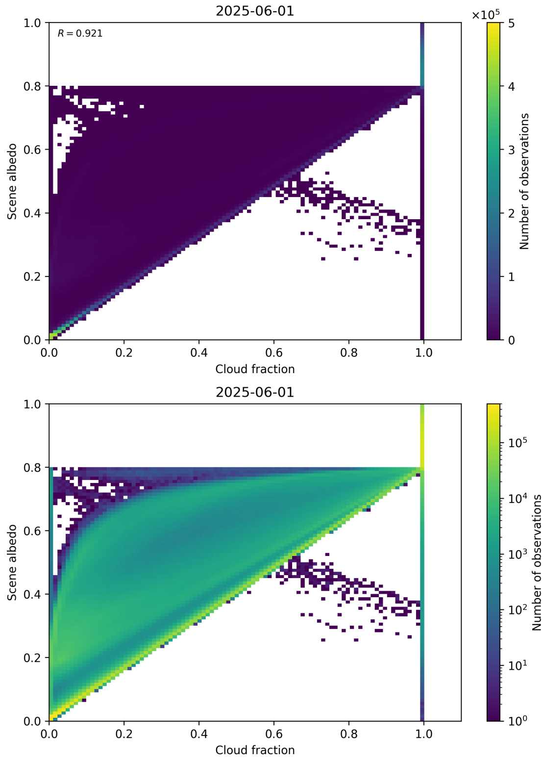
Figure 75: Scatter density plot of “Cloud fraction” against “Scene albedo” for 2025-06-01 to 2025-06-02.
