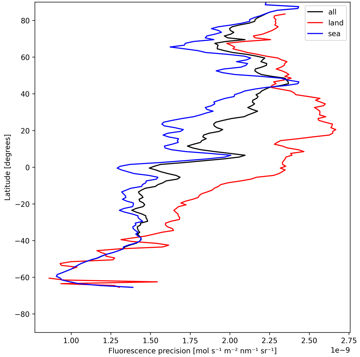
Figure 24: Zonal average of “Fluorescence precision” for 2025-06-01 to 2025-06-02.
