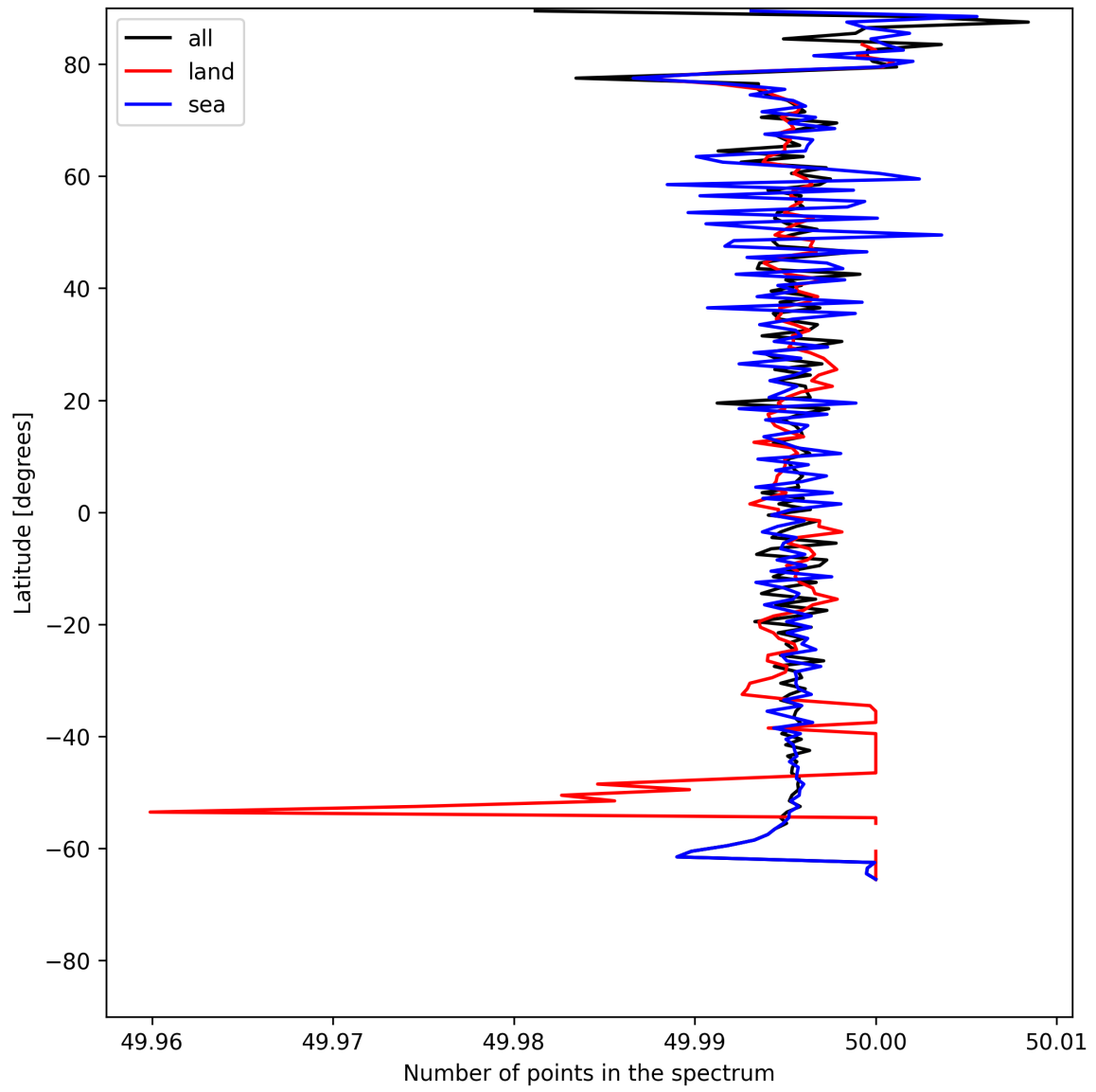
Figure 27: Zonal average of “Number of points in the spectrum” for 2025-06-01 to 2025-06-02.
