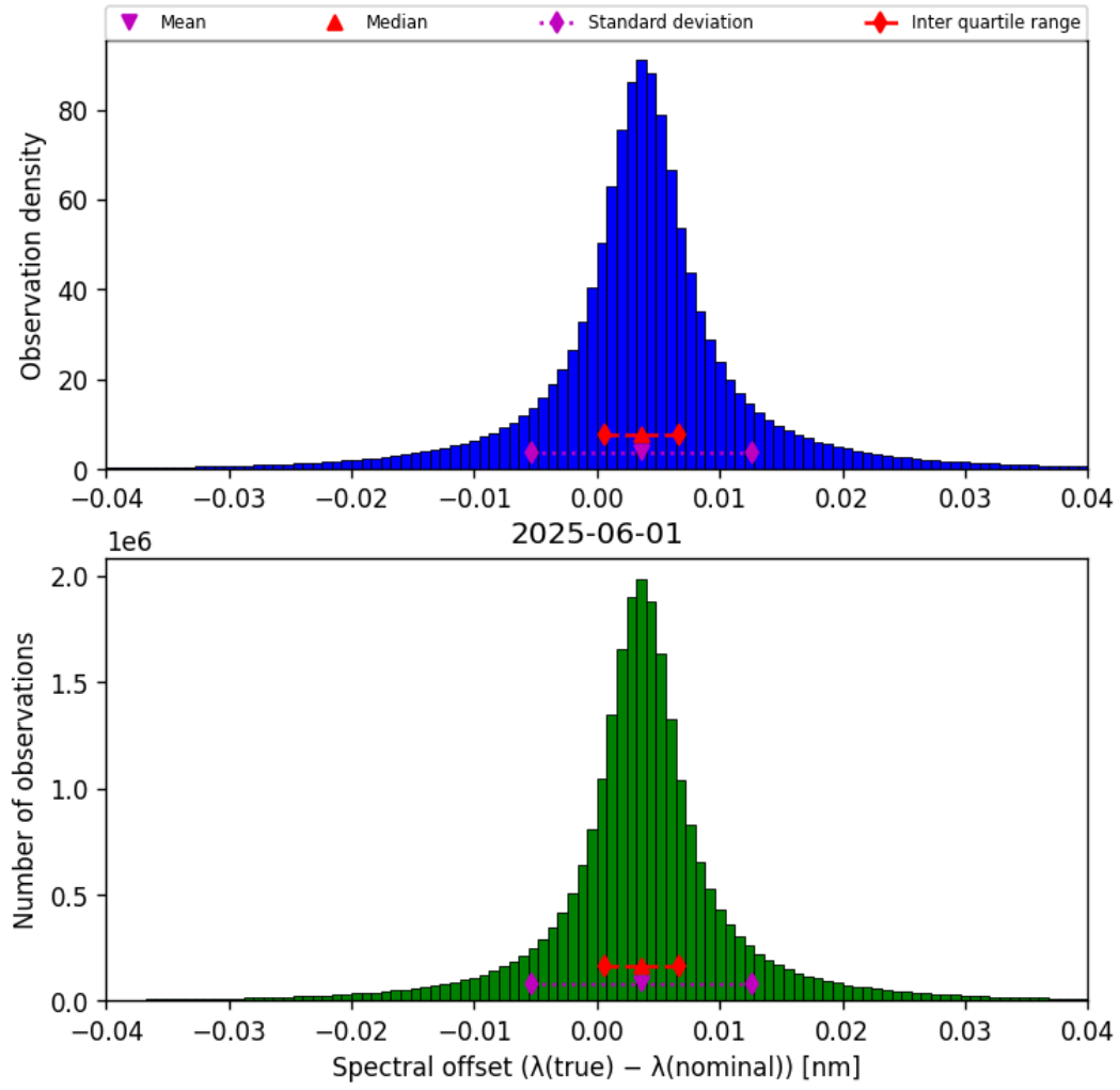
Figure 45: Histogram of “Spectral offset ( \lambda_{\text{true}} - \lambda_{\text{nominal}} )” for 2025-06-01 to 2025-06-02
