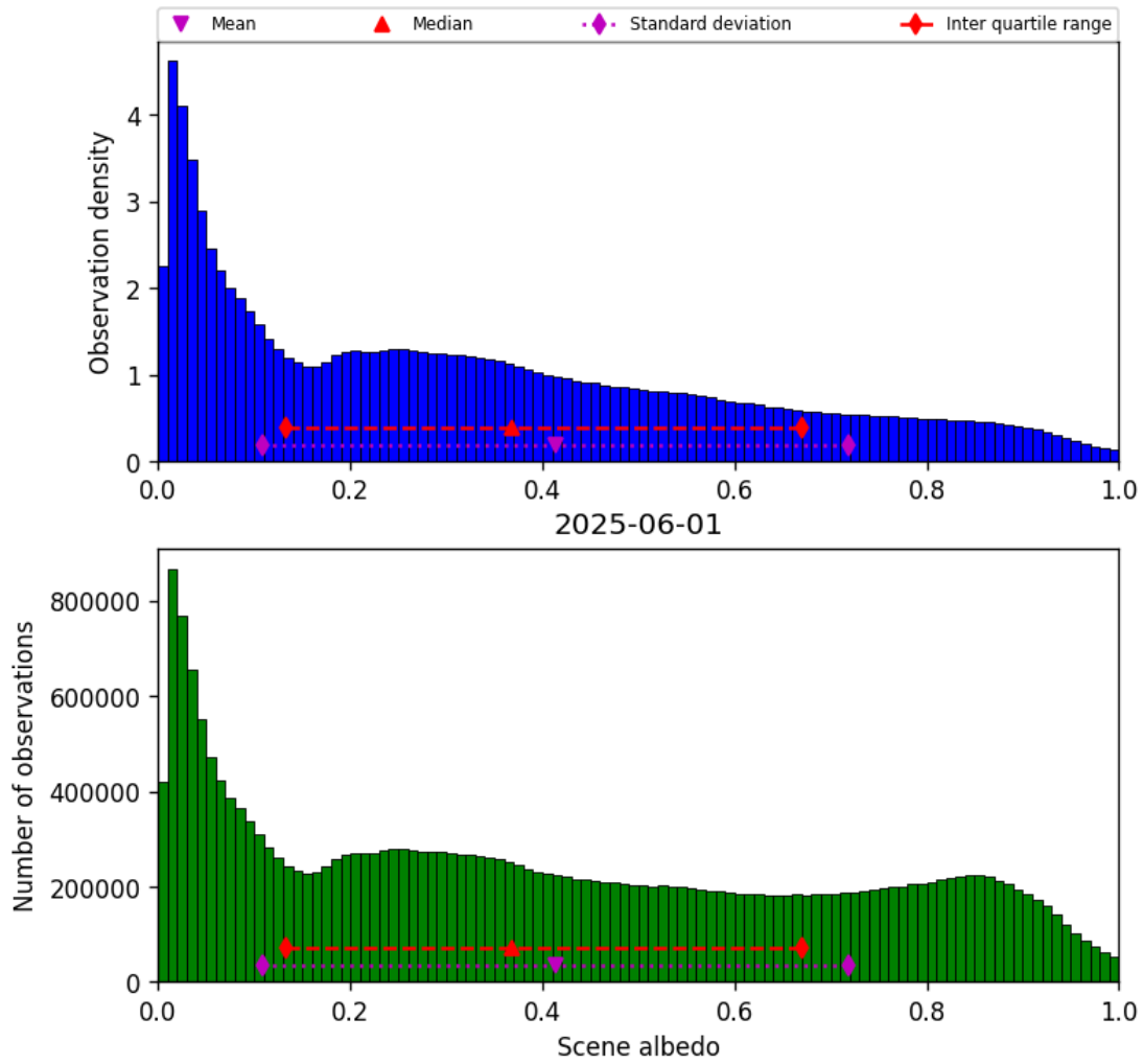
Figure 34: Histogram of “Scene albedo” for 2025-06-01 to 2025-06-02
