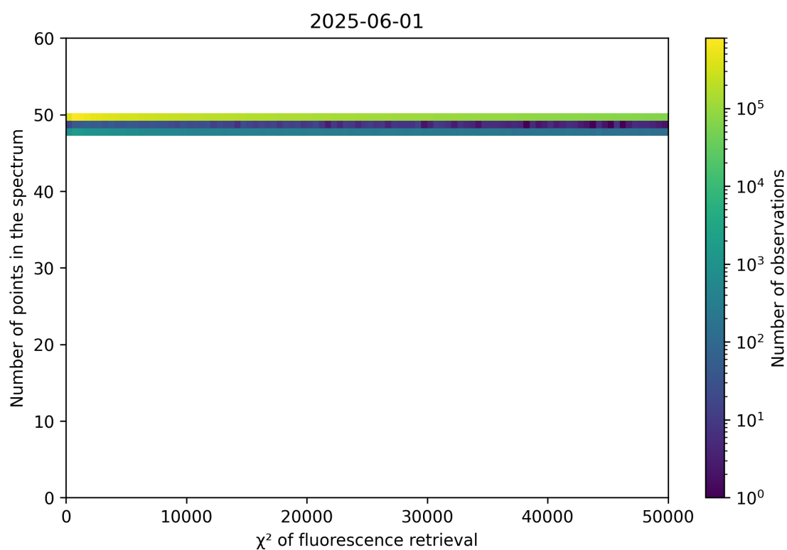
Figure 68: Scatter density plot of “ \chi^2 of fluorescence retrieval” against “Number of points in the spectrum” for 2025-06-01 to 2025-06-02.
