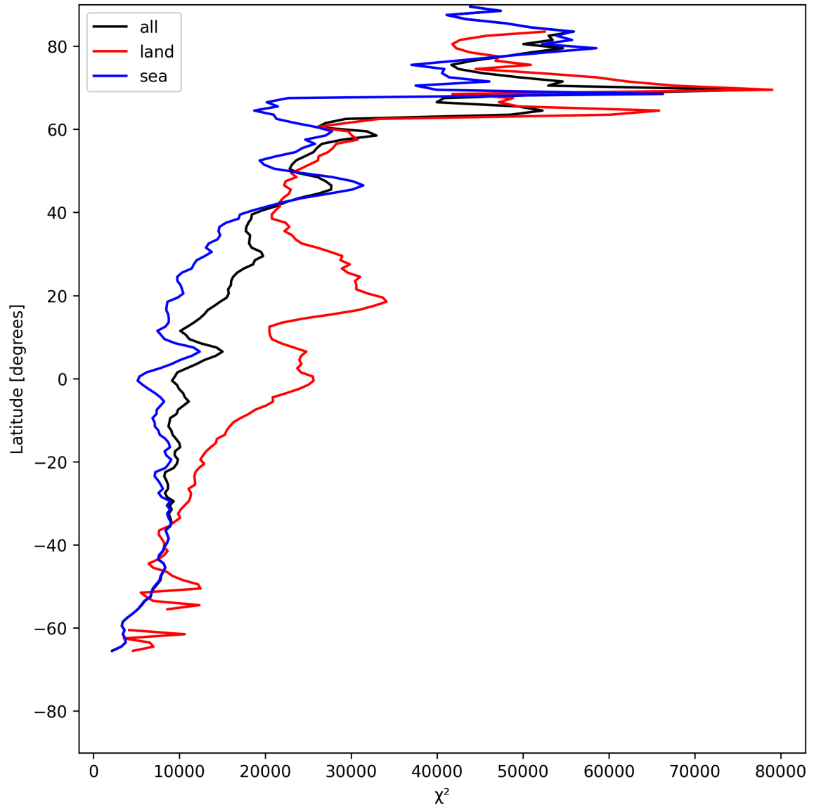
Figure 21: Zonal average of “ \chi^2 ” for 2025-06-01 to 2025-06-02.
