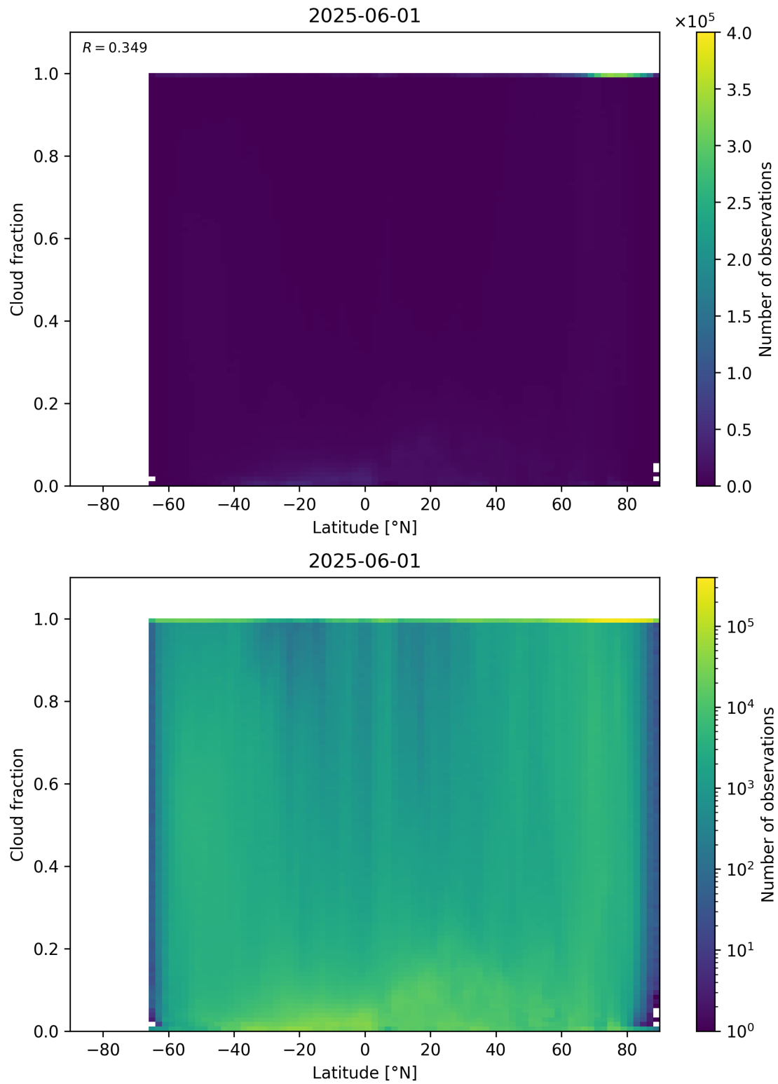
Figure 90: Scatter density plot of “Latitude” against “Cloud fraction” for 2025-06-01 to 2025-06-02.
