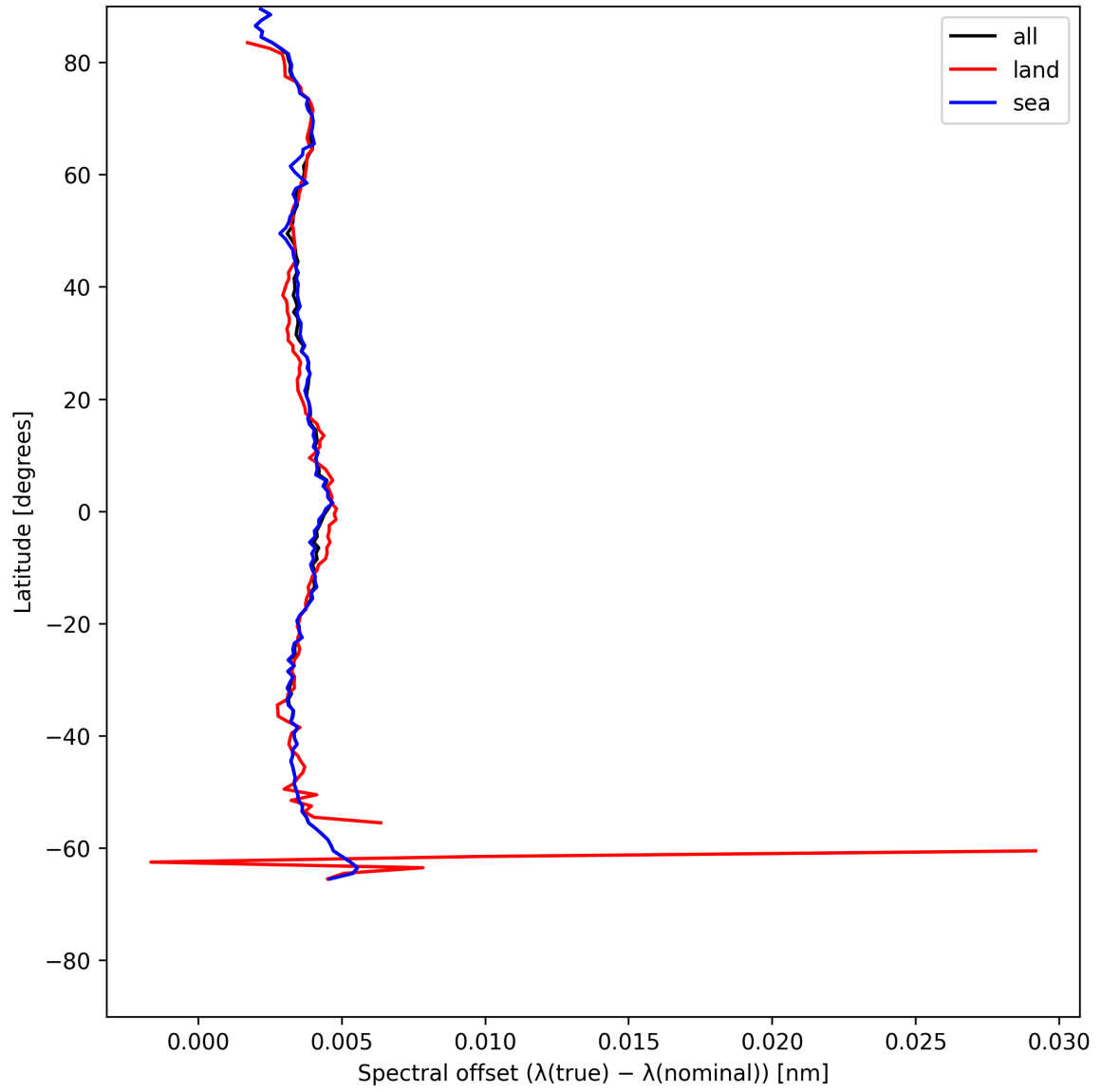
Figure 28: Zonal average of “Spectral offset ( \lambda_{\text{true}} - \lambda_{\text{nominal}} )” for 2025-06-01 to 2025-06-02.
