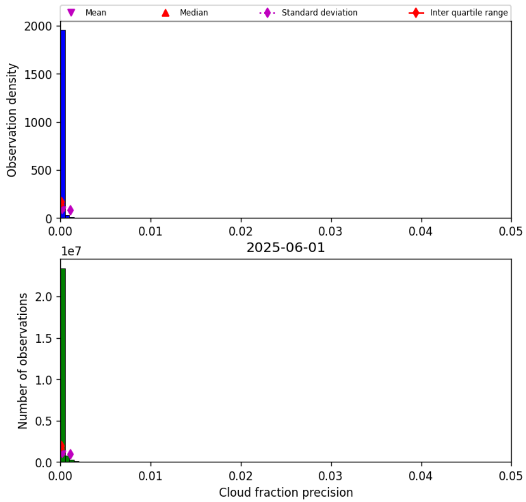
Figure 33: Histogram of “Cloud fraction precision” for 2025-06-01 to 2025-06-02
