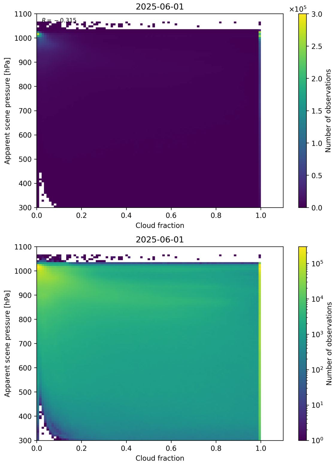
Figure 70: Scatter density plot of “Cloud fraction” against “Apparent scene pressure” for 2025-06-01 to 2025-06-02.
