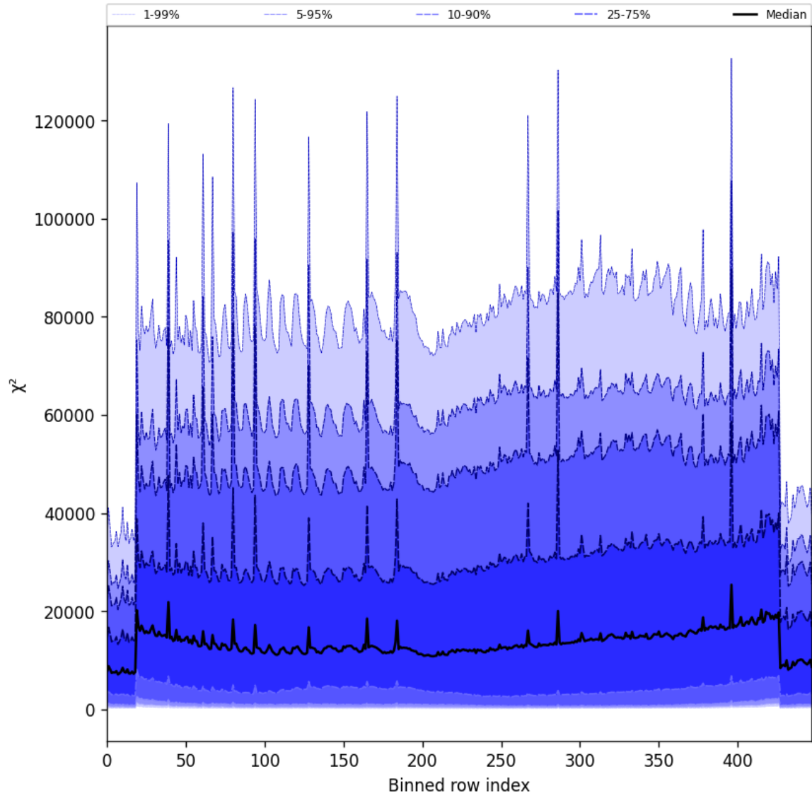
Figure 55: Along track statistics of “ \chi^2 ” for 2025-06-01 to 2025-06-02
