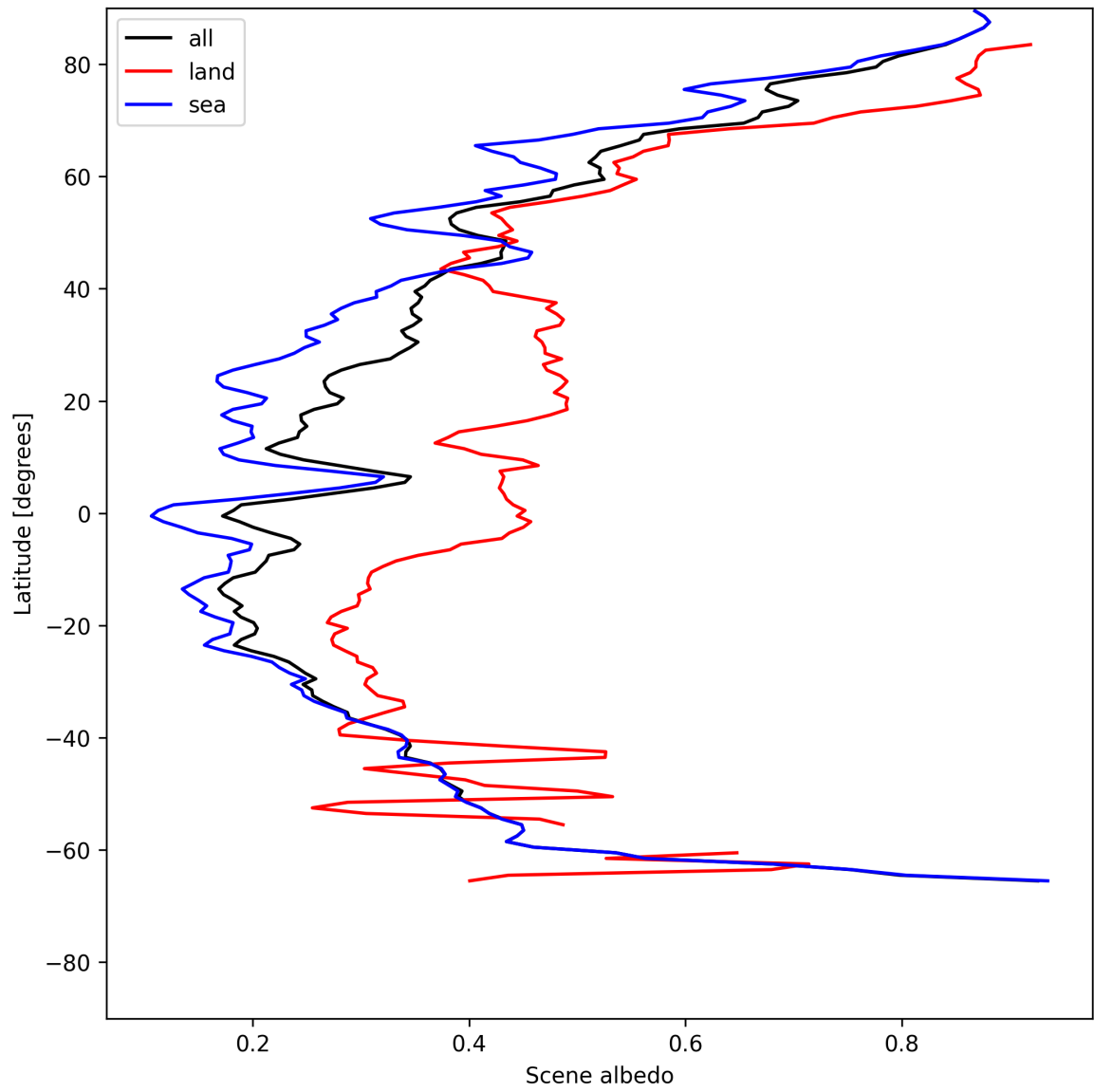
Figure 17: Zonal average of “Scene albedo” for 2025-06-01 to 2025-06-02.
