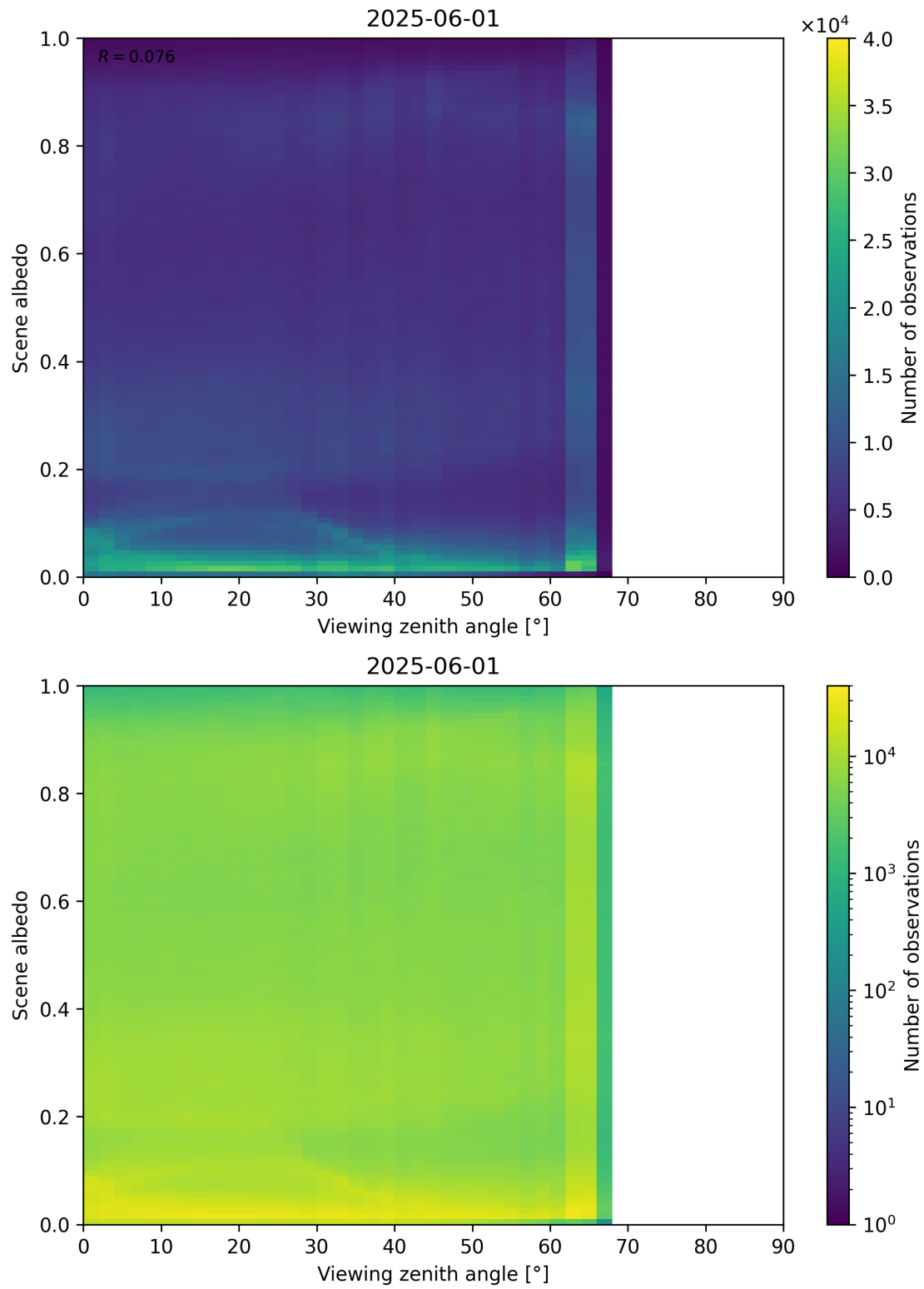
Figure 126: Scatter density plot of “Viewing zenith angle” against “Scene albedo” for 2025-06-01 to 2025-06-02.
