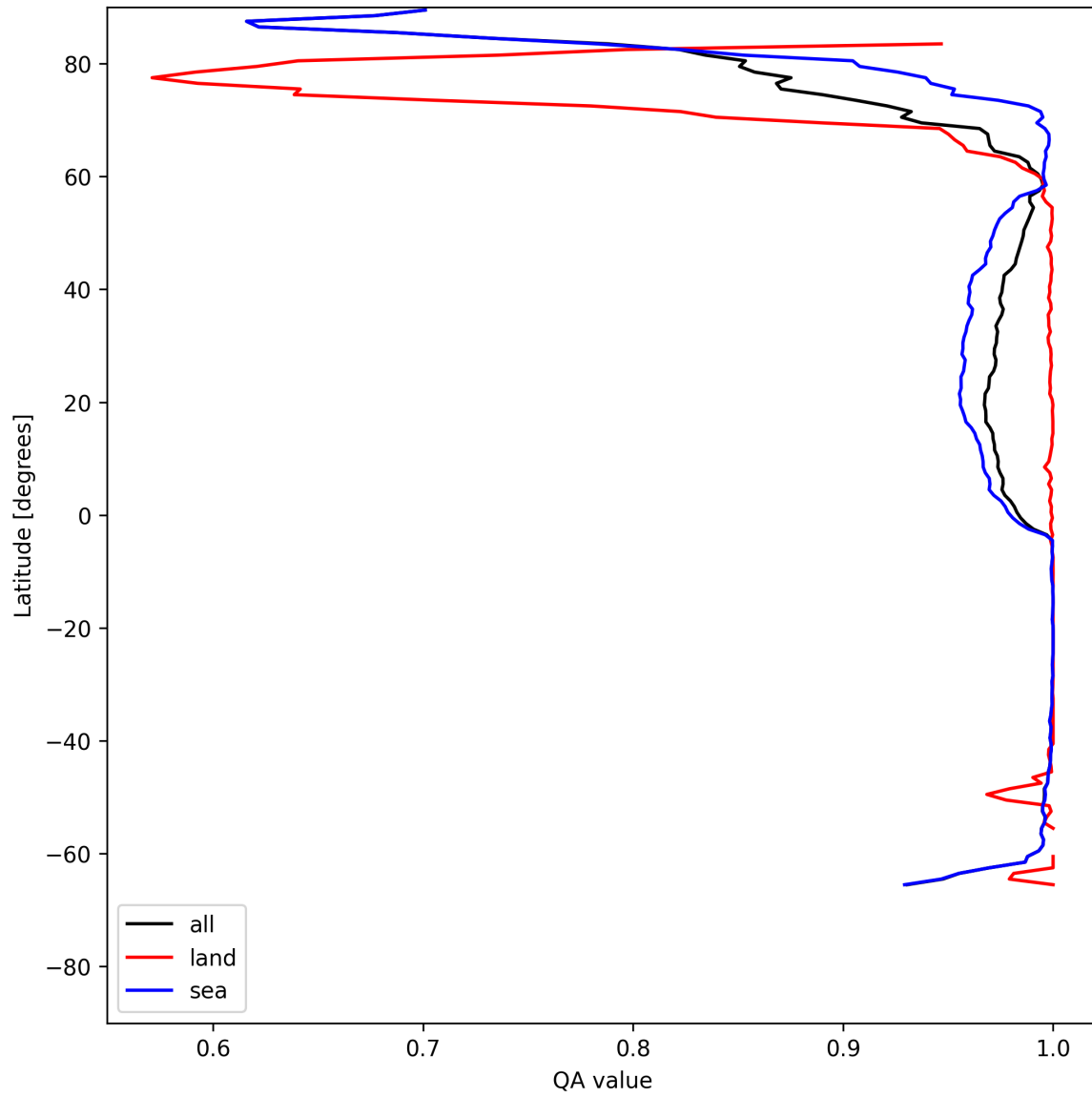
Figure 12: Zonal average of “QA value” for 2025-06-01 to 2025-06-02.
