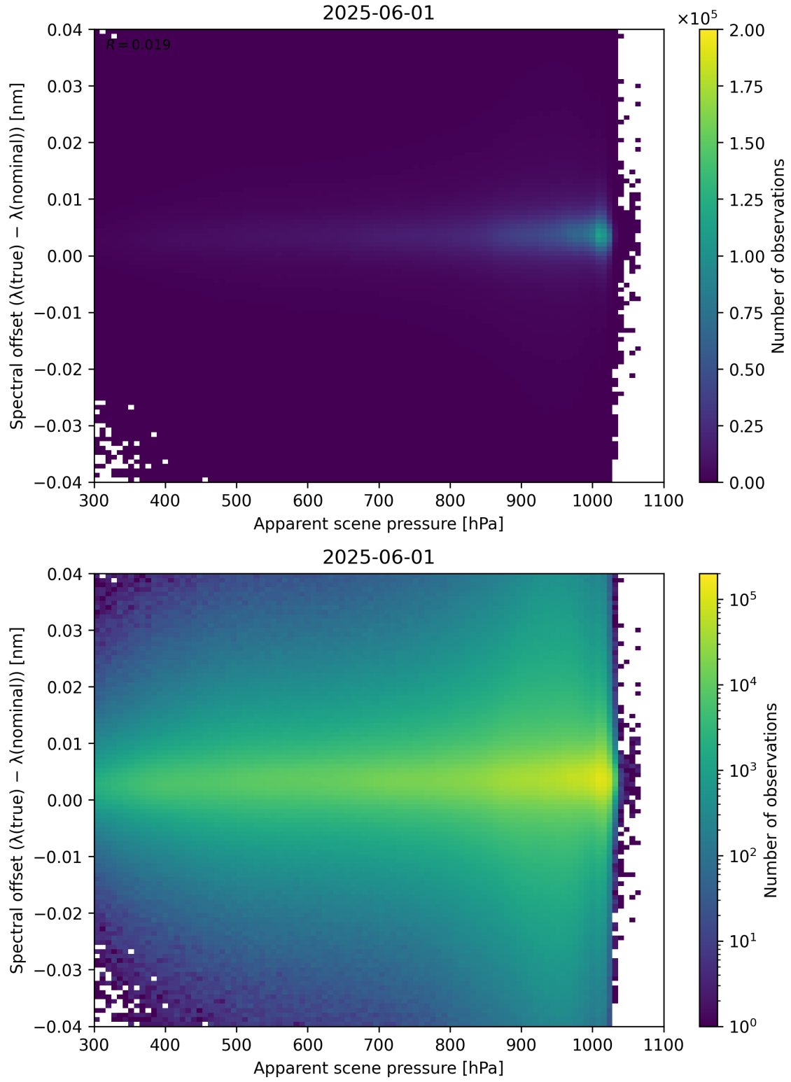
Figure 67: Scatter density plot of “Apparent scene pressure” against “Spectral offset ( \lambda_{\text{true}} - \lambda_{\text{nominal}} )” for 2025-06-01 to 2025-06-02.
