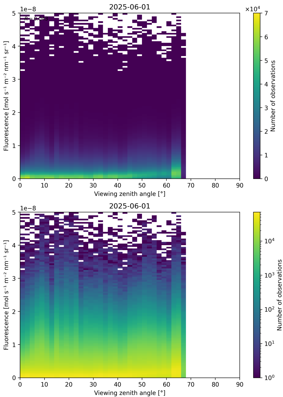
Figure 122: Scatter density plot of “Viewing zenith angle” against “Fluorescence” for 2025-06-01 to 2025-06-02.
