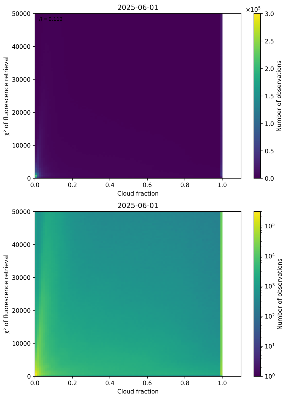
Figure 71: Scatter density plot of “Cloud fraction” against “ \chi^2 of fluorescence retrieval” for 2025-06-01 to 2025-06-02.
