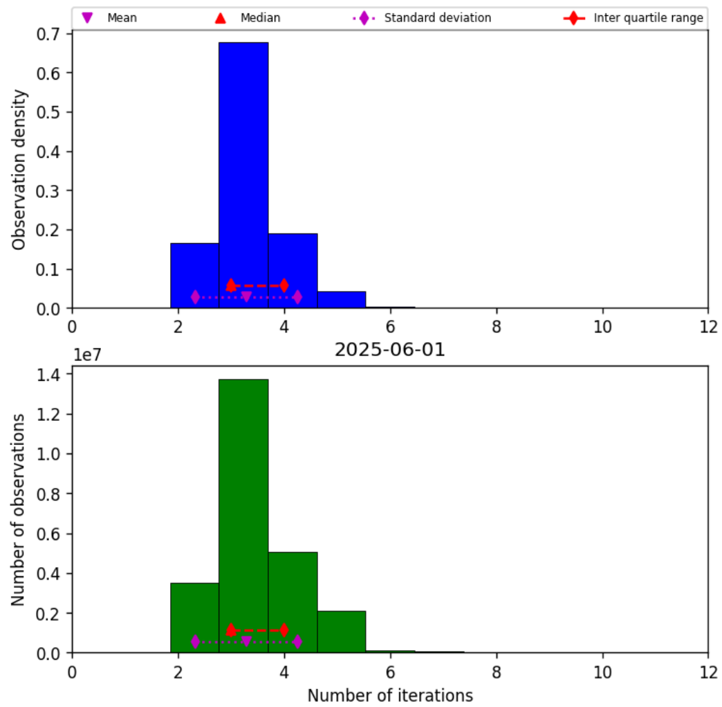
Figure 39: Histogram of “Number of iterations” for 2025-06-01 to 2025-06-02
