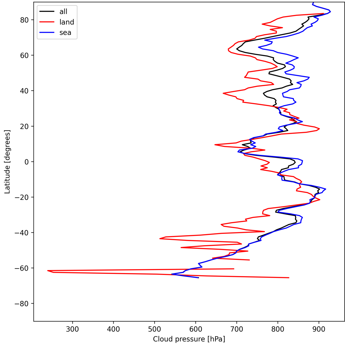
Figure 13: Zonal average of “Cloud pressure” for 2025-06-01 to 2025-06-02.
