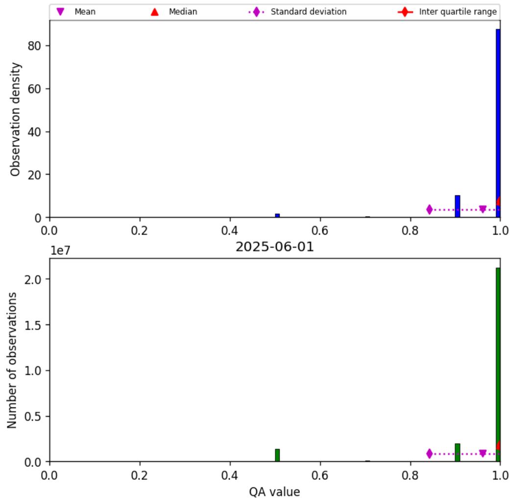
Figure 29: Histogram of “QA value” for 2025-06-01 to 2025-06-02
