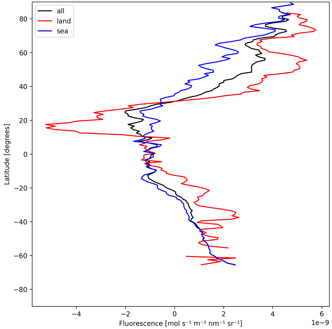
Figure 23: Zonal average of “Fluorescence” for 2025-06-01 to 2025-06-02.
