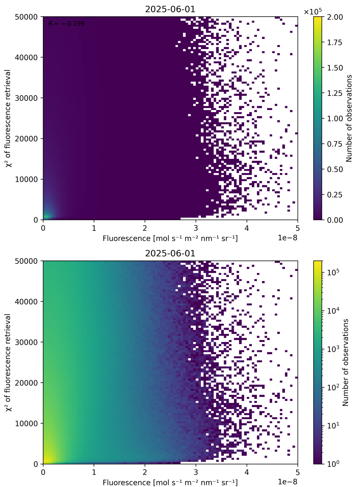
Figure 85: Scatter density plot of “Fluorescence” against “ \chi^2 of fluorescence retrieval” for 2025-06-01 to 2025-06-02.
