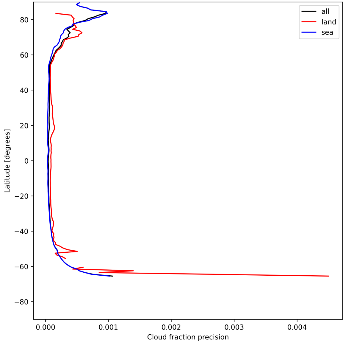
Figure 16: Zonal average of “Cloud fraction precision” for 2025-06-01 to 2025-06-02.
