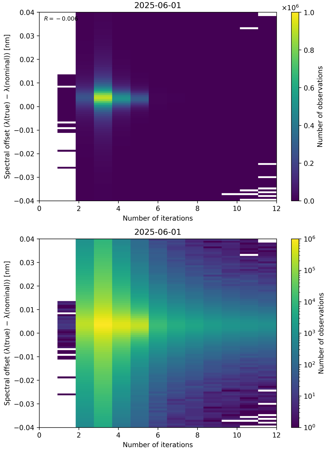
Figure 100: Scatter density plot of “Number of iterations” against “Spectral offset ( \lambda_{\text{true}} - \lambda_{\text{nominal}} )” for 2025-06-01 to 2025-06-02.
