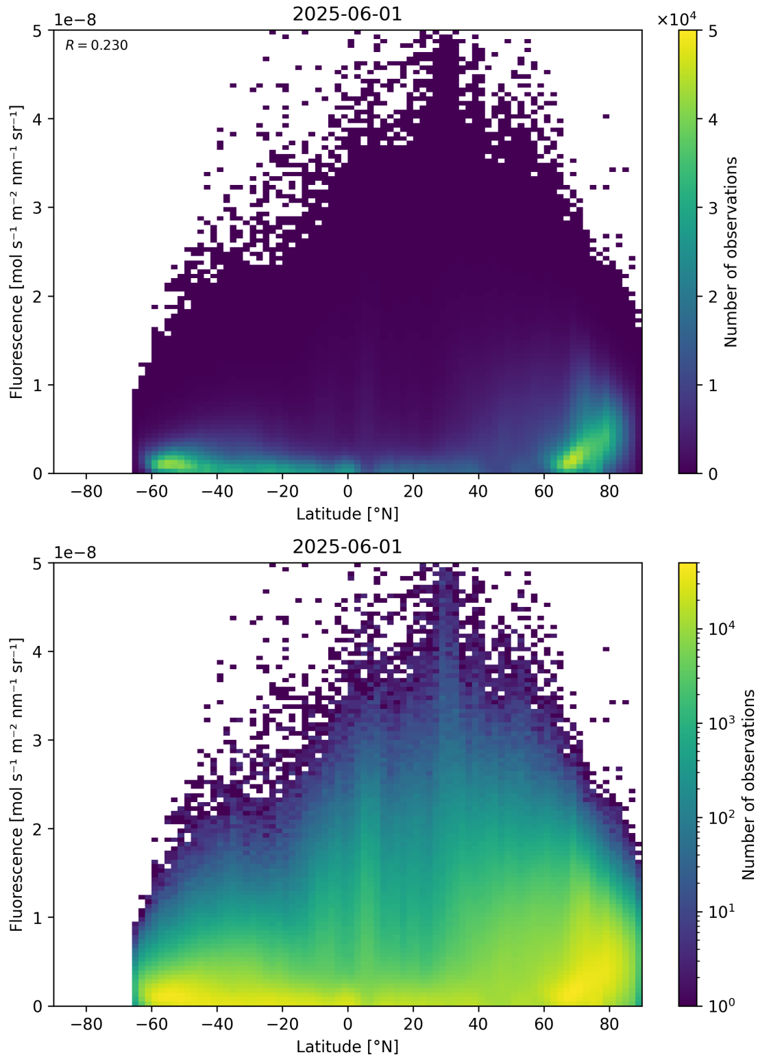
Figure 92: Scatter density plot of “Latitude” against “Fluorescence” for 2025-06-01 to 2025-06-02.
