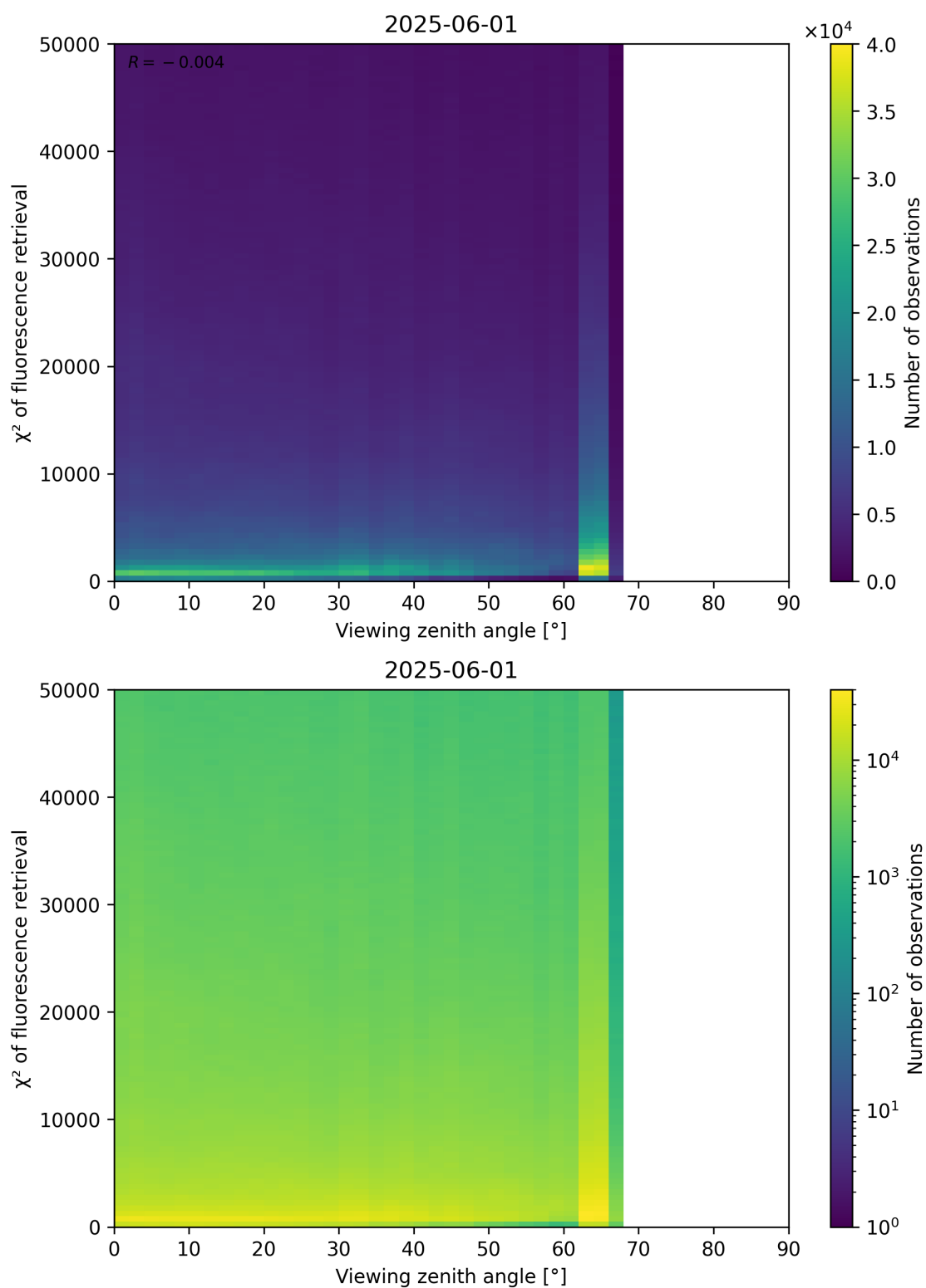
Figure 119: Scatter density plot of “Viewing zenith angle” against “ \chi^2 of fluorescence retrieval” for 2025-06-01 to 2025-06-02.
