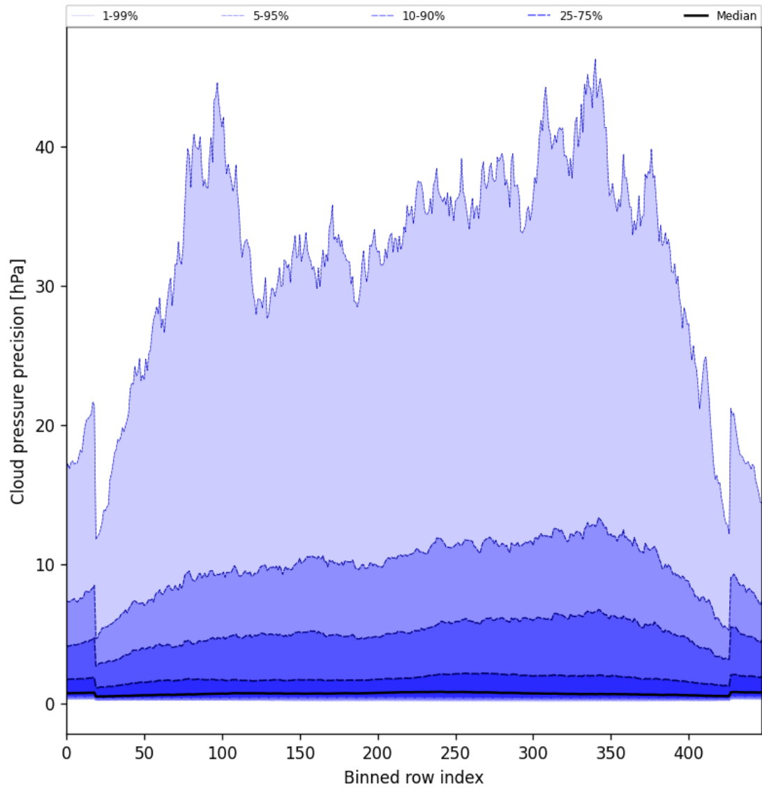
Figure 48: Along track statistics of “Cloud pressure precision” for 2025-06-01 to 2025-06-02
