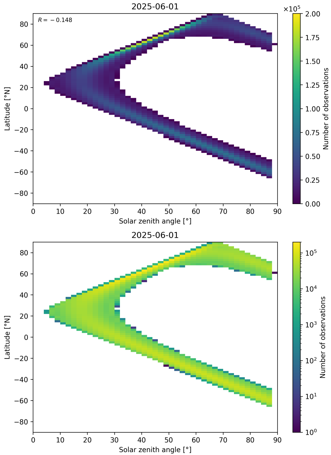
Figure 113: Scatter density plot of “Solar zenith angle” against “Latitude” for 2025-06-01 to 2025-06-02.
