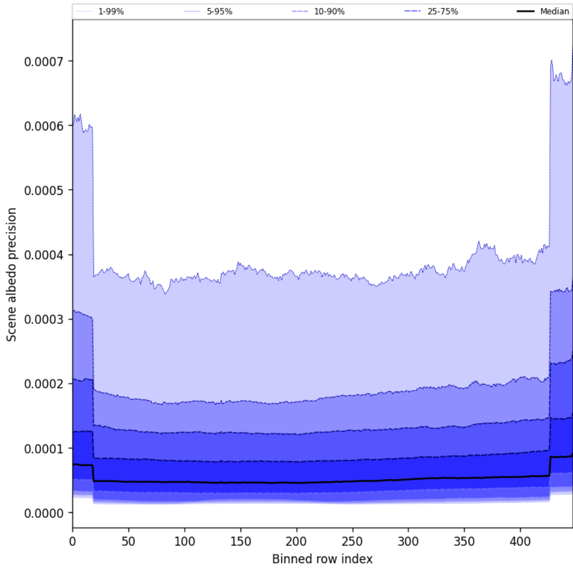
Figure 52: Along track statistics of “Scene albedo precision” for 2025-06-01 to 2025-06-02
