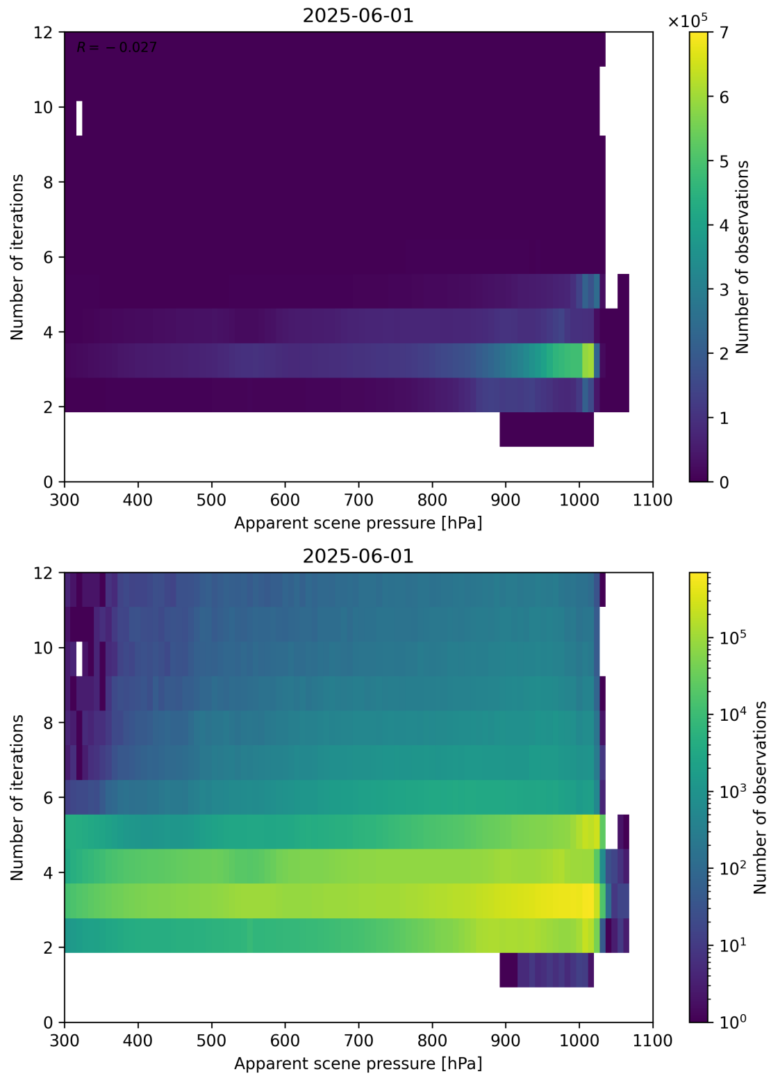
Figure 65: Scatter density plot of “Apparent scene pressure” against “Number of iterations” for 2025-06-01 to 2025-06-02.
