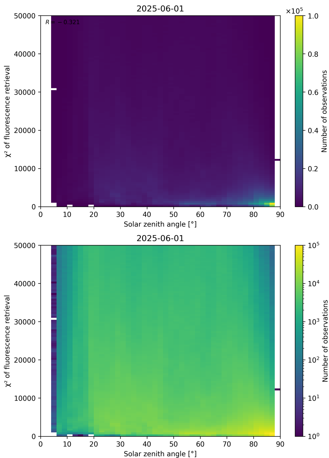
Figure 109: Scatter density plot of “Solar zenith angle” against “ \chi^2 of fluorescence retrieval” for 2025-06-01 to 2025-06-02.
