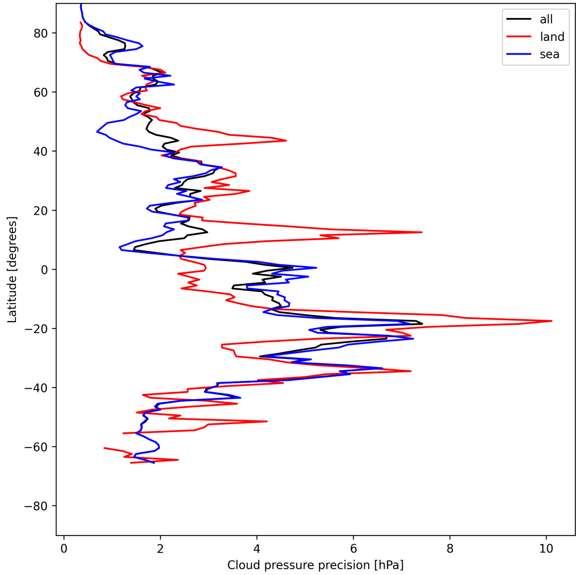
Figure 14: Zonal average of “Cloud pressure precision” for 2025-06-01 to 2025-06-02.
