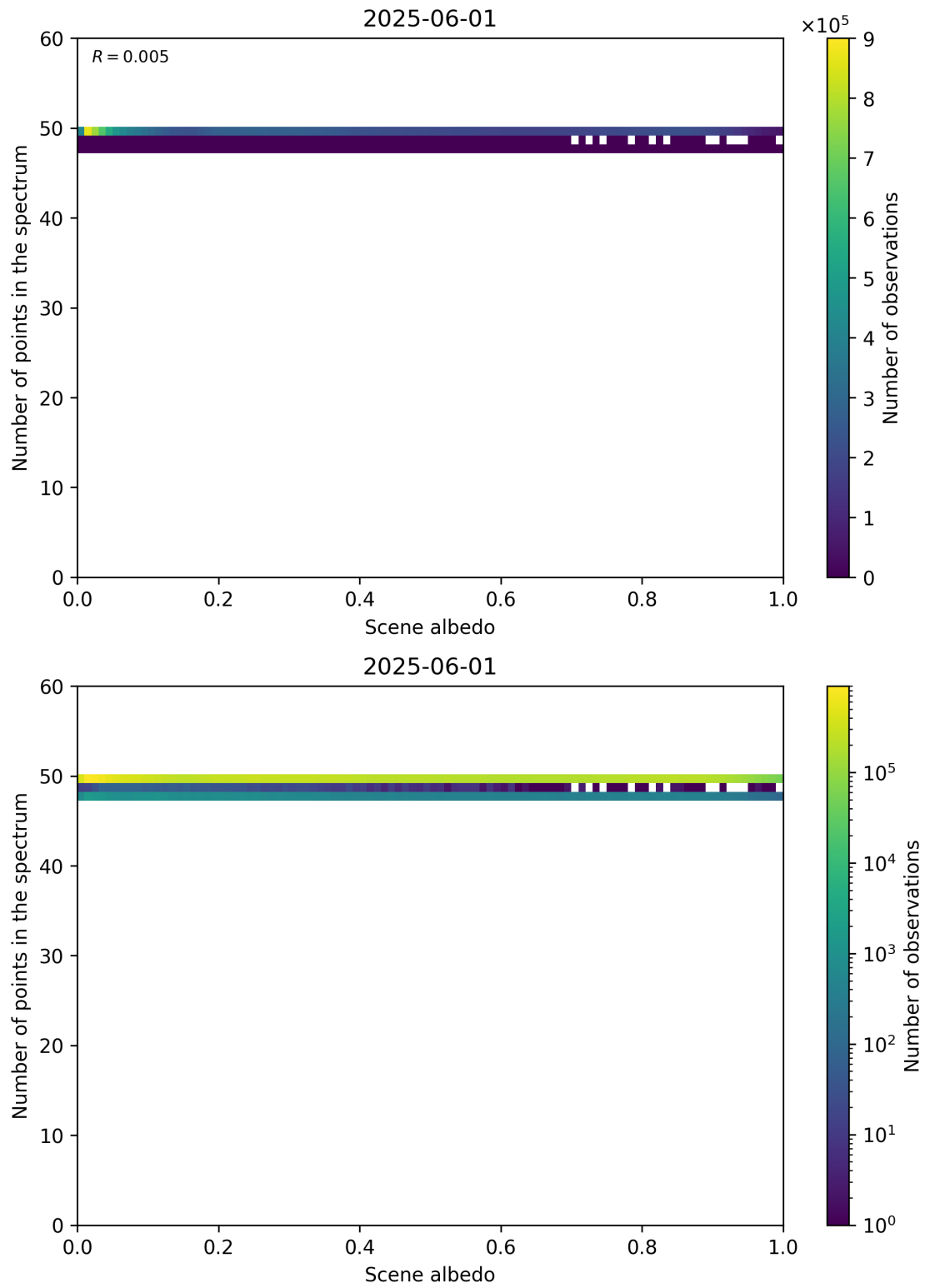
Figure 106: Scatter density plot of “Scene albedo” against “Number of points in the spectrum” for 2025-06-01 to 2025-06-02.
