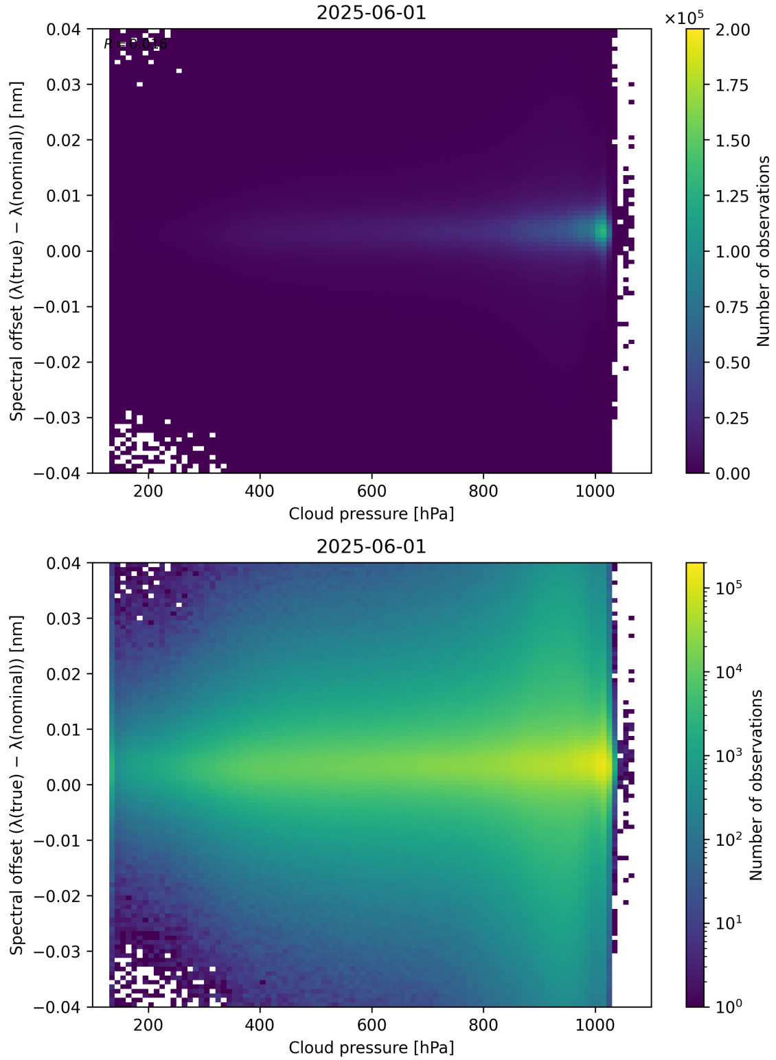
Figure 84: Scatter density plot of “Cloud pressure” against “Spectral offset ( \lambda_{\text{true}} - \lambda_{\text{nominal}} )” for 2025-06-01 to 2025-06-02.
