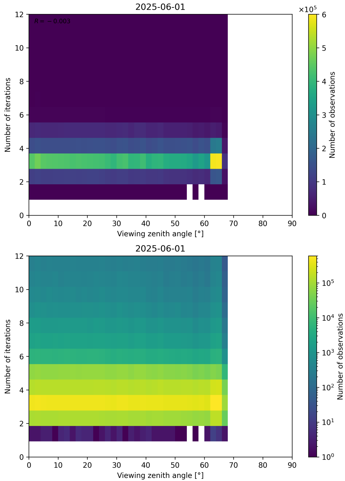
Figure 124: Scatter density plot of “Viewing zenith angle” against “Number of iterations” for 2025-06-01 to 2025-06-02.
