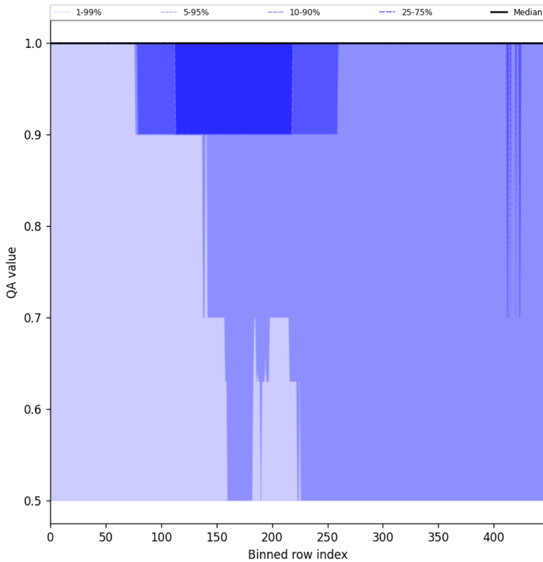
Figure 46: Along track statistics of “QA value” for 2025-06-01 to 2025-06-02
