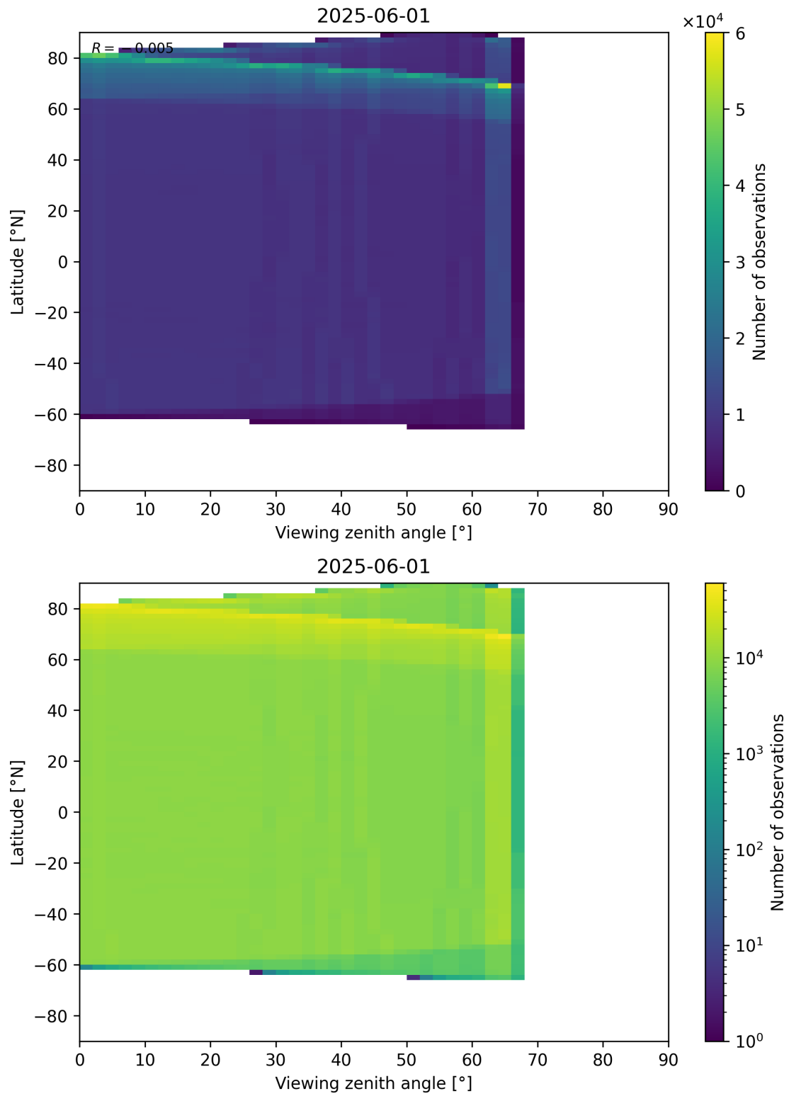
Figure 123: Scatter density plot of “Viewing zenith angle” against “Latitude” for 2025-06-01 to 2025-06-02.
