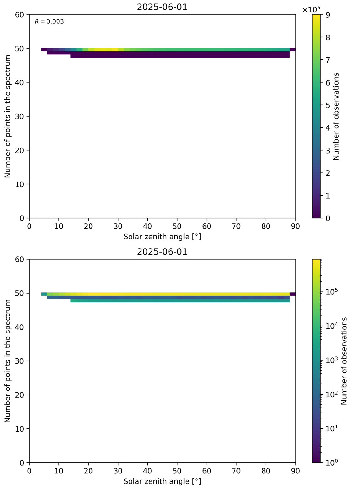
Figure 115: Scatter density plot of “Solar zenith angle” against “Number of points in the spectrum” for 2025-06-01 to 2025-06-02.
