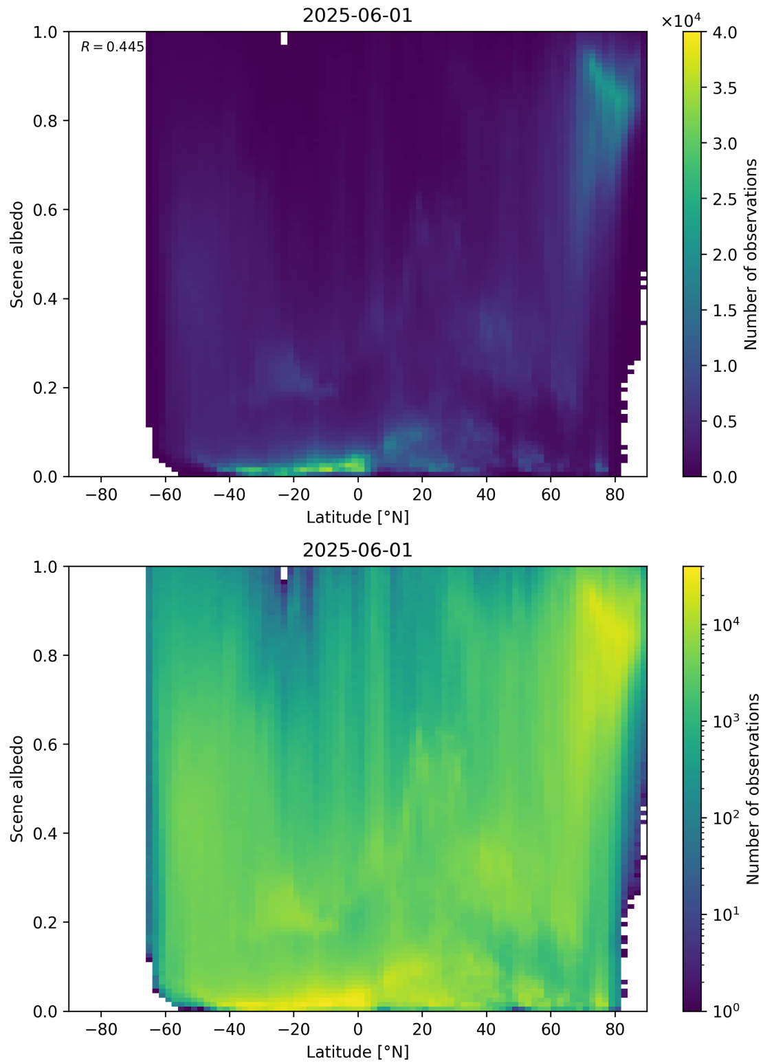
Figure 95: Scatter density plot of “Latitude” against “Scene albedo” for 2025-06-01 to 2025-06-02.
