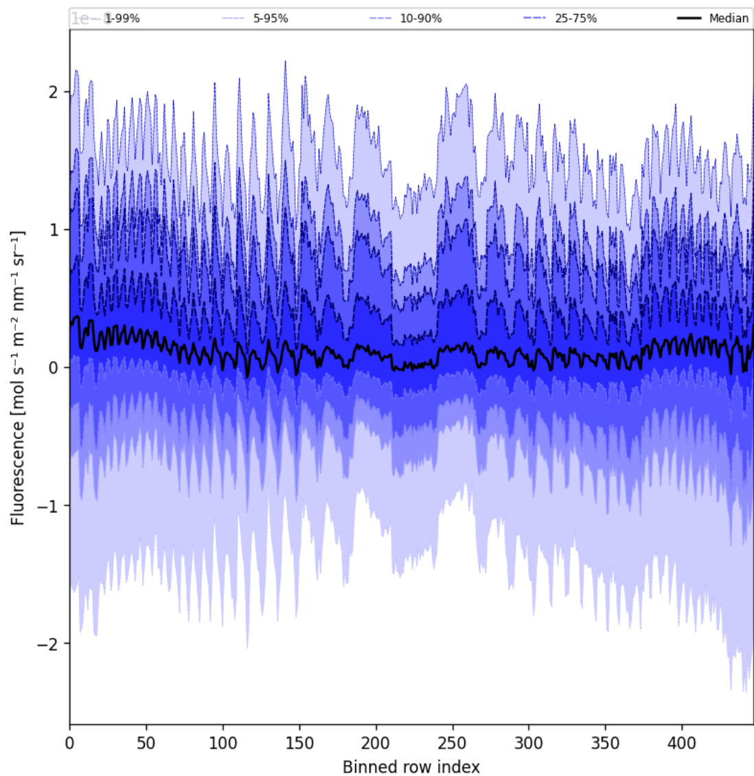
Figure 57: Along track statistics of “Fluorescence” for 2025-06-01 to 2025-06-02
