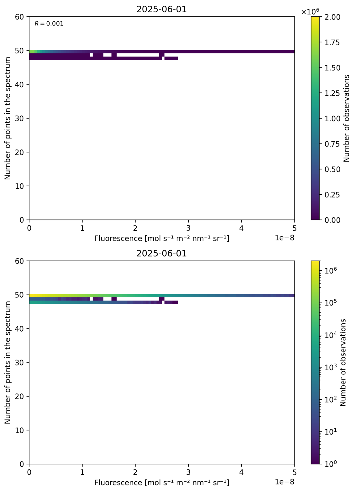
Figure 86: Scatter density plot of “Fluorescence” against “Number of points in the spectrum” for 2025-06-01 to 2025-06-02.
