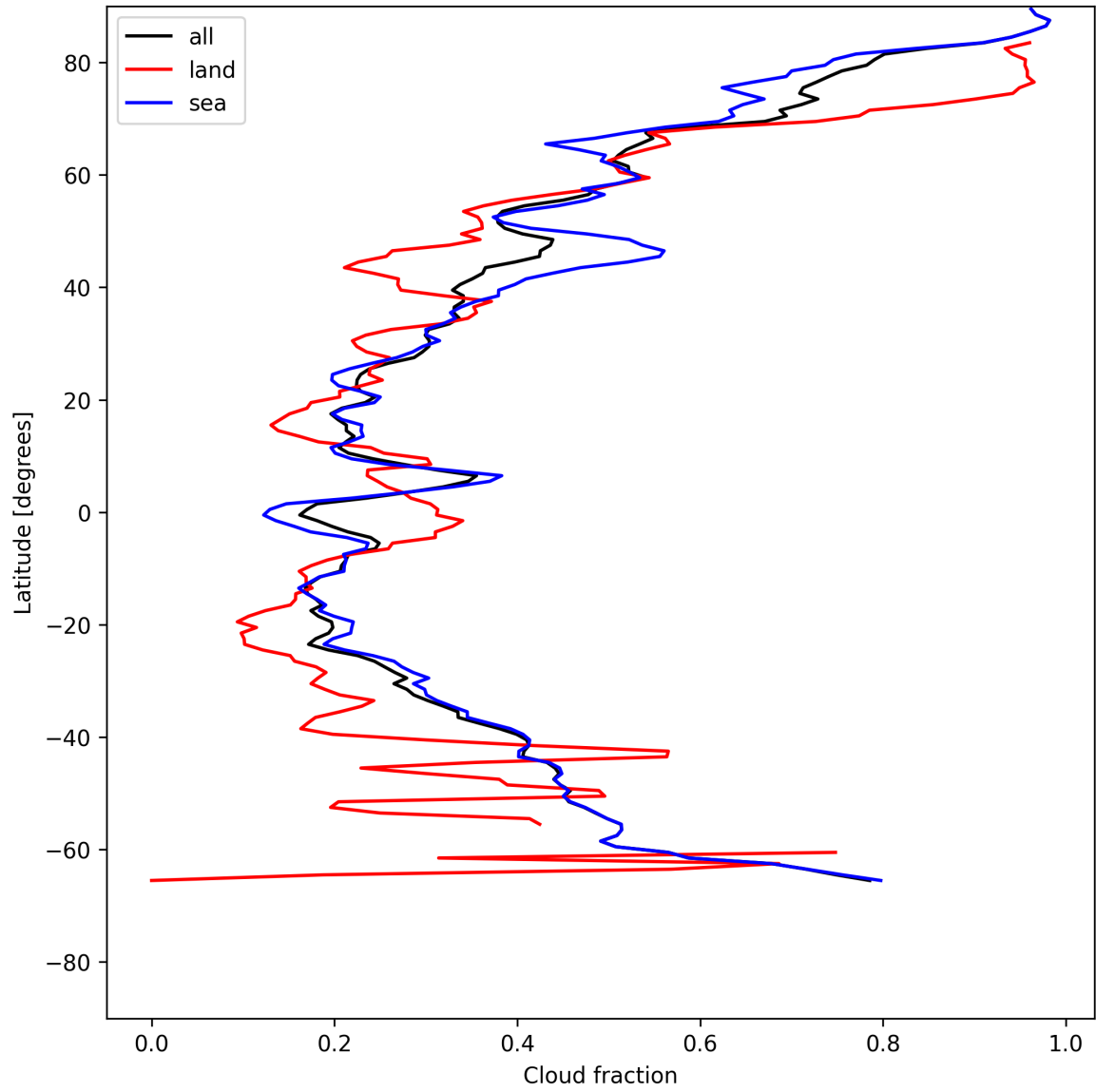
Figure 15: Zonal average of “Cloud fraction” for 2025-06-01 to 2025-06-02.
