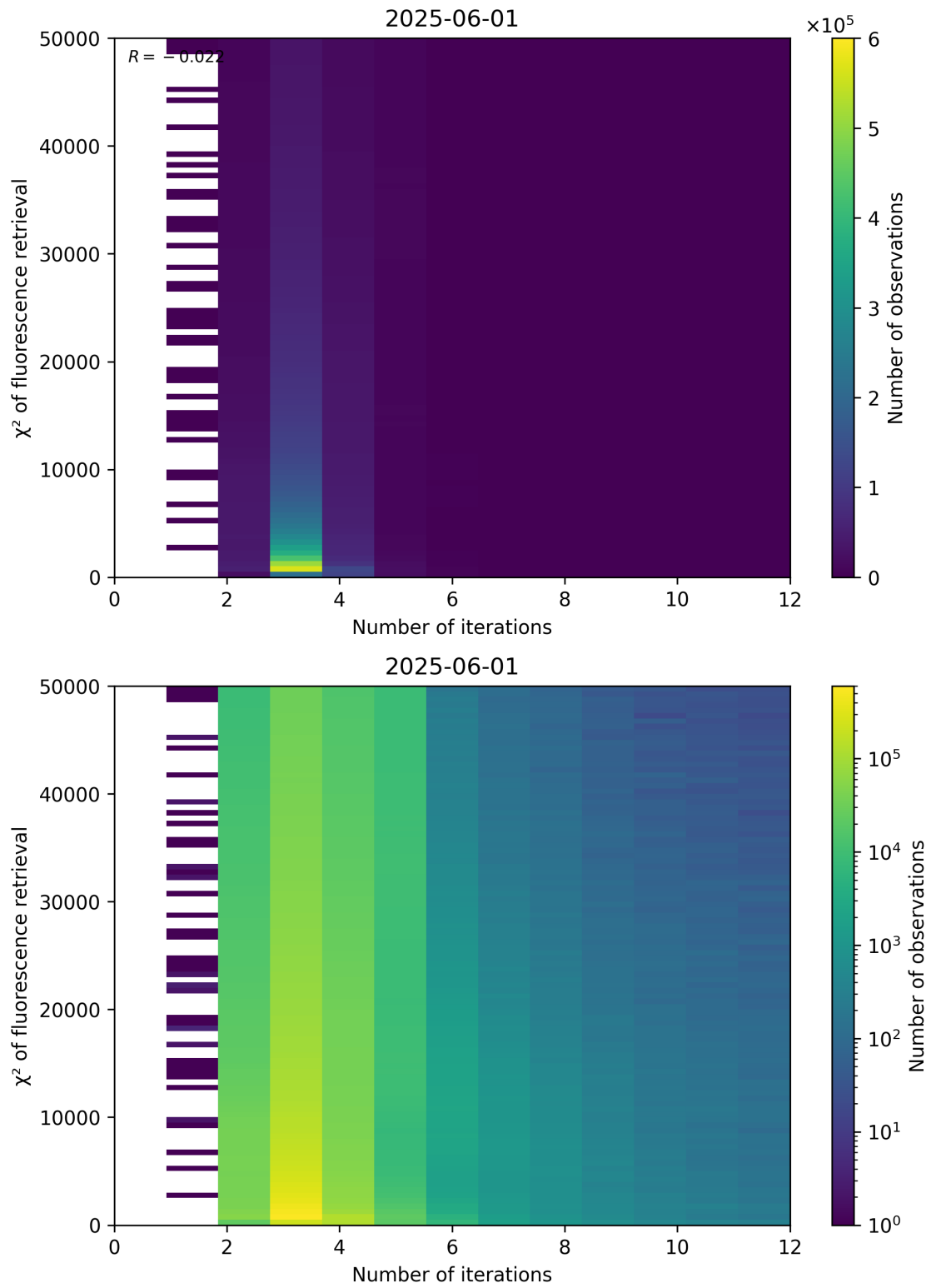
Figure 97: Scatter density plot of “Number of iterations” against “ \chi^2 of fluorescence retrieval” for 2025-06-01 to 2025-06-02.
