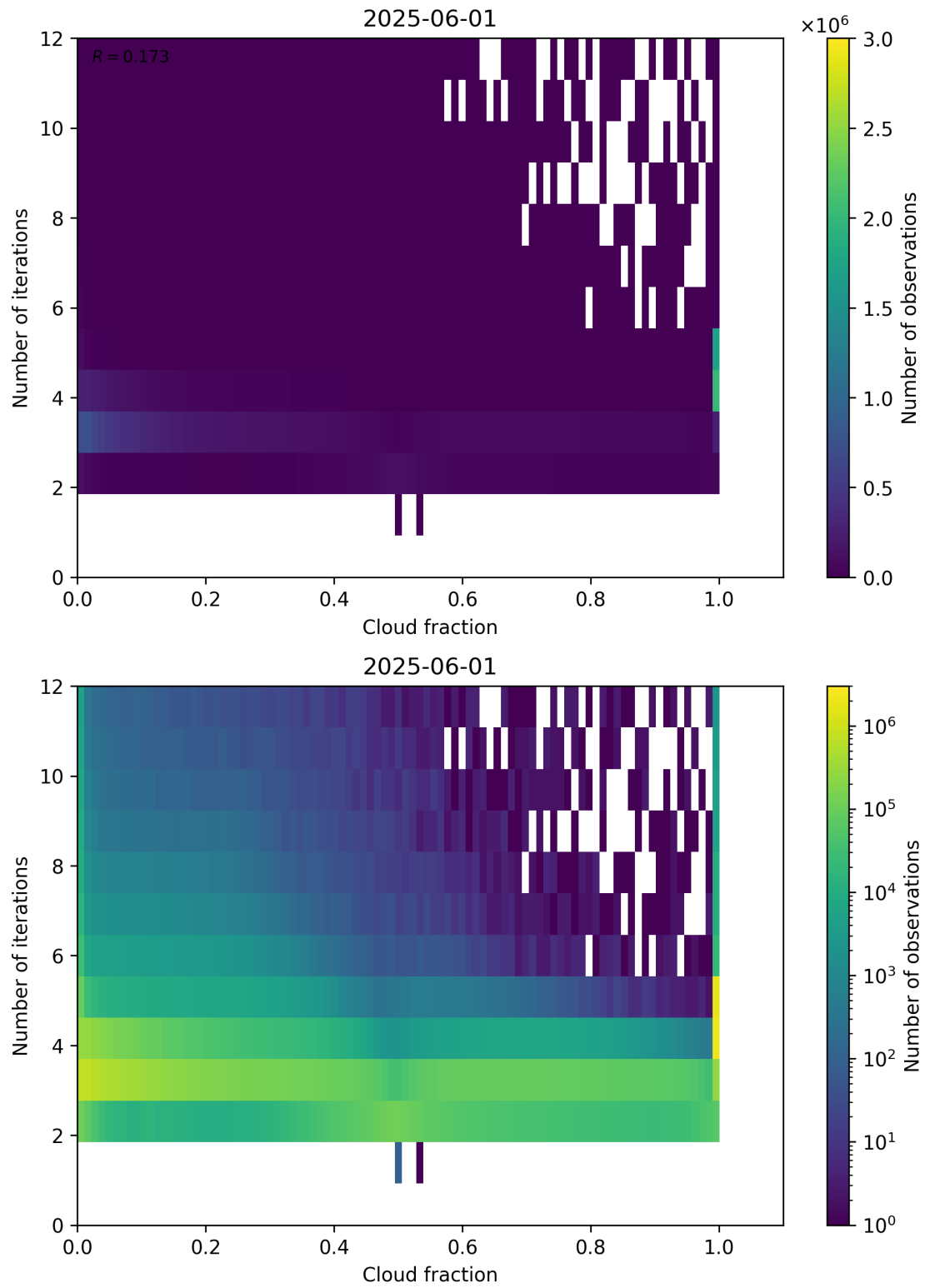
Figure 73: Scatter density plot of “Cloud fraction” against “Number of iterations” for 2025-06-01 to 2025-06-02.
