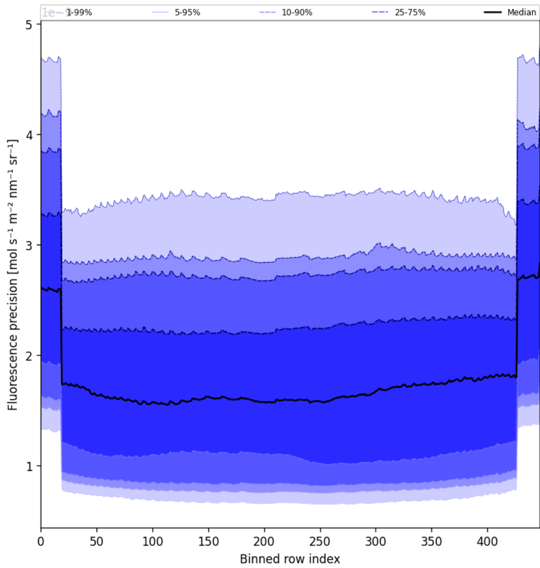
Figure 58: Along track statistics of “Fluorescence precision” for 2025-06-01 to 2025-06-02
