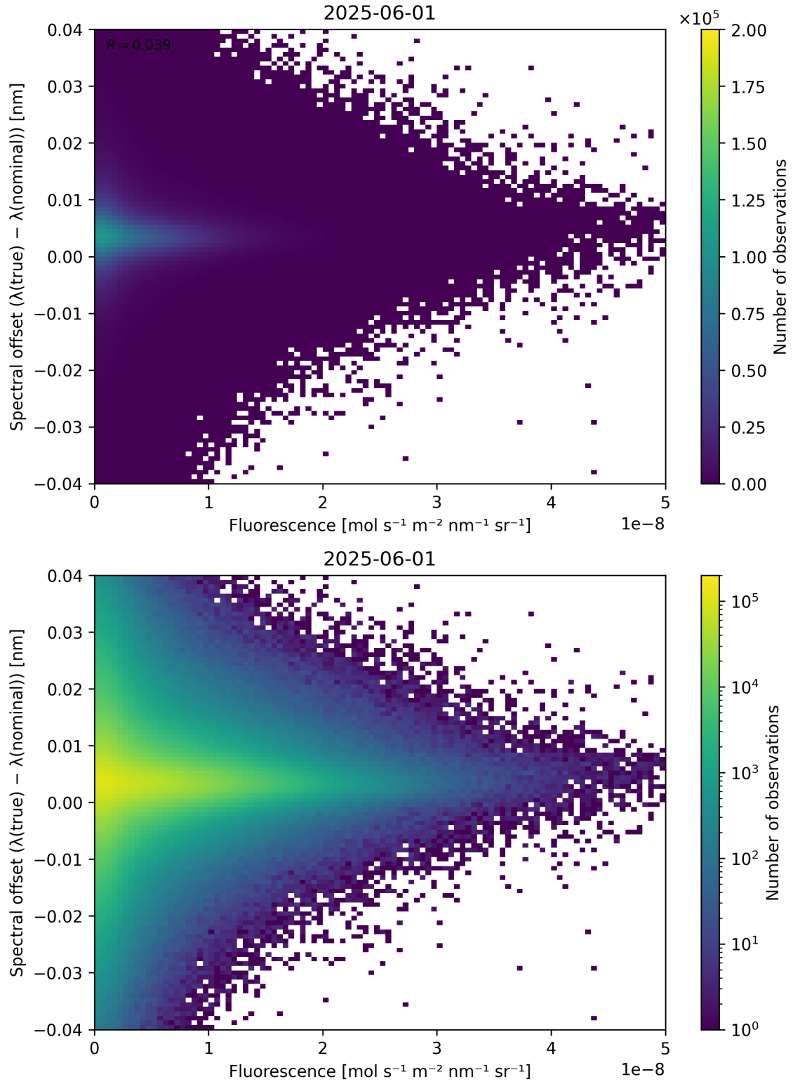
Figure 87: Scatter density plot of “Fluorescence” against “Spectral offset ( \lambda_{\text{true}} - \lambda_{\text{nominal}} )” for 2025-06-01 to 2025-06-02.
