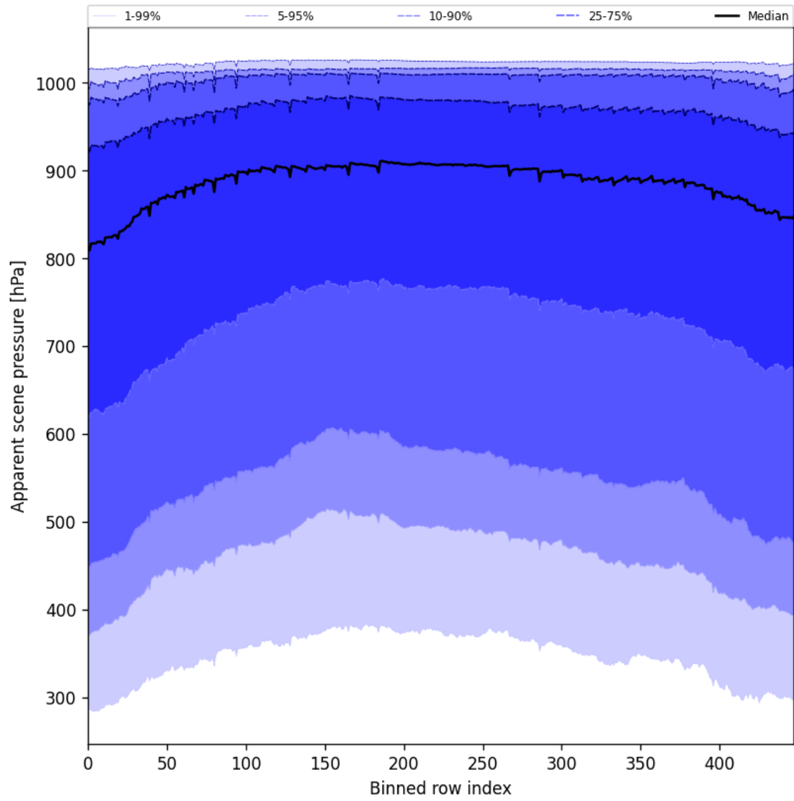
Figure 53: Along track statistics of “Apparent scene pressure” for 2025-06-01 to 2025-06-02
