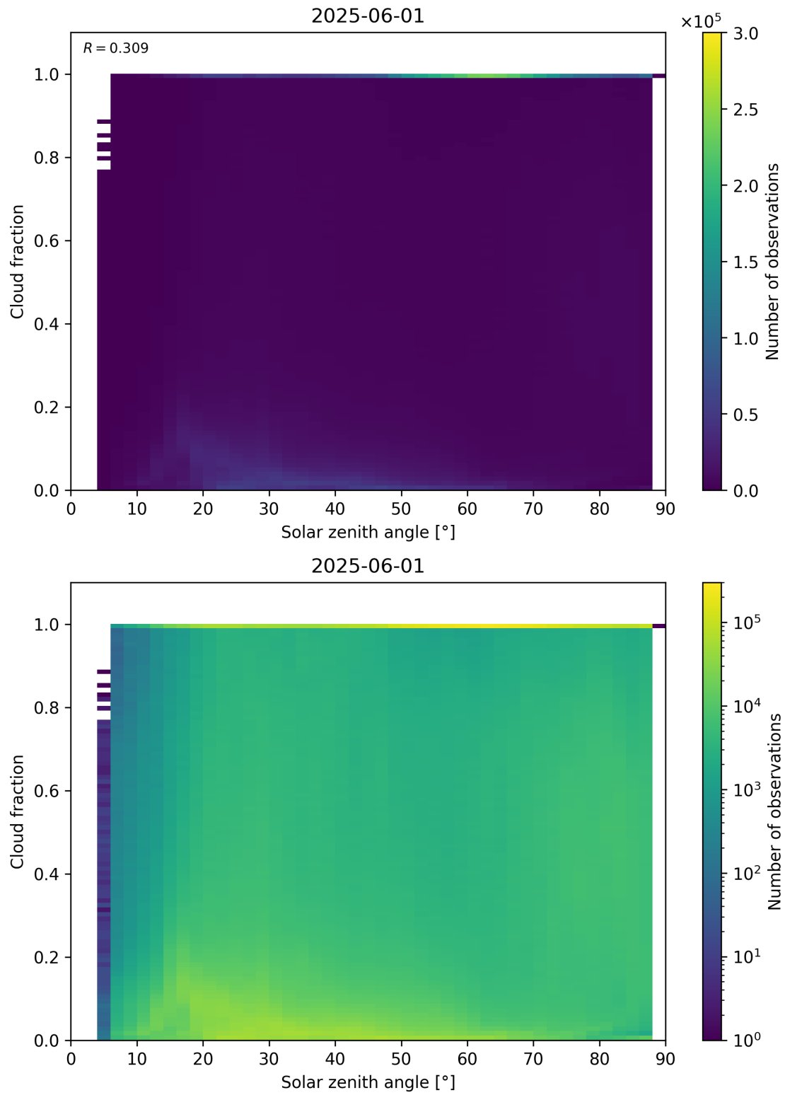
Figure 110: Scatter density plot of “Solar zenith angle” against “Cloud fraction” for 2025-06-01 to 2025-06-02.
