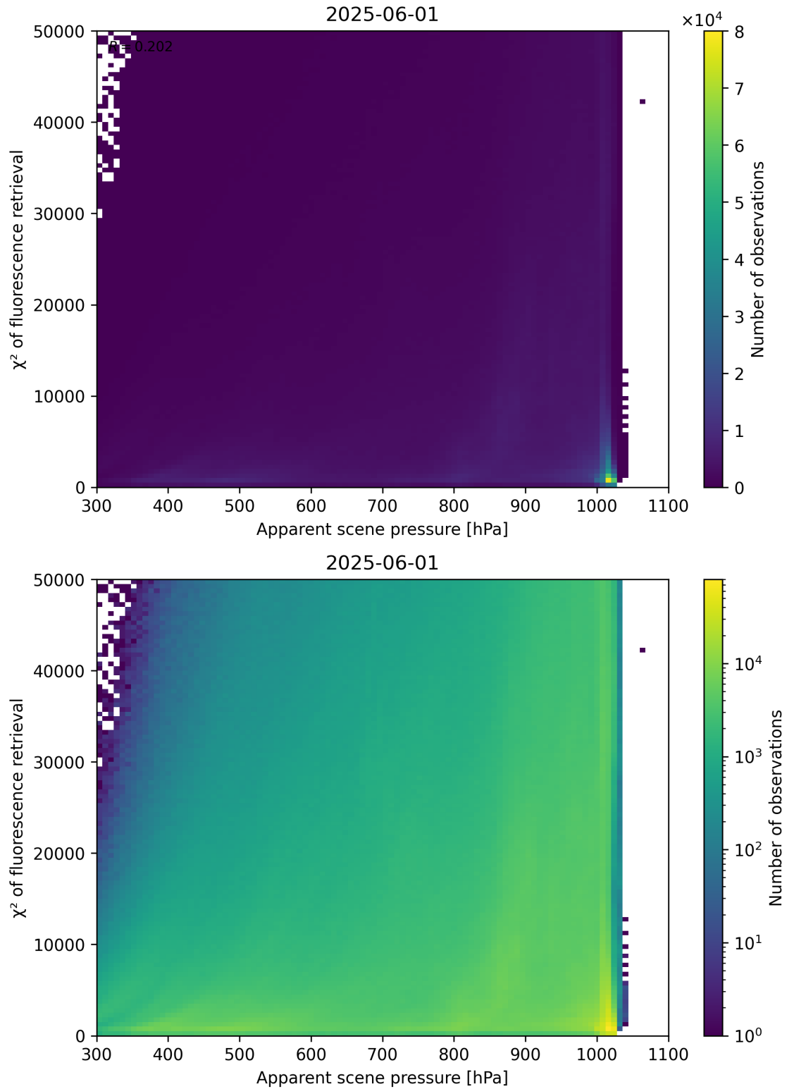
Figure 63: Scatter density plot of “Apparent scene pressure” against “ \chi^2 of fluorescence retrieval” for 2025-06-01 to 2025-06-02.
