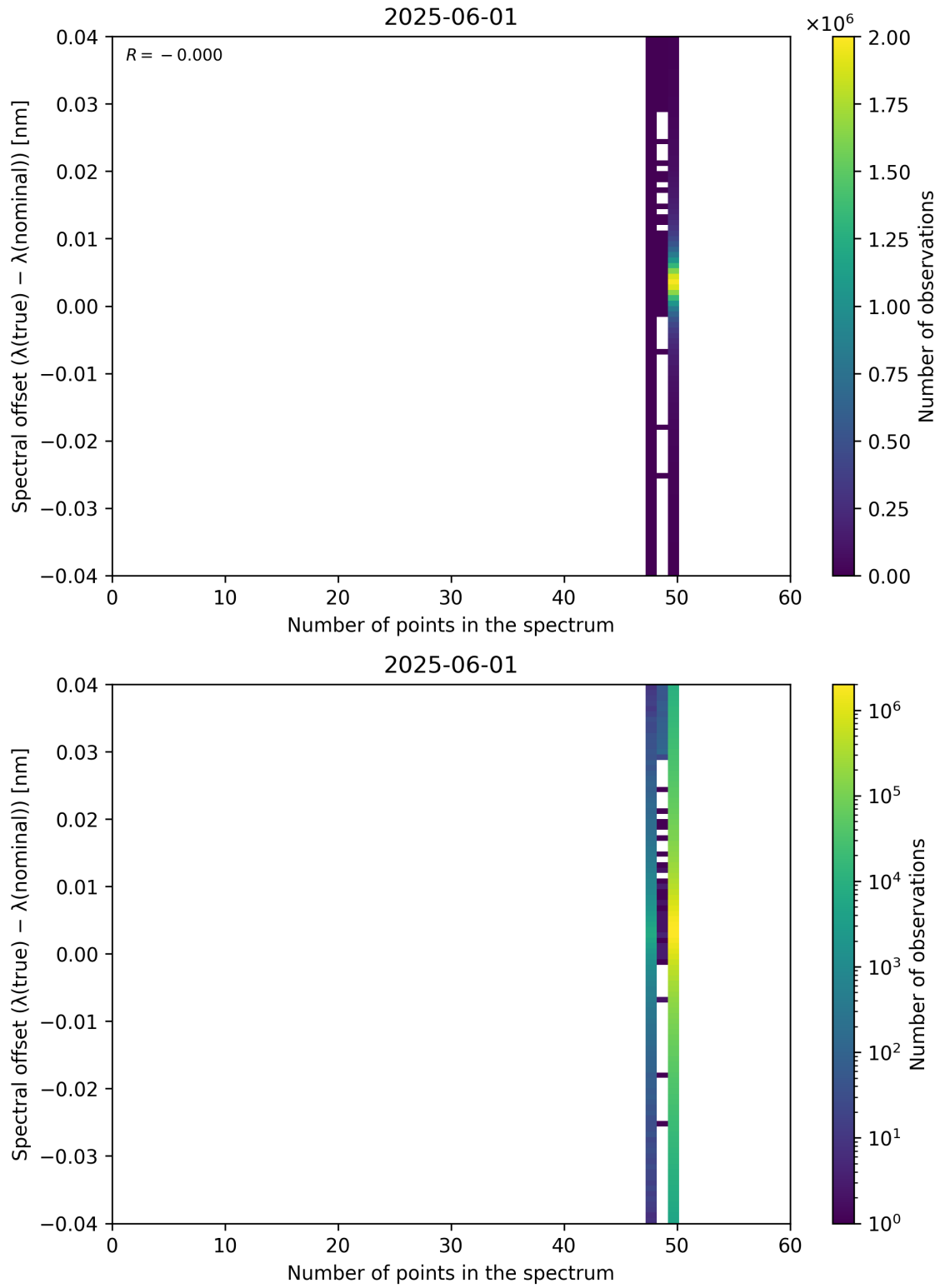
Figure 101: Scatter density plot of “Number of points in the spectrum” against “Spectral offset ( \lambda_{\text{true}} - \lambda_{\text{nominal}} )” for 2025-06-01 to 2025-06-02.
