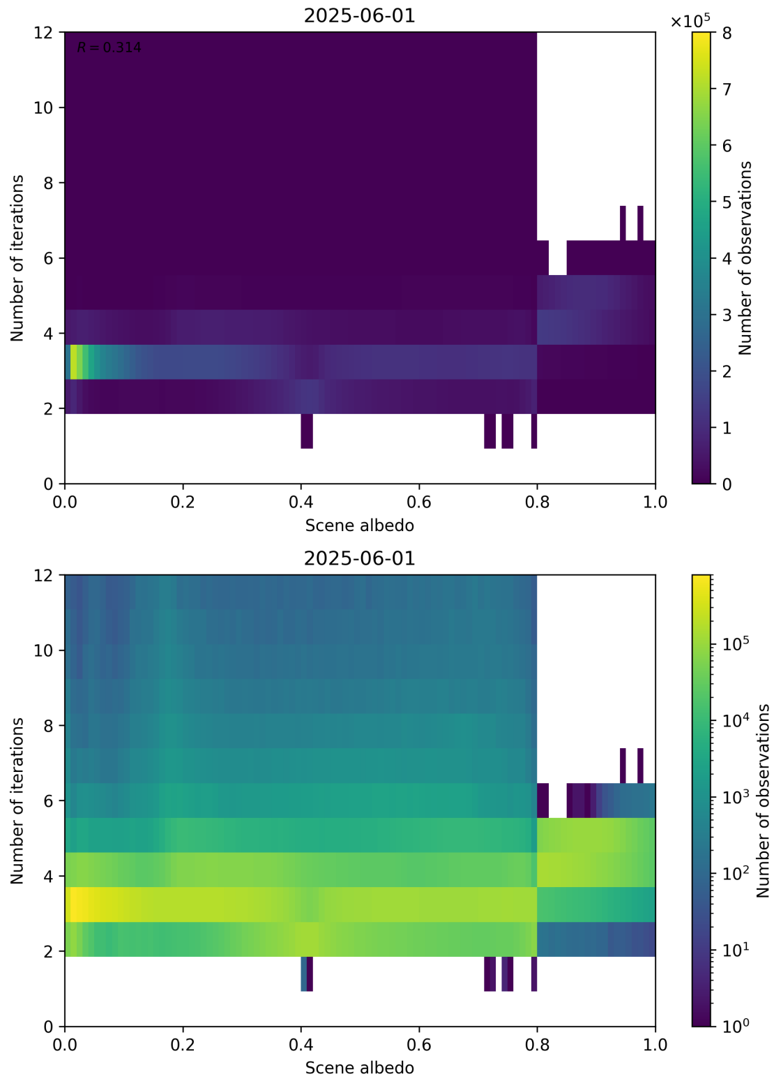
Figure 105: Scatter density plot of “Scene albedo” against “Number of iterations” for 2025-06-01 to 2025-06-02.
