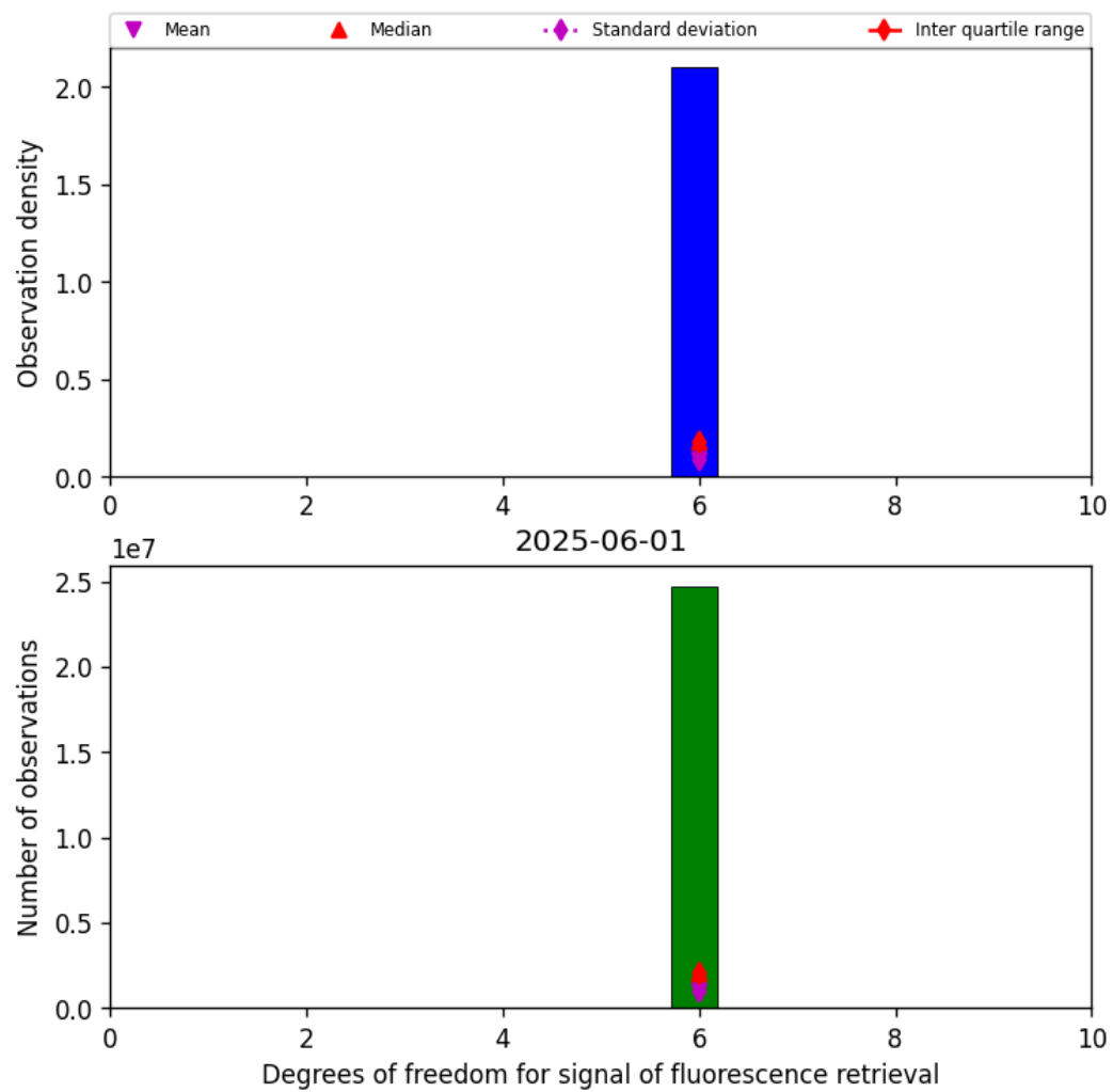
Figure 43: Histogram of “Degrees of freedom for signal of fluorescence retrieval” for 2025-06-01 to 2025-06-02
