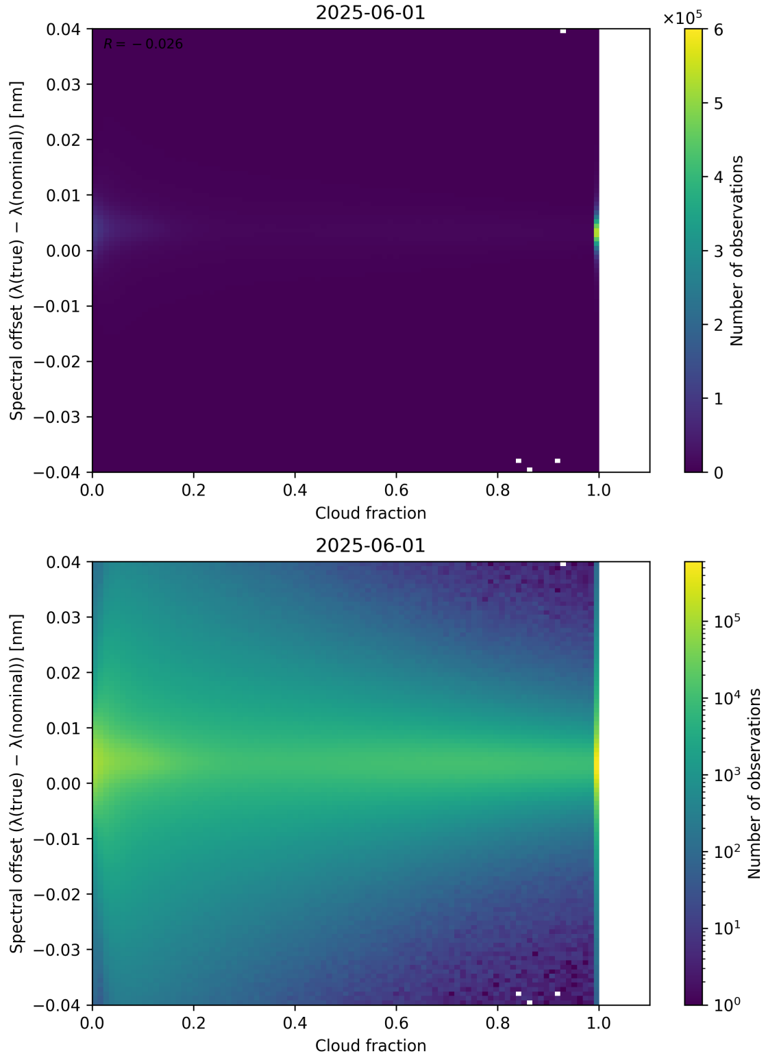
Figure 76: Scatter density plot of “Cloud fraction” against “Spectral offset ( \lambda_{\text{true}} - \lambda_{\text{nominal}} )” for 2025-06-01 to 2025-06-02.
