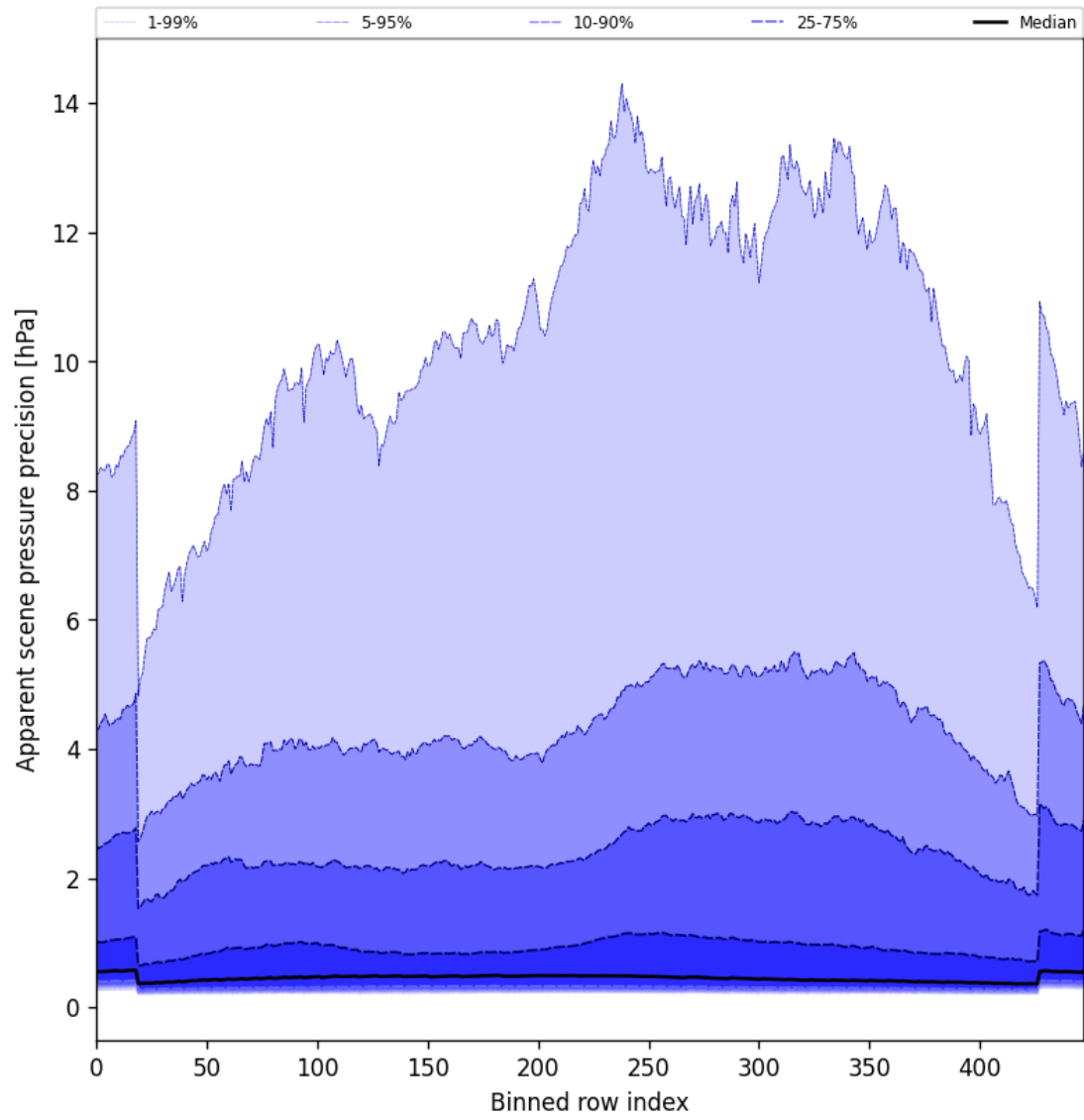
Figure 54: Along track statistics of “Apparent scene pressure precision” for 2025-06-01 to 2025-06-02
