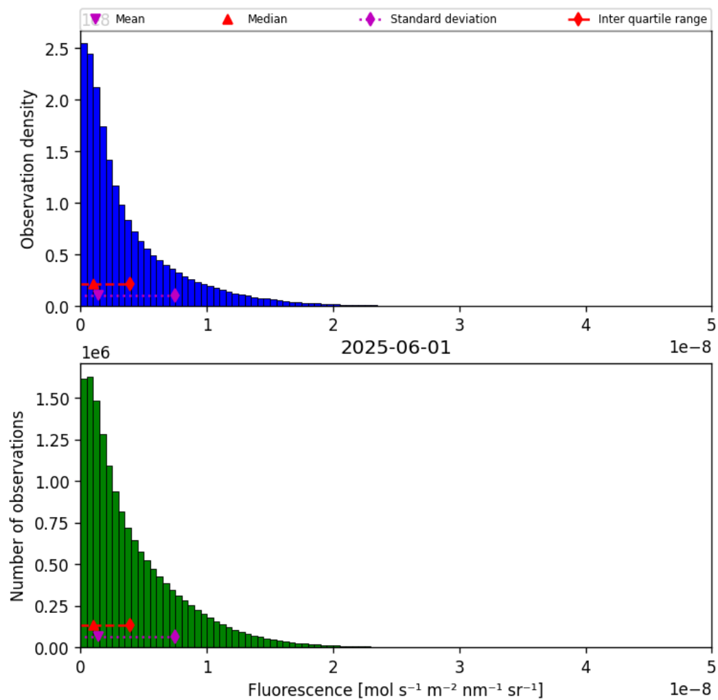
Figure 40: Histogram of “Fluorescence” for 2025-06-01 to 2025-06-02
