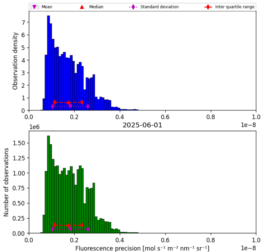
Figure 41: Histogram of “Fluorescence precision” for 2025-06-01 to 2025-06-02
