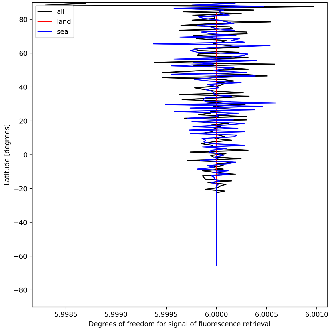
Figure 26: Zonal average of “Degrees of freedom for signal of fluorescence retrieval” for 2025-06-01 to 2025-06-02.
