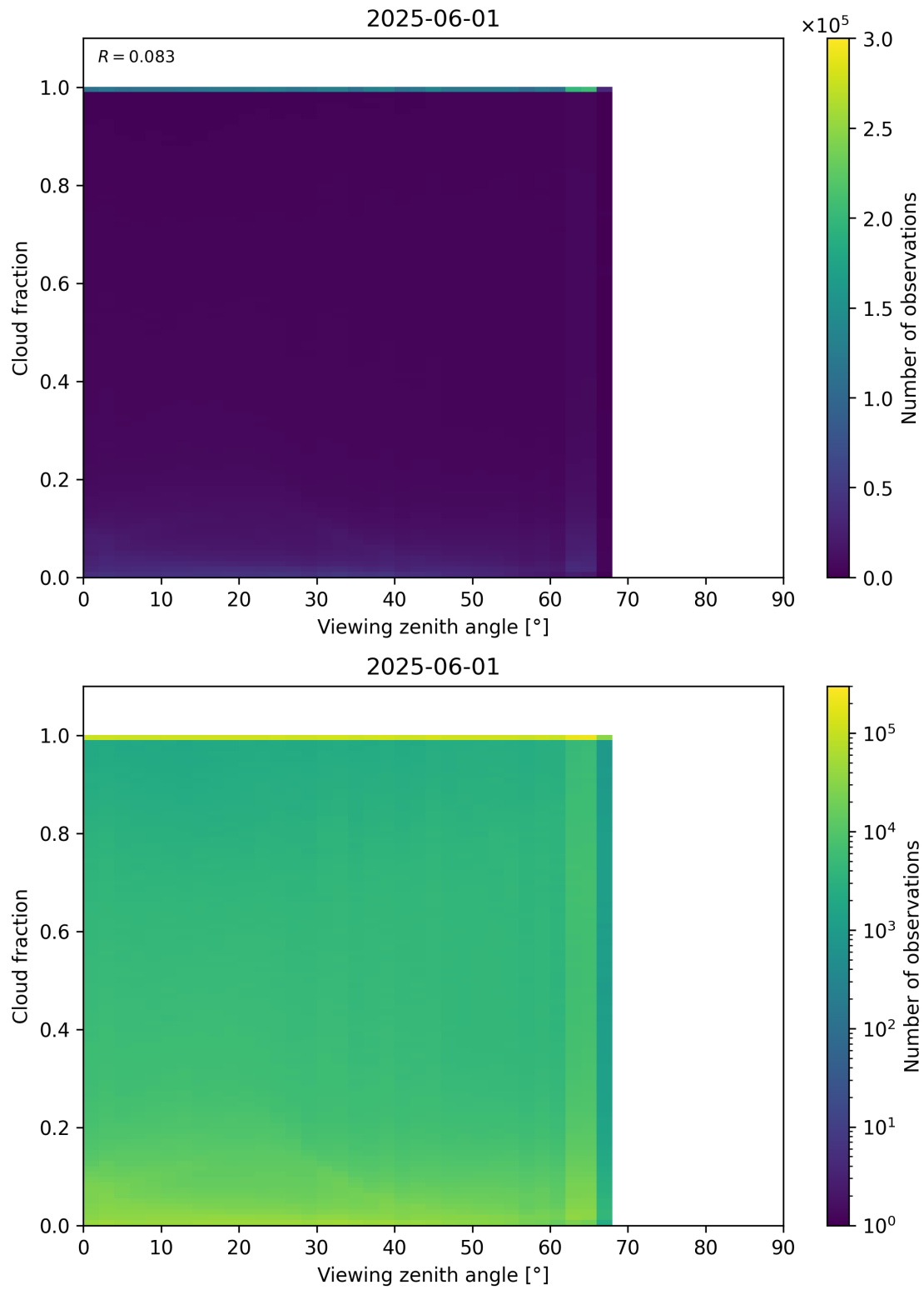
Figure 120: Scatter density plot of “Viewing zenith angle” against “Cloud fraction” for 2025-06-01 to 2025-06-02.
