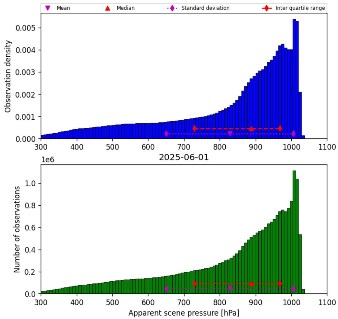
Figure 36: Histogram of “Apparent scene pressure” for 2025-06-01 to 2025-06-02
