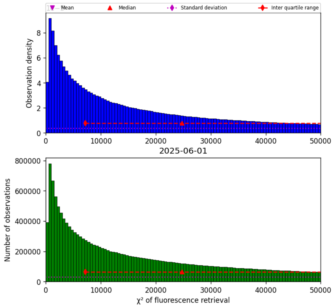
Figure 42: Histogram of “ \chi^2 of fluorescence retrieval” for 2025-06-01 to 2025-06-02
