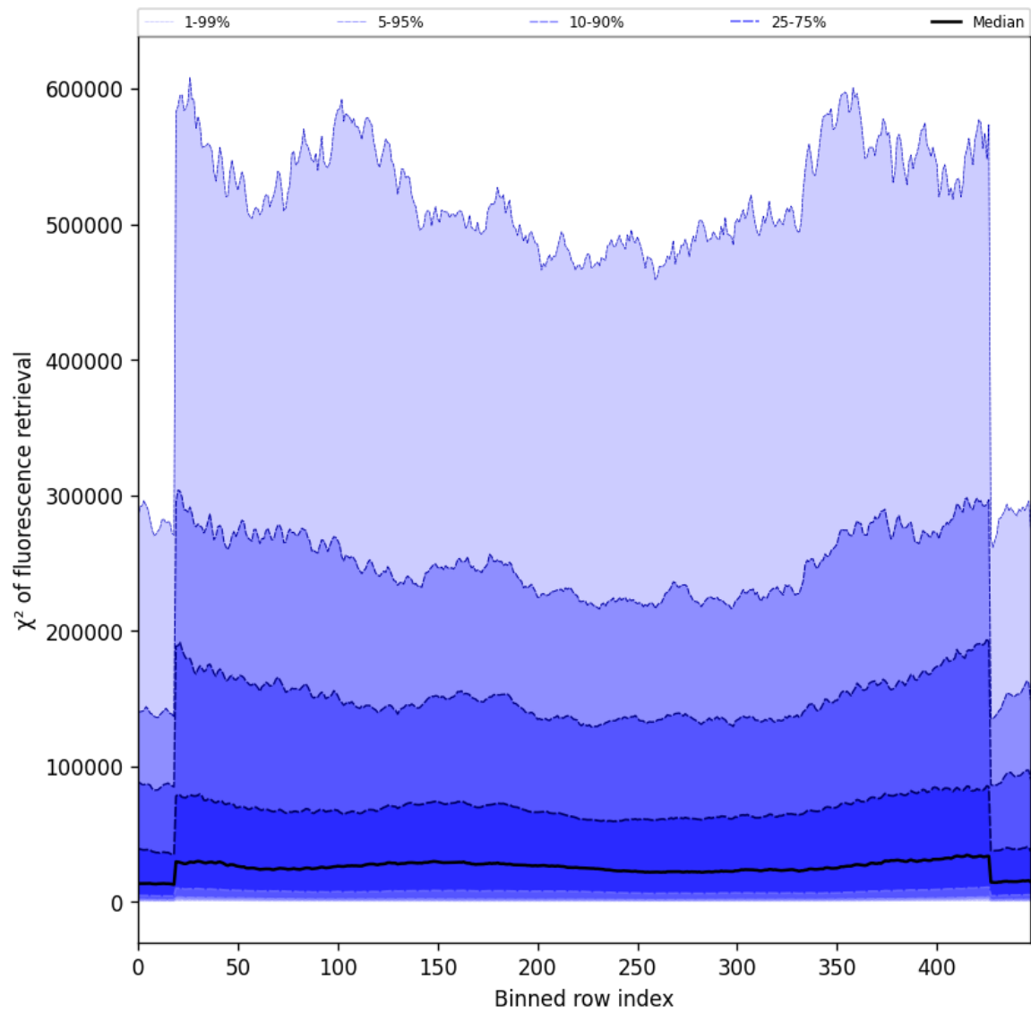
Figure 59: Along track statistics of “ \chi^2 of fluorescence retrieval” for 2025-06-01 to 2025-06-02
