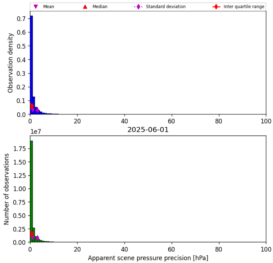
Figure 37: Histogram of "Apparent scene pressure precision" for 2025-06-01 to 2025-06-02
