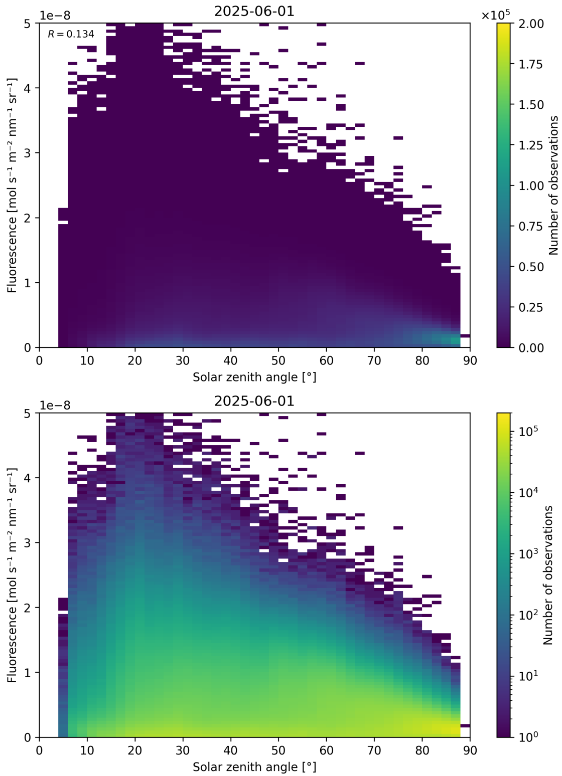
Figure 112: Scatter density plot of “Solar zenith angle” against “Fluorescence” for 2025-06-01 to 2025-06-02.
