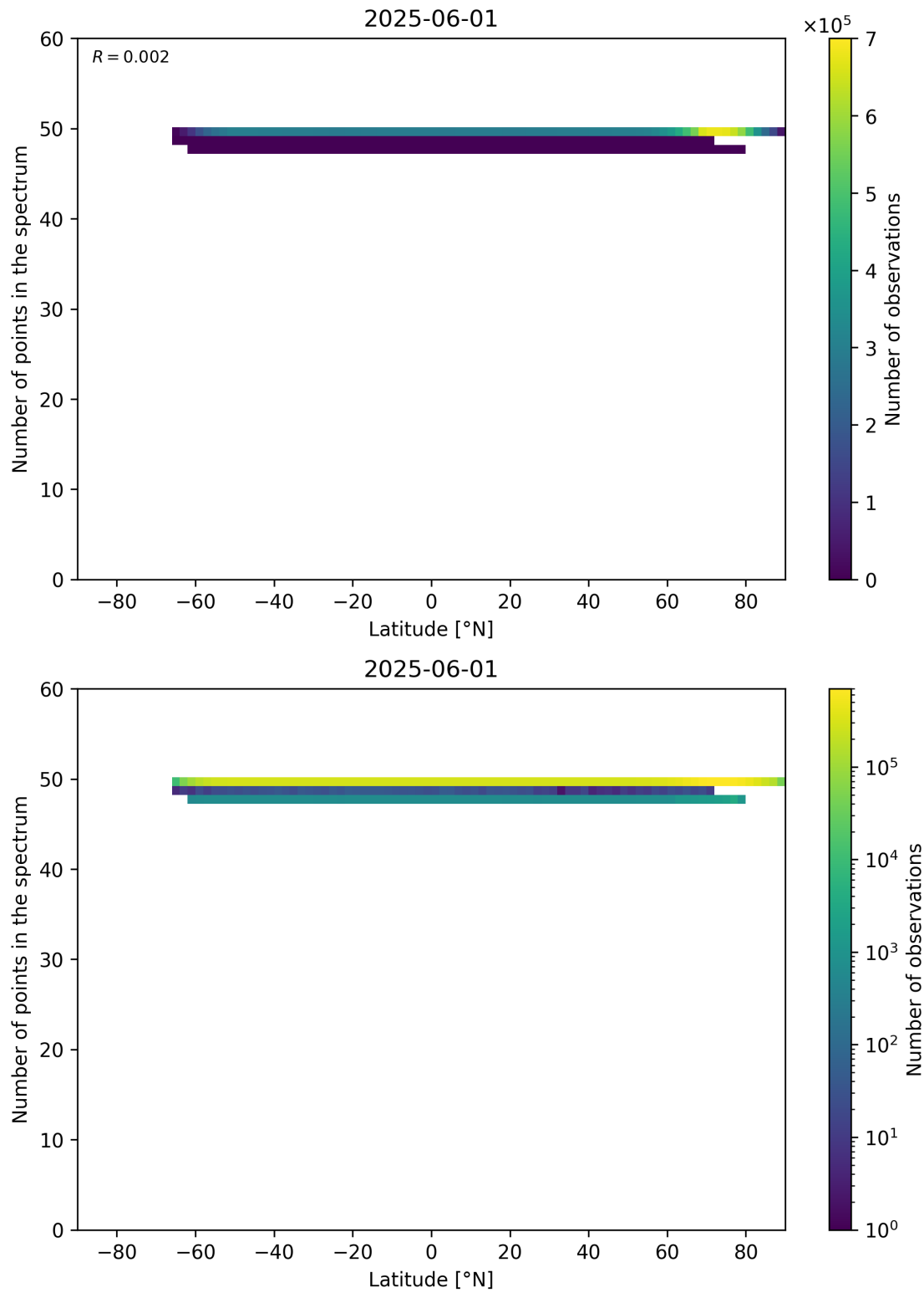
Figure 94: Scatter density plot of “Latitude” against “Number of points in the spectrum” for 2025-06-01 to 2025-06-02.
