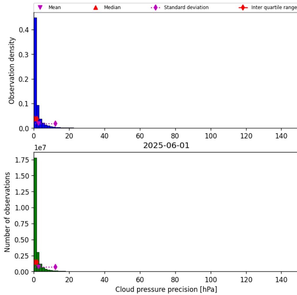
Figure 31: Histogram of "Cloud pressure precision" for 2025-06-01 to 2025-06-02
