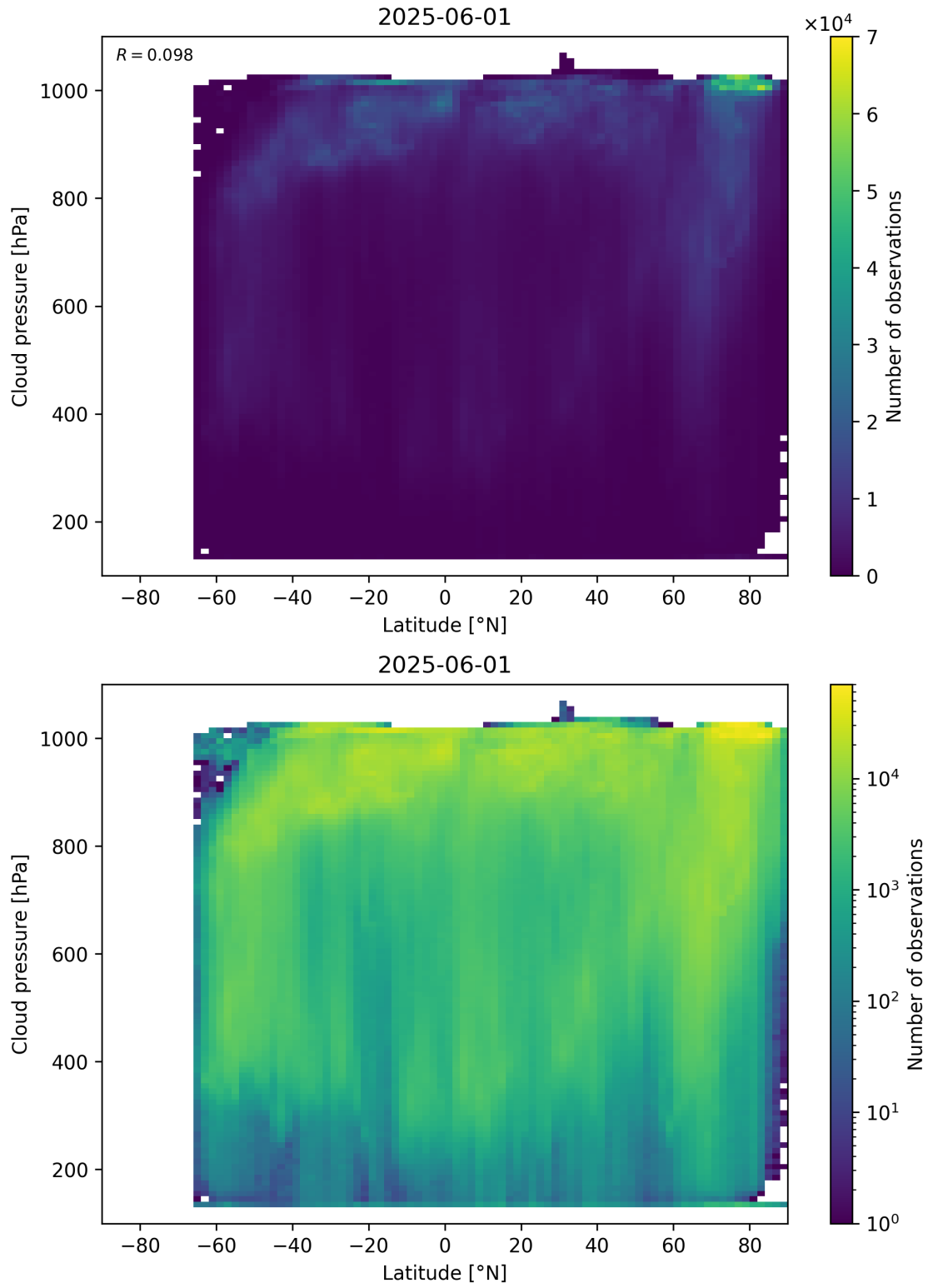
Figure 91: Scatter density plot of “Latitude” against “Cloud pressure” for 2025-06-01 to 2025-06-02.
