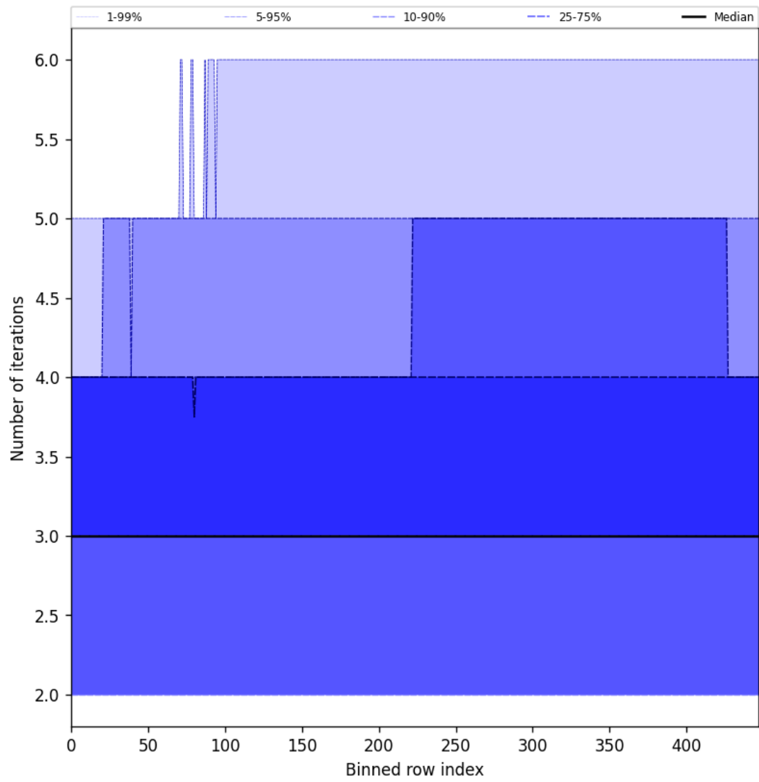
Figure 56: Along track statistics of “Number of iterations” for 2025-06-01 to 2025-06-02
