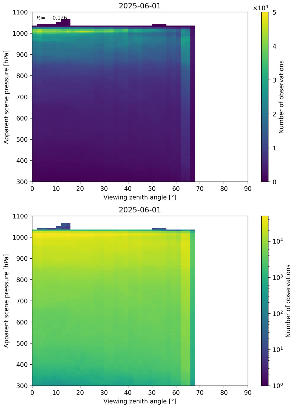
Figure 118: Scatter density plot of “Viewing zenith angle” against “Apparent scene pressure” for 2025-06-01 to 2025-06-02.
