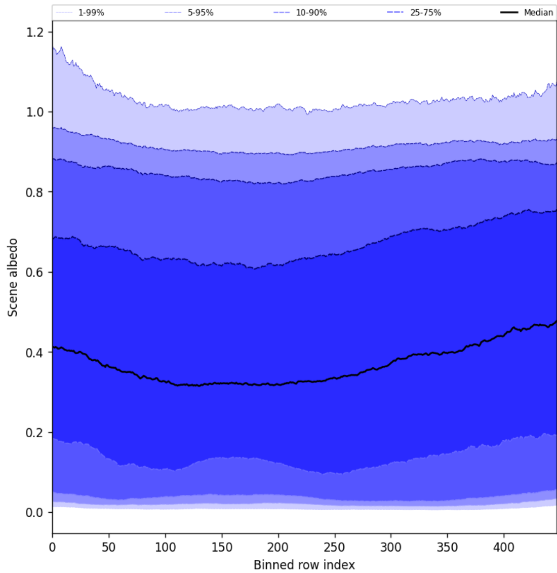
Figure 51: Along track statistics of “Scene albedo” for 2025-06-01 to 2025-06-02
