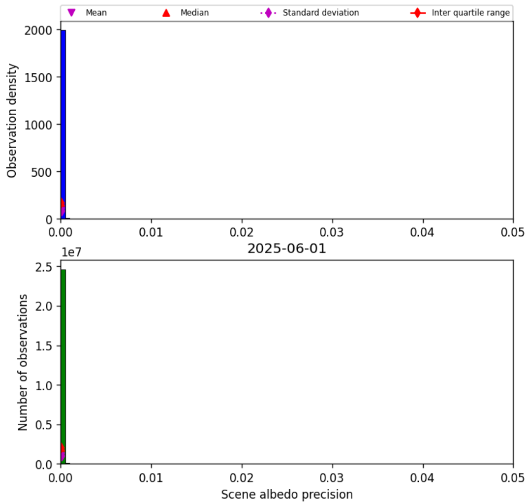
Figure 35: Histogram of “Scene albedo precision” for 2025-06-01 to 2025-06-02
