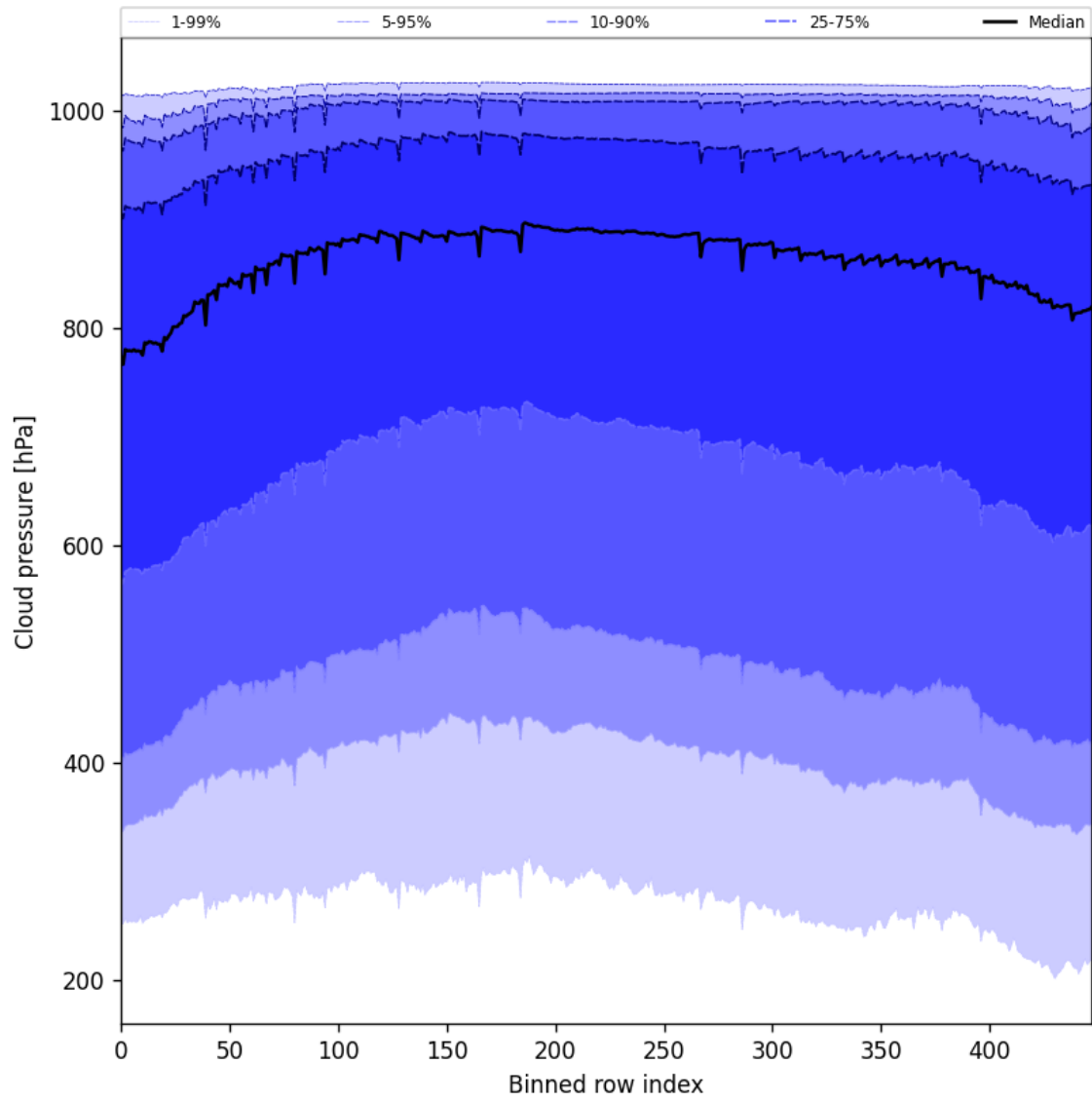
Figure 47: Along track statistics of “Cloud pressure” for 2025-06-01 to 2025-06-02
