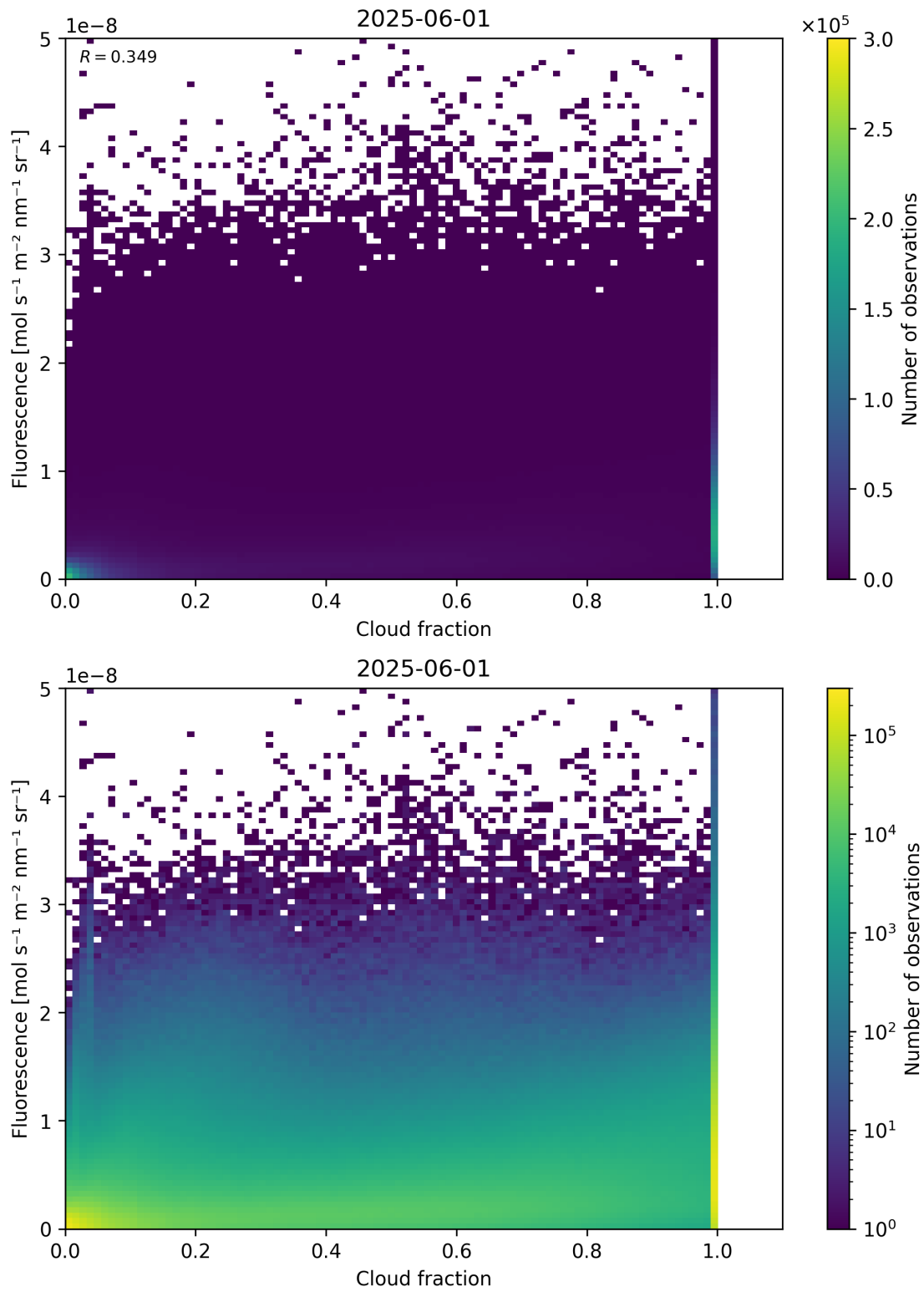
Figure 72: Scatter density plot of “Cloud fraction” against “Fluorescence” for 2025-06-01 to 2025-06-02.
