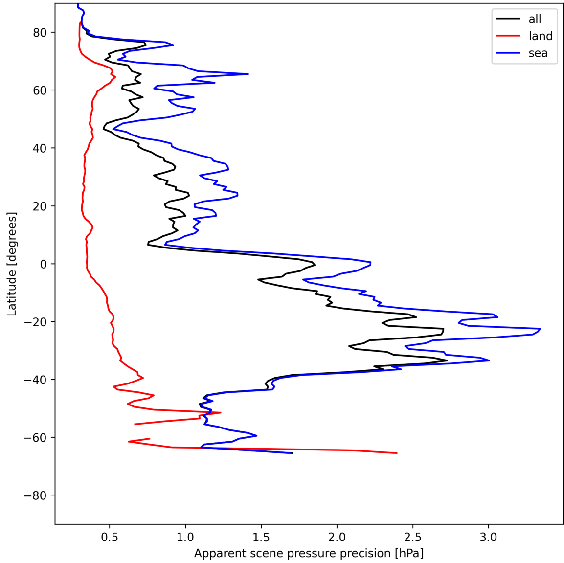
Figure 20: Zonal average of “Apparent scene pressure precision” for 2025-06-01 to 2025-06-02.
