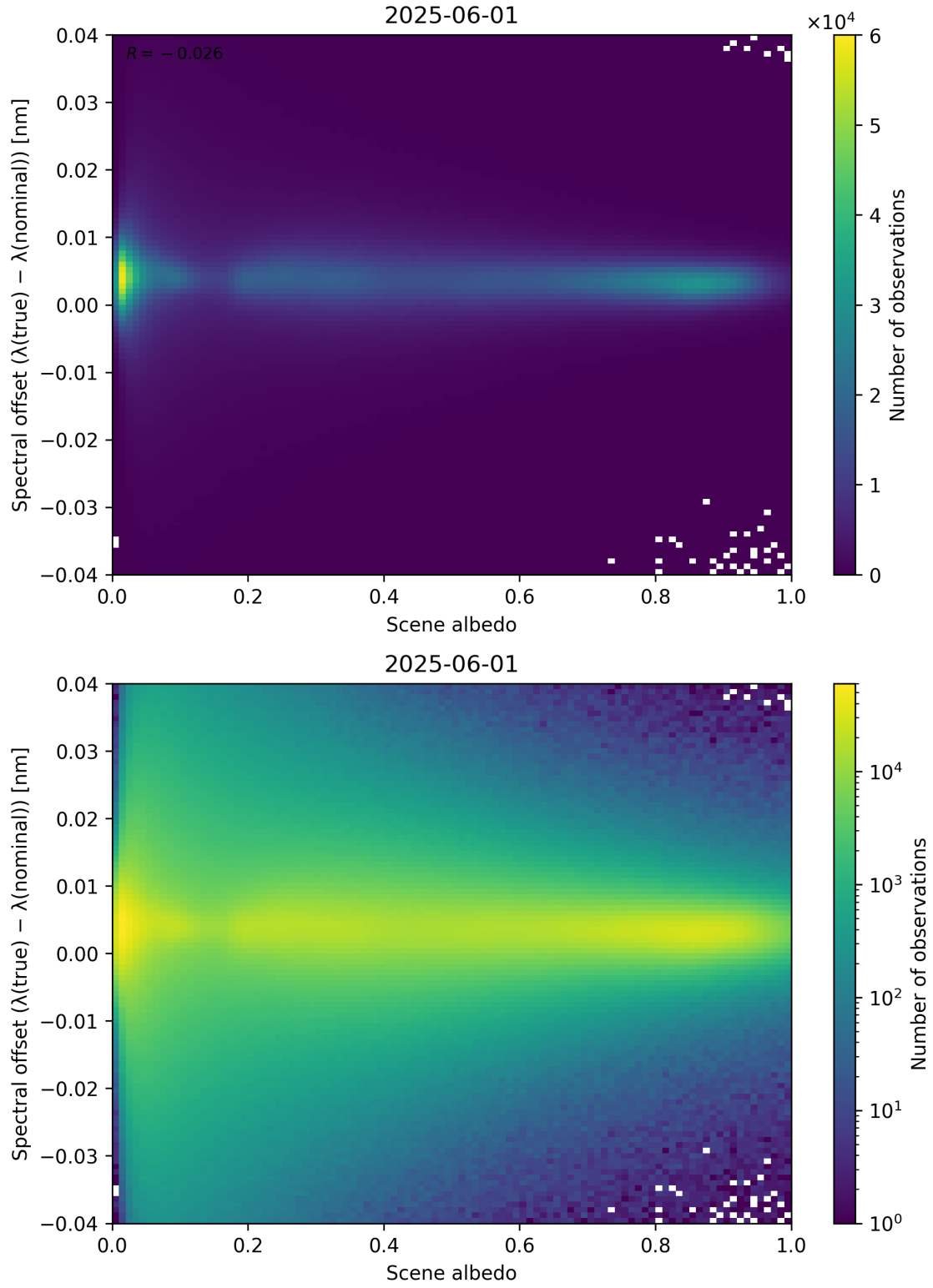
Figure 107: Scatter density plot of “Scene albedo” against “Spectral offset ( \lambda_{\text{true}} - \lambda_{\text{nominal}} )” for 2025-06-01 to 2025-06-02.
