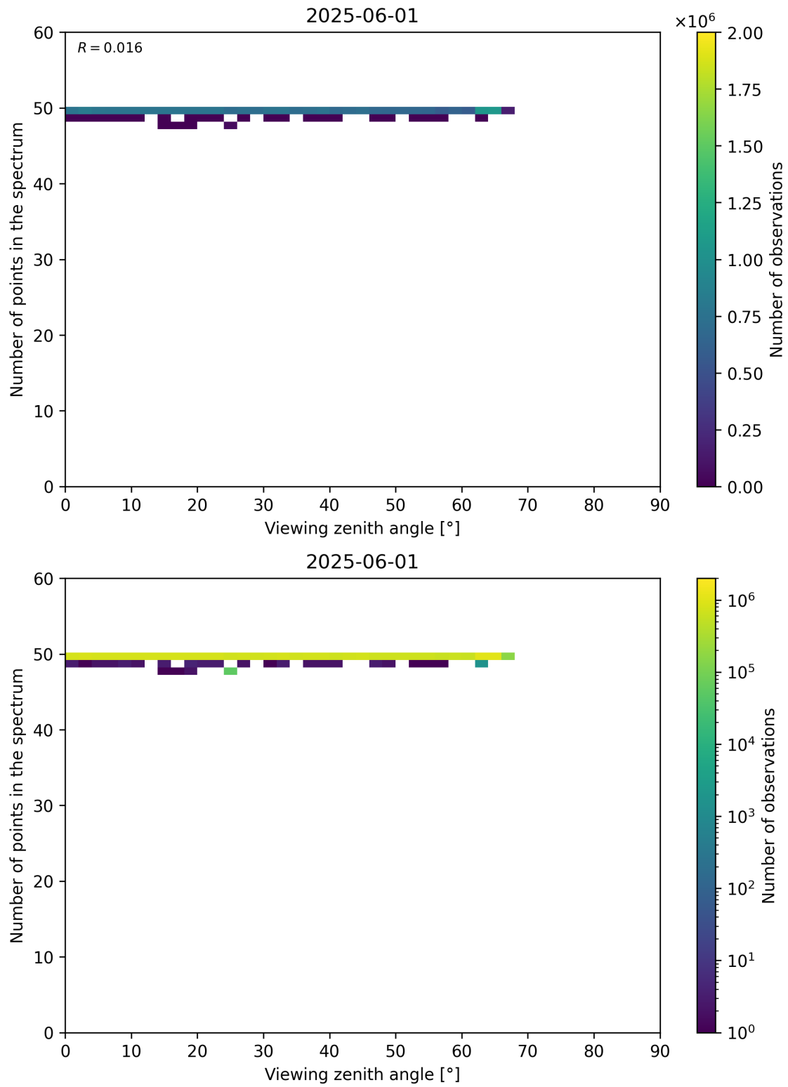
Figure 125: Scatter density plot of “Viewing zenith angle” against “Number of points in the spectrum” for 2025-06-01 to 2025-06-02.
