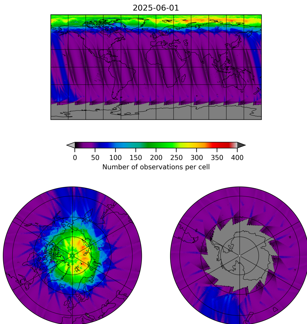
Figure 11: Map of the number of observations for 2025-06-01 to 2025-06-02
