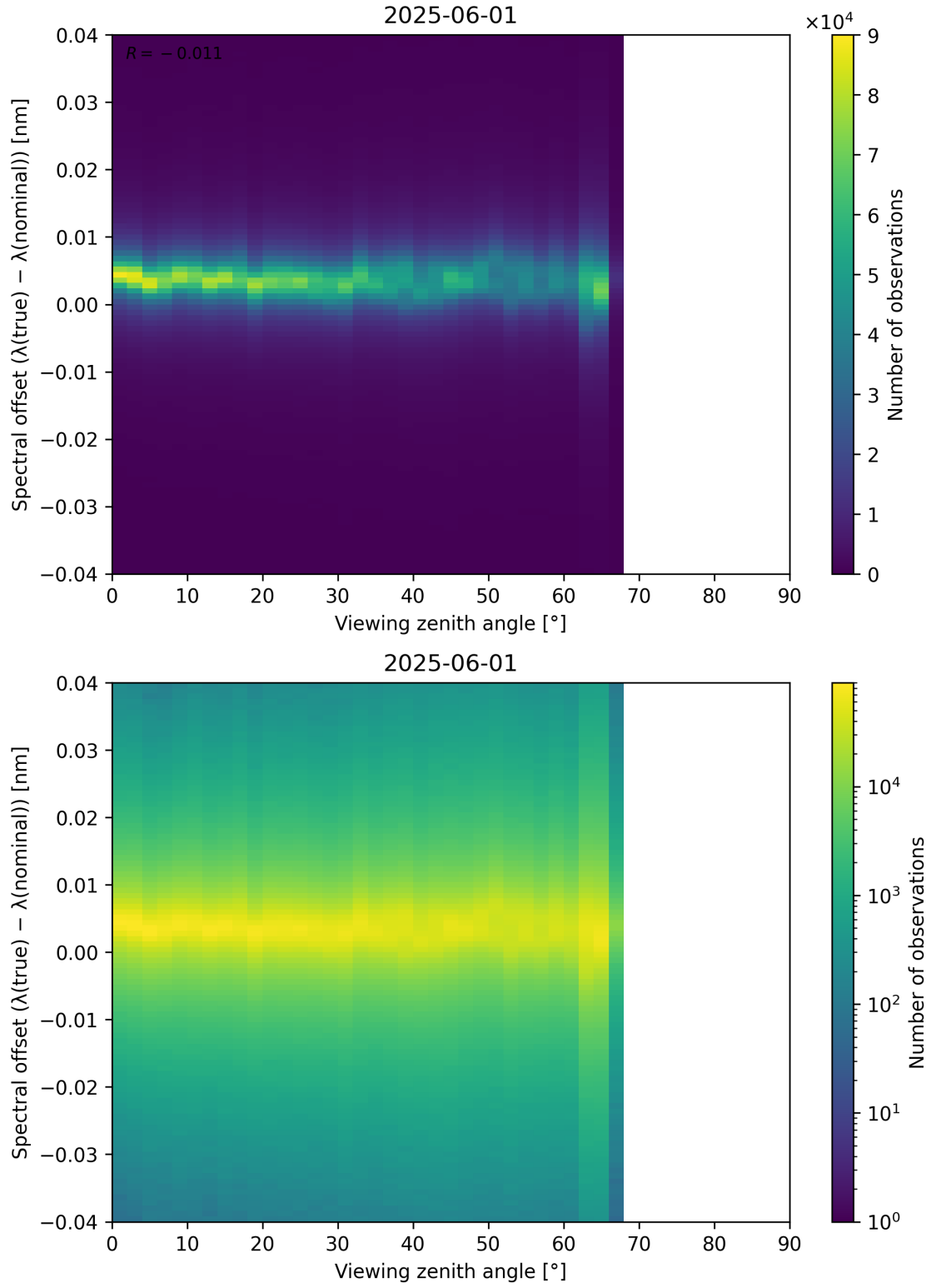
Figure 128: Scatter density plot of “Viewing zenith angle” against “Spectral offset ( \lambda_{\text{true}} - \lambda_{\text{nominal}} )” for 2025-06-01 to 2025-06-02.
