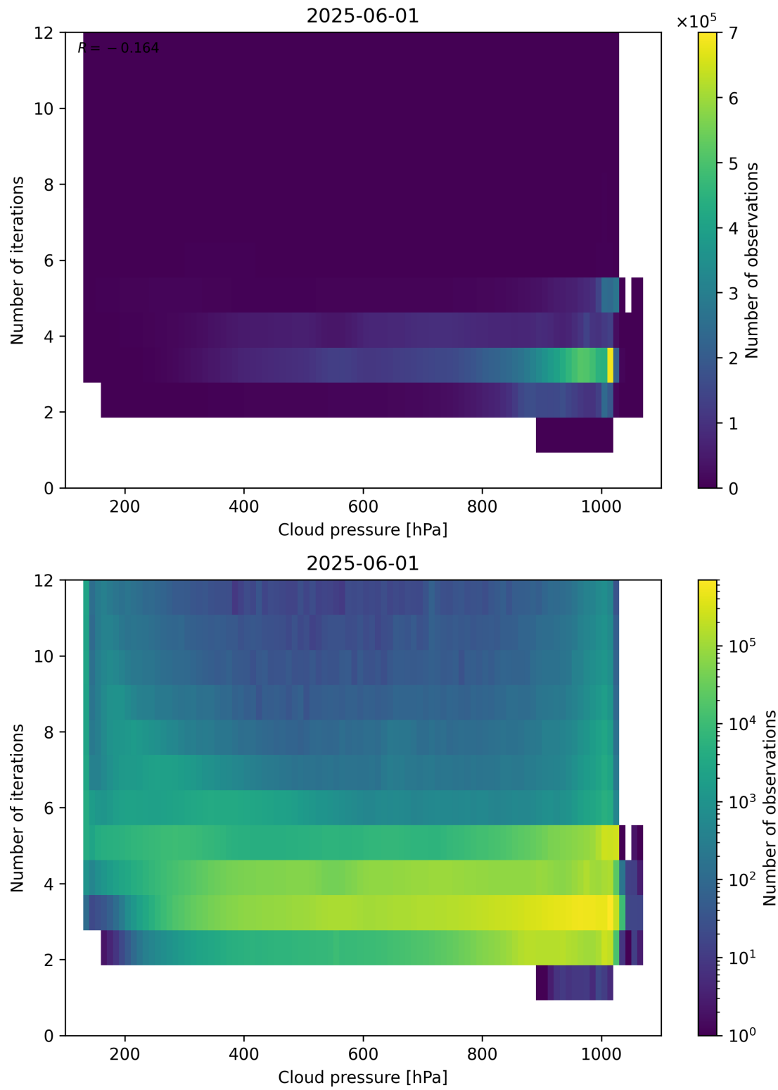
Figure 81: Scatter density plot of “Cloud pressure” against “Number of iterations” for 2025-06-01 to 2025-06-02.
