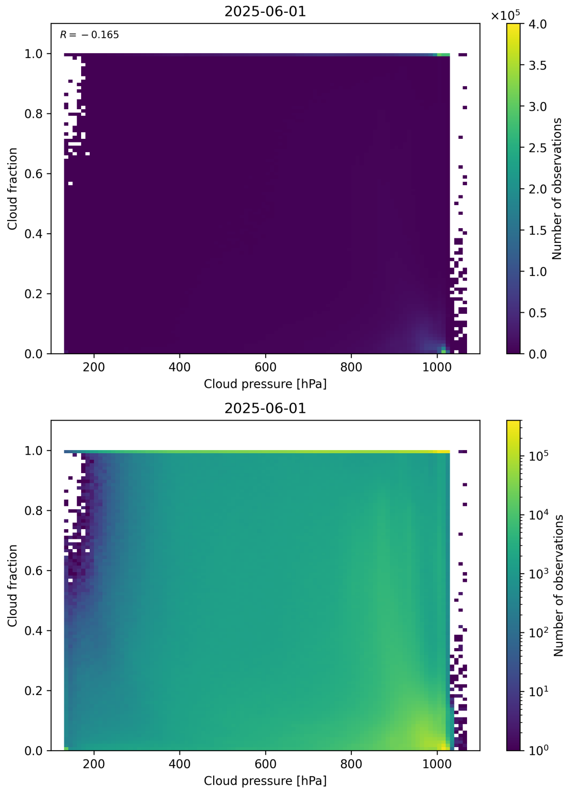
Figure 79: Scatter density plot of “Cloud pressure” against “Cloud fraction” for 2025-06-01 to 2025-06-02.
