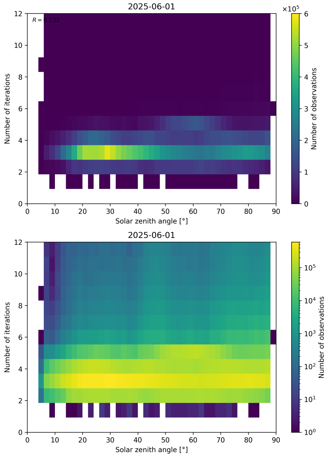
Figure 114: Scatter density plot of “Solar zenith angle” against “Number of iterations” for 2025-06-01 to 2025-06-02.
