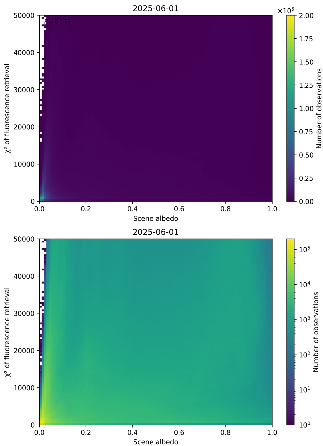
Figure 103: Scatter density plot of “Scene albedo” against “ \chi^2 of fluorescence retrieval” for 2025-06-01 to 2025-06-02.
