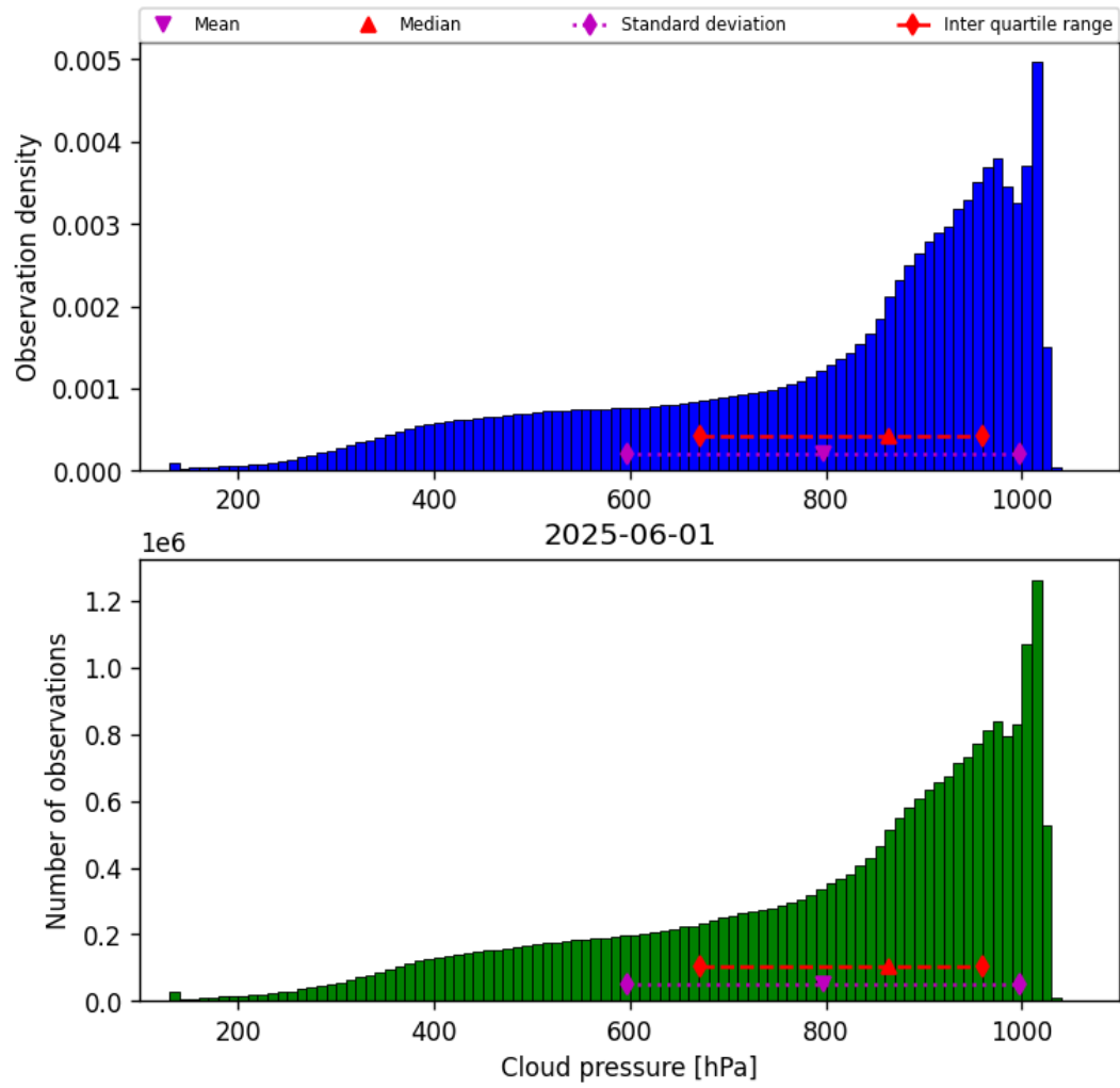
Figure 30: Histogram of “Cloud pressure” for 2025-06-01 to 2025-06-02
