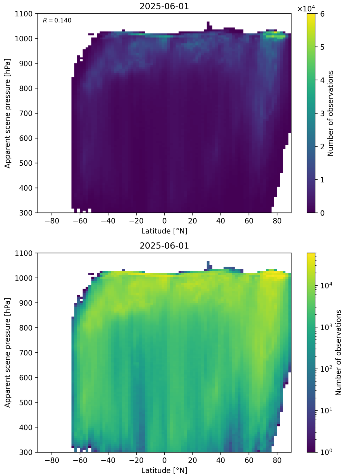
Figure 88: Scatter density plot of “Latitude” against “Apparent scene pressure” for 2025-06-01 to 2025-06-02.
