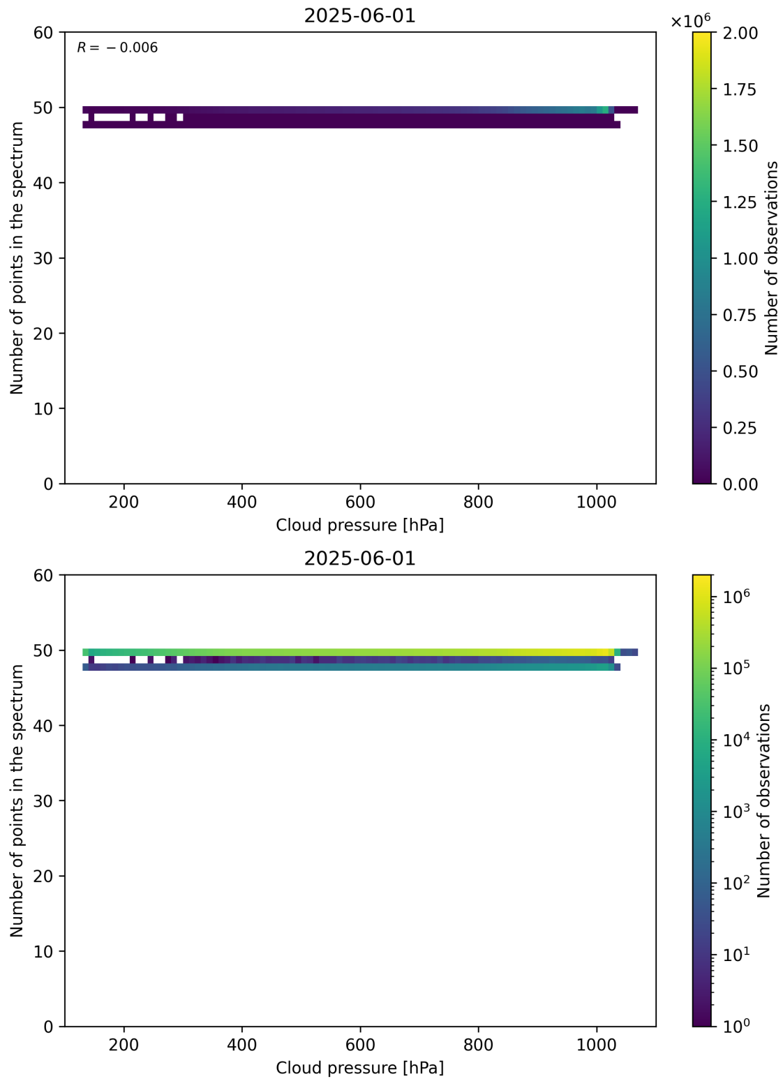
Figure 82: Scatter density plot of “Cloud pressure” against “Number of points in the spectrum” for 2025-06-01 to 2025-06-02.
