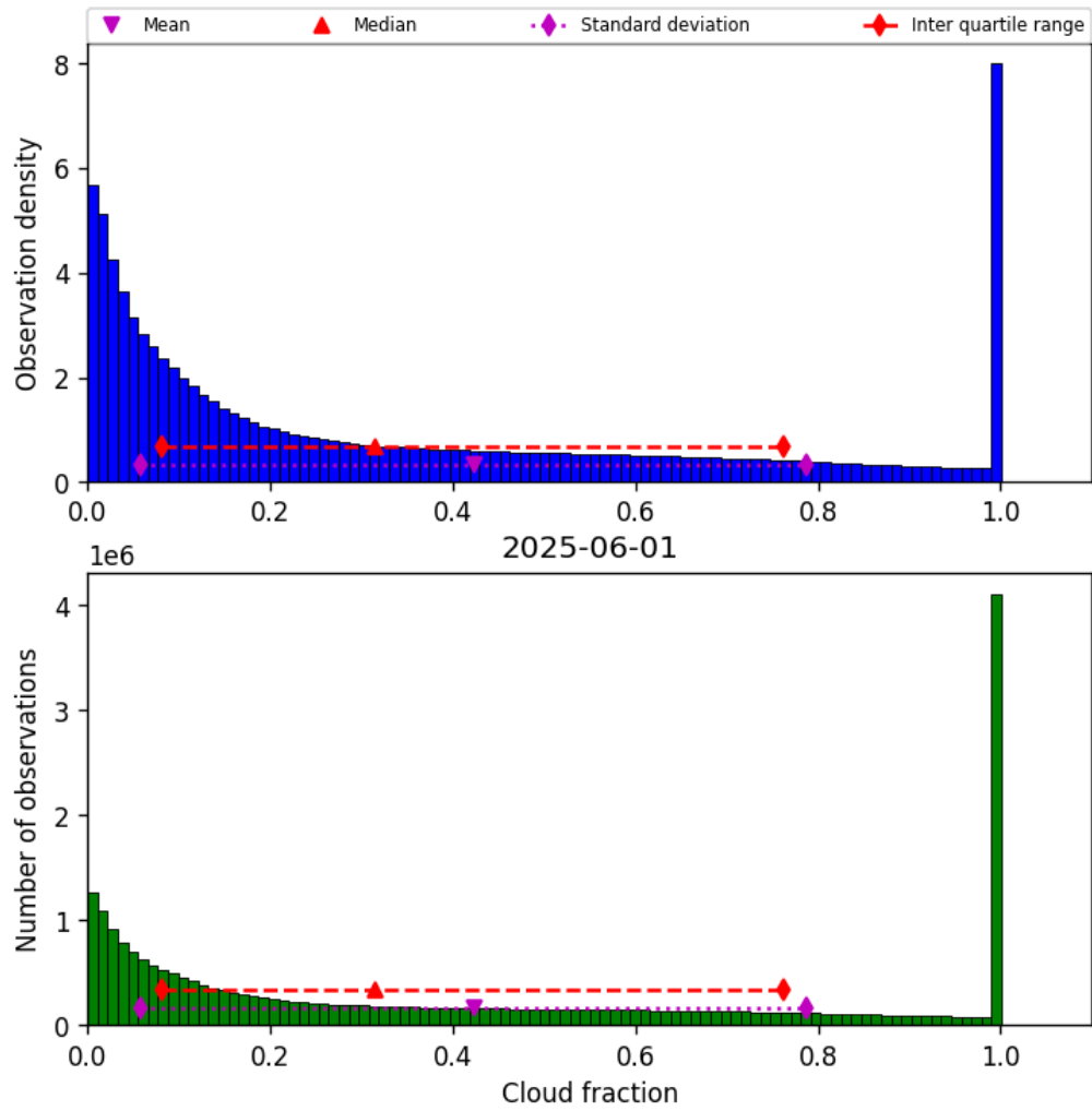
Figure 32: Histogram of “Cloud fraction” for 2025-06-01 to 2025-06-02
