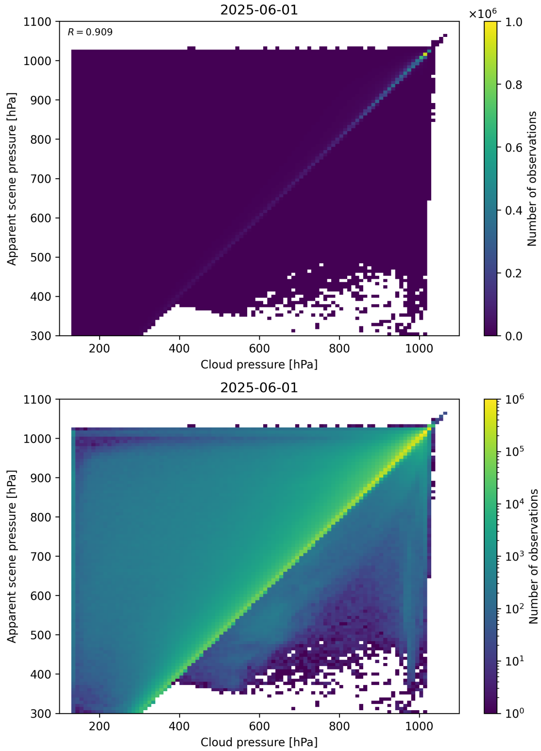
Figure 77: Scatter density plot of “Cloud pressure” against “Apparent scene pressure” for 2025-06-01 to 2025-06-02.
