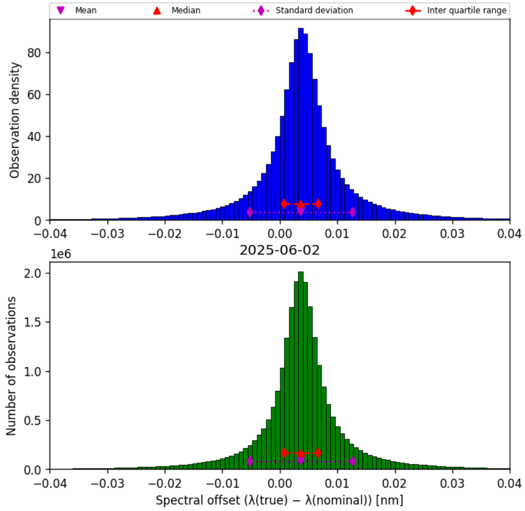
Figure 45: Histogram of “Spectral offset ( \lambda_{\text{true}} - \lambda_{\text{nominal}} )” for 2025-06-01 to 2025-06-03
