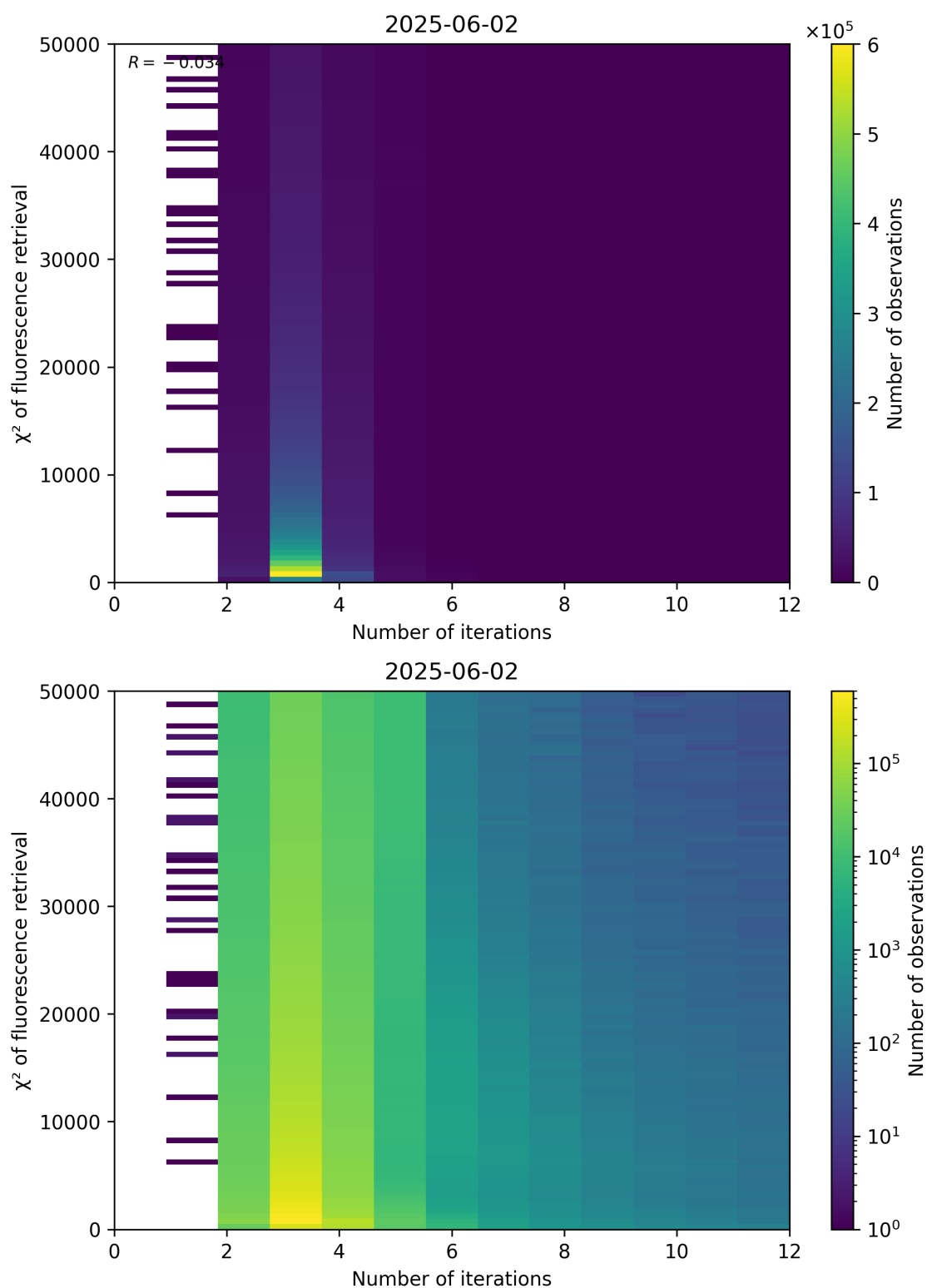
Figure 97: Scatter density plot of “Number of iterations” against “ \chi^2 of fluorescence retrieval” for 2025-06-01 to 2025-06-03.
