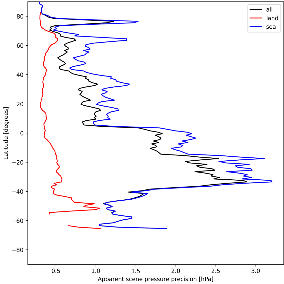
Figure 20: Zonal average of “Apparent scene pressure precision” for 2025-06-01 to 2025-06-03.
