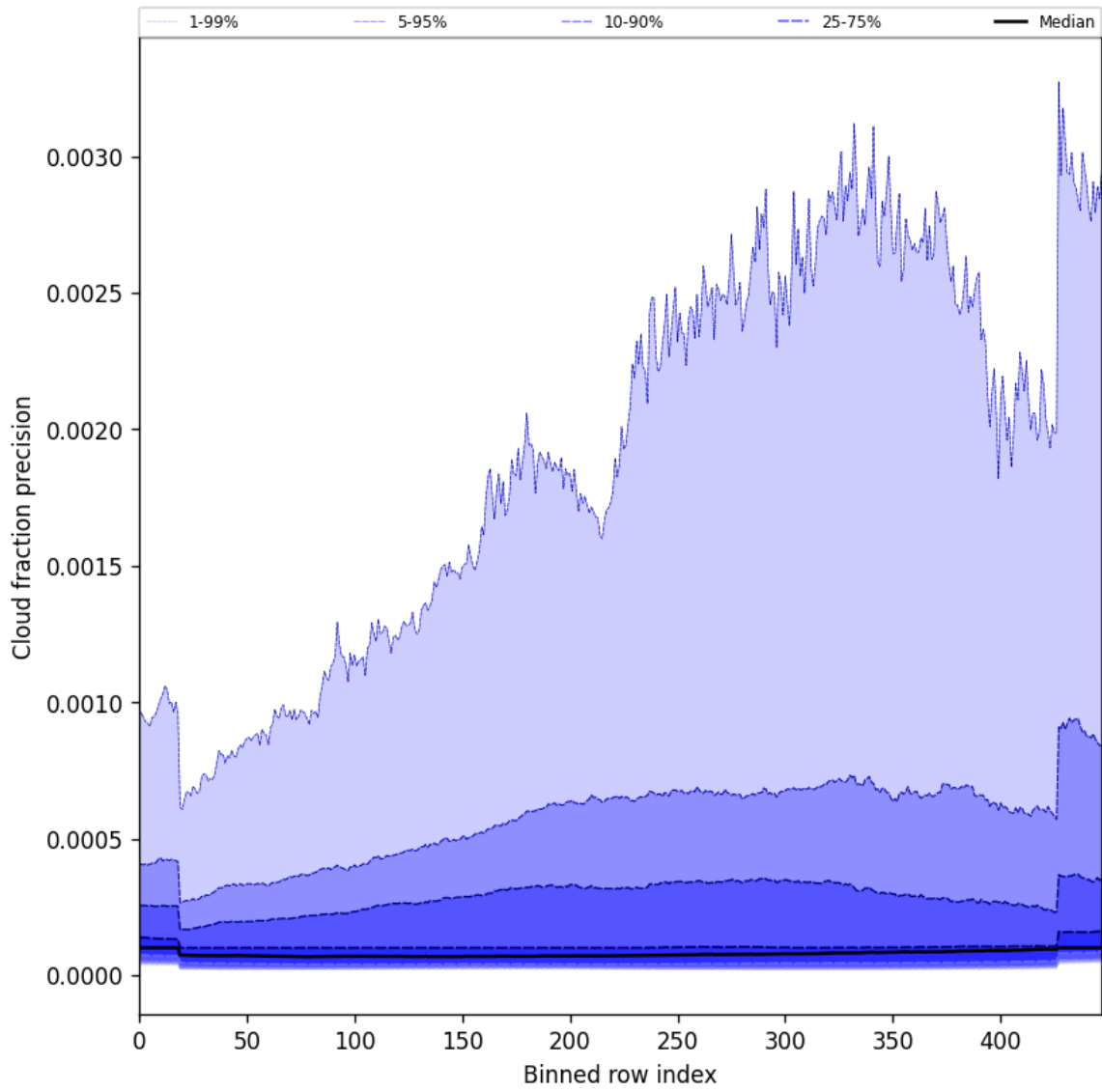
Figure 50: Along track statistics of “Cloud fraction precision” for 2025-06-01 to 2025-06-03
