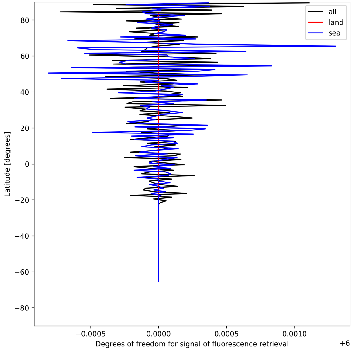
Figure 26: Zonal average of “Degrees of freedom for signal of fluorescence retrieval” for 2025-06-01 to 2025-06-03.
