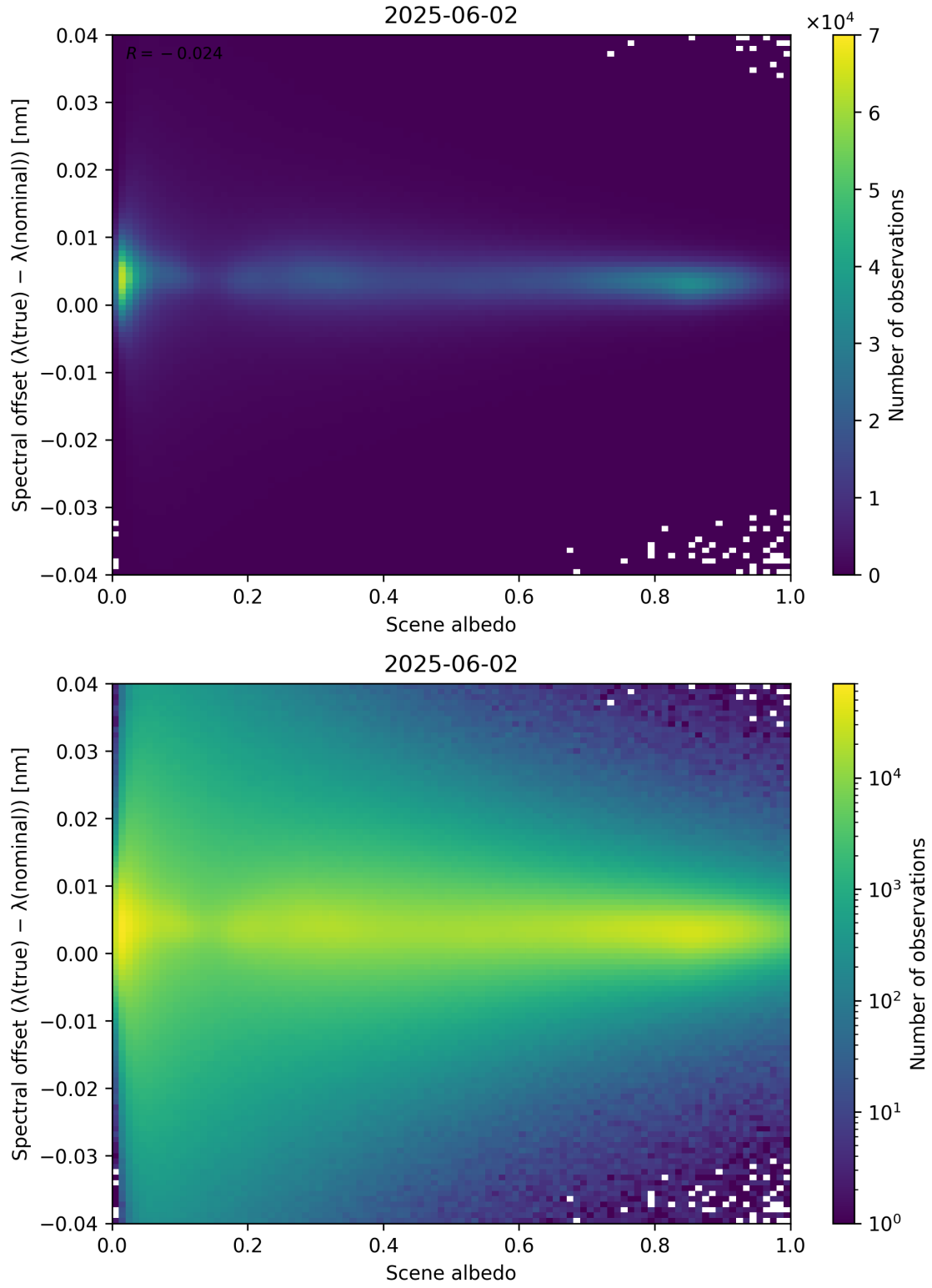
Figure 107: Scatter density plot of “Scene albedo” against “Spectral offset ( \lambda_{\text{true}} - \lambda_{\text{nominal}} )” for 2025-06-01 to 2025-06-03.
