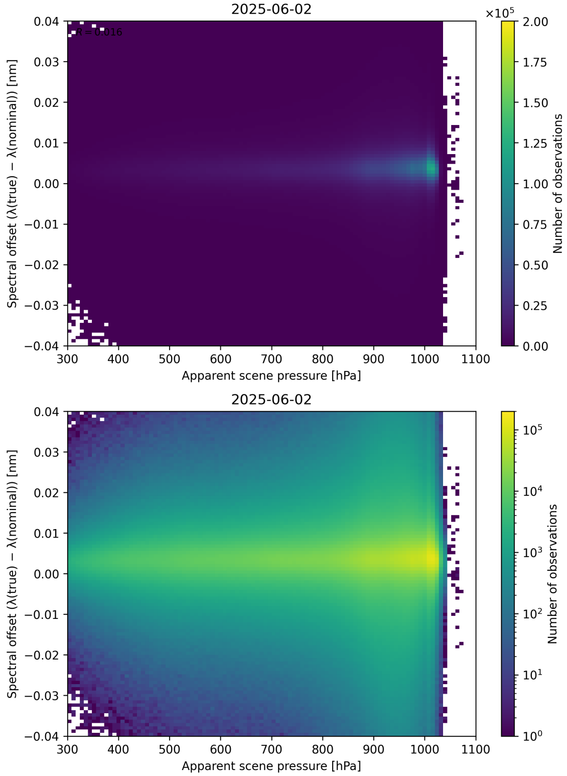
Figure 67: Scatter density plot of “Apparent scene pressure” against “Spectral offset ( \lambda_{\text{true}} - \lambda_{\text{nominal}} )” for 2025-06-01 to 2025-06-03.
