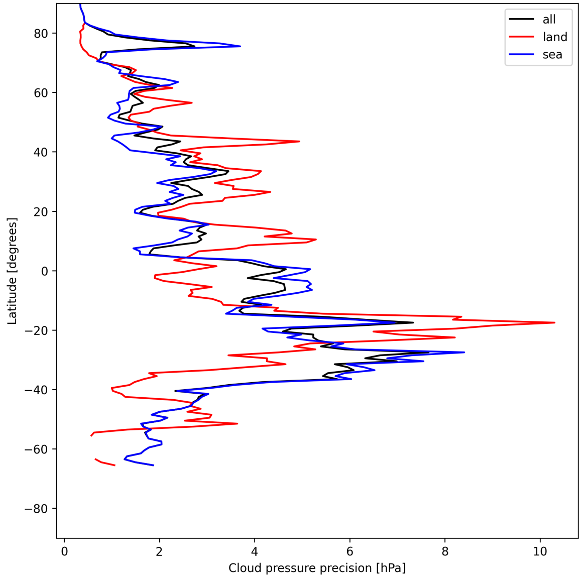
Figure 14: Zonal average of “Cloud pressure precision” for 2025-06-01 to 2025-06-03.
