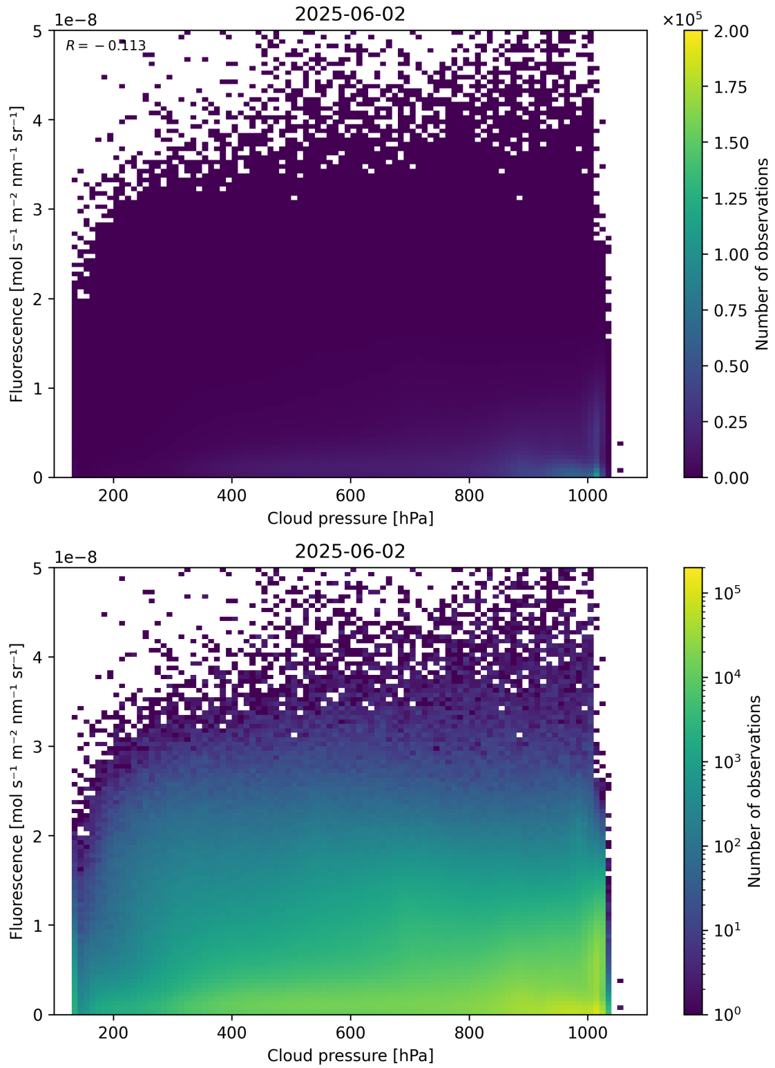
Figure 80: Scatter density plot of “Cloud pressure” against “Fluorescence” for 2025-06-01 to 2025-06-03.
