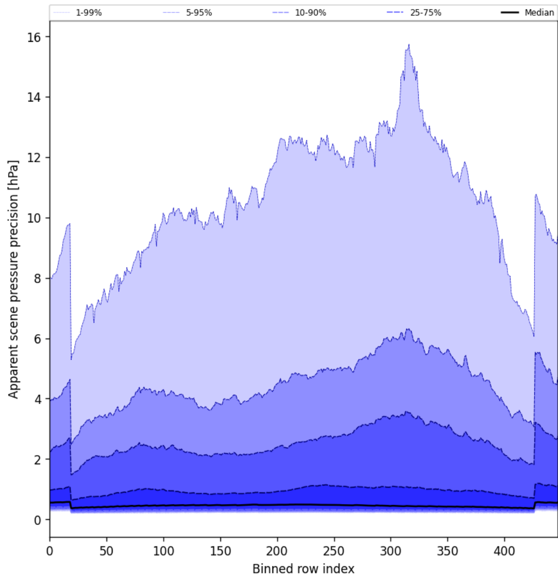
Figure 54: Along track statistics of “Apparent scene pressure precision” for 2025-06-01 to 2025-06-03
