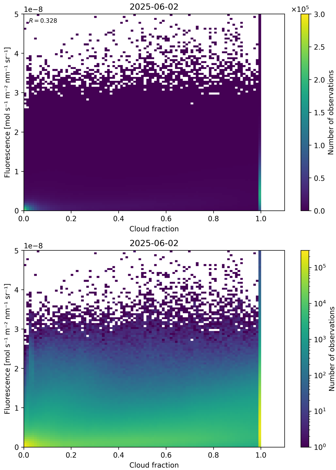
Figure 72: Scatter density plot of “Cloud fraction” against “Fluorescence” for 2025-06-01 to 2025-06-03.
