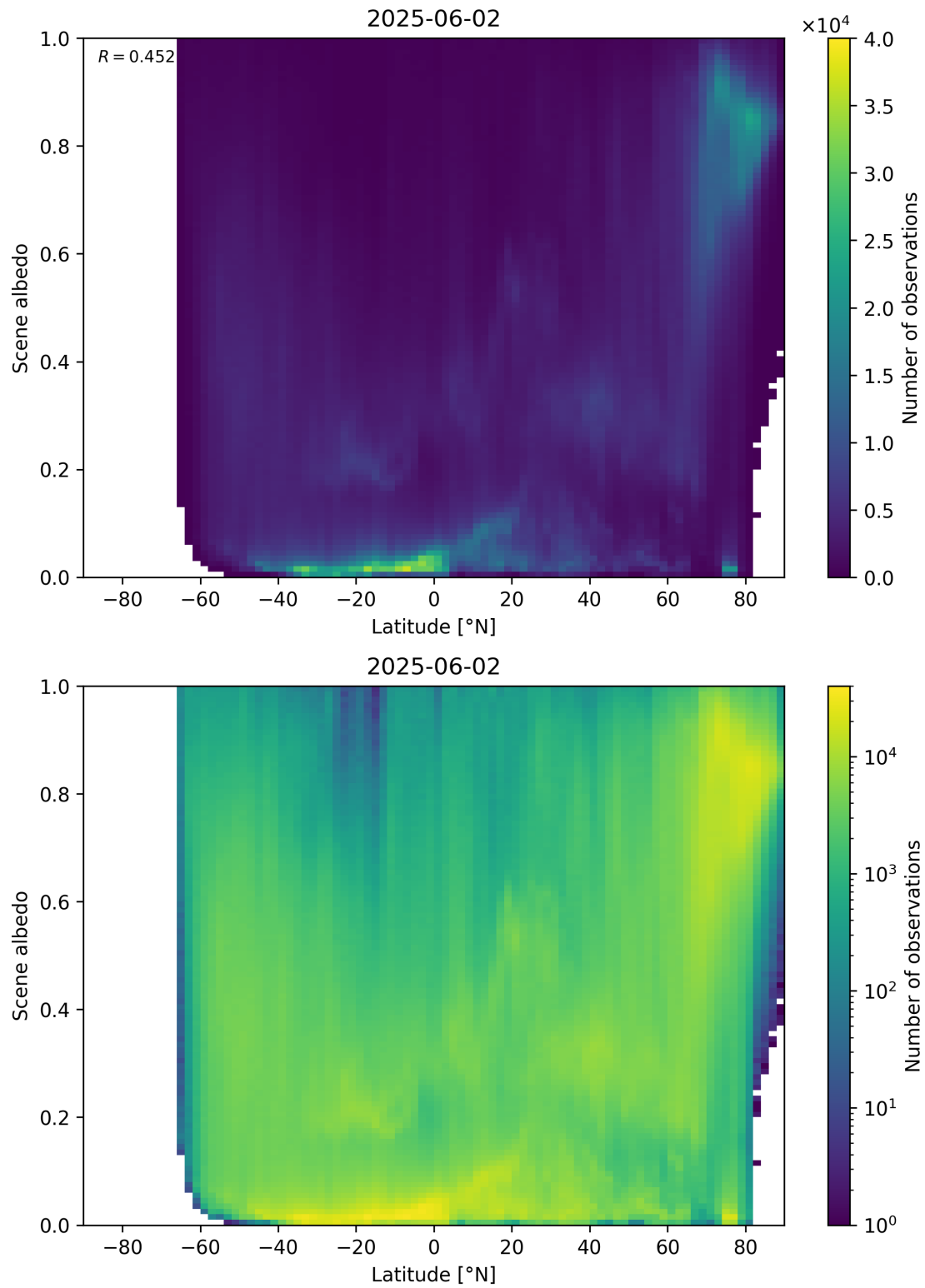
Figure 95: Scatter density plot of “Latitude” against “Scene albedo” for 2025-06-01 to 2025-06-03.
