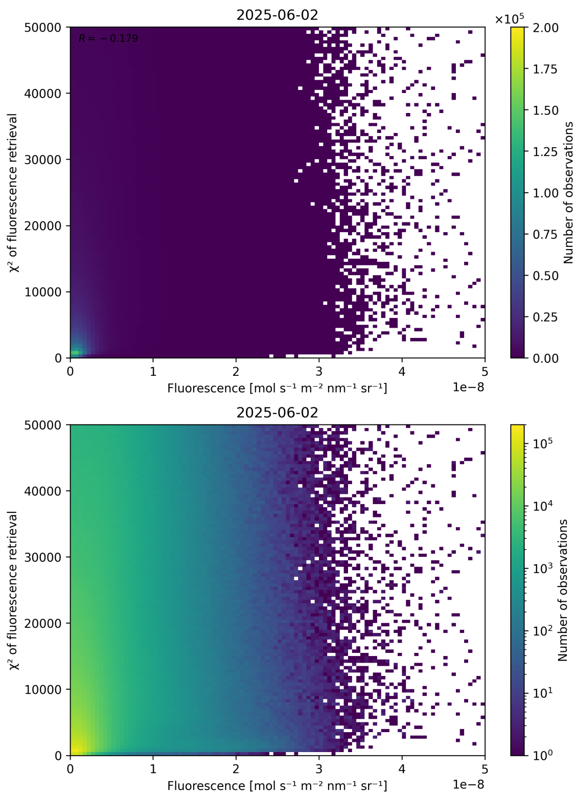
Figure 85: Scatter density plot of “Fluorescence” against “ \chi^2 of fluorescence retrieval” for 2025-06-01 to 2025-06-03.
