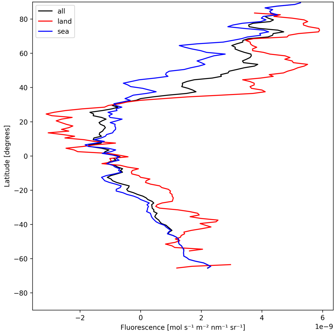
Figure 23: Zonal average of “Fluorescence” for 2025-06-01 to 2025-06-03.
