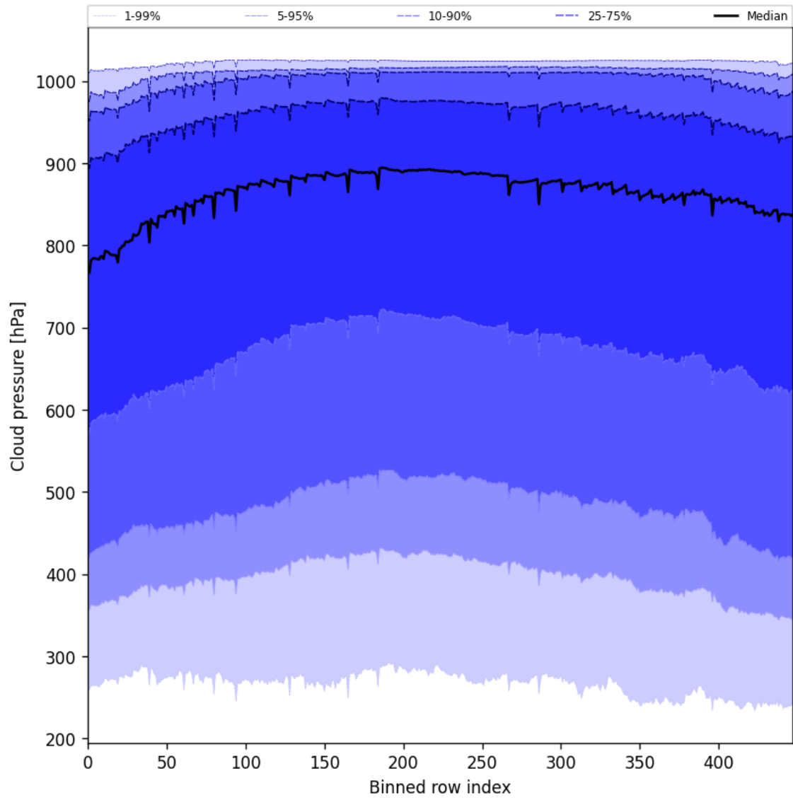
Figure 47: Along track statistics of “Cloud pressure” for 2025-06-01 to 2025-06-03
