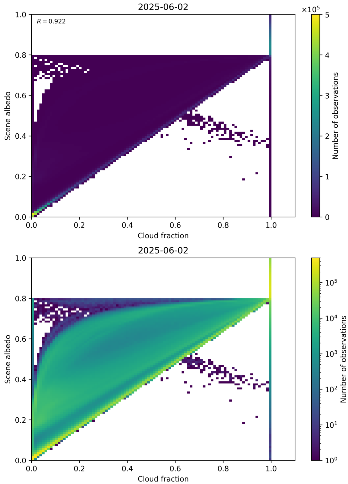
Figure 75: Scatter density plot of “Cloud fraction” against “Scene albedo” for 2025-06-01 to 2025-06-03.
