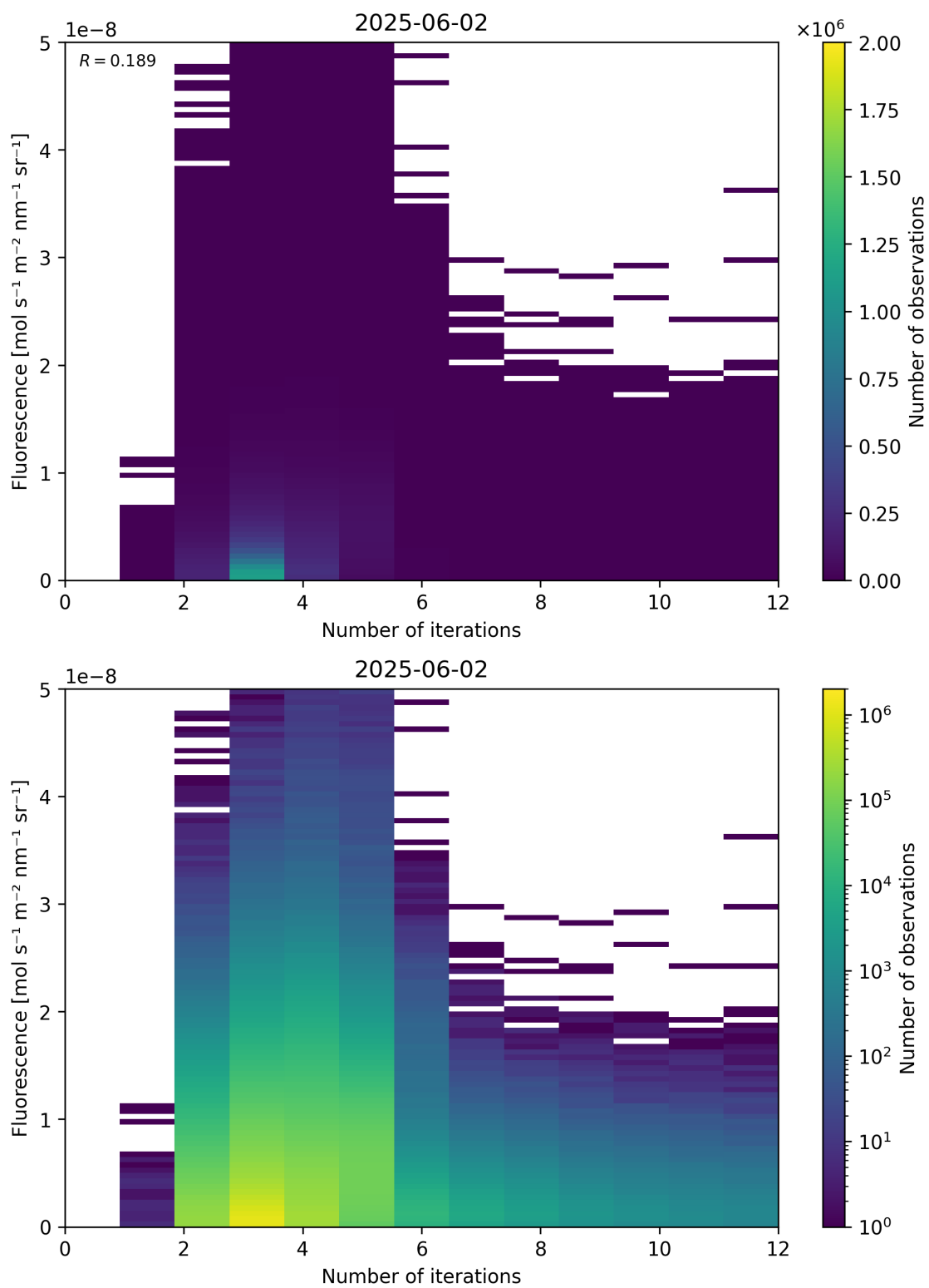
Figure 98: Scatter density plot of “Number of iterations” against “Fluorescence” for 2025-06-01 to 2025-06-03.
