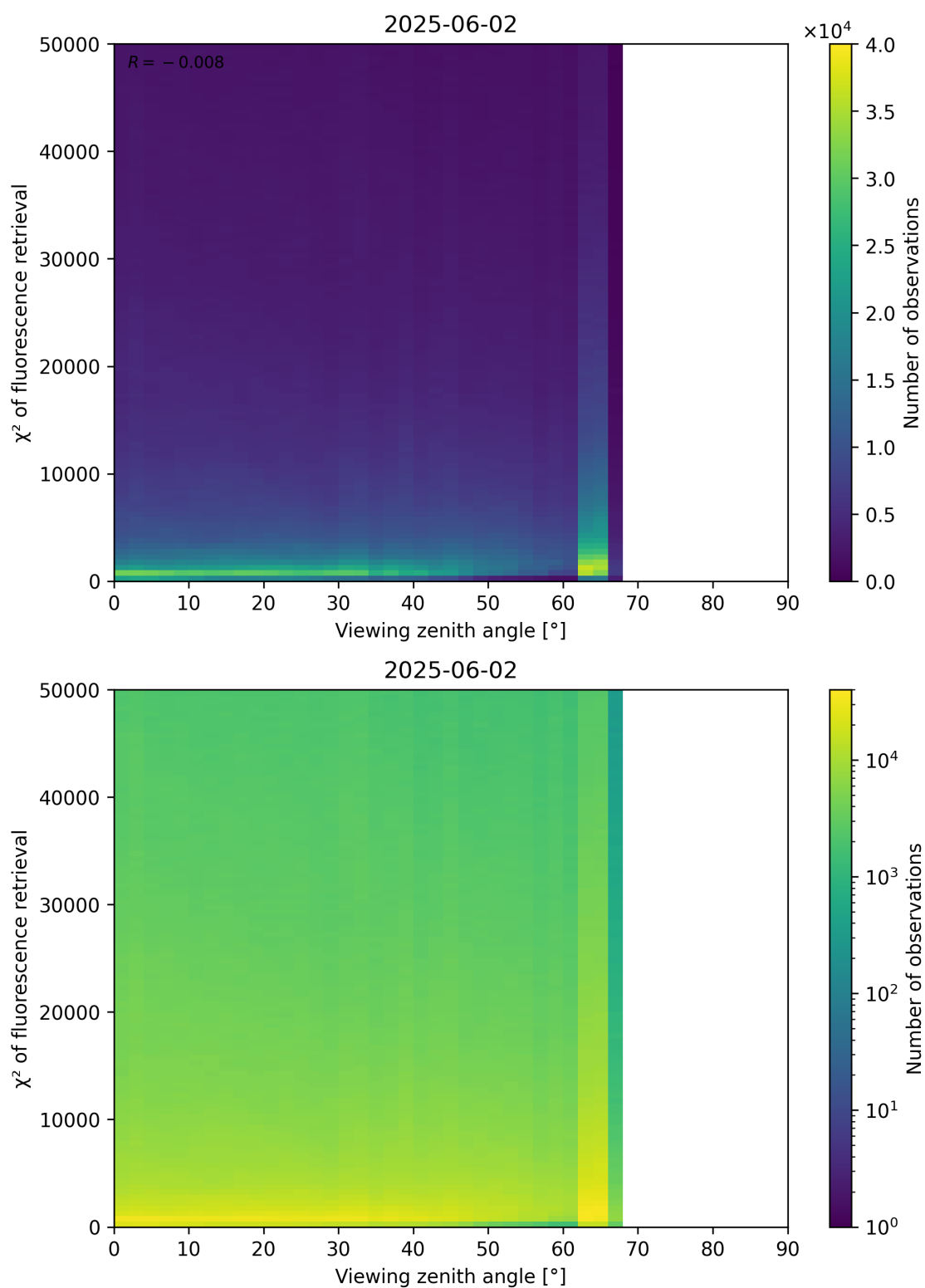
Figure 119: Scatter density plot of “Viewing zenith angle” against “ \chi^2 of fluorescence retrieval” for 2025-06-01 to 2025-06-03.
