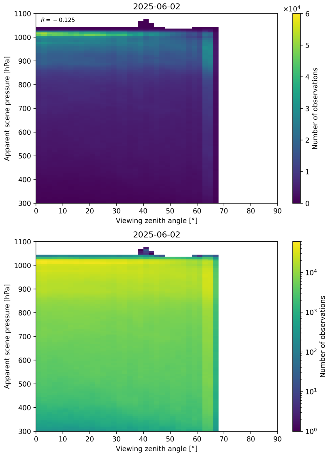
Figure 118: Scatter density plot of “Viewing zenith angle” against “Apparent scene pressure” for 2025-06-01 to 2025-06-03.
