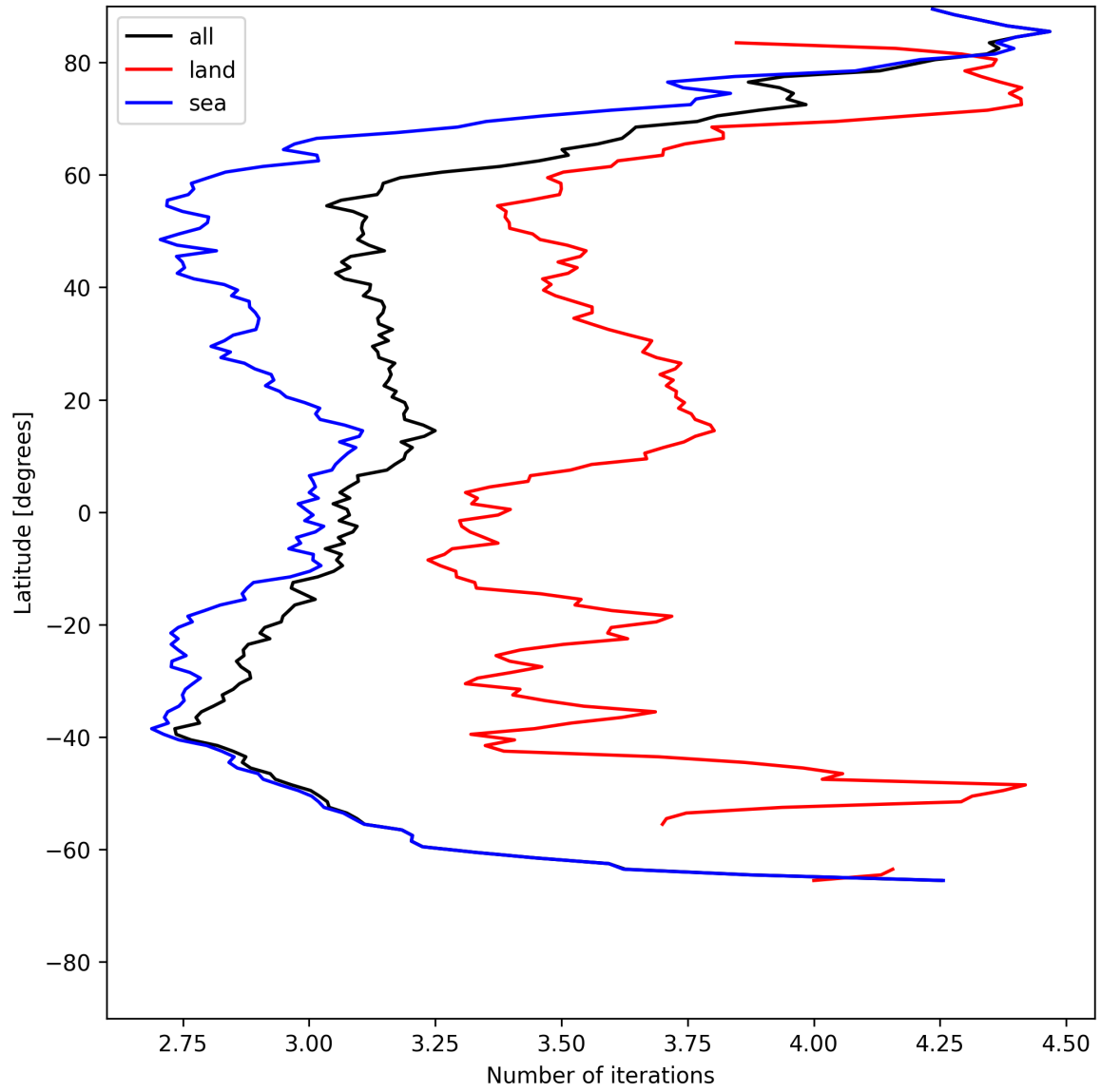
Figure 22: Zonal average of “Number of iterations” for 2025-06-01 to 2025-06-03.
