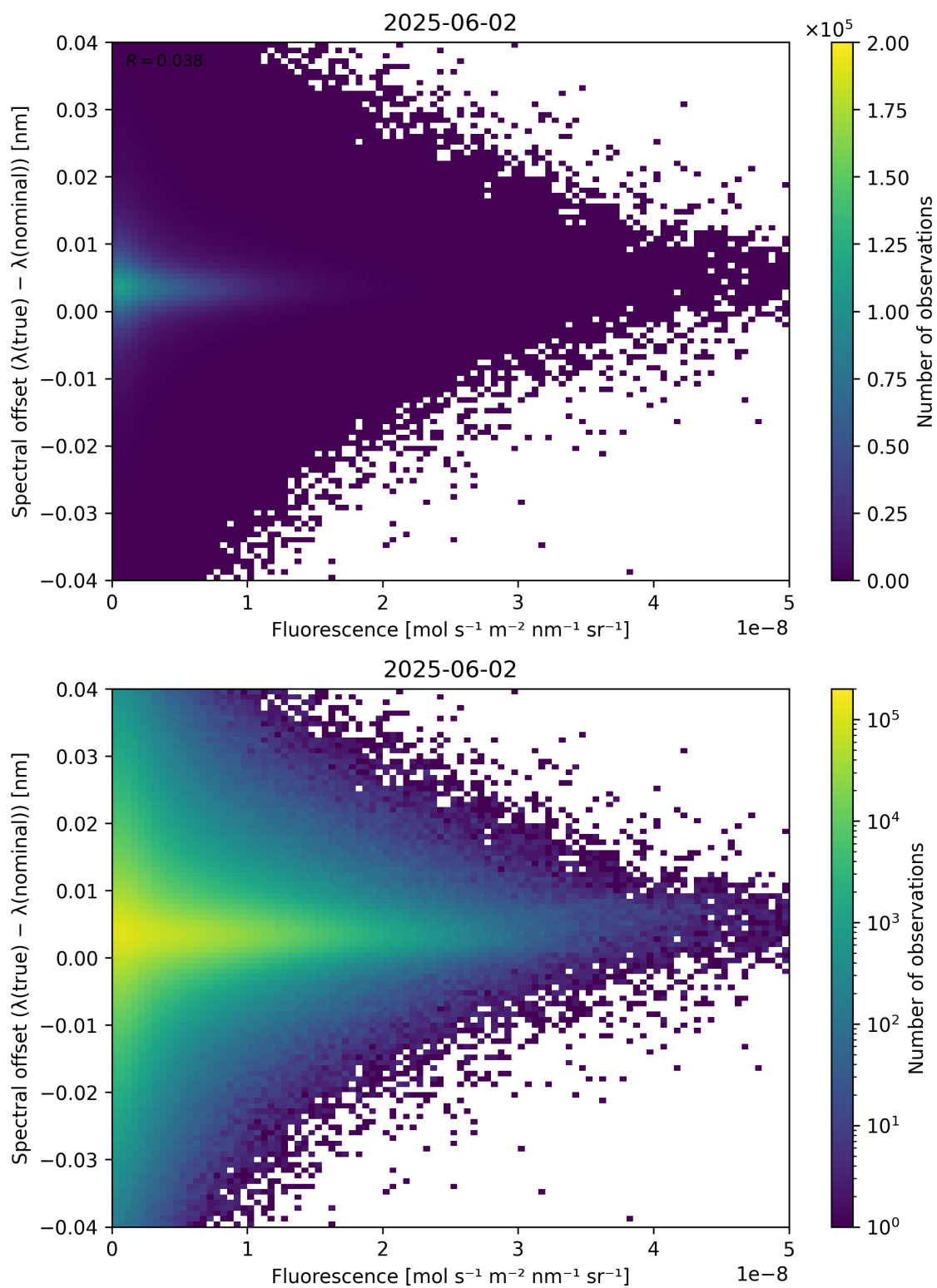
Figure 87: Scatter density plot of “Fluorescence” against “Spectral offset ( \lambda_{\text{true}} - \lambda_{\text{nominal}} )” for 2025-06-01 to 2025-06-03.
