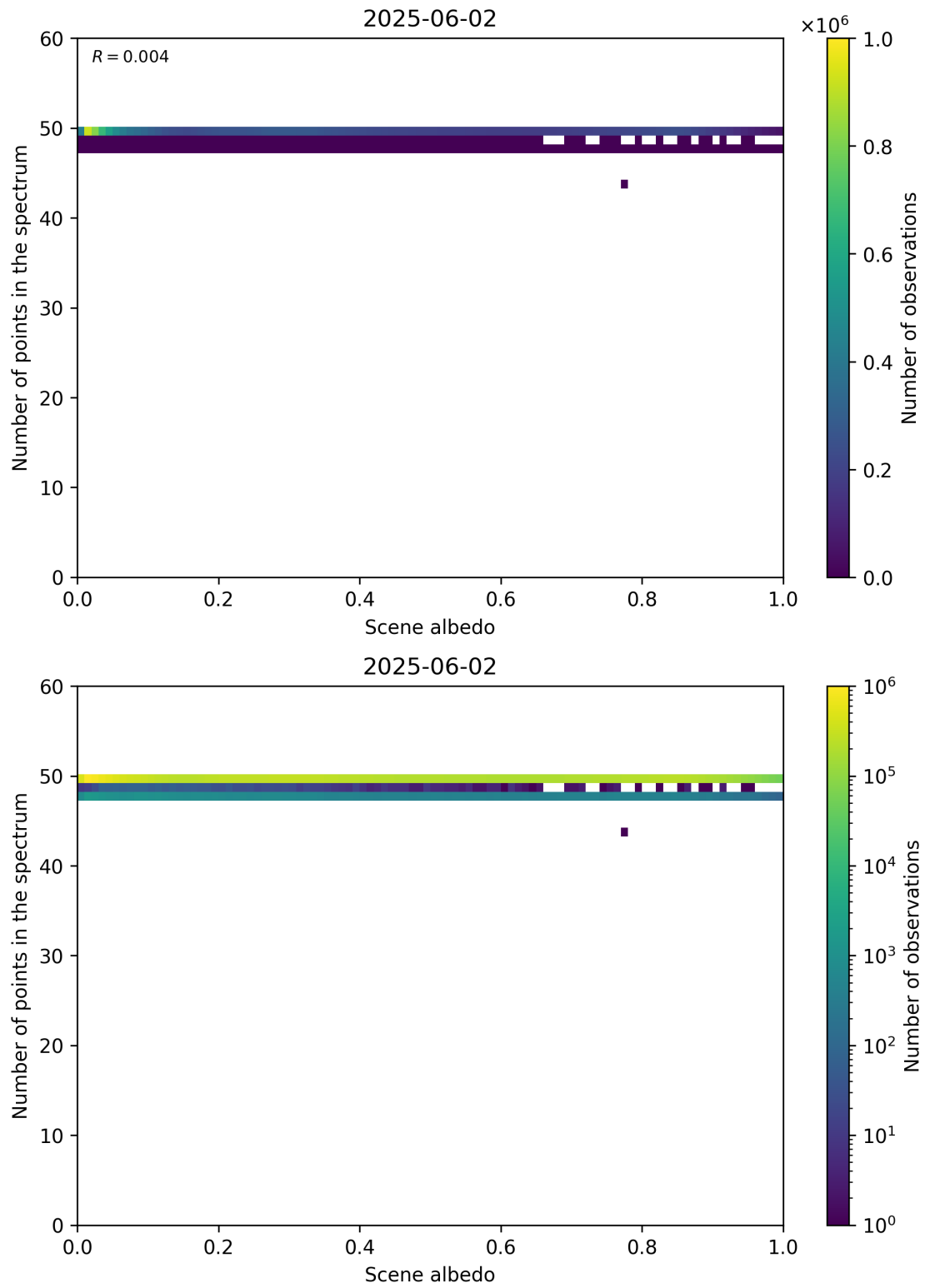
Figure 106: Scatter density plot of “Scene albedo” against “Number of points in the spectrum” for 2025-06-01 to 2025-06-03.
