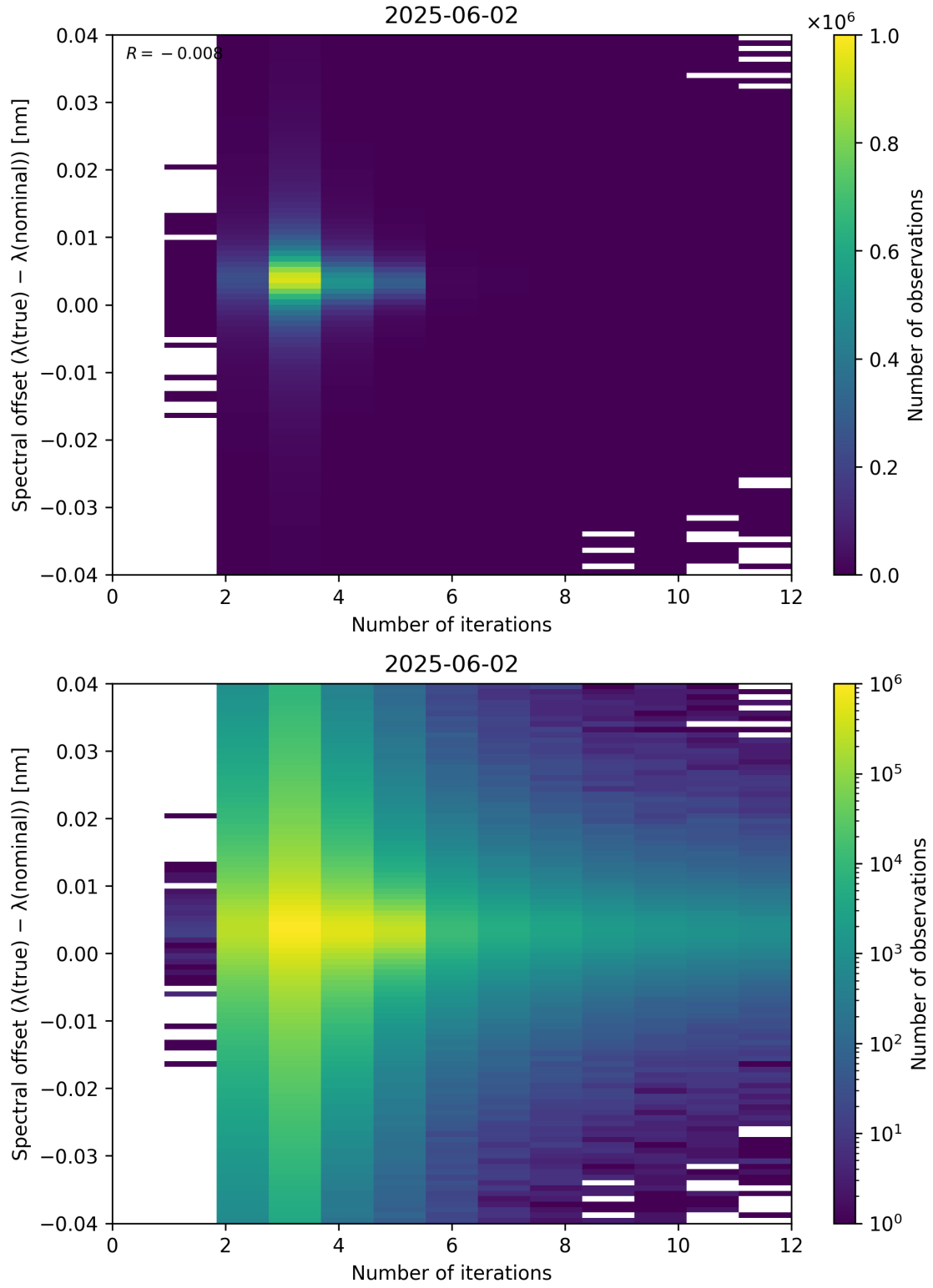
Figure 100: Scatter density plot of “Number of iterations” against “Spectral offset ( \lambda_{\text{true}} - \lambda_{\text{nominal}} )” for 2025-06-01 to 2025-06-03.
