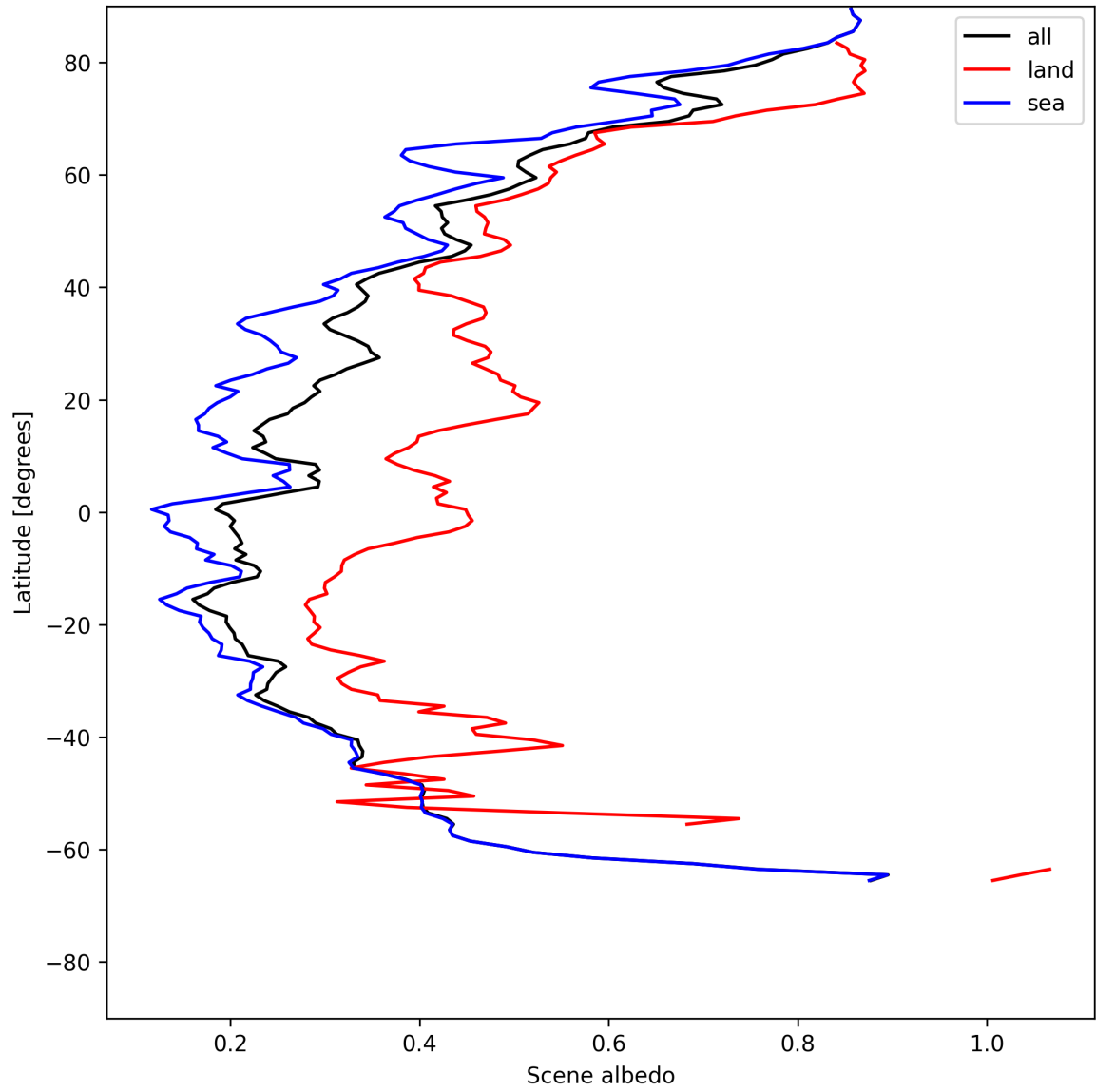
Figure 17: Zonal average of “Scene albedo” for 2025-06-01 to 2025-06-03.
