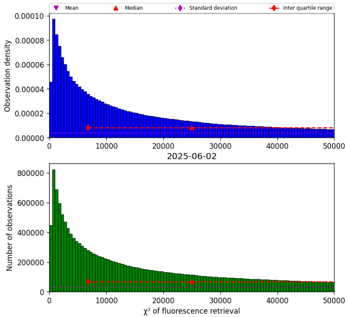
Figure 42: Histogram of “ \chi^2 of fluorescence retrieval” for 2025-06-01 to 2025-06-03
