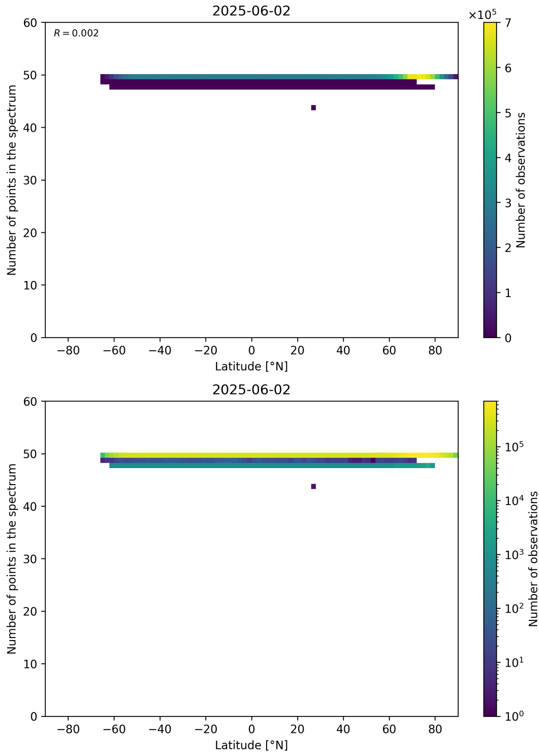
Figure 94: Scatter density plot of “Latitude” against “Number of points in the spectrum” for 2025-06-01 to 2025-06-03.
