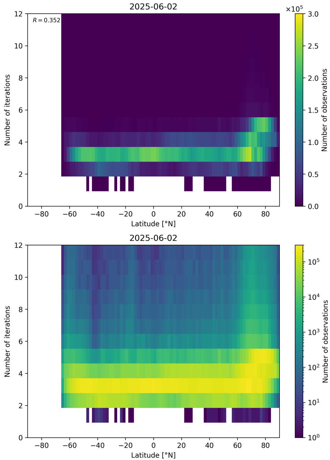
Figure 93: Scatter density plot of “Latitude” against “Number of iterations” for 2025-06-01 to 2025-06-03.
