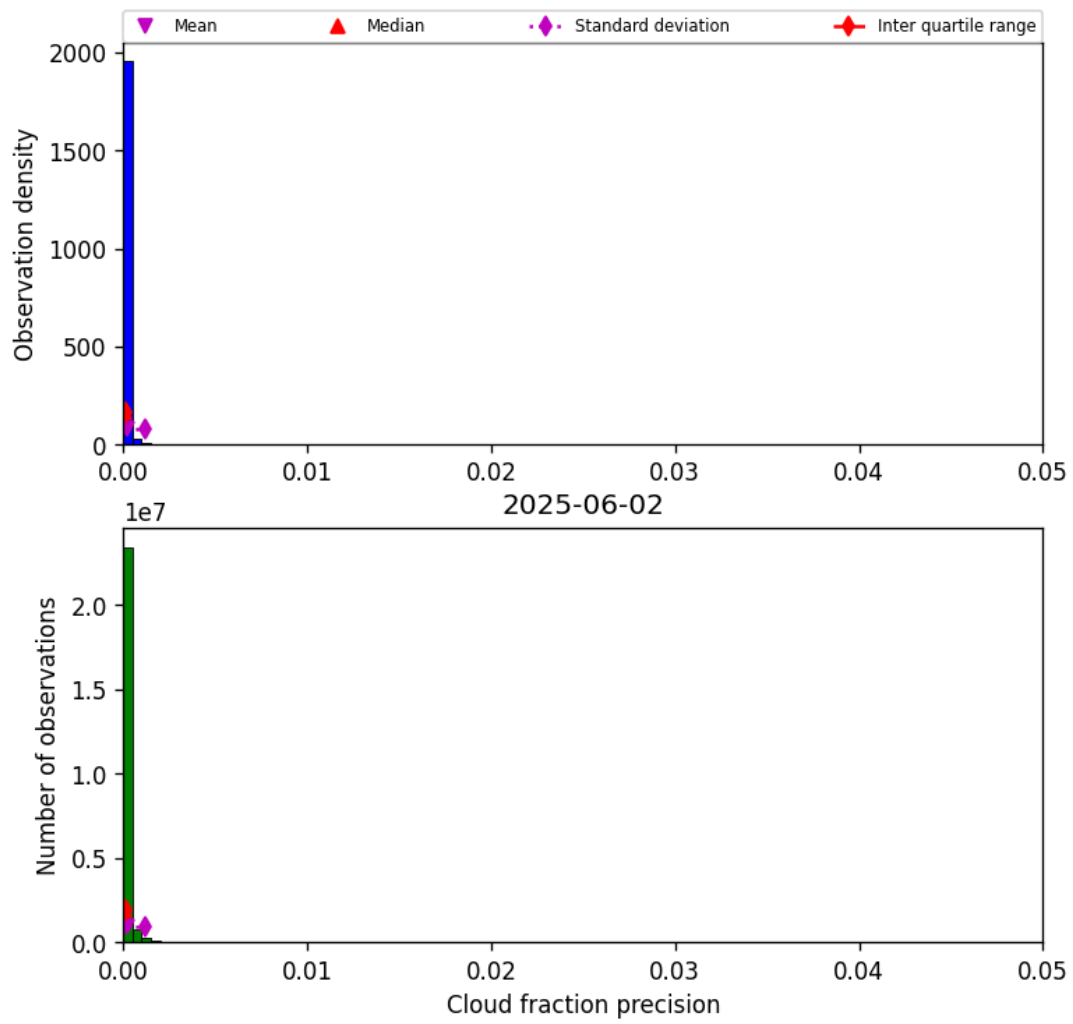
Figure 33: Histogram of “Cloud fraction precision” for 2025-06-01 to 2025-06-03
