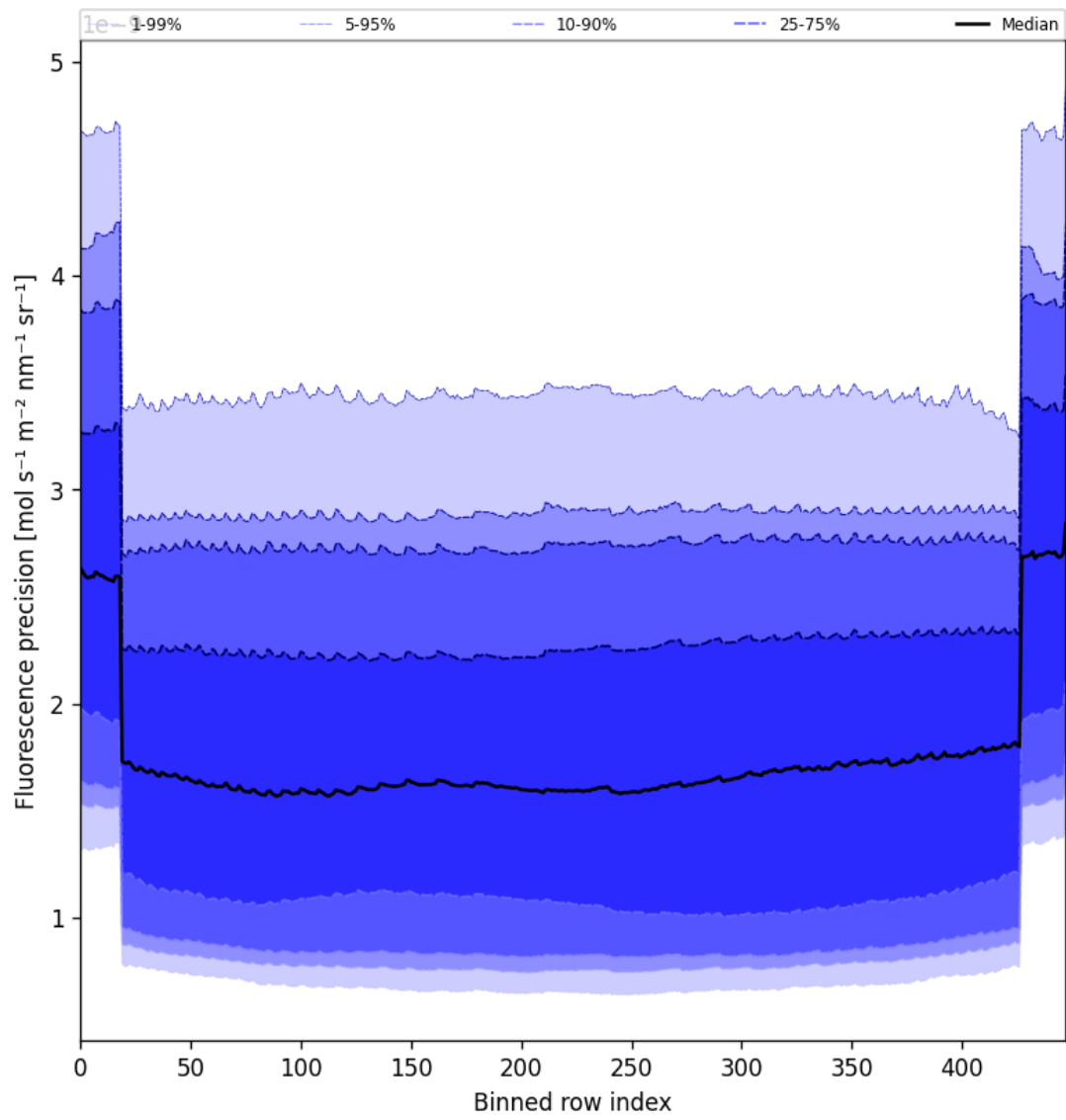
Figure 58: Along track statistics of “Fluorescence precision” for 2025-06-01 to 2025-06-03
