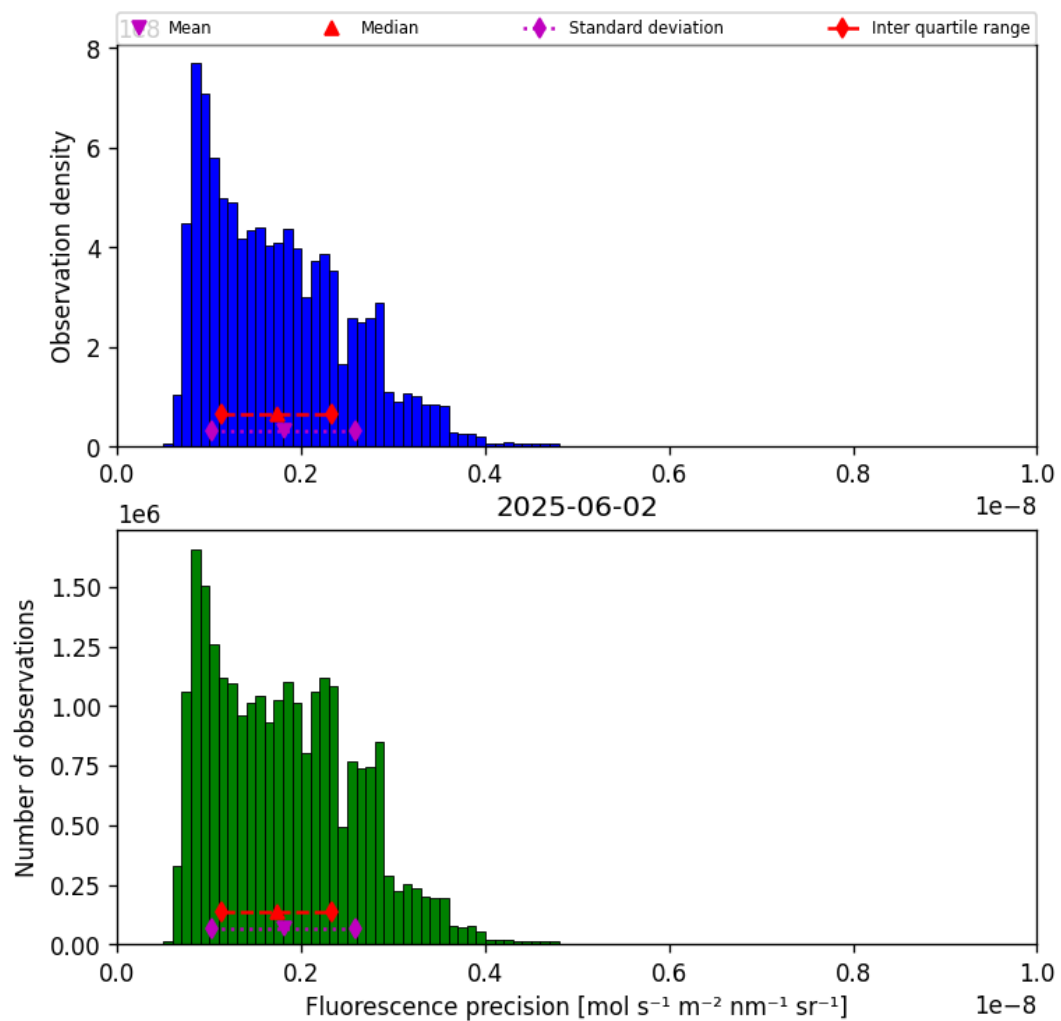
Figure 41: Histogram of “Fluorescence precision” for 2025-06-01 to 2025-06-03
