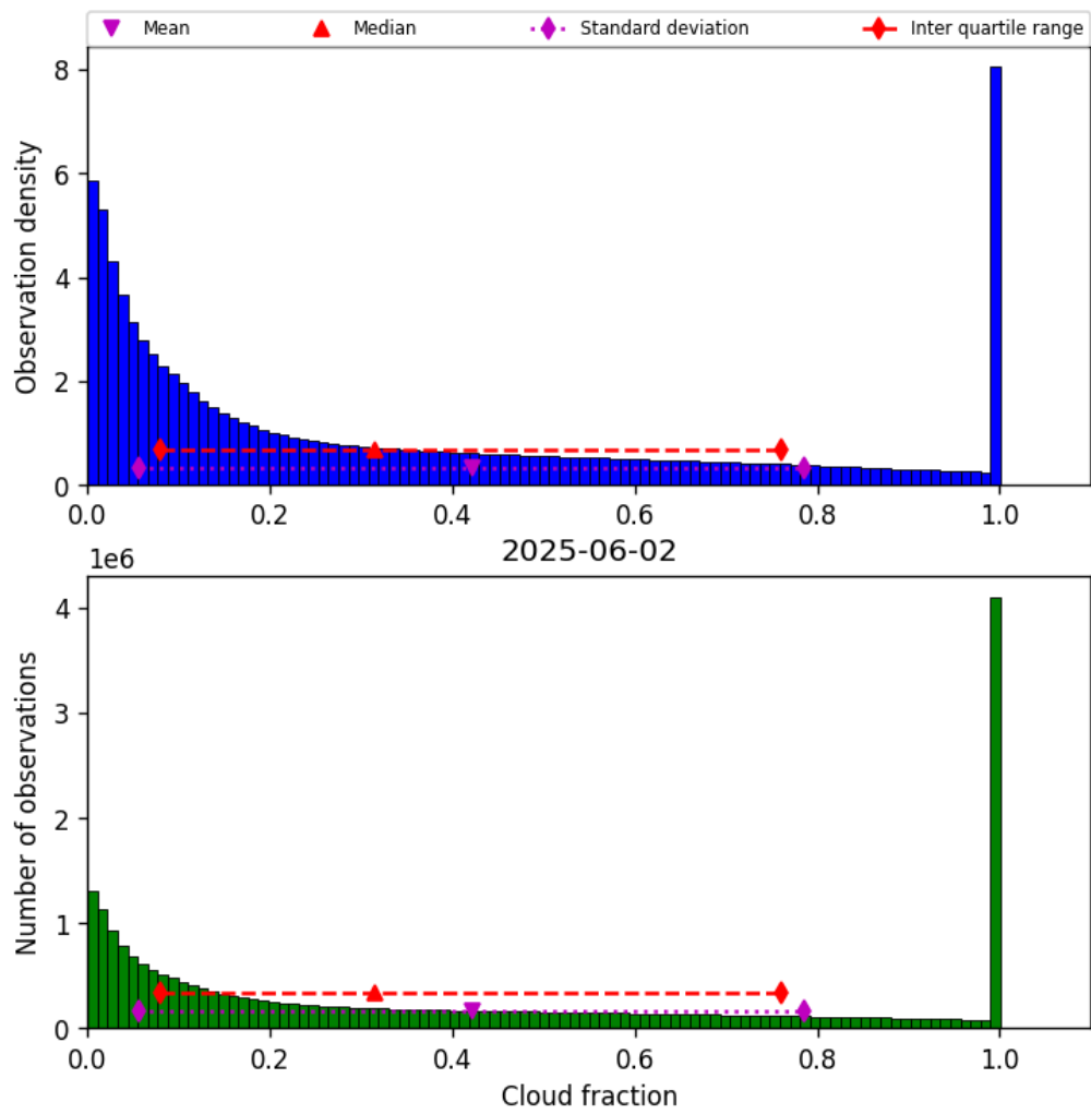
Figure 32: Histogram of “Cloud fraction” for 2025-06-01 to 2025-06-03
