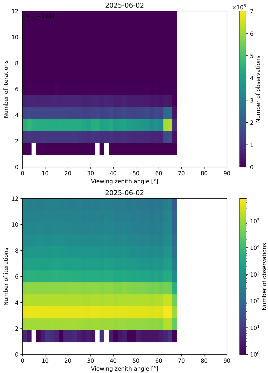
Figure 124: Scatter density plot of “Viewing zenith angle” against “Number of iterations” for 2025-06-01 to 2025-06-03.
