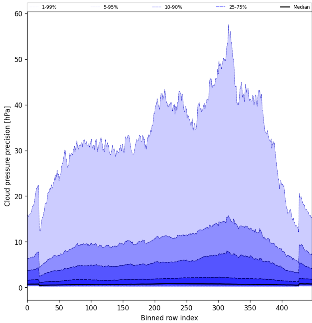
Figure 48: Along track statistics of “Cloud pressure precision” for 2025-06-01 to 2025-06-03
