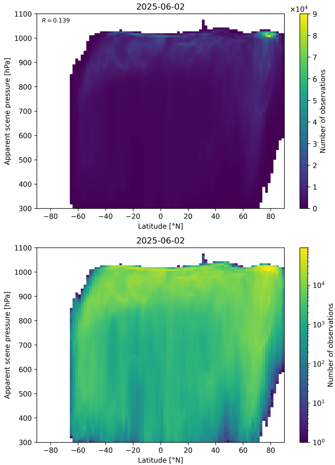
Figure 88: Scatter density plot of “Latitude” against “Apparent scene pressure” for 2025-06-01 to 2025-06-03.
