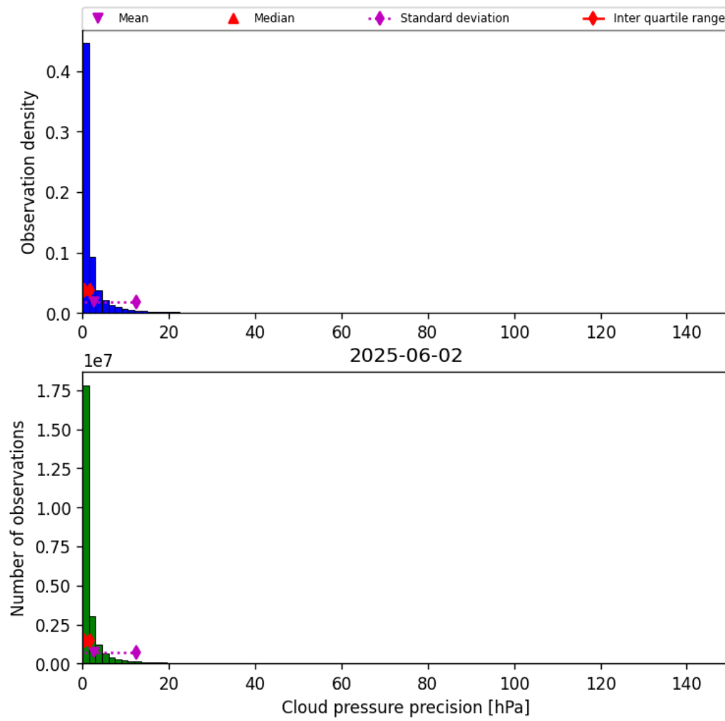
Figure 31: Histogram of “Cloud pressure precision” for 2025-06-01 to 2025-06-03
