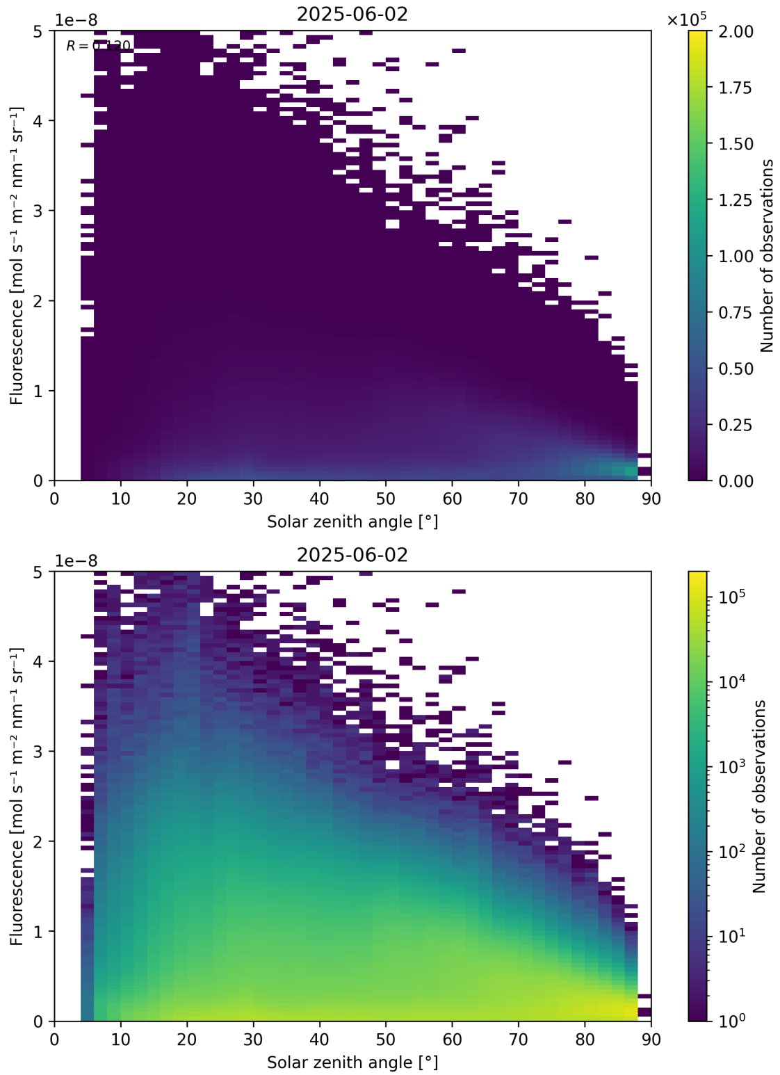
Figure 112: Scatter density plot of “Solar zenith angle” against “Fluorescence” for 2025-06-01 to 2025-06-03.
