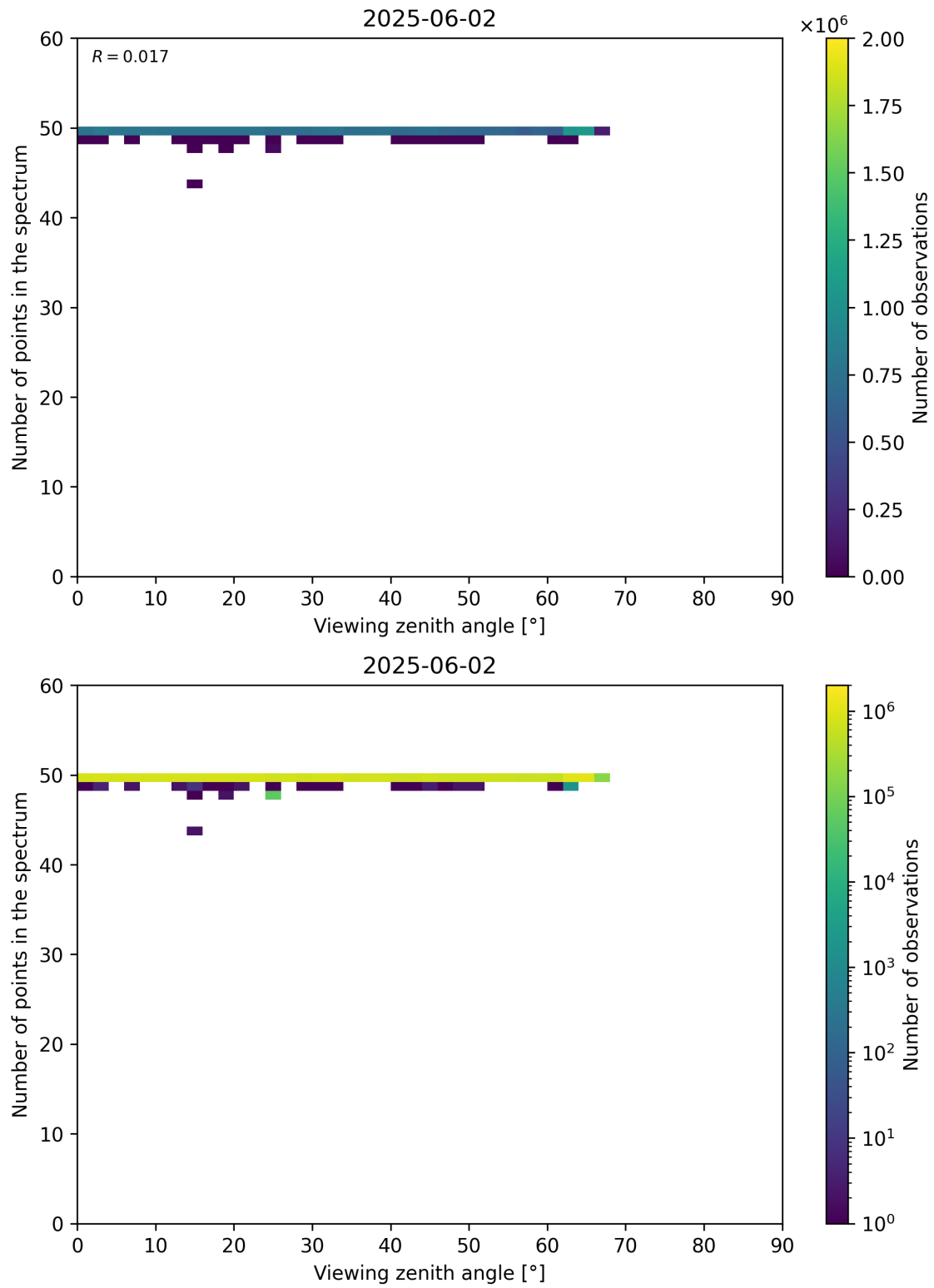
Figure 125: Scatter density plot of “Viewing zenith angle” against “Number of points in the spectrum” for 2025-06-01 to 2025-06-03.
