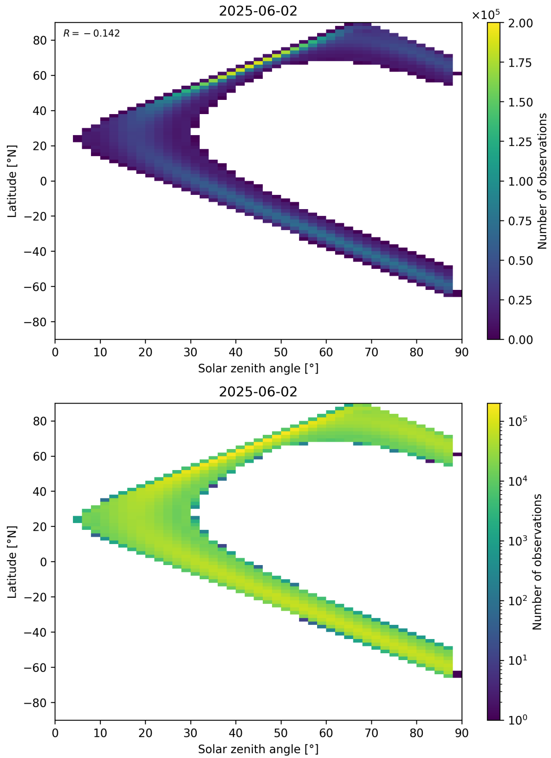
Figure 113: Scatter density plot of “Solar zenith angle” against “Latitude” for 2025-06-01 to 2025-06-03.
