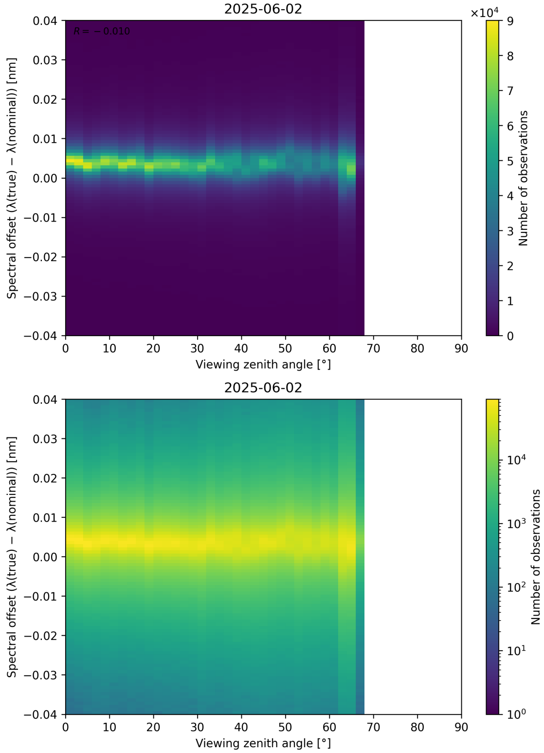
Figure 128: Scatter density plot of “Viewing zenith angle” against “Spectral offset ( \lambda_{\text{true}} - \lambda_{\text{nominal}} )” for 2025-06-01 to 2025-06-03.
