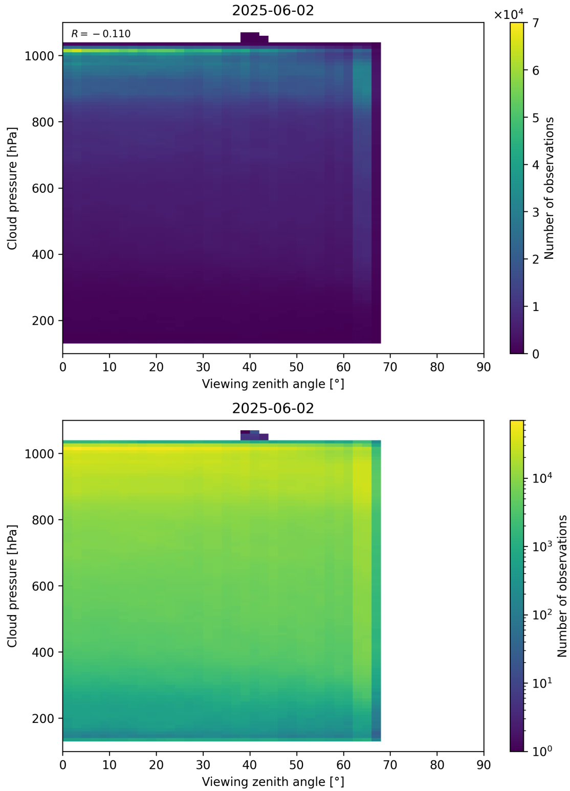
Figure 121: Scatter density plot of “Viewing zenith angle” against “Cloud pressure” for 2025-06-01 to 2025-06-03.
