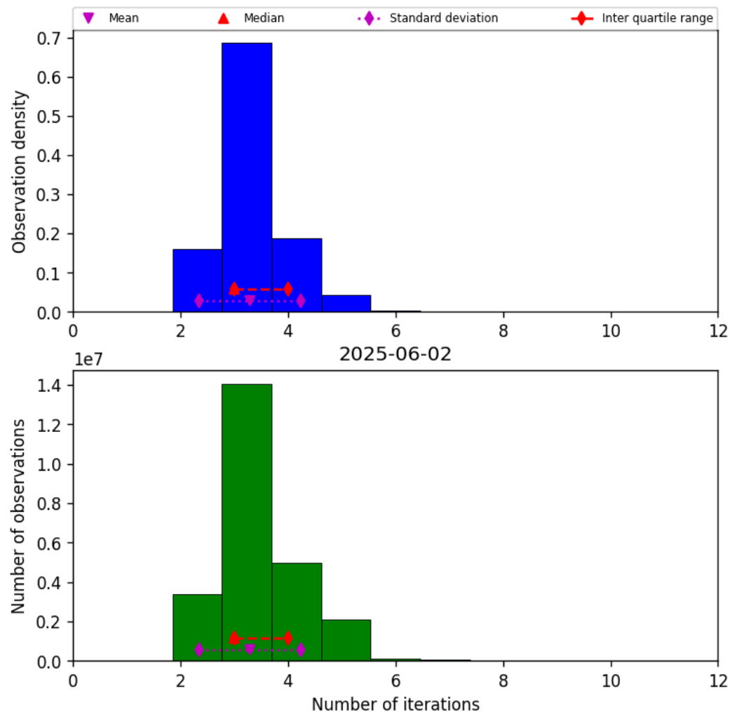
Figure 39: Histogram of “Number of iterations” for 2025-06-01 to 2025-06-03
