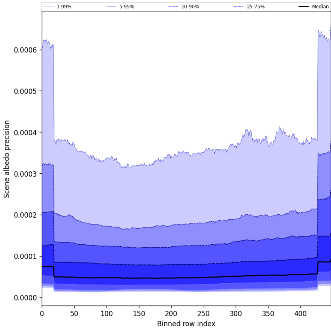
Figure 52: Along track statistics of “Scene albedo precision” for 2025-06-01 to 2025-06-03
