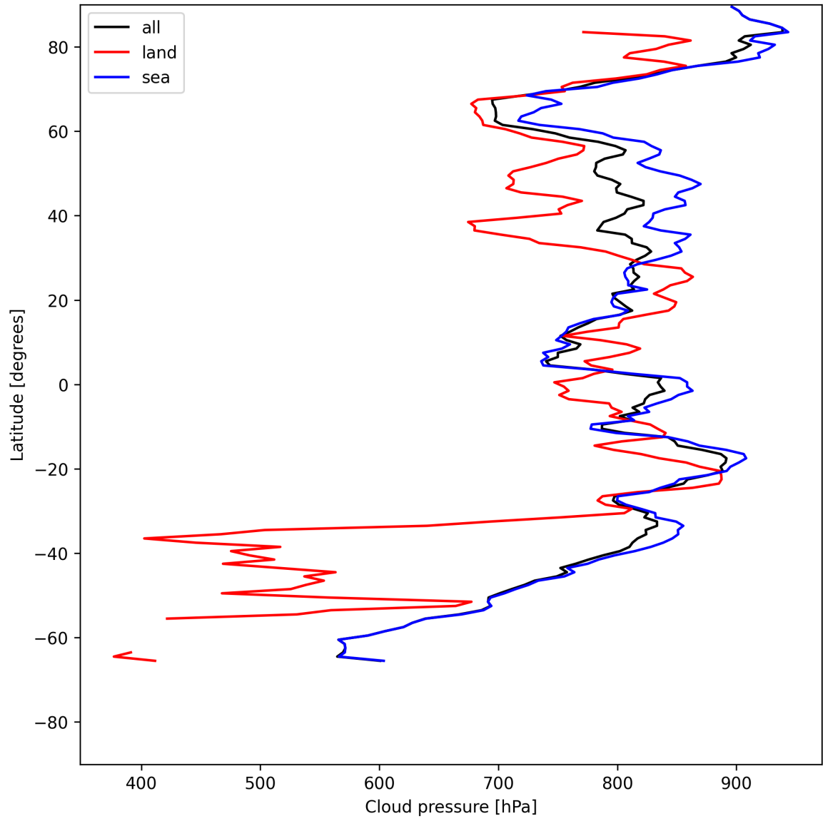
Figure 13: Zonal average of “Cloud pressure” for 2025-06-01 to 2025-06-03.
