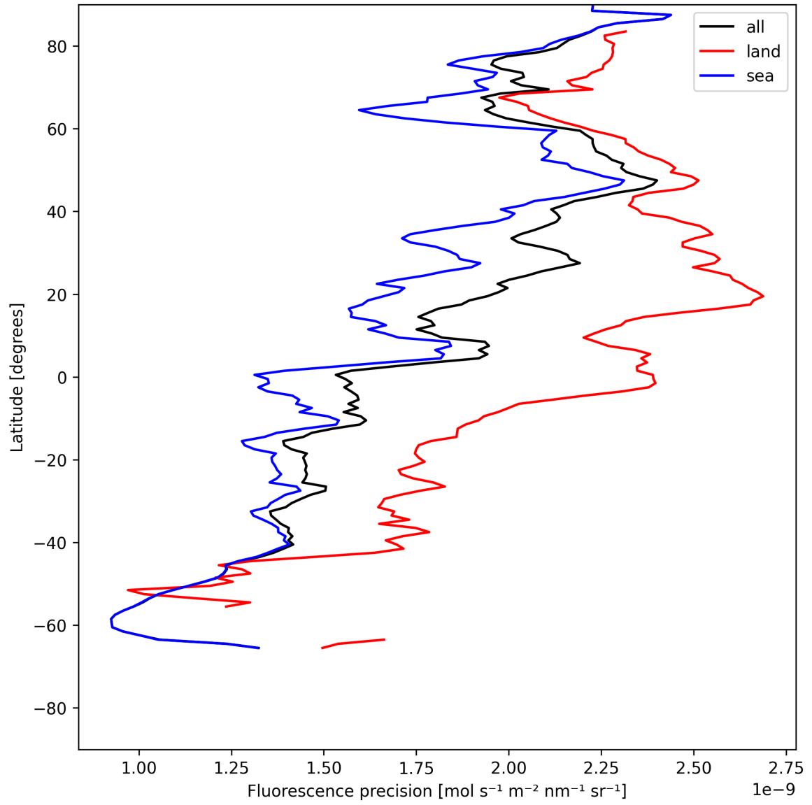
Figure 24: Zonal average of “Fluorescence precision” for 2025-06-01 to 2025-06-03.
