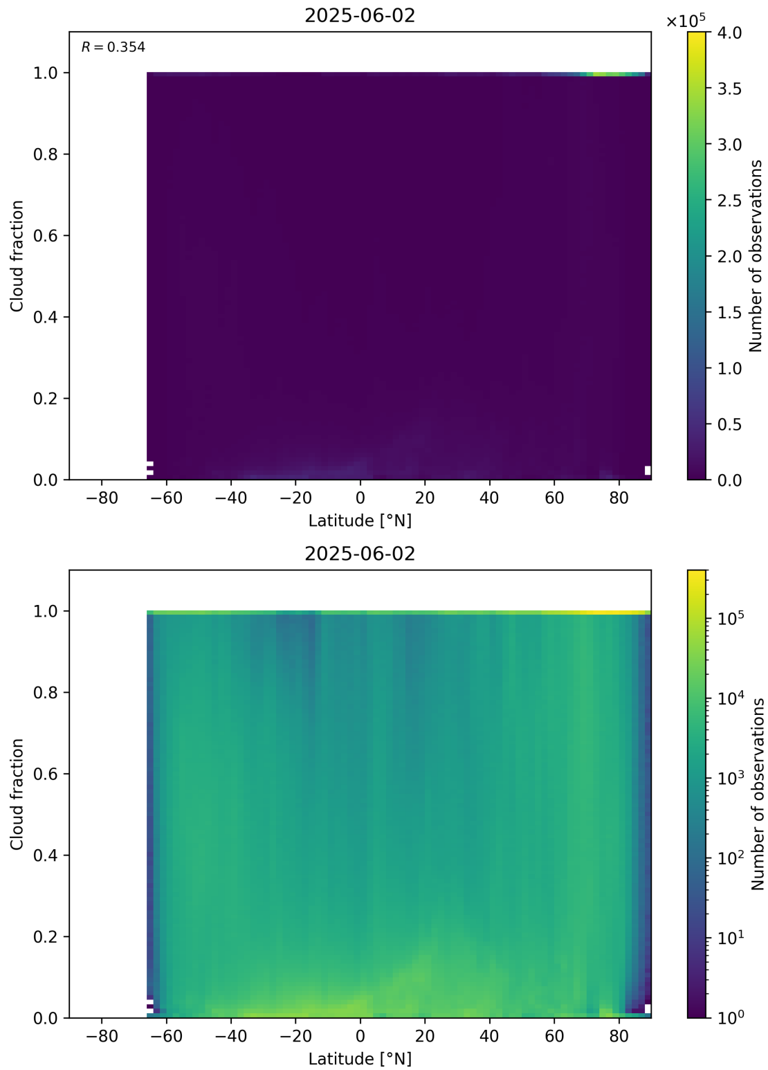
Figure 90: Scatter density plot of “Latitude” against “Cloud fraction” for 2025-06-01 to 2025-06-03.
