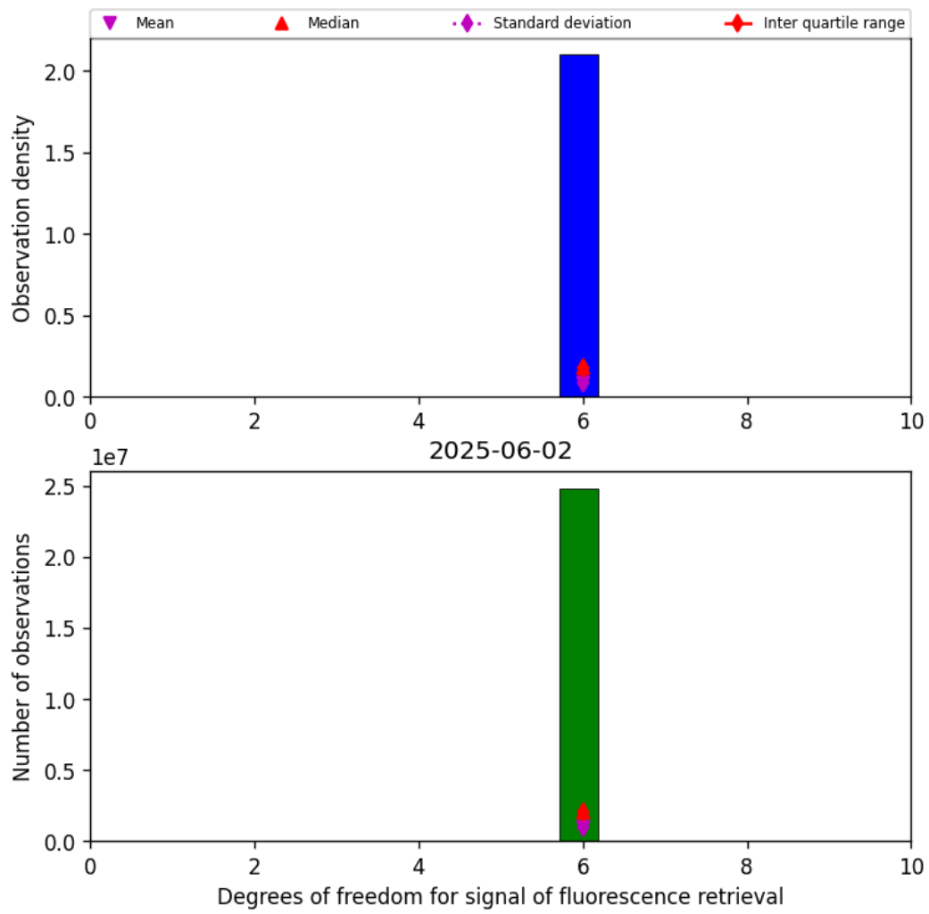
Figure 43: Histogram of “Degrees of freedom for signal of fluorescence retrieval” for 2025-06-01 to 2025-06-03
