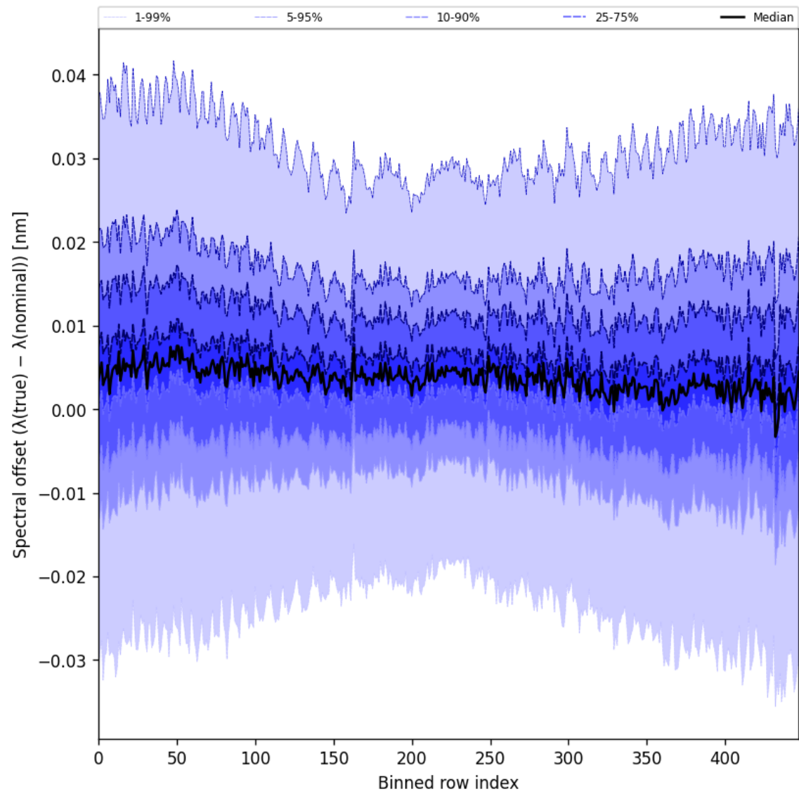
Figure 62: Along track statistics of “Spectral offset ( \lambda_{\text{true}} - \lambda_{\text{nominal}} )” for 2025-06-01 to 2025-06-03
