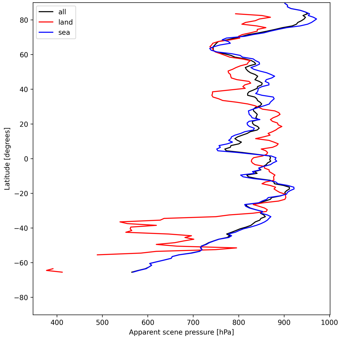
Figure 19: Zonal average of “Apparent scene pressure” for 2025-06-01 to 2025-06-03.
