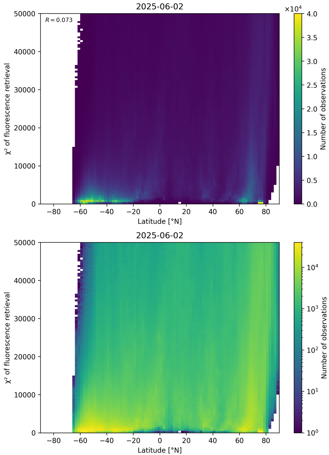
Figure 89: Scatter density plot of “Latitude” against “ \chi^2 of fluorescence retrieval” for 2025-06-01 to 2025-06-03.
