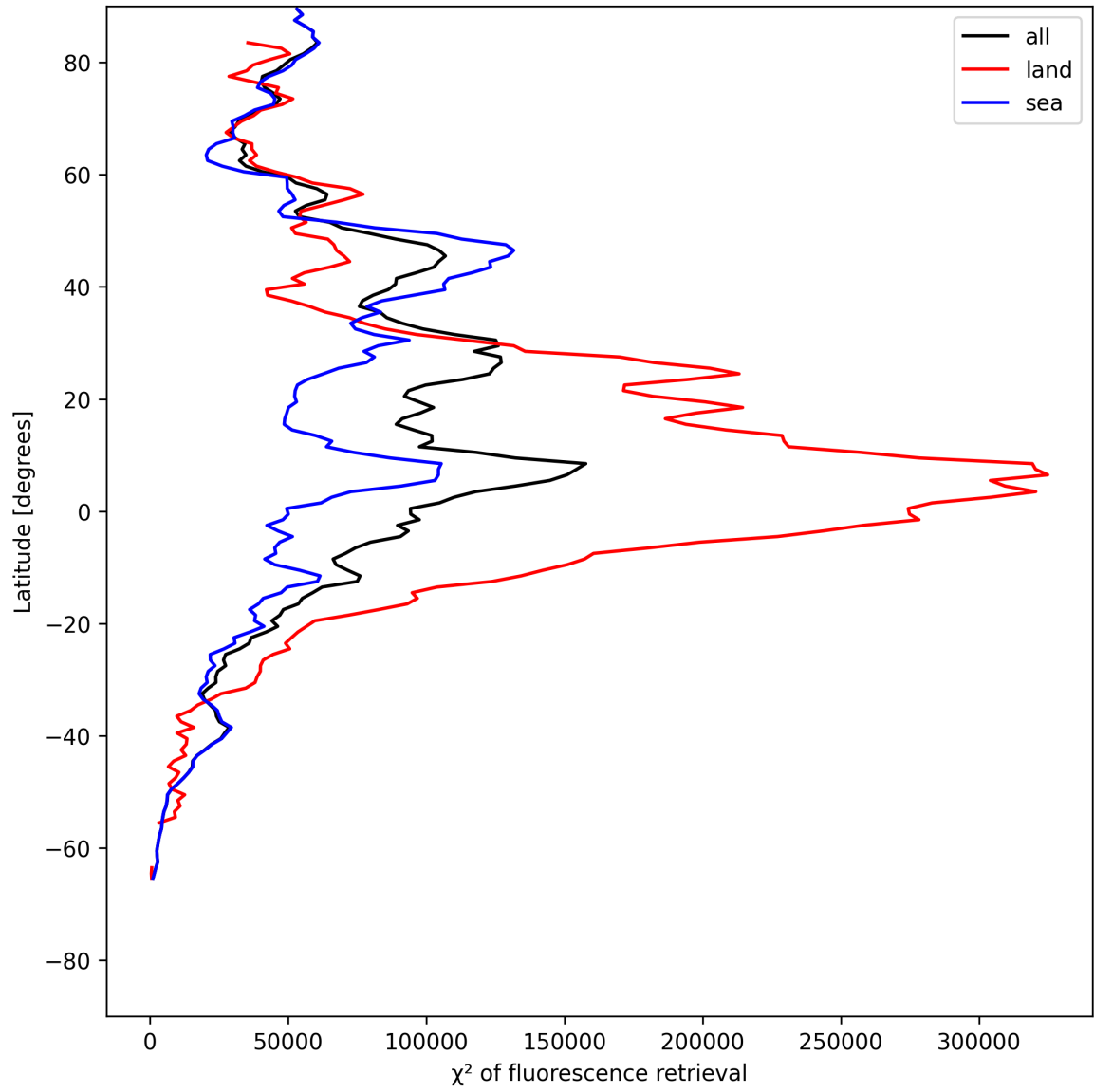
Figure 25: Zonal average of “ \chi^2 of fluorescence retrieval” for 2025-06-01 to 2025-06-03.
