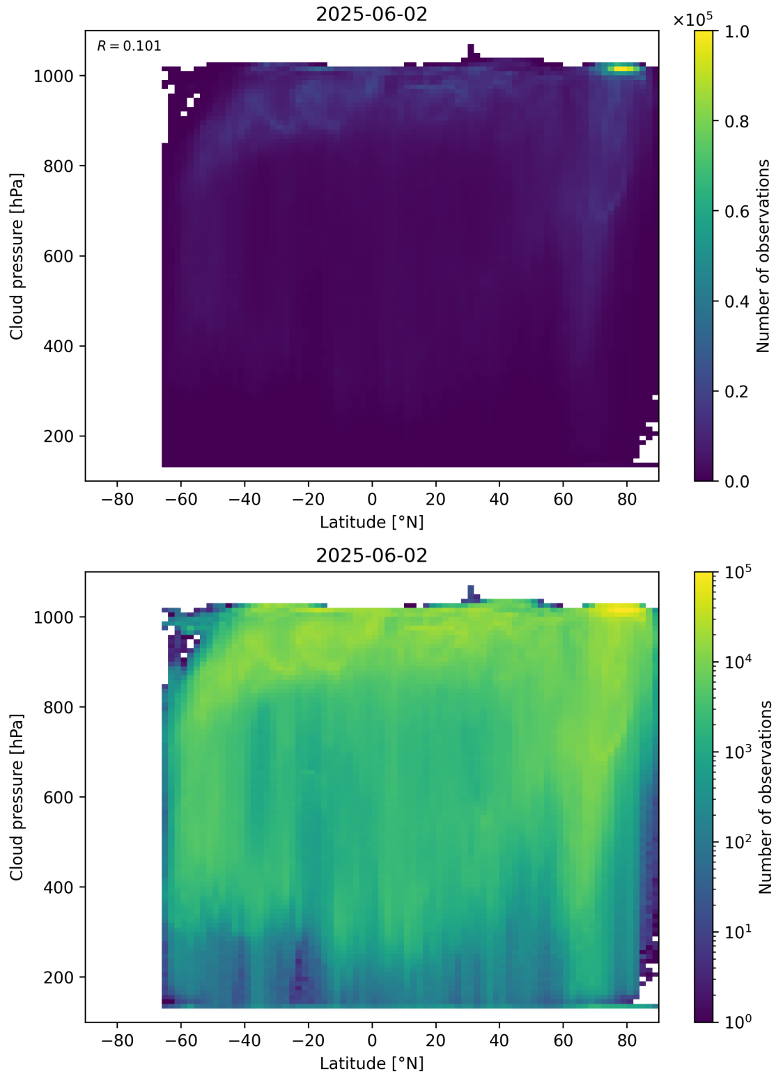
Figure 91: Scatter density plot of “Latitude” against “Cloud pressure” for 2025-06-01 to 2025-06-03.
