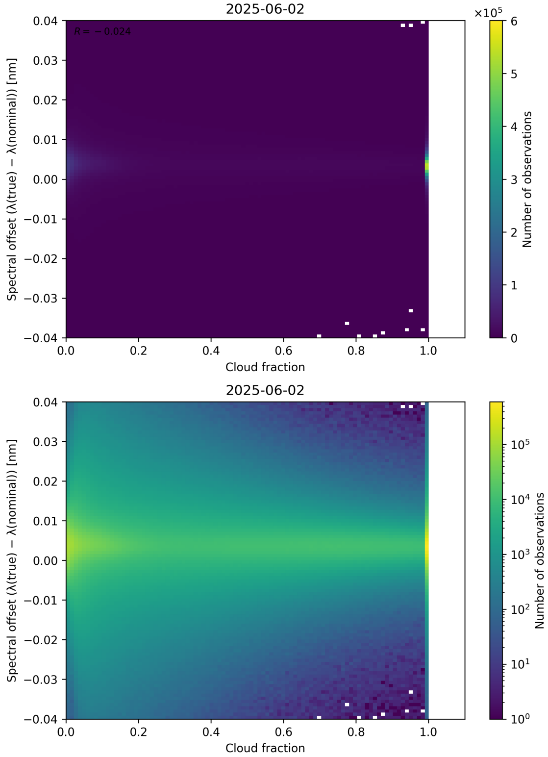
Figure 76: Scatter density plot of “Cloud fraction” against “Spectral offset ( \lambda_{\text{true}} - \lambda_{\text{nominal}} )” for 2025-06-01 to 2025-06-03.
