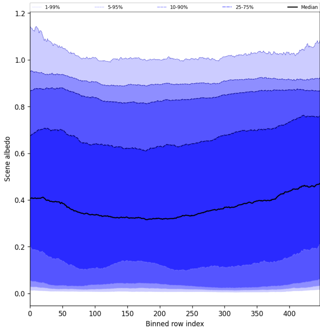
Figure 51: Along track statistics of “Scene albedo” for 2025-06-01 to 2025-06-03
