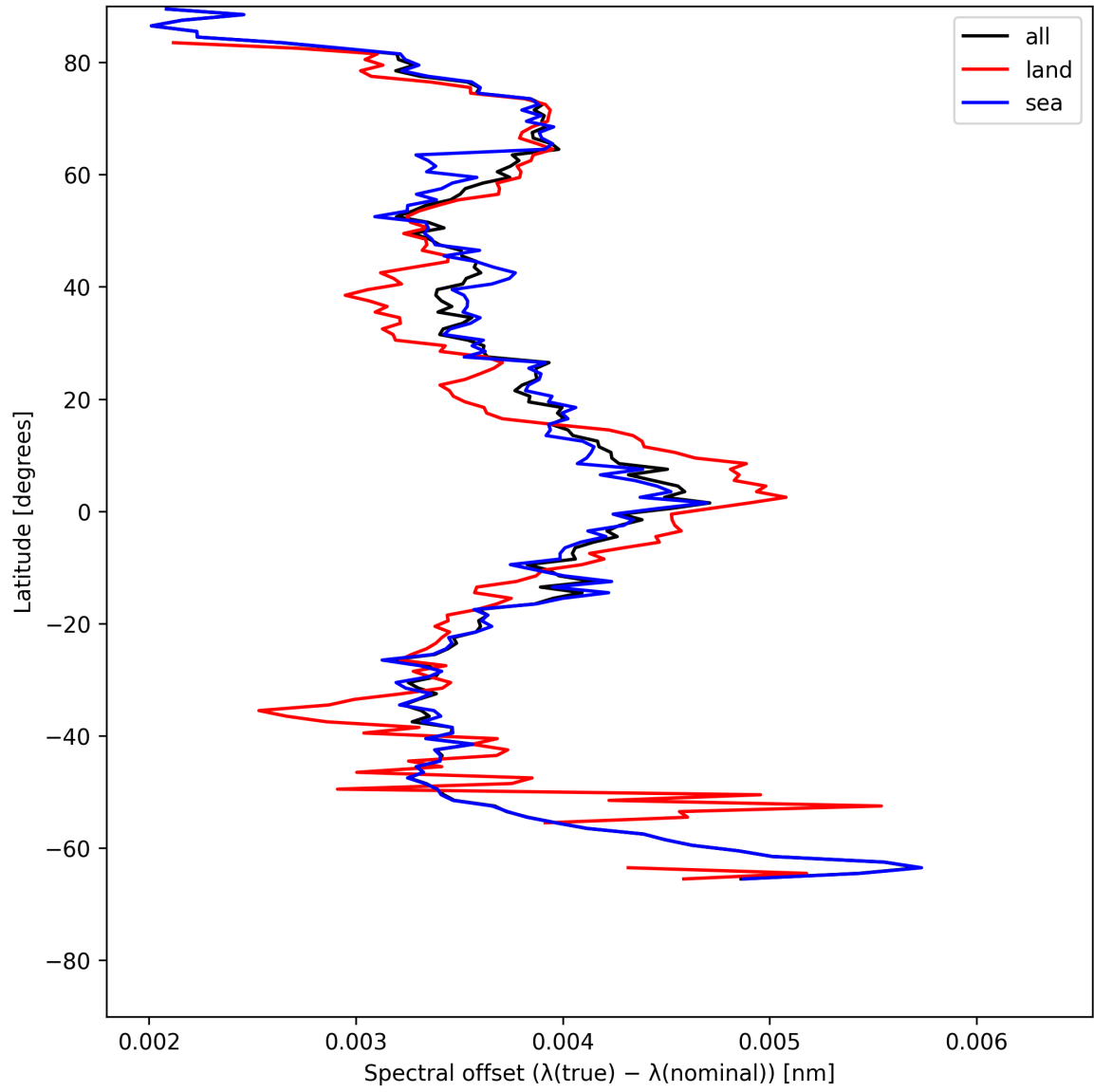
Figure 28: Zonal average of “Spectral offset ( \lambda_{\text{true}} - \lambda_{\text{nominal}} )” for 2025-06-01 to 2025-06-03.
