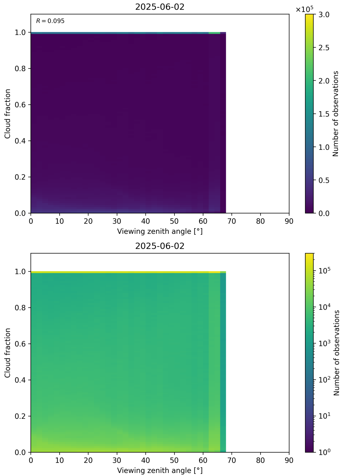
Figure 120: Scatter density plot of “Viewing zenith angle” against “Cloud fraction” for 2025-06-01 to 2025-06-03.
