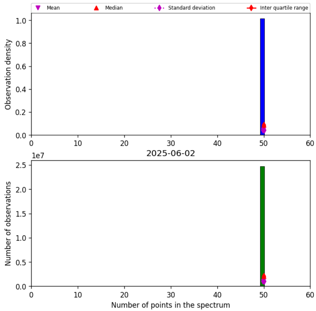
Figure 44: Histogram of “Number of points in the spectrum” for 2025-06-01 to 2025-06-03
