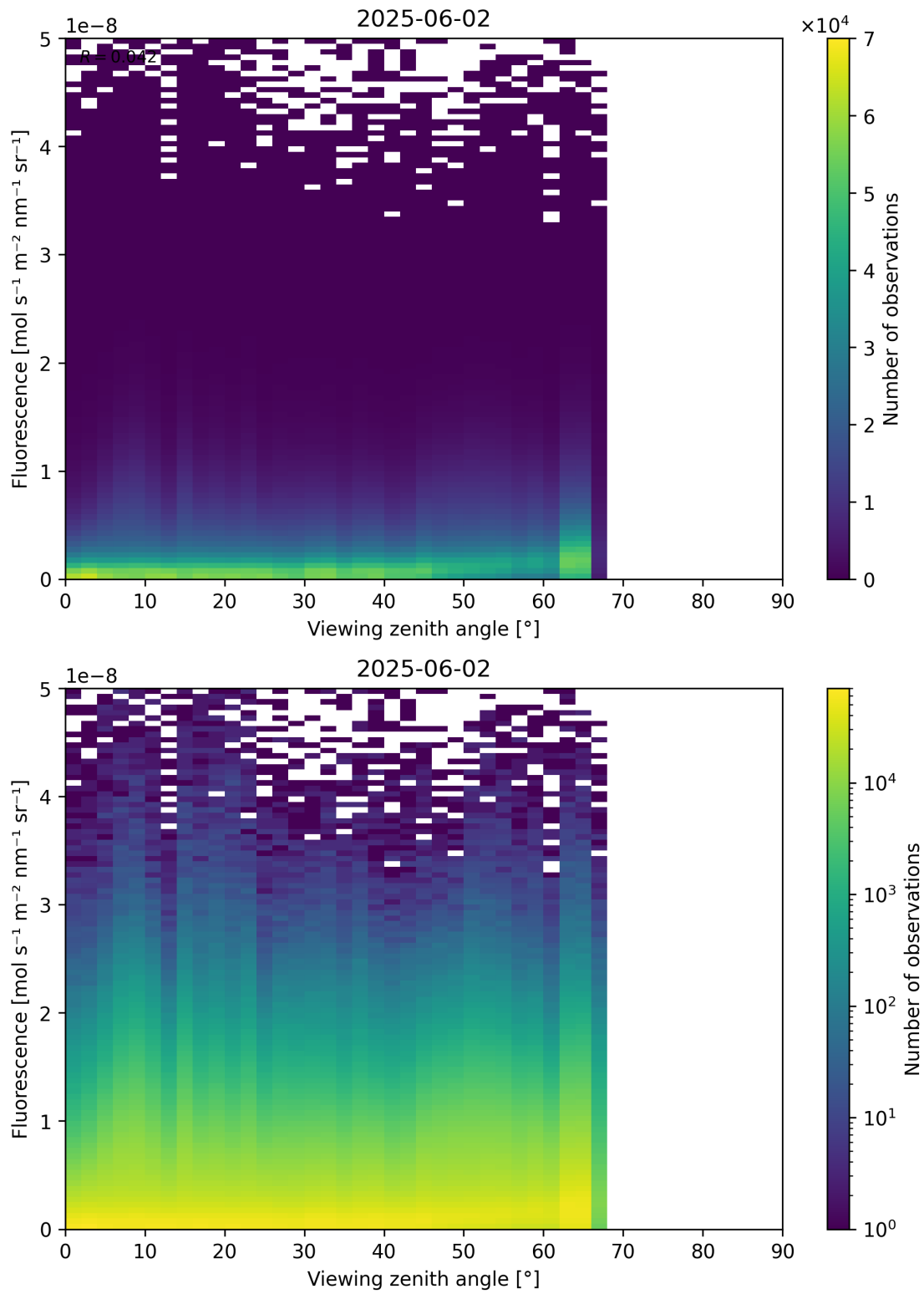
Figure 122: Scatter density plot of “Viewing zenith angle” against “Fluorescence” for 2025-06-01 to 2025-06-03.
