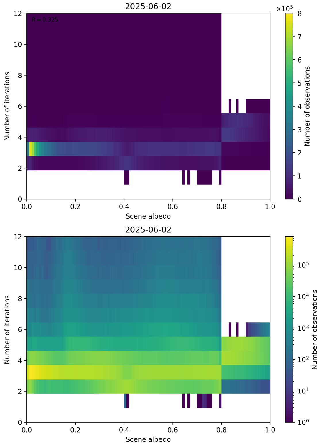
Figure 105: Scatter density plot of “Scene albedo” against “Number of iterations” for 2025-06-01 to 2025-06-03.
