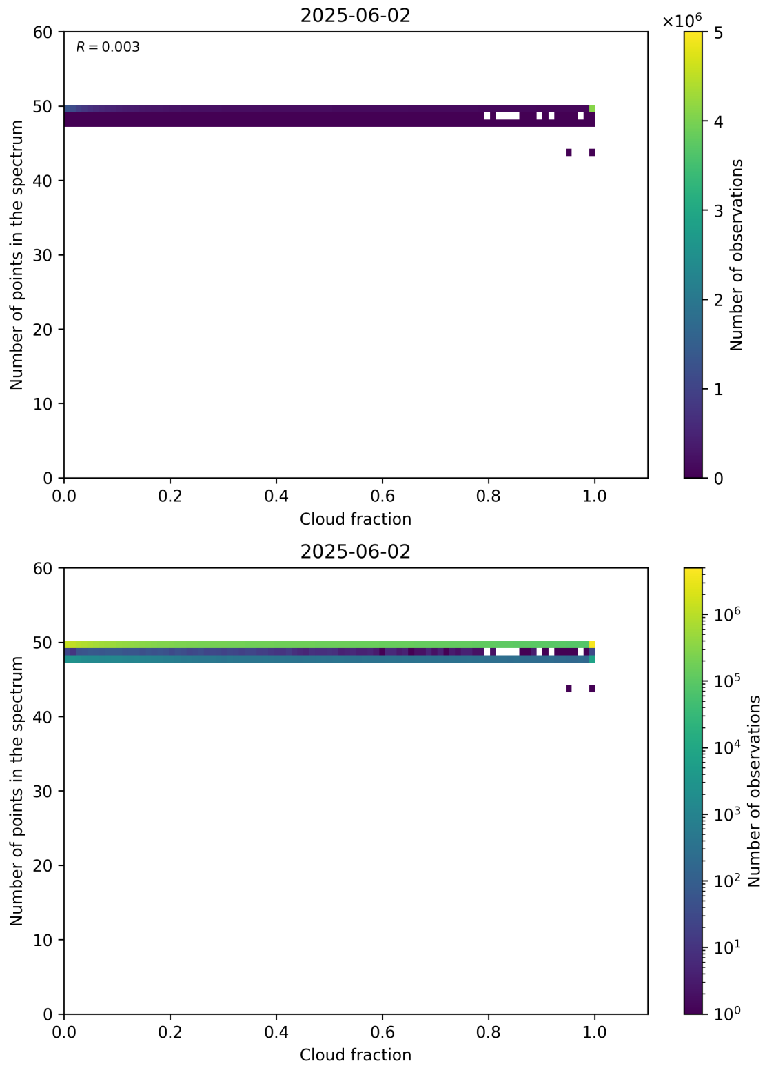
Figure 74: Scatter density plot of “Cloud fraction” against “Number of points in the spectrum” for 2025-06-01 to 2025-06-03.
