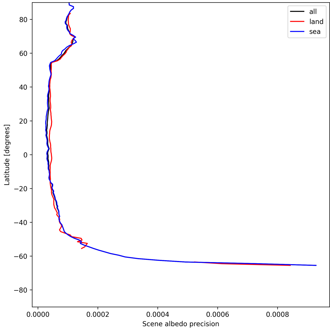
Figure 18: Zonal average of “Scene albedo precision” for 2025-06-01 to 2025-06-03.
