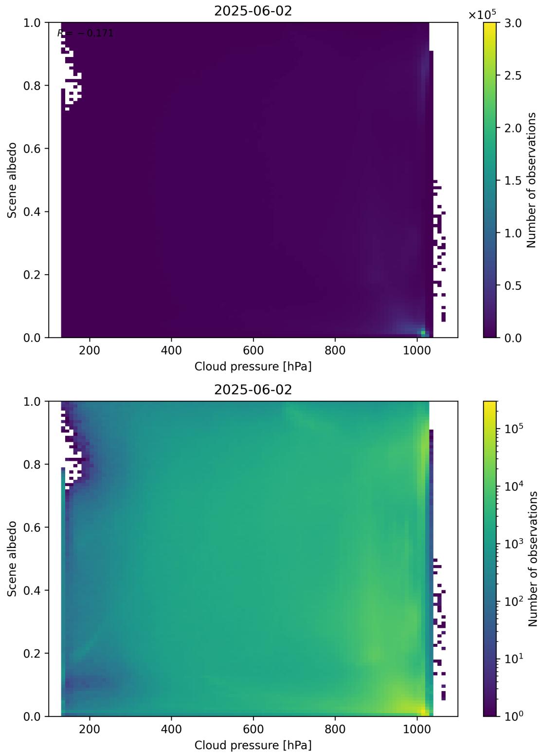
Figure 83: Scatter density plot of “Cloud pressure” against “Scene albedo” for 2025-06-01 to 2025-06-03.
