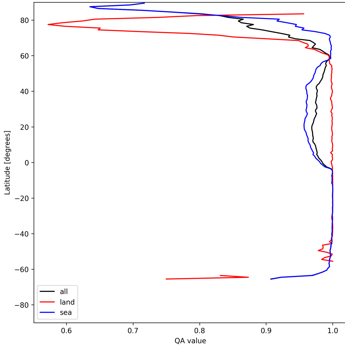
Figure 12: Zonal average of “QA value” for 2025-06-01 to 2025-06-03.
