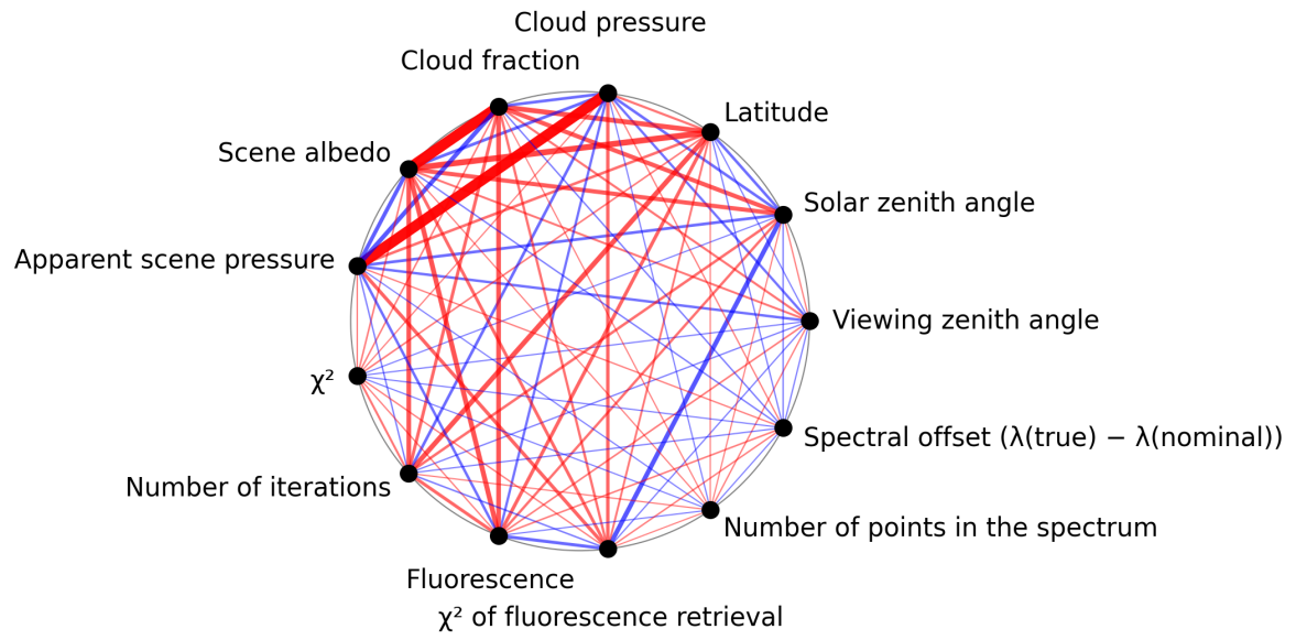
Figure 1: Map of correlation graph for 2025-06-01 to 2025-06-03.
