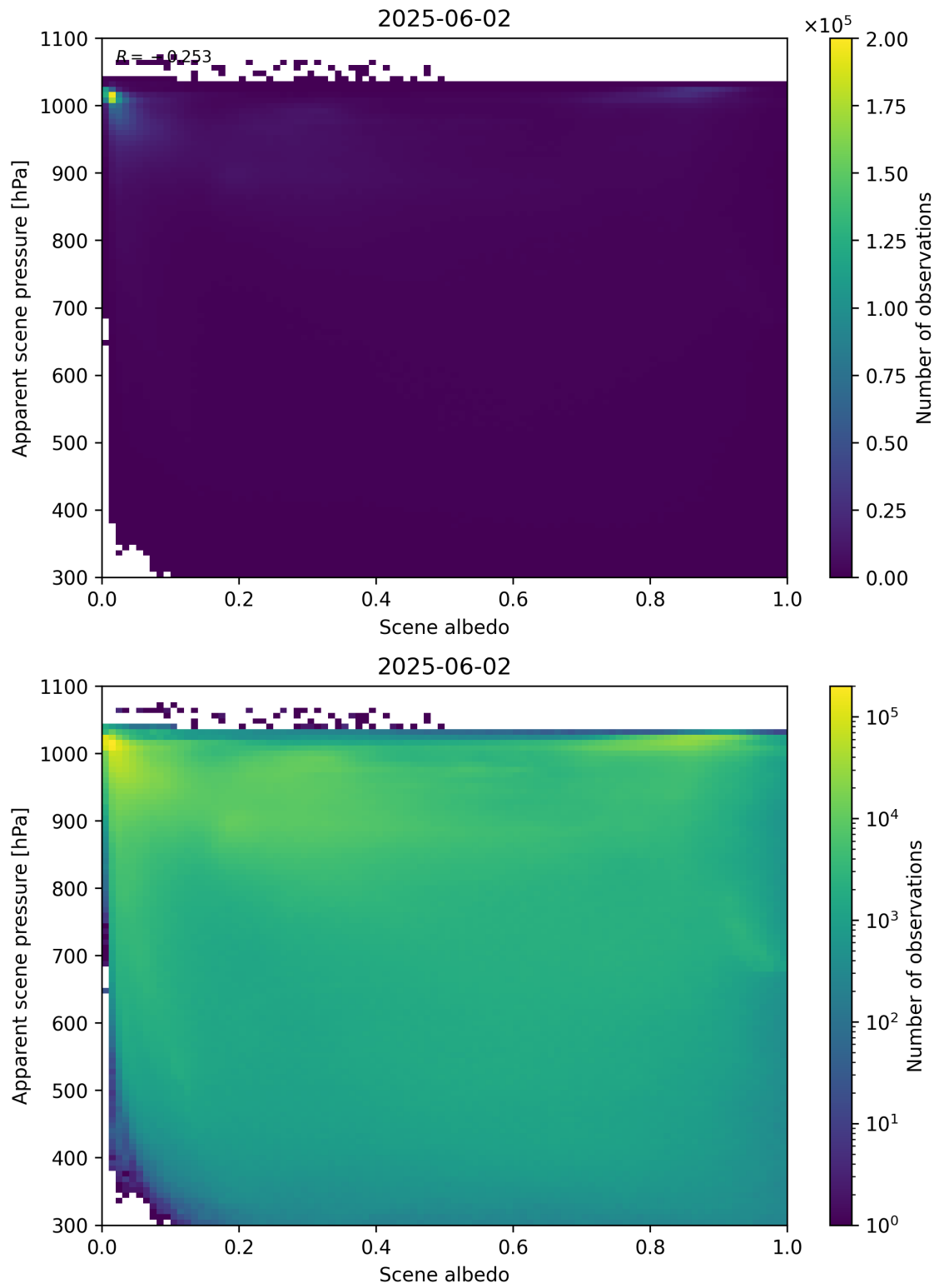
Figure 102: Scatter density plot of “Scene albedo” against “Apparent scene pressure” for 2025-06-01 to 2025-06-03.
