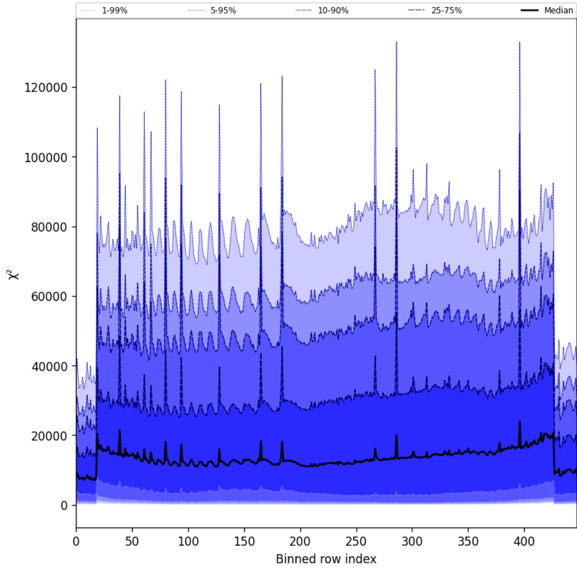
Figure 55: Along track statistics of “ \chi^2 ” for 2025-06-01 to 2025-06-03
