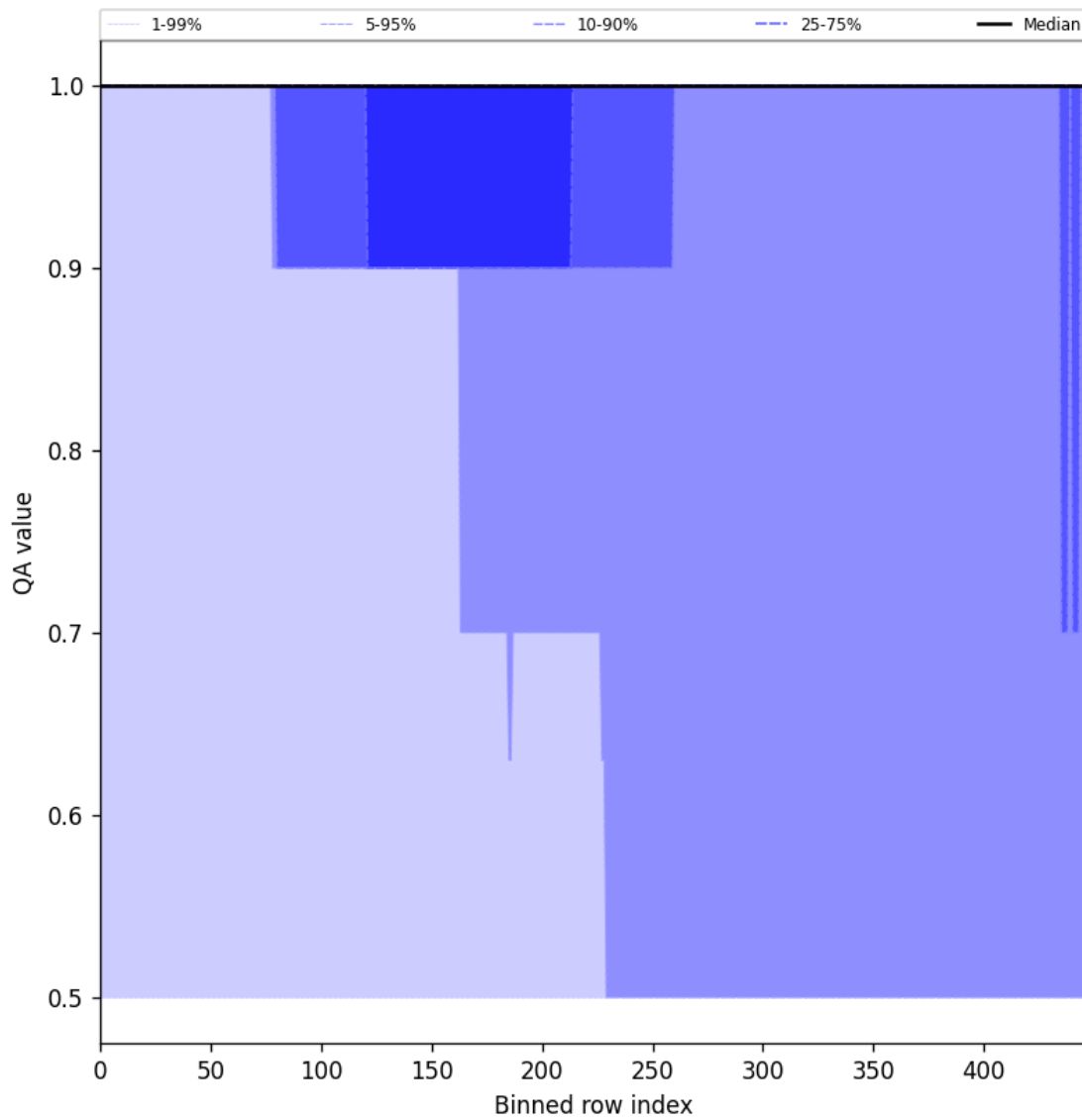
Figure 46: Along track statistics of “QA value” for 2025-06-01 to 2025-06-03
