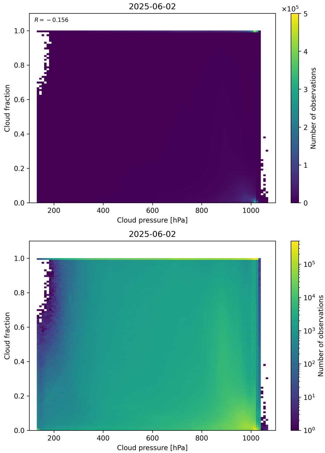
Figure 79: Scatter density plot of “Cloud pressure” against “Cloud fraction” for 2025-06-01 to 2025-06-03.
