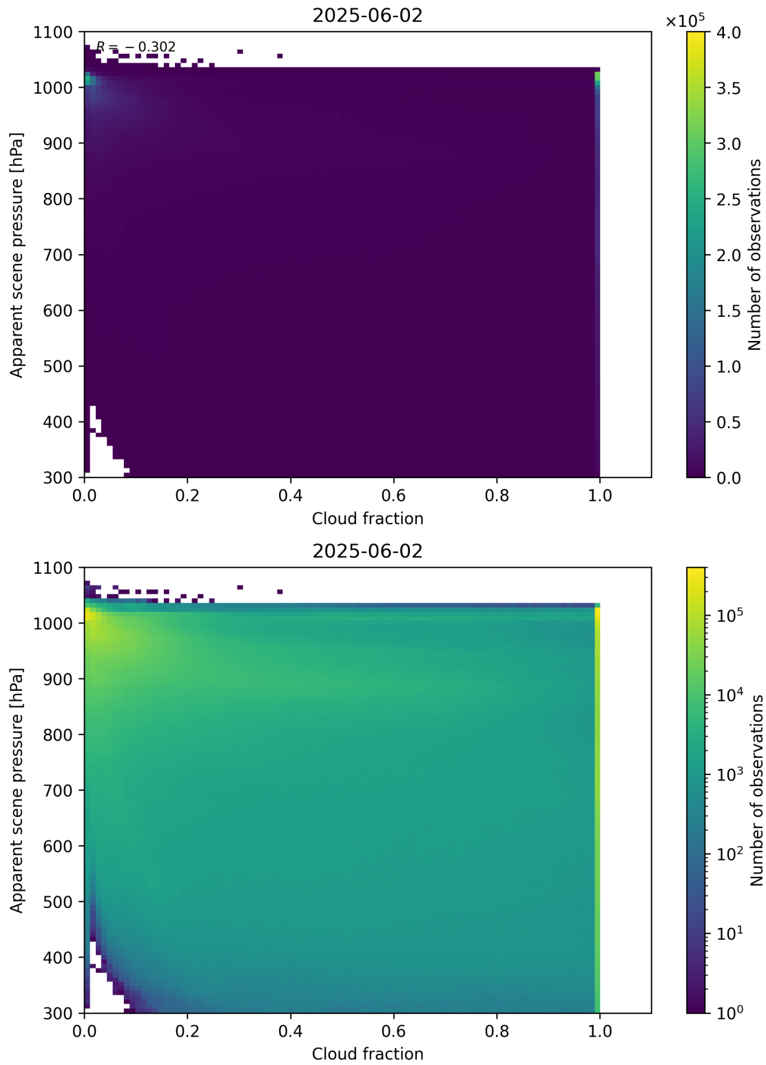
Figure 70: Scatter density plot of “Cloud fraction” against “Apparent scene pressure” for 2025-06-01 to 2025-06-03.
