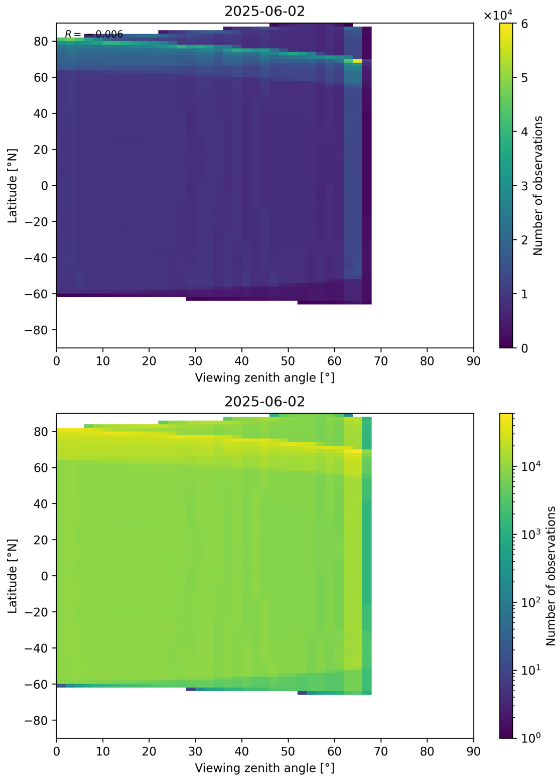
Figure 123: Scatter density plot of “Viewing zenith angle” against “Latitude” for 2025-06-01 to 2025-06-03.
