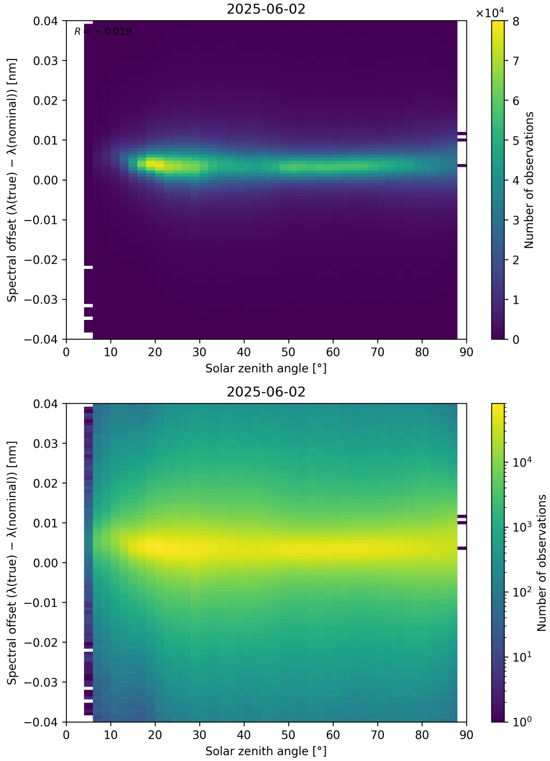
Figure 117: Scatter density plot of “Solar zenith angle” against “Spectral offset ( \lambda_{\text{true}} - \lambda_{\text{nominal}} )” for 2025-06-01 to 2025-06-03.
