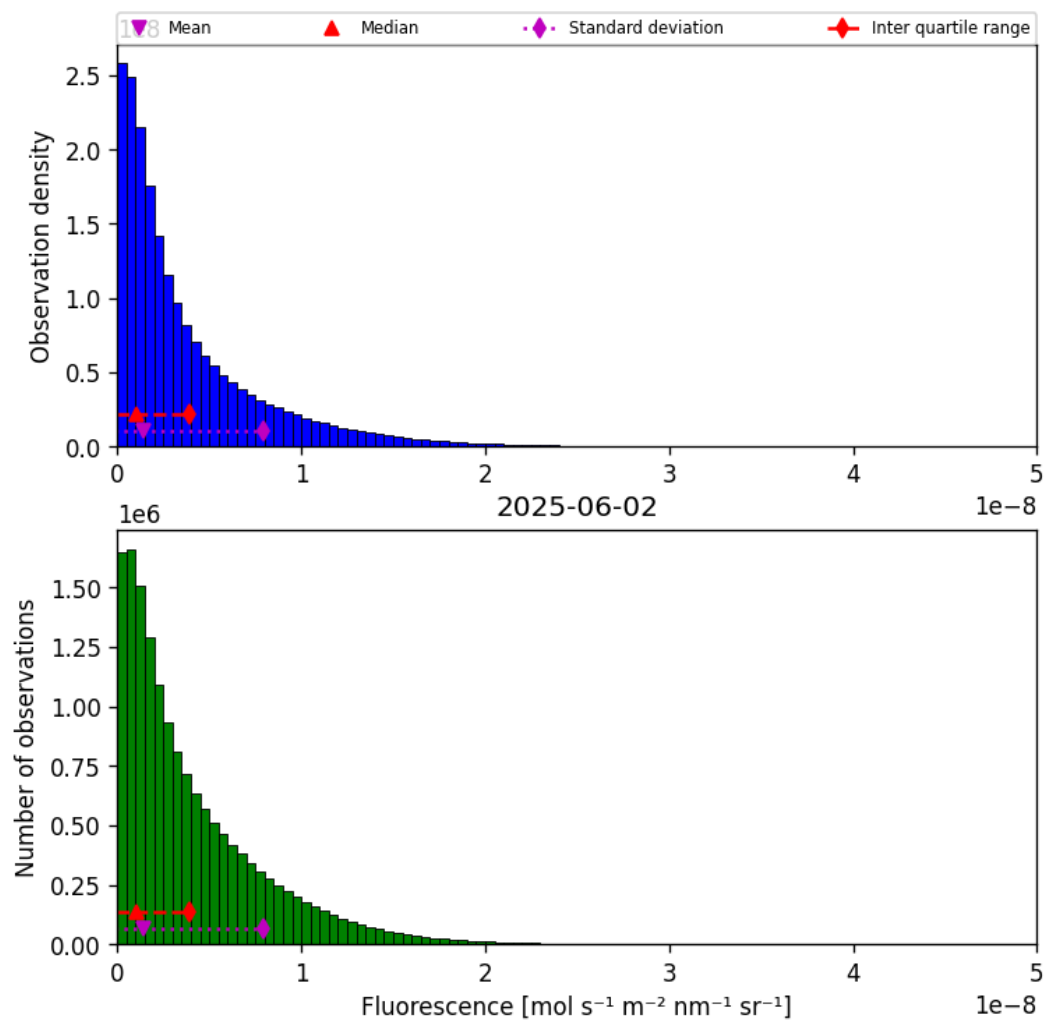
Figure 40: Histogram of “Fluorescence” for 2025-06-01 to 2025-06-03
