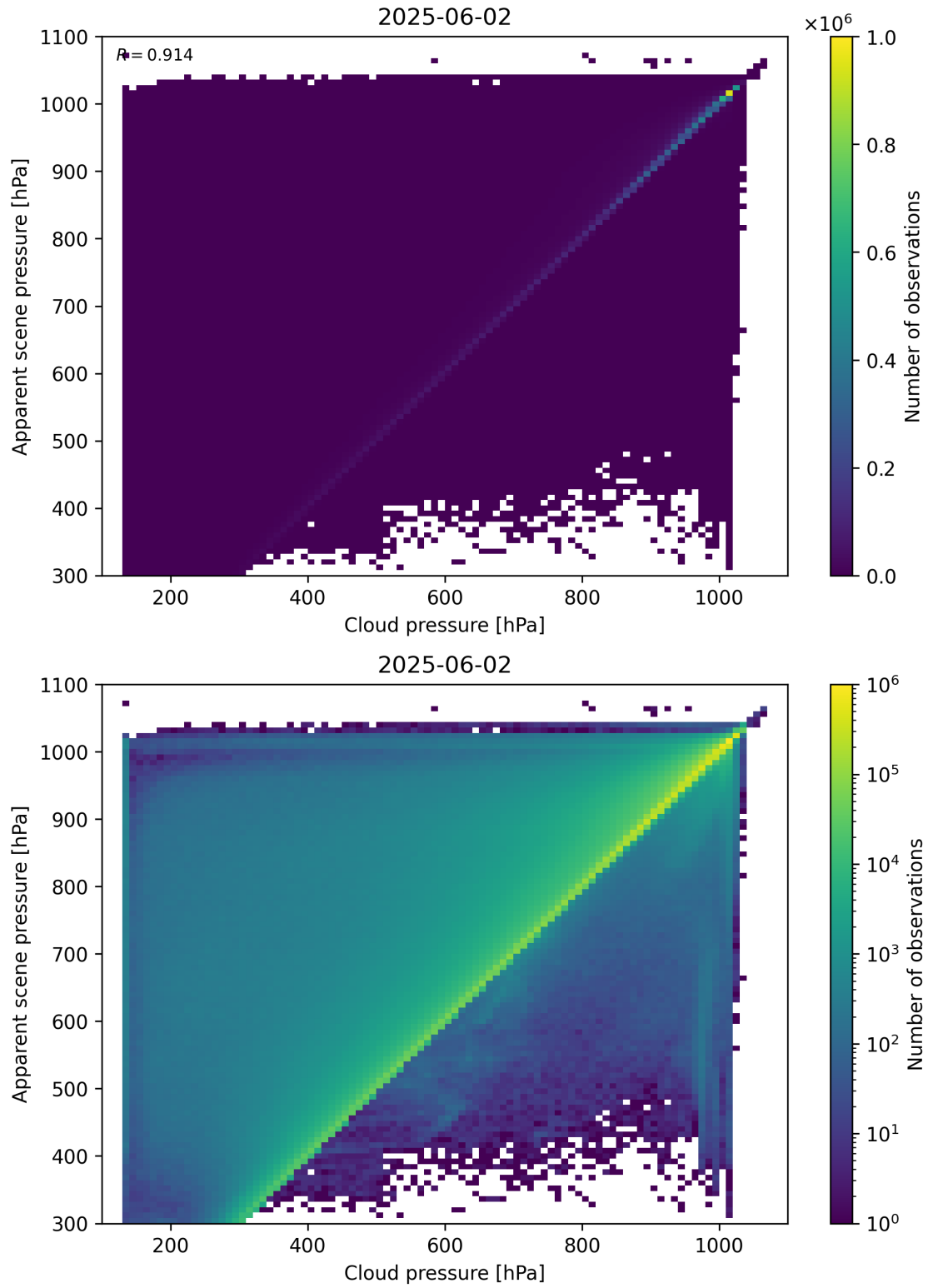
Figure 77: Scatter density plot of “Cloud pressure” against “Apparent scene pressure” for 2025-06-01 to 2025-06-03.
