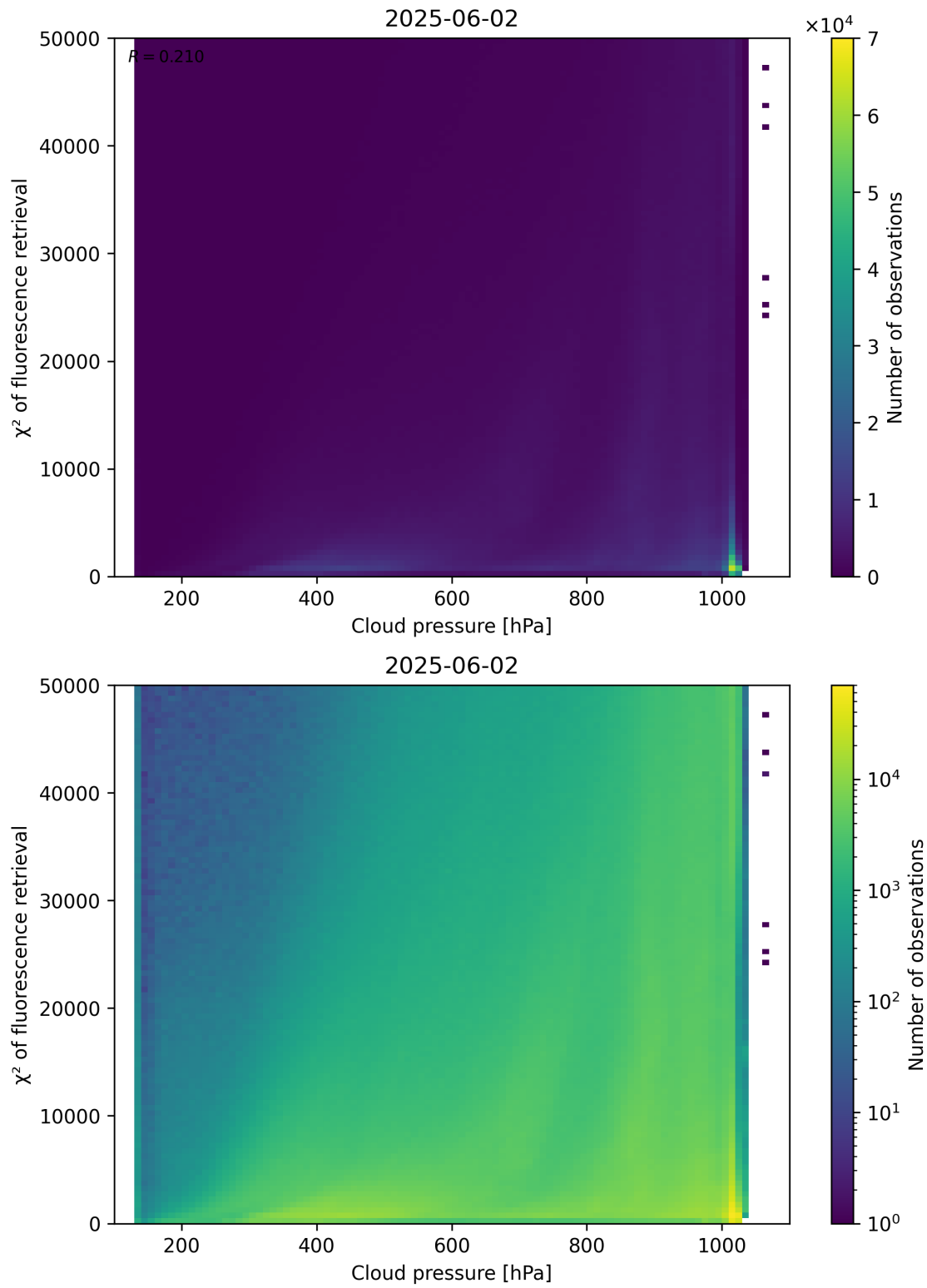
Figure 78: Scatter density plot of “Cloud pressure” against “ \chi^2 of fluorescence retrieval” for 2025-06-01 to 2025-06-03.
