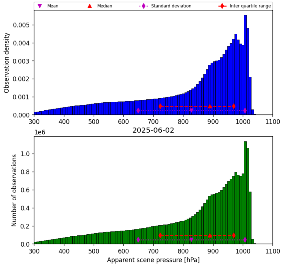
Figure 36: Histogram of “Apparent scene pressure” for 2025-06-01 to 2025-06-03
