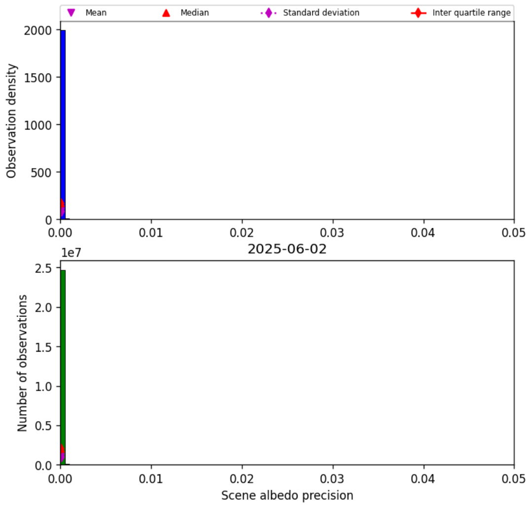
Figure 35: Histogram of “Scene albedo precision” for 2025-06-01 to 2025-06-03
