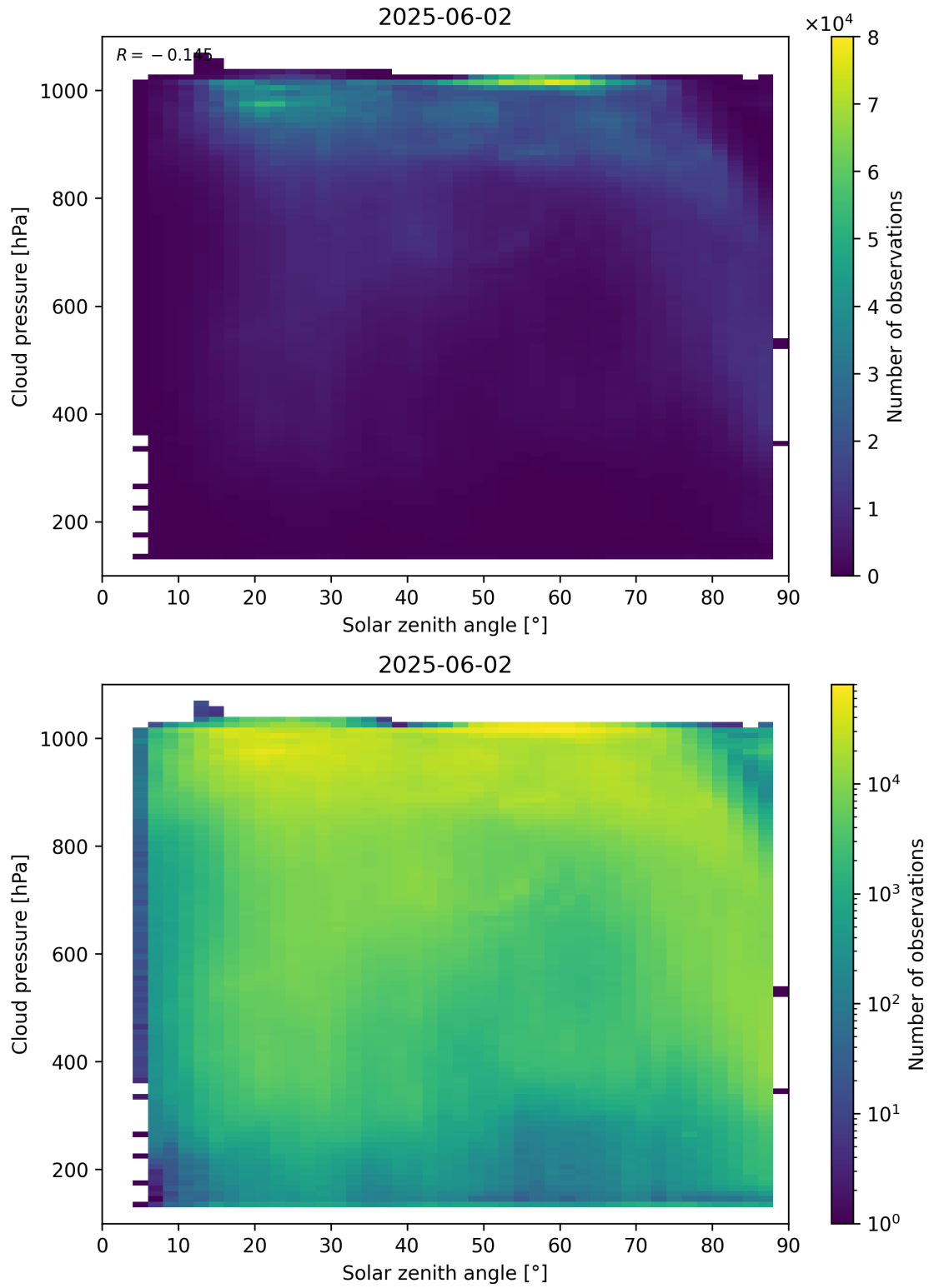
Figure 111: Scatter density plot of “Solar zenith angle” against “Cloud pressure” for 2025-06-01 to 2025-06-03.
