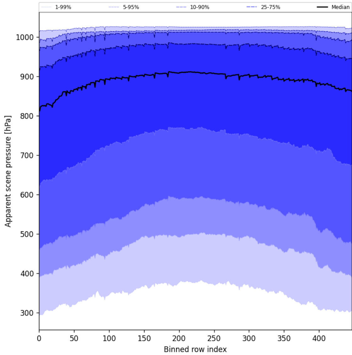
Figure 53: Along track statistics of “Apparent scene pressure” for 2025-06-01 to 2025-06-03
