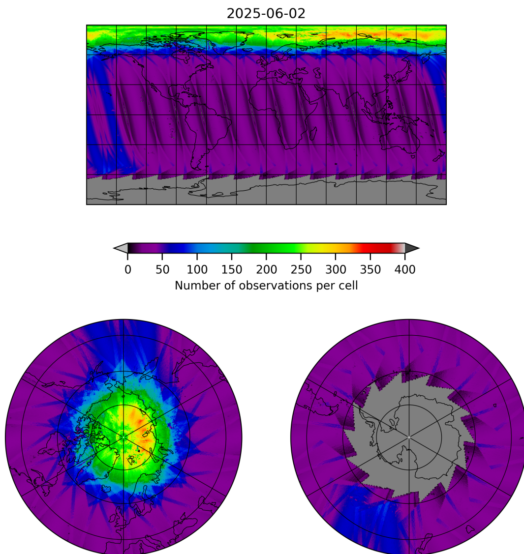
Figure 11: Map of the number of observations for 2025-06-01 to 2025-06-03
