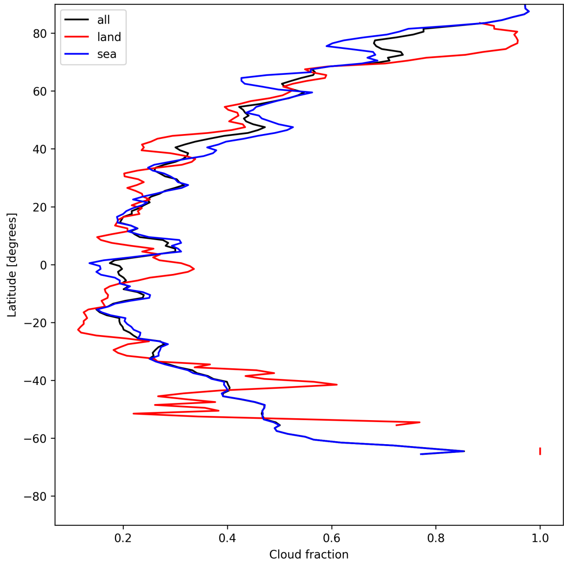
Figure 15: Zonal average of “Cloud fraction” for 2025-06-01 to 2025-06-03.
