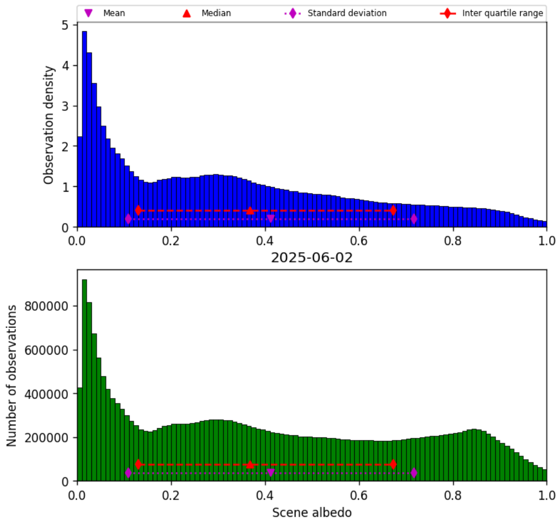
Figure 34: Histogram of “Scene albedo” for 2025-06-01 to 2025-06-03
