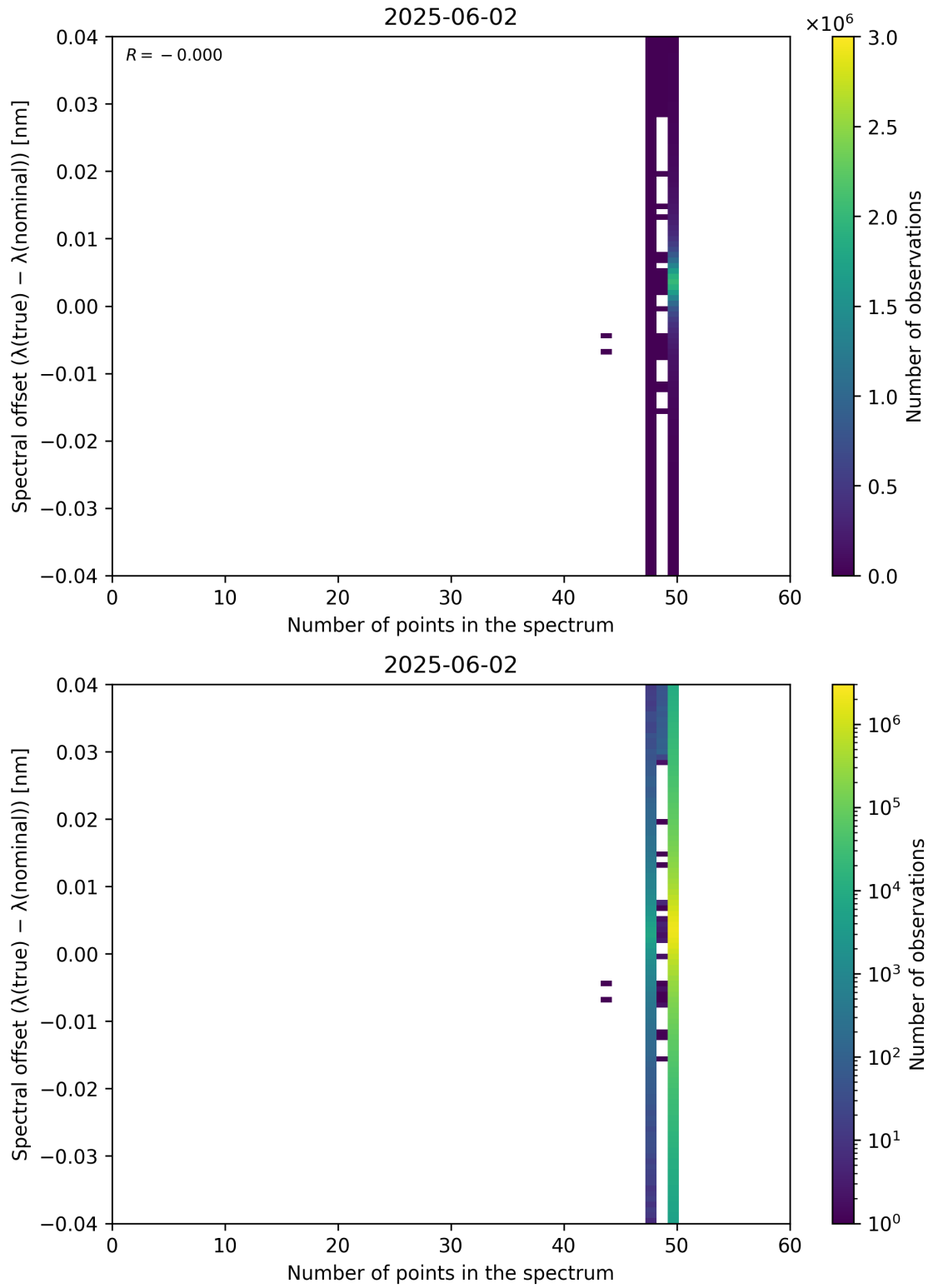
Figure 101: Scatter density plot of “Number of points in the spectrum” against “Spectral offset ( \lambda_{\text{true}} - \lambda_{\text{nominal}} )” for 2025-06-01 to 2025-06-03.
