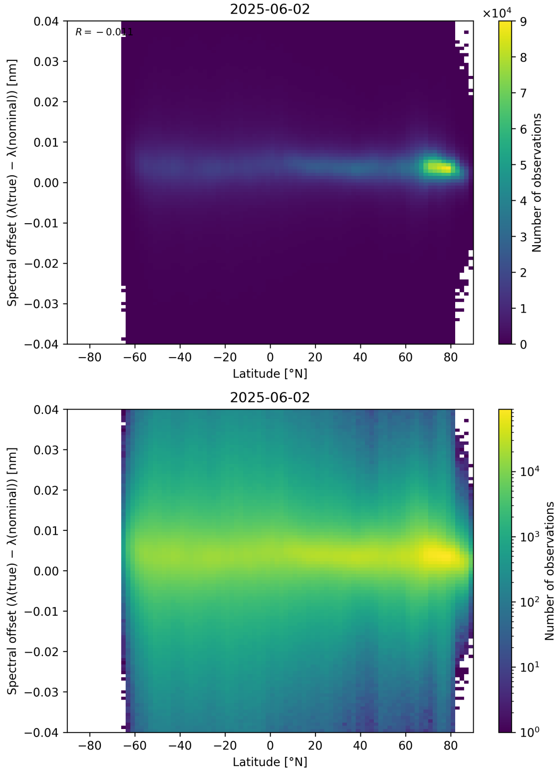
Figure 96: Scatter density plot of “Latitude” against “Spectral offset ( \lambda_{\text{true}} - \lambda_{\text{nominal}} )” for 2025-06-01 to 2025-06-03.
