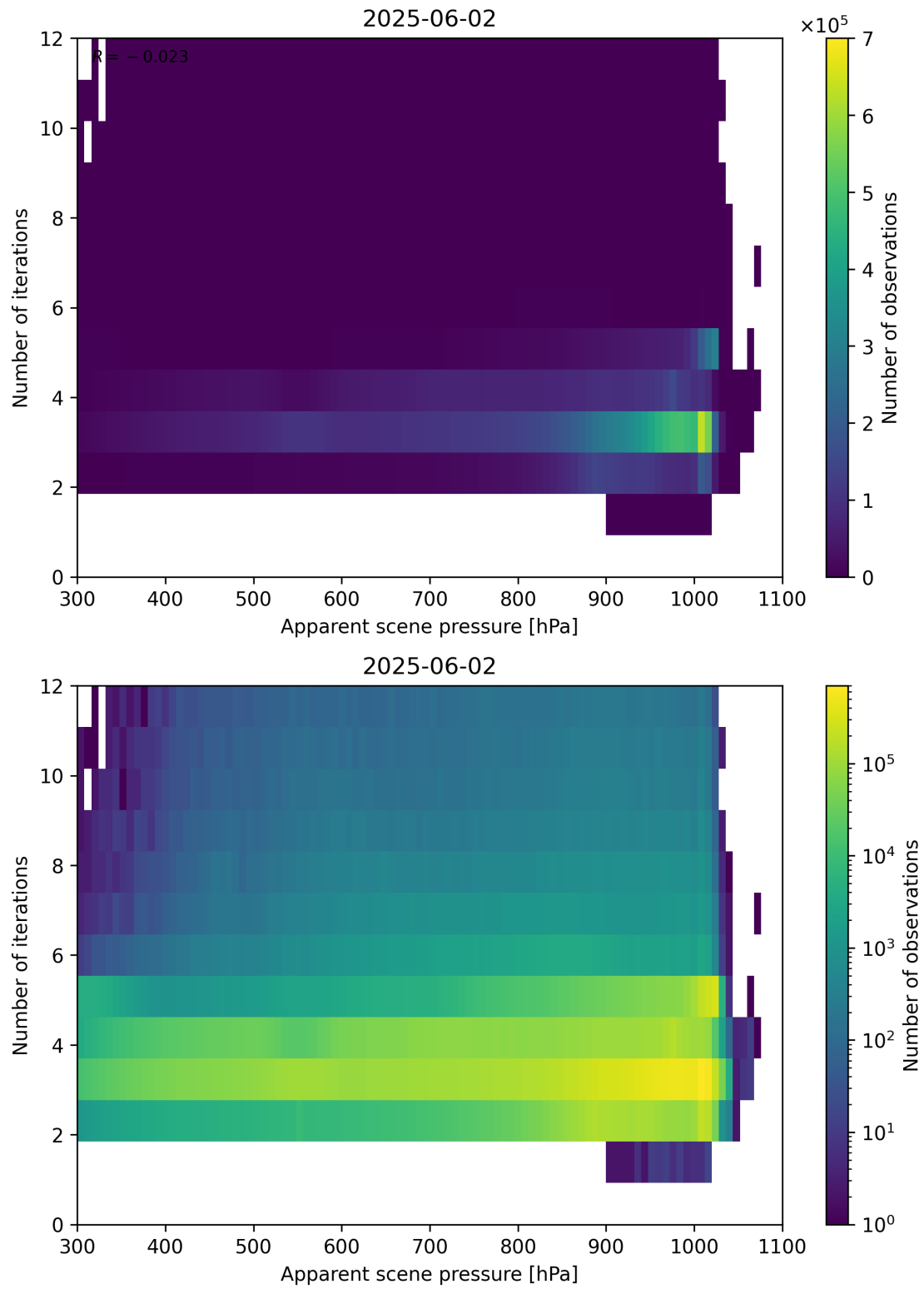
Figure 65: Scatter density plot of “Apparent scene pressure” against “Number of iterations” for 2025-06-01 to 2025-06-03.
