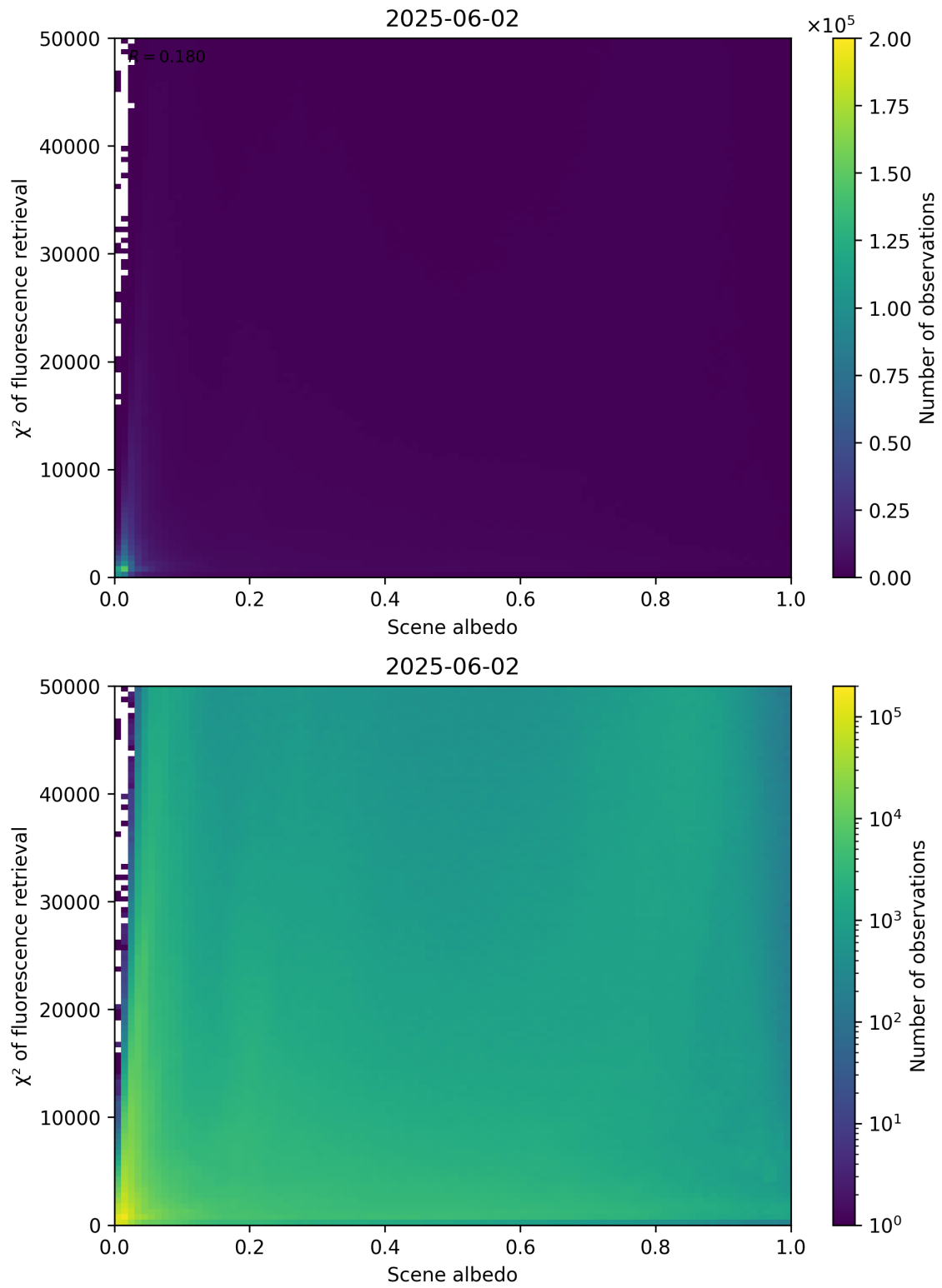
Figure 103: Scatter density plot of “Scene albedo” against “ \chi^2 of fluorescence retrieval” for 2025-06-01 to 2025-06-03.
