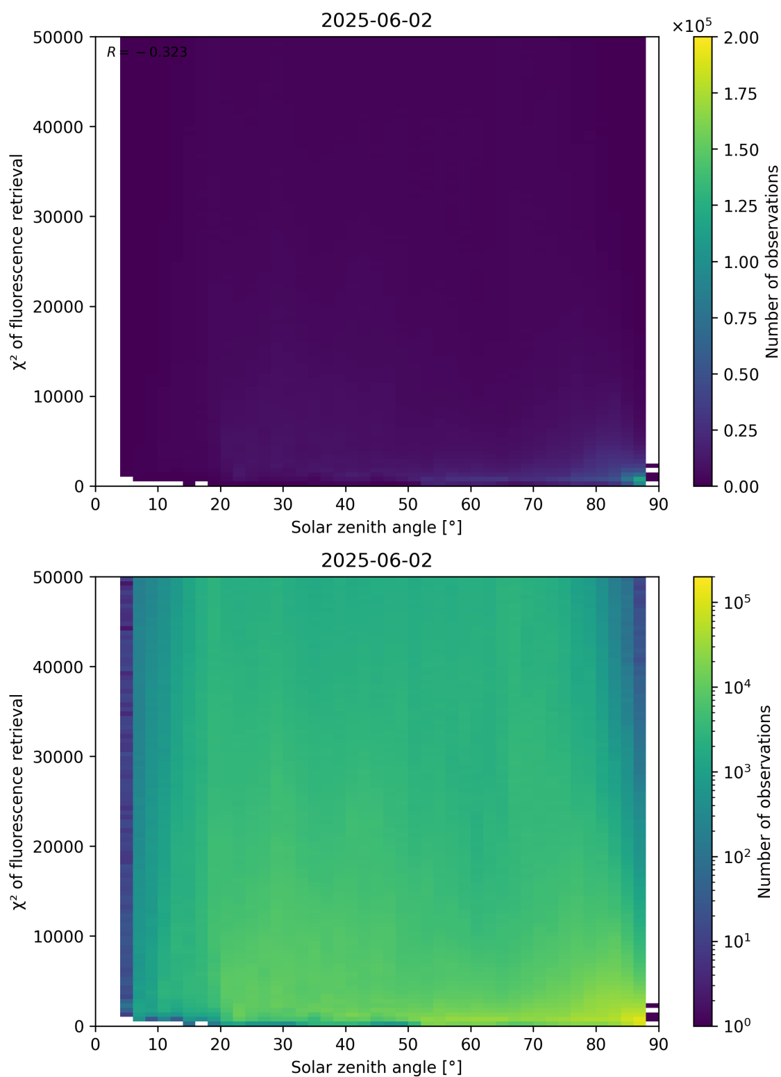
Figure 109: Scatter density plot of “Solar zenith angle” against “ \chi^2 of fluorescence retrieval” for 2025-06-01 to 2025-06-03.
