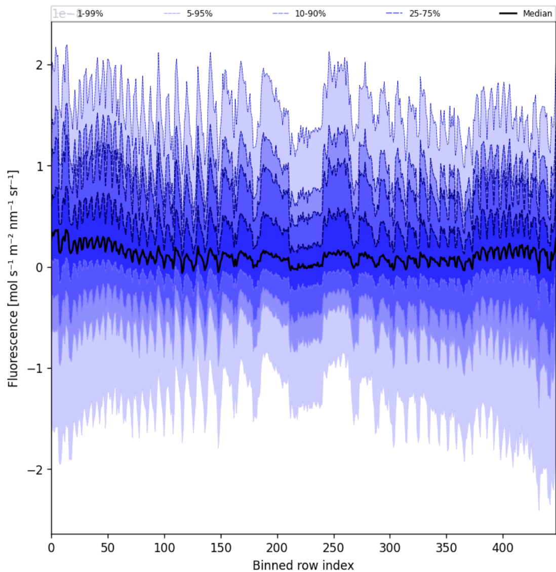
Figure 57: Along track statistics of "Fluorescence" for 2025-06-01 to 2025-06-03
