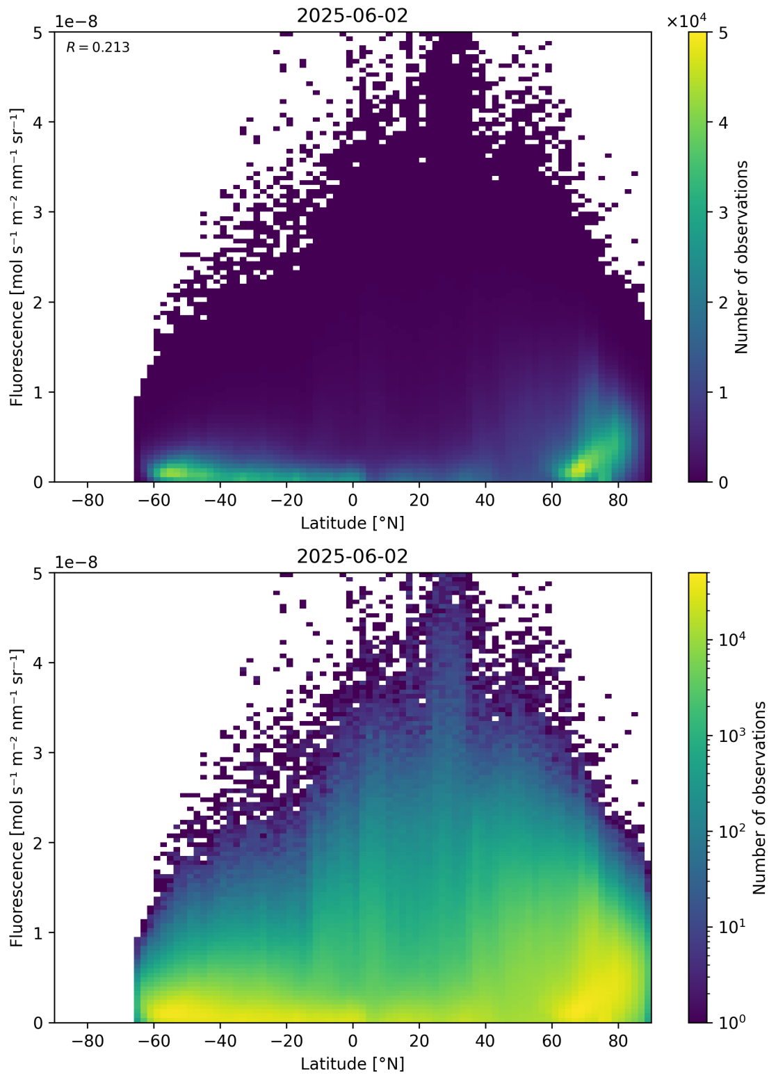
Figure 92: Scatter density plot of “Latitude” against “Fluorescence” for 2025-06-01 to 2025-06-03.
