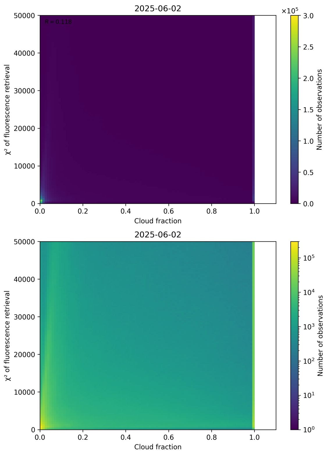
Figure 71: Scatter density plot of “Cloud fraction” against “ \chi^2 of fluorescence retrieval” for 2025-06-01 to 2025-06-03.
