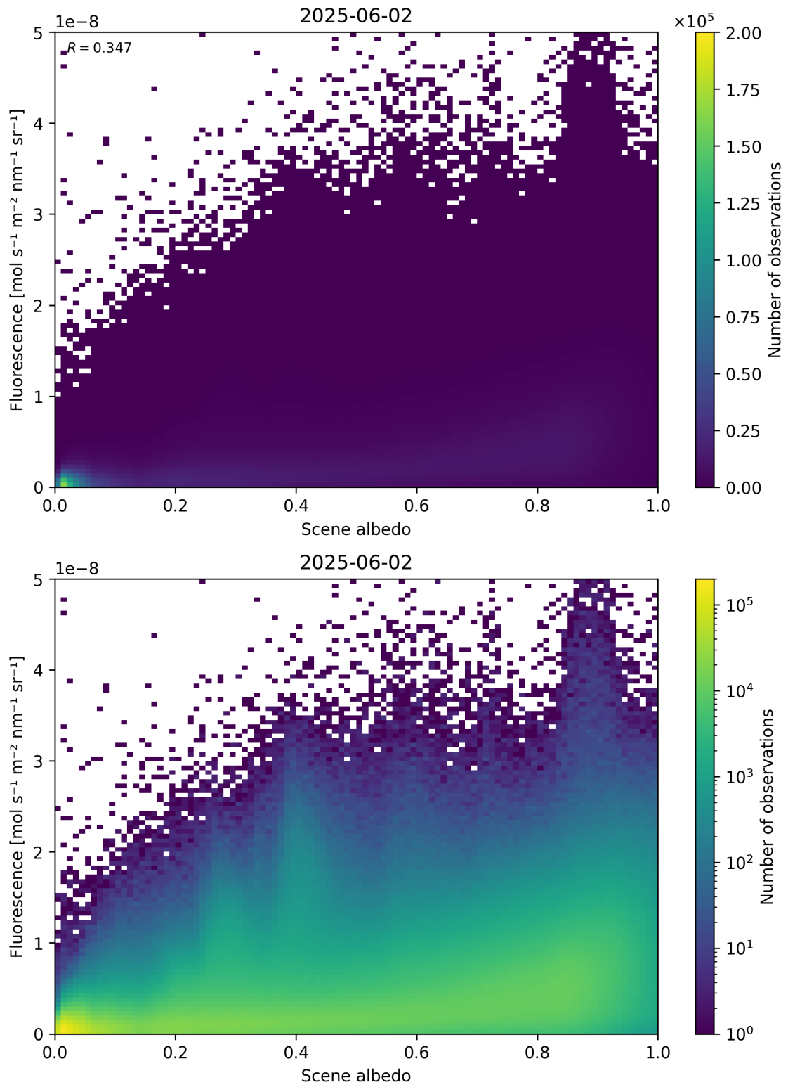
Figure 104: Scatter density plot of “Scene albedo” against “Fluorescence” for 2025-06-01 to 2025-06-03.
