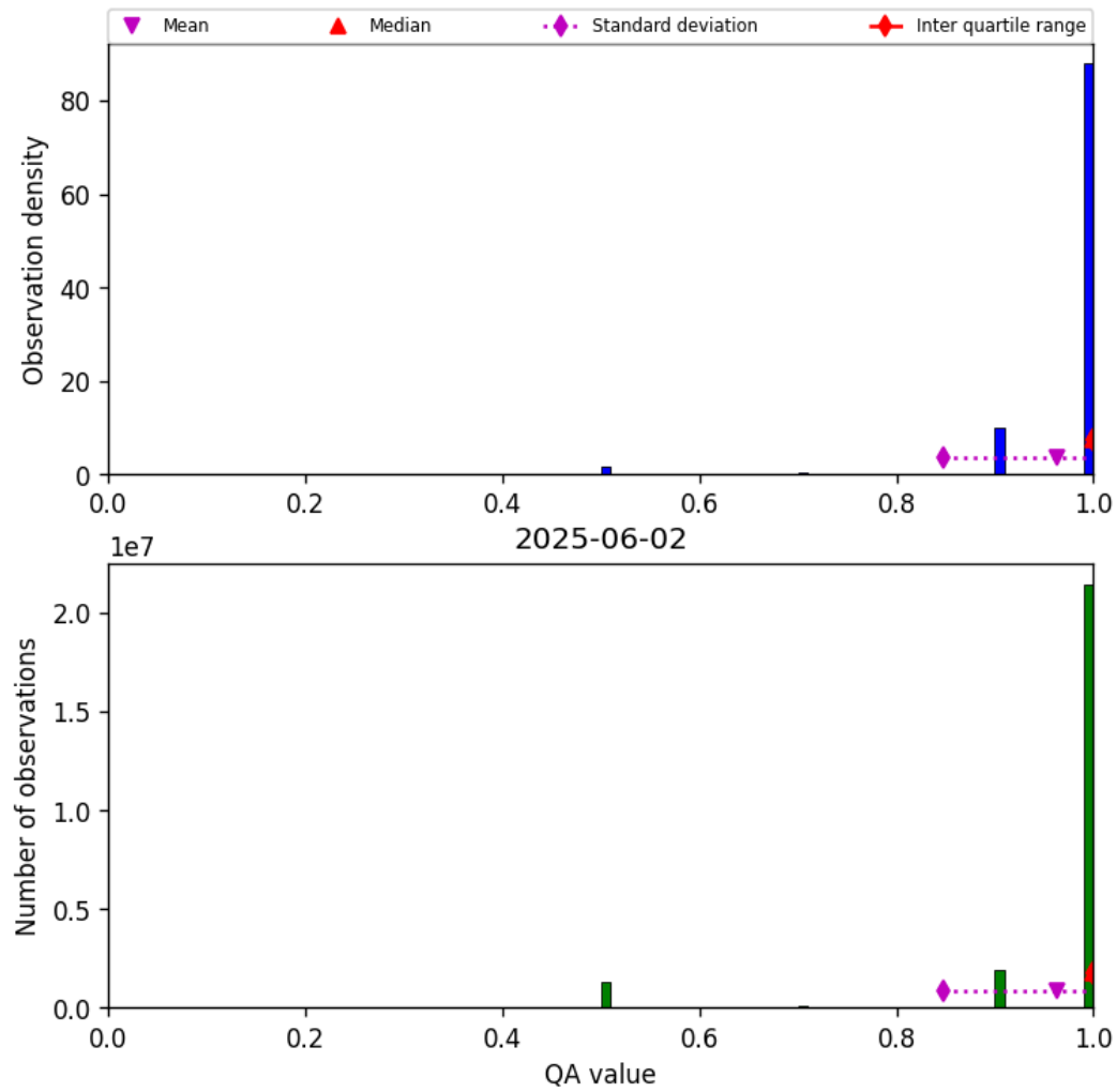
Figure 29: Histogram of “QA value” for 2025-06-01 to 2025-06-03
