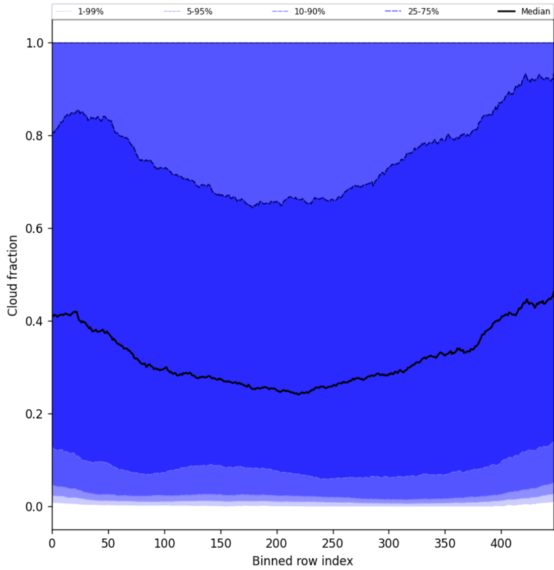
Figure 49: Along track statistics of “Cloud fraction” for 2025-06-01 to 2025-06-03
