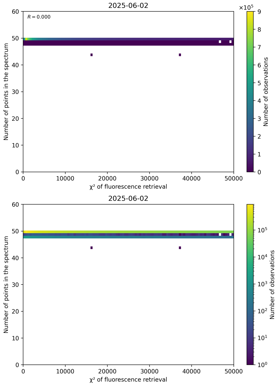
Figure 68: Scatter density plot of “ \chi^2 of fluorescence retrieval” against “Number of points in the spectrum” for 2025-06-01 to 2025-06-03.
