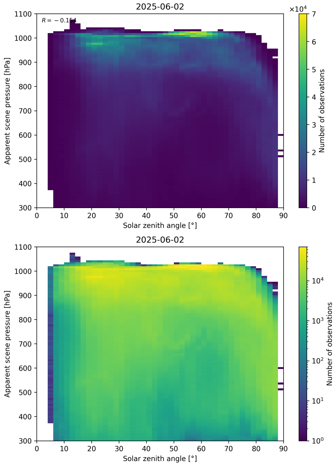
Figure 108: Scatter density plot of “Solar zenith angle” against “Apparent scene pressure” for 2025-06-01 to 2025-06-03.
