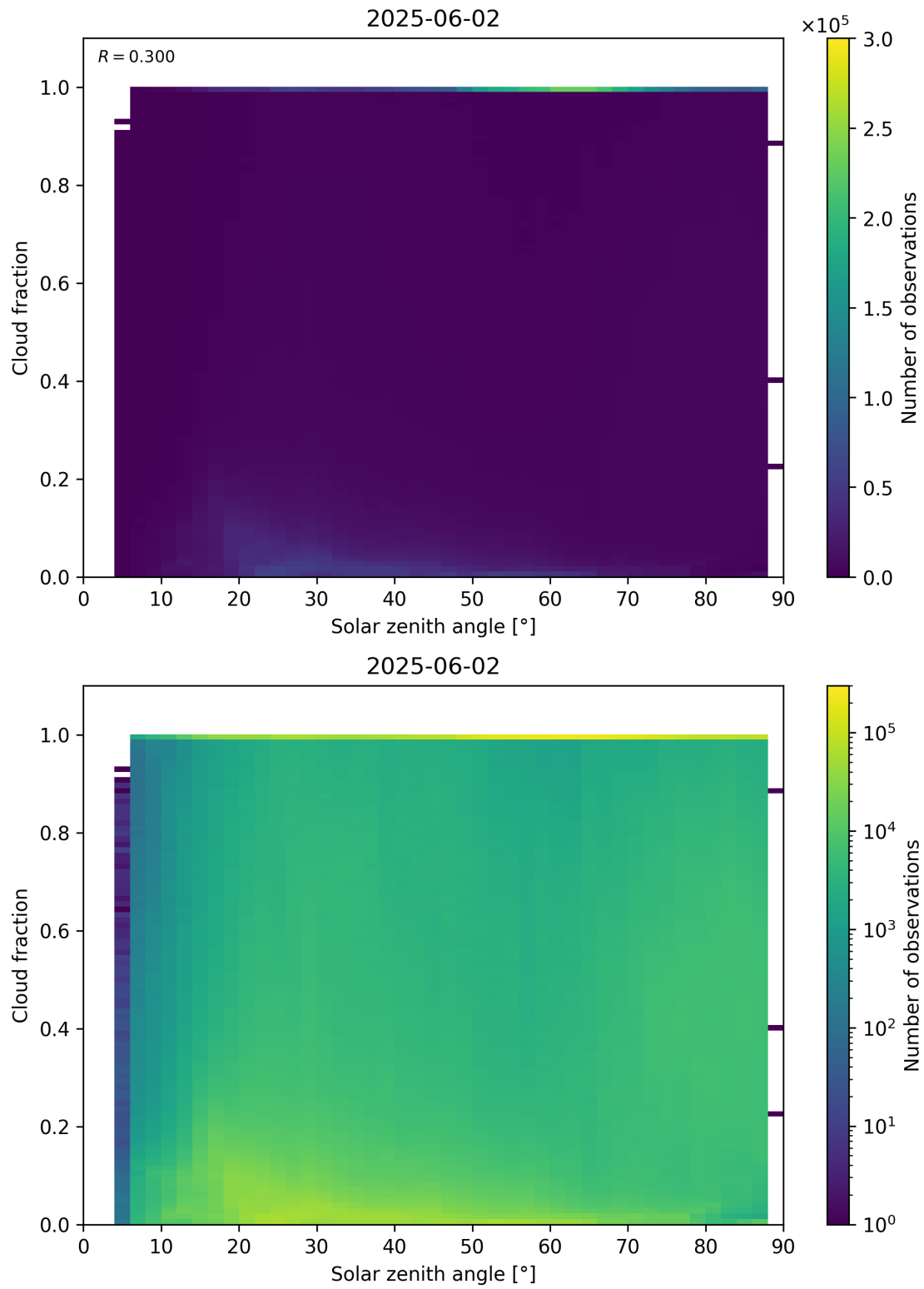
Figure 110: Scatter density plot of “Solar zenith angle” against “Cloud fraction” for 2025-06-01 to 2025-06-03.
