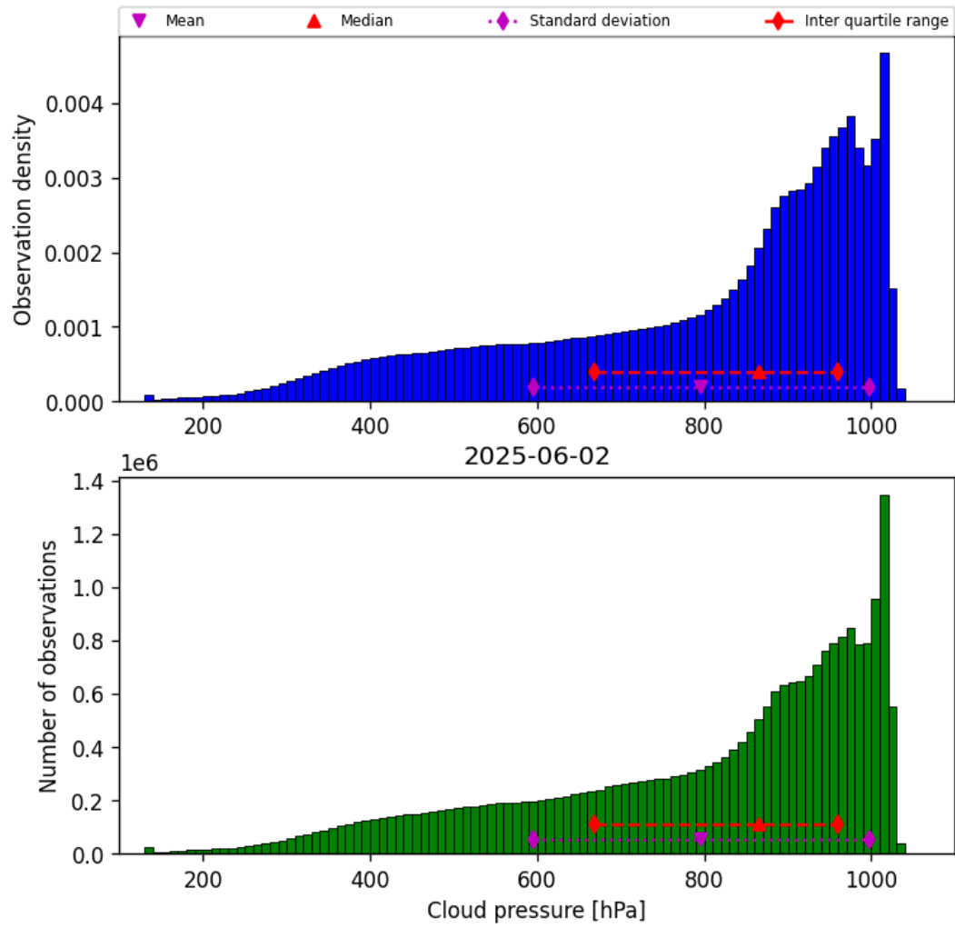
Figure 30: Histogram of “Cloud pressure” for 2025-06-01 to 2025-06-03
