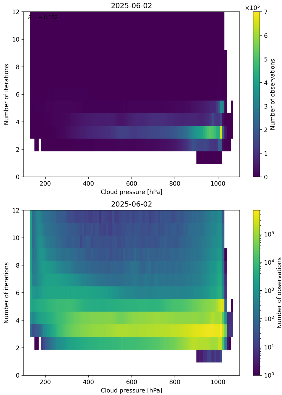
Figure 81: Scatter density plot of “Cloud pressure” against “Number of iterations” for 2025-06-01 to 2025-06-03.
