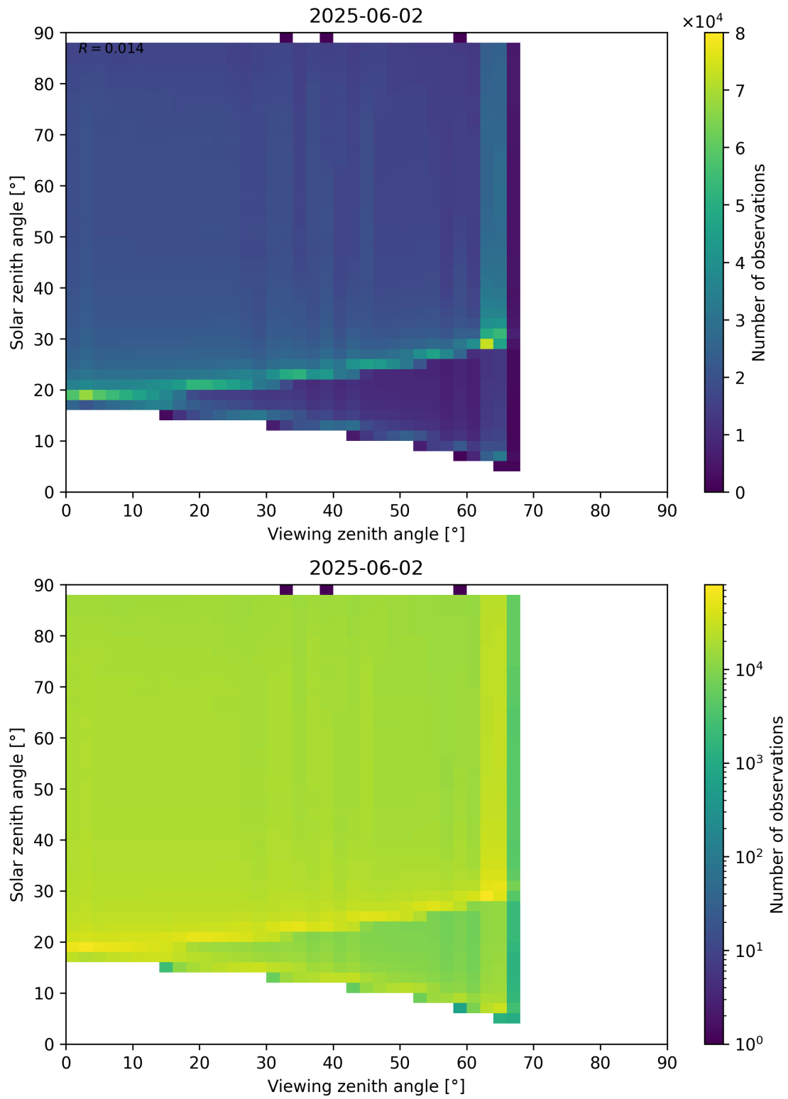
Figure 127: Scatter density plot of “Viewing zenith angle” against “Solar zenith angle” for 2025-06-01 to 2025-06-03.
