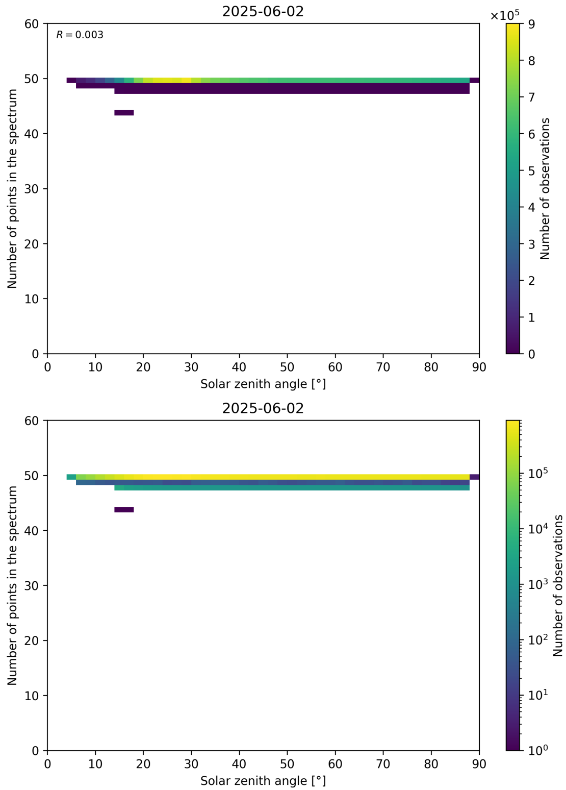
Figure 115: Scatter density plot of “Solar zenith angle” against “Number of points in the spectrum” for 2025-06-01 to 2025-06-03.
