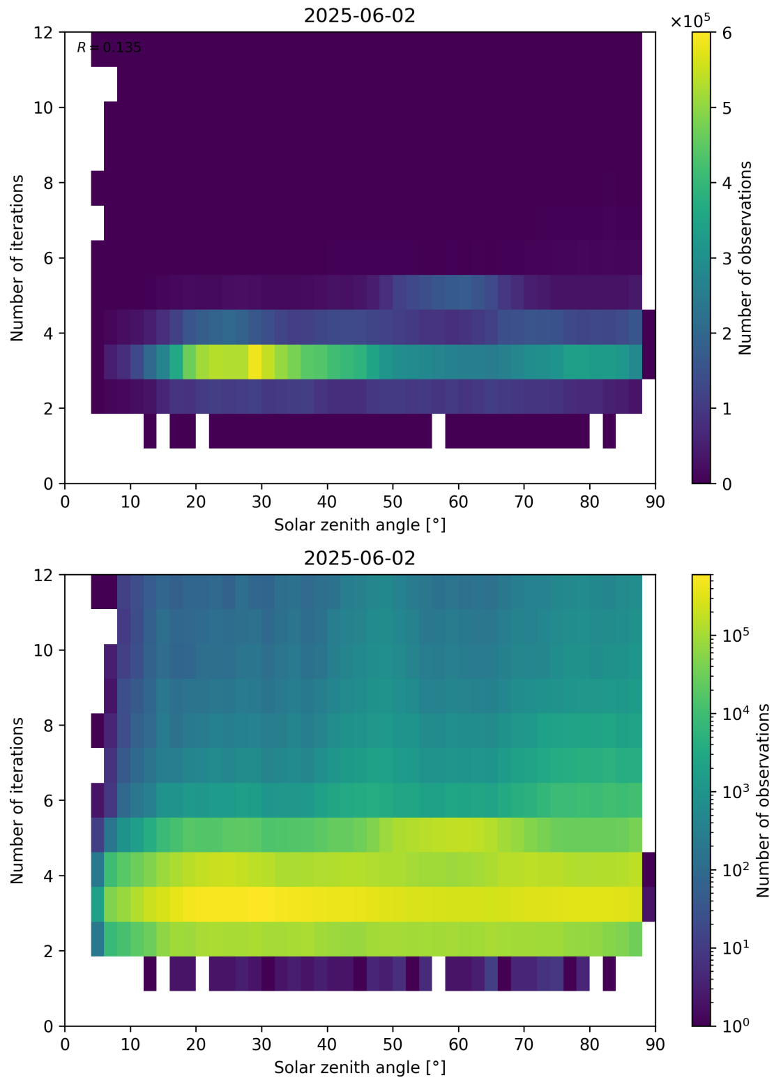
Figure 114: Scatter density plot of “Solar zenith angle” against “Number of iterations” for 2025-06-01 to 2025-06-03.
