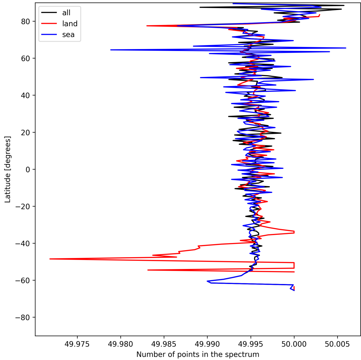
Figure 27: Zonal average of “Number of points in the spectrum” for 2025-06-01 to 2025-06-03.
