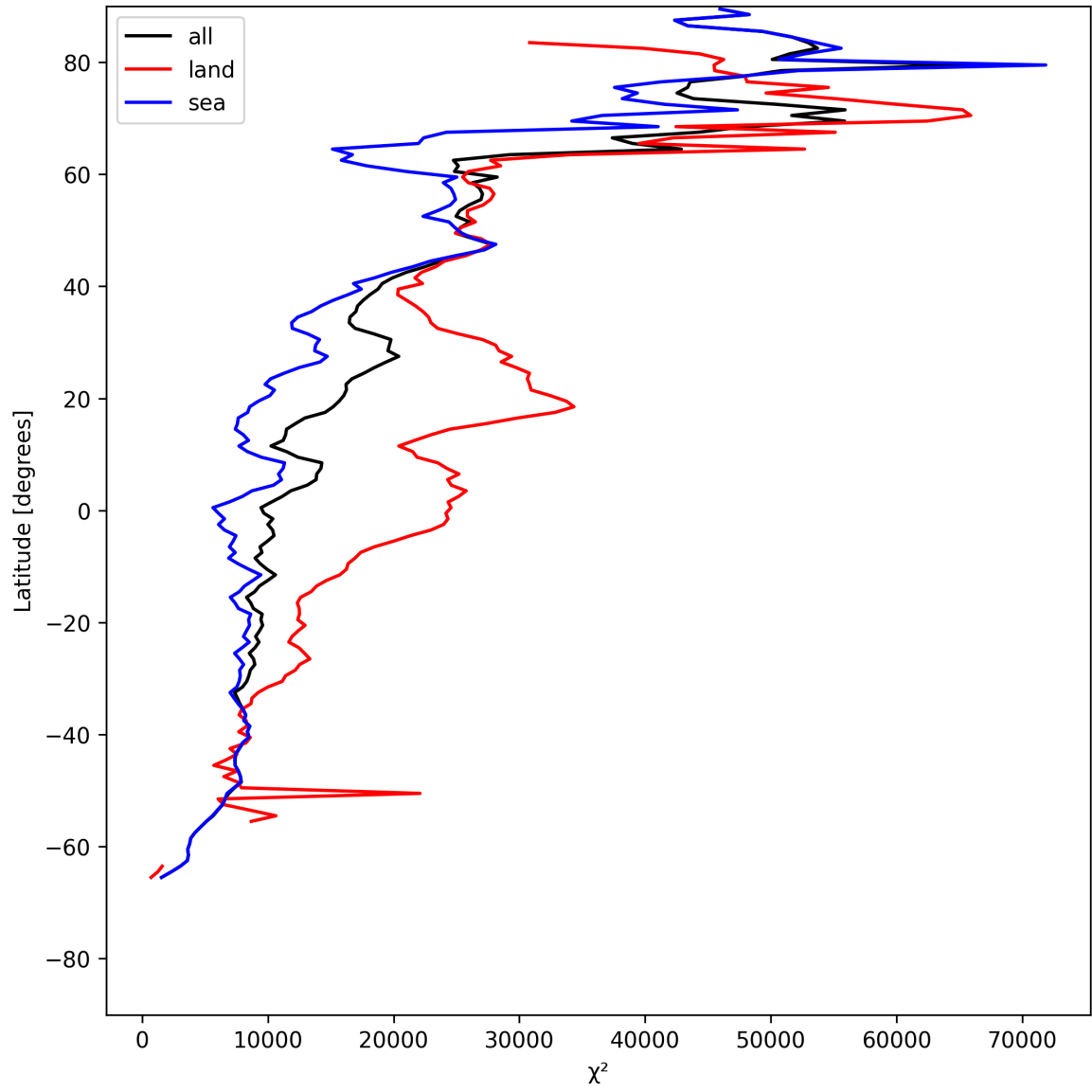
Figure 21: Zonal average of “ \chi^2 ” for 2025-06-01 to 2025-06-03.
