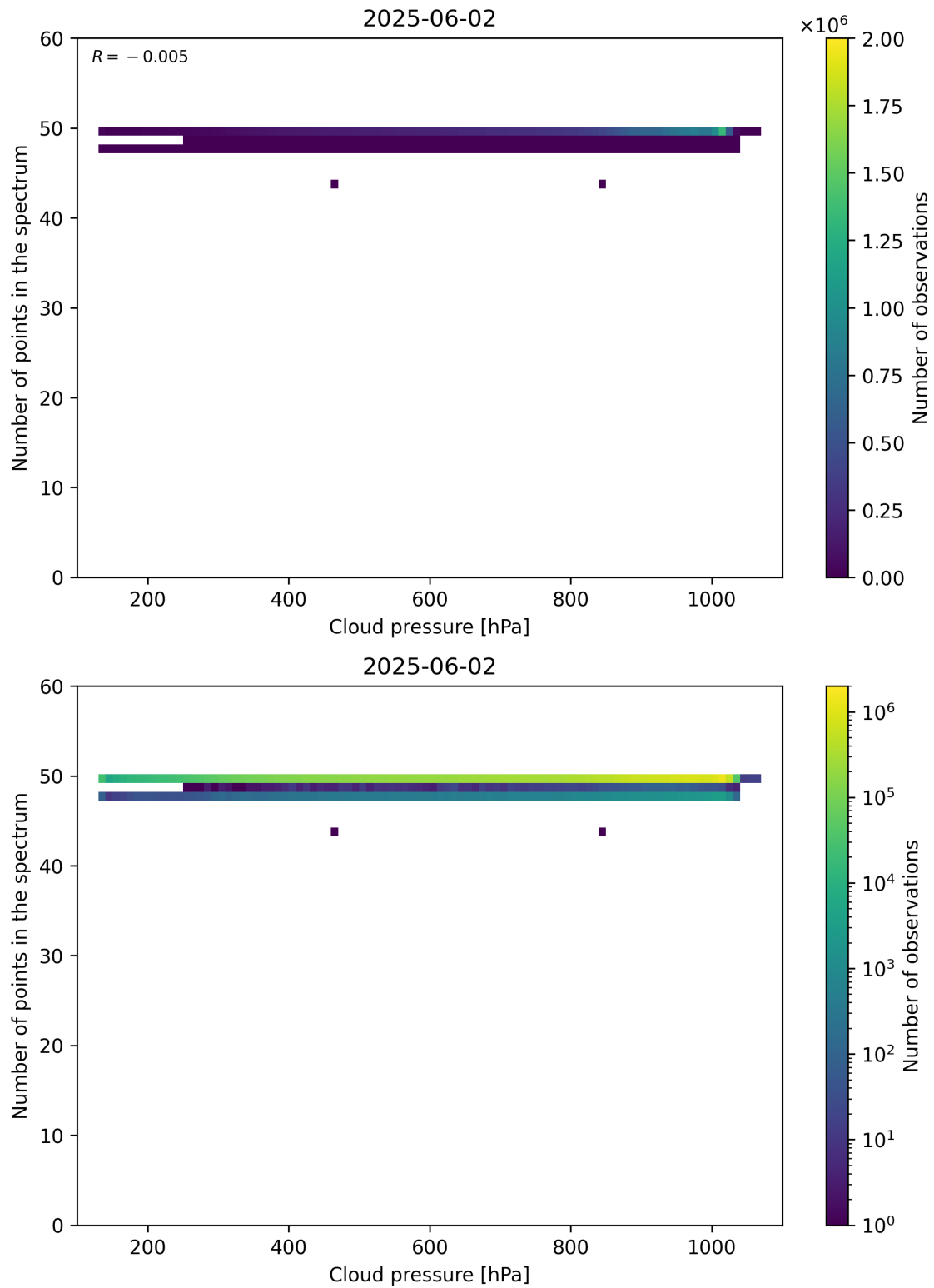
Figure 82: Scatter density plot of “Cloud pressure” against “Number of points in the spectrum” for 2025-06-01 to 2025-06-03.
