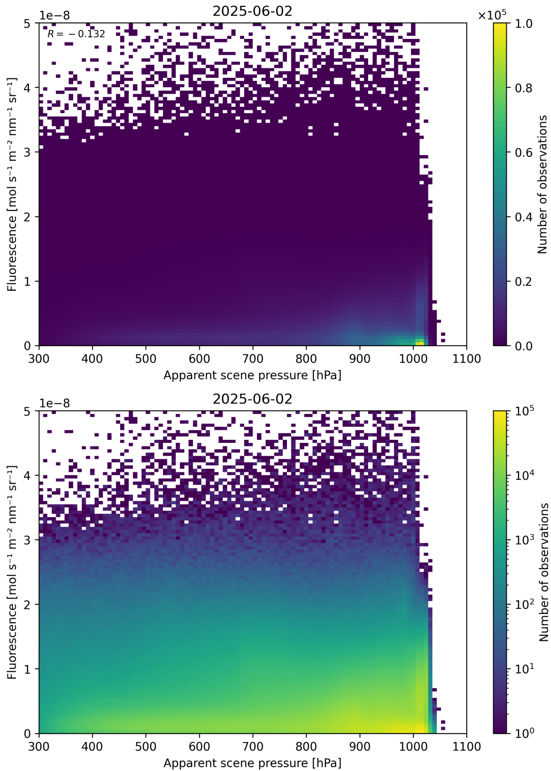
Figure 64: Scatter density plot of “Apparent scene pressure” against “Fluorescence” for 2025-06-01 to 2025-06-03.
