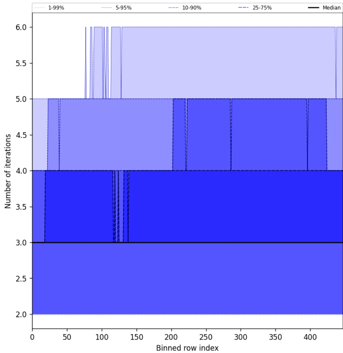
Figure 56: Along track statistics of “Number of iterations” for 2025-06-01 to 2025-06-03
