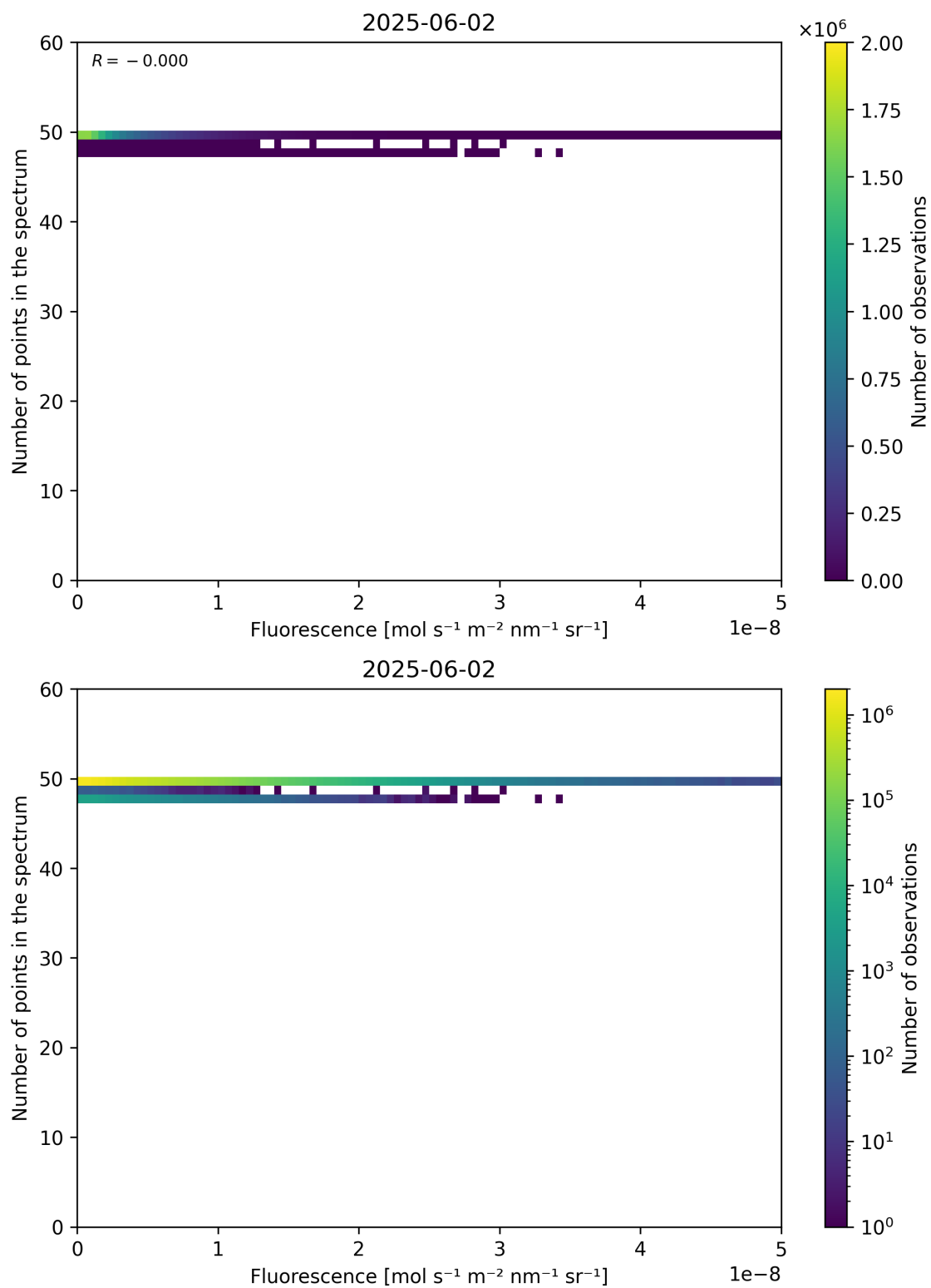
Figure 86: Scatter density plot of “Fluorescence” against “Number of points in the spectrum” for 2025-06-01 to 2025-06-03.
