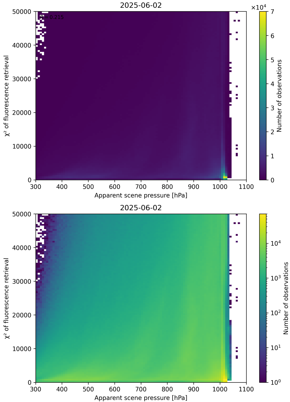
Figure 63: Scatter density plot of “Apparent scene pressure” against “ \chi^2 of fluorescence retrieval” for 2025-06-01 to 2025-06-03.
