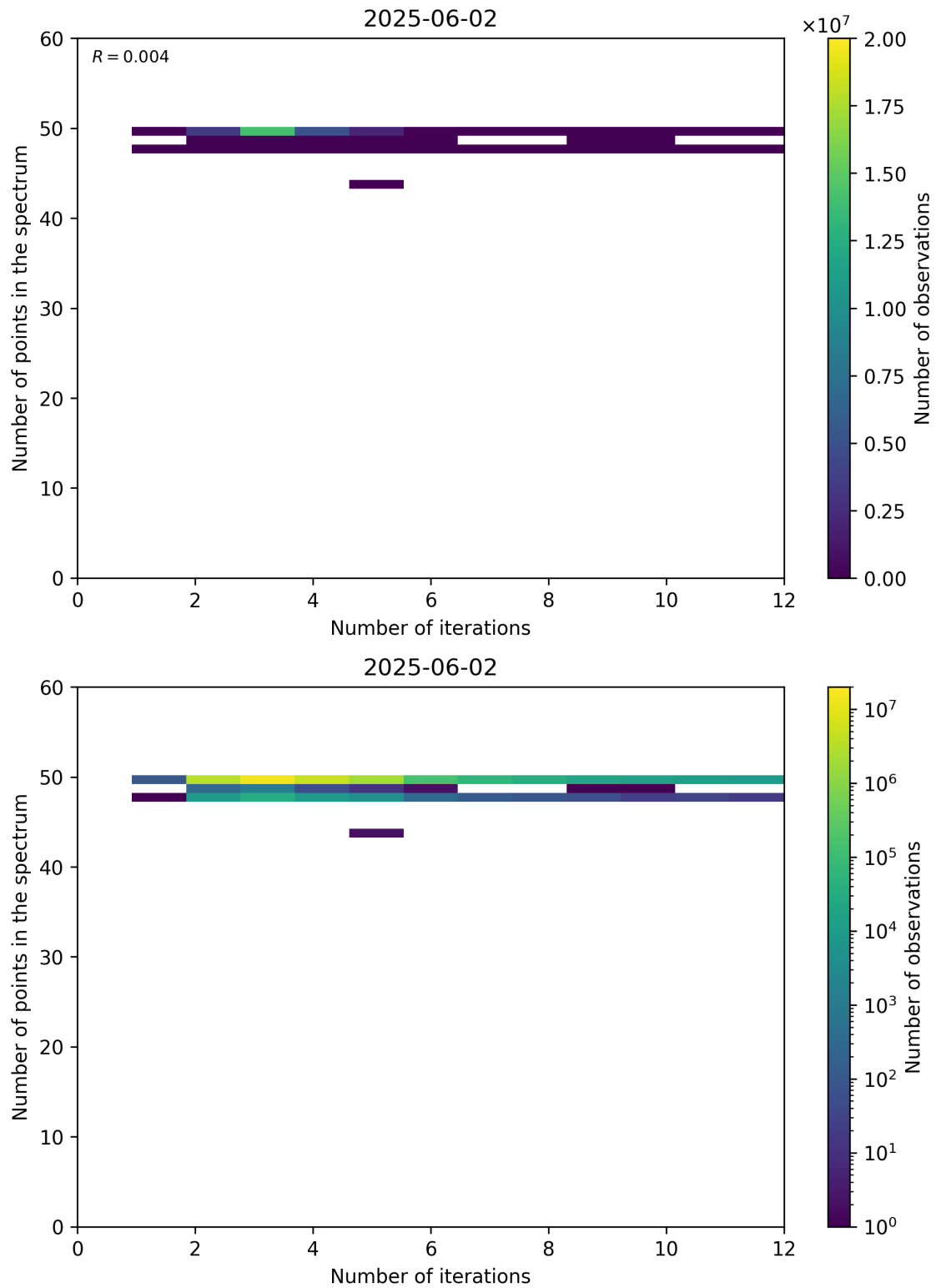
Figure 99: Scatter density plot of “Number of iterations” against “Number of points in the spectrum” for 2025-06-01 to 2025-06-03.
