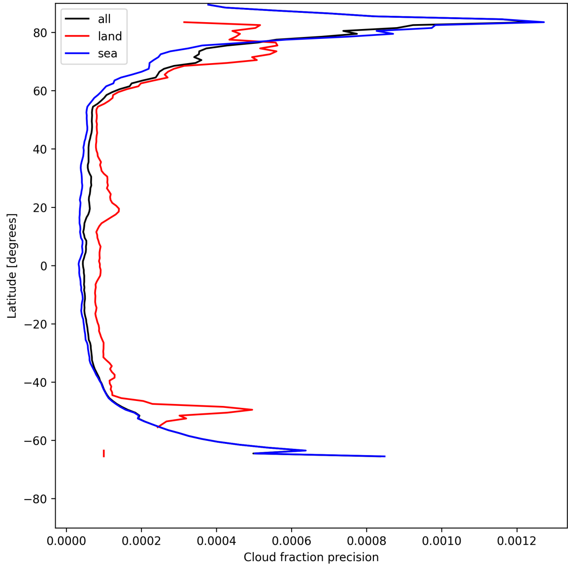
Figure 16: Zonal average of “Cloud fraction precision” for 2025-06-01 to 2025-06-03.
