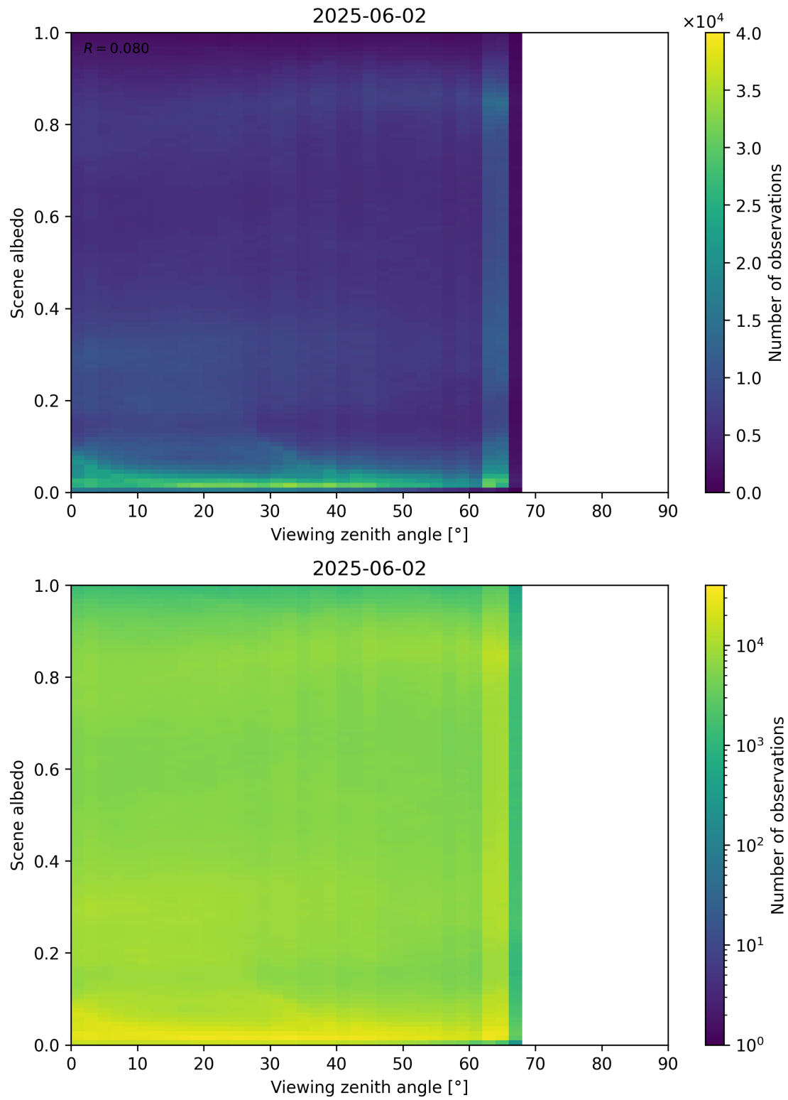
Figure 126: Scatter density plot of “Viewing zenith angle” against “Scene albedo” for 2025-06-01 to 2025-06-03.
