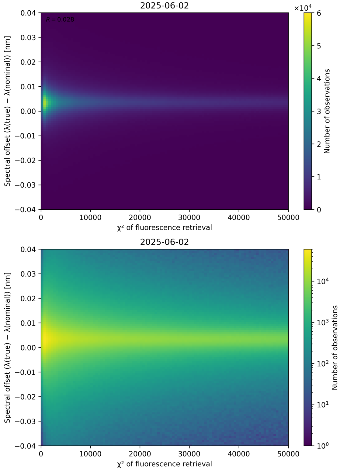
Figure 69: Scatter density plot of “ \chi^2 of fluorescence retrieval” against “Spectral offset ( \lambda_{\text{true}} - \lambda_{\text{nominal}} )” for 2025-06-01 to 2025-06-03.
