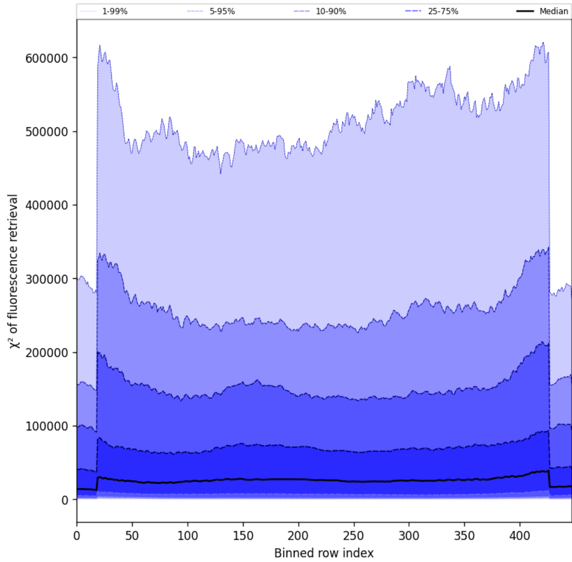
Figure 59: Along track statistics of “ \chi^2 of fluorescence retrieval” for 2025-06-01 to 2025-06-03
