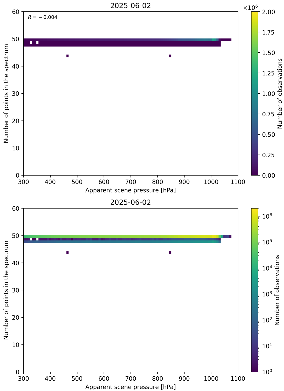
Figure 66: Scatter density plot of “Apparent scene pressure” against “Number of points in the spectrum” for 2025-06-01 to 2025-06-03.
