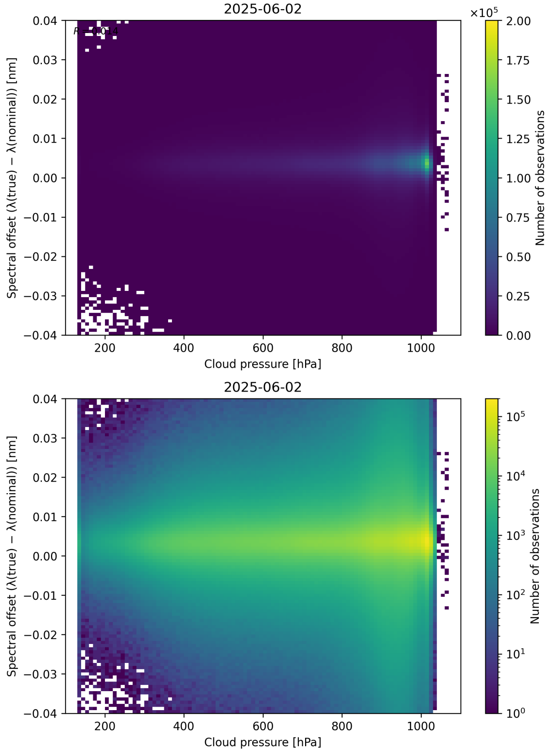
Figure 84: Scatter density plot of “Cloud pressure” against “Spectral offset ( \lambda_{\text{true}} - \lambda_{\text{nominal}} )” for 2025-06-01 to 2025-06-03.
