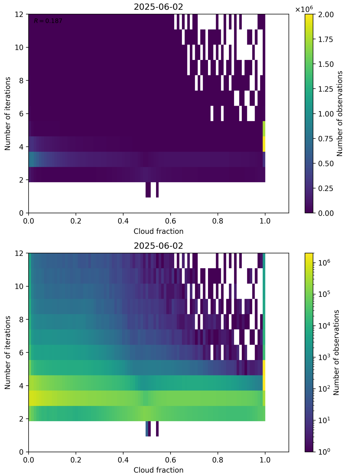
Figure 73: Scatter density plot of “Cloud fraction” against “Number of iterations” for 2025-06-01 to 2025-06-03.
