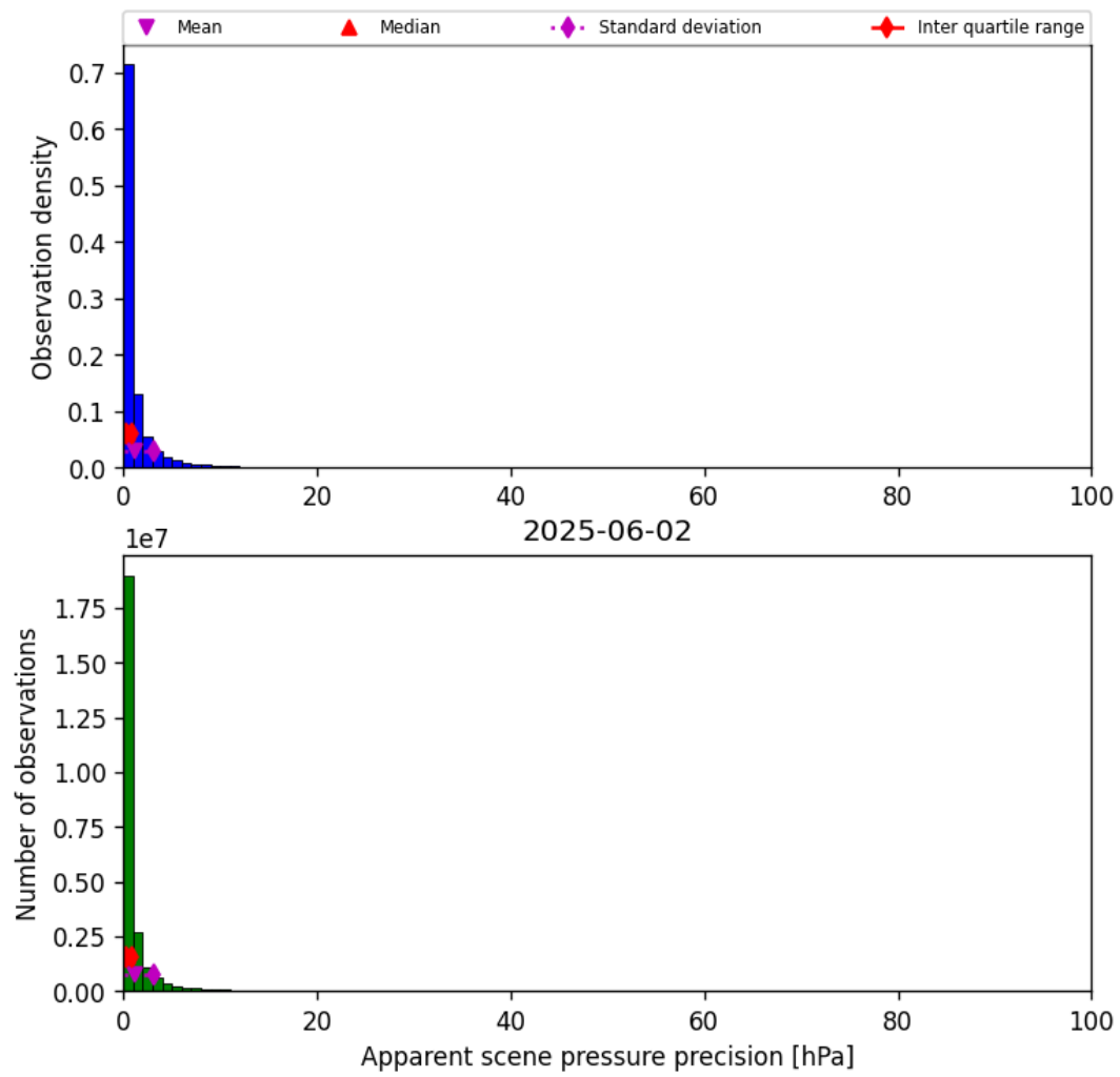
Figure 37: Histogram of “Apparent scene pressure precision” for 2025-06-01 to 2025-06-03
