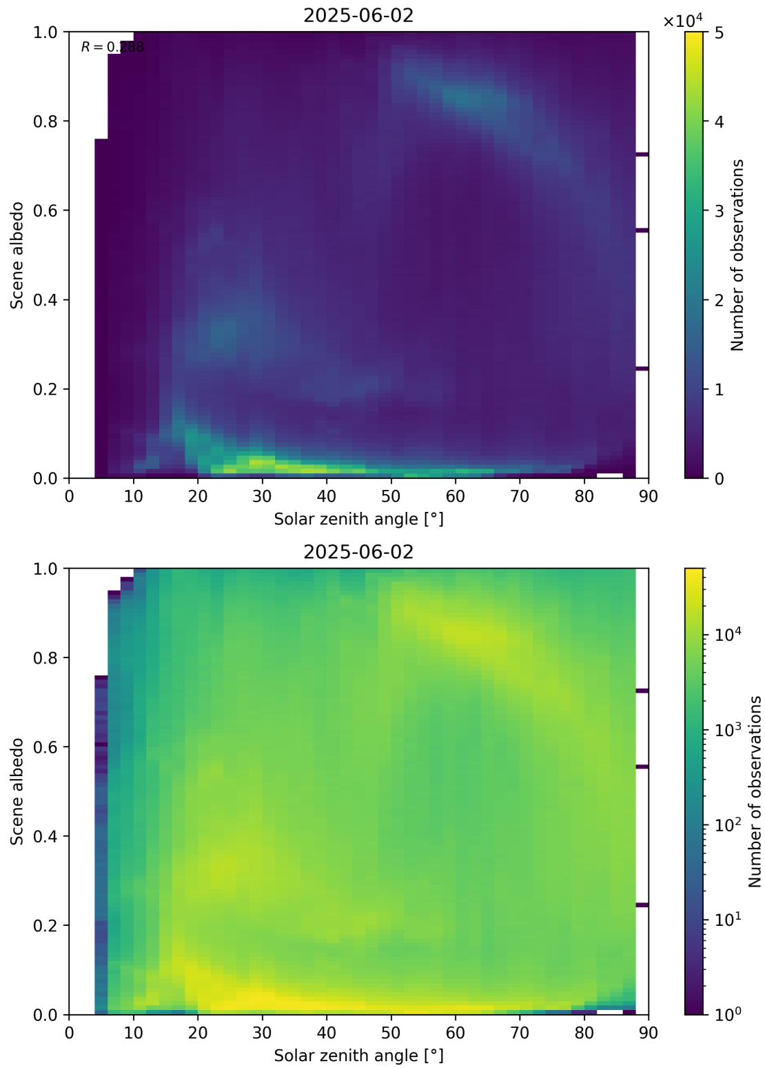
Figure 116: Scatter density plot of “Solar zenith angle” against “Scene albedo” for 2025-06-01 to 2025-06-03.
