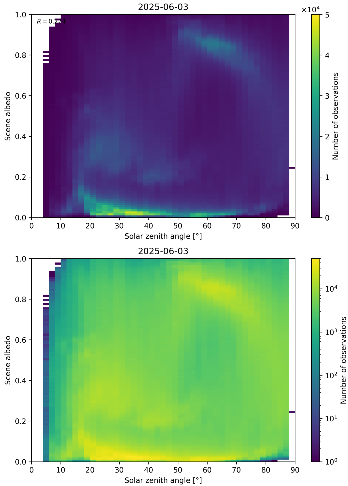
Figure 116: Scatter density plot of “Solar zenith angle” against “Scene albedo” for 2025-06-02 to 2025-06-04.
