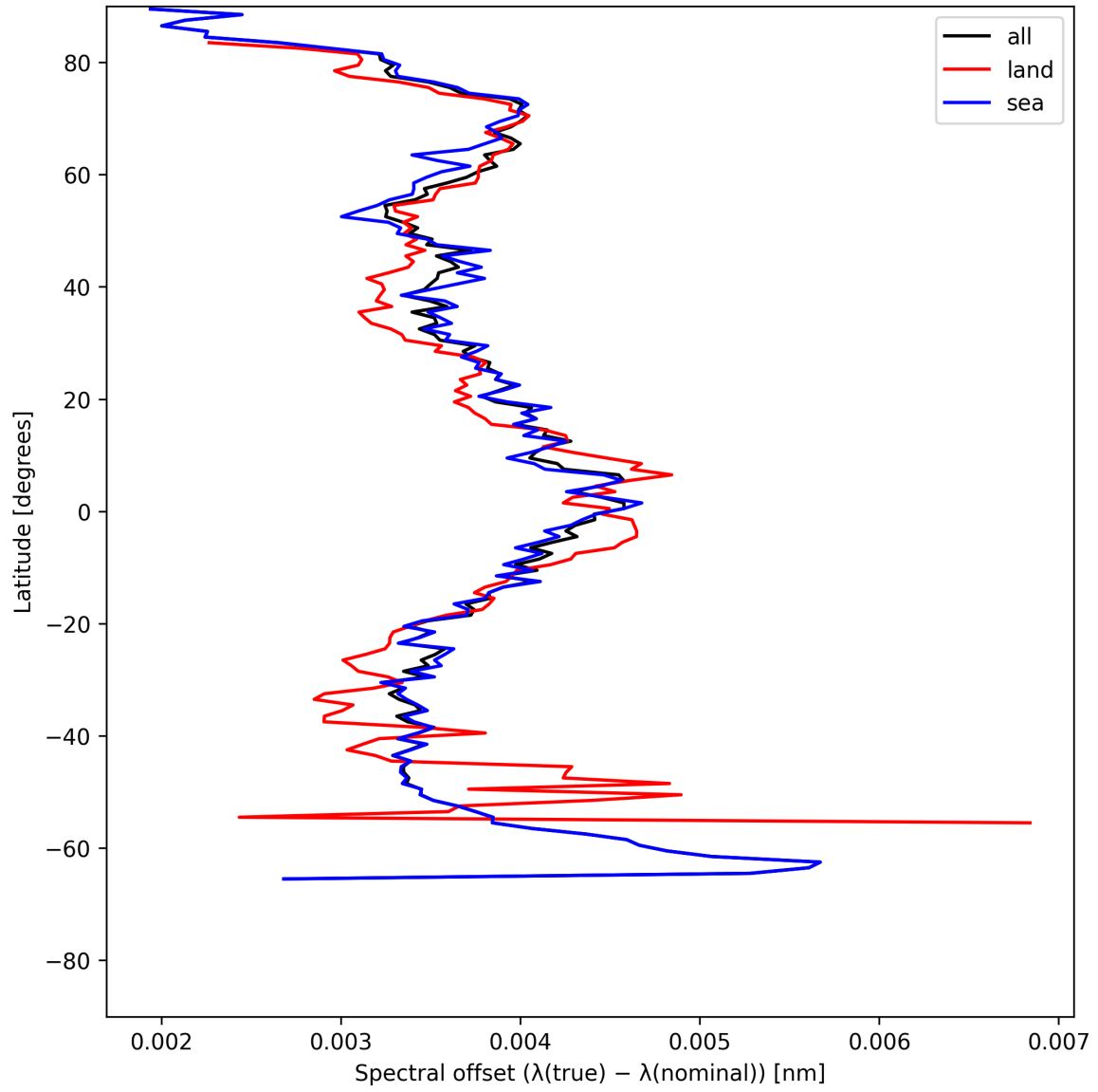
Figure 28: Zonal average of “Spectral offset ( \lambda_{\text{true}} - \lambda_{\text{nominal}} )” for 2025-06-02 to 2025-06-04.
