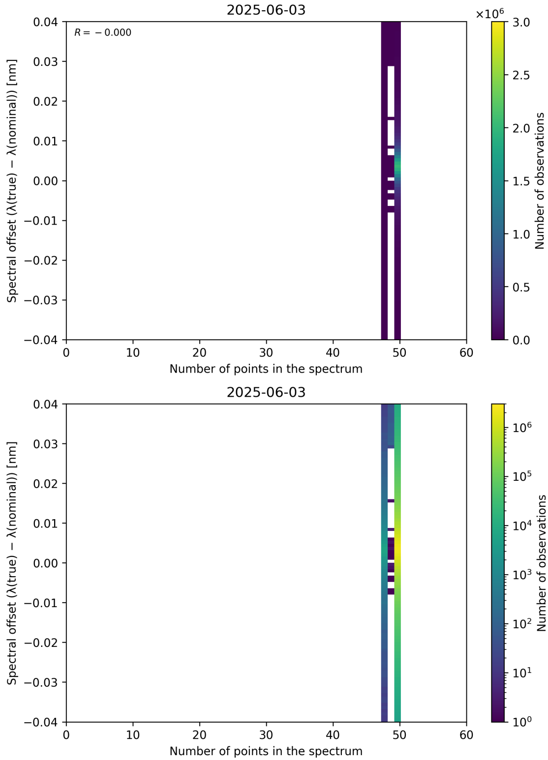
Figure 101: Scatter density plot of “Number of points in the spectrum” against “Spectral offset ( \lambda_{\text{true}} - \lambda_{\text{nominal}} )” for 2025-06-02 to 2025-06-04.
