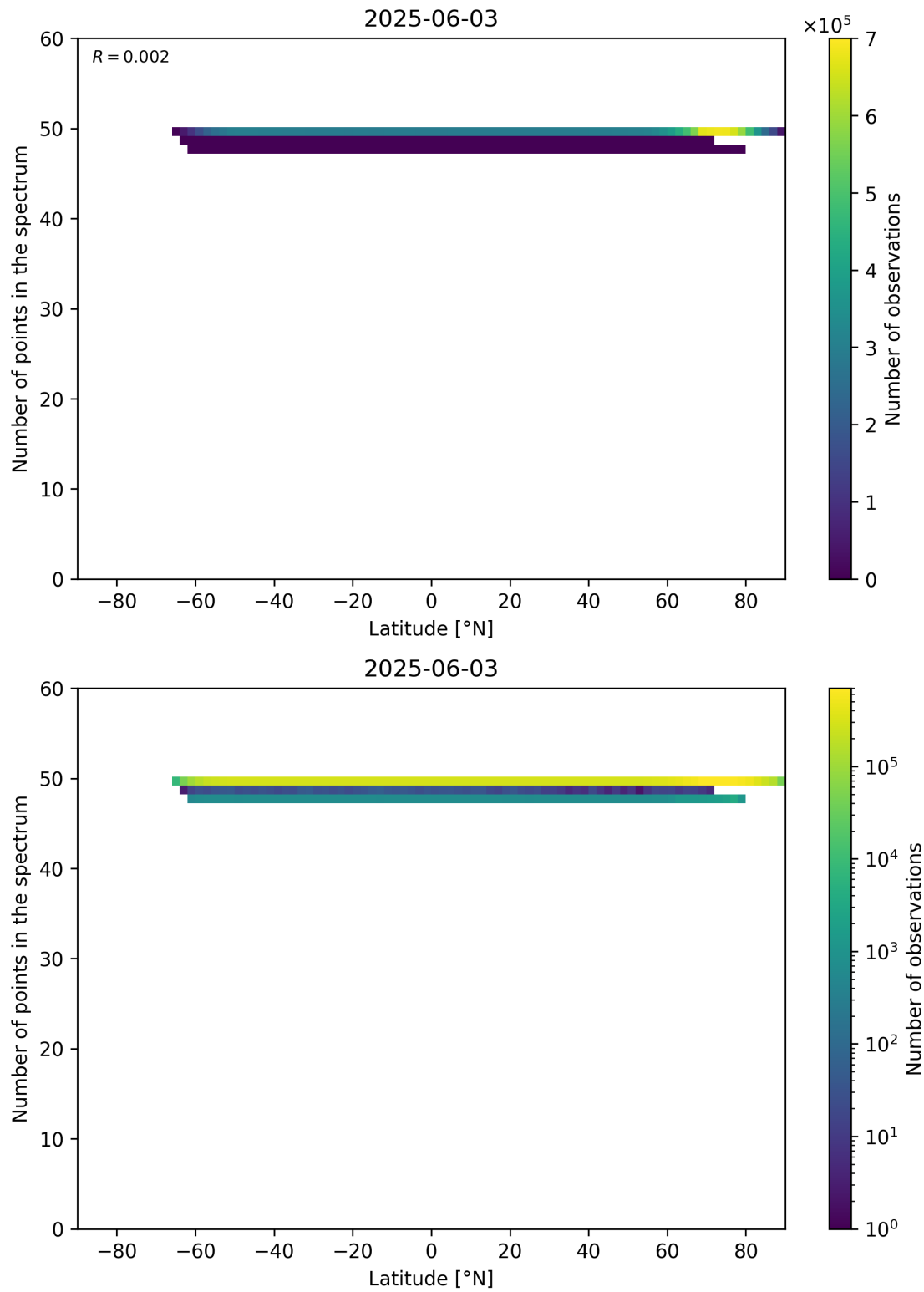
Figure 94: Scatter density plot of “Latitude” against “Number of points in the spectrum” for 2025-06-02 to 2025-06-04.
