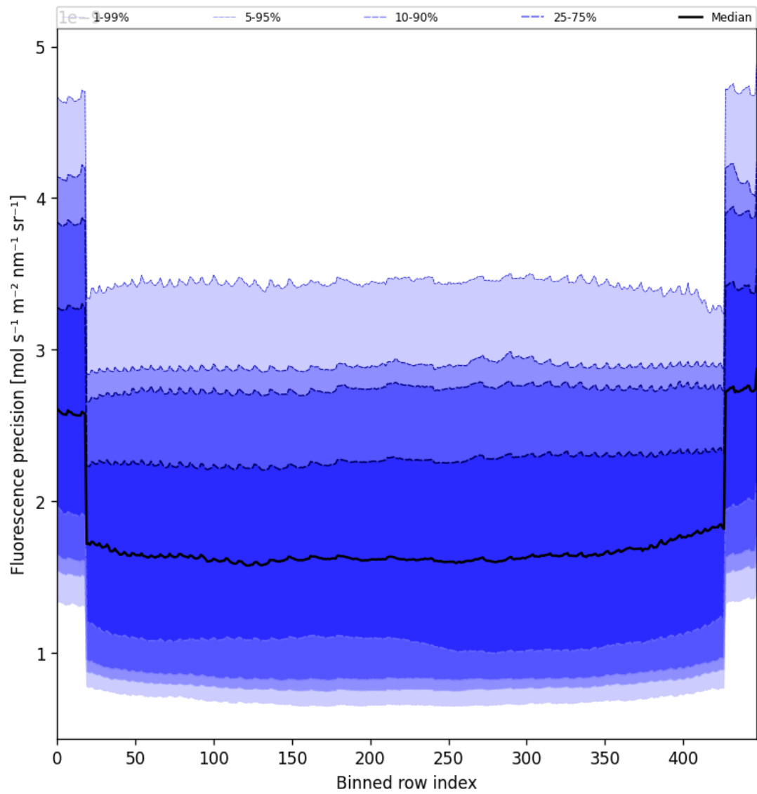
Figure 58: Along track statistics of “Fluorescence precision” for 2025-06-02 to 2025-06-04
