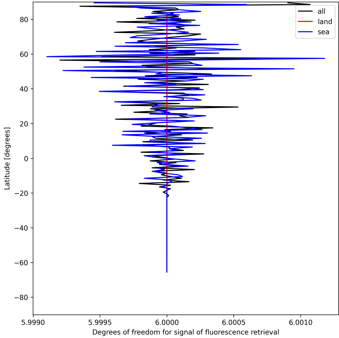
Figure 26: Zonal average of “Degrees of freedom for signal of fluorescence retrieval” for 2025-06-02 to 2025-06-04.
