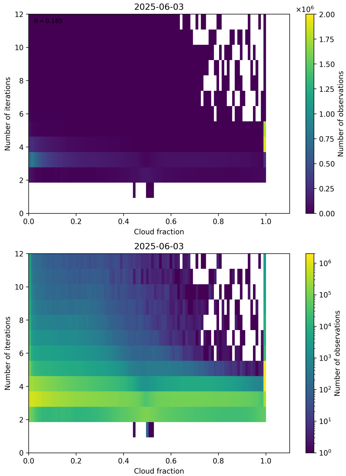
Figure 73: Scatter density plot of “Cloud fraction” against “Number of iterations” for 2025-06-02 to 2025-06-04.
