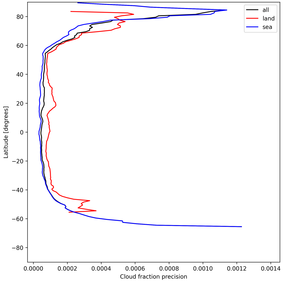
Figure 16: Zonal average of “Cloud fraction precision” for 2025-06-02 to 2025-06-04.
