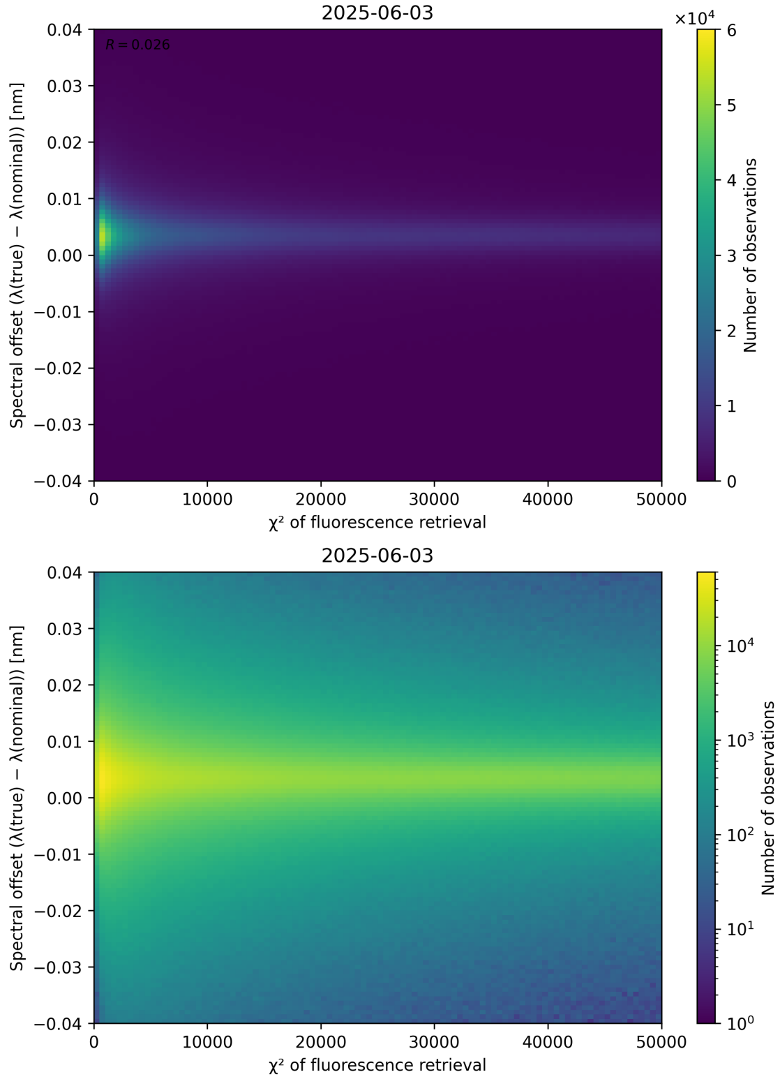
Figure 69: Scatter density plot of “ \chi^2 of fluorescence retrieval” against “Spectral offset ( \lambda_{\text{true}} - \lambda_{\text{nominal}} )” for 2025-06-02 to 2025-06-04.
