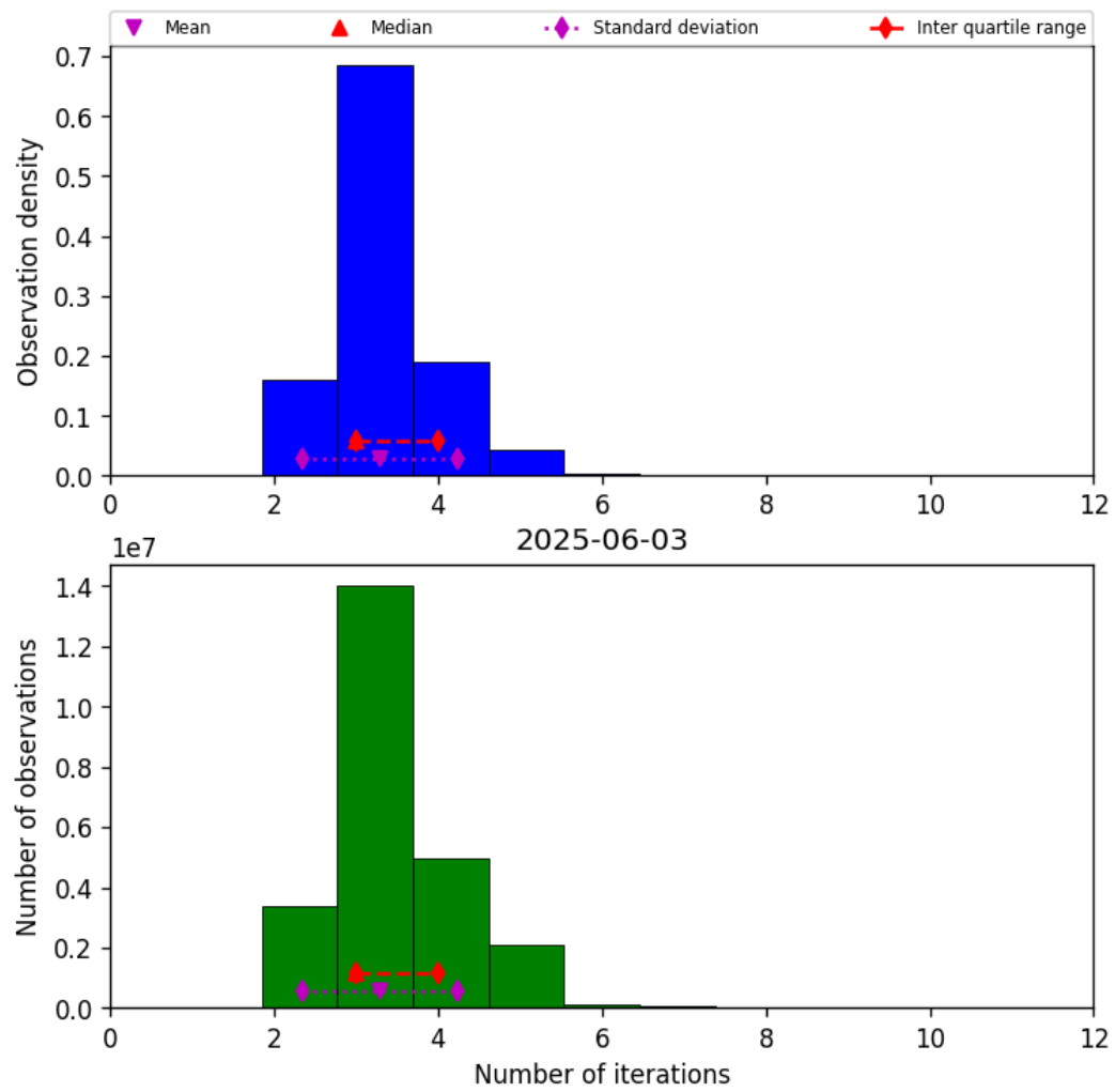
Figure 39: Histogram of “Number of iterations” for 2025-06-02 to 2025-06-04
