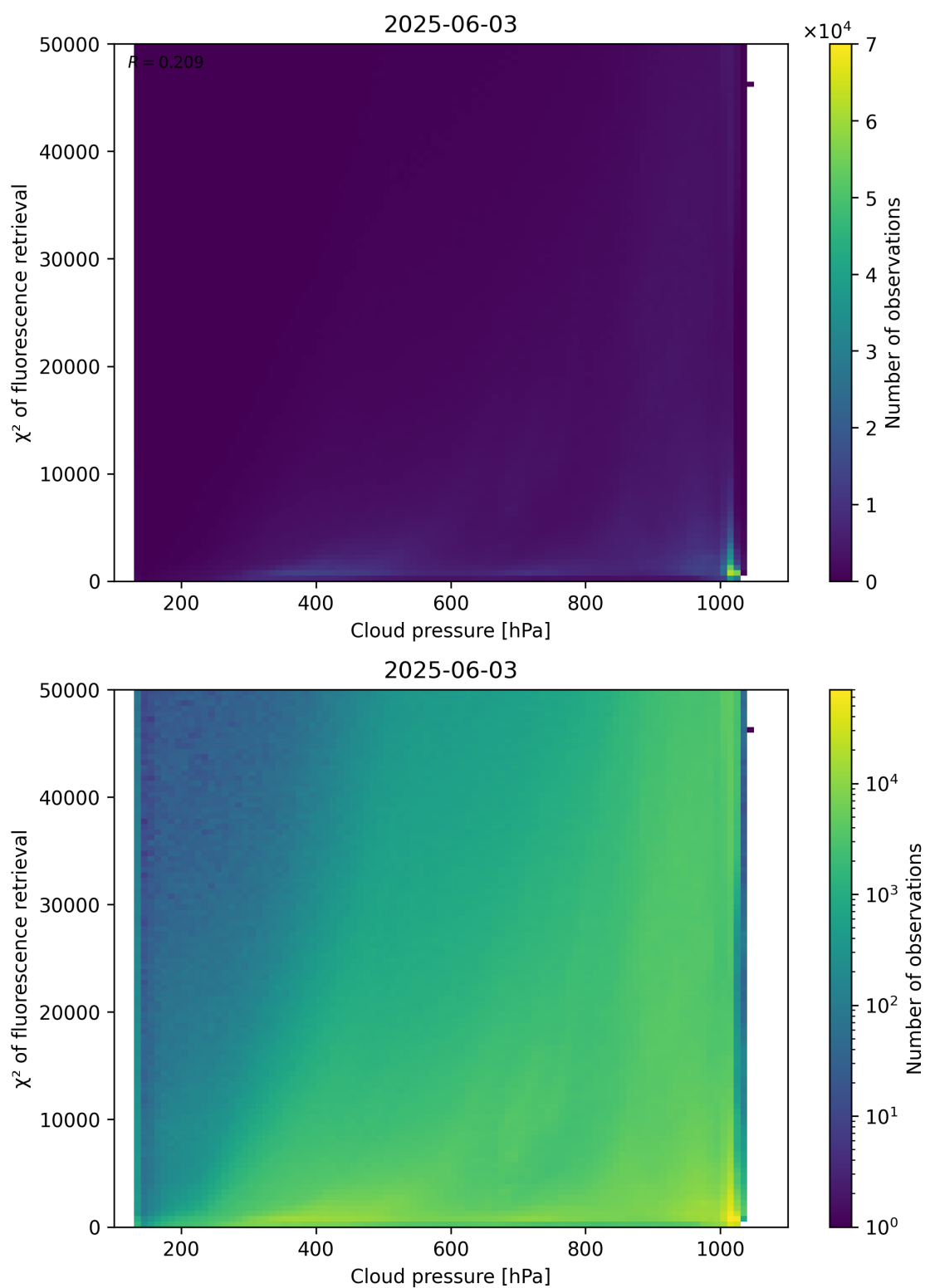
Figure 78: Scatter density plot of “Cloud pressure” against “ \chi^2 of fluorescence retrieval” for 2025-06-02 to 2025-06-04.
