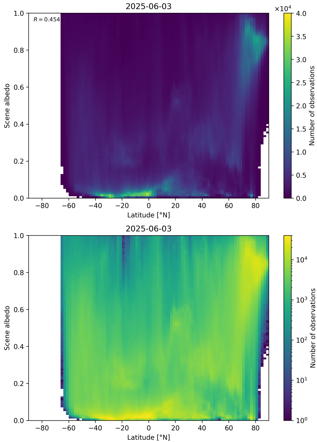
Figure 95: Scatter density plot of “Latitude” against “Scene albedo” for 2025-06-02 to 2025-06-04.
