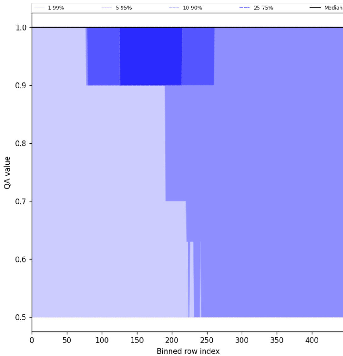
Figure 46: Along track statistics of “QA value” for 2025-06-02 to 2025-06-04
