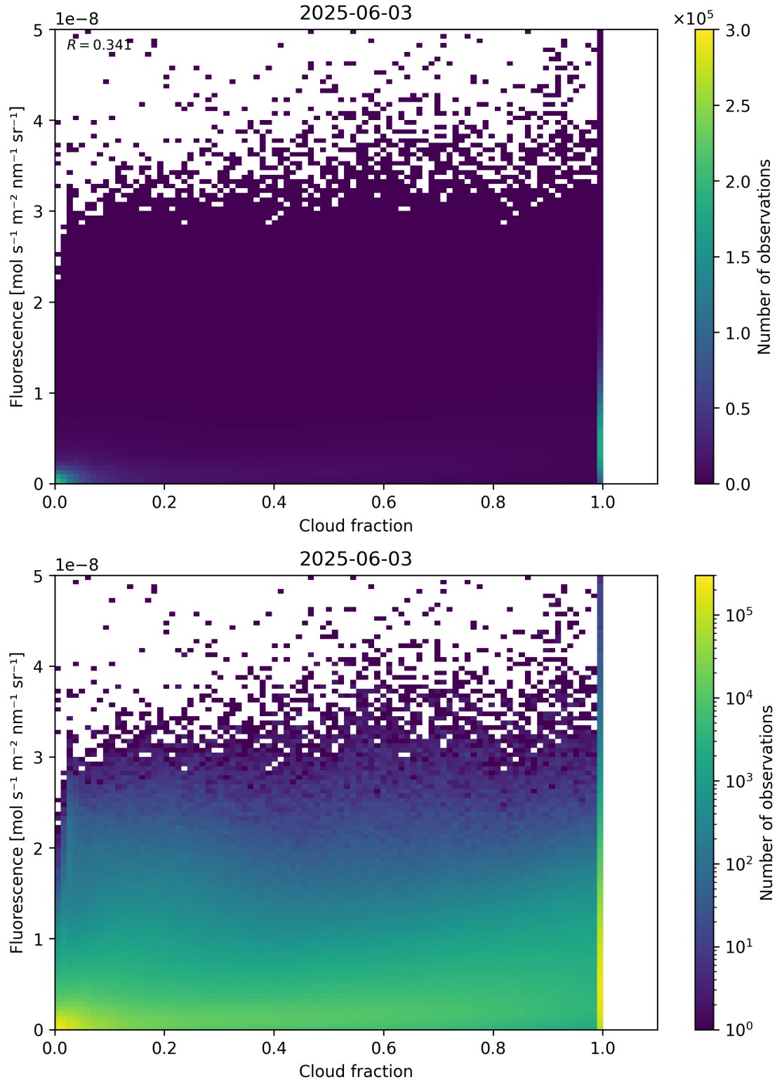
Figure 72: Scatter density plot of “Cloud fraction” against “Fluorescence” for 2025-06-02 to 2025-06-04.
