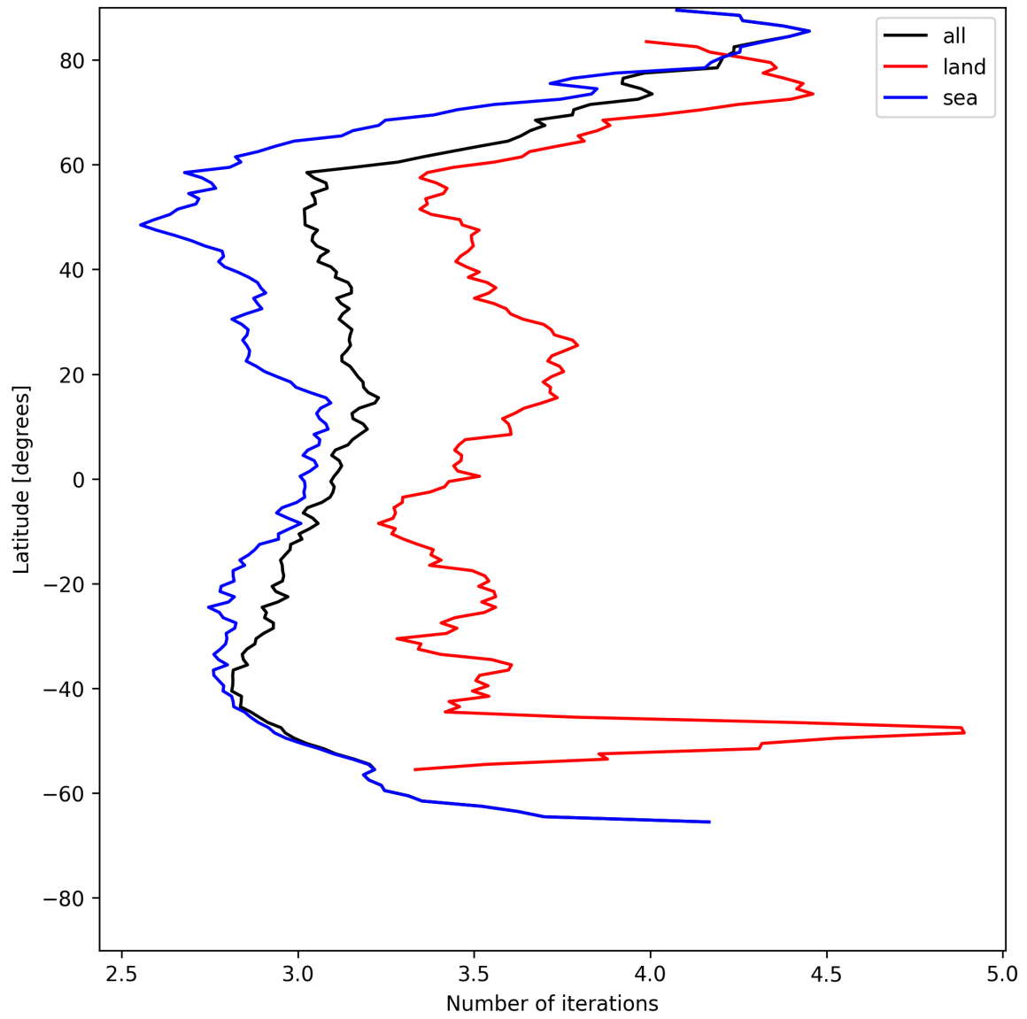
Figure 22: Zonal average of “Number of iterations” for 2025-06-02 to 2025-06-04.
