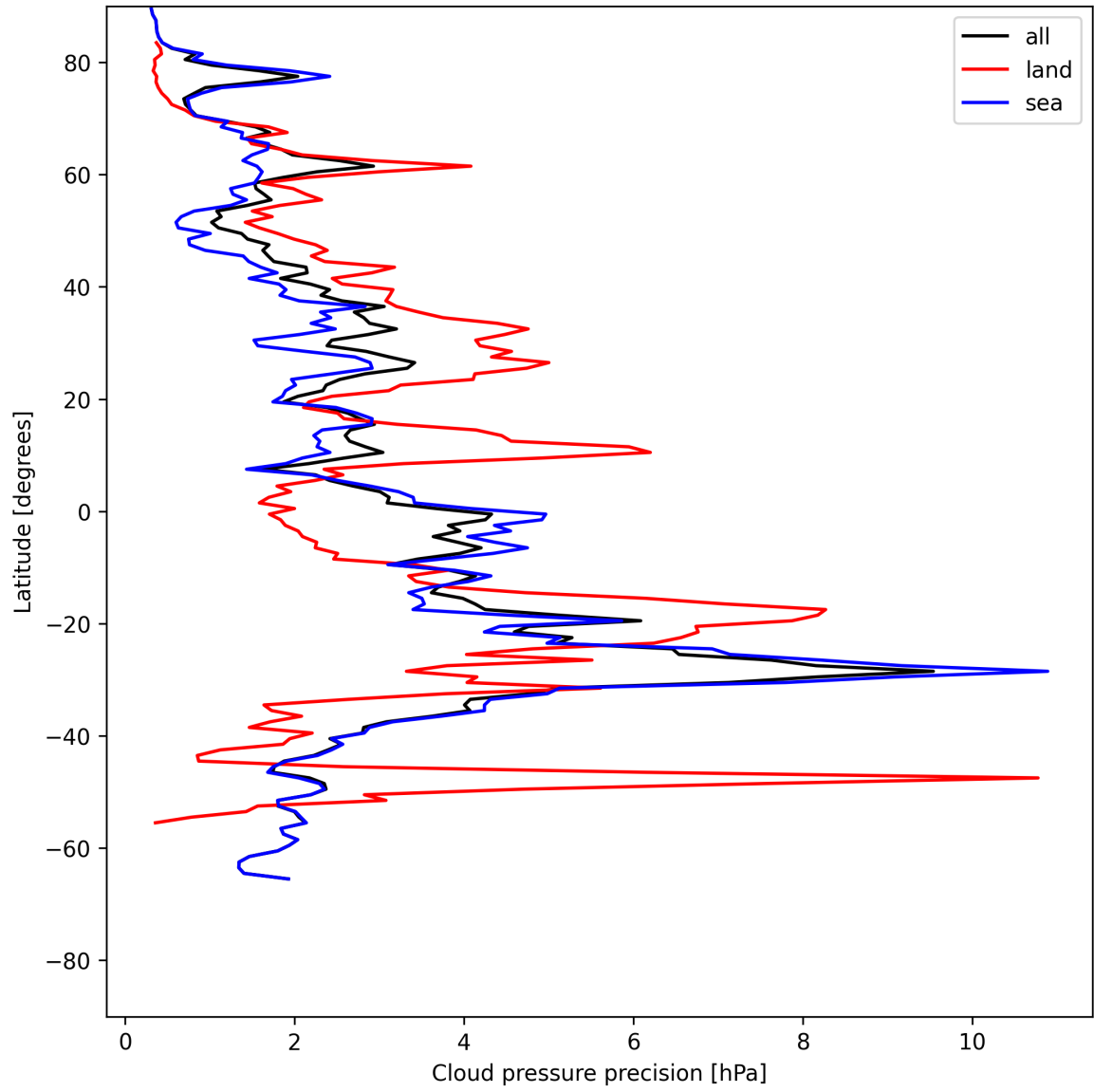
Figure 14: Zonal average of “Cloud pressure precision” for 2025-06-02 to 2025-06-04.
