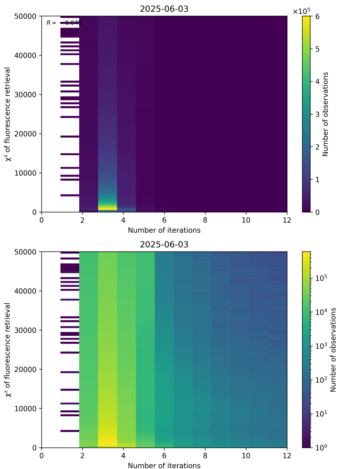
Figure 97: Scatter density plot of “Number of iterations” against “ \chi^2 of fluorescence retrieval” for 2025-06-02 to 2025-06-04.
