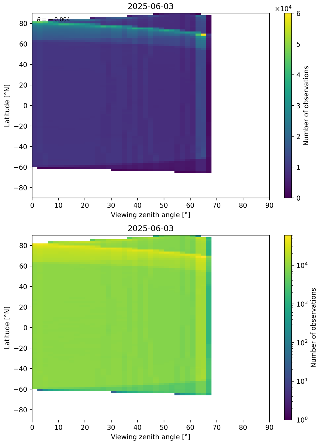
Figure 123: Scatter density plot of “Viewing zenith angle” against “Latitude” for 2025-06-02 to 2025-06-04.
