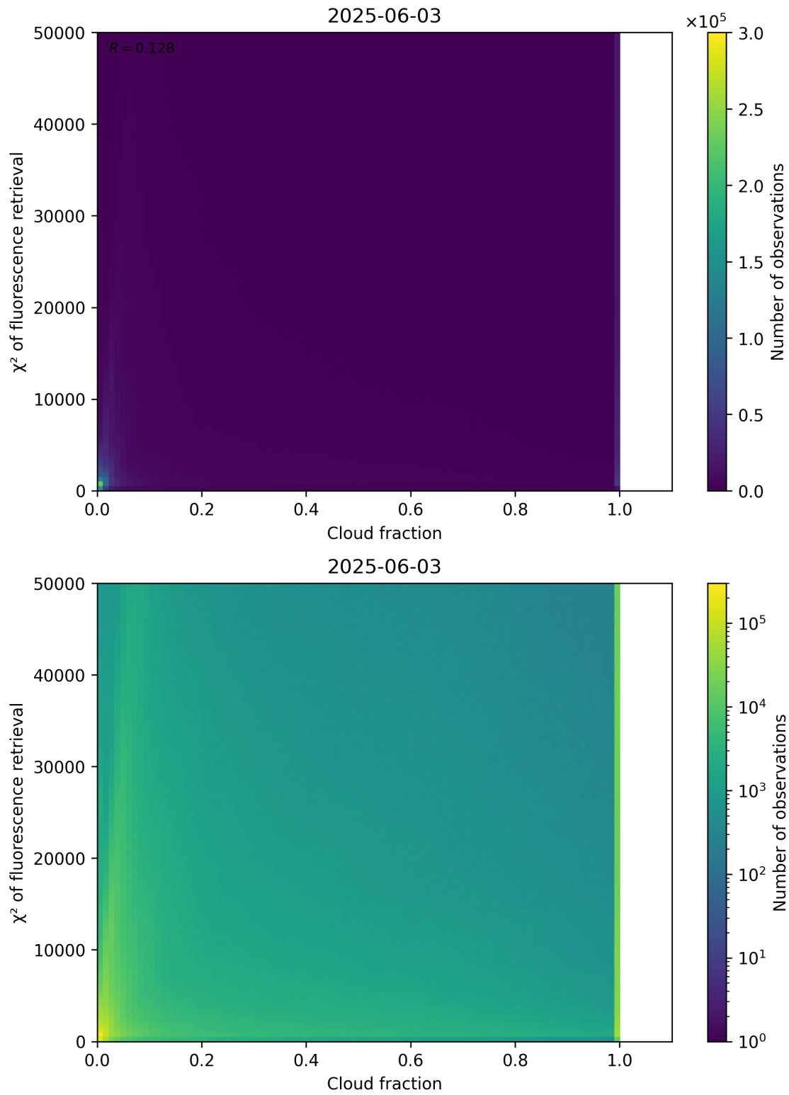
Figure 71: Scatter density plot of “Cloud fraction” against “ \chi^2 of fluorescence retrieval” for 2025-06-02 to 2025-06-04.
