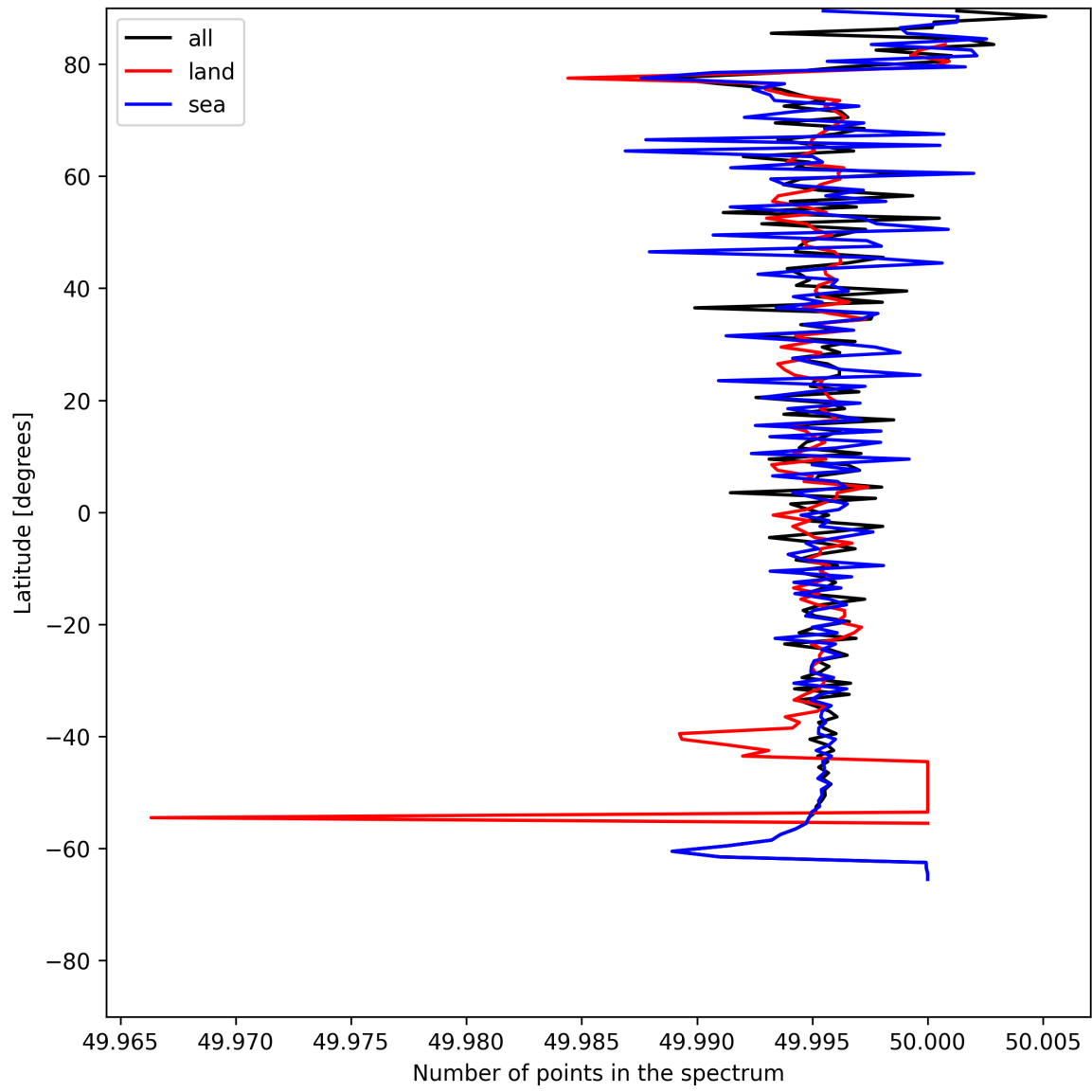
Figure 27: Zonal average of “Number of points in the spectrum” for 2025-06-02 to 2025-06-04.
