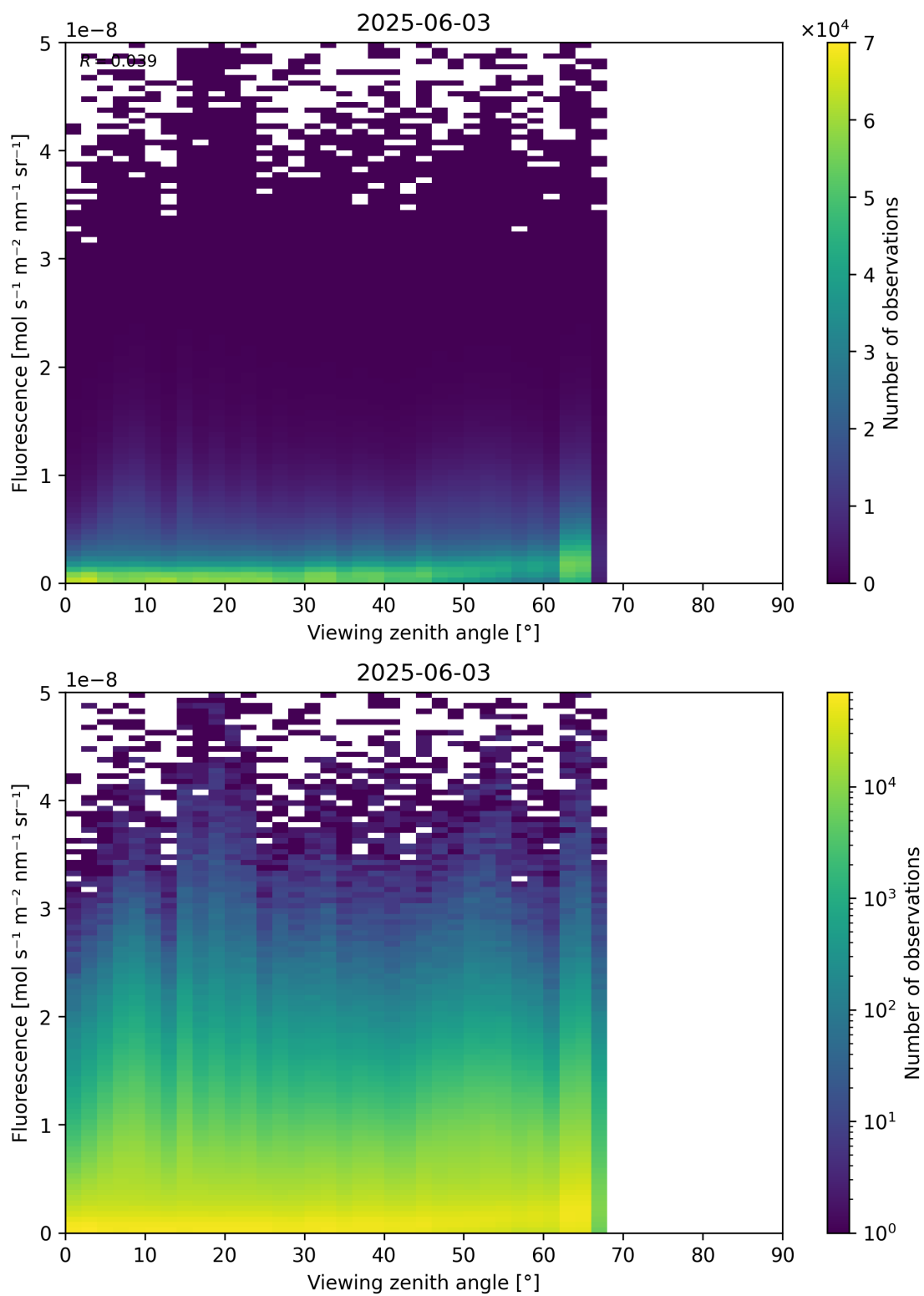
Figure 122: Scatter density plot of "Viewing zenith angle" against "Fluorescence" for 2025-06-02 to 2025-06-04.
