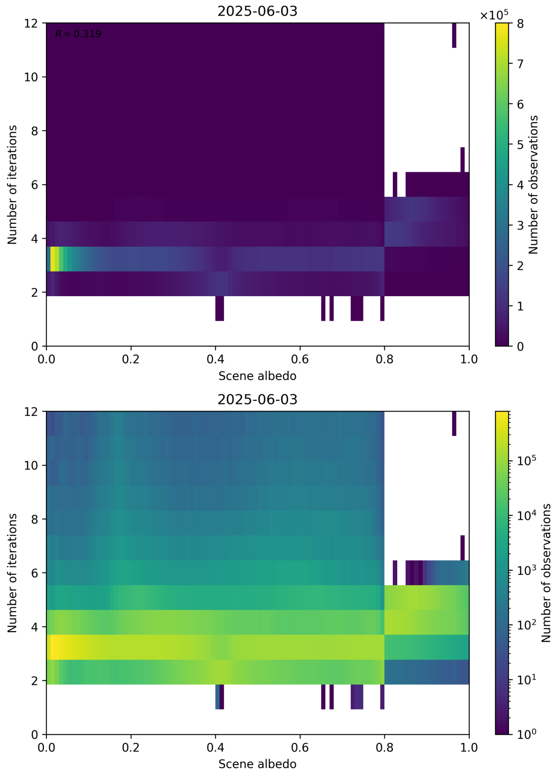
Figure 105: Scatter density plot of “Scene albedo” against “Number of iterations” for 2025-06-02 to 2025-06-04.
