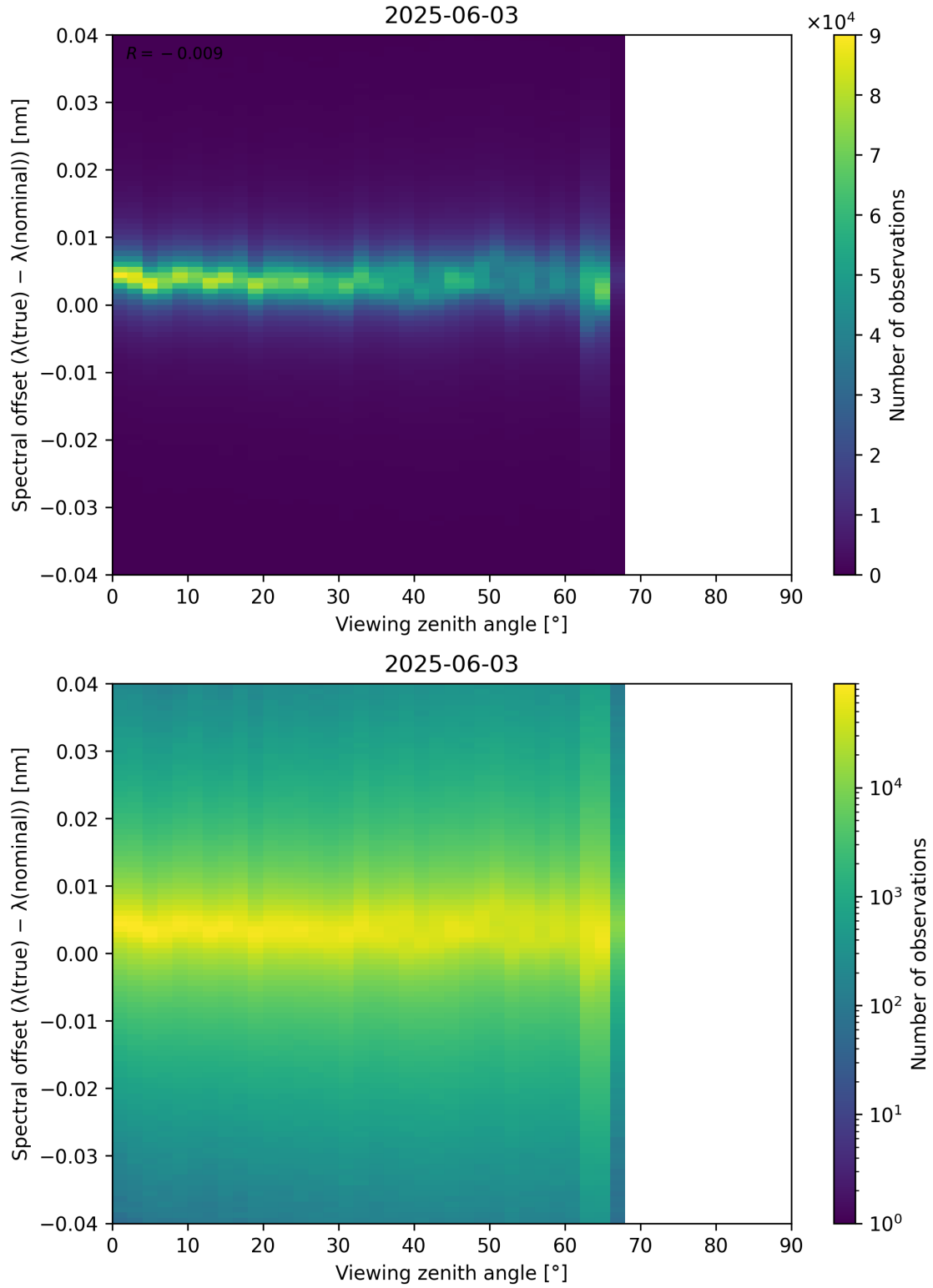
Figure 128: Scatter density plot of “Viewing zenith angle” against “Spectral offset ( \lambda_{\text{true}} - \lambda_{\text{nominal}} )” for 2025-06-02 to 2025-06-04.
