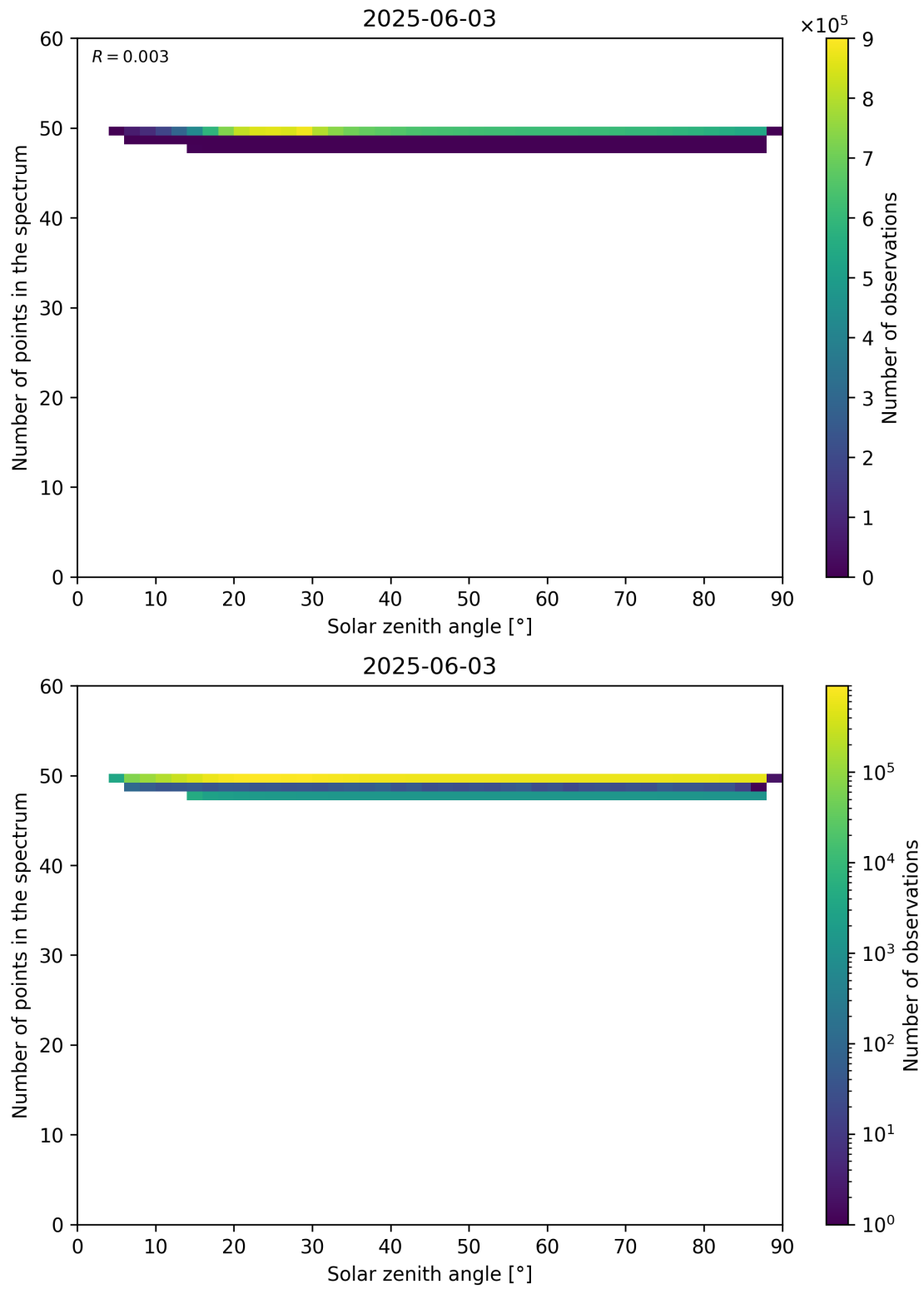
Figure 115: Scatter density plot of “Solar zenith angle” against “Number of points in the spectrum” for 2025-06-02 to 2025-06-04.
