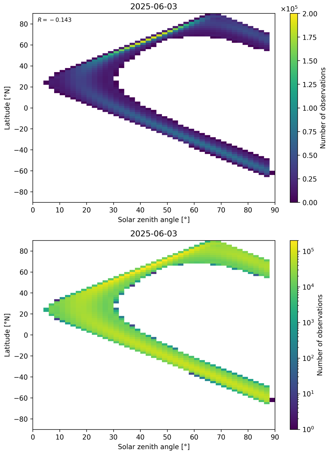
Figure 113: Scatter density plot of “Solar zenith angle” against “Latitude” for 2025-06-02 to 2025-06-04.
