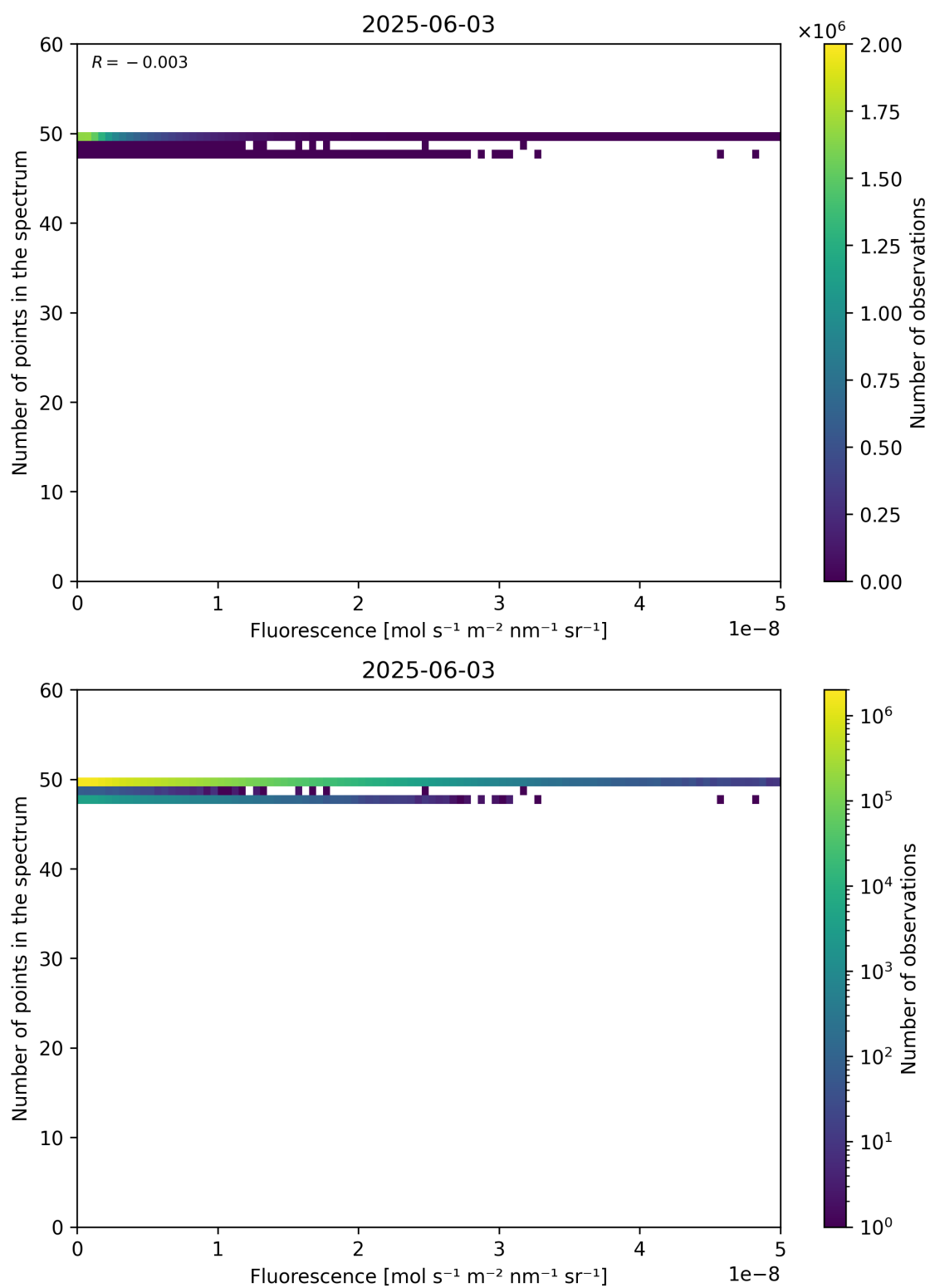
Figure 86: Scatter density plot of “Fluorescence” against “Number of points in the spectrum” for 2025-06-02 to 2025-06-04.
