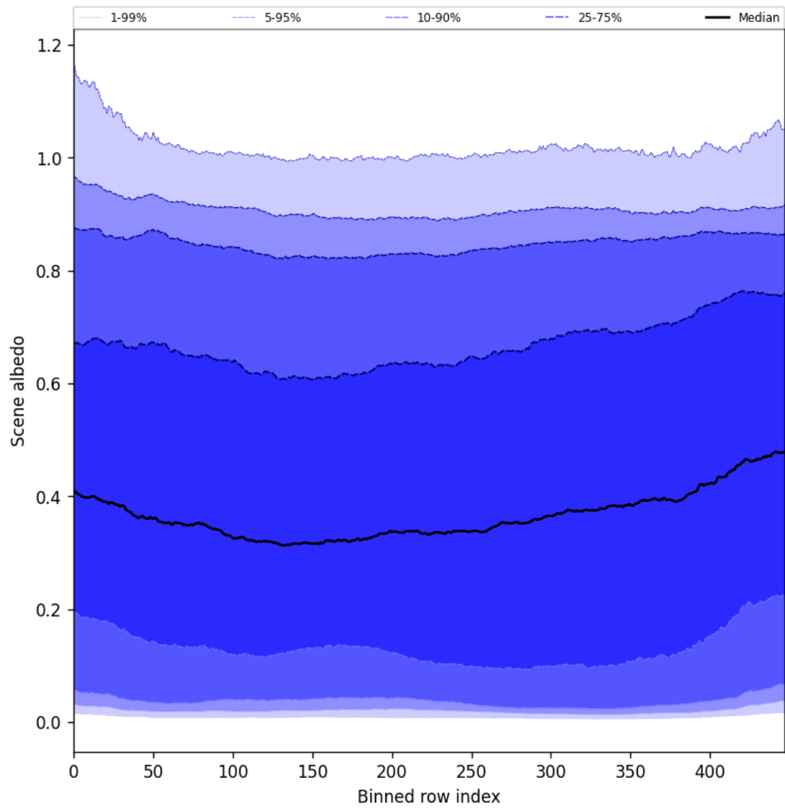
Figure 51: Along track statistics of “Scene albedo” for 2025-06-02 to 2025-06-04
