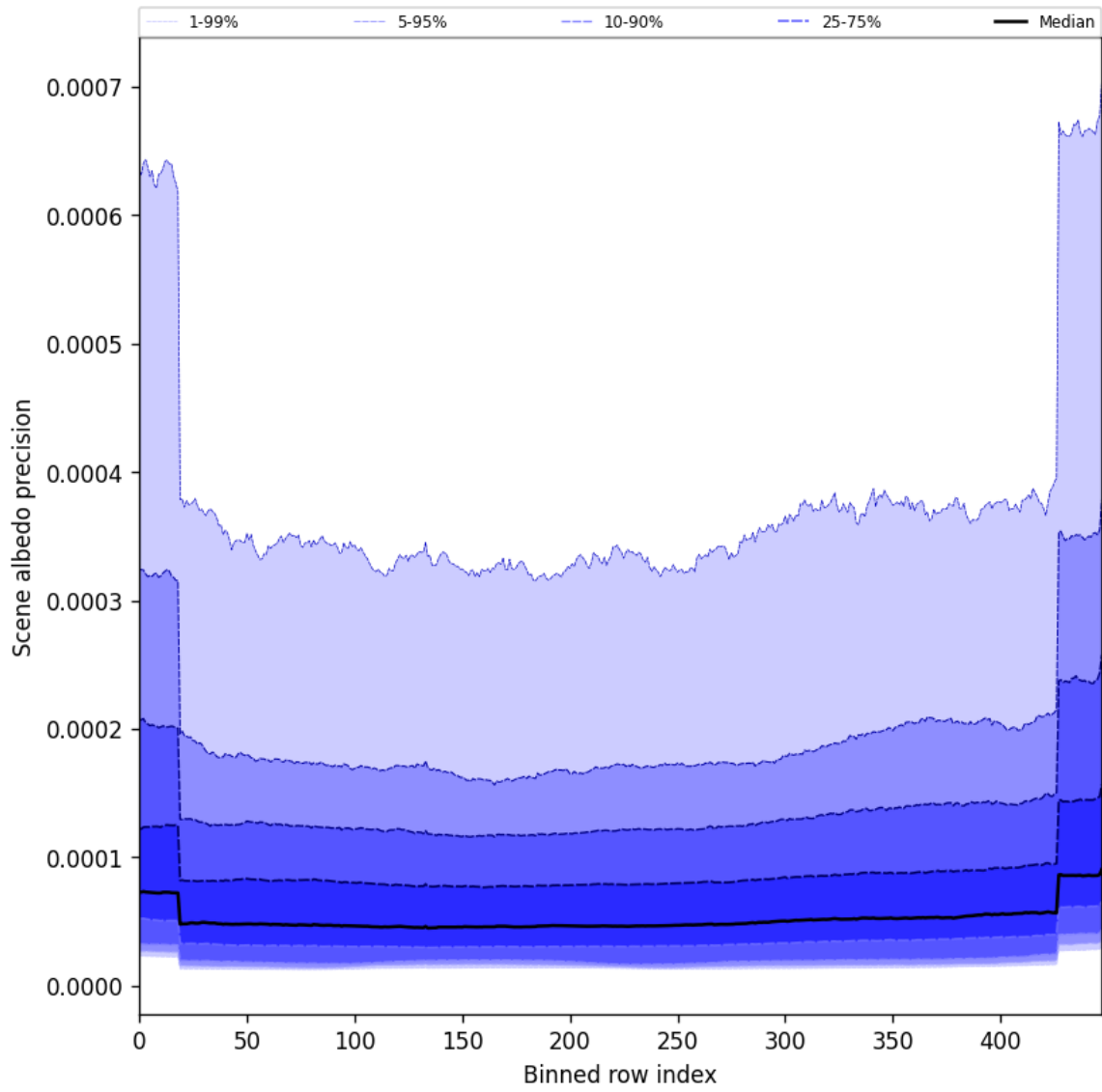
Figure 52: Along track statistics of “Scene albedo precision” for 2025-06-02 to 2025-06-04
