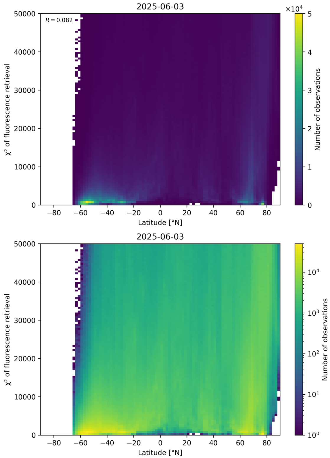
Figure 89: Scatter density plot of “Latitude” against “ \chi^2 of fluorescence retrieval” for 2025-06-02 to 2025-06-04.
