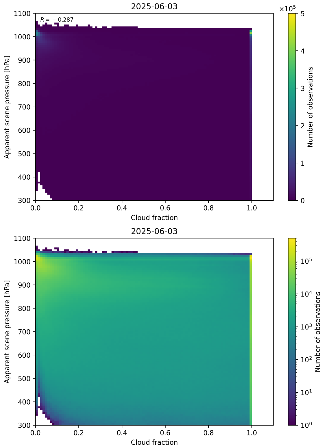
Figure 70: Scatter density plot of “Cloud fraction” against “Apparent scene pressure” for 2025-06-02 to 2025-06-04.
