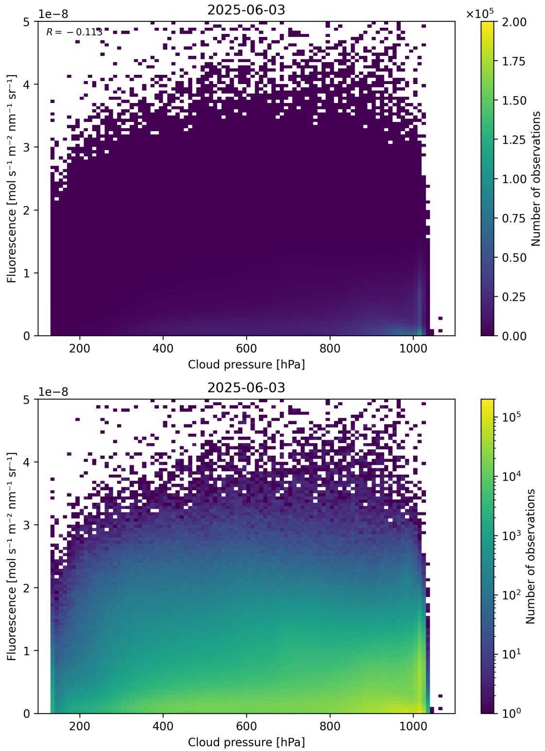
Figure 80: Scatter density plot of “Cloud pressure” against “Fluorescence” for 2025-06-02 to 2025-06-04.
