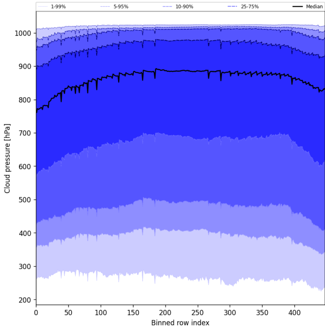
Figure 47: Along track statistics of “Cloud pressure” for 2025-06-02 to 2025-06-04
