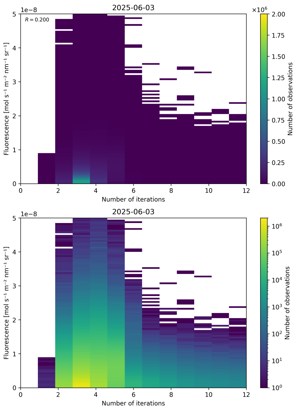
Figure 98: Scatter density plot of “Number of iterations” against “Fluorescence” for 2025-06-02 to 2025-06-04.
