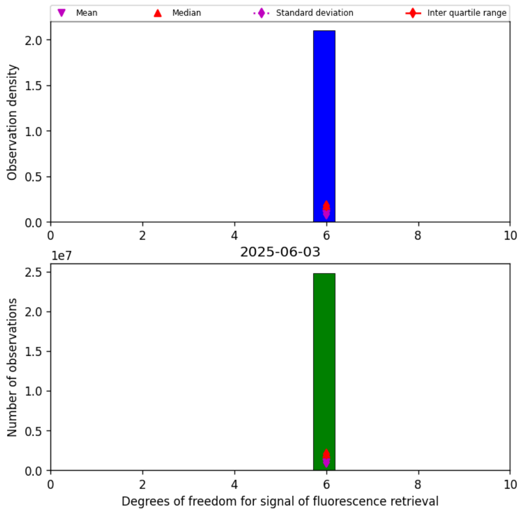
Figure 43: Histogram of “Degrees of freedom for signal of fluorescence retrieval” for 2025-06-02 to 2025-06-04
