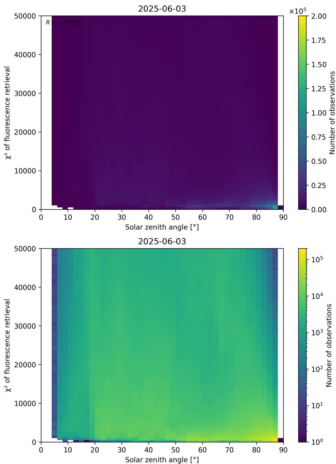
Figure 109: Scatter density plot of “Solar zenith angle” against “ \chi^2 of fluorescence retrieval” for 2025-06-02 to 2025-06-04.
