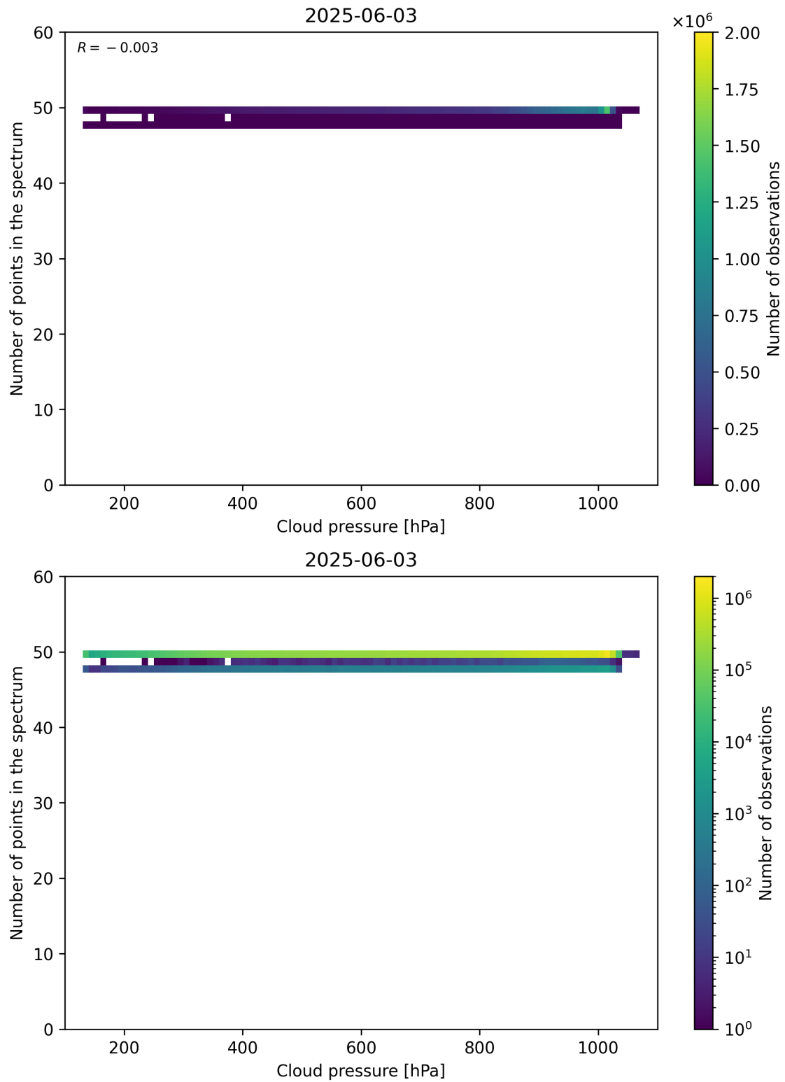
Figure 82: Scatter density plot of “Cloud pressure” against “Number of points in the spectrum” for 2025-06-02 to 2025-06-04.
