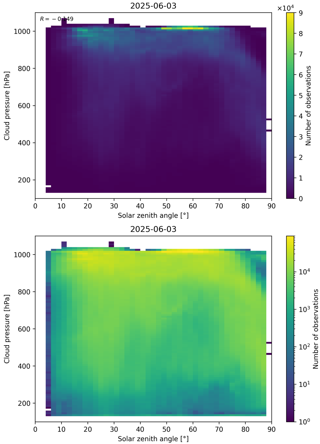
Figure 111: Scatter density plot of “Solar zenith angle” against “Cloud pressure” for 2025-06-02 to 2025-06-04.
