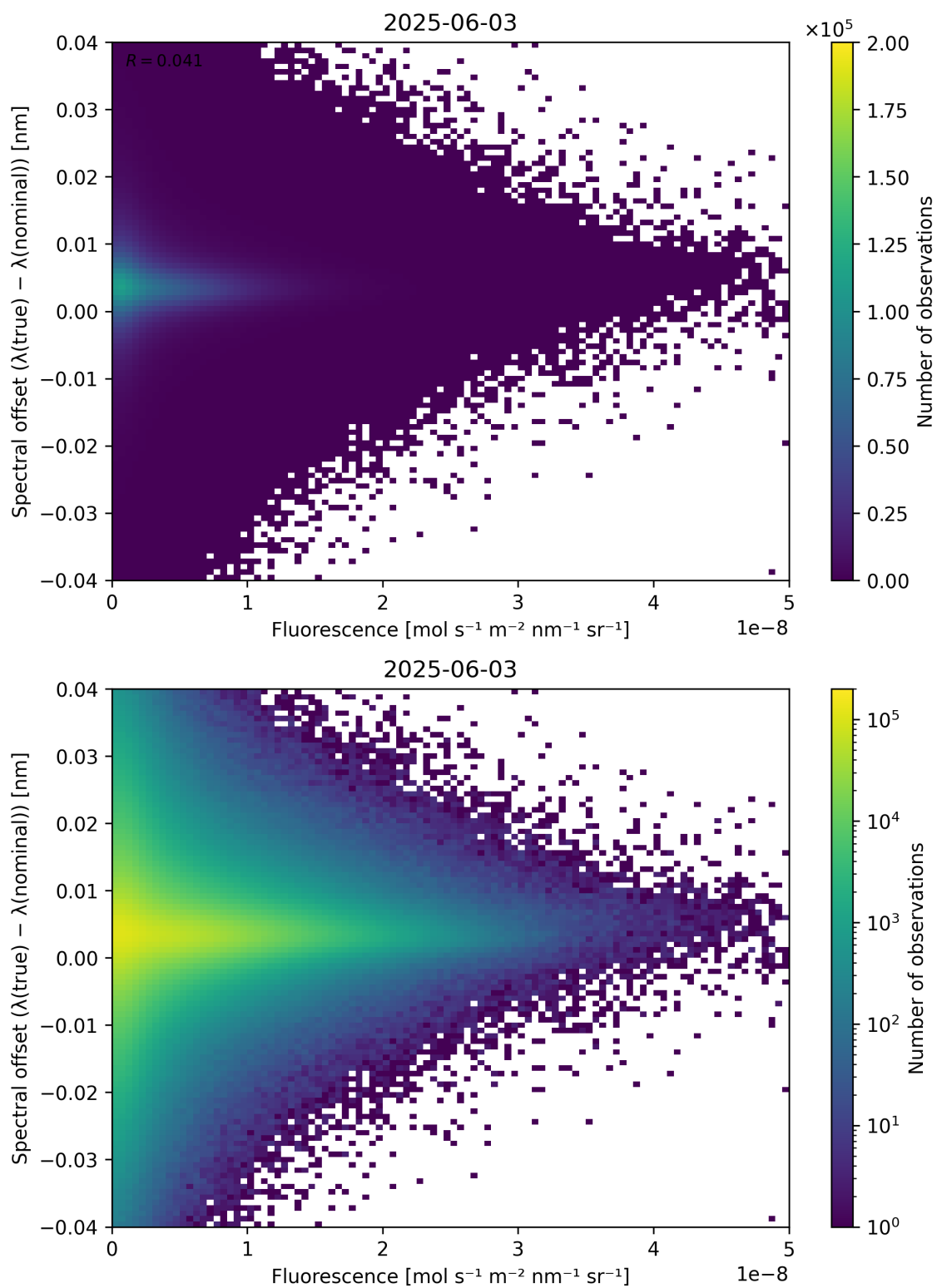
Figure 87: Scatter density plot of “Fluorescence” against “Spectral offset ( \lambda_{\text{true}} - \lambda_{\text{nominal}} )” for 2025-06-02 to 2025-06-04.
