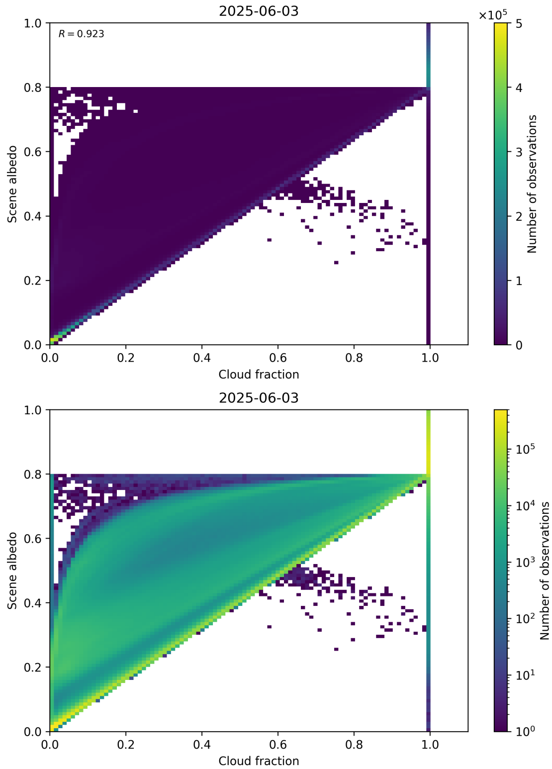
Figure 75: Scatter density plot of “Cloud fraction” against “Scene albedo” for 2025-06-02 to 2025-06-04.
