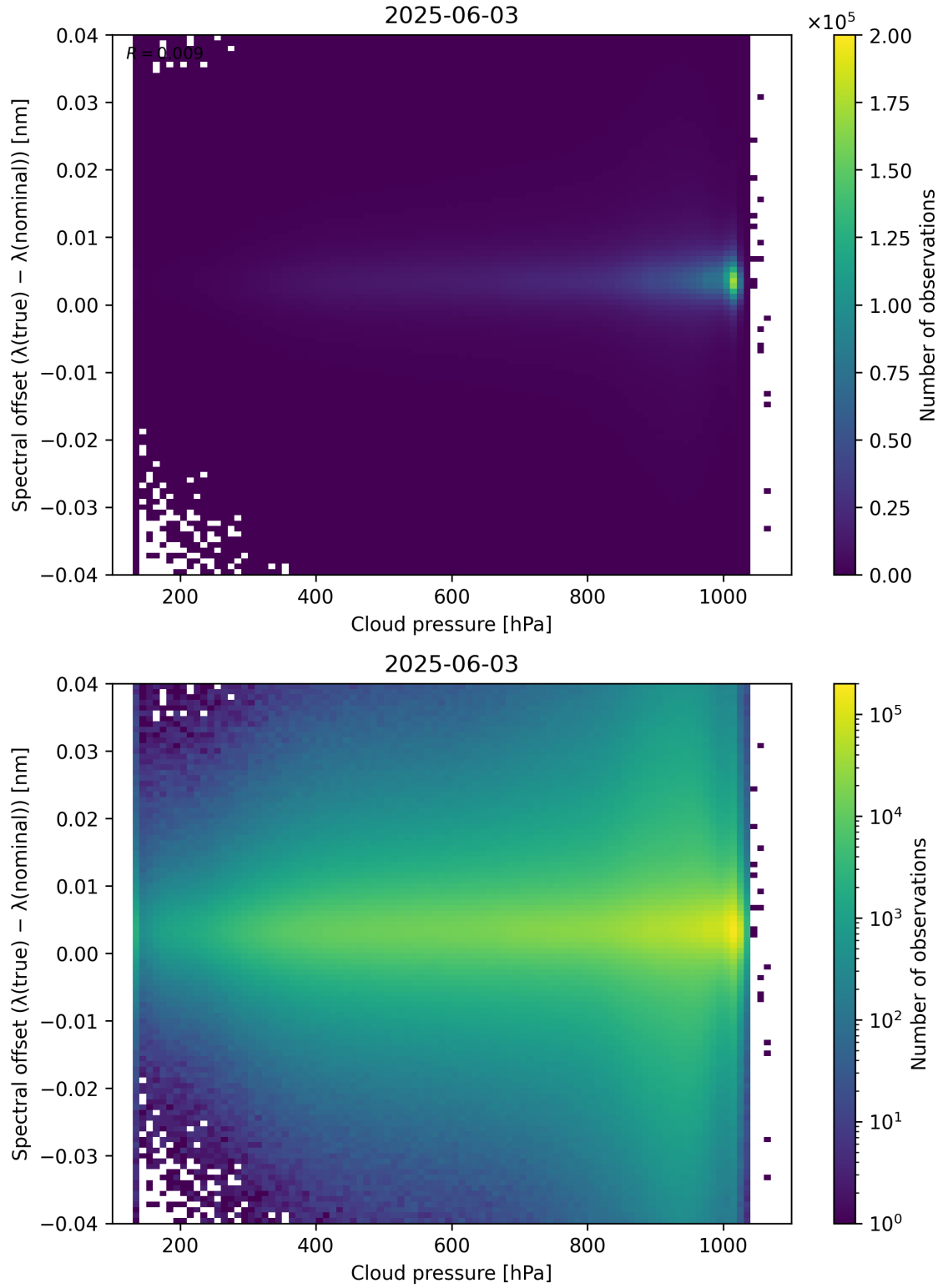
Figure 84: Scatter density plot of “Cloud pressure” against “Spectral offset ( \lambda_{\text{true}} - \lambda_{\text{nominal}} )” for 2025-06-02 to 2025-06-04.
