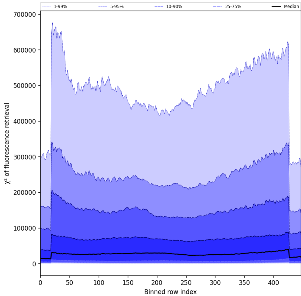
Figure 59: Along track statistics of “ \chi^2 of fluorescence retrieval” for 2025-06-02 to 2025-06-04
