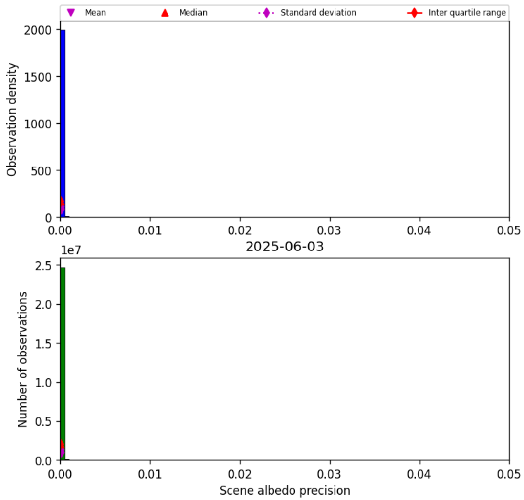
Figure 35: Histogram of “Scene albedo precision” for 2025-06-02 to 2025-06-04
