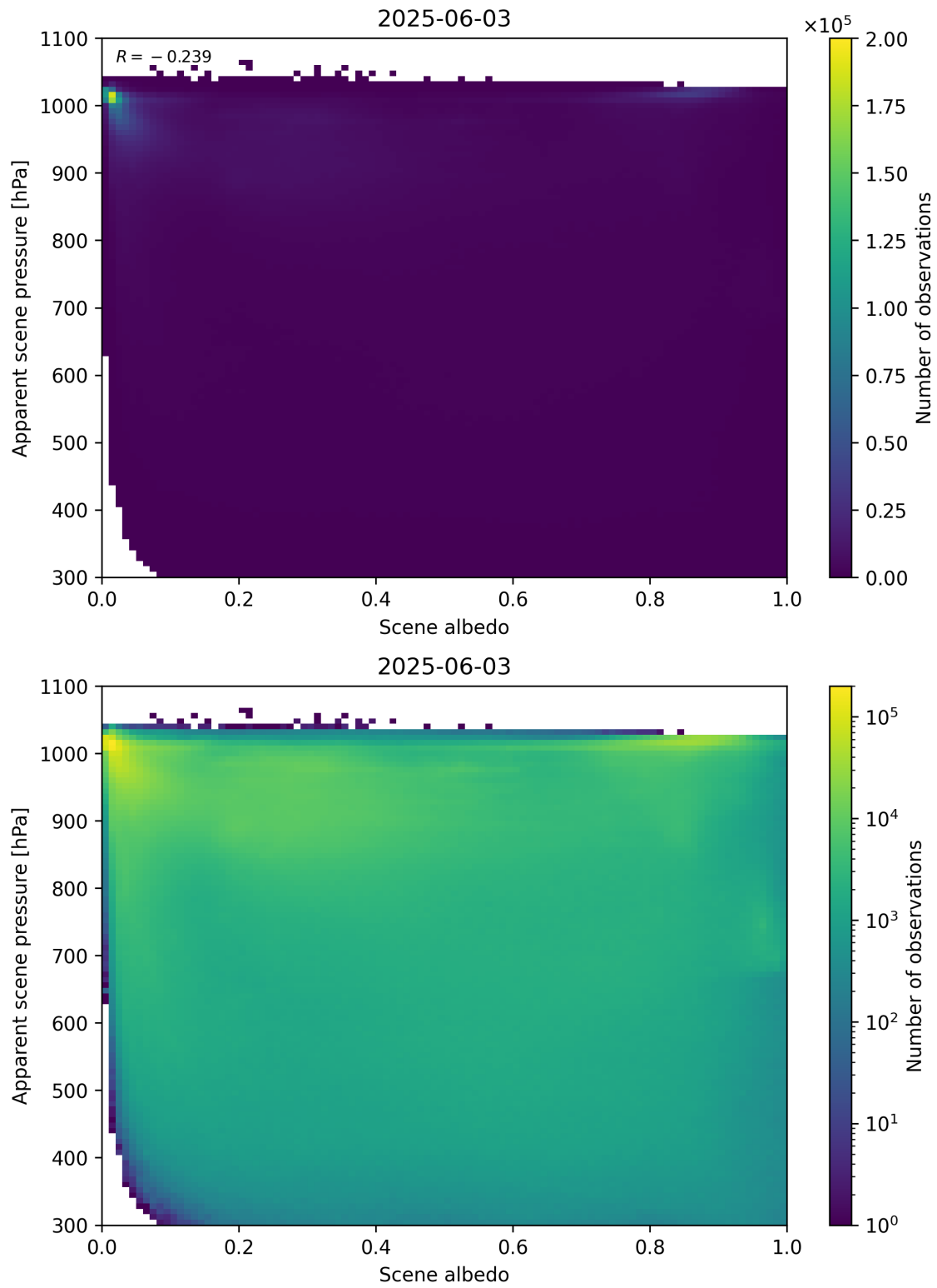
Figure 102: Scatter density plot of “Scene albedo” against “Apparent scene pressure” for 2025-06-02 to 2025-06-04.
