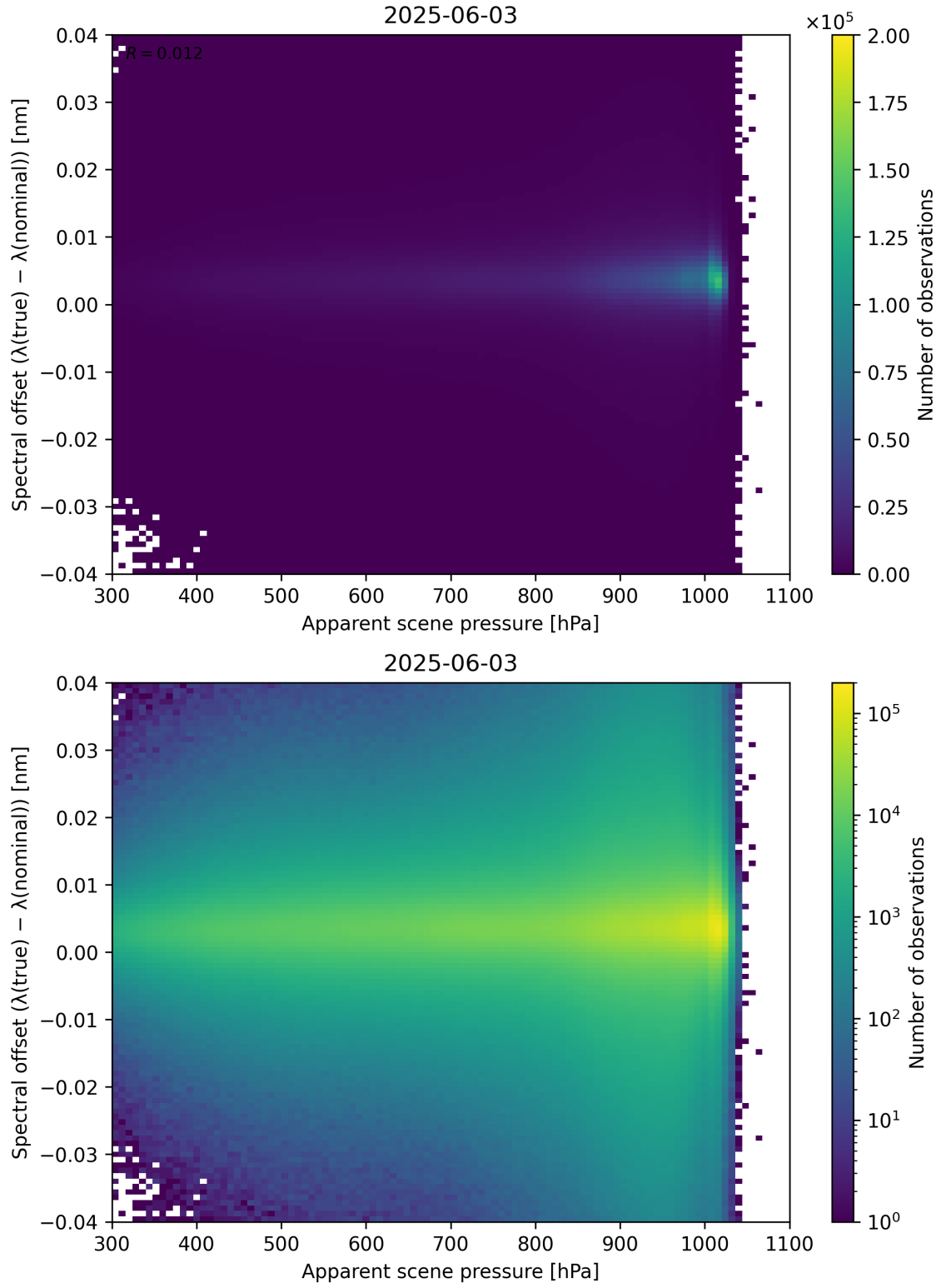
Figure 67: Scatter density plot of “Apparent scene pressure” against “Spectral offset ( \lambda_{\text{true}} - \lambda_{\text{nominal}} )” for 2025-06-02 to 2025-06-04.
