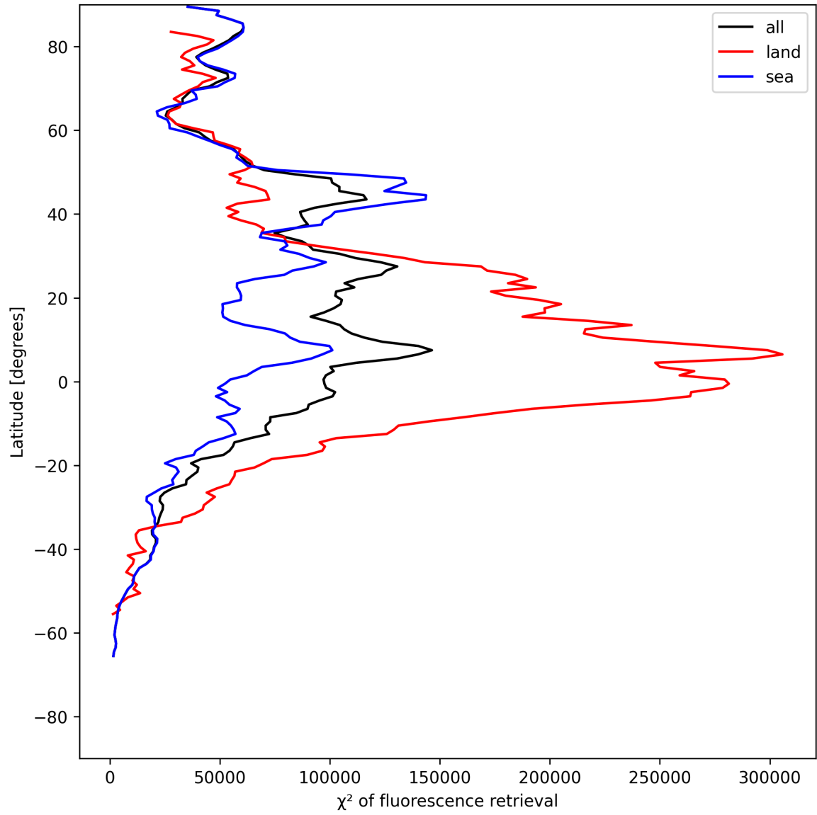
Figure 25: Zonal average of “ \chi^2 of fluorescence retrieval” for 2025-06-02 to 2025-06-04.
