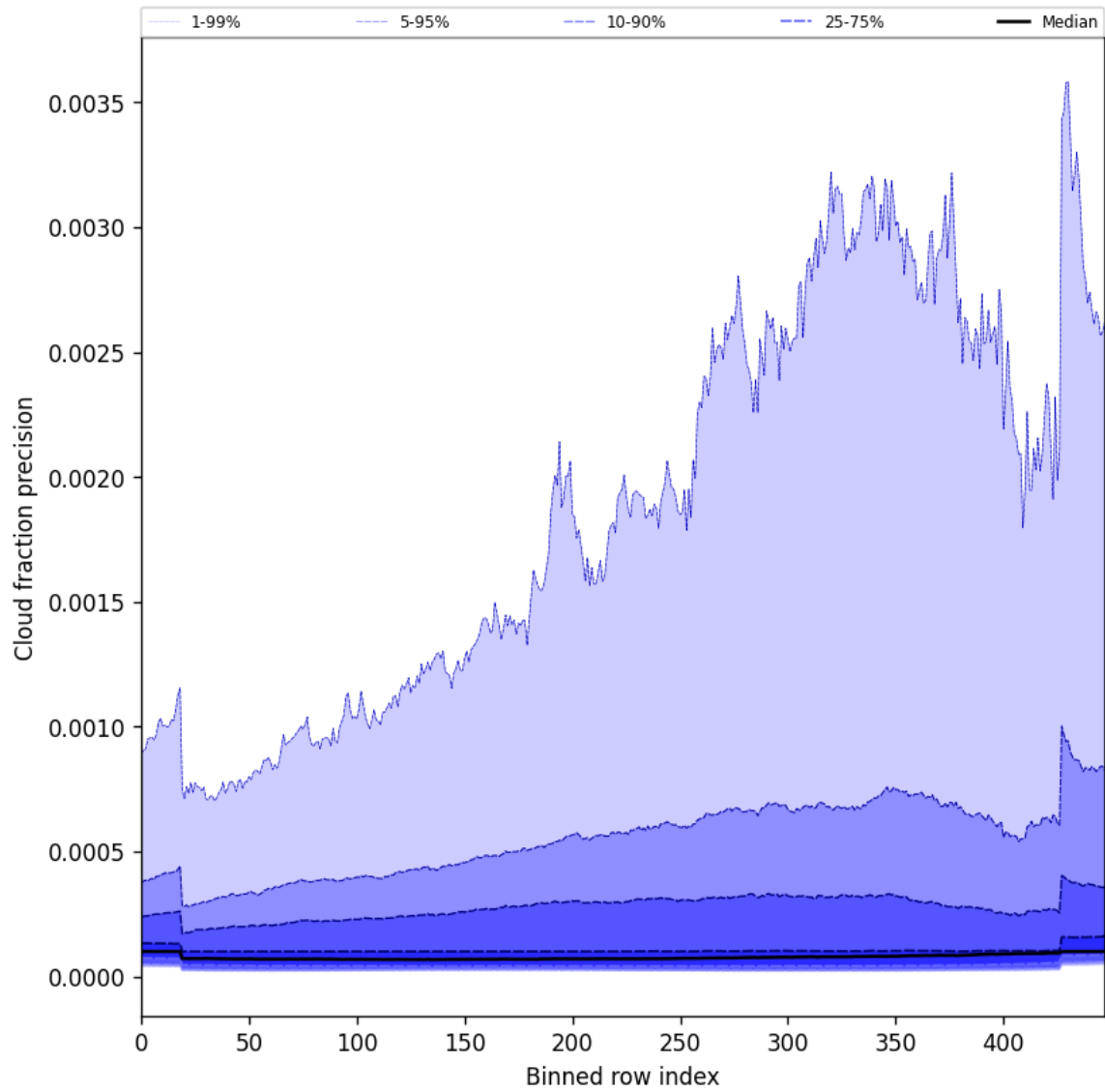
Figure 50: Along track statistics of “Cloud fraction precision” for 2025-06-02 to 2025-06-04
