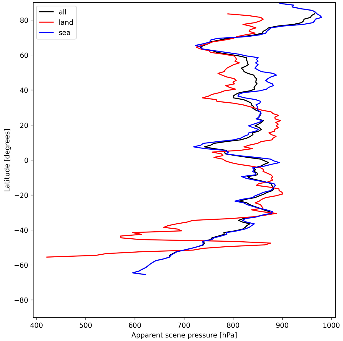
Figure 19: Zonal average of “Apparent scene pressure” for 2025-06-02 to 2025-06-04.
