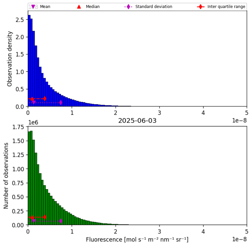
Figure 40: Histogram of “Fluorescence” for 2025-06-02 to 2025-06-04
