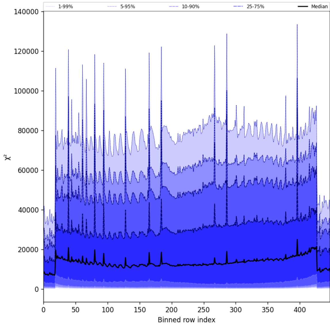
Figure 55: Along track statistics of “ \chi^2 ” for 2025-06-02 to 2025-06-04
