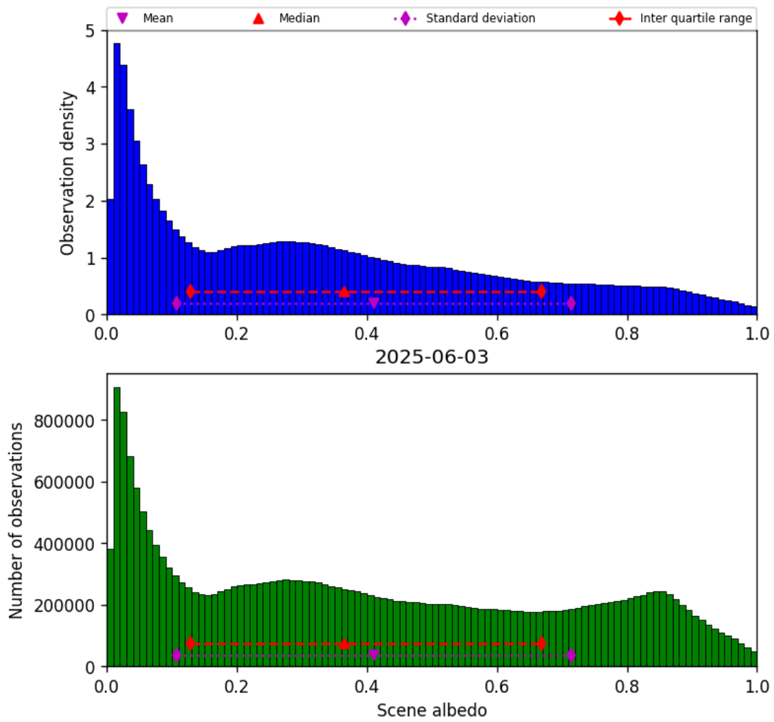
Figure 34: Histogram of “Scene albedo” for 2025-06-02 to 2025-06-04
