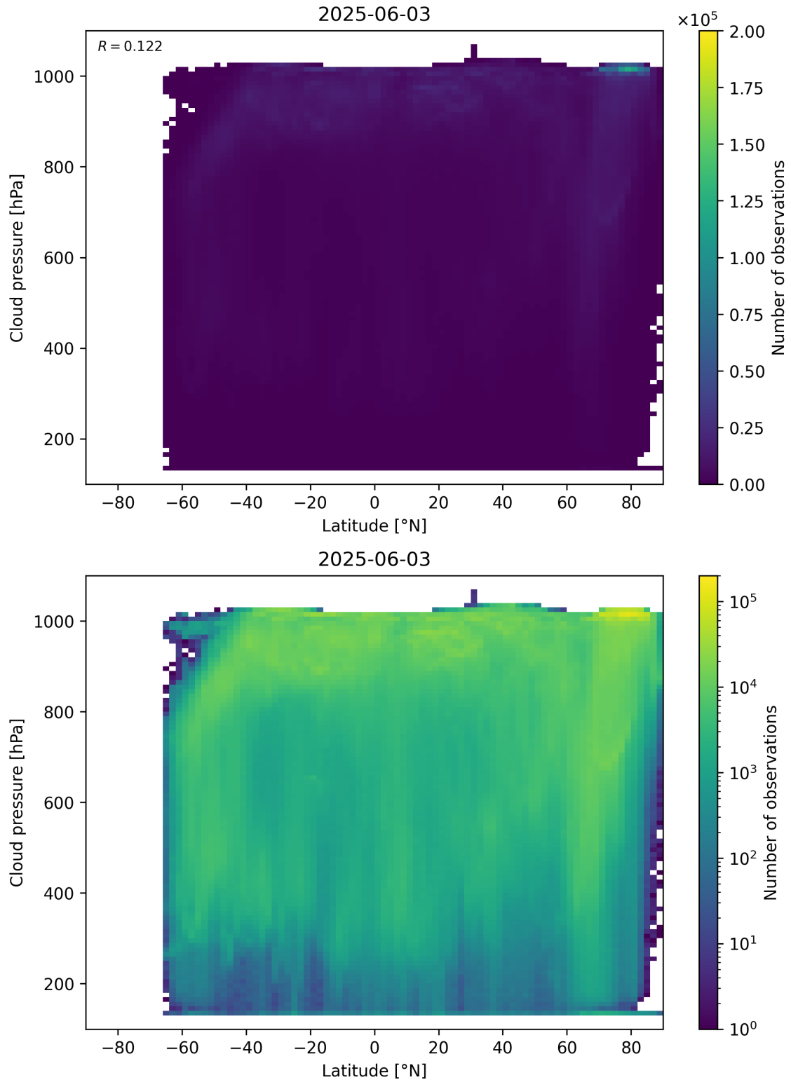
Figure 91: Scatter density plot of “Latitude” against “Cloud pressure” for 2025-06-02 to 2025-06-04.
