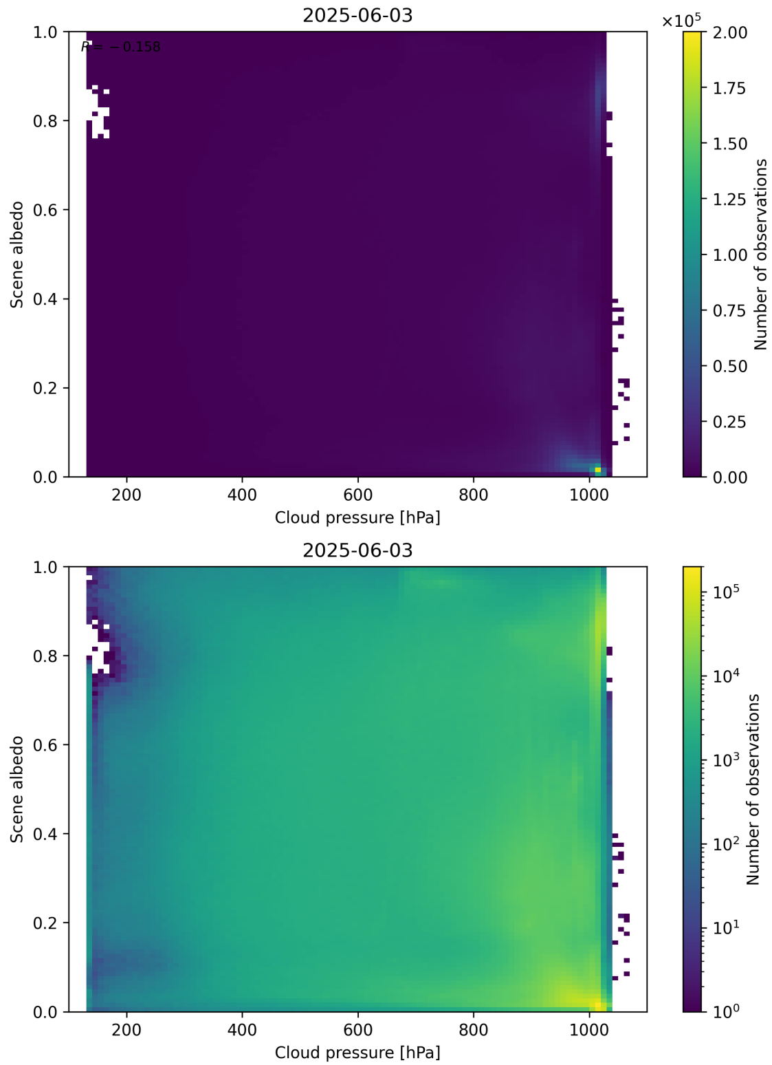
Figure 83: Scatter density plot of “Cloud pressure” against “Scene albedo” for 2025-06-02 to 2025-06-04.
