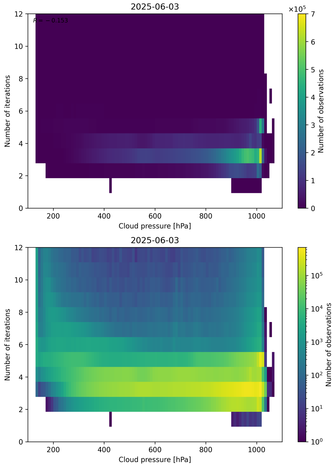
Figure 81: Scatter density plot of “Cloud pressure” against “Number of iterations” for 2025-06-02 to 2025-06-04.
