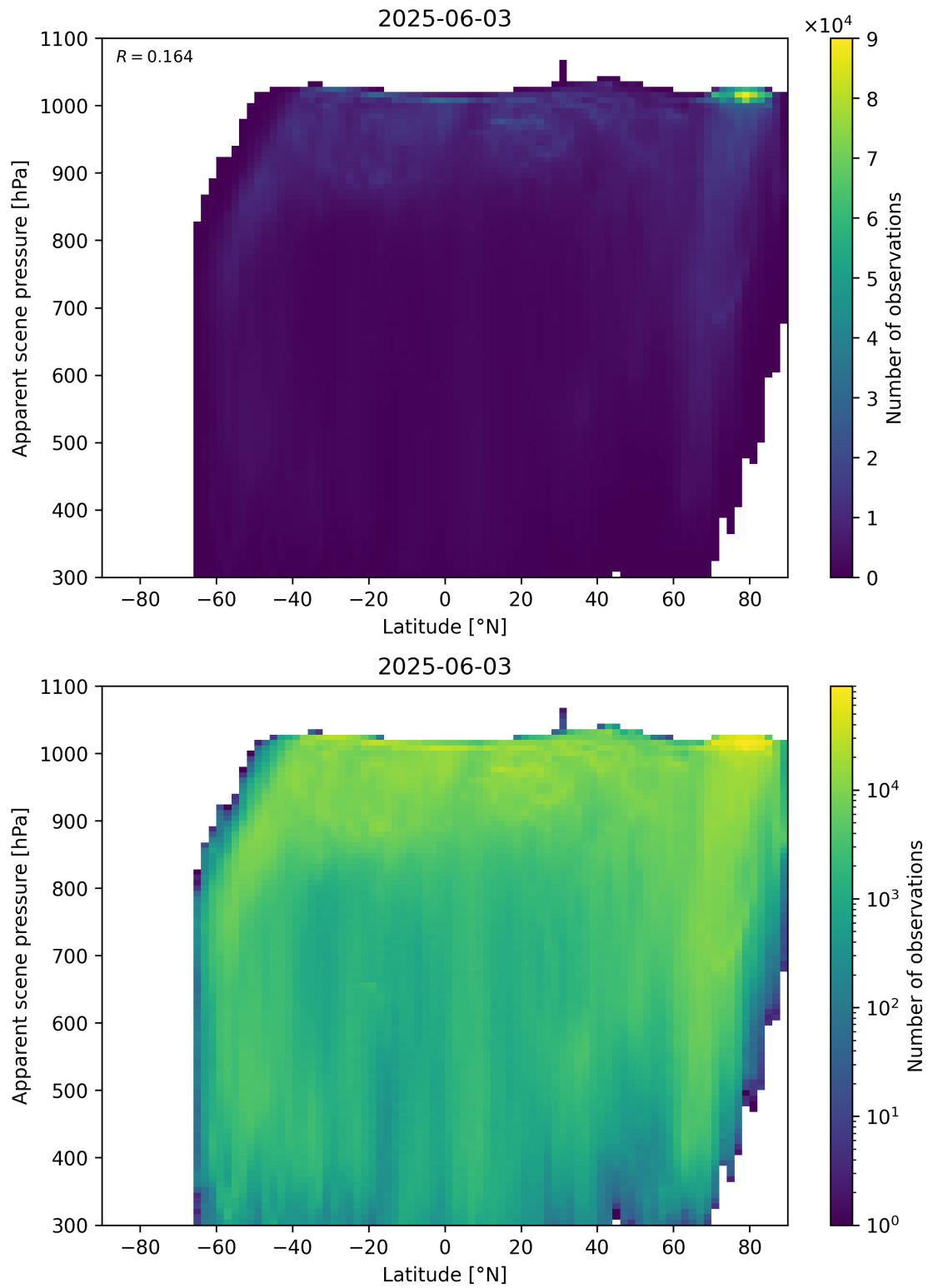
Figure 88: Scatter density plot of “Latitude” against “Apparent scene pressure” for 2025-06-02 to 2025-06-04.
