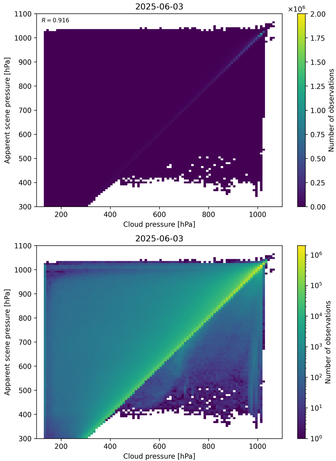
Figure 77: Scatter density plot of “Cloud pressure” against “Apparent scene pressure” for 2025-06-02 to 2025-06-04.
