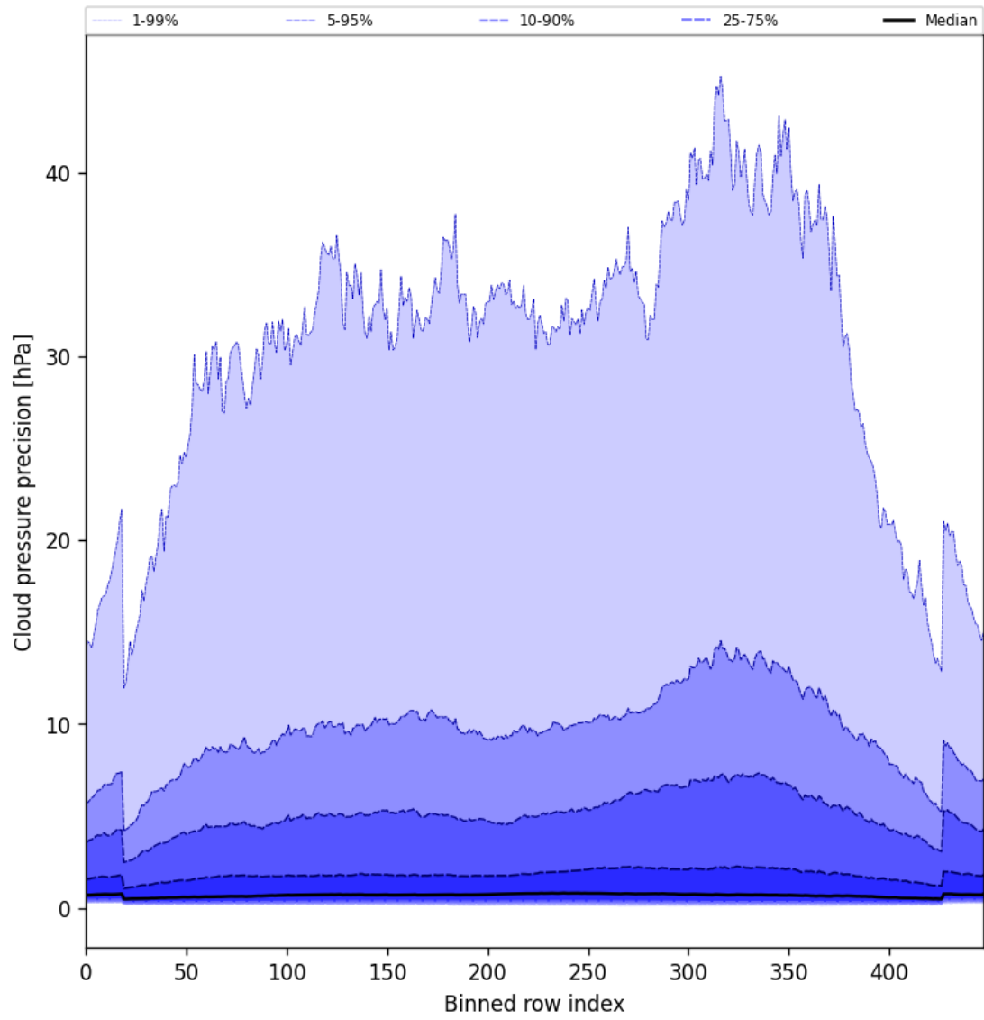
Figure 48: Along track statistics of “Cloud pressure precision” for 2025-06-02 to 2025-06-04
