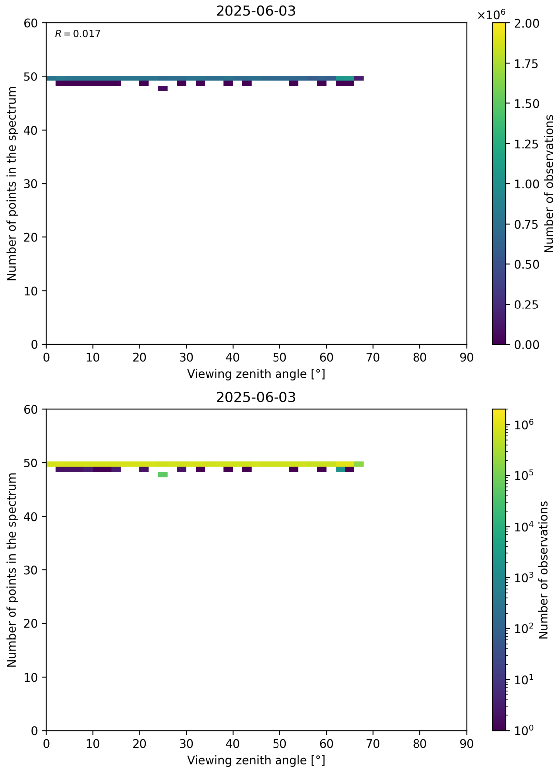
Figure 125: Scatter density plot of “Viewing zenith angle” against “Number of points in the spectrum” for 2025-06-02 to 2025-06-04.
