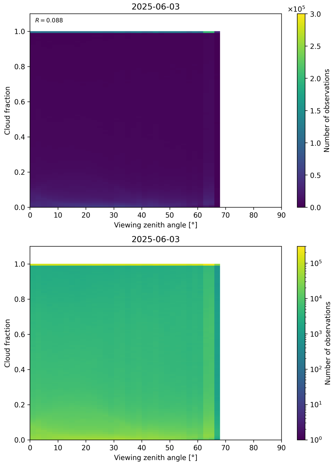
Figure 120: Scatter density plot of “Viewing zenith angle” against “Cloud fraction” for 2025-06-02 to 2025-06-04.
