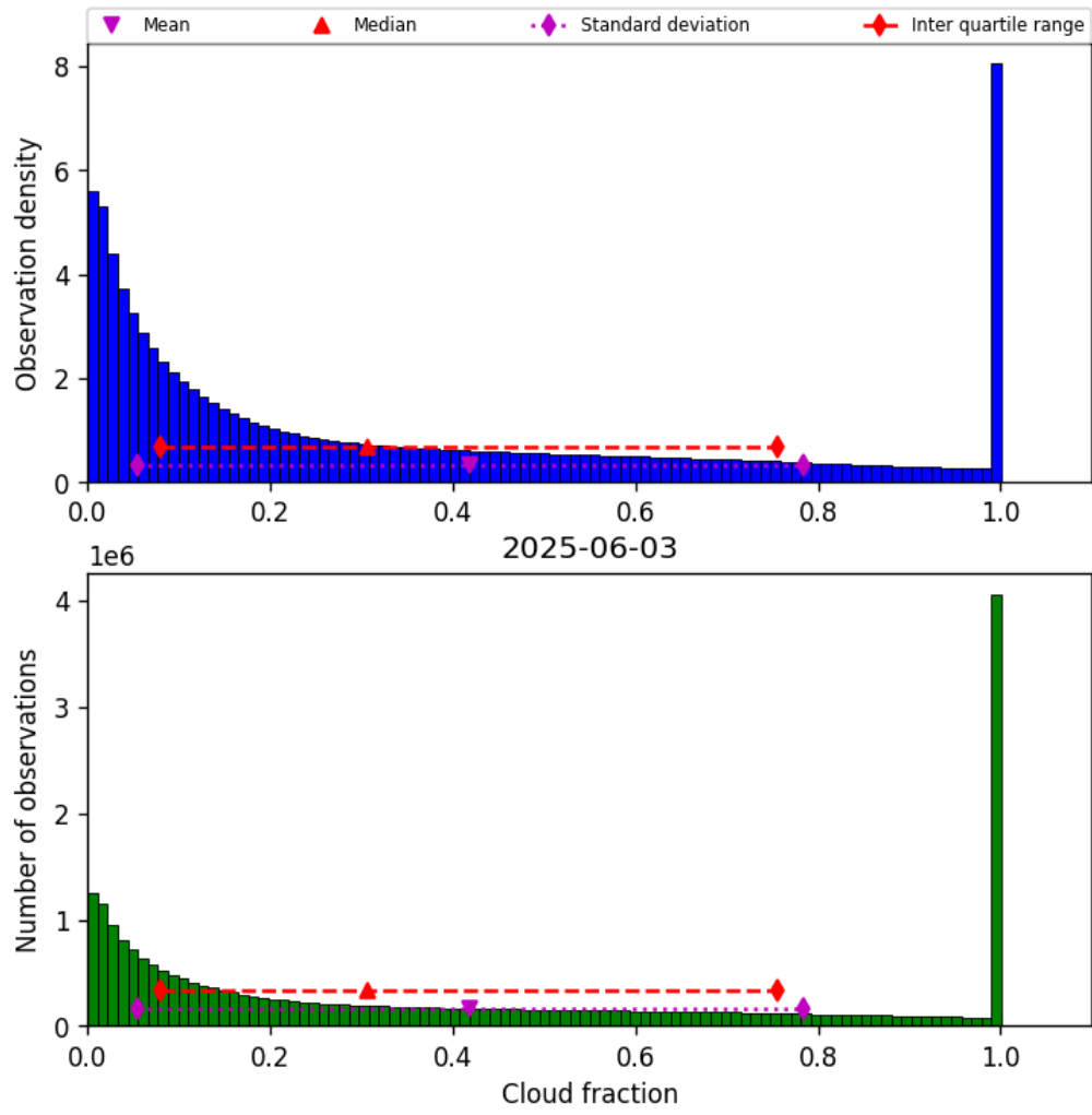
Figure 32: Histogram of “Cloud fraction” for 2025-06-02 to 2025-06-04
