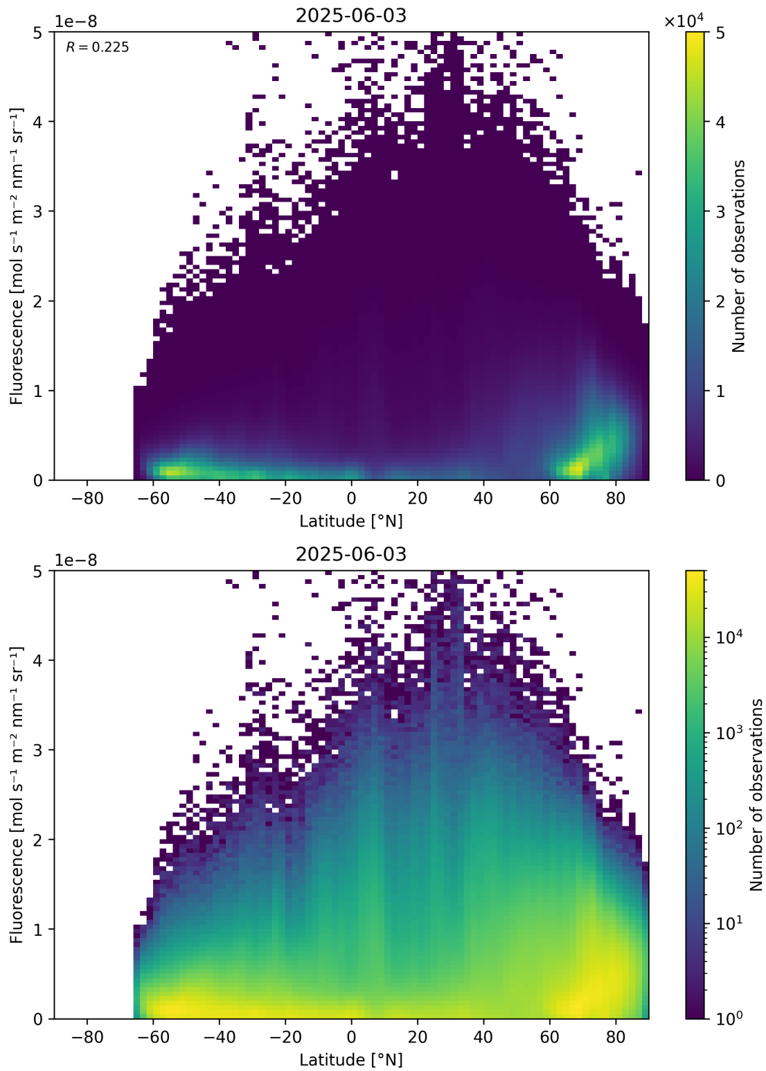
Figure 92: Scatter density plot of “Latitude” against “Fluorescence” for 2025-06-02 to 2025-06-04.
