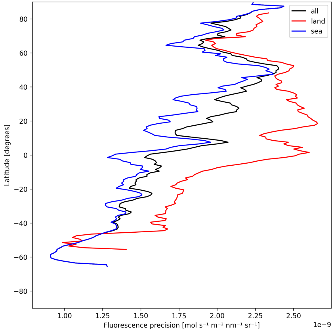
Figure 24: Zonal average of “Fluorescence precision” for 2025-06-02 to 2025-06-04.
