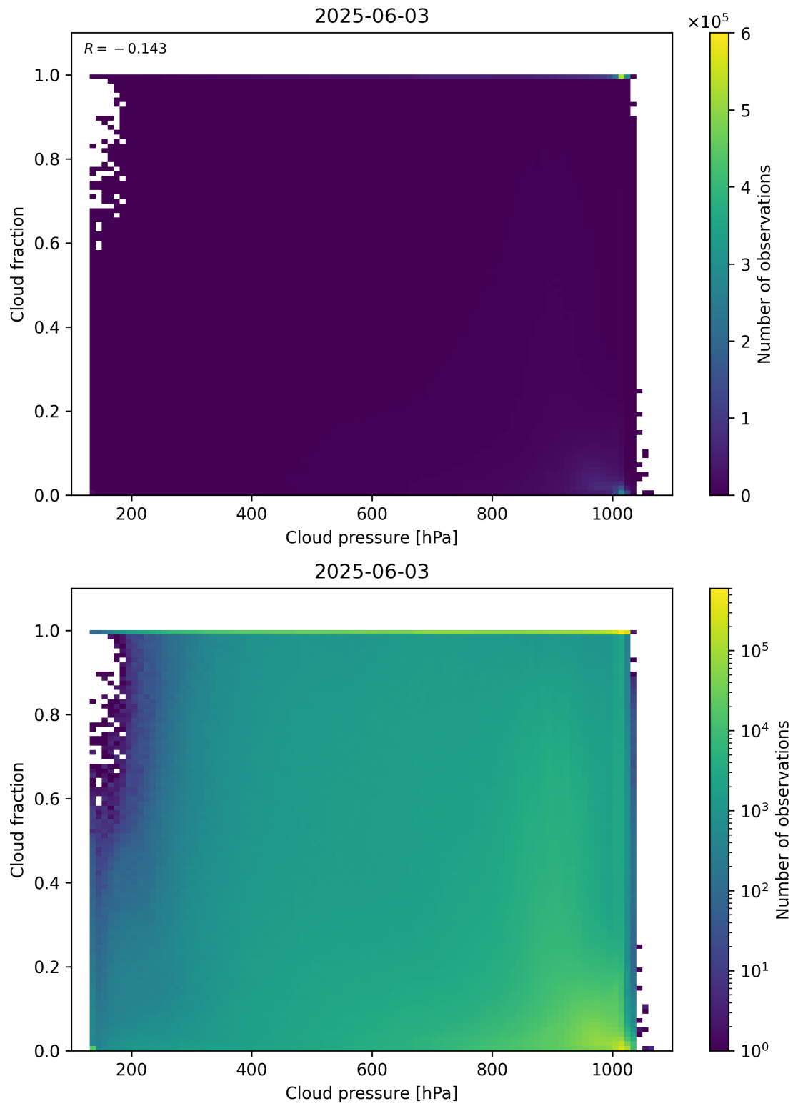
Figure 79: Scatter density plot of “Cloud pressure” against “Cloud fraction” for 2025-06-02 to 2025-06-04.
