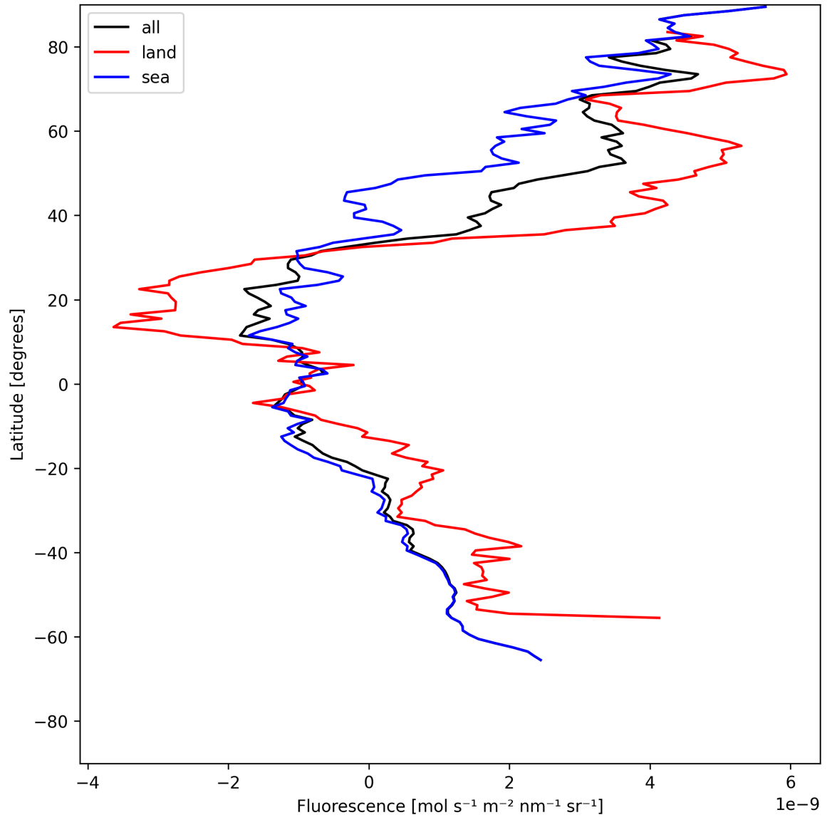
Figure 23: Zonal average of “Fluorescence” for 2025-06-02 to 2025-06-04.
