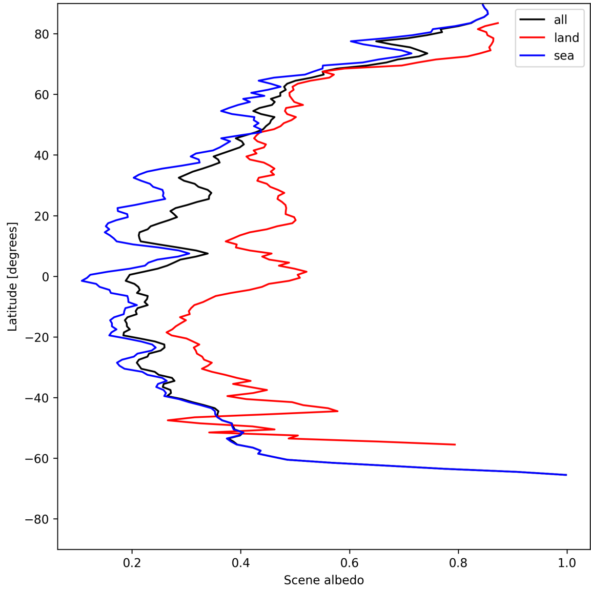
Figure 17: Zonal average of “Scene albedo” for 2025-06-02 to 2025-06-04.
