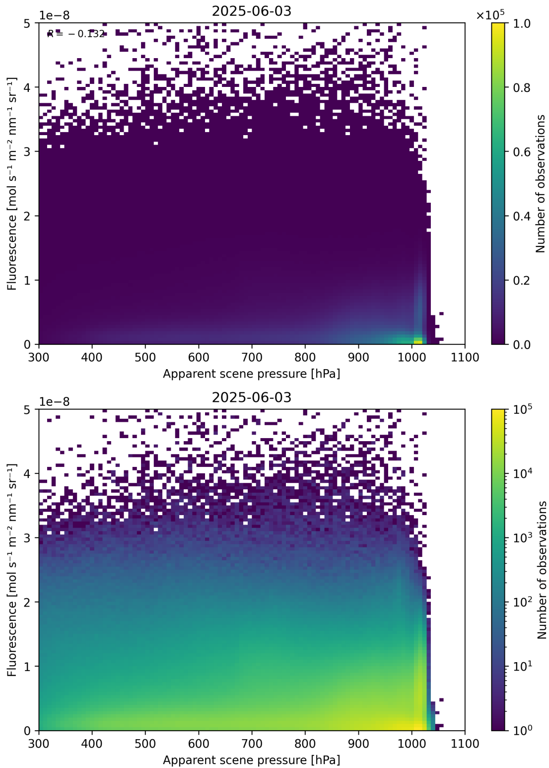
Figure 64: Scatter density plot of “Apparent scene pressure” against “Fluorescence” for 2025-06-02 to 2025-06-04.
