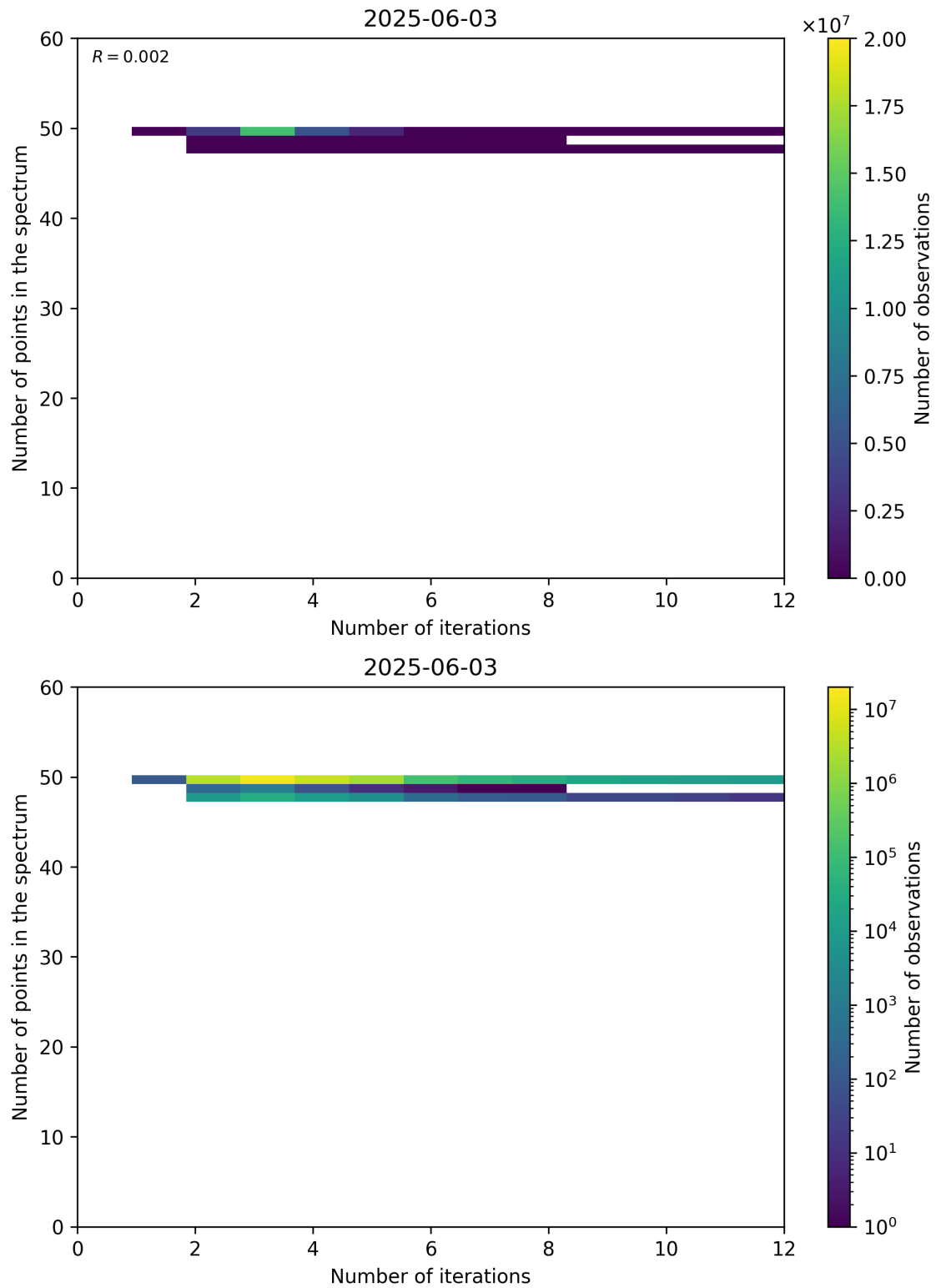
Figure 99: Scatter density plot of “Number of iterations” against “Number of points in the spectrum” for 2025-06-02 to 2025-06-04.
