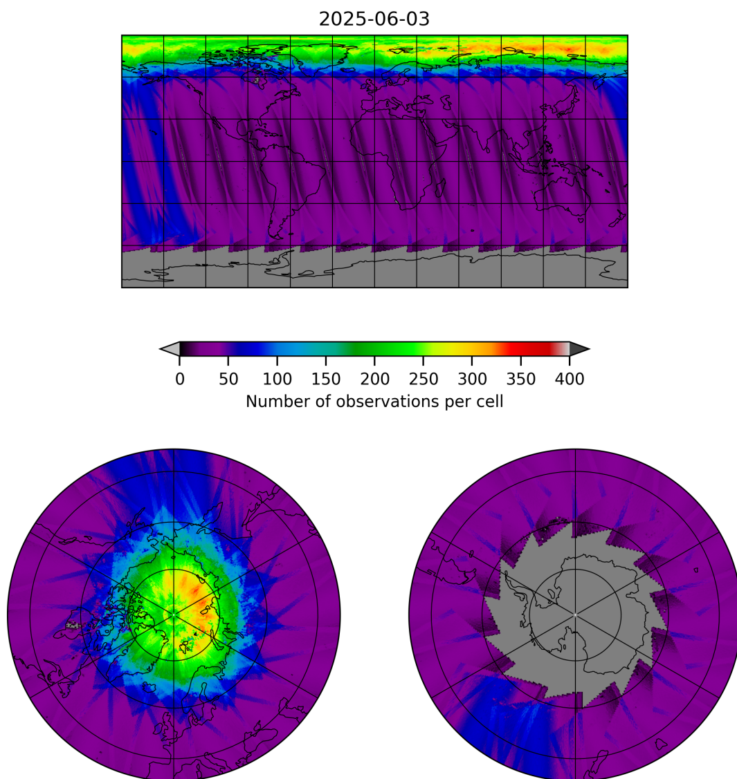
Figure 11: Map of the number of observations for 2025-06-02 to 2025-06-04
