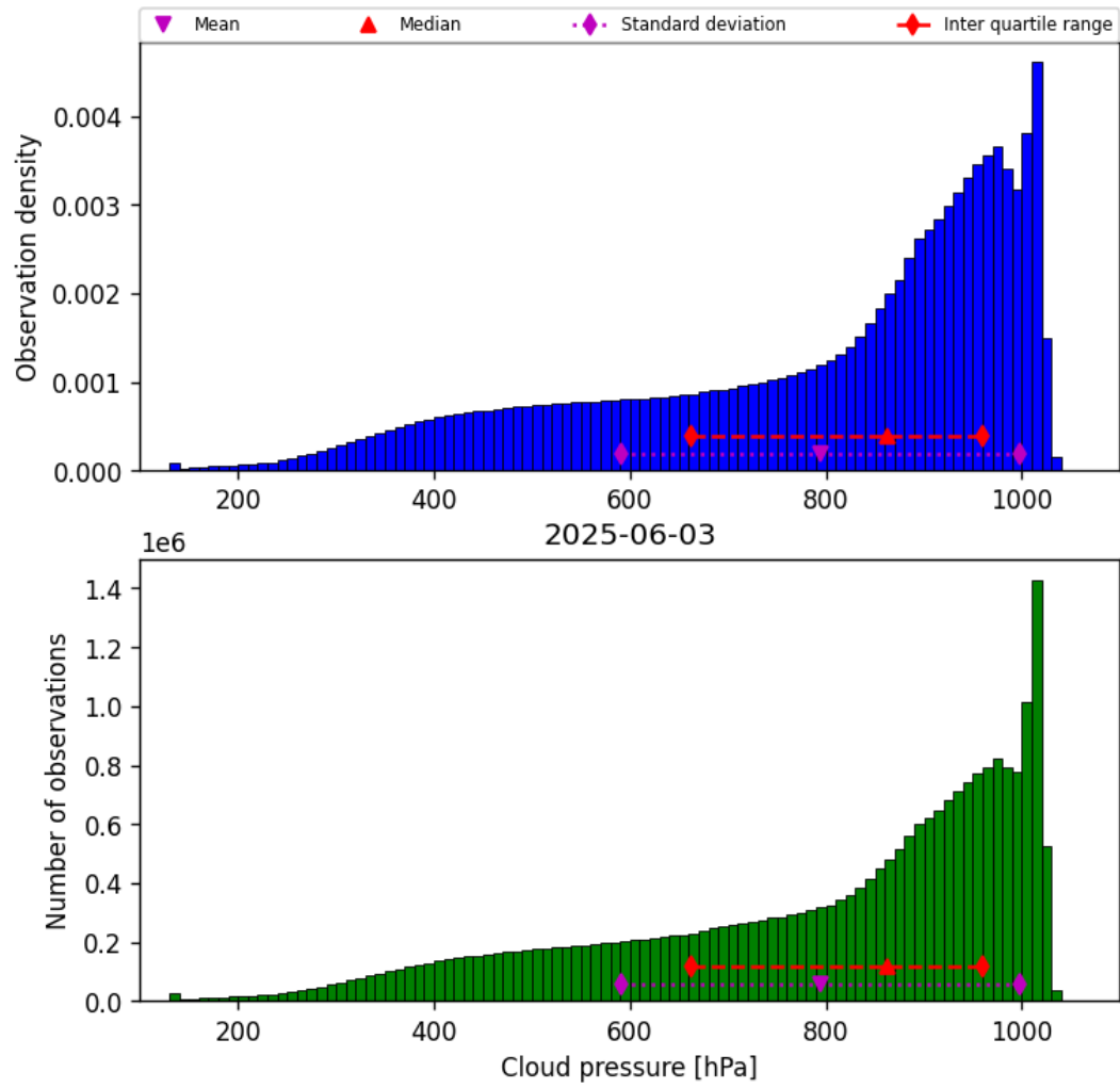
Figure 30: Histogram of “Cloud pressure” for 2025-06-02 to 2025-06-04
