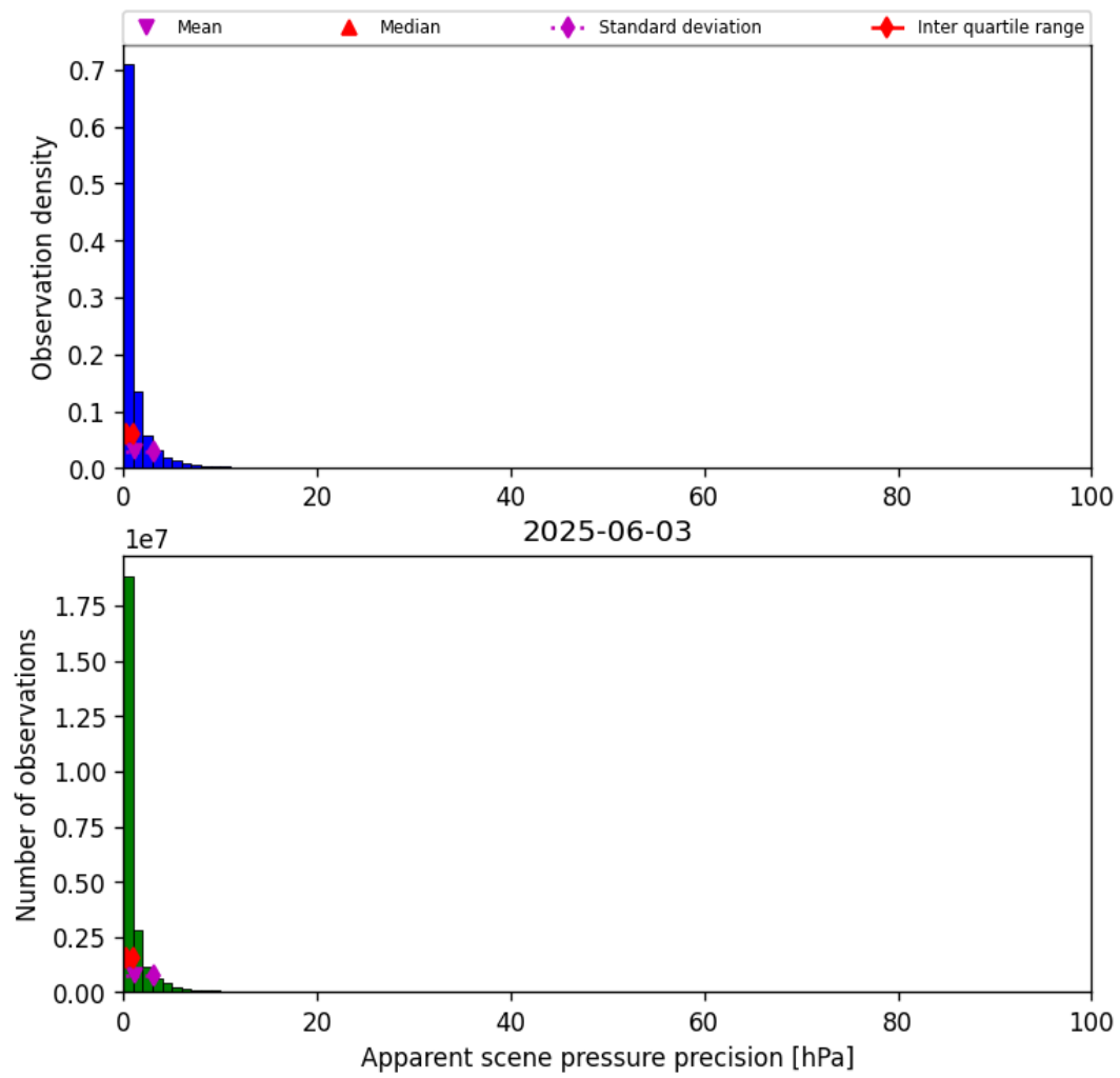
Figure 37: Histogram of “Apparent scene pressure precision” for 2025-06-02 to 2025-06-04
