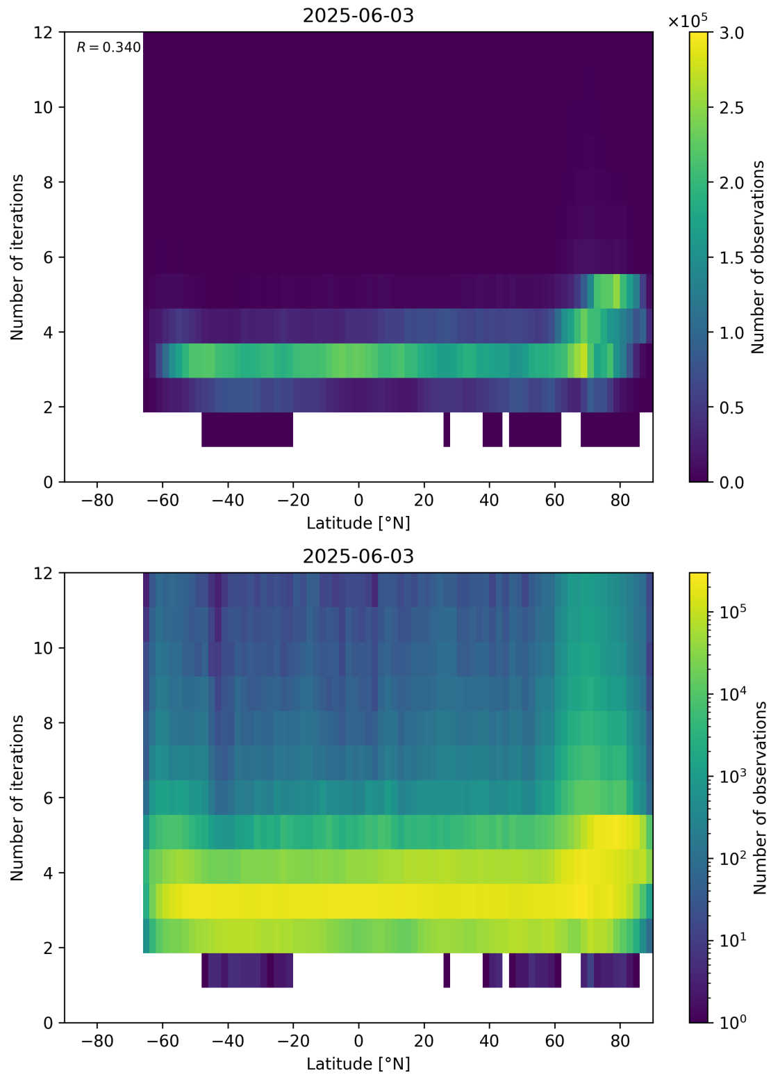
Figure 93: Scatter density plot of “Latitude” against “Number of iterations” for 2025-06-02 to 2025-06-04.
