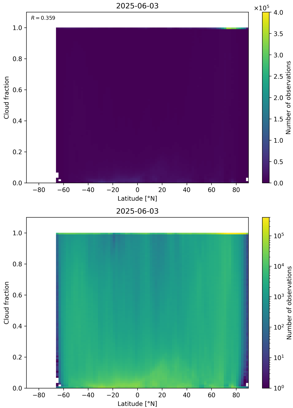
Figure 90: Scatter density plot of “Latitude” against “Cloud fraction” for 2025-06-02 to 2025-06-04.
