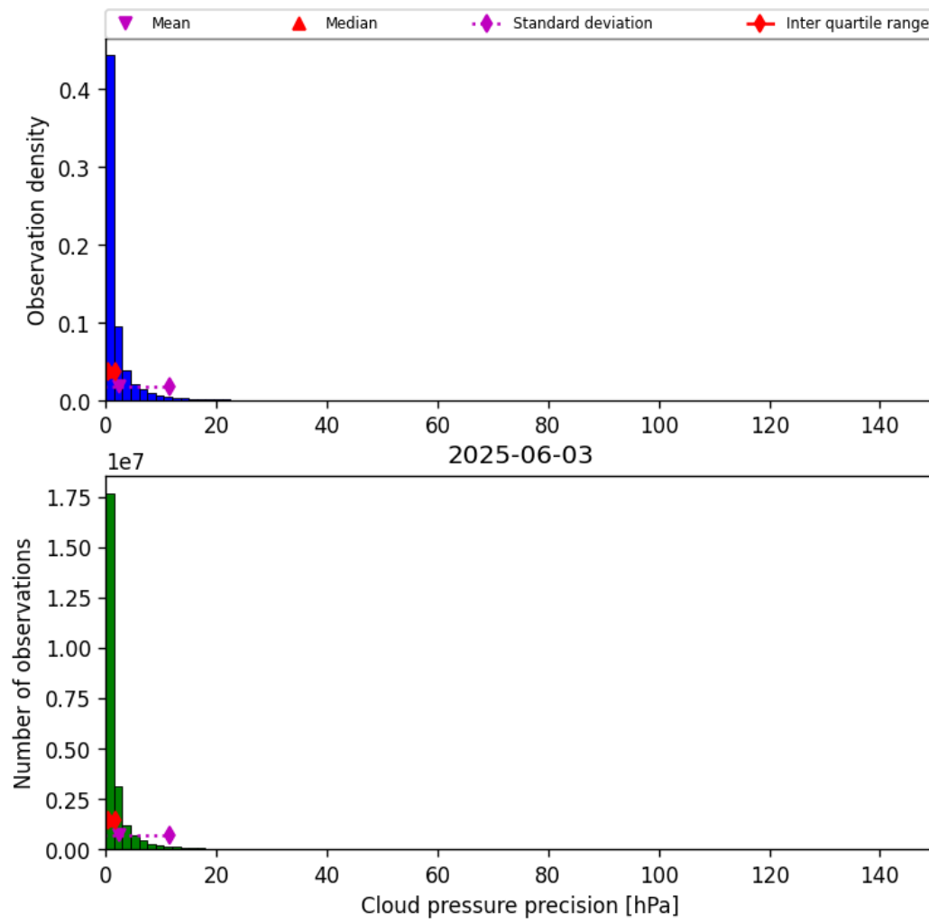
Figure 31: Histogram of “Cloud pressure precision” for 2025-06-02 to 2025-06-04
