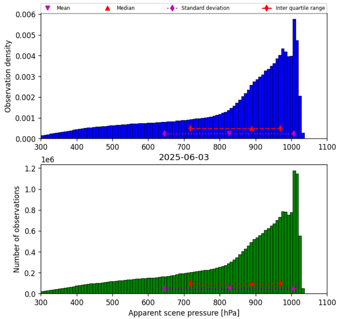
Figure 36: Histogram of “Apparent scene pressure” for 2025-06-02 to 2025-06-04
