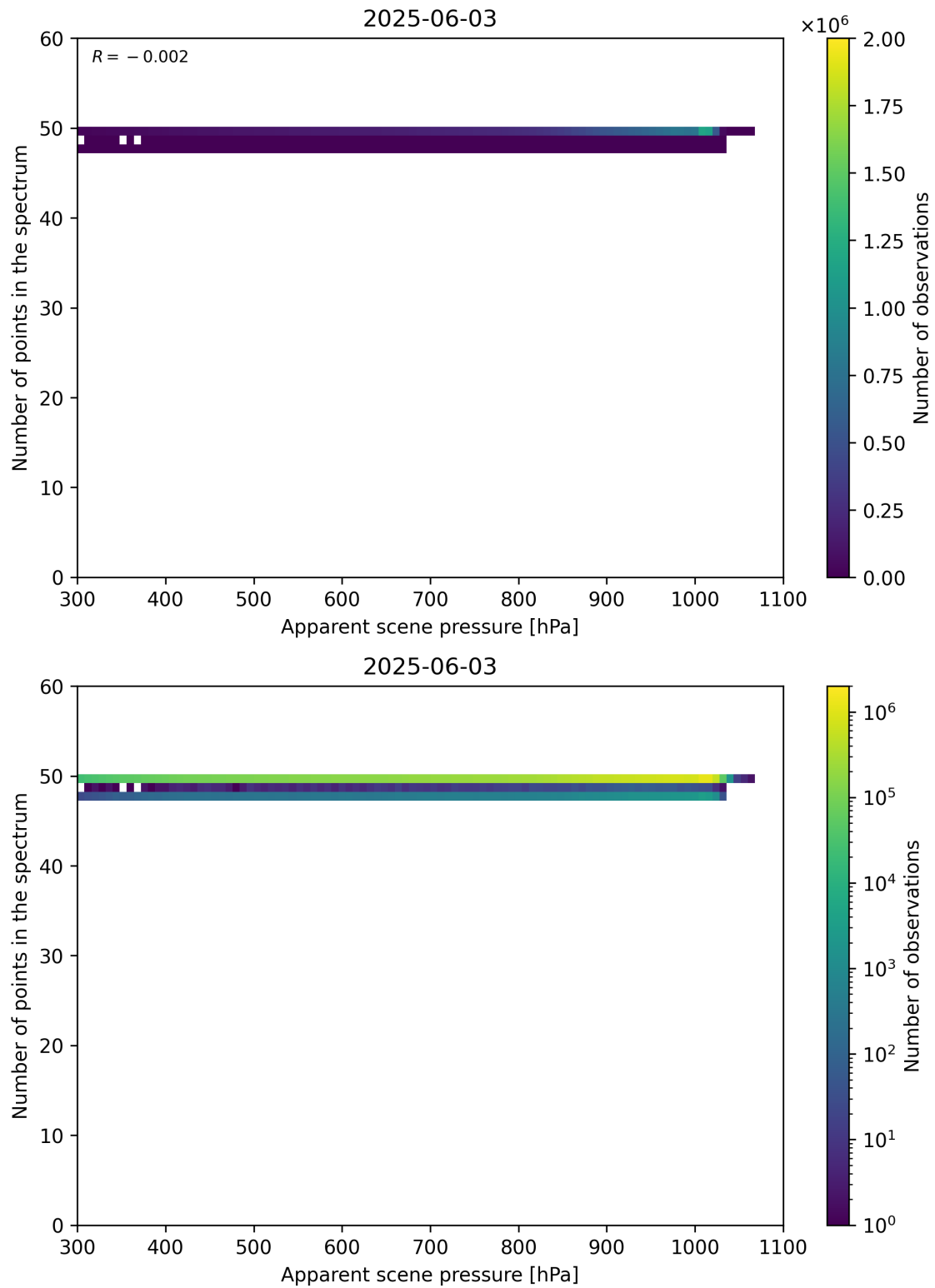
Figure 66: Scatter density plot of “Apparent scene pressure” against “Number of points in the spectrum” for 2025-06-02 to 2025-06-04.
