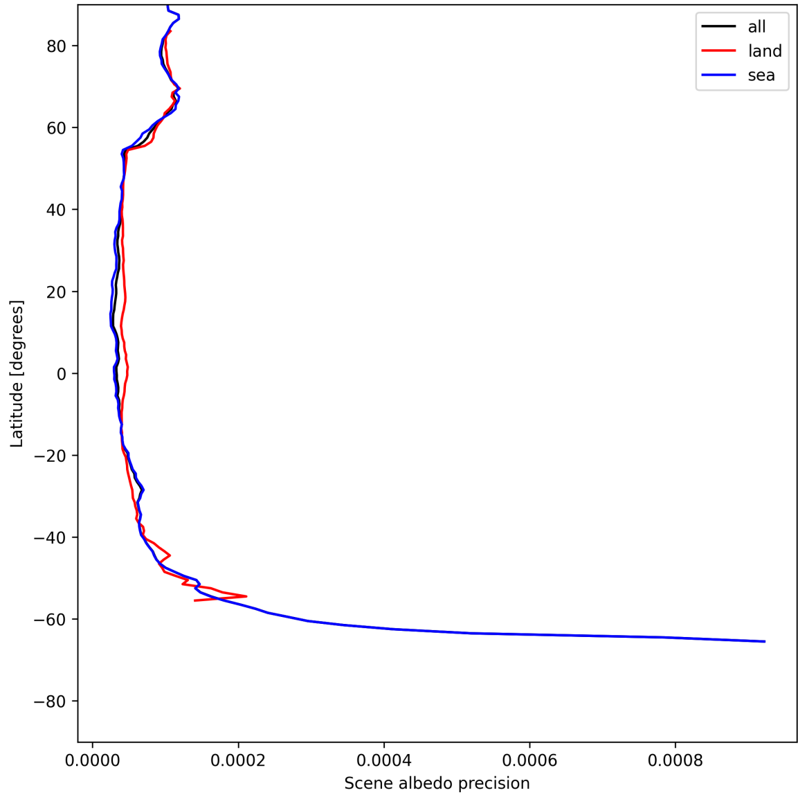
Figure 18: Zonal average of “Scene albedo precision” for 2025-06-02 to 2025-06-04.
