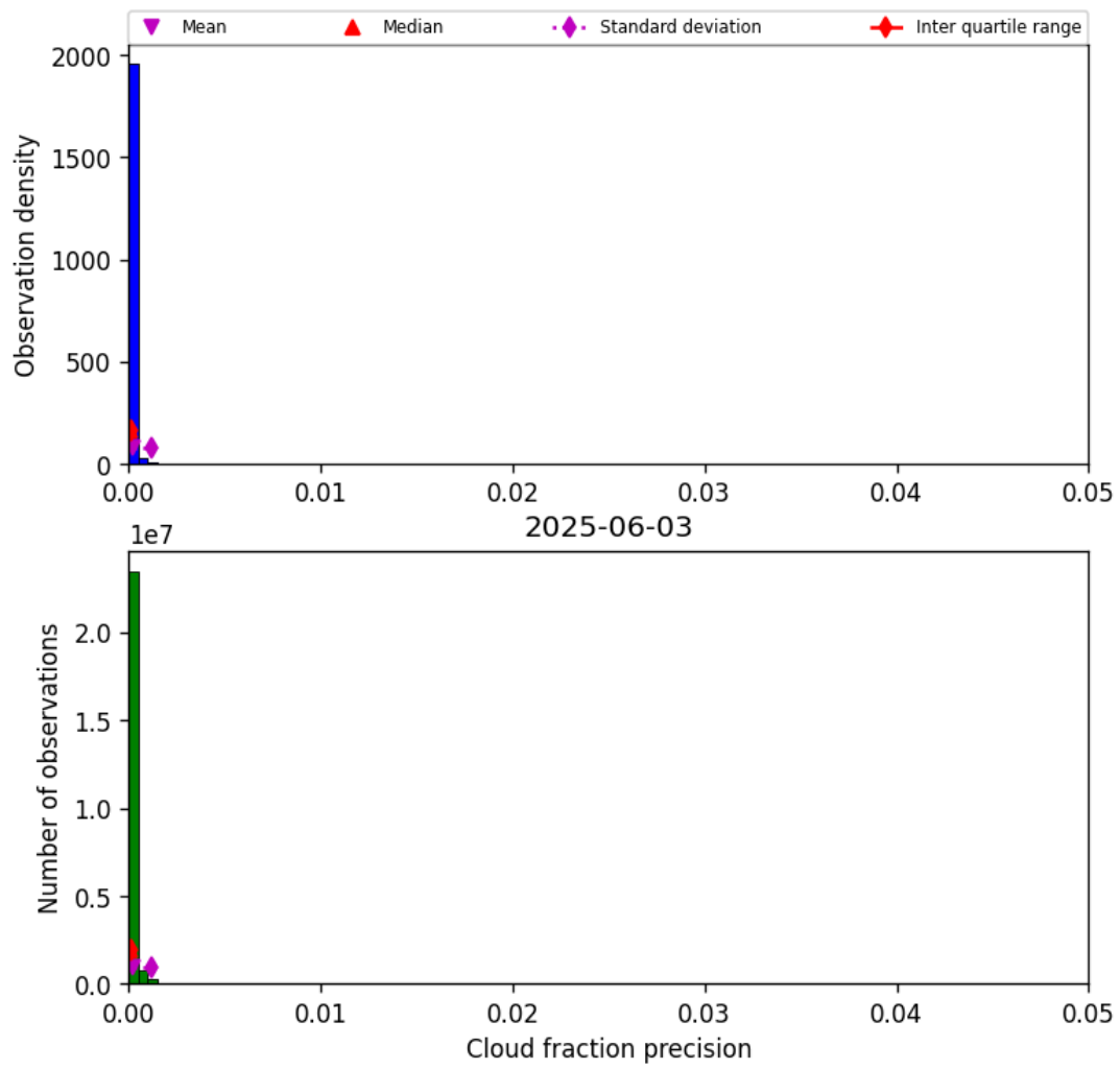
Figure 33: Histogram of “Cloud fraction precision” for 2025-06-02 to 2025-06-04
