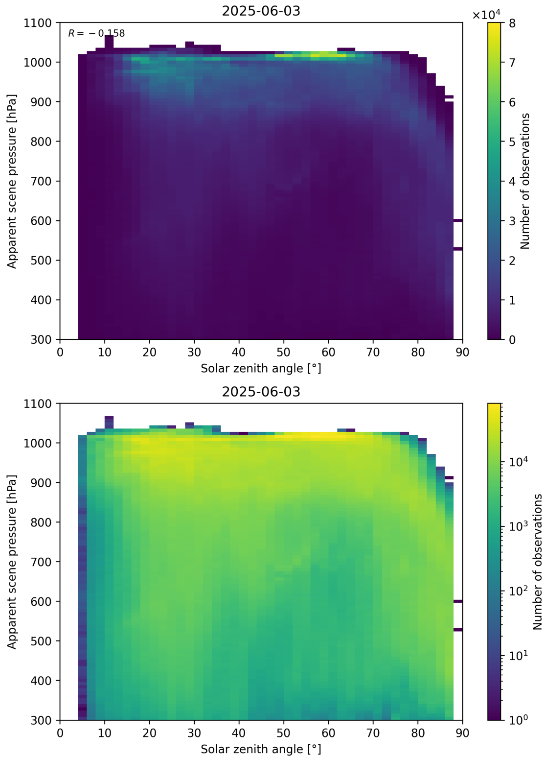
Figure 108: Scatter density plot of “Solar zenith angle” against “Apparent scene pressure” for 2025-06-02 to 2025-06-04.
