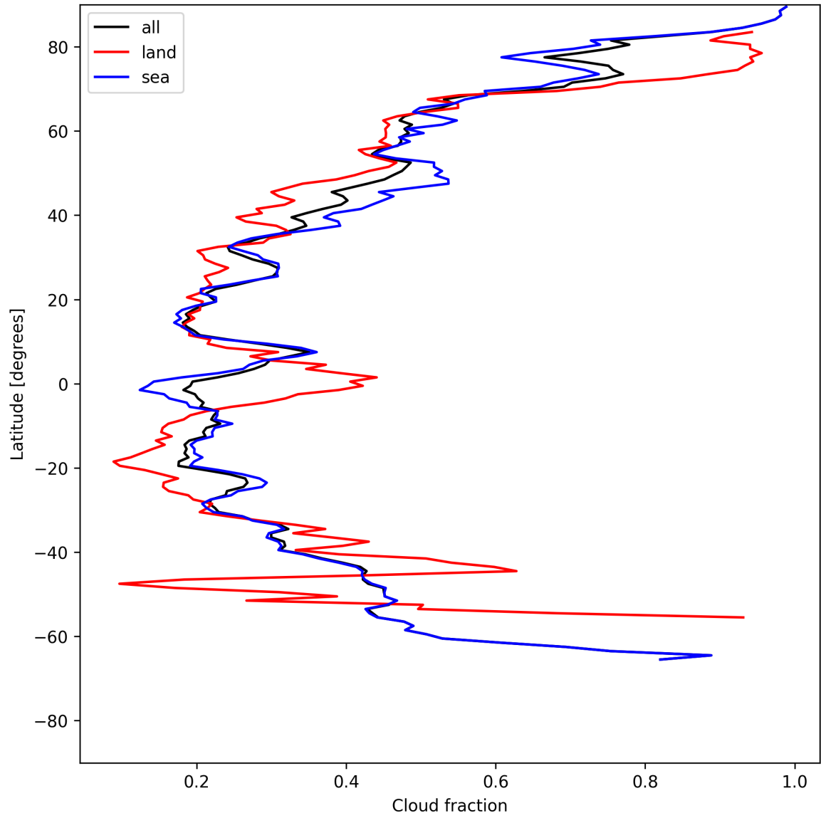
Figure 15: Zonal average of “Cloud fraction” for 2025-06-02 to 2025-06-04.
