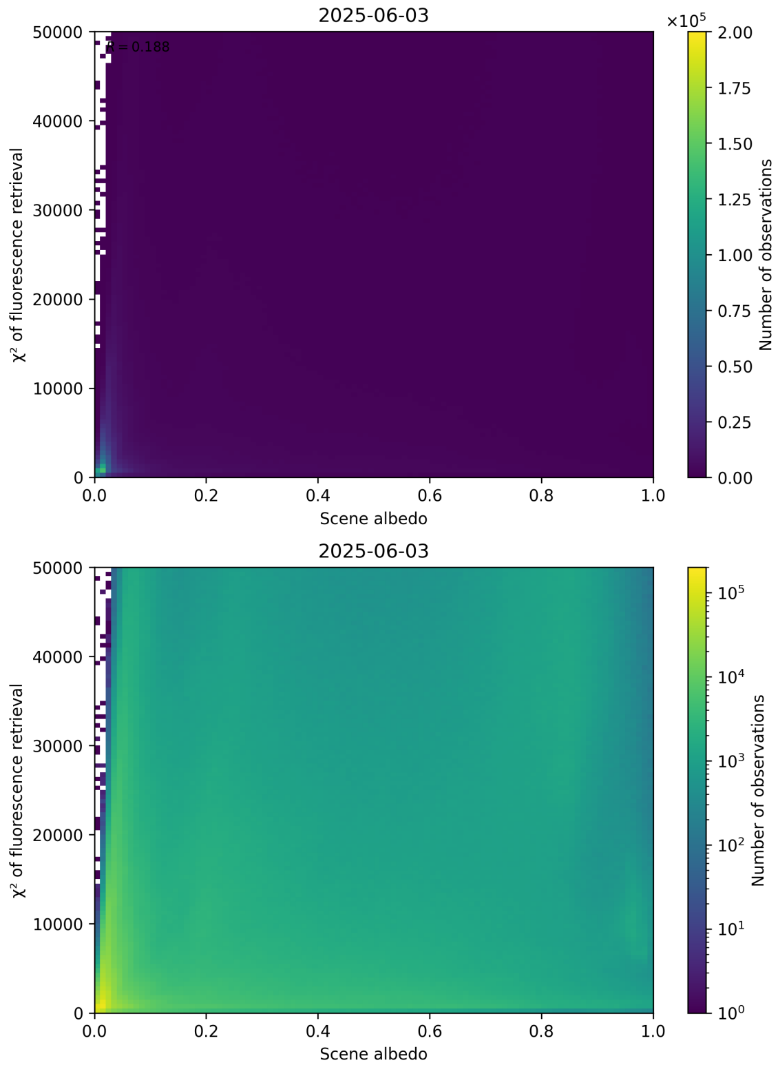
Figure 103: Scatter density plot of “Scene albedo” against “ \chi^2 of fluorescence retrieval” for 2025-06-02 to 2025-06-04.
