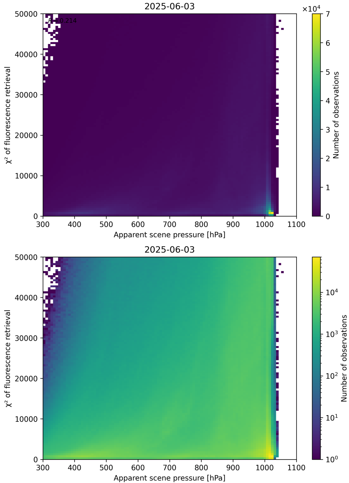
Figure 63: Scatter density plot of “Apparent scene pressure” against “ \chi^2 of fluorescence retrieval” for 2025-06-02 to 2025-06-04.
