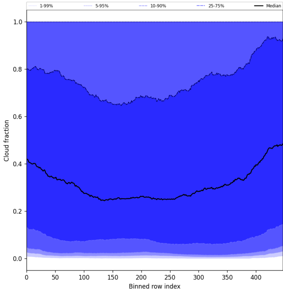
Figure 49: Along track statistics of “Cloud fraction” for 2025-06-02 to 2025-06-04
