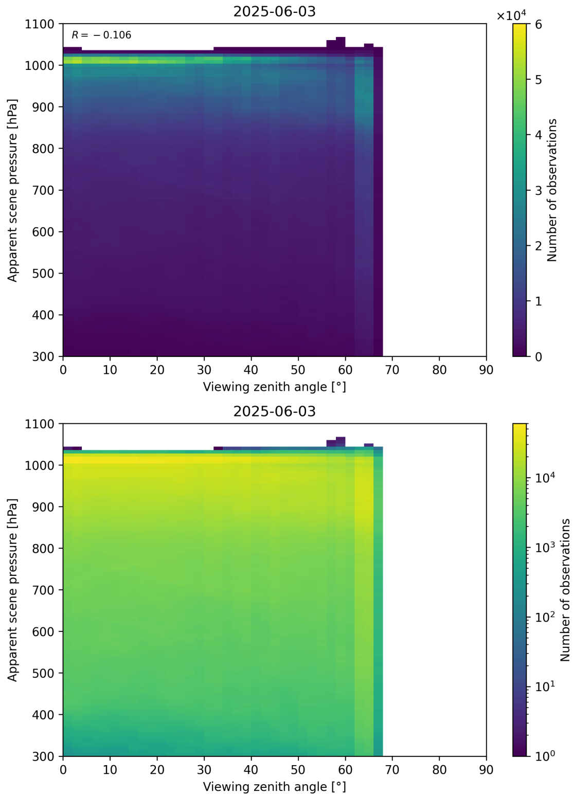
Figure 118: Scatter density plot of “Viewing zenith angle” against “Apparent scene pressure” for 2025-06-02 to 2025-06-04.
