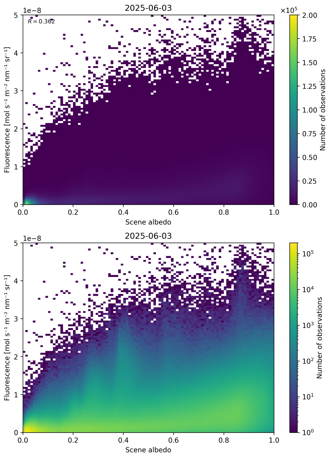
Figure 104: Scatter density plot of “Scene albedo” against “Fluorescence” for 2025-06-02 to 2025-06-04.
