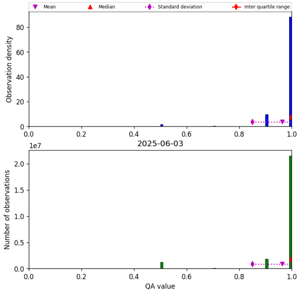
Figure 29: Histogram of “QA value” for 2025-06-02 to 2025-06-04
