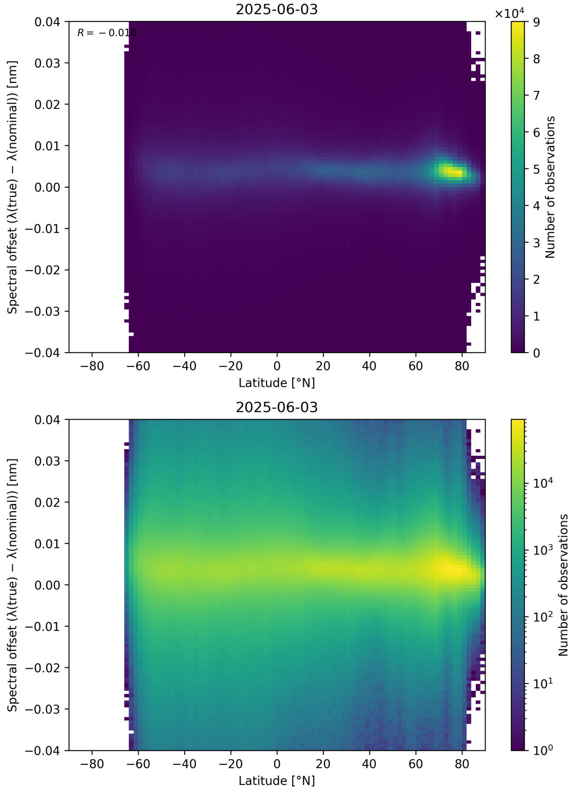
Figure 96: Scatter density plot of “Latitude” against “Spectral offset ( \lambda_{\text{true}} - \lambda_{\text{nominal}} )” for 2025-06-02 to 2025-06-04.
