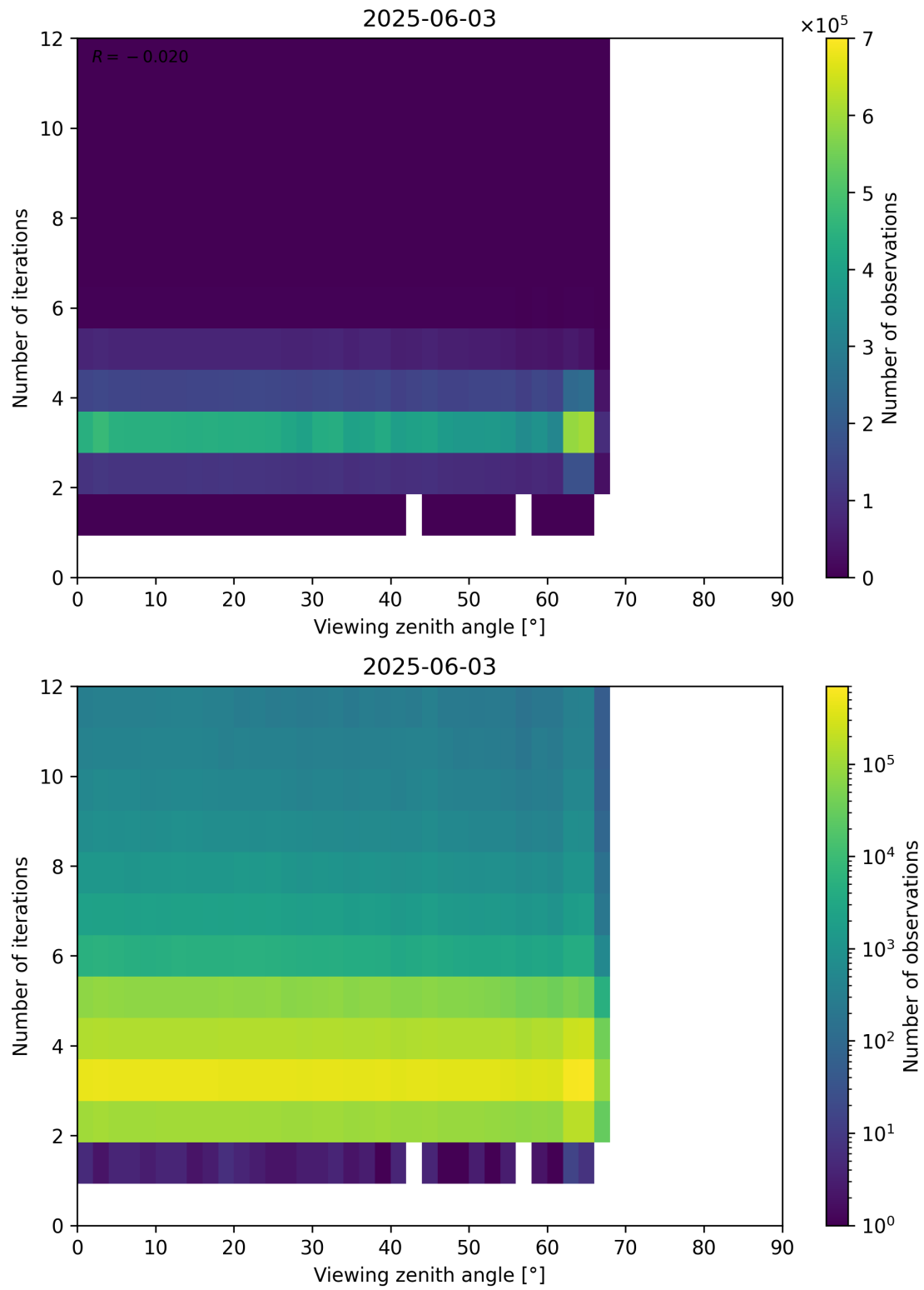
Figure 124: Scatter density plot of “Viewing zenith angle” against “Number of iterations” for 2025-06-02 to 2025-06-04.
