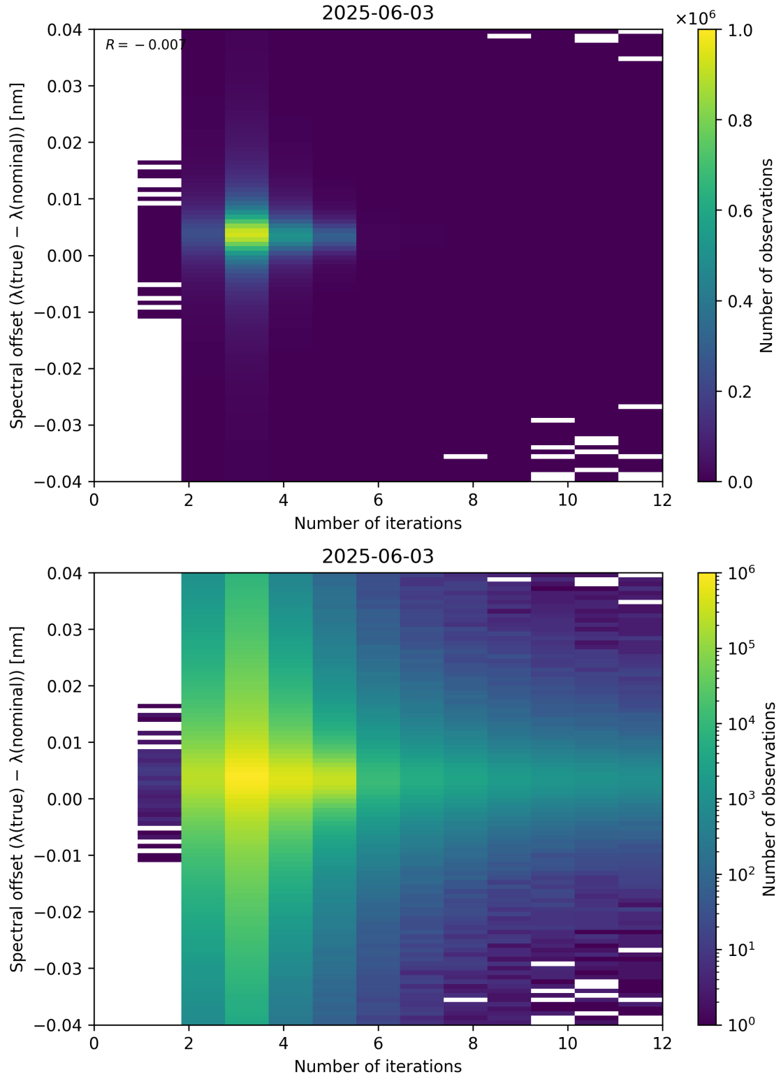
Figure 100: Scatter density plot of “Number of iterations” against “Spectral offset ( \lambda_{\text{true}} - \lambda_{\text{nominal}} )” for 2025-06-02 to 2025-06-04.
