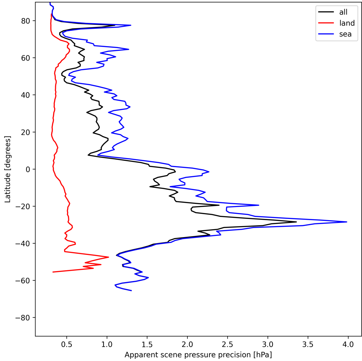
Figure 20: Zonal average of “Apparent scene pressure precision” for 2025-06-02 to 2025-06-04.
