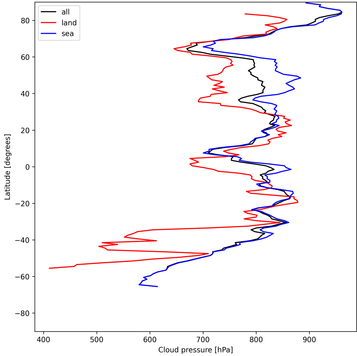
Figure 13: Zonal average of “Cloud pressure” for 2025-06-02 to 2025-06-04.
