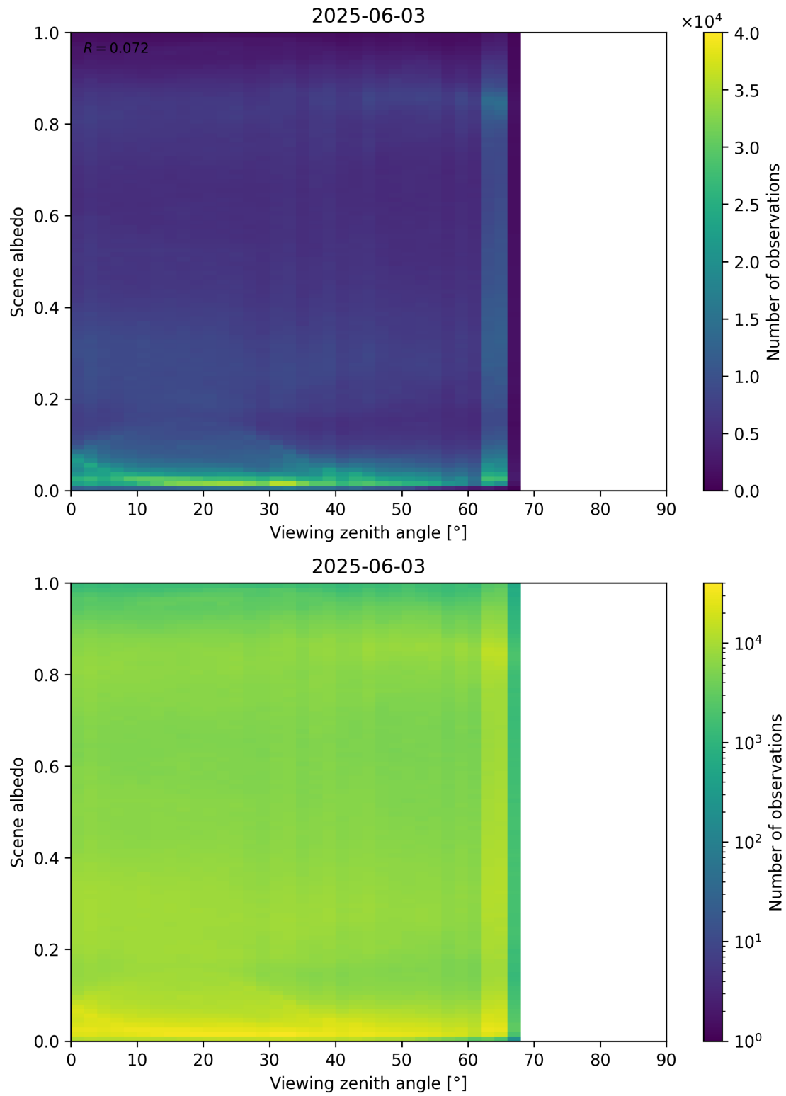
Figure 126: Scatter density plot of “Viewing zenith angle” against “Scene albedo” for 2025-06-02 to 2025-06-04.
