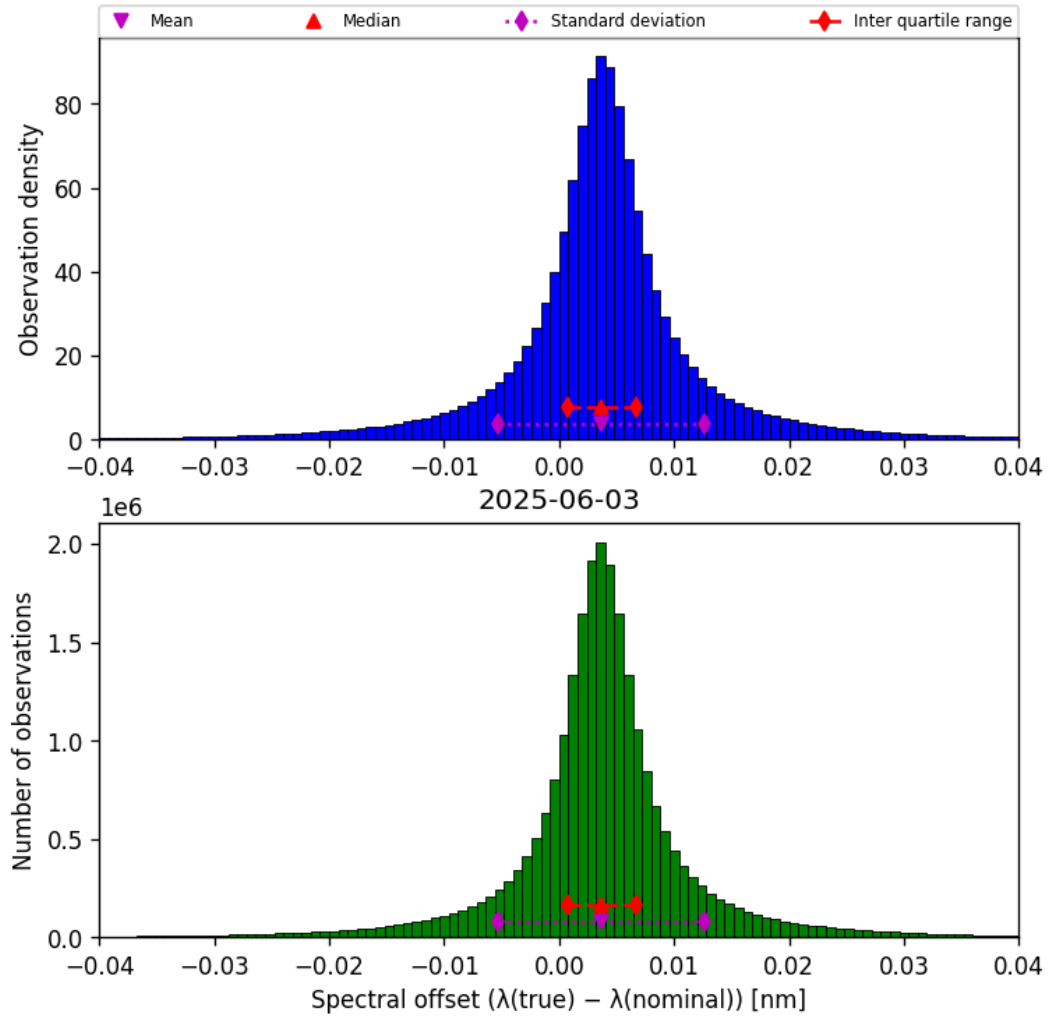
Figure 45: Histogram of “Spectral offset ( \lambda_{\text{true}} - \lambda_{\text{nominal}} )” for 2025-06-02 to 2025-06-04
