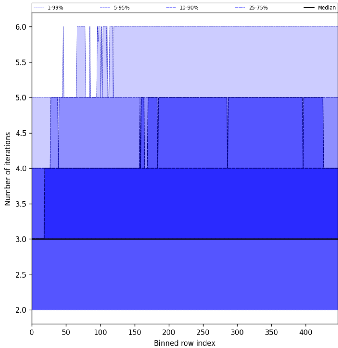
Figure 56: Along track statistics of “Number of iterations” for 2025-06-02 to 2025-06-04
