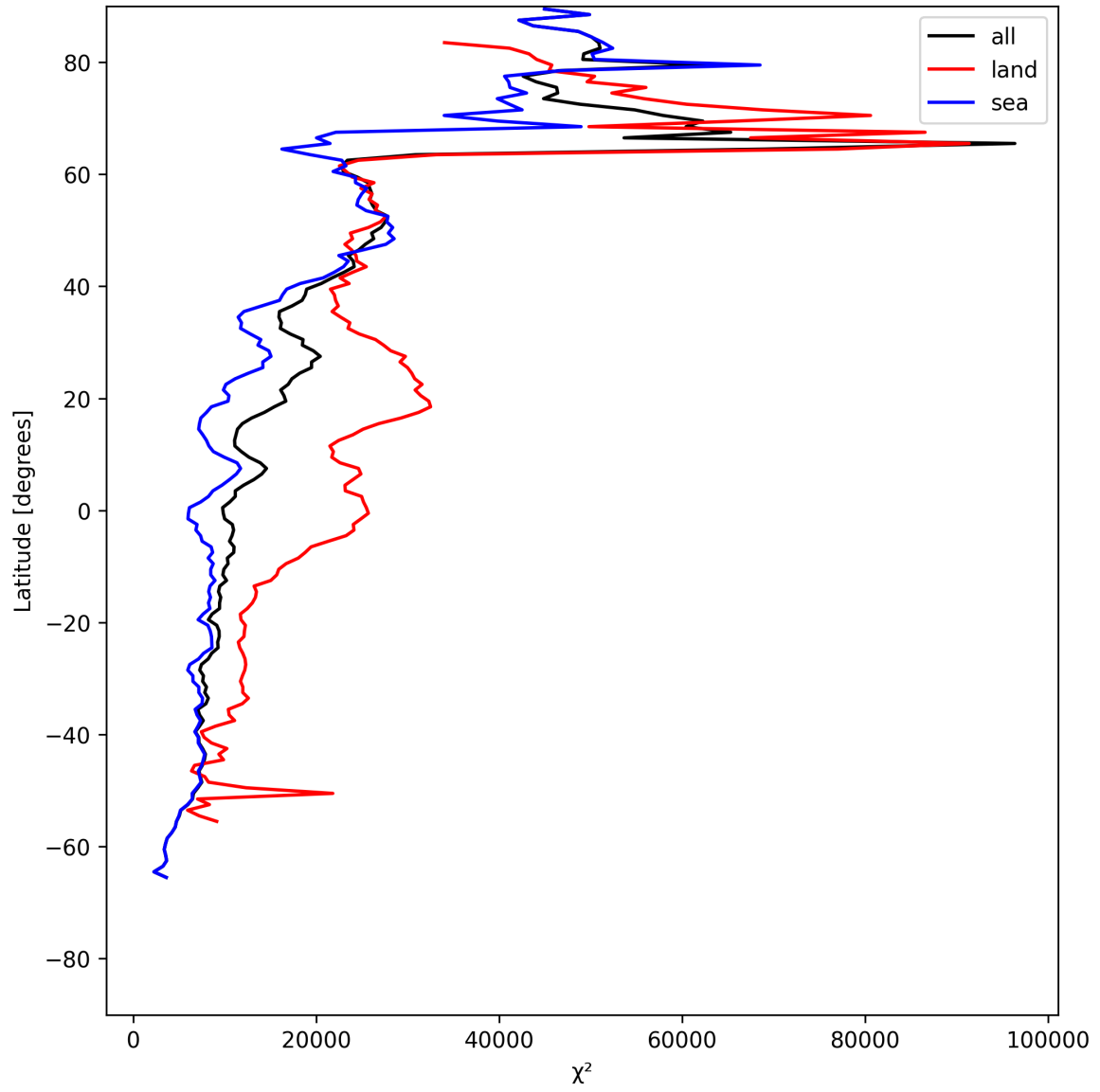
Figure 21: Zonal average of “ \chi^2 ” for 2025-06-02 to 2025-06-04.
