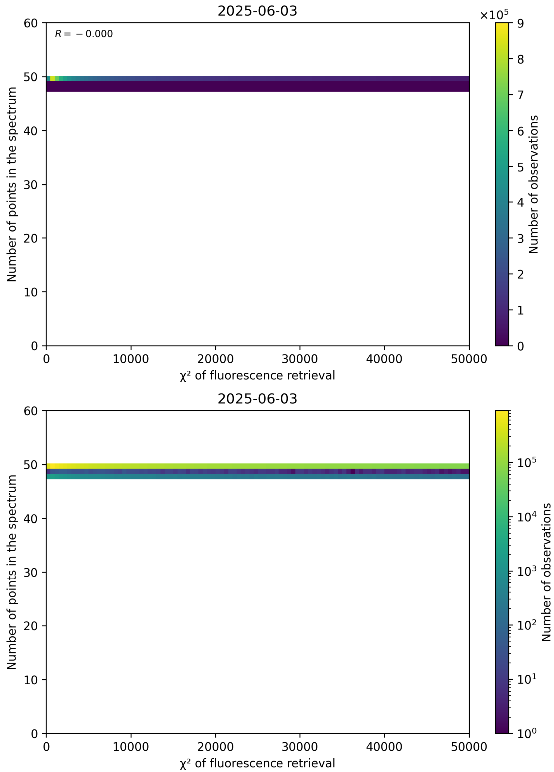
Figure 68: Scatter density plot of “ \chi^2 of fluorescence retrieval” against “Number of points in the spectrum” for 2025-06-02 to 2025-06-04.
