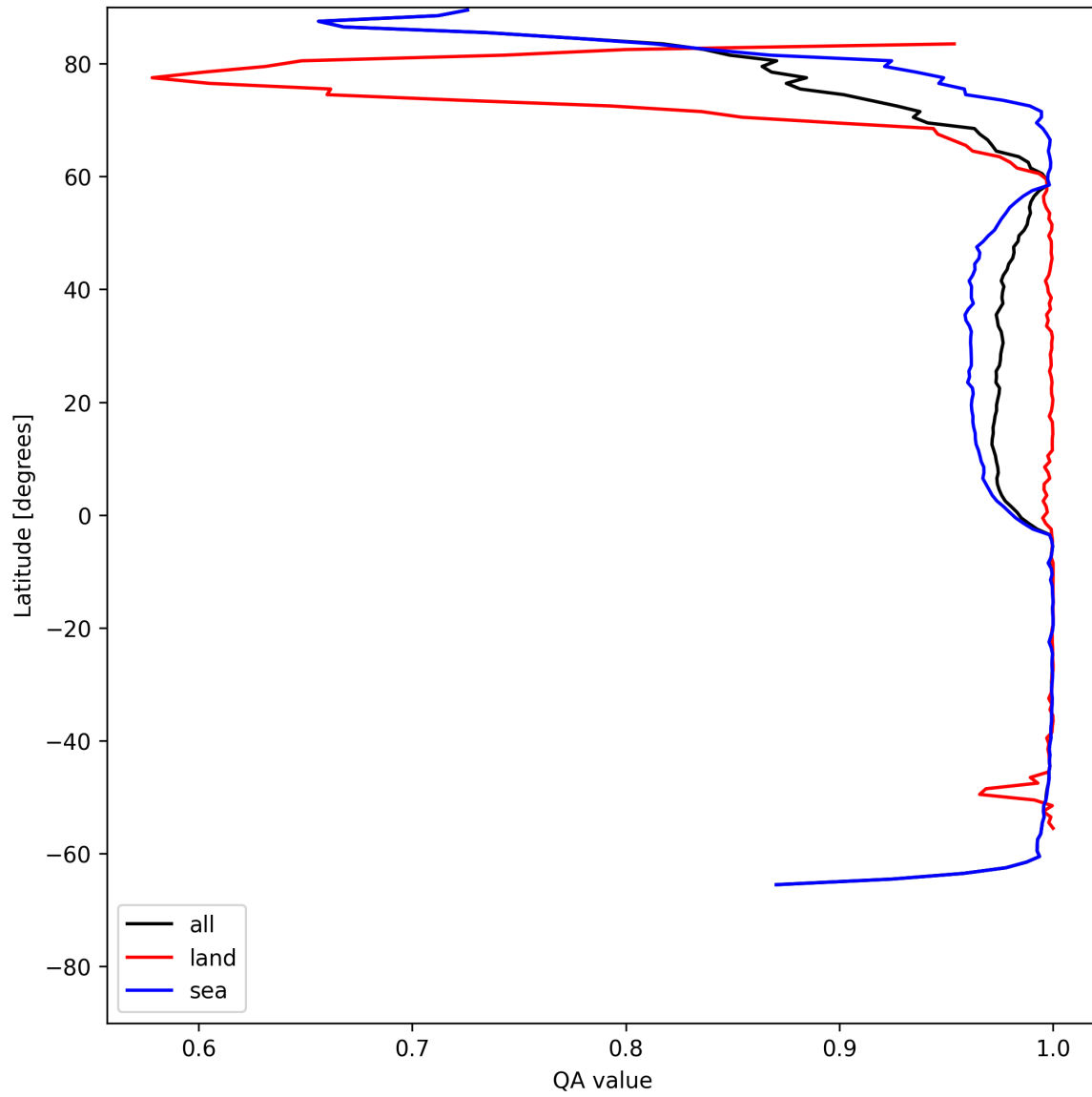
Figure 12: Zonal average of “QA value” for 2025-06-02 to 2025-06-04.
