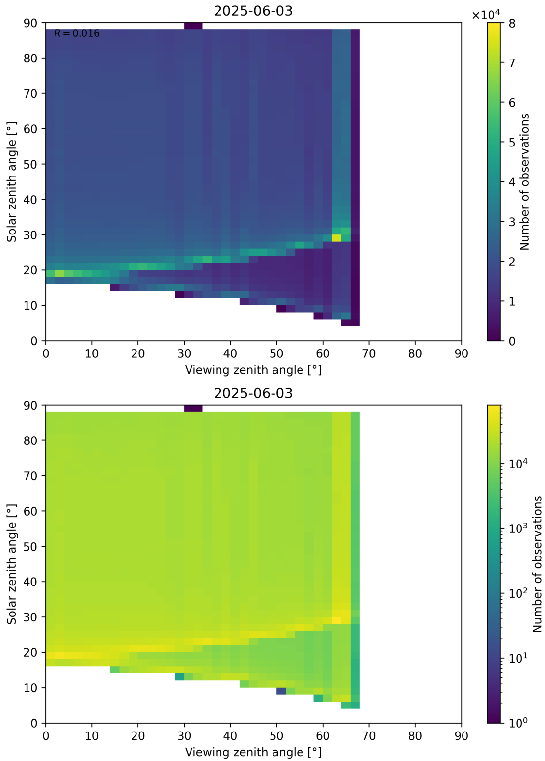
Figure 127: Scatter density plot of “Viewing zenith angle” against “Solar zenith angle” for 2025-06-02 to 2025-06-04.
