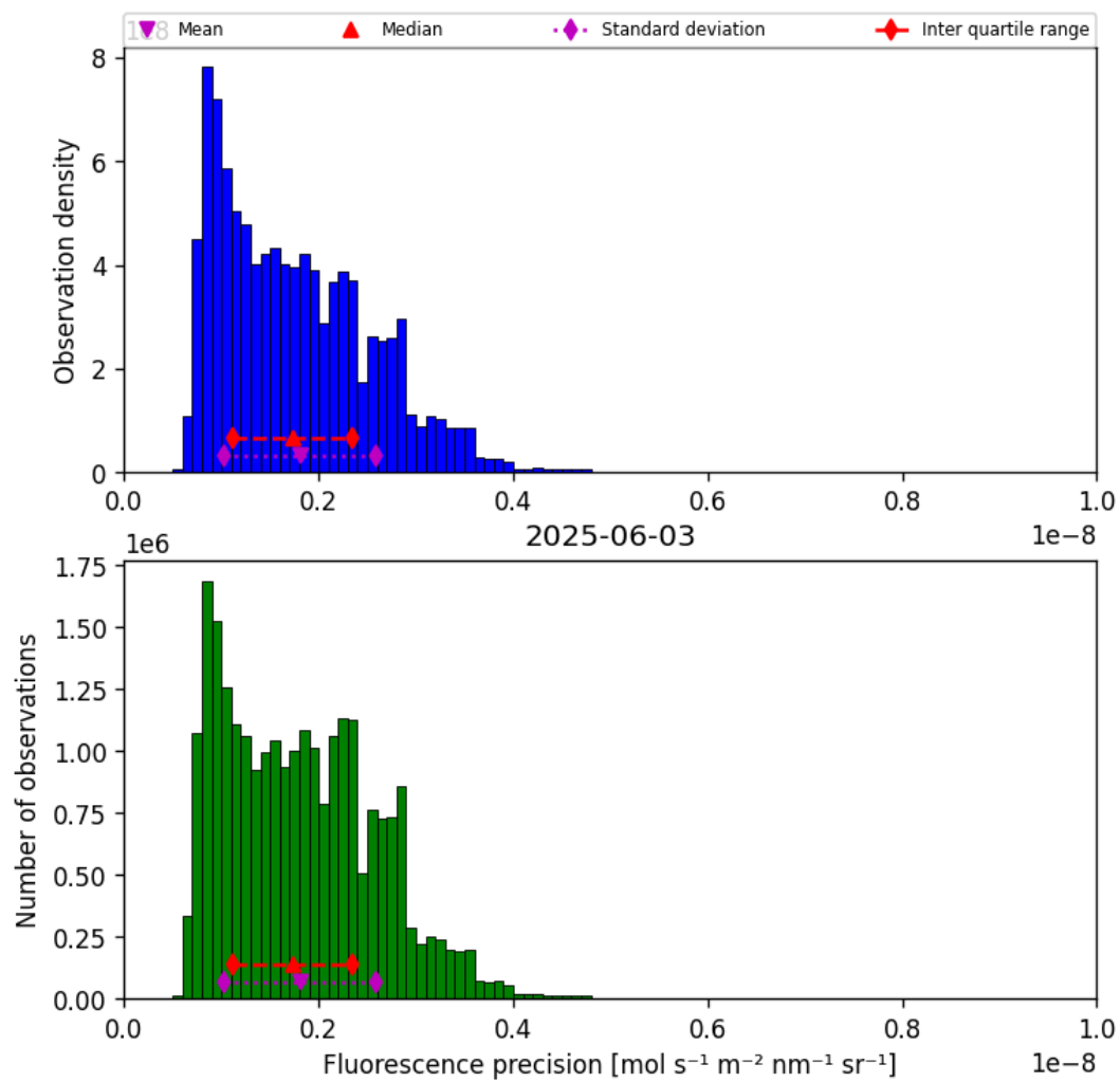
Figure 41: Histogram of “Fluorescence precision” for 2025-06-02 to 2025-06-04
