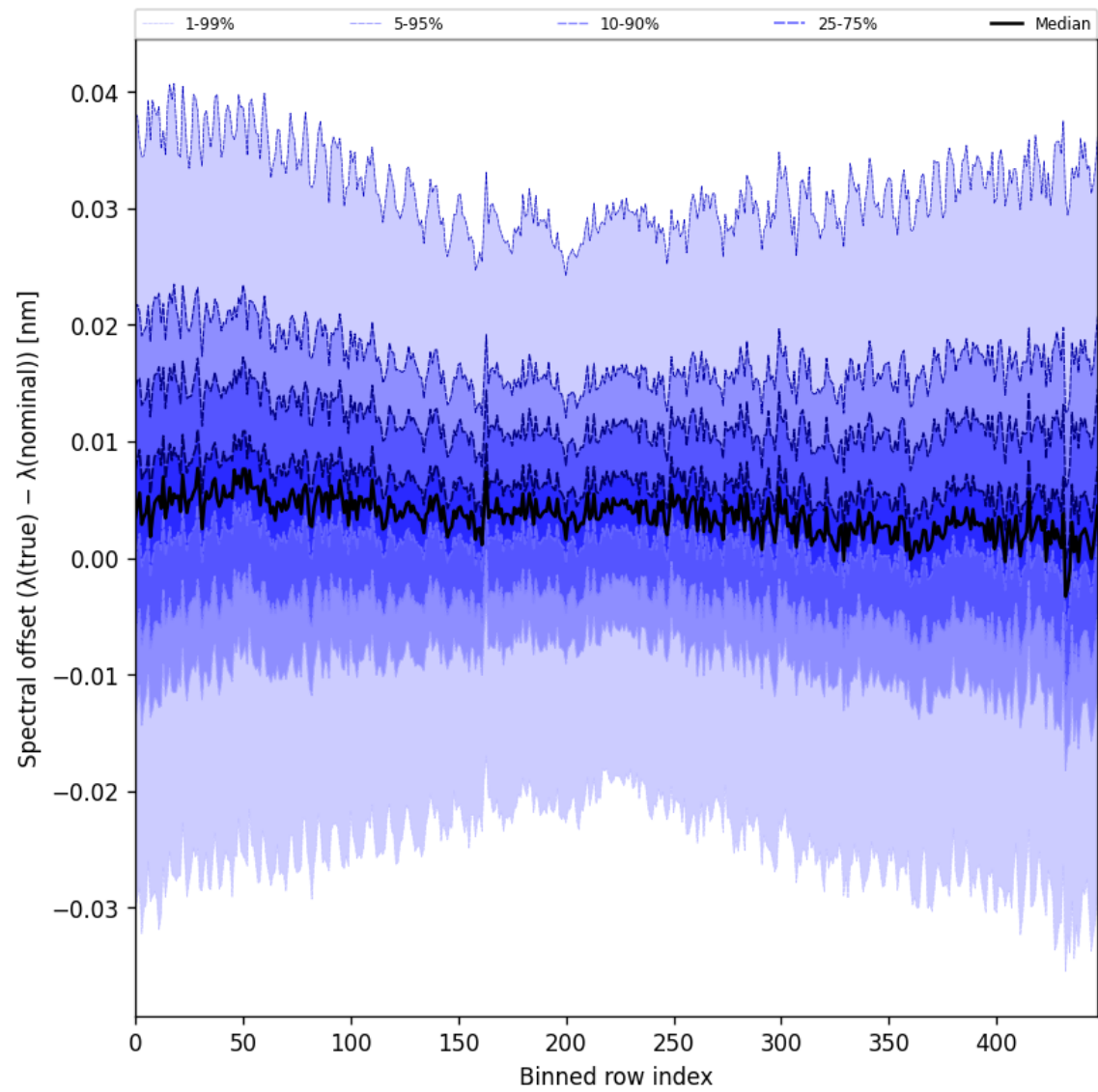
Figure 62: Along track statistics of “Spectral offset ( \lambda_{\text{true}} - \lambda_{\text{nominal}} )” for 2025-06-02 to 2025-06-04
