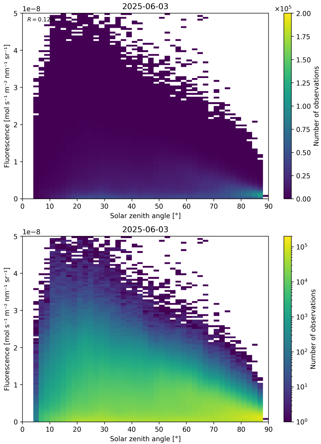
Figure 112: Scatter density plot of “Solar zenith angle” against “Fluorescence” for 2025-06-02 to 2025-06-04.
