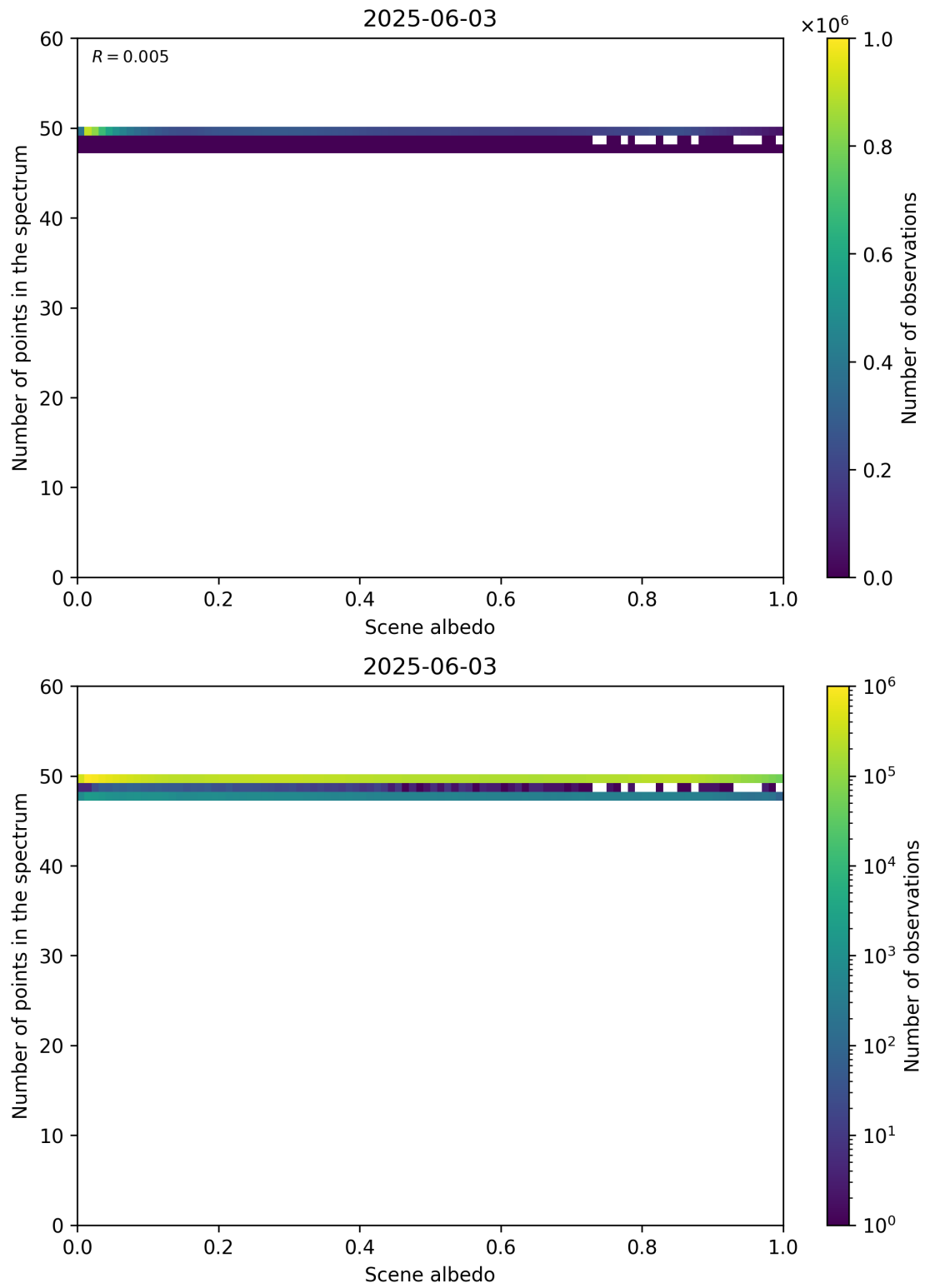
Figure 106: Scatter density plot of “Scene albedo” against “Number of points in the spectrum” for 2025-06-02 to 2025-06-04.
