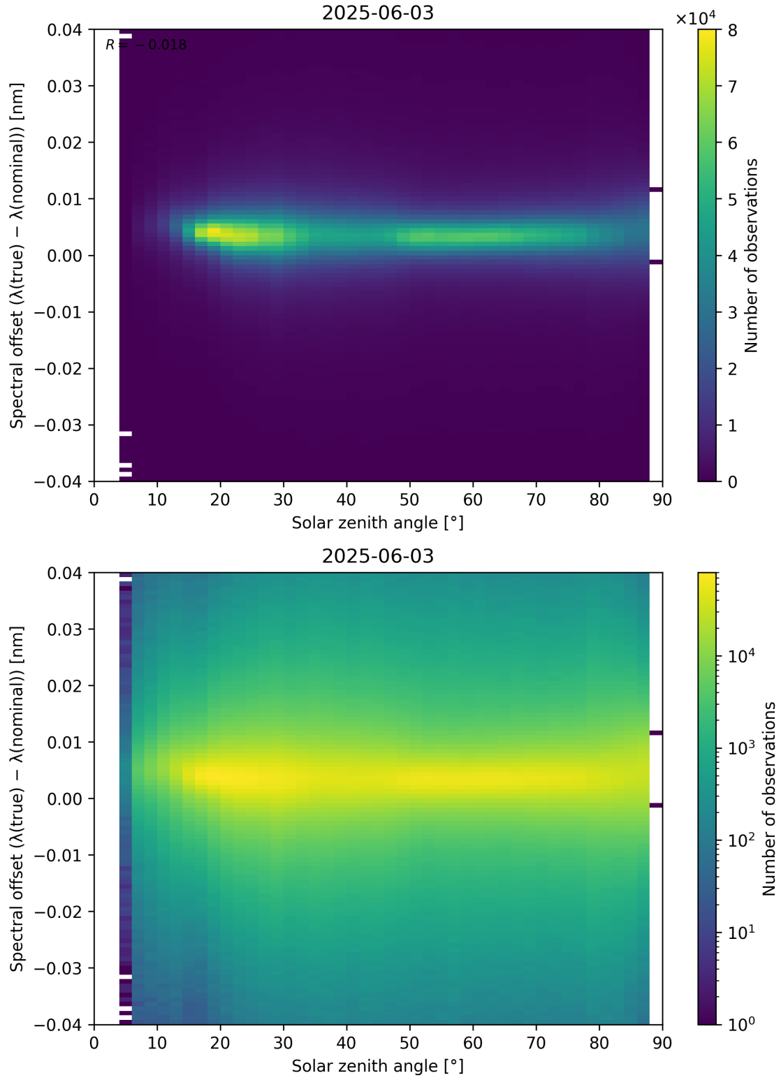
Figure 117: Scatter density plot of “Solar zenith angle” against “Spectral offset ( \lambda_{\text{true}} - \lambda_{\text{nominal}} )” for 2025-06-02 to 2025-06-04.
