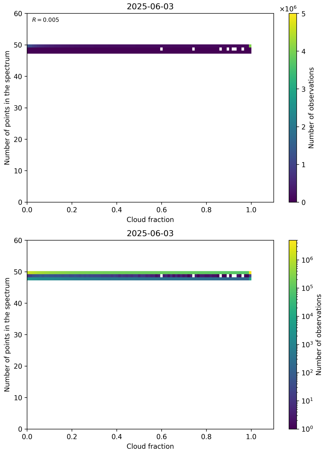
Figure 74: Scatter density plot of “Cloud fraction” against “Number of points in the spectrum” for 2025-06-02 to 2025-06-04.
