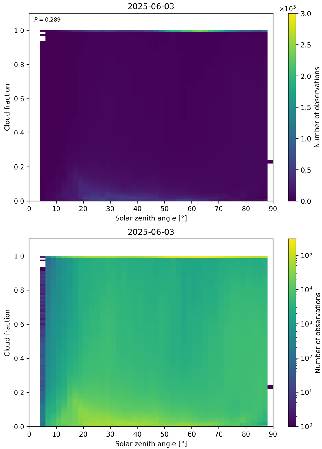
Figure 110: Scatter density plot of “Solar zenith angle” against “Cloud fraction” for 2025-06-02 to 2025-06-04.
