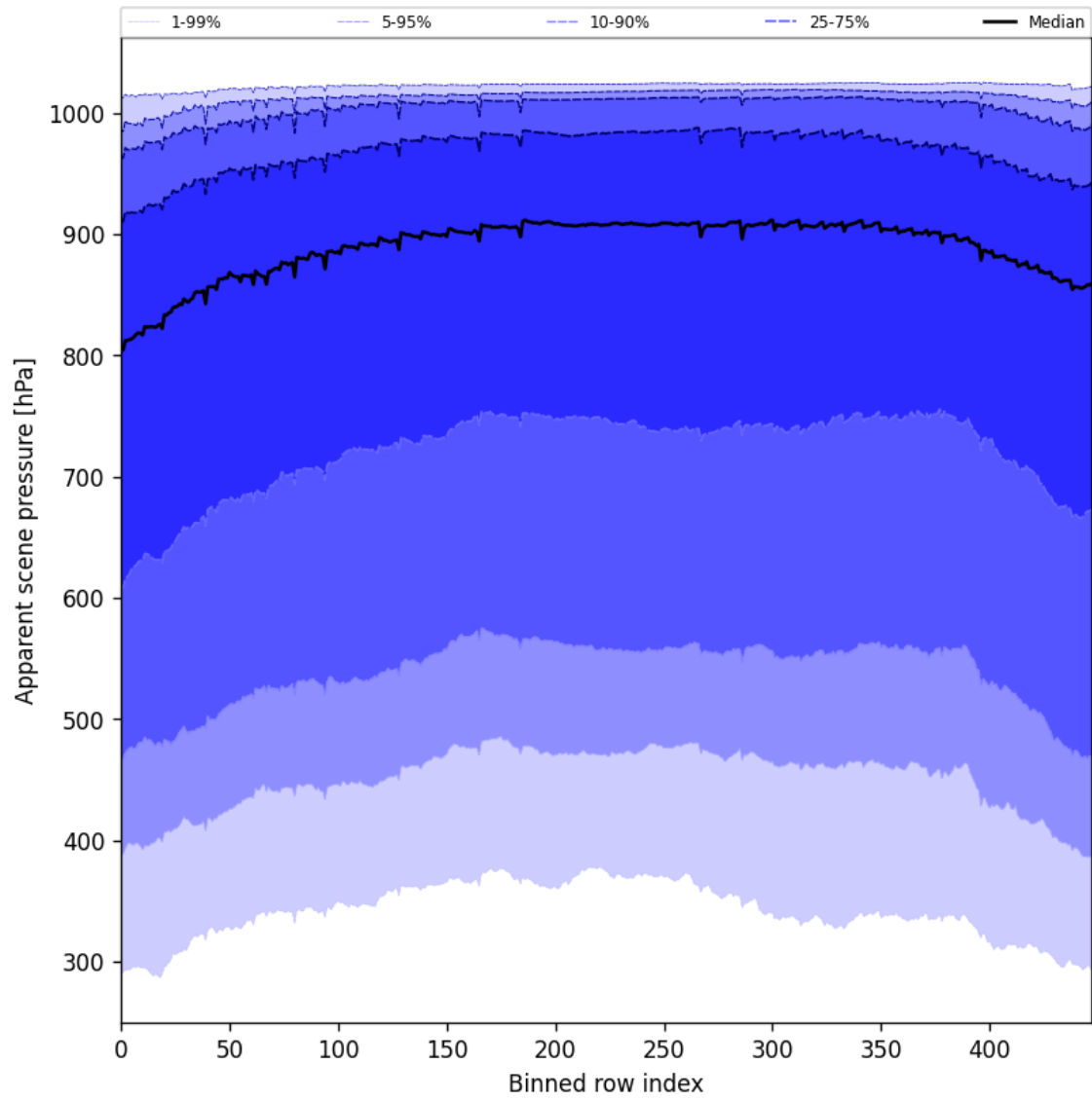
Figure 53: Along track statistics of “Apparent scene pressure” for 2025-06-02 to 2025-06-04
