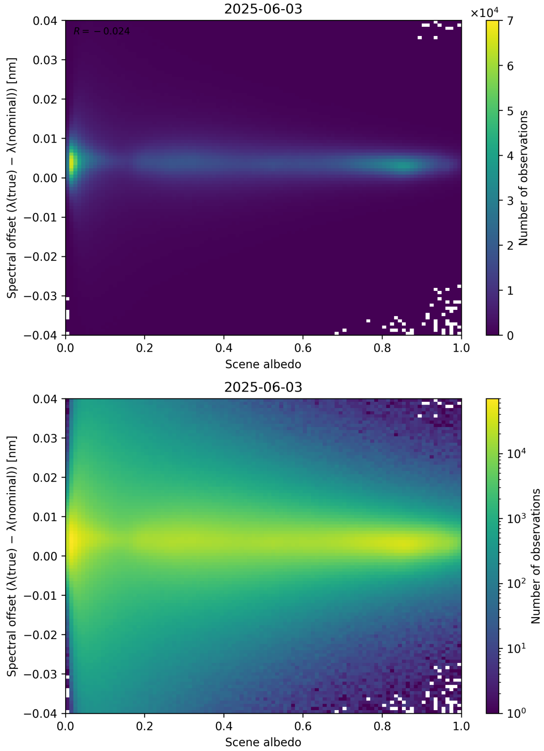
Figure 107: Scatter density plot of “Scene albedo” against “Spectral offset ( \lambda_{\text{true}} - \lambda_{\text{nominal}} )” for 2025-06-02 to 2025-06-04.
