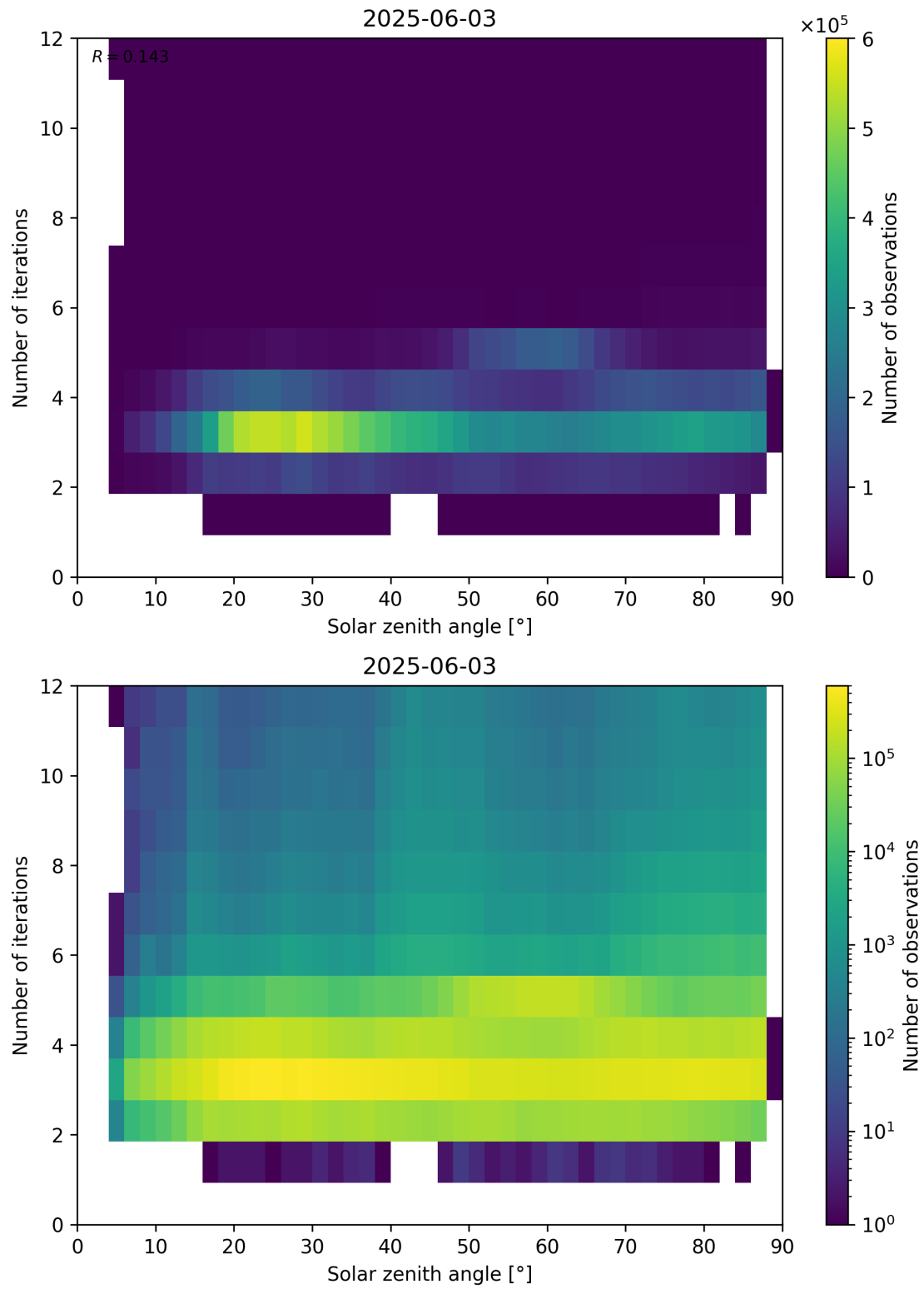
Figure 114: Scatter density plot of “Solar zenith angle” against “Number of iterations” for 2025-06-02 to 2025-06-04.
