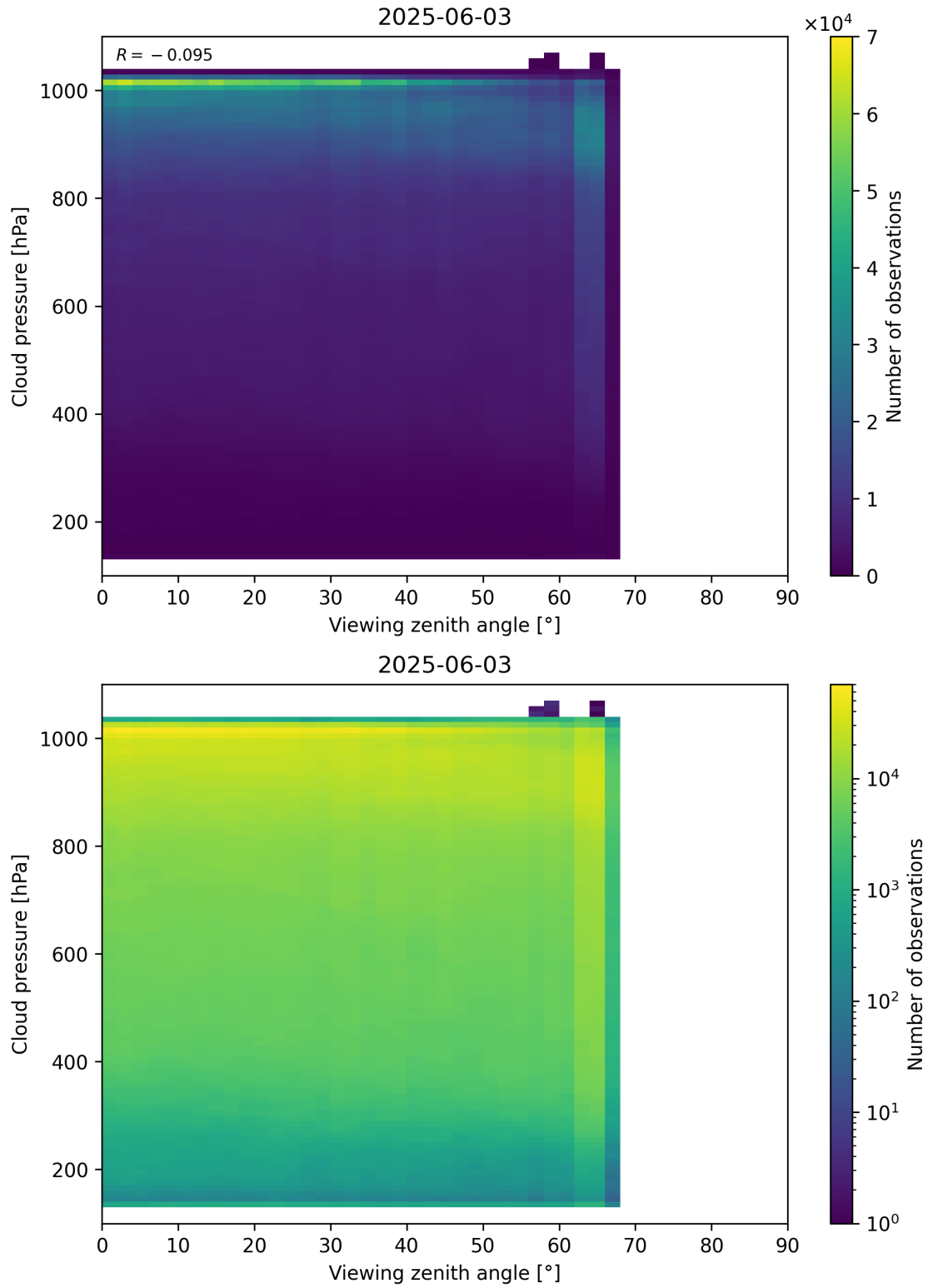
Figure 121: Scatter density plot of “Viewing zenith angle” against “Cloud pressure” for 2025-06-02 to 2025-06-04.
