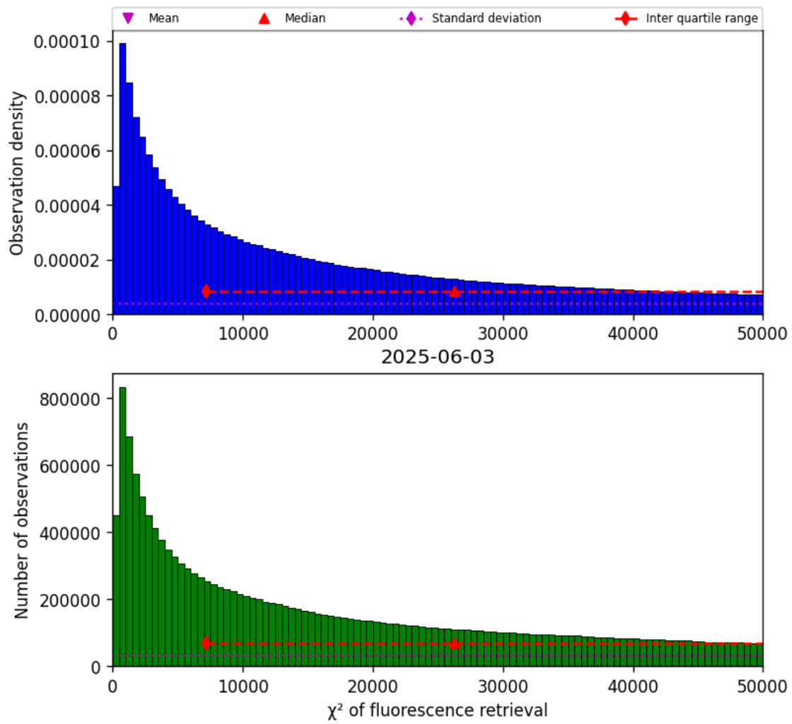
Figure 42: Histogram of “ \chi^2 of fluorescence retrieval” for 2025-06-02 to 2025-06-04
