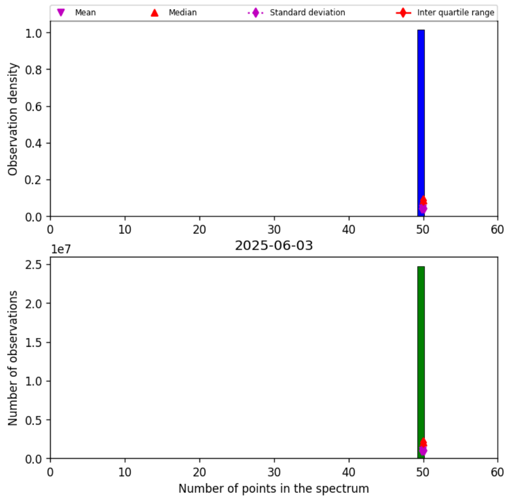
Figure 44: Histogram of “Number of points in the spectrum” for 2025-06-02 to 2025-06-04
