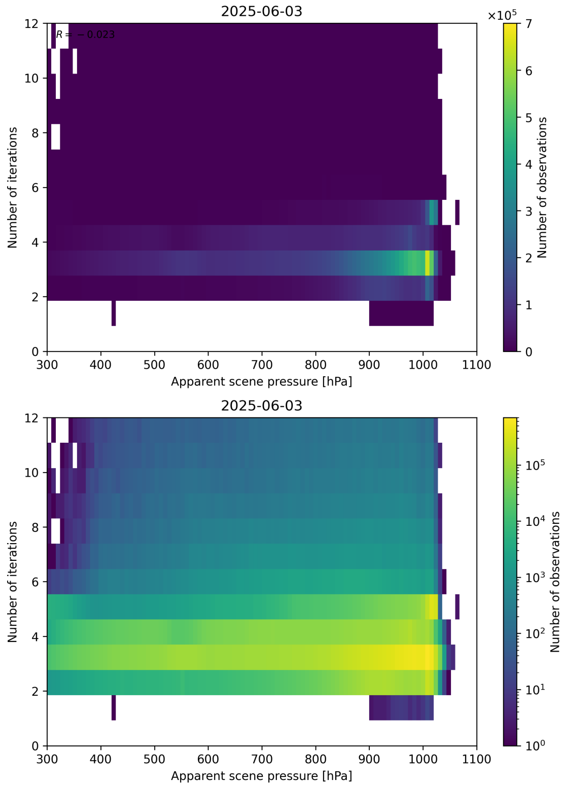
Figure 65: Scatter density plot of “Apparent scene pressure” against “Number of iterations” for 2025-06-02 to 2025-06-04.
