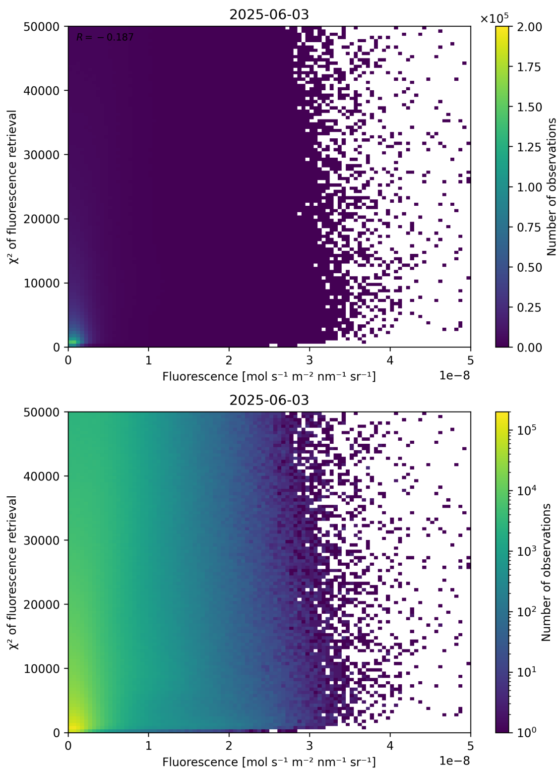
Figure 85: Scatter density plot of “Fluorescence” against “ \chi^2 of fluorescence retrieval” for 2025-06-02 to 2025-06-04.
