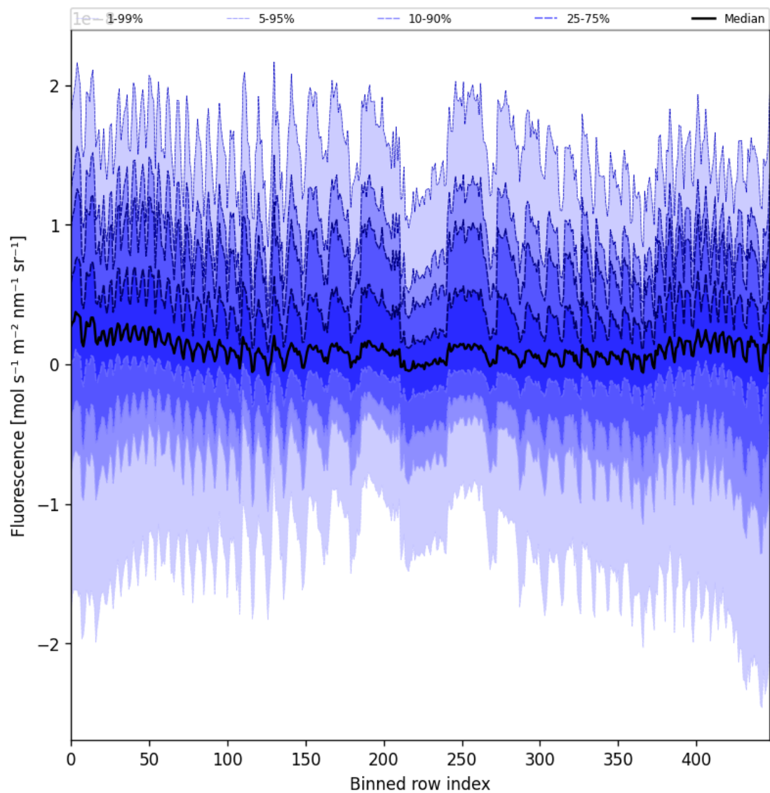
Figure 57: Along track statistics of “Fluorescence” for 2025-06-02 to 2025-06-04
