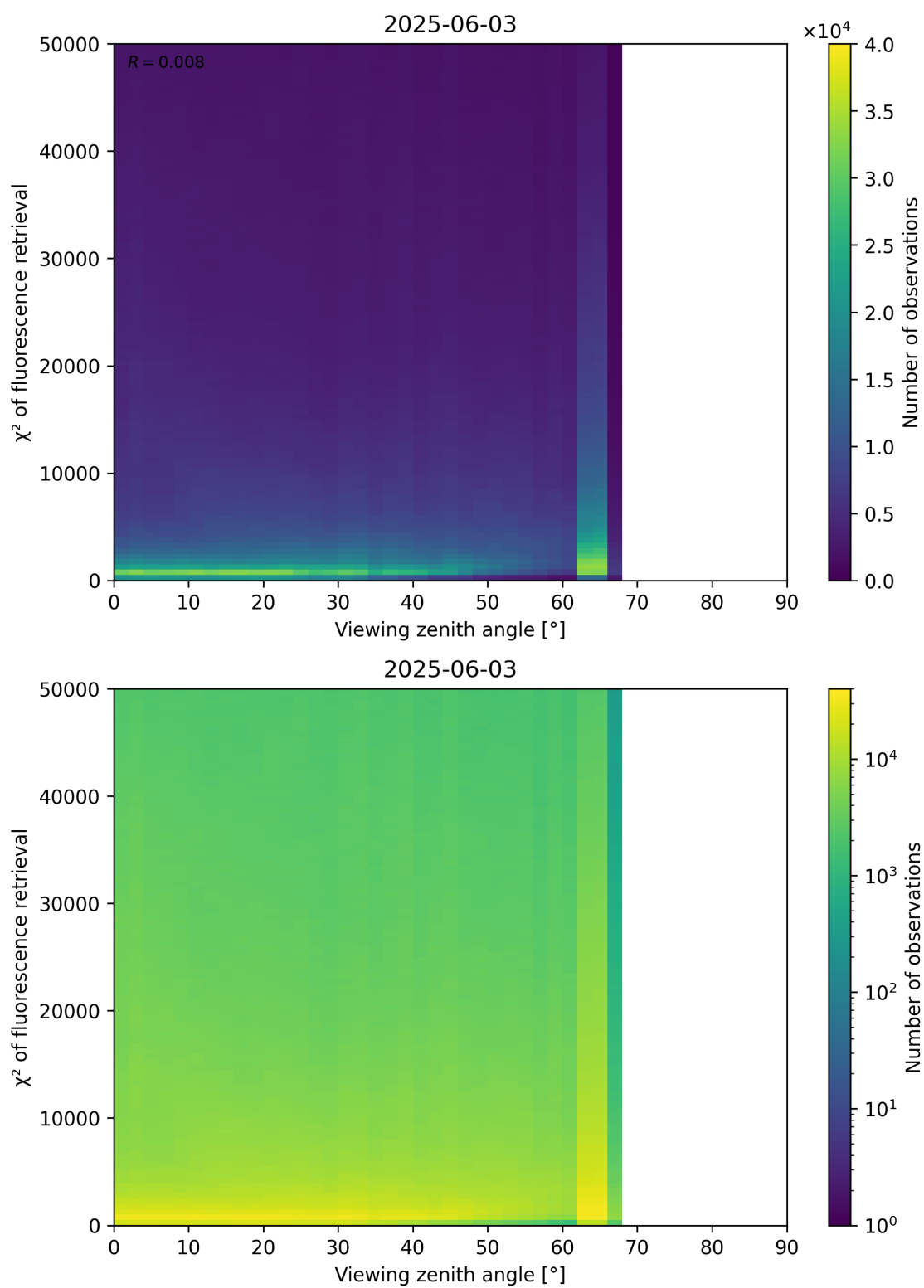
Figure 119: Scatter density plot of “Viewing zenith angle” against “ \chi^2 of fluorescence retrieval” for 2025-06-02 to 2025-06-04.
