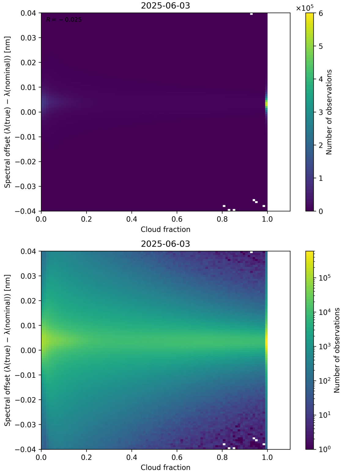
Figure 76: Scatter density plot of “Cloud fraction” against “Spectral offset ( \lambda_{\text{true}} - \lambda_{\text{nominal}} )” for 2025-06-02 to 2025-06-04.
