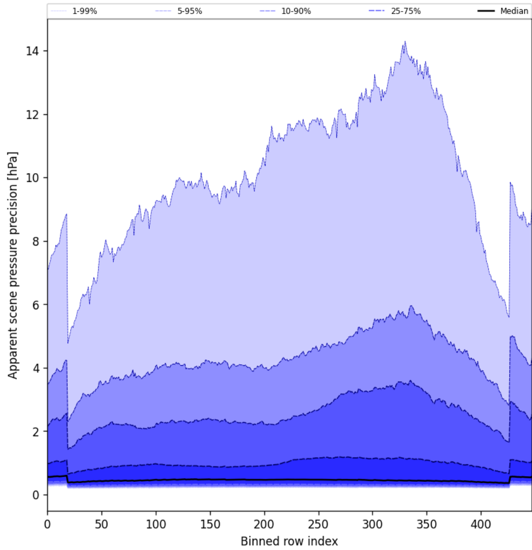
Figure 54: Along track statistics of “Apparent scene pressure precision” for 2025-06-02 to 2025-06-04
