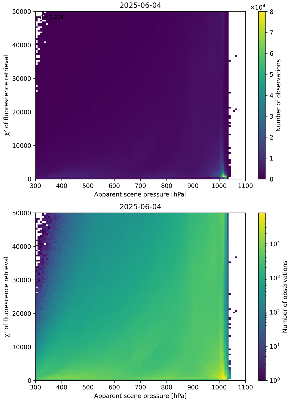
Figure 63: Scatter density plot of “Apparent scene pressure” against “ \chi^2 of fluorescence retrieval” for 2025-06-03 to 2025-06-05.
