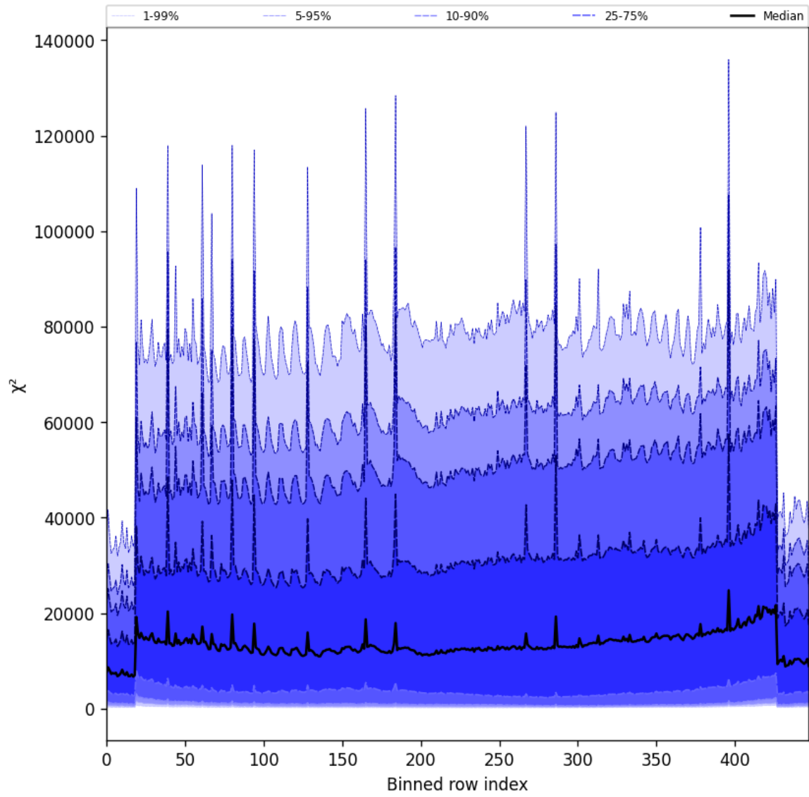
Figure 55: Along track statistics of “ \chi^2 ” for 2025-06-03 to 2025-06-05
