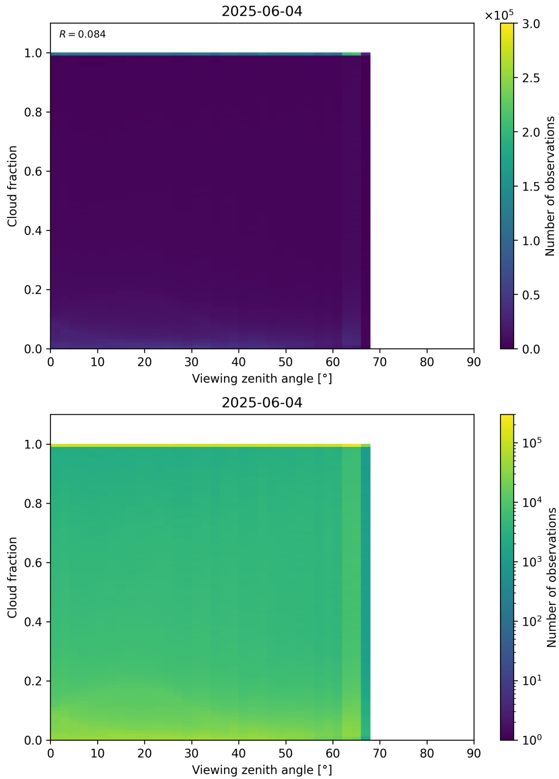
Figure 120: Scatter density plot of “Viewing zenith angle” against “Cloud fraction” for 2025-06-03 to 2025-06-05.
