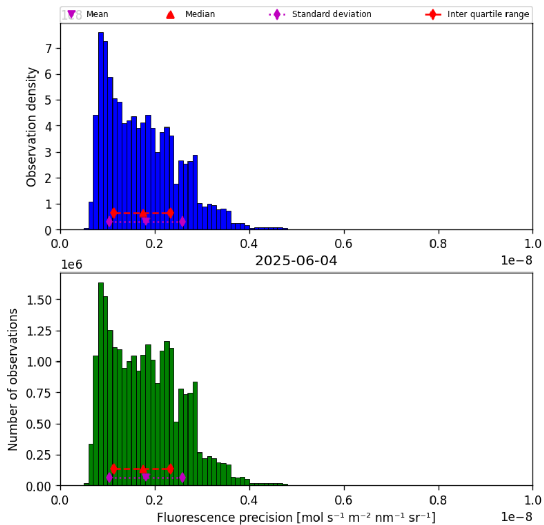
Figure 41: Histogram of “Fluorescence precision” for 2025-06-03 to 2025-06-05
