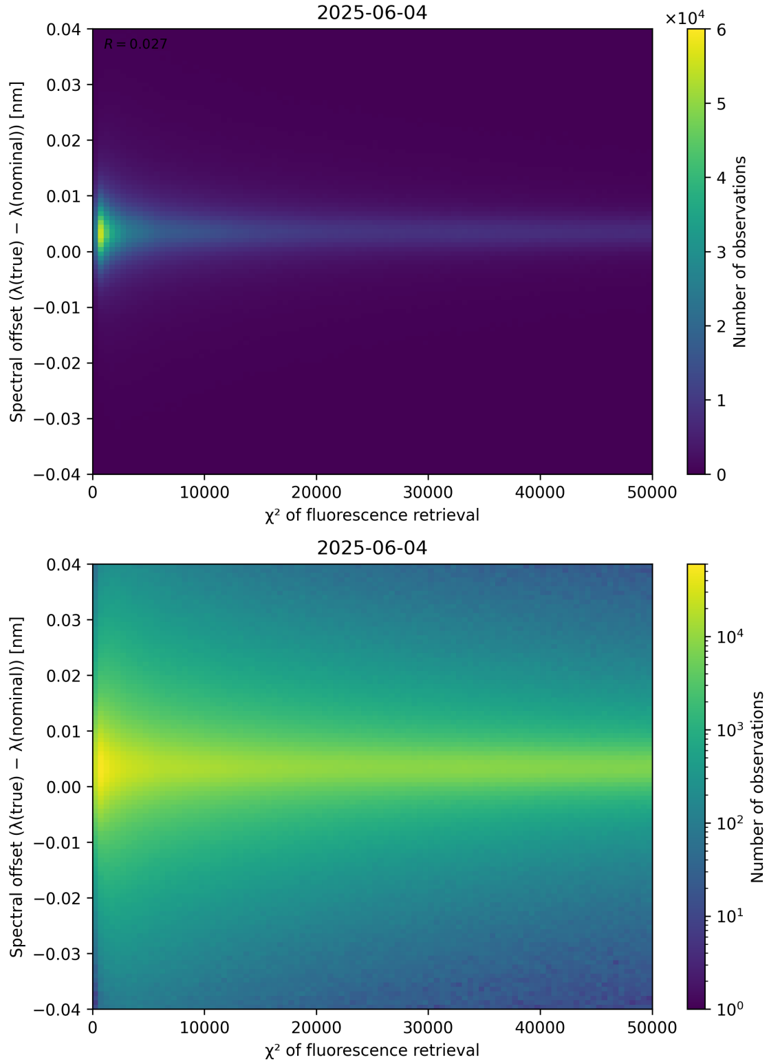
Figure 69: Scatter density plot of “ \chi^2 of fluorescence retrieval” against “Spectral offset ( \lambda_{\text{true}} - \lambda_{\text{nominal}} )” for 2025-06-03 to 2025-06-05.
