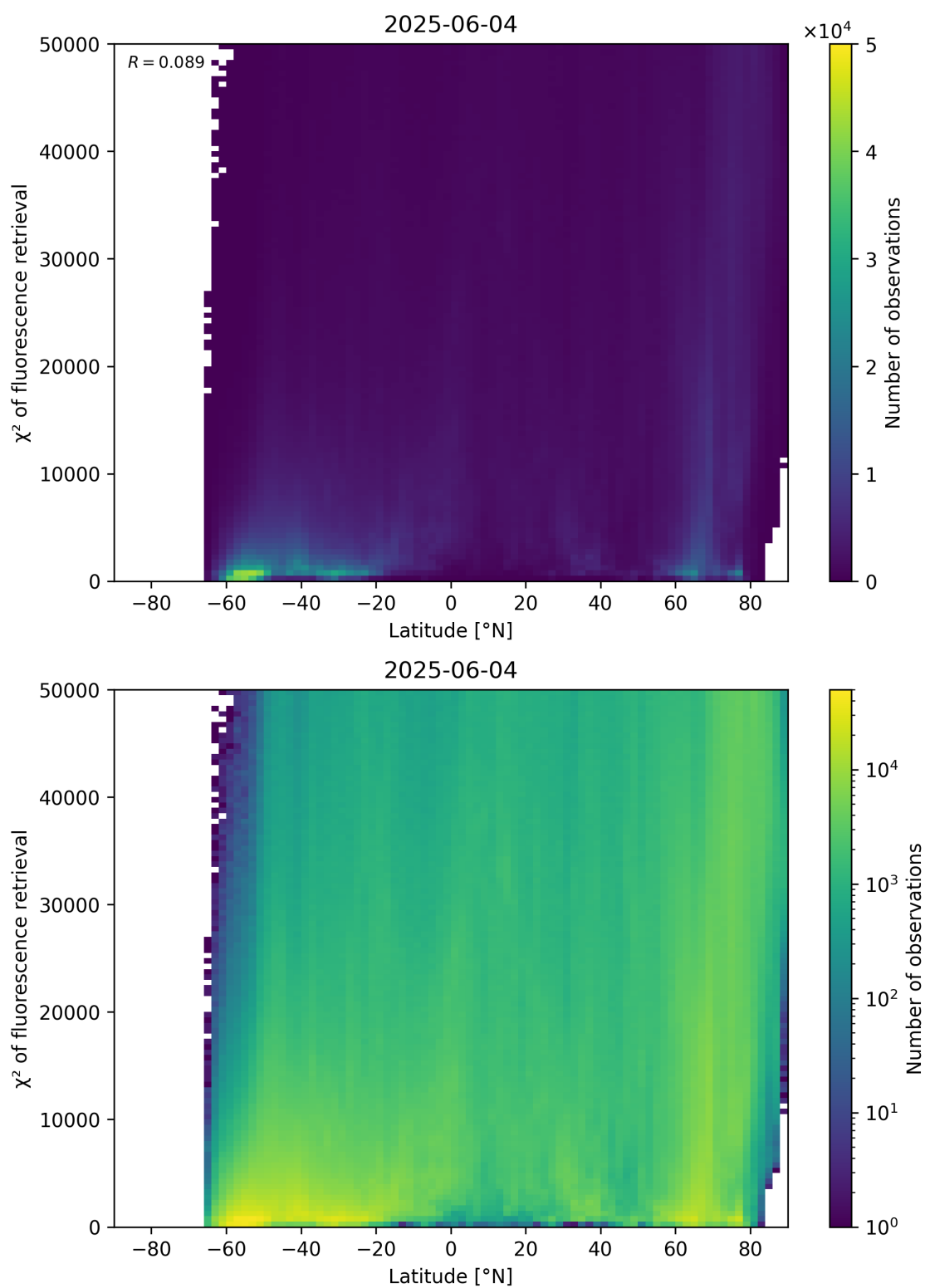
Figure 89: Scatter density plot of “Latitude” against “ \chi^2 of fluorescence retrieval” for 2025-06-03 to 2025-06-05.
