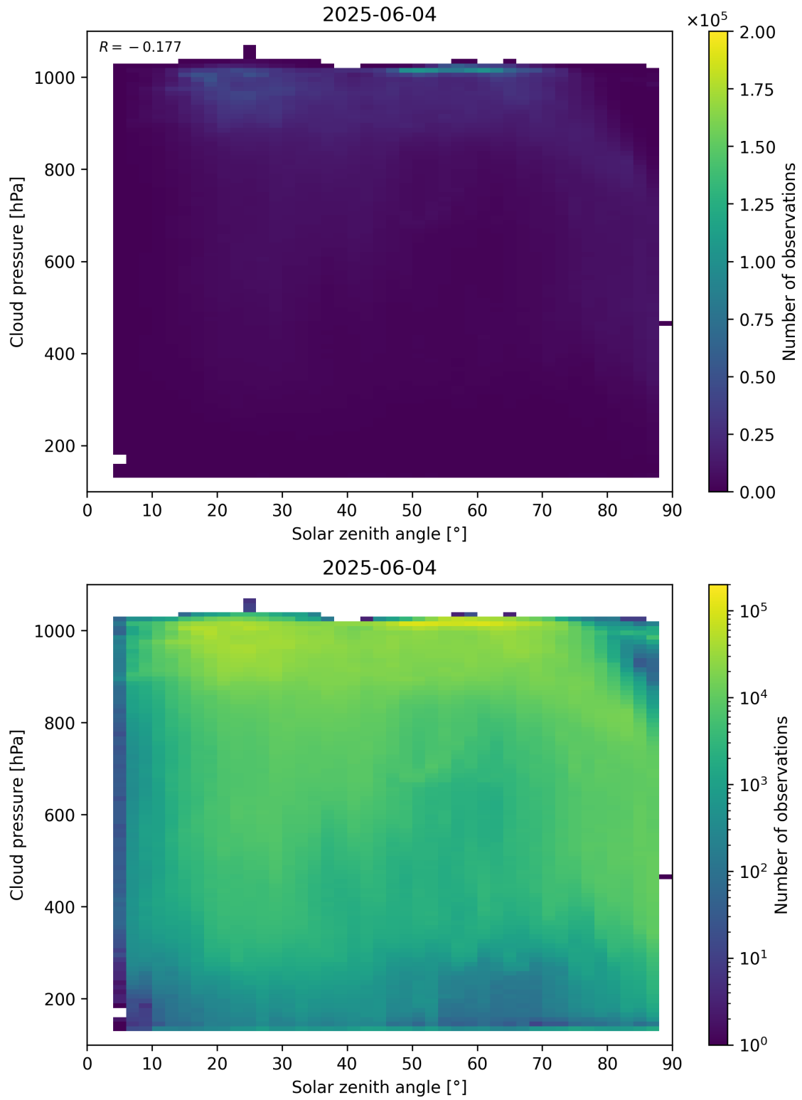
Figure 111: Scatter density plot of “Solar zenith angle” against “Cloud pressure” for 2025-06-03 to 2025-06-05.
