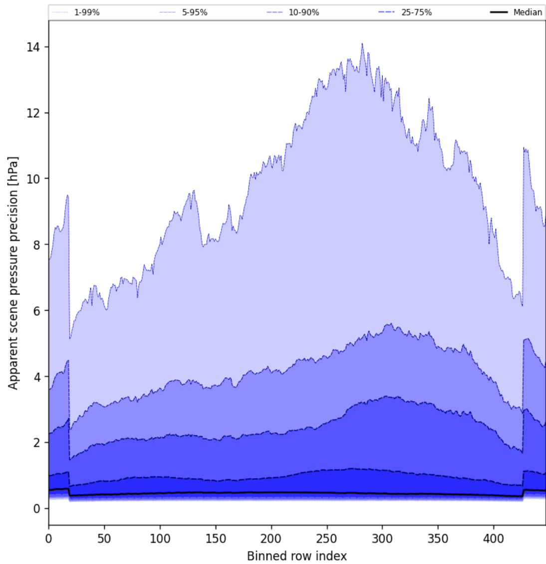
Figure 54: Along track statistics of “Apparent scene pressure precision” for 2025-06-03 to 2025-06-05
