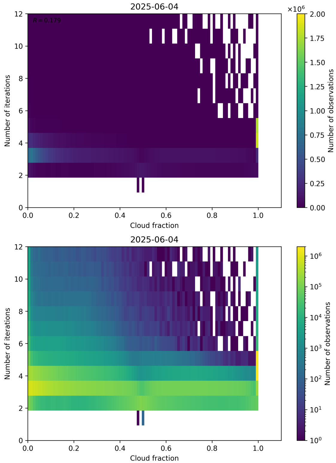
Figure 73: Scatter density plot of “Cloud fraction” against “Number of iterations” for 2025-06-03 to 2025-06-05.
