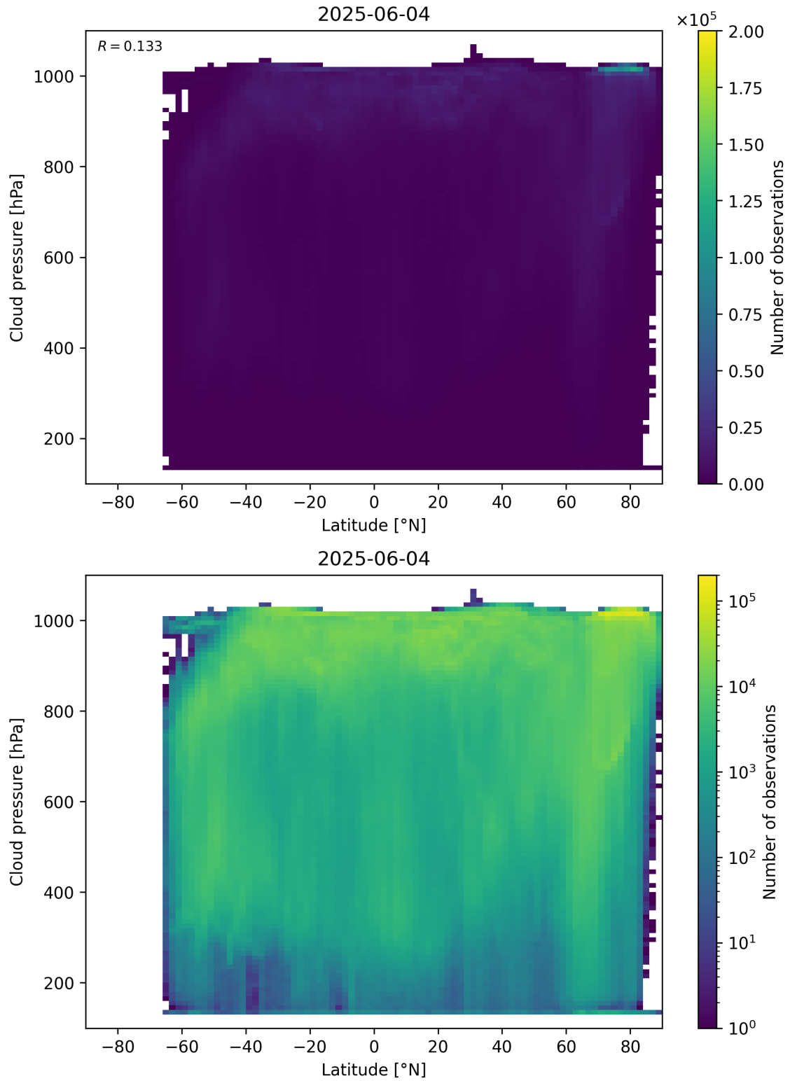
Figure 91: Scatter density plot of “Latitude” against “Cloud pressure” for 2025-06-03 to 2025-06-05.
