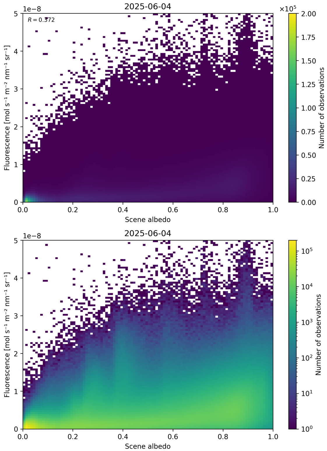
Figure 104: Scatter density plot of “Scene albedo” against “Fluorescence” for 2025-06-03 to 2025-06-05.
