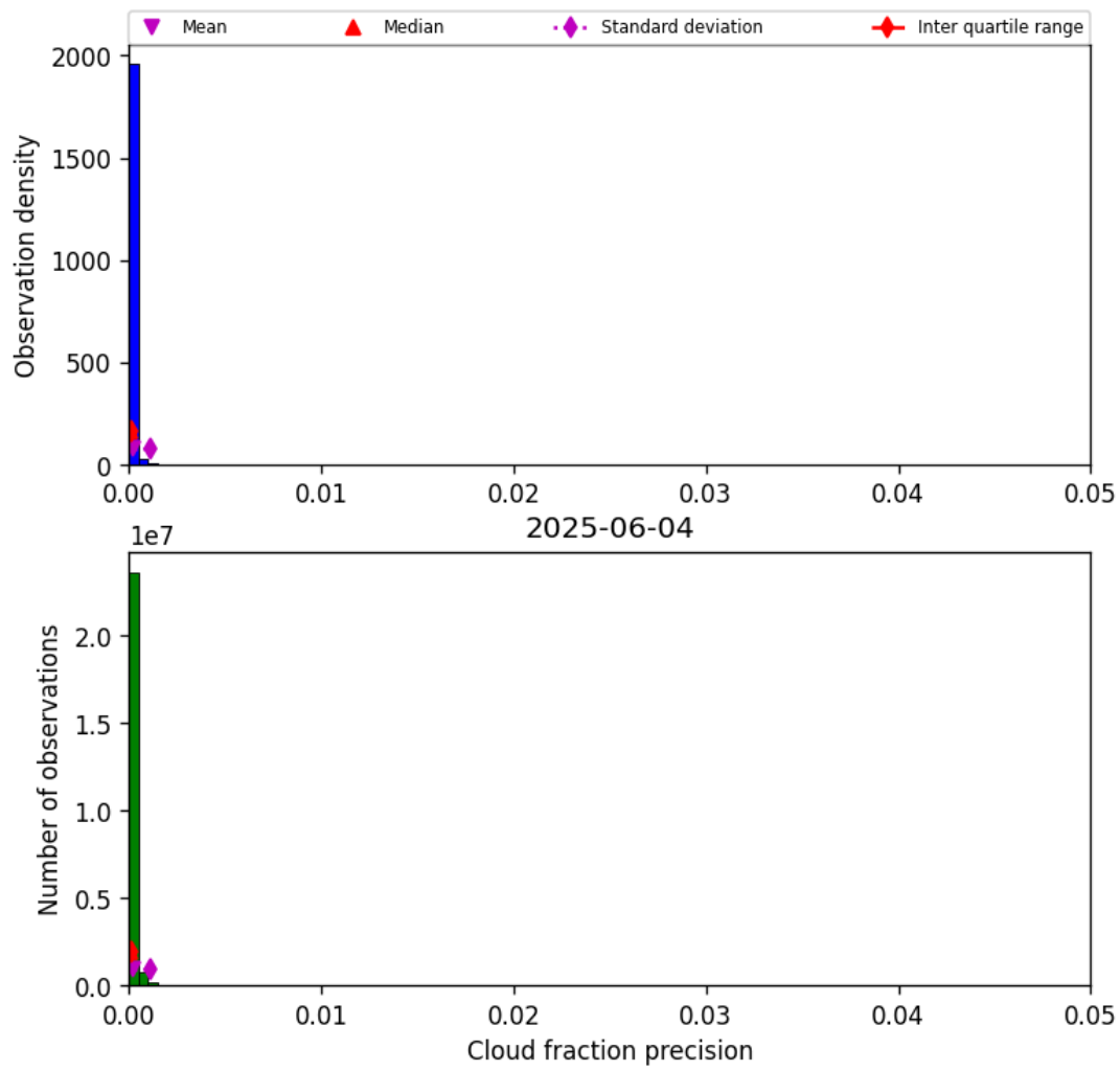
Figure 33: Histogram of “Cloud fraction precision” for 2025-06-03 to 2025-06-05
