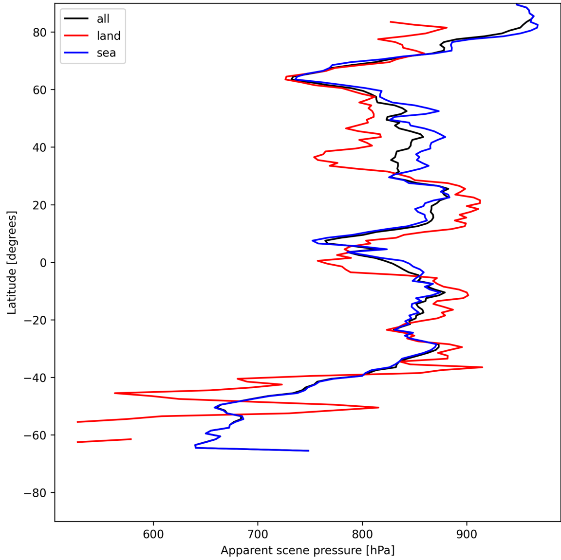
Figure 19: Zonal average of “Apparent scene pressure” for 2025-06-03 to 2025-06-05.
