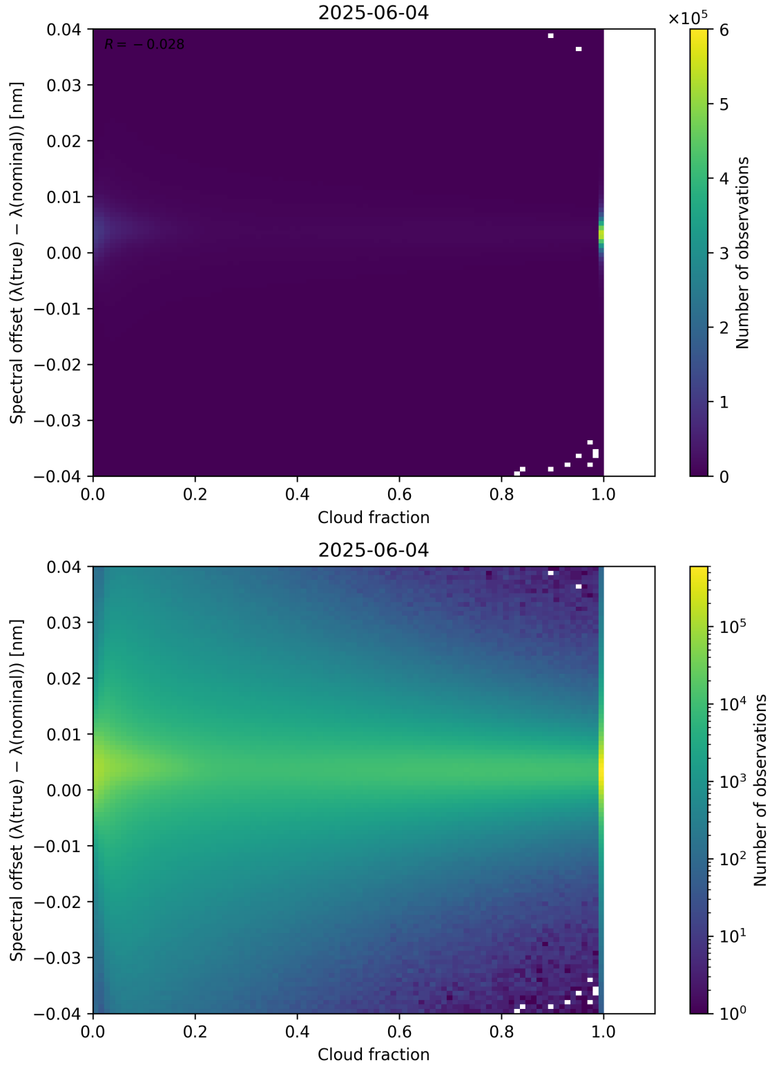
Figure 76: Scatter density plot of “Cloud fraction” against “Spectral offset ( \lambda_{\text{true}} - \lambda_{\text{nominal}} )” for 2025-06-03 to 2025-06-05.
