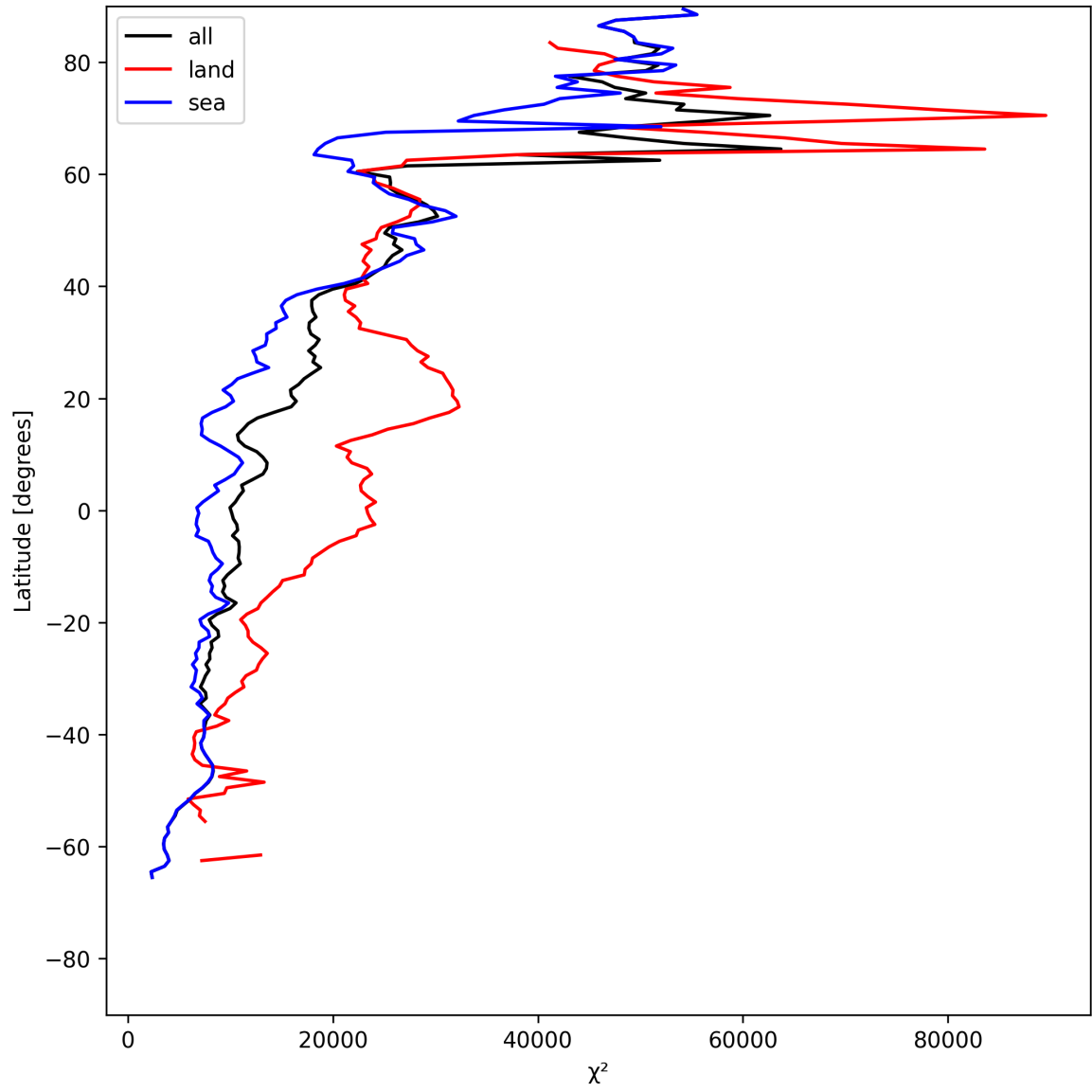
Figure 21: Zonal average of “ \chi^2 ” for 2025-06-03 to 2025-06-05.
