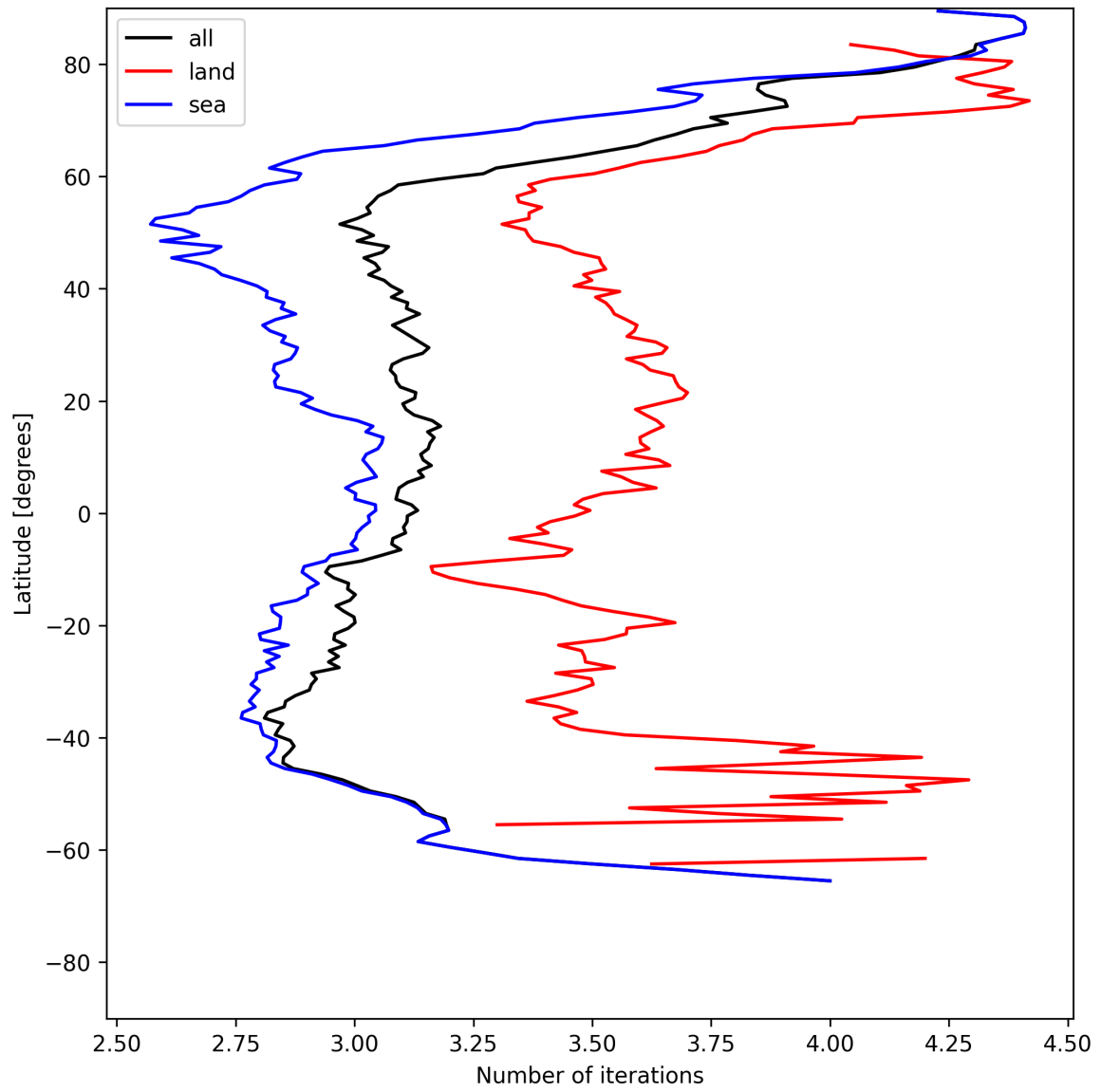
Figure 22: Zonal average of “Number of iterations” for 2025-06-03 to 2025-06-05.
