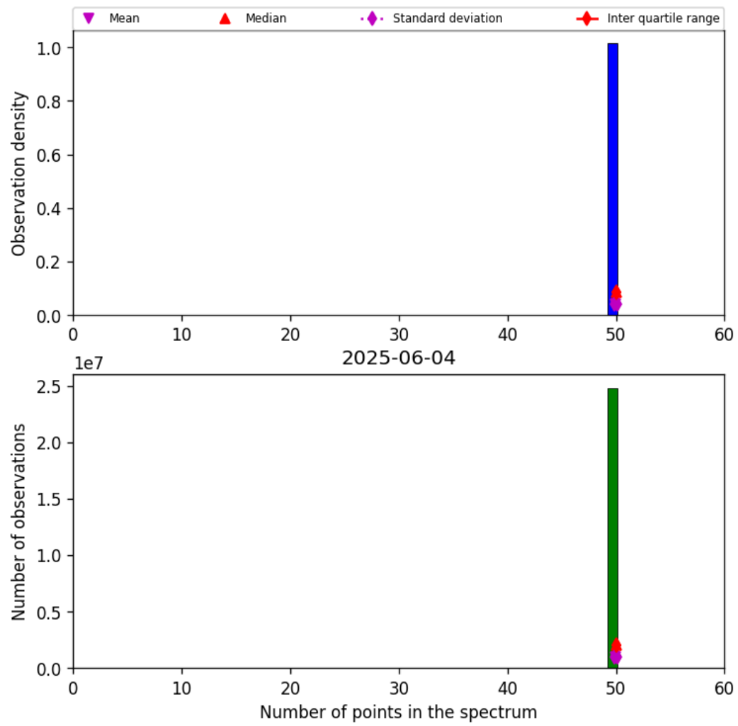
Figure 44: Histogram of “Number of points in the spectrum” for 2025-06-03 to 2025-06-05
