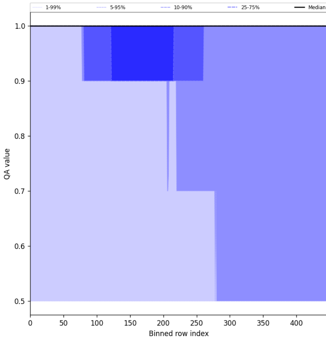
Figure 46: Along track statistics of “QA value” for 2025-06-03 to 2025-06-05
