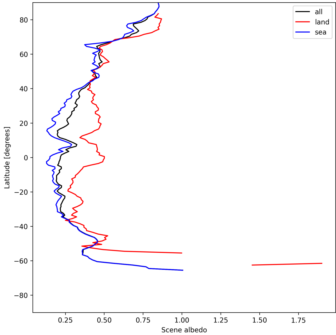
Figure 17: Zonal average of “Scene albedo” for 2025-06-03 to 2025-06-05.
