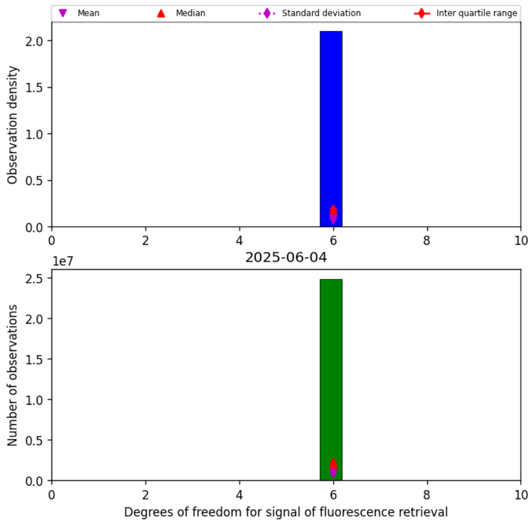
Figure 43: Histogram of “Degrees of freedom for signal of fluorescence retrieval” for 2025-06-03 to 2025-06-05
