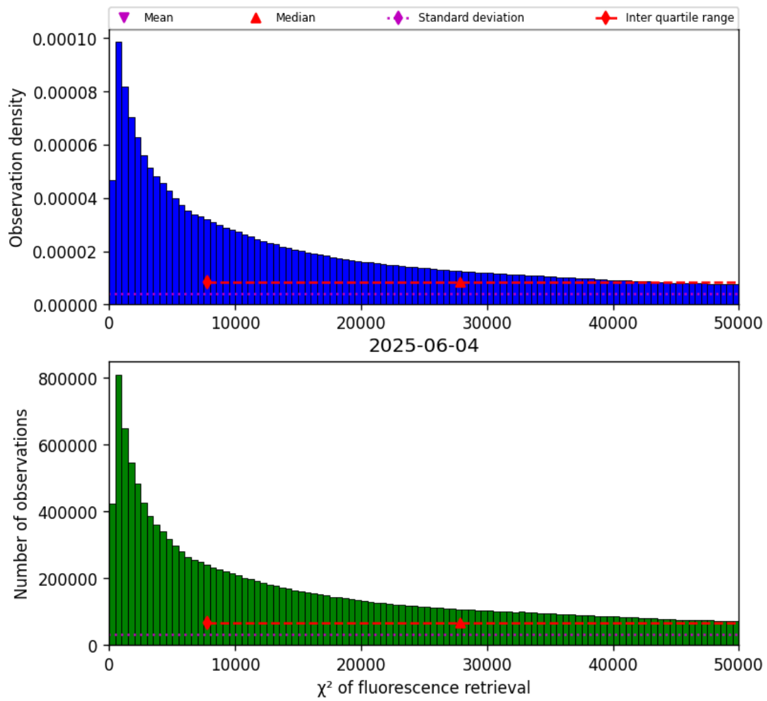
Figure 42: Histogram of “ \chi^2 of fluorescence retrieval” for 2025-06-03 to 2025-06-05
