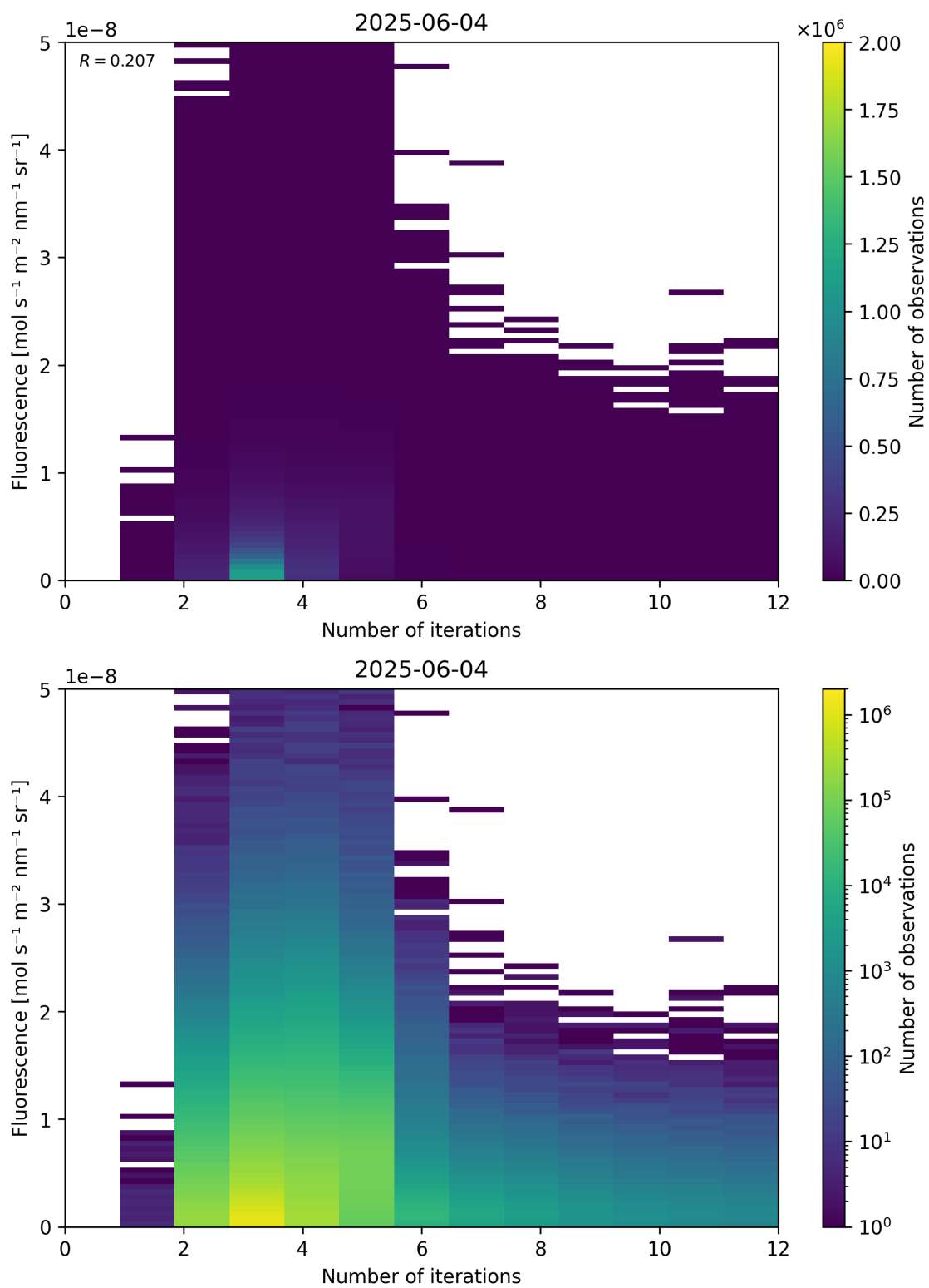
Figure 98: Scatter density plot of “Number of iterations” against “Fluorescence” for 2025-06-03 to 2025-06-05.
