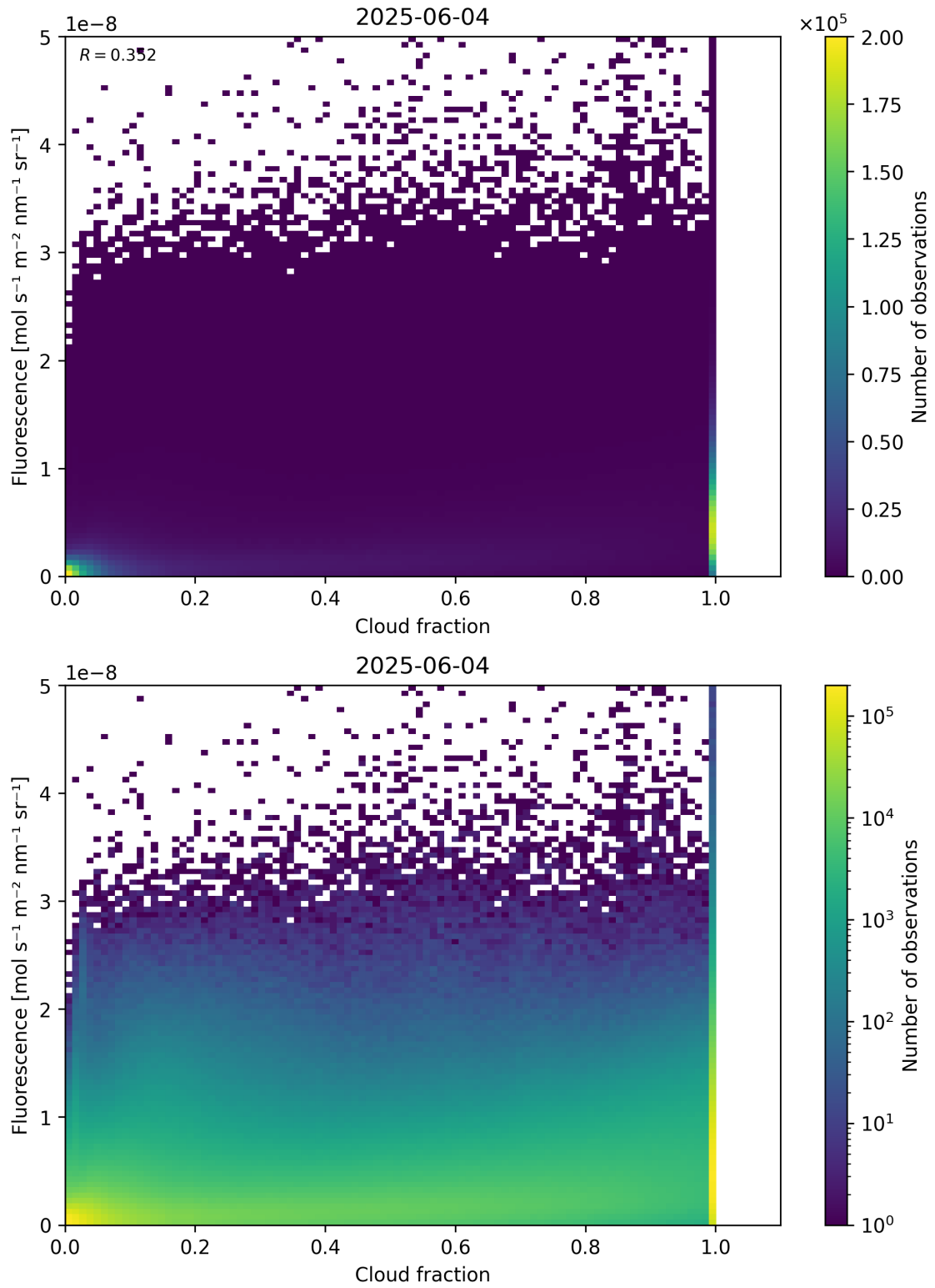
Figure 72: Scatter density plot of “Cloud fraction” against “Fluorescence” for 2025-06-03 to 2025-06-05.
