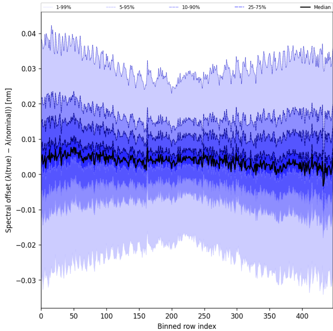
Figure 62: Along track statistics of “Spectral offset ( \lambda_{\text{true}} - \lambda_{\text{nominal}} )” for 2025-06-03 to 2025-06-05
