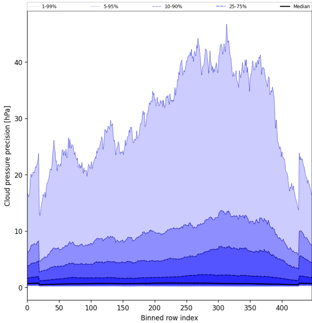
Figure 48: Along track statistics of “Cloud pressure precision” for 2025-06-03 to 2025-06-05
