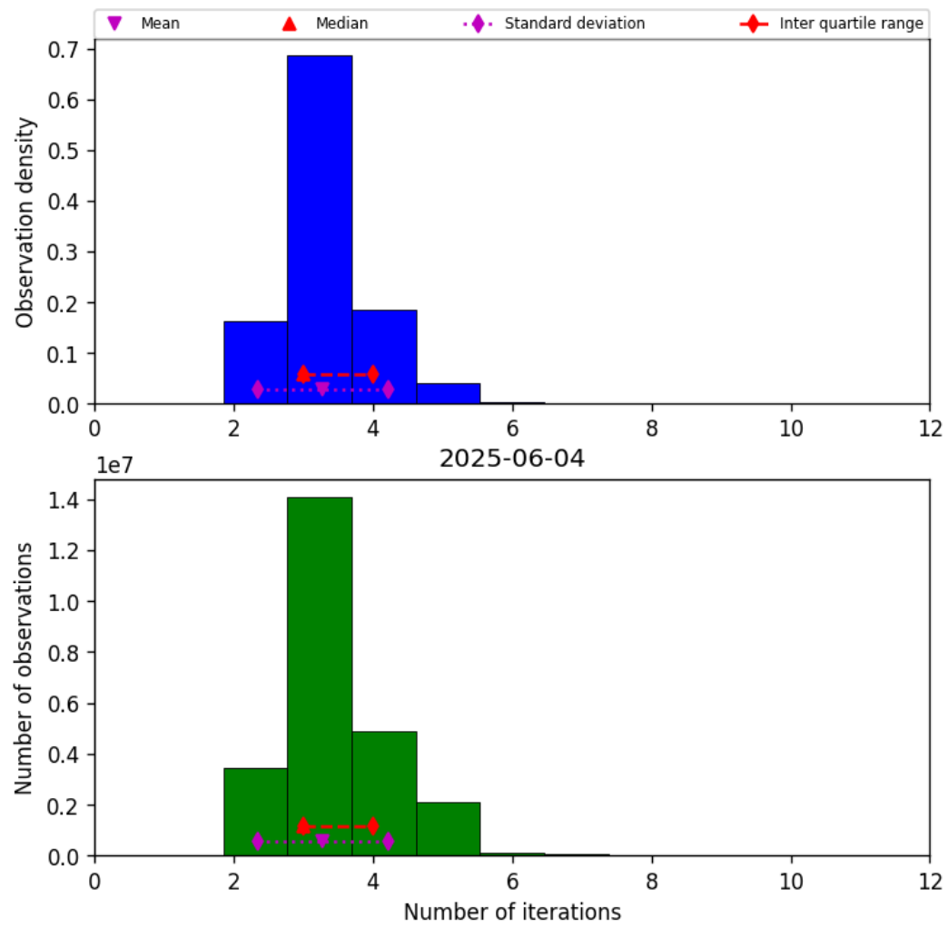
Figure 39: Histogram of “Number of iterations” for 2025-06-03 to 2025-06-05
