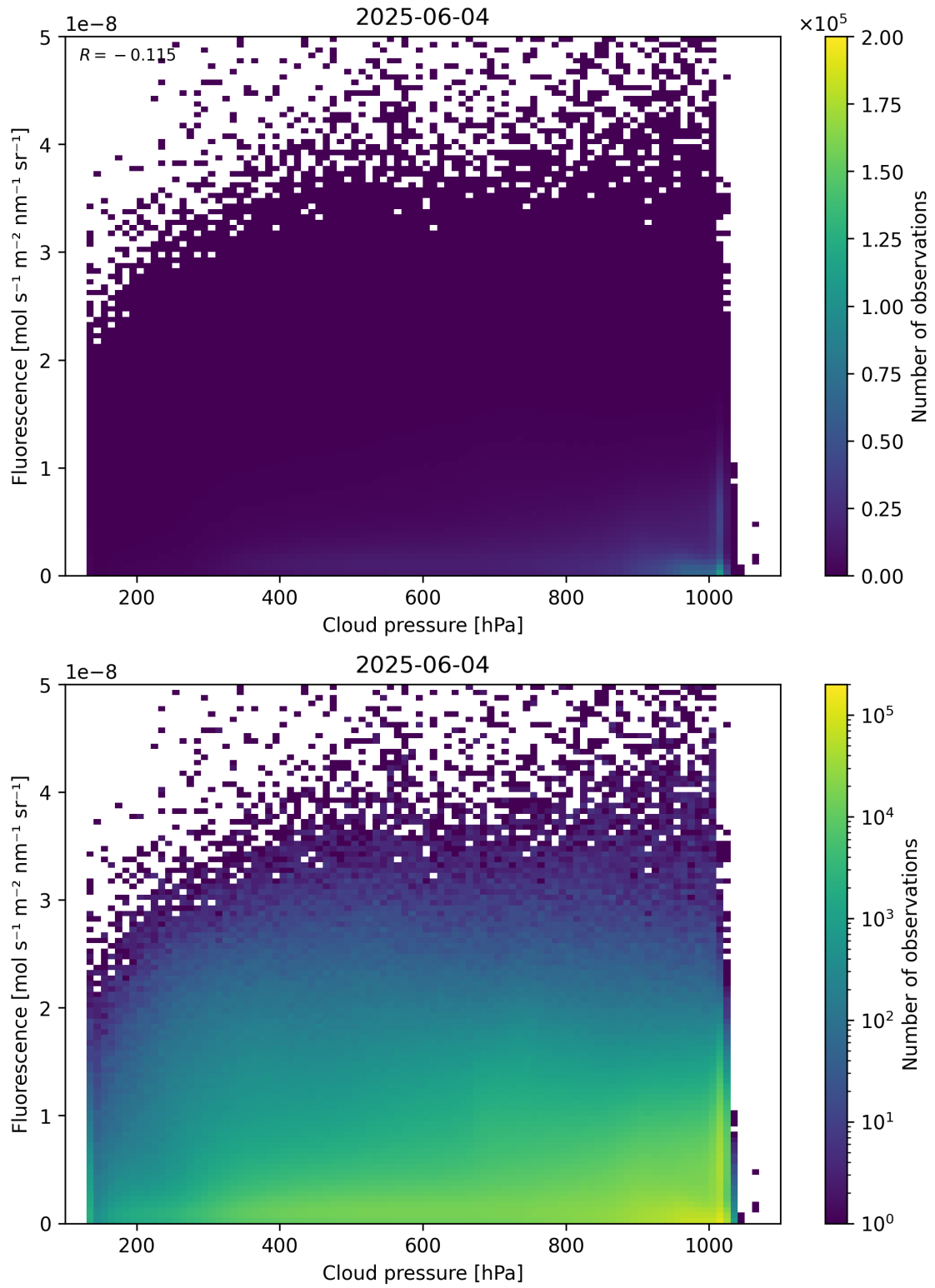
Figure 80: Scatter density plot of “Cloud pressure” against “Fluorescence” for 2025-06-03 to 2025-06-05.
