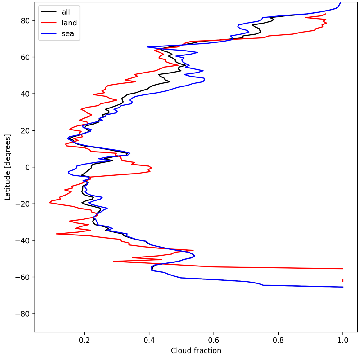
Figure 15: Zonal average of “Cloud fraction” for 2025-06-03 to 2025-06-05.
