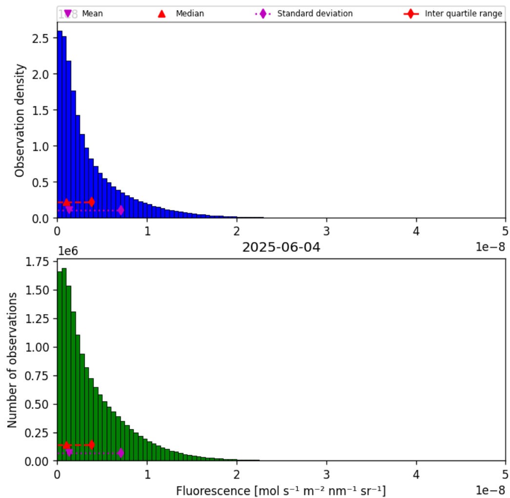
Figure 40: Histogram of “Fluorescence” for 2025-06-03 to 2025-06-05
