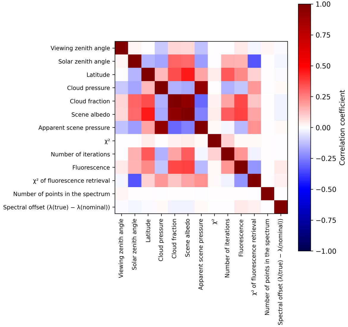
Figure 2: Map of correlation matrix for 2025-06-03 to 2025-06-05.
