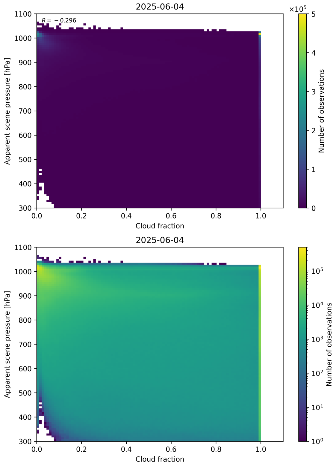
Figure 70: Scatter density plot of “Cloud fraction” against “Apparent scene pressure” for 2025-06-03 to 2025-06-05.
