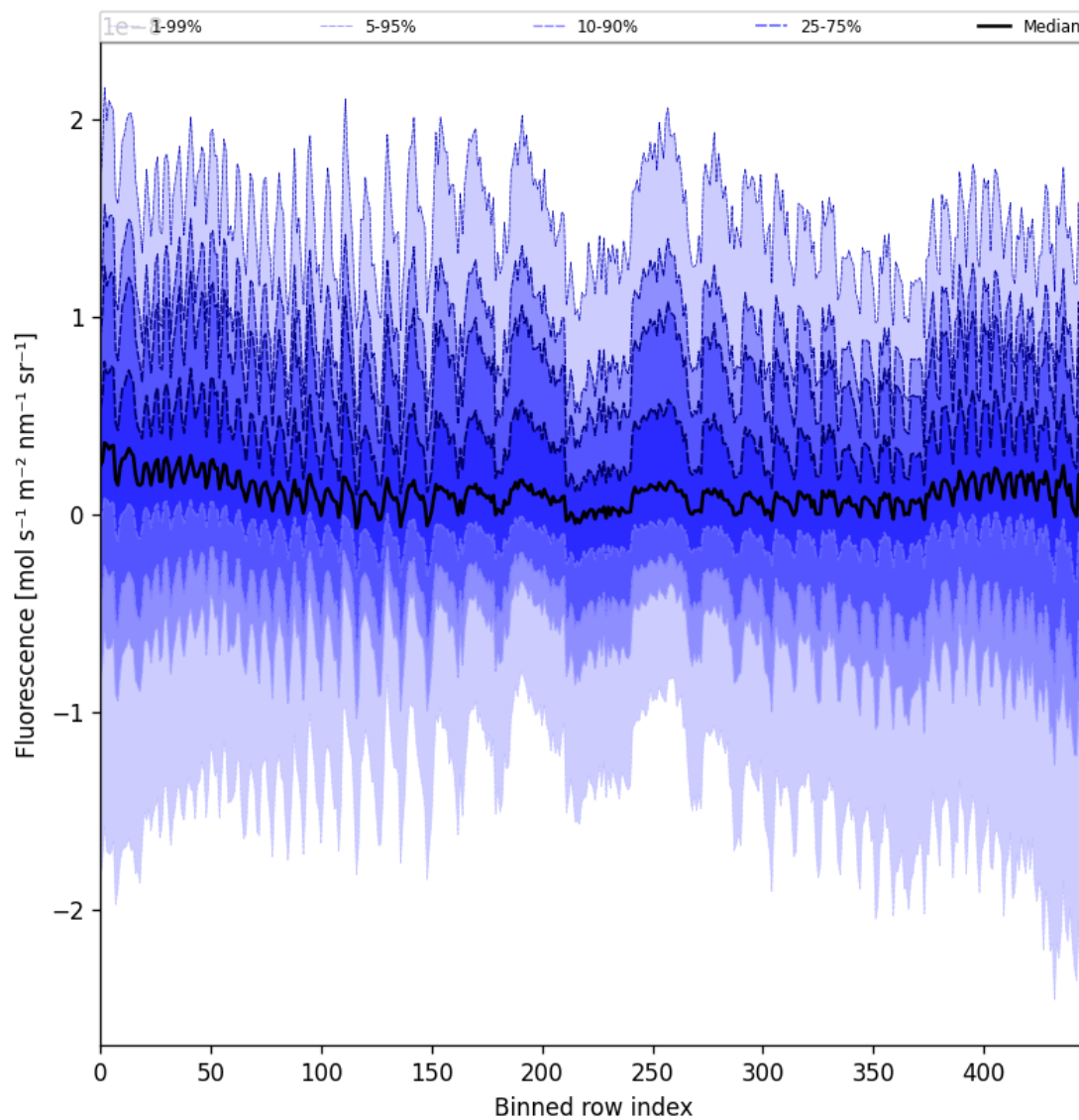
Figure 57: Along track statistics of “Fluorescence” for 2025-06-03 to 2025-06-05
