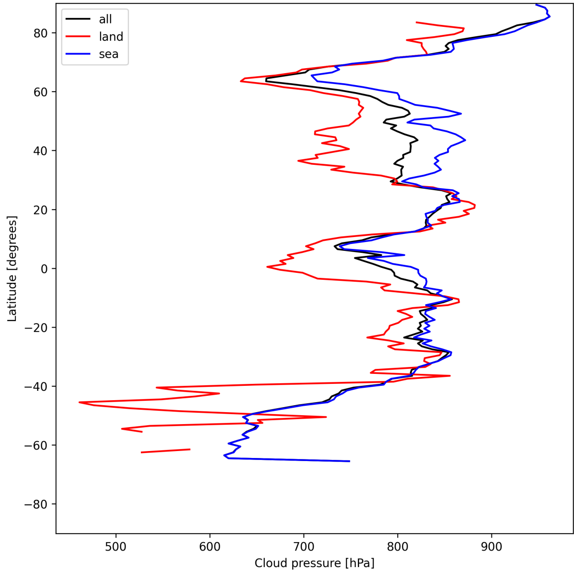
Figure 13: Zonal average of “Cloud pressure” for 2025-06-03 to 2025-06-05.
