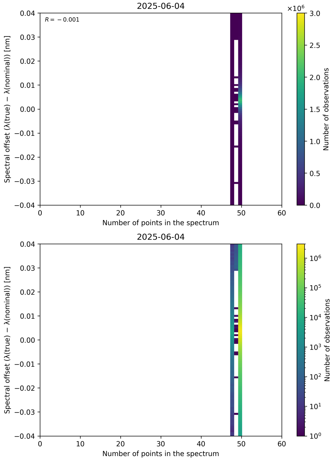
Figure 101: Scatter density plot of “Number of points in the spectrum” against “Spectral offset ( \lambda_{\text{true}} - \lambda_{\text{nominal}} )” for 2025-06-03 to 2025-06-05.
