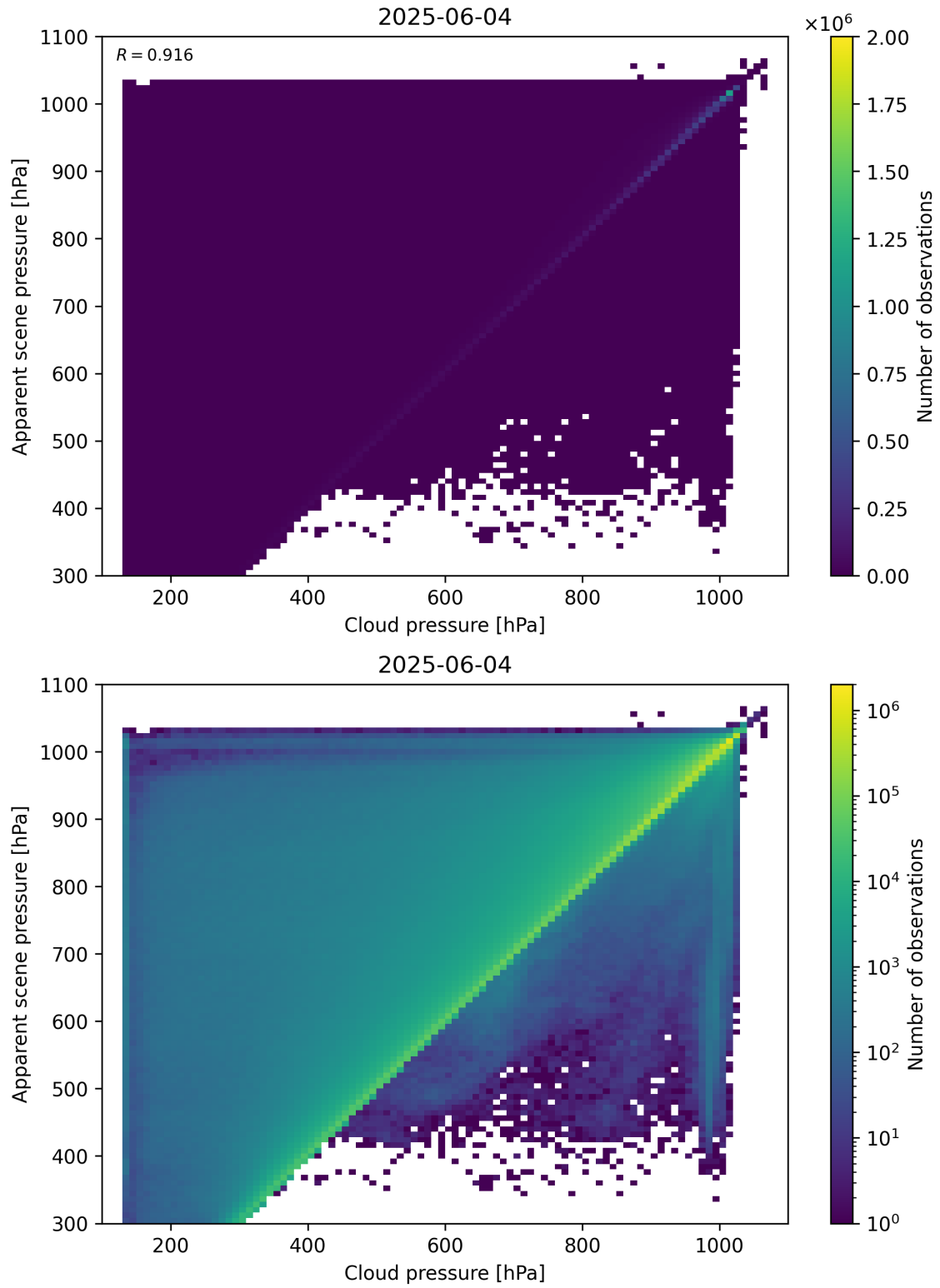
Figure 77: Scatter density plot of “Cloud pressure” against “Apparent scene pressure” for 2025-06-03 to 2025-06-05.
