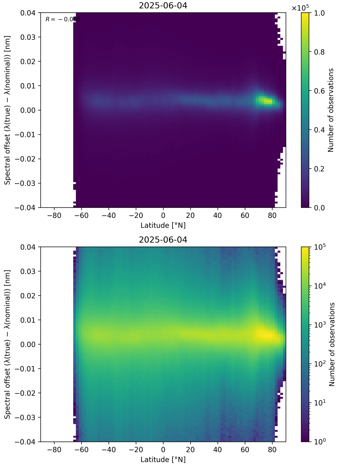
Figure 96: Scatter density plot of “Latitude” against “Spectral offset ( \lambda_{\text{true}} - \lambda_{\text{nominal}} )” for 2025-06-03 to 2025-06-05.
