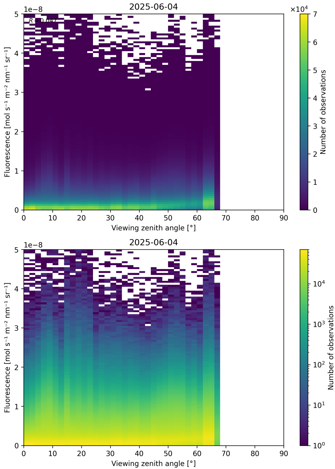
Figure 122: Scatter density plot of “Viewing zenith angle” against “Fluorescence” for 2025-06-03 to 2025-06-05.
