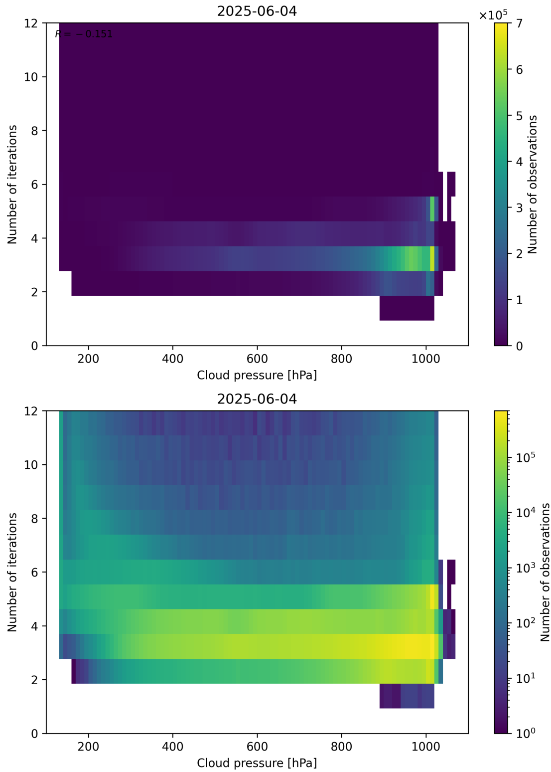
Figure 81: Scatter density plot of “Cloud pressure” against “Number of iterations” for 2025-06-03 to 2025-06-05.
