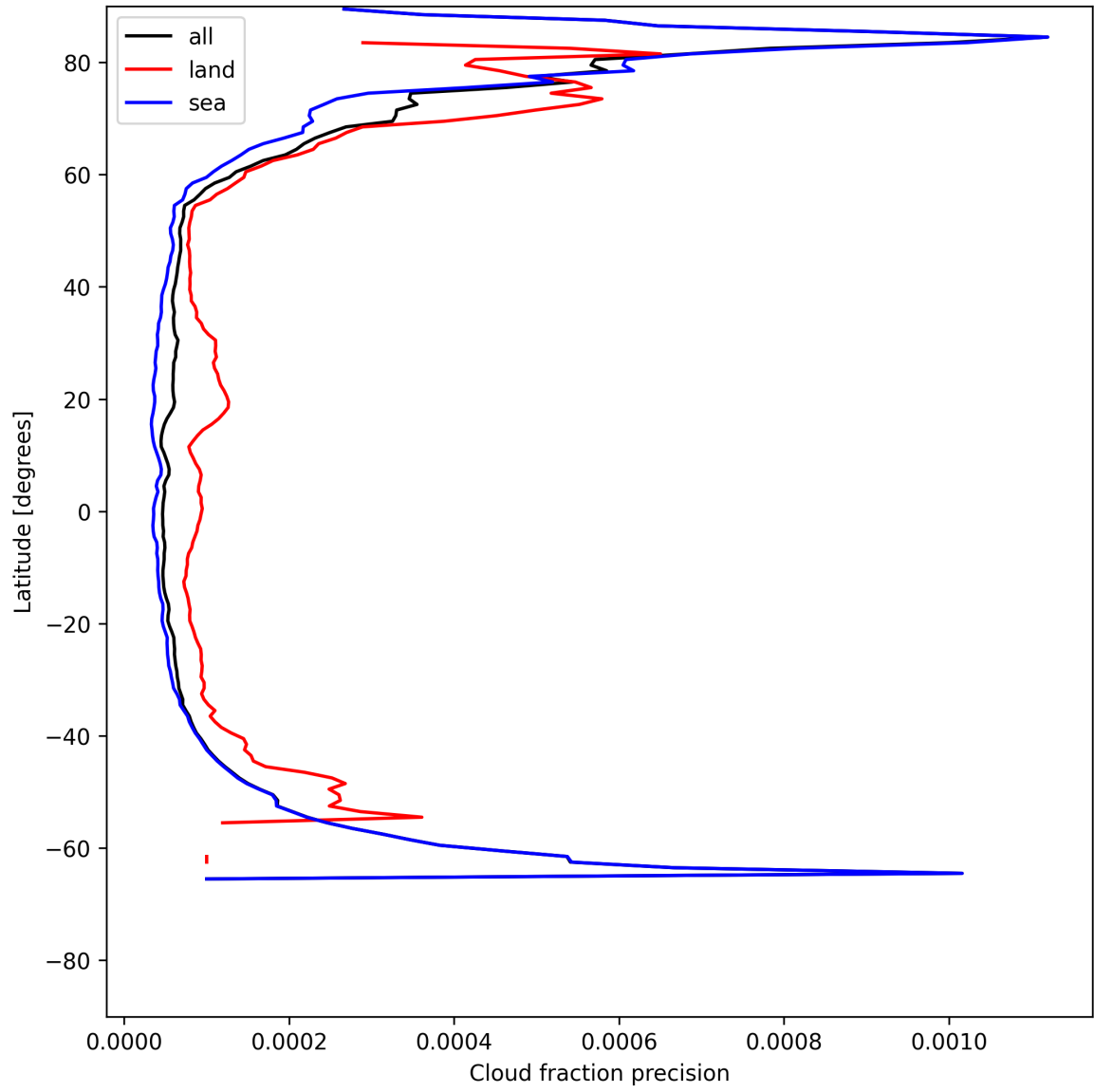
Figure 16: Zonal average of “Cloud fraction precision” for 2025-06-03 to 2025-06-05.
