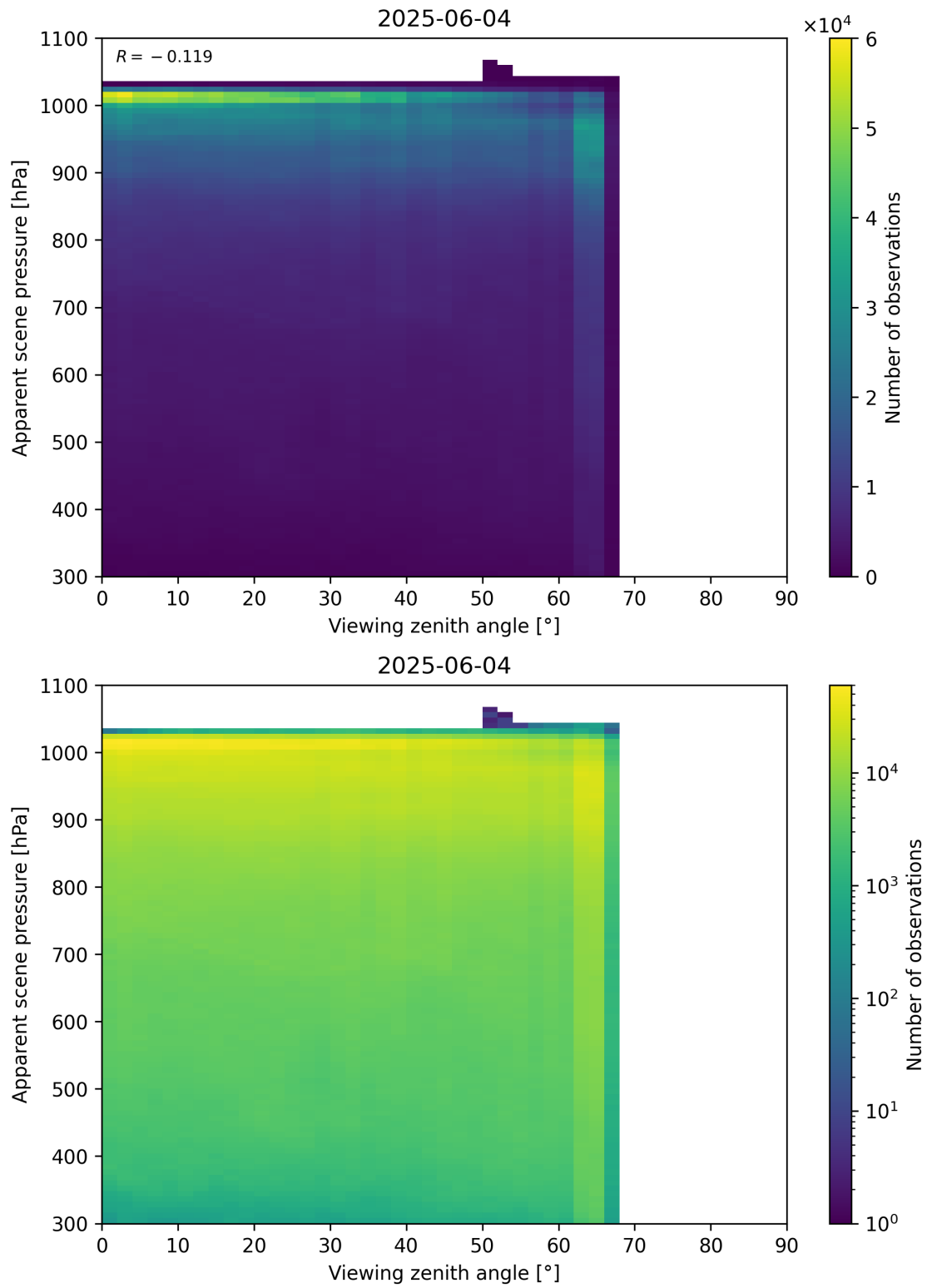
Figure 118: Scatter density plot of “Viewing zenith angle” against “Apparent scene pressure” for 2025-06-03 to 2025-06-05.
