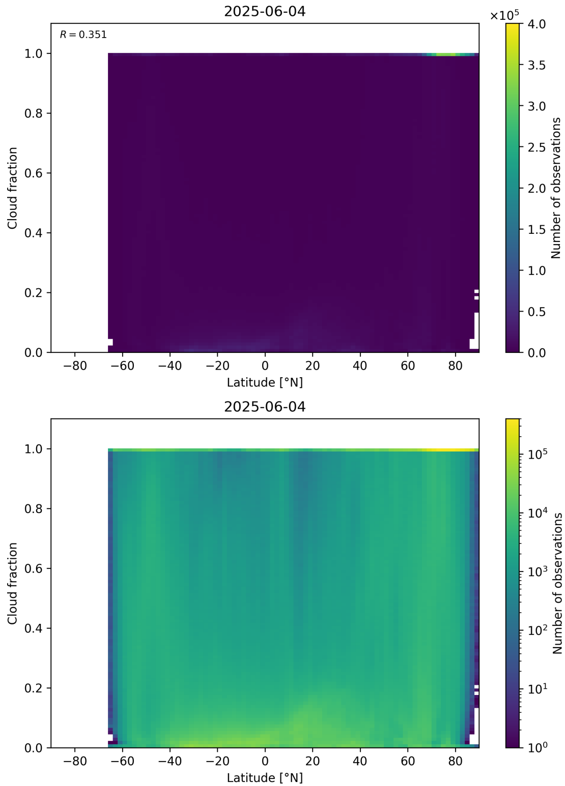
Figure 90: Scatter density plot of “Latitude” against “Cloud fraction” for 2025-06-03 to 2025-06-05.
