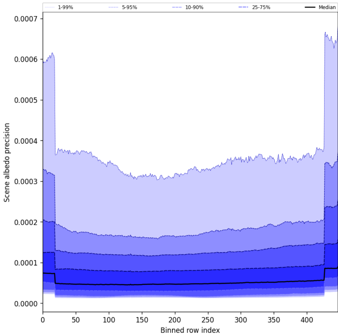
Figure 52: Along track statistics of “Scene albedo precision” for 2025-06-03 to 2025-06-05
