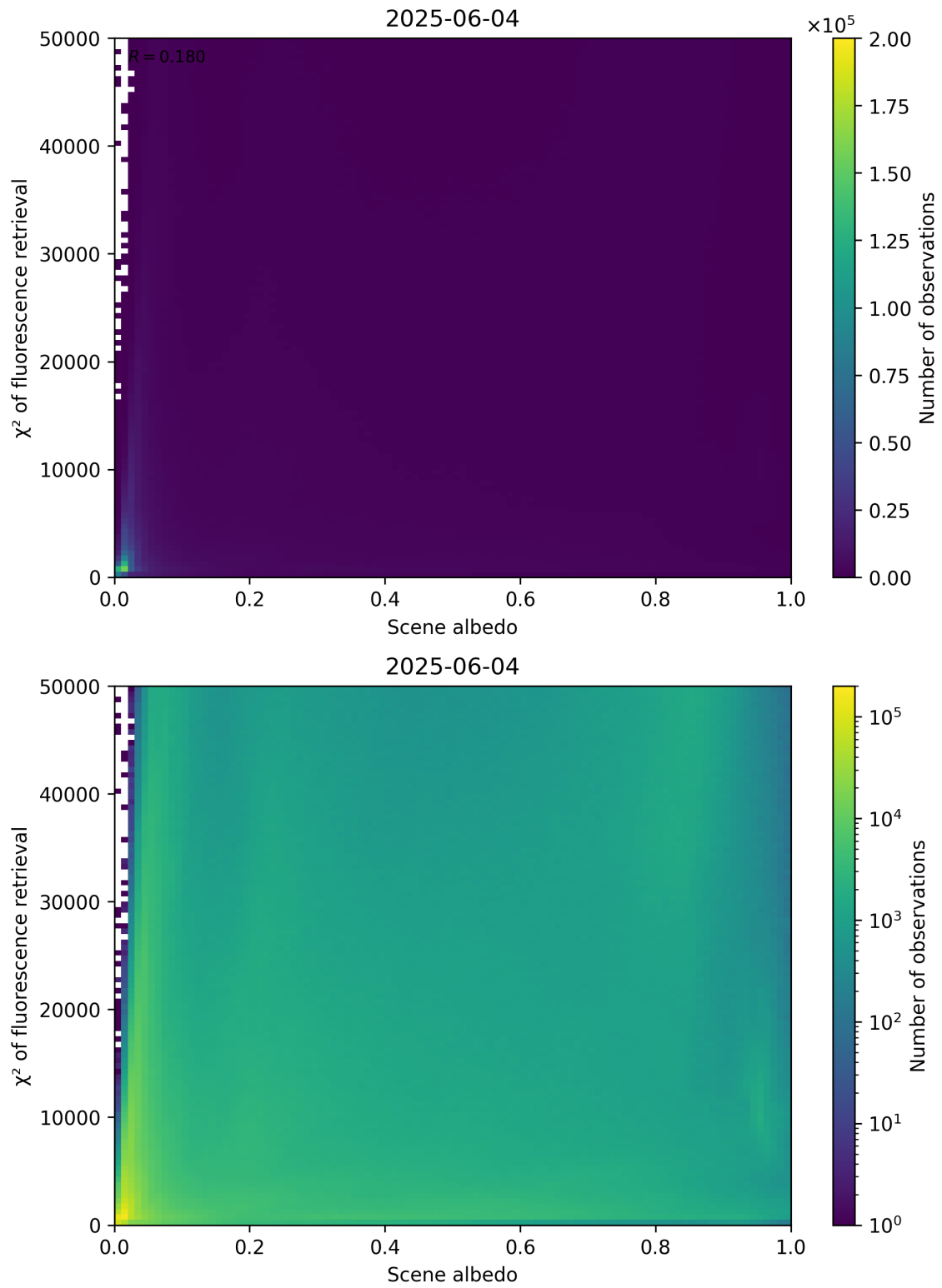
Figure 103: Scatter density plot of “Scene albedo” against “ \chi^2 of fluorescence retrieval” for 2025-06-03 to 2025-06-05.
