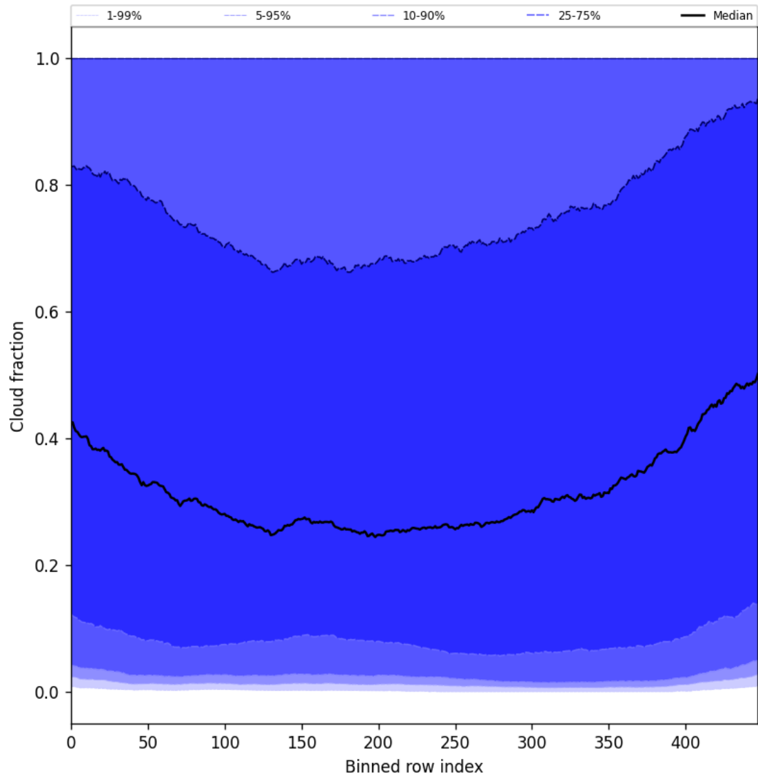
Figure 49: Along track statistics of “Cloud fraction” for 2025-06-03 to 2025-06-05
