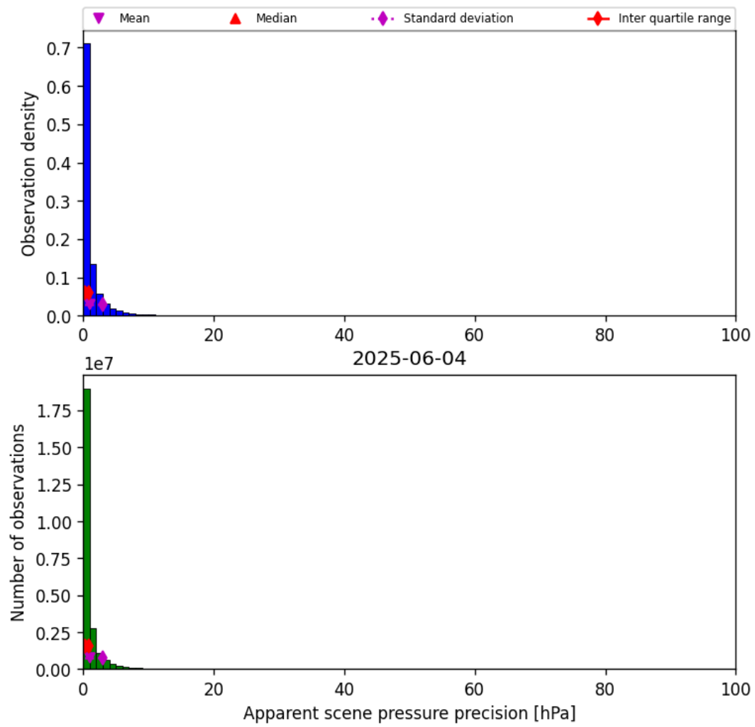
Figure 37: Histogram of “Apparent scene pressure precision” for 2025-06-03 to 2025-06-05
