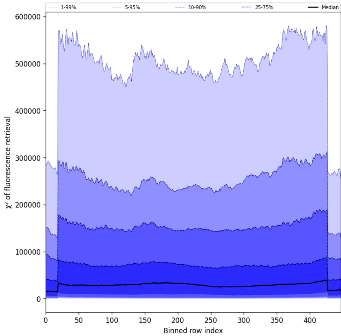
Figure 59: Along track statistics of “ \chi^2 of fluorescence retrieval” for 2025-06-03 to 2025-06-05
