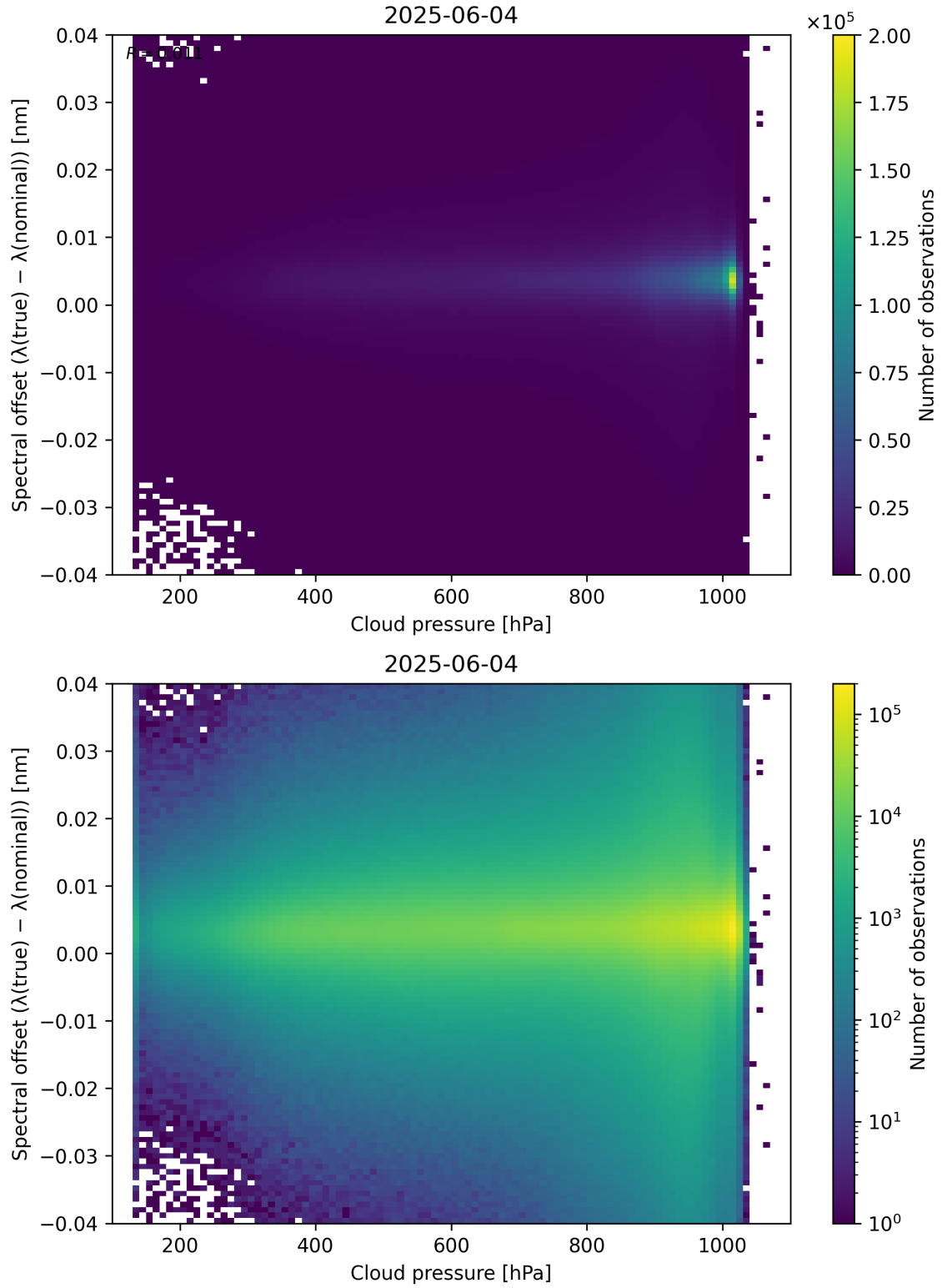
Figure 84: Scatter density plot of “Cloud pressure” against “Spectral offset ( \lambda_{\text{true}} - \lambda_{\text{nominal}} )” for 2025-06-03 to 2025-06-05.
