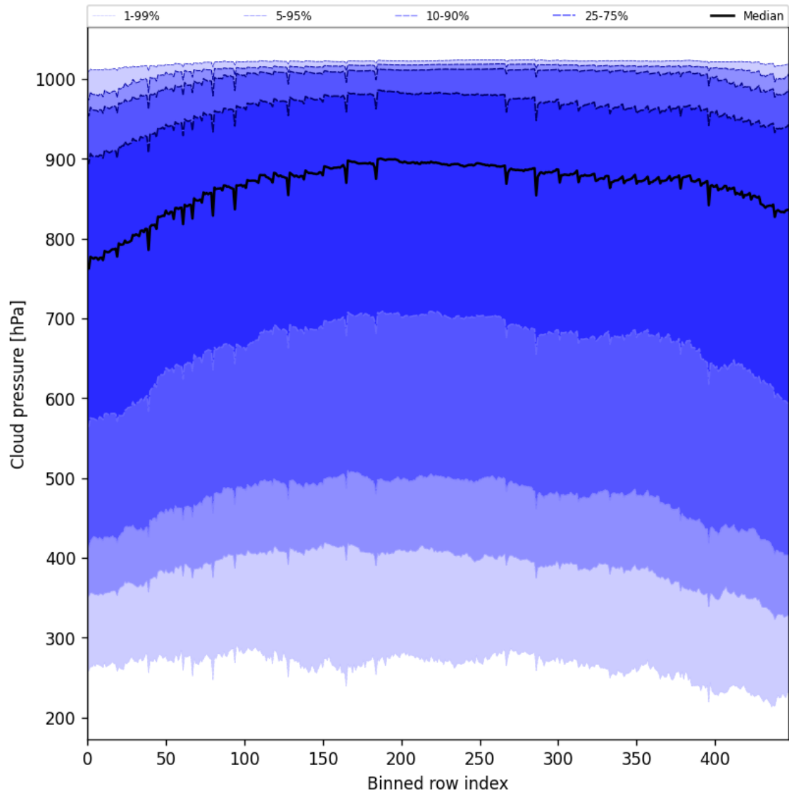
Figure 47: Along track statistics of “Cloud pressure” for 2025-06-03 to 2025-06-05
