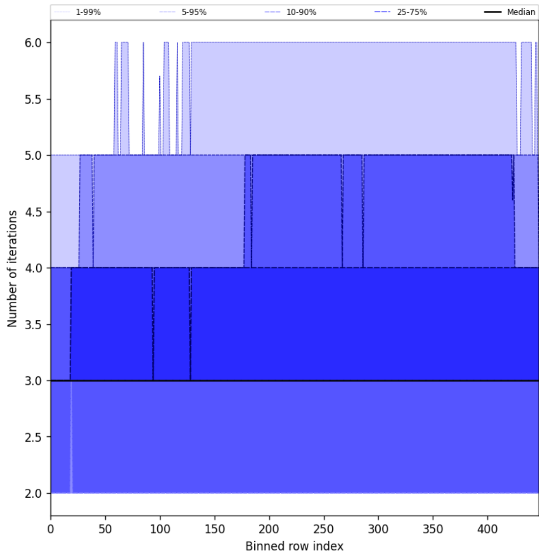
Figure 56: Along track statistics of “Number of iterations” for 2025-06-03 to 2025-06-05
