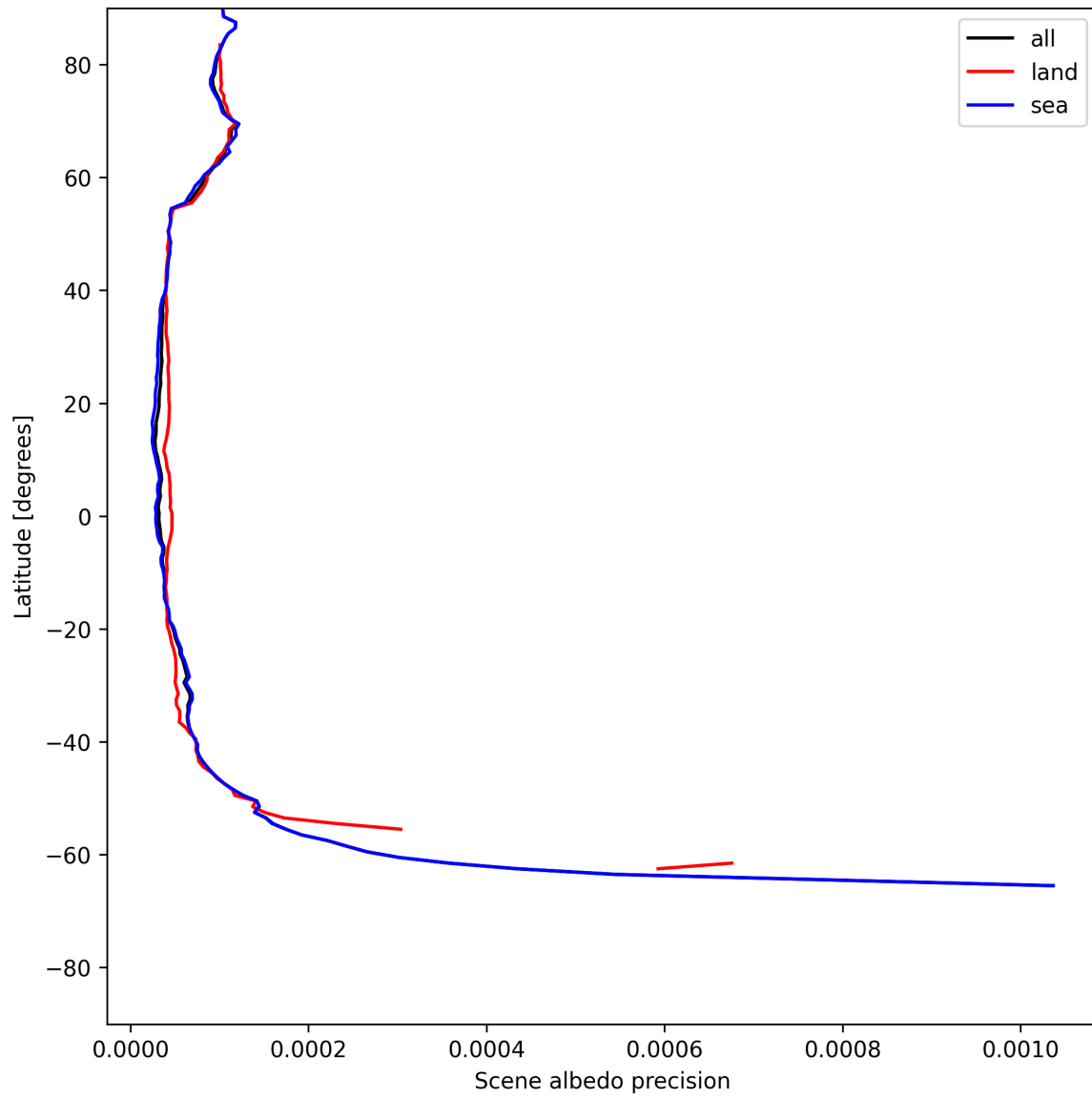
Figure 18: Zonal average of “Scene albedo precision” for 2025-06-03 to 2025-06-05.
