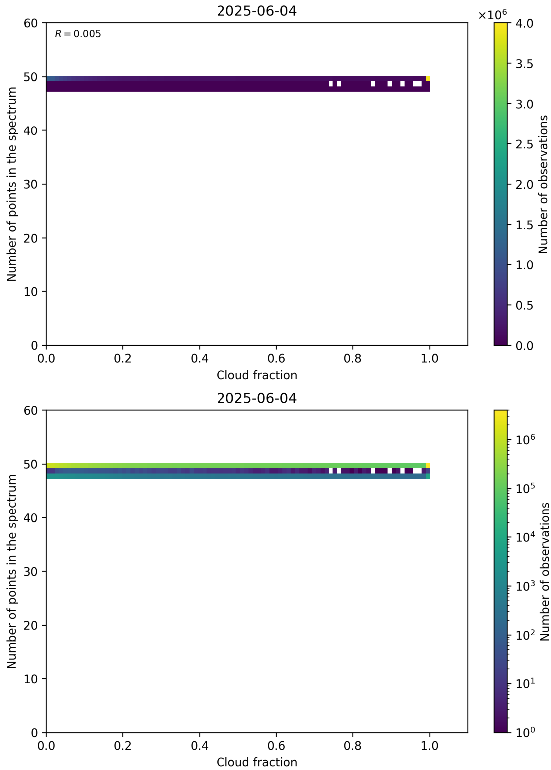
Figure 74: Scatter density plot of “Cloud fraction” against “Number of points in the spectrum” for 2025-06-03 to 2025-06-05.
