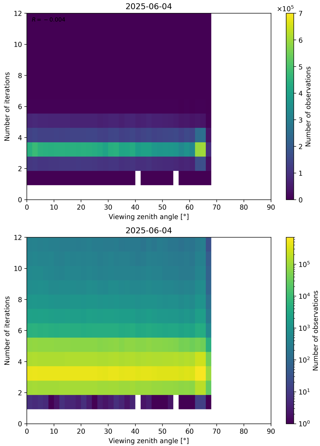
Figure 124: Scatter density plot of “Viewing zenith angle” against “Number of iterations” for 2025-06-03 to 2025-06-05.
