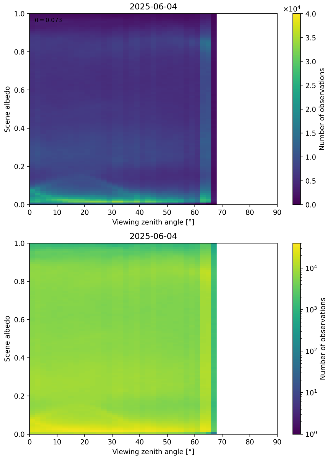
Figure 126: Scatter density plot of “Viewing zenith angle” against “Scene albedo” for 2025-06-03 to 2025-06-05.
