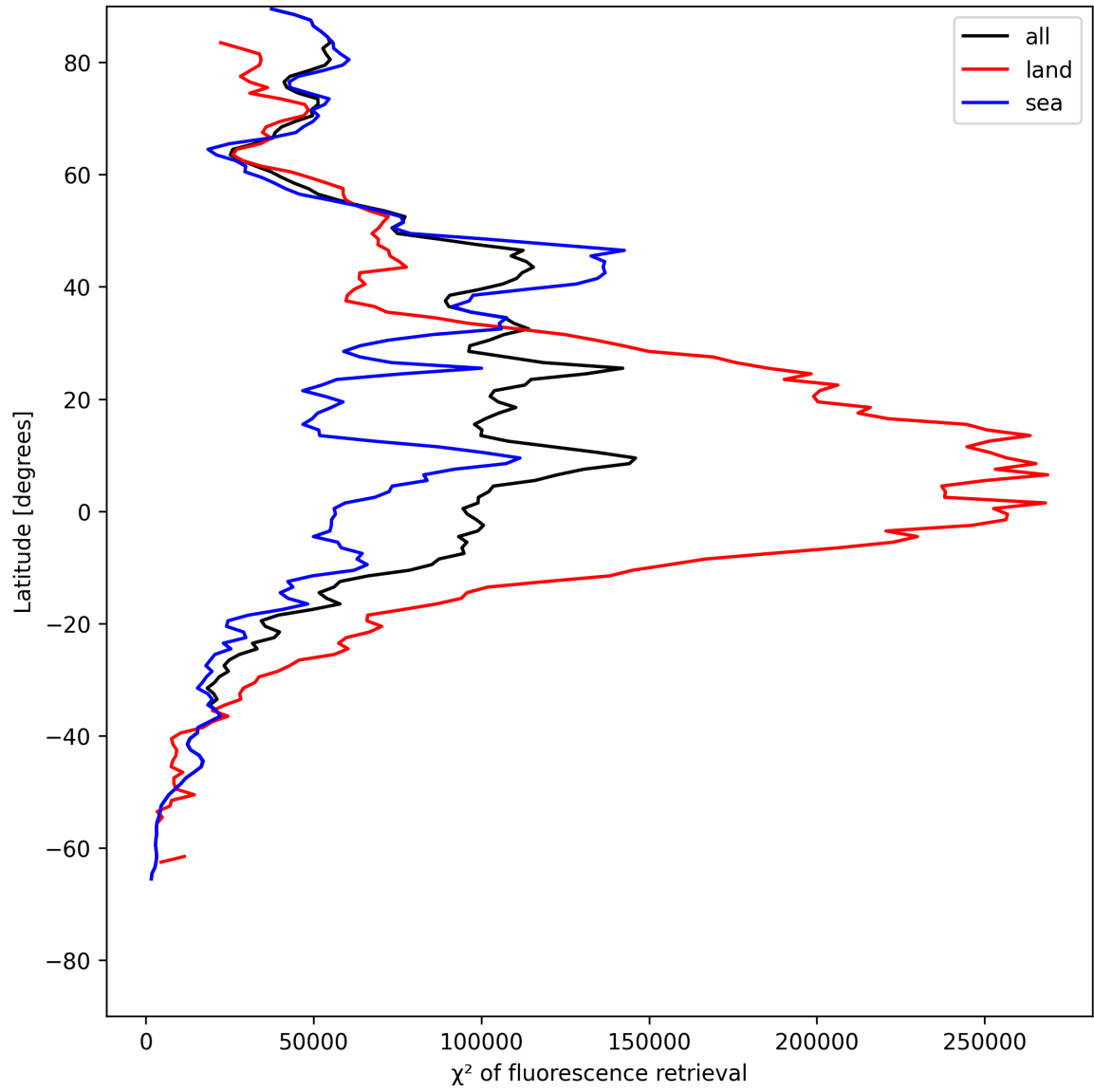
Figure 25: Zonal average of “ \chi^2 of fluorescence retrieval” for 2025-06-03 to 2025-06-05.
