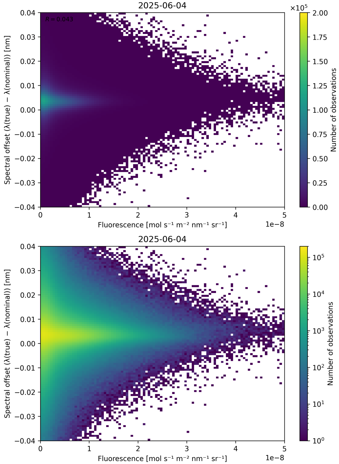
Figure 87: Scatter density plot of “Fluorescence” against “Spectral offset ( \lambda_{\text{true}} - \lambda_{\text{nominal}} )” for 2025-06-03 to 2025-06-05.
