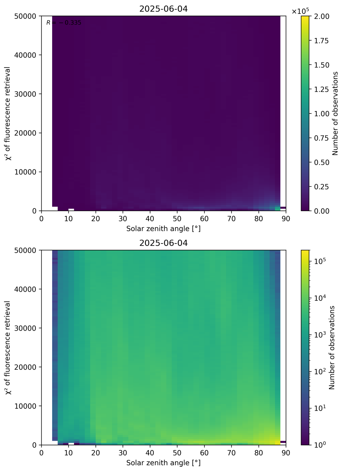
Figure 109: Scatter density plot of “Solar zenith angle” against “ \chi^2 of fluorescence retrieval” for 2025-06-03 to 2025-06-05.
