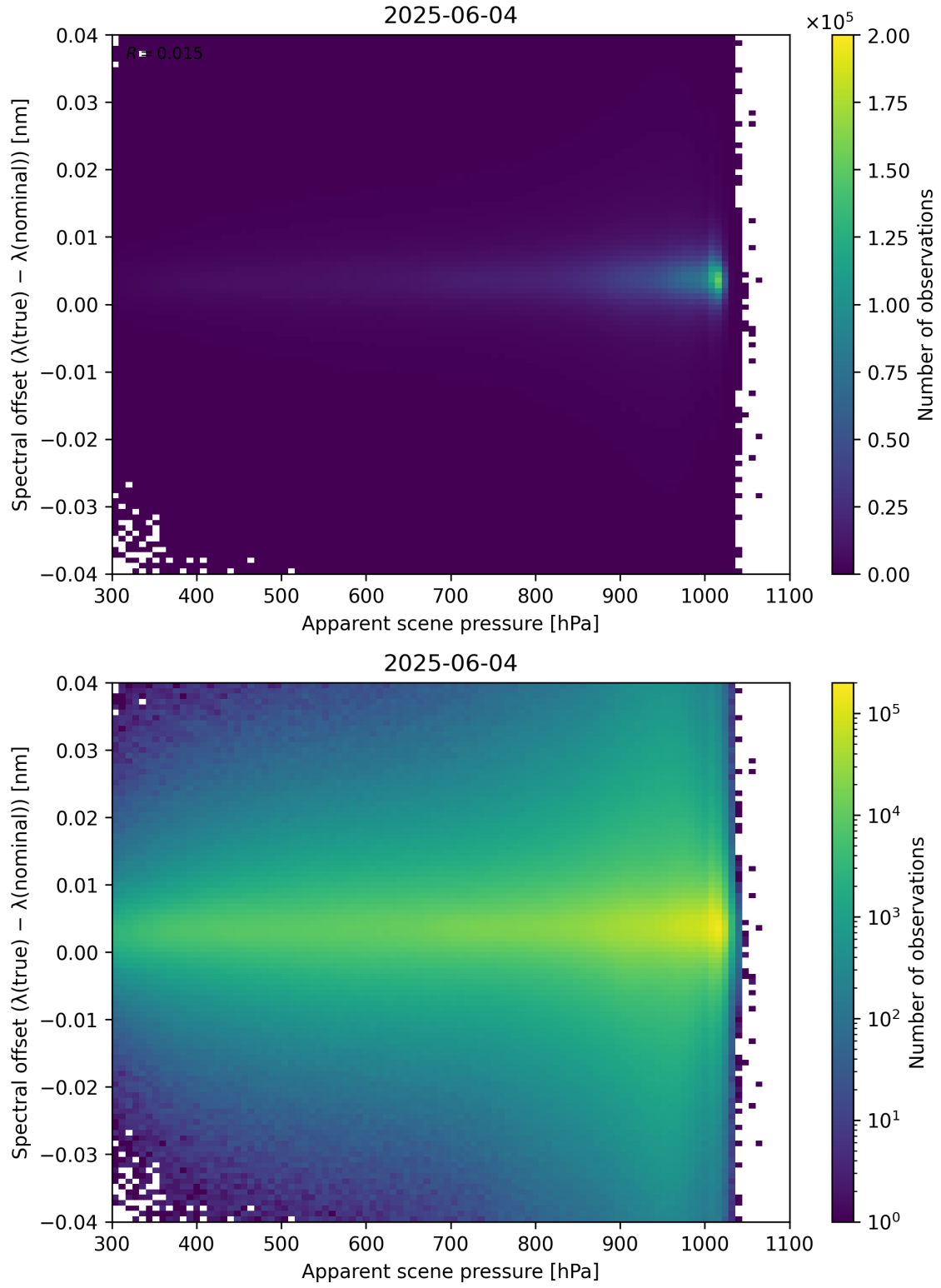
Figure 67: Scatter density plot of “Apparent scene pressure” against “Spectral offset ( \lambda_{\text{true}} - \lambda_{\text{nominal}} )” for 2025-06-03 to 2025-06-05.
