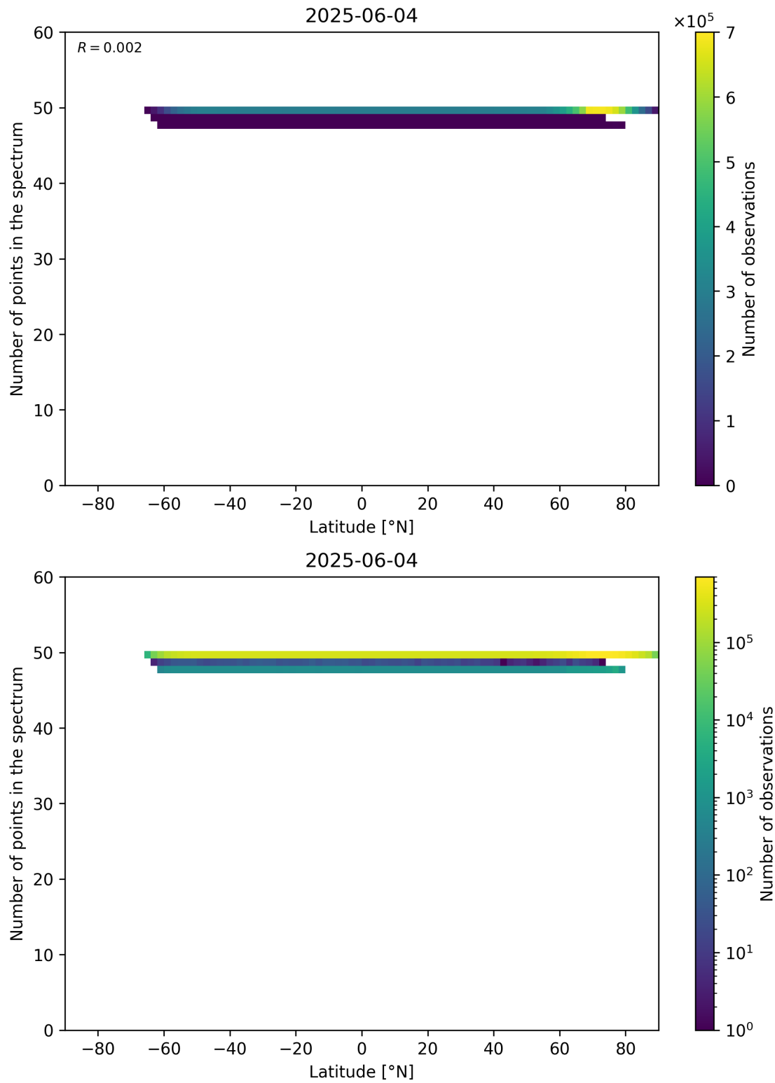
Figure 94: Scatter density plot of “Latitude” against “Number of points in the spectrum” for 2025-06-03 to 2025-06-05.
