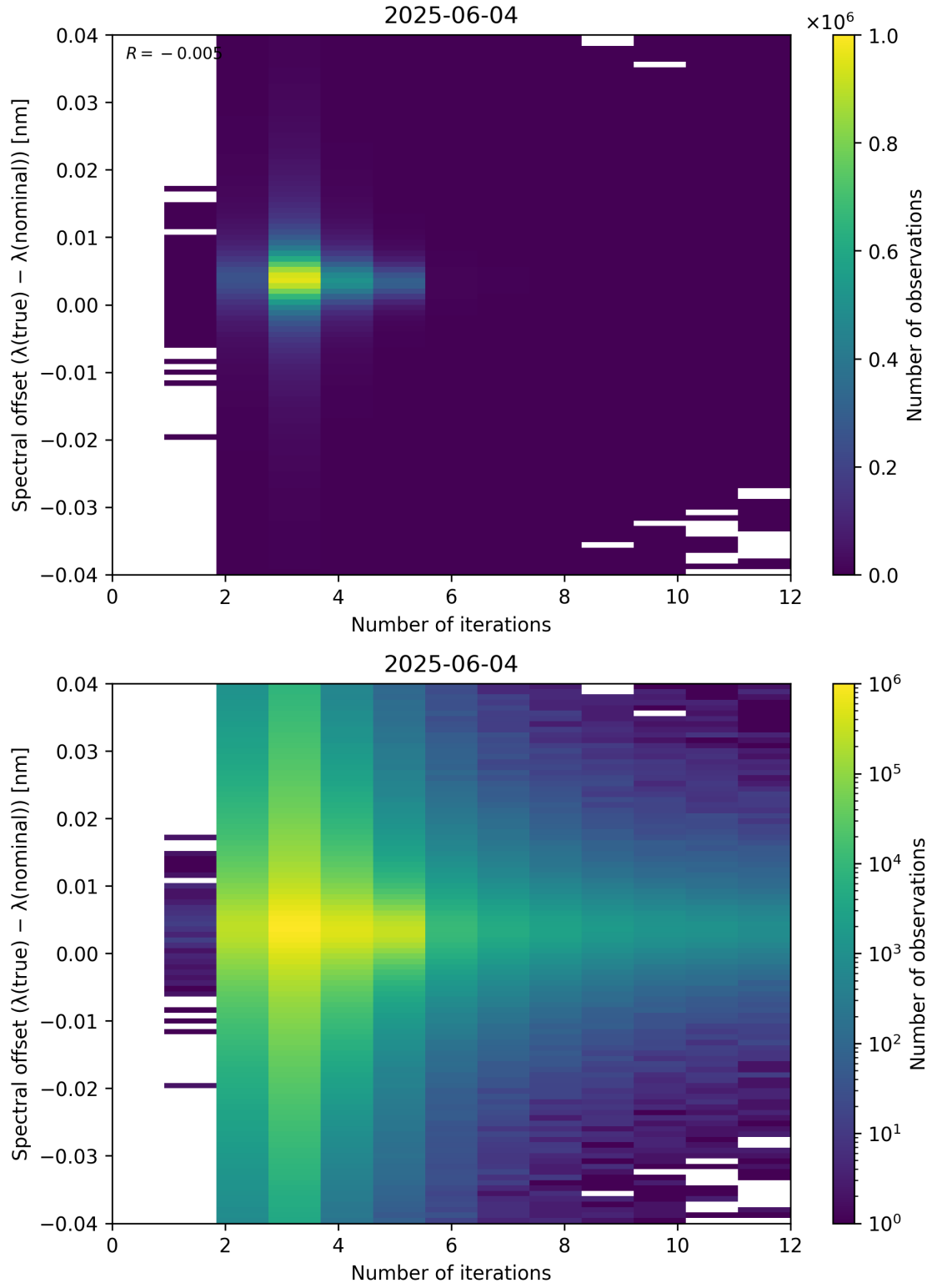
Figure 100: Scatter density plot of “Number of iterations” against “Spectral offset ( \lambda_{\text{true}} - \lambda_{\text{nominal}} )” for 2025-06-03 to 2025-06-05.
