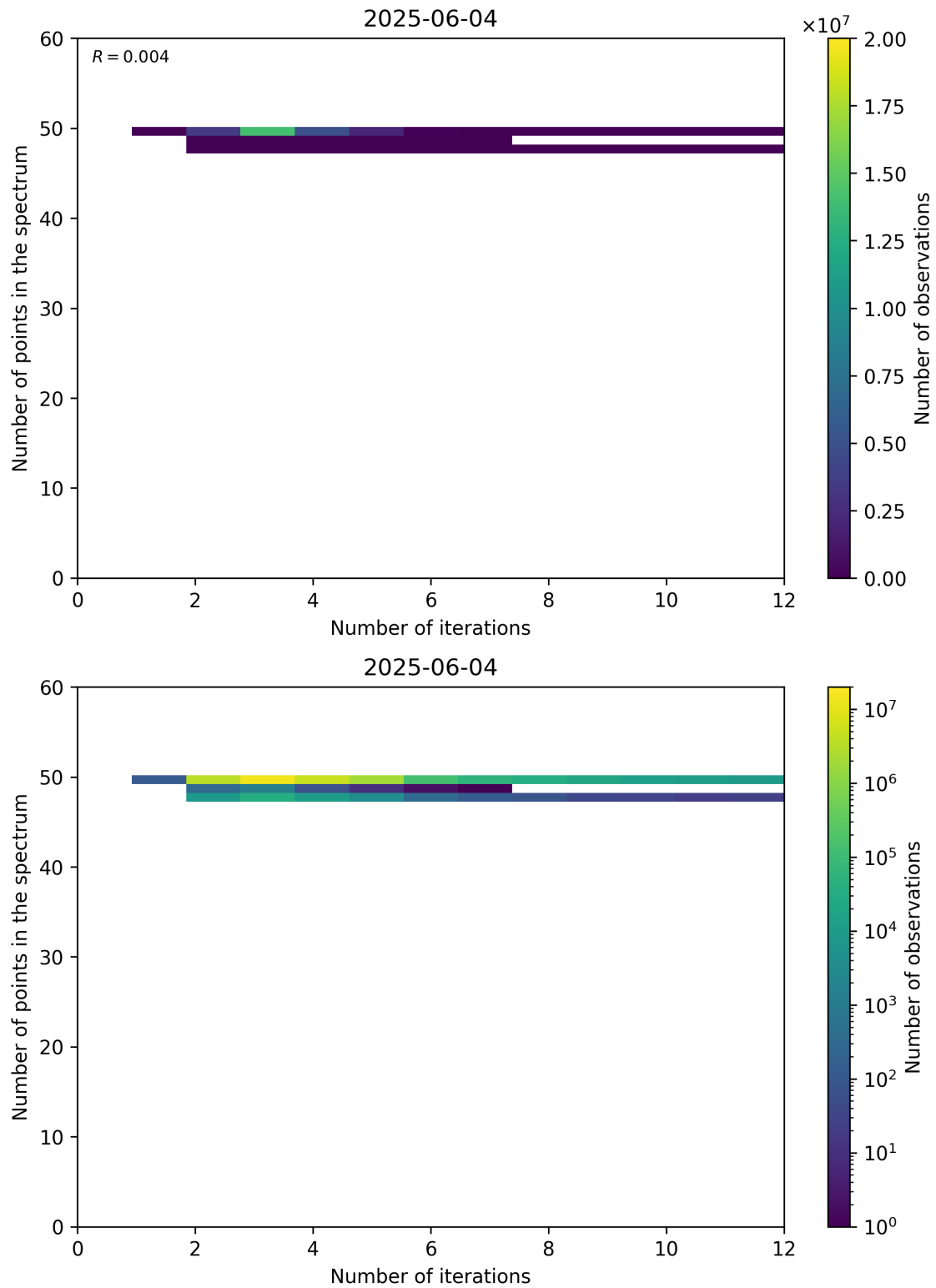
Figure 99: Scatter density plot of “Number of iterations” against “Number of points in the spectrum” for 2025-06-03 to 2025-06-05.
