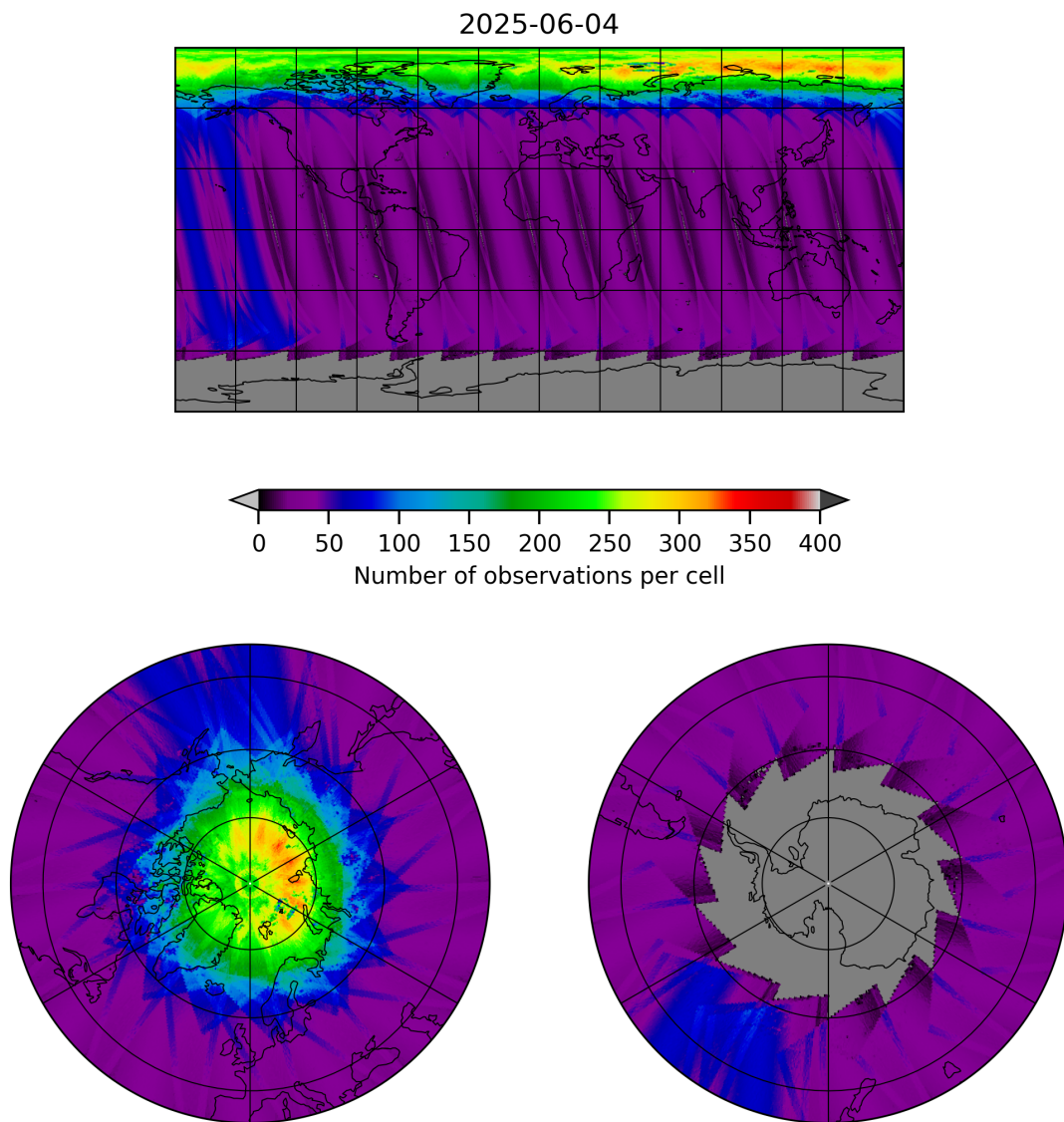
Figure 11: Map of the number of observations for 2025-06-03 to 2025-06-05
