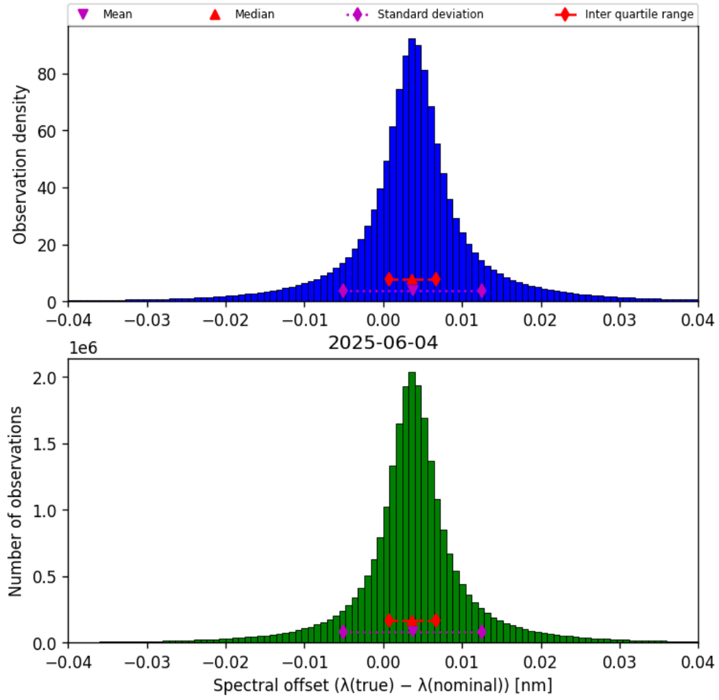
Figure 45: Histogram of “Spectral offset ( \lambda_{\text{true}} - \lambda_{\text{nominal}} )” for 2025-06-03 to 2025-06-05
