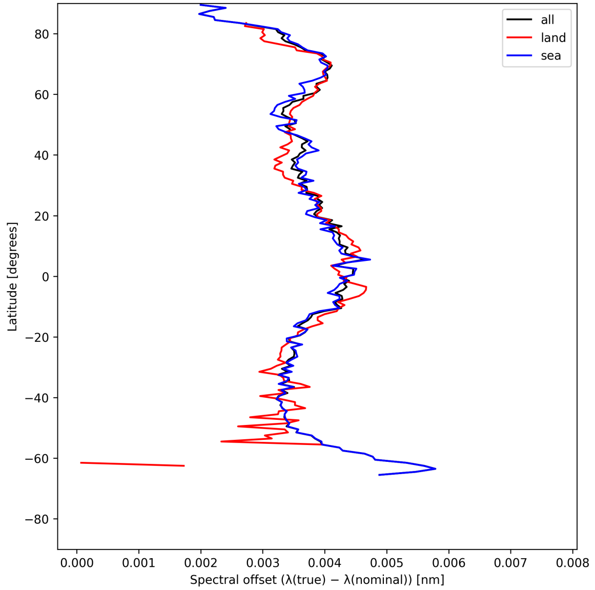
Figure 28: Zonal average of “Spectral offset ( \lambda_{\text{true}} - \lambda_{\text{nominal}} )” for 2025-06-03 to 2025-06-05.
