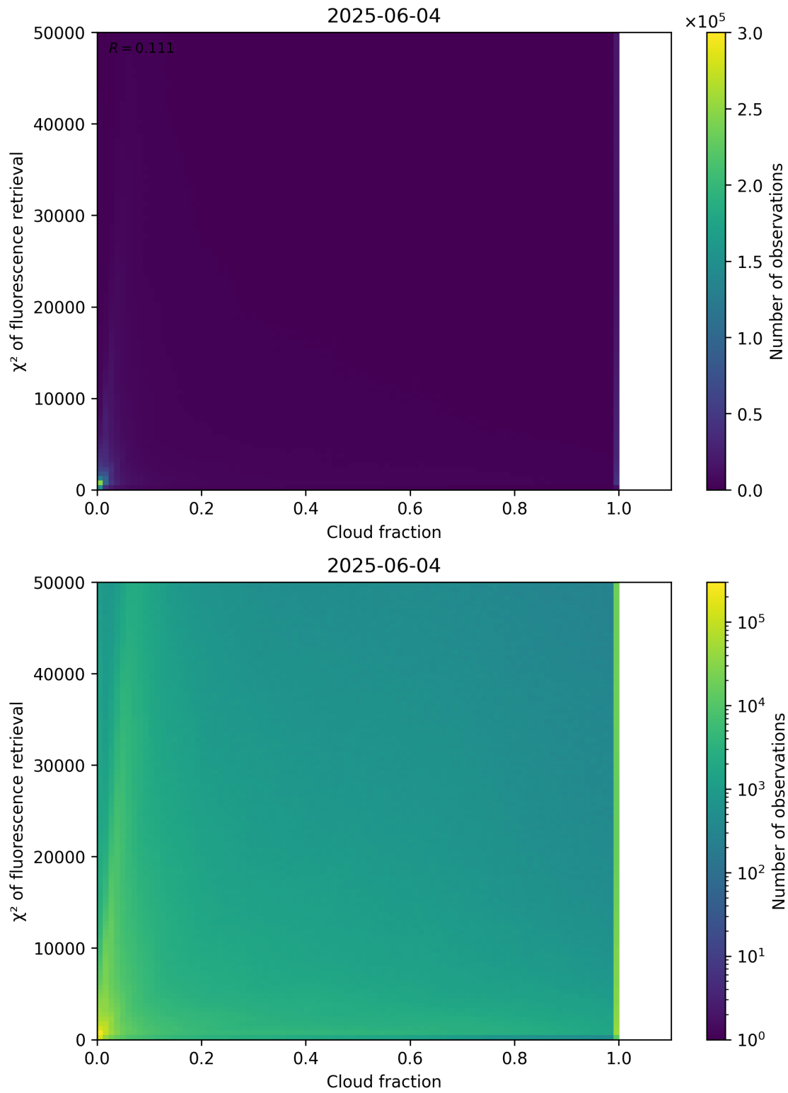
Figure 71: Scatter density plot of “Cloud fraction” against “ \chi^2 of fluorescence retrieval” for 2025-06-03 to 2025-06-05.
