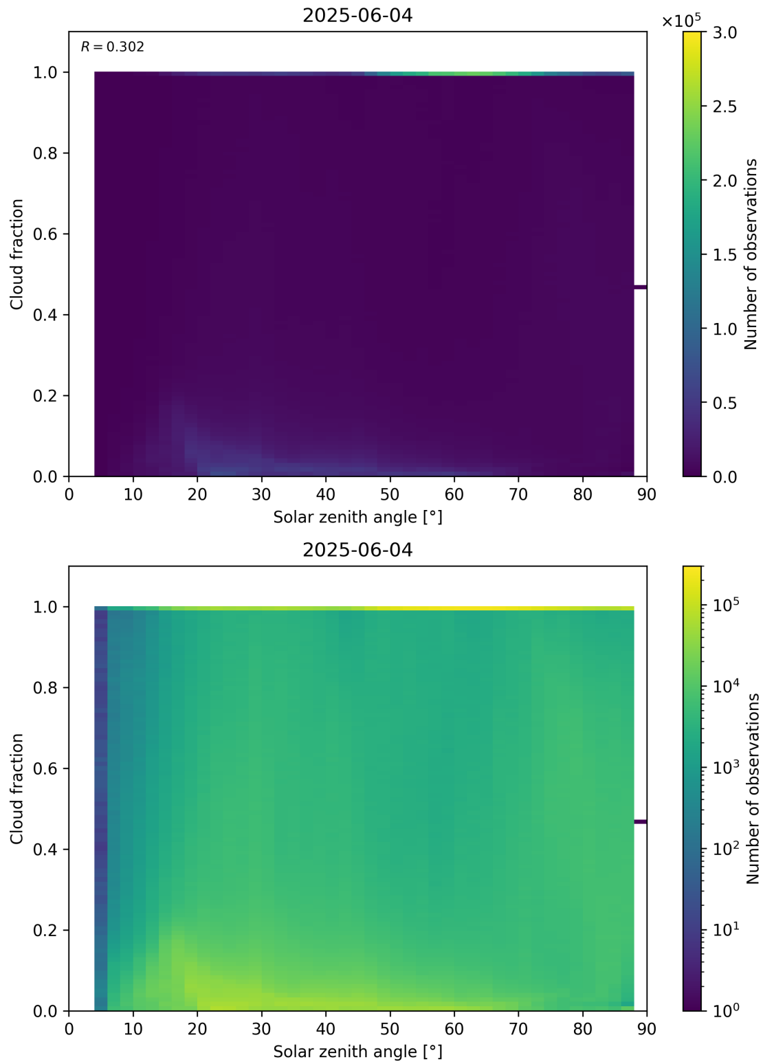
Figure 110: Scatter density plot of “Solar zenith angle” against “Cloud fraction” for 2025-06-03 to 2025-06-05.
