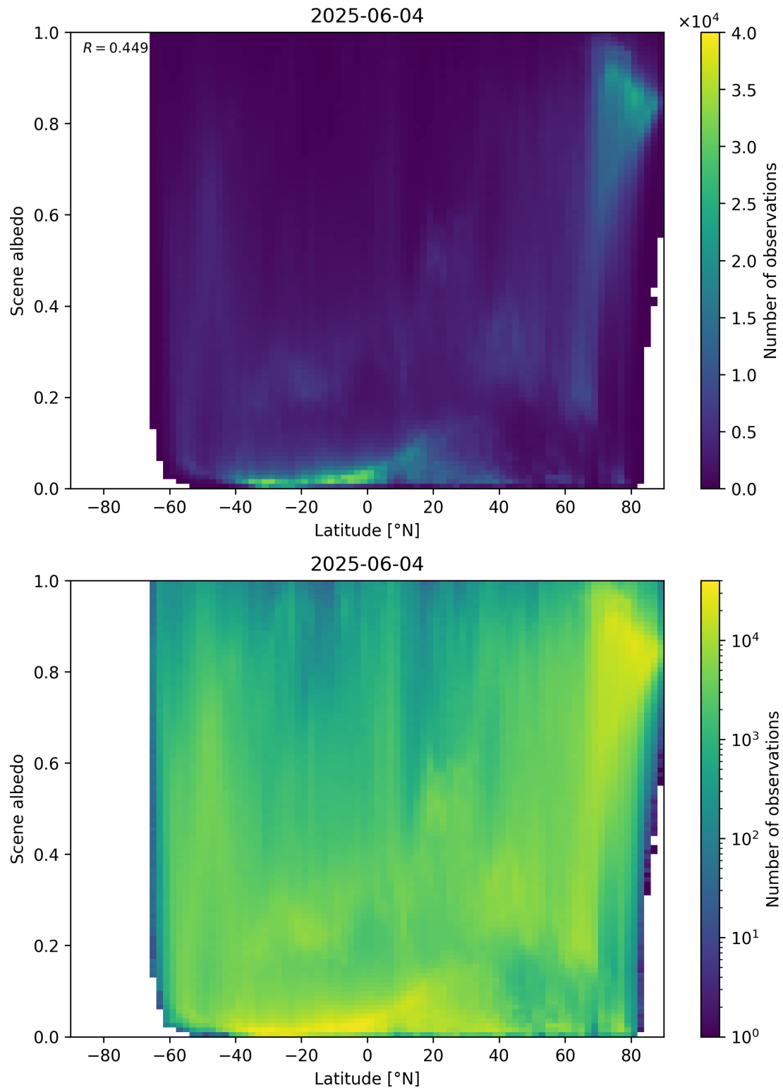
Figure 95: Scatter density plot of “Latitude” against “Scene albedo” for 2025-06-03 to 2025-06-05.
