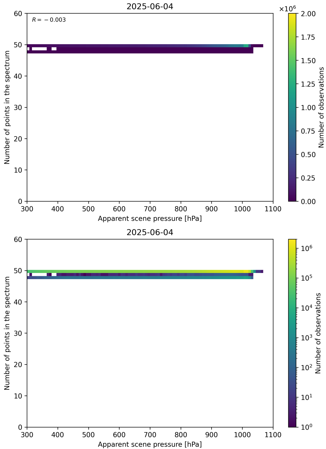
Figure 66: Scatter density plot of “Apparent scene pressure” against “Number of points in the spectrum” for 2025-06-03 to 2025-06-05.
