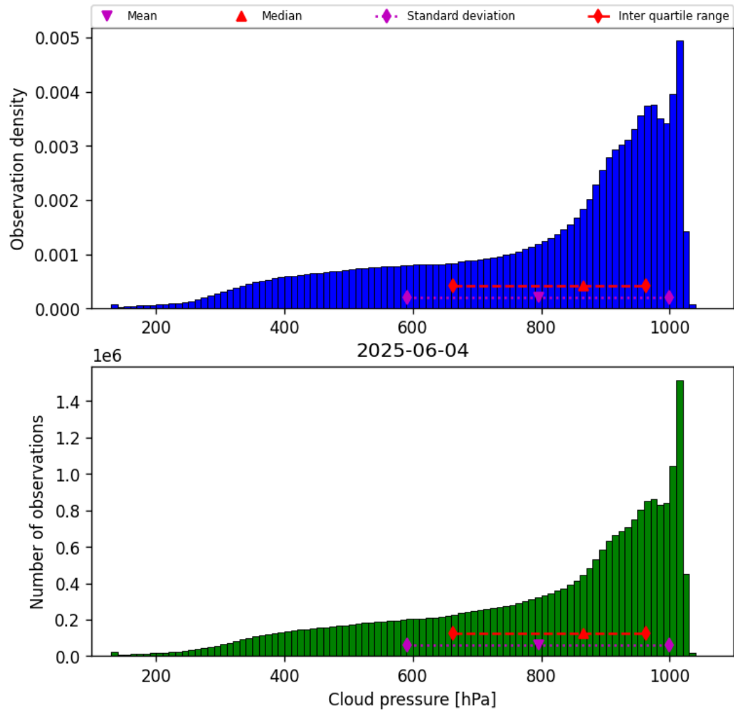
Figure 30: Histogram of “Cloud pressure” for 2025-06-03 to 2025-06-05
