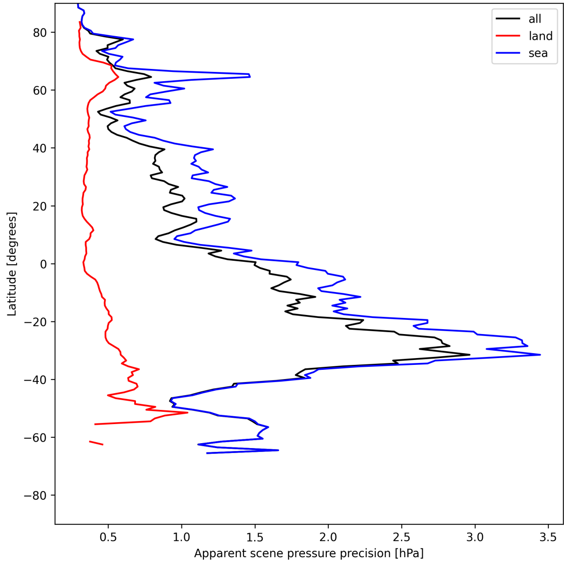
Figure 20: Zonal average of “Apparent scene pressure precision” for 2025-06-03 to 2025-06-05.
