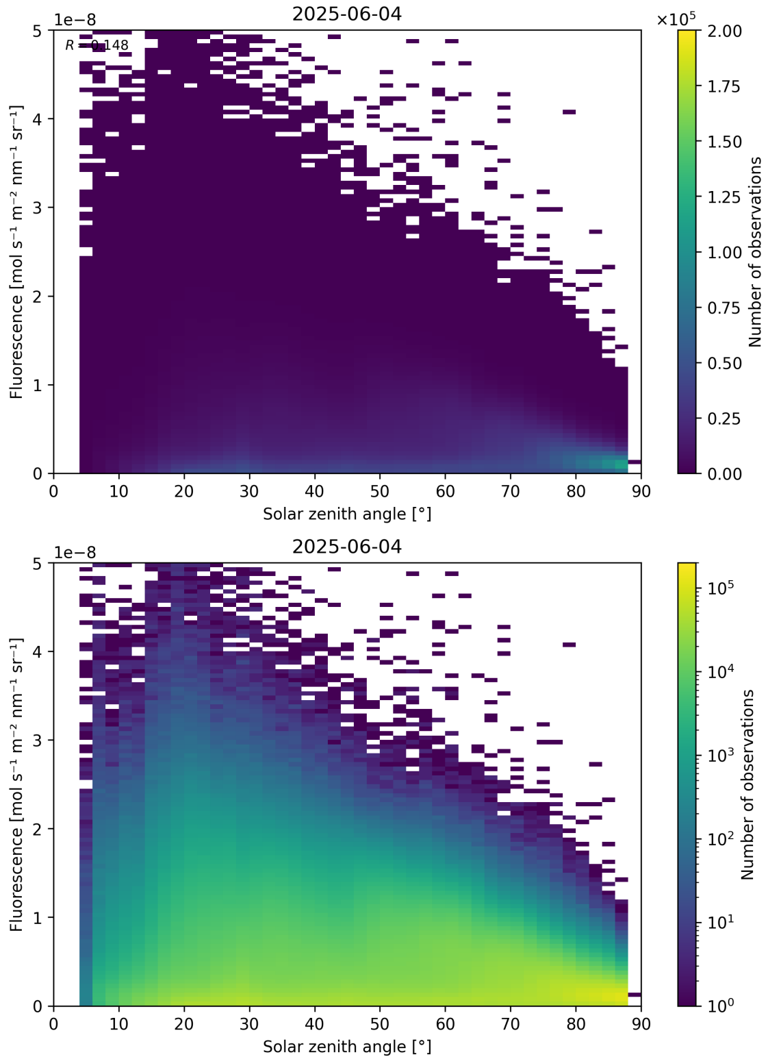
Figure 112: Scatter density plot of “Solar zenith angle” against “Fluorescence” for 2025-06-03 to 2025-06-05.
