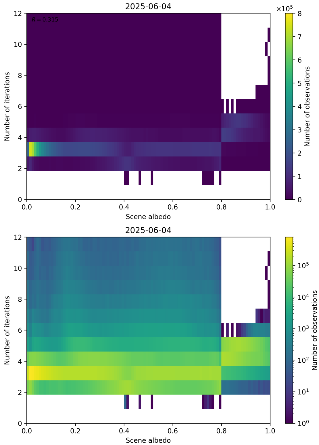
Figure 105: Scatter density plot of “Scene albedo” against “Number of iterations” for 2025-06-03 to 2025-06-05.
