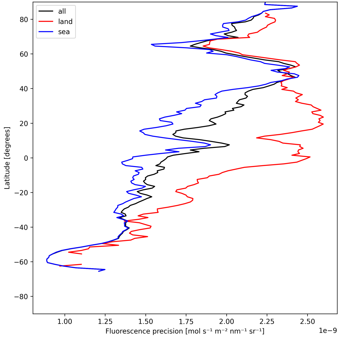
Figure 24: Zonal average of “Fluorescence precision” for 2025-06-03 to 2025-06-05.
