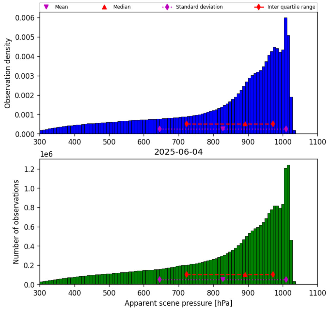
Figure 36: Histogram of “Apparent scene pressure” for 2025-06-03 to 2025-06-05
