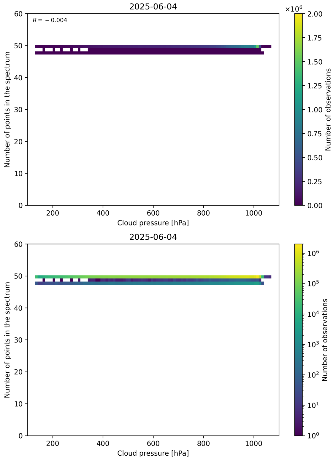
Figure 82: Scatter density plot of “Cloud pressure” against “Number of points in the spectrum” for 2025-06-03 to 2025-06-05.
