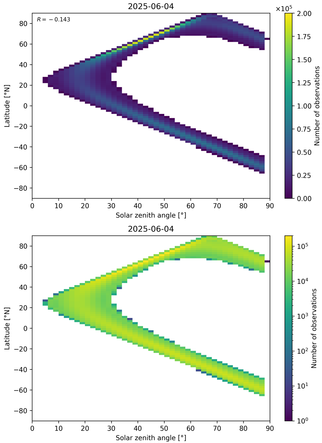
Figure 113: Scatter density plot of “Solar zenith angle” against “Latitude” for 2025-06-03 to 2025-06-05.
