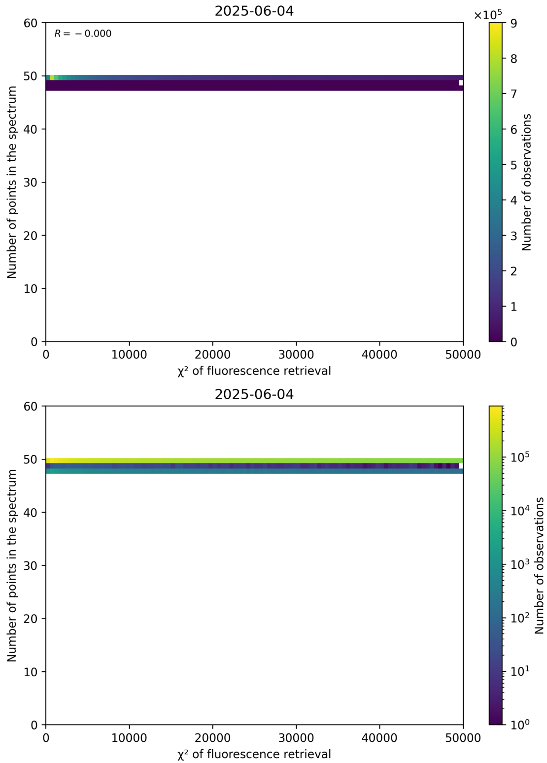
Figure 68: Scatter density plot of “ \chi^2 of fluorescence retrieval” against “Number of points in the spectrum” for 2025-06-03 to 2025-06-05.
