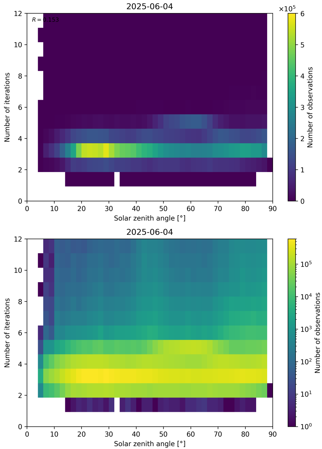
Figure 114: Scatter density plot of “Solar zenith angle” against “Number of iterations” for 2025-06-03 to 2025-06-05.
