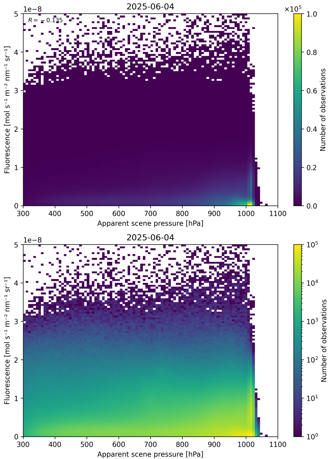
Figure 64: Scatter density plot of “Apparent scene pressure” against “Fluorescence” for 2025-06-03 to 2025-06-05.
