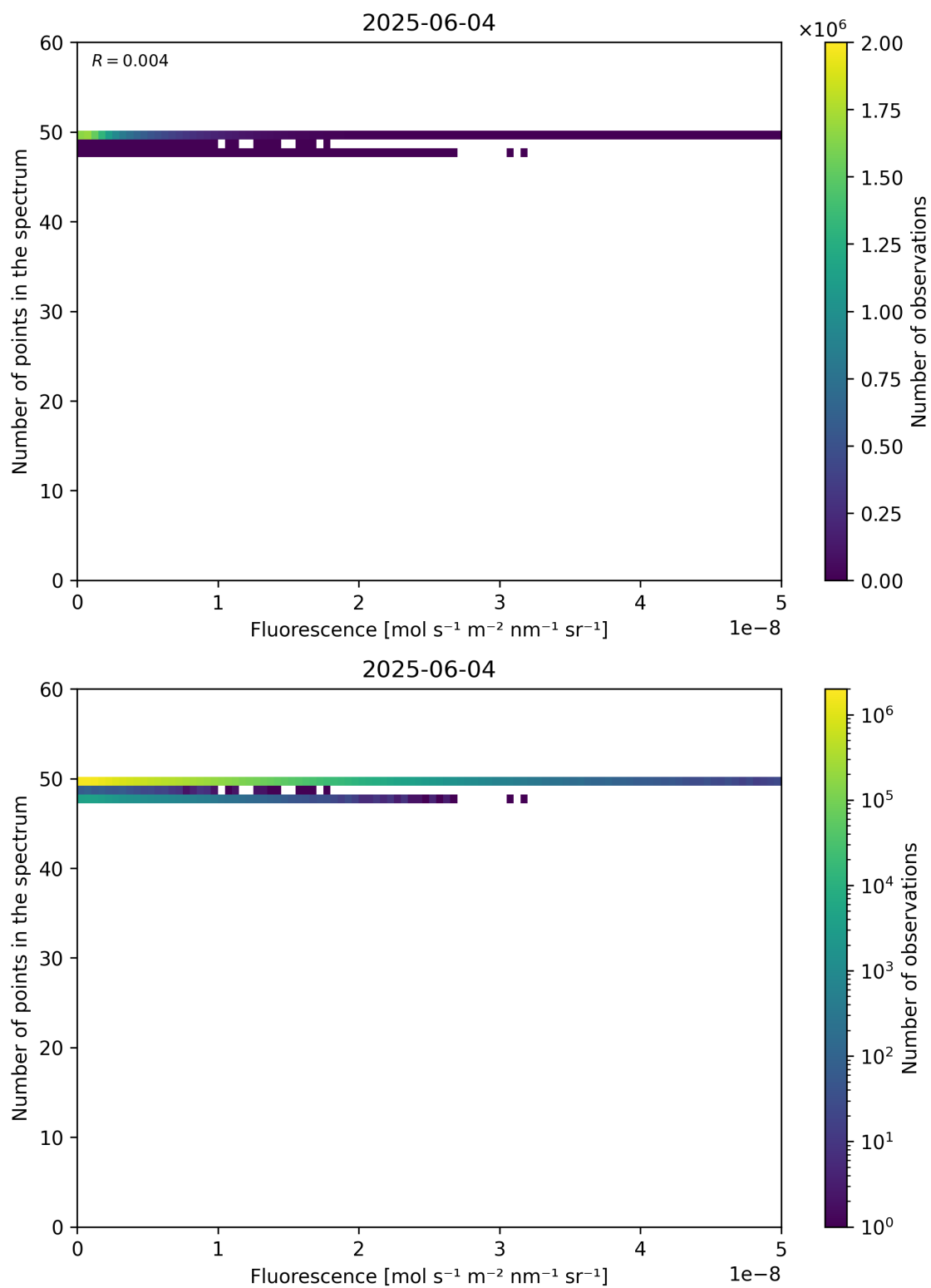
Figure 86: Scatter density plot of “Fluorescence” against “Number of points in the spectrum” for 2025-06-03 to 2025-06-05.
