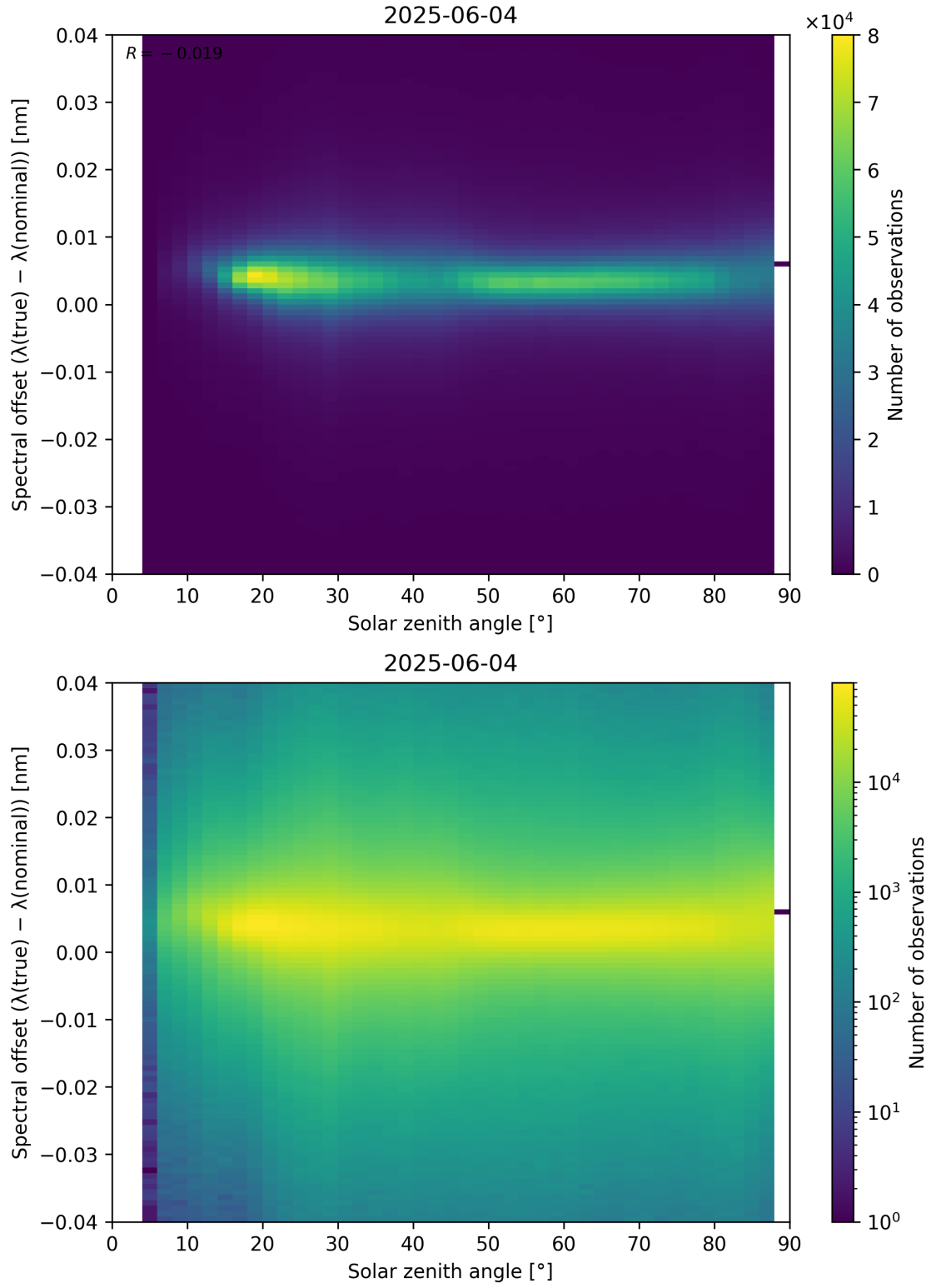
Figure 117: Scatter density plot of “Solar zenith angle” against “Spectral offset ( \lambda_{\text{true}} - \lambda_{\text{nominal}} )” for 2025-06-03 to 2025-06-05.
