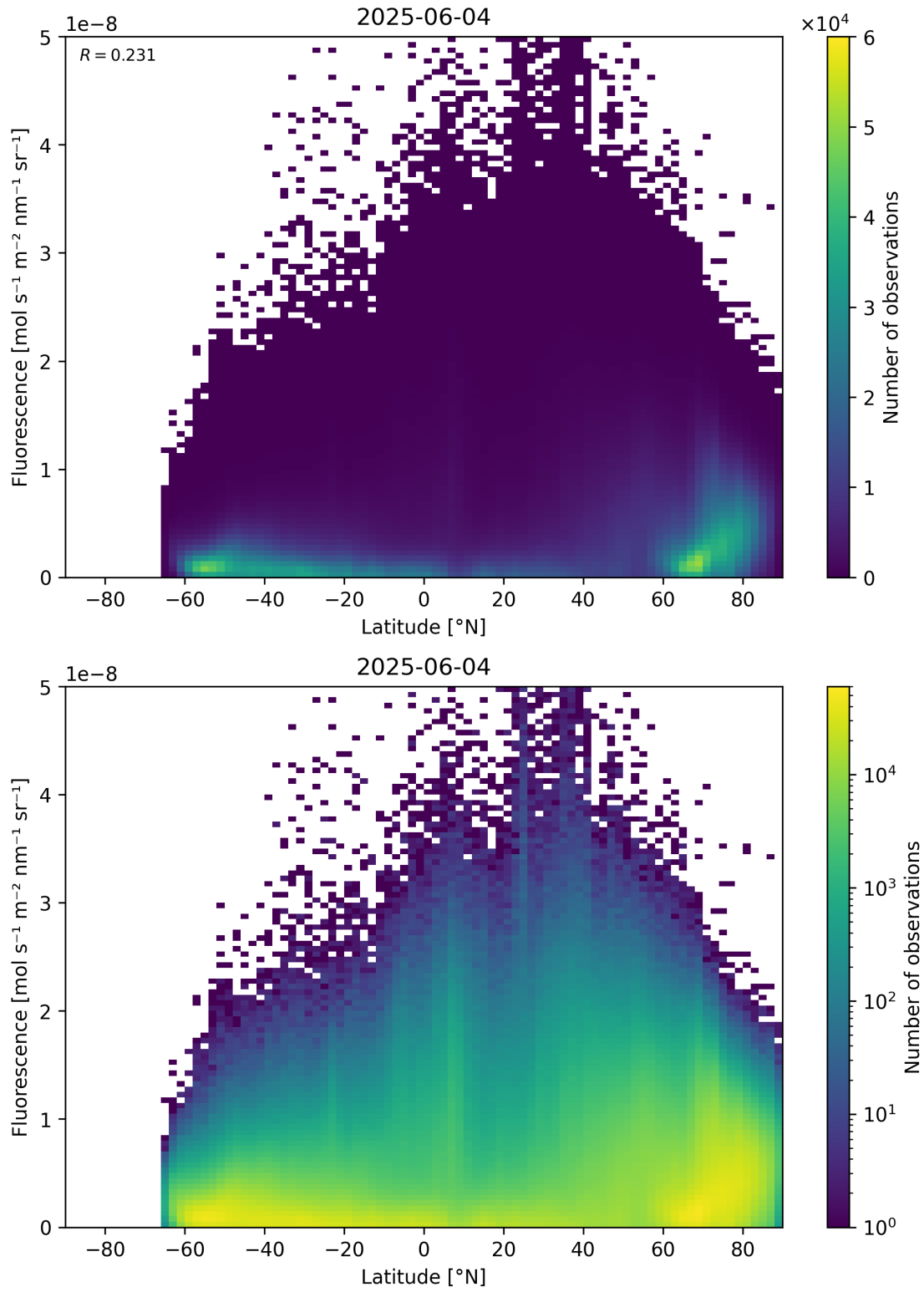
Figure 92: Scatter density plot of “Latitude” against “Fluorescence” for 2025-06-03 to 2025-06-05.
