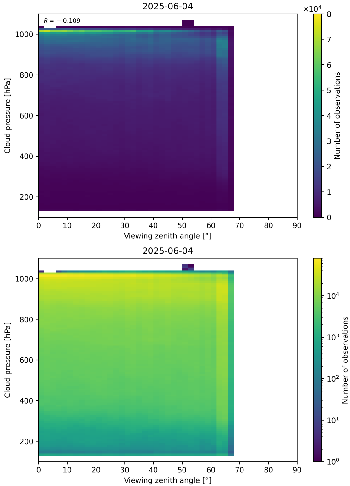
Figure 121: Scatter density plot of “Viewing zenith angle” against “Cloud pressure” for 2025-06-03 to 2025-06-05.
