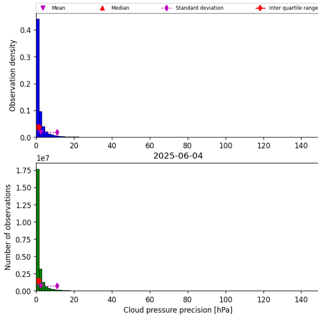
Figure 31: Histogram of “Cloud pressure precision” for 2025-06-03 to 2025-06-05
