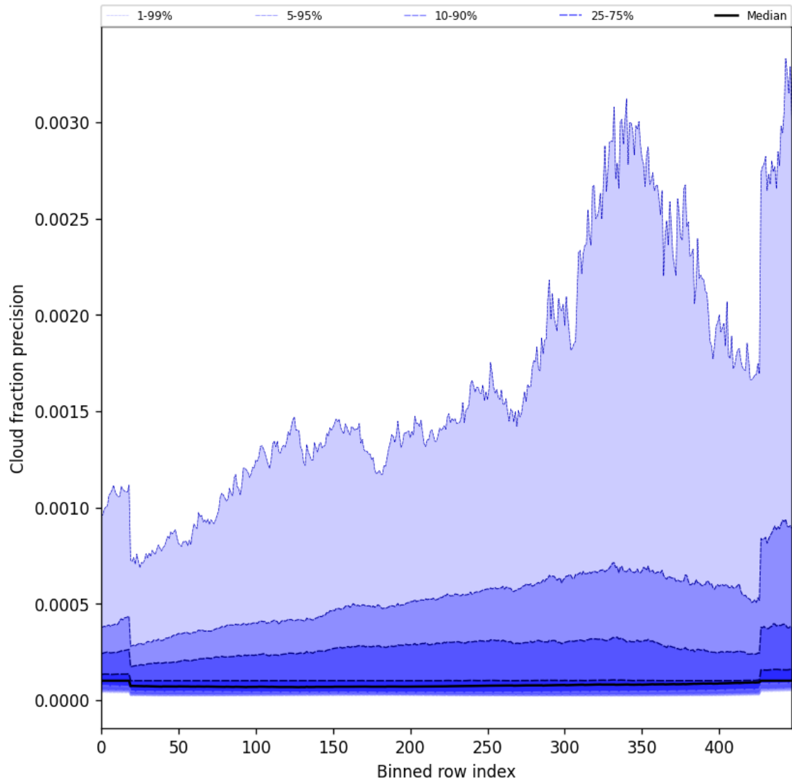
Figure 50: Along track statistics of “Cloud fraction precision” for 2025-06-03 to 2025-06-05
