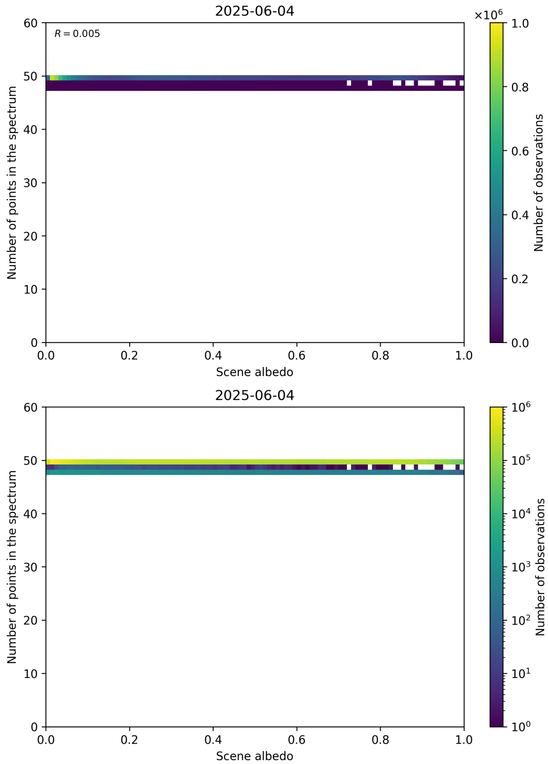
Figure 106: Scatter density plot of “Scene albedo” against “Number of points in the spectrum” for 2025-06-03 to 2025-06-05.
