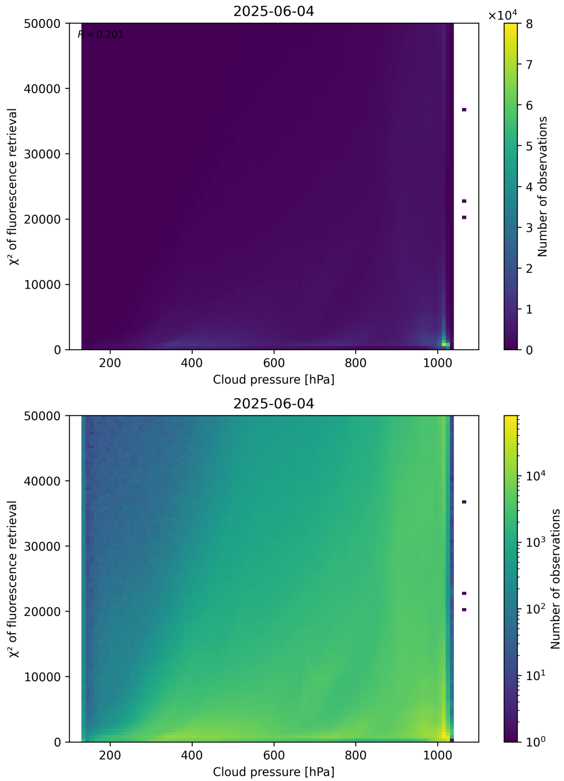
Figure 78: Scatter density plot of “Cloud pressure” against “ \chi^2 of fluorescence retrieval” for 2025-06-03 to 2025-06-05.
