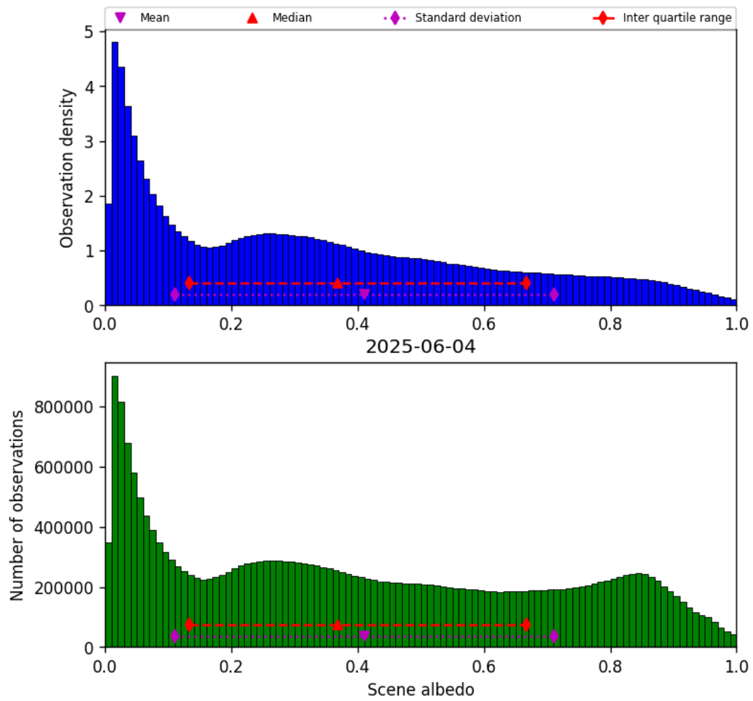
Figure 34: Histogram of “Scene albedo” for 2025-06-03 to 2025-06-05
