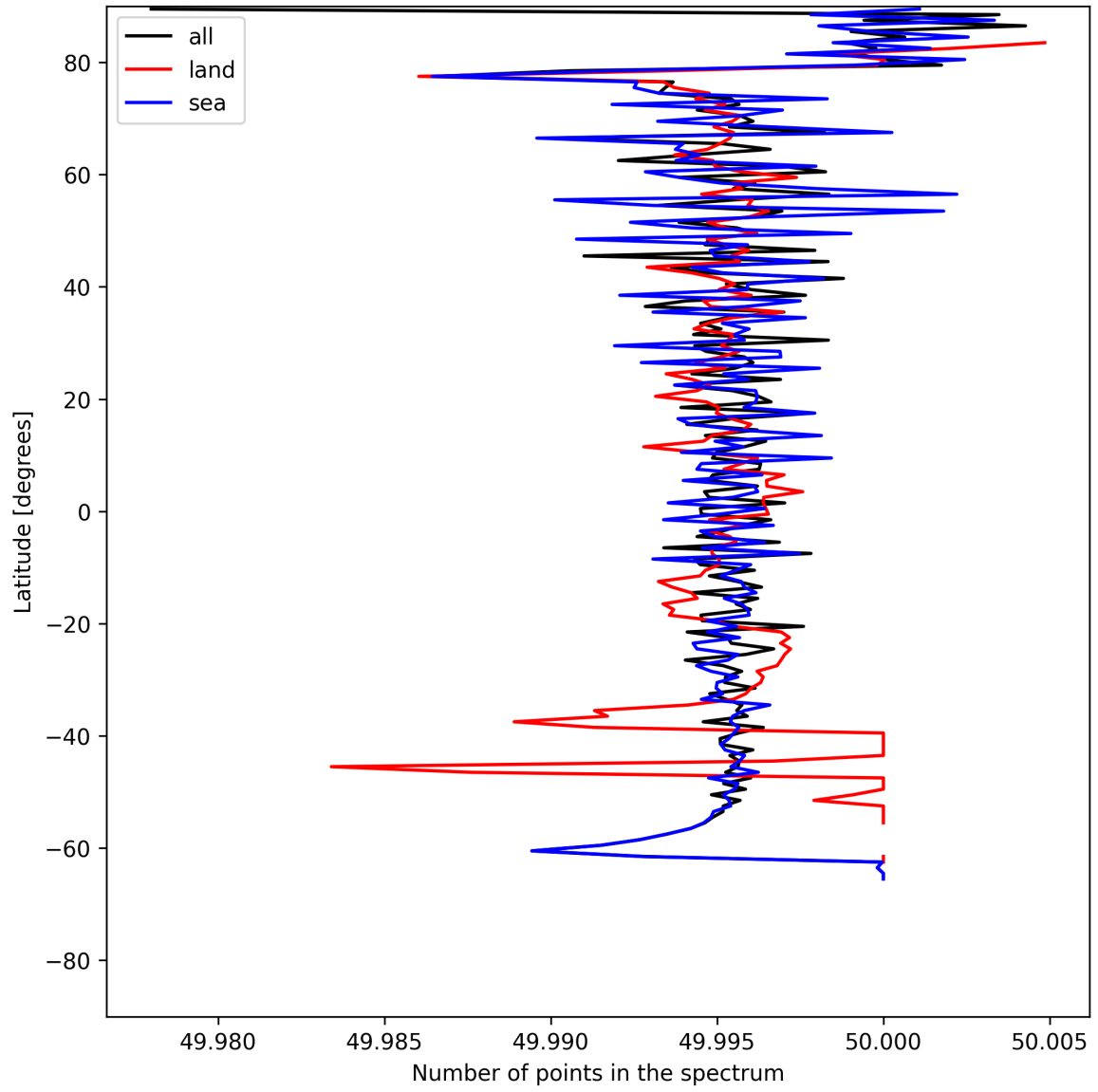
Figure 27: Zonal average of “Number of points in the spectrum” for 2025-06-03 to 2025-06-05.
