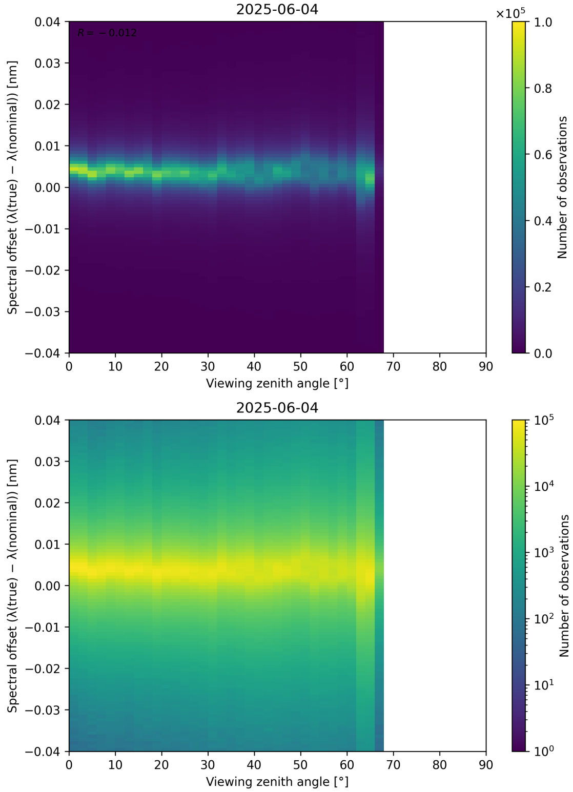
Figure 128: Scatter density plot of “Viewing zenith angle” against “Spectral offset ( \lambda_{\text{true}} - \lambda_{\text{nominal}} )” for 2025-06-03 to 2025-06-05.
