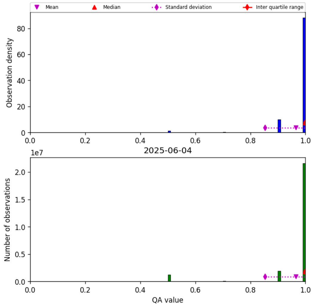
Figure 29: Histogram of “QA value” for 2025-06-03 to 2025-06-05
