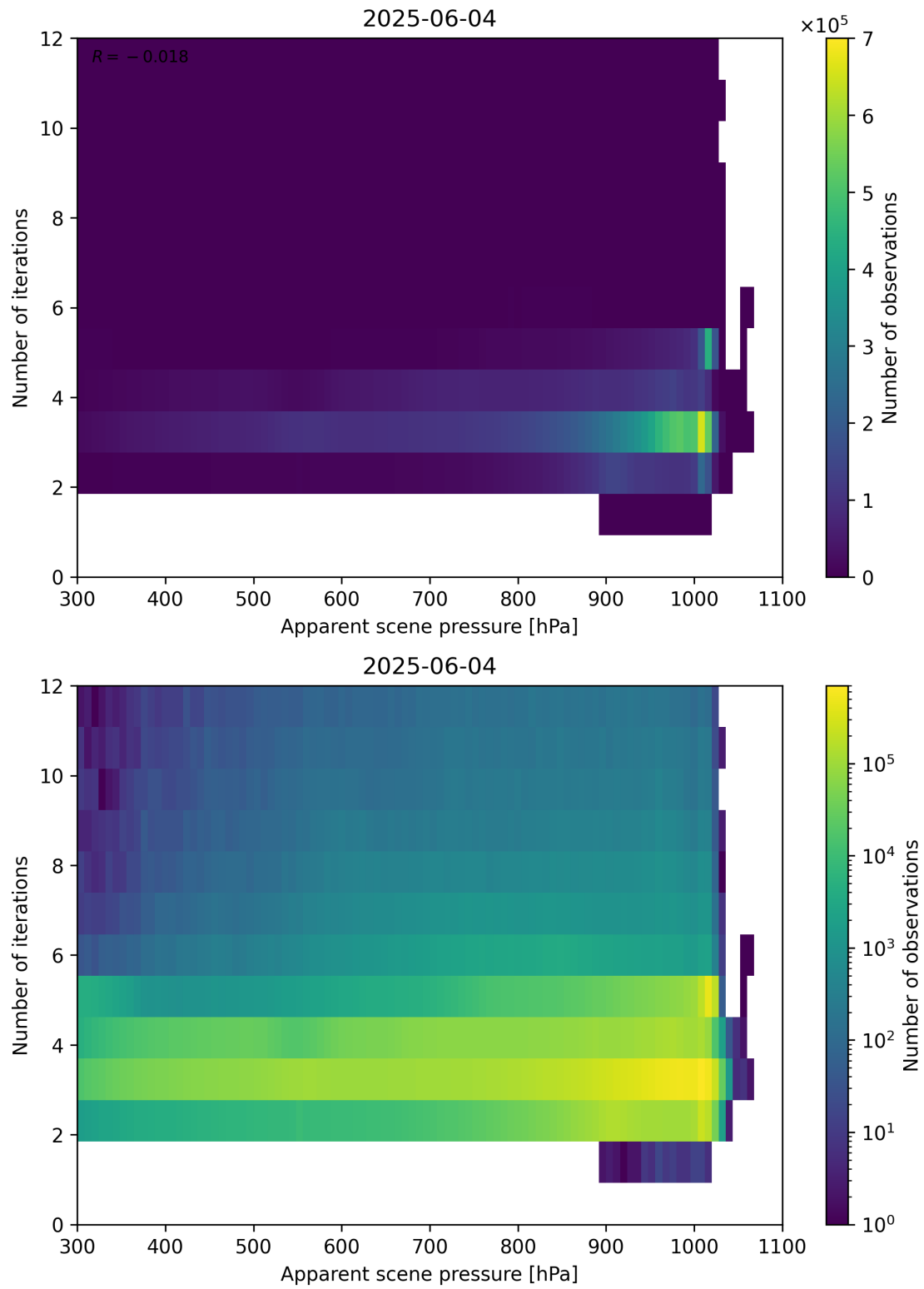
Figure 65: Scatter density plot of “Apparent scene pressure” against “Number of iterations” for 2025-06-03 to 2025-06-05.
