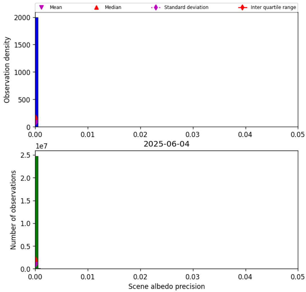
Figure 35: Histogram of “Scene albedo precision” for 2025-06-03 to 2025-06-05
