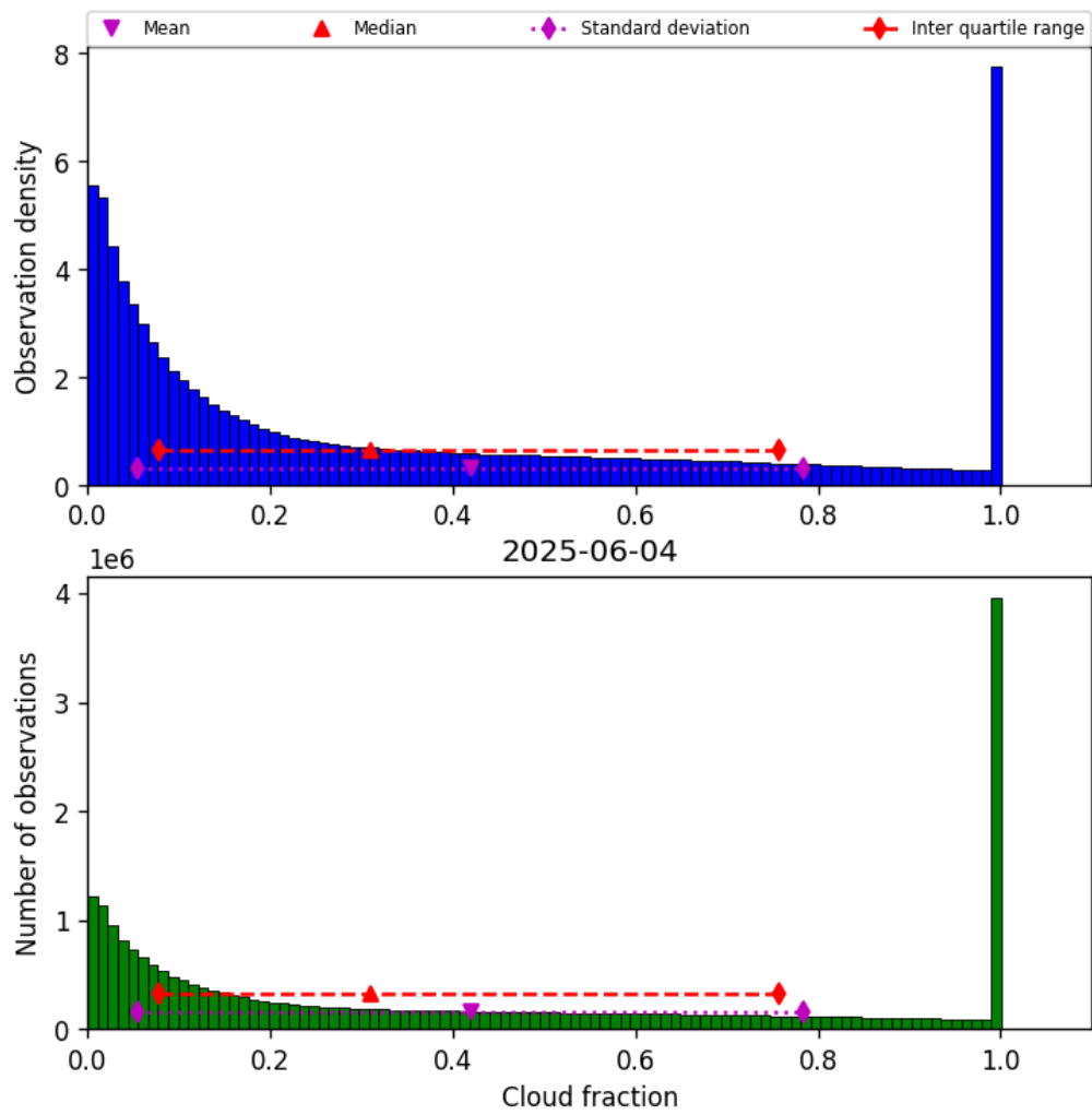
Figure 32: Histogram of “Cloud fraction” for 2025-06-03 to 2025-06-05
