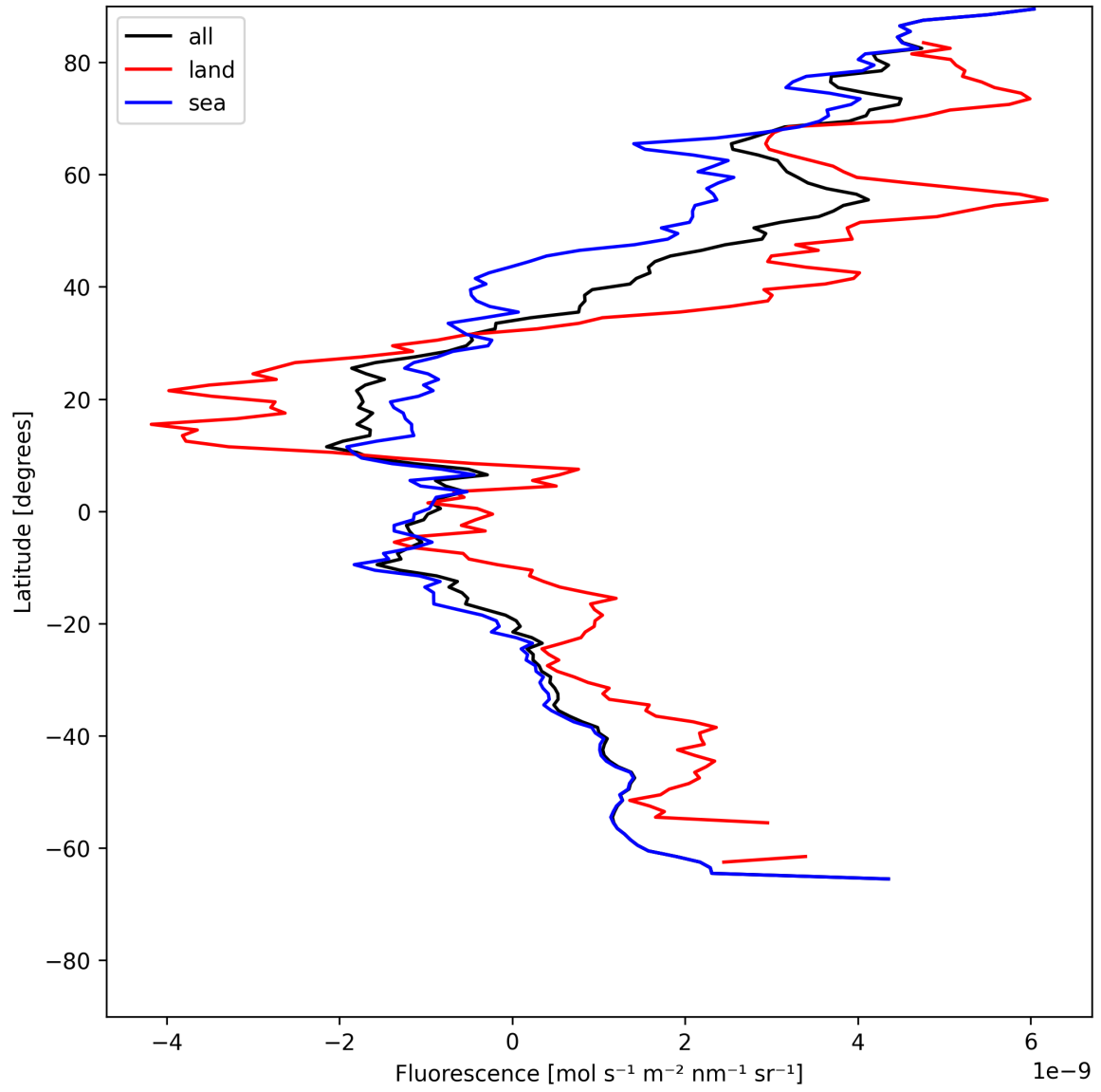
Figure 23: Zonal average of “Fluorescence” for 2025-06-03 to 2025-06-05.
