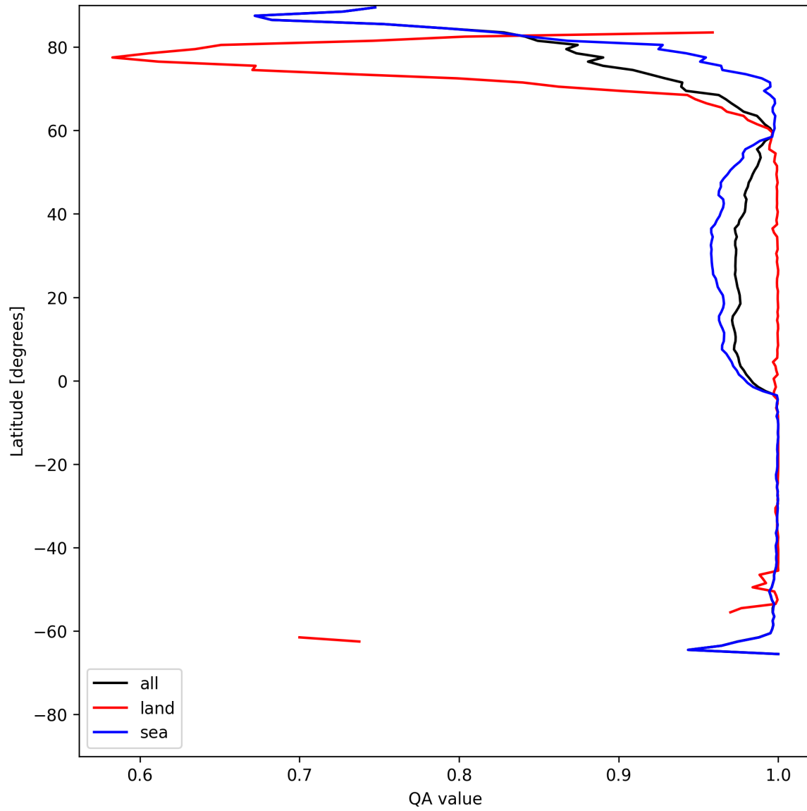
Figure 12: Zonal average of “QA value” for 2025-06-03 to 2025-06-05.
