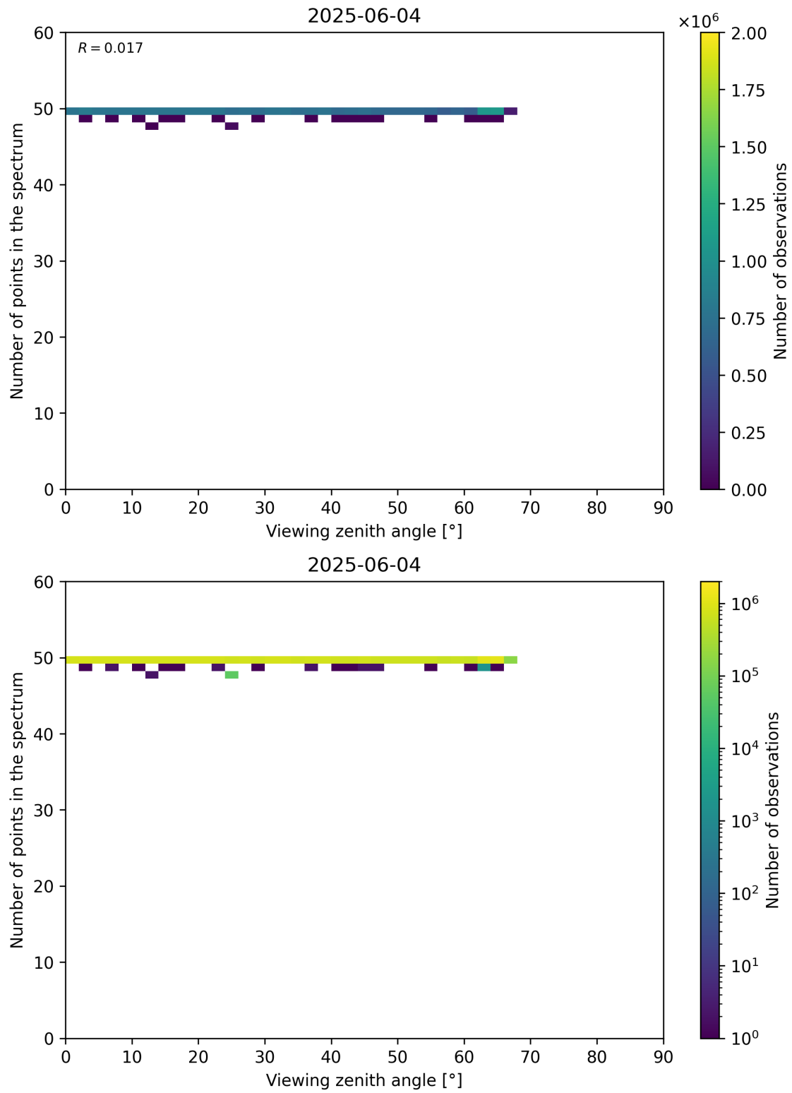
Figure 125: Scatter density plot of “Viewing zenith angle” against “Number of points in the spectrum” for 2025-06-03 to 2025-06-05.
