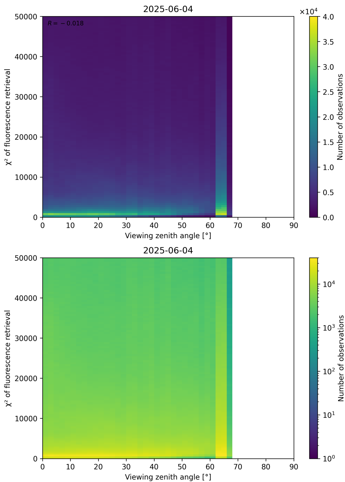
Figure 119: Scatter density plot of “Viewing zenith angle” against “ \chi^2 of fluorescence retrieval” for 2025-06-03 to 2025-06-05.
