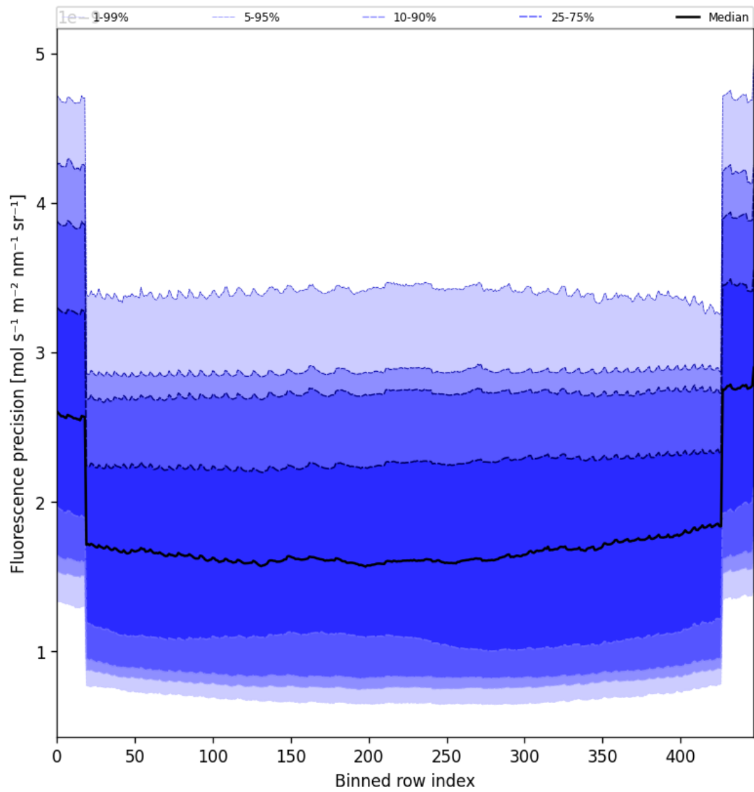
Figure 58: Along track statistics of “Fluorescence precision” for 2025-06-03 to 2025-06-05
