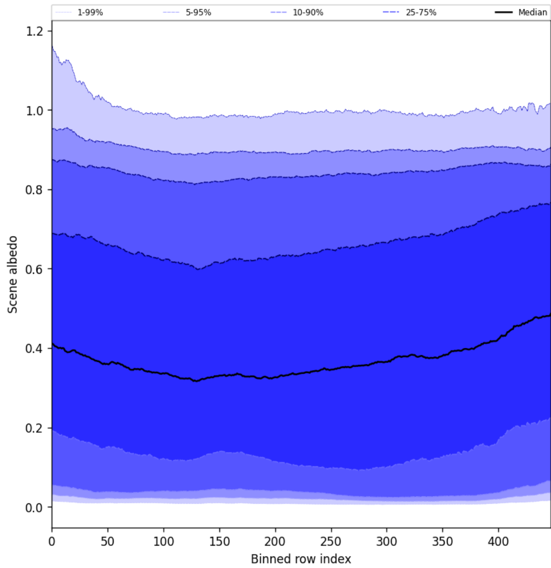
Figure 51: Along track statistics of “Scene albedo” for 2025-06-03 to 2025-06-05
