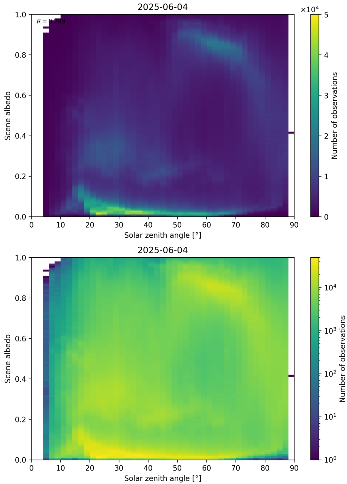
Figure 116: Scatter density plot of “Solar zenith angle” against “Scene albedo” for 2025-06-03 to 2025-06-05.
