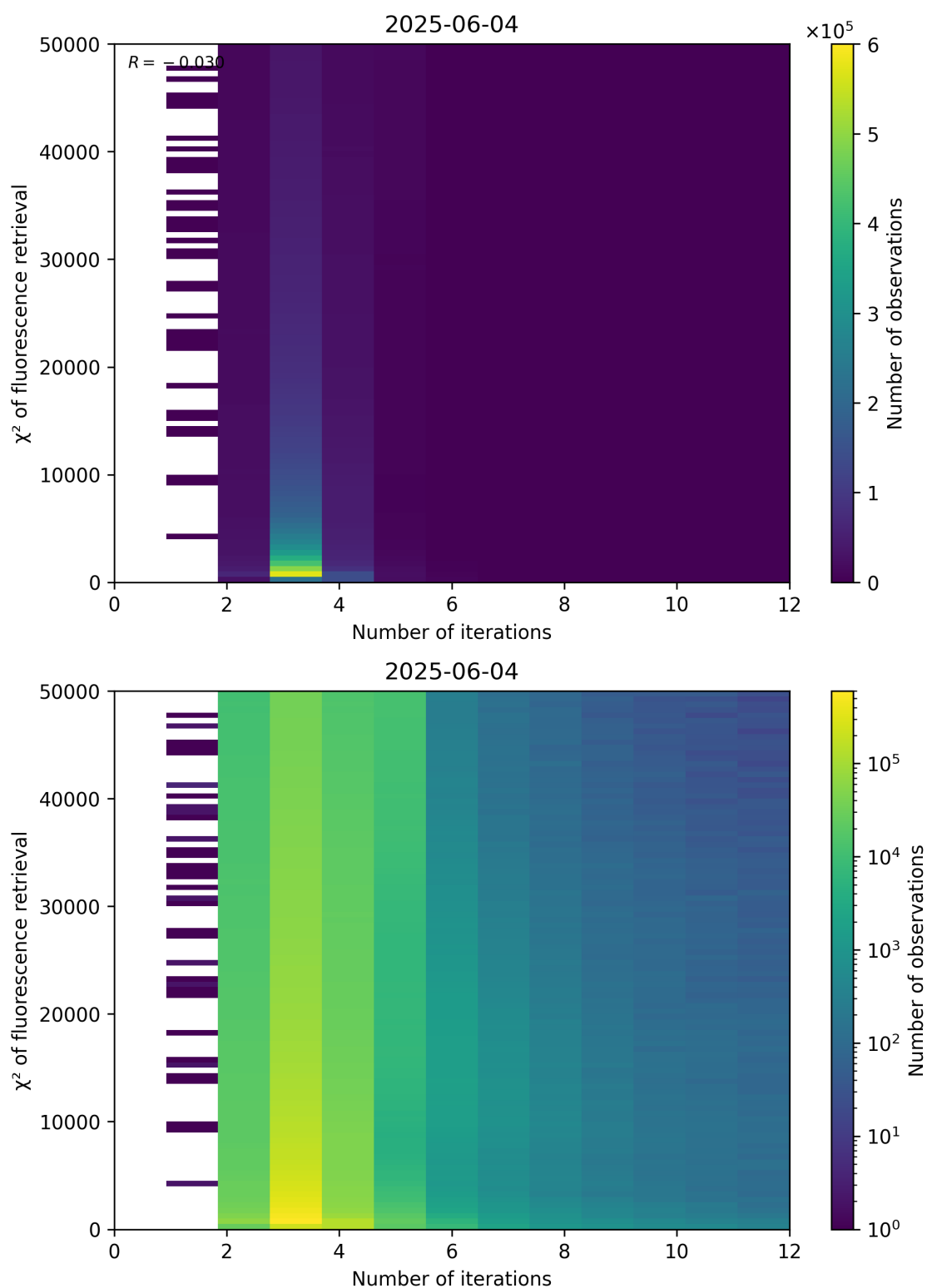
Figure 97: Scatter density plot of “Number of iterations” against “ \chi^2 of fluorescence retrieval” for 2025-06-03 to 2025-06-05.
