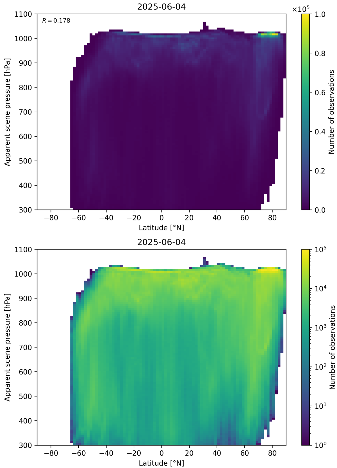
Figure 88: Scatter density plot of “Latitude” against “Apparent scene pressure” for 2025-06-03 to 2025-06-05.
