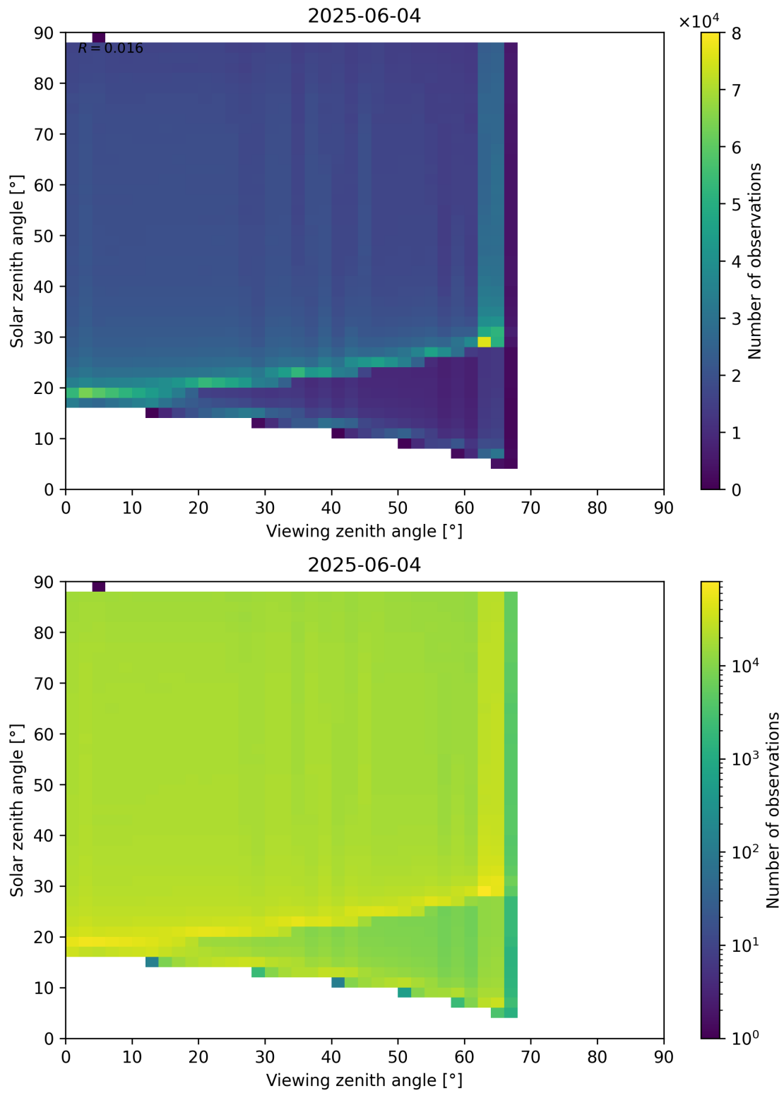
Figure 127: Scatter density plot of “Viewing zenith angle” against “Solar zenith angle” for 2025-06-03 to 2025-06-05.
