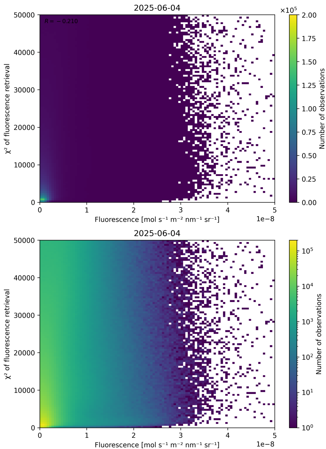
Figure 85: Scatter density plot of “Fluorescence” against “ \chi^2 of fluorescence retrieval” for 2025-06-03 to 2025-06-05.
