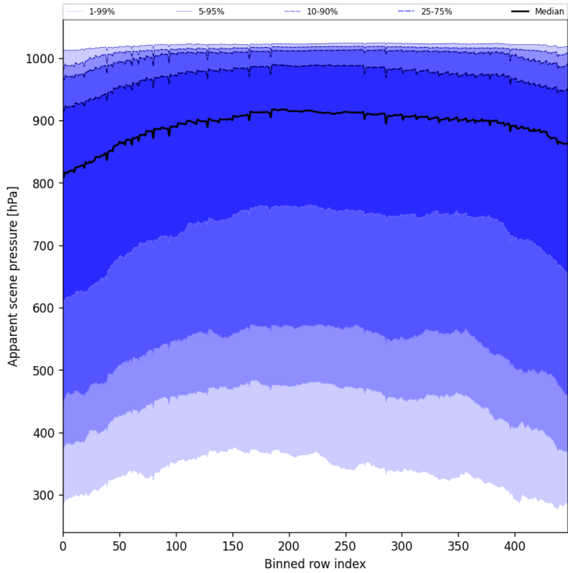
Figure 53: Along track statistics of “Apparent scene pressure” for 2025-06-03 to 2025-06-05
