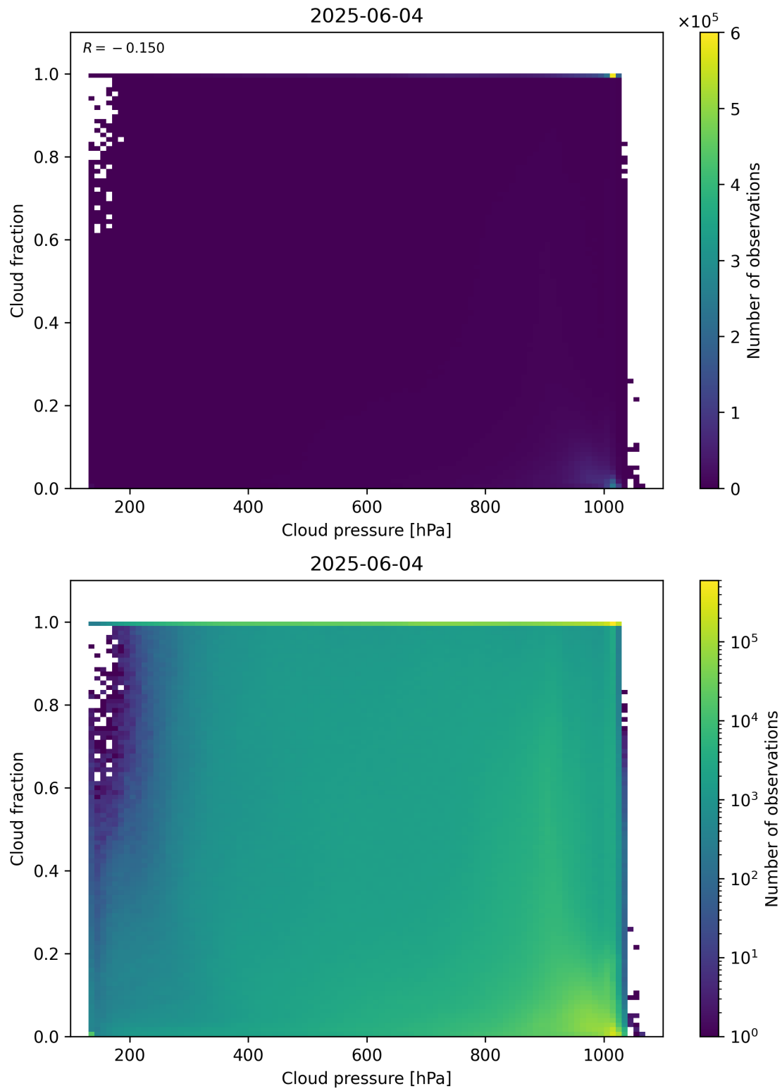
Figure 79: Scatter density plot of “Cloud pressure” against “Cloud fraction” for 2025-06-03 to 2025-06-05.
