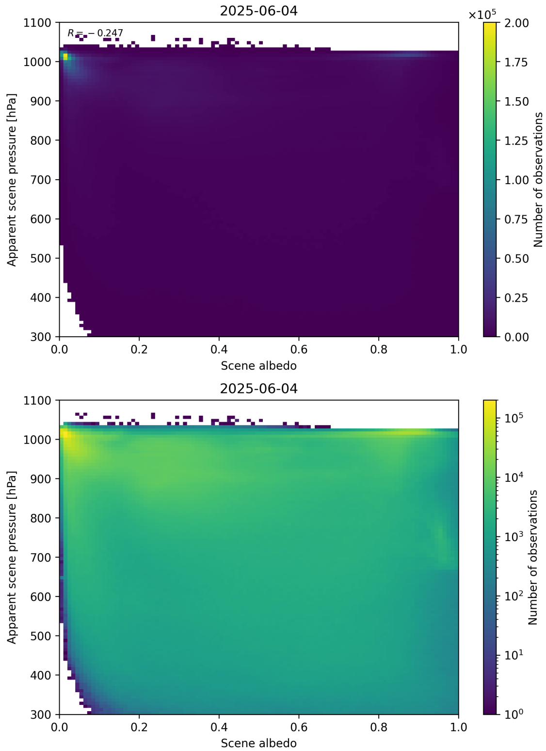
Figure 102: Scatter density plot of “Scene albedo” against “Apparent scene pressure” for 2025-06-03 to 2025-06-05.
