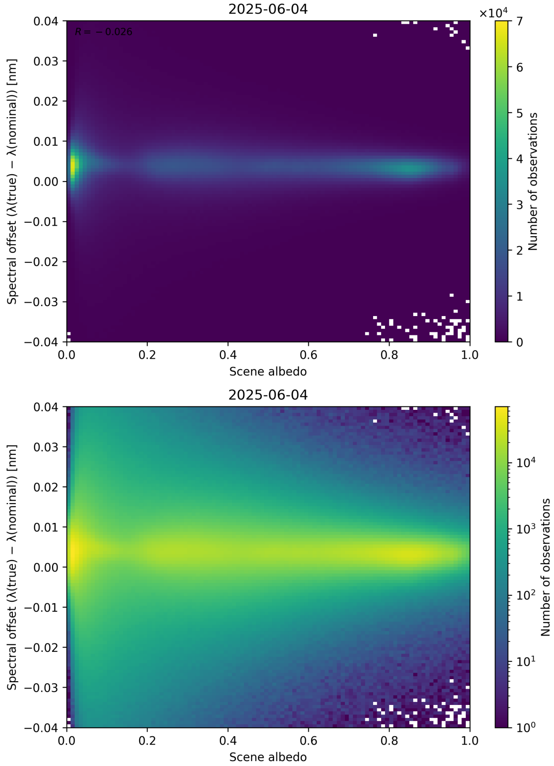
Figure 107: Scatter density plot of “Scene albedo” against “Spectral offset ( \lambda_{\text{true}} - \lambda_{\text{nominal}} )” for 2025-06-03 to 2025-06-05.
