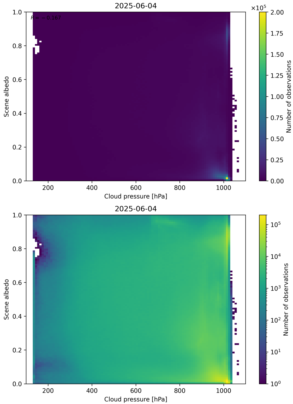
Figure 83: Scatter density plot of “Cloud pressure” against “Scene albedo” for 2025-06-03 to 2025-06-05.
