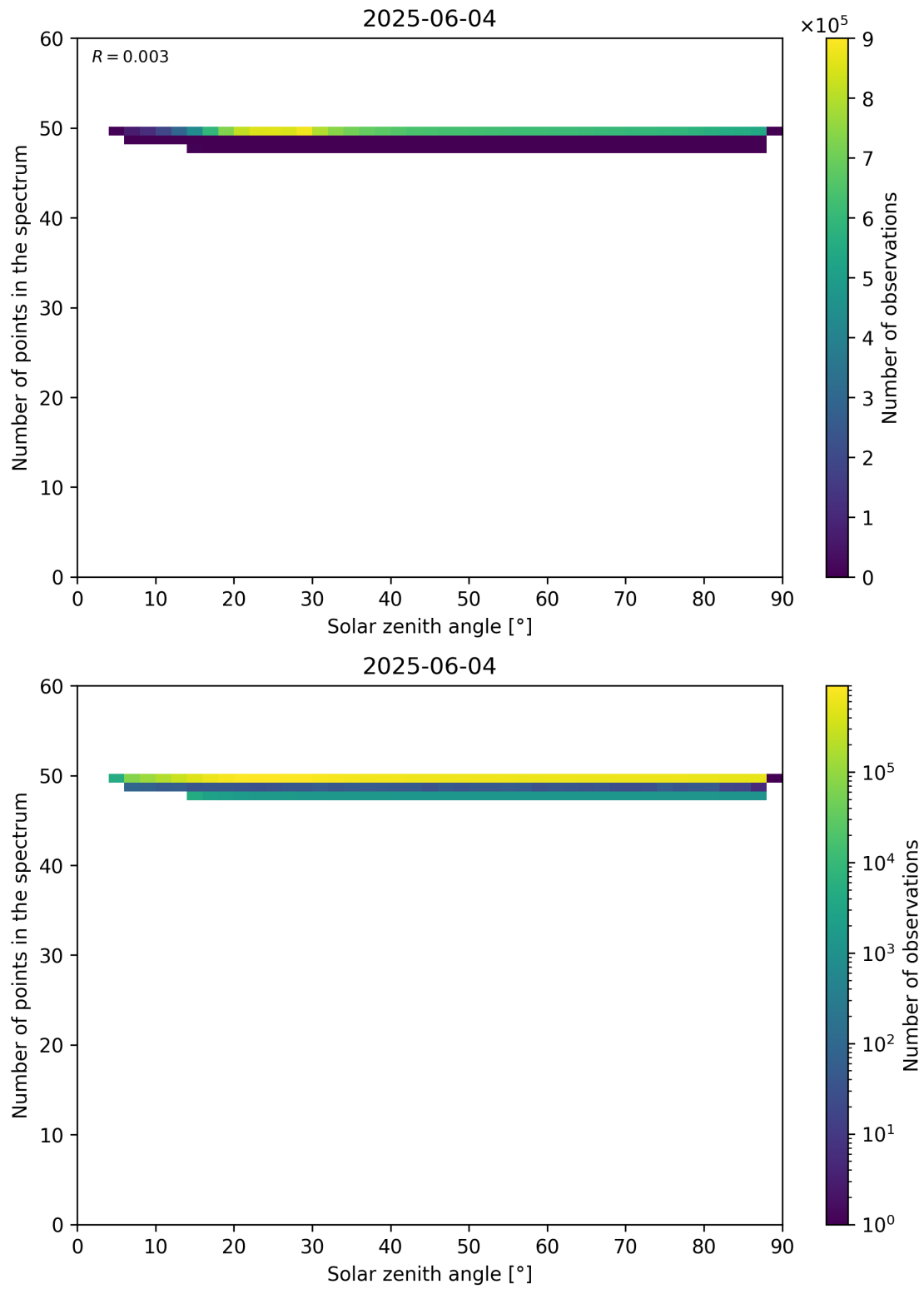
Figure 115: Scatter density plot of “Solar zenith angle” against “Number of points in the spectrum” for 2025-06-03 to 2025-06-05.
