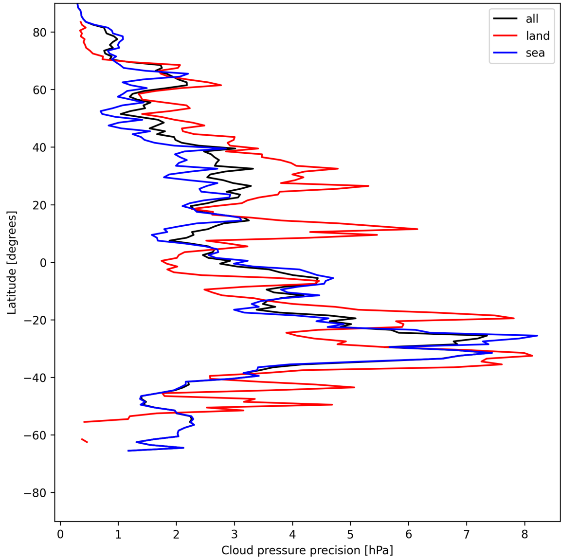
Figure 14: Zonal average of “Cloud pressure precision” for 2025-06-03 to 2025-06-05.
