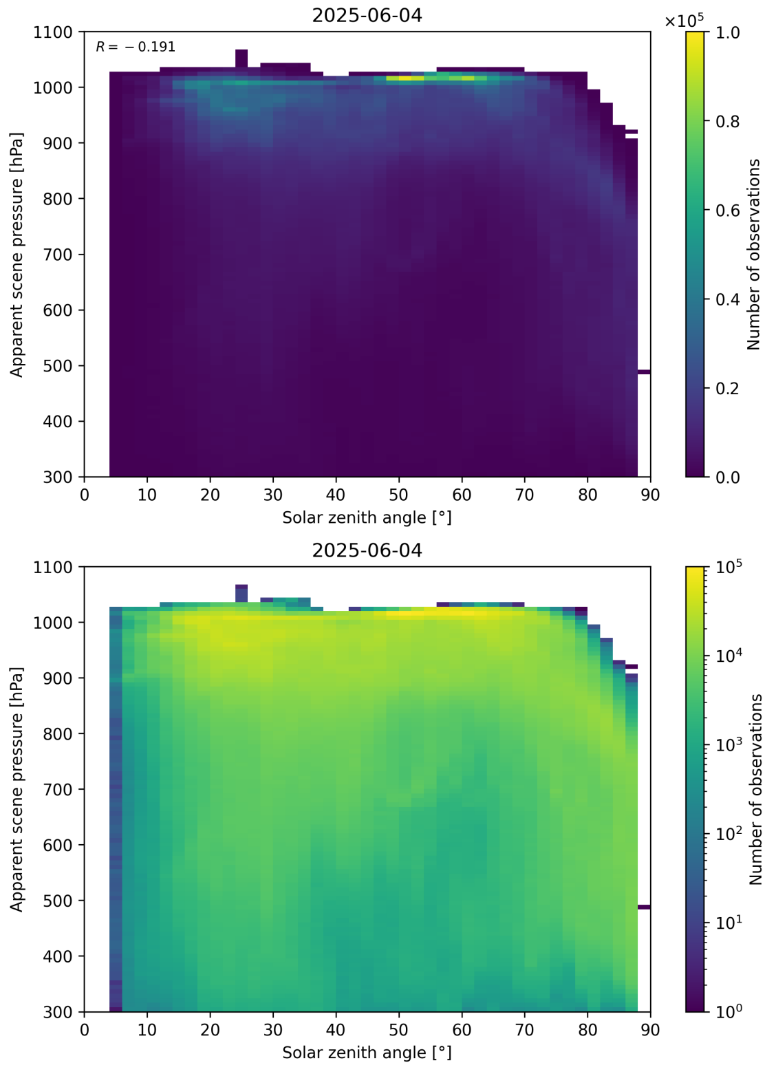
Figure 108: Scatter density plot of “Solar zenith angle” against “Apparent scene pressure” for 2025-06-03 to 2025-06-05.
