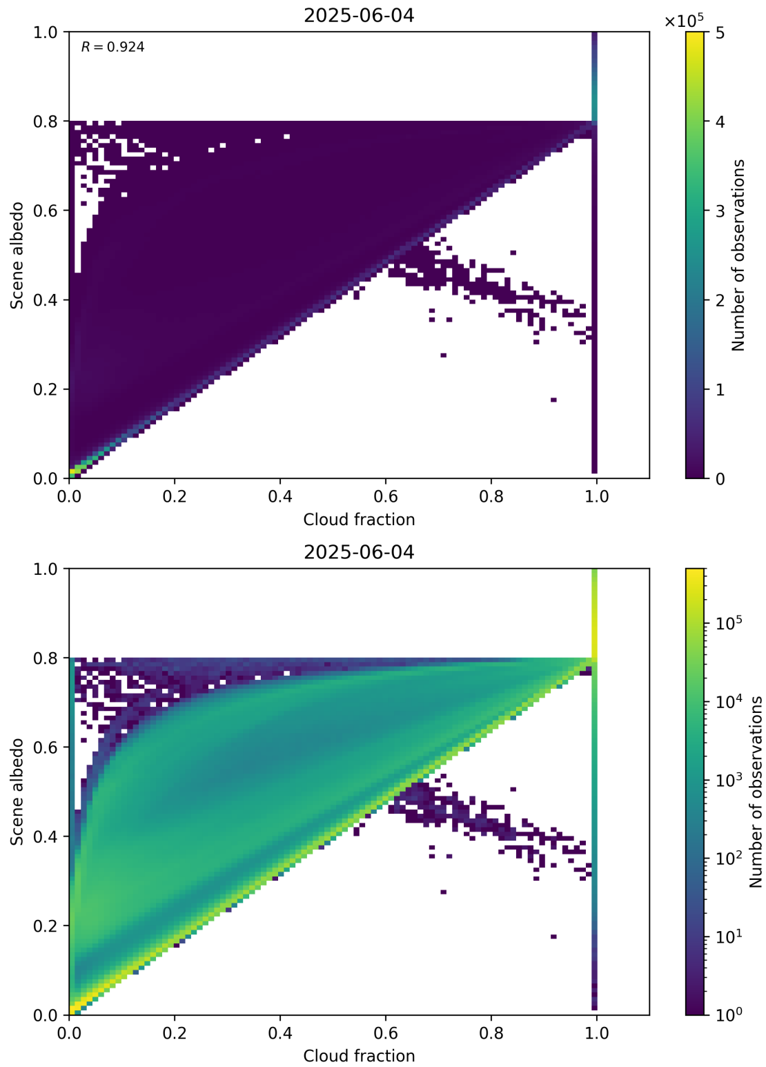
Figure 75: Scatter density plot of “Cloud fraction” against “Scene albedo” for 2025-06-03 to 2025-06-05.
