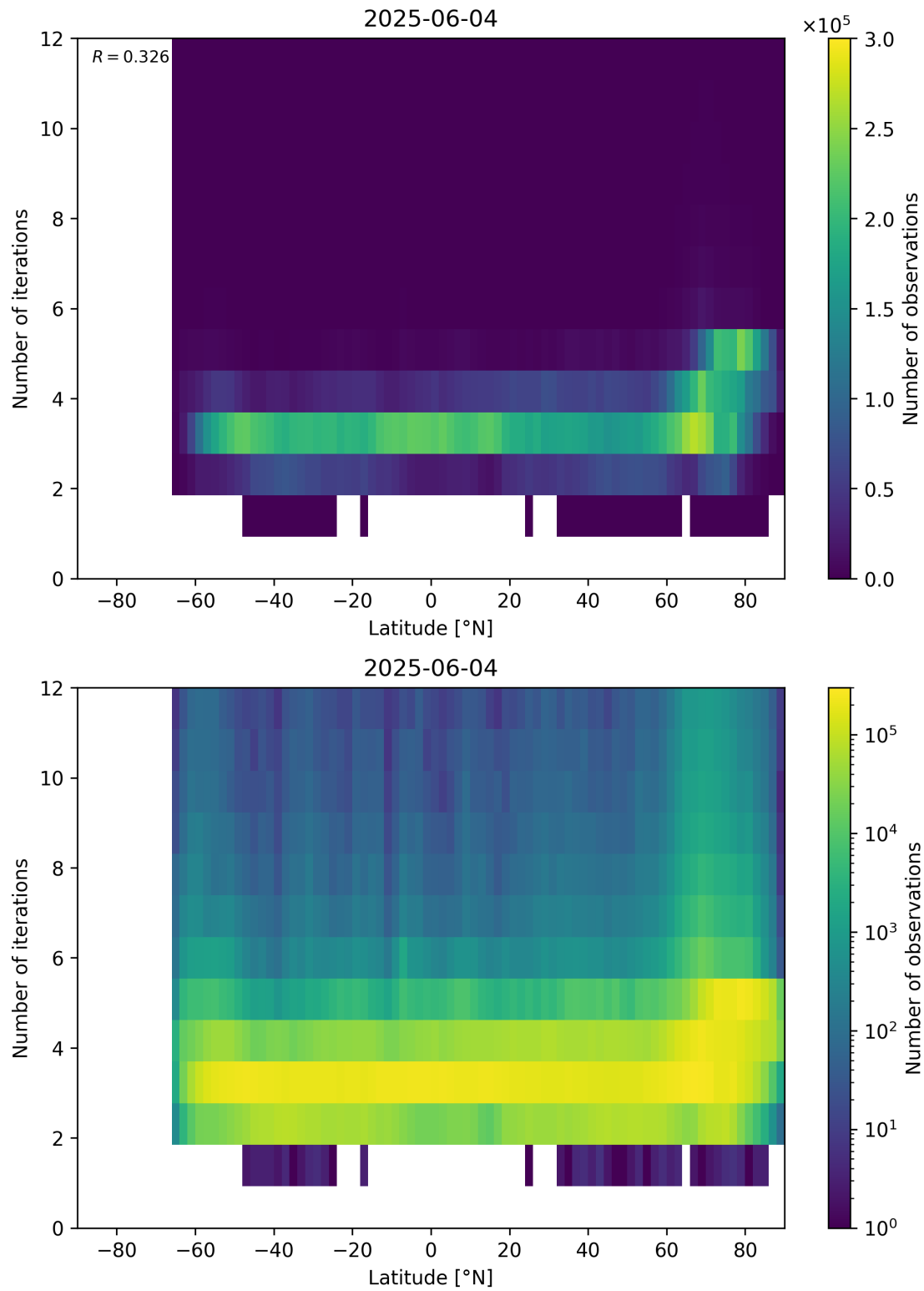
Figure 93: Scatter density plot of “Latitude” against “Number of iterations” for 2025-06-03 to 2025-06-05.
