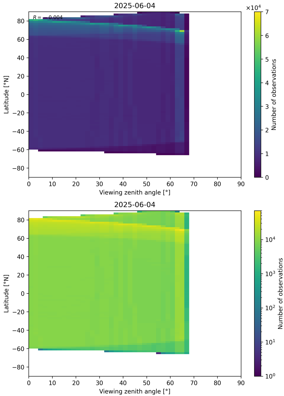
Figure 123: Scatter density plot of “Viewing zenith angle” against “Latitude” for 2025-06-03 to 2025-06-05.
