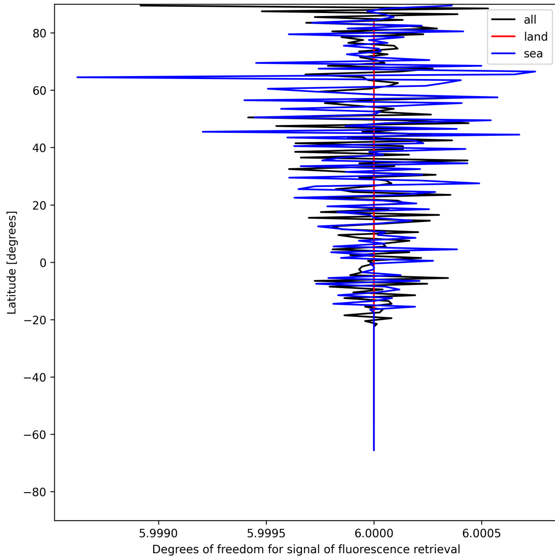
Figure 26: Zonal average of “Degrees of freedom for signal of fluorescence retrieval” for 2025-06-03 to 2025-06-05.
