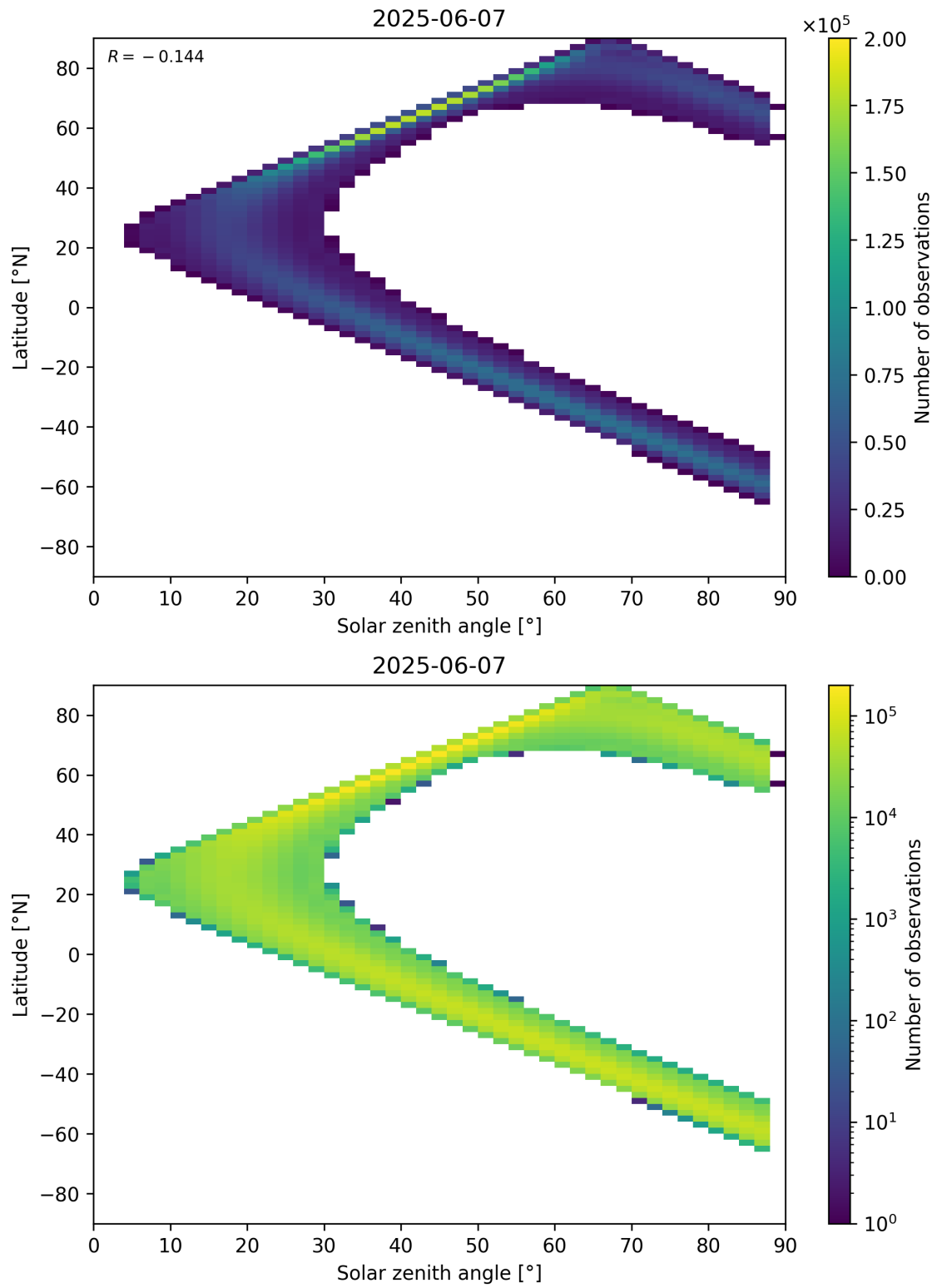
Figure 113: Scatter density plot of “Solar zenith angle” against “Latitude” for 2025-06-06 to 2025-06-08.
