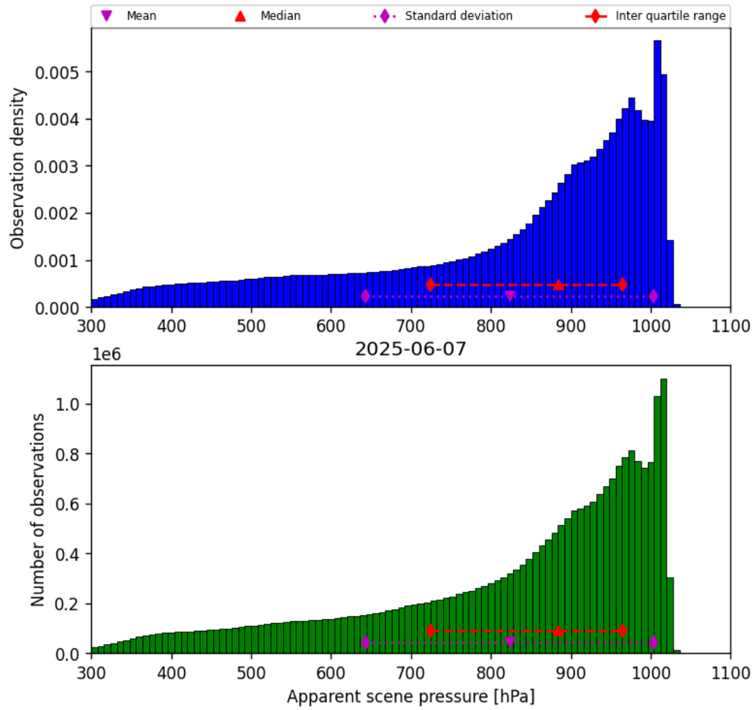
Figure 36: Histogram of “Apparent scene pressure” for 2025-06-06 to 2025-06-08
