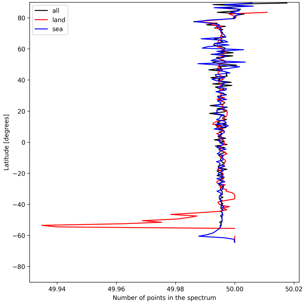
Figure 27: Zonal average of “Number of points in the spectrum” for 2025-06-06 to 2025-06-08.
