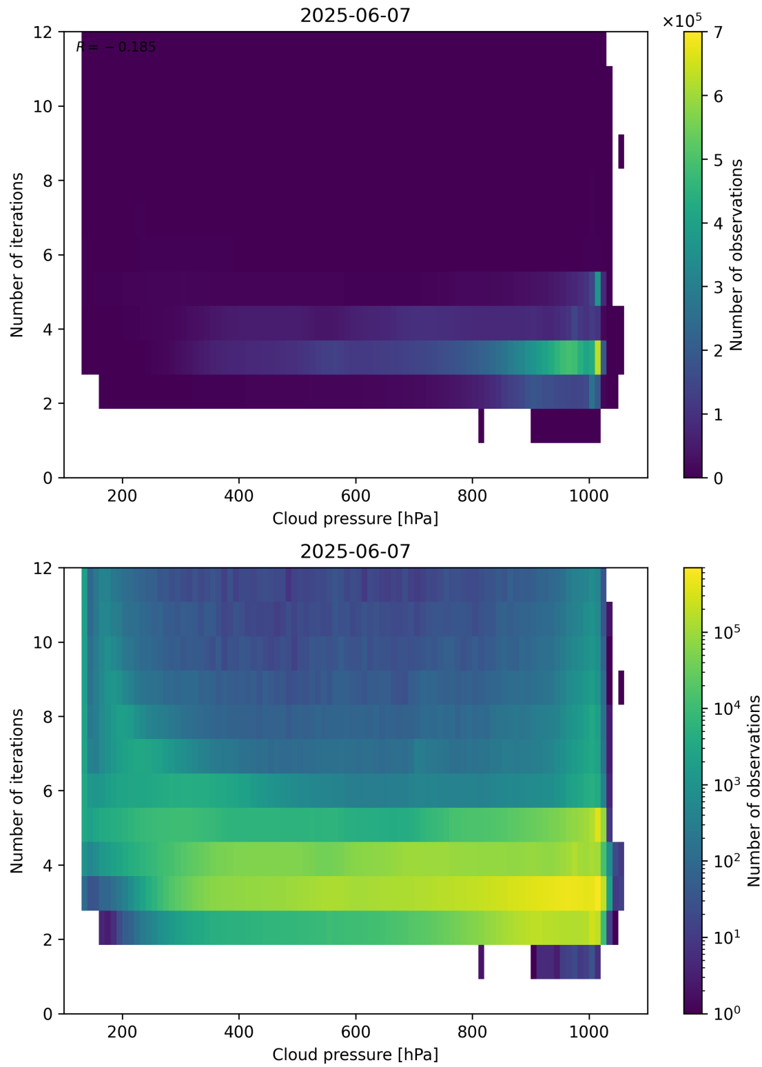
Figure 81: Scatter density plot of “Cloud pressure” against “Number of iterations” for 2025-06-06 to 2025-06-08.
