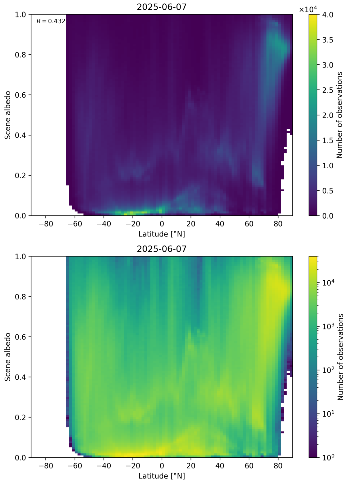
Figure 95: Scatter density plot of “Latitude” against “Scene albedo” for 2025-06-06 to 2025-06-08.
