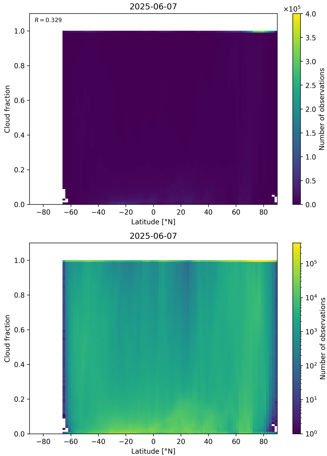
Figure 90: Scatter density plot of “Latitude” against “Cloud fraction” for 2025-06-06 to 2025-06-08.
