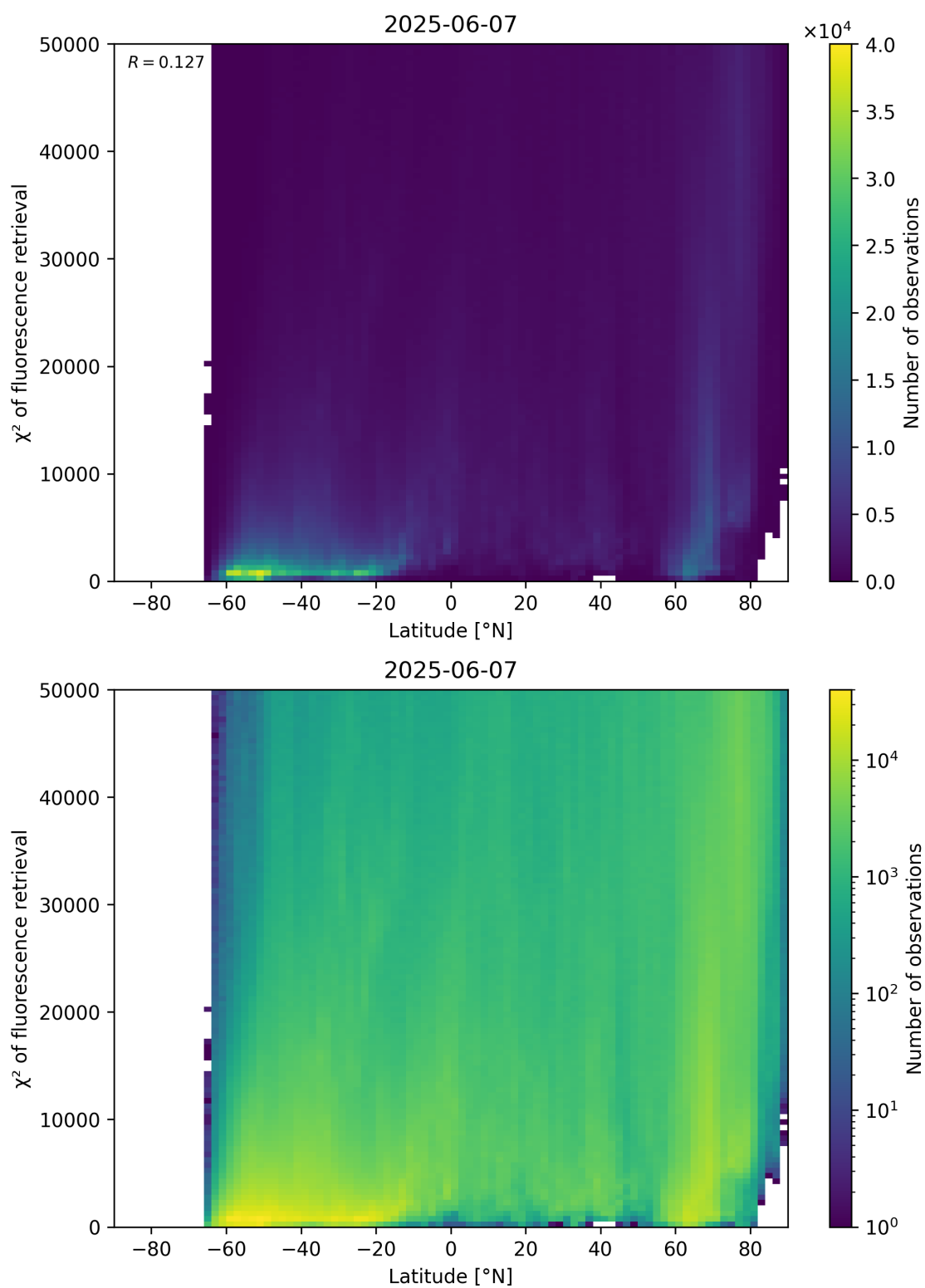
Figure 89: Scatter density plot of “Latitude” against “ \chi^2 of fluorescence retrieval” for 2025-06-06 to 2025-06-08.
