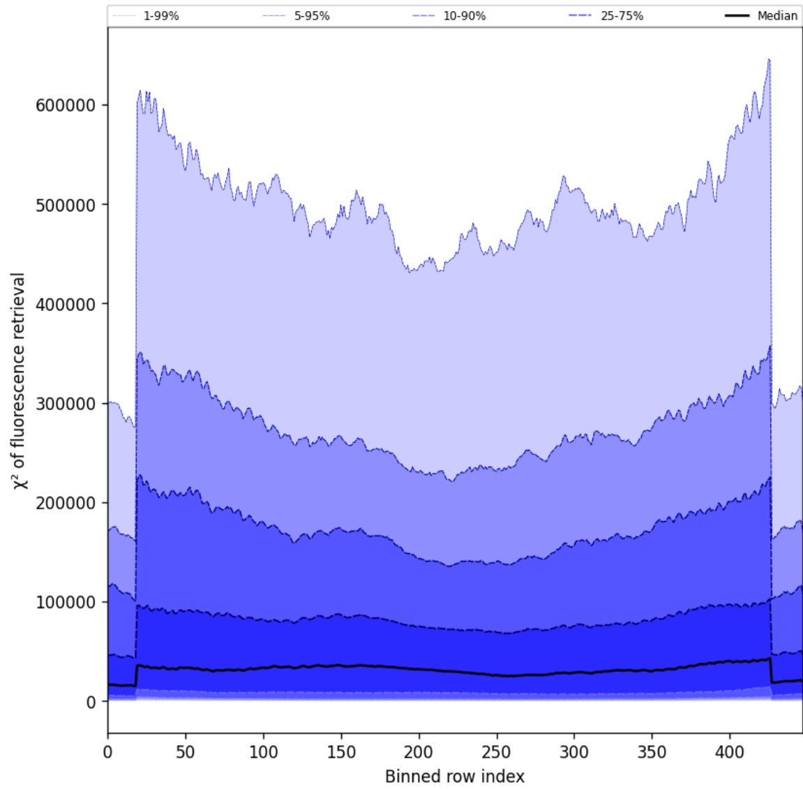
Figure 59: Along track statistics of “ \chi^2 of fluorescence retrieval” for 2025-06-06 to 2025-06-08
