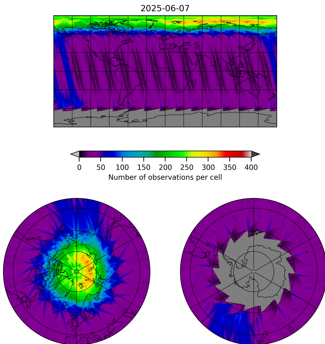
Figure 11: Map of the number of observations for 2025-06-06 to 2025-06-08
