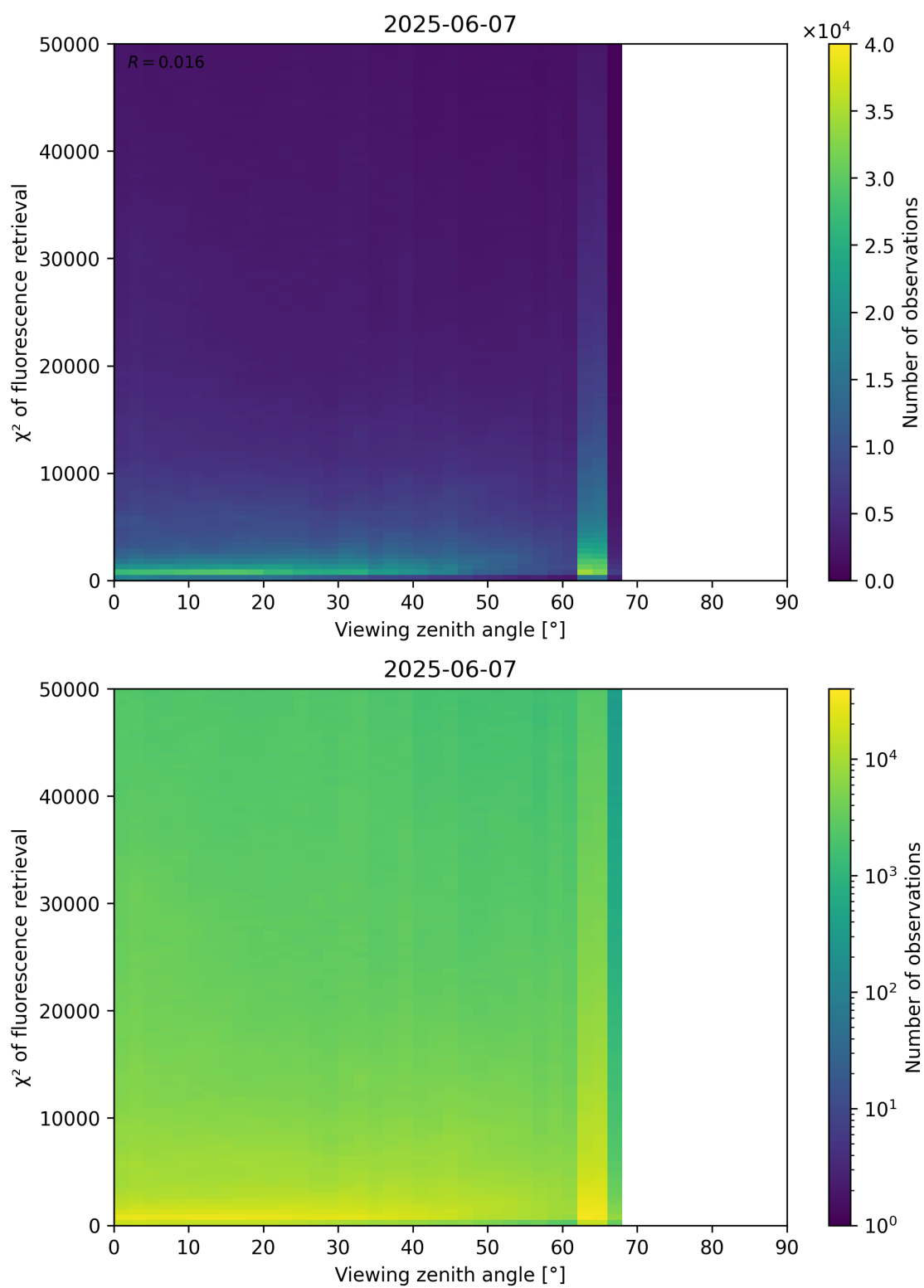
Figure 119: Scatter density plot of “Viewing zenith angle” against “ \chi^2 of fluorescence retrieval” for 2025-06-06 to 2025-06-08.
