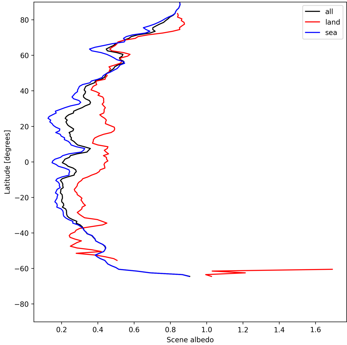
Figure 17: Zonal average of “Scene albedo” for 2025-06-06 to 2025-06-08.
