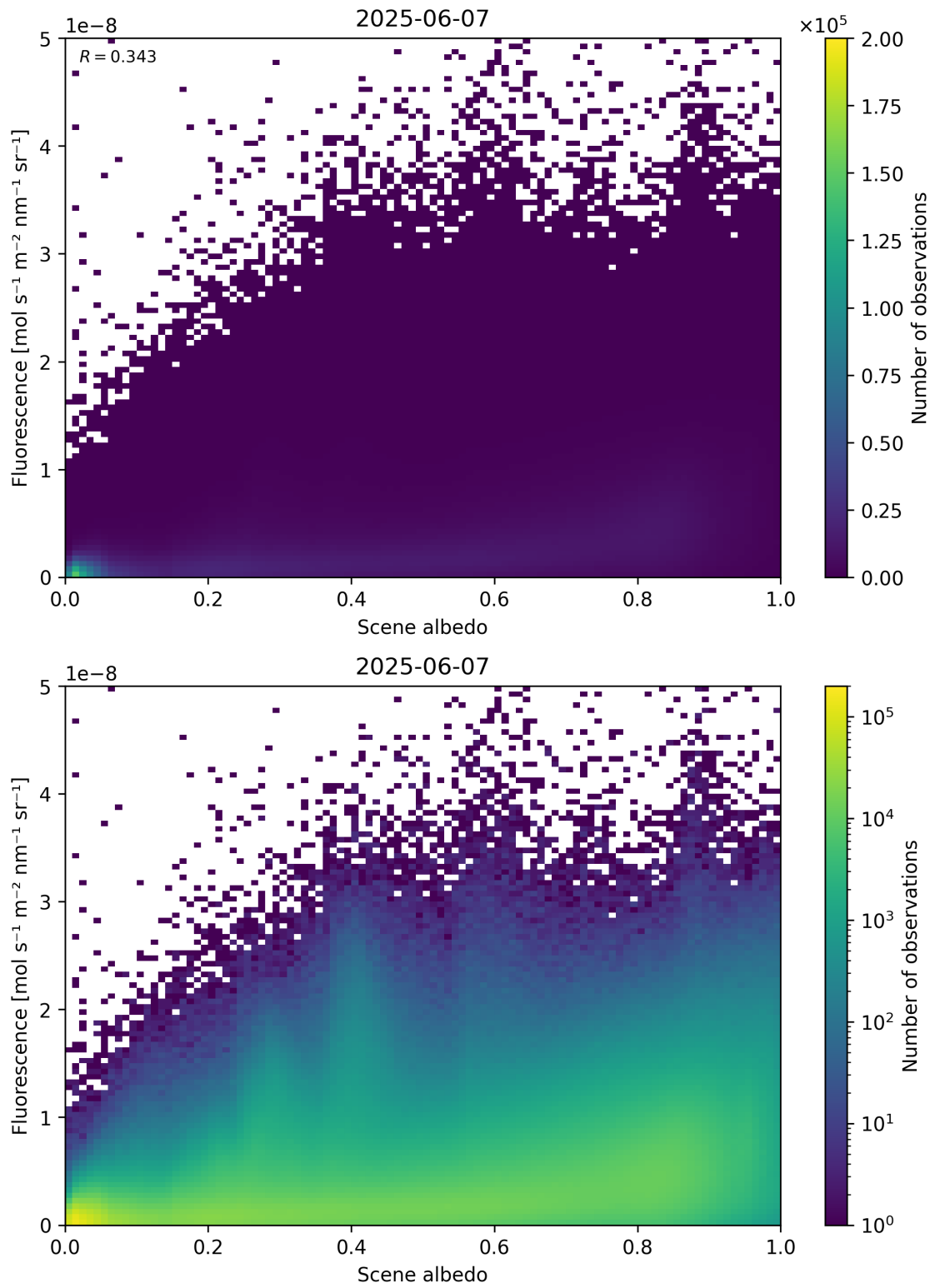
Figure 104: Scatter density plot of “Scene albedo” against “Fluorescence” for 2025-06-06 to 2025-06-08.
