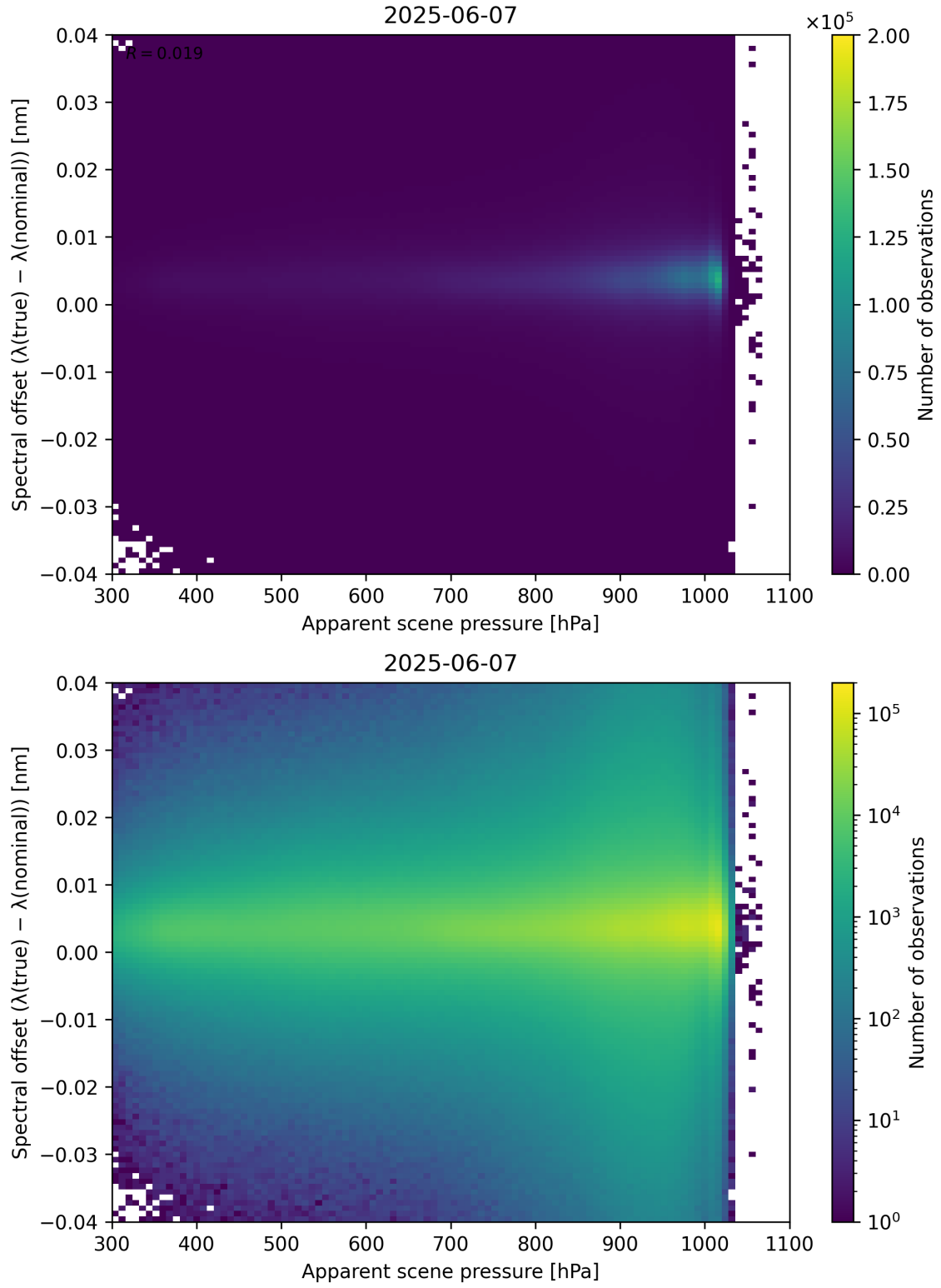
Figure 67: Scatter density plot of “Apparent scene pressure” against “Spectral offset ( \lambda_{\text{true}} - \lambda_{\text{nominal}} )” for 2025-06-06 to 2025-06-08.
