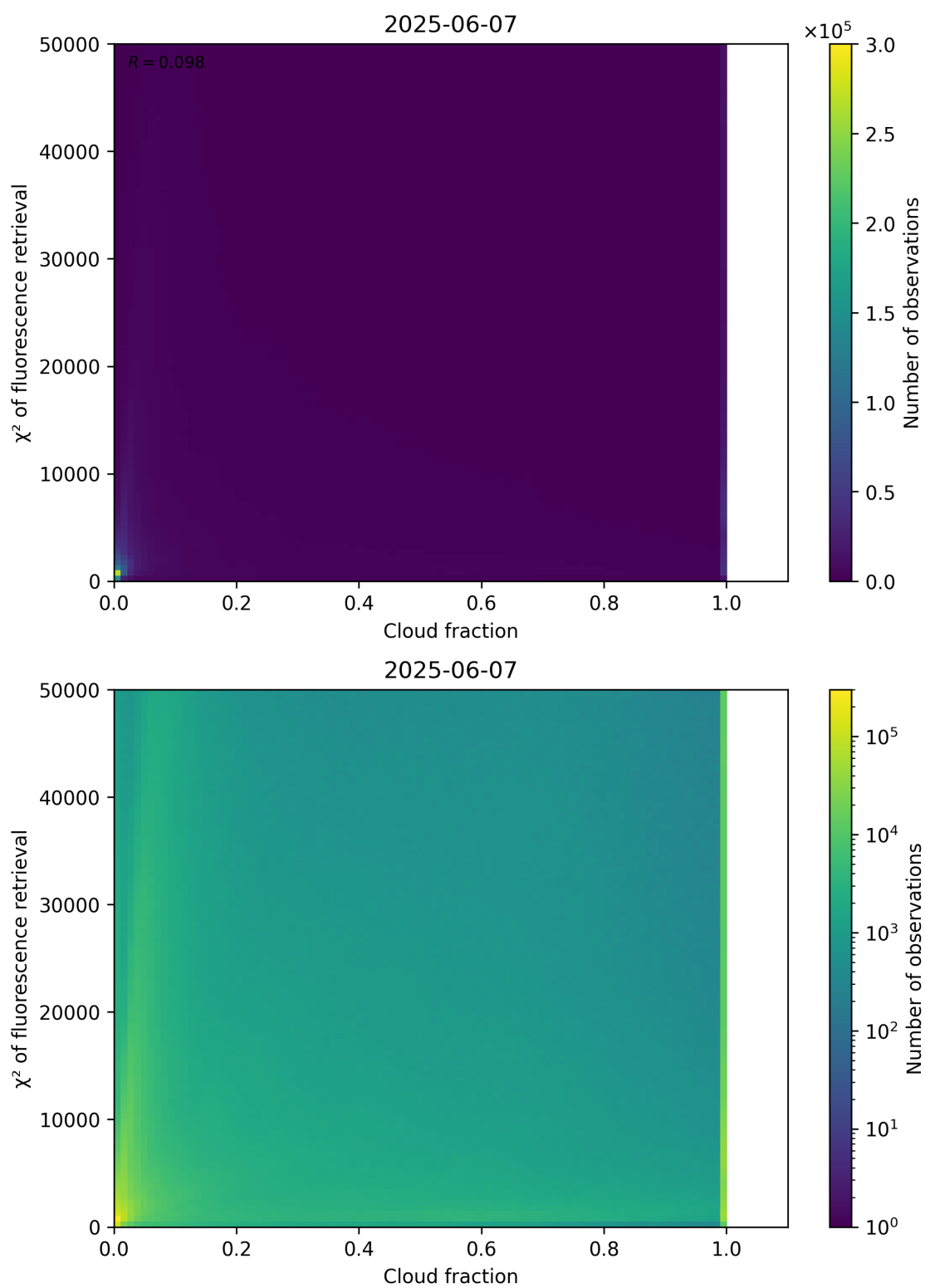
Figure 71: Scatter density plot of “Cloud fraction” against “ \chi^2 of fluorescence retrieval” for 2025-06-06 to 2025-06-08.
