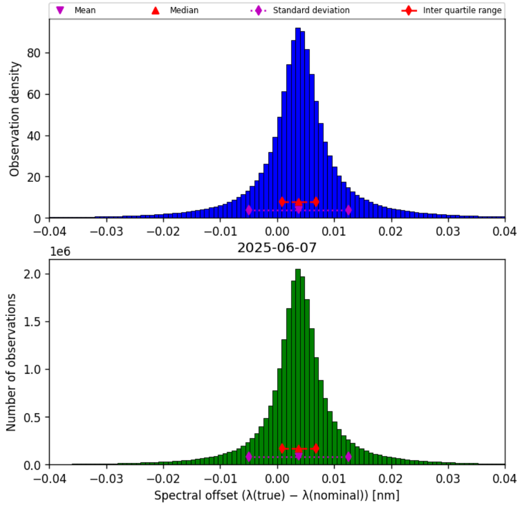
Figure 45: Histogram of “Spectral offset ( \lambda_{\text{true}} - \lambda_{\text{nominal}} )” for 2025-06-06 to 2025-06-08
