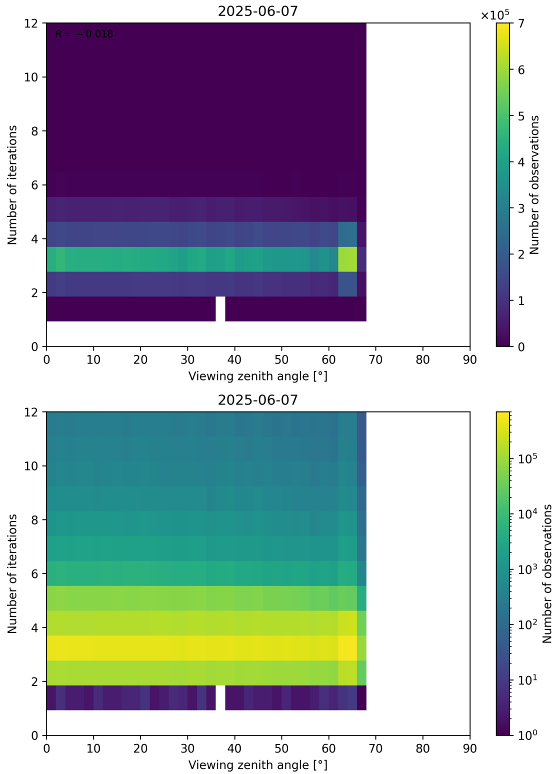
Figure 124: Scatter density plot of “Viewing zenith angle” against “Number of iterations” for 2025-06-06 to 2025-06-08.
