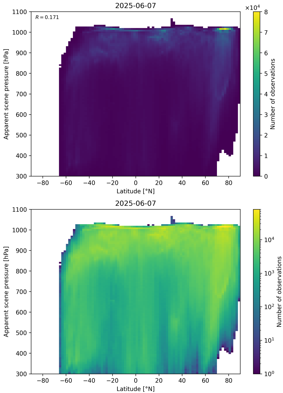
Figure 88: Scatter density plot of “Latitude” against “Apparent scene pressure” for 2025-06-06 to 2025-06-08.
