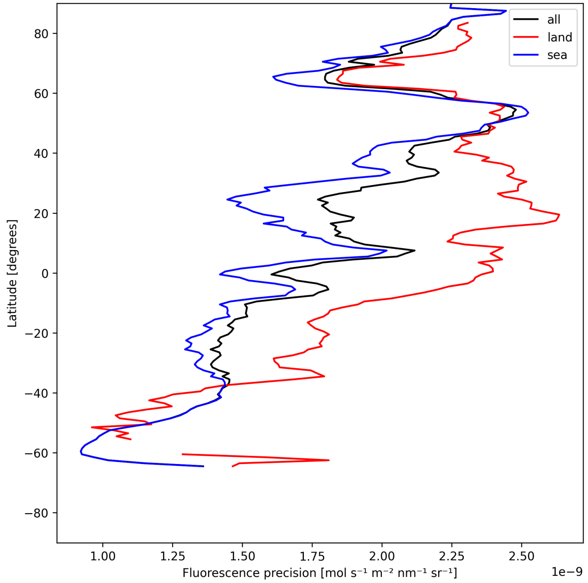
Figure 24: Zonal average of “Fluorescence precision” for 2025-06-06 to 2025-06-08.
