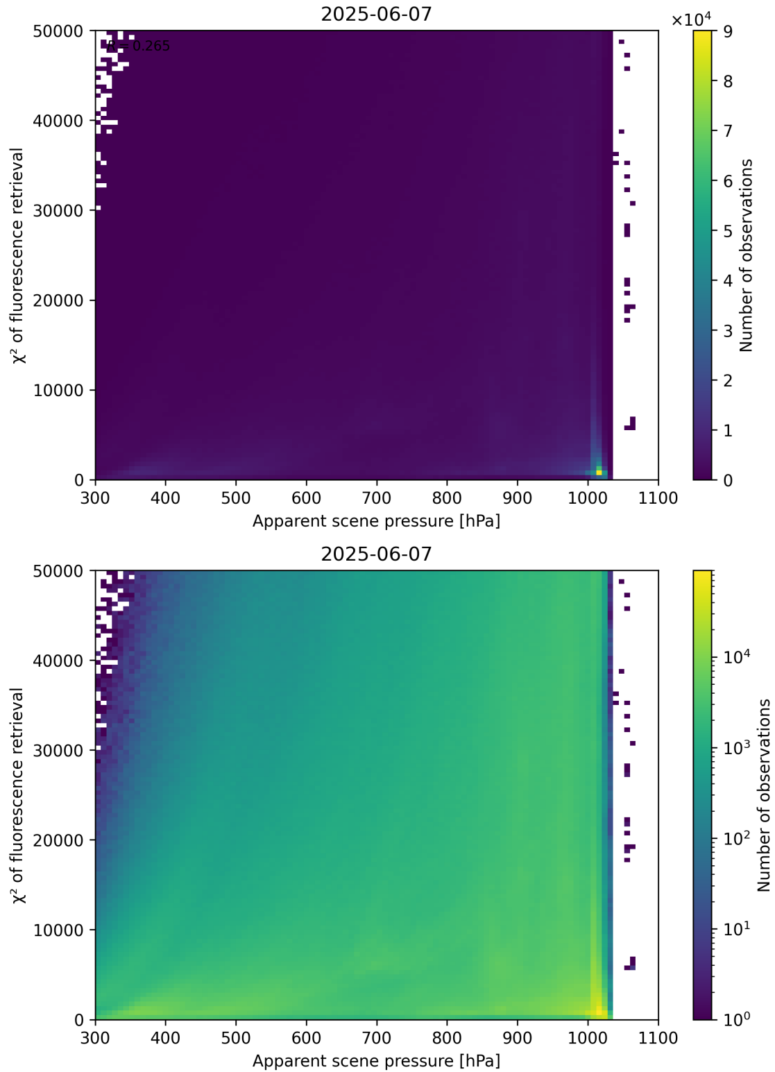
Figure 63: Scatter density plot of “Apparent scene pressure” against “ \chi^2 of fluorescence retrieval” for 2025-06-06 to 2025-06-08.
