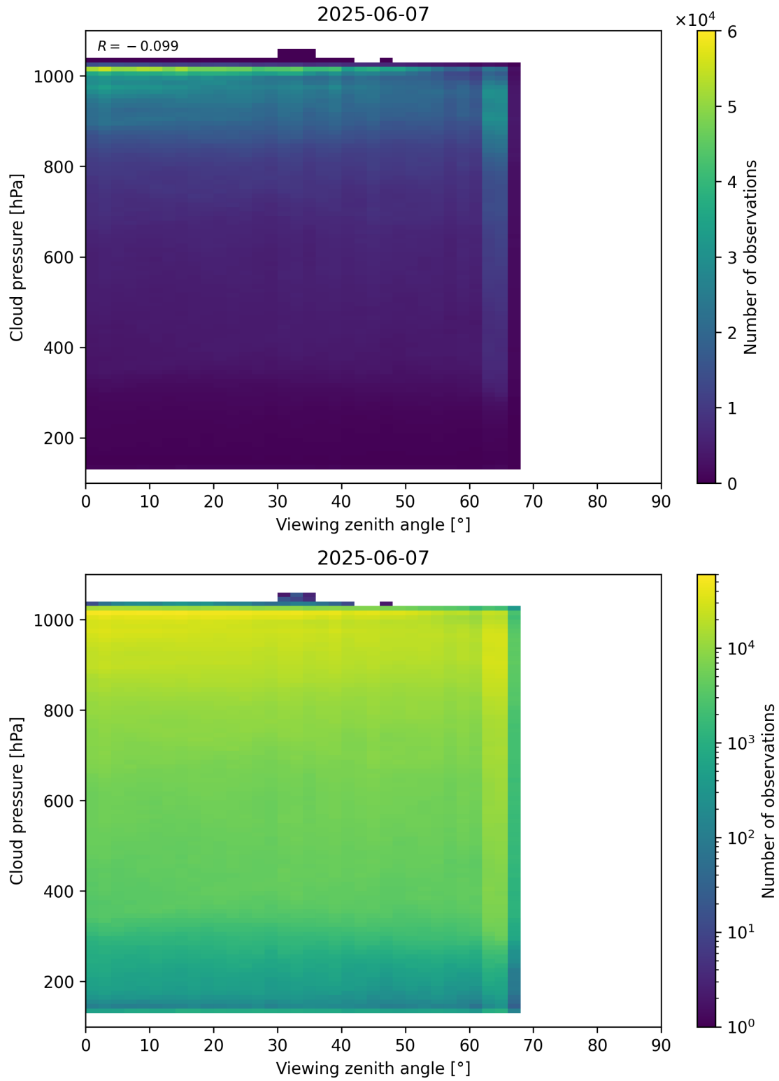
Figure 121: Scatter density plot of “Viewing zenith angle” against “Cloud pressure” for 2025-06-06 to 2025-06-08.
