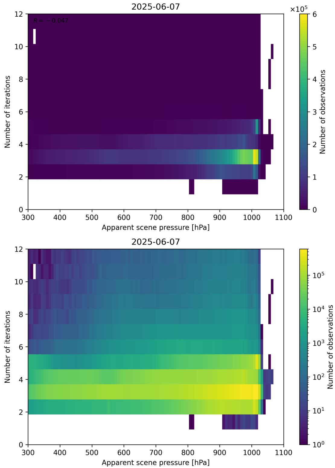
Figure 65: Scatter density plot of “Apparent scene pressure” against “Number of iterations” for 2025-06-06 to 2025-06-08.
