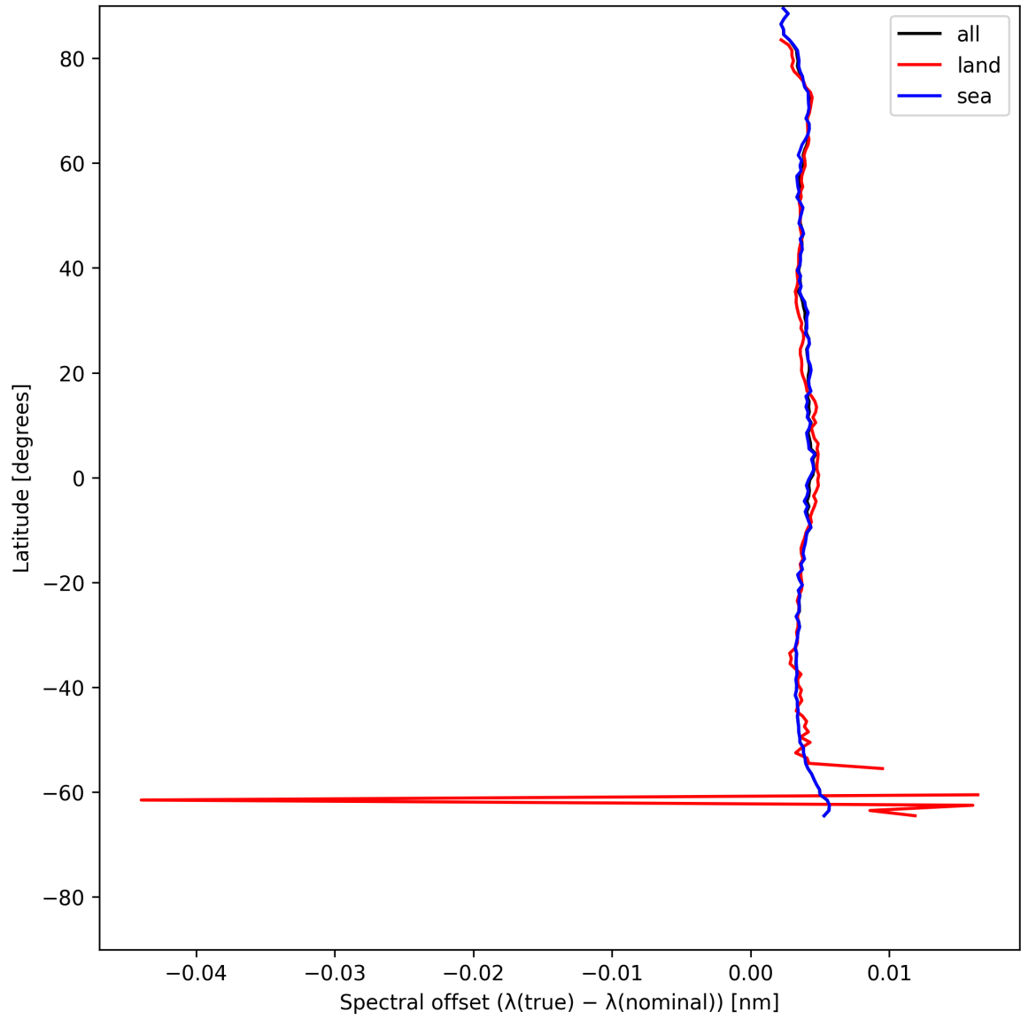
Figure 28: Zonal average of “Spectral offset ( \lambda_{\text{true}} - \lambda_{\text{nominal}} )” for 2025-06-06 to 2025-06-08.
