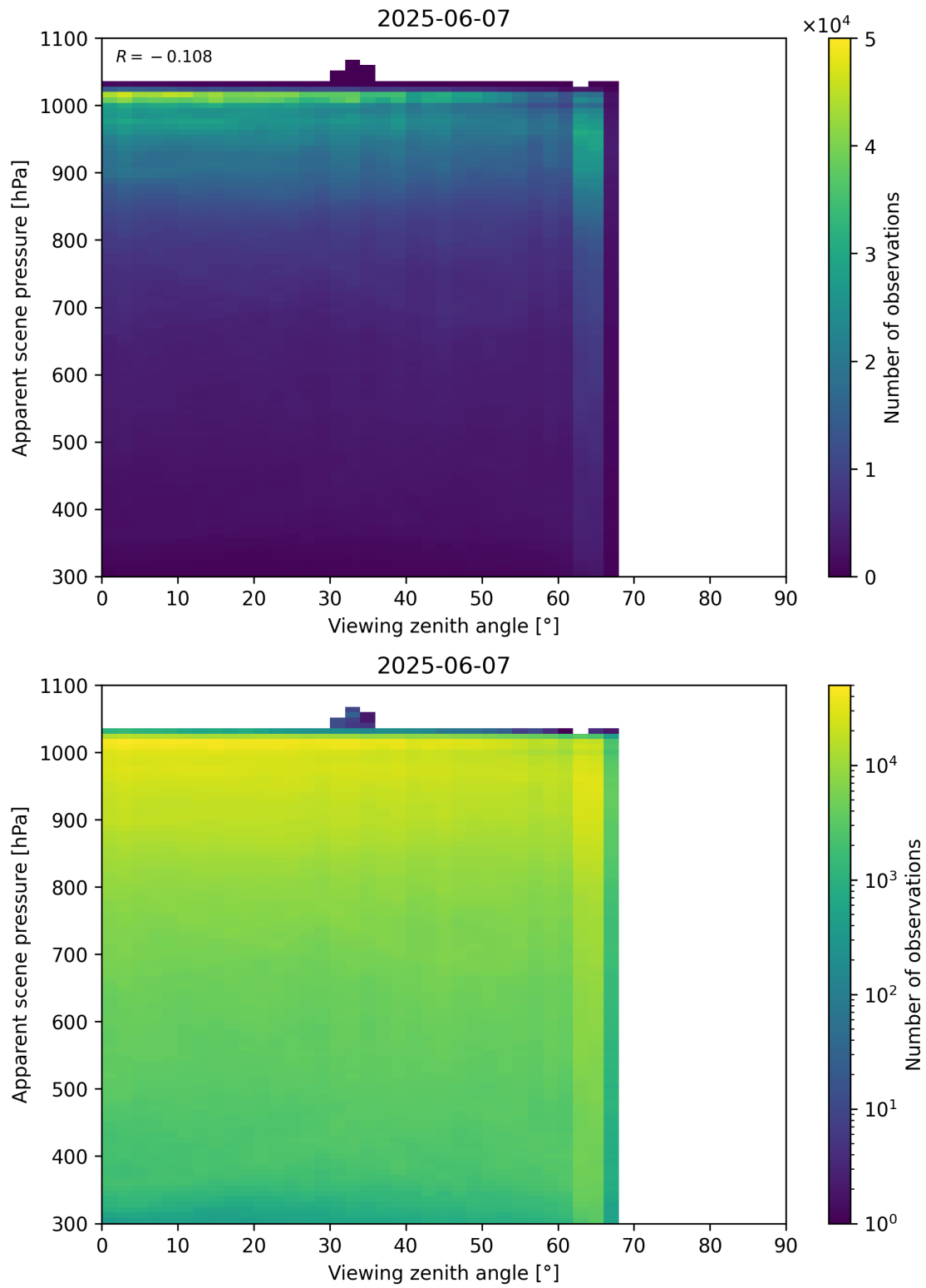
Figure 118: Scatter density plot of “Viewing zenith angle” against “Apparent scene pressure” for 2025-06-06 to 2025-06-08.
