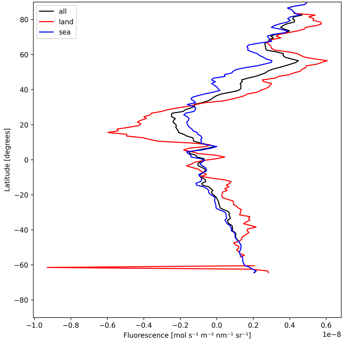
Figure 23: Zonal average of “Fluorescence” for 2025-06-06 to 2025-06-08.
