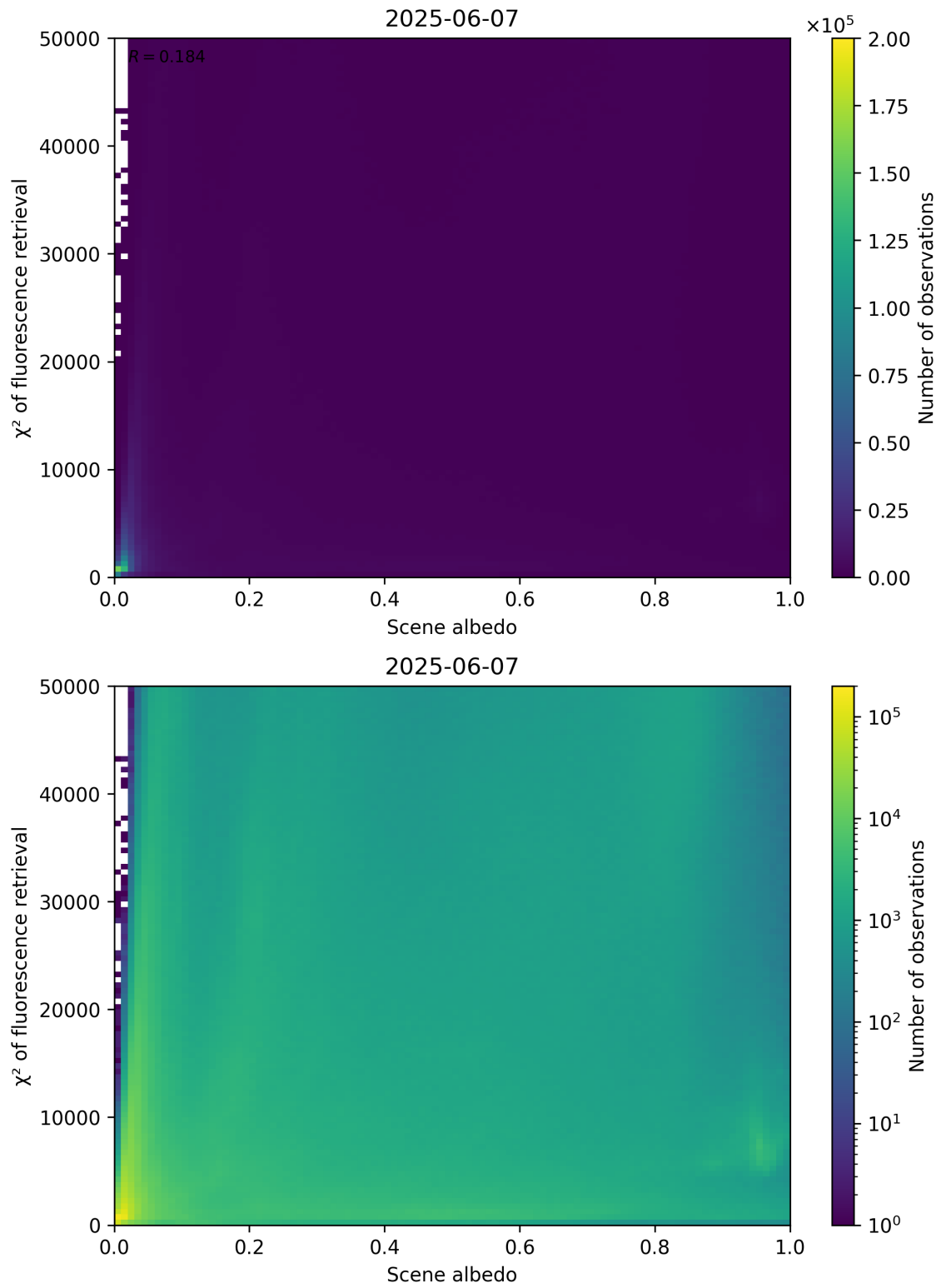
Figure 103: Scatter density plot of “Scene albedo” against “ \chi^2 of fluorescence retrieval” for 2025-06-06 to 2025-06-08.
