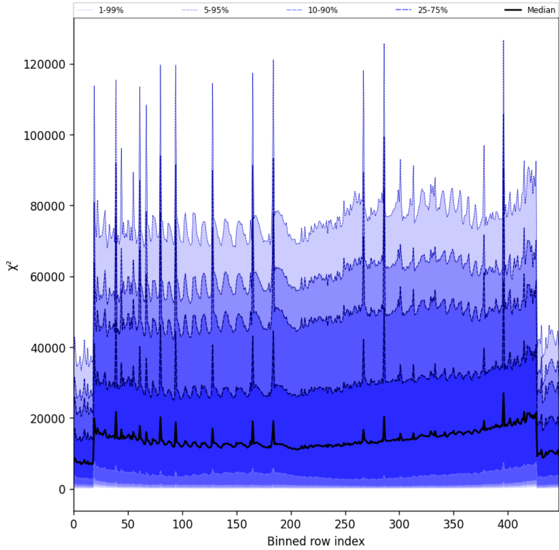
Figure 55: Along track statistics of “ \chi^2 ” for 2025-06-06 to 2025-06-08
