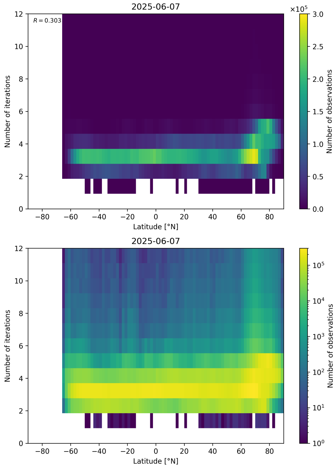
Figure 93: Scatter density plot of “Latitude” against “Number of iterations” for 2025-06-06 to 2025-06-08.
