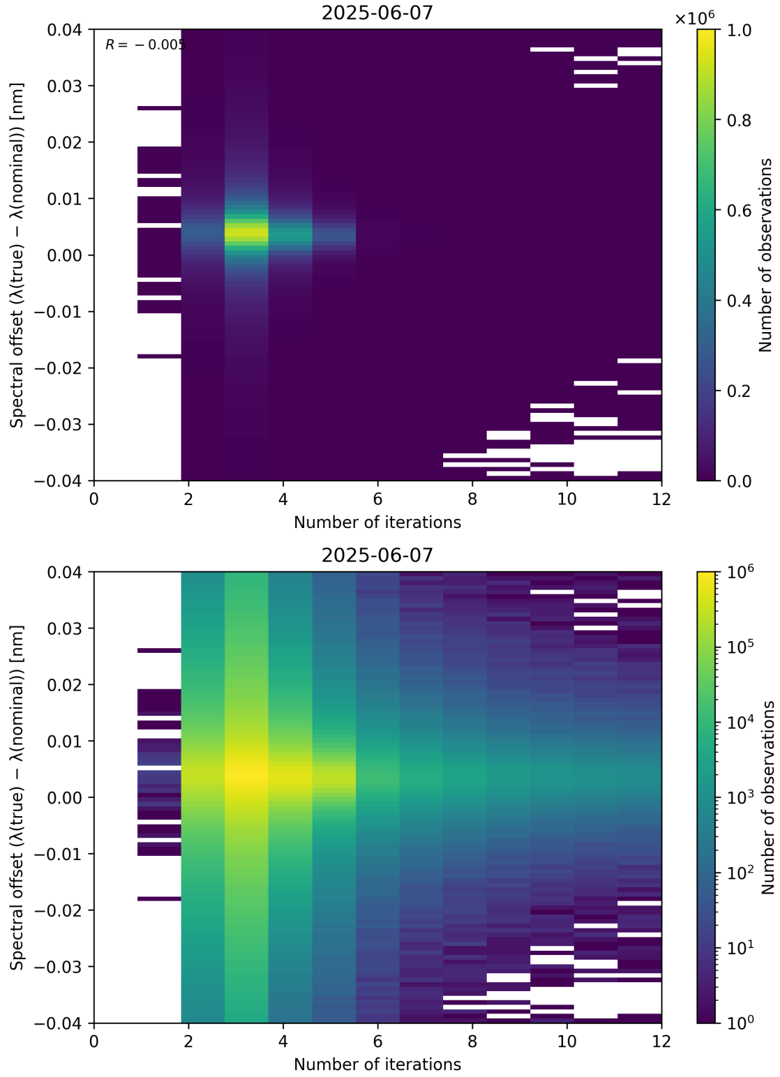
Figure 100: Scatter density plot of “Number of iterations” against “Spectral offset ( \lambda_{\text{true}} - \lambda_{\text{nominal}} )” for 2025-06-06 to 2025-06-08.
