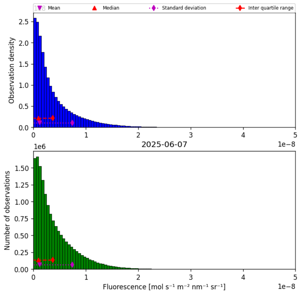
Figure 40: Histogram of “Fluorescence” for 2025-06-06 to 2025-06-08
