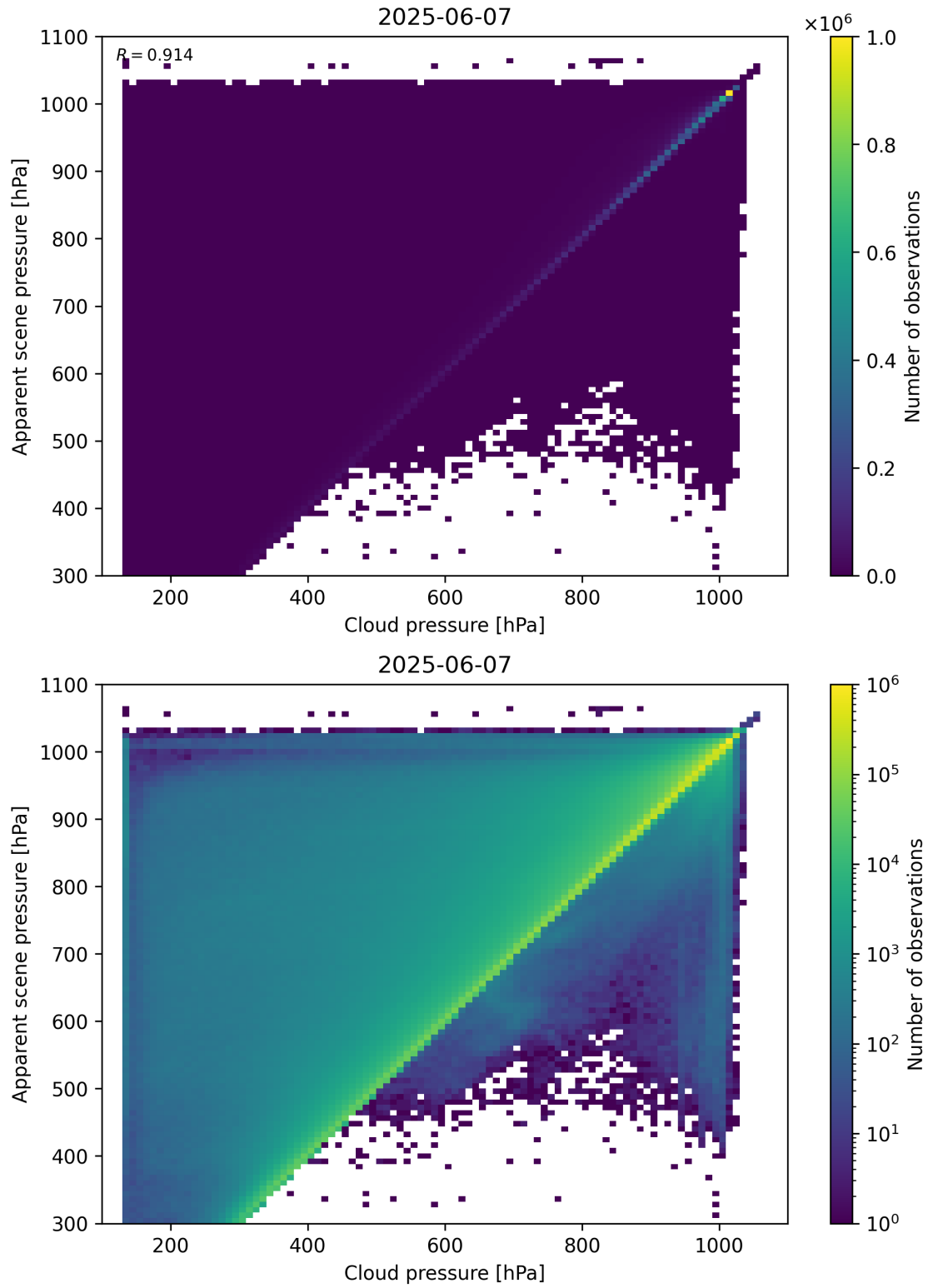
Figure 77: Scatter density plot of “Cloud pressure” against “Apparent scene pressure” for 2025-06-06 to 2025-06-08.
