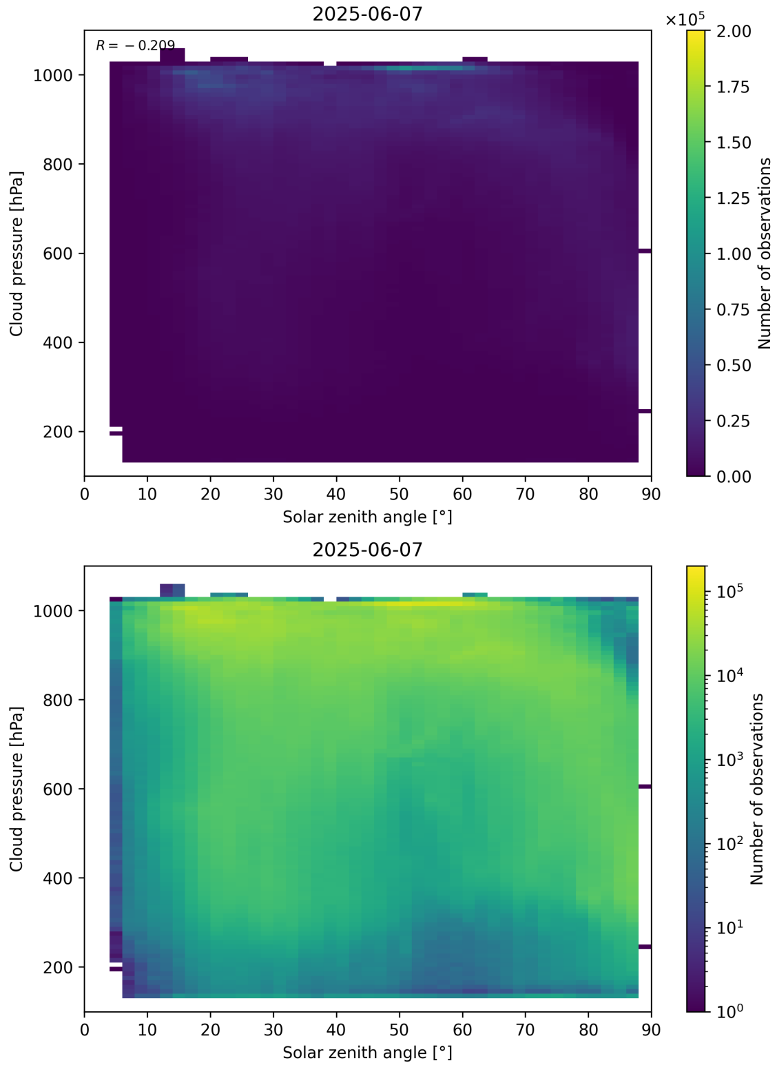
Figure 111: Scatter density plot of “Solar zenith angle” against “Cloud pressure” for 2025-06-06 to 2025-06-08.
