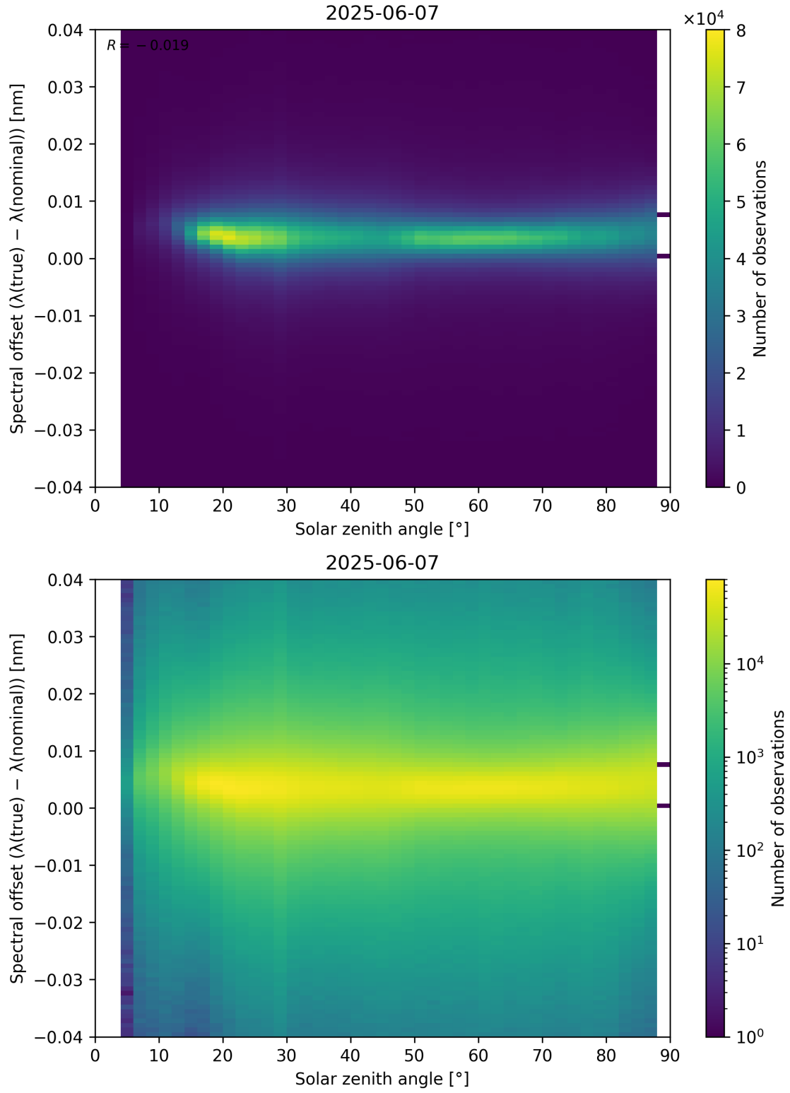
Figure 117: Scatter density plot of “Solar zenith angle” against “Spectral offset ( \lambda_{\text{true}} - \lambda_{\text{nominal}} )” for 2025-06-06 to 2025-06-08.
