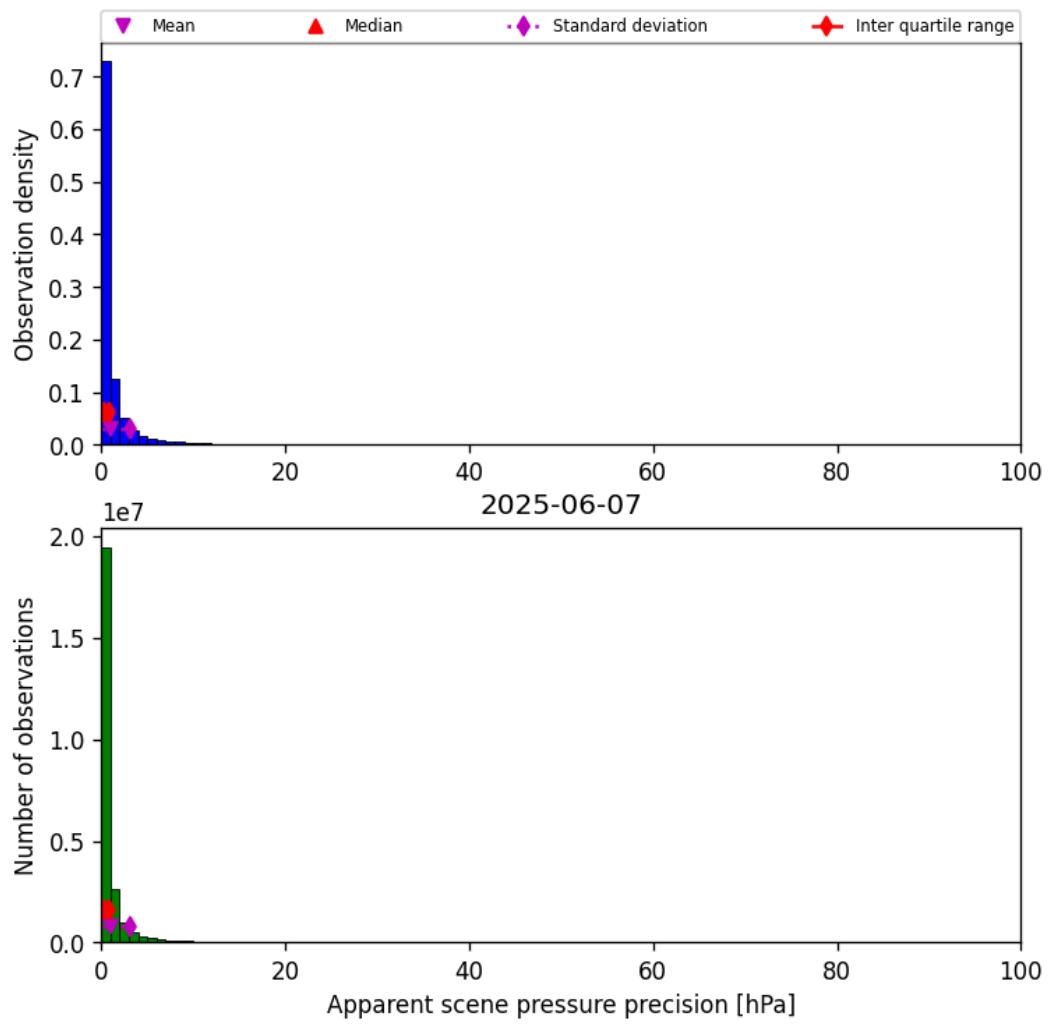
Figure 37: Histogram of “Apparent scene pressure precision” for 2025-06-06 to 2025-06-08
