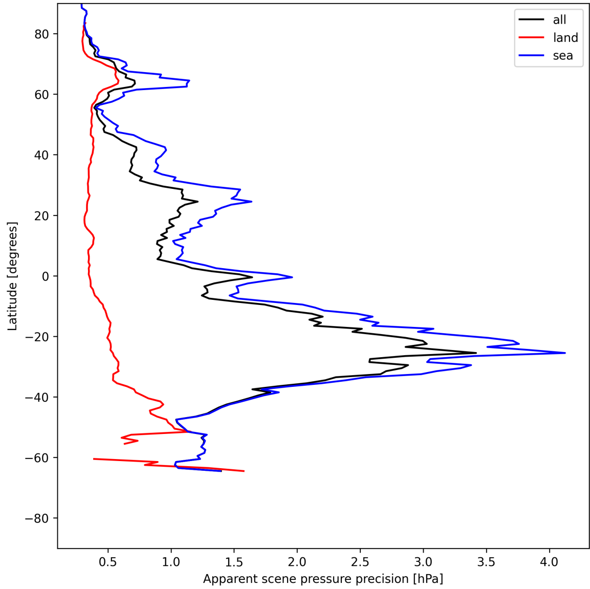
Figure 20: Zonal average of “Apparent scene pressure precision” for 2025-06-06 to 2025-06-08.
