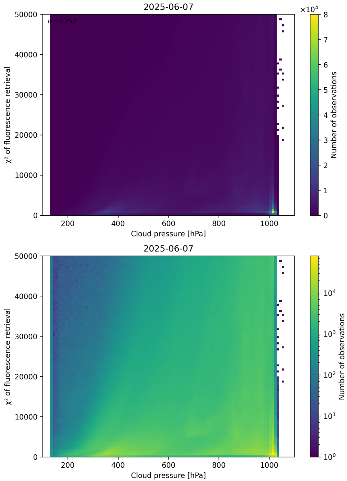
Figure 78: Scatter density plot of “Cloud pressure” against “ \chi^2 of fluorescence retrieval” for 2025-06-06 to 2025-06-08.
