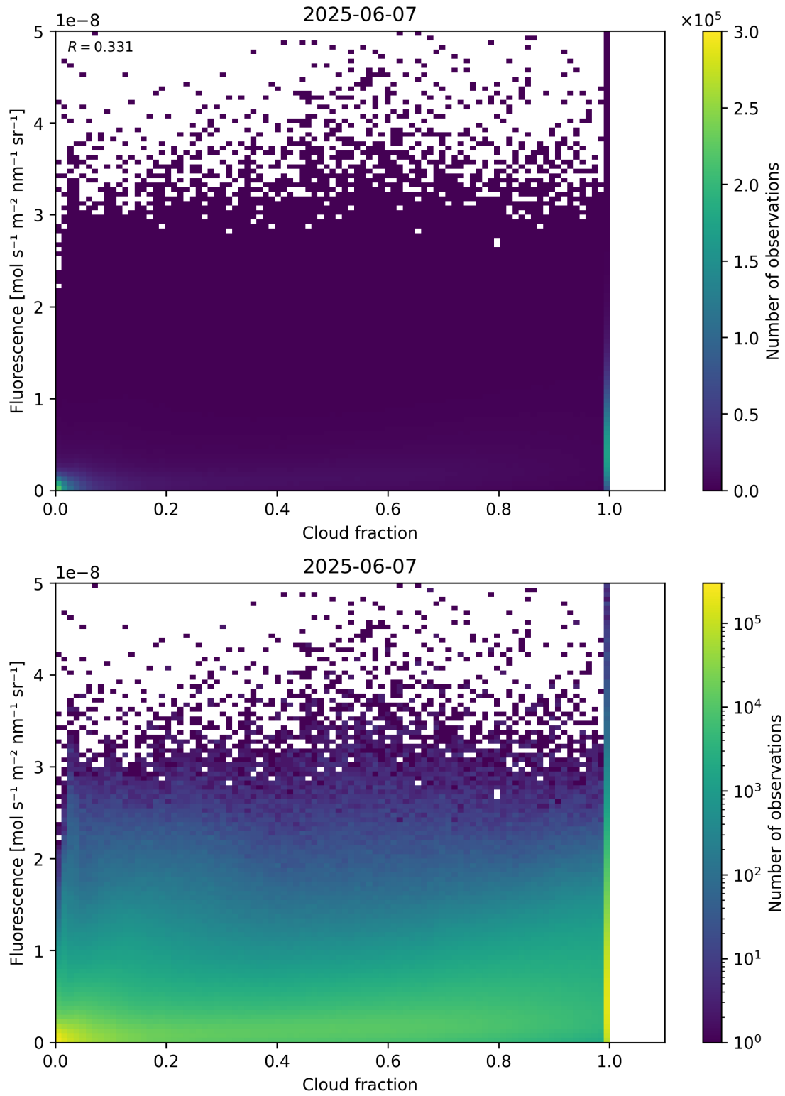
Figure 72: Scatter density plot of “Cloud fraction” against “Fluorescence” for 2025-06-06 to 2025-06-08.
