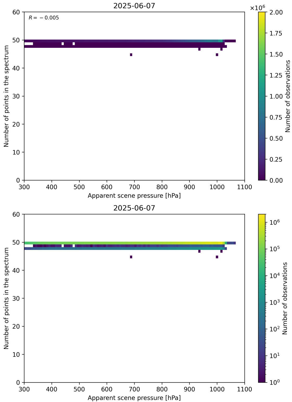
Figure 66: Scatter density plot of “Apparent scene pressure” against “Number of points in the spectrum” for 2025-06-06 to 2025-06-08.
