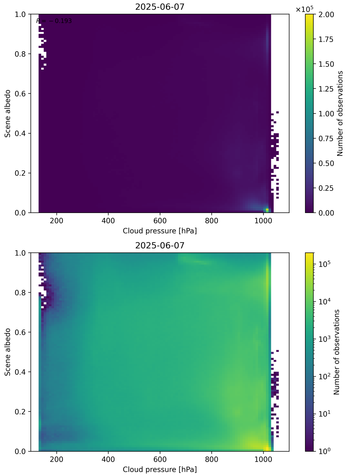
Figure 83: Scatter density plot of “Cloud pressure” against “Scene albedo” for 2025-06-06 to 2025-06-08.
