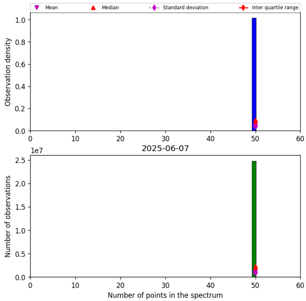
Figure 44: Histogram of “Number of points in the spectrum” for 2025-06-06 to 2025-06-08
