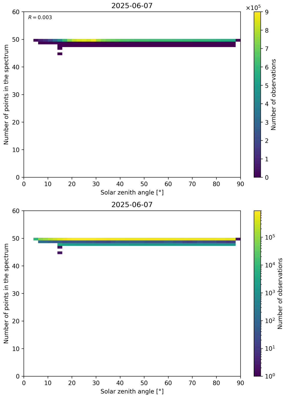
Figure 115: Scatter density plot of “Solar zenith angle” against “Number of points in the spectrum” for 2025-06-06 to 2025-06-08.
