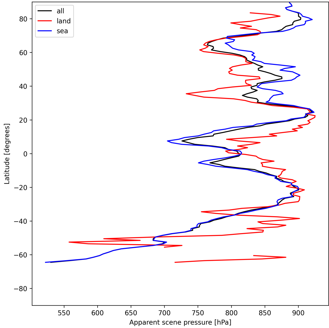
Figure 19: Zonal average of “Apparent scene pressure” for 2025-06-06 to 2025-06-08.
