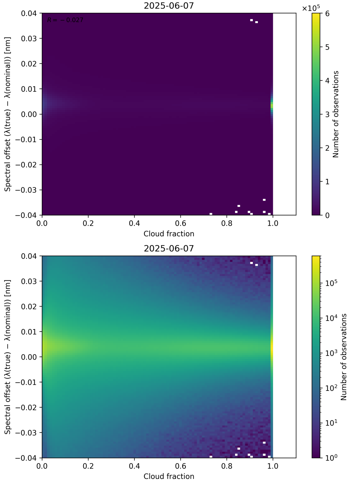
Figure 76: Scatter density plot of “Cloud fraction” against “Spectral offset ( \lambda_{\text{true}} - \lambda_{\text{nominal}} )” for 2025-06-06 to 2025-06-08.
