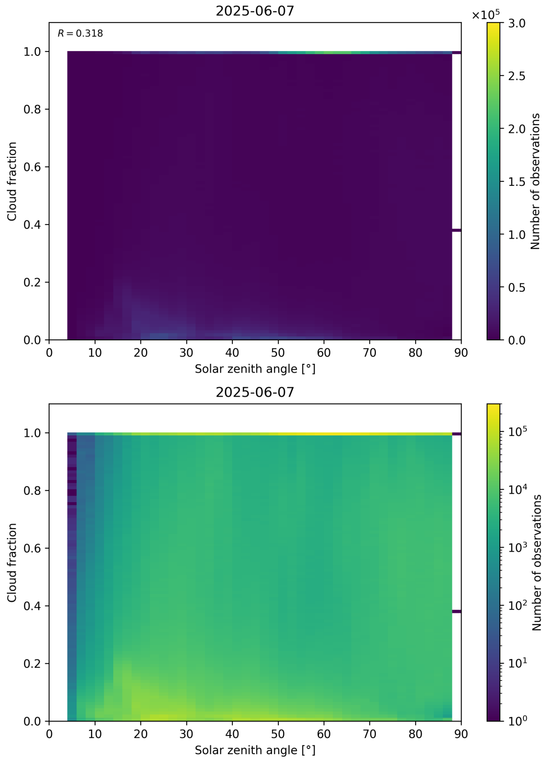
Figure 110: Scatter density plot of “Solar zenith angle” against “Cloud fraction” for 2025-06-06 to 2025-06-08.
