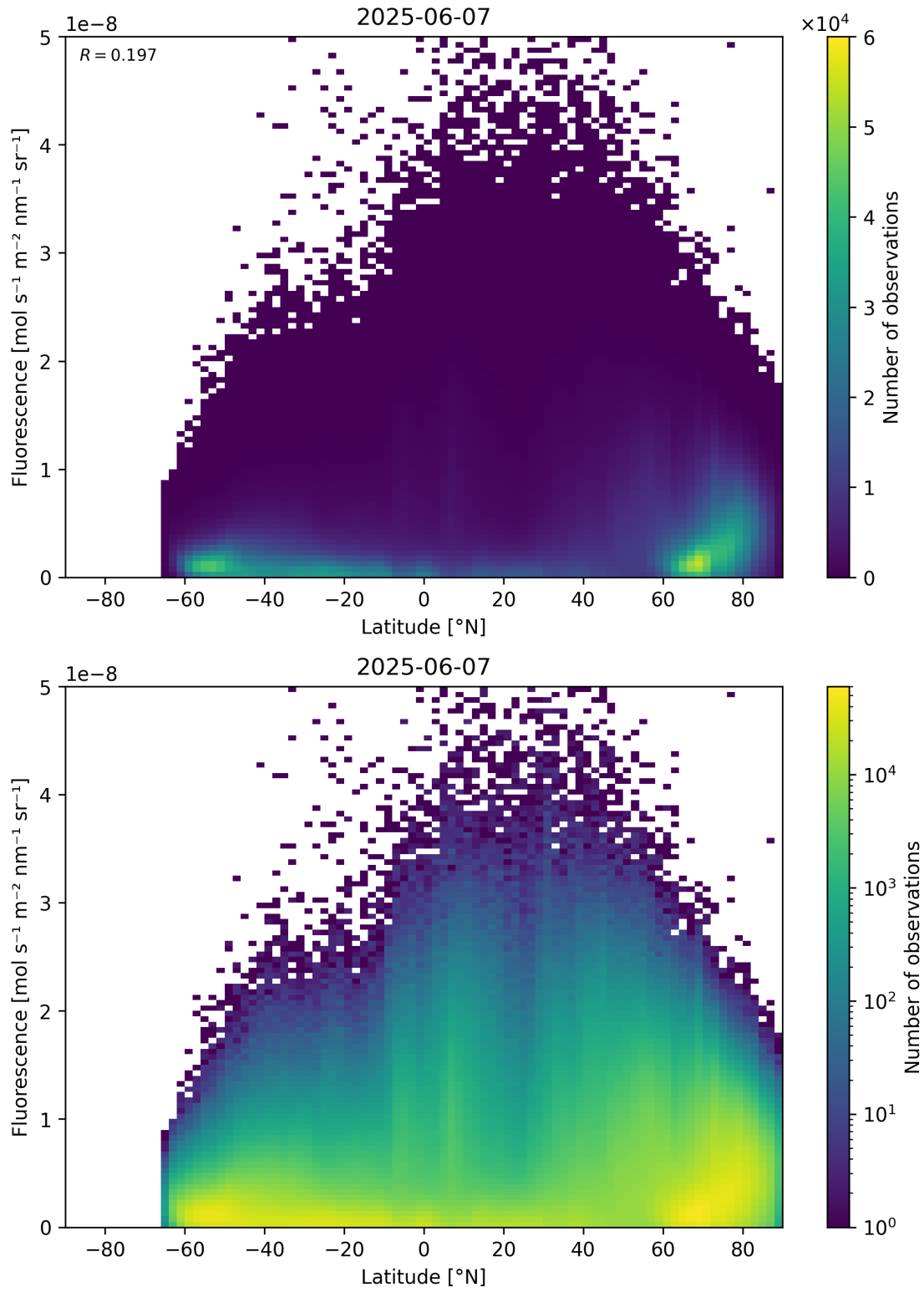
Figure 92: Scatter density plot of “Latitude” against “Fluorescence” for 2025-06-06 to 2025-06-08.
