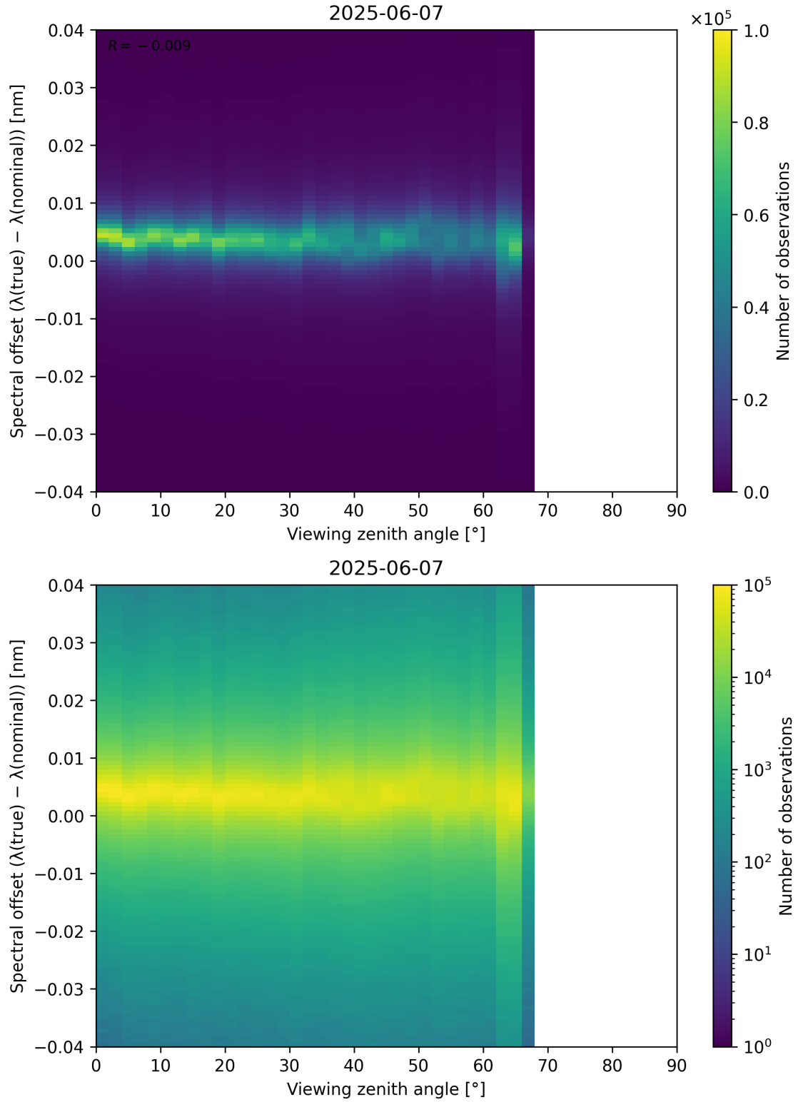
Figure 128: Scatter density plot of “Viewing zenith angle” against “Spectral offset ( \lambda_{\text{true}} - \lambda_{\text{nominal}} )” for 2025-06-06 to 2025-06-08.
