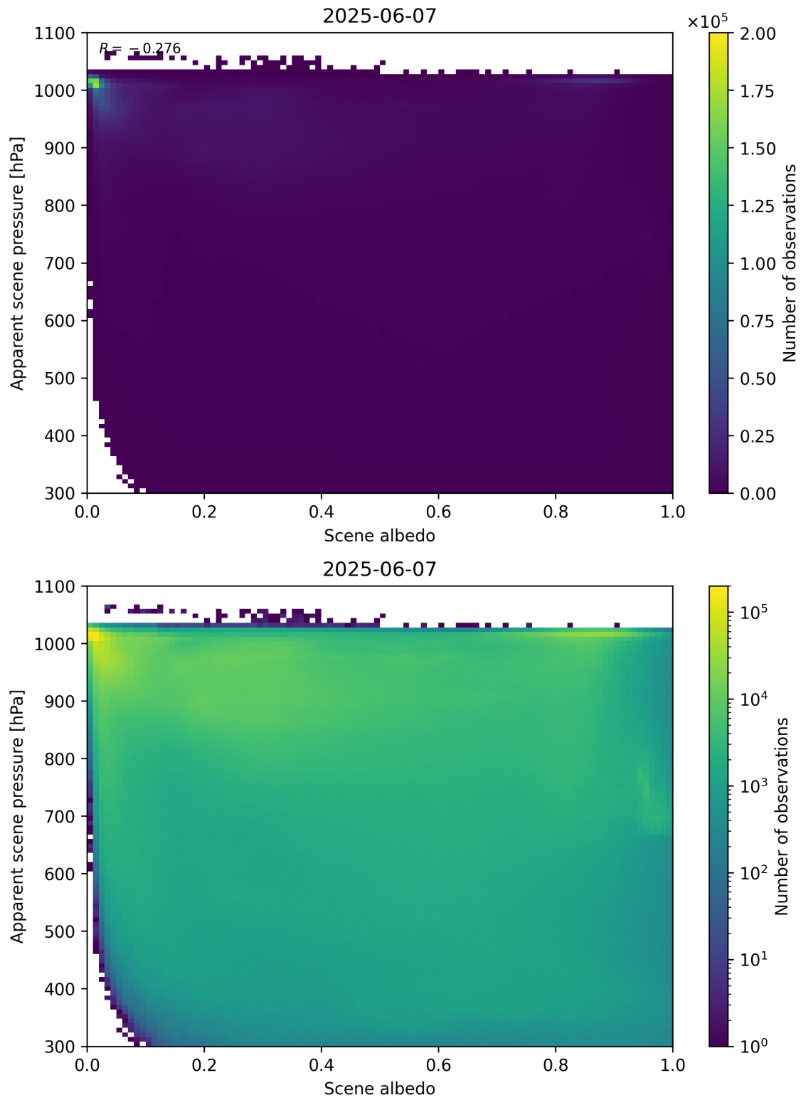
Figure 102: Scatter density plot of “Scene albedo” against “Apparent scene pressure” for 2025-06-06 to 2025-06-08.
