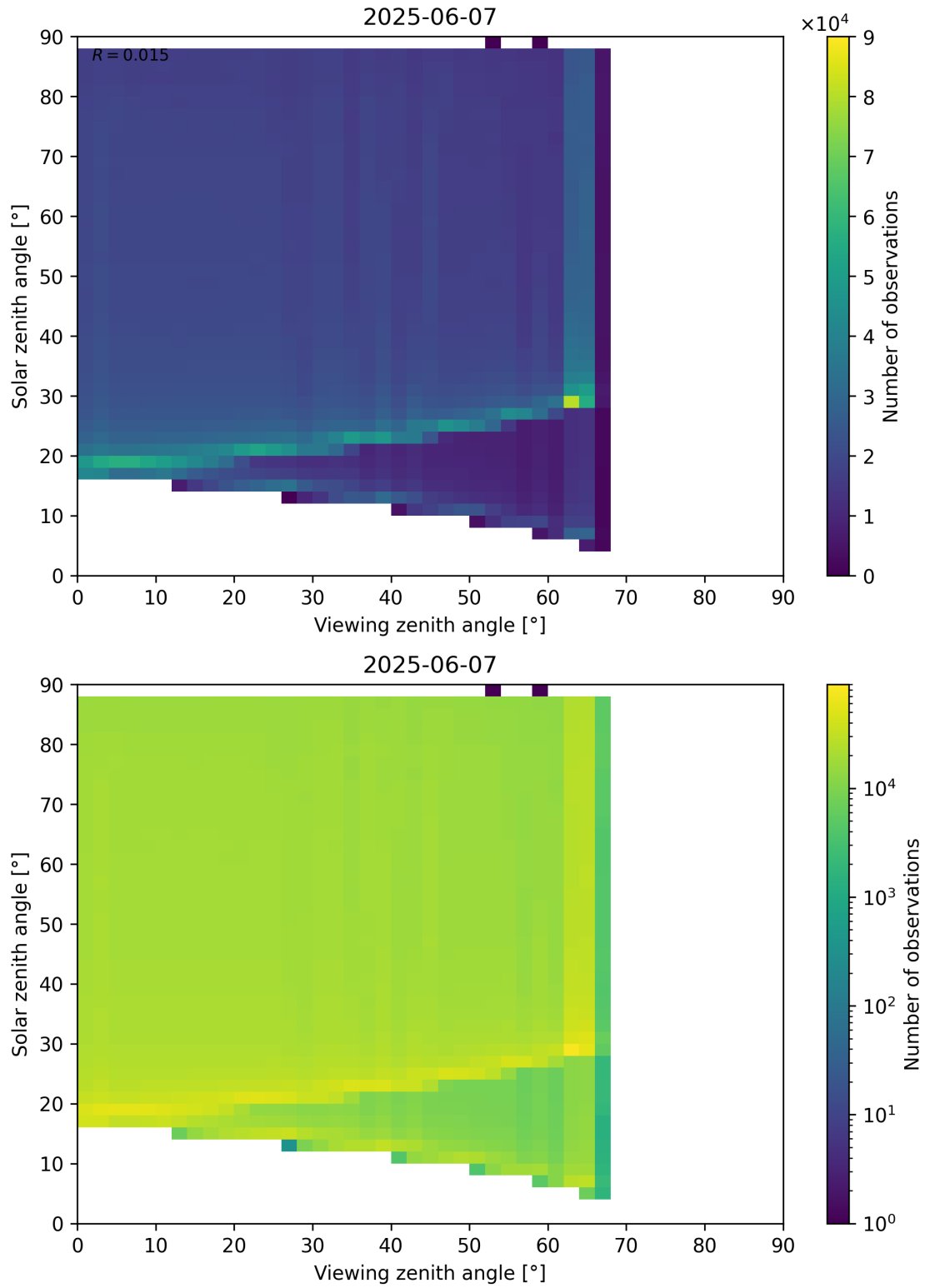
Figure 127: Scatter density plot of “Viewing zenith angle” against “Solar zenith angle” for 2025-06-06 to 2025-06-08.
