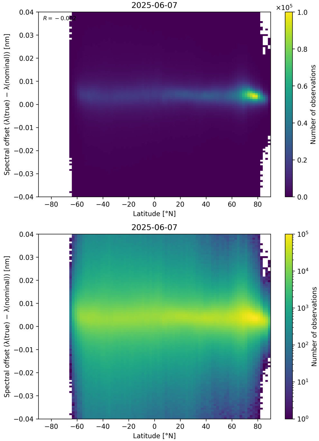
Figure 96: Scatter density plot of “Latitude” against “Spectral offset ( \lambda_{\text{true}} - \lambda_{\text{nominal}} )” for 2025-06-06 to 2025-06-08.
