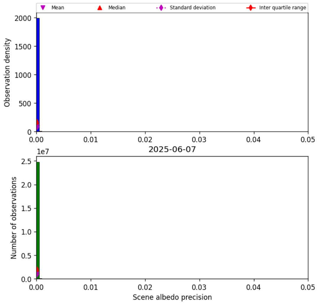
Figure 35: Histogram of “Scene albedo precision” for 2025-06-06 to 2025-06-08
