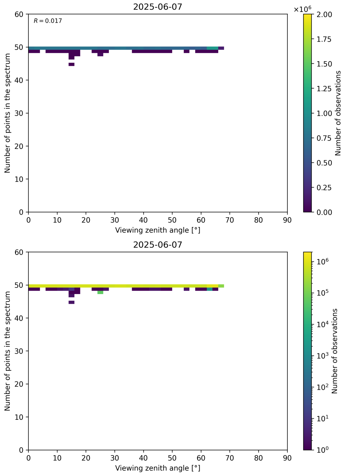
Figure 125: Scatter density plot of “Viewing zenith angle” against “Number of points in the spectrum” for 2025-06-06 to 2025-06-08.
