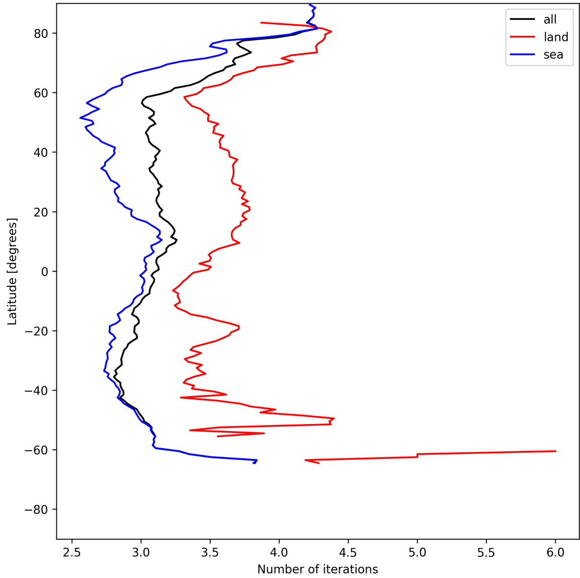
Figure 22: Zonal average of “Number of iterations” for 2025-06-06 to 2025-06-08.
