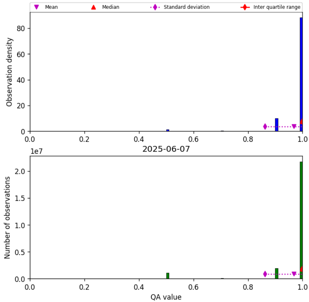
Figure 29: Histogram of “QA value” for 2025-06-06 to 2025-06-08
