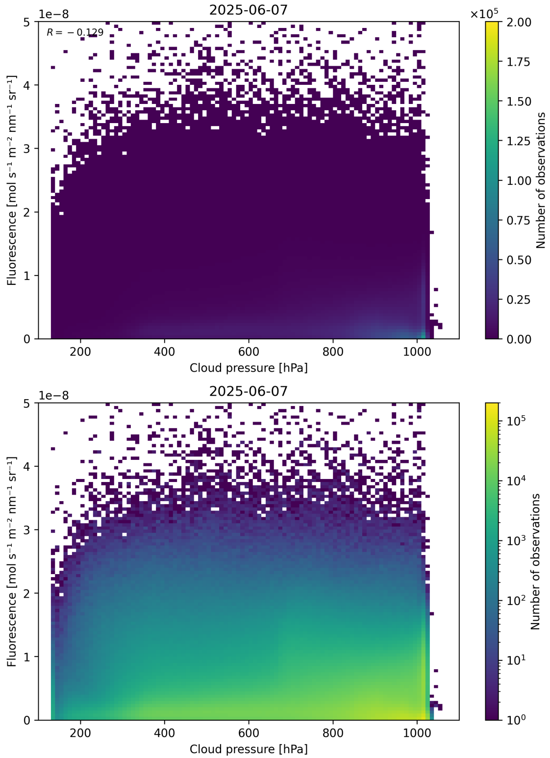
Figure 80: Scatter density plot of “Cloud pressure” against “Fluorescence” for 2025-06-06 to 2025-06-08.
