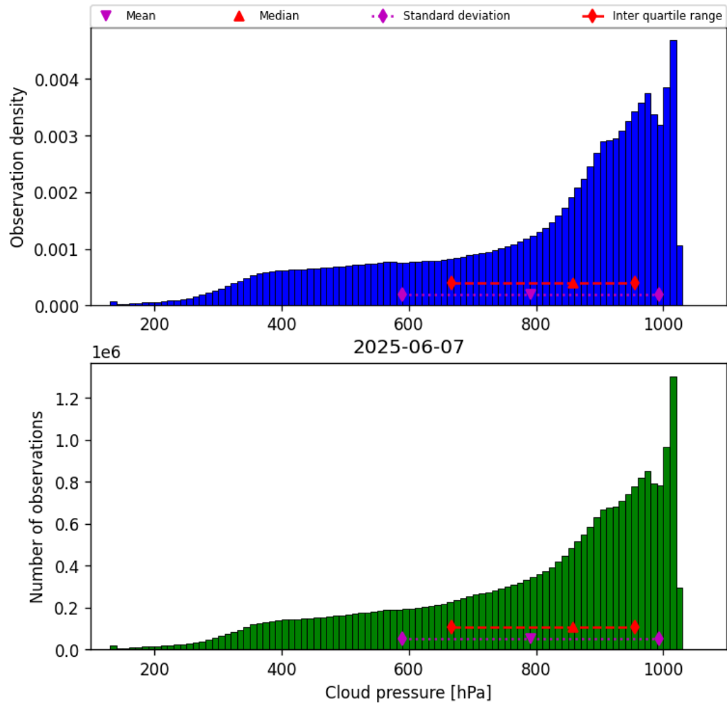
Figure 30: Histogram of “Cloud pressure” for 2025-06-06 to 2025-06-08
