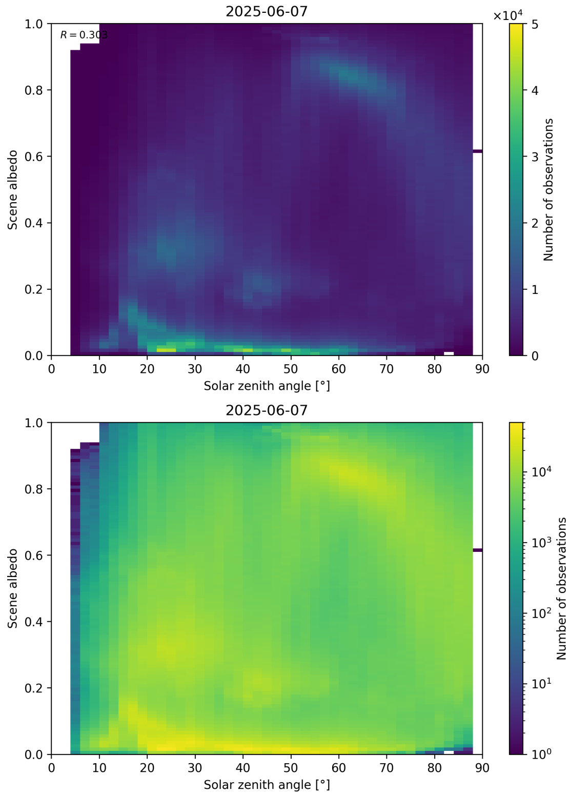
Figure 116: Scatter density plot of “Solar zenith angle” against “Scene albedo” for 2025-06-06 to 2025-06-08.
