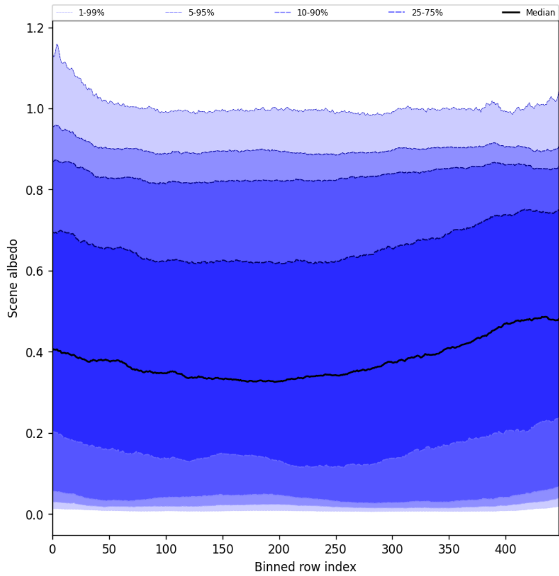
Figure 51: Along track statistics of “Scene albedo” for 2025-06-06 to 2025-06-08
