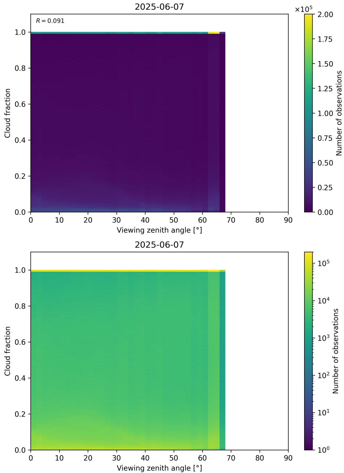
Figure 120: Scatter density plot of “Viewing zenith angle” against “Cloud fraction” for 2025-06-06 to 2025-06-08.
