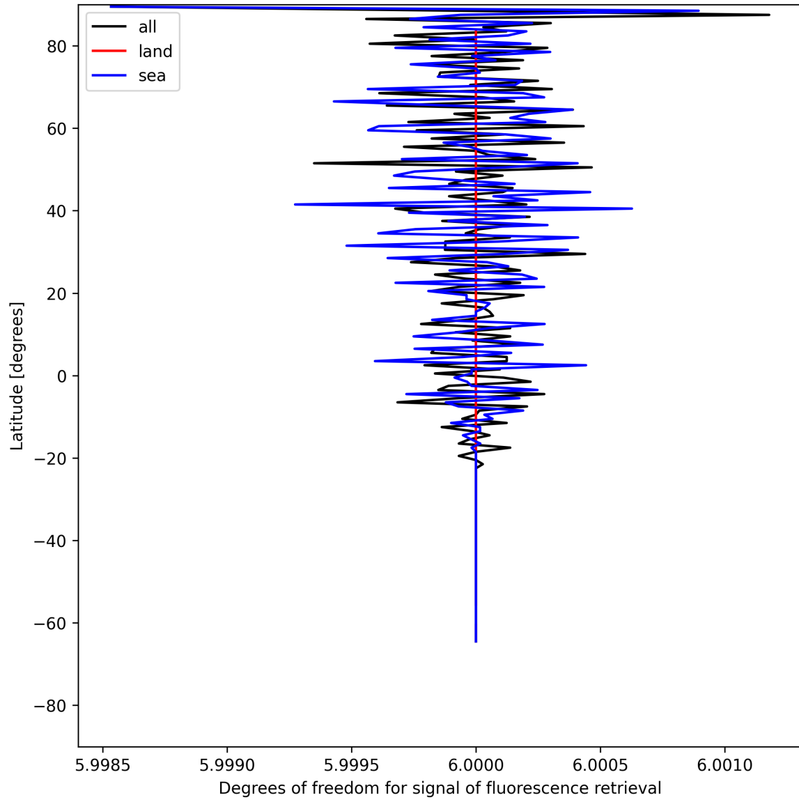
Figure 26: Zonal average of “Degrees of freedom for signal of fluorescence retrieval” for 2025-06-06 to 2025-06-08.
