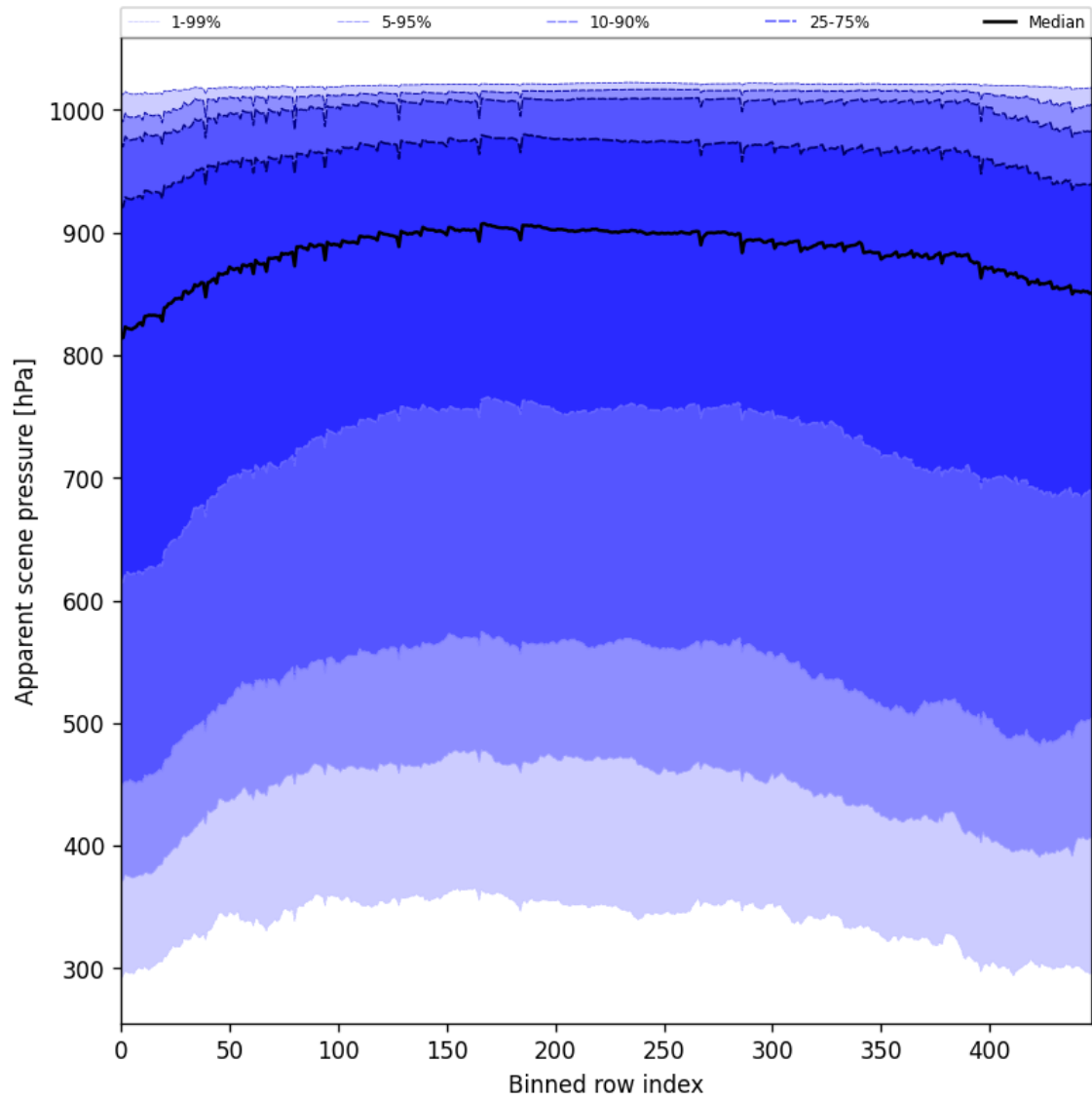
Figure 53: Along track statistics of “Apparent scene pressure” for 2025-06-06 to 2025-06-08
