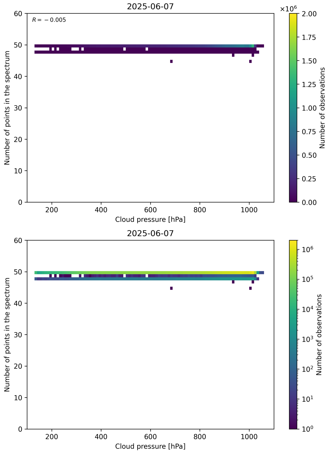
Figure 82: Scatter density plot of “Cloud pressure” against “Number of points in the spectrum” for 2025-06-06 to 2025-06-08.
