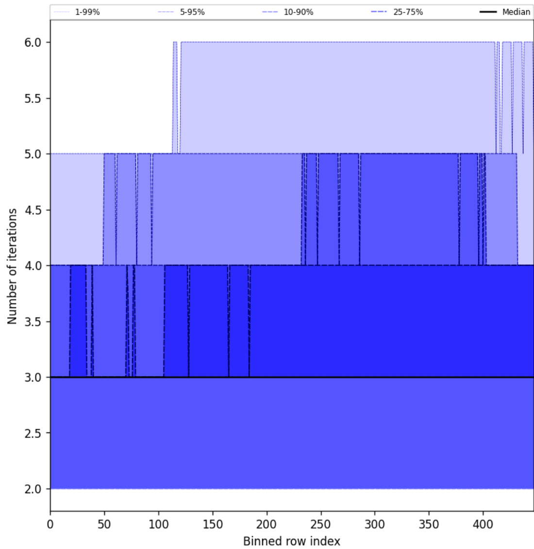
Figure 56: Along track statistics of “Number of iterations” for 2025-06-06 to 2025-06-08
