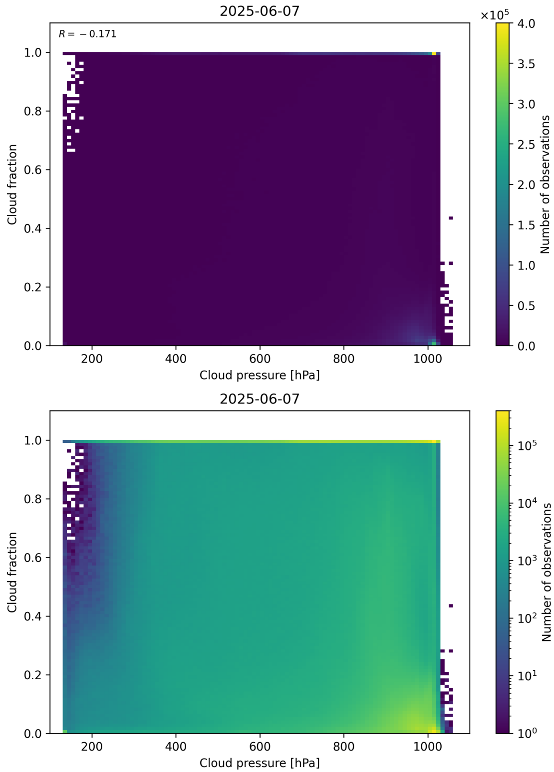
Figure 79: Scatter density plot of “Cloud pressure” against “Cloud fraction” for 2025-06-06 to 2025-06-08.
