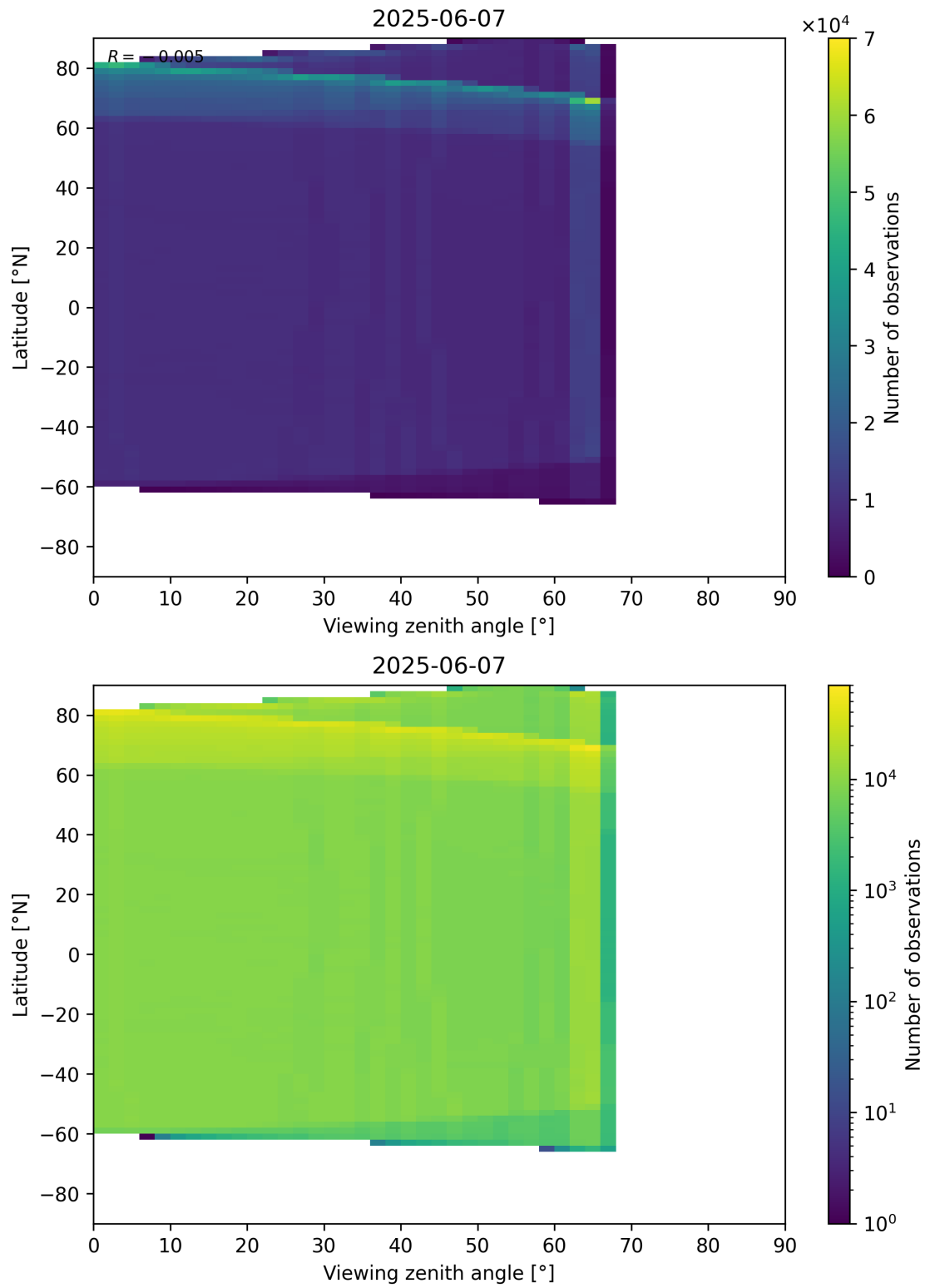
Figure 123: Scatter density plot of “Viewing zenith angle” against “Latitude” for 2025-06-06 to 2025-06-08.
