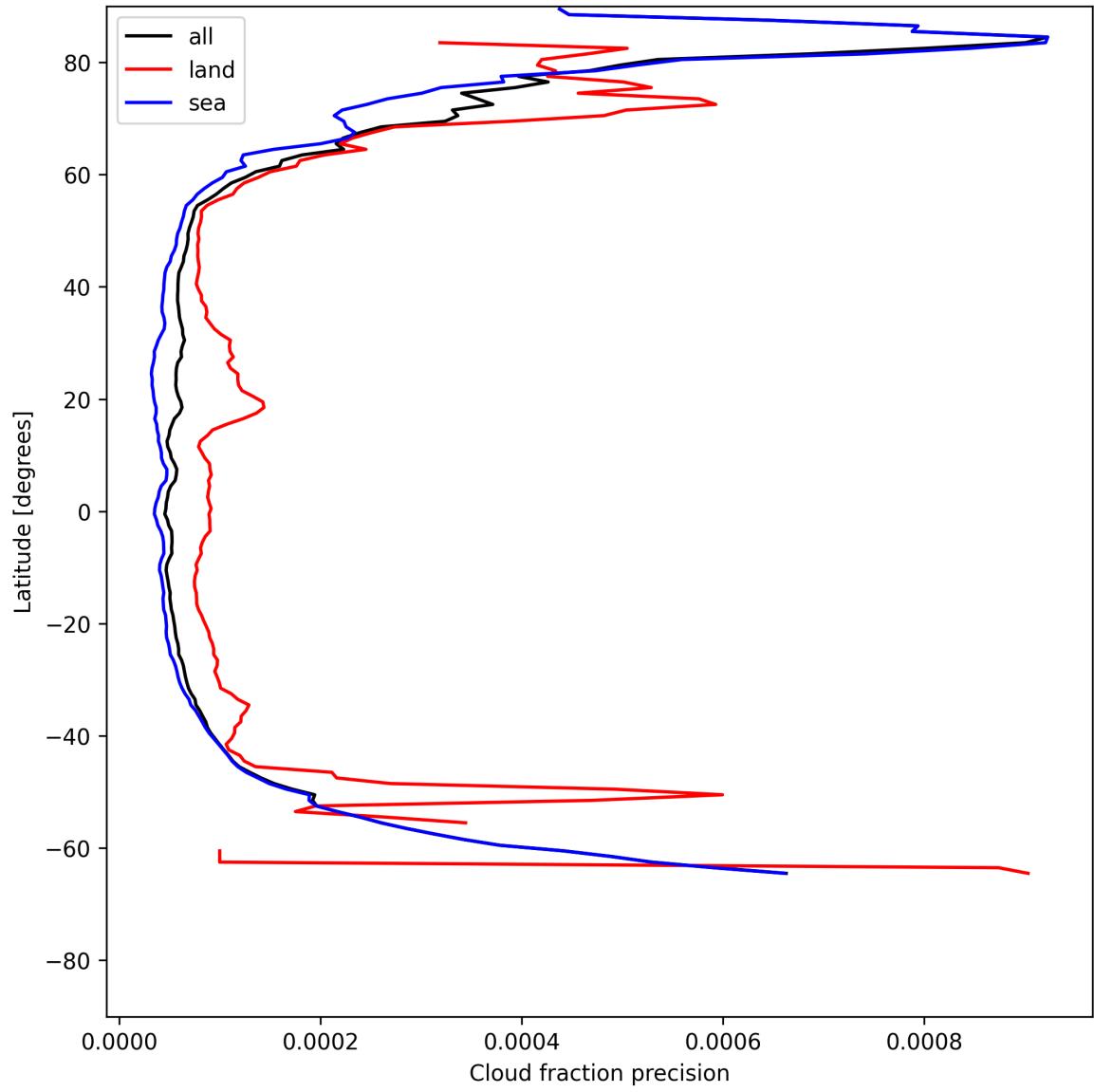
Figure 16: Zonal average of “Cloud fraction precision” for 2025-06-06 to 2025-06-08.
