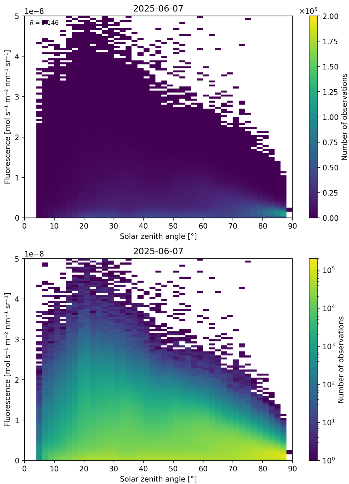
Figure 112: Scatter density plot of “Solar zenith angle” against “Fluorescence” for 2025-06-06 to 2025-06-08.
