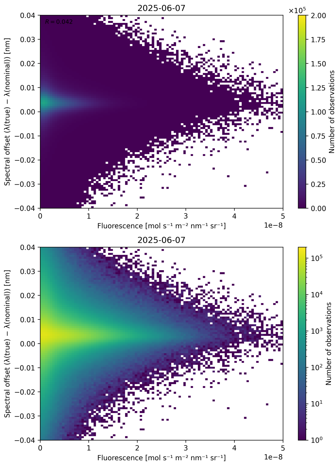
Figure 87: Scatter density plot of “Fluorescence” against “Spectral offset ( \lambda_{\text{true}} - \lambda_{\text{nominal}} )” for 2025-06-06 to 2025-06-08.
