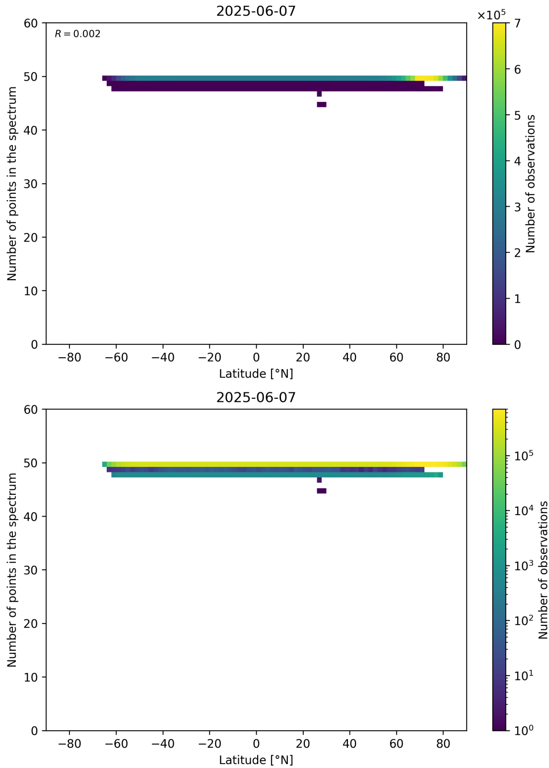
Figure 94: Scatter density plot of “Latitude” against “Number of points in the spectrum” for 2025-06-06 to 2025-06-08.
