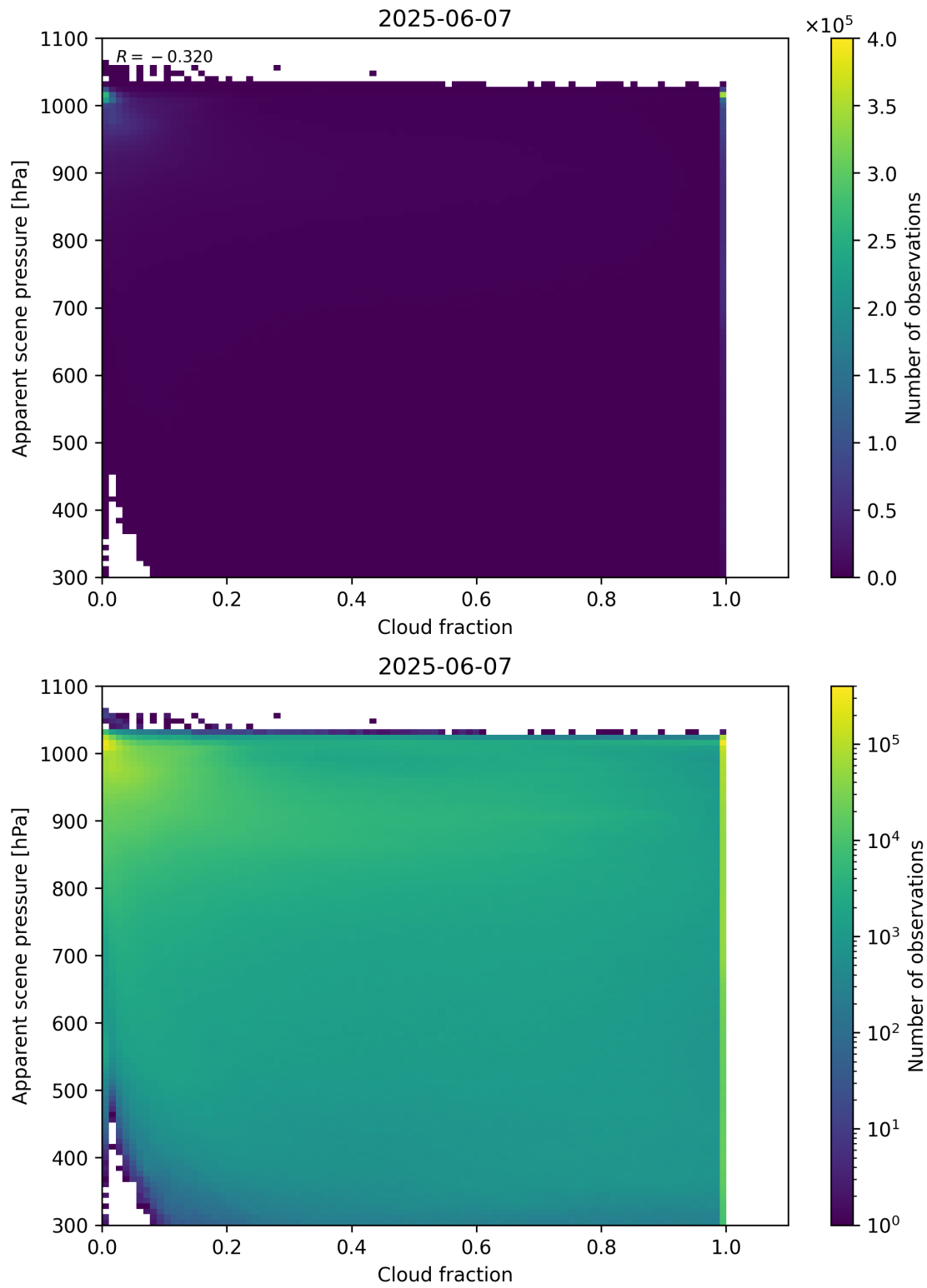
Figure 70: Scatter density plot of “Cloud fraction” against “Apparent scene pressure” for 2025-06-06 to 2025-06-08.
