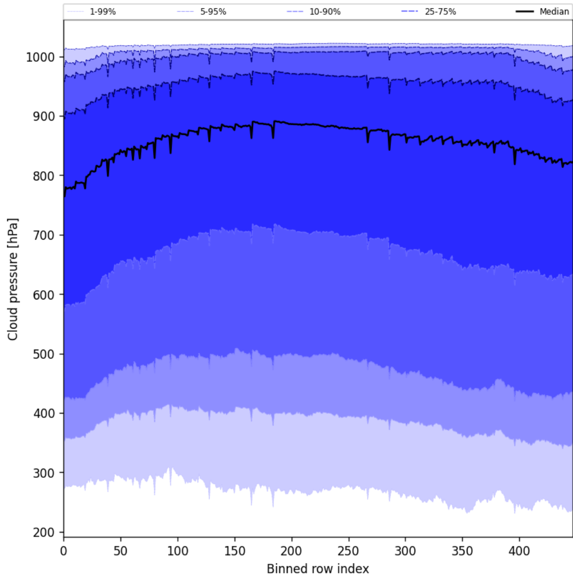
Figure 47: Along track statistics of “Cloud pressure” for 2025-06-06 to 2025-06-08
