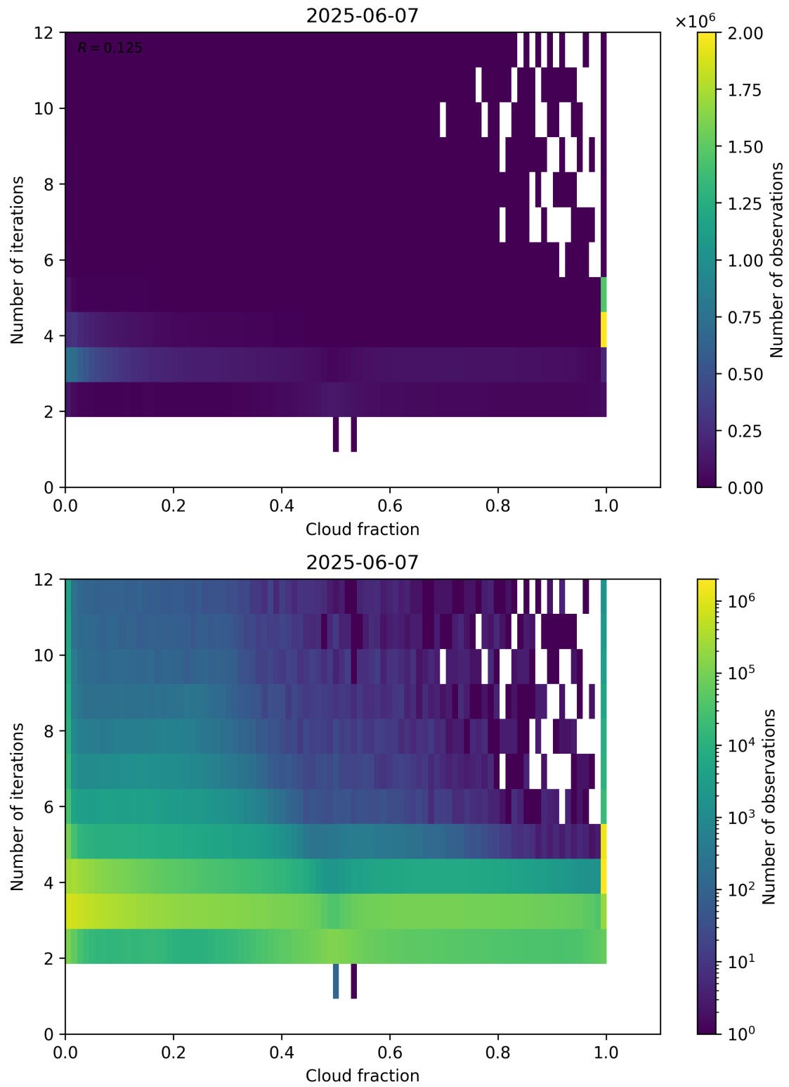
Figure 73: Scatter density plot of “Cloud fraction” against “Number of iterations” for 2025-06-06 to 2025-06-08.
