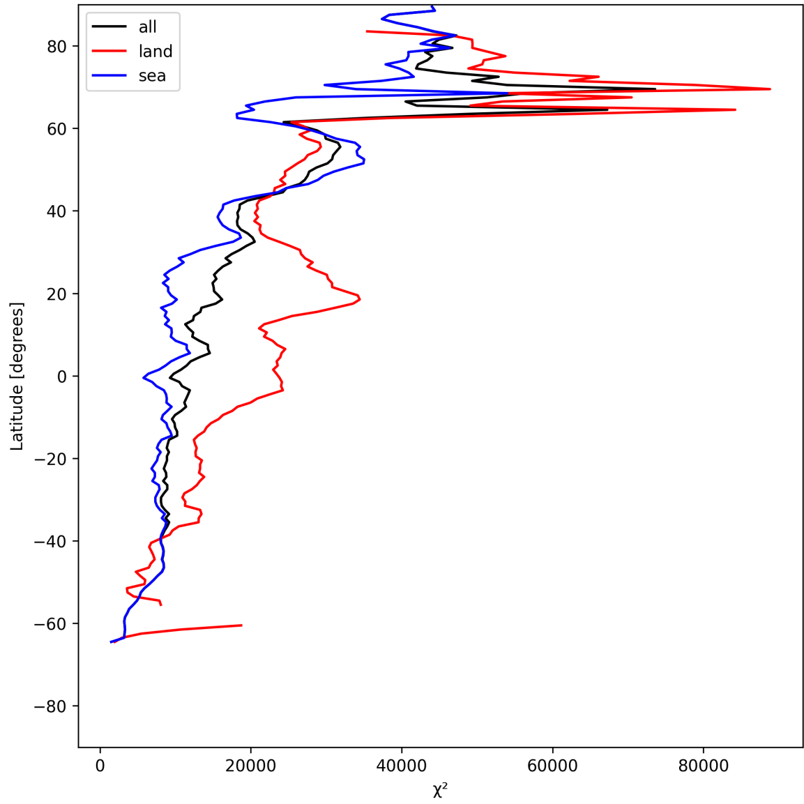
Figure 21: Zonal average of “ \chi^2 ” for 2025-06-06 to 2025-06-08.
