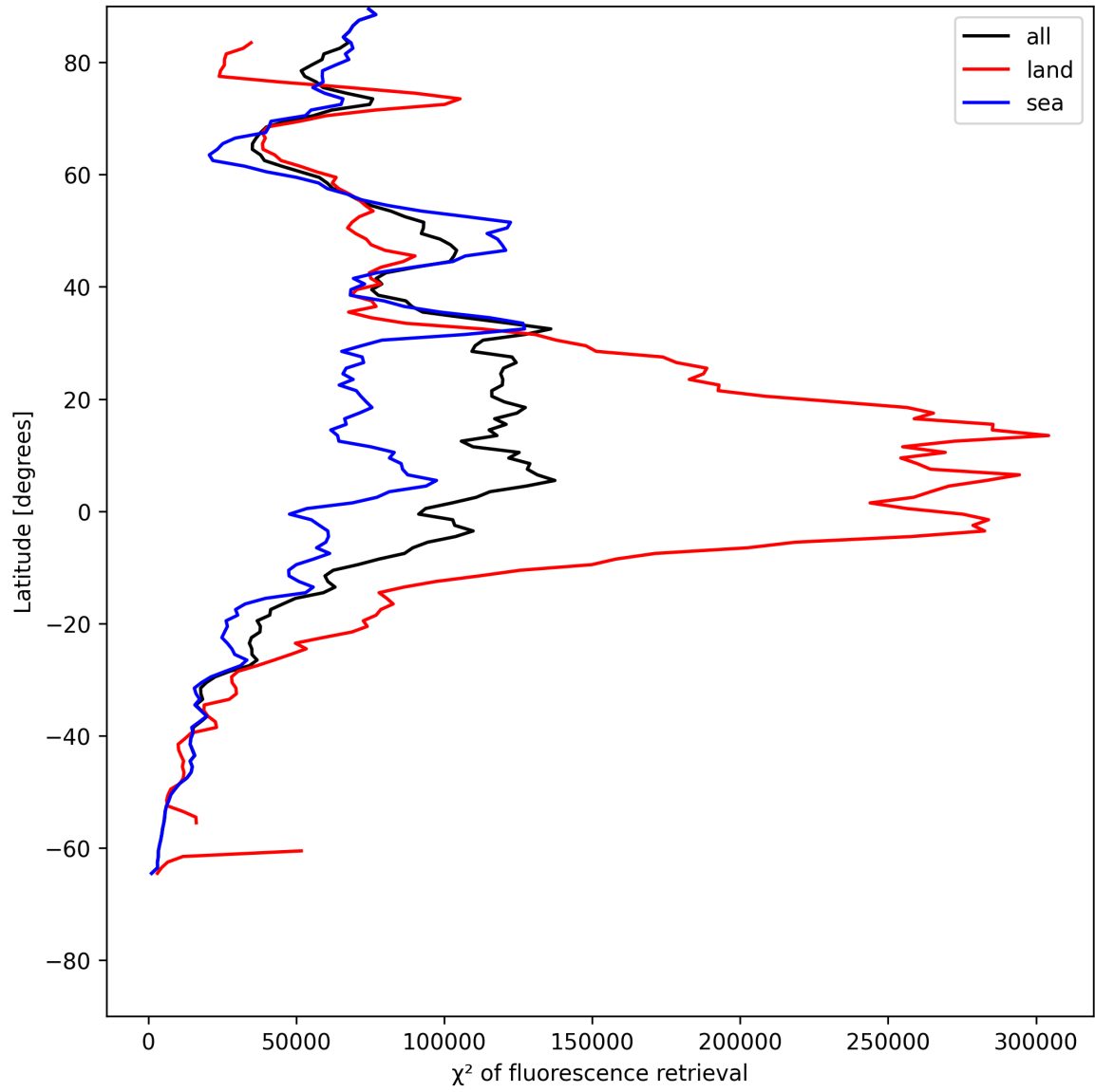
Figure 25: Zonal average of “ \chi^2 of fluorescence retrieval” for 2025-06-06 to 2025-06-08.
