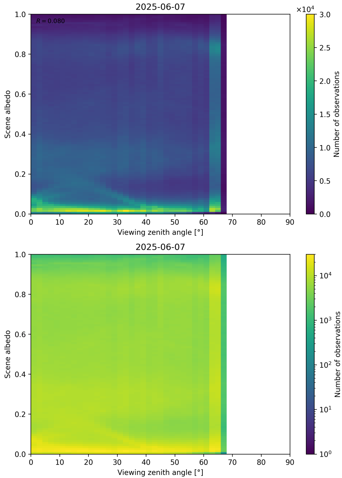
Figure 126: Scatter density plot of “Viewing zenith angle” against “Scene albedo” for 2025-06-06 to 2025-06-08.
