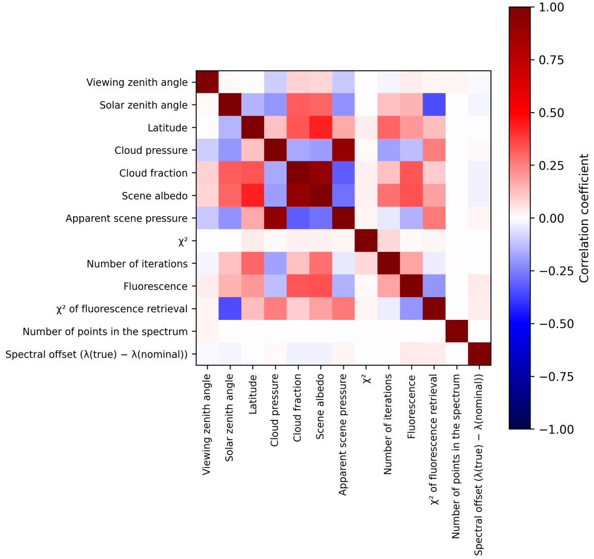
Figure 2: Map of correlation matrix for 2025-06-06 to 2025-06-08.
