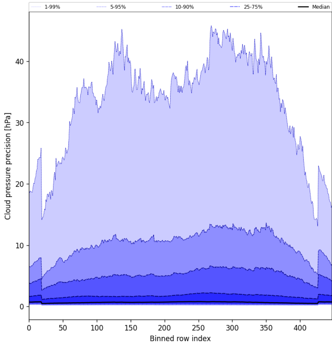
Figure 48: Along track statistics of “Cloud pressure precision” for 2025-06-06 to 2025-06-08
