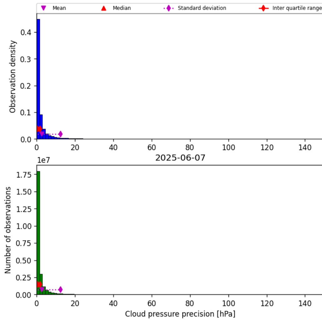
Figure 31: Histogram of “Cloud pressure precision” for 2025-06-06 to 2025-06-08
