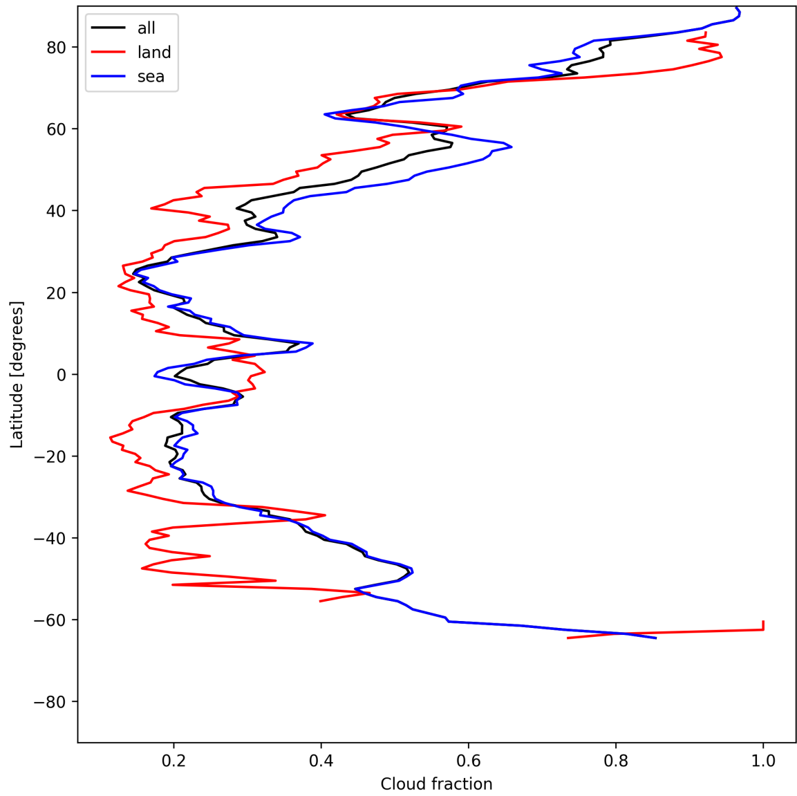
Figure 15: Zonal average of “Cloud fraction” for 2025-06-06 to 2025-06-08.
