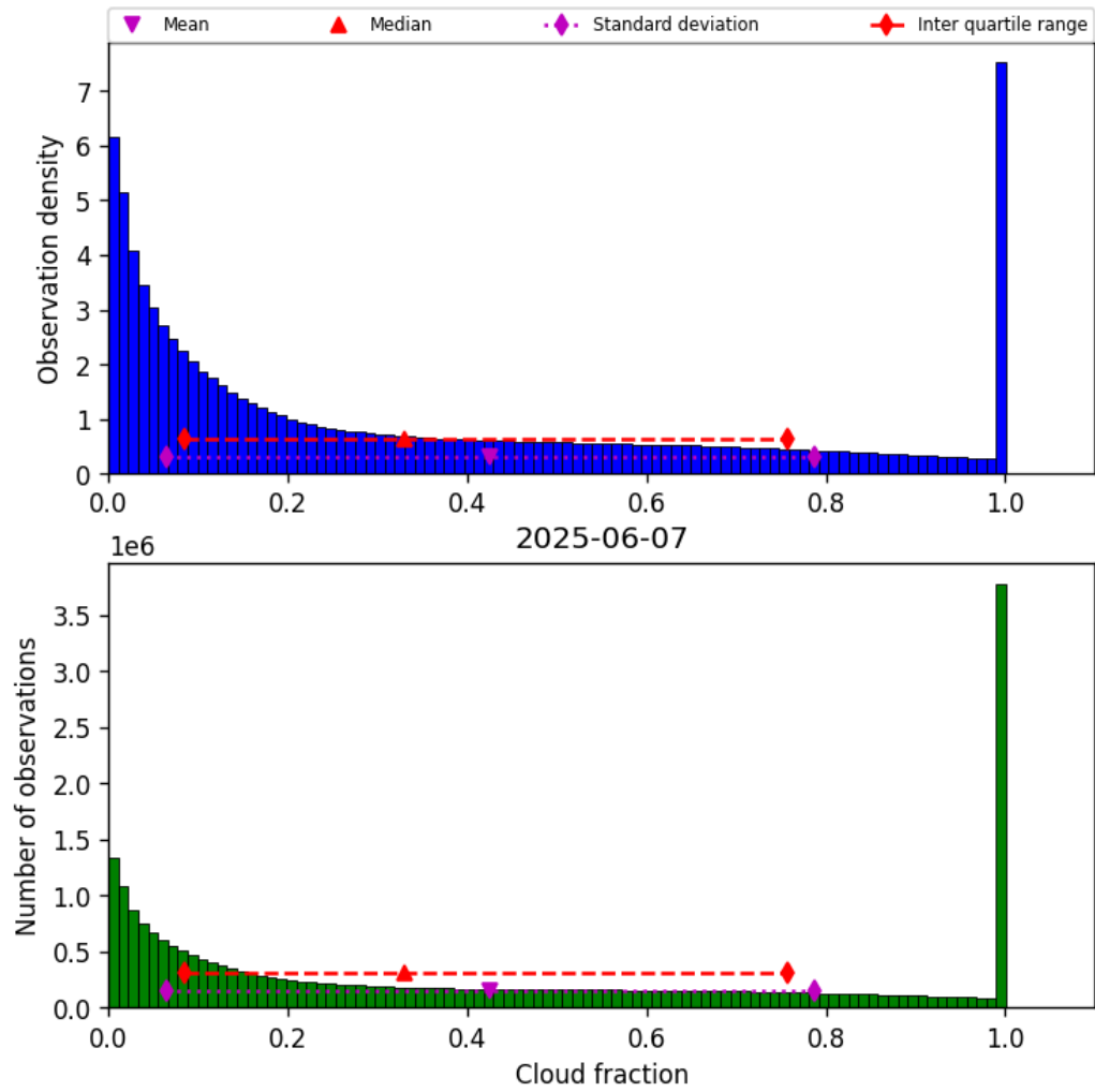
Figure 32: Histogram of “Cloud fraction” for 2025-06-06 to 2025-06-08
