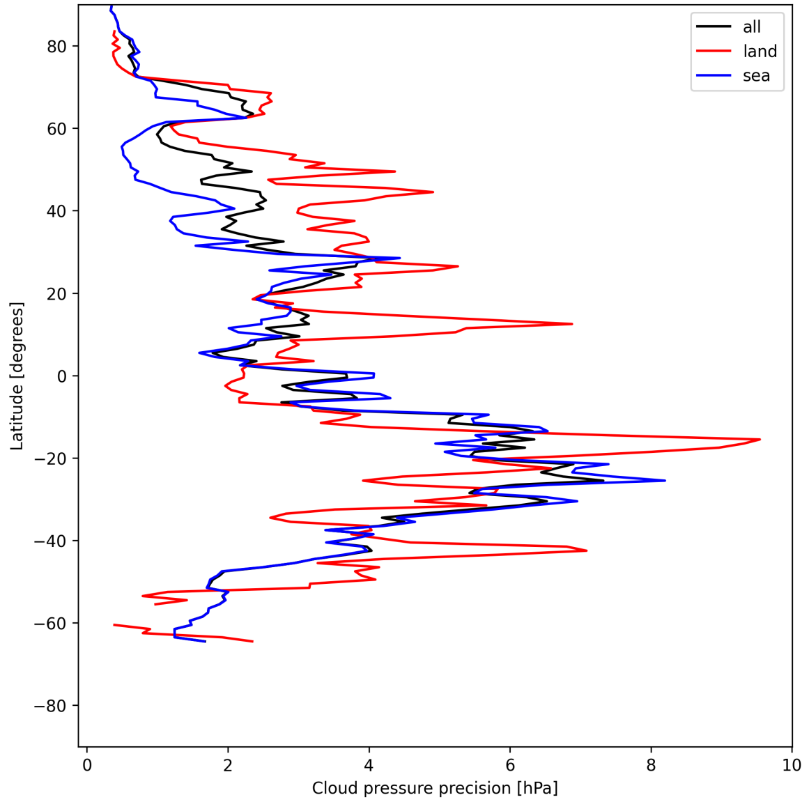
Figure 14: Zonal average of “Cloud pressure precision” for 2025-06-06 to 2025-06-08.
