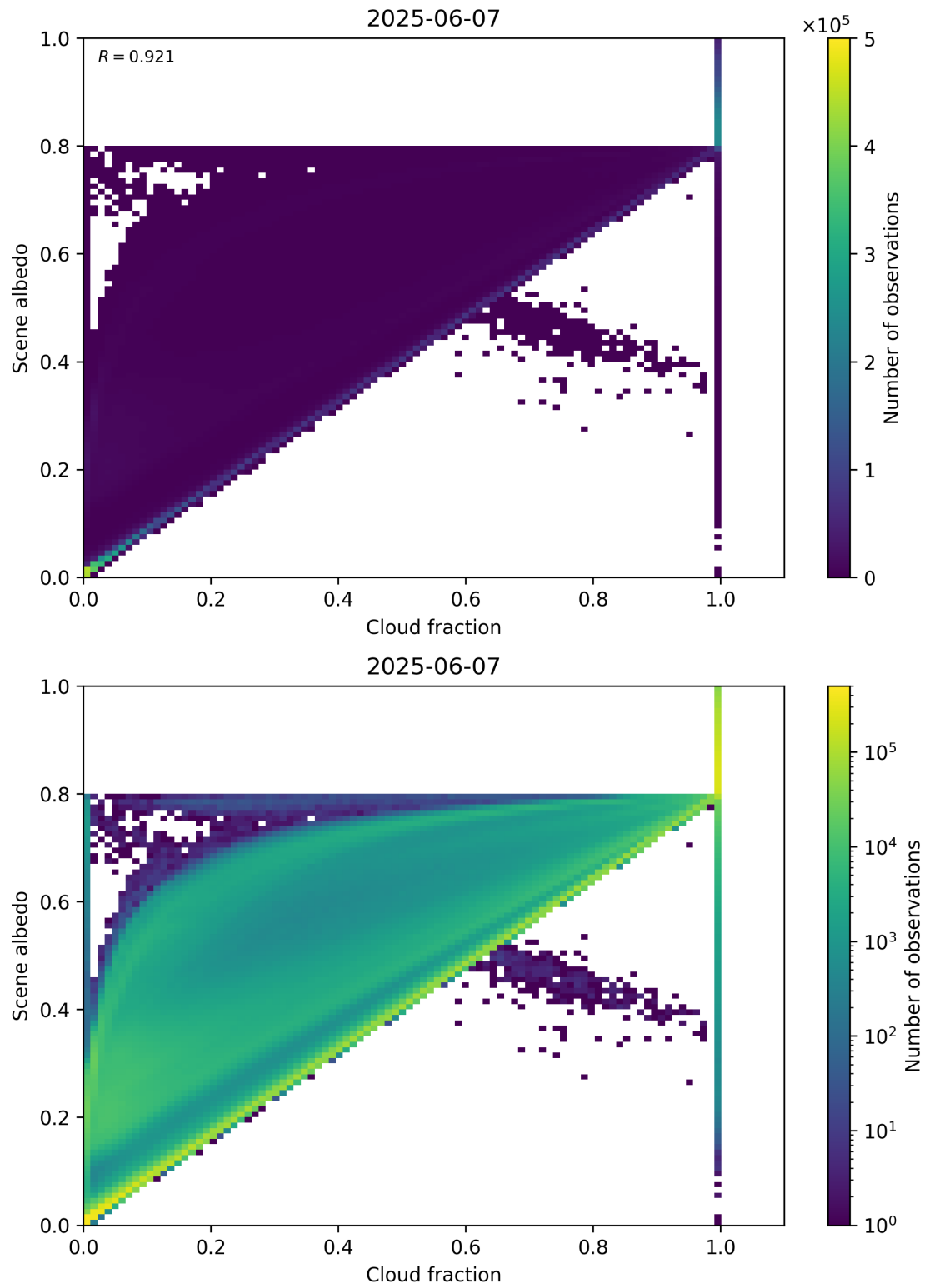
Figure 75: Scatter density plot of “Cloud fraction” against “Scene albedo” for 2025-06-06 to 2025-06-08.
