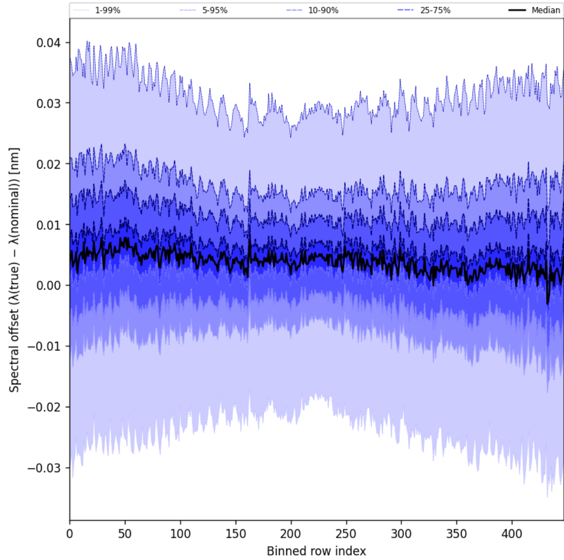
Figure 62: Along track statistics of “Spectral offset ( \lambda_{\text{true}} - \lambda_{\text{nominal}} )” for 2025-06-06 to 2025-06-08
