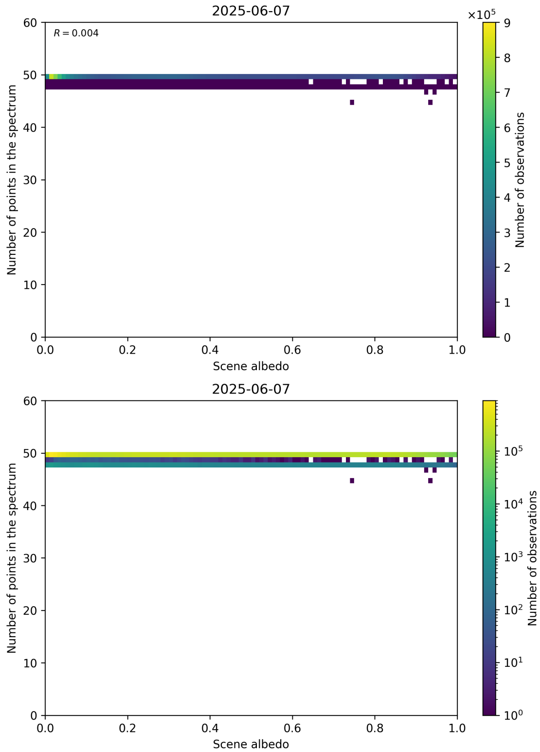
Figure 106: Scatter density plot of “Scene albedo” against “Number of points in the spectrum” for 2025-06-06 to 2025-06-08.
