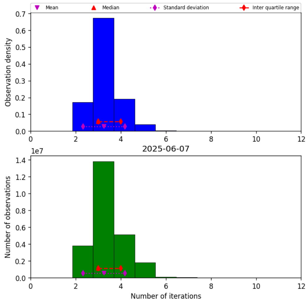
Figure 39: Histogram of “Number of iterations” for 2025-06-06 to 2025-06-08
