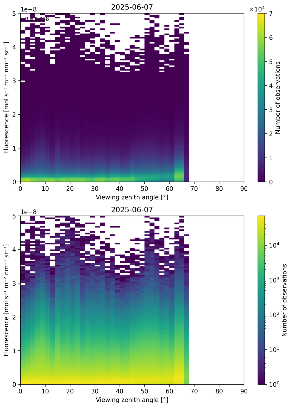
Figure 122: Scatter density plot of “Viewing zenith angle” against “Fluorescence” for 2025-06-06 to 2025-06-08.
