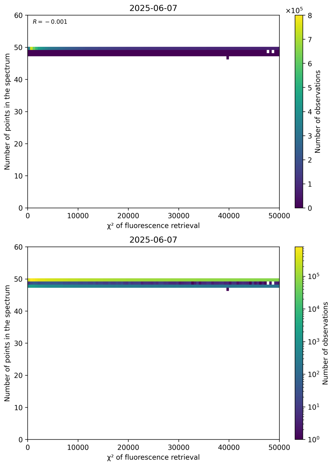
Figure 68: Scatter density plot of “ \chi^2 of fluorescence retrieval” against “Number of points in the spectrum” for 2025-06-06 to 2025-06-08.
