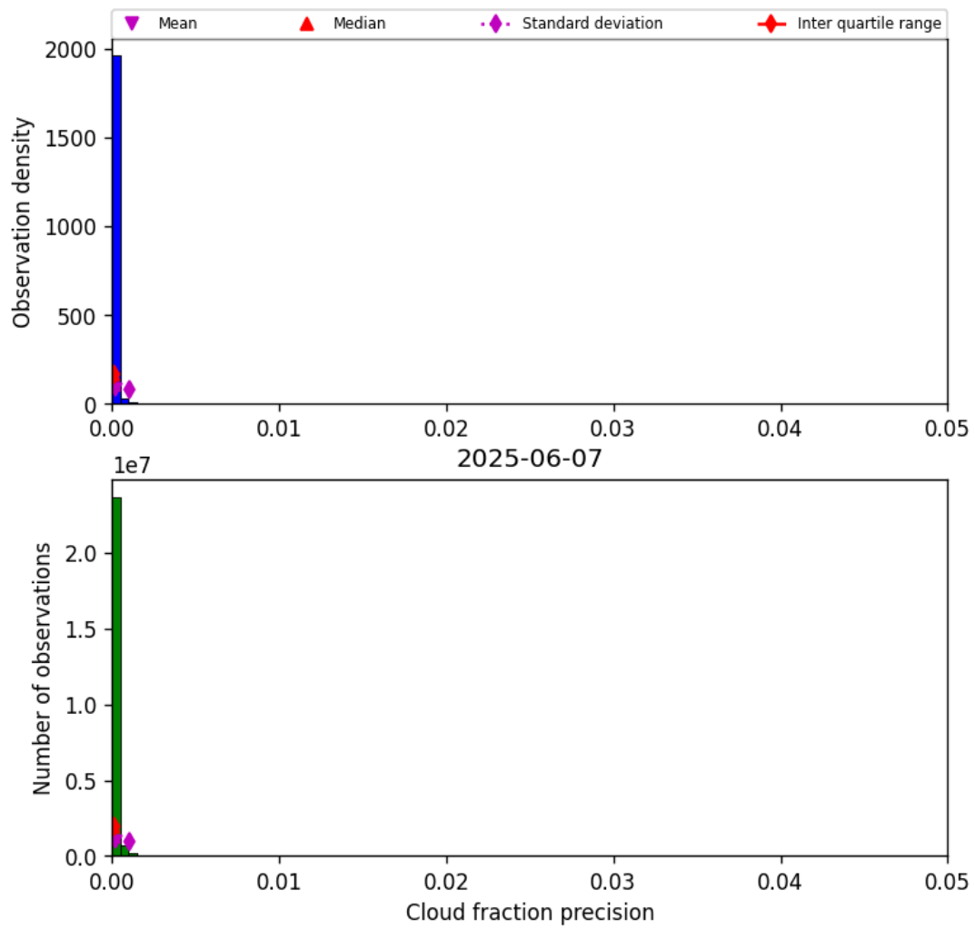
Figure 33: Histogram of “Cloud fraction precision” for 2025-06-06 to 2025-06-08
