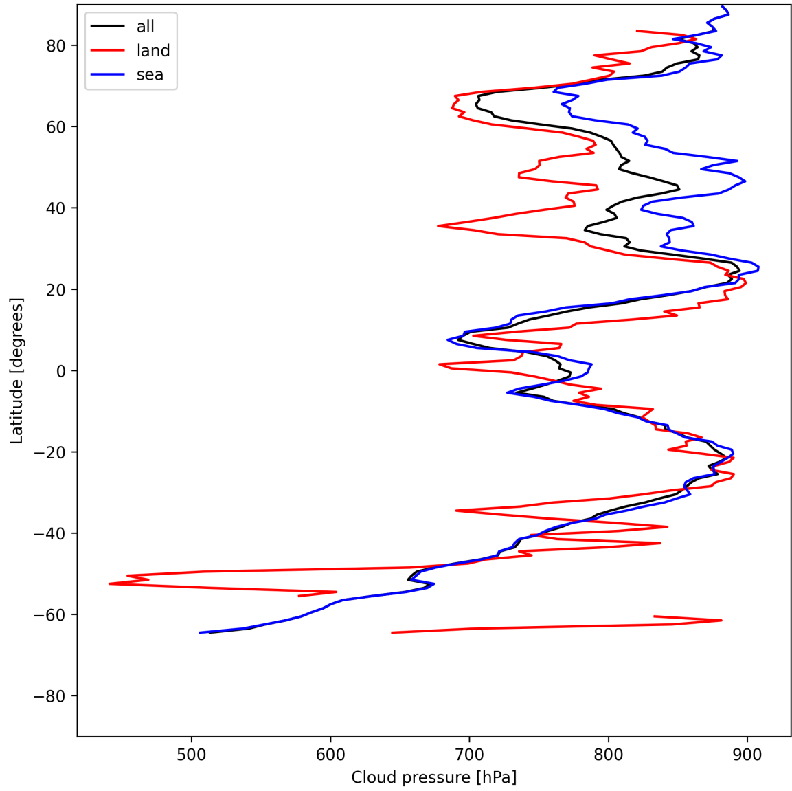
Figure 13: Zonal average of “Cloud pressure” for 2025-06-06 to 2025-06-08.
