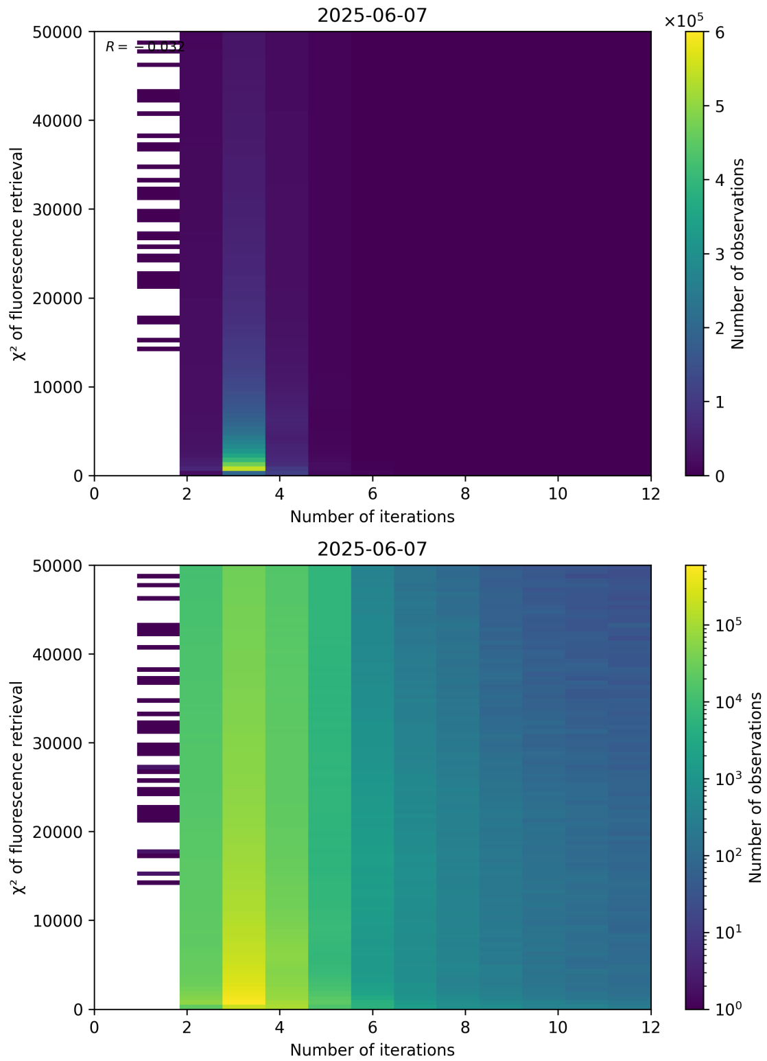
Figure 97: Scatter density plot of “Number of iterations” against “ \chi^2 of fluorescence retrieval” for 2025-06-06 to 2025-06-08.
