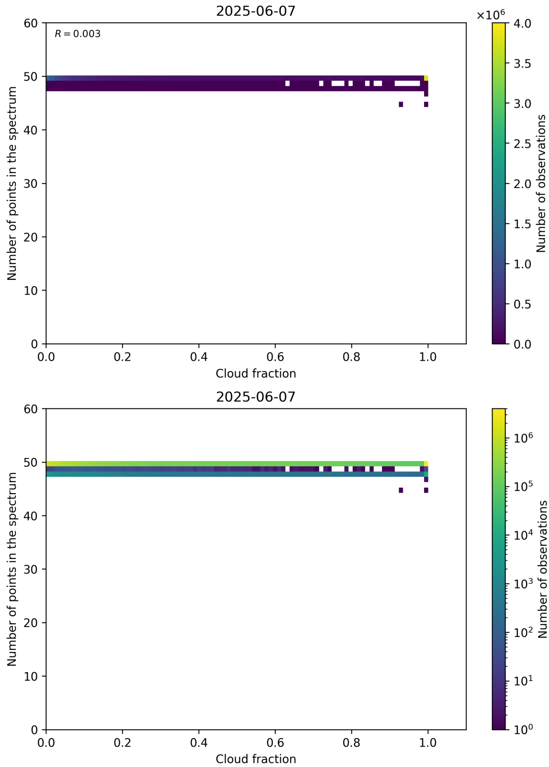
Figure 74: Scatter density plot of “Cloud fraction” against “Number of points in the spectrum” for 2025-06-06 to 2025-06-08.
