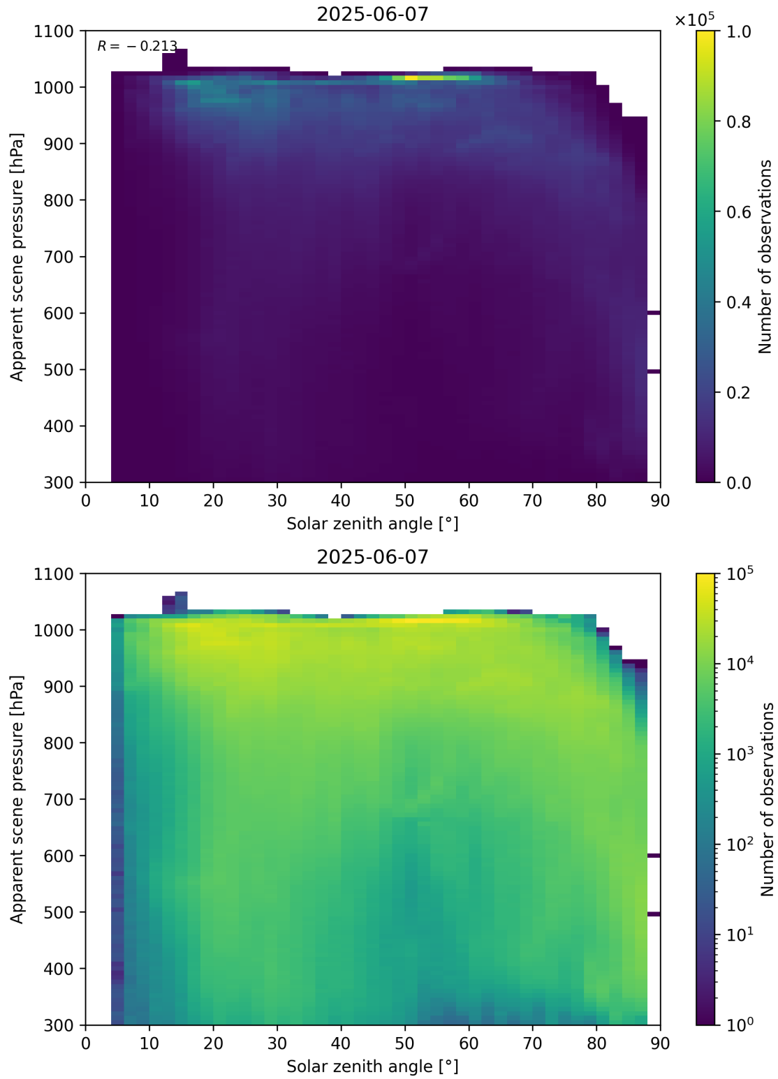
Figure 108: Scatter density plot of “Solar zenith angle” against “Apparent scene pressure” for 2025-06-06 to 2025-06-08.
