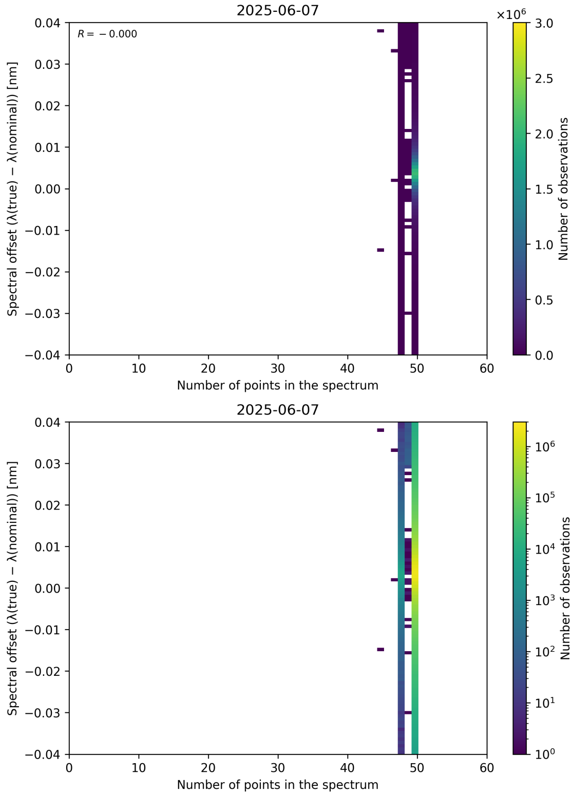
Figure 101: Scatter density plot of “Number of points in the spectrum” against “Spectral offset ( \lambda_{\text{true}} - \lambda_{\text{nominal}} )” for 2025-06-06 to 2025-06-08.
