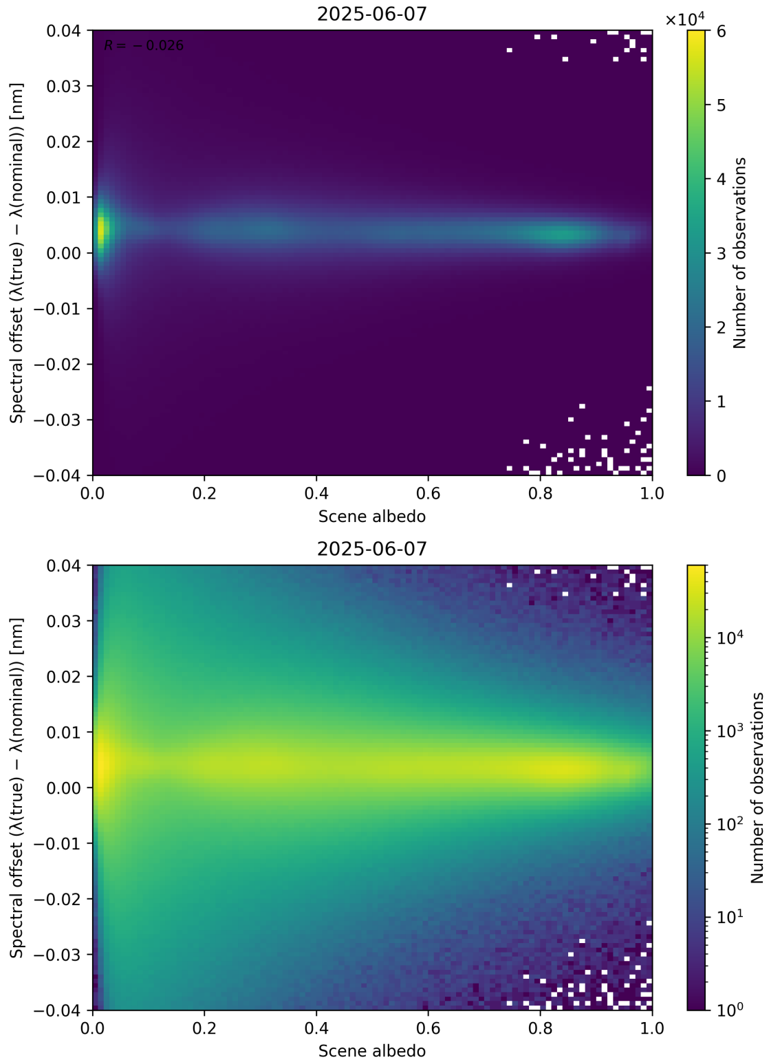
Figure 107: Scatter density plot of “Scene albedo” against “Spectral offset ( \lambda_{\text{true}} - \lambda_{\text{nominal}} )” for 2025-06-06 to 2025-06-08.
