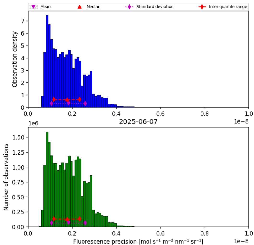
Figure 41: Histogram of “Fluorescence precision” for 2025-06-06 to 2025-06-08
