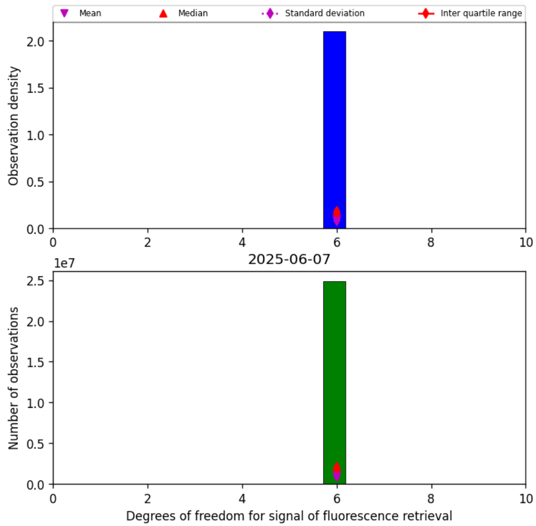
Figure 43: Histogram of "Degrees of freedom for signal of fluorescence retrieval" for 2025-06-06 to 2025-06-08
