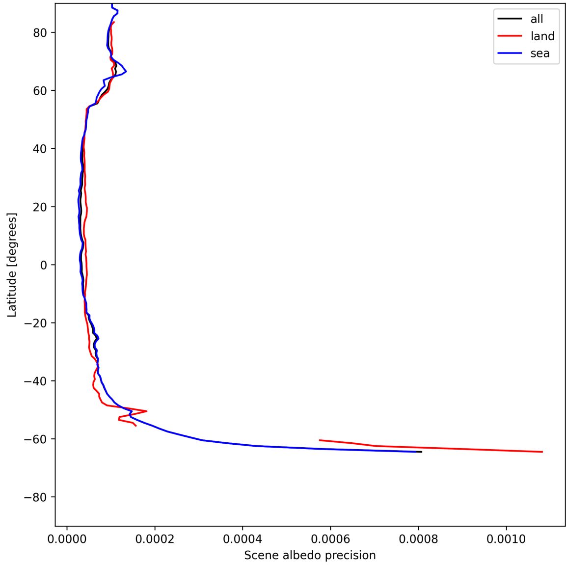
Figure 18: Zonal average of “Scene albedo precision” for 2025-06-06 to 2025-06-08.
