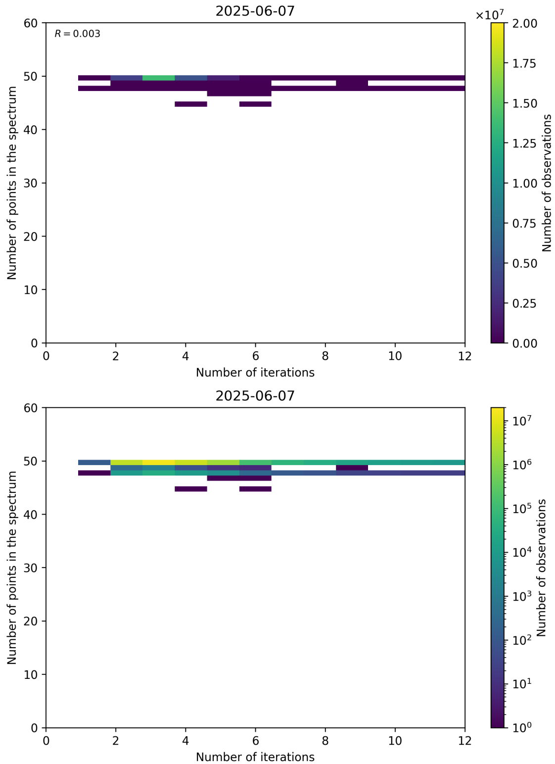
Figure 99: Scatter density plot of “Number of iterations” against “Number of points in the spectrum” for 2025-06-06 to 2025-06-08.
