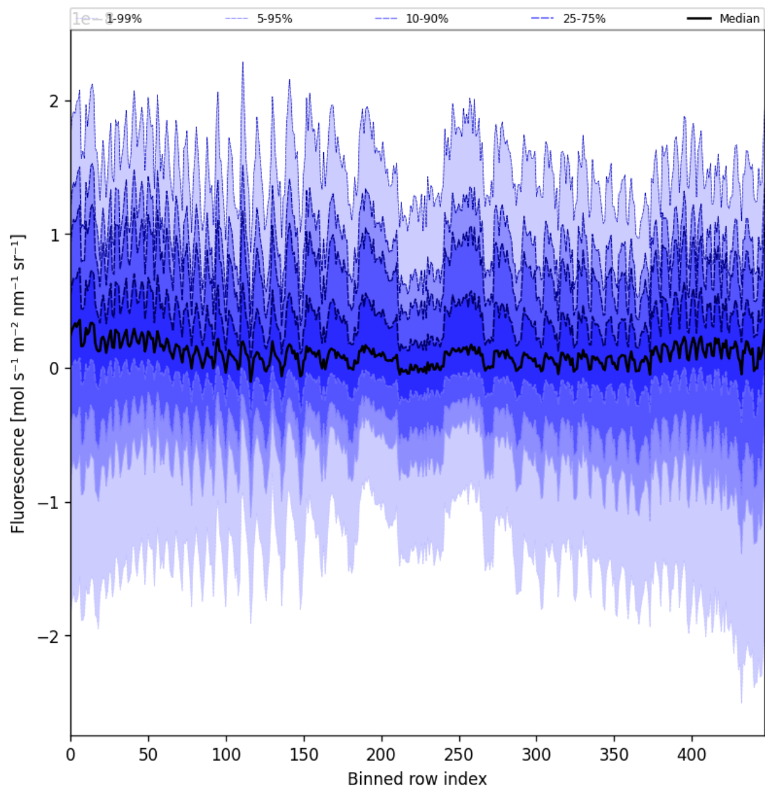
Figure 57: Along track statistics of “Fluorescence” for 2025-06-06 to 2025-06-08
