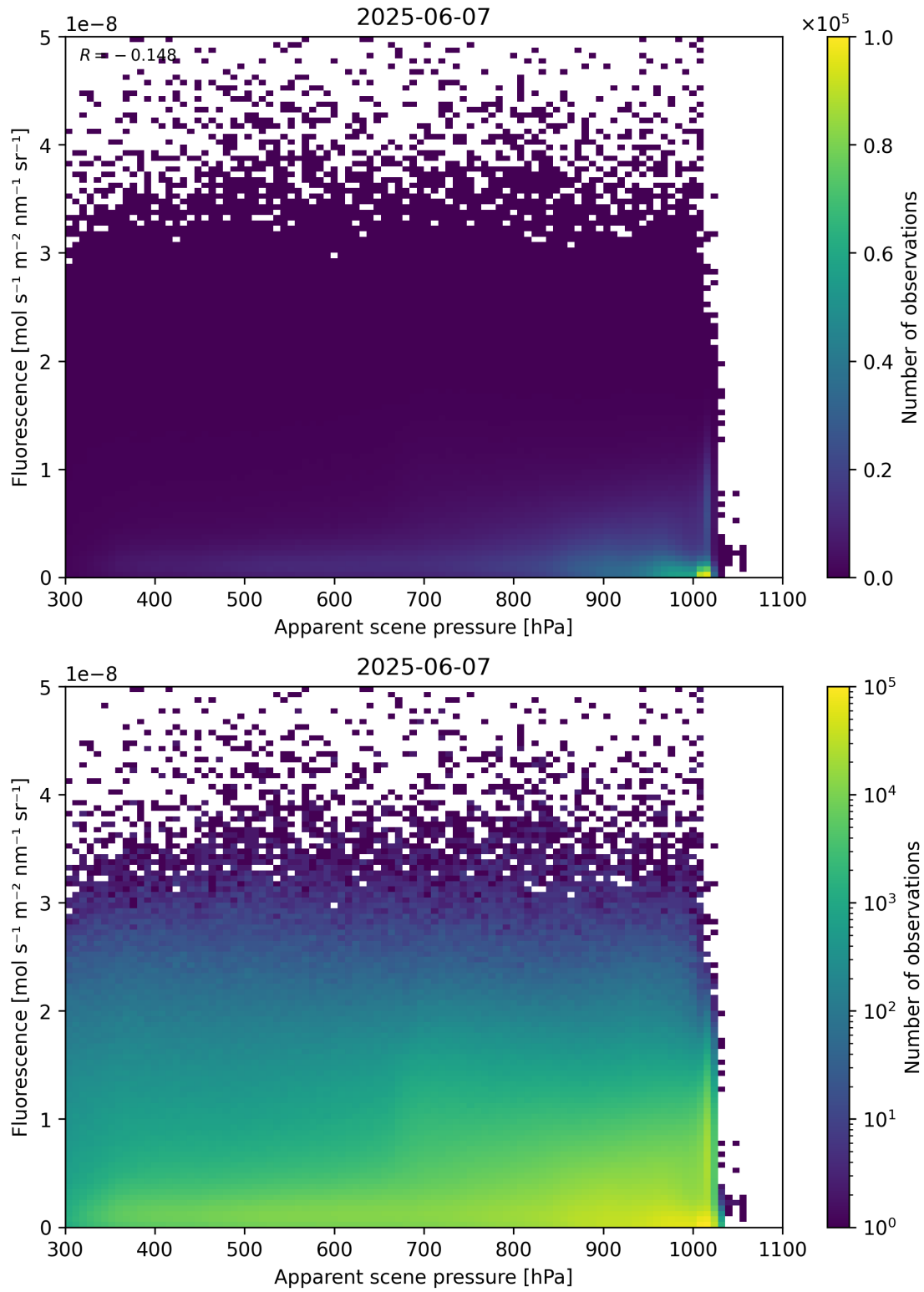
Figure 64: Scatter density plot of “Apparent scene pressure” against “Fluorescence” for 2025-06-06 to 2025-06-08.
