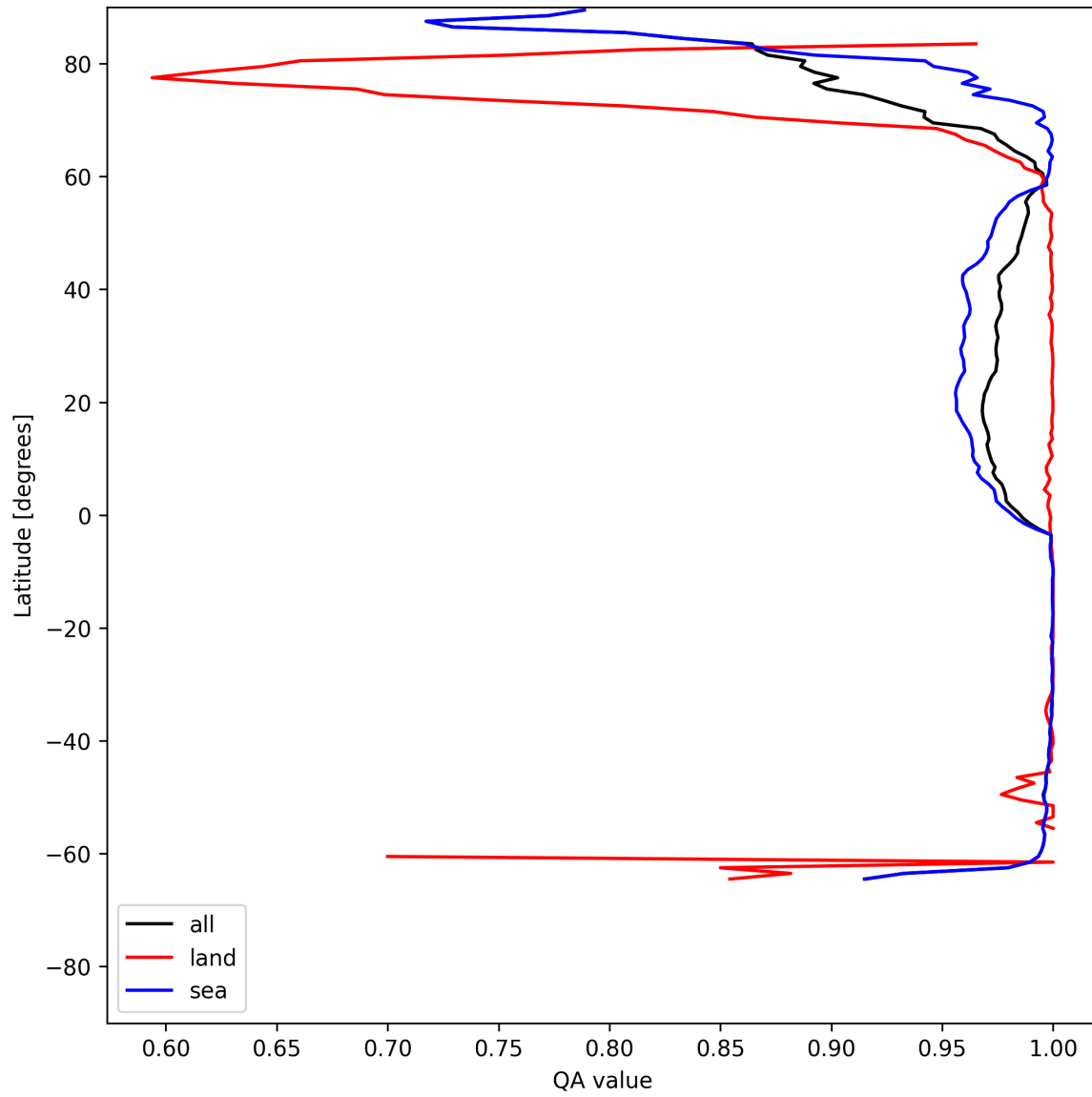
Figure 12: Zonal average of “QA value” for 2025-06-06 to 2025-06-08.
