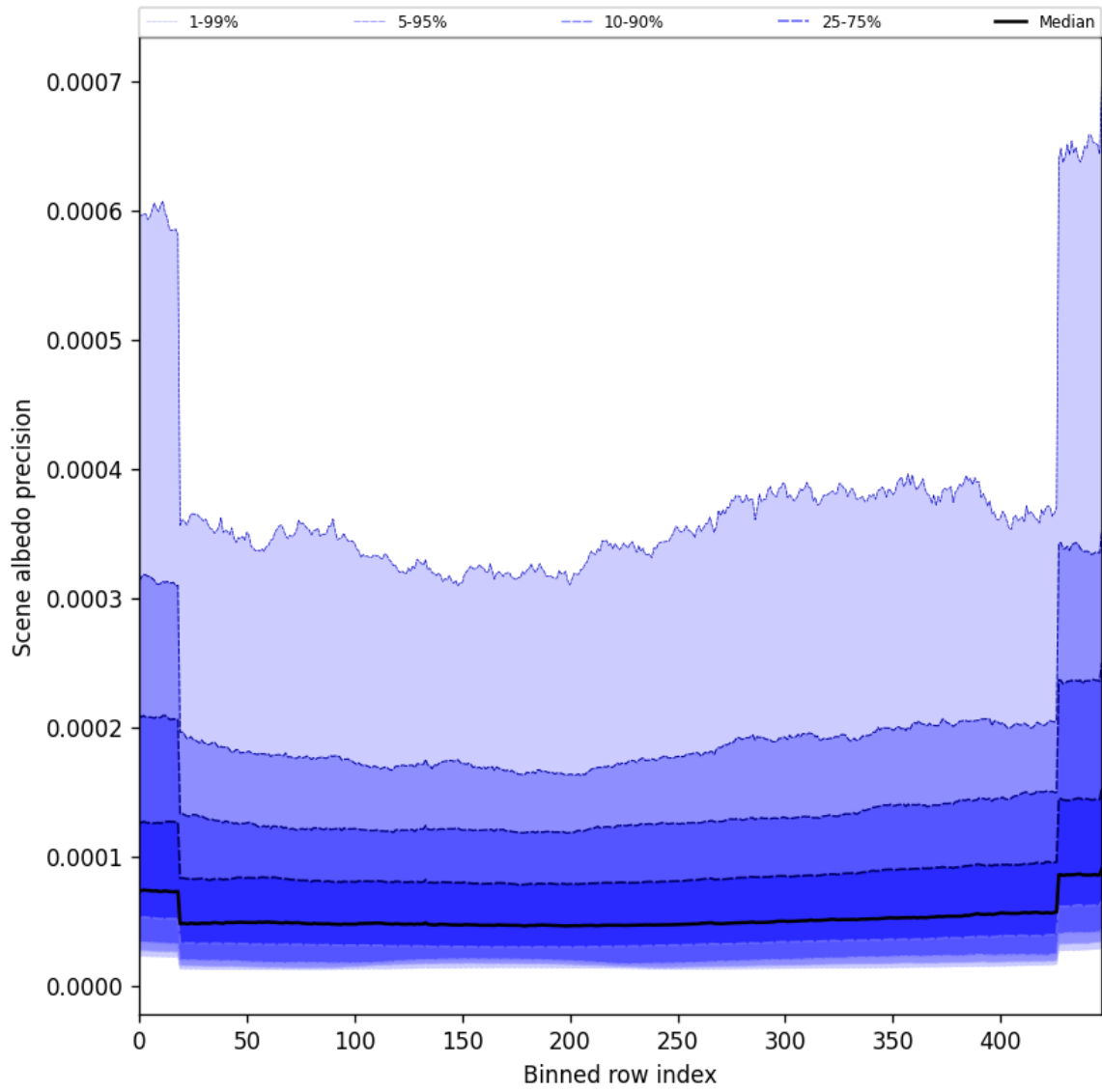
Figure 52: Along track statistics of “Scene albedo precision” for 2025-06-06 to 2025-06-08
