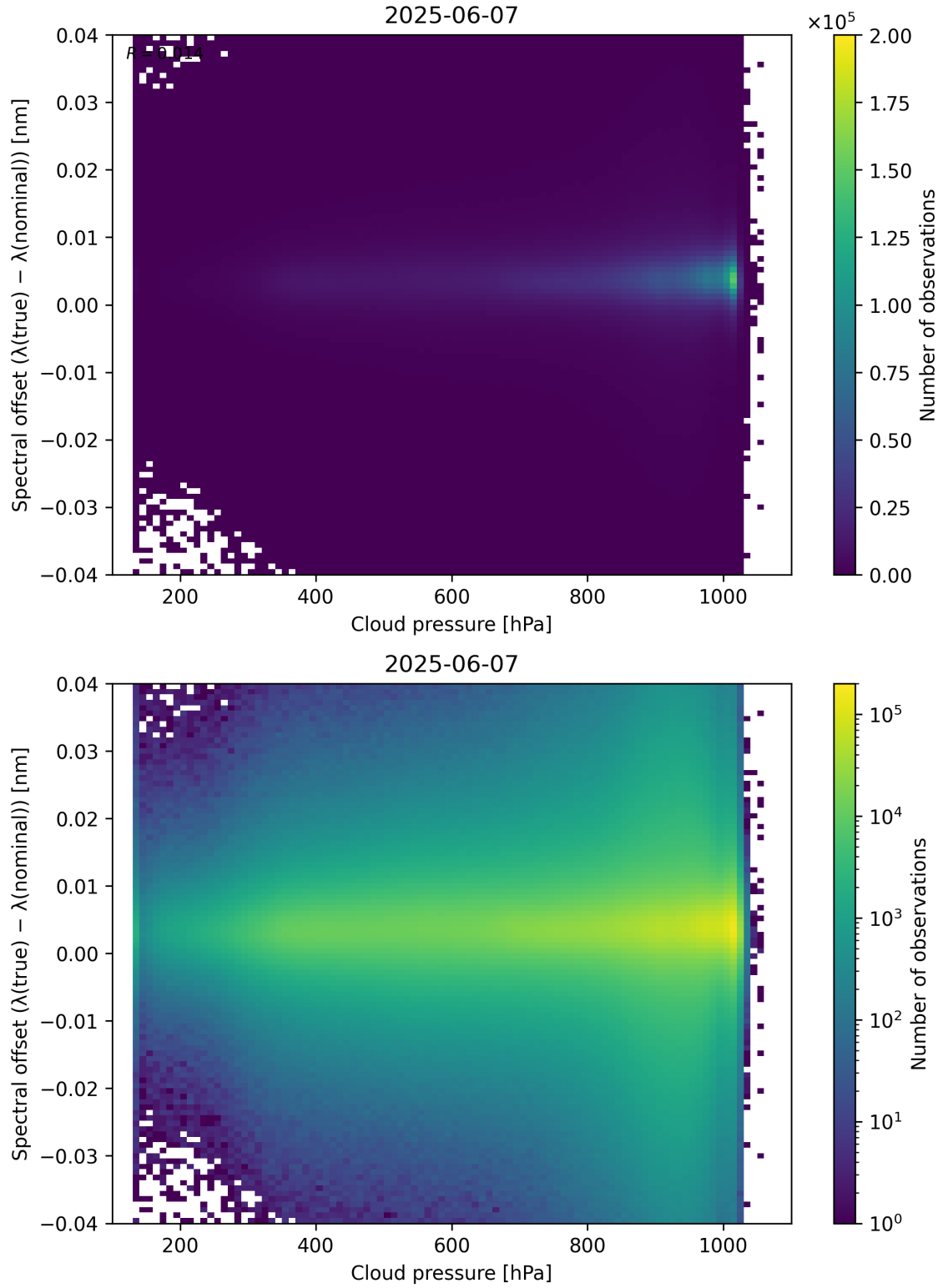
Figure 84: Scatter density plot of “Cloud pressure” against “Spectral offset ( \lambda_{\text{true}} - \lambda_{\text{nominal}} )” for 2025-06-06 to 2025-06-08.
