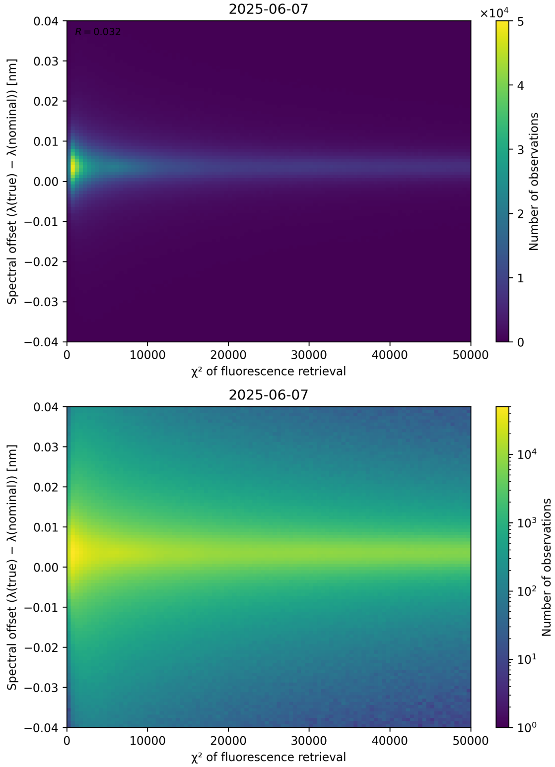
Figure 69: Scatter density plot of " \chi^2 of fluorescence retrieval" against "Spectral offset ( \lambda_{\text{true}} - \lambda_{\text{nominal}} )" for 2025-06-06 to 2025-06-08.
