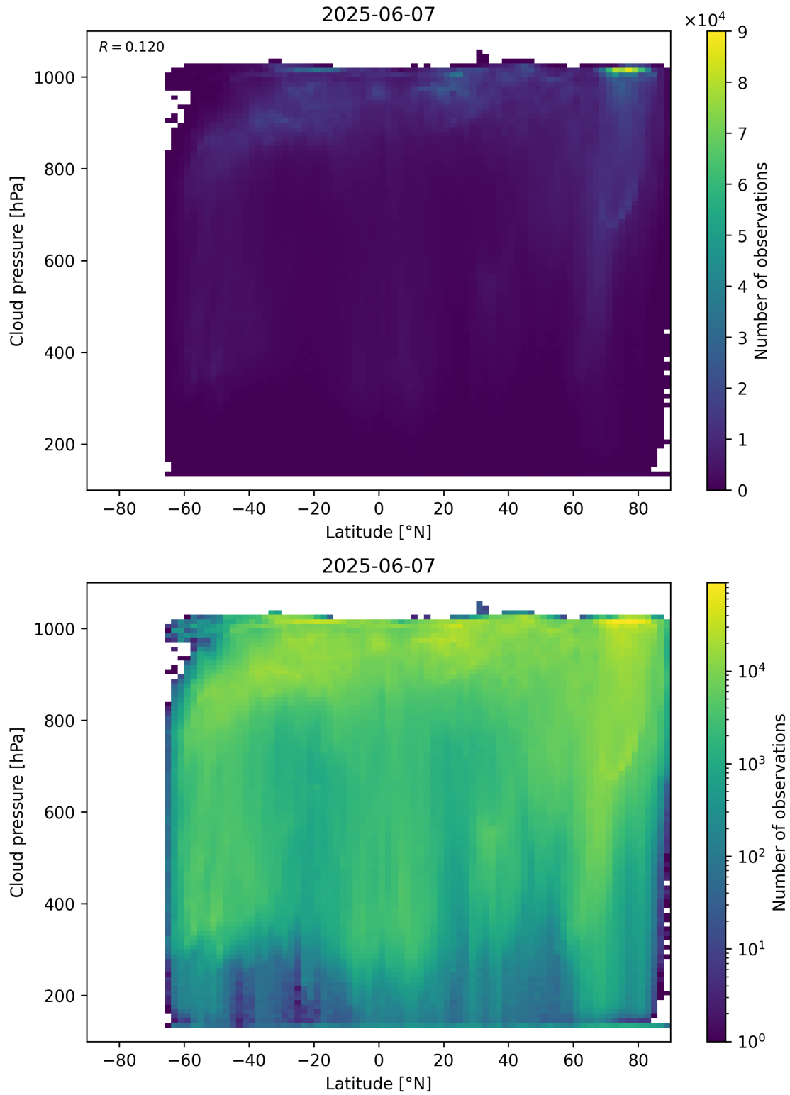
Figure 91: Scatter density plot of “Latitude” against “Cloud pressure” for 2025-06-06 to 2025-06-08.
