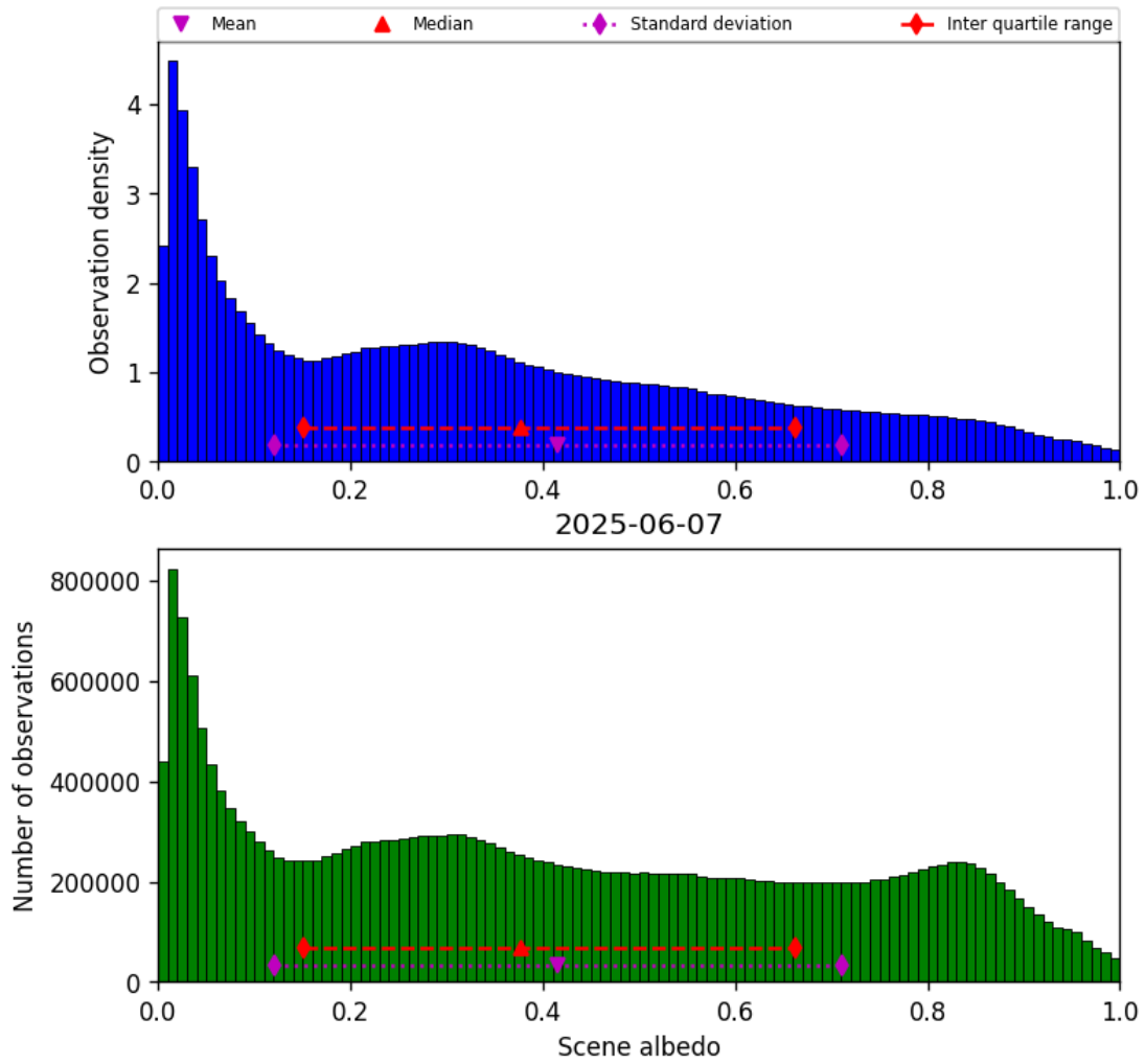
Figure 34: Histogram of “Scene albedo” for 2025-06-06 to 2025-06-08
