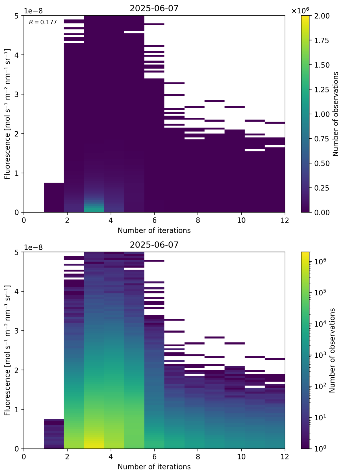
Figure 98: Scatter density plot of “Number of iterations” against “Fluorescence” for 2025-06-06 to 2025-06-08.
