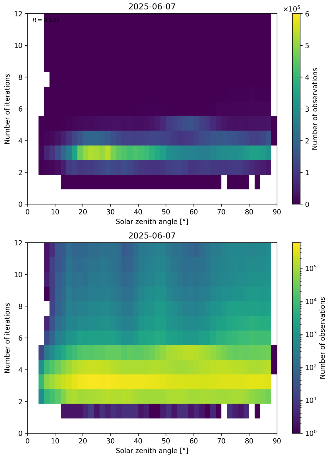
Figure 114: Scatter density plot of “Solar zenith angle” against “Number of iterations” for 2025-06-06 to 2025-06-08.
