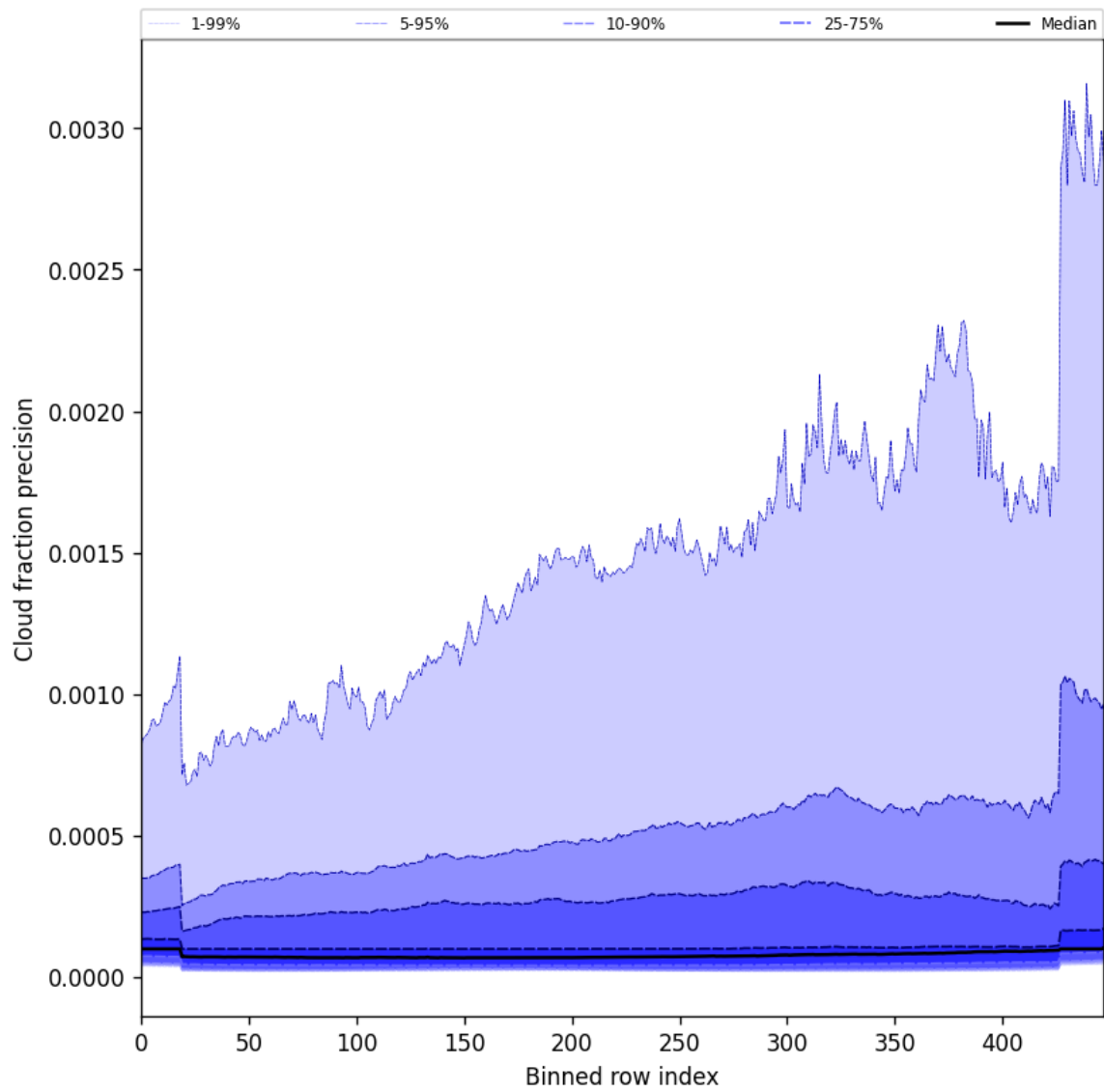
Figure 50: Along track statistics of “Cloud fraction precision” for 2025-06-06 to 2025-06-08
