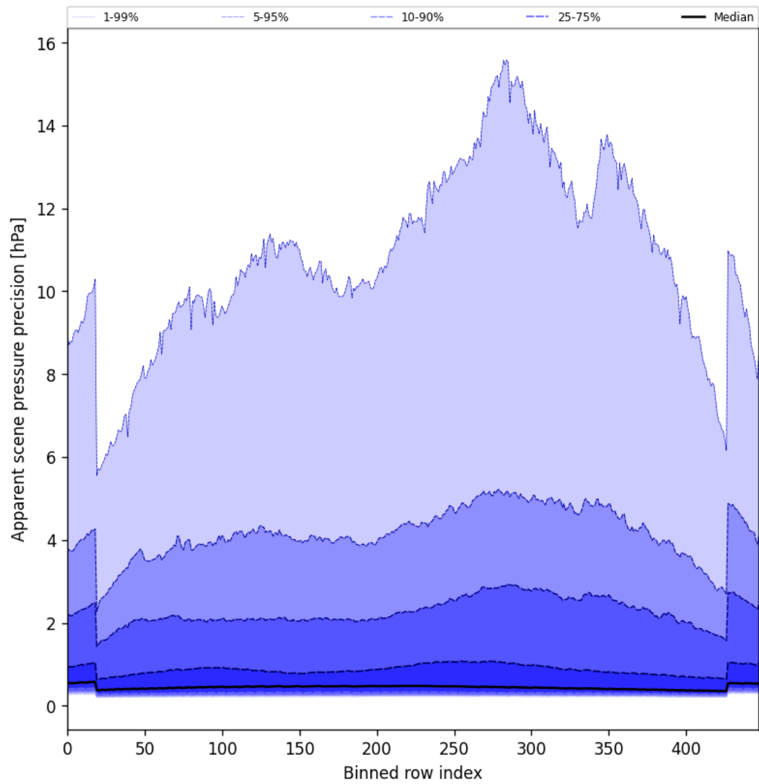
Figure 54: Along track statistics of “Apparent scene pressure precision” for 2025-06-06 to 2025-06-08
