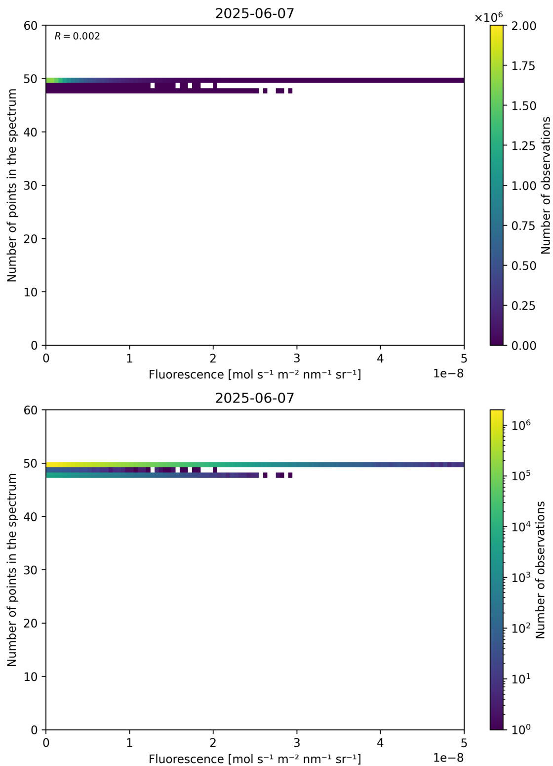
Figure 86: Scatter density plot of “Fluorescence” against “Number of points in the spectrum” for 2025-06-06 to 2025-06-08.
