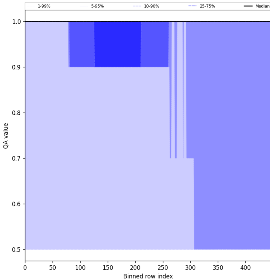
Figure 46: Along track statistics of “QA value” for 2025-06-06 to 2025-06-08
