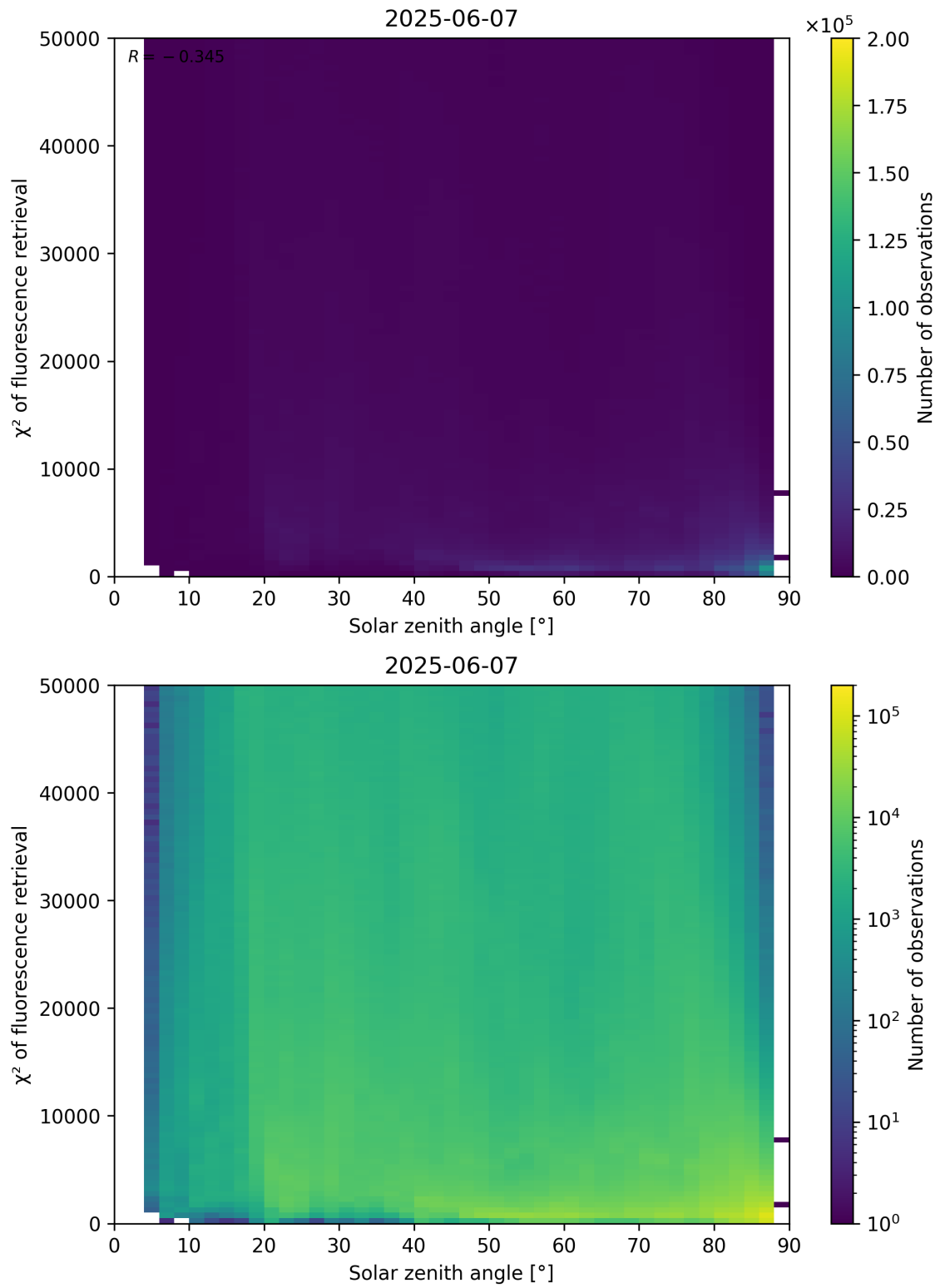
Figure 109: Scatter density plot of “Solar zenith angle” against “ \chi^2 of fluorescence retrieval” for 2025-06-06 to 2025-06-08.
