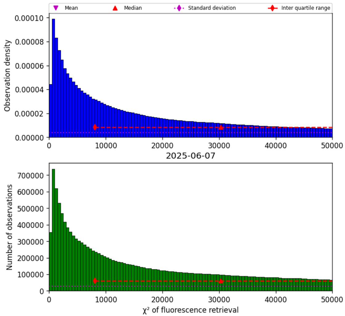
Figure 42: Histogram of “ \chi^2 of fluorescence retrieval” for 2025-06-06 to 2025-06-08
