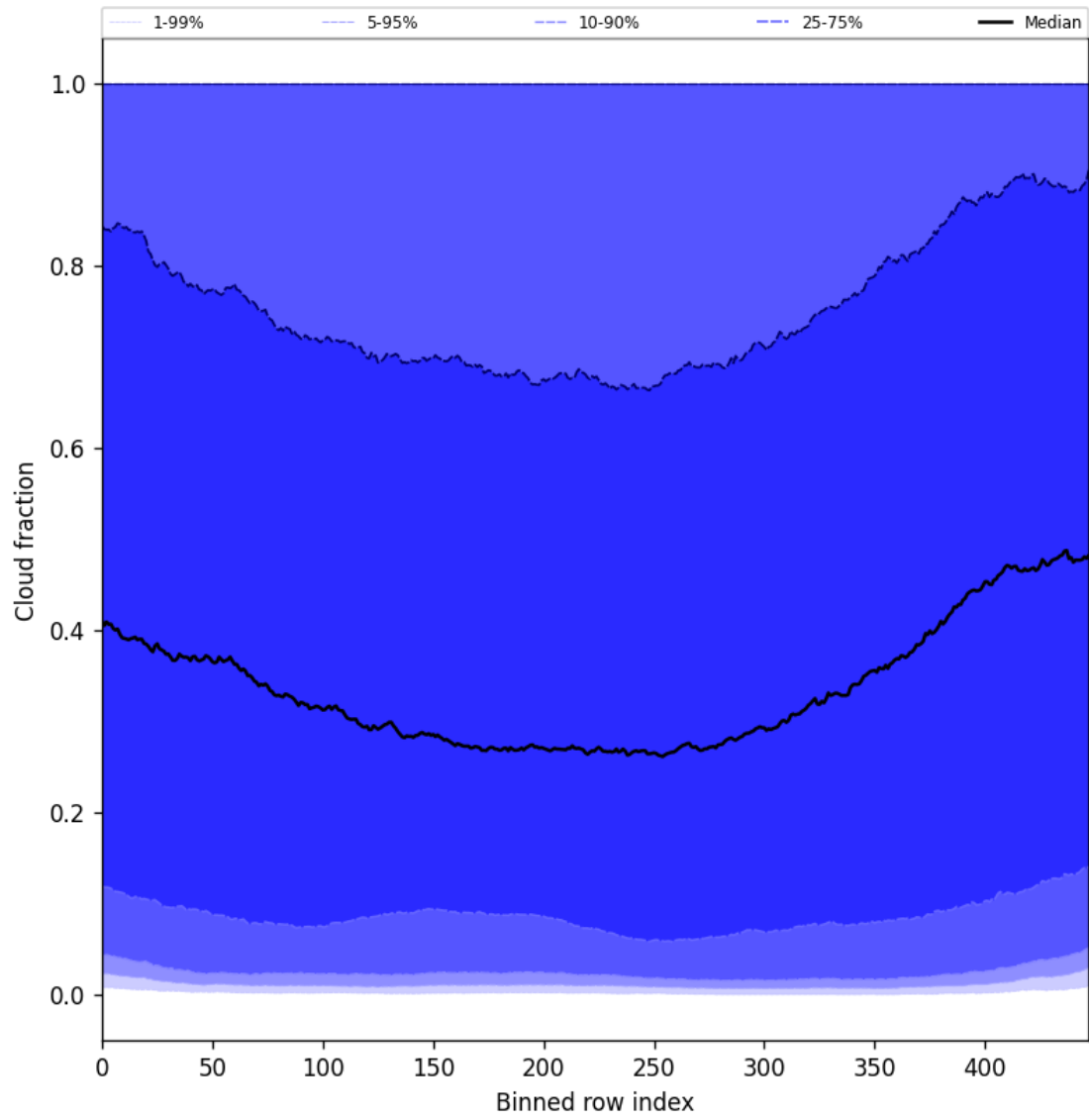
Figure 49: Along track statistics of “Cloud fraction” for 2025-06-06 to 2025-06-08
