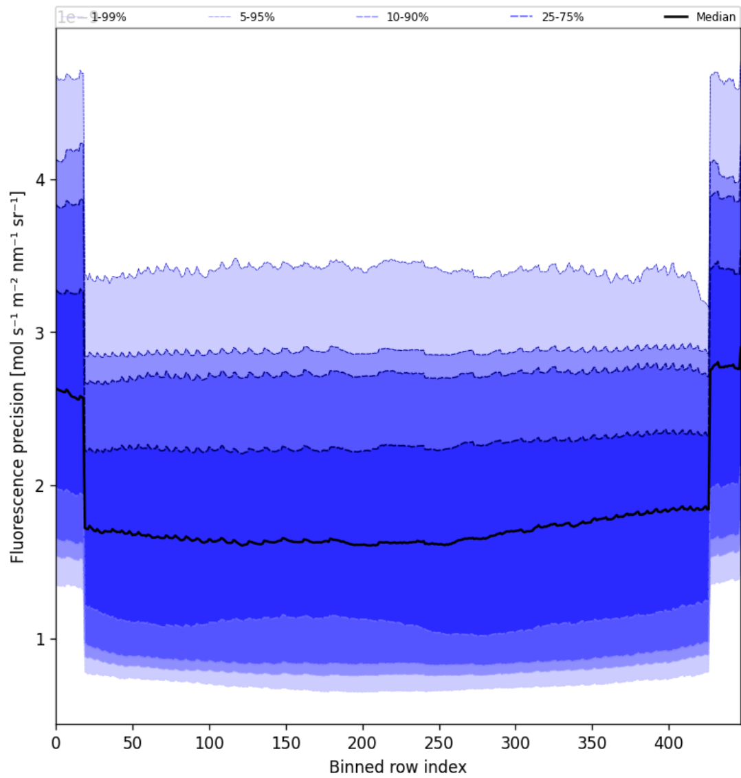
Figure 58: Along track statistics of “Fluorescence precision” for 2025-06-06 to 2025-06-08
