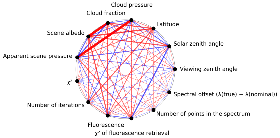
Figure 1: Map of correlation graph for 2025-06-06 to 2025-06-08.
