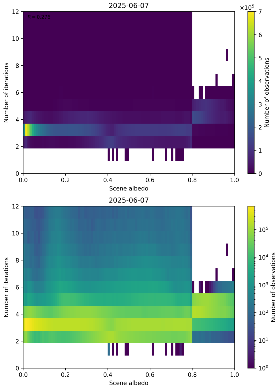
Figure 105: Scatter density plot of “Scene albedo” against “Number of iterations” for 2025-06-06 to 2025-06-08.
