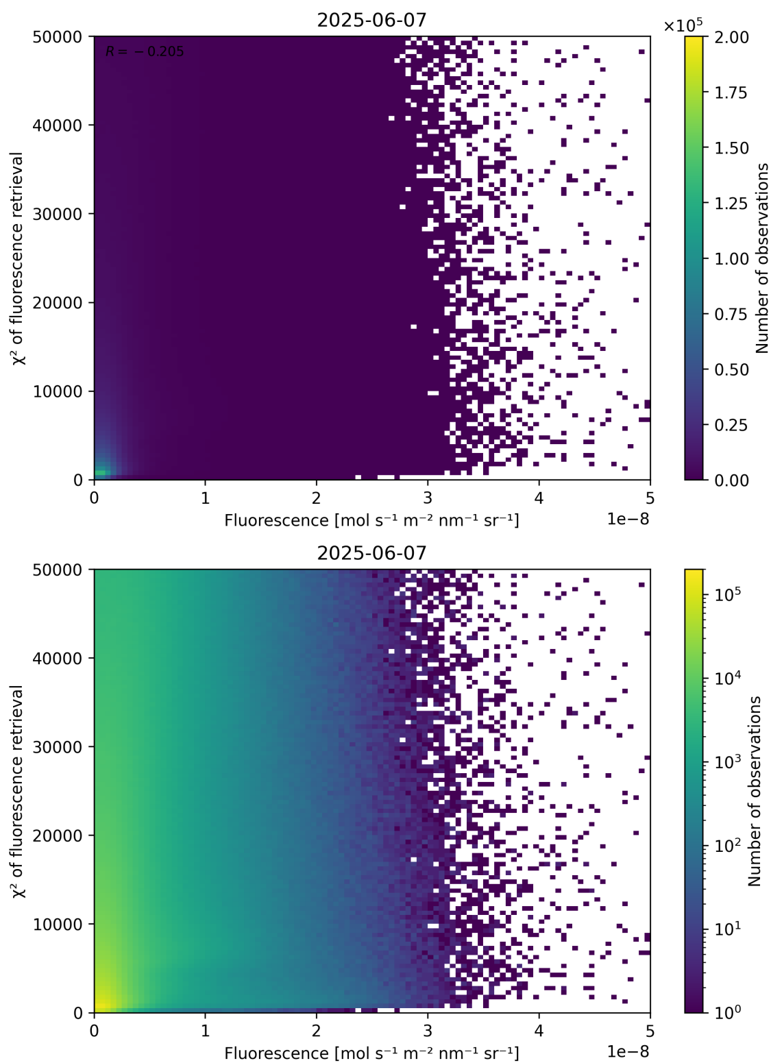
Figure 85: Scatter density plot of “Fluorescence” against “ \chi^2 of fluorescence retrieval” for 2025-06-06 to 2025-06-08.
