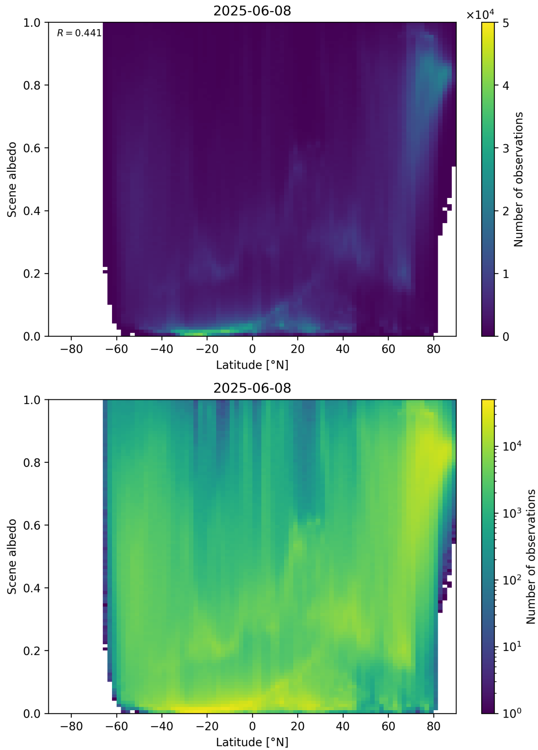
Figure 95: Scatter density plot of “Latitude” against “Scene albedo” for 2025-06-07 to 2025-06-09.
