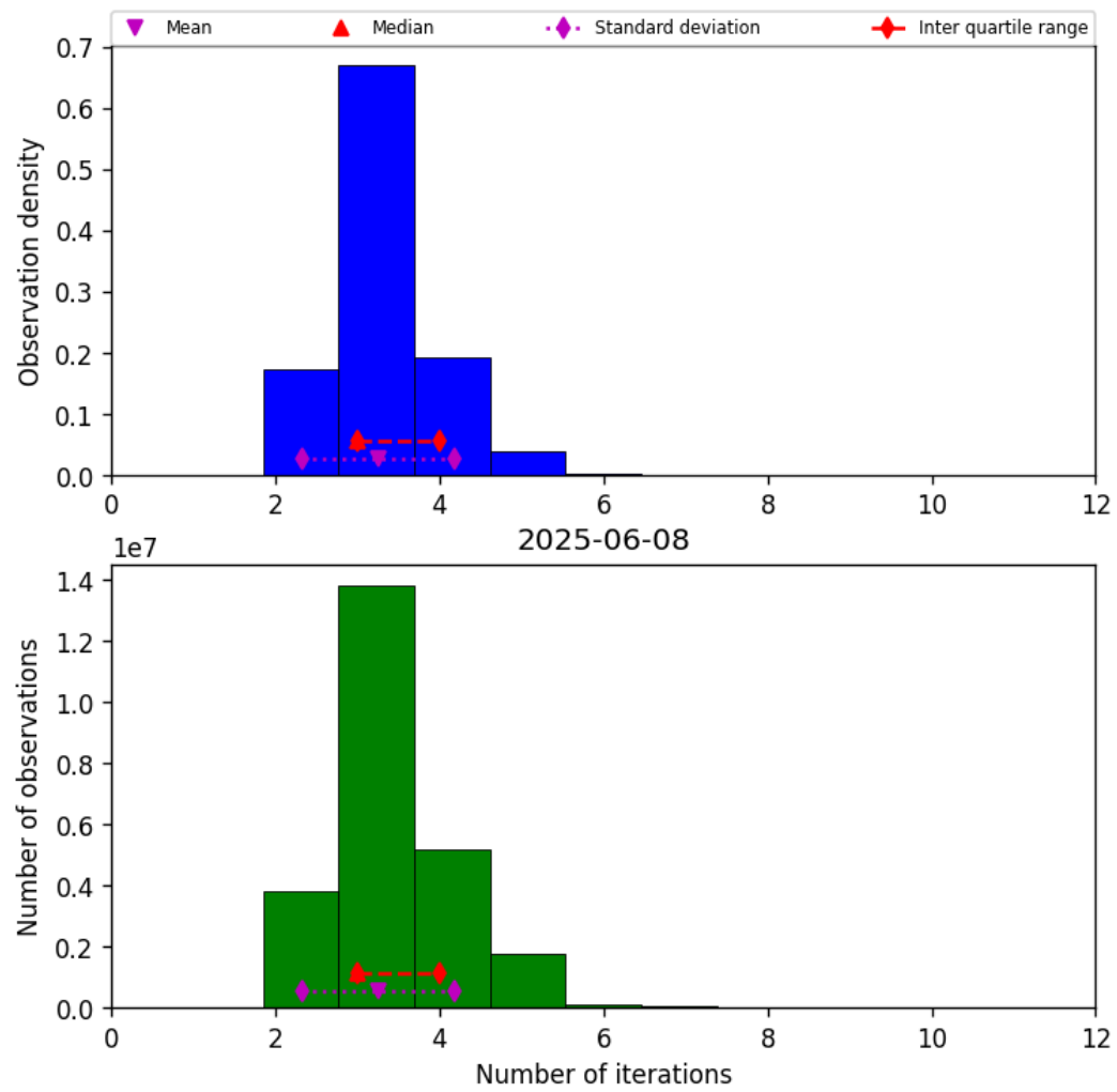
Figure 39: Histogram of “Number of iterations” for 2025-06-07 to 2025-06-09
