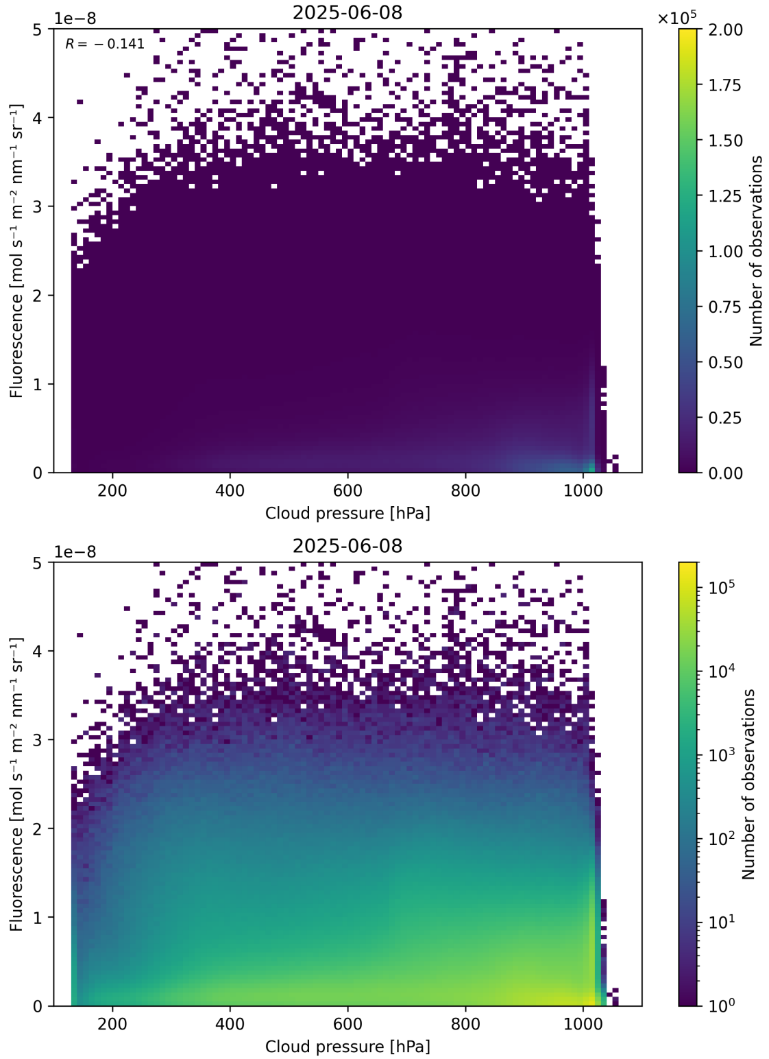
Figure 80: Scatter density plot of “Cloud pressure” against “Fluorescence” for 2025-06-07 to 2025-06-09.
