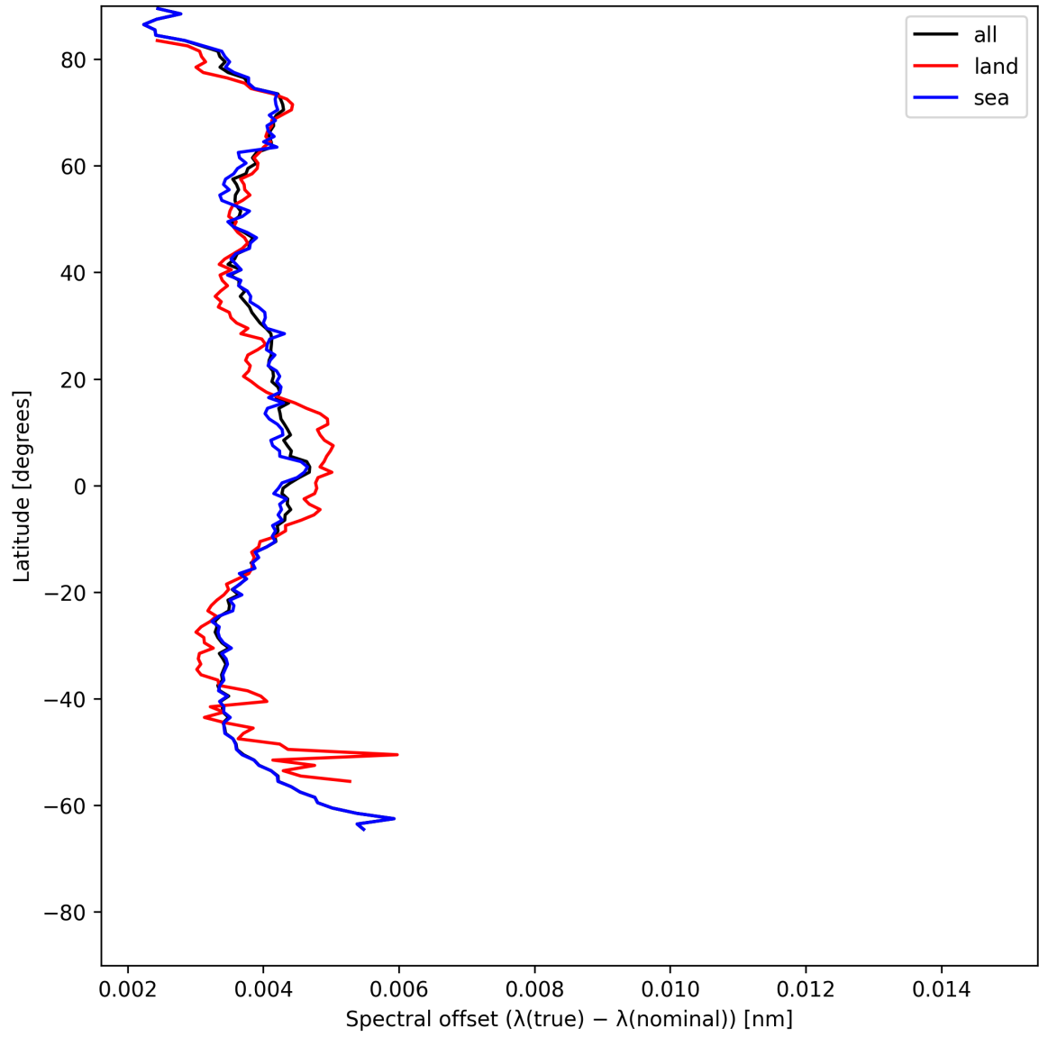
Figure 28: Zonal average of “Spectral offset ( \lambda_{\text{true}} - \lambda_{\text{nominal}} )” for 2025-06-07 to 2025-06-09.
