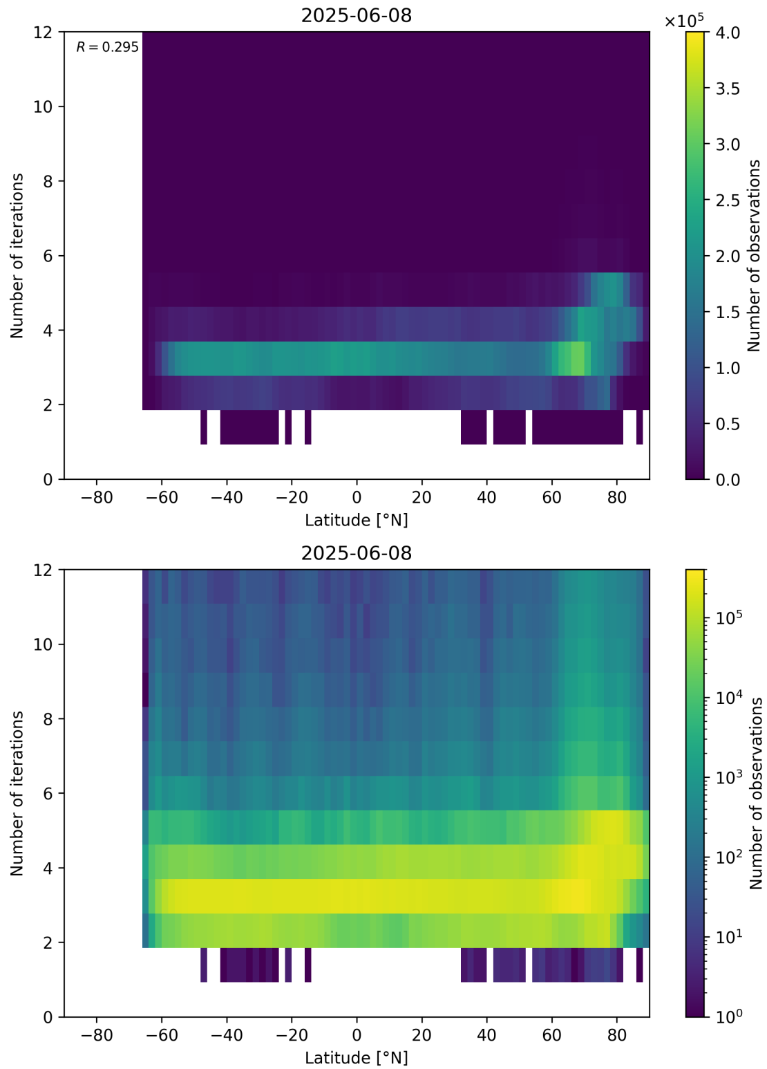
Figure 93: Scatter density plot of “Latitude” against “Number of iterations” for 2025-06-07 to 2025-06-09.
