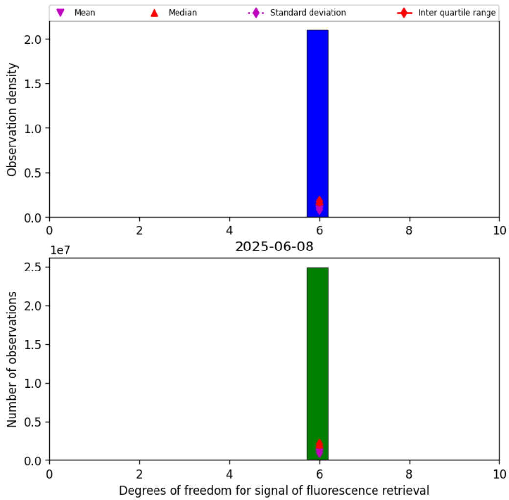
Figure 43: Histogram of “Degrees of freedom for signal of fluorescence retrieval” for 2025-06-07 to 2025-06-09
