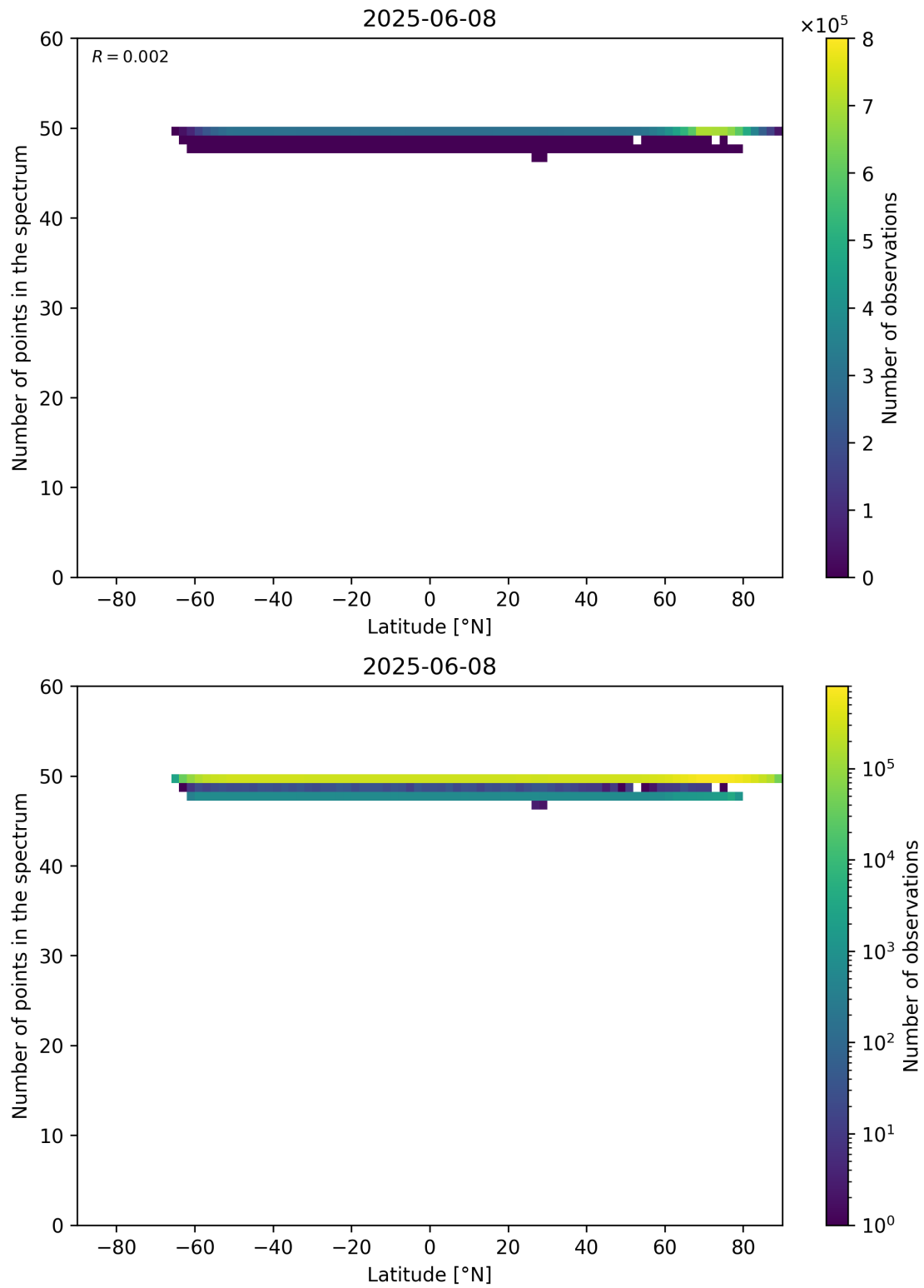
Figure 94: Scatter density plot of “Latitude” against “Number of points in the spectrum” for 2025-06-07 to 2025-06-09.
