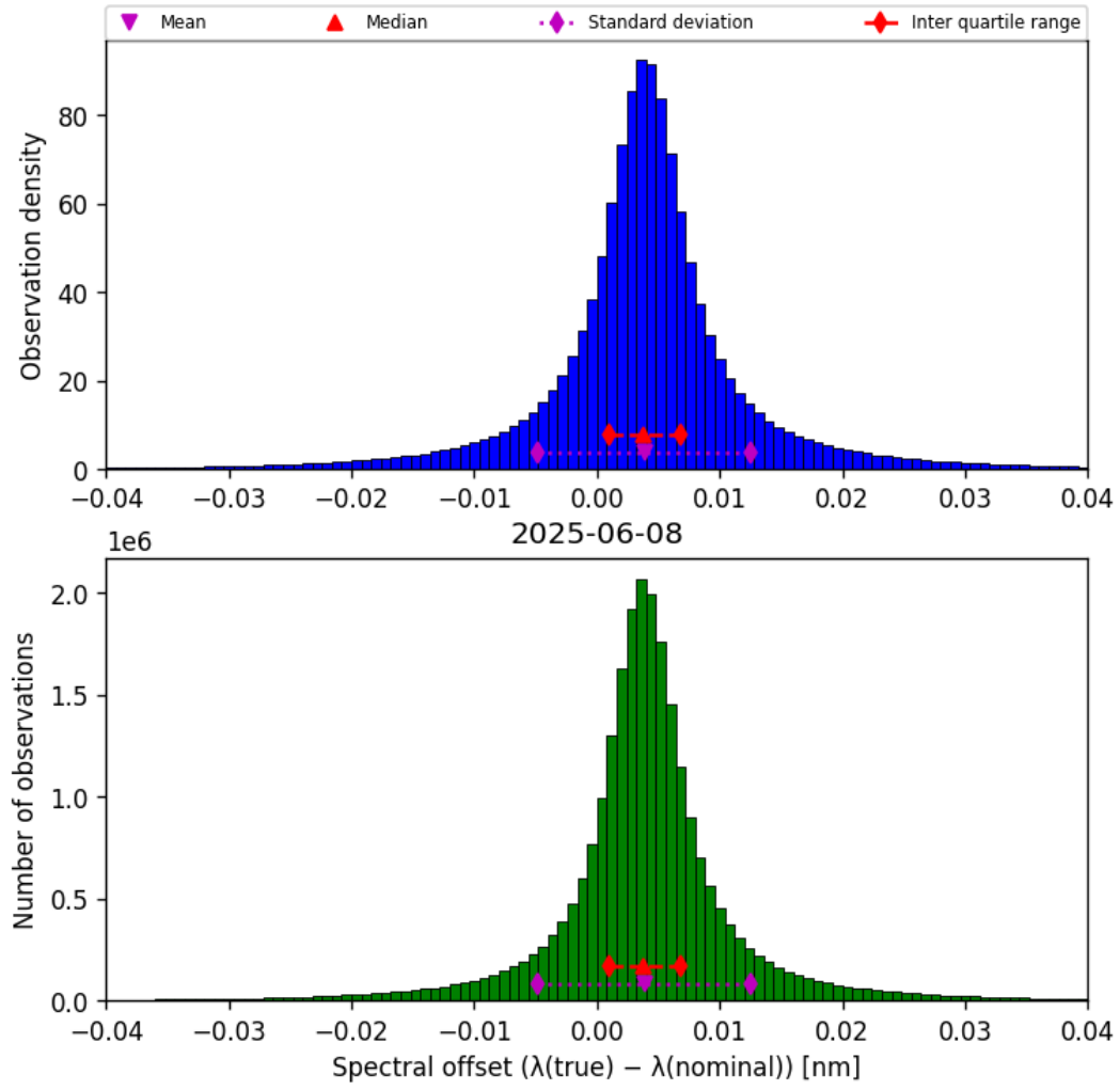
Figure 45: Histogram of “Spectral offset ( \lambda_{\text{true}} - \lambda_{\text{nominal}} )” for 2025-06-07 to 2025-06-09
