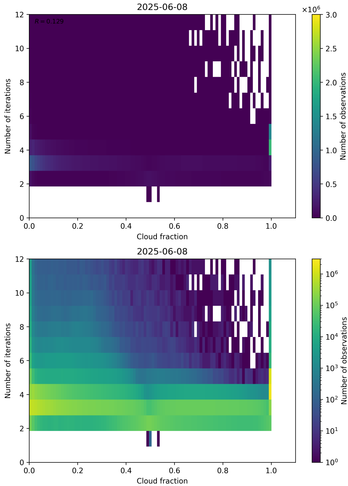
Figure 73: Scatter density plot of “Cloud fraction” against “Number of iterations” for 2025-06-07 to 2025-06-09.
