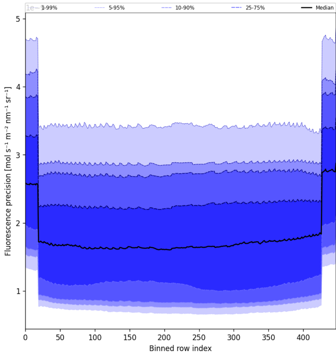
Figure 58: Along track statistics of “Fluorescence precision” for 2025-06-07 to 2025-06-09
