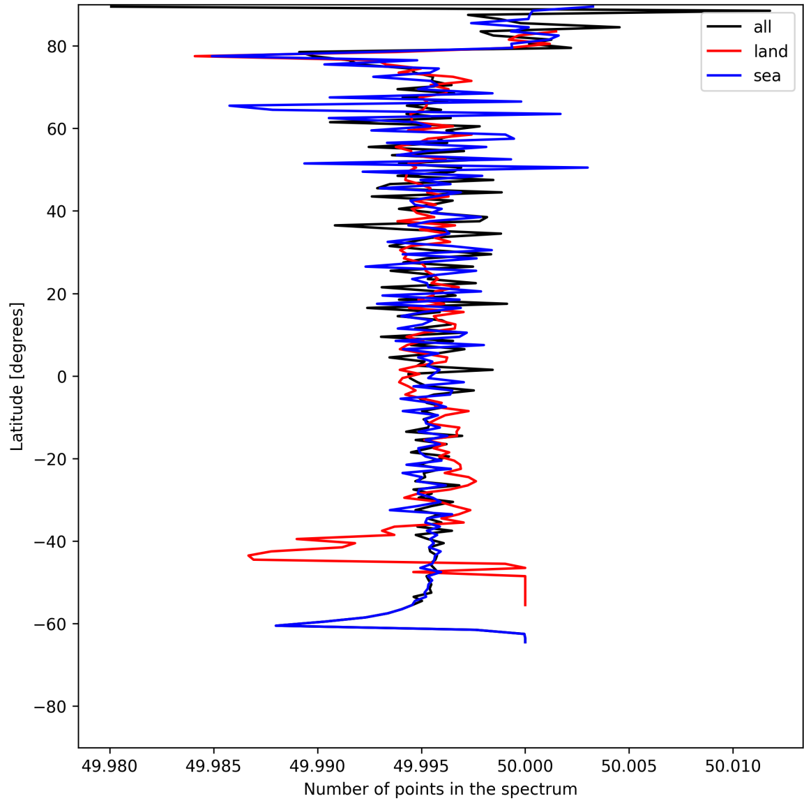
Figure 27: Zonal average of “Number of points in the spectrum” for 2025-06-07 to 2025-06-09.
