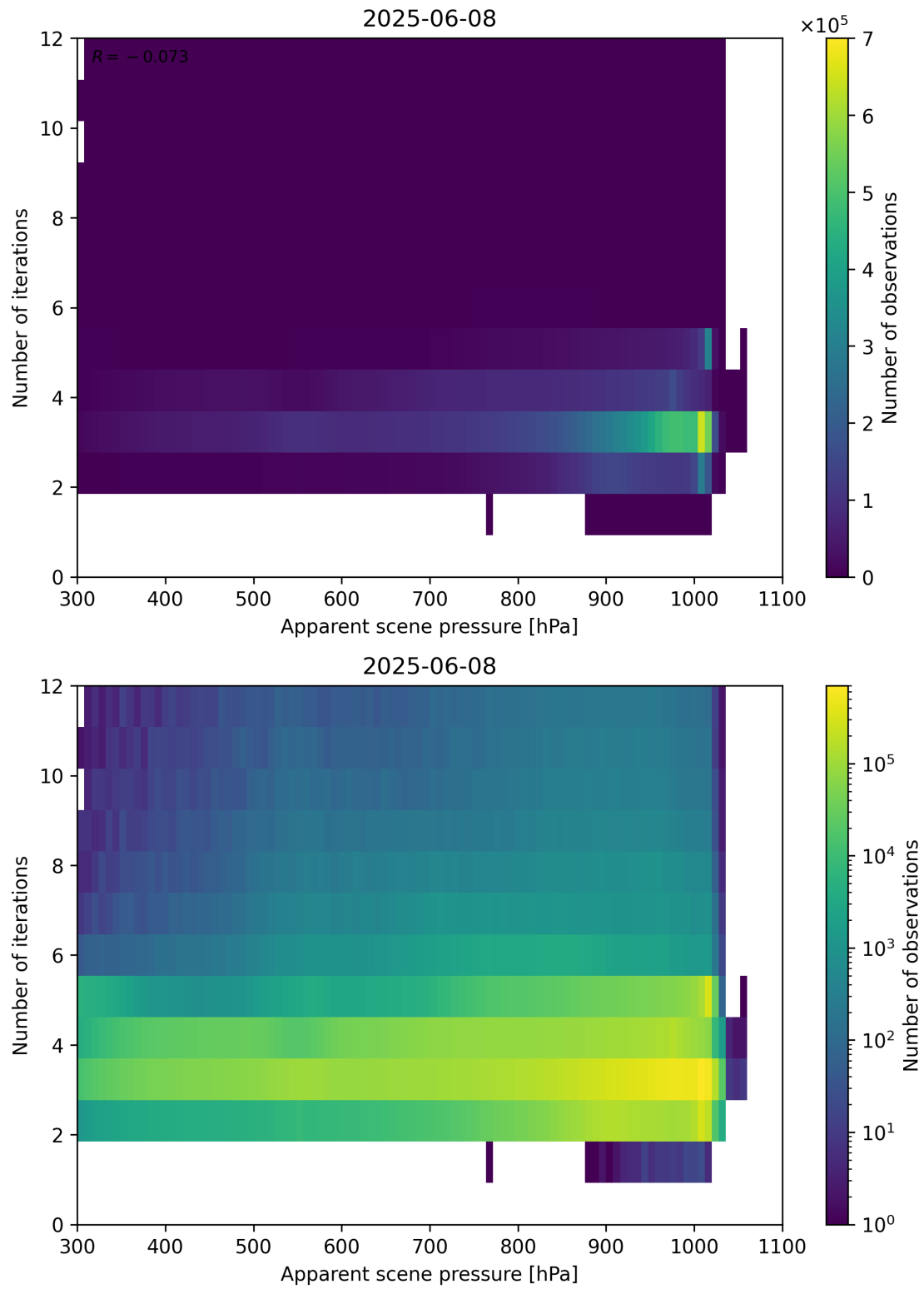
Figure 65: Scatter density plot of “Apparent scene pressure” against “Number of iterations” for 2025-06-07 to 2025-06-09.
