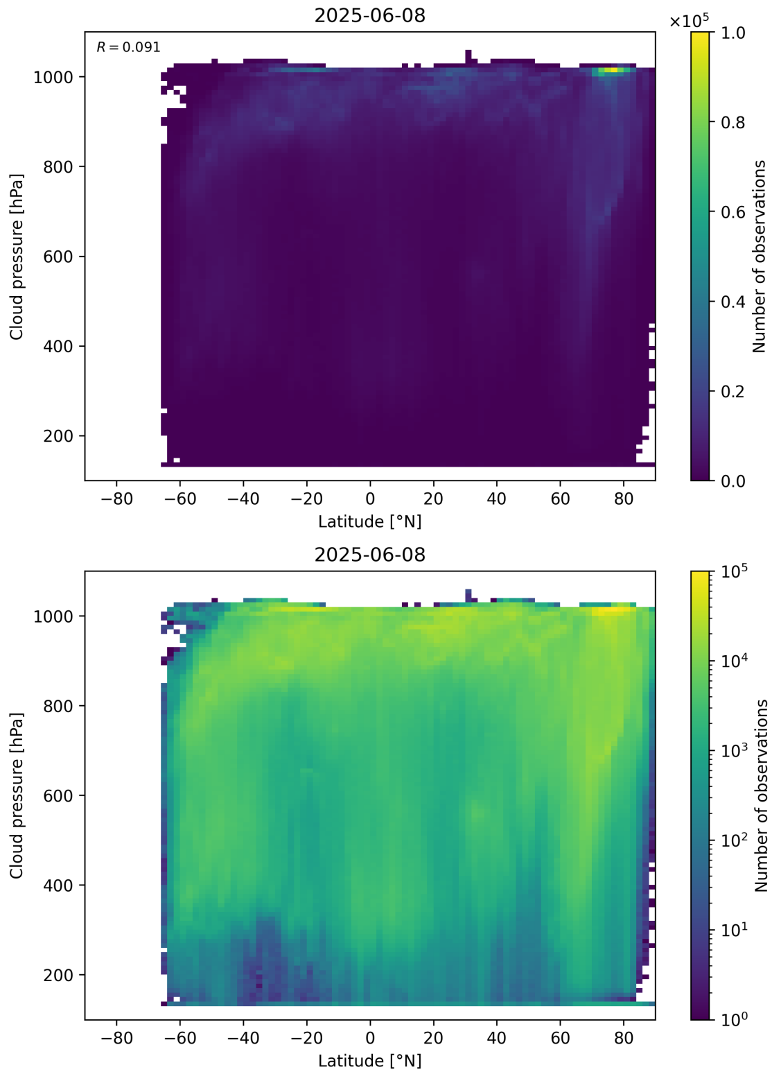
Figure 91: Scatter density plot of “Latitude” against “Cloud pressure” for 2025-06-07 to 2025-06-09.
