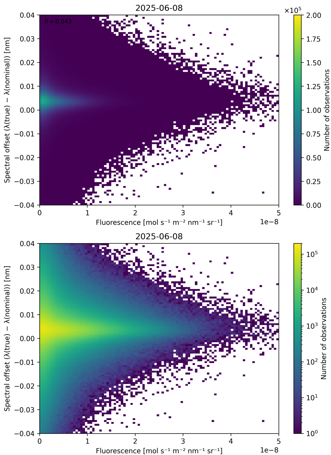
Figure 87: Scatter density plot of “Fluorescence” against “Spectral offset ( \lambda_{\text{true}} - \lambda_{\text{nominal}} )” for 2025-06-07 to 2025-06-09.
