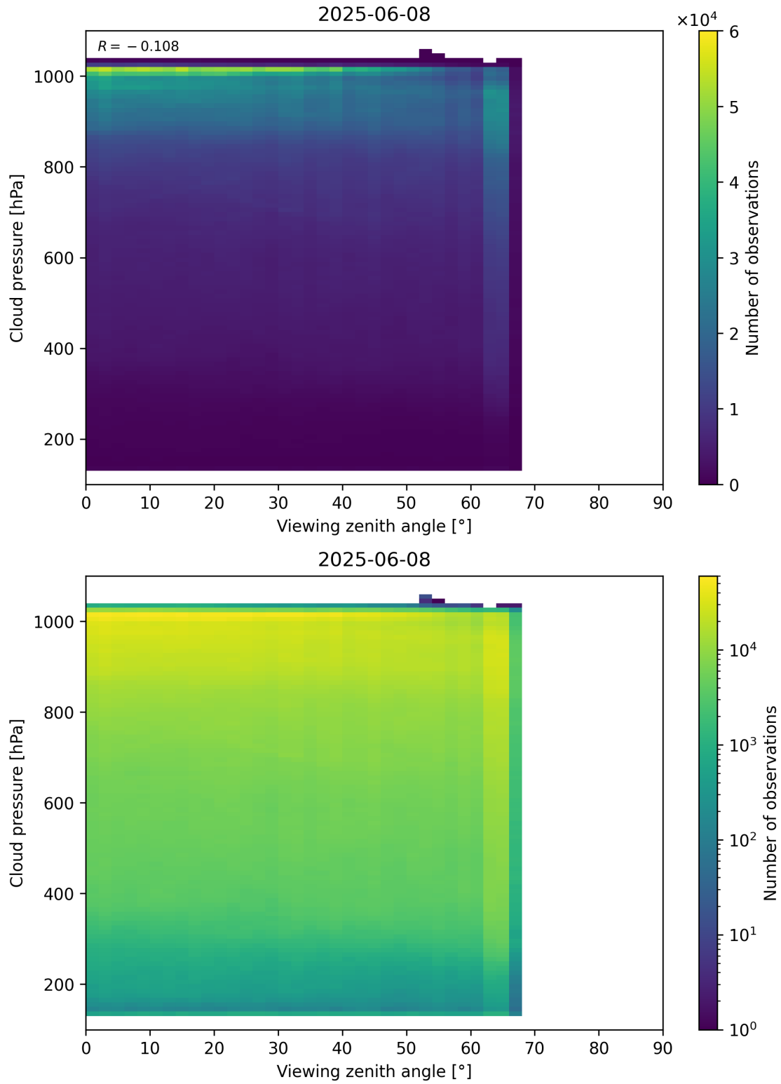
Figure 121: Scatter density plot of “Viewing zenith angle” against “Cloud pressure” for 2025-06-07 to 2025-06-09.
