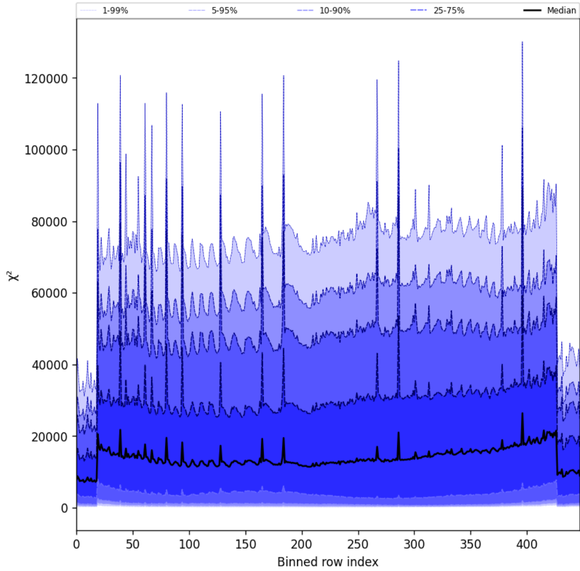
Figure 55: Along track statistics of “ \chi^2 ” for 2025-06-07 to 2025-06-09
