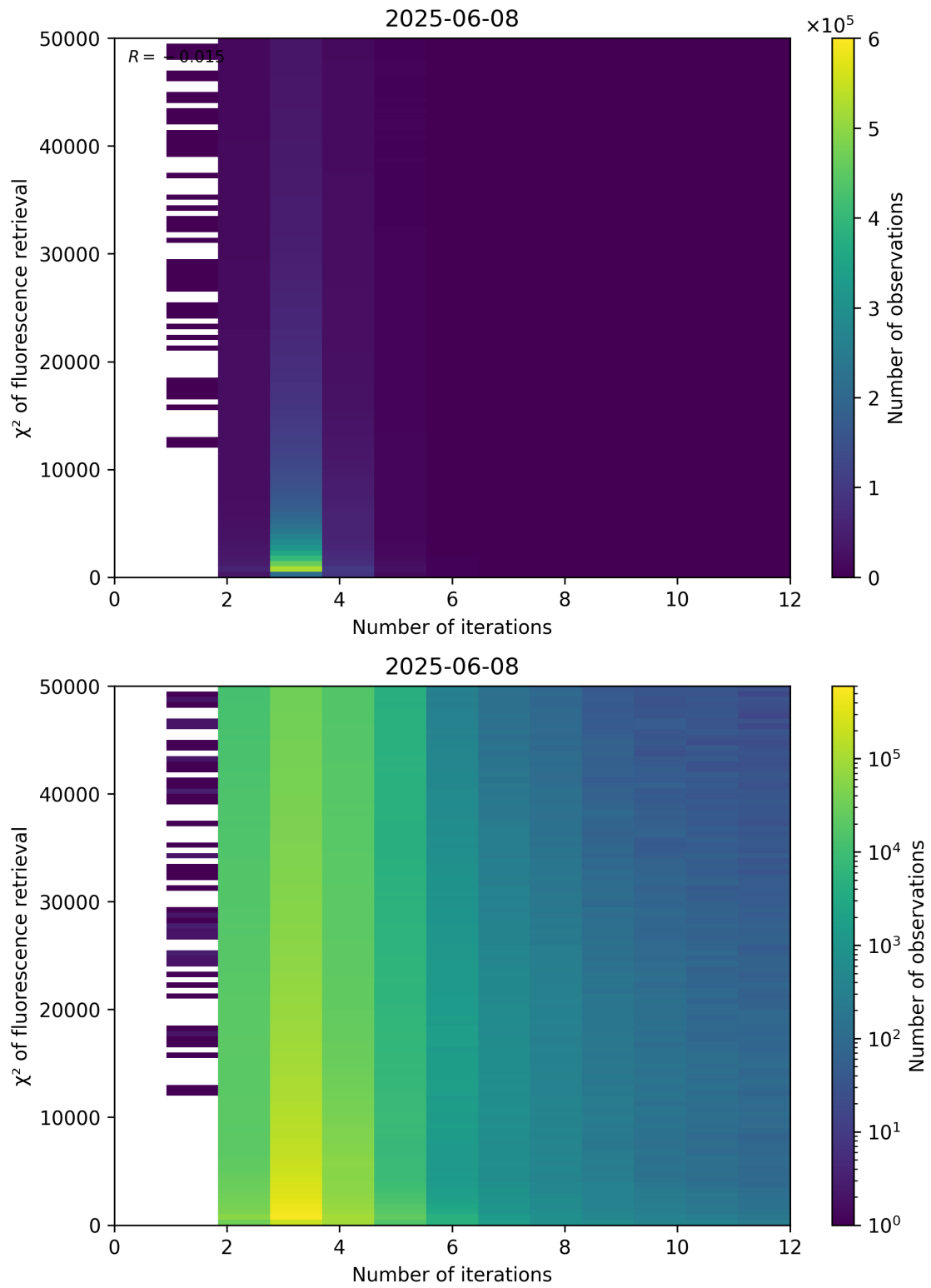
Figure 97: Scatter density plot of “Number of iterations” against “ \chi^2 of fluorescence retrieval” for 2025-06-07 to 2025-06-09.
