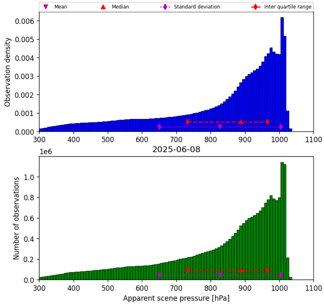
Figure 36: Histogram of “Apparent scene pressure” for 2025-06-07 to 2025-06-09
