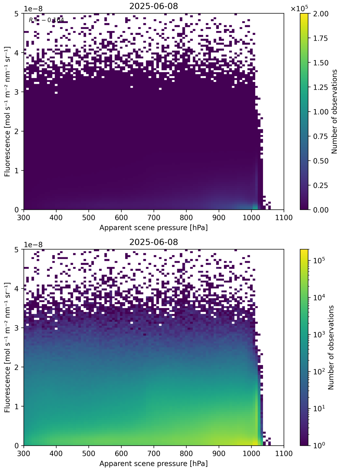
Figure 64: Scatter density plot of “Apparent scene pressure” against “Fluorescence” for 2025-06-07 to 2025-06-09.
