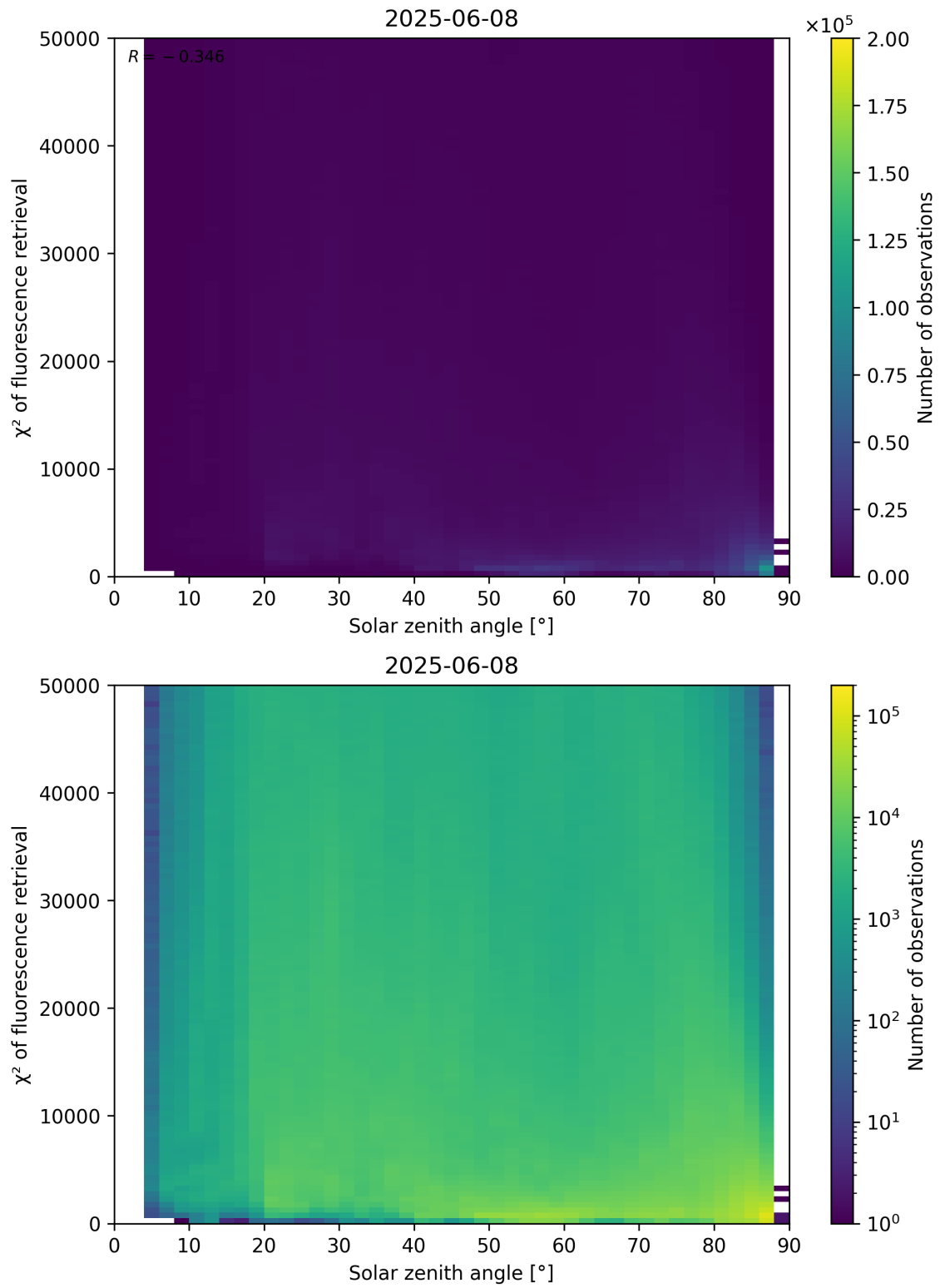
Figure 109: Scatter density plot of “Solar zenith angle” against “ \chi^2 of fluorescence retrieval” for 2025-06-07 to 2025-06-09.
