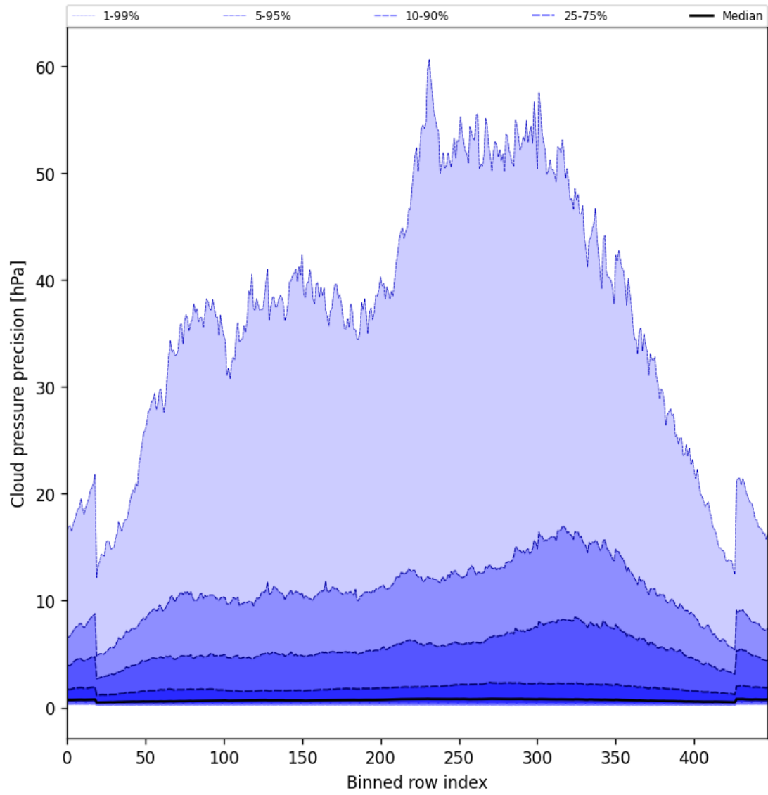
Figure 48: Along track statistics of “Cloud pressure precision” for 2025-06-07 to 2025-06-09
