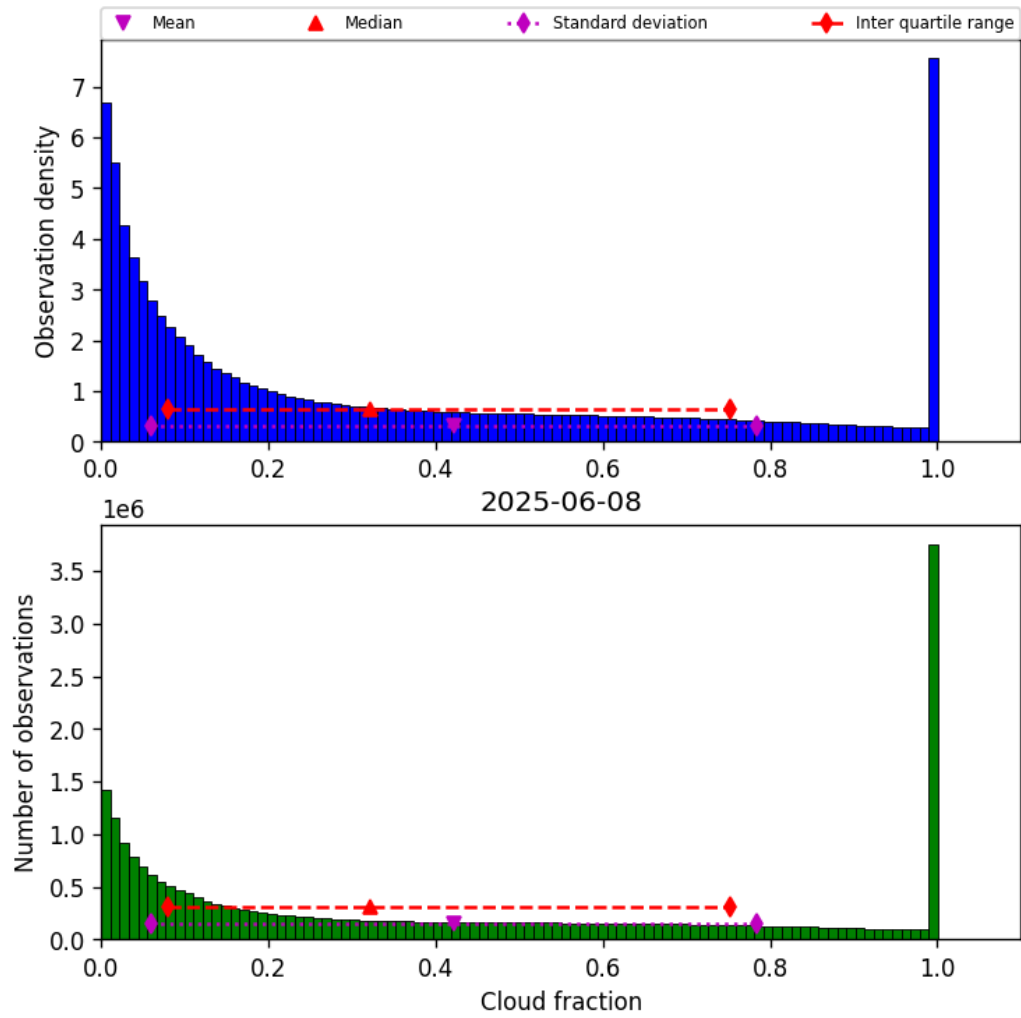
Figure 32: Histogram of “Cloud fraction” for 2025-06-07 to 2025-06-09
