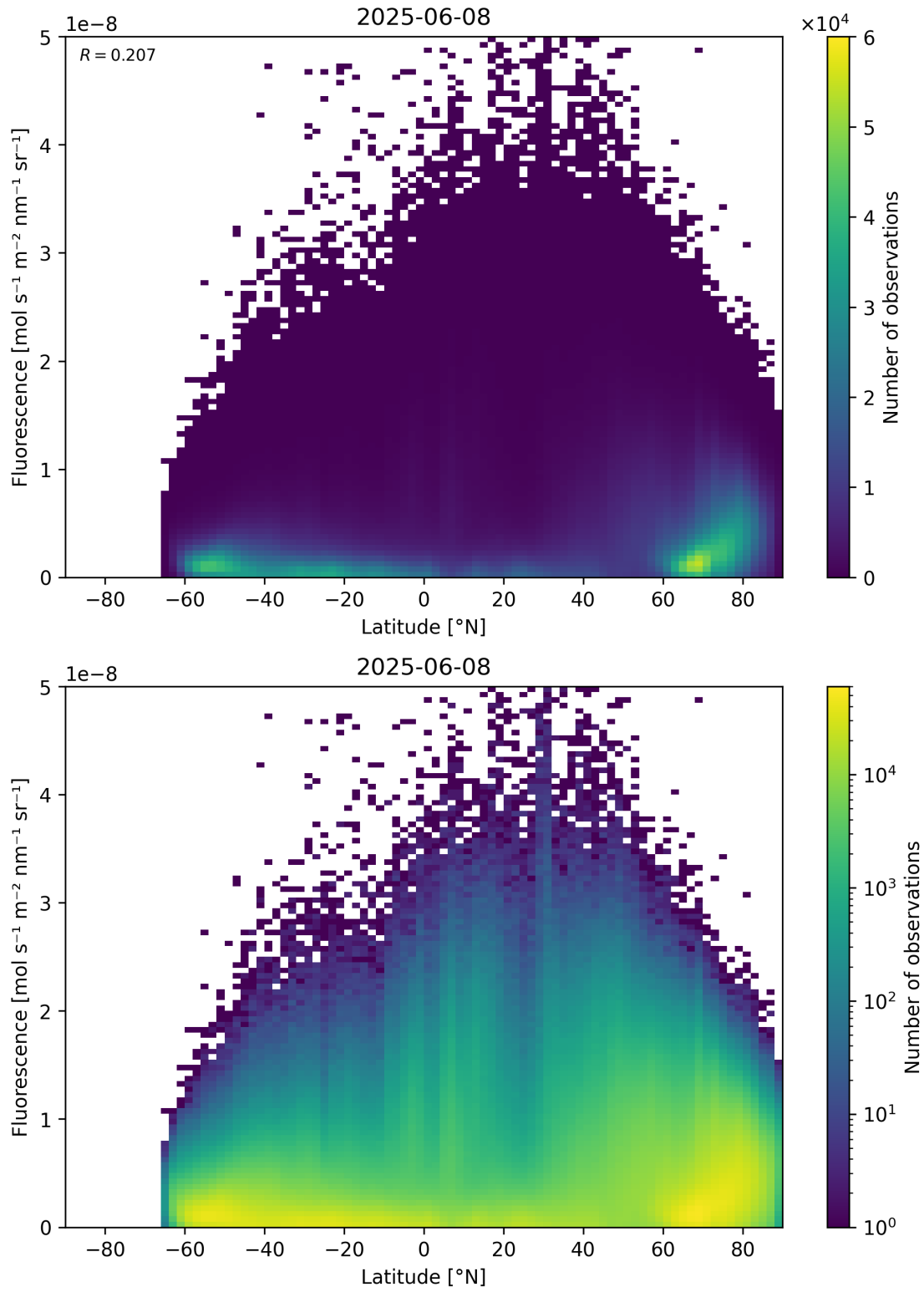
Figure 92: Scatter density plot of “Latitude” against “Fluorescence” for 2025-06-07 to 2025-06-09.
