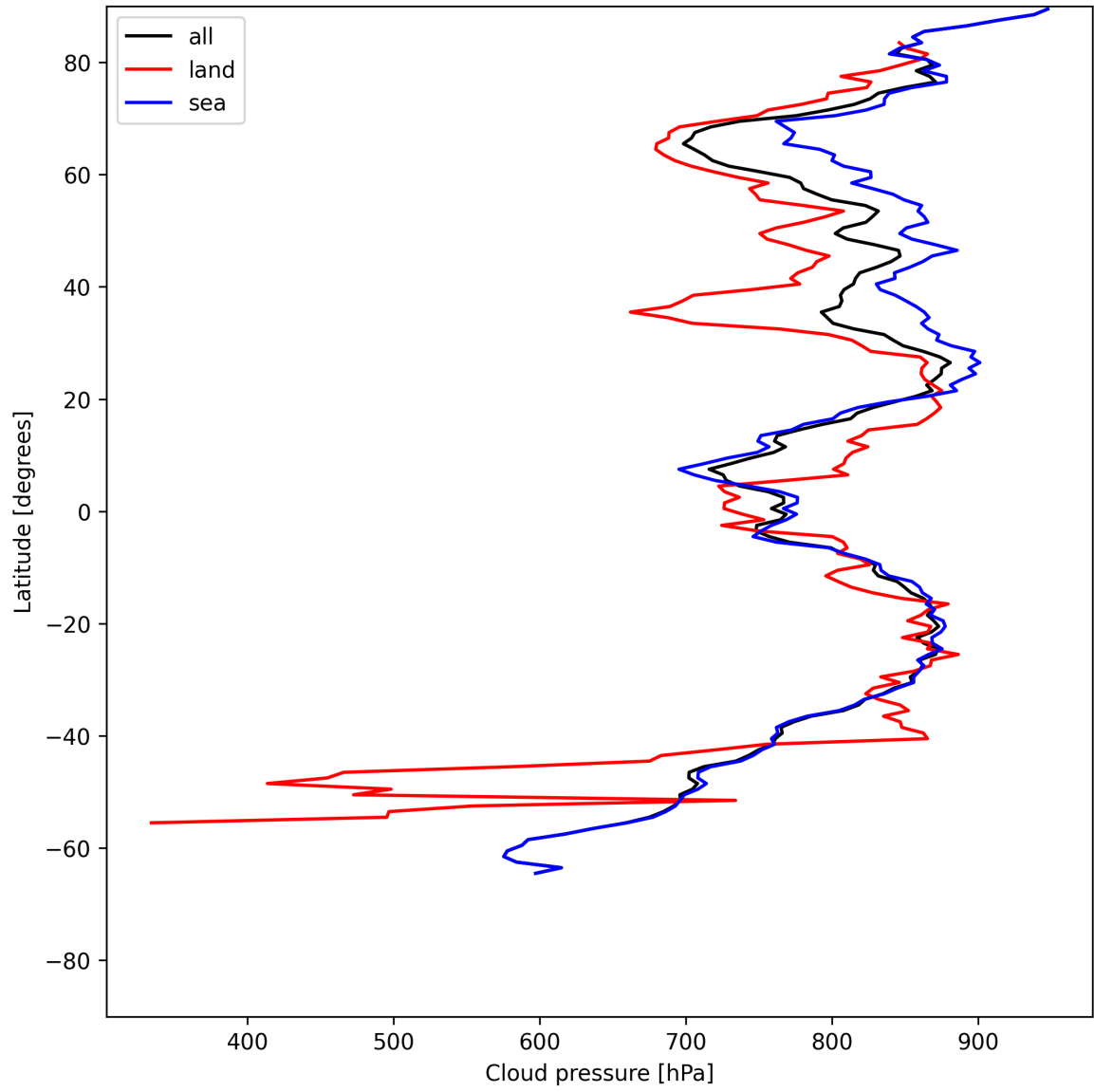
Figure 13: Zonal average of “Cloud pressure” for 2025-06-07 to 2025-06-09.
