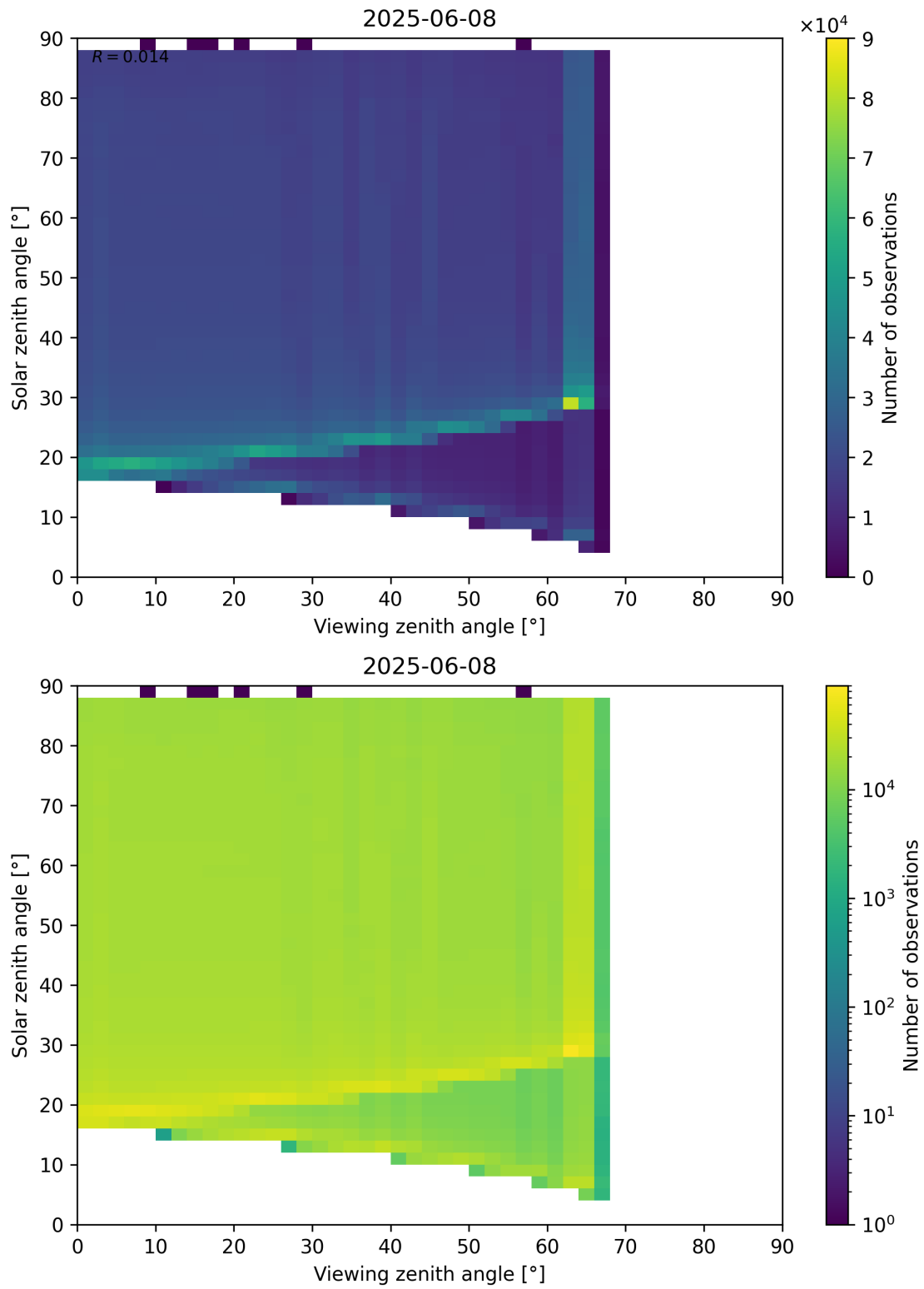
Figure 127: Scatter density plot of “Viewing zenith angle” against “Solar zenith angle” for 2025-06-07 to 2025-06-09.
