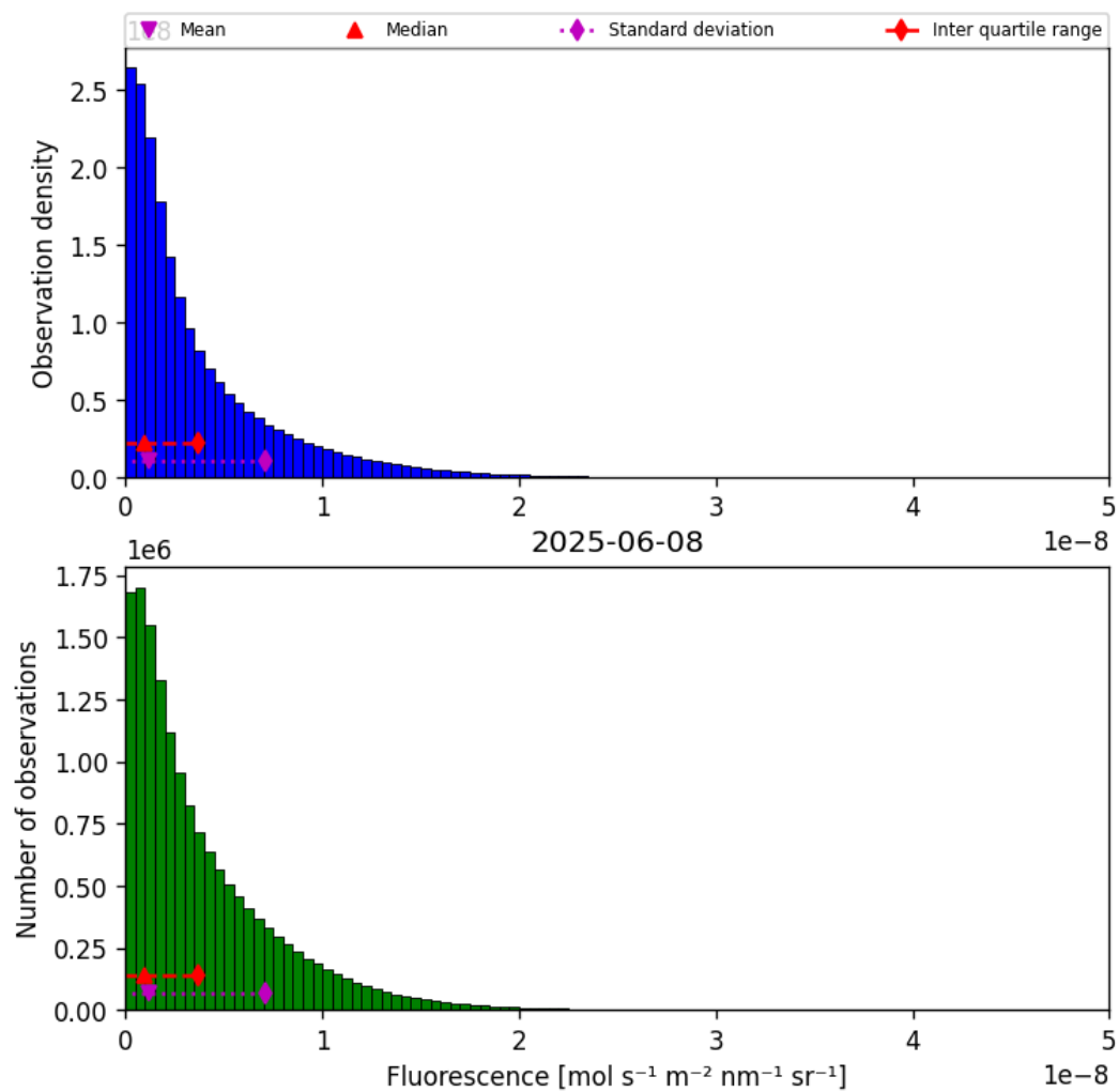
Figure 40: Histogram of “Fluorescence” for 2025-06-07 to 2025-06-09
