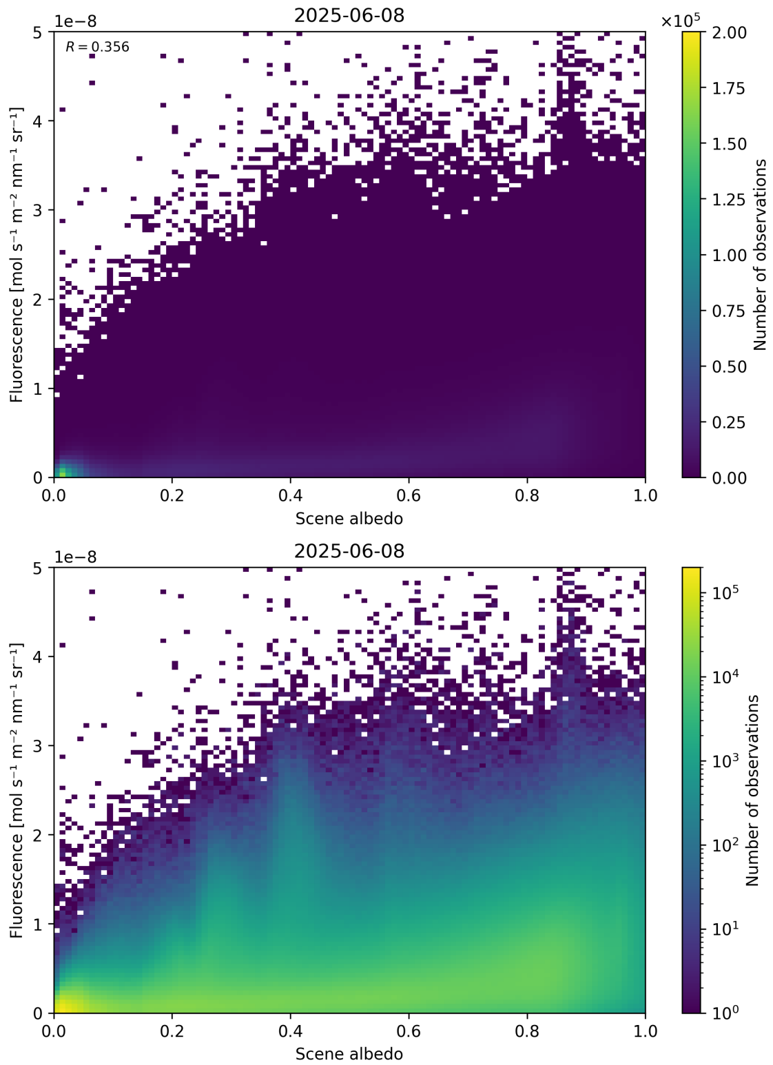
Figure 104: Scatter density plot of “Scene albedo” against “Fluorescence” for 2025-06-07 to 2025-06-09.
