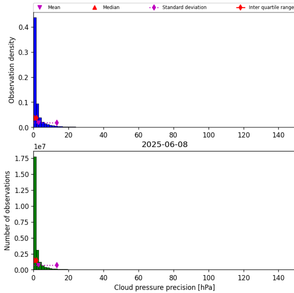
Figure 31: Histogram of “Cloud pressure precision” for 2025-06-07 to 2025-06-09
