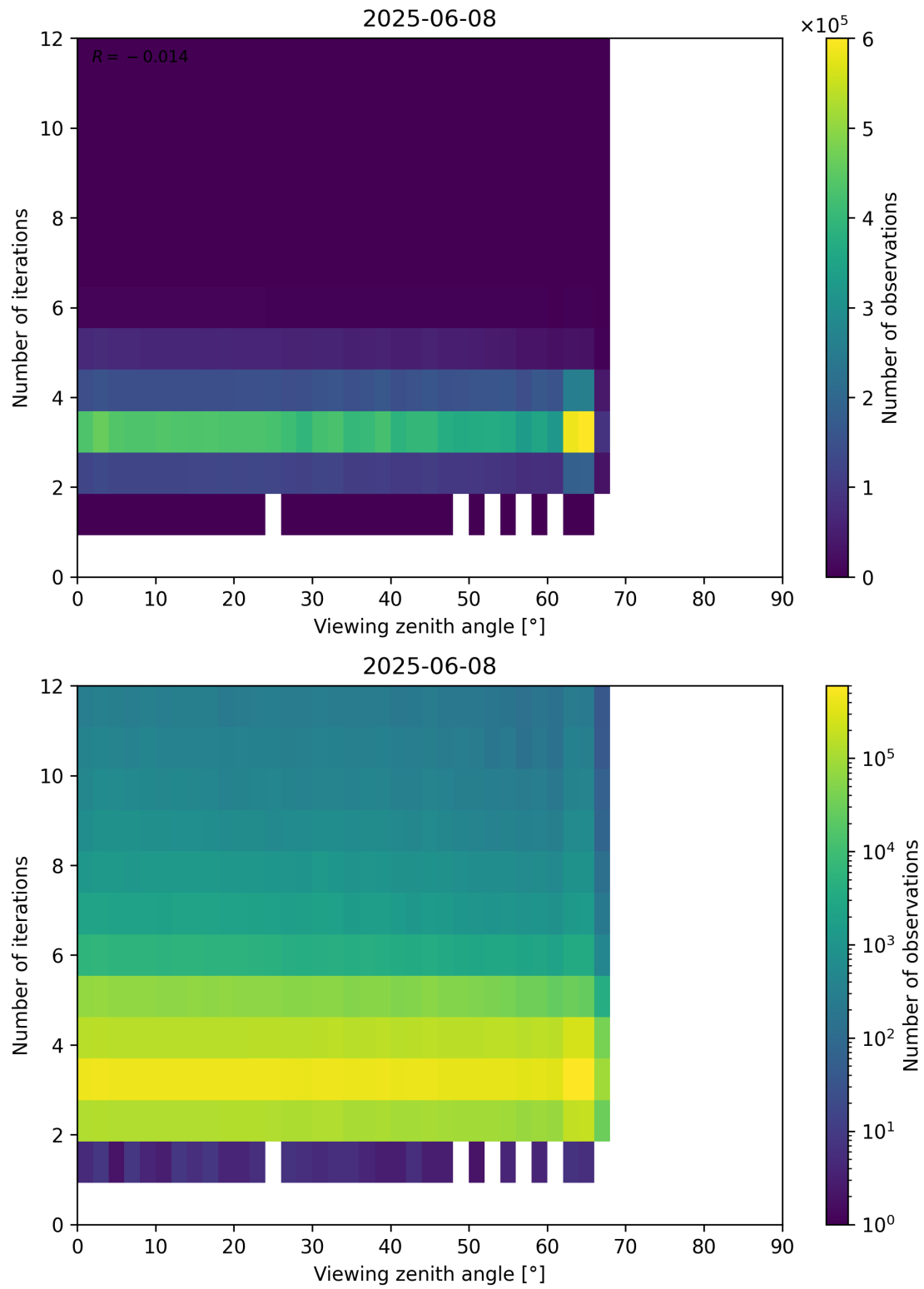
Figure 124: Scatter density plot of “Viewing zenith angle” against “Number of iterations” for 2025-06-07 to 2025-06-09.
