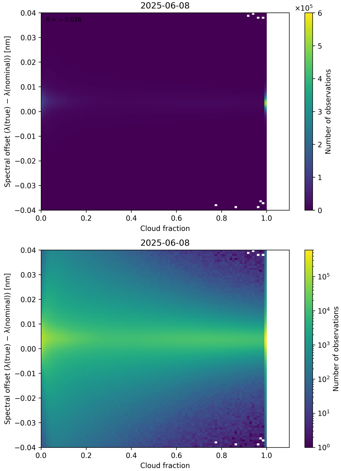
Figure 76: Scatter density plot of “Cloud fraction” against “Spectral offset ( \lambda_{\text{true}} - \lambda_{\text{nominal}} )” for 2025-06-07 to 2025-06-09.
