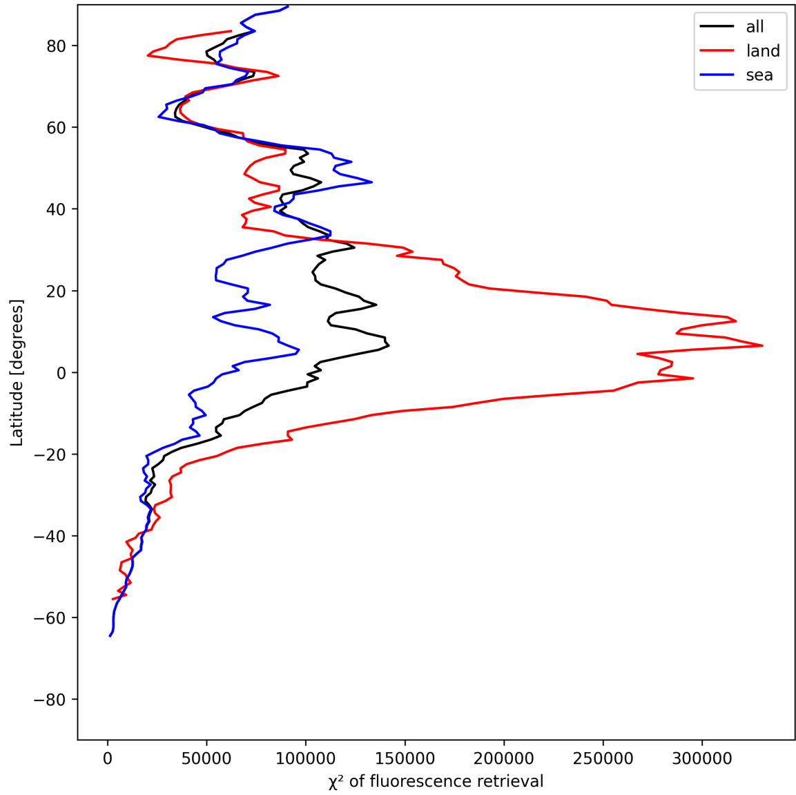
Figure 25: Zonal average of “ \chi^2 of fluorescence retrieval” for 2025-06-07 to 2025-06-09.
