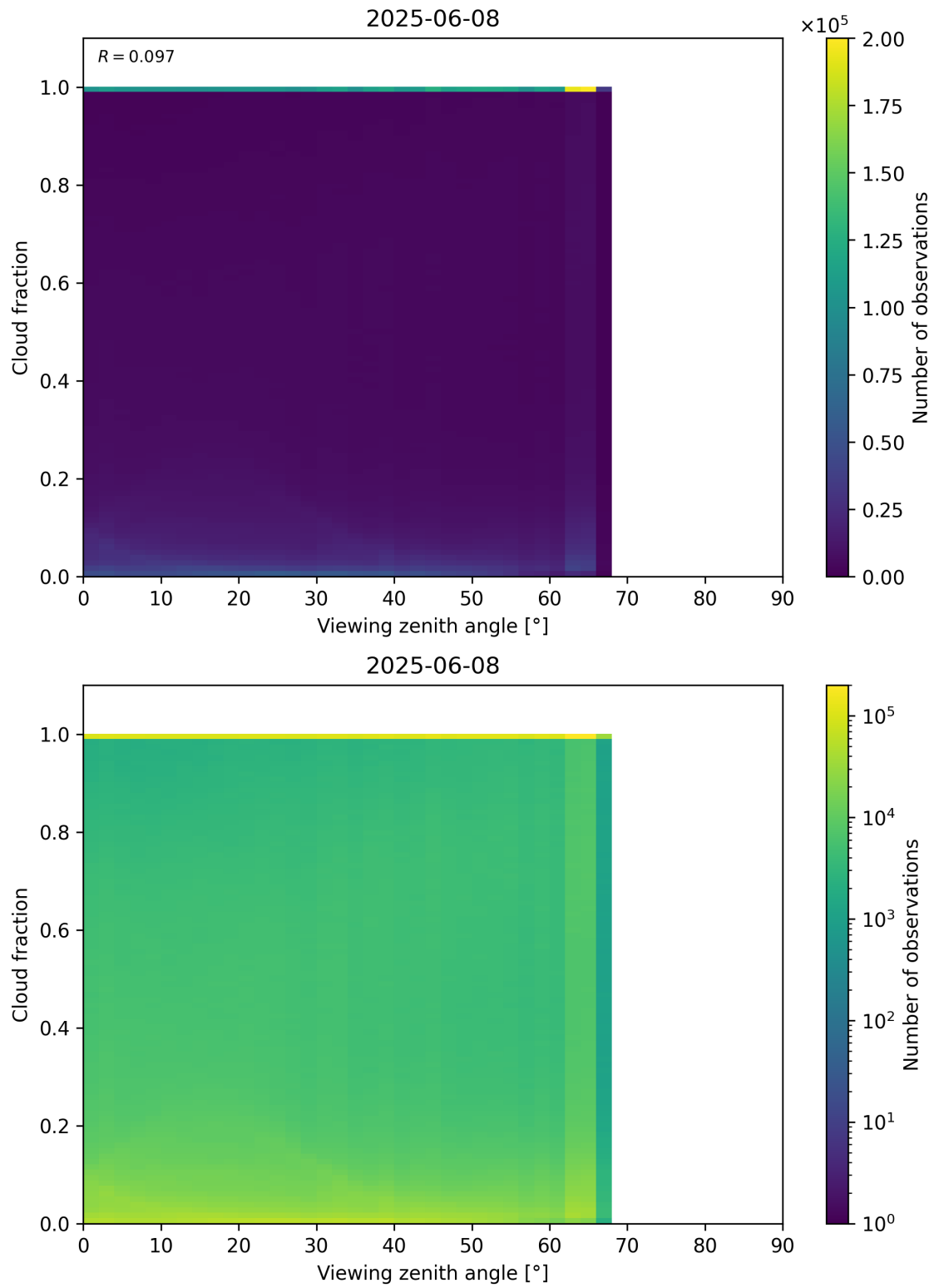
Figure 120: Scatter density plot of “Viewing zenith angle” against “Cloud fraction” for 2025-06-07 to 2025-06-09.
