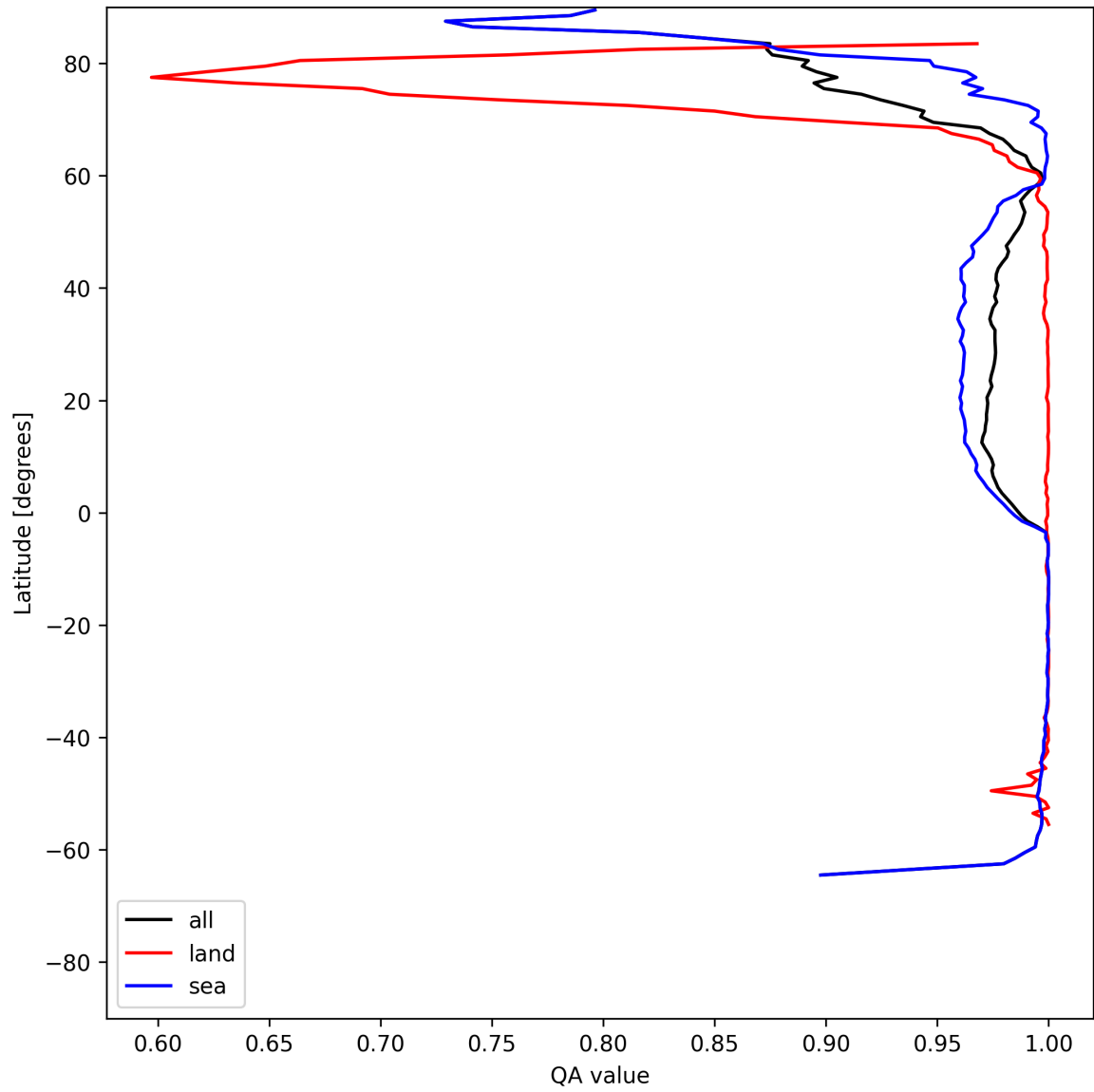
Figure 12: Zonal average of “QA value” for 2025-06-07 to 2025-06-09.
