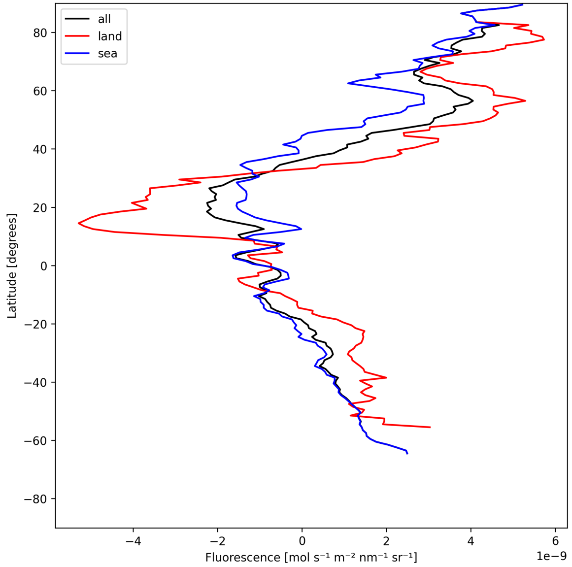
Figure 23: Zonal average of “Fluorescence” for 2025-06-07 to 2025-06-09.
