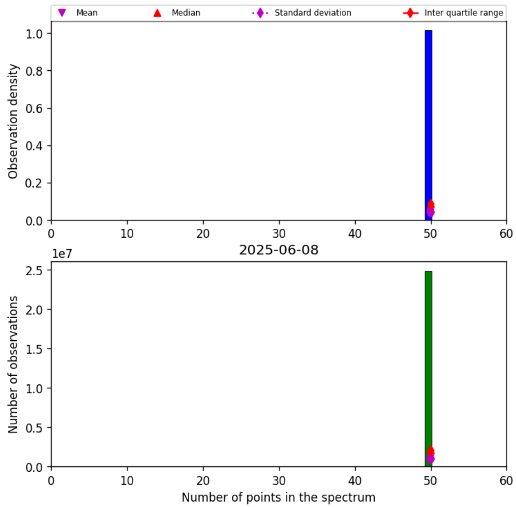
Figure 44: Histogram of “Number of points in the spectrum” for 2025-06-07 to 2025-06-09
