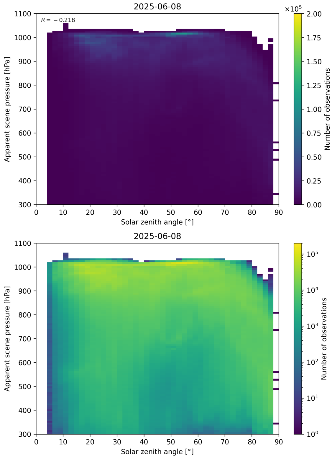
Figure 108: Scatter density plot of “Solar zenith angle” against “Apparent scene pressure” for 2025-06-07 to 2025-06-09.
