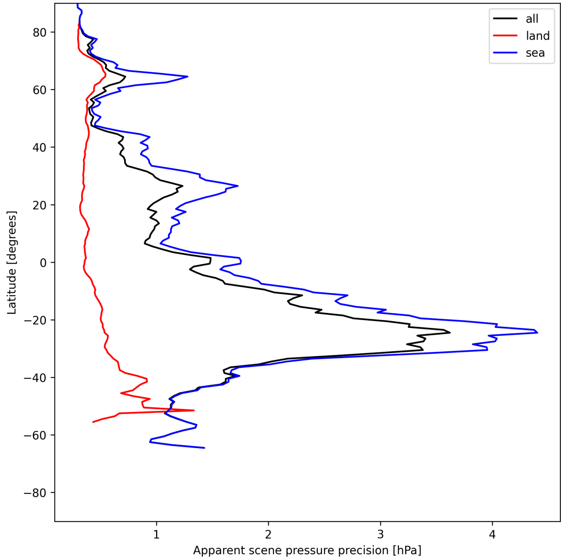
Figure 20: Zonal average of “Apparent scene pressure precision” for 2025-06-07 to 2025-06-09.
