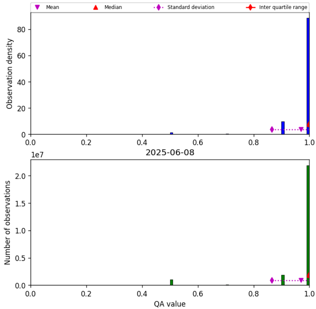
Figure 29: Histogram of “QA value” for 2025-06-07 to 2025-06-09
