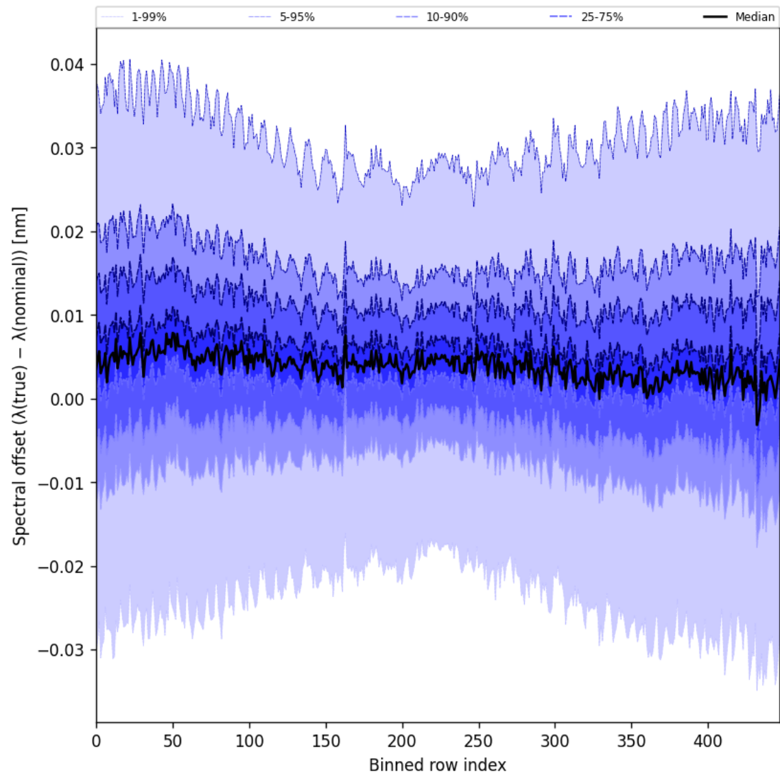
Figure 62: Along track statistics of “Spectral offset ( \lambda_{\text{true}} - \lambda_{\text{nominal}} )” for 2025-06-07 to 2025-06-09
