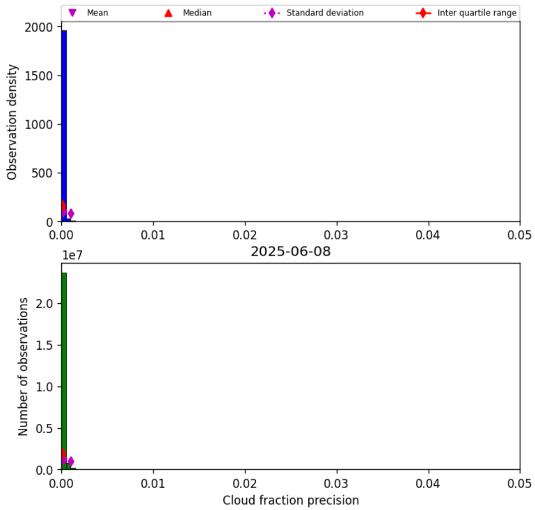
Figure 33: Histogram of “Cloud fraction precision” for 2025-06-07 to 2025-06-09
