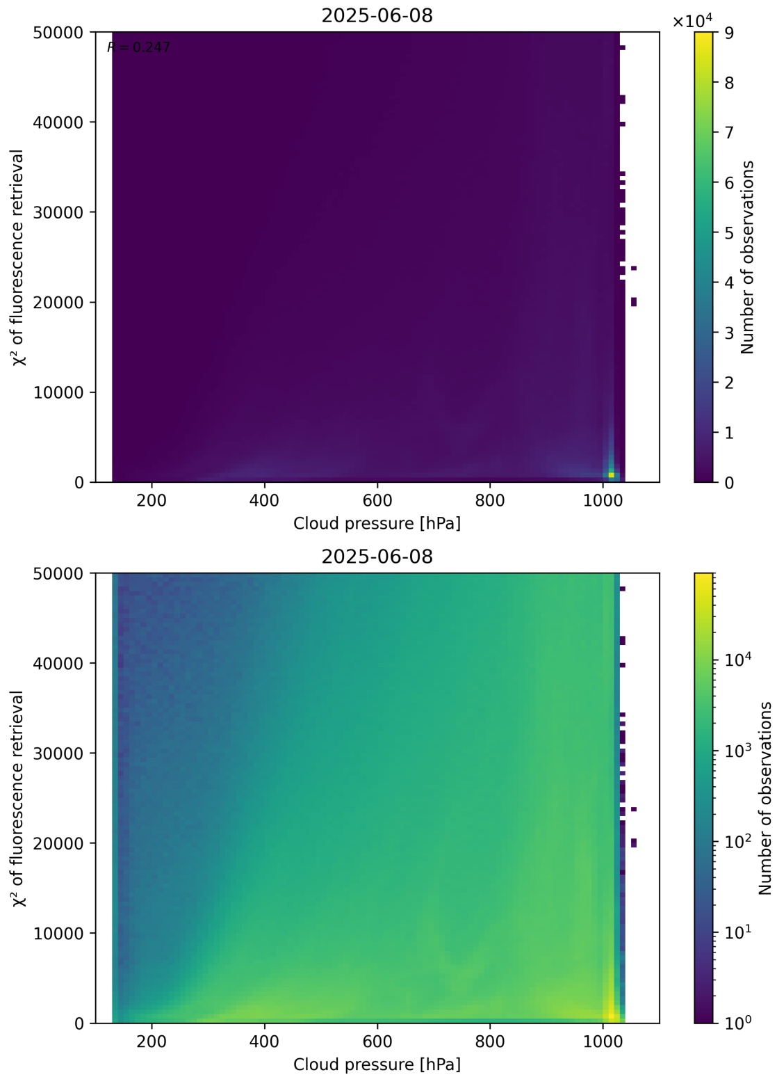
Figure 78: Scatter density plot of “Cloud pressure” against “ \chi^2 of fluorescence retrieval” for 2025-06-07 to 2025-06-09.
