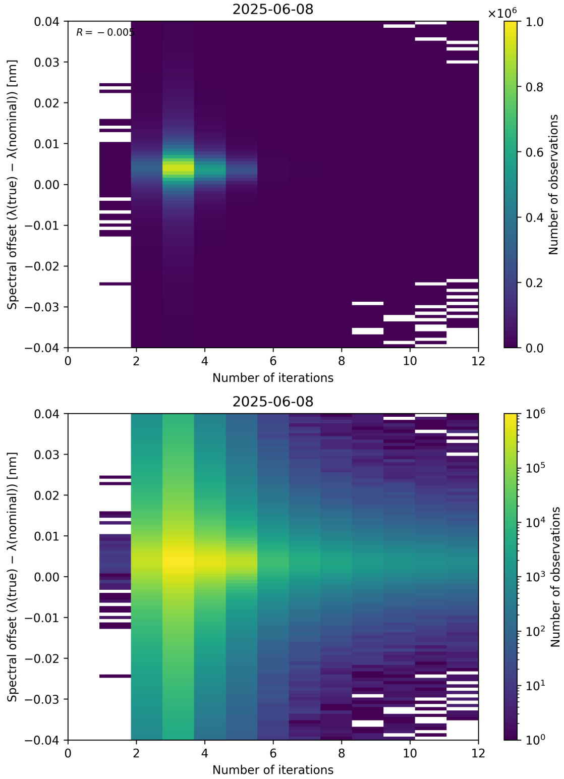
Figure 100: Scatter density plot of “Number of iterations” against “Spectral offset ( \lambda_{\text{true}} - \lambda_{\text{nominal}} )” for 2025-06-07 to 2025-06-09.
