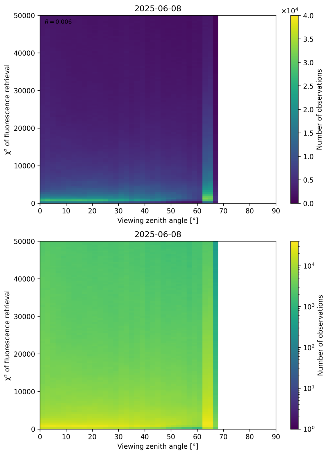
Figure 119: Scatter density plot of “Viewing zenith angle” against “ \chi^2 of fluorescence retrieval” for 2025-06-07 to 2025-06-09.
