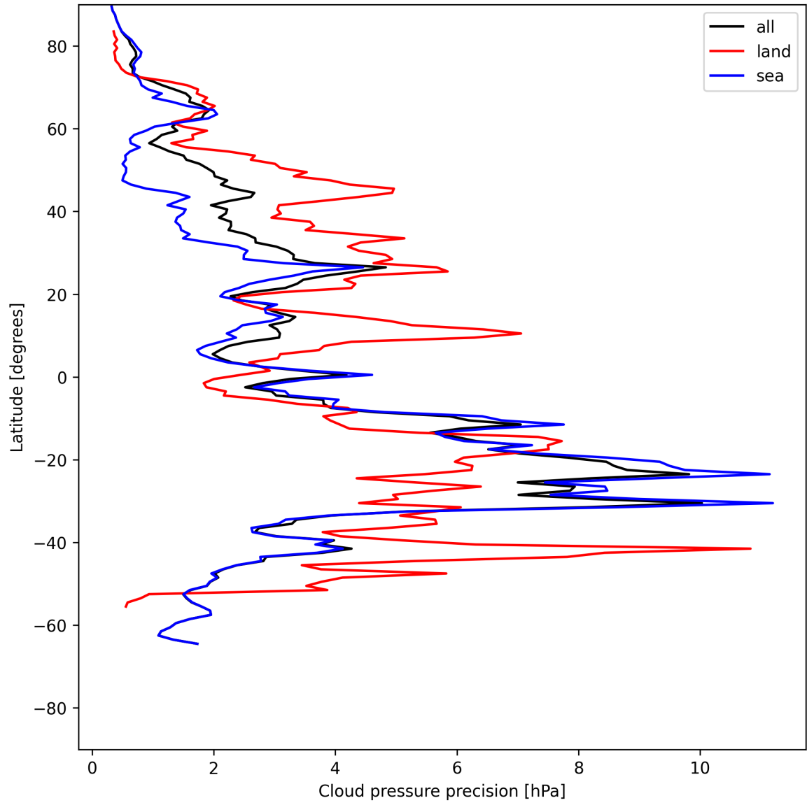
Figure 14: Zonal average of “Cloud pressure precision” for 2025-06-07 to 2025-06-09.
