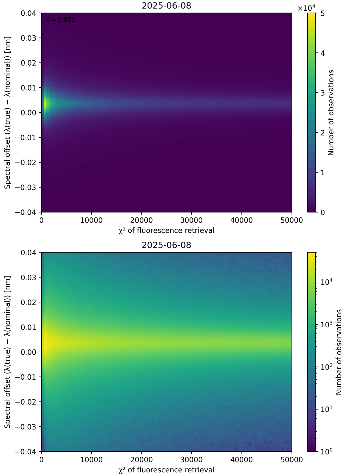
Figure 69: Scatter density plot of “ \chi^2 of fluorescence retrieval” against “Spectral offset ( \lambda_{\text{true}} - \lambda_{\text{nominal}} )” for 2025-06-07 to 2025-06-09.
