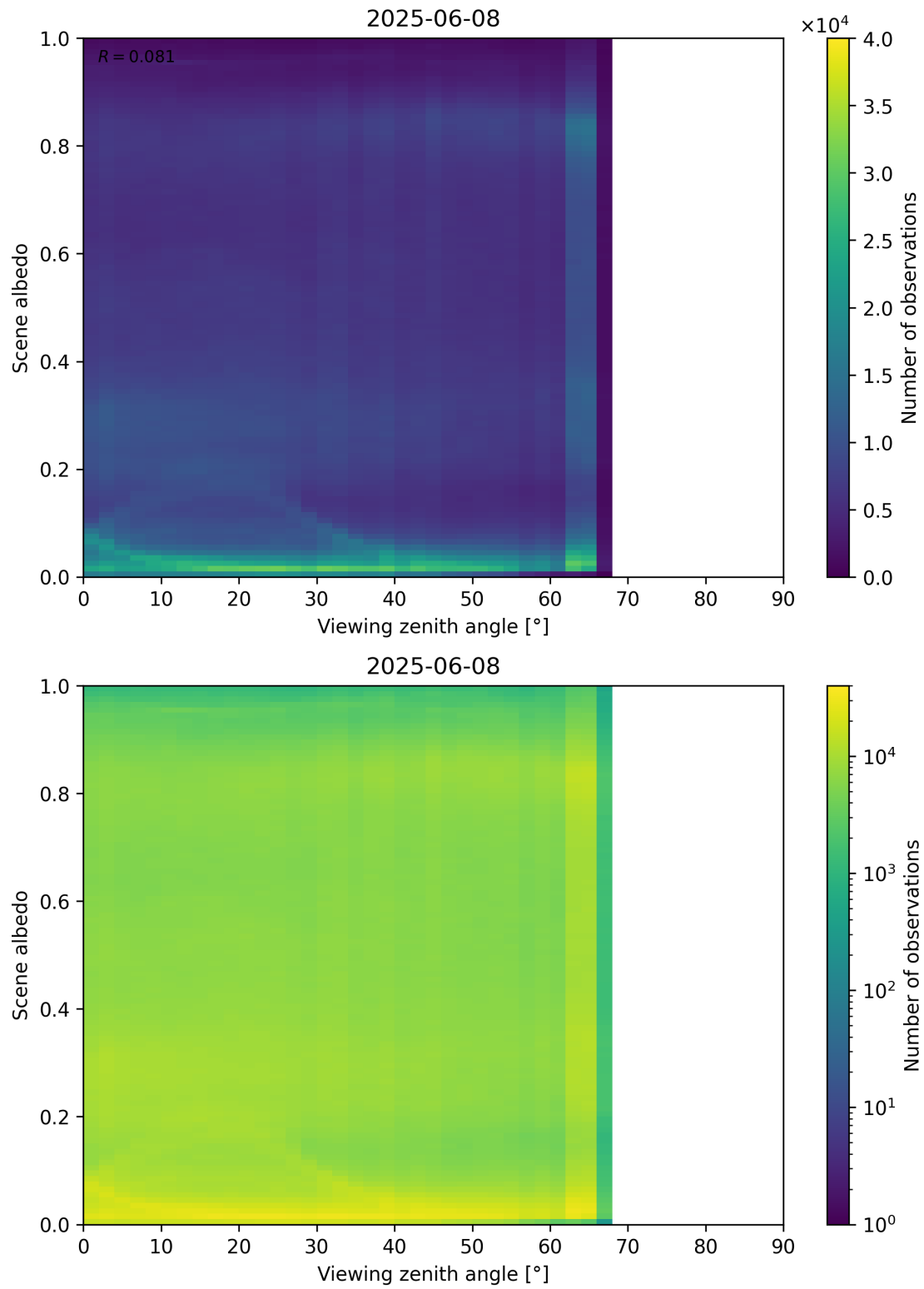
Figure 126: Scatter density plot of “Viewing zenith angle” against “Scene albedo” for 2025-06-07 to 2025-06-09.
