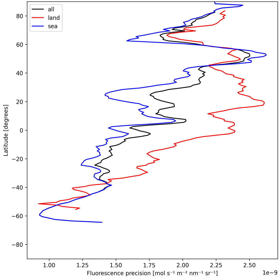
Figure 24: Zonal average of “Fluorescence precision” for 2025-06-07 to 2025-06-09.
