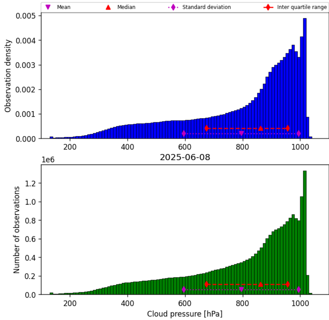
Figure 30: Histogram of “Cloud pressure” for 2025-06-07 to 2025-06-09
