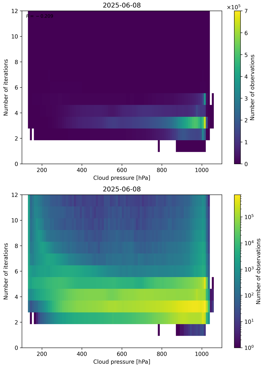
Figure 81: Scatter density plot of “Cloud pressure” against “Number of iterations” for 2025-06-07 to 2025-06-09.
