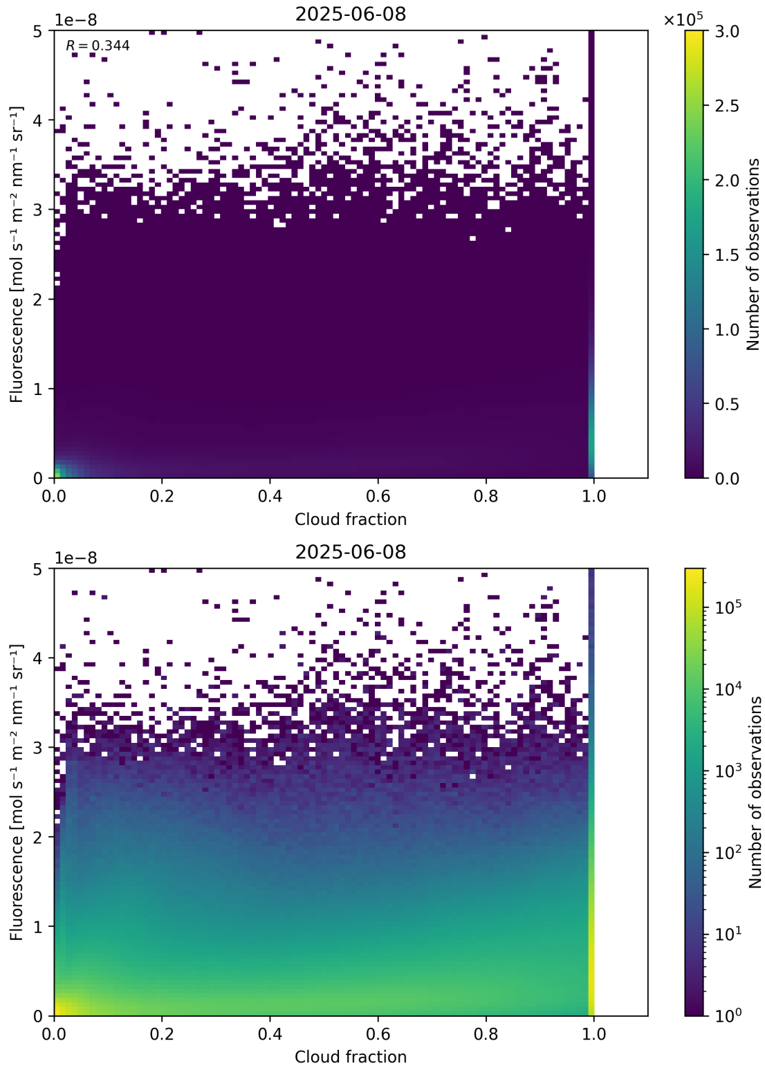
Figure 72: Scatter density plot of “Cloud fraction” against “Fluorescence” for 2025-06-07 to 2025-06-09.
