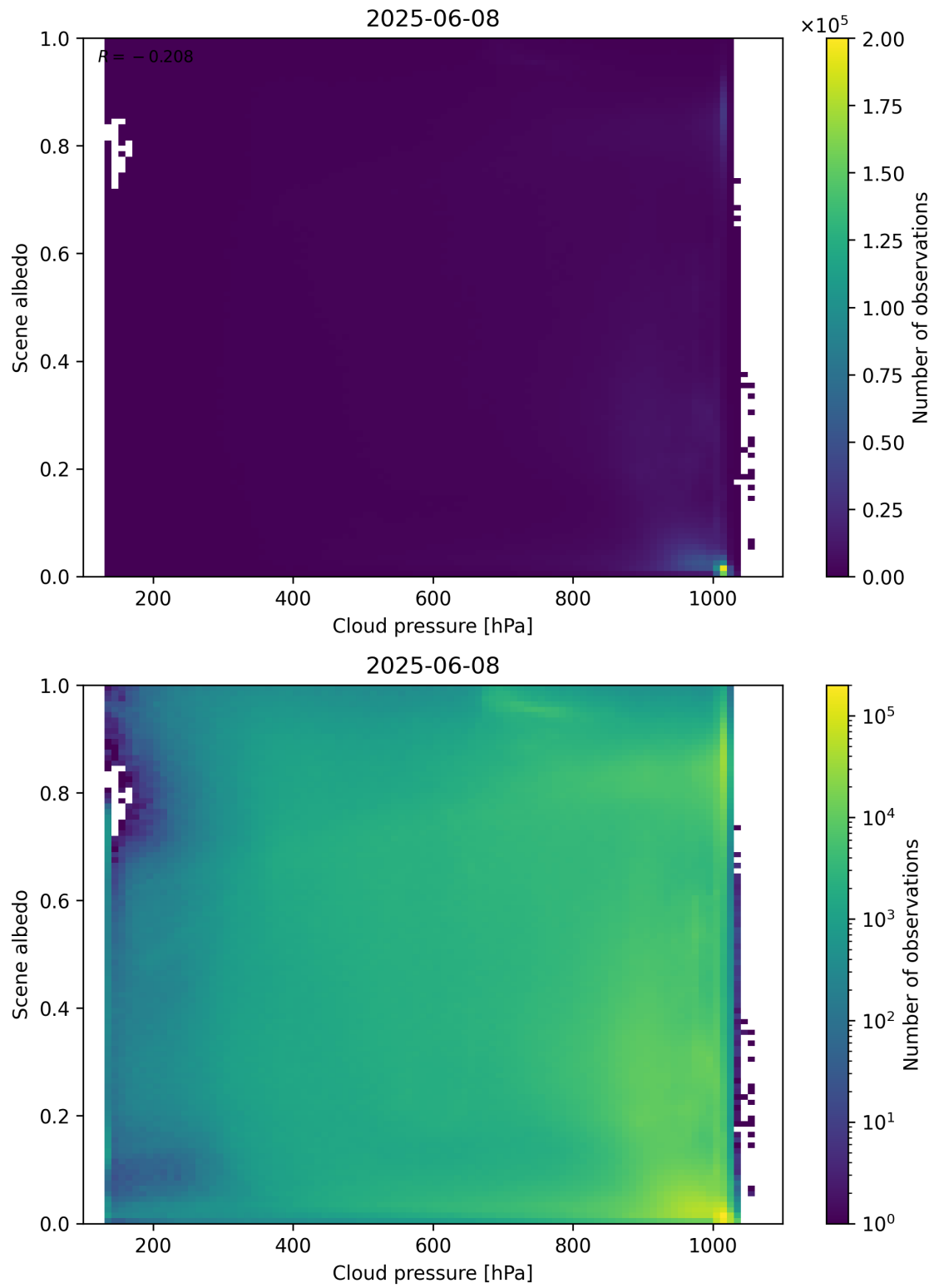
Figure 83: Scatter density plot of “Cloud pressure” against “Scene albedo” for 2025-06-07 to 2025-06-09.
