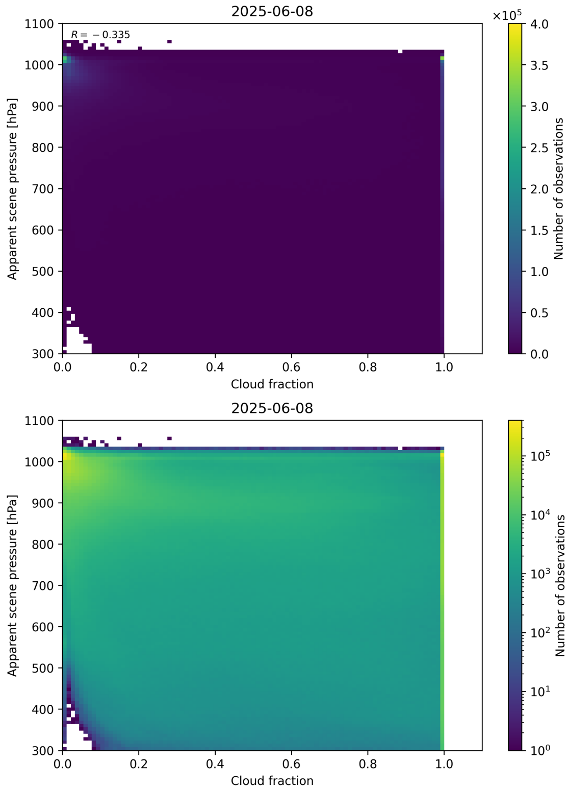
Figure 70: Scatter density plot of “Cloud fraction” against “Apparent scene pressure” for 2025-06-07 to 2025-06-09.
