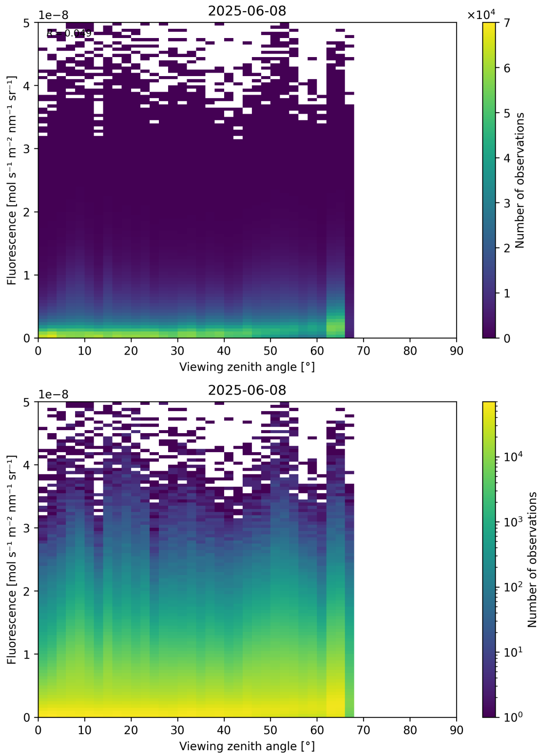
Figure 122: Scatter density plot of “Viewing zenith angle” against “Fluorescence” for 2025-06-07 to 2025-06-09.
