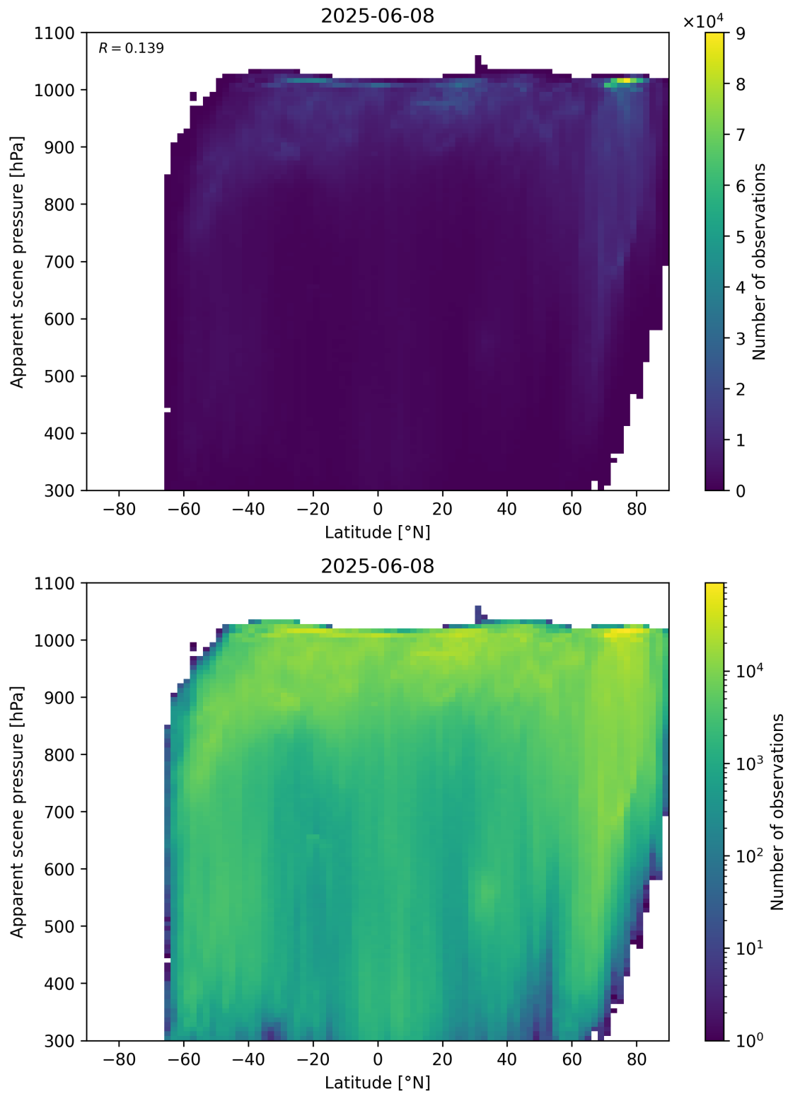
Figure 88: Scatter density plot of “Latitude” against “Apparent scene pressure” for 2025-06-07 to 2025-06-09.
