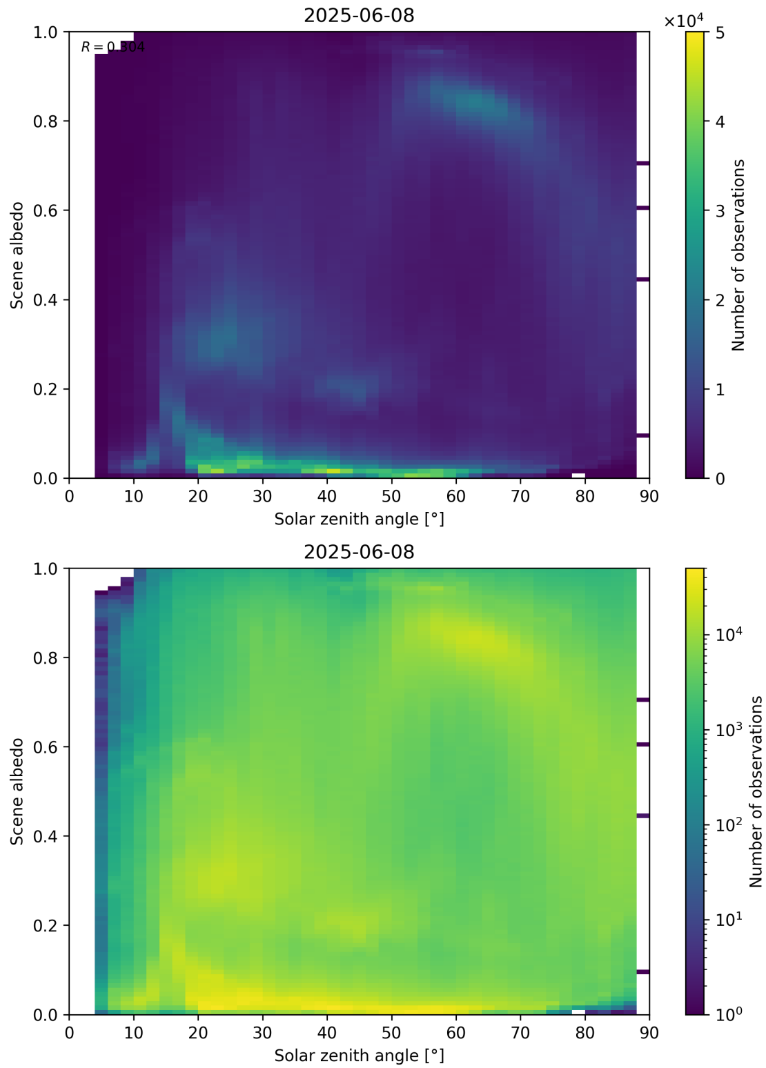
Figure 116: Scatter density plot of “Solar zenith angle” against “Scene albedo” for 2025-06-07 to 2025-06-09.
