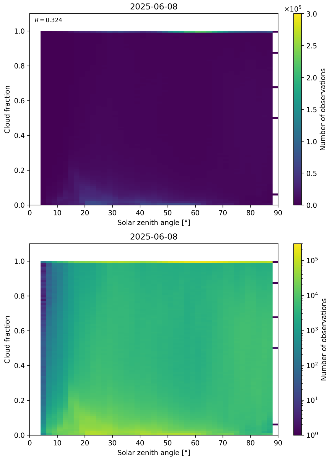
Figure 110: Scatter density plot of “Solar zenith angle” against “Cloud fraction” for 2025-06-07 to 2025-06-09.
