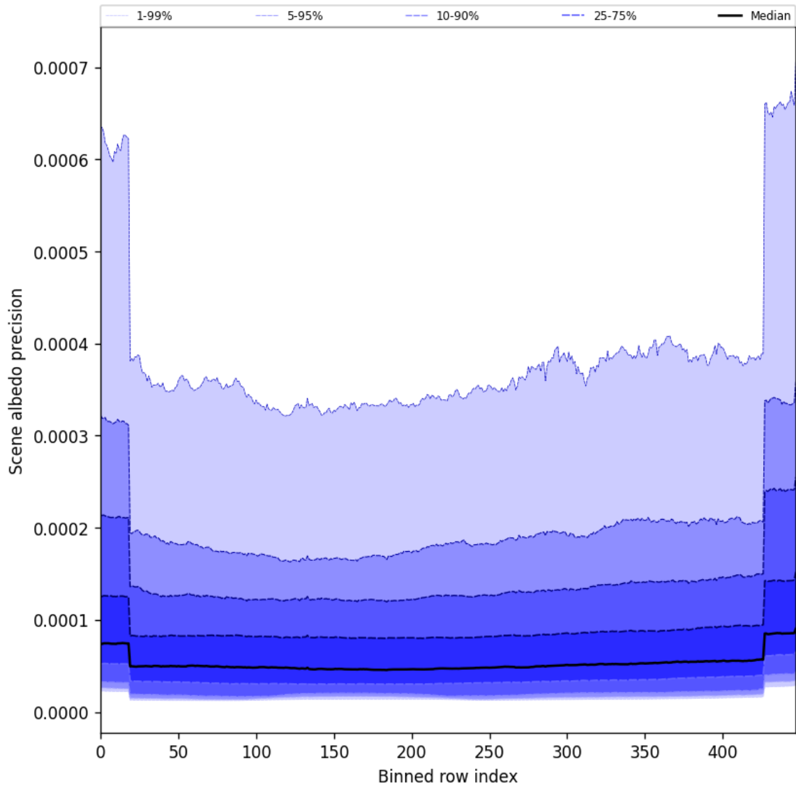
Figure 52: Along track statistics of “Scene albedo precision” for 2025-06-07 to 2025-06-09
