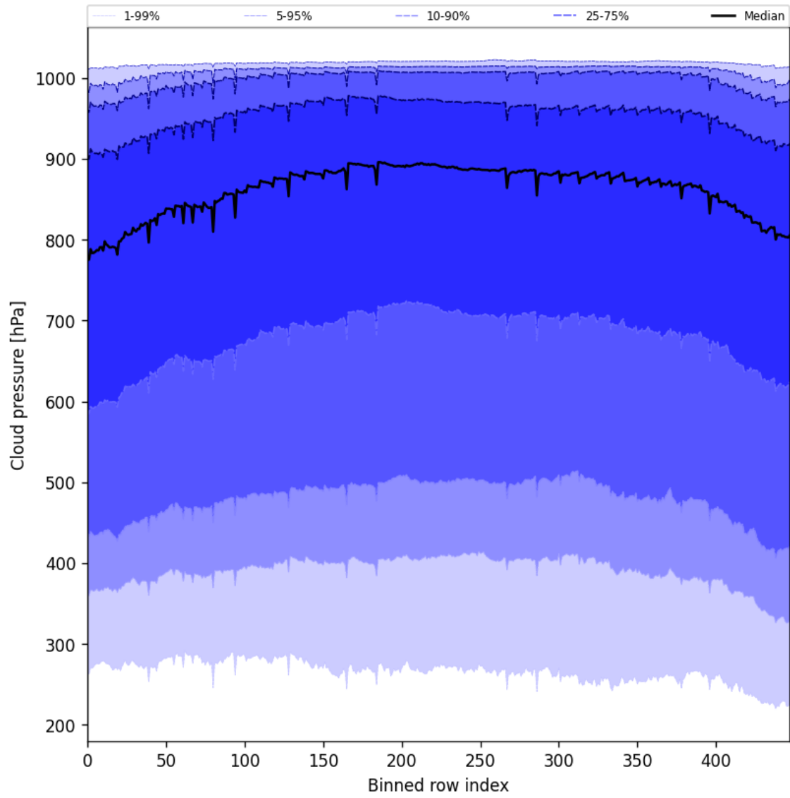
Figure 47: Along track statistics of “Cloud pressure” for 2025-06-07 to 2025-06-09
