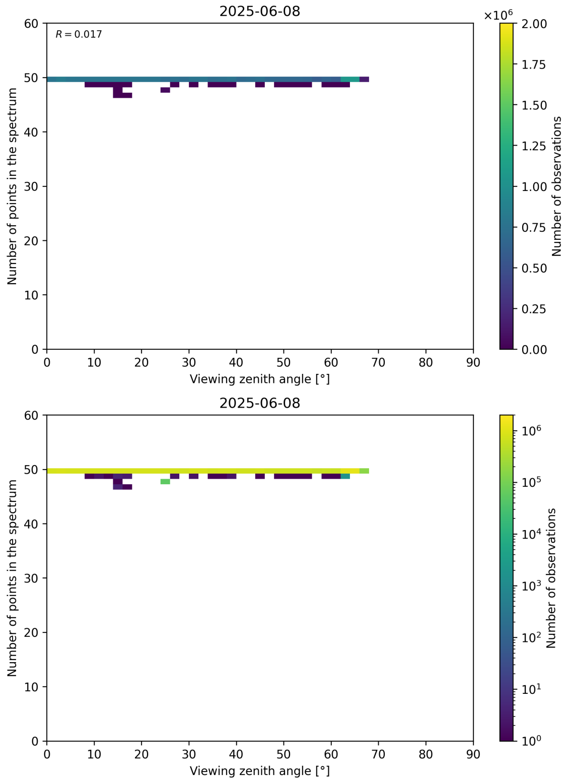
Figure 125: Scatter density plot of “Viewing zenith angle” against “Number of points in the spectrum” for 2025-06-07 to 2025-06-09.
