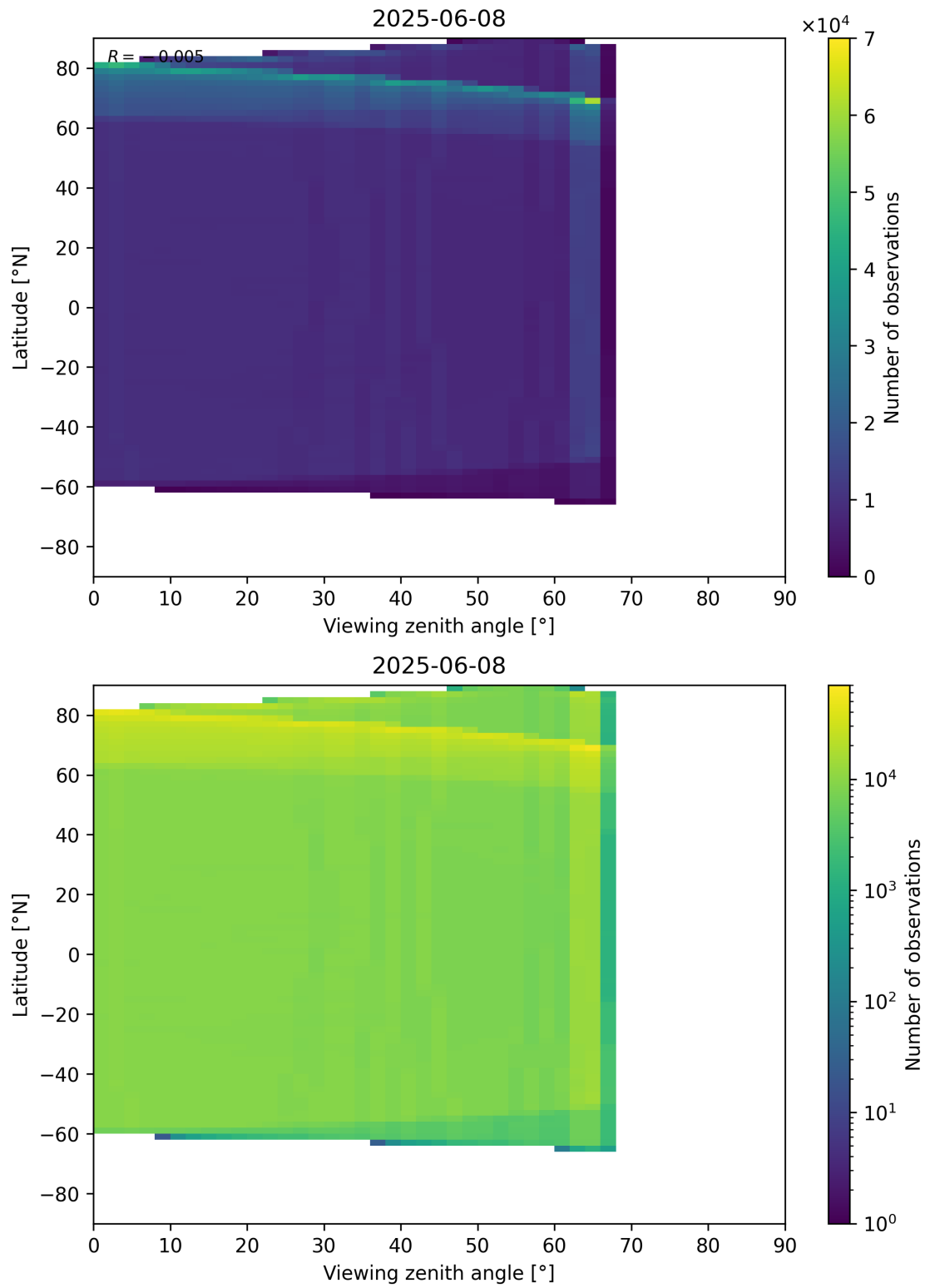
Figure 123: Scatter density plot of “Viewing zenith angle” against “Latitude” for 2025-06-07 to 2025-06-09.
