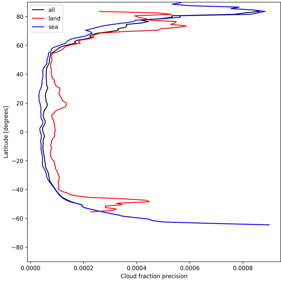
Figure 16: Zonal average of “Cloud fraction precision” for 2025-06-07 to 2025-06-09.
