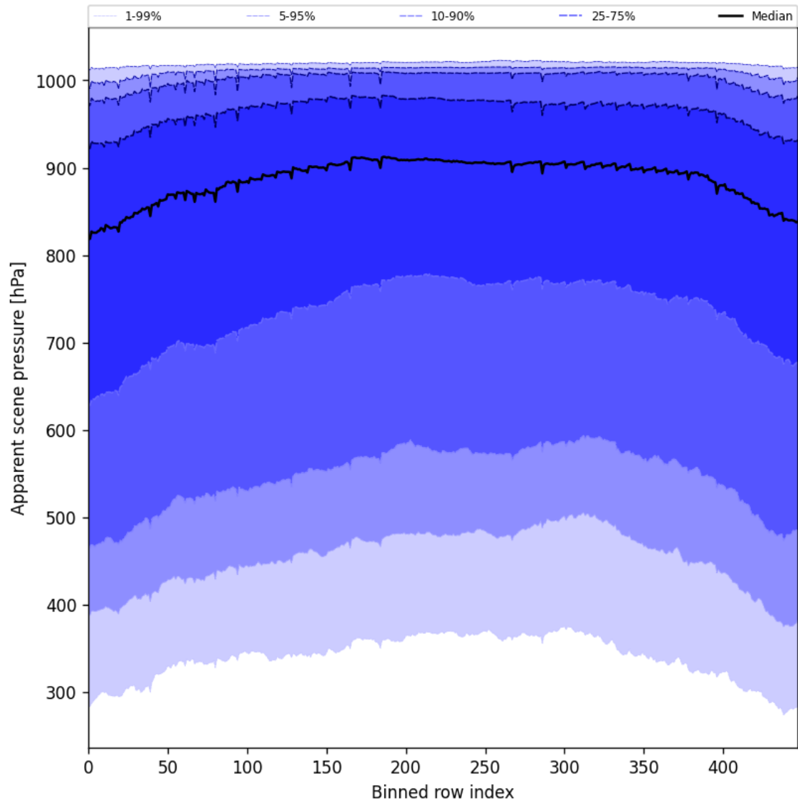
Figure 53: Along track statistics of “Apparent scene pressure” for 2025-06-07 to 2025-06-09
