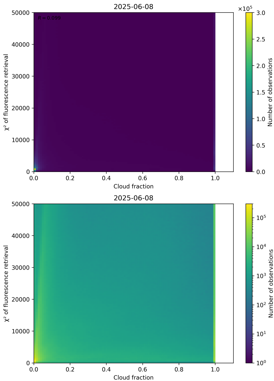
Figure 71: Scatter density plot of “Cloud fraction” against “ \chi^2 of fluorescence retrieval” for 2025-06-07 to 2025-06-09.
