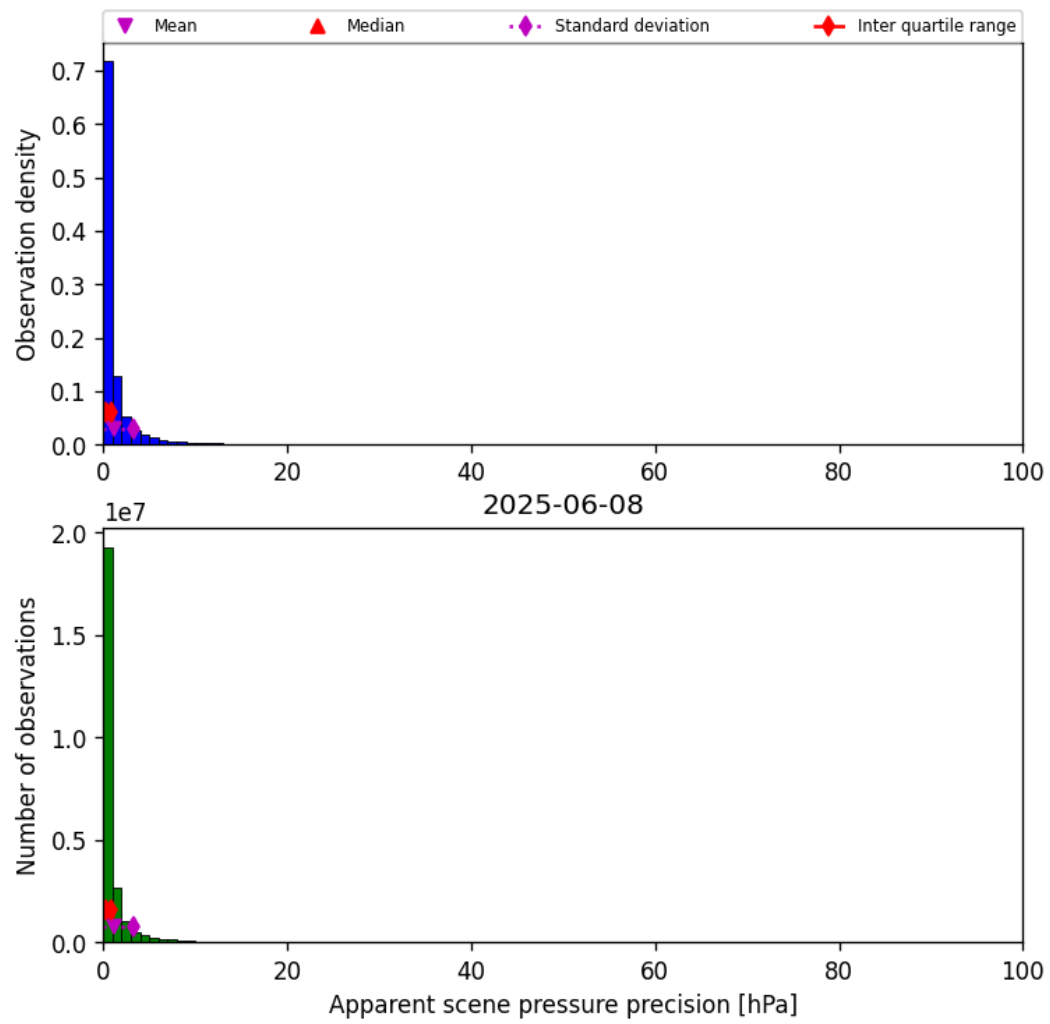
Figure 37: Histogram of “Apparent scene pressure precision” for 2025-06-07 to 2025-06-09
