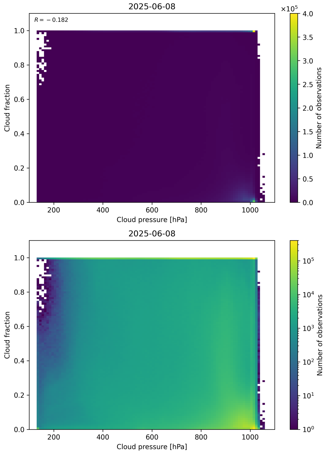
Figure 79: Scatter density plot of “Cloud pressure” against “Cloud fraction” for 2025-06-07 to 2025-06-09.
