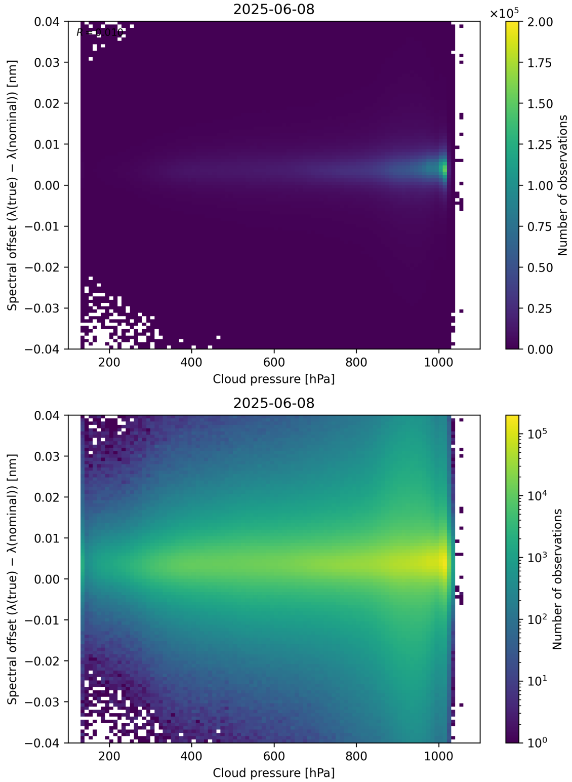
Figure 84: Scatter density plot of “Cloud pressure” against “Spectral offset ( \lambda_{\text{true}} - \lambda_{\text{nominal}} )” for 2025-06-07 to 2025-06-09.
