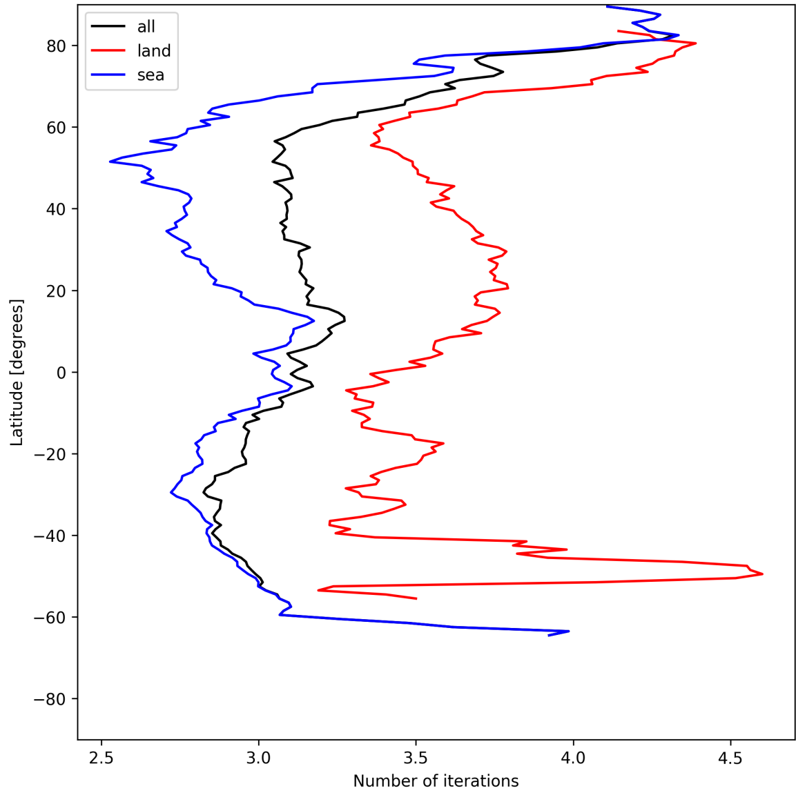
Figure 22: Zonal average of “Number of iterations” for 2025-06-07 to 2025-06-09.
