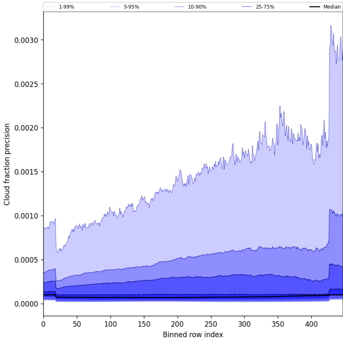
Figure 50: Along track statistics of “Cloud fraction precision” for 2025-06-07 to 2025-06-09
