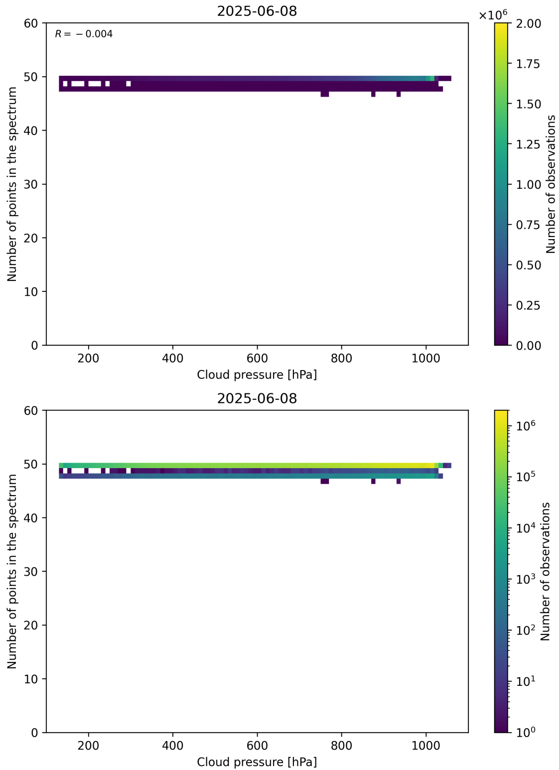
Figure 82: Scatter density plot of “Cloud pressure” against “Number of points in the spectrum” for 2025-06-07 to 2025-06-09.
