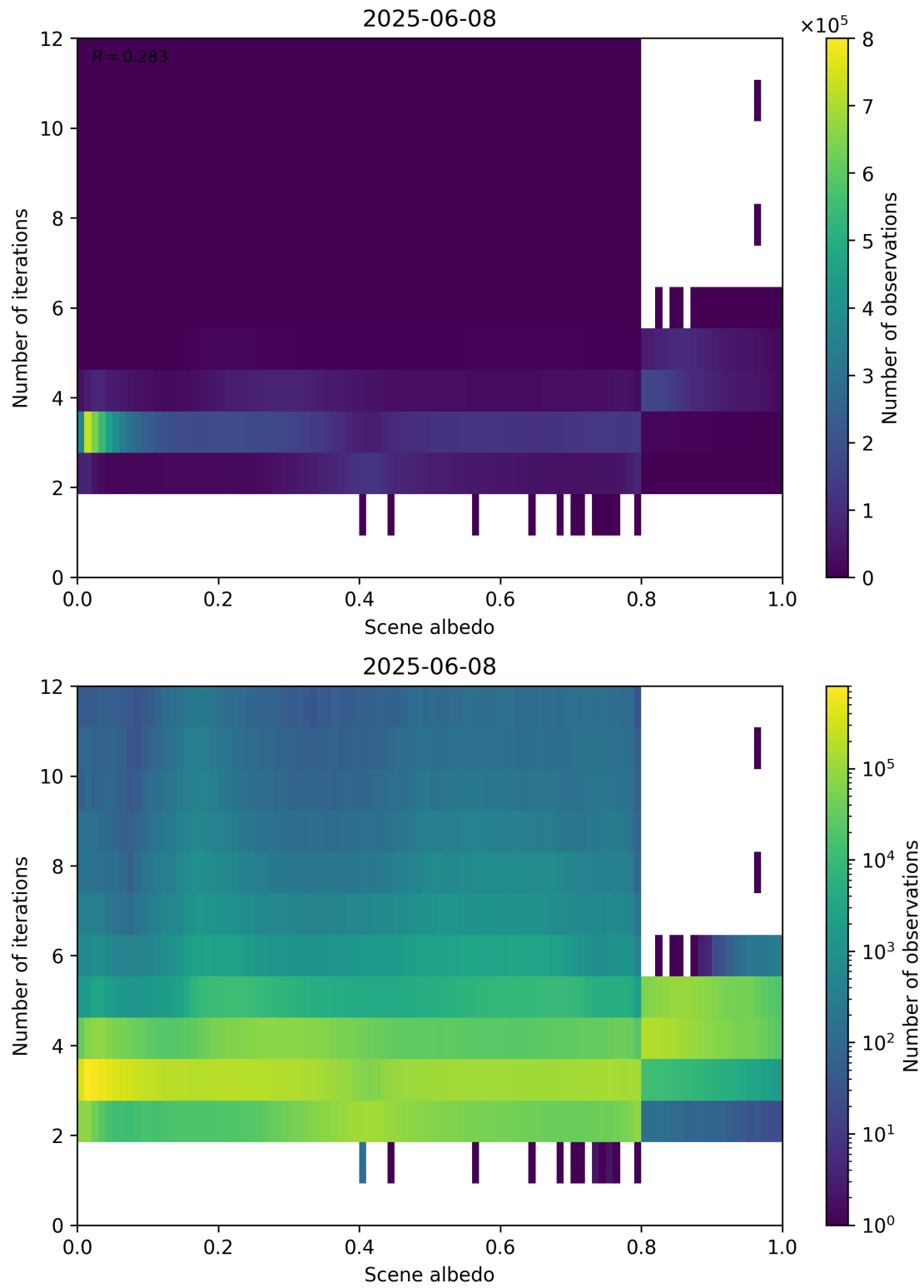
Figure 105: Scatter density plot of “Scene albedo” against “Number of iterations” for 2025-06-07 to 2025-06-09.
