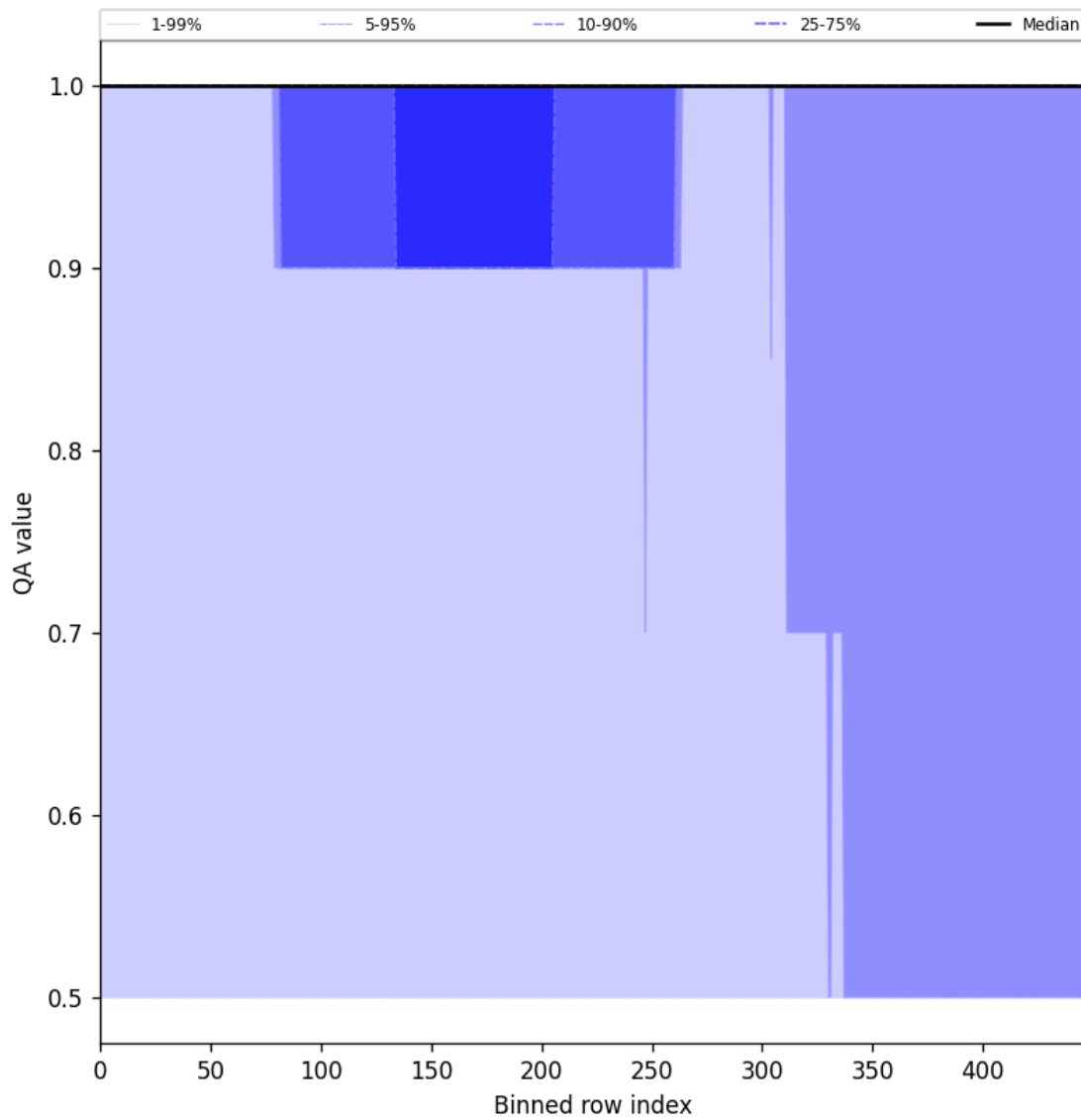
Figure 46: Along track statistics of “QA value” for 2025-06-07 to 2025-06-09
