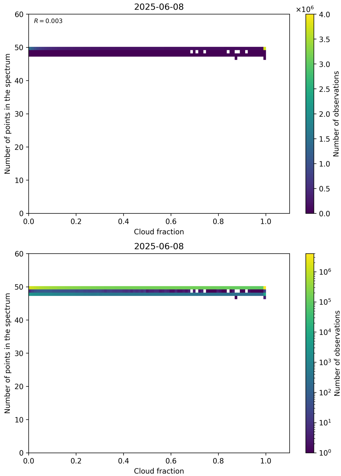
Figure 74: Scatter density plot of “Cloud fraction” against “Number of points in the spectrum” for 2025-06-07 to 2025-06-09.
