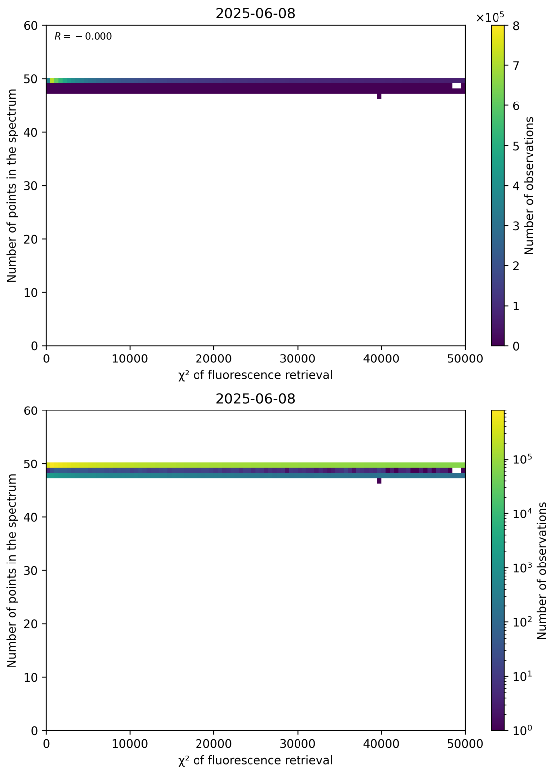
Figure 68: Scatter density plot of " \chi^2 of fluorescence retrieval" against "Number of points in the spectrum" for 2025-06-07 to 2025-06-09.
