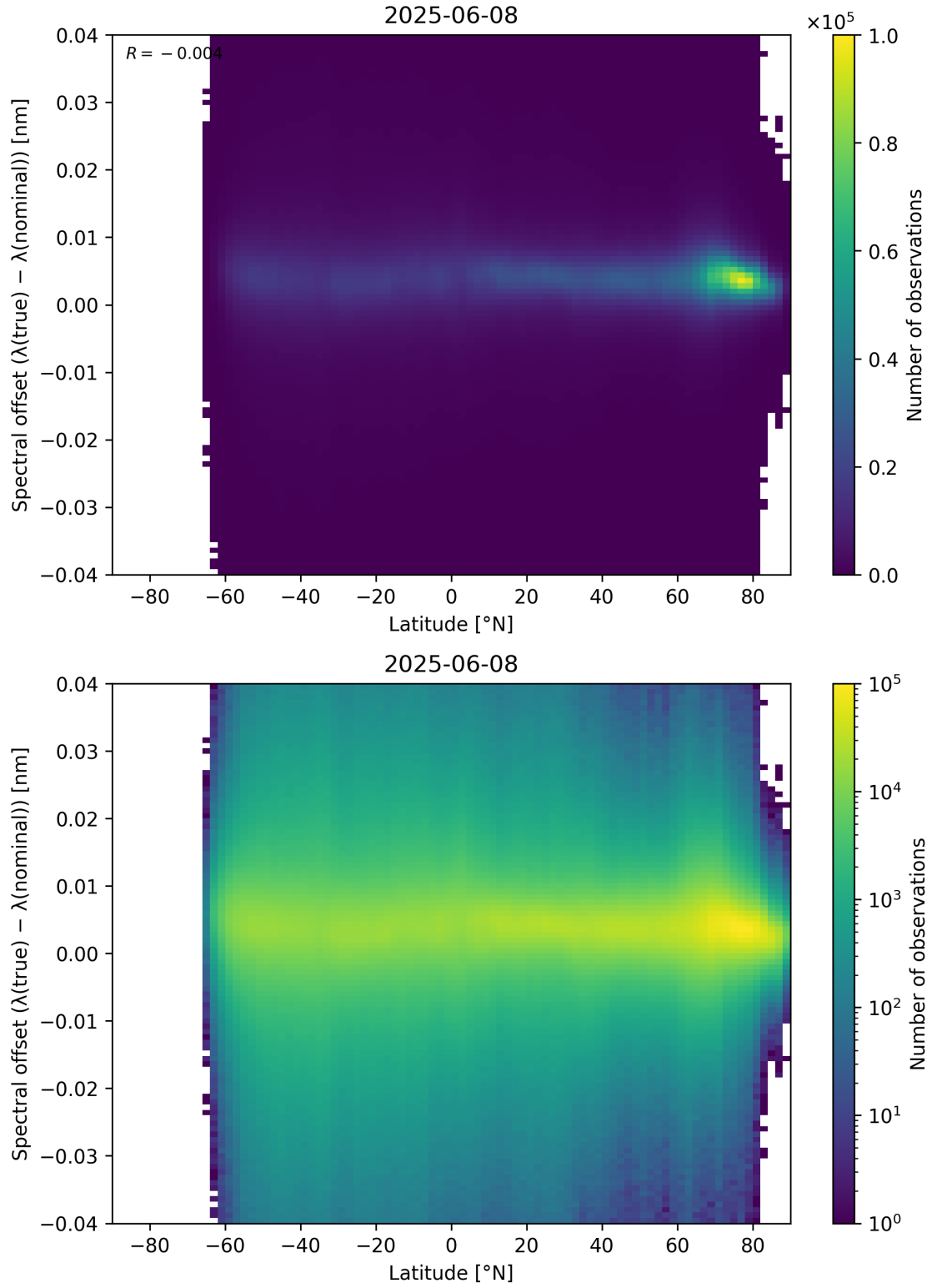
Figure 96: Scatter density plot of “Latitude” against “Spectral offset ( \lambda_{\text{true}} - \lambda_{\text{nominal}} )” for 2025-06-07 to 2025-06-09.
