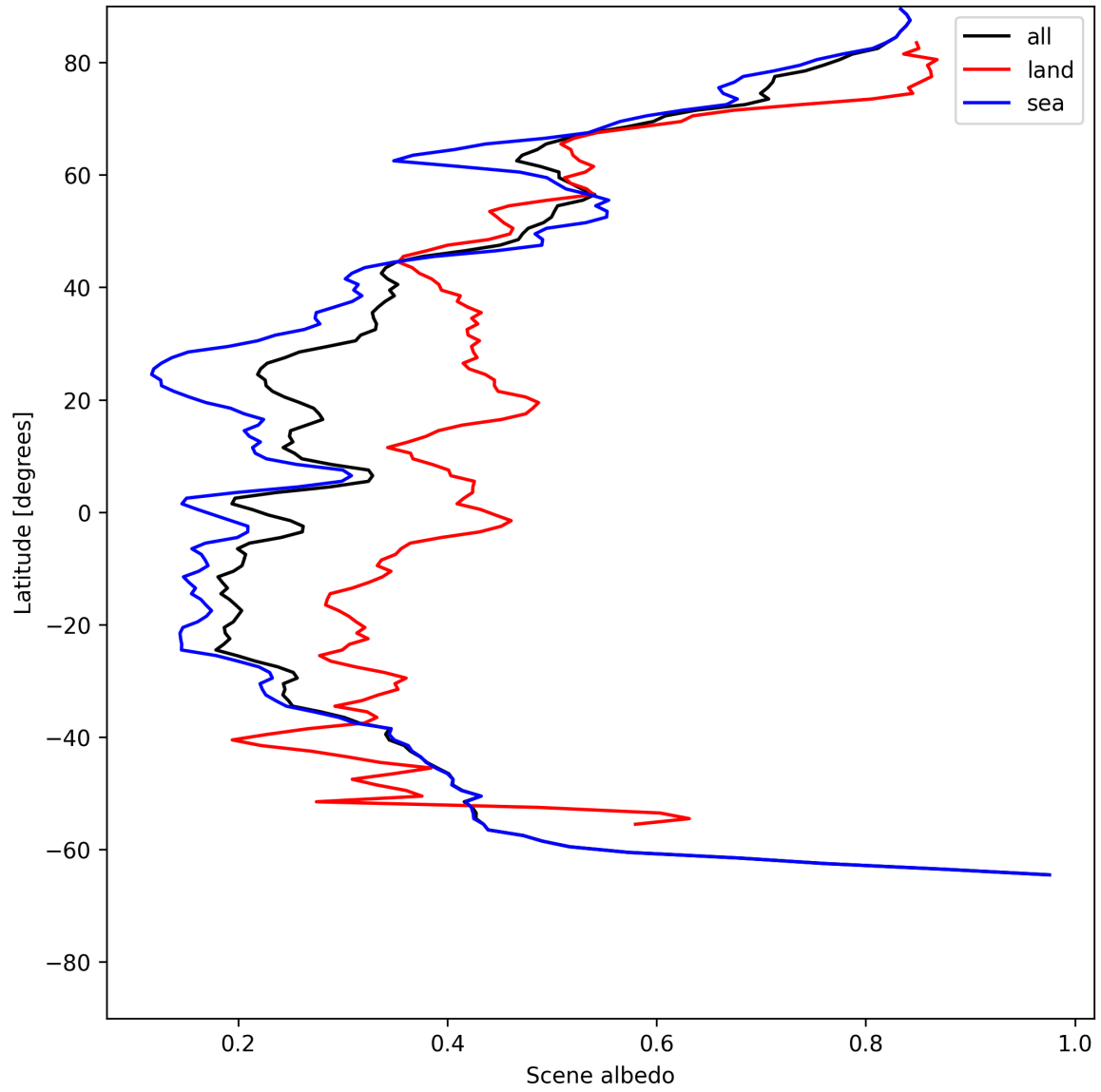
Figure 17: Zonal average of “Scene albedo” for 2025-06-07 to 2025-06-09.
