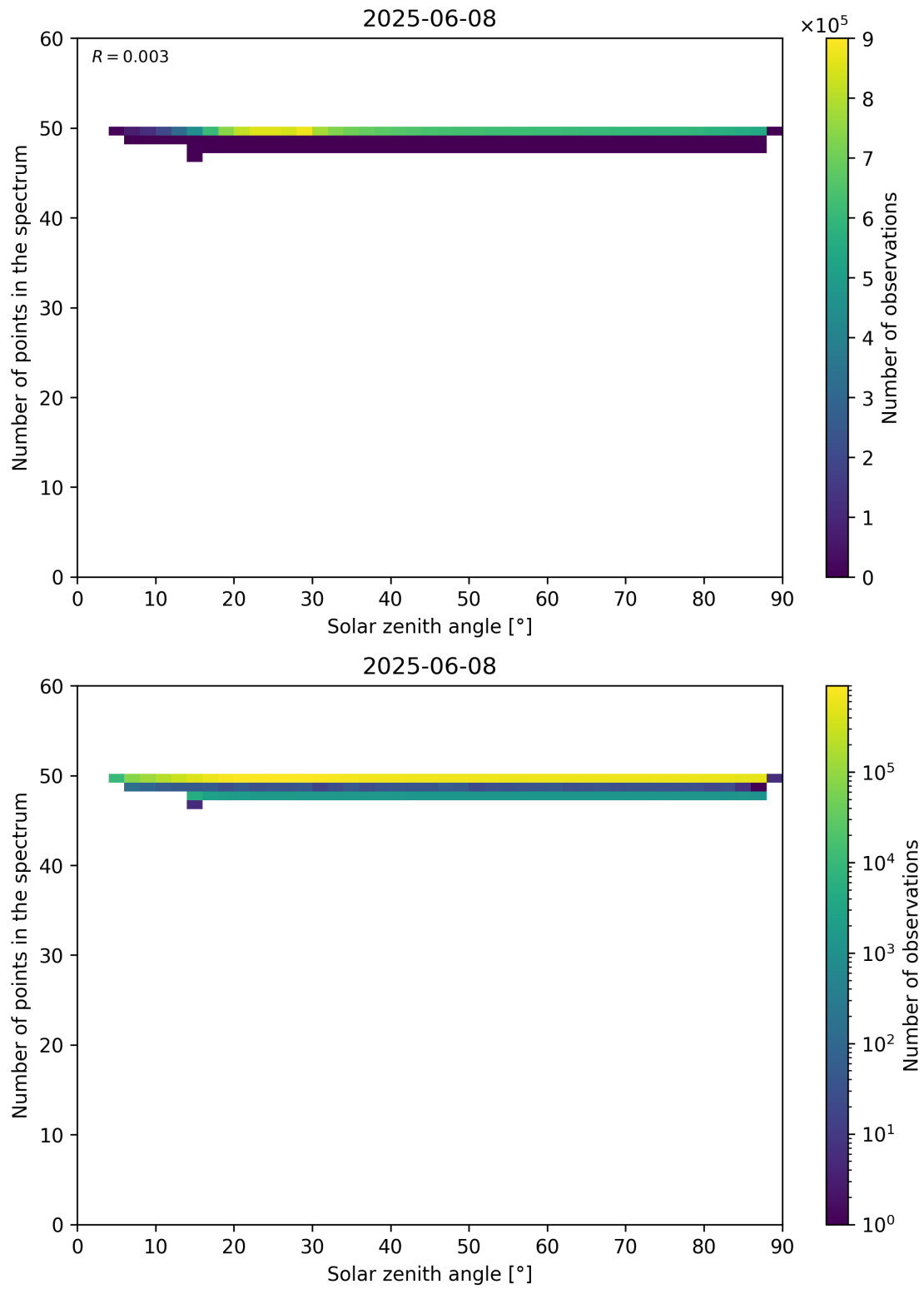
Figure 115: Scatter density plot of “Solar zenith angle” against “Number of points in the spectrum” for 2025-06-07 to 2025-06-09.
