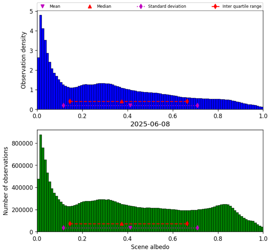
Figure 34: Histogram of “Scene albedo” for 2025-06-07 to 2025-06-09
