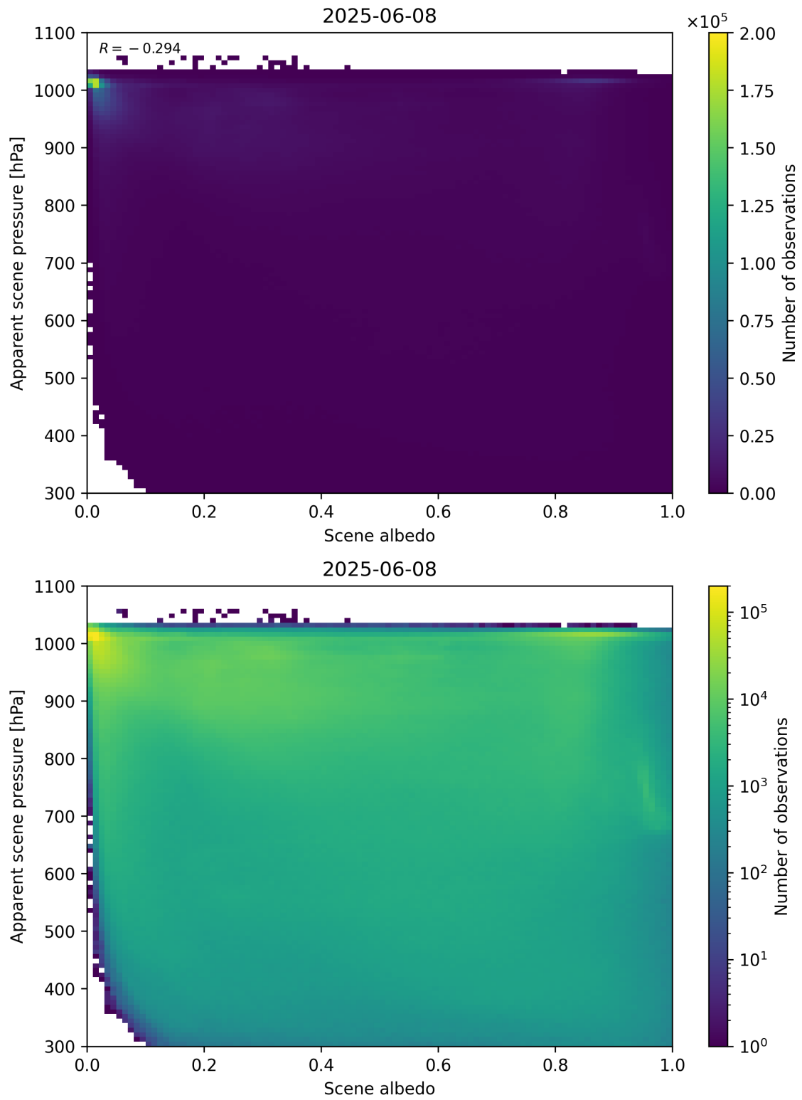
Figure 102: Scatter density plot of “Scene albedo” against “Apparent scene pressure” for 2025-06-07 to 2025-06-09.
