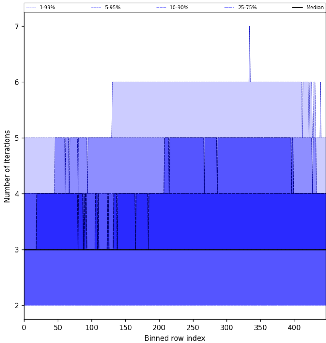
Figure 56: Along track statistics of “Number of iterations” for 2025-06-07 to 2025-06-09
