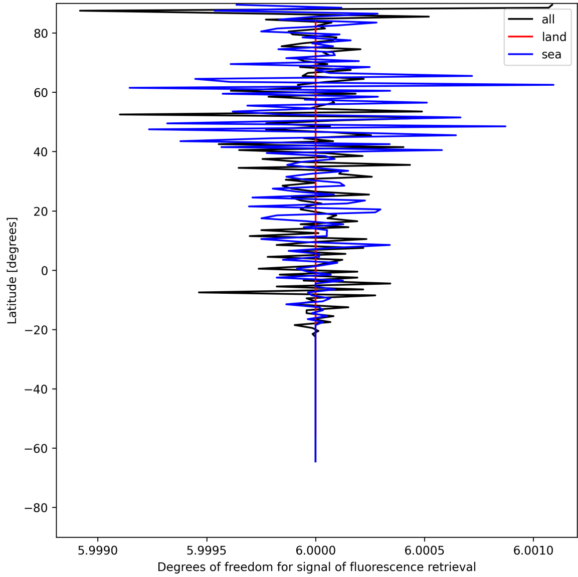
Figure 26: Zonal average of “Degrees of freedom for signal of fluorescence retrieval” for 2025-06-07 to 2025-06-09.
