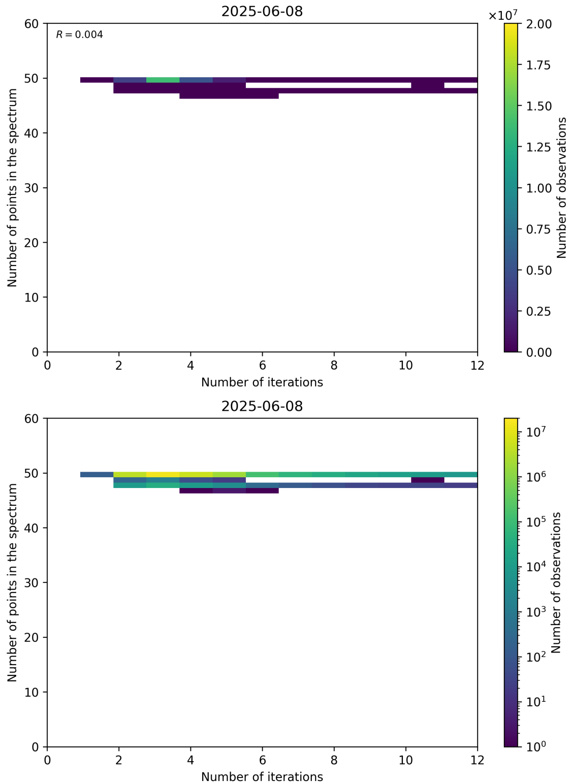
Figure 99: Scatter density plot of “Number of iterations” against “Number of points in the spectrum” for 2025-06-07 to 2025-06-09.
