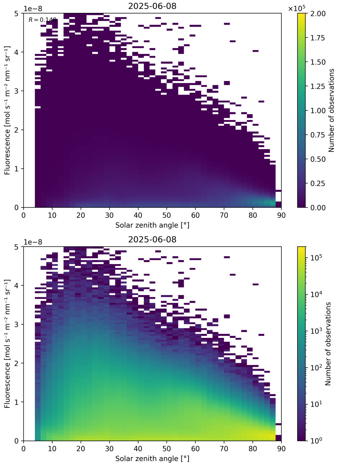
Figure 112: Scatter density plot of “Solar zenith angle” against “Fluorescence” for 2025-06-07 to 2025-06-09.
