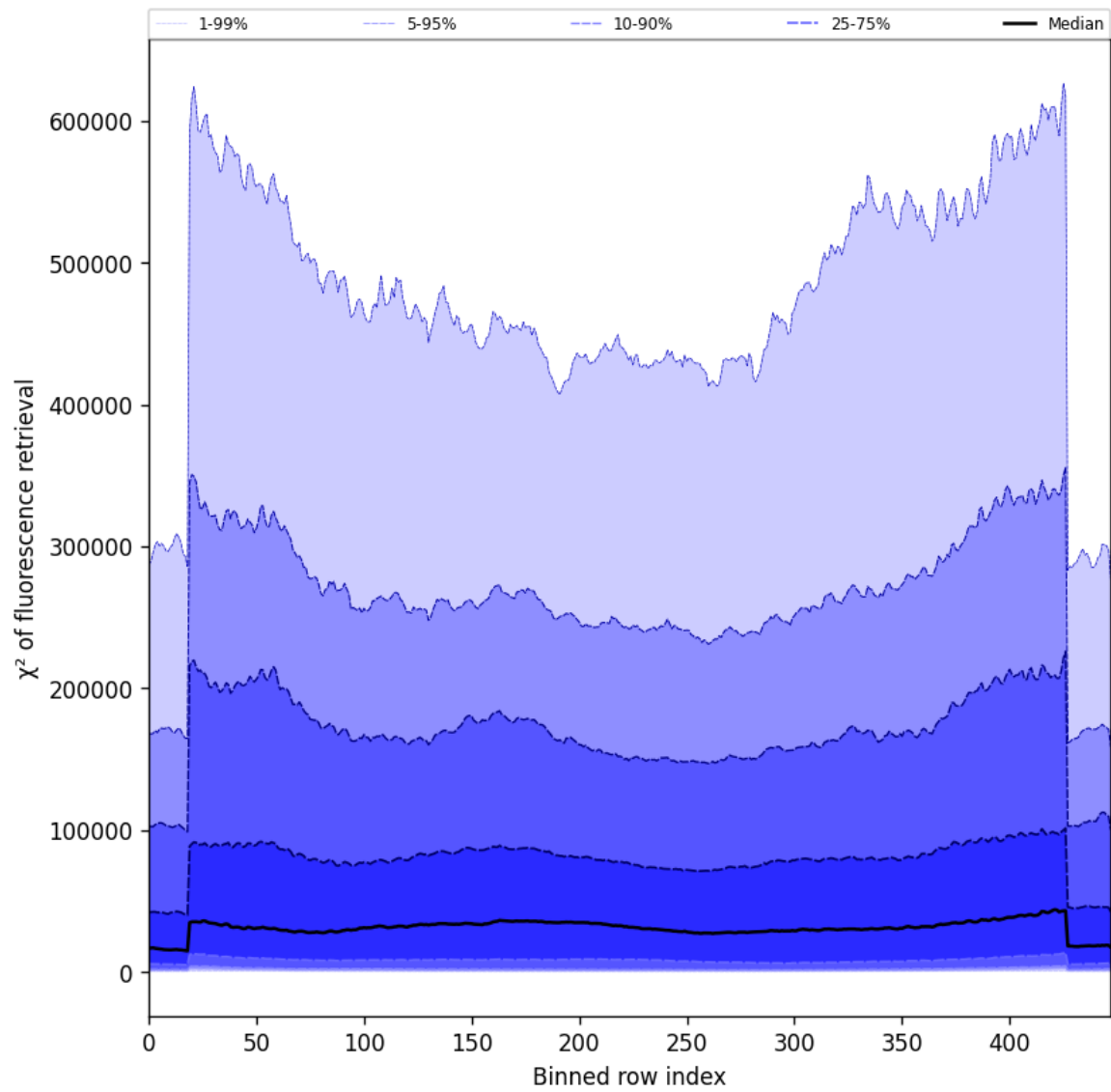
Figure 59: Along track statistics of “ \chi^2 of fluorescence retrieval” for 2025-06-07 to 2025-06-09
