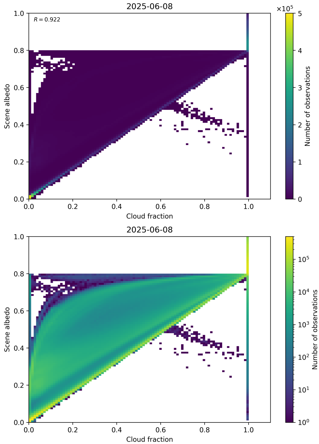
Figure 75: Scatter density plot of “Cloud fraction” against “Scene albedo” for 2025-06-07 to 2025-06-09.
