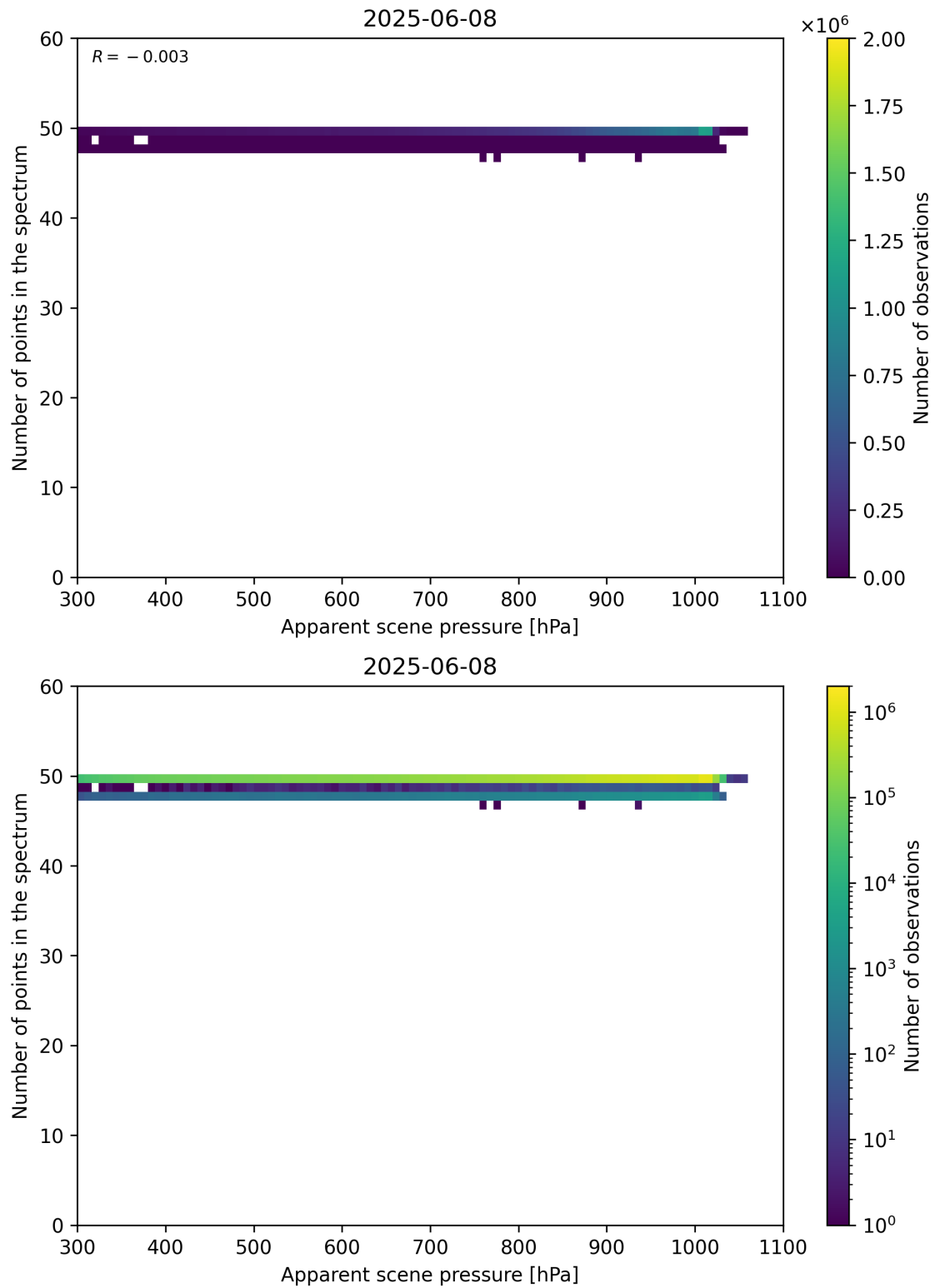
Figure 66: Scatter density plot of “Apparent scene pressure” against “Number of points in the spectrum” for 2025-06-07 to 2025-06-09.
