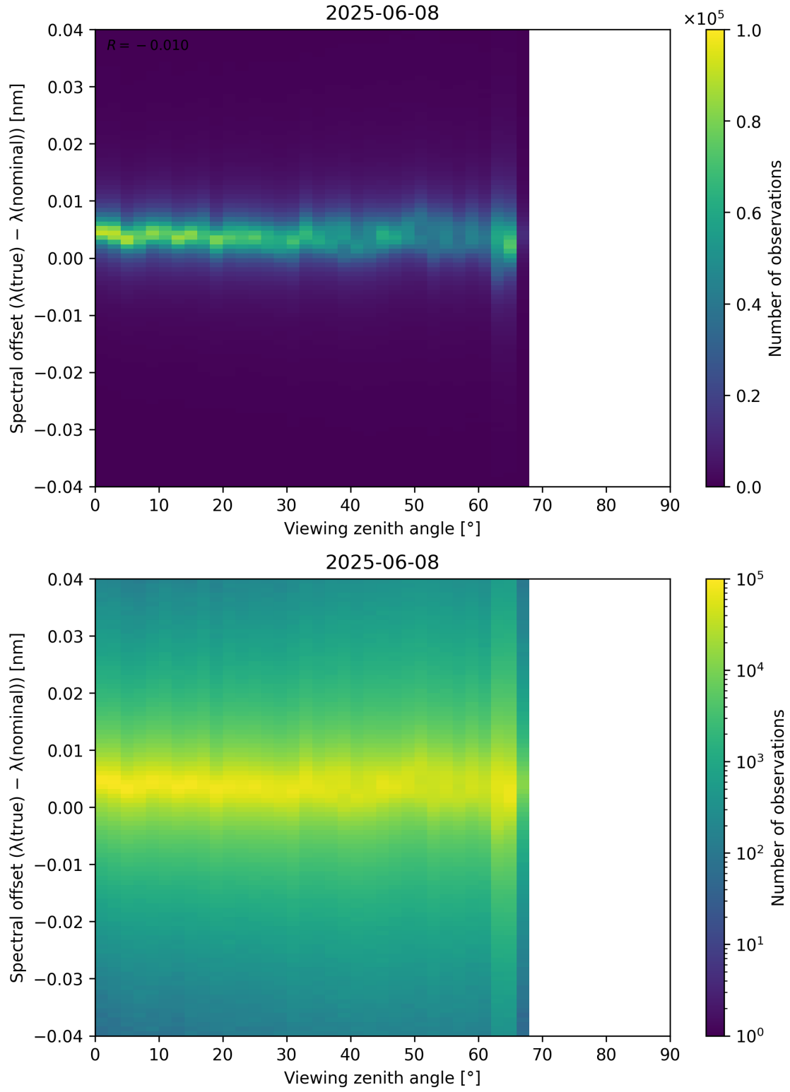
Figure 128: Scatter density plot of “Viewing zenith angle” against “Spectral offset ( \lambda_{\text{true}} - \lambda_{\text{nominal}} )” for 2025-06-07 to 2025-06-09.
