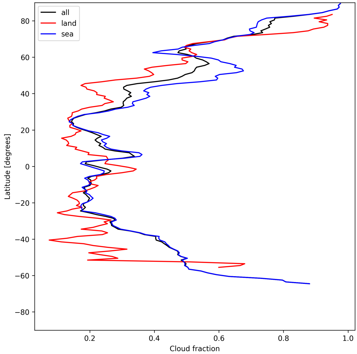
Figure 15: Zonal average of “Cloud fraction” for 2025-06-07 to 2025-06-09.
