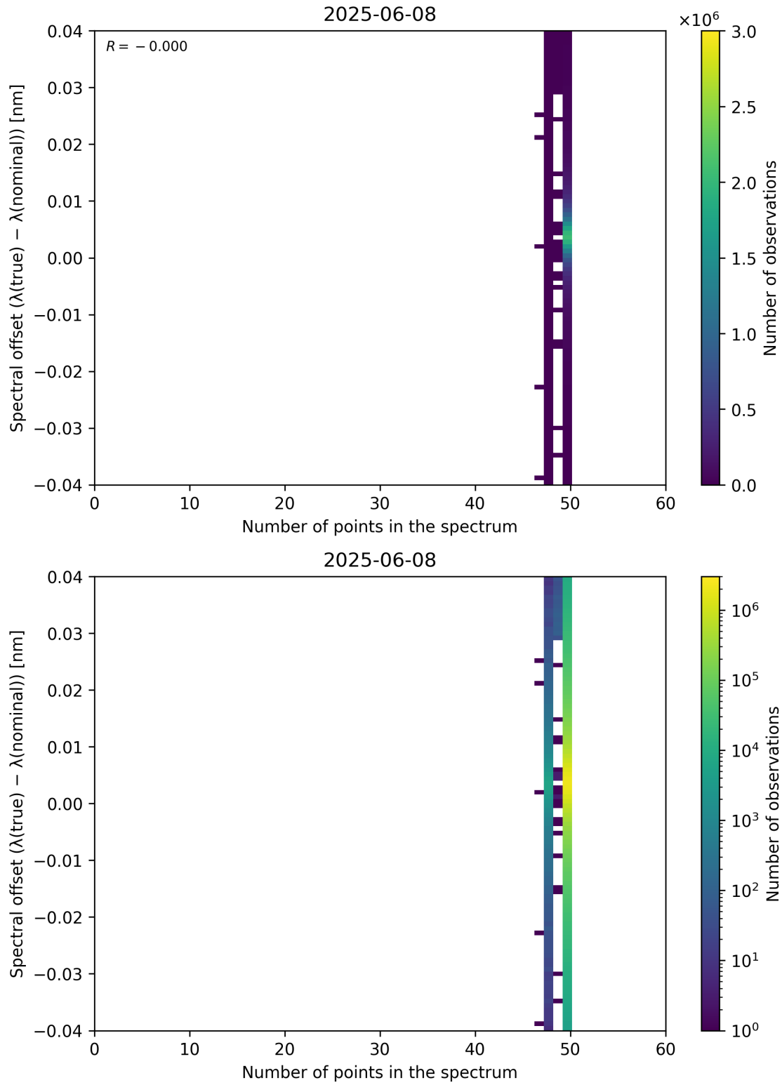
Figure 101: Scatter density plot of “Number of points in the spectrum” against “Spectral offset ( \lambda_{\text{true}} - \lambda_{\text{nominal}} )” for 2025-06-07 to 2025-06-09.
