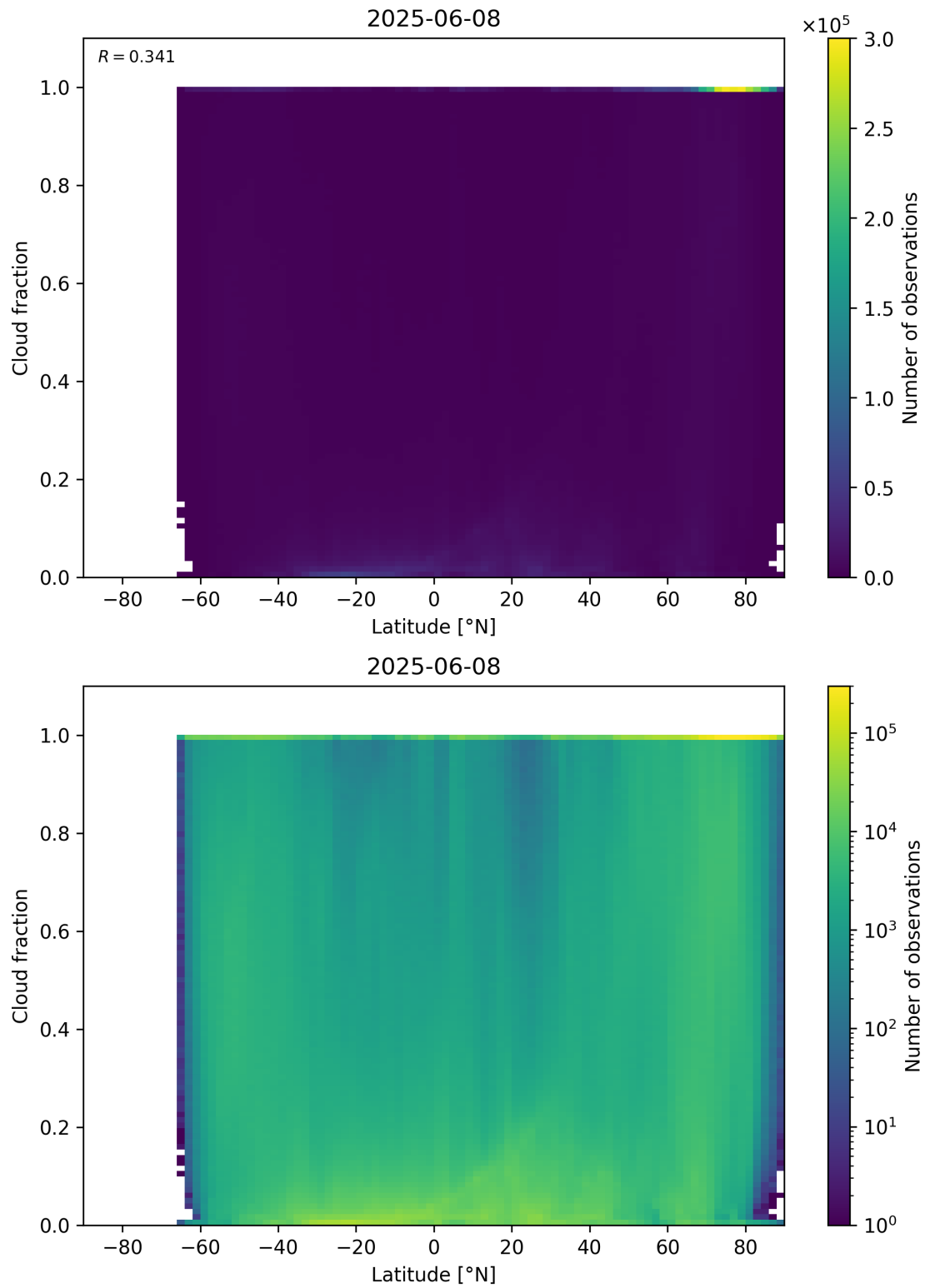
Figure 90: Scatter density plot of “Latitude” against “Cloud fraction” for 2025-06-07 to 2025-06-09.
