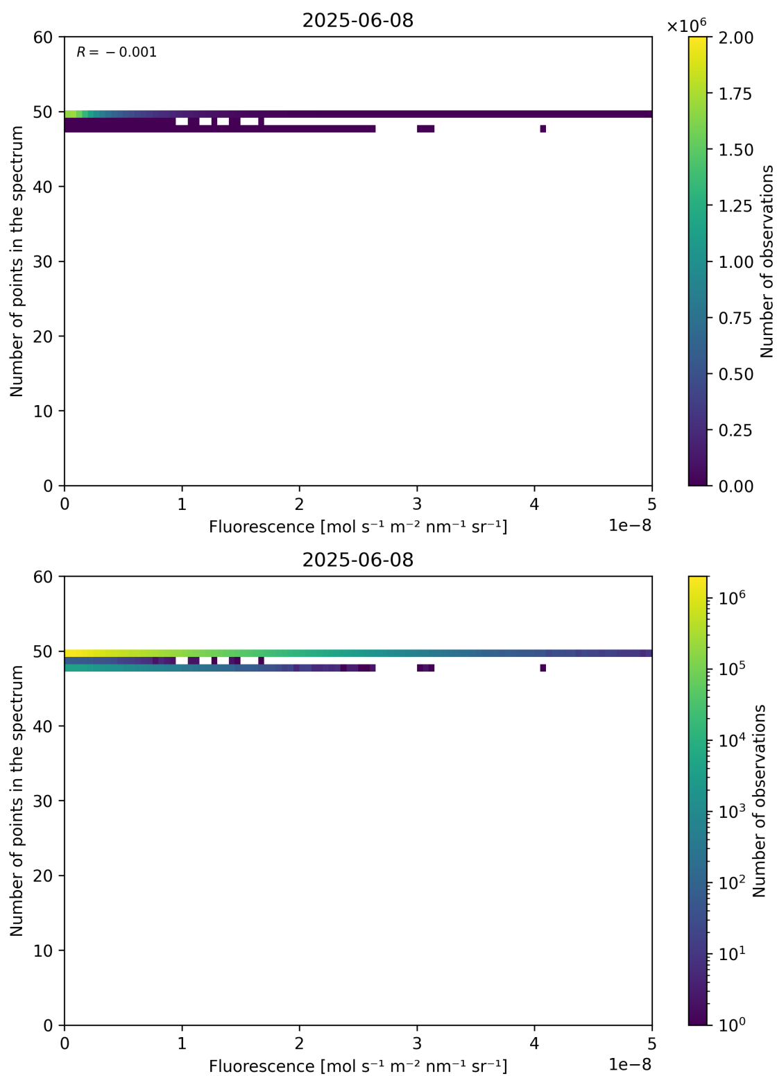
Figure 86: Scatter density plot of “Fluorescence” against “Number of points in the spectrum” for 2025-06-07 to 2025-06-09.
