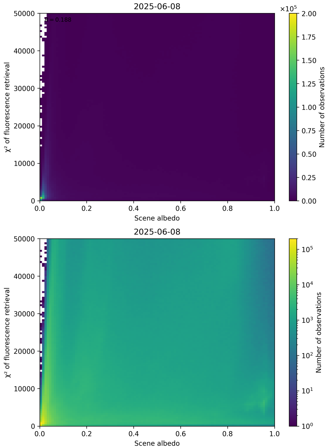
Figure 103: Scatter density plot of “Scene albedo” against “ \chi^2 of fluorescence retrieval” for 2025-06-07 to 2025-06-09.
