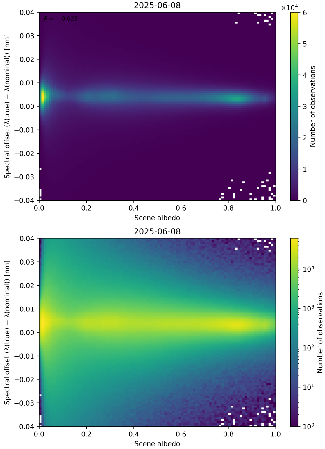
Figure 107: Scatter density plot of “Scene albedo” against “Spectral offset ( \lambda_{\text{true}} - \lambda_{\text{nominal}} )” for 2025-06-07 to 2025-06-09.
