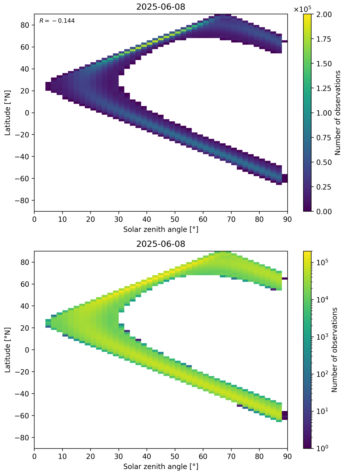
Figure 113: Scatter density plot of “Solar zenith angle” against “Latitude” for 2025-06-07 to 2025-06-09.
