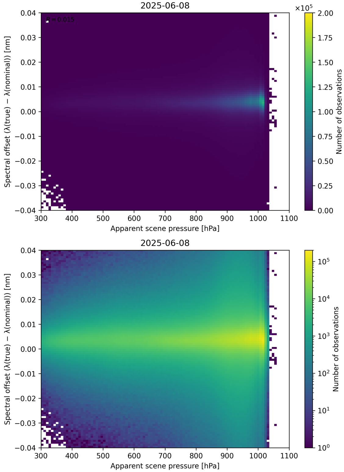
Figure 67: Scatter density plot of “Apparent scene pressure” against “Spectral offset ( \lambda_{\text{true}} - \lambda_{\text{nominal}} )” for 2025-06-07 to 2025-06-09.
