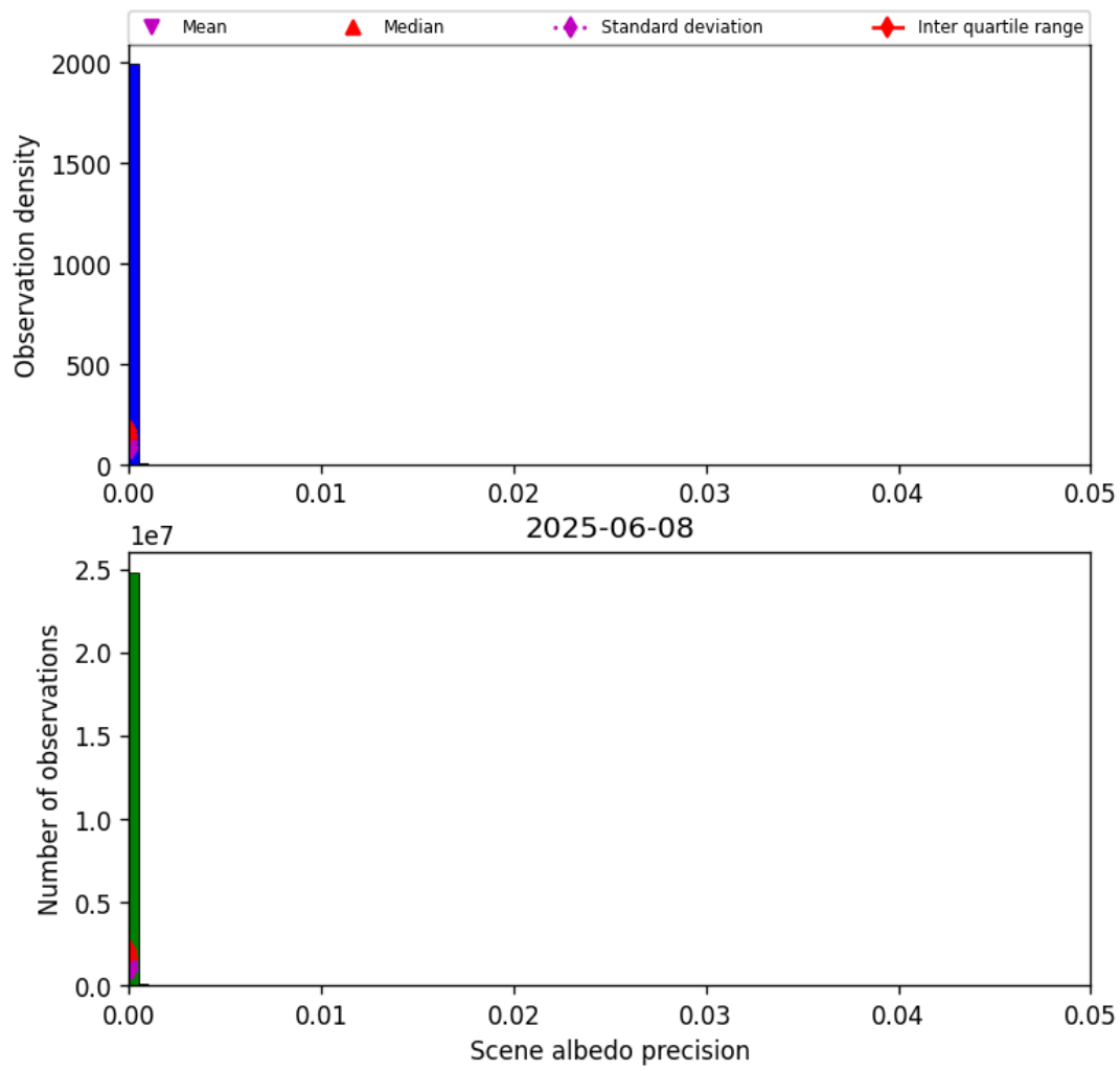
Figure 35: Histogram of “Scene albedo precision” for 2025-06-07 to 2025-06-09
