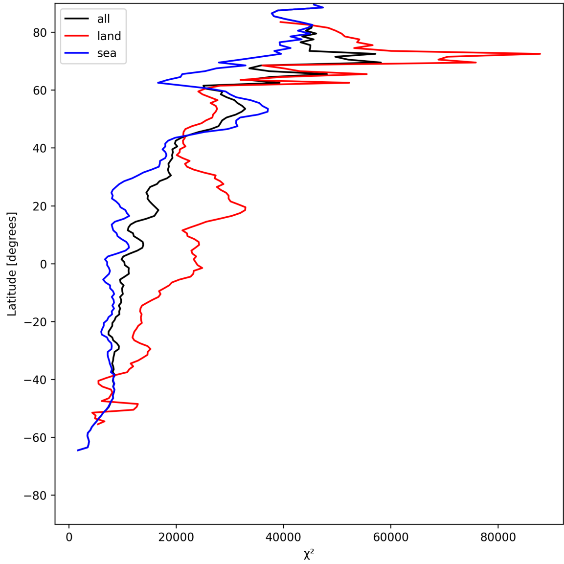
Figure 21: Zonal average of “ \chi^2 ” for 2025-06-07 to 2025-06-09.
