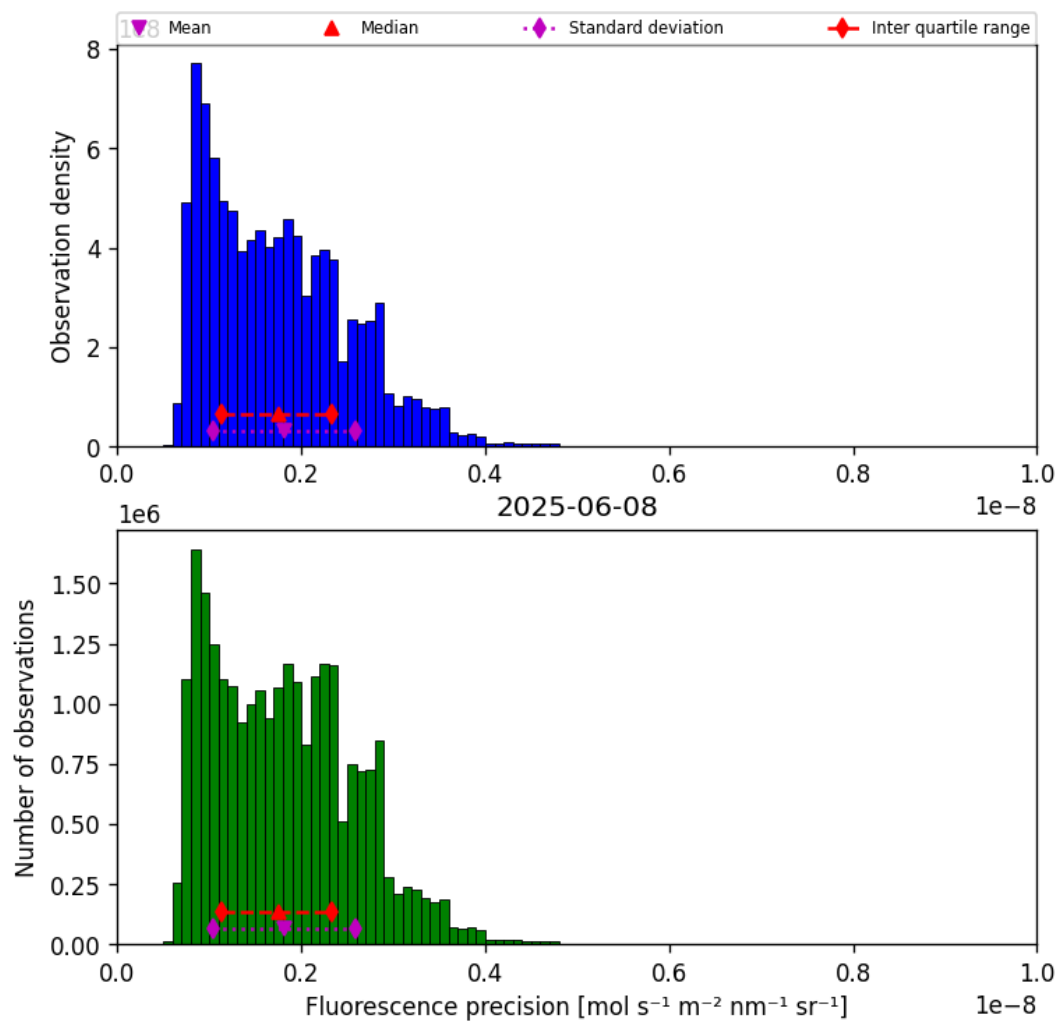
Figure 41: Histogram of “Fluorescence precision” for 2025-06-07 to 2025-06-09
