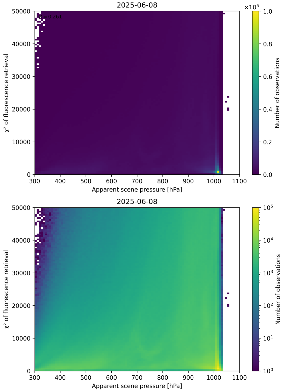
Figure 63: Scatter density plot of “Apparent scene pressure” against “ \chi^2 of fluorescence retrieval” for 2025-06-07 to 2025-06-09.
