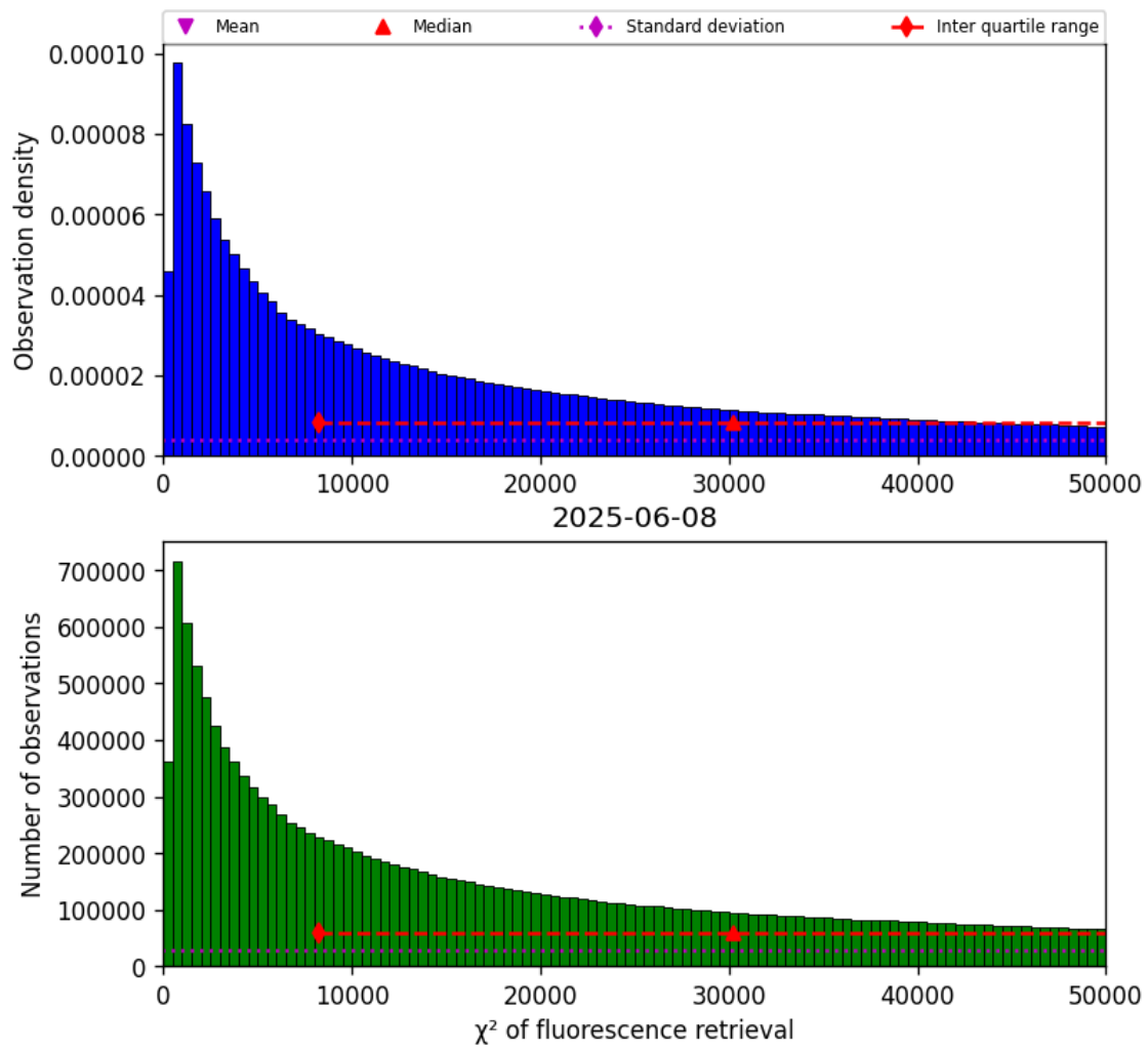
Figure 42: Histogram of “ \chi^2 of fluorescence retrieval” for 2025-06-07 to 2025-06-09
