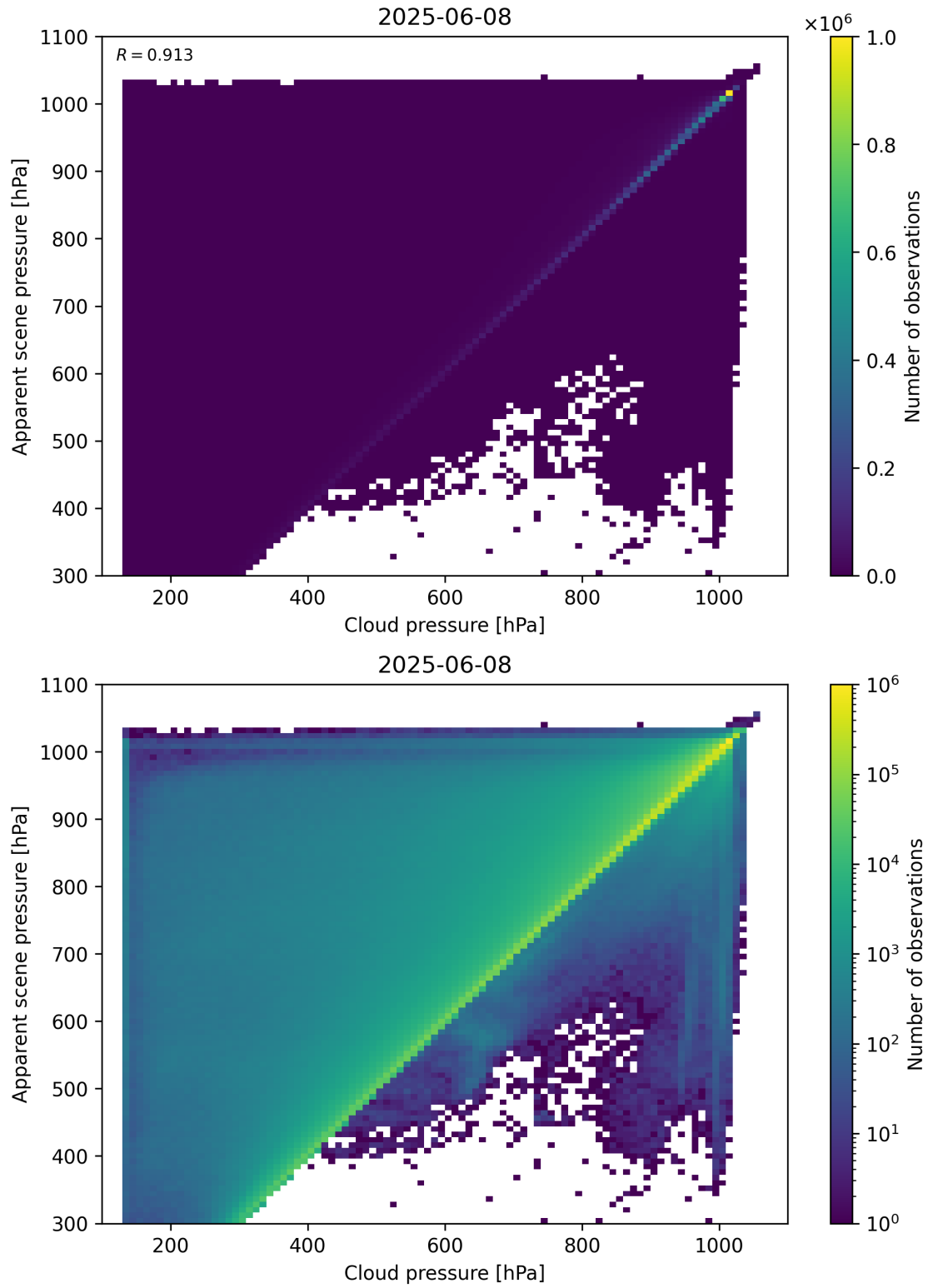
Figure 77: Scatter density plot of “Cloud pressure” against “Apparent scene pressure” for 2025-06-07 to 2025-06-09.
