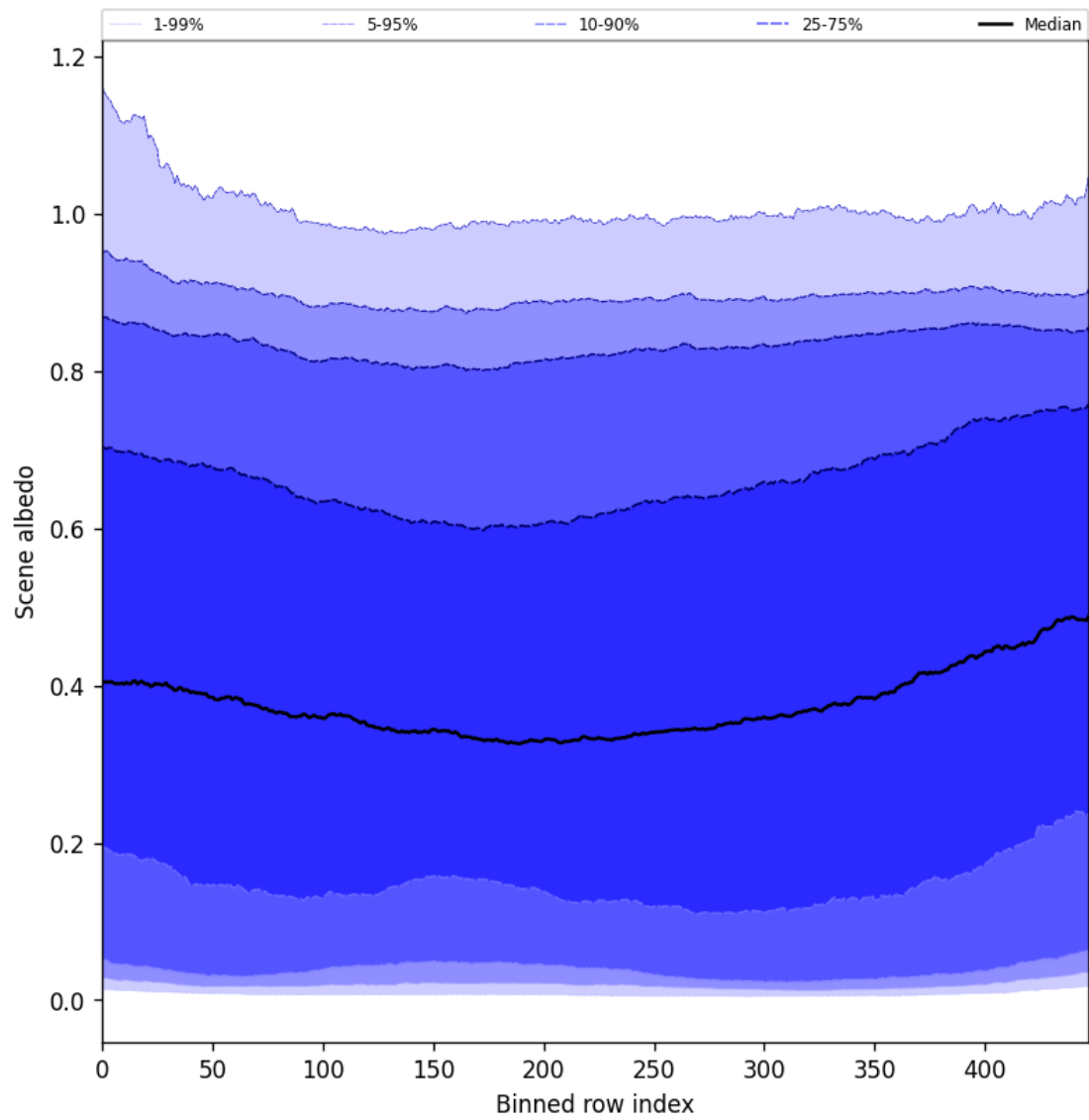
Figure 51: Along track statistics of “Scene albedo” for 2025-06-07 to 2025-06-09
