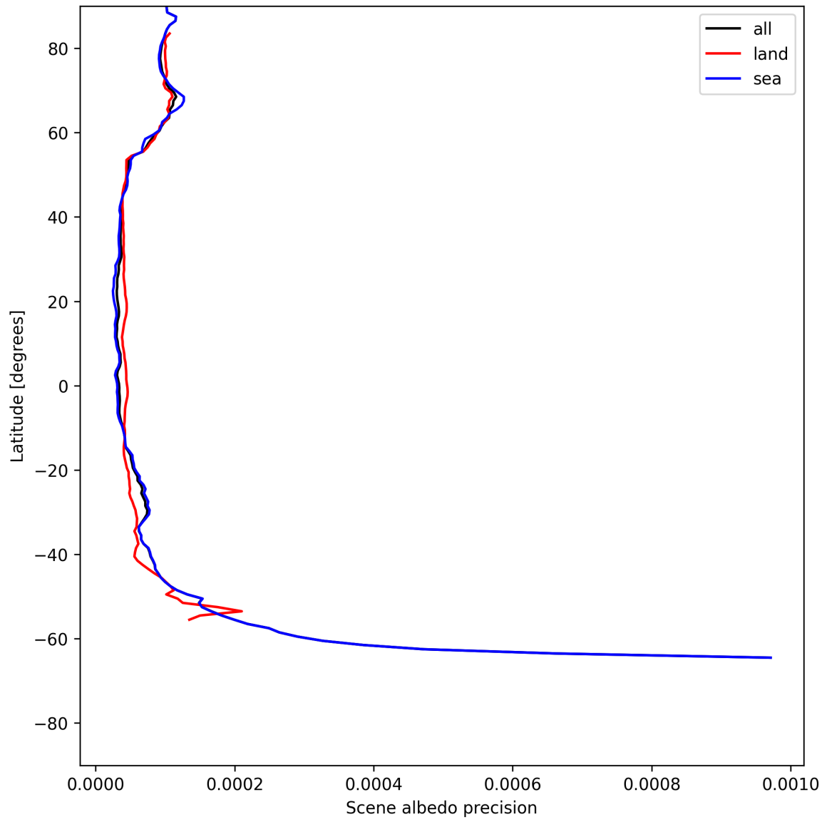
Figure 18: Zonal average of “Scene albedo precision” for 2025-06-07 to 2025-06-09.
