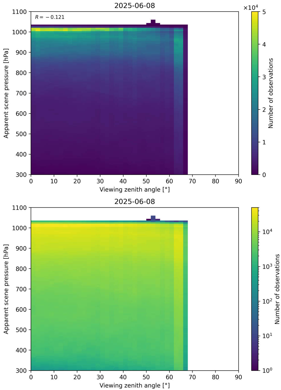
Figure 118: Scatter density plot of “Viewing zenith angle” against “Apparent scene pressure” for 2025-06-07 to 2025-06-09.
