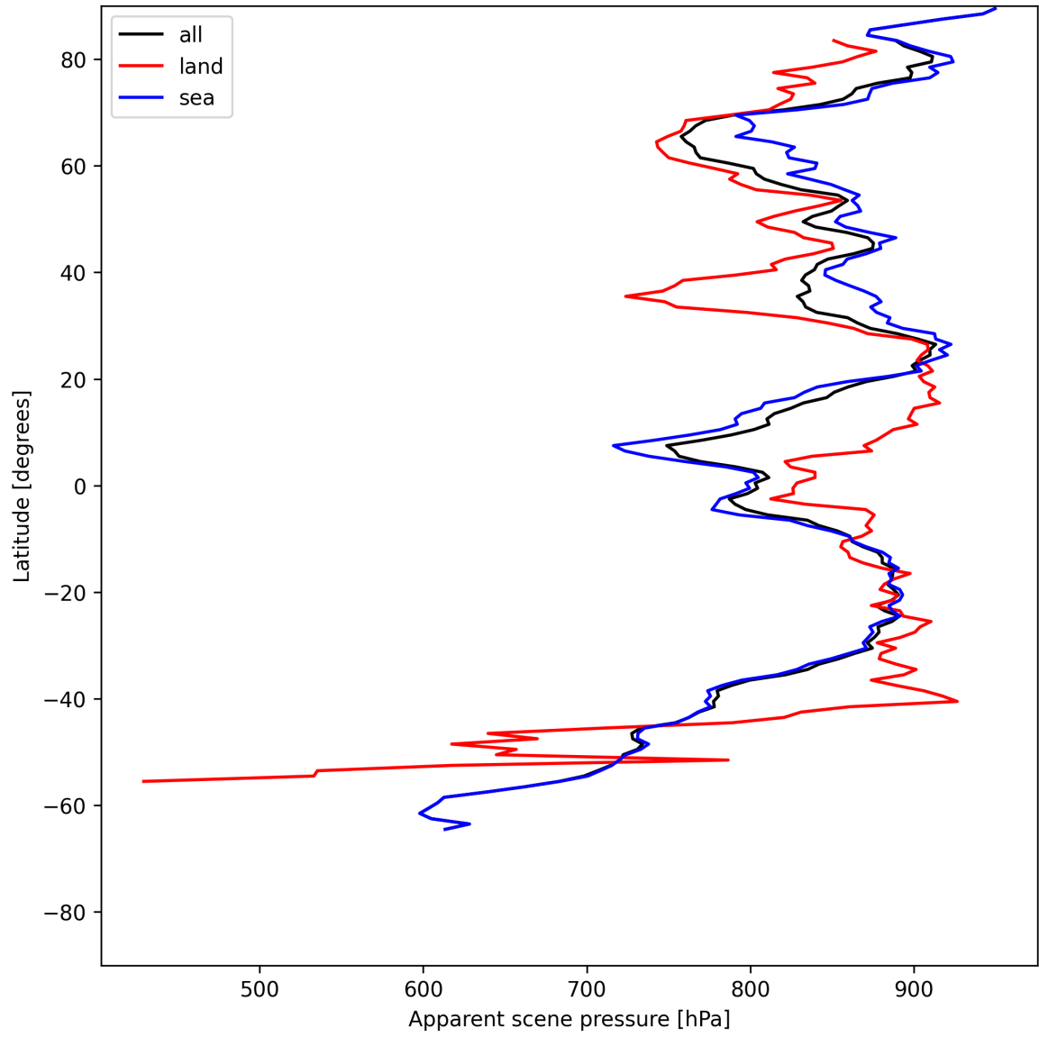
Figure 19: Zonal average of “Apparent scene pressure” for 2025-06-07 to 2025-06-09.
