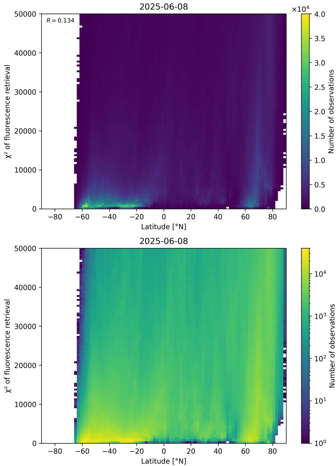
Figure 89: Scatter density plot of “Latitude” against “ \chi^2 of fluorescence retrieval” for 2025-06-07 to 2025-06-09.
