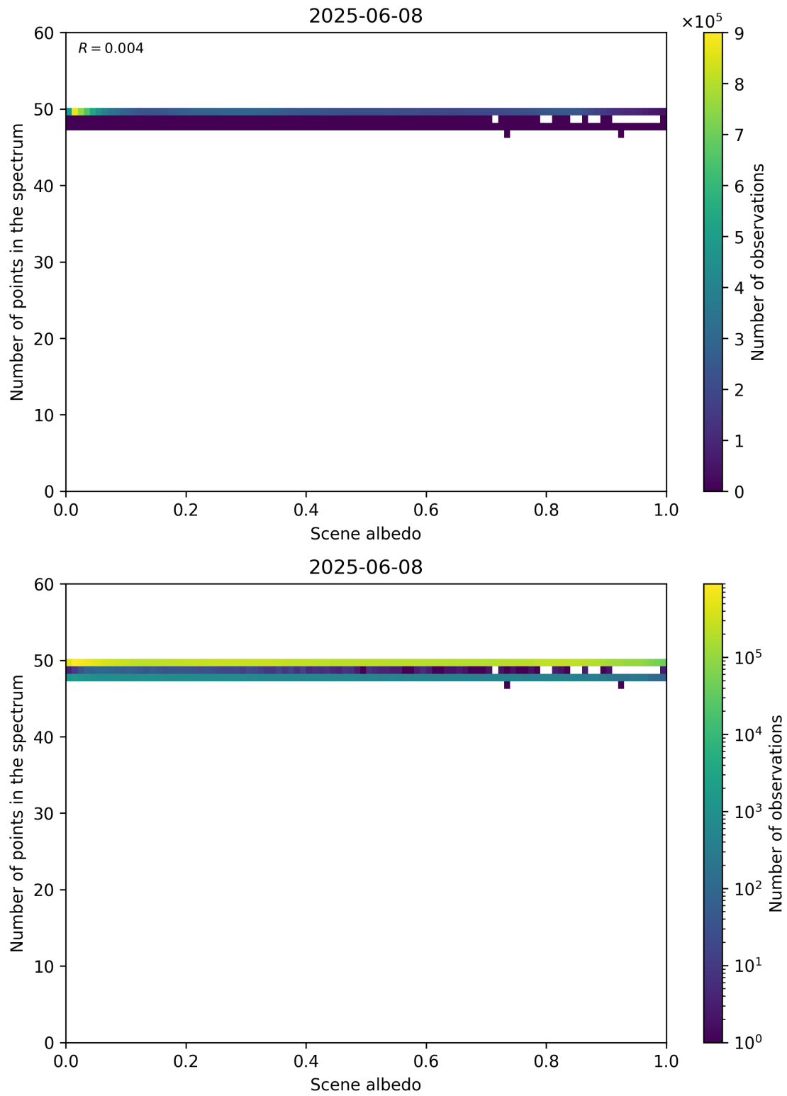
Figure 106: Scatter density plot of “Scene albedo” against “Number of points in the spectrum” for 2025-06-07 to 2025-06-09.
