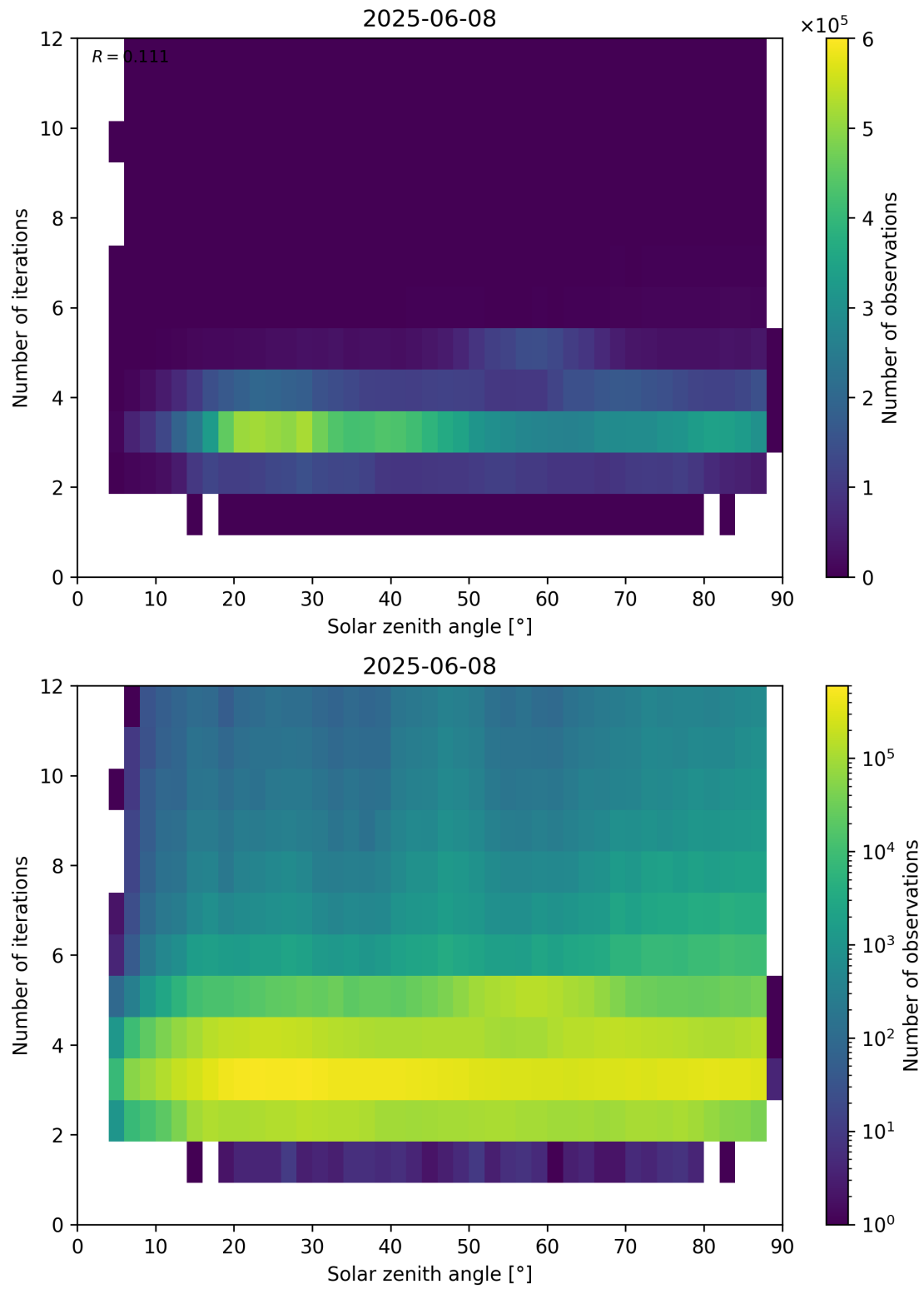
Figure 114: Scatter density plot of “Solar zenith angle” against “Number of iterations” for 2025-06-07 to 2025-06-09.
