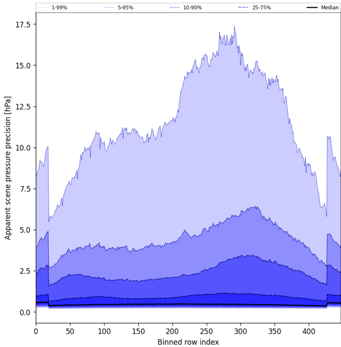
Figure 54: Along track statistics of “Apparent scene pressure precision” for 2025-06-07 to 2025-06-09
