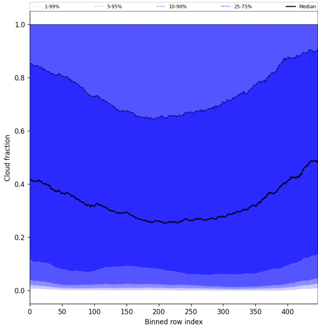
Figure 49: Along track statistics of “Cloud fraction” for 2025-06-07 to 2025-06-09
