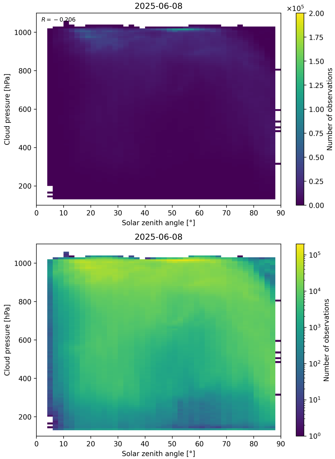
Figure 111: Scatter density plot of “Solar zenith angle” against “Cloud pressure” for 2025-06-07 to 2025-06-09.
