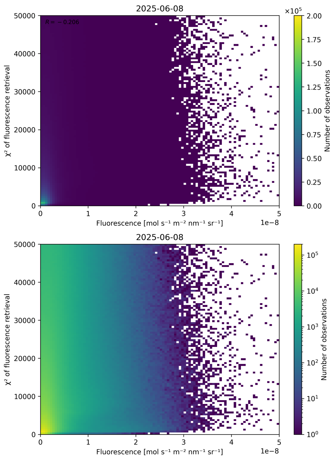
Figure 85: Scatter density plot of “Fluorescence” against “ \chi^2 of fluorescence retrieval” for 2025-06-07 to 2025-06-09.
