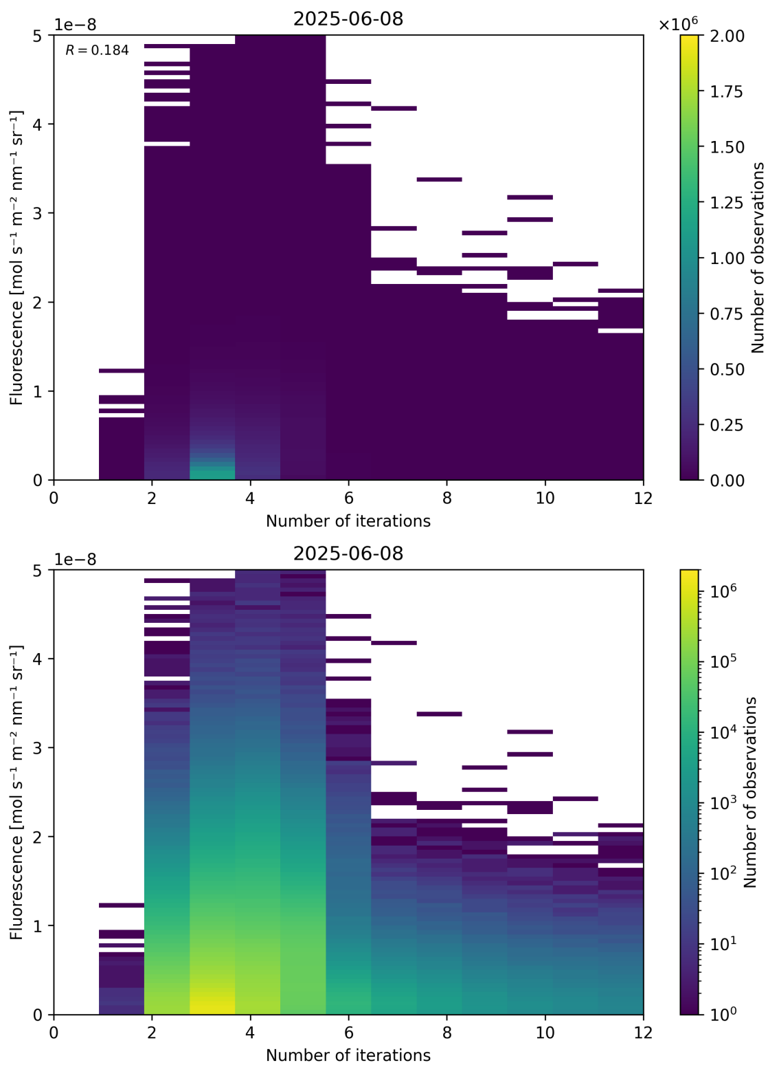
Figure 98: Scatter density plot of “Number of iterations” against “Fluorescence” for 2025-06-07 to 2025-06-09.
