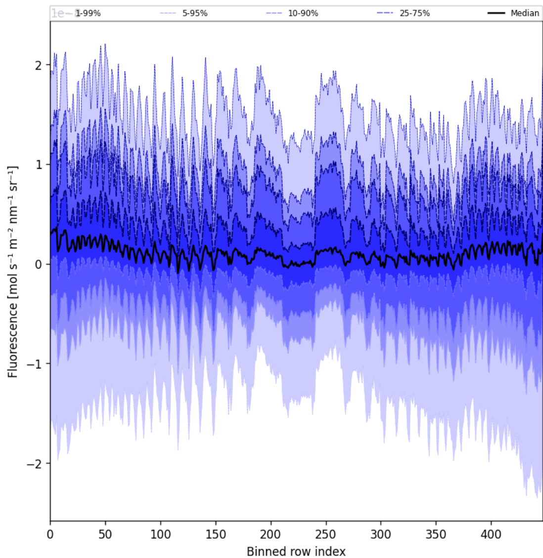
Figure 57: Along track statistics of “Fluorescence” for 2025-06-07 to 2025-06-09
