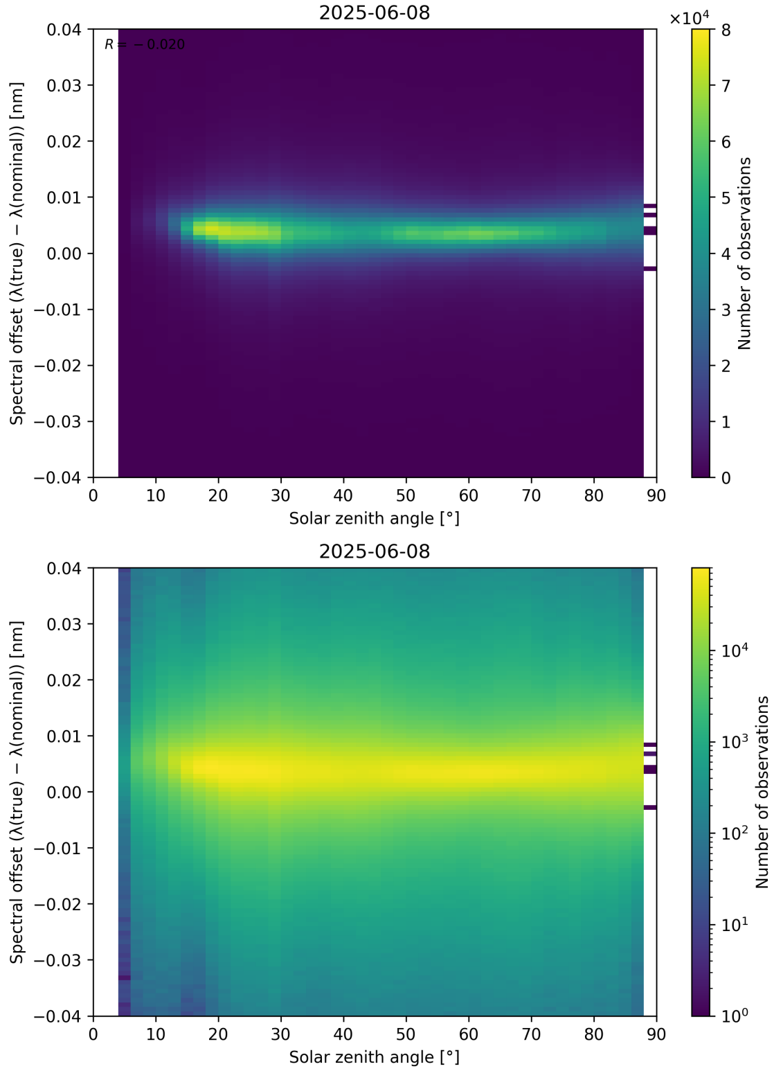
Figure 117: Scatter density plot of “Solar zenith angle” against “Spectral offset ( \lambda_{\text{true}} - \lambda_{\text{nominal}} )” for 2025-06-07 to 2025-06-09.
