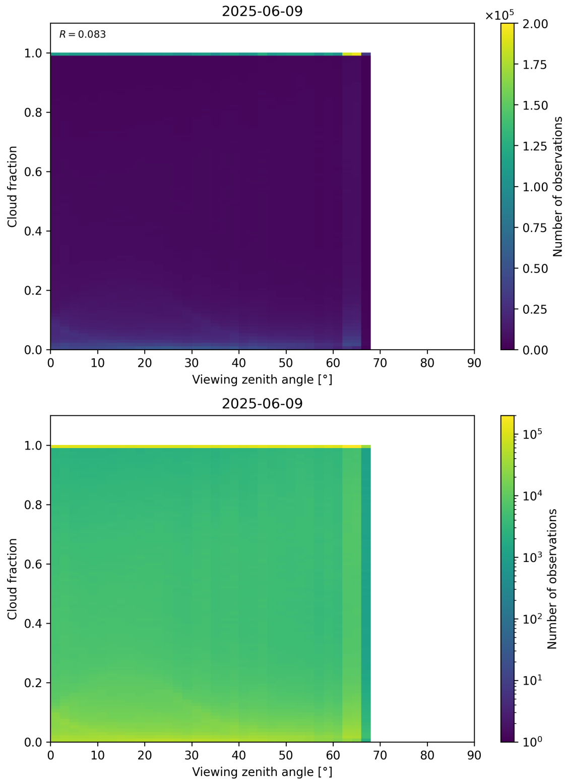
Figure 120: Scatter density plot of “Viewing zenith angle” against “Cloud fraction” for 2025-06-08 to 2025-06-10.
