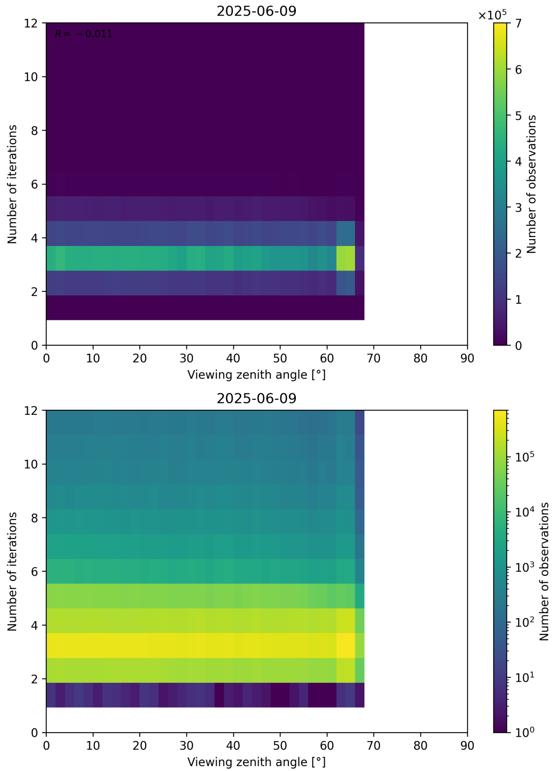
Figure 124: Scatter density plot of “Viewing zenith angle” against “Number of iterations” for 2025-06-08 to 2025-06-10.
