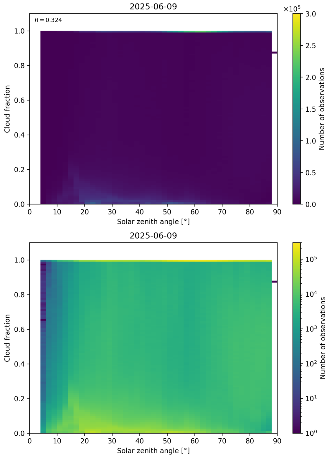
Figure 110: Scatter density plot of “Solar zenith angle” against “Cloud fraction” for 2025-06-08 to 2025-06-10.
