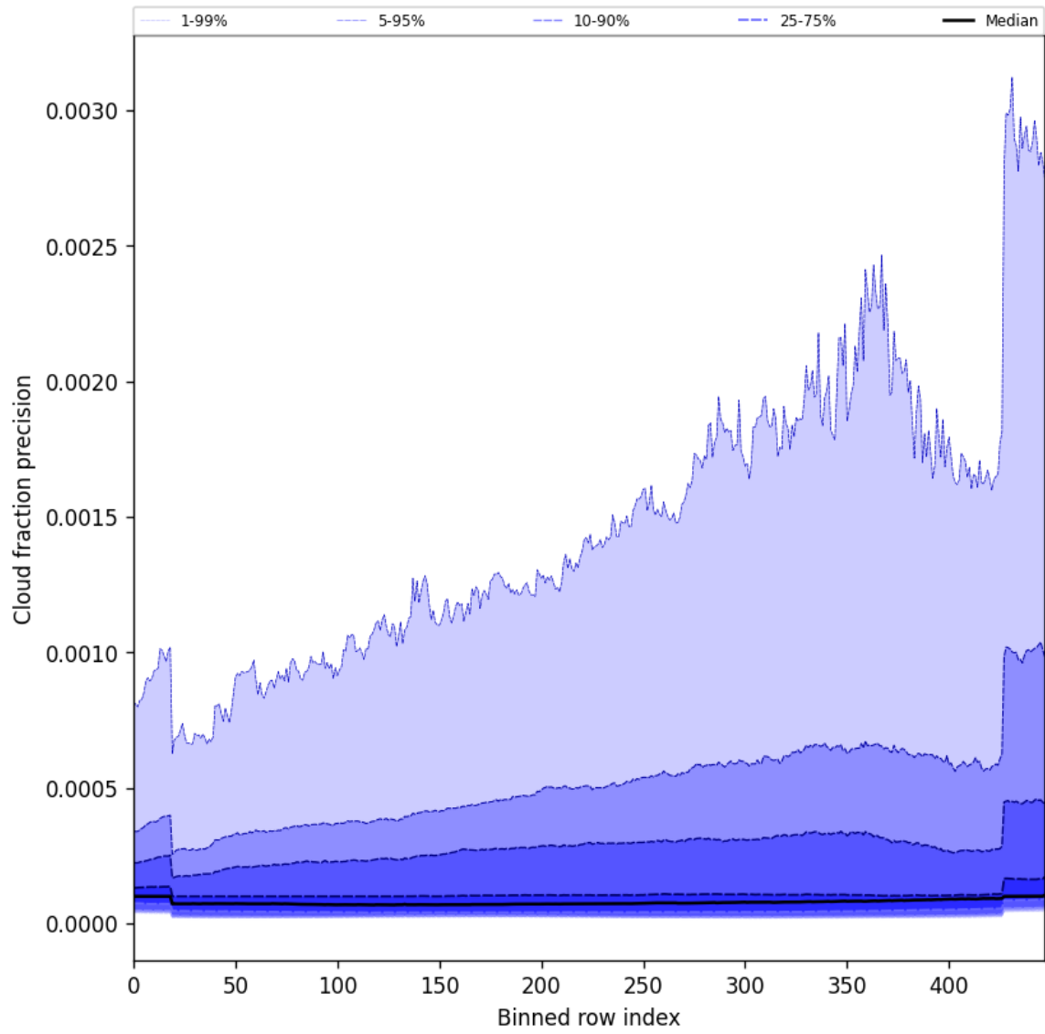
Figure 50: Along track statistics of “Cloud fraction precision” for 2025-06-08 to 2025-06-10
