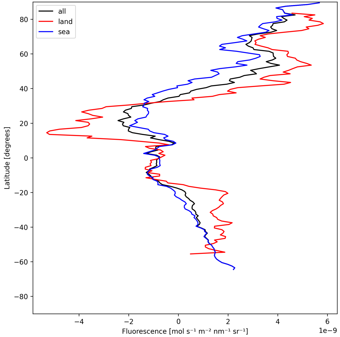
Figure 23: Zonal average of “Fluorescence” for 2025-06-08 to 2025-06-10.
