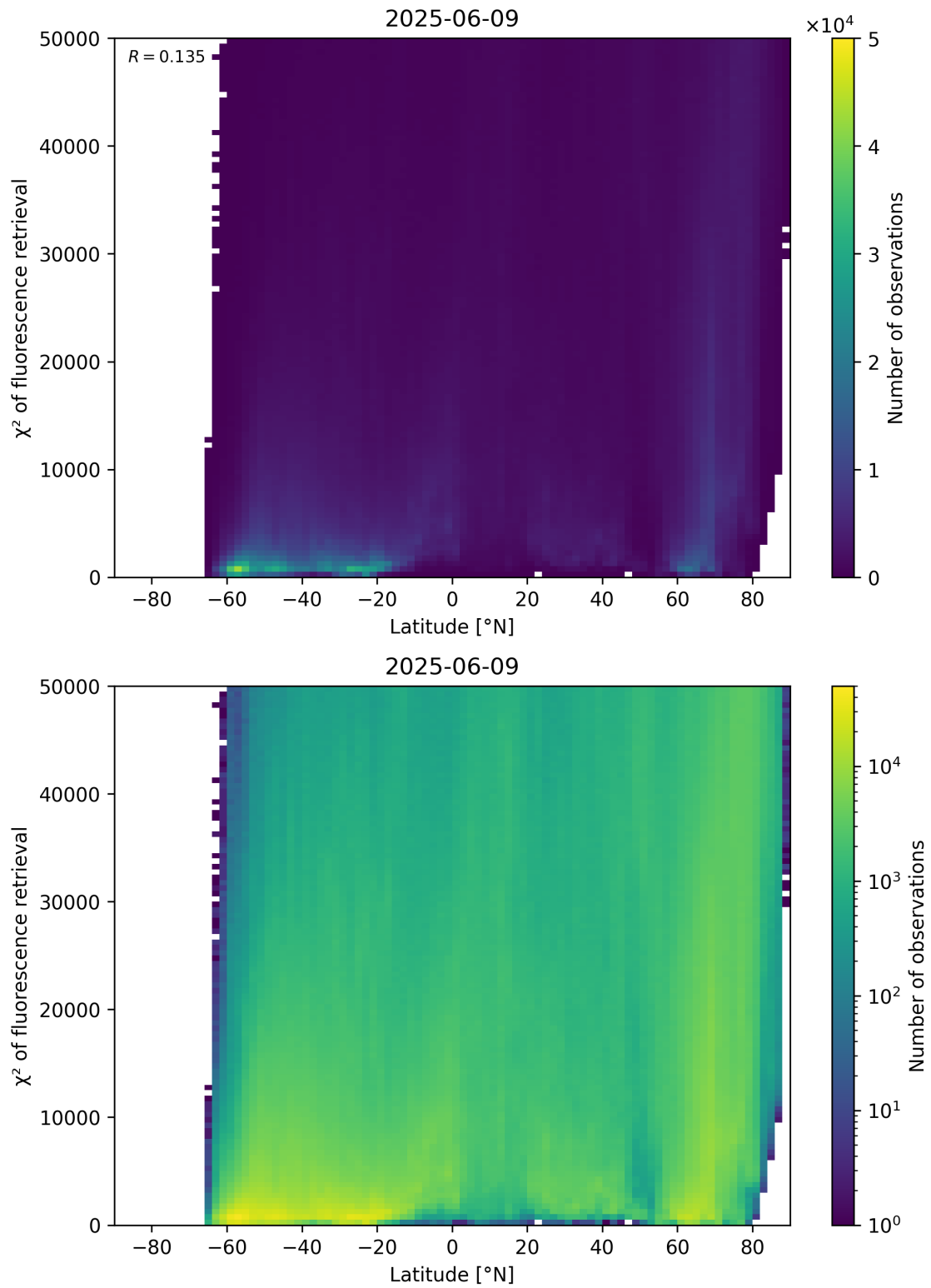
Figure 89: Scatter density plot of “Latitude” against “ \chi^2 of fluorescence retrieval” for 2025-06-08 to 2025-06-10.
