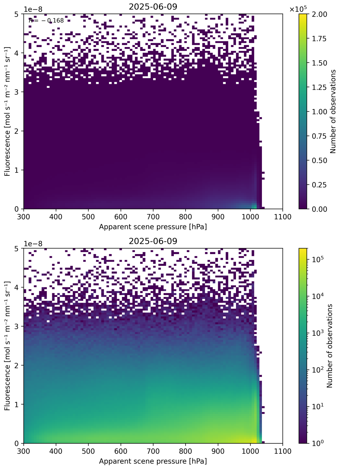
Figure 64: Scatter density plot of “Apparent scene pressure” against “Fluorescence” for 2025-06-08 to 2025-06-10.
