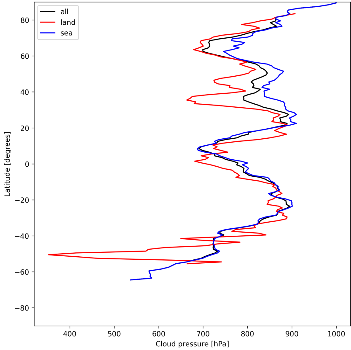
Figure 13: Zonal average of “Cloud pressure” for 2025-06-08 to 2025-06-10.
