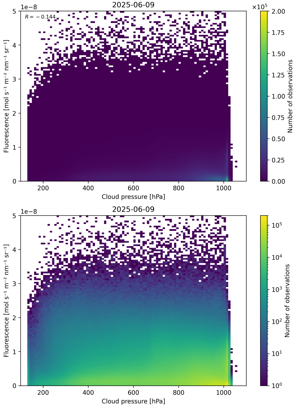
Figure 80: Scatter density plot of “Cloud pressure” against “Fluorescence” for 2025-06-08 to 2025-06-10.
