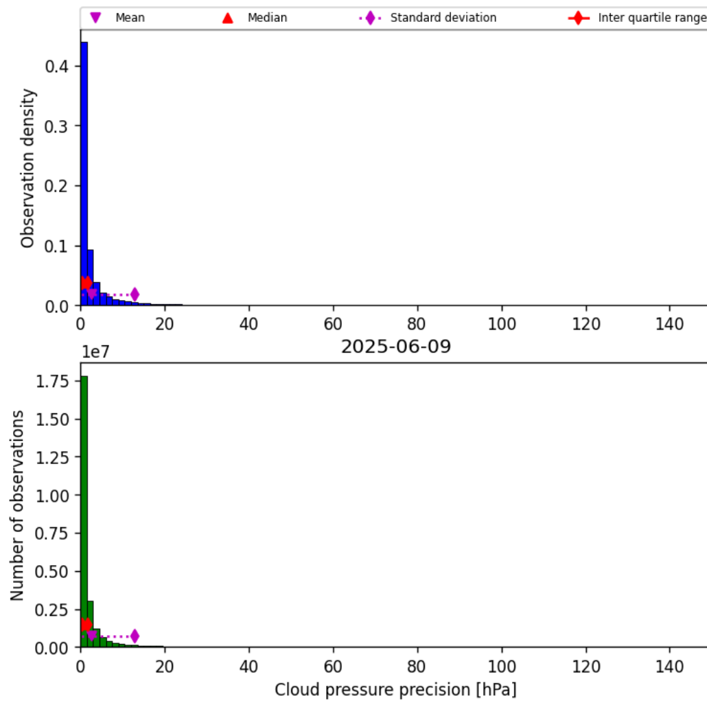
Figure 31: Histogram of “Cloud pressure precision” for 2025-06-08 to 2025-06-10
