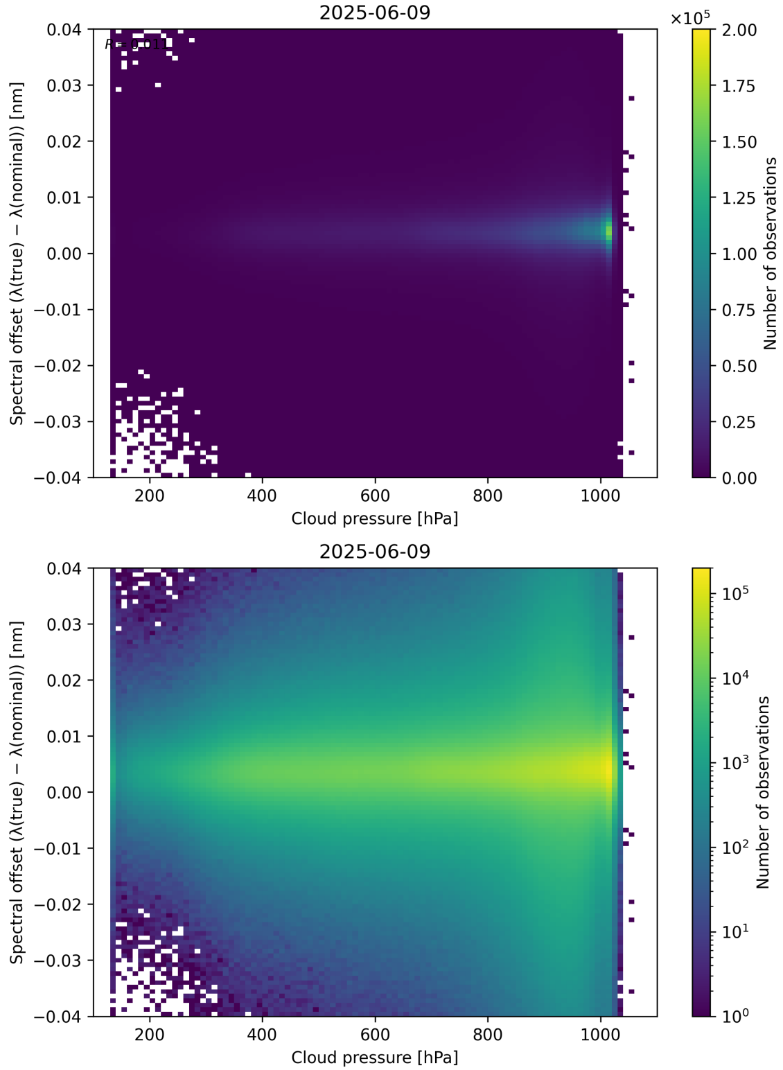
Figure 84: Scatter density plot of “Cloud pressure” against “Spectral offset ( \lambda_{\text{true}} - \lambda_{\text{nominal}} )” for 2025-06-08 to 2025-06-10.
