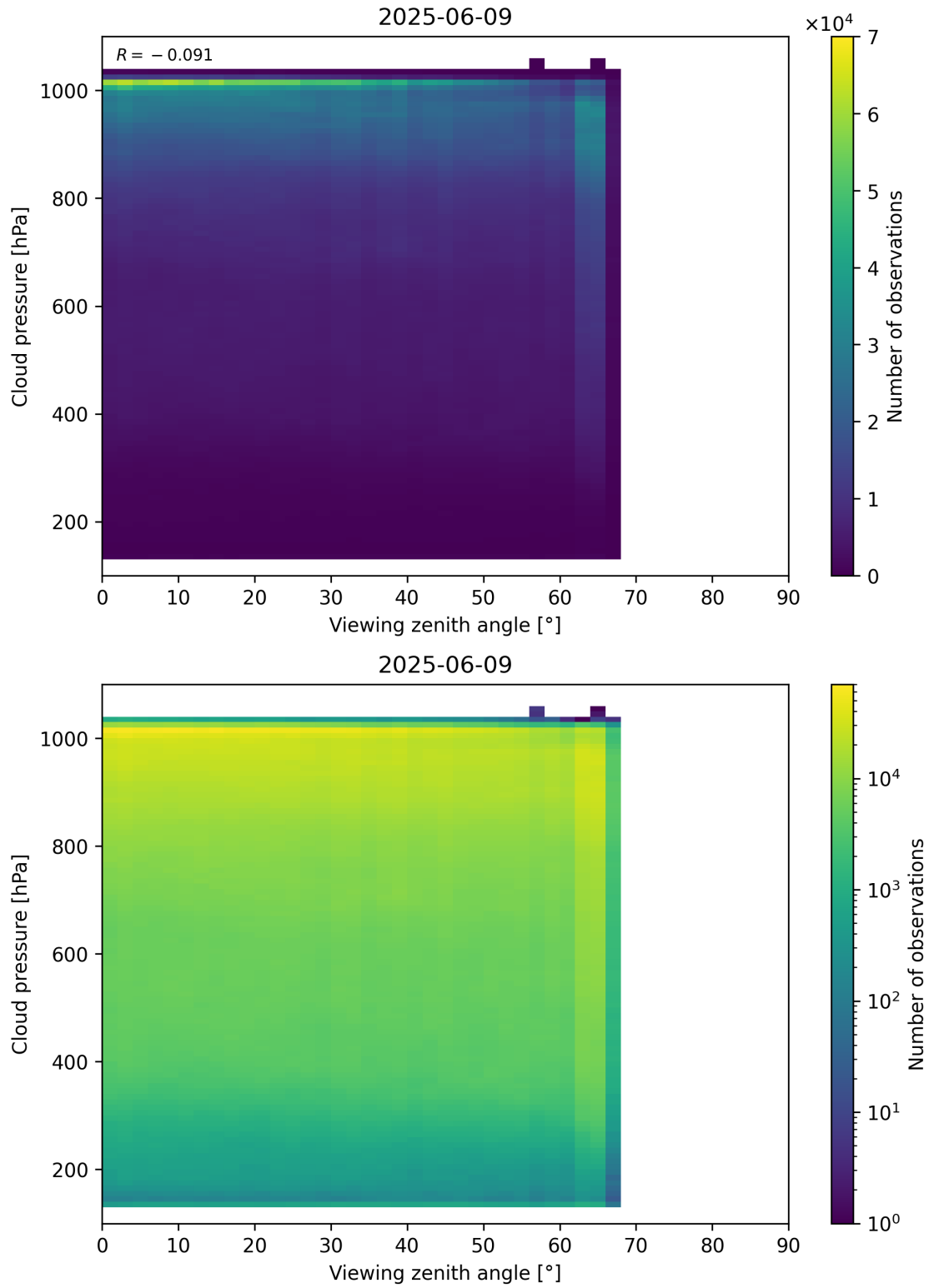
Figure 121: Scatter density plot of “Viewing zenith angle” against “Cloud pressure” for 2025-06-08 to 2025-06-10.
