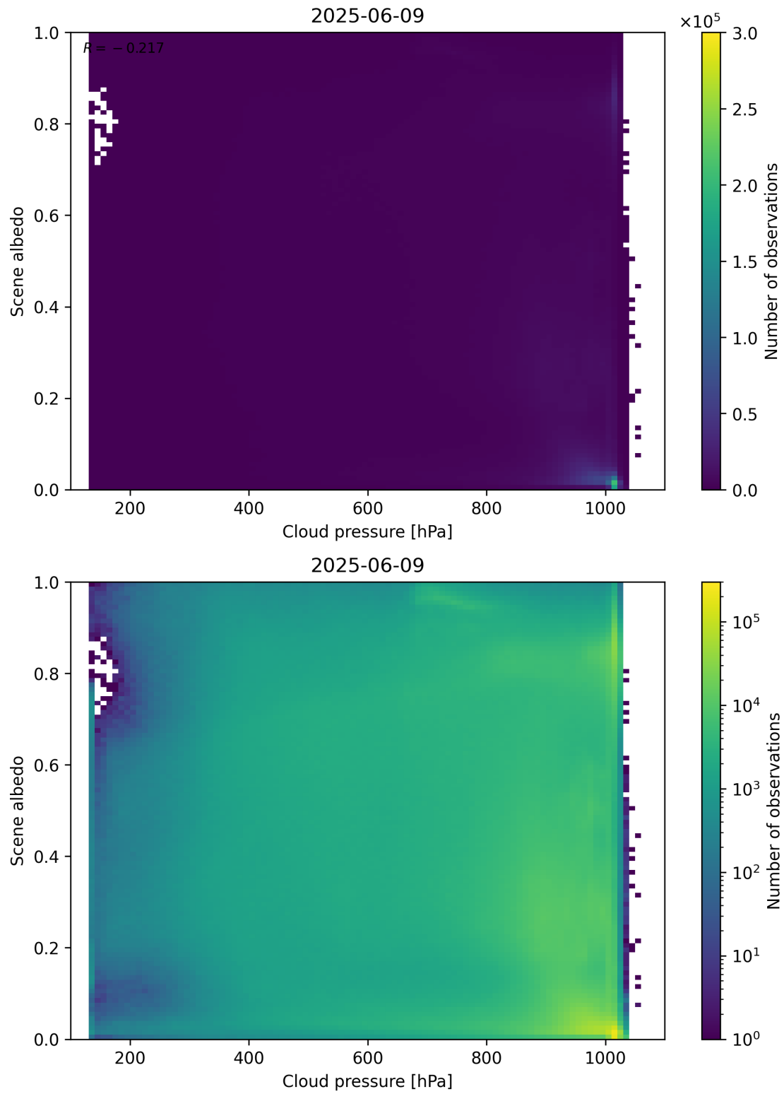
Figure 83: Scatter density plot of “Cloud pressure” against “Scene albedo” for 2025-06-08 to 2025-06-10.
