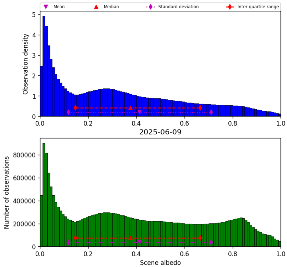
Figure 34: Histogram of “Scene albedo” for 2025-06-08 to 2025-06-10
