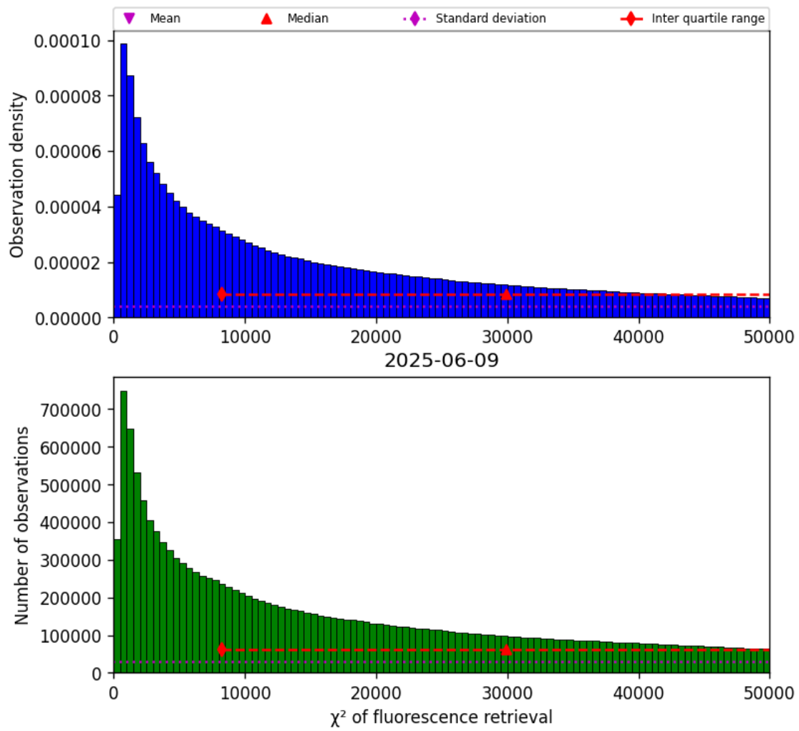
Figure 42: Histogram of “ \chi^2 of fluorescence retrieval” for 2025-06-08 to 2025-06-10
