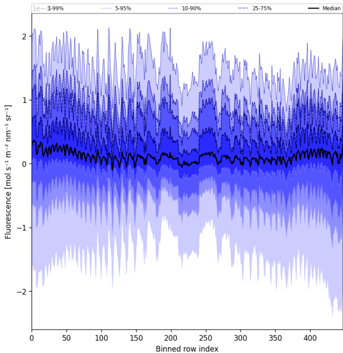
Figure 57: Along track statistics of “Fluorescence” for 2025-06-08 to 2025-06-10
