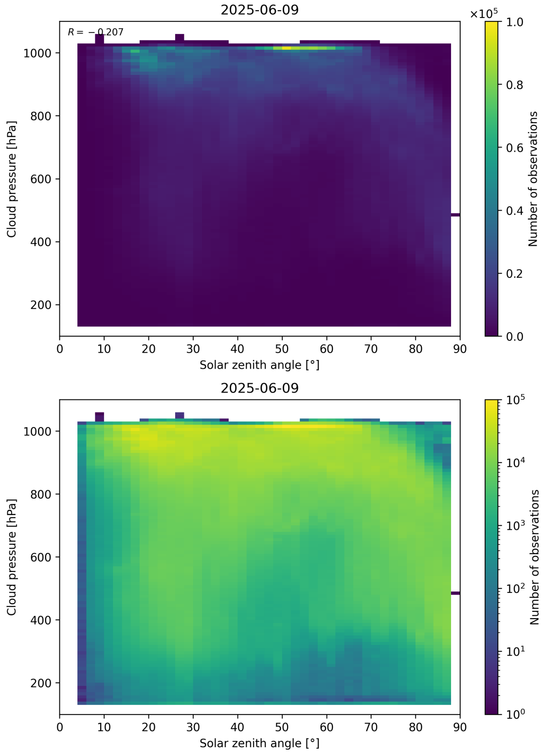
Figure 111: Scatter density plot of “Solar zenith angle” against “Cloud pressure” for 2025-06-08 to 2025-06-10.
