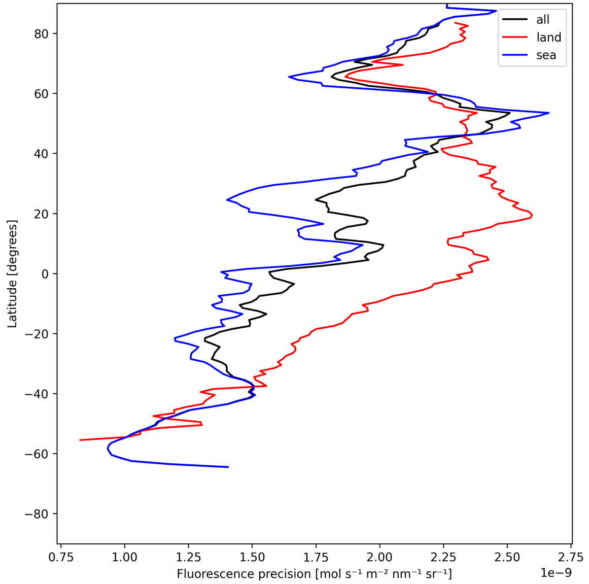
Figure 24: Zonal average of “Fluorescence precision” for 2025-06-08 to 2025-06-10.
