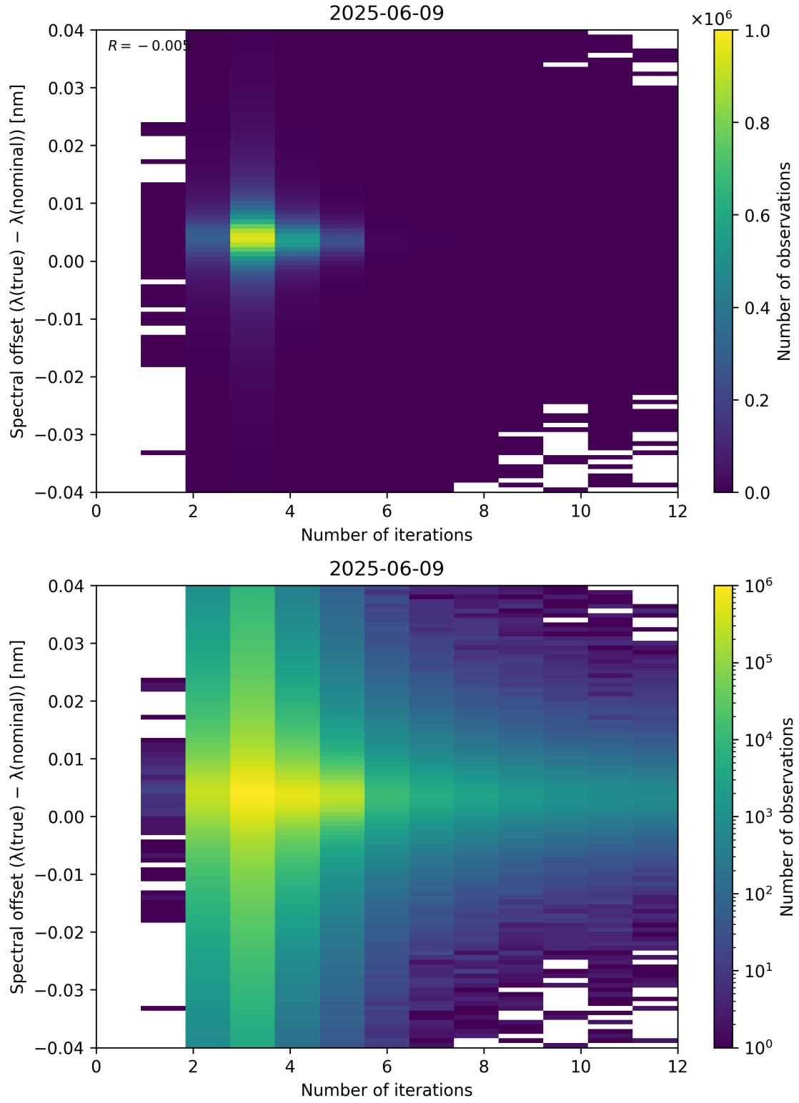
Figure 100: Scatter density plot of “Number of iterations” against “Spectral offset ( \lambda_{\text{true}} - \lambda_{\text{nominal}} )” for 2025-06-08 to 2025-06-10.
