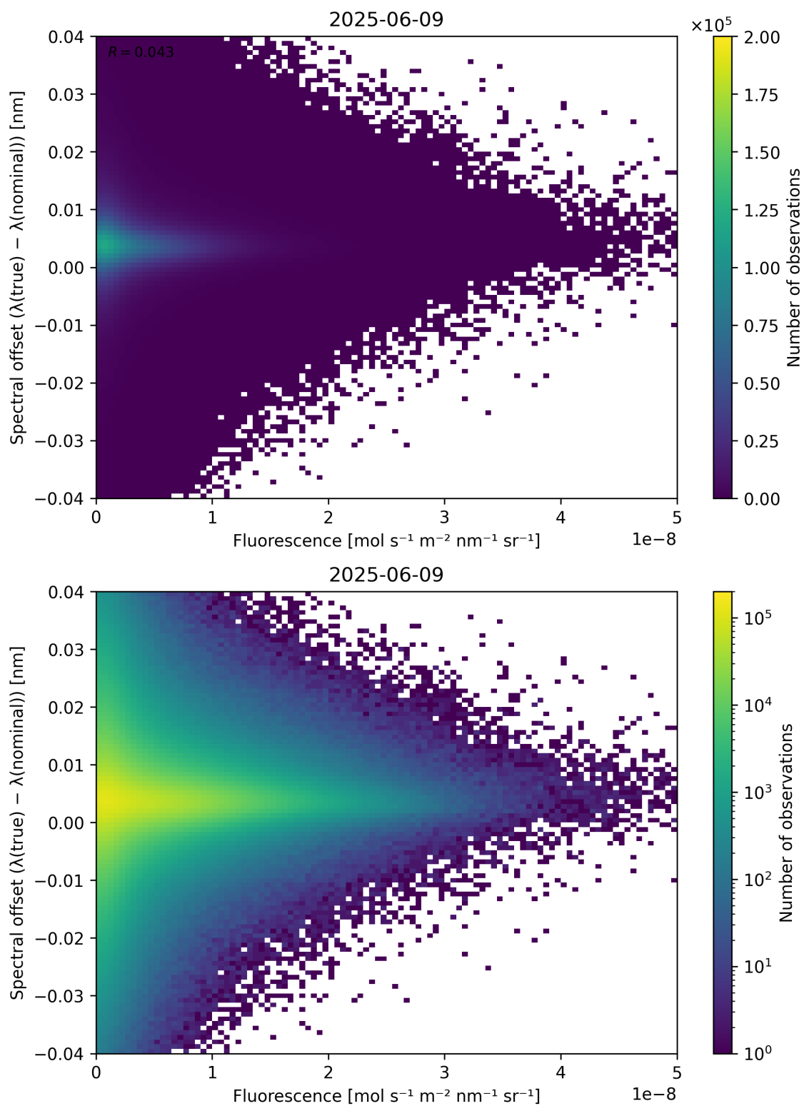
Figure 87: Scatter density plot of “Fluorescence” against “Spectral offset ( \lambda_{\text{true}} - \lambda_{\text{nominal}} )” for 2025-06-08 to 2025-06-10.
