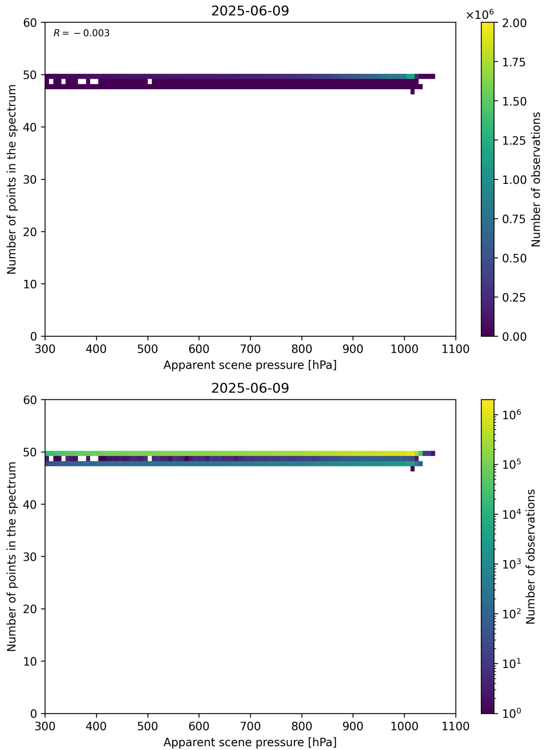
Figure 66: Scatter density plot of “Apparent scene pressure” against “Number of points in the spectrum” for 2025-06-08 to 2025-06-10.
