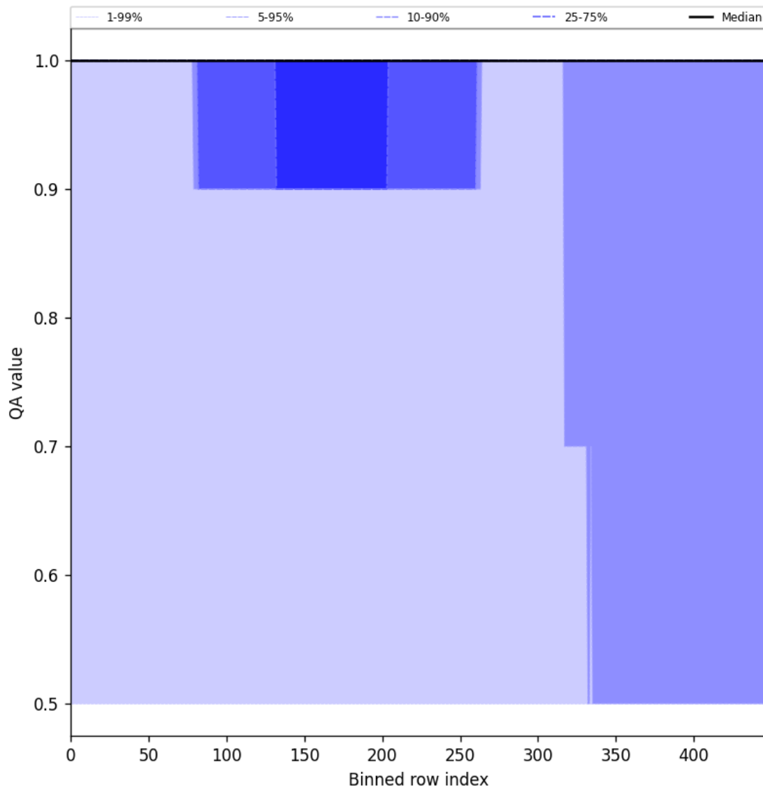
Figure 46: Along track statistics of “QA value” for 2025-06-08 to 2025-06-10
