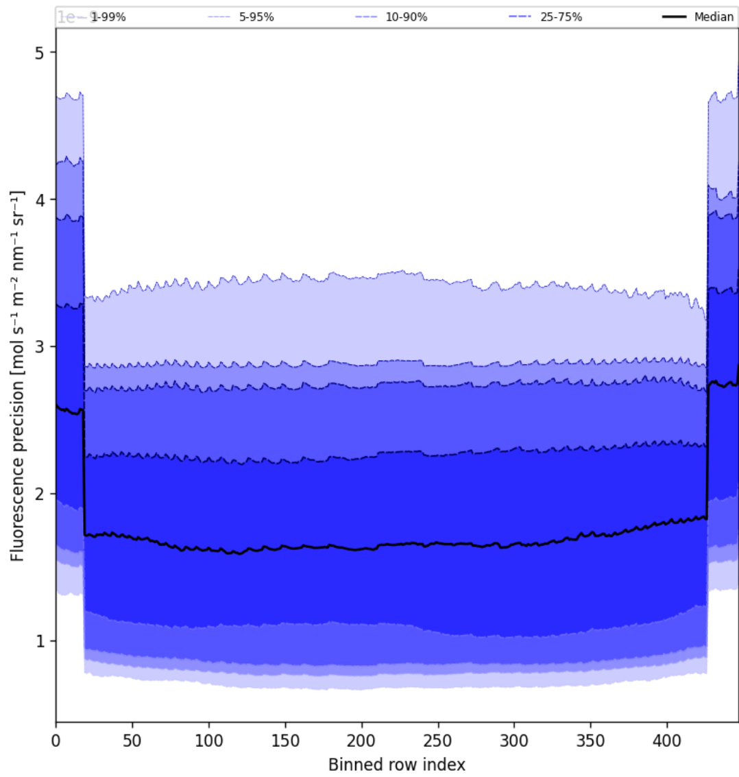
Figure 58: Along track statistics of “Fluorescence precision” for 2025-06-08 to 2025-06-10
