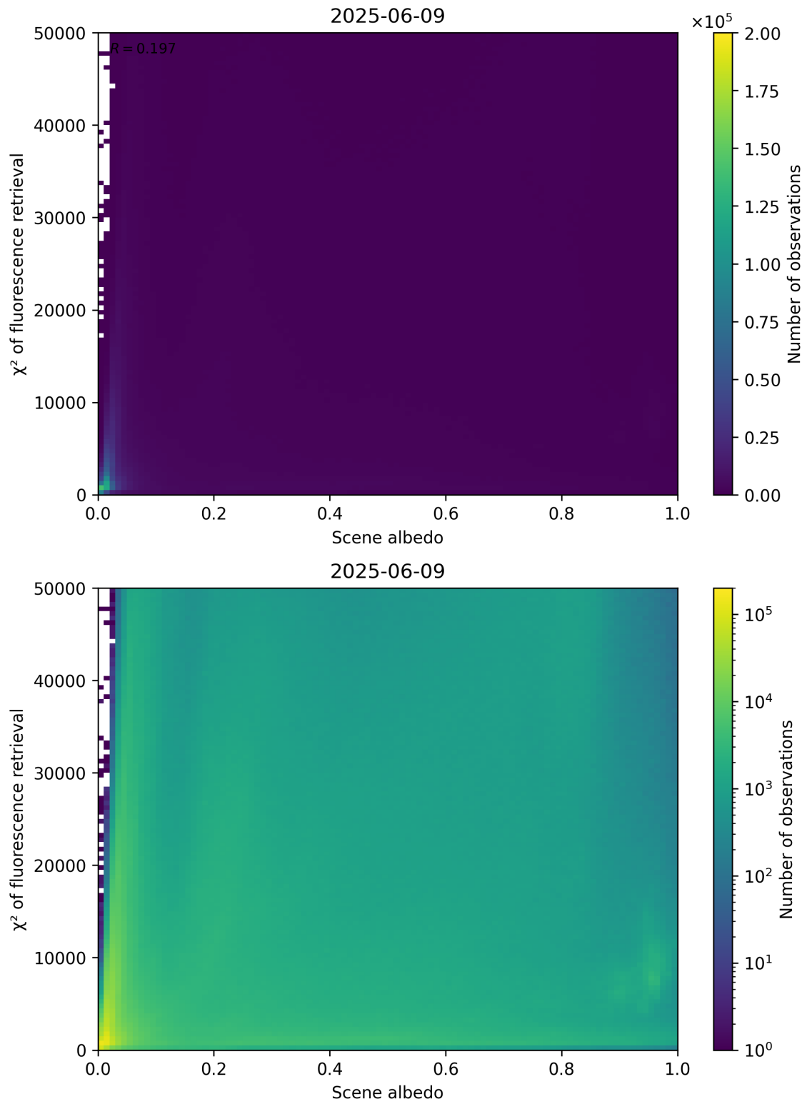
Figure 103: Scatter density plot of “Scene albedo” against “ \chi^2 of fluorescence retrieval” for 2025-06-08 to 2025-06-10.
