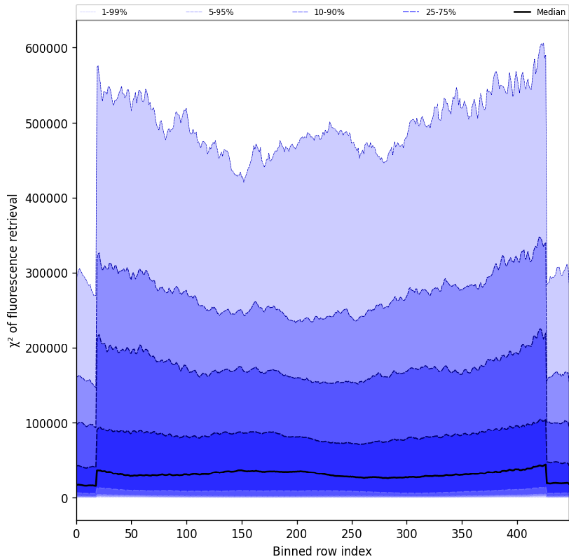
Figure 59: Along track statistics of “ \chi^2 of fluorescence retrieval” for 2025-06-08 to 2025-06-10
