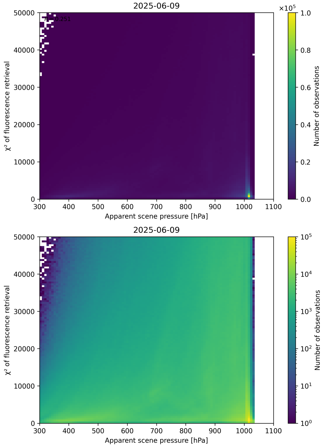
Figure 63: Scatter density plot of “Apparent scene pressure” against “ \chi^2 of fluorescence retrieval” for 2025-06-08 to 2025-06-10.
