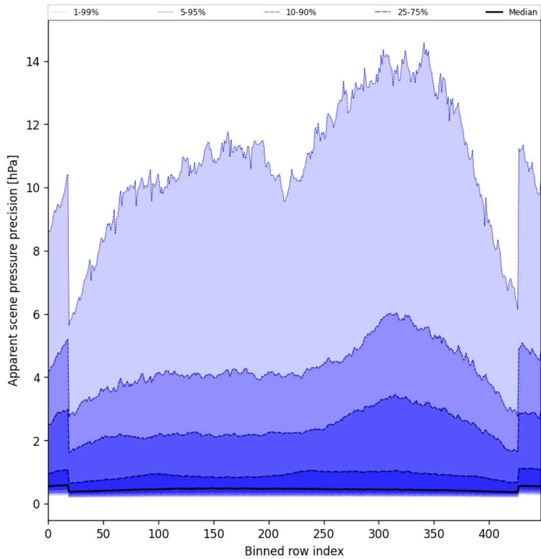
Figure 54: Along track statistics of “Apparent scene pressure precision” for 2025-06-08 to 2025-06-10
