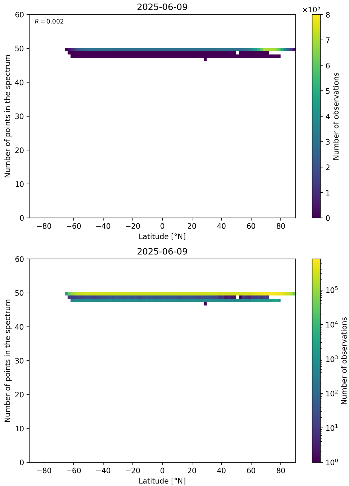
Figure 94: Scatter density plot of “Latitude” against “Number of points in the spectrum” for 2025-06-08 to 2025-06-10.
