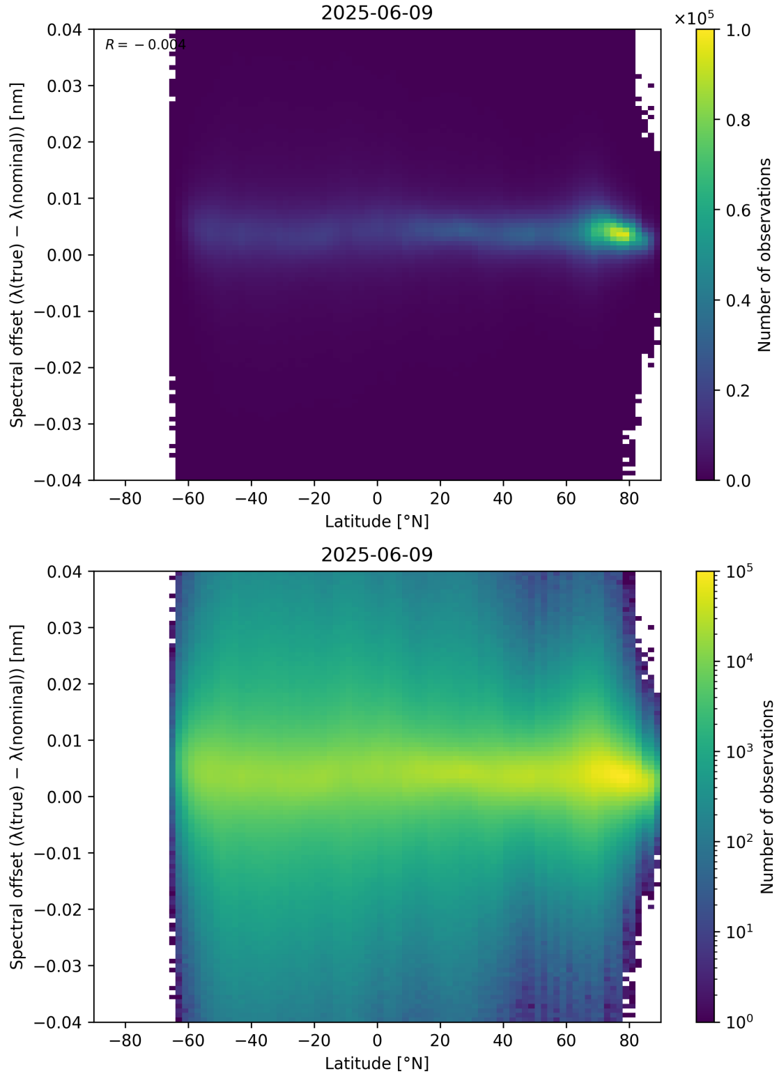
Figure 96: Scatter density plot of “Latitude” against “Spectral offset ( \lambda_{\text{true}} - \lambda_{\text{nominal}} )” for 2025-06-08 to 2025-06-10.
