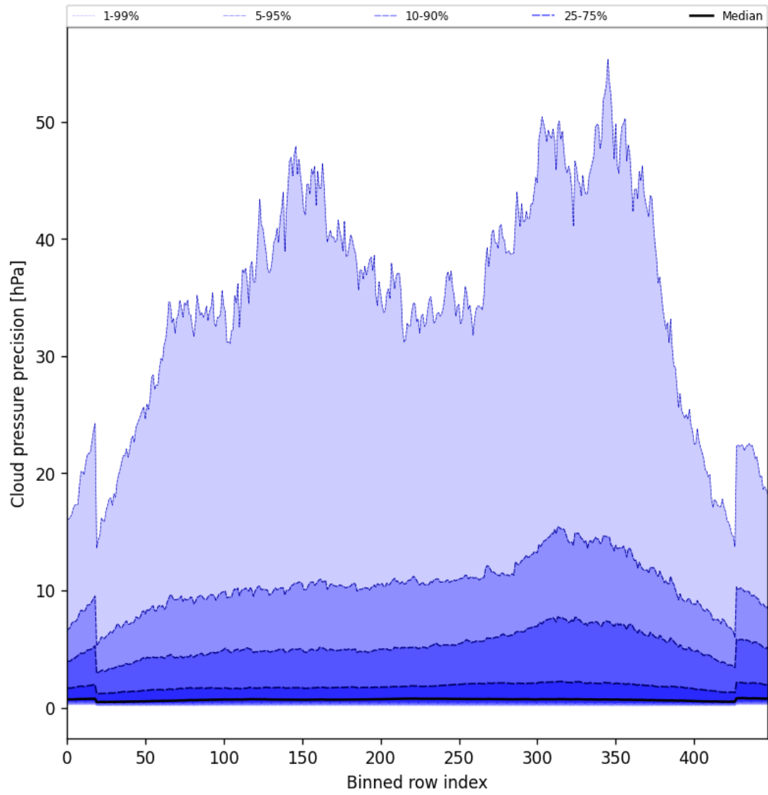
Figure 48: Along track statistics of “Cloud pressure precision” for 2025-06-08 to 2025-06-10
