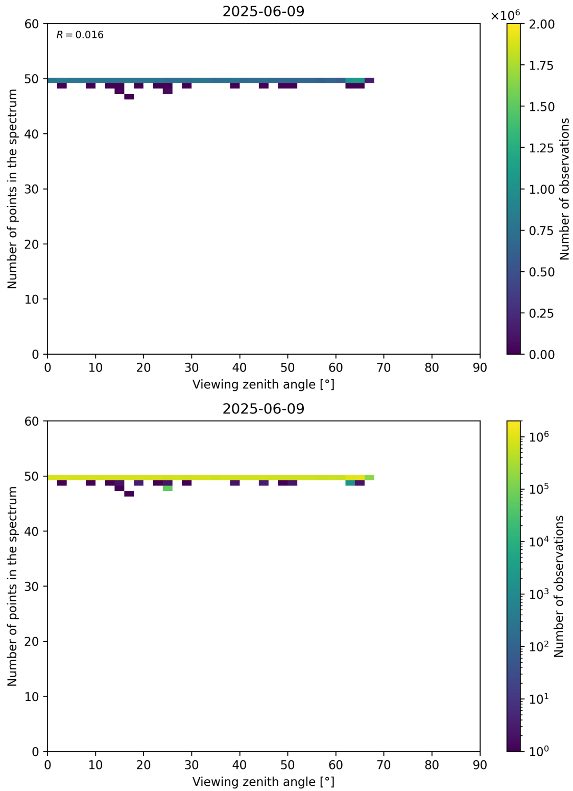
Figure 125: Scatter density plot of “Viewing zenith angle” against “Number of points in the spectrum” for 2025-06-08 to 2025-06-10.
