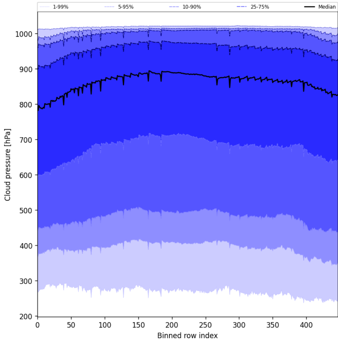
Figure 47: Along track statistics of “Cloud pressure” for 2025-06-08 to 2025-06-10
