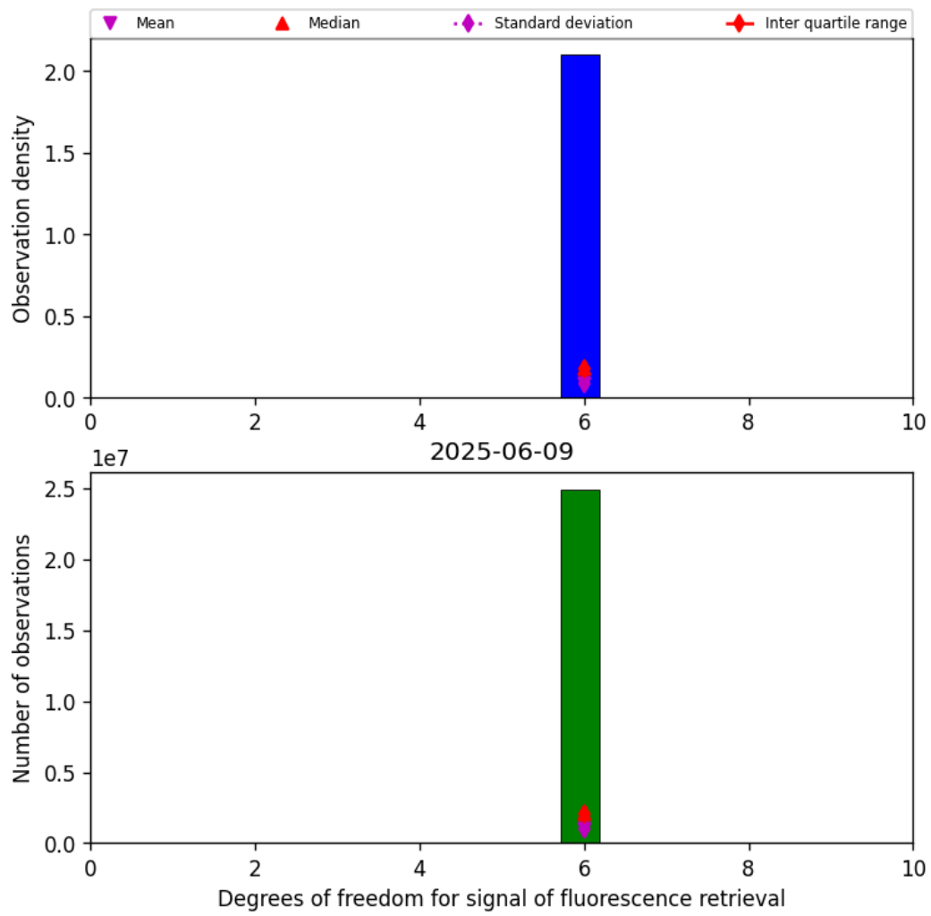
Figure 43: Histogram of "Degrees of freedom for signal of fluorescence retrieval" for 2025-06-08 to 2025-06-10
