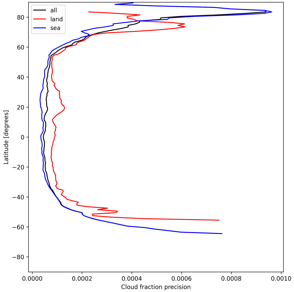
Figure 16: Zonal average of “Cloud fraction precision” for 2025-06-08 to 2025-06-10.
