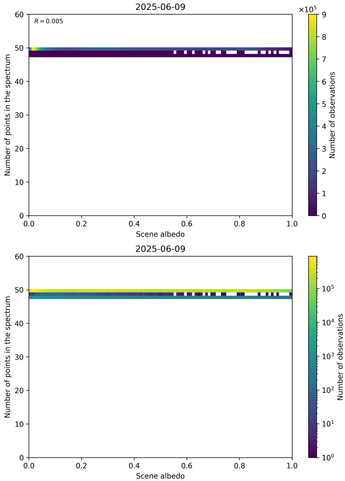
Figure 106: Scatter density plot of “Scene albedo” against “Number of points in the spectrum” for 2025-06-08 to 2025-06-10.
