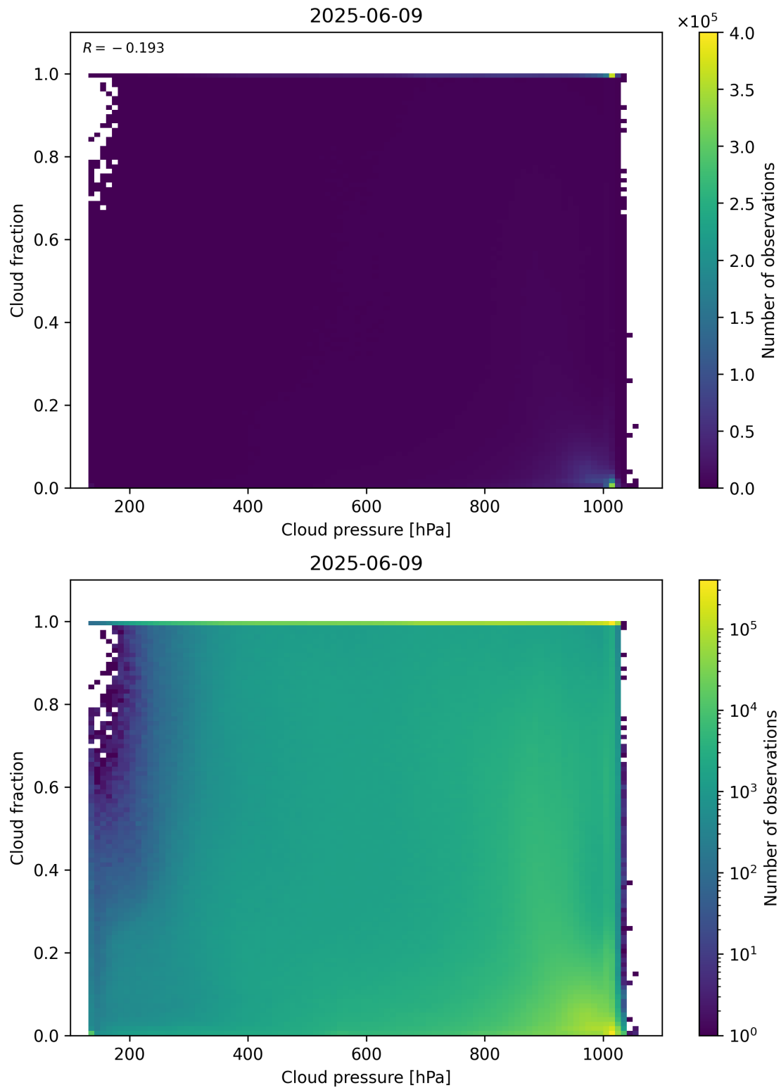
Figure 79: Scatter density plot of “Cloud pressure” against “Cloud fraction” for 2025-06-08 to 2025-06-10.
