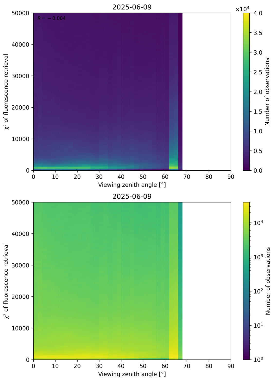
Figure 119: Scatter density plot of “Viewing zenith angle” against “ \chi^2 of fluorescence retrieval” for 2025-06-08 to 2025-06-10.
