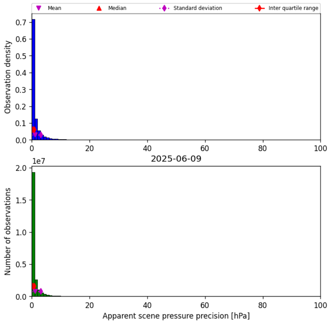
Figure 37: Histogram of “Apparent scene pressure precision” for 2025-06-08 to 2025-06-10
