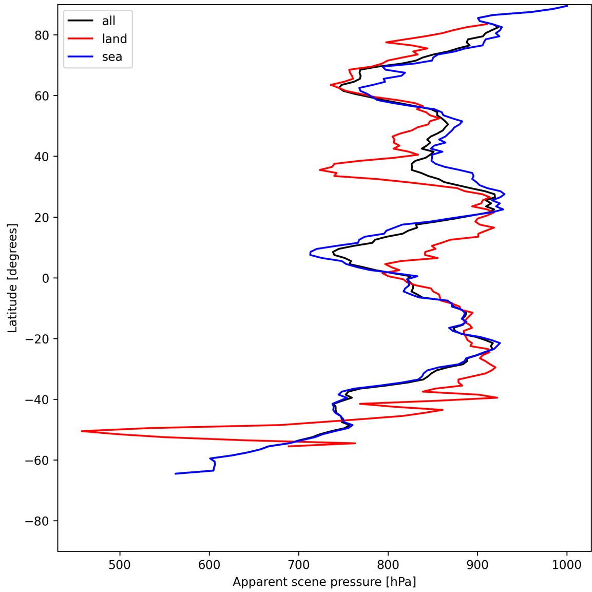
Figure 19: Zonal average of “Apparent scene pressure” for 2025-06-08 to 2025-06-10.
