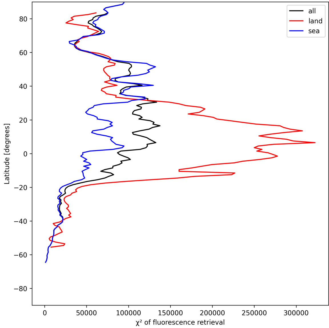
Figure 25: Zonal average of “ \chi^2 of fluorescence retrieval” for 2025-06-08 to 2025-06-10.
