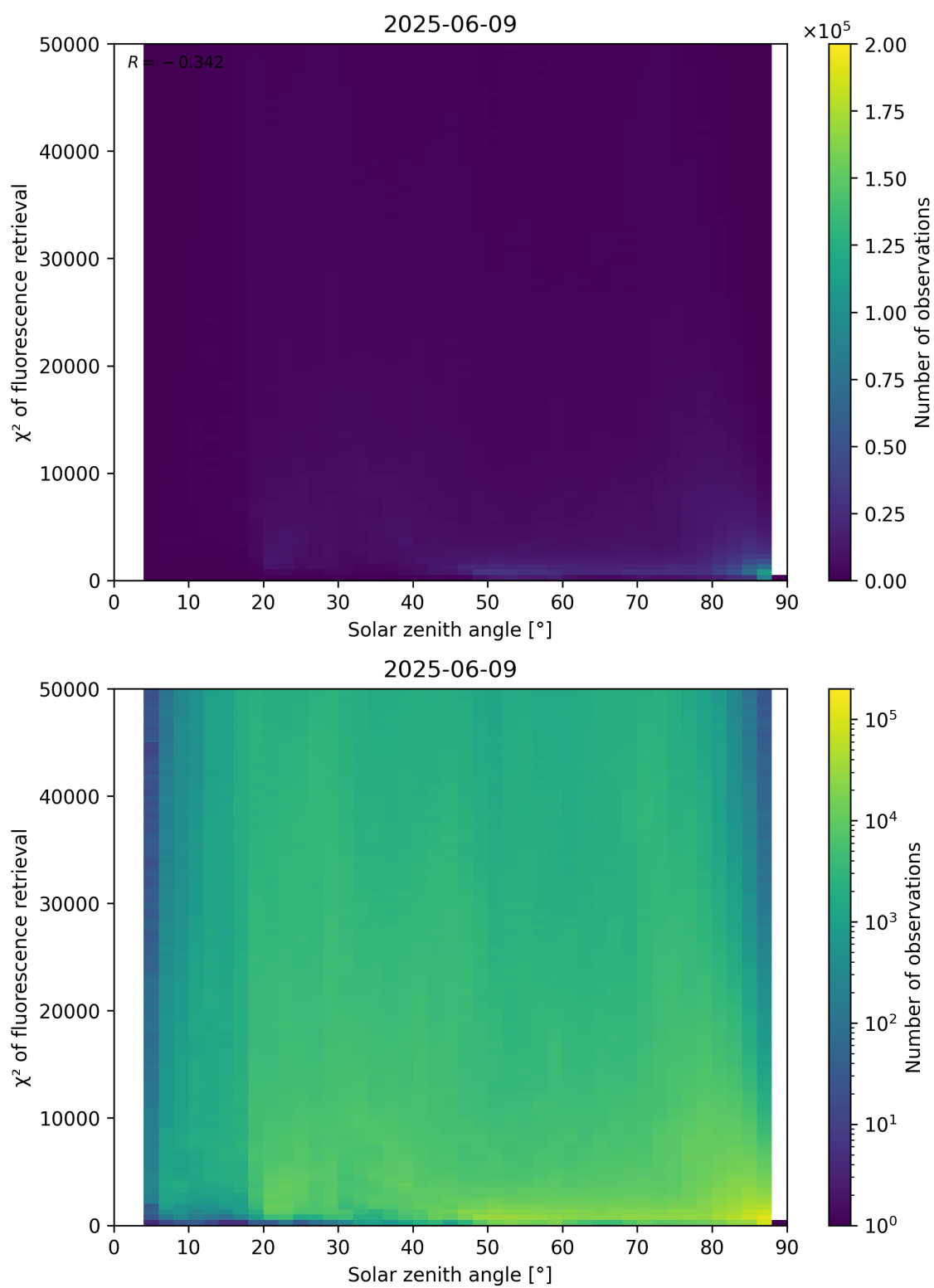
Figure 109: Scatter density plot of “Solar zenith angle” against “ \chi^2 of fluorescence retrieval” for 2025-06-08 to 2025-06-10.
