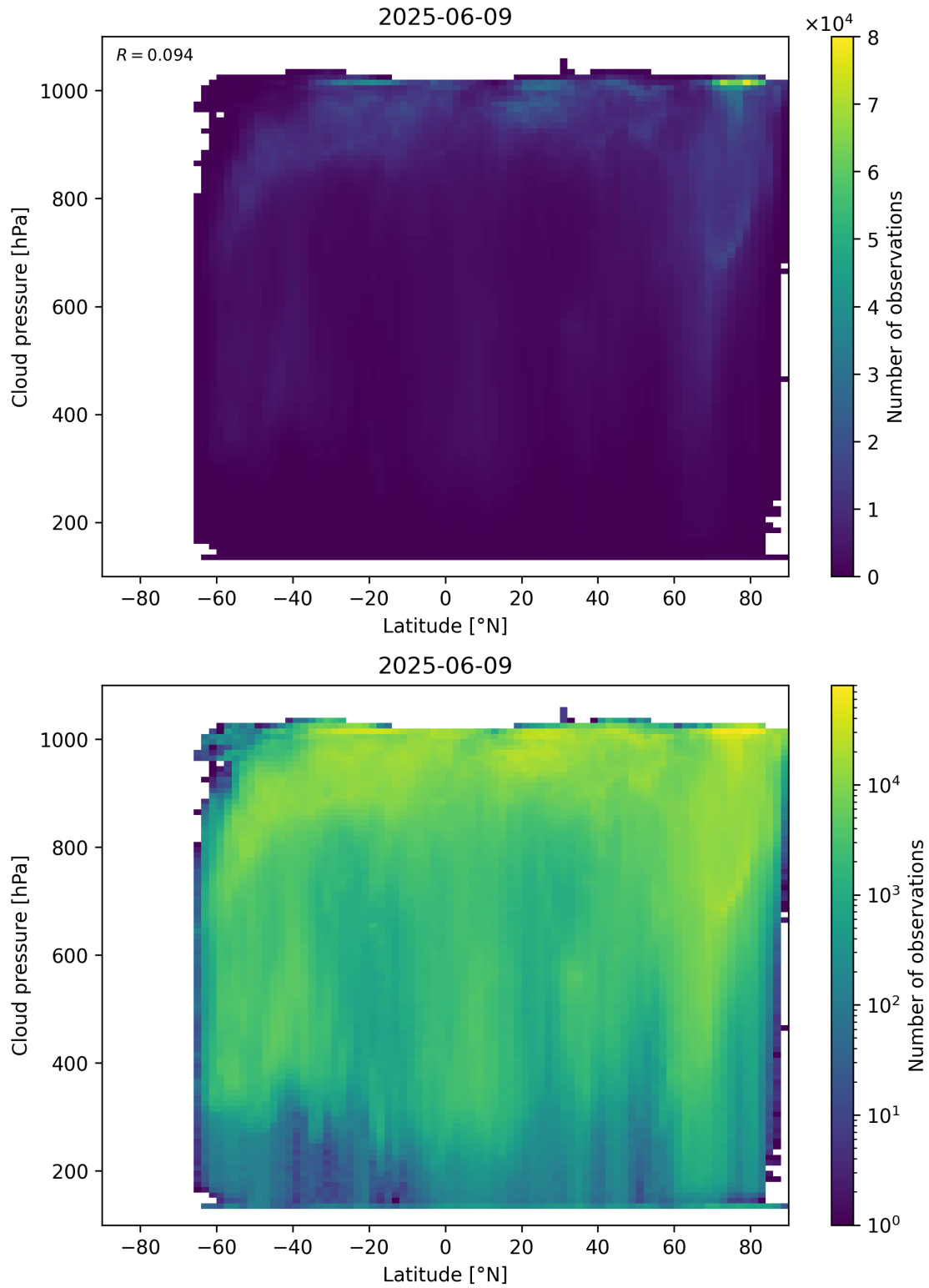
Figure 91: Scatter density plot of “Latitude” against “Cloud pressure” for 2025-06-08 to 2025-06-10.
