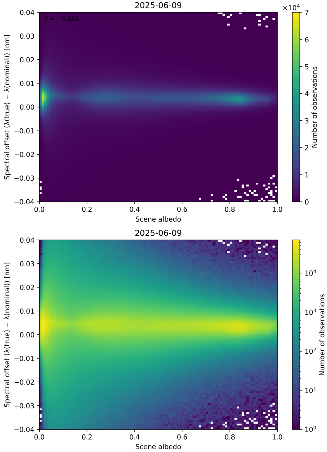
Figure 107: Scatter density plot of “Scene albedo” against “Spectral offset ( \lambda_{\text{true}} - \lambda_{\text{nominal}} )” for 2025-06-08 to 2025-06-10.
