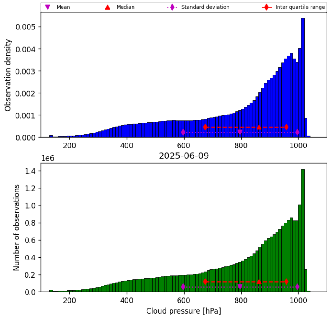
Figure 30: Histogram of “Cloud pressure” for 2025-06-08 to 2025-06-10
