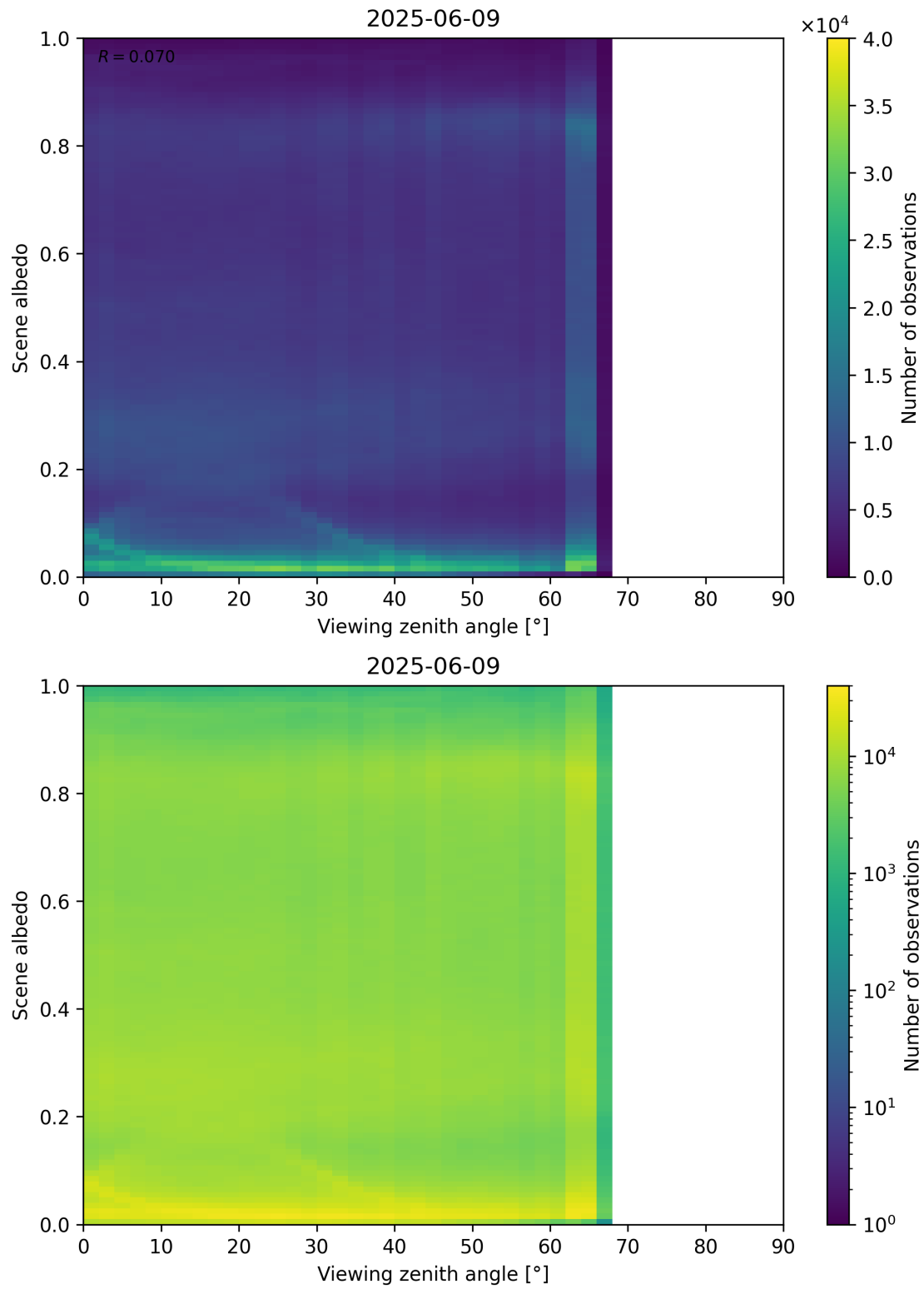
Figure 126: Scatter density plot of “Viewing zenith angle” against “Scene albedo” for 2025-06-08 to 2025-06-10.
