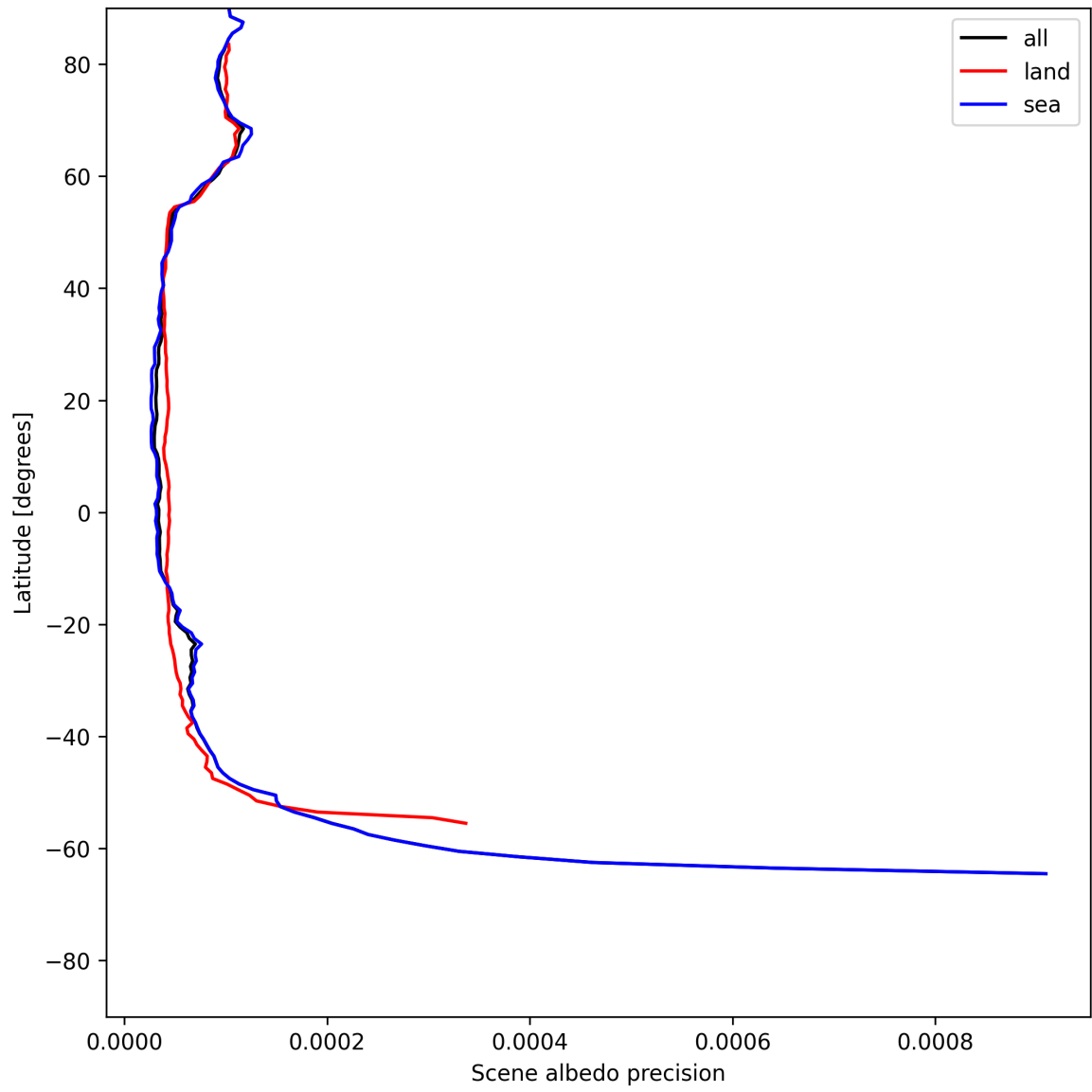
Figure 18: Zonal average of “Scene albedo precision” for 2025-06-08 to 2025-06-10.
