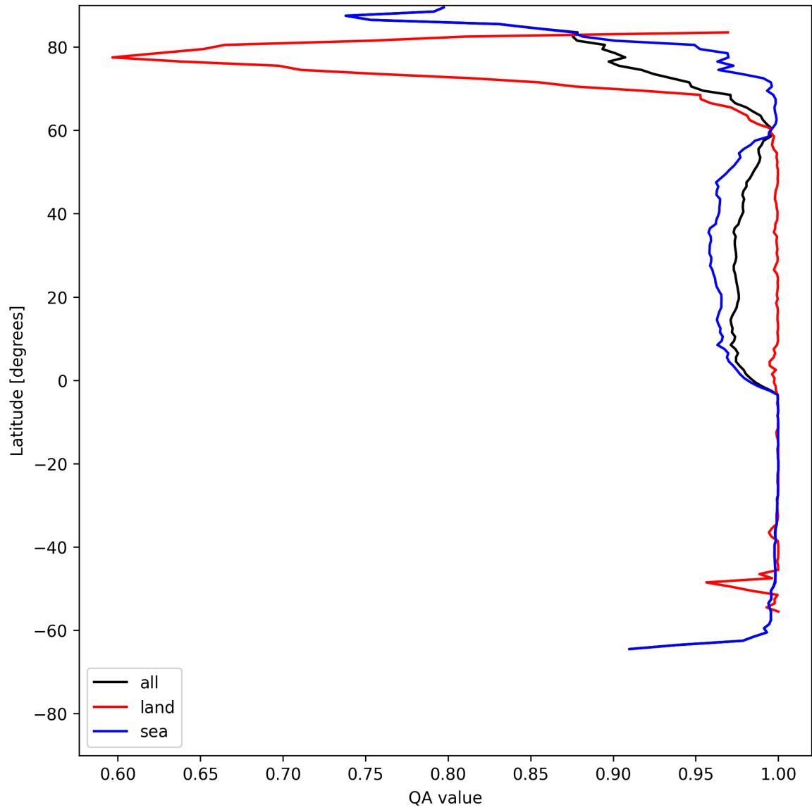
Figure 12: Zonal average of “QA value” for 2025-06-08 to 2025-06-10.
