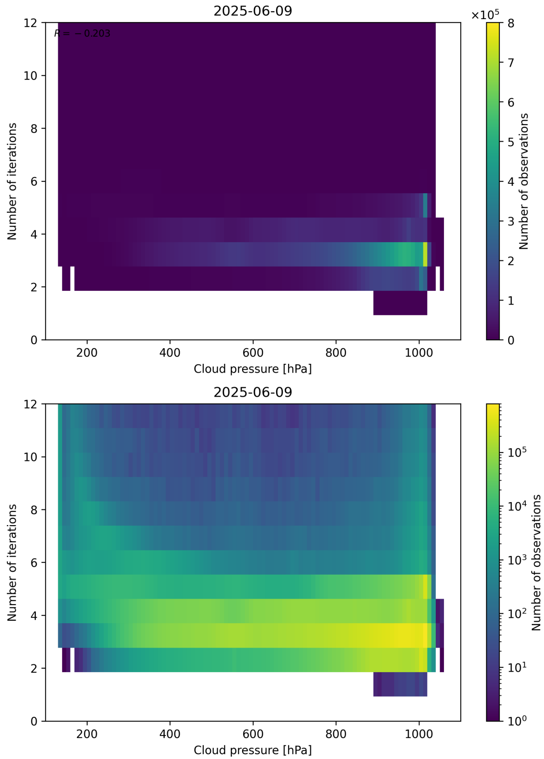
Figure 81: Scatter density plot of “Cloud pressure” against “Number of iterations” for 2025-06-08 to 2025-06-10.
