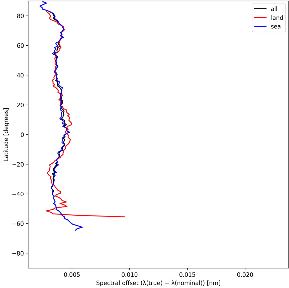
Figure 28: Zonal average of “Spectral offset ( \lambda_{\text{true}} - \lambda_{\text{nominal}} )” for 2025-06-08 to 2025-06-10.
