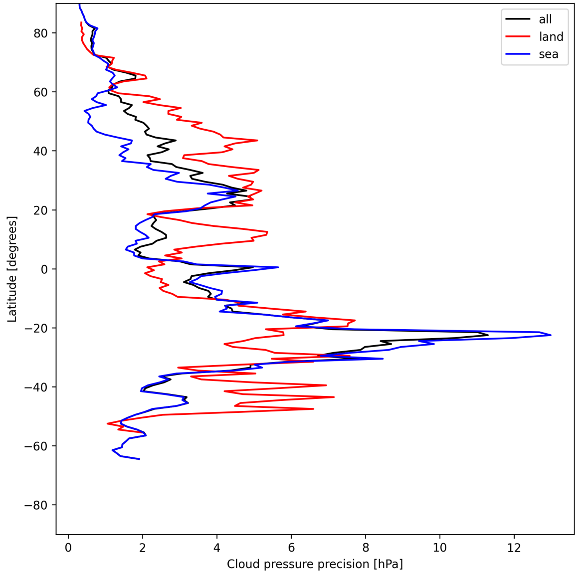
Figure 14: Zonal average of “Cloud pressure precision” for 2025-06-08 to 2025-06-10.
