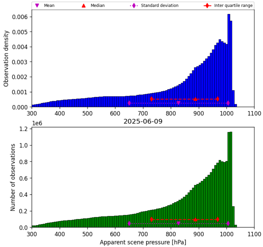
Figure 36: Histogram of “Apparent scene pressure” for 2025-06-08 to 2025-06-10
