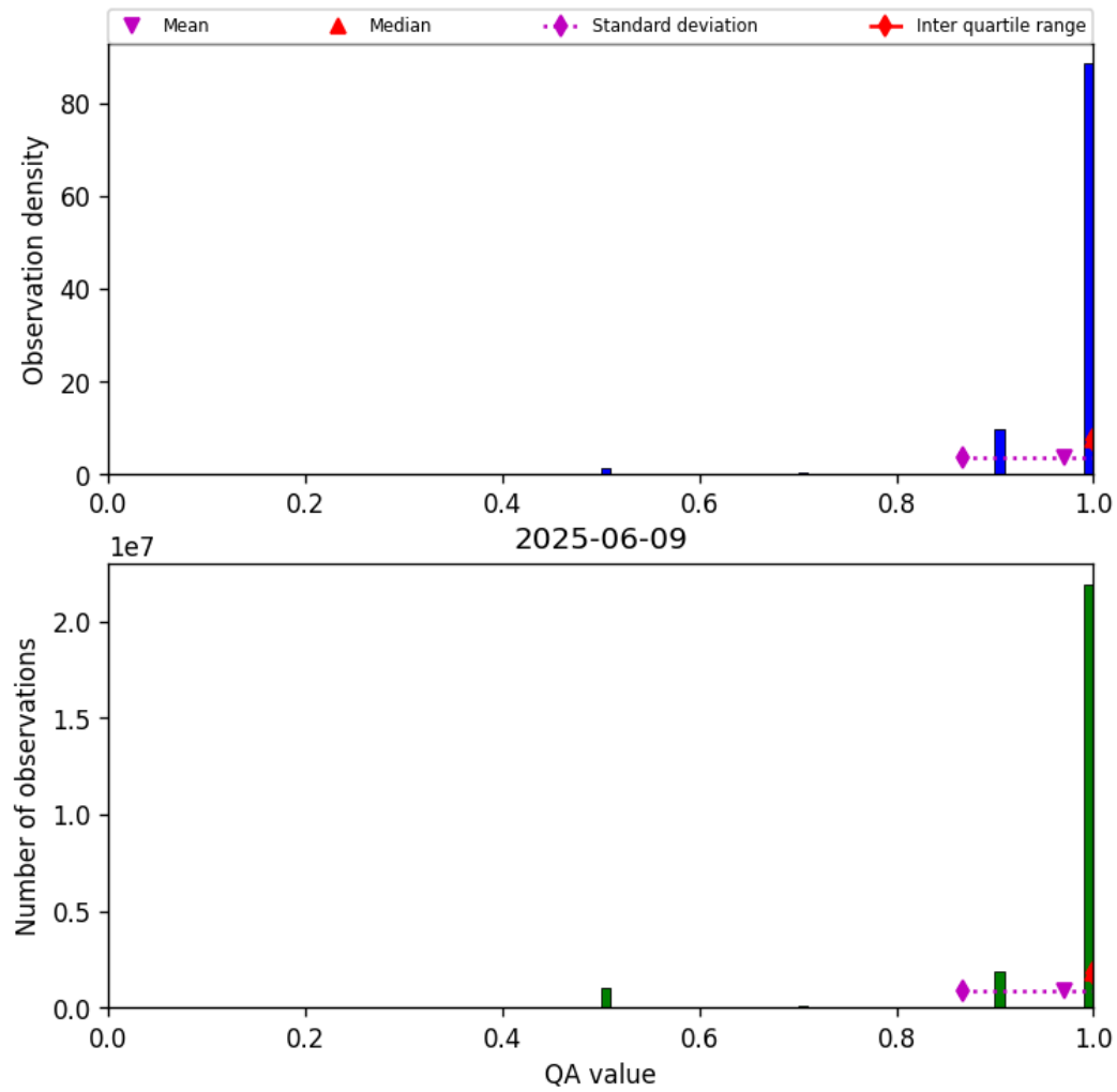
Figure 29: Histogram of “QA value” for 2025-06-08 to 2025-06-10
