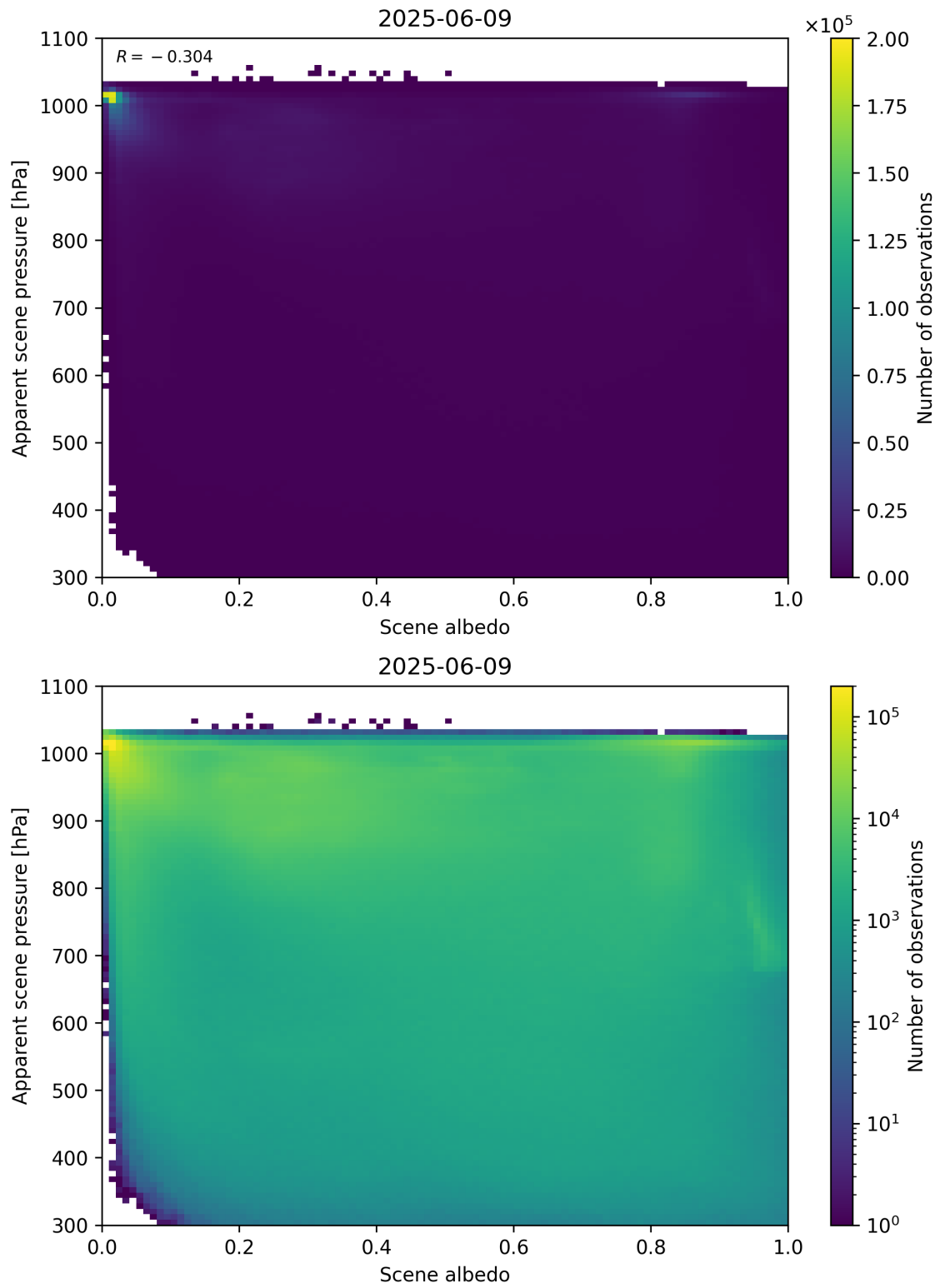
Figure 102: Scatter density plot of “Scene albedo” against “Apparent scene pressure” for 2025-06-08 to 2025-06-10.
