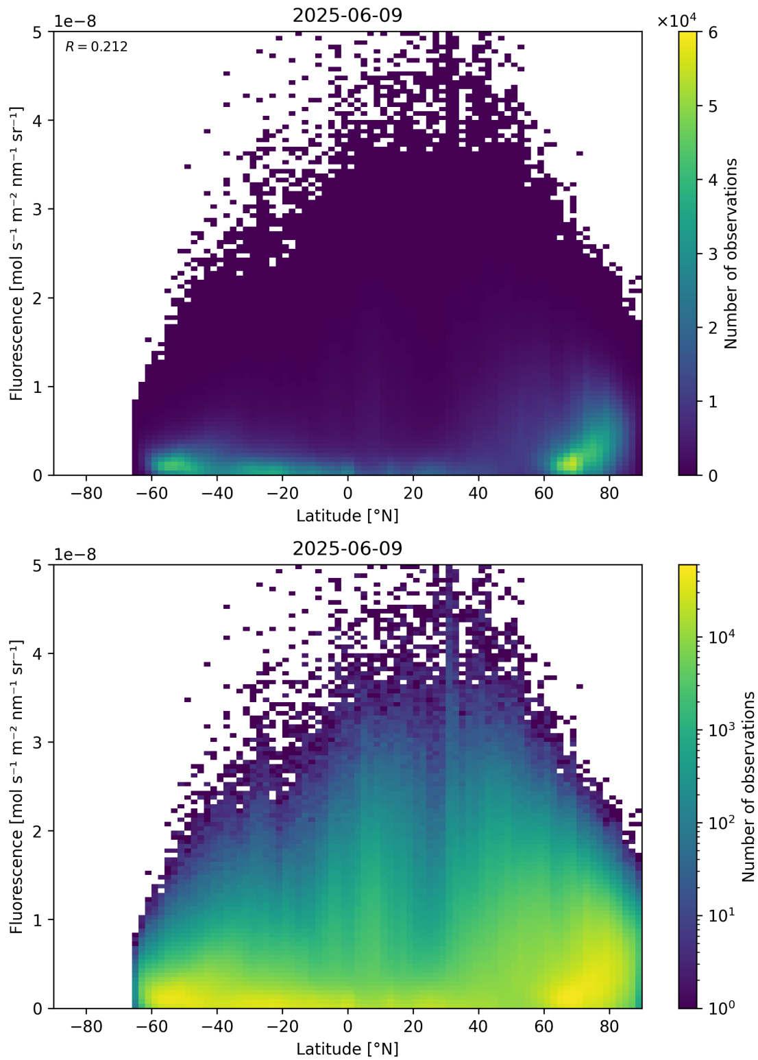
Figure 92: Scatter density plot of “Latitude” against “Fluorescence” for 2025-06-08 to 2025-06-10.
