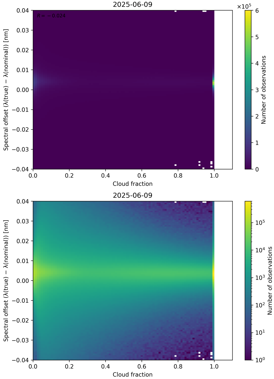
Figure 76: Scatter density plot of “Cloud fraction” against “Spectral offset ( \lambda_{\text{true}} - \lambda_{\text{nominal}} )” for 2025-06-08 to 2025-06-10.
