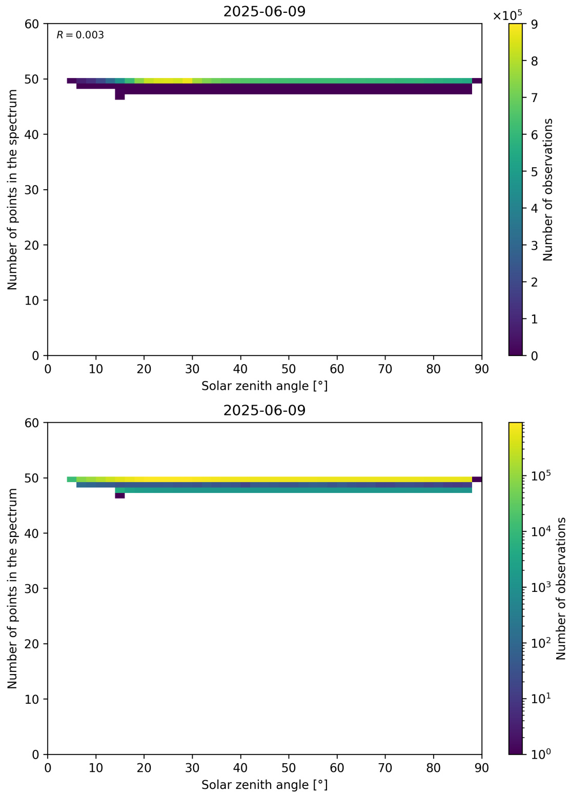
Figure 115: Scatter density plot of “Solar zenith angle” against “Number of points in the spectrum” for 2025-06-08 to 2025-06-10.
