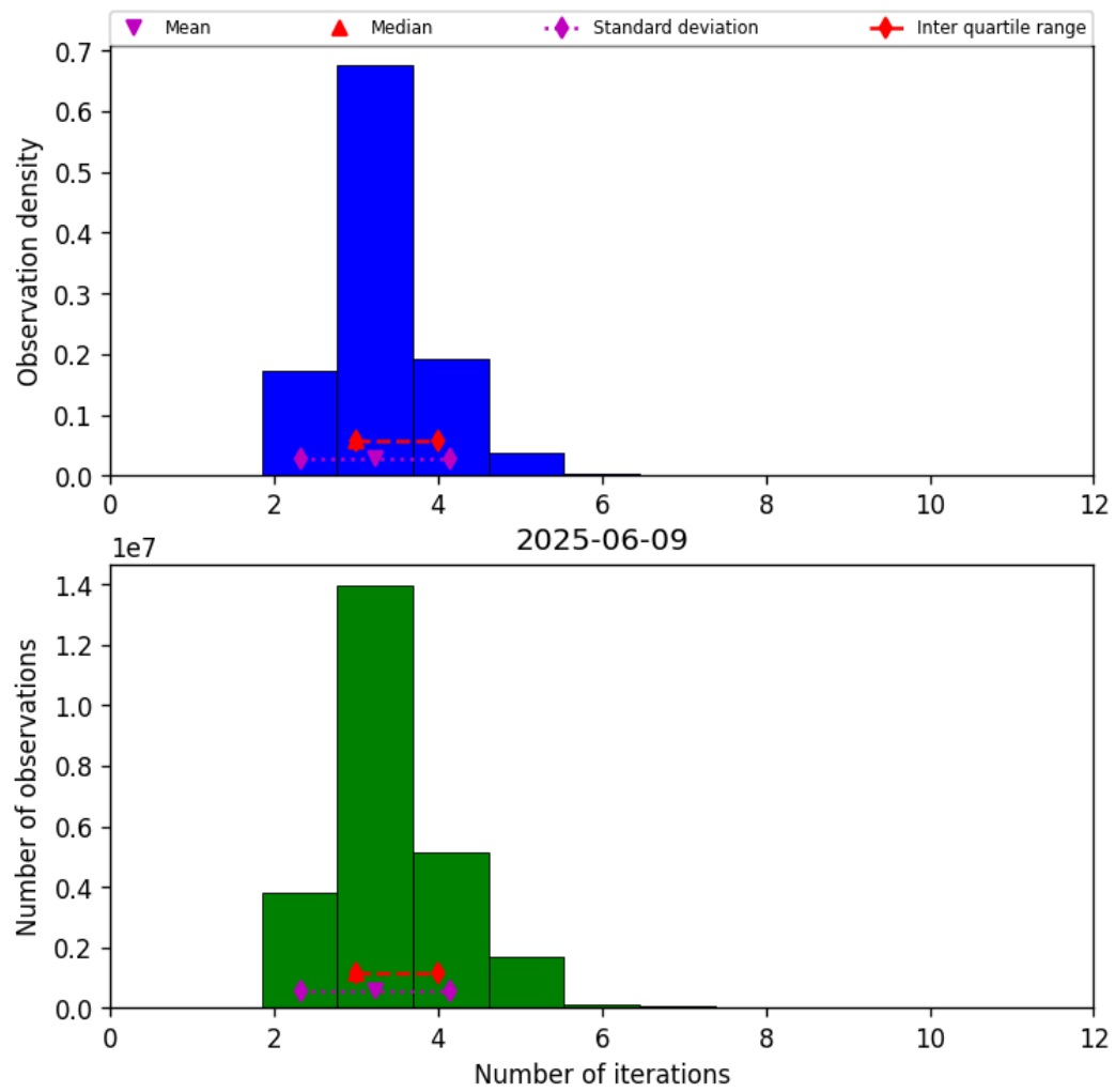
Figure 39: Histogram of “Number of iterations” for 2025-06-08 to 2025-06-10
