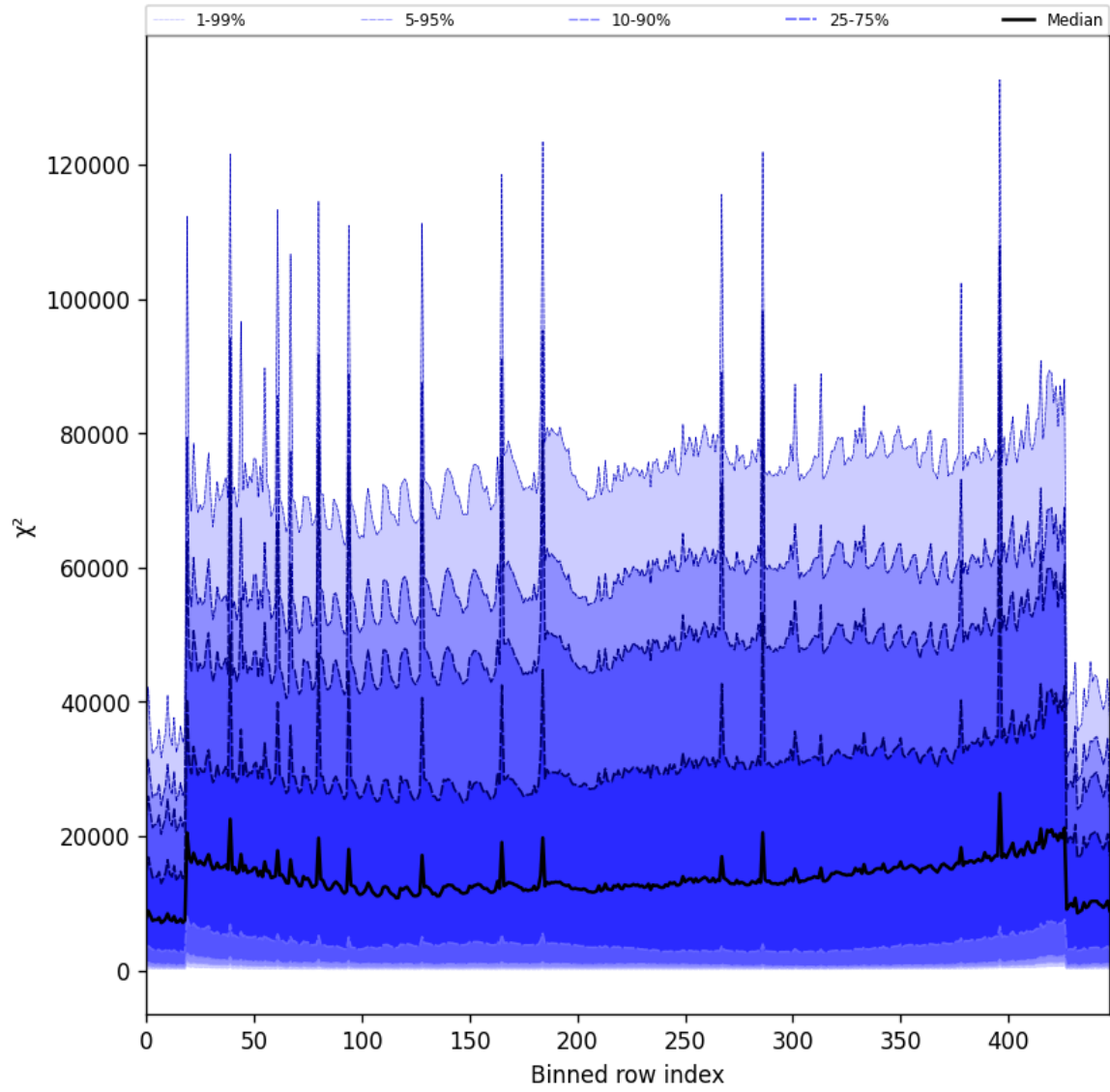
Figure 55: Along track statistics of “ \chi^2 ” for 2025-06-08 to 2025-06-10
