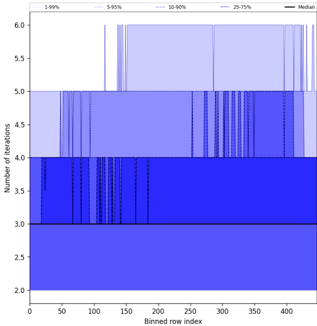
Figure 56: Along track statistics of “Number of iterations” for 2025-06-08 to 2025-06-10
