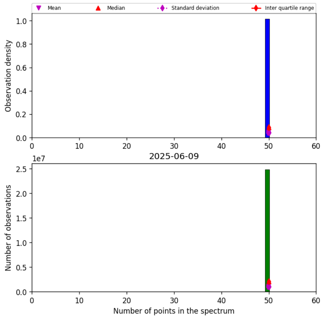
Figure 44: Histogram of “Number of points in the spectrum” for 2025-06-08 to 2025-06-10
