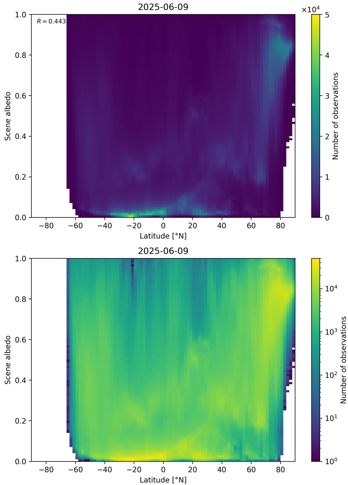
Figure 95: Scatter density plot of “Latitude” against “Scene albedo” for 2025-06-08 to 2025-06-10.
