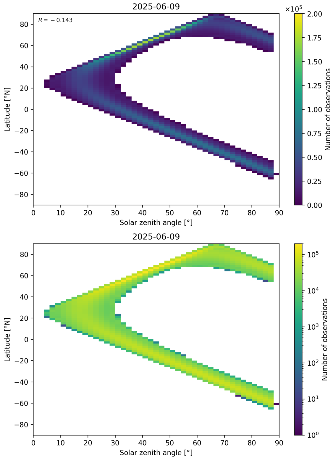
Figure 113: Scatter density plot of “Solar zenith angle” against “Latitude” for 2025-06-08 to 2025-06-10.
