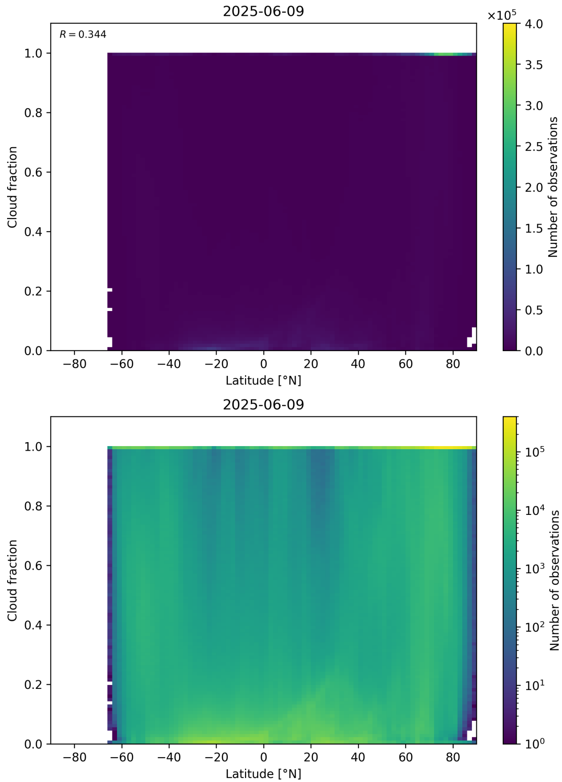
Figure 90: Scatter density plot of “Latitude” against “Cloud fraction” for 2025-06-08 to 2025-06-10.
