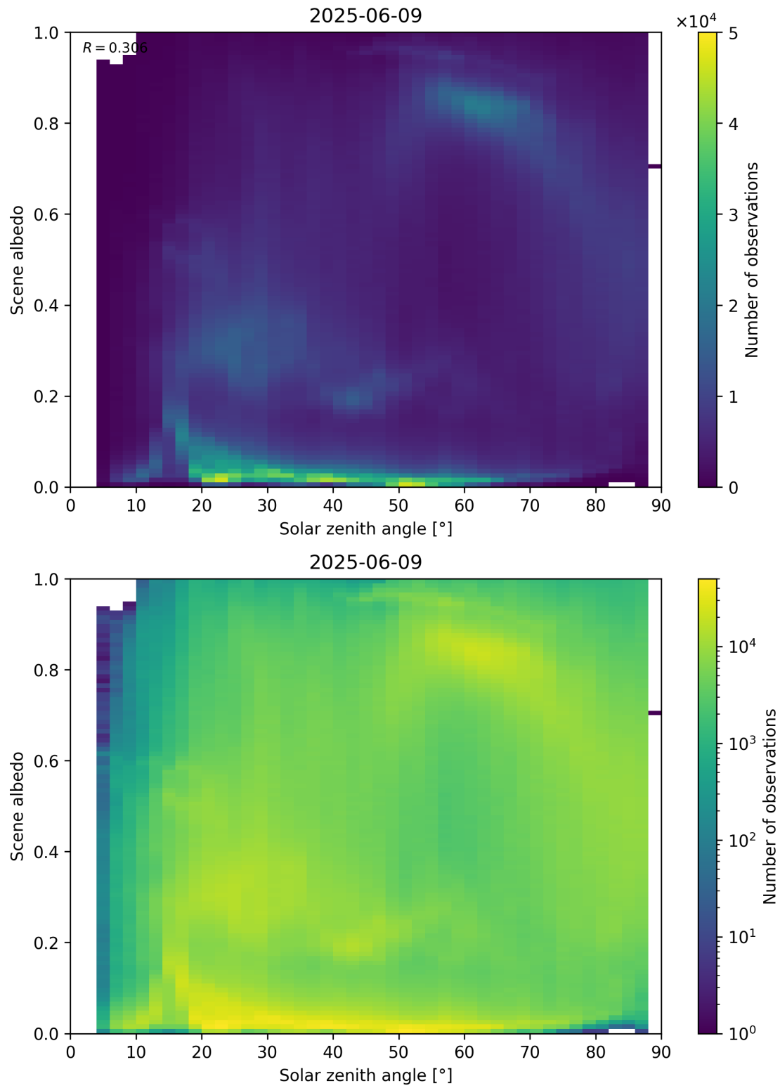
Figure 116: Scatter density plot of “Solar zenith angle” against “Scene albedo” for 2025-06-08 to 2025-06-10.
