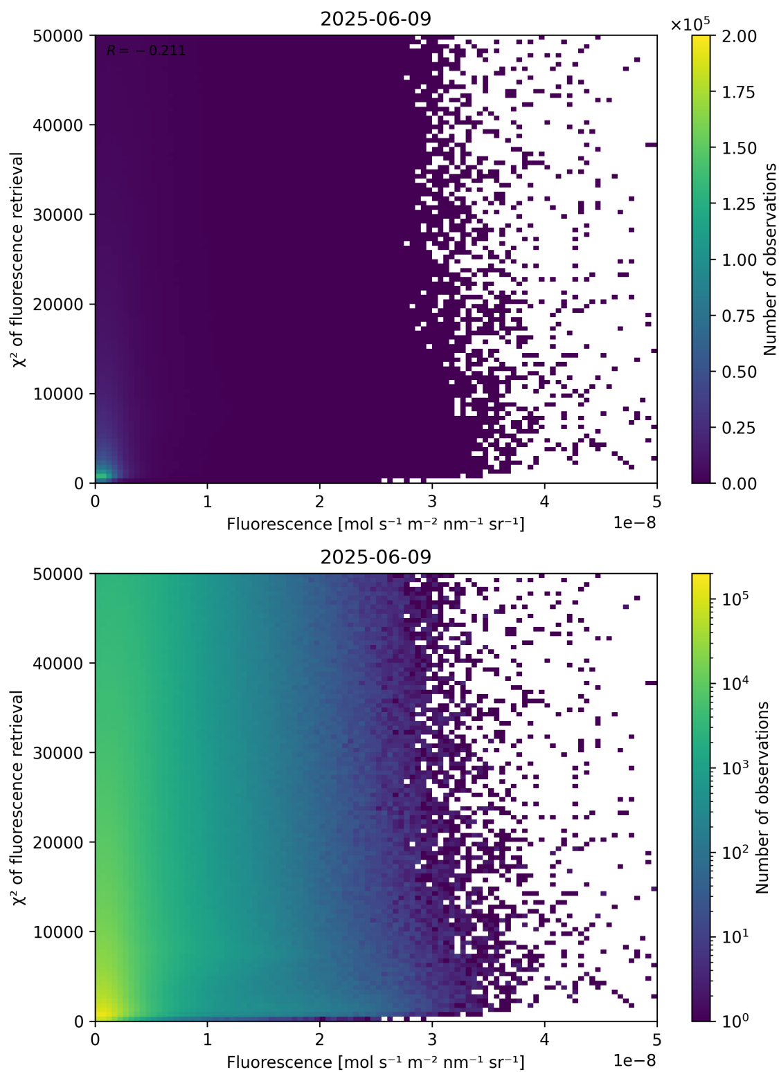
Figure 85: Scatter density plot of “Fluorescence” against “ \chi^2 of fluorescence retrieval” for 2025-06-08 to 2025-06-10.
