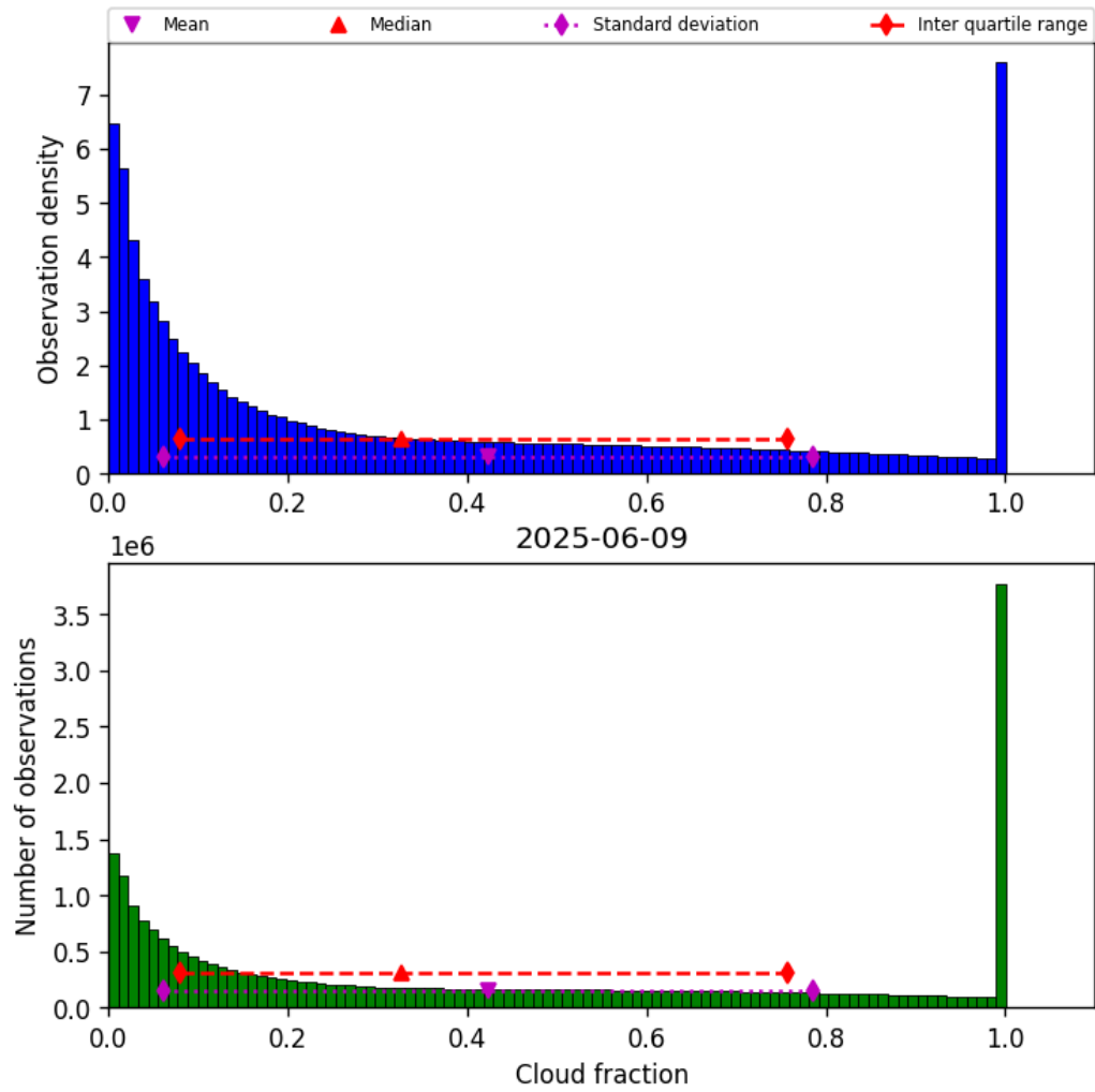
Figure 32: Histogram of “Cloud fraction” for 2025-06-08 to 2025-06-10
