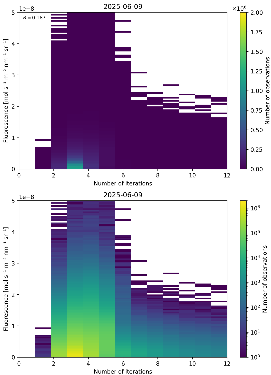
Figure 98: Scatter density plot of “Number of iterations” against “Fluorescence” for 2025-06-08 to 2025-06-10.
