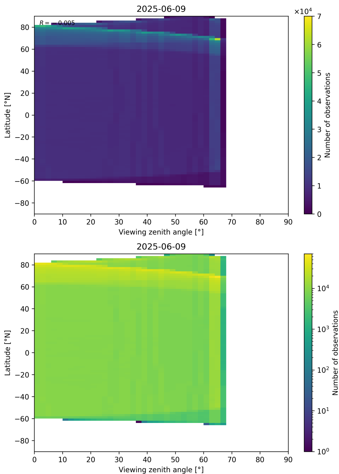
Figure 123: Scatter density plot of “Viewing zenith angle” against “Latitude” for 2025-06-08 to 2025-06-10.
