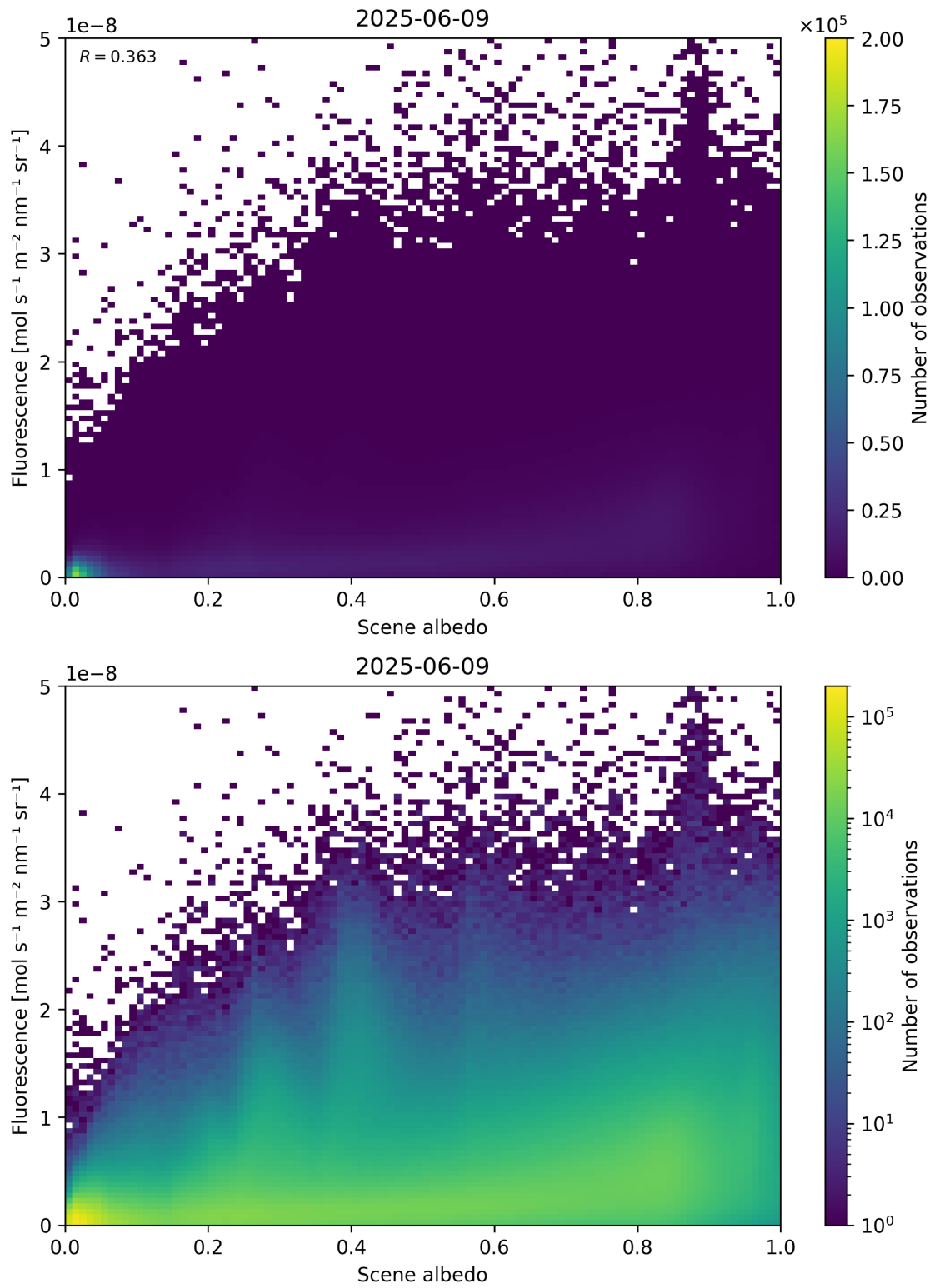
Figure 104: Scatter density plot of “Scene albedo” against “Fluorescence” for 2025-06-08 to 2025-06-10.
