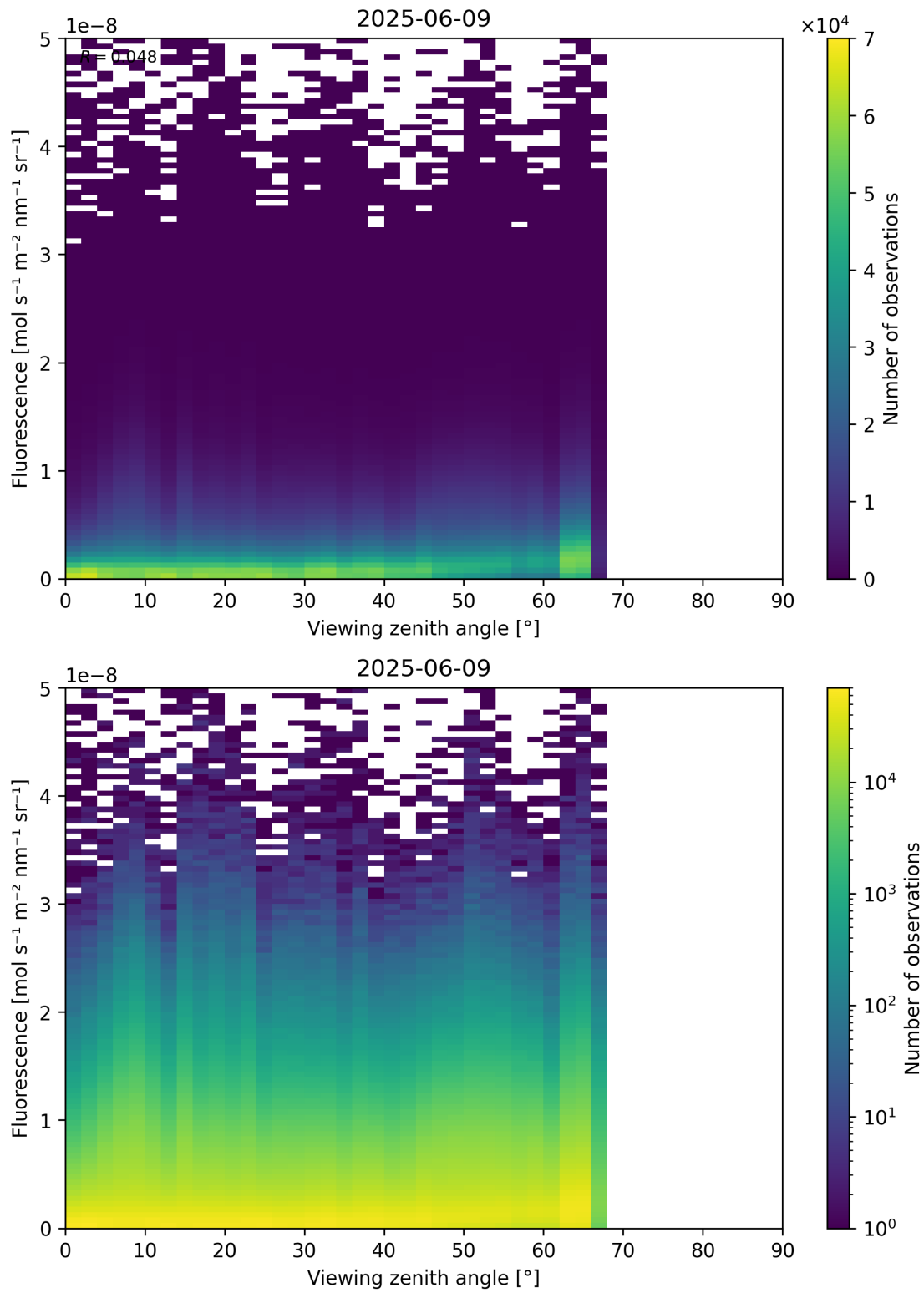
Figure 122: Scatter density plot of "Viewing zenith angle" against "Fluorescence" for 2025-06-08 to 2025-06-10.
