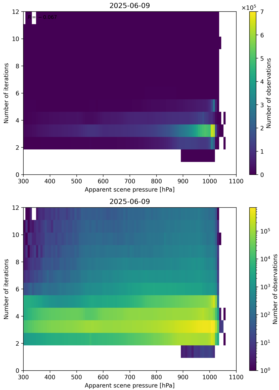
Figure 65: Scatter density plot of “Apparent scene pressure” against “Number of iterations” for 2025-06-08 to 2025-06-10.
