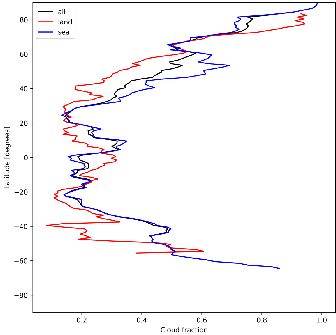
Figure 15: Zonal average of “Cloud fraction” for 2025-06-08 to 2025-06-10.
