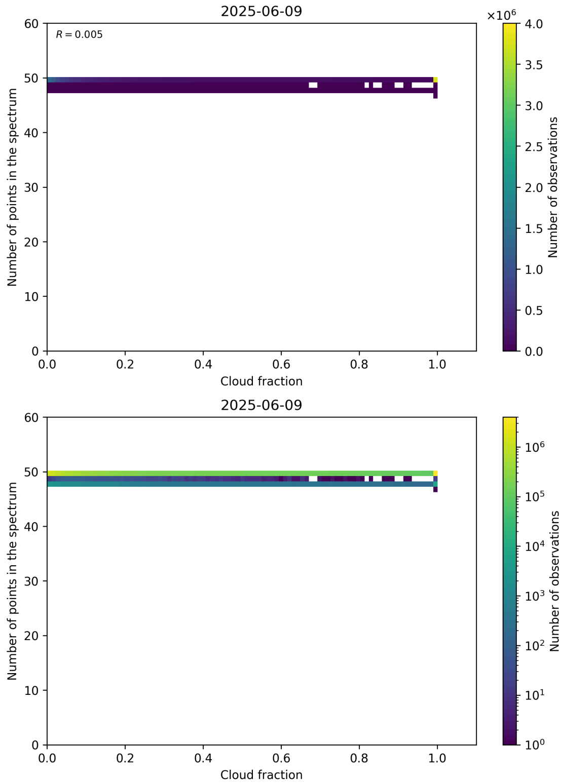
Figure 74: Scatter density plot of “Cloud fraction” against “Number of points in the spectrum” for 2025-06-08 to 2025-06-10.
