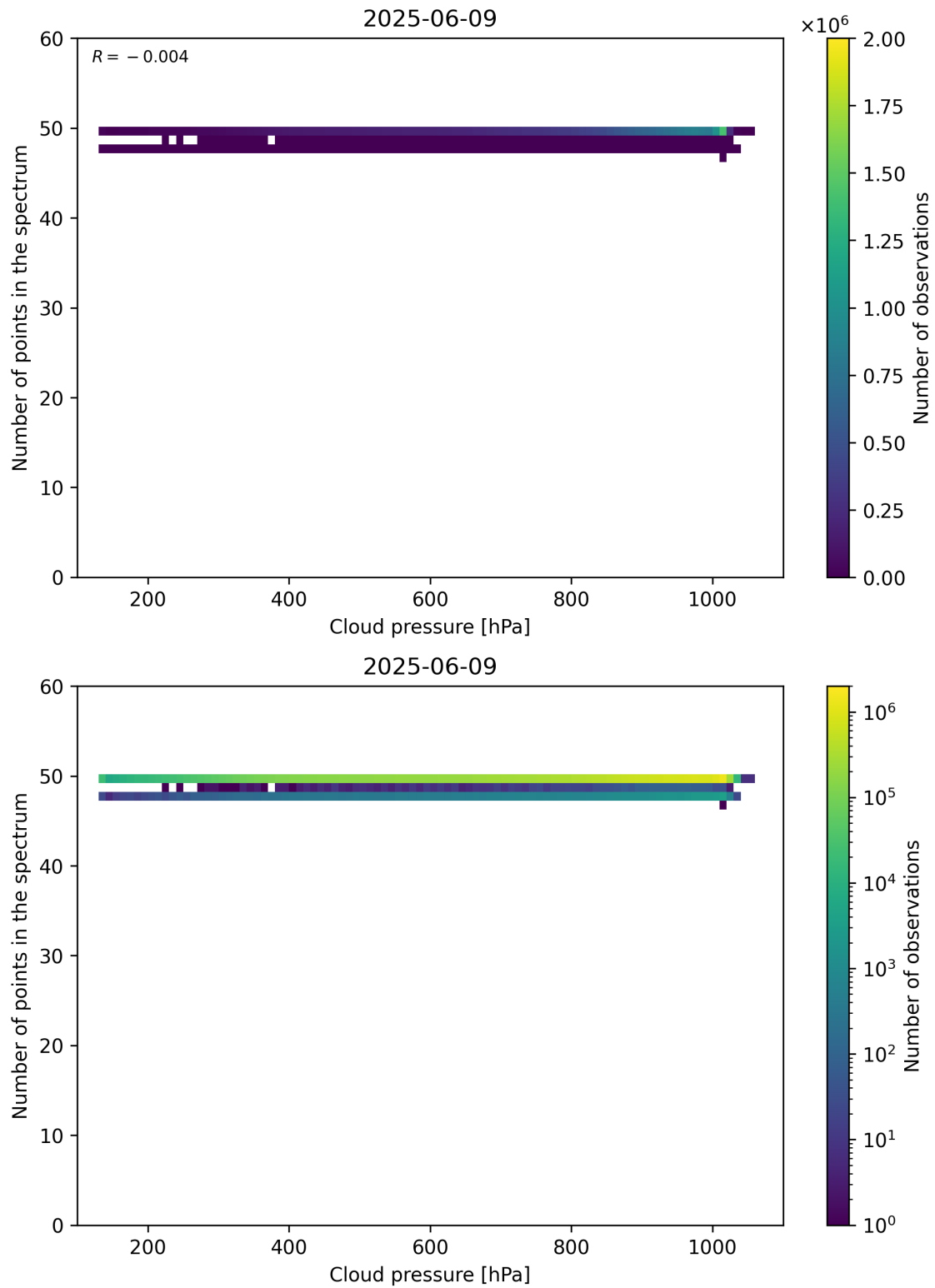
Figure 82: Scatter density plot of “Cloud pressure” against “Number of points in the spectrum” for 2025-06-08 to 2025-06-10.
