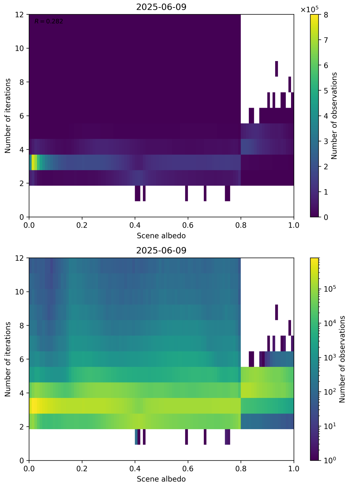
Figure 105: Scatter density plot of “Scene albedo” against “Number of iterations” for 2025-06-08 to 2025-06-10.
