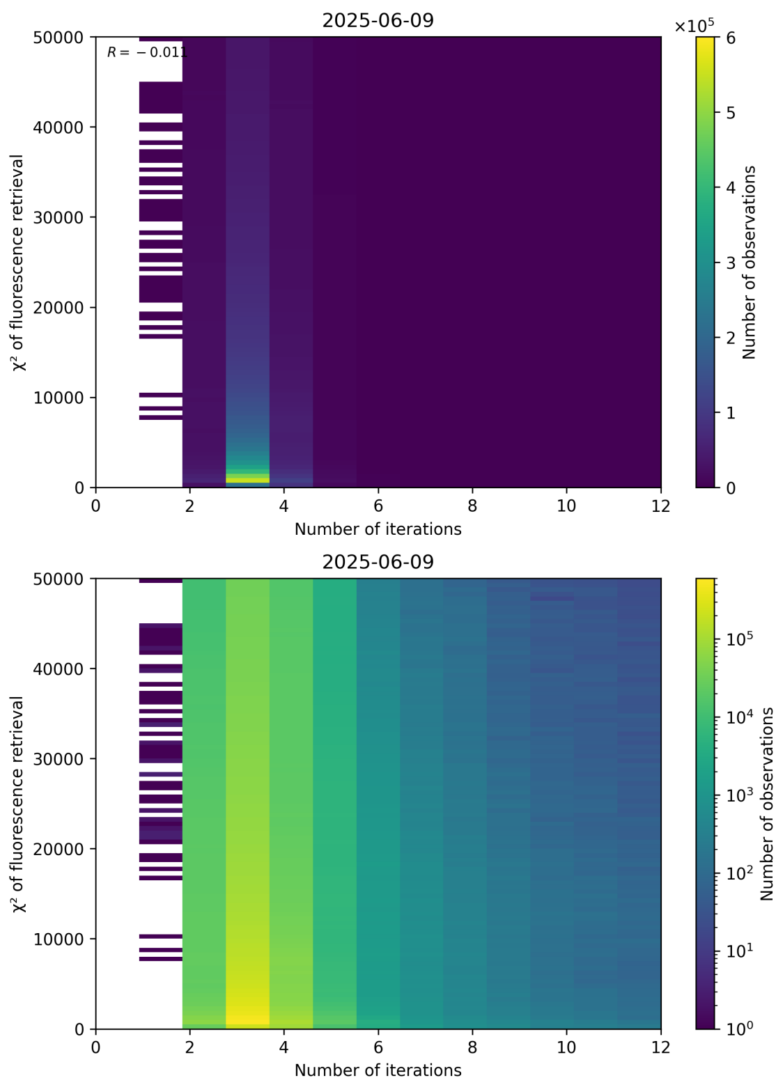
Figure 97: Scatter density plot of “Number of iterations” against “ \chi^2 of fluorescence retrieval” for 2025-06-08 to 2025-06-10.
