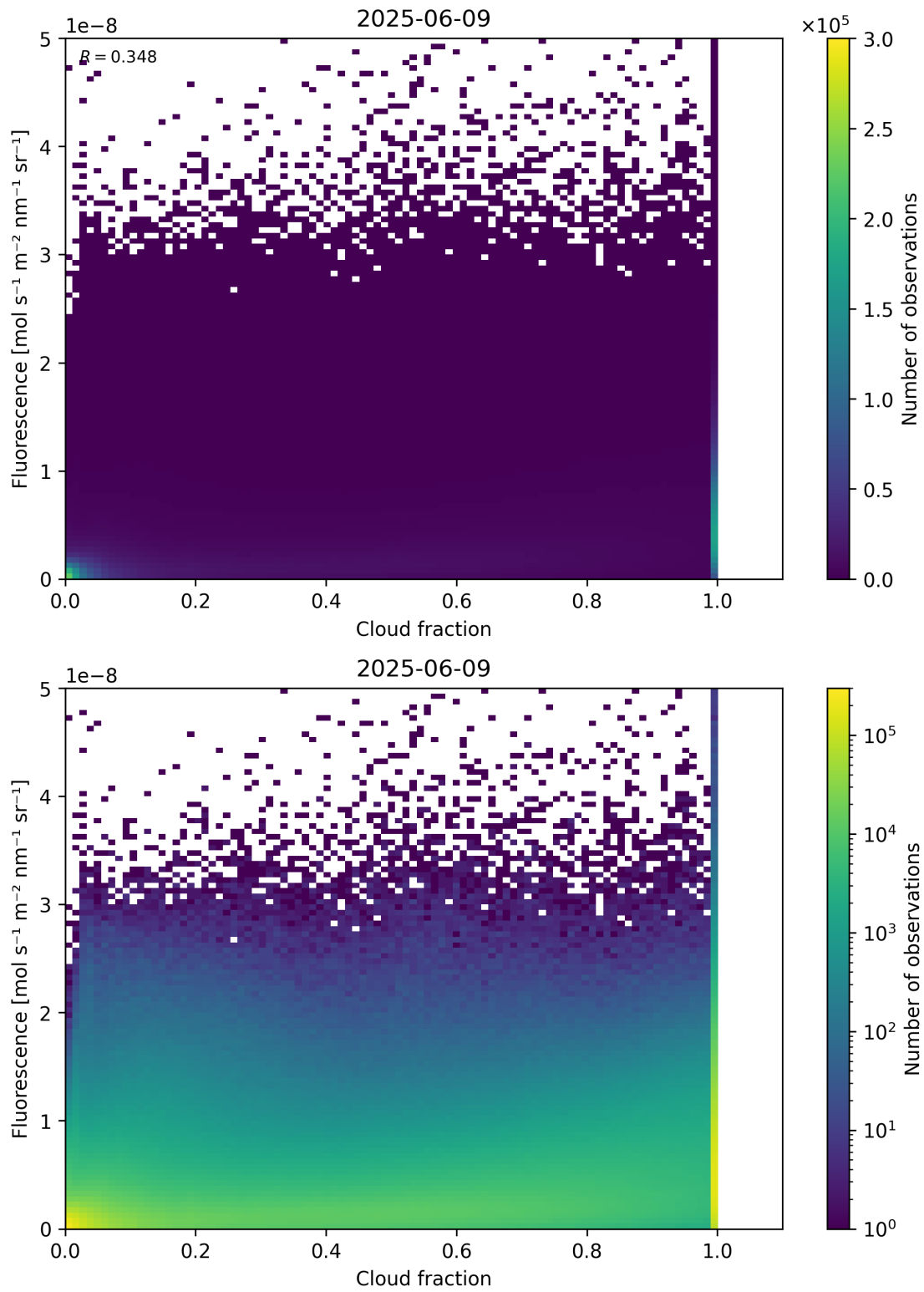
Figure 72: Scatter density plot of “Cloud fraction” against “Fluorescence” for 2025-06-08 to 2025-06-10.
