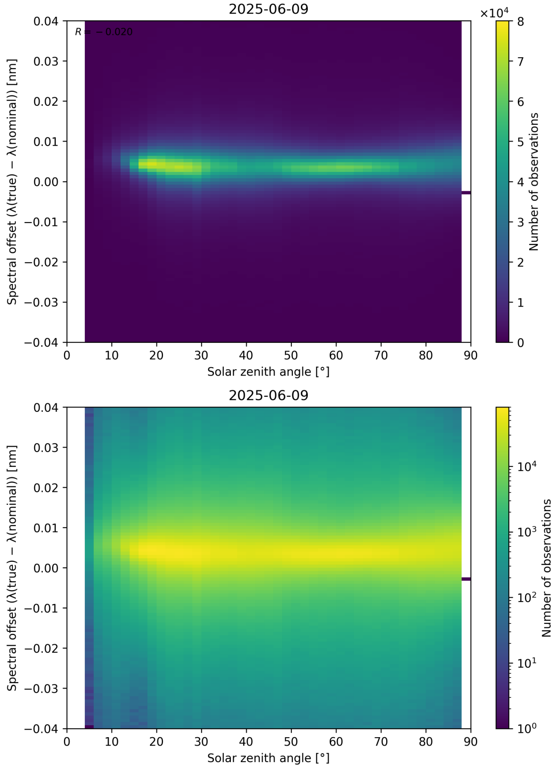
Figure 117: Scatter density plot of “Solar zenith angle” against “Spectral offset ( \lambda_{\text{true}} - \lambda_{\text{nominal}} )” for 2025-06-08 to 2025-06-10.
