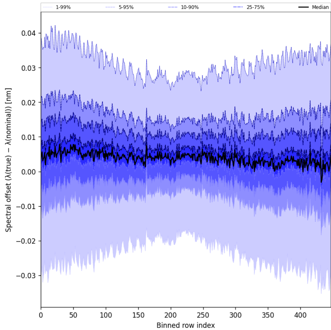
Figure 62: Along track statistics of “Spectral offset ( \lambda_{\text{true}} - \lambda_{\text{nominal}} )” for 2025-06-08 to 2025-06-10
