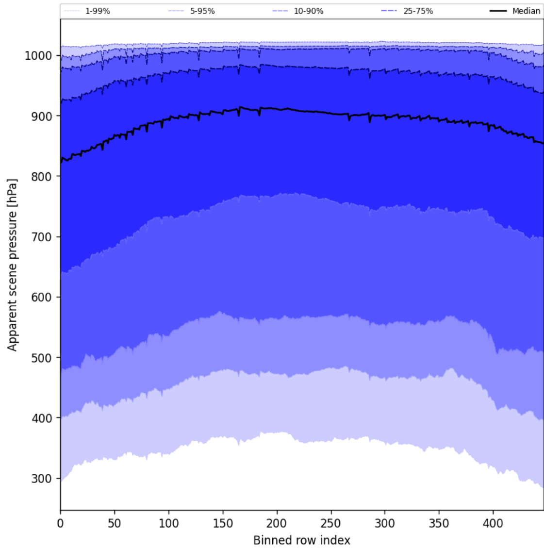
Figure 53: Along track statistics of “Apparent scene pressure” for 2025-06-08 to 2025-06-10
