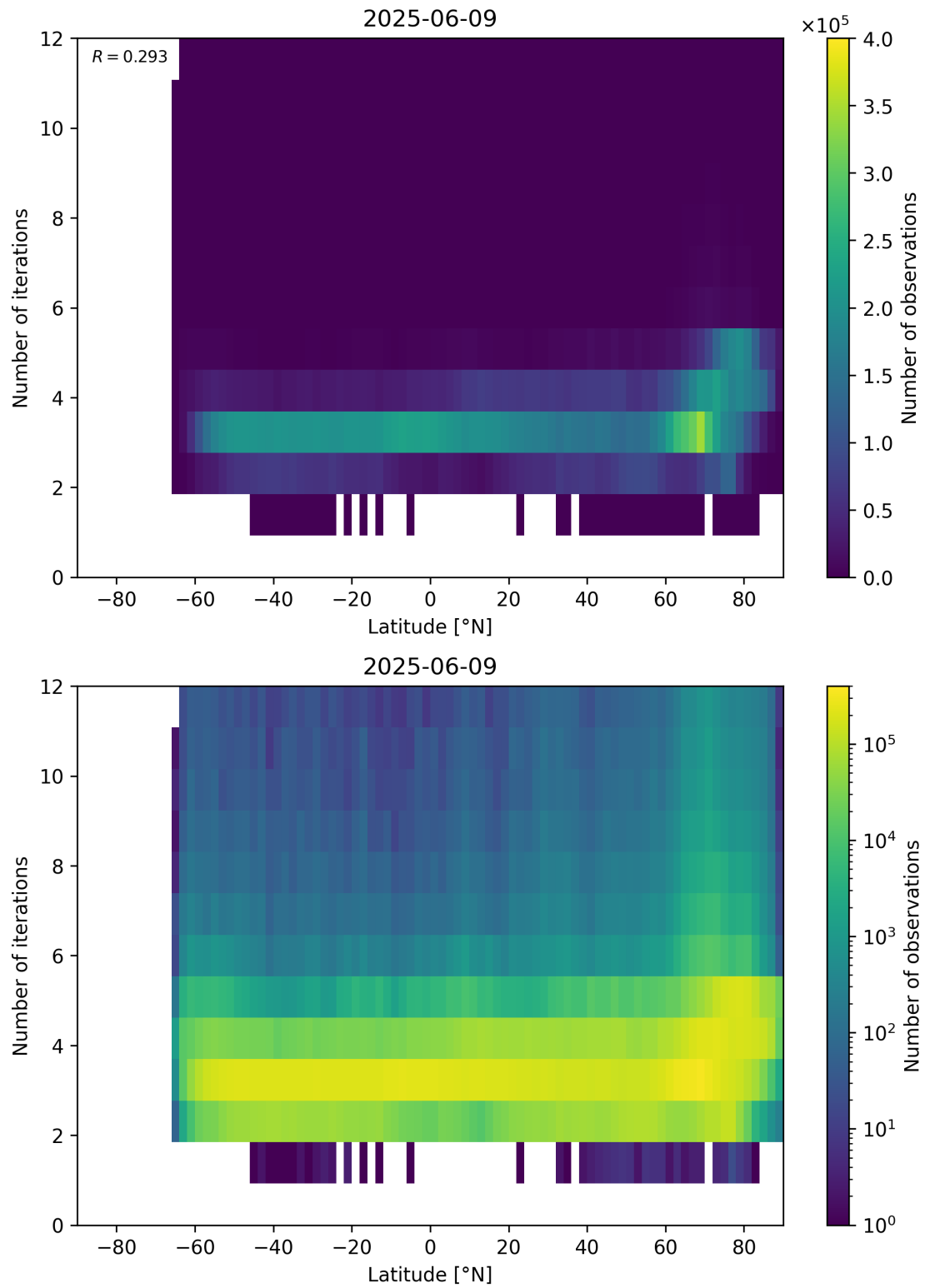
Figure 93: Scatter density plot of “Latitude” against “Number of iterations” for 2025-06-08 to 2025-06-10.
