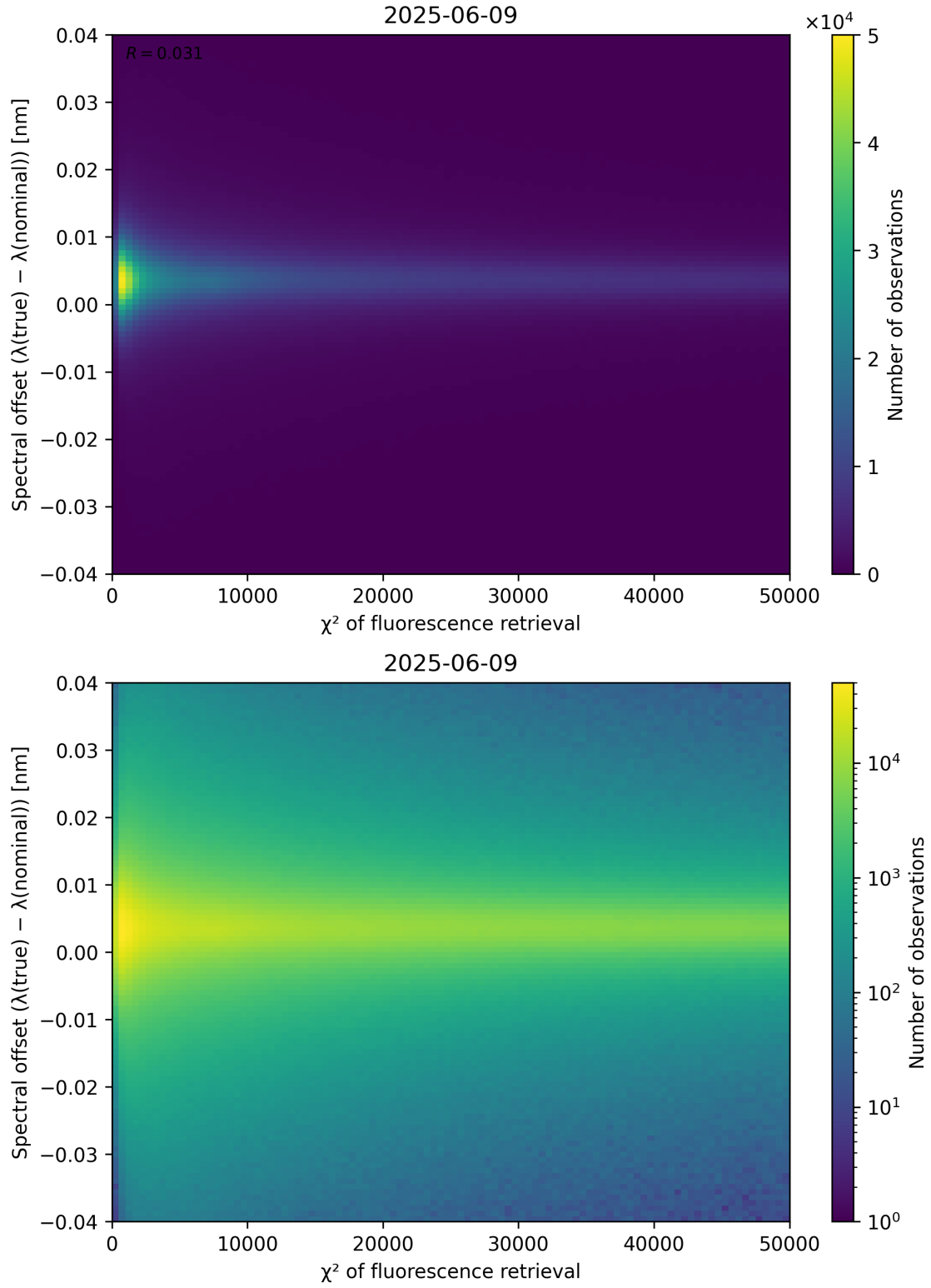
Figure 69: Scatter density plot of “ \chi^2 of fluorescence retrieval” against “Spectral offset ( \lambda_{\text{true}} - \lambda_{\text{nominal}} )” for 2025-06-08 to 2025-06-10.
