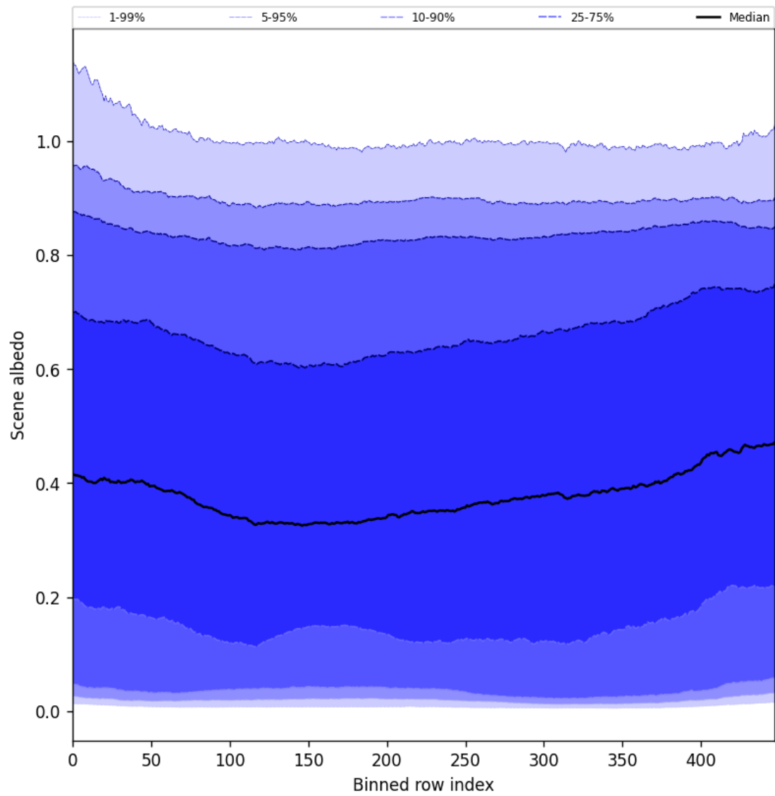
Figure 51: Along track statistics of “Scene albedo” for 2025-06-08 to 2025-06-10
