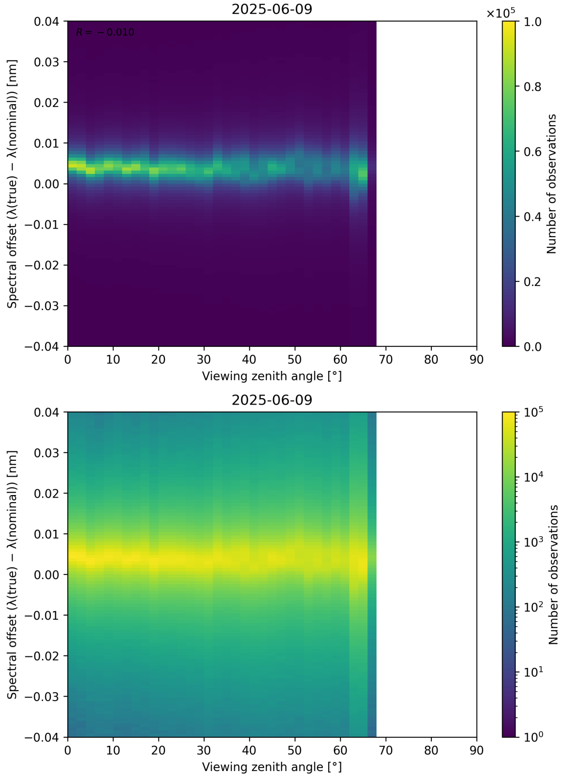
Figure 128: Scatter density plot of “Viewing zenith angle” against “Spectral offset ( \lambda_{\text{true}} - \lambda_{\text{nominal}} )” for 2025-06-08 to 2025-06-10.
