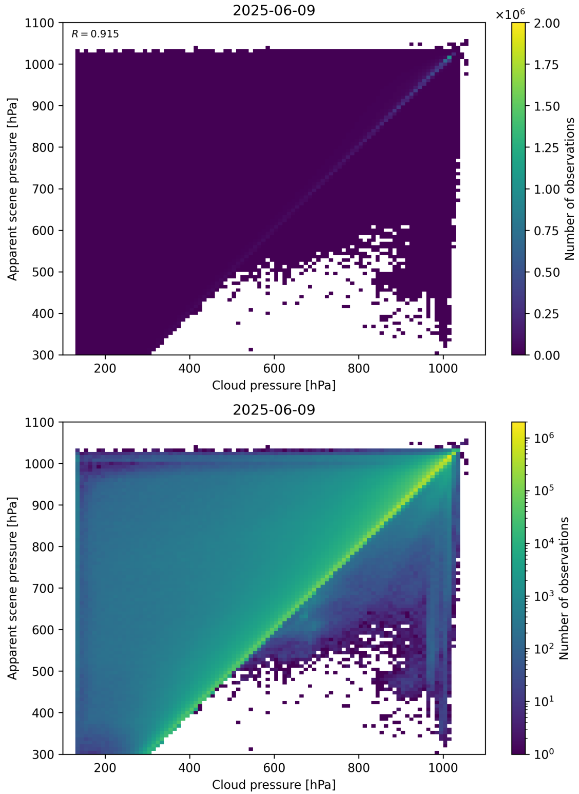
Figure 77: Scatter density plot of “Cloud pressure” against “Apparent scene pressure” for 2025-06-08 to 2025-06-10.
