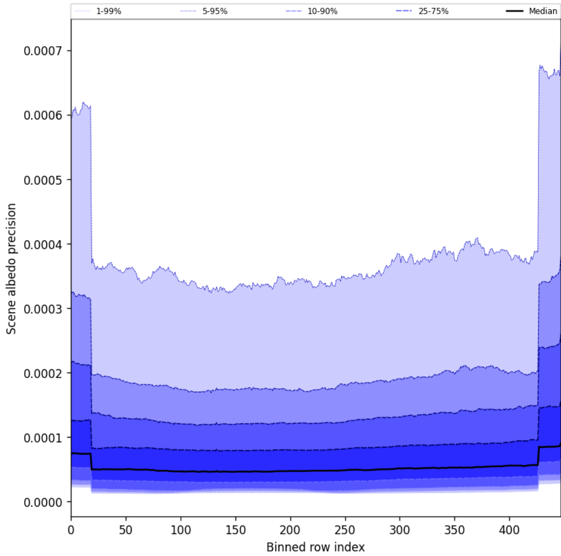
Figure 52: Along track statistics of “Scene albedo precision” for 2025-06-08 to 2025-06-10
