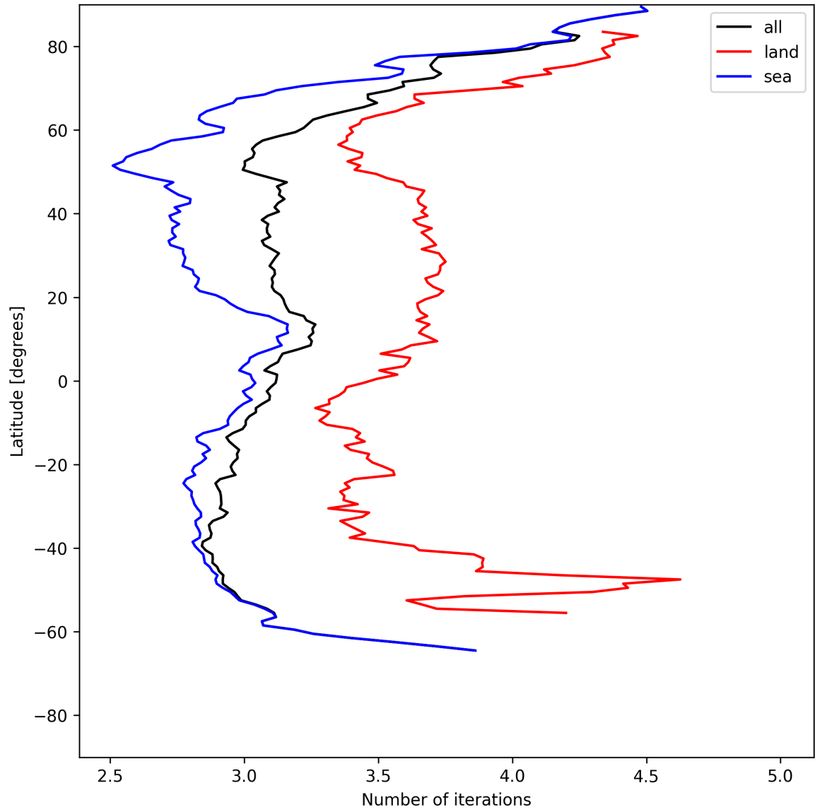
Figure 22: Zonal average of “Number of iterations” for 2025-06-08 to 2025-06-10.
