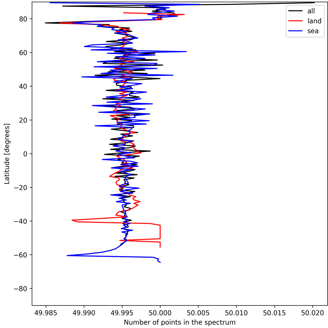
Figure 27: Zonal average of “Number of points in the spectrum” for 2025-06-08 to 2025-06-10.
