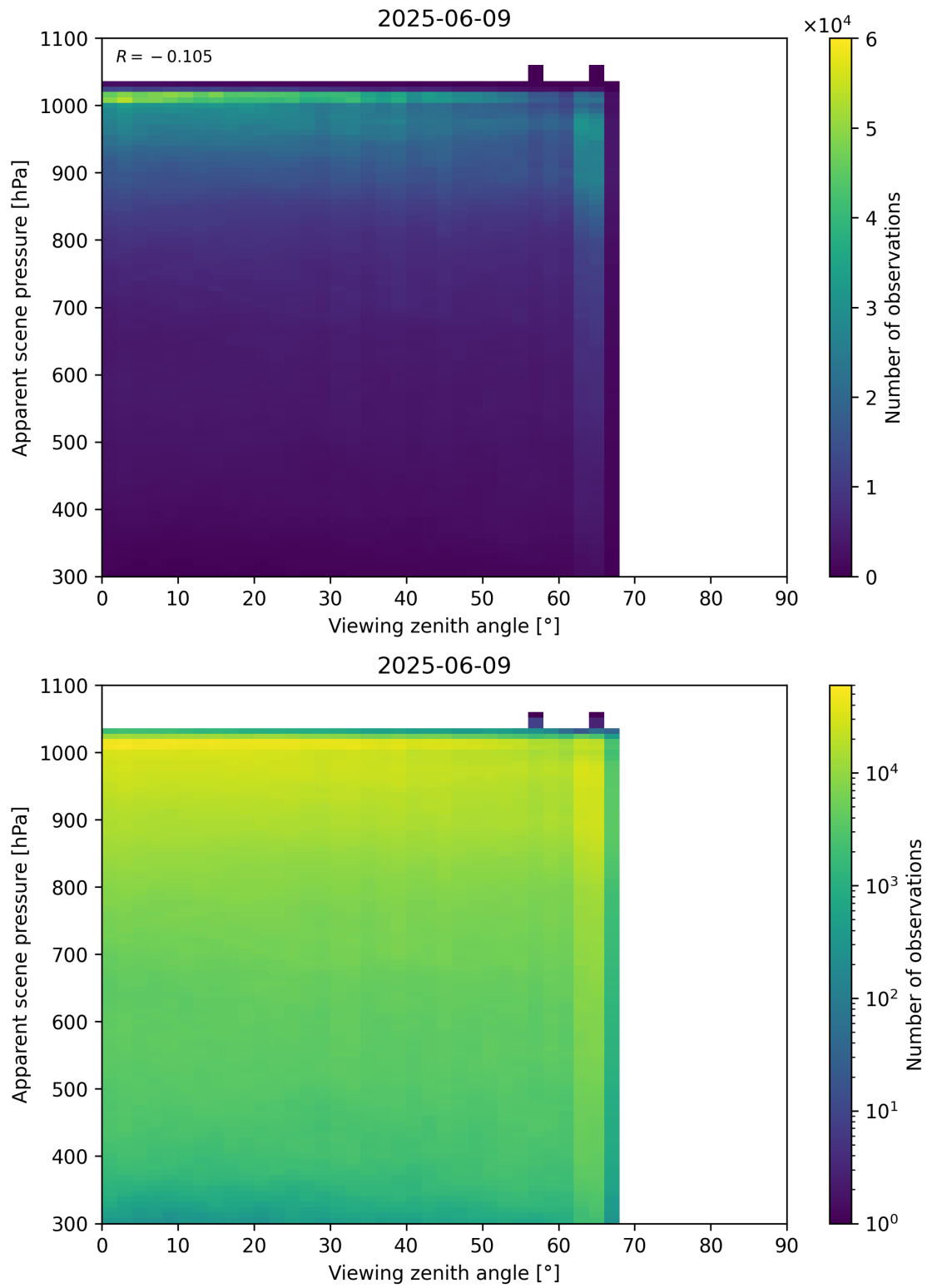
Figure 118: Scatter density plot of “Viewing zenith angle” against “Apparent scene pressure” for 2025-06-08 to 2025-06-10.
