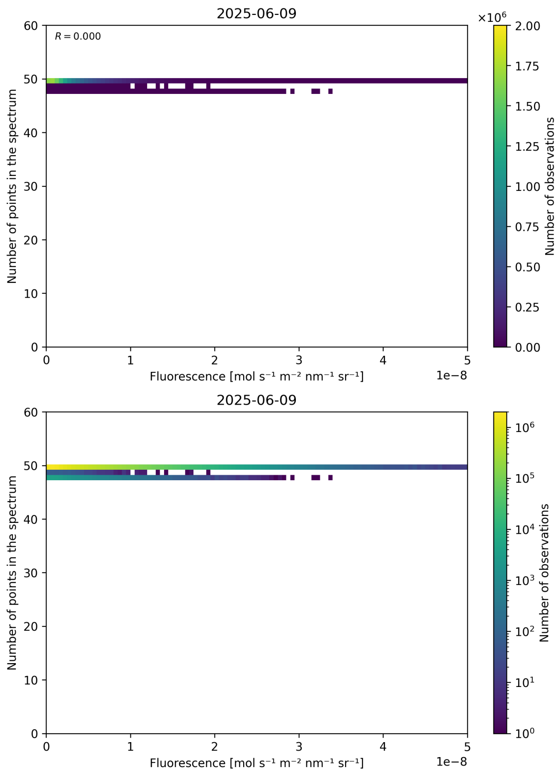
Figure 86: Scatter density plot of “Fluorescence” against “Number of points in the spectrum” for 2025-06-08 to 2025-06-10.
