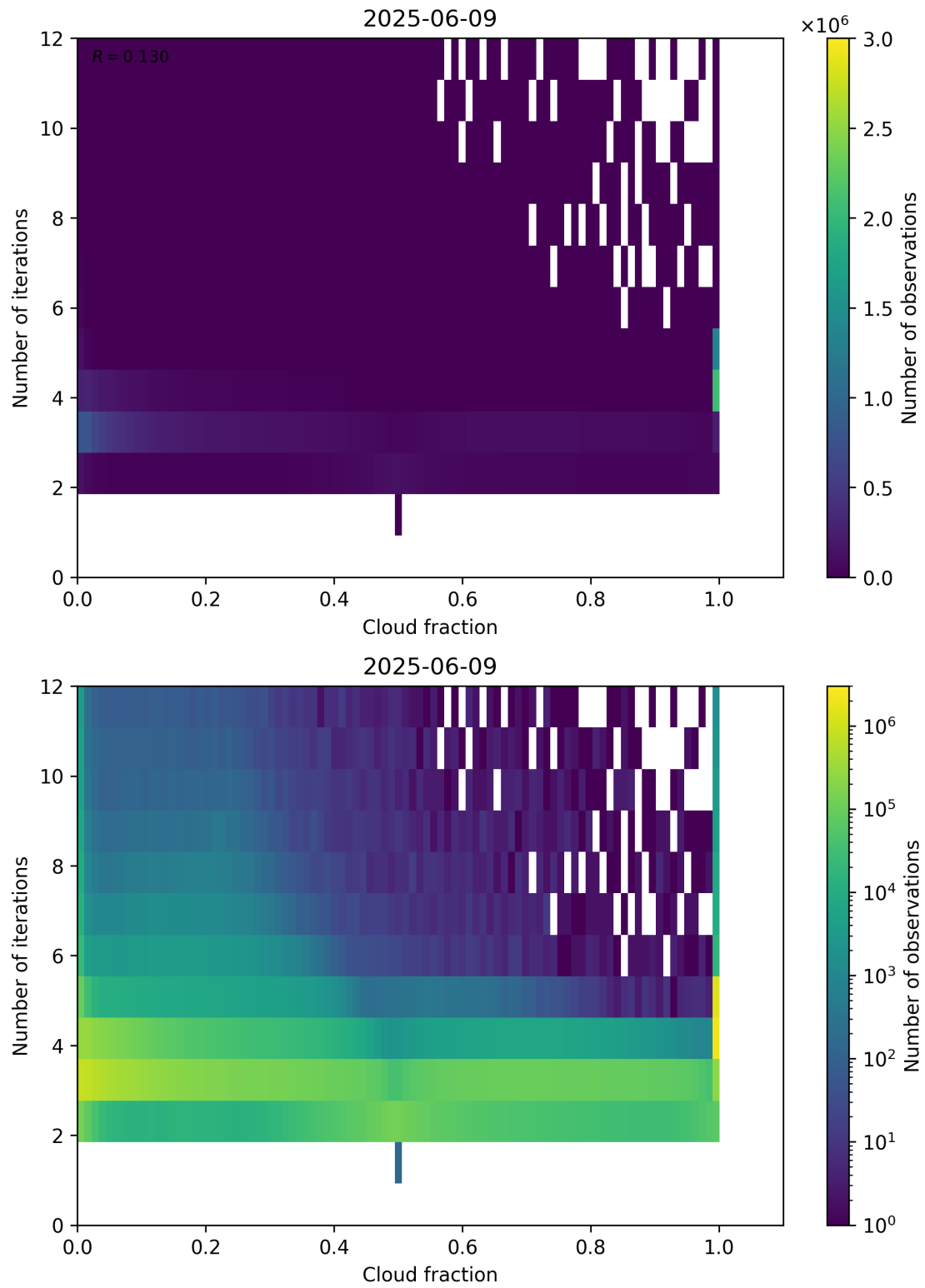
Figure 73: Scatter density plot of “Cloud fraction” against “Number of iterations” for 2025-06-08 to 2025-06-10.
