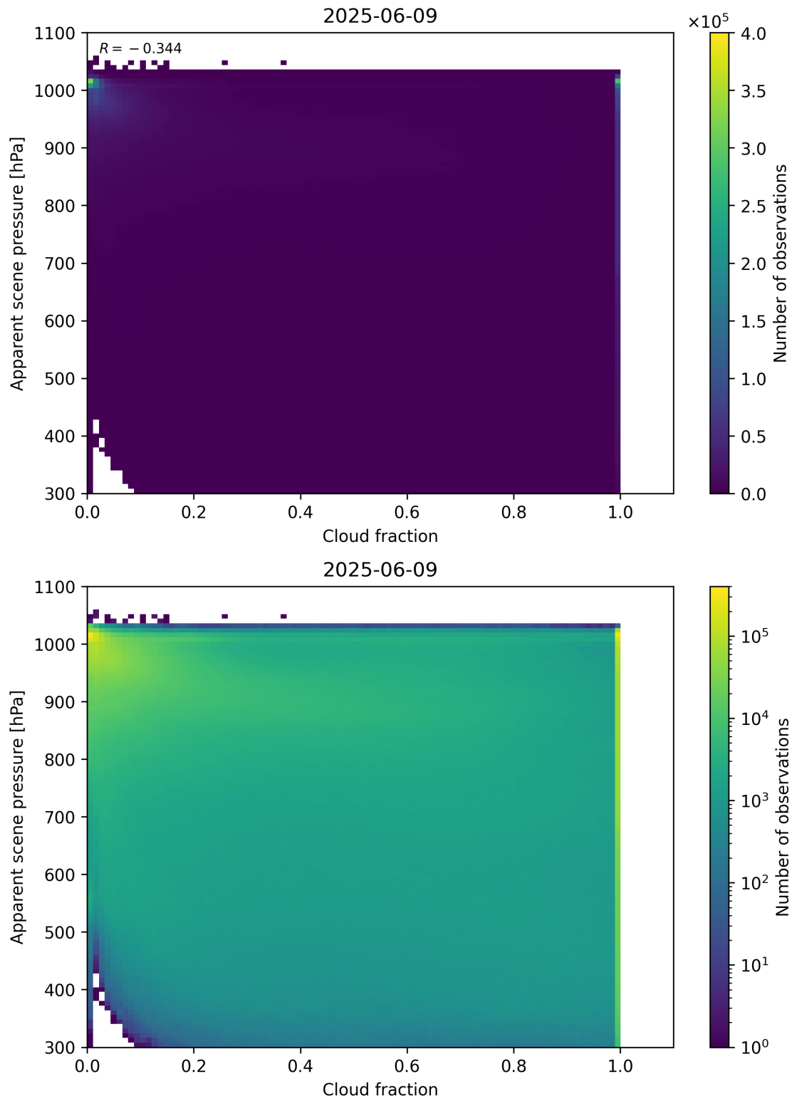
Figure 70: Scatter density plot of “Cloud fraction” against “Apparent scene pressure” for 2025-06-08 to 2025-06-10.
