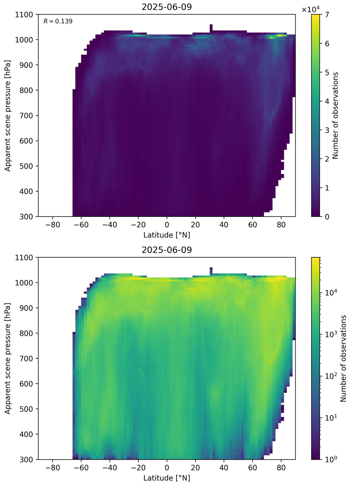
Figure 88: Scatter density plot of “Latitude” against “Apparent scene pressure” for 2025-06-08 to 2025-06-10.
