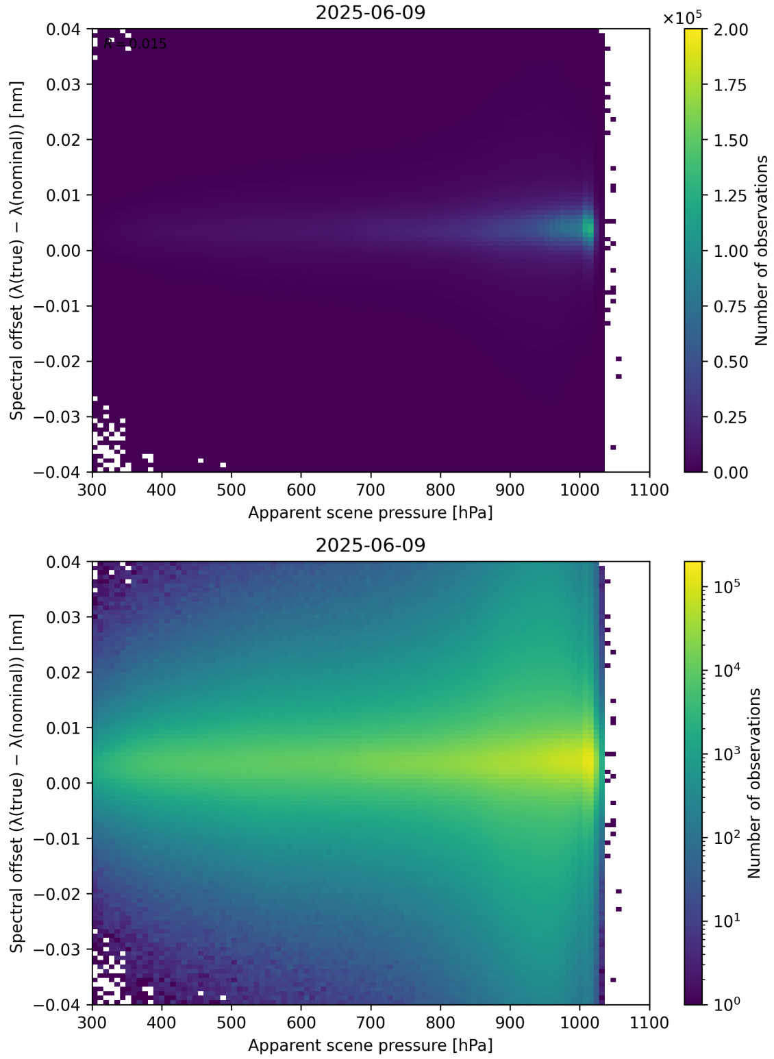
Figure 67: Scatter density plot of “Apparent scene pressure” against “Spectral offset ( \lambda_{\text{true}} - \lambda_{\text{nominal}} )” for 2025-06-08 to 2025-06-10.
