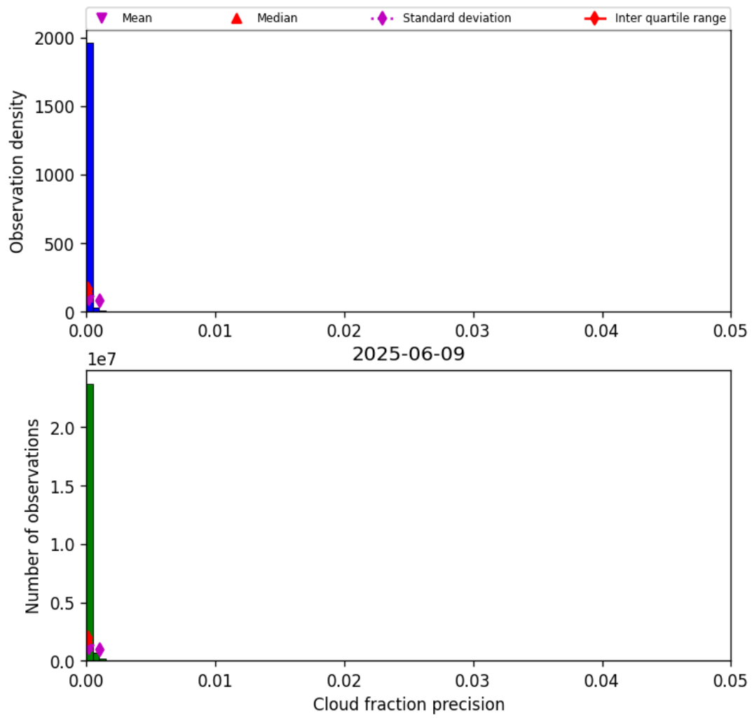
Figure 33: Histogram of “Cloud fraction precision” for 2025-06-08 to 2025-06-10
