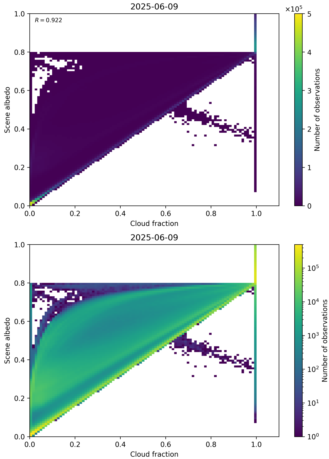
Figure 75: Scatter density plot of “Cloud fraction” against “Scene albedo” for 2025-06-08 to 2025-06-10.
