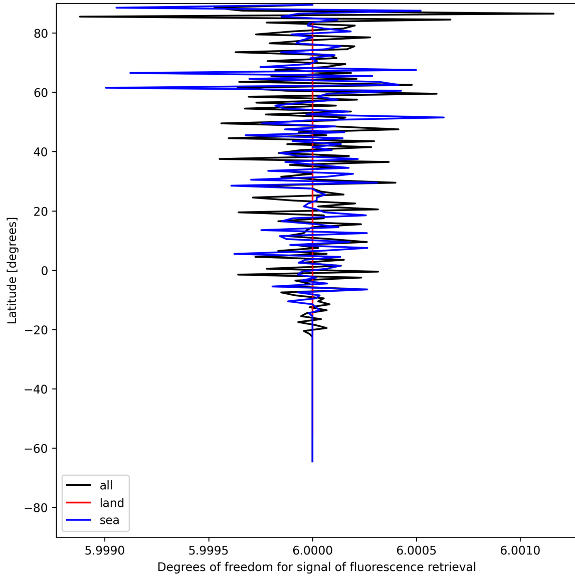
Figure 26: Zonal average of “Degrees of freedom for signal of fluorescence retrieval” for 2025-06-08 to 2025-06-10.
