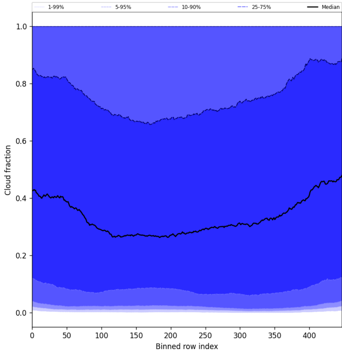
Figure 49: Along track statistics of “Cloud fraction” for 2025-06-08 to 2025-06-10
