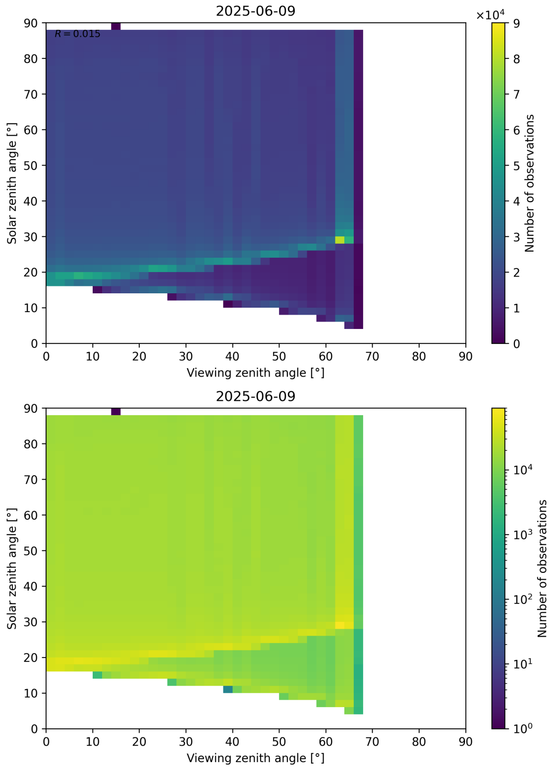
Figure 127: Scatter density plot of “Viewing zenith angle” against “Solar zenith angle” for 2025-06-08 to 2025-06-10.
