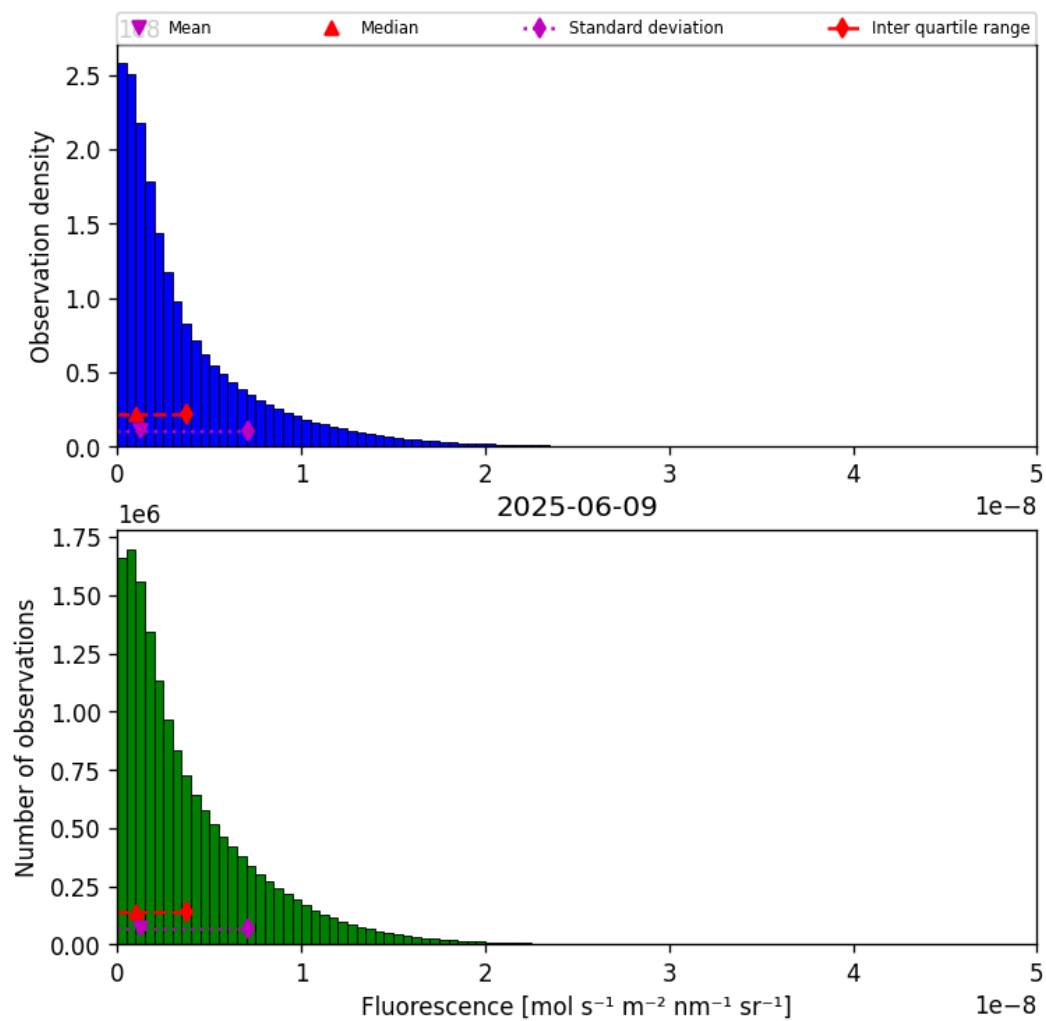
Figure 40: Histogram of “Fluorescence” for 2025-06-08 to 2025-06-10
