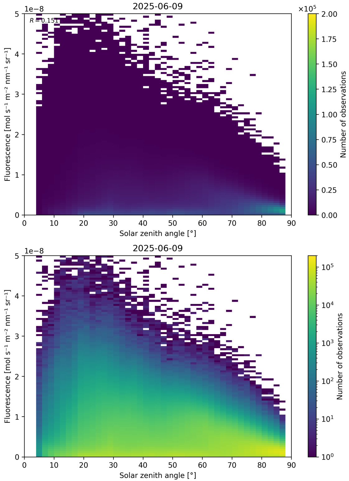
Figure 112: Scatter density plot of “Solar zenith angle” against “Fluorescence” for 2025-06-08 to 2025-06-10.
