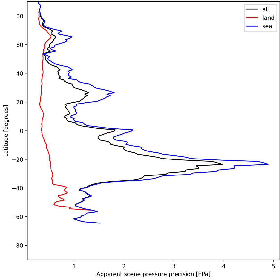
Figure 20: Zonal average of “Apparent scene pressure precision” for 2025-06-08 to 2025-06-10.
