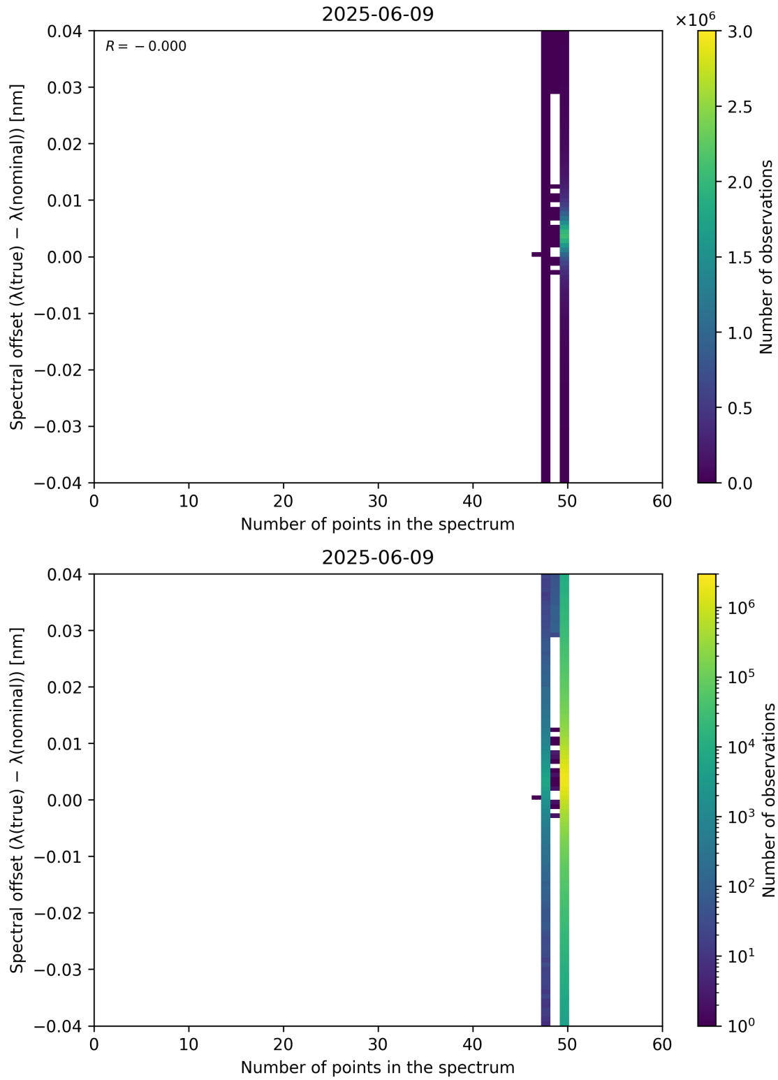
Figure 101: Scatter density plot of “Number of points in the spectrum” against “Spectral offset ( \lambda_{\text{true}} - \lambda_{\text{nominal}} )” for 2025-06-08 to 2025-06-10.
