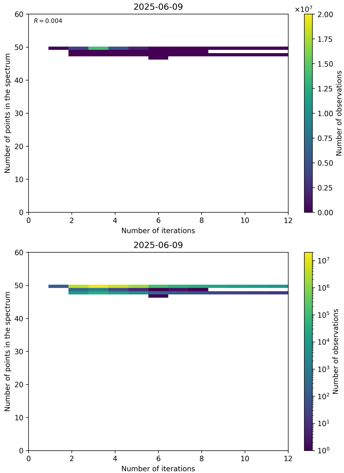
Figure 99: Scatter density plot of “Number of iterations” against “Number of points in the spectrum” for 2025-06-08 to 2025-06-10.
