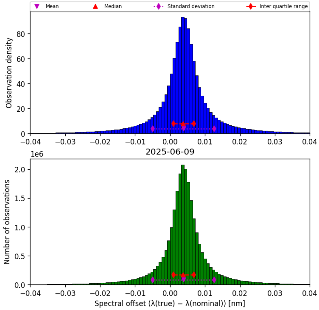
Figure 45: Histogram of “Spectral offset ( \lambda_{\text{true}} - \lambda_{\text{nominal}} )” for 2025-06-08 to 2025-06-10
