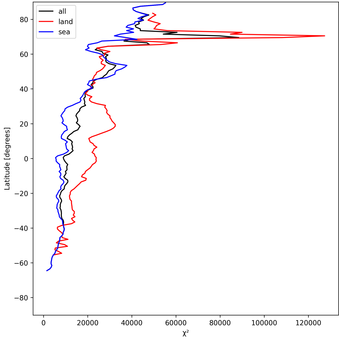
Figure 21: Zonal average of “ \chi^2 ” for 2025-06-08 to 2025-06-10.
