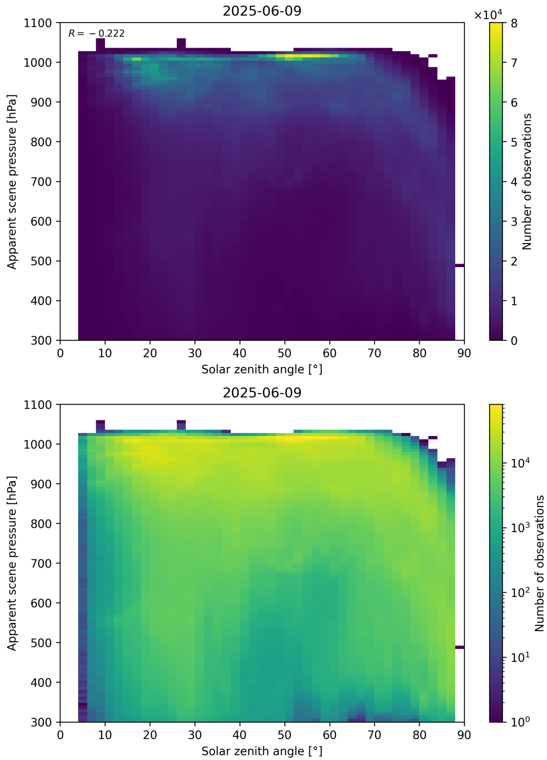
Figure 108: Scatter density plot of “Solar zenith angle” against “Apparent scene pressure” for 2025-06-08 to 2025-06-10.
