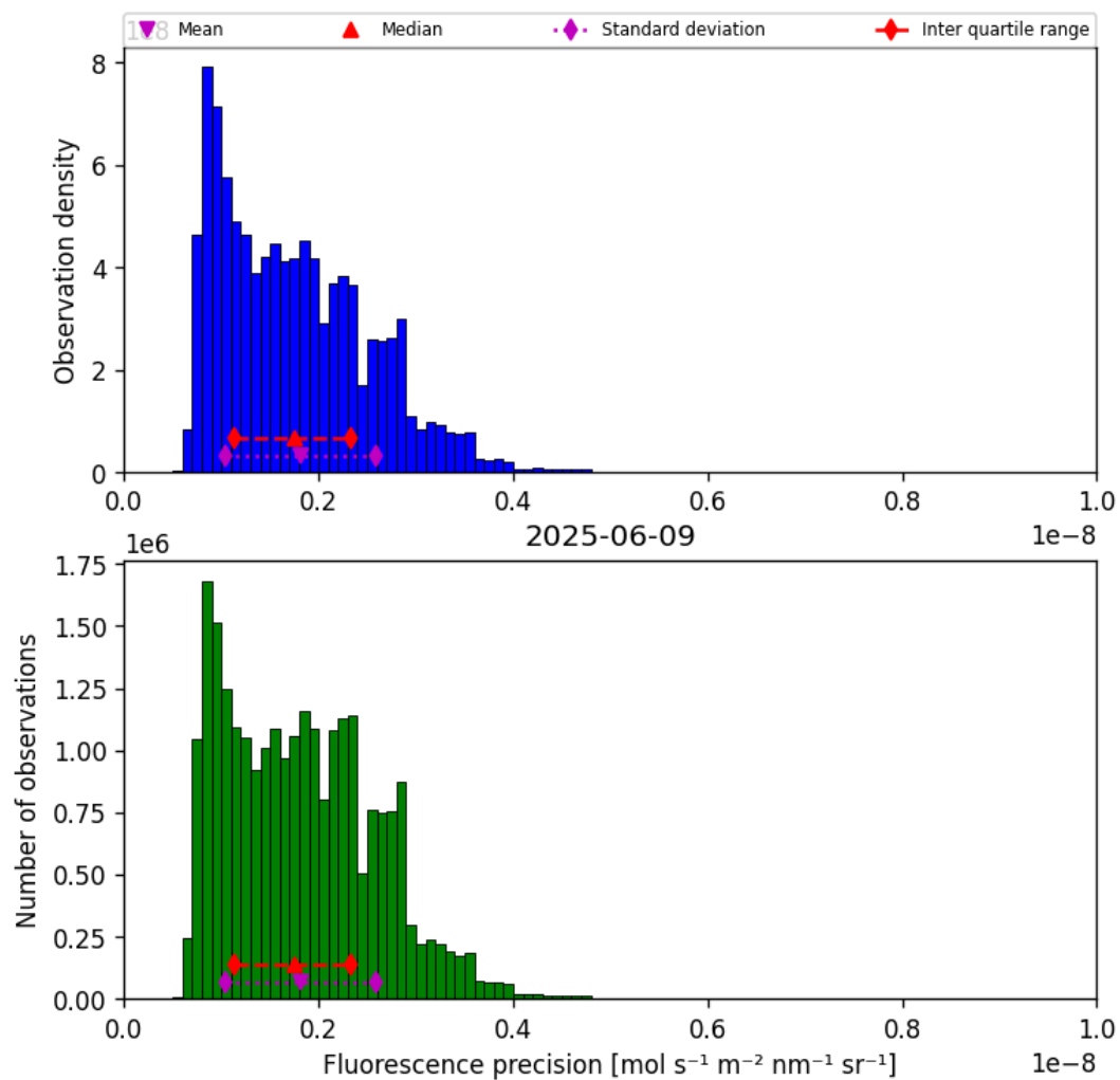
Figure 41: Histogram of “Fluorescence precision” for 2025-06-08 to 2025-06-10
