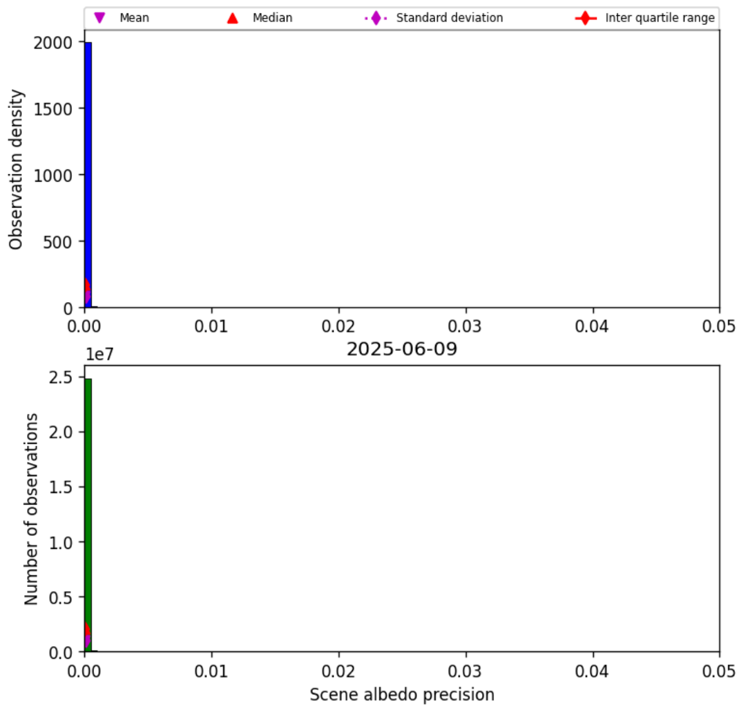
Figure 35: Histogram of “Scene albedo precision” for 2025-06-08 to 2025-06-10
