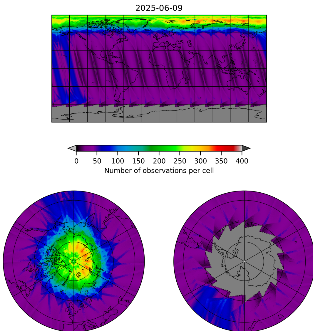
Figure 11: Map of the number of observations for 2025-06-08 to 2025-06-10
