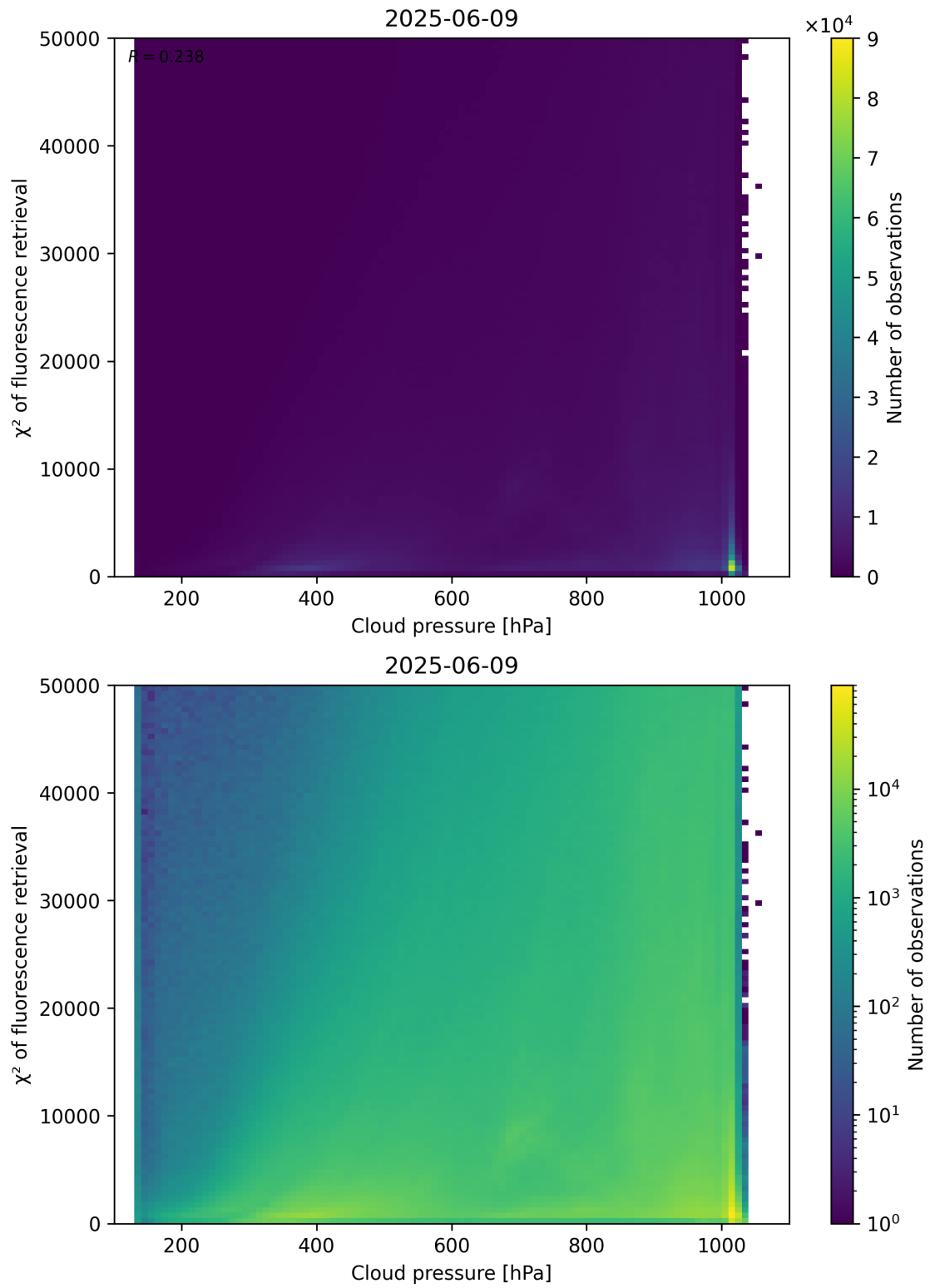
Figure 78: Scatter density plot of “Cloud pressure” against “ \chi^2 of fluorescence retrieval” for 2025-06-08 to 2025-06-10.
