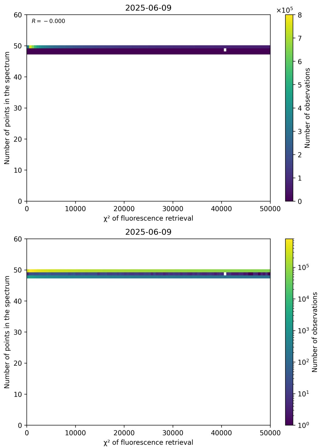
Figure 68: Scatter density plot of “ \chi^2 of fluorescence retrieval” against “Number of points in the spectrum” for 2025-06-08 to 2025-06-10.
