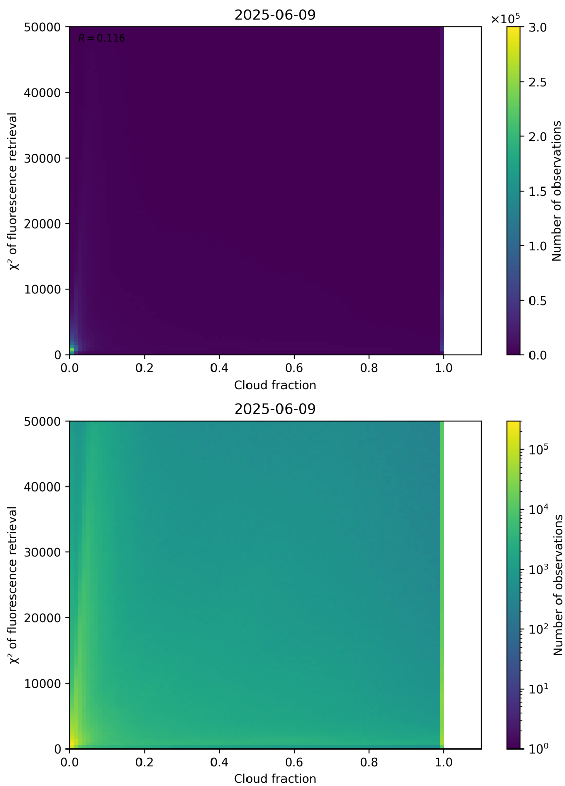
Figure 71: Scatter density plot of “Cloud fraction” against “ \chi^2 of fluorescence retrieval” for 2025-06-08 to 2025-06-10.
