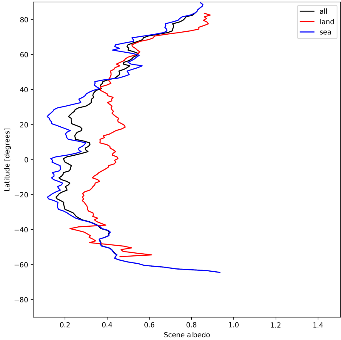
Figure 17: Zonal average of “Scene albedo” for 2025-06-08 to 2025-06-10.
