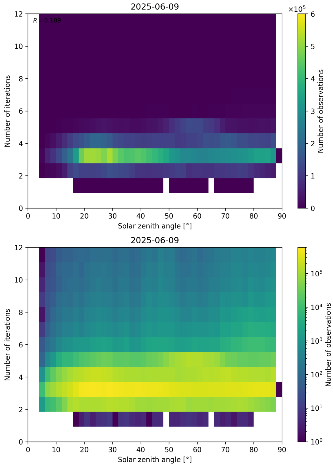
Figure 114: Scatter density plot of “Solar zenith angle” against “Number of iterations” for 2025-06-08 to 2025-06-10.
