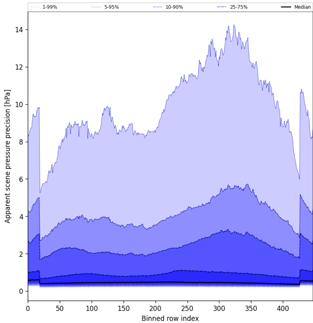
Figure 54: Along track statistics of “Apparent scene pressure precision” for 2025-06-09 to 2025-06-11
