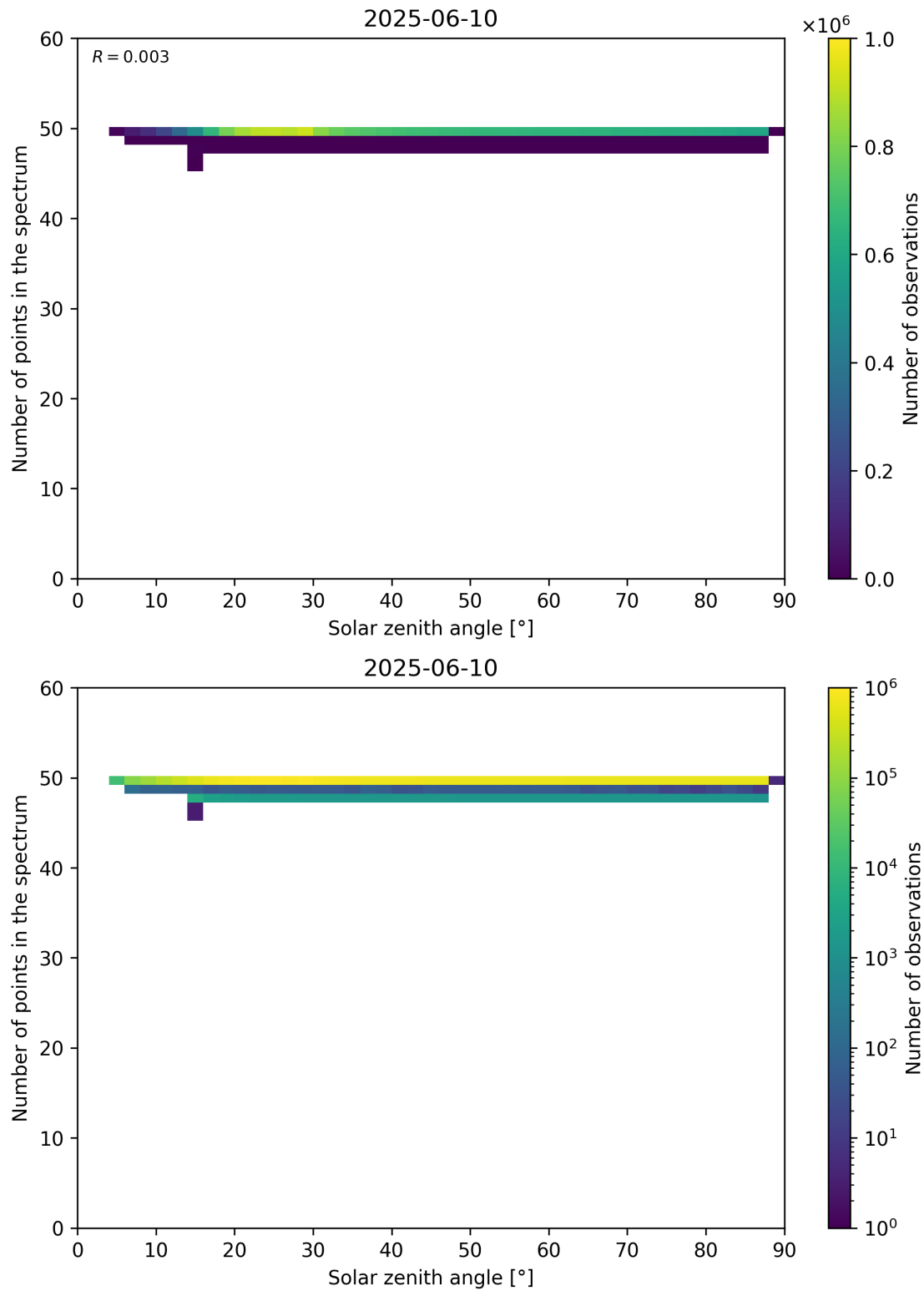
Figure 115: Scatter density plot of “Solar zenith angle” against “Number of points in the spectrum” for 2025-06-09 to 2025-06-11.
