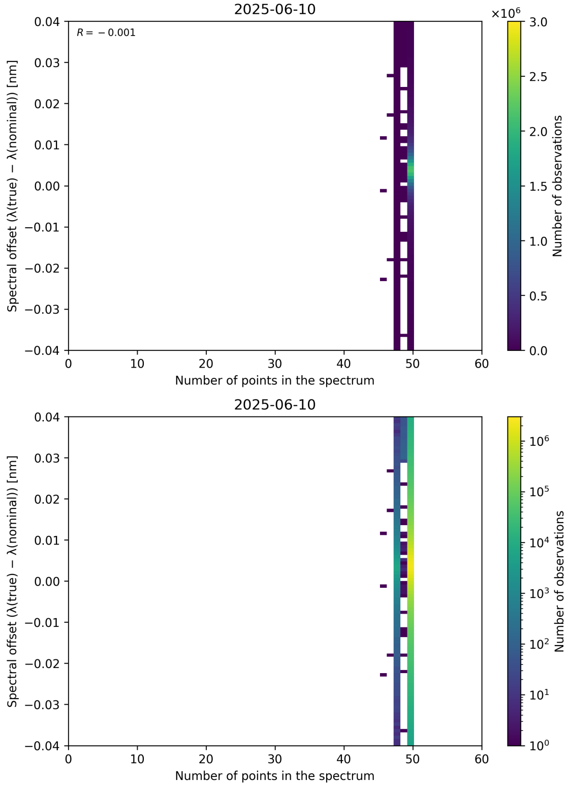
Figure 101: Scatter density plot of “Number of points in the spectrum” against “Spectral offset ( \lambda_{\text{true}} - \lambda_{\text{nominal}} )” for 2025-06-09 to 2025-06-11.
