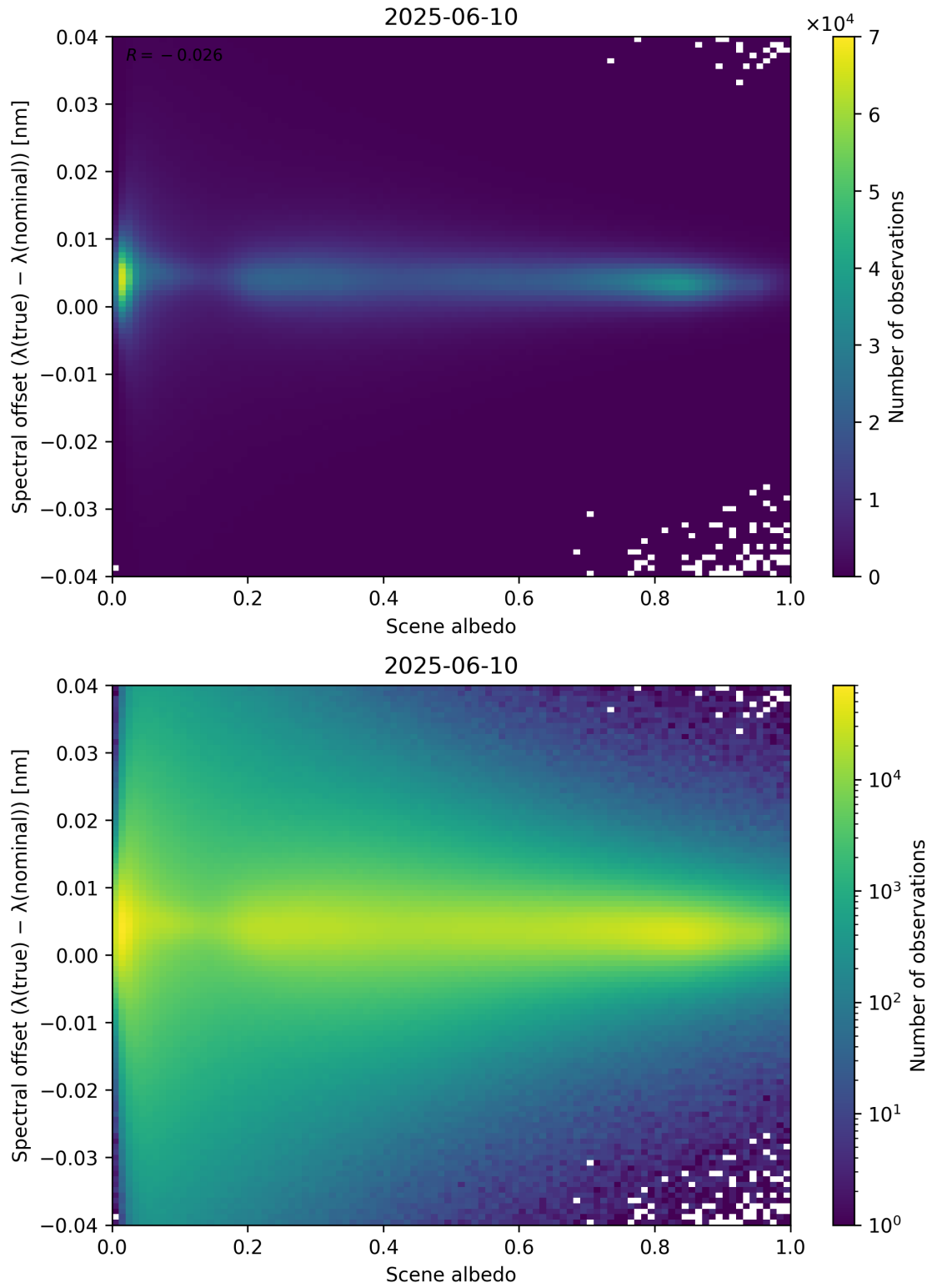
Figure 107: Scatter density plot of “Scene albedo” against “Spectral offset ( \lambda_{\text{true}} - \lambda_{\text{nominal}} )” for 2025-06-09 to 2025-06-11.
