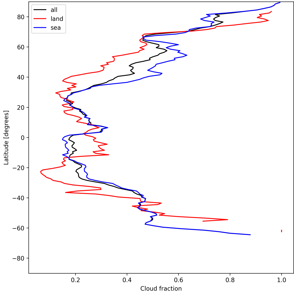
Figure 15: Zonal average of “Cloud fraction” for 2025-06-09 to 2025-06-11.
