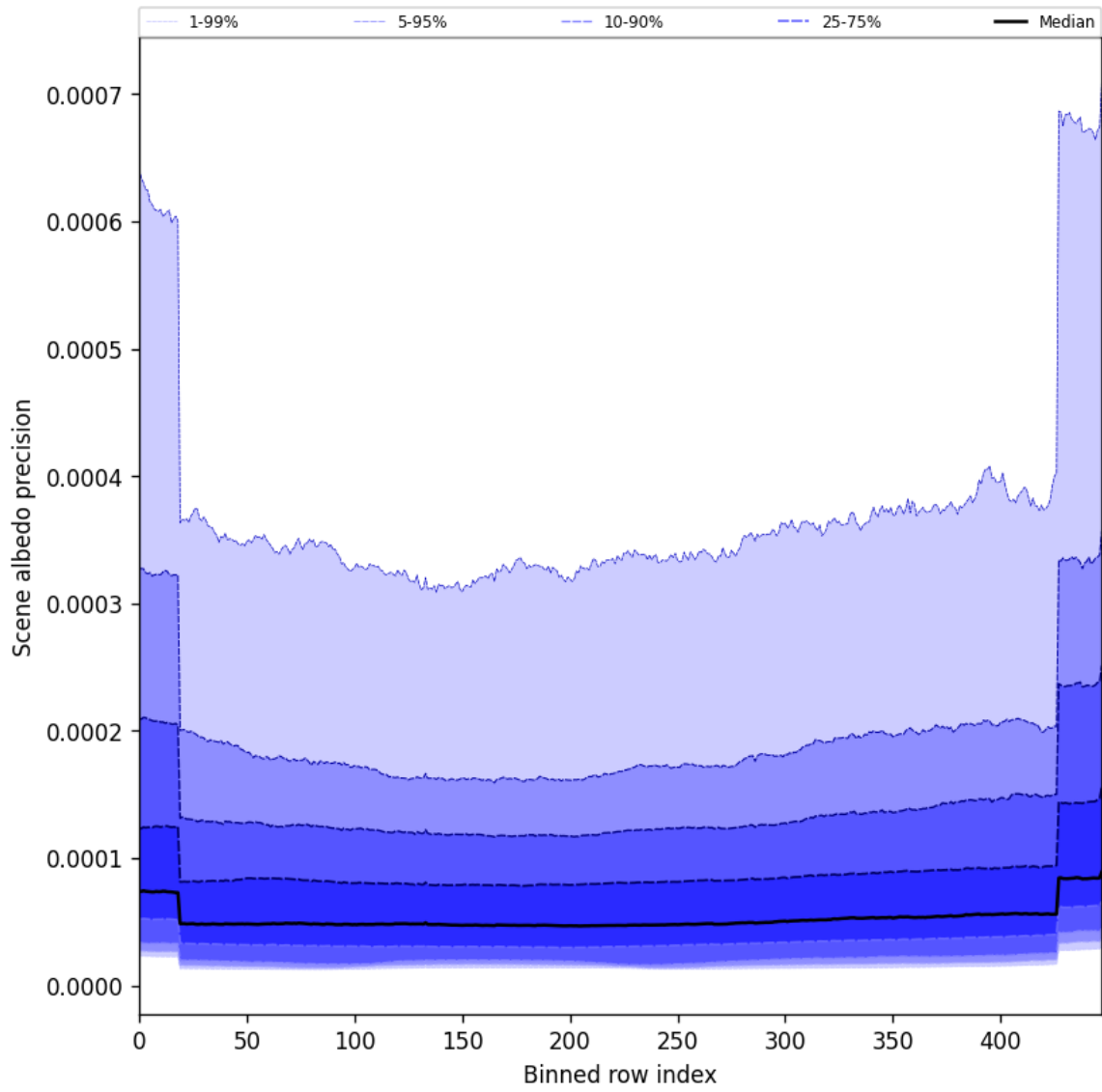
Figure 52: Along track statistics of “Scene albedo precision” for 2025-06-09 to 2025-06-11
