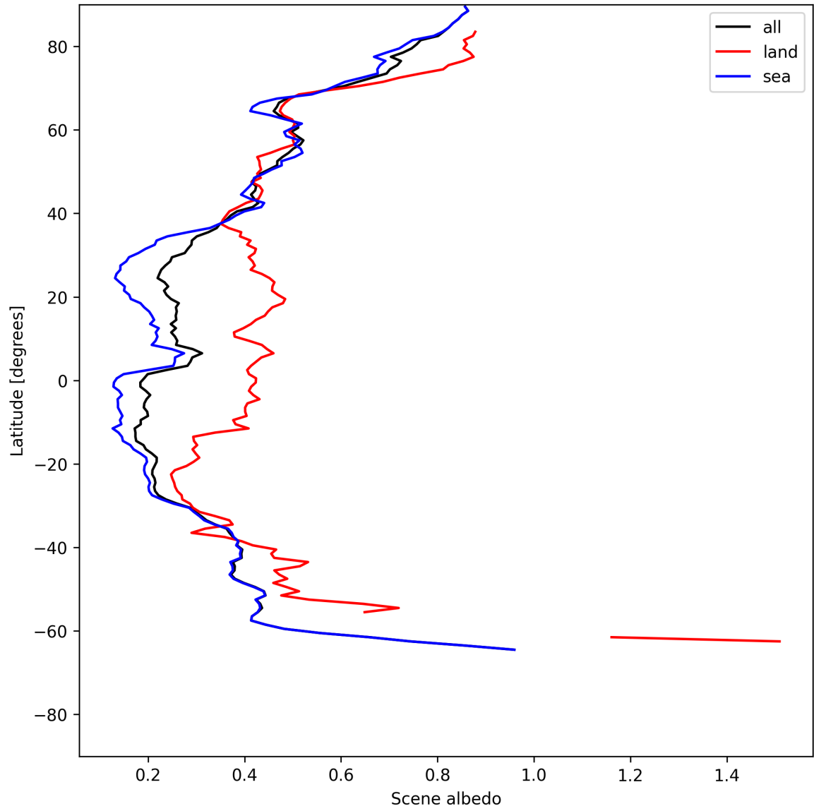
Figure 17: Zonal average of “Scene albedo” for 2025-06-09 to 2025-06-11.
