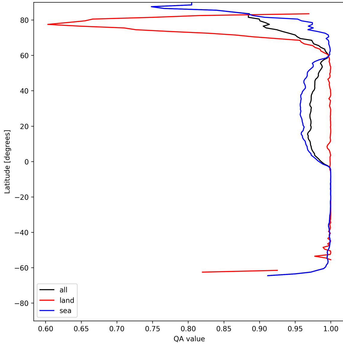
Figure 12: Zonal average of “QA value” for 2025-06-09 to 2025-06-11.
