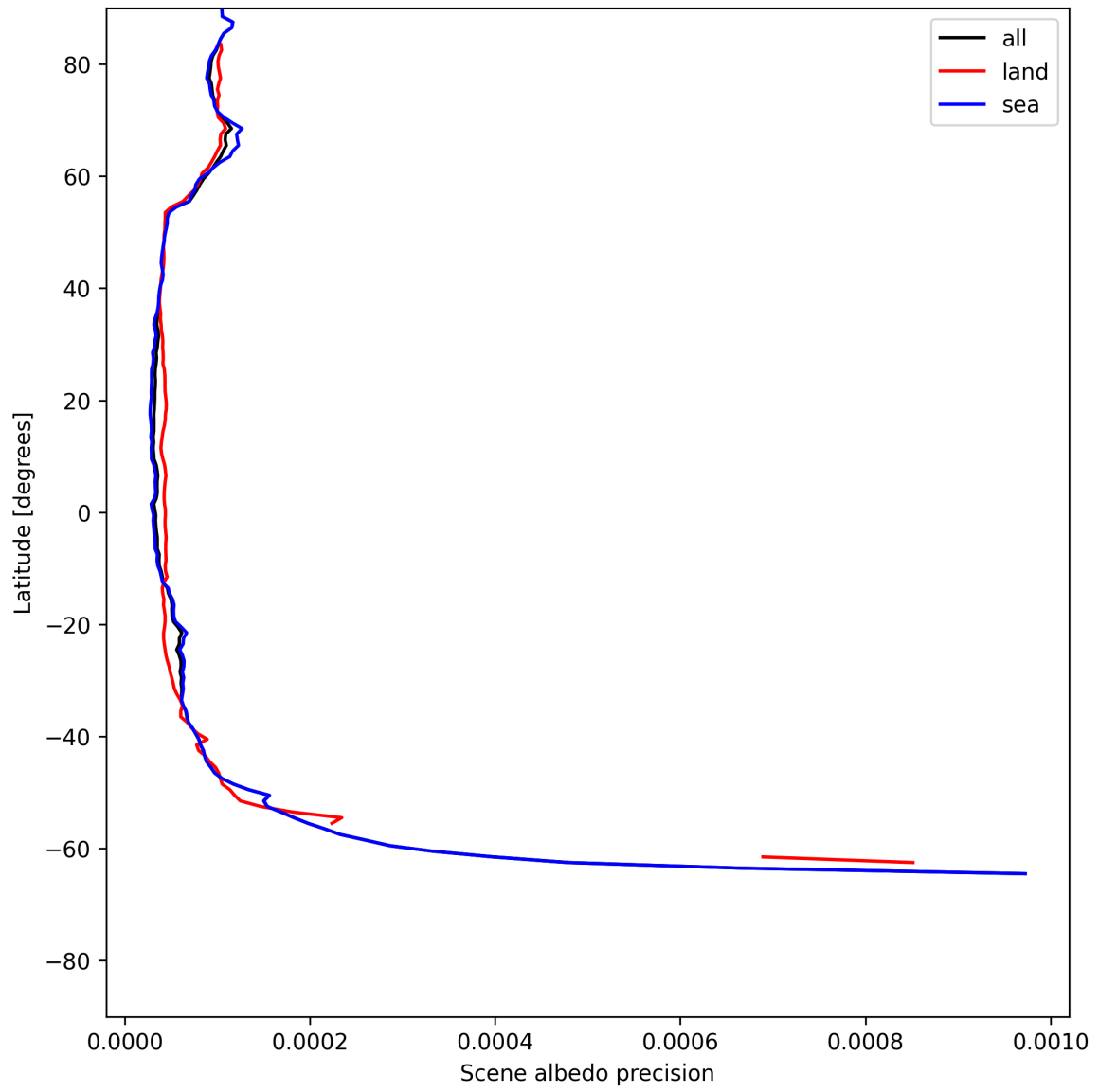
Figure 18: Zonal average of “Scene albedo precision” for 2025-06-09 to 2025-06-11.
