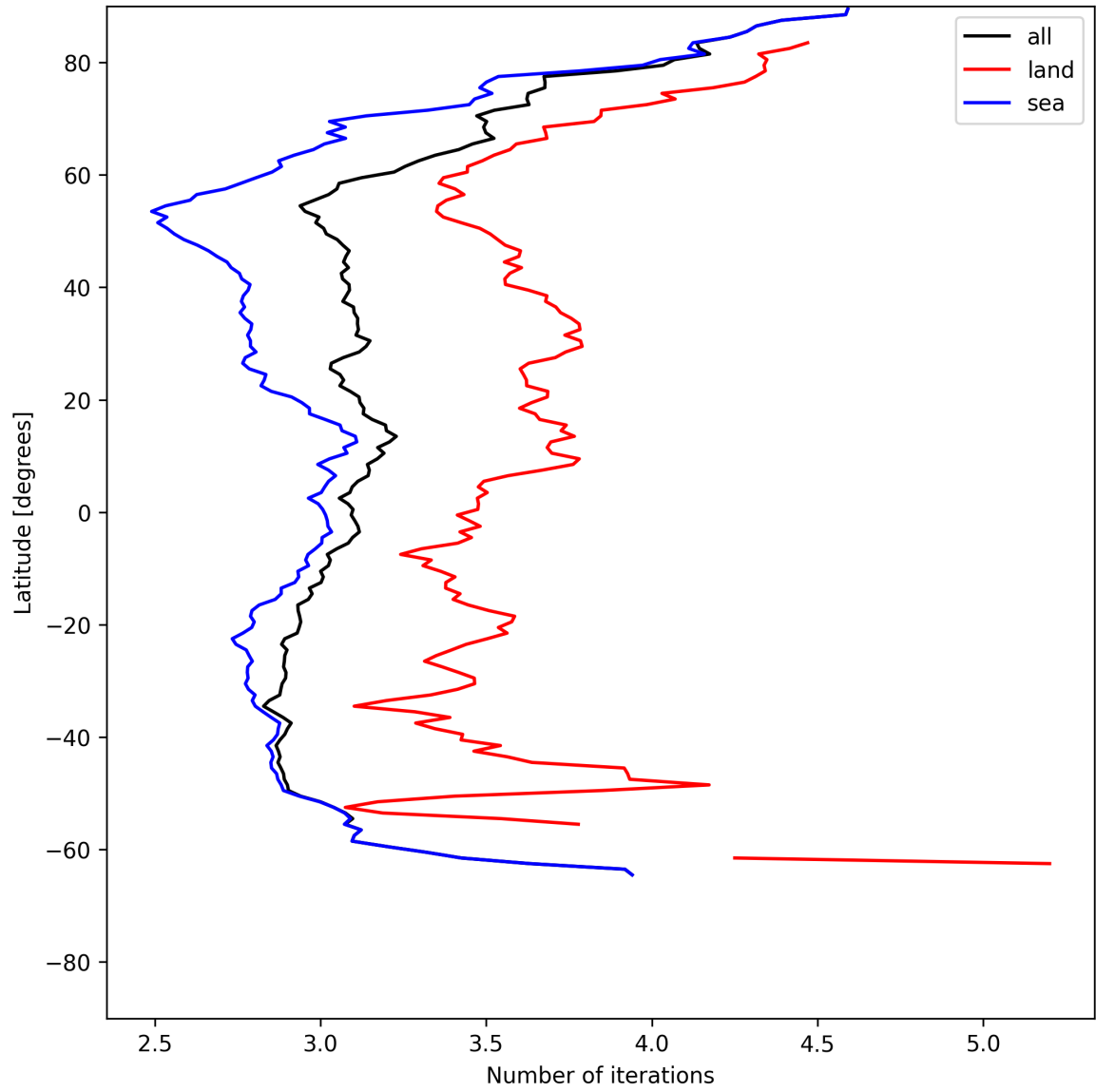
Figure 22: Zonal average of “Number of iterations” for 2025-06-09 to 2025-06-11.
