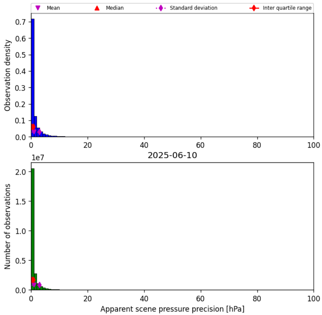
Figure 37: Histogram of “Apparent scene pressure precision” for 2025-06-09 to 2025-06-11
