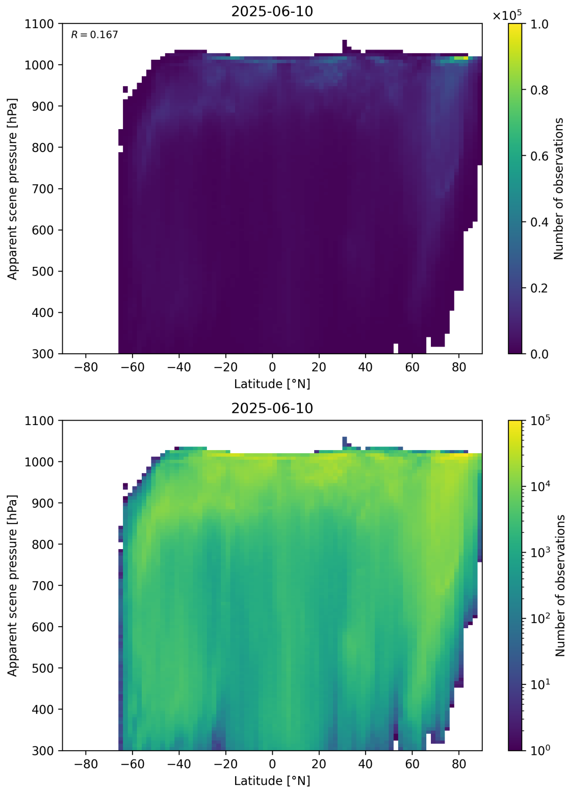
Figure 88: Scatter density plot of “Latitude” against “Apparent scene pressure” for 2025-06-09 to 2025-06-11.
