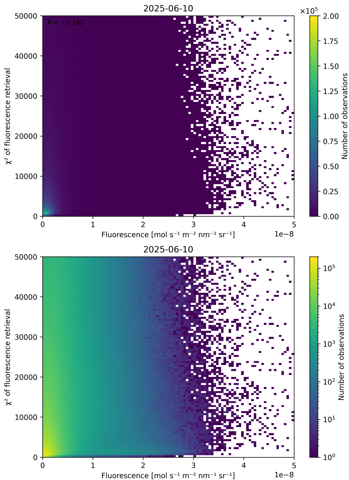
Figure 85: Scatter density plot of “Fluorescence” against “ \chi^2 of fluorescence retrieval” for 2025-06-09 to 2025-06-11.
