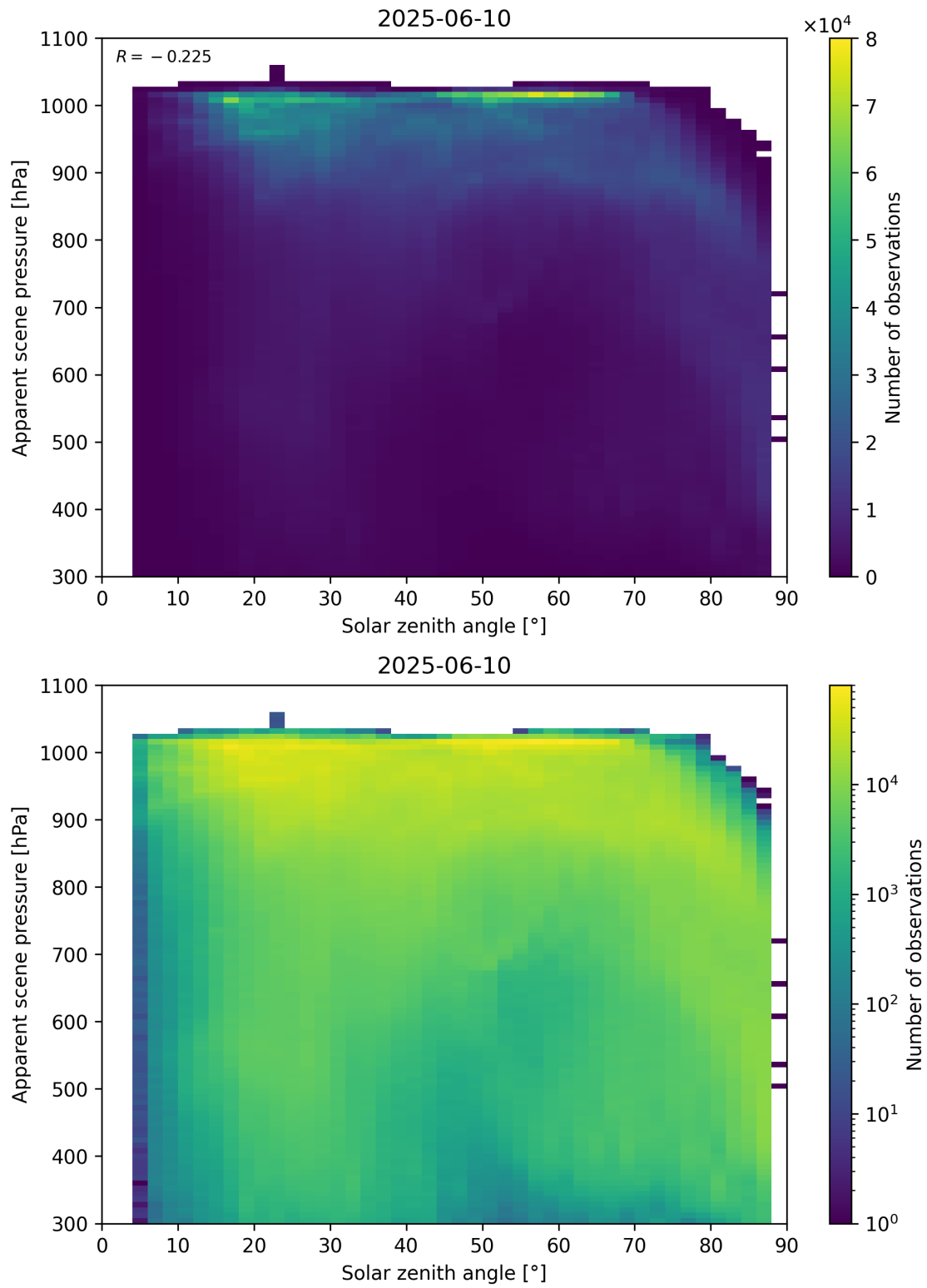
Figure 108: Scatter density plot of “Solar zenith angle” against “Apparent scene pressure” for 2025-06-09 to 2025-06-11.
