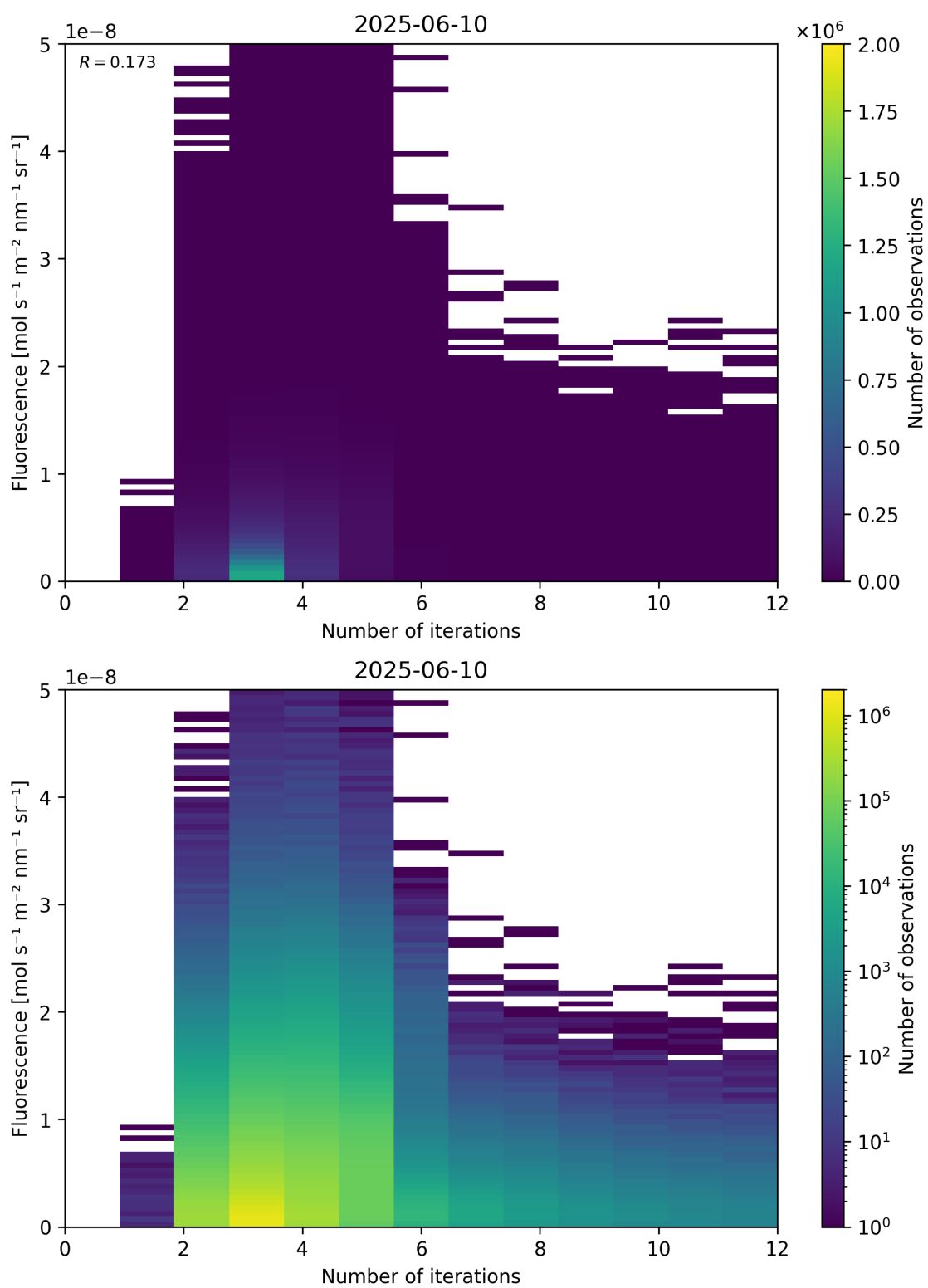
Figure 98: Scatter density plot of “Number of iterations” against “Fluorescence” for 2025-06-09 to 2025-06-11.
