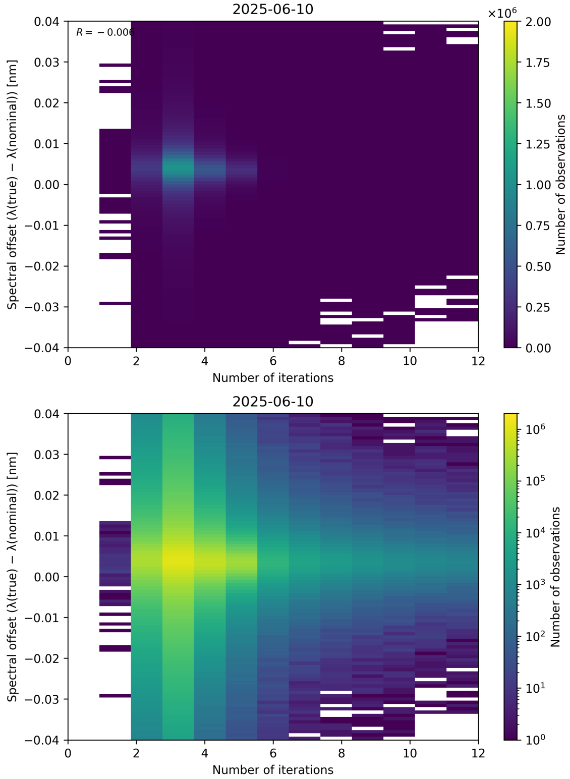
Figure 100: Scatter density plot of “Number of iterations” against “Spectral offset ( \lambda_{\text{true}} - \lambda_{\text{nominal}} )” for 2025-06-09 to 2025-06-11.
