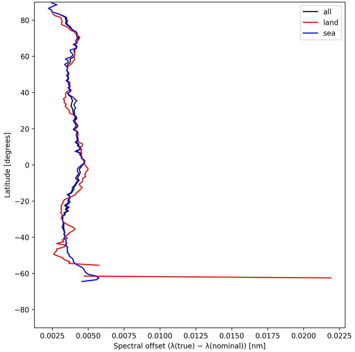
Figure 28: Zonal average of “Spectral offset ( \lambda_{\text{true}} - \lambda_{\text{nominal}} )” for 2025-06-09 to 2025-06-11.
