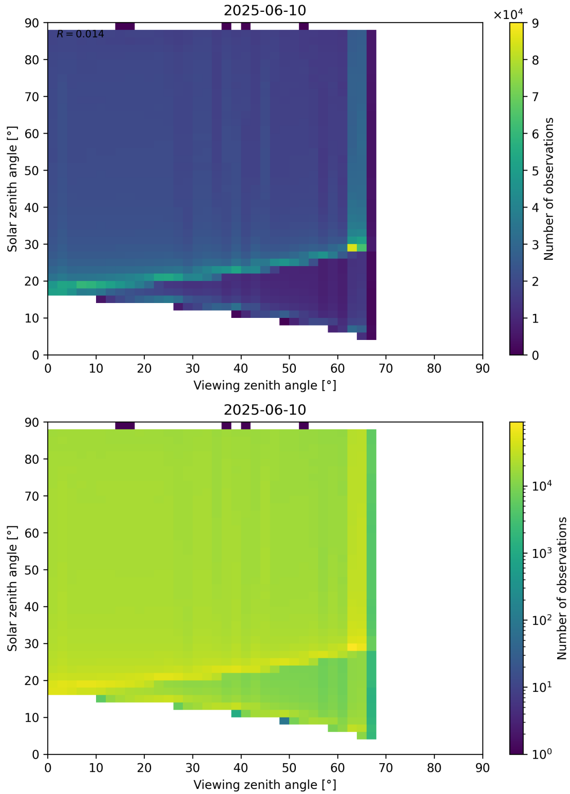
Figure 127: Scatter density plot of “Viewing zenith angle” against “Solar zenith angle” for 2025-06-09 to 2025-06-11.
