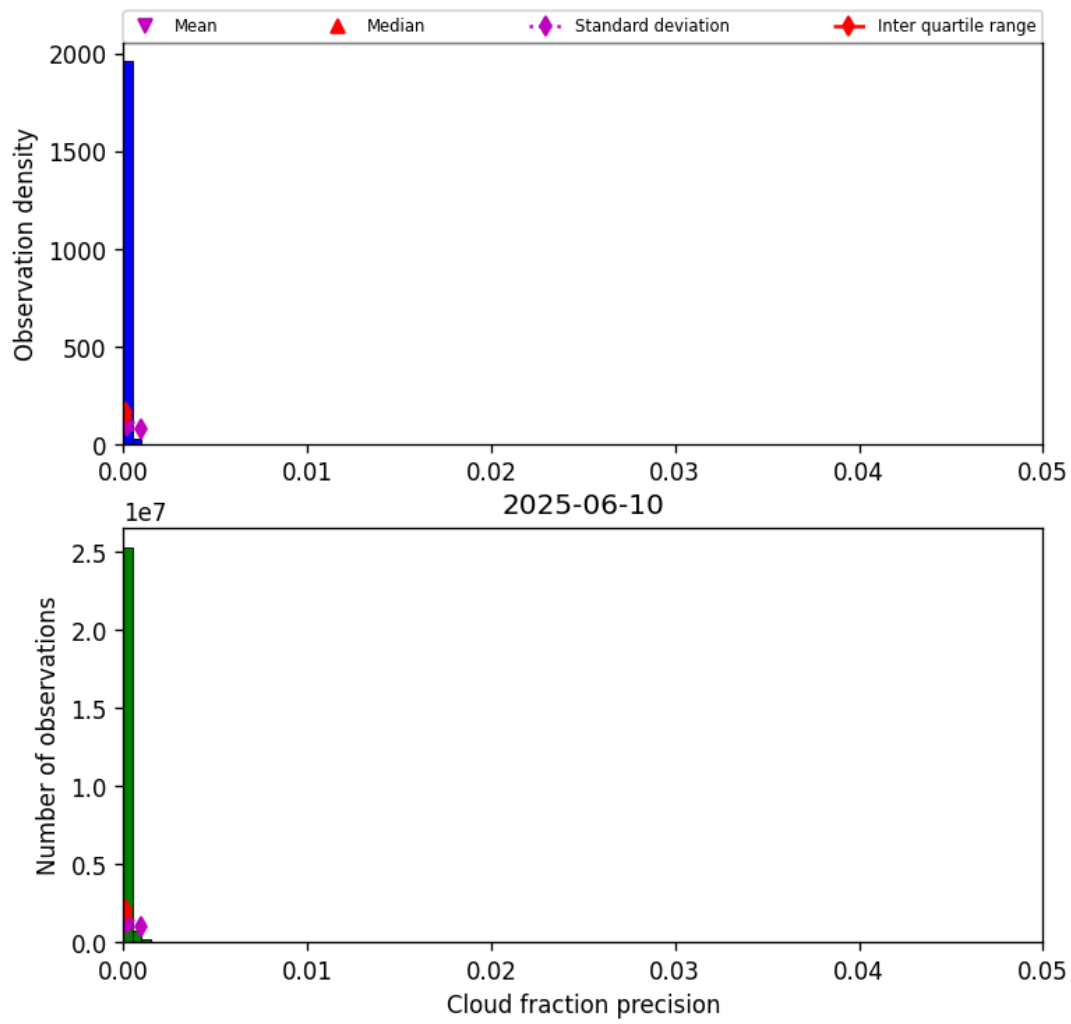
Figure 33: Histogram of “Cloud fraction precision” for 2025-06-09 to 2025-06-11
