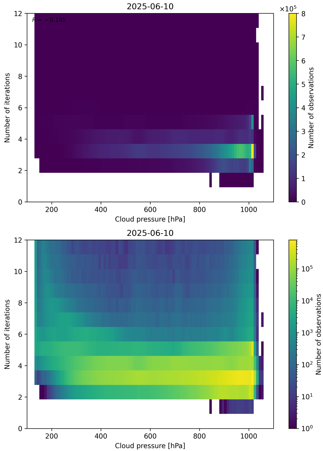
Figure 81: Scatter density plot of “Cloud pressure” against “Number of iterations” for 2025-06-09 to 2025-06-11.
