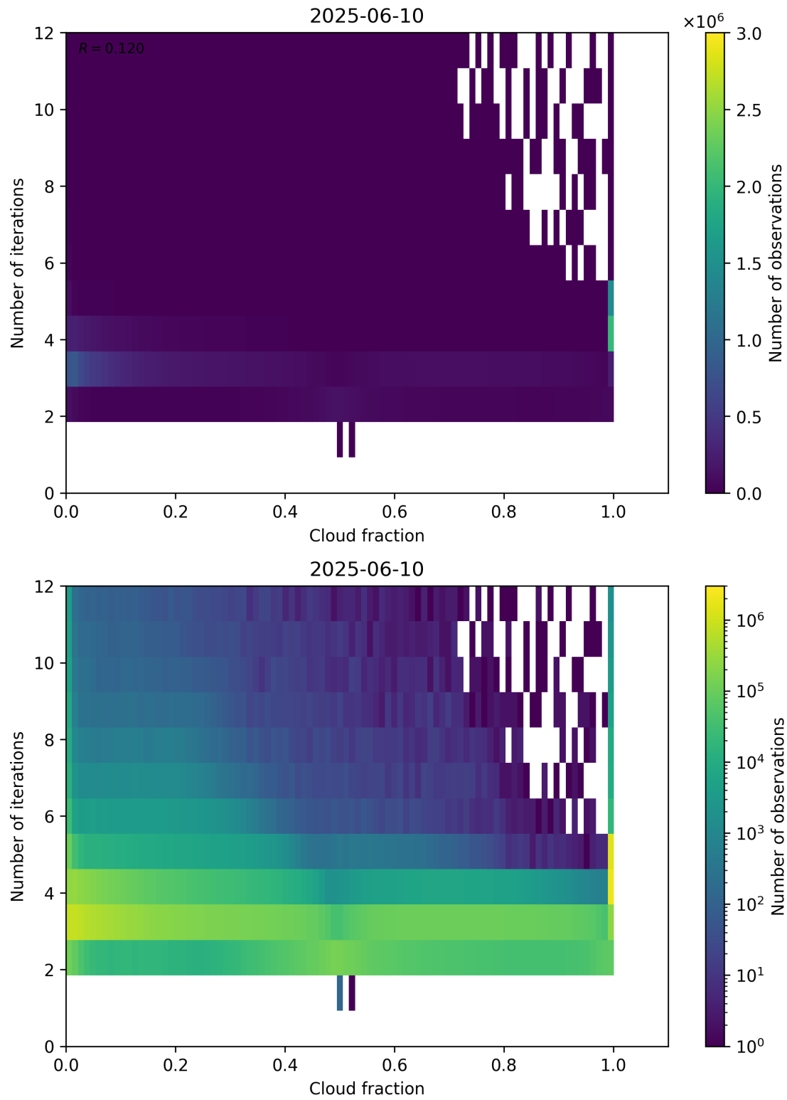
Figure 73: Scatter density plot of “Cloud fraction” against “Number of iterations” for 2025-06-09 to 2025-06-11.
