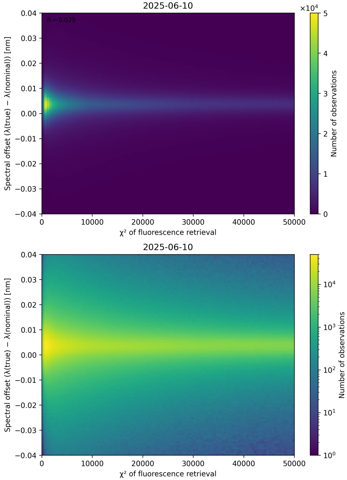
Figure 69: Scatter density plot of “ \chi^2 of fluorescence retrieval” against “Spectral offset ( \lambda_{\text{true}} - \lambda_{\text{nominal}} )” for 2025-06-09 to 2025-06-11.
