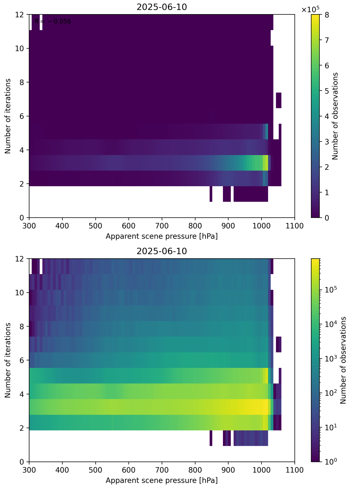
Figure 65: Scatter density plot of “Apparent scene pressure” against “Number of iterations” for 2025-06-09 to 2025-06-11.
