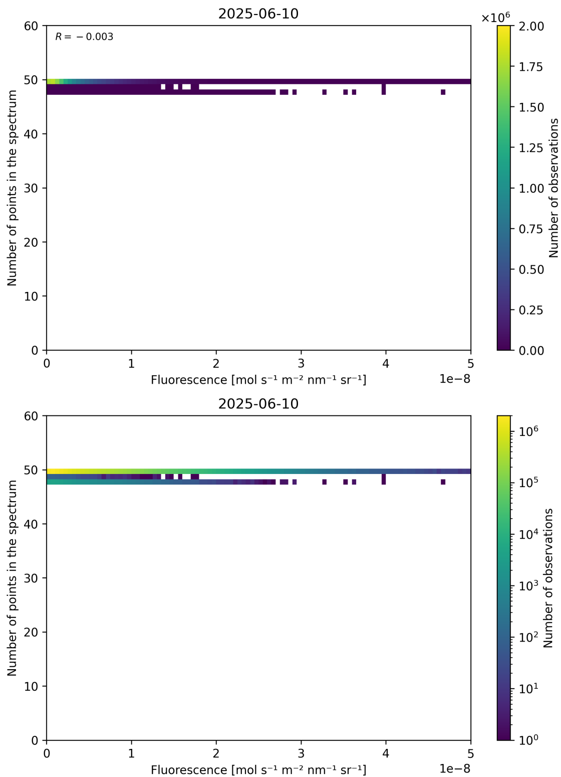
Figure 86: Scatter density plot of “Fluorescence” against “Number of points in the spectrum” for 2025-06-09 to 2025-06-11.
