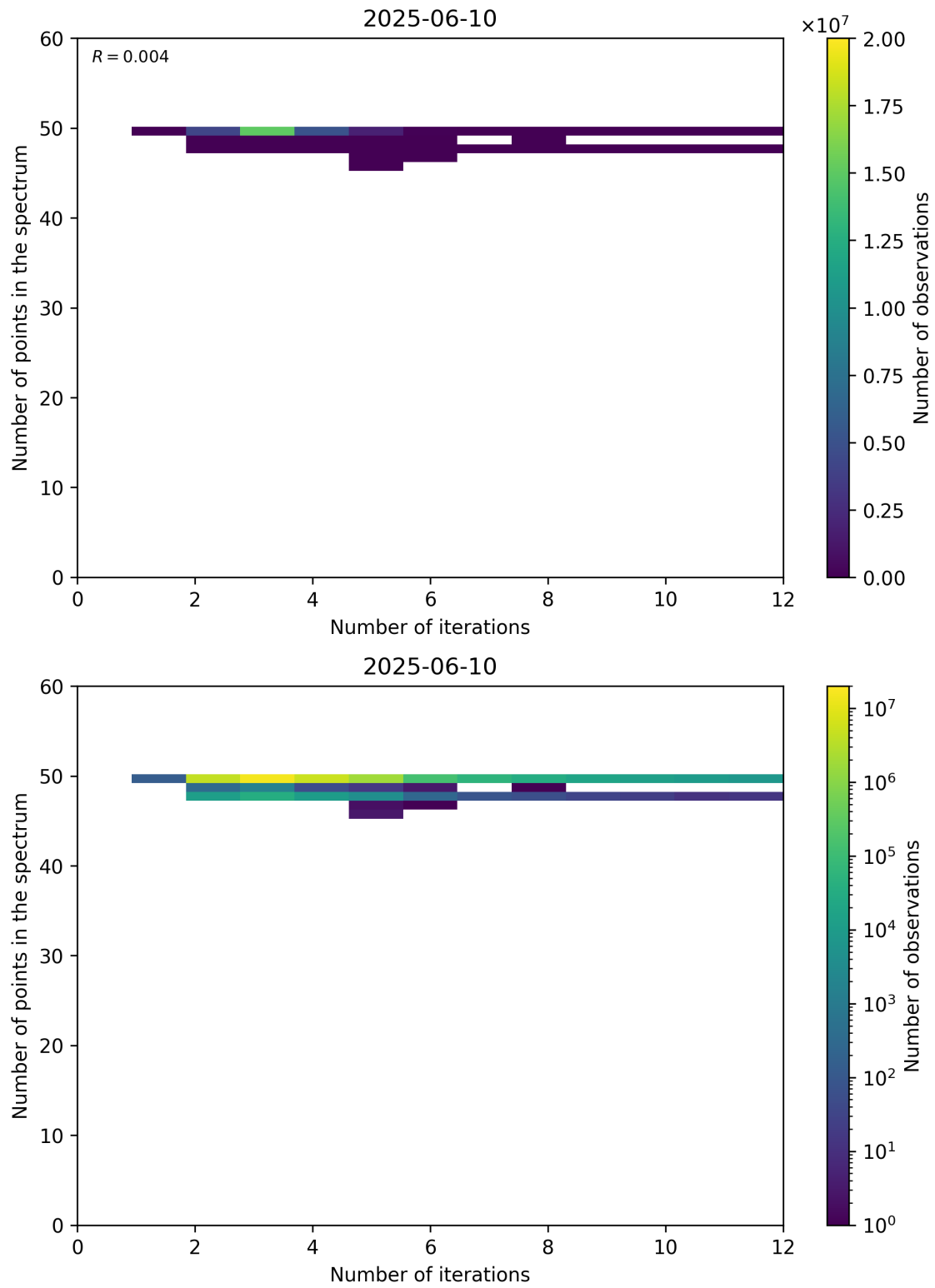
Figure 99: Scatter density plot of “Number of iterations” against “Number of points in the spectrum” for 2025-06-09 to 2025-06-11.
