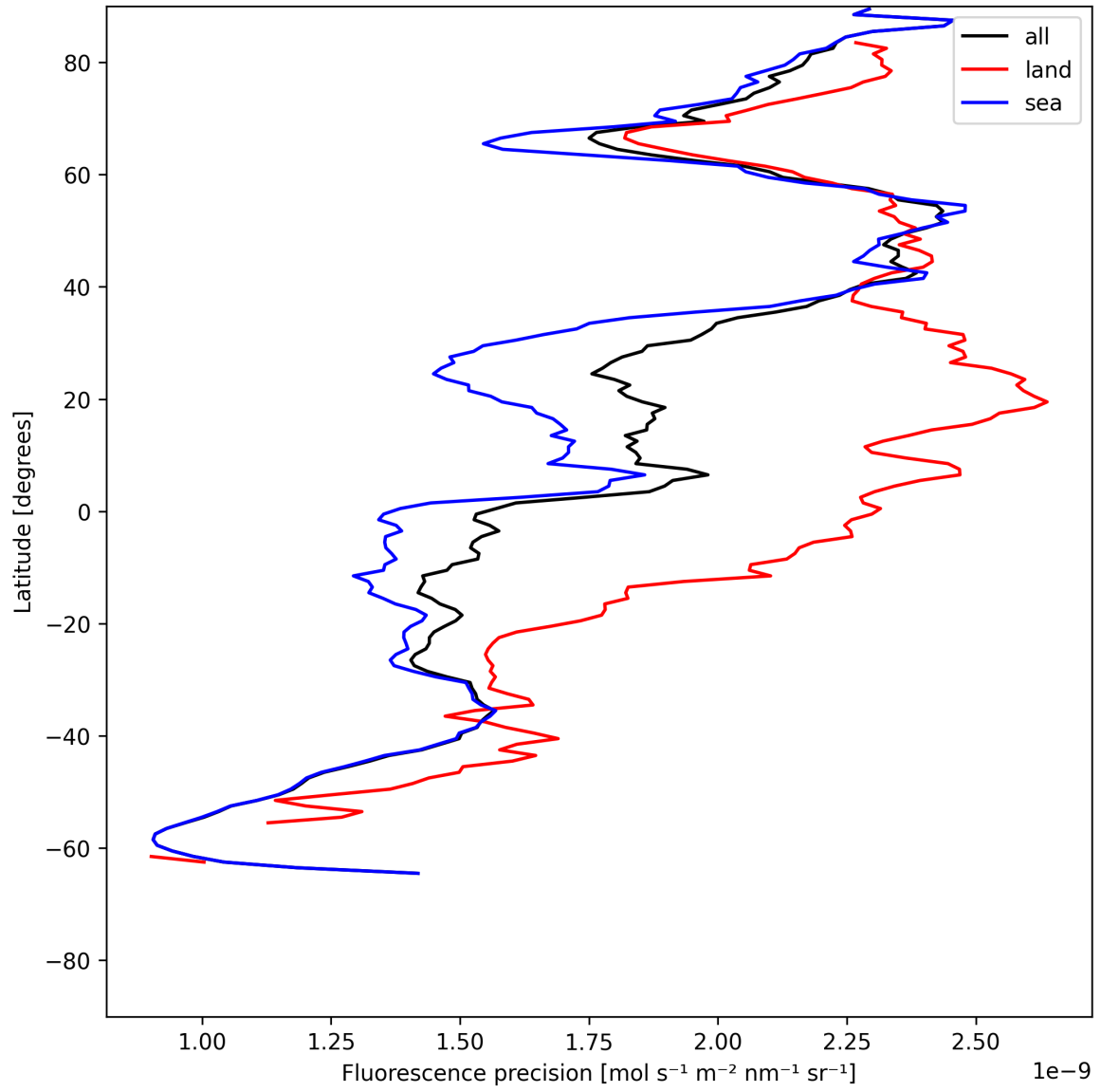
Figure 24: Zonal average of “Fluorescence precision” for 2025-06-09 to 2025-06-11.
