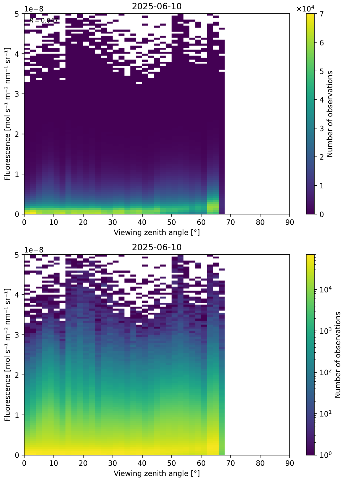
Figure 122: Scatter density plot of “Viewing zenith angle” against “Fluorescence” for 2025-06-09 to 2025-06-11.
