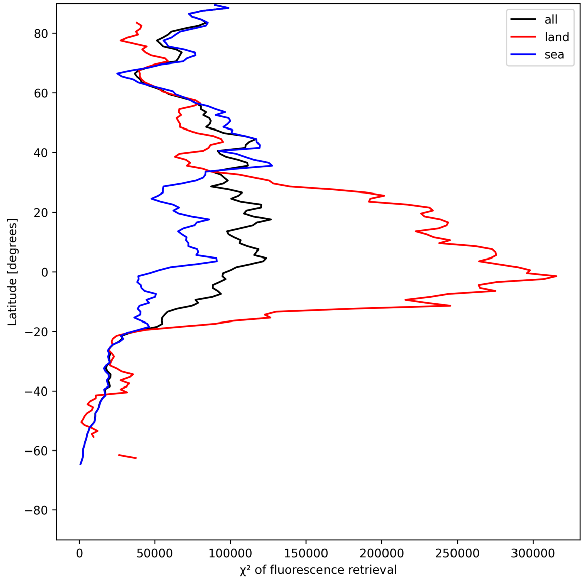
Figure 25: Zonal average of “ \chi^2 of fluorescence retrieval” for 2025-06-09 to 2025-06-11.
