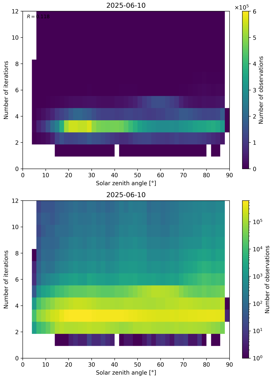
Figure 114: Scatter density plot of “Solar zenith angle” against “Number of iterations” for 2025-06-09 to 2025-06-11.
