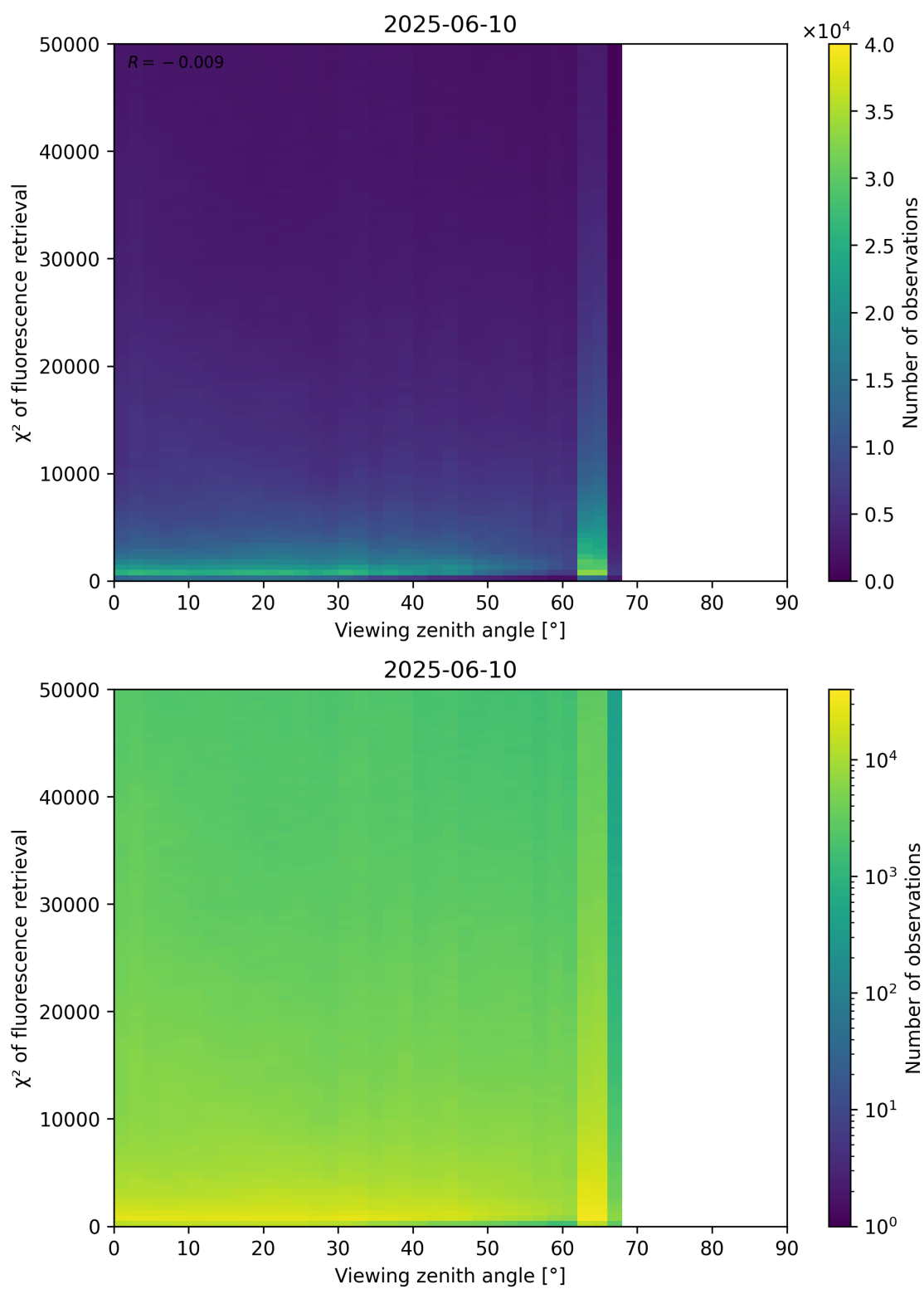
Figure 119: Scatter density plot of “Viewing zenith angle” against “ \chi^2 of fluorescence retrieval” for 2025-06-09 to 2025-06-11.
