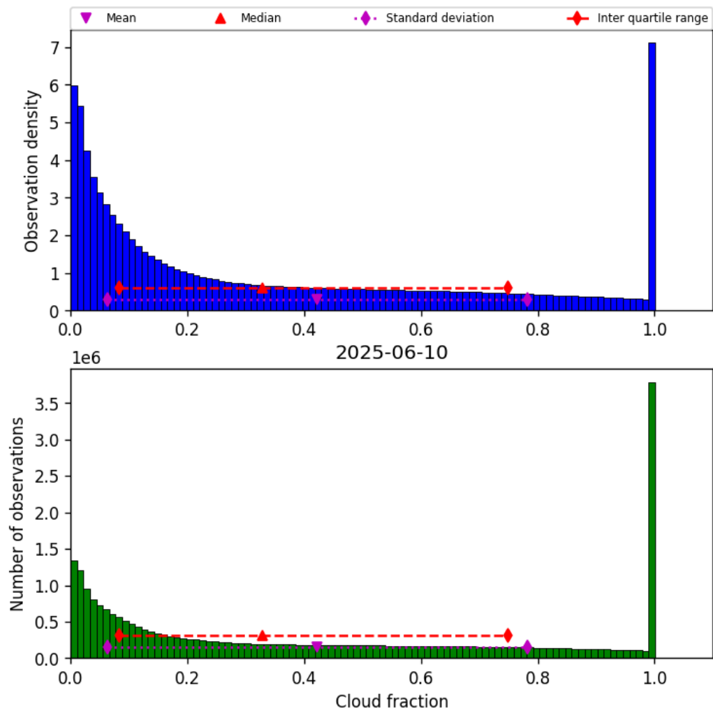
Figure 32: Histogram of “Cloud fraction” for 2025-06-09 to 2025-06-11
