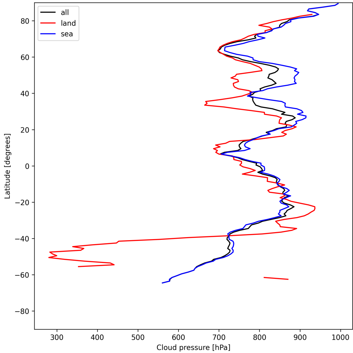
Figure 13: Zonal average of “Cloud pressure” for 2025-06-09 to 2025-06-11.
