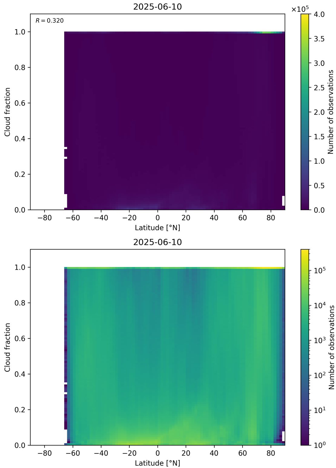
Figure 90: Scatter density plot of “Latitude” against “Cloud fraction” for 2025-06-09 to 2025-06-11.
