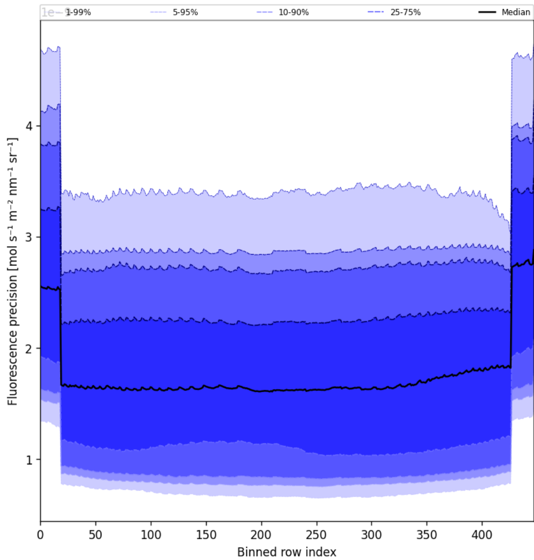
Figure 58: Along track statistics of “Fluorescence precision” for 2025-06-09 to 2025-06-11
