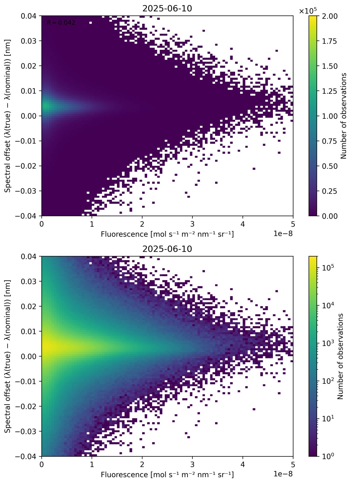
Figure 87: Scatter density plot of “Fluorescence” against “Spectral offset ( \lambda_{\text{true}} - \lambda_{\text{nominal}} )” for 2025-06-09 to 2025-06-11.
