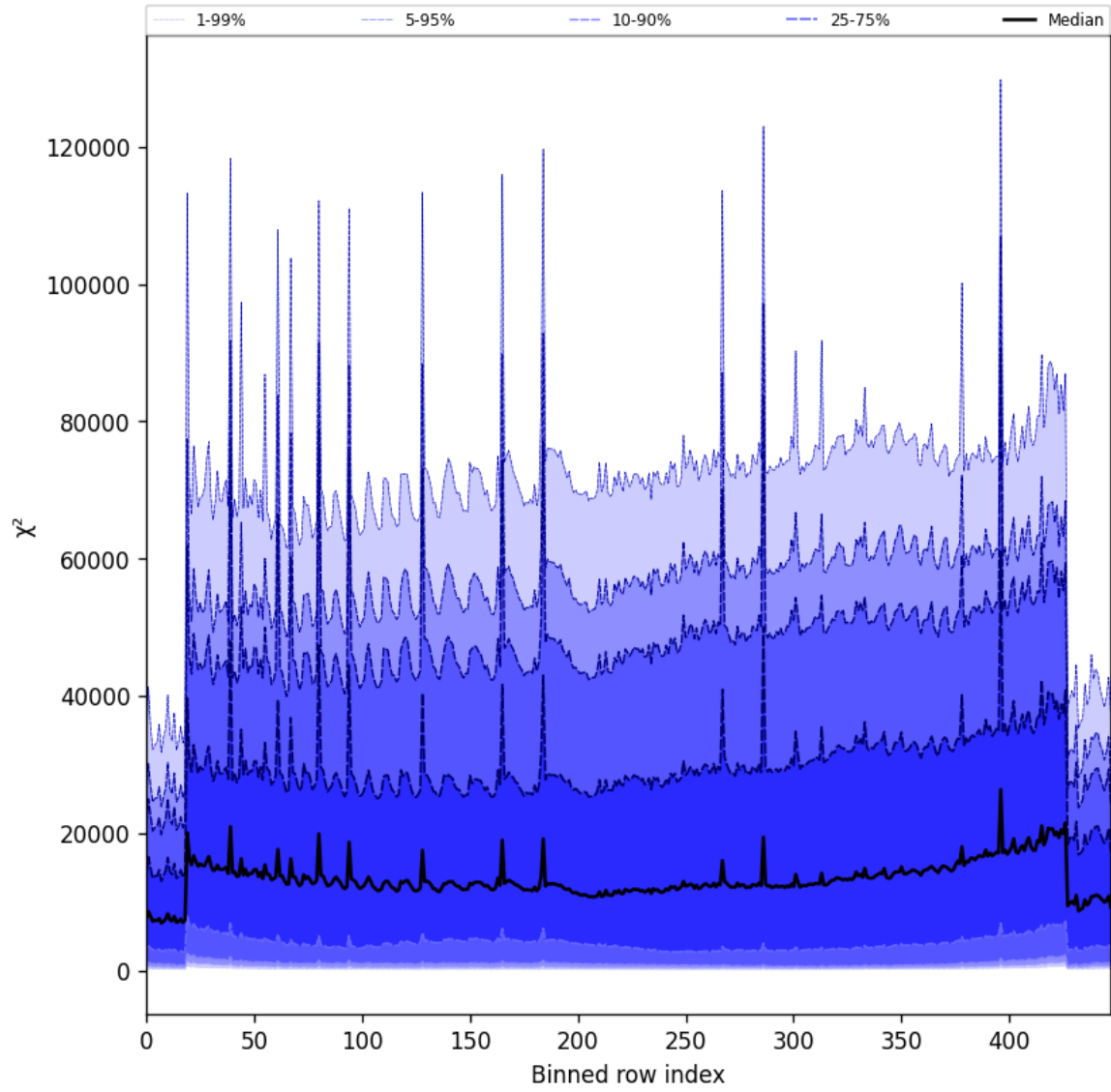
Figure 55: Along track statistics of “ \chi^2 ” for 2025-06-09 to 2025-06-11
