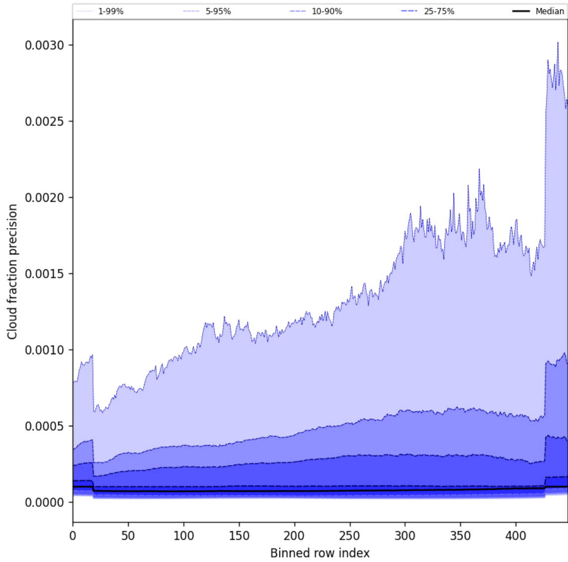
Figure 50: Along track statistics of “Cloud fraction precision” for 2025-06-09 to 2025-06-11
