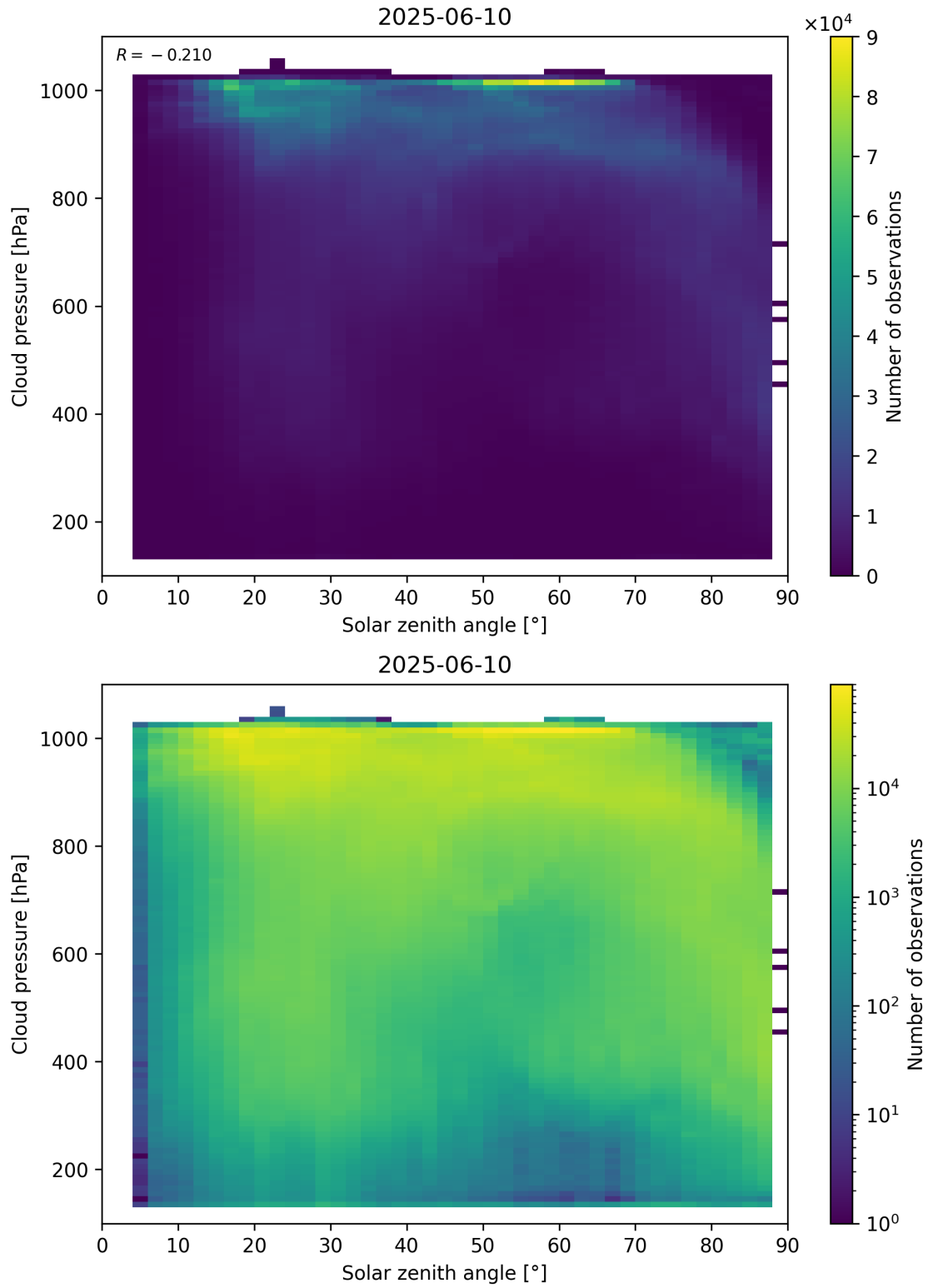
Figure 111: Scatter density plot of “Solar zenith angle” against “Cloud pressure” for 2025-06-09 to 2025-06-11.
