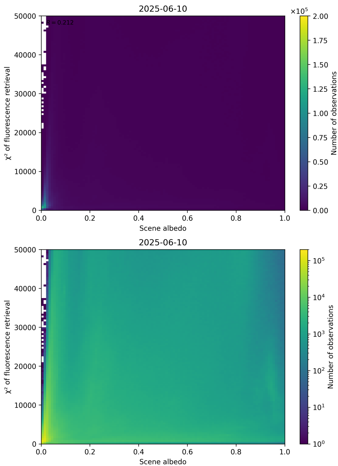
Figure 103: Scatter density plot of “Scene albedo” against “ \chi^2 of fluorescence retrieval” for 2025-06-09 to 2025-06-11.
