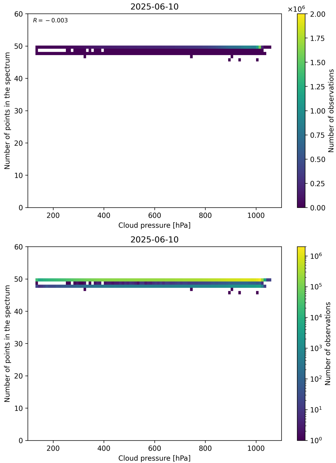
Figure 82: Scatter density plot of “Cloud pressure” against “Number of points in the spectrum” for 2025-06-09 to 2025-06-11.
