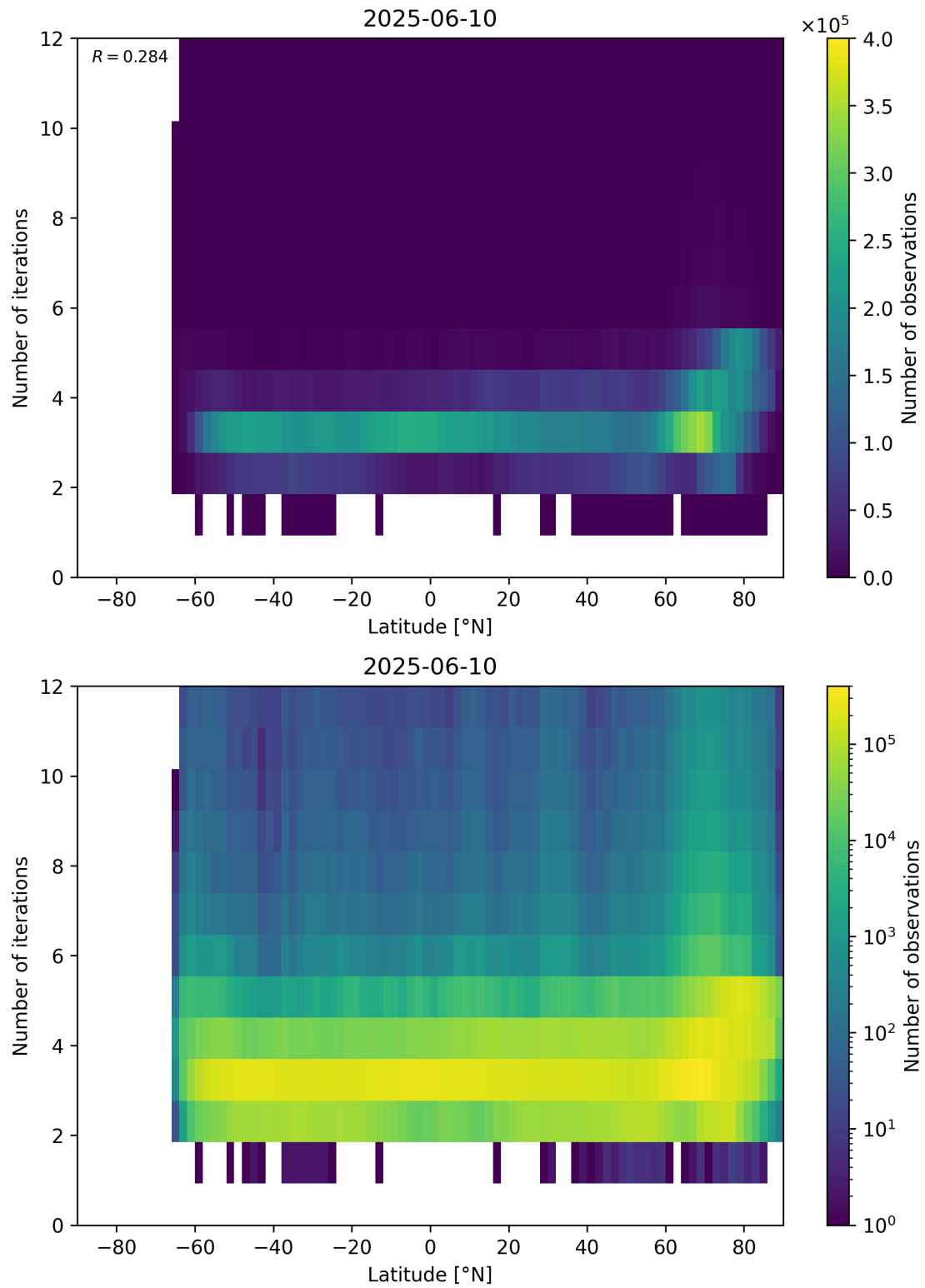
Figure 93: Scatter density plot of “Latitude” against “Number of iterations” for 2025-06-09 to 2025-06-11.
