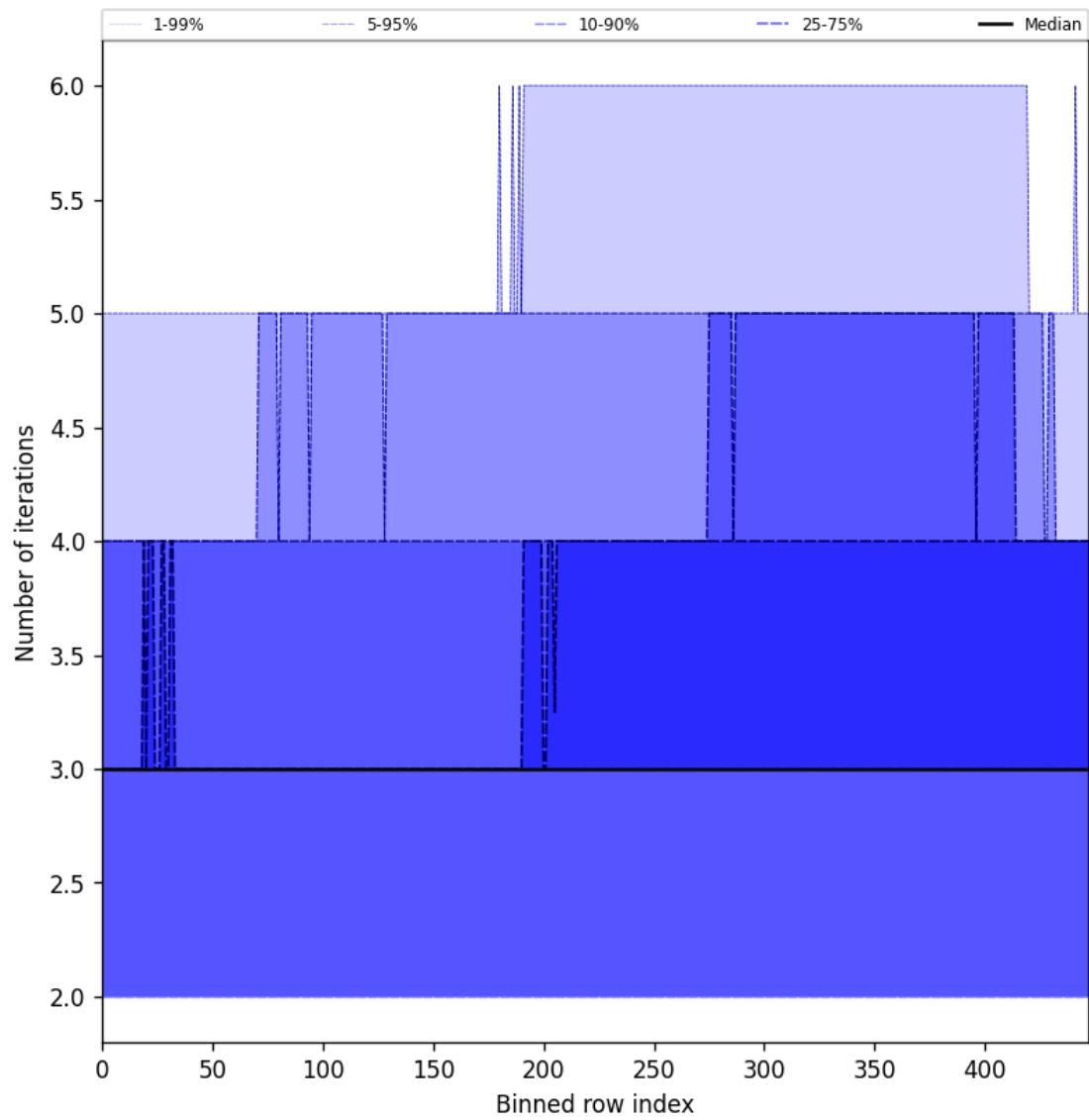
Figure 56: Along track statistics of “Number of iterations” for 2025-06-09 to 2025-06-11
