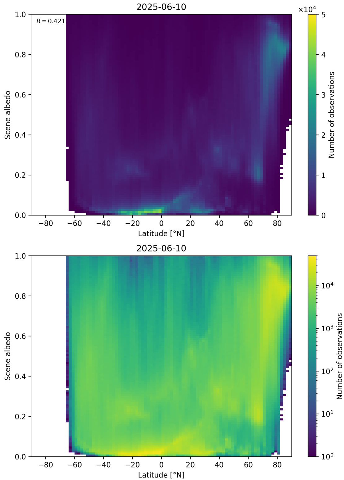
Figure 95: Scatter density plot of “Latitude” against “Scene albedo” for 2025-06-09 to 2025-06-11.
