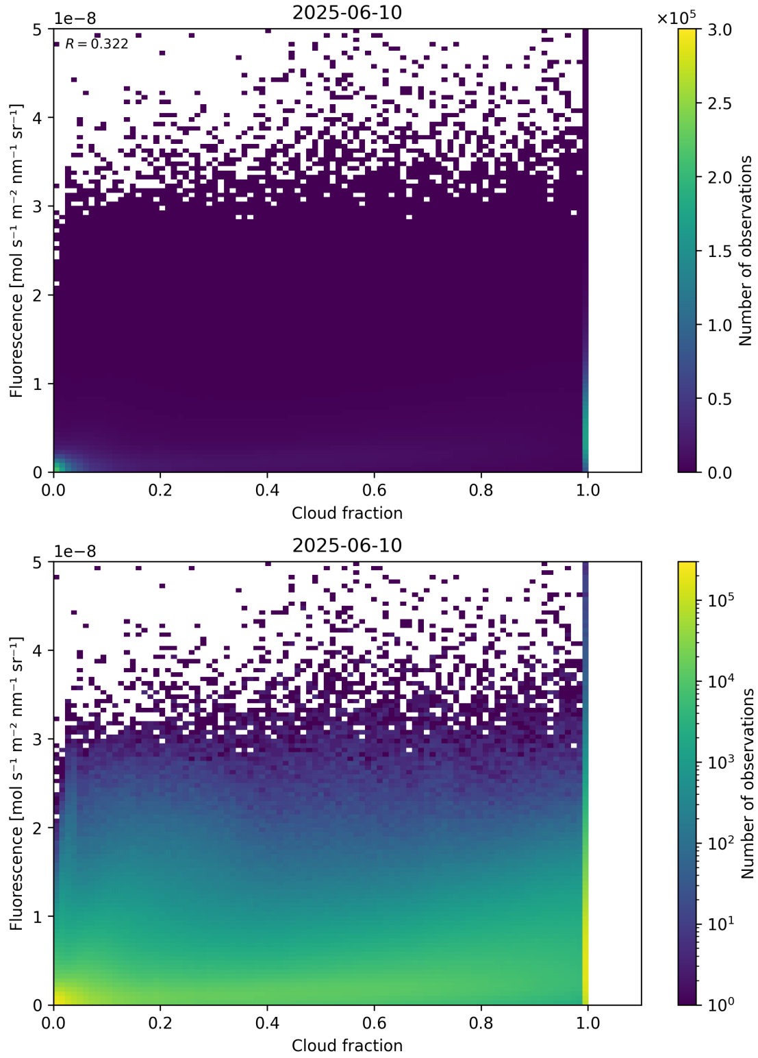
Figure 72: Scatter density plot of “Cloud fraction” against “Fluorescence” for 2025-06-09 to 2025-06-11.
