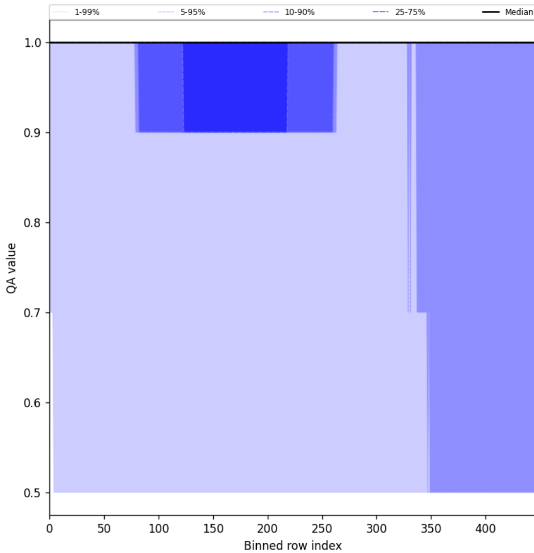
Figure 46: Along track statistics of “QA value” for 2025-06-09 to 2025-06-11
