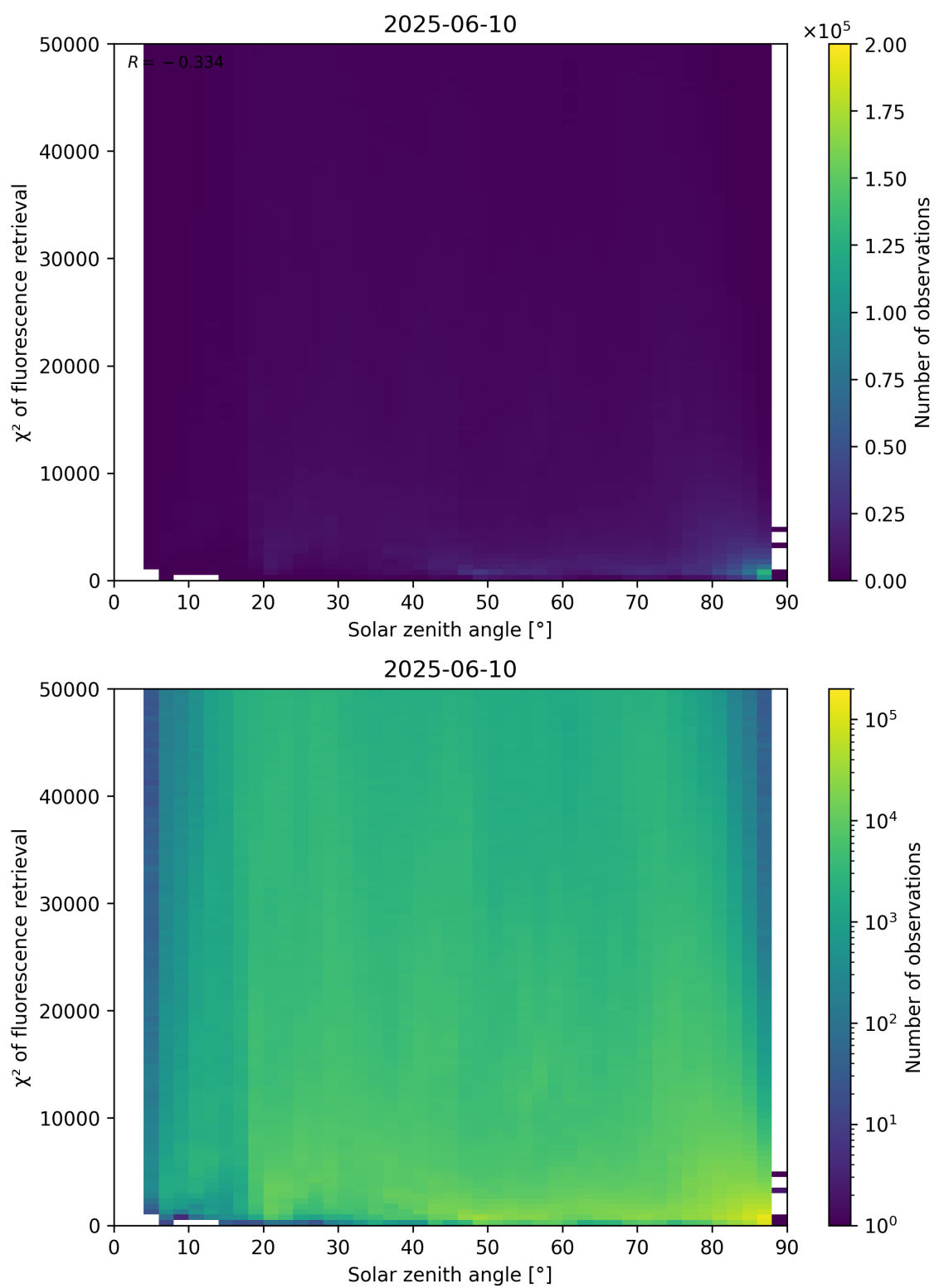
Figure 109: Scatter density plot of “Solar zenith angle” against “ \chi^2 of fluorescence retrieval” for 2025-06-09 to 2025-06-11.
