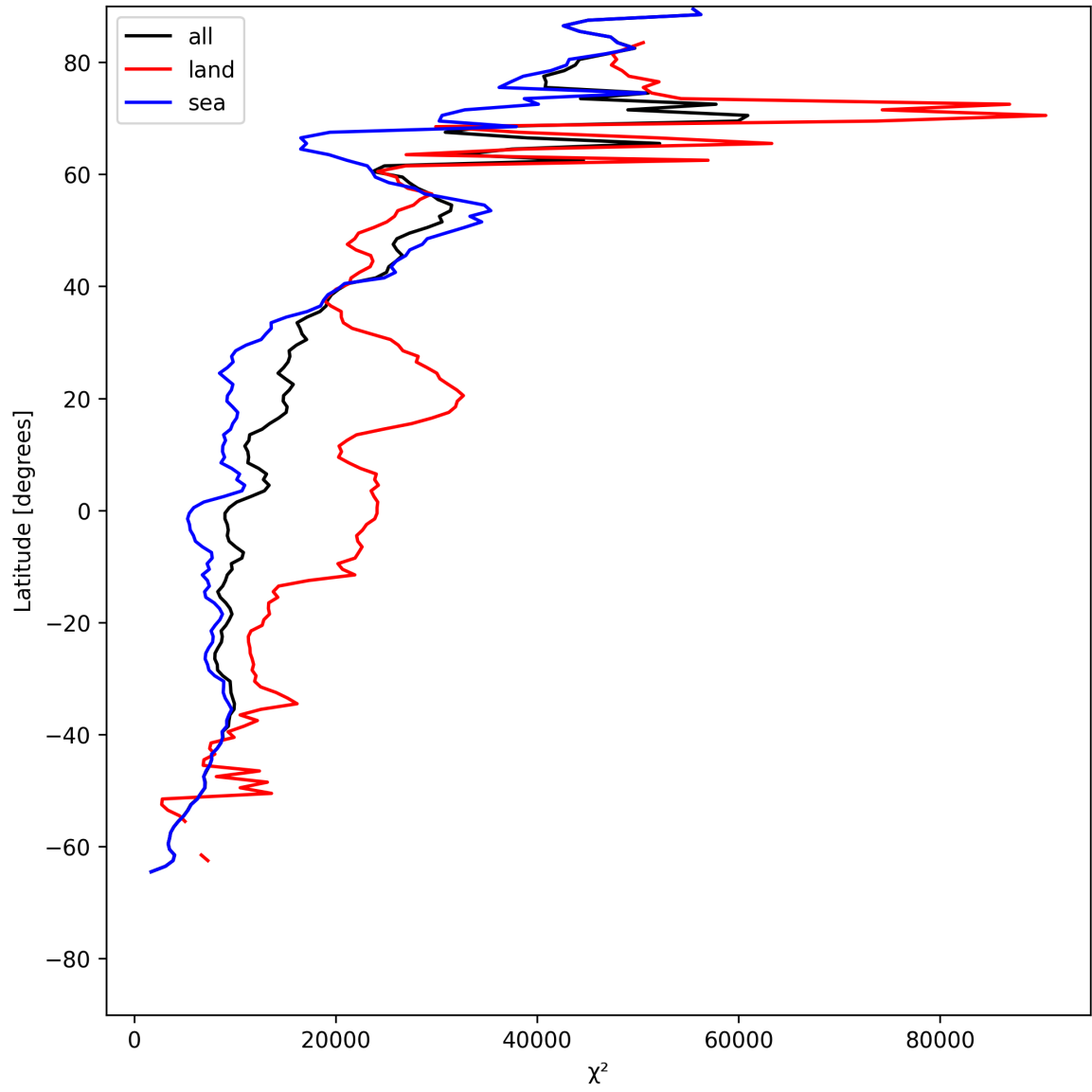
Figure 21: Zonal average of “ \chi^2 ” for 2025-06-09 to 2025-06-11.
