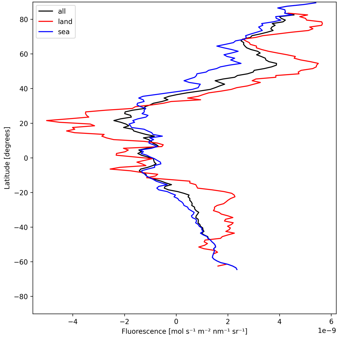
Figure 23: Zonal average of “Fluorescence” for 2025-06-09 to 2025-06-11.
