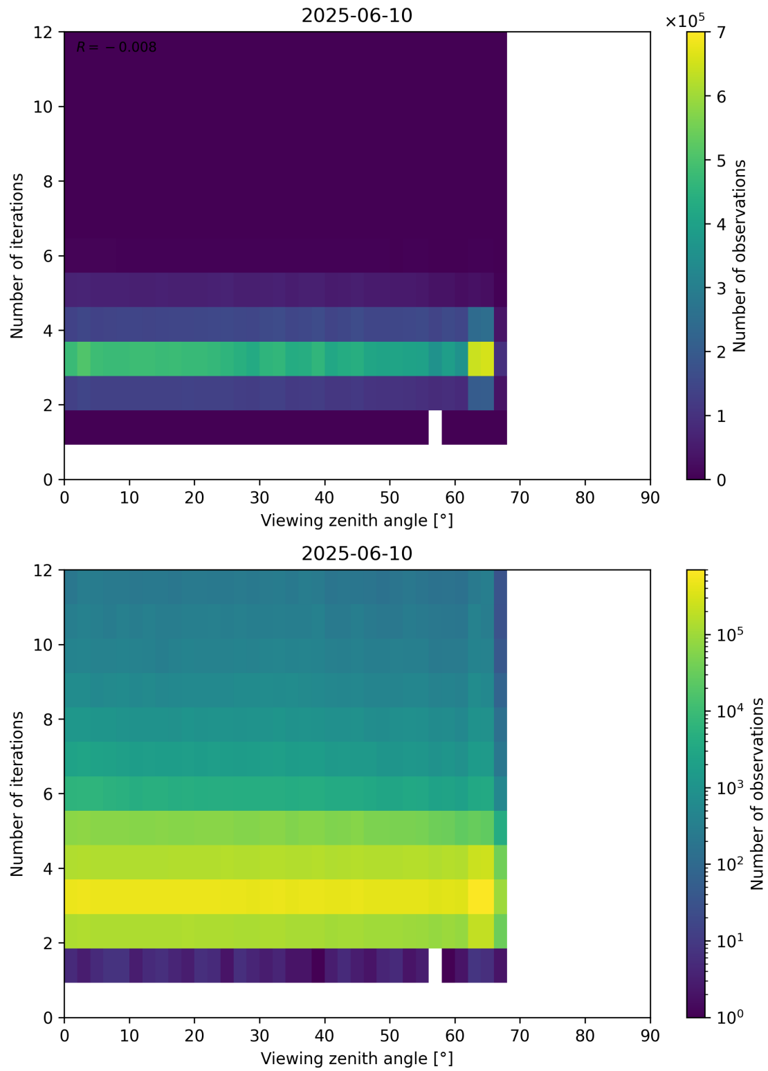
Figure 124: Scatter density plot of “Viewing zenith angle” against “Number of iterations” for 2025-06-09 to 2025-06-11.
