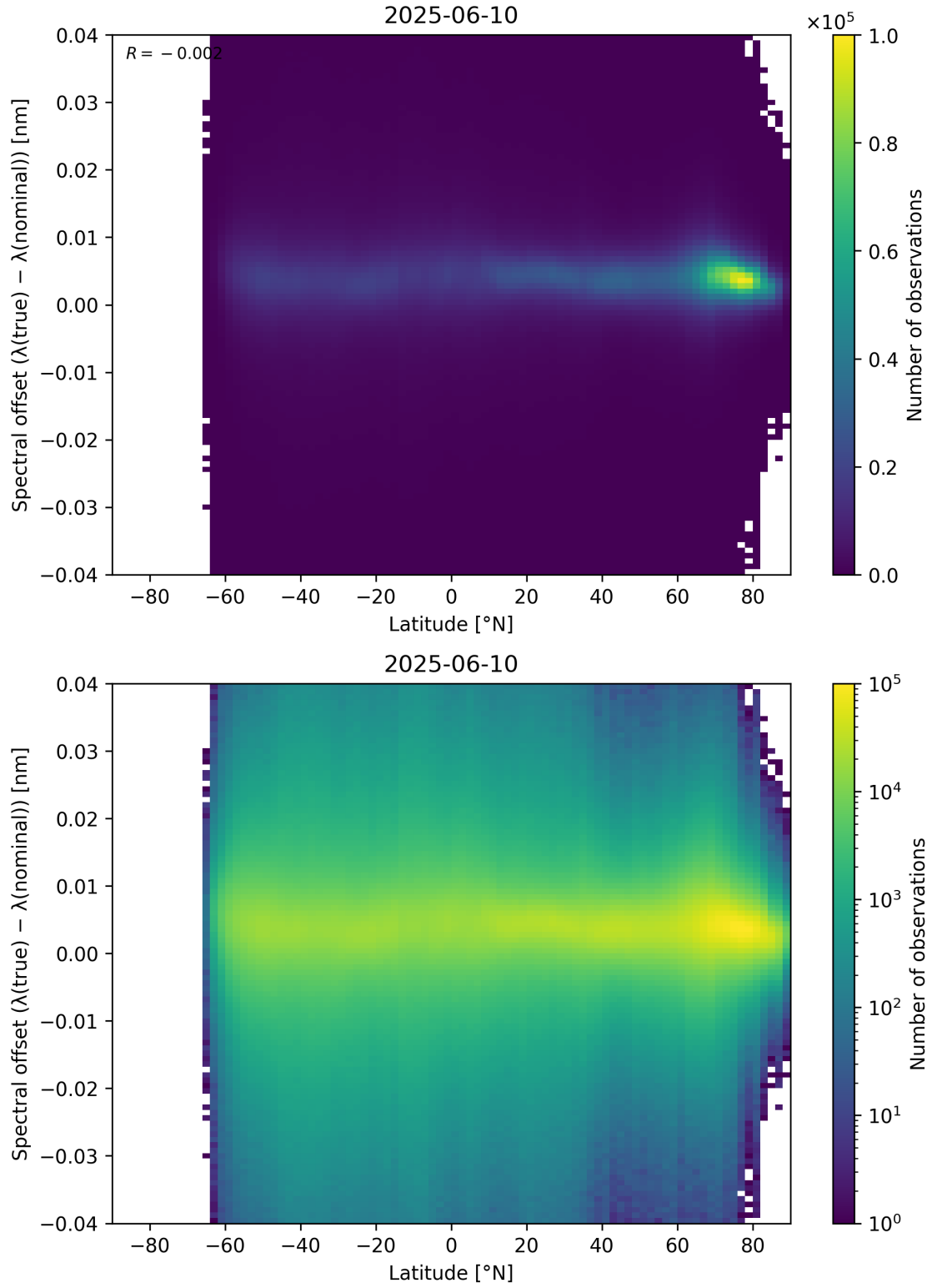
Figure 96: Scatter density plot of “Latitude” against “Spectral offset ( \lambda_{\text{true}} - \lambda_{\text{nominal}} )” for 2025-06-09 to 2025-06-11.
