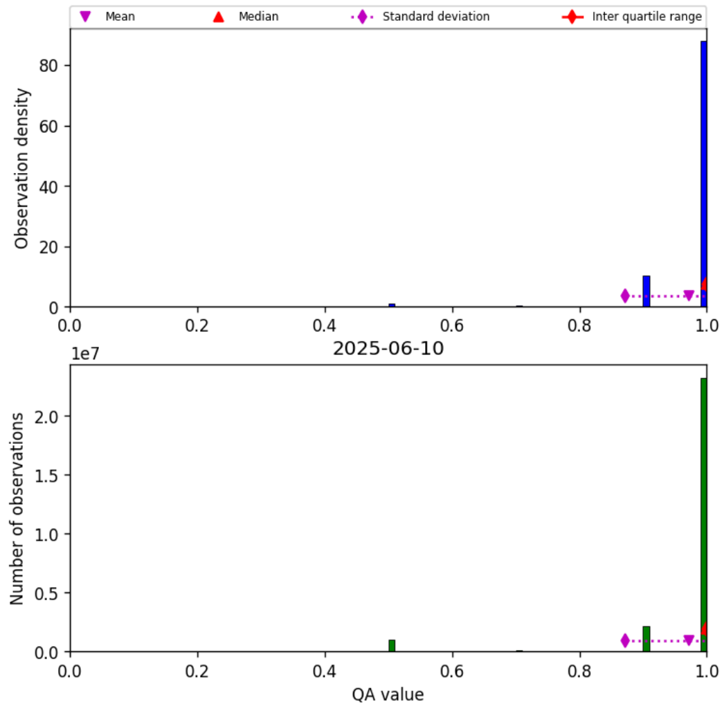
Figure 29: Histogram of “QA value” for 2025-06-09 to 2025-06-11
