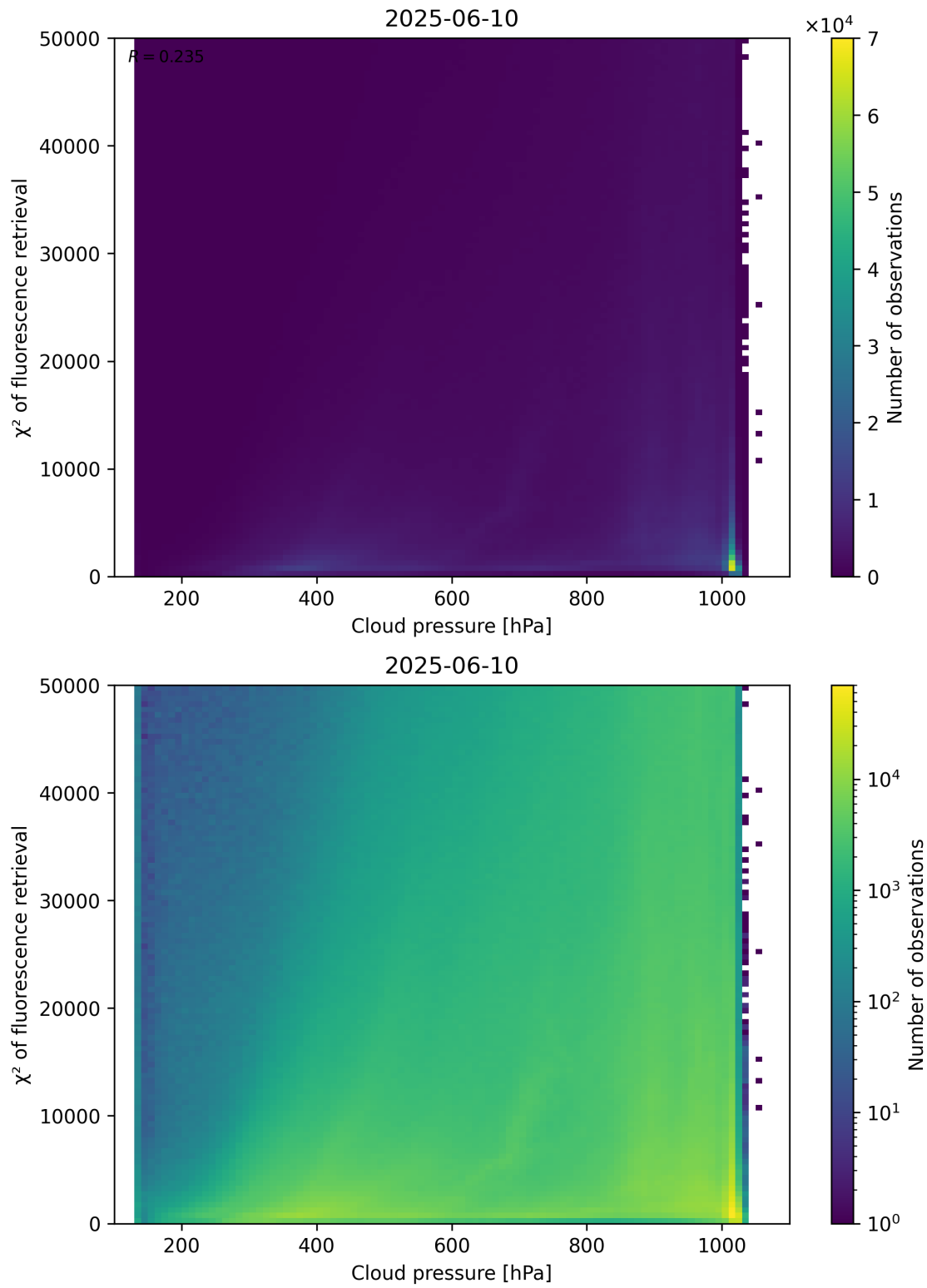
Figure 78: Scatter density plot of “Cloud pressure” against “ \chi^2 of fluorescence retrieval” for 2025-06-09 to 2025-06-11.
