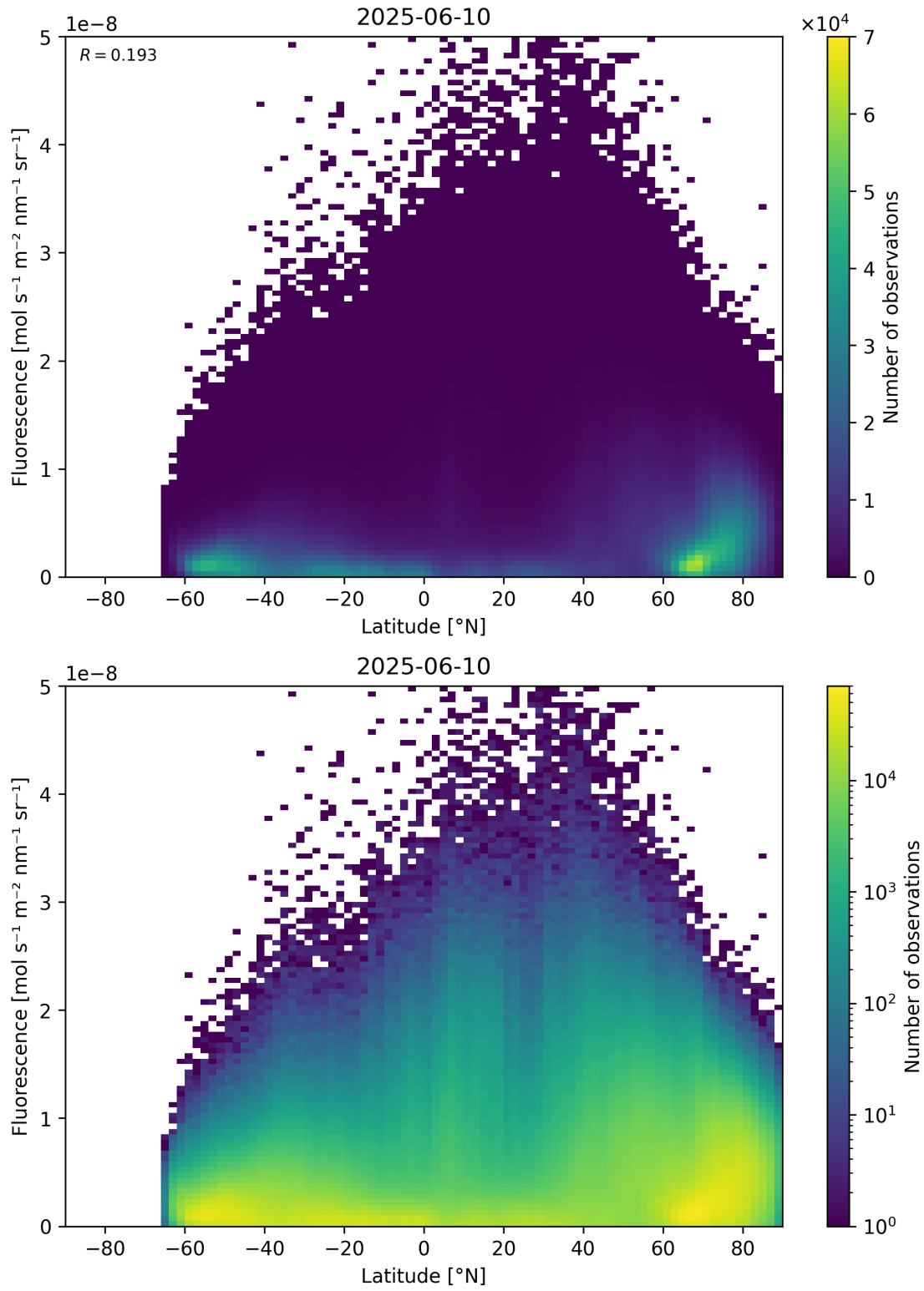
Figure 92: Scatter density plot of “Latitude” against “Fluorescence” for 2025-06-09 to 2025-06-11.
