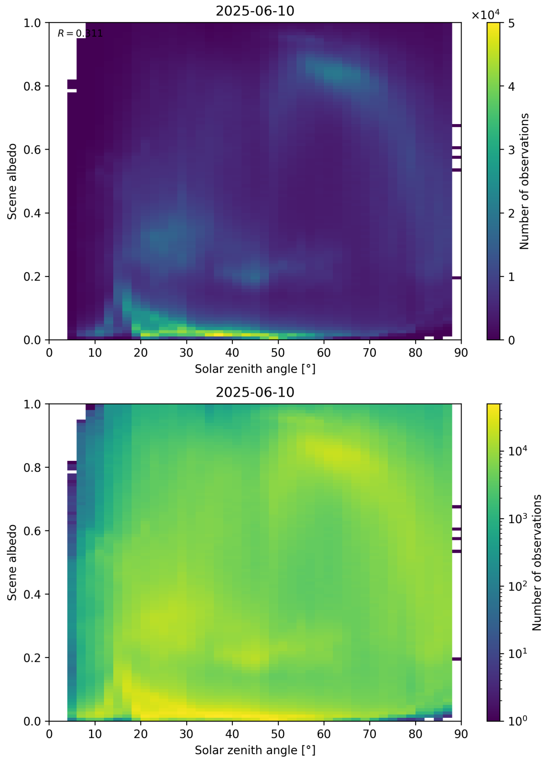
Figure 116: Scatter density plot of “Solar zenith angle” against “Scene albedo” for 2025-06-09 to 2025-06-11.
