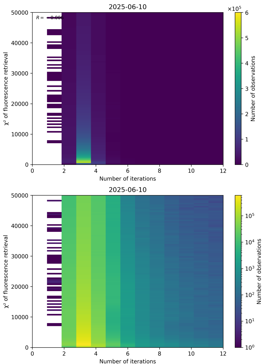
Figure 97: Scatter density plot of “Number of iterations” against “ \chi^2 of fluorescence retrieval” for 2025-06-09 to 2025-06-11.
