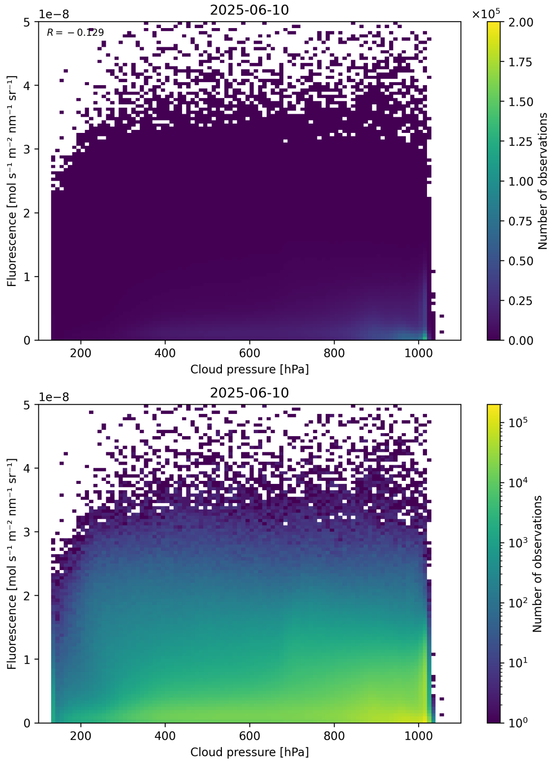
Figure 80: Scatter density plot of “Cloud pressure” against “Fluorescence” for 2025-06-09 to 2025-06-11.
