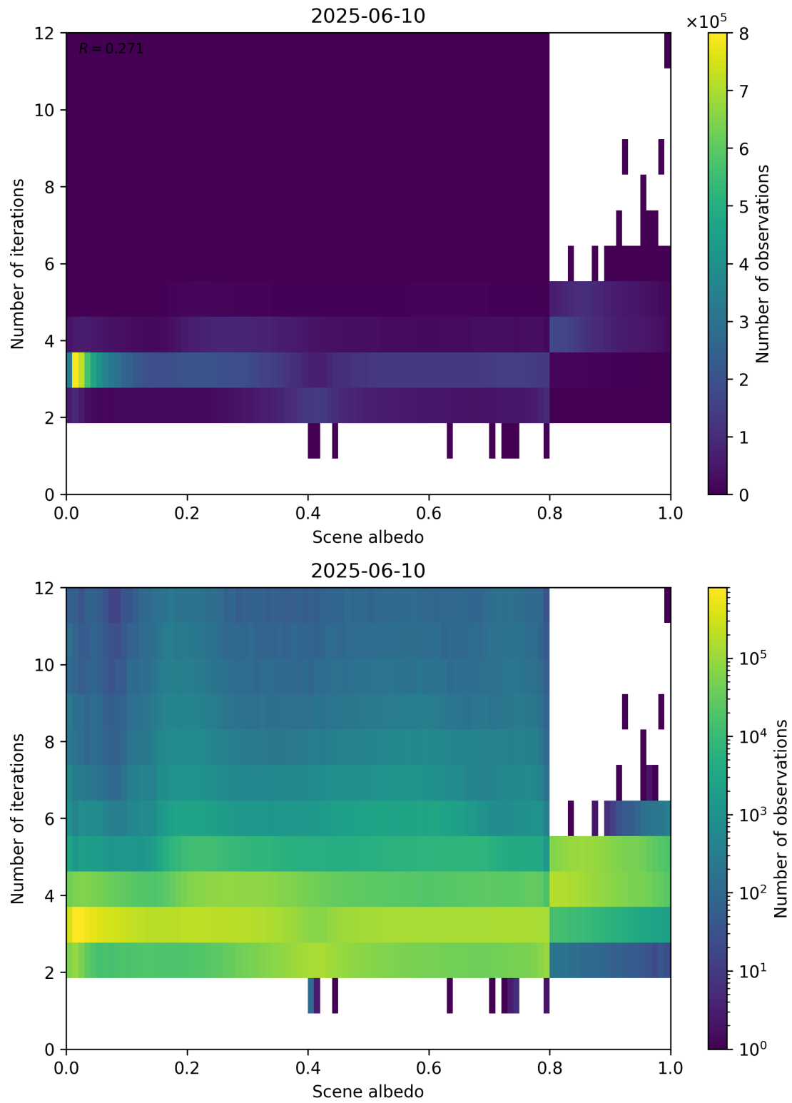
Figure 105: Scatter density plot of “Scene albedo” against “Number of iterations” for 2025-06-09 to 2025-06-11.
