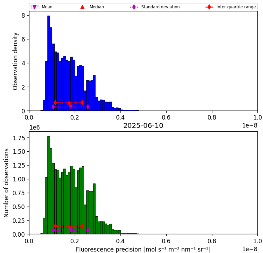
Figure 41: Histogram of “Fluorescence precision” for 2025-06-09 to 2025-06-11
