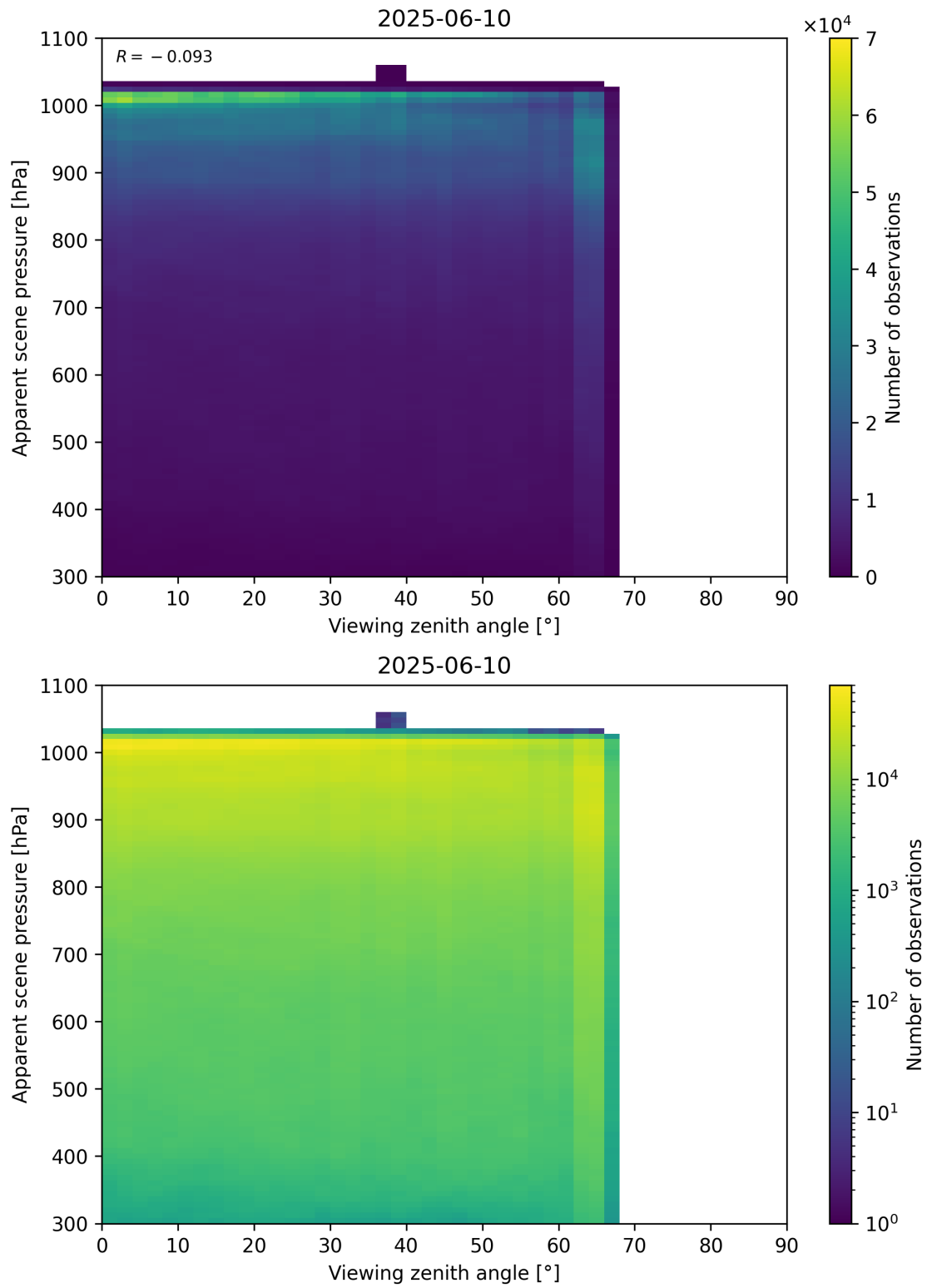
Figure 118: Scatter density plot of “Viewing zenith angle” against “Apparent scene pressure” for 2025-06-09 to 2025-06-11.
