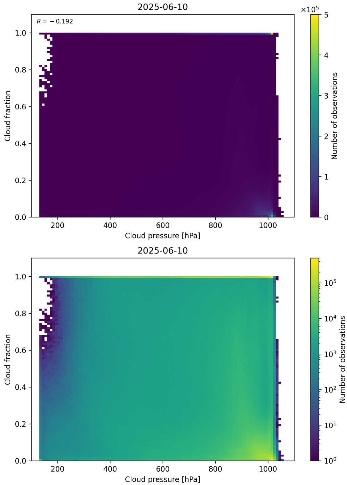
Figure 79: Scatter density plot of “Cloud pressure” against “Cloud fraction” for 2025-06-09 to 2025-06-11.
