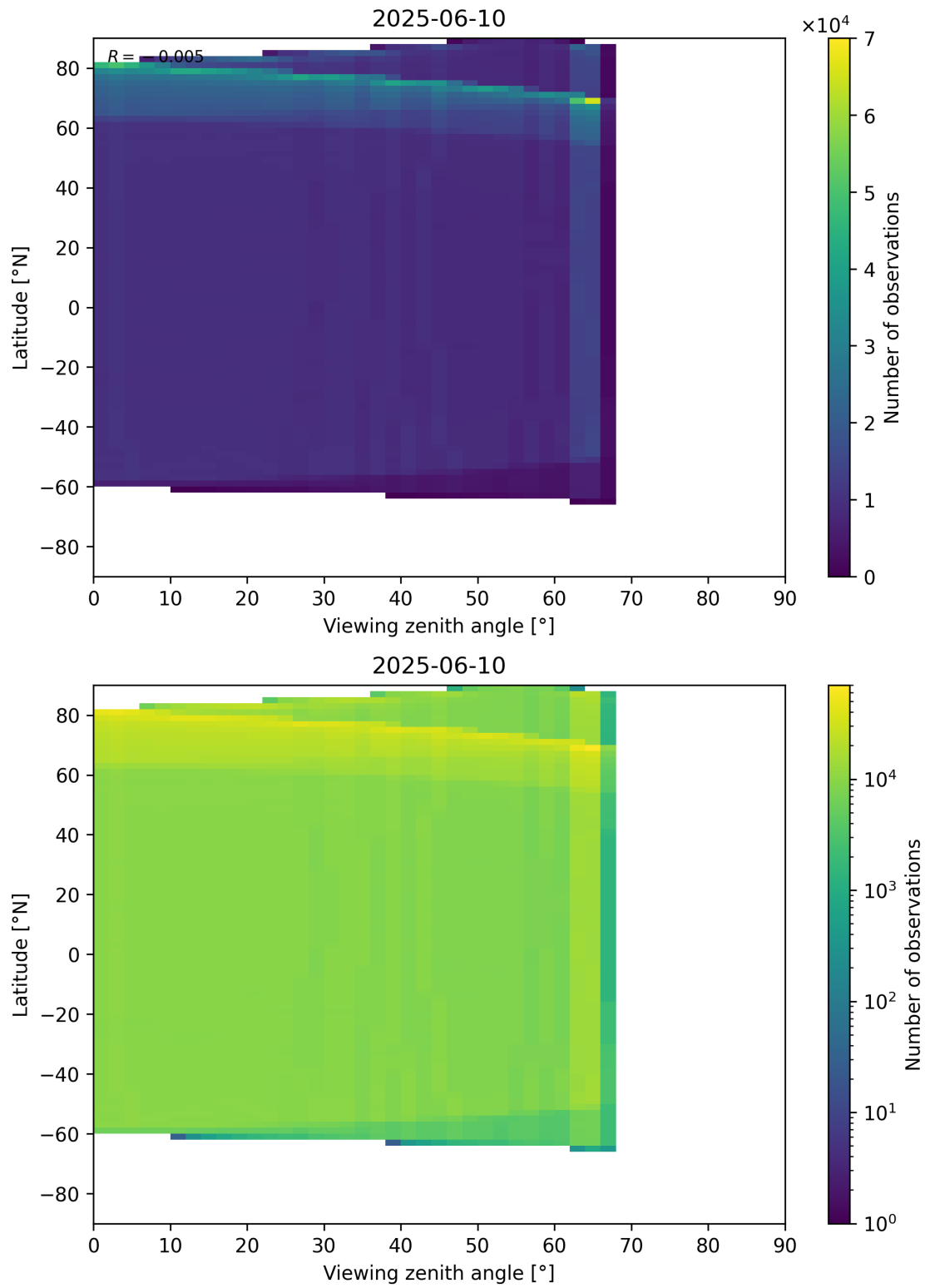
Figure 123: Scatter density plot of “Viewing zenith angle” against “Latitude” for 2025-06-09 to 2025-06-11.
