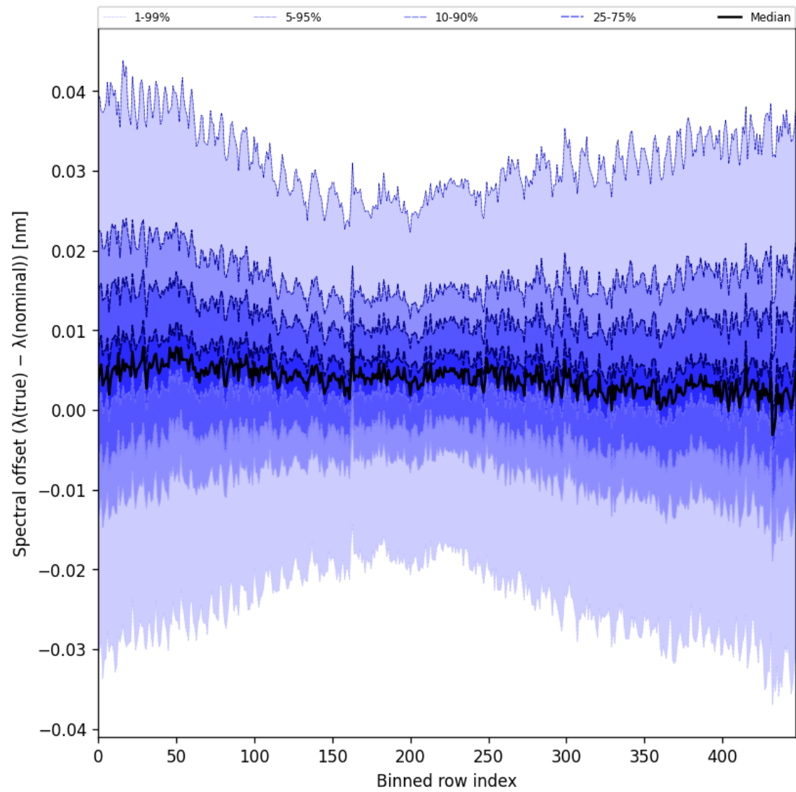
Figure 62: Along track statistics of “Spectral offset ( \lambda_{\text{true}} - \lambda_{\text{nominal}} )” for 2025-06-09 to 2025-06-11
