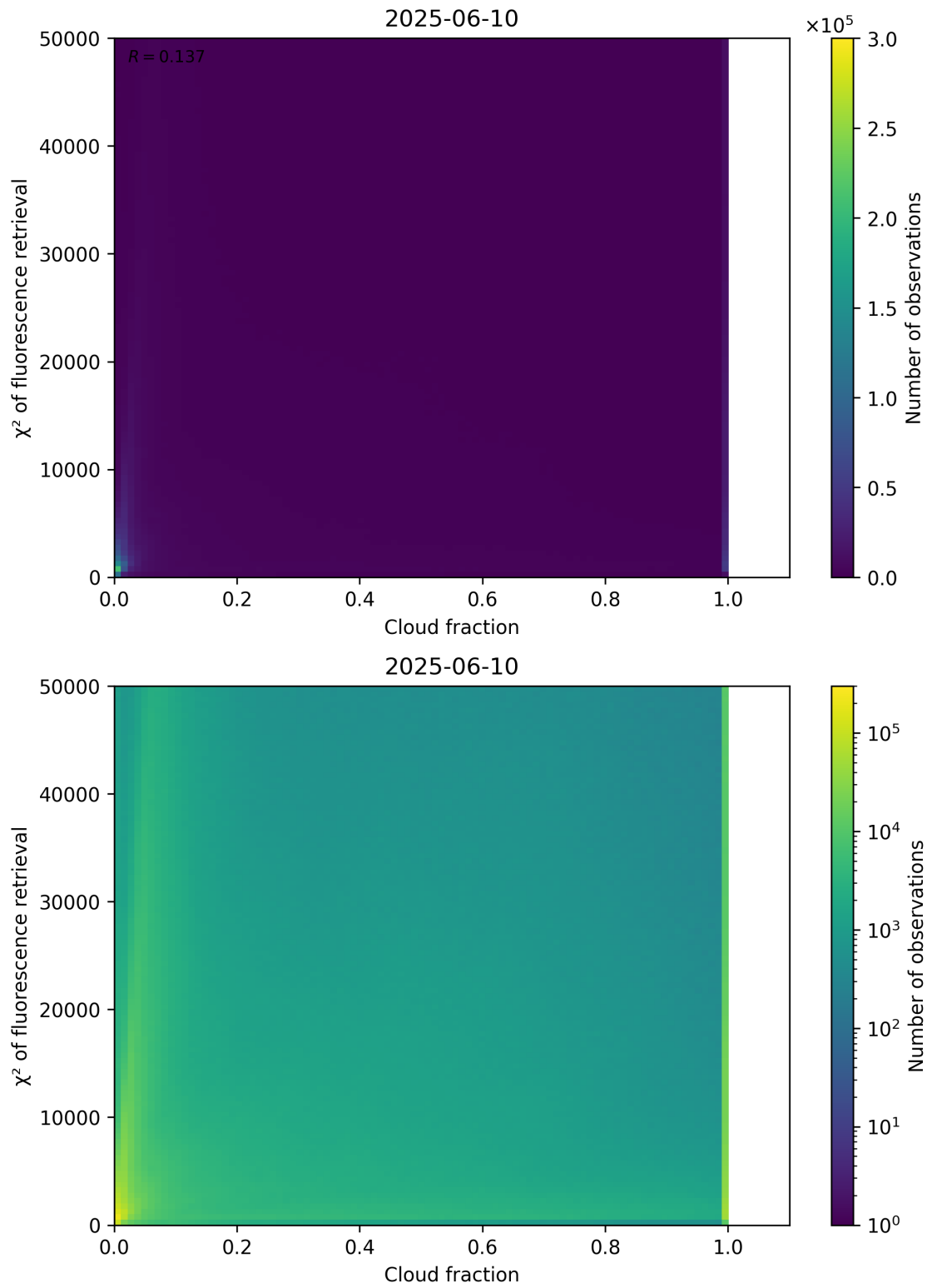
Figure 71: Scatter density plot of “Cloud fraction” against “ \chi^2 of fluorescence retrieval” for 2025-06-09 to 2025-06-11.
