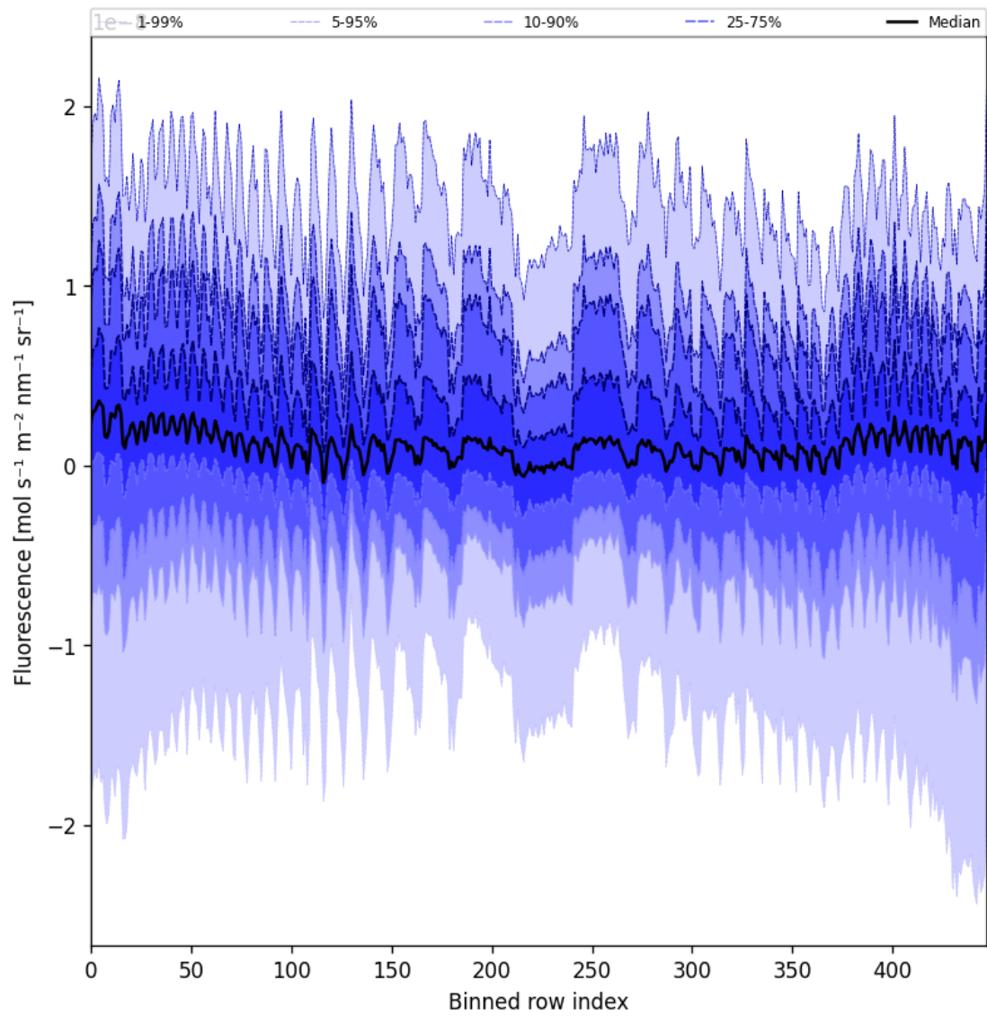
Figure 57: Along track statistics of “Fluorescence” for 2025-06-09 to 2025-06-11
