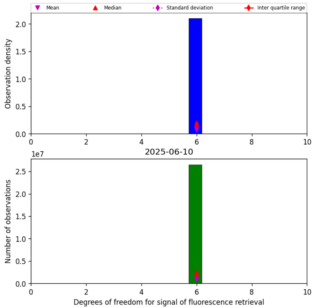
Figure 43: Histogram of "Degrees of freedom for signal of fluorescence retrieval" for 2025-06-09 to 2025-06-11
