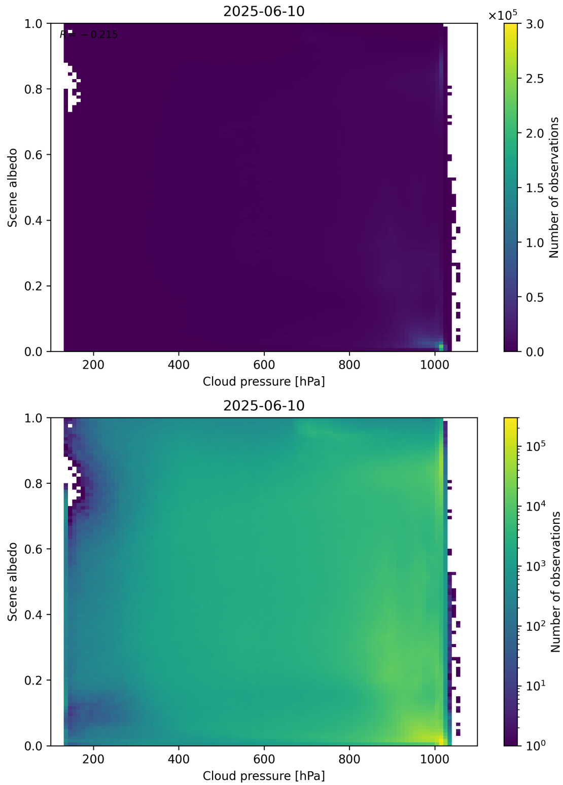
Figure 83: Scatter density plot of “Cloud pressure” against “Scene albedo” for 2025-06-09 to 2025-06-11.
