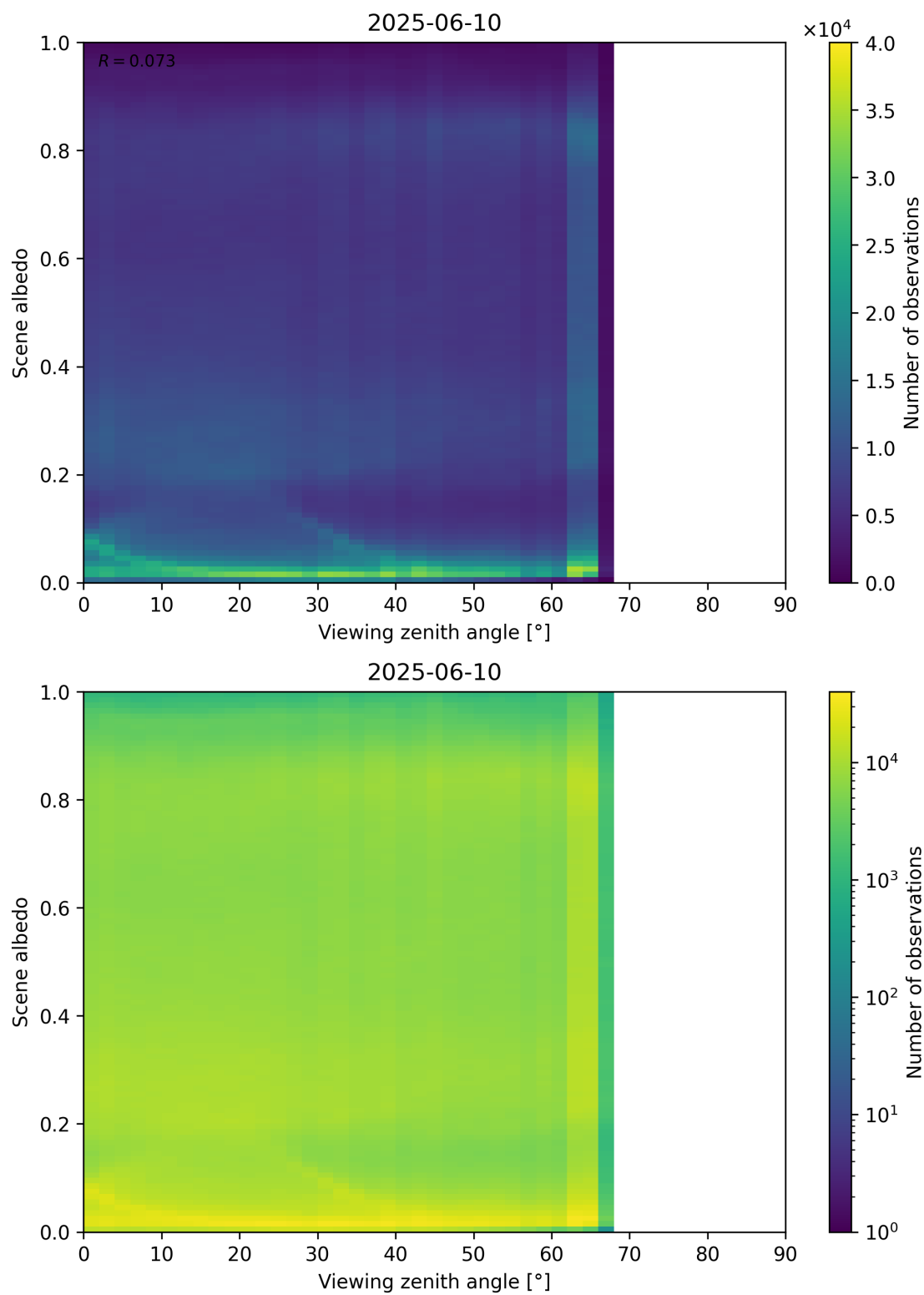
Figure 126: Scatter density plot of “Viewing zenith angle” against “Scene albedo” for 2025-06-09 to 2025-06-11.
