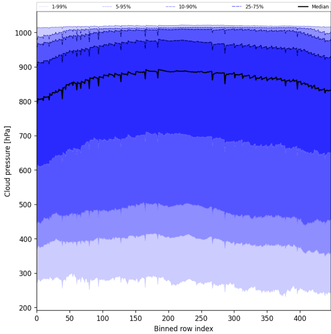
Figure 47: Along track statistics of “Cloud pressure” for 2025-06-09 to 2025-06-11
