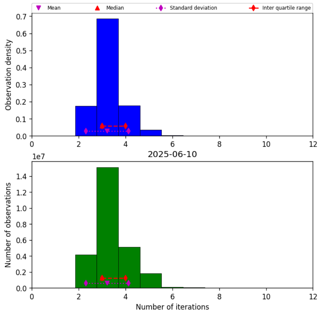
Figure 39: Histogram of “Number of iterations” for 2025-06-09 to 2025-06-11
