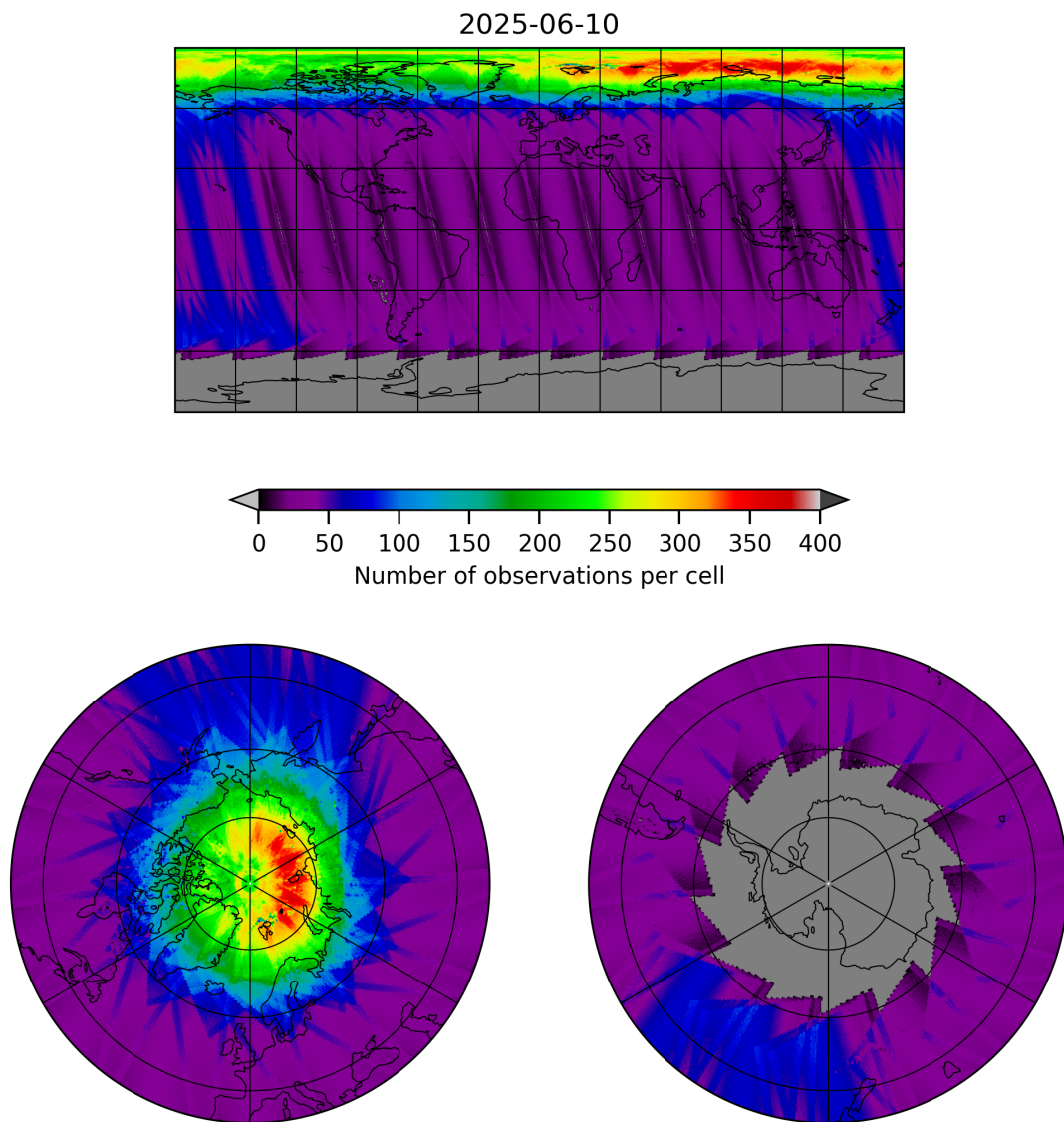
Figure 11: Map of the number of observations for 2025-06-09 to 2025-06-11
