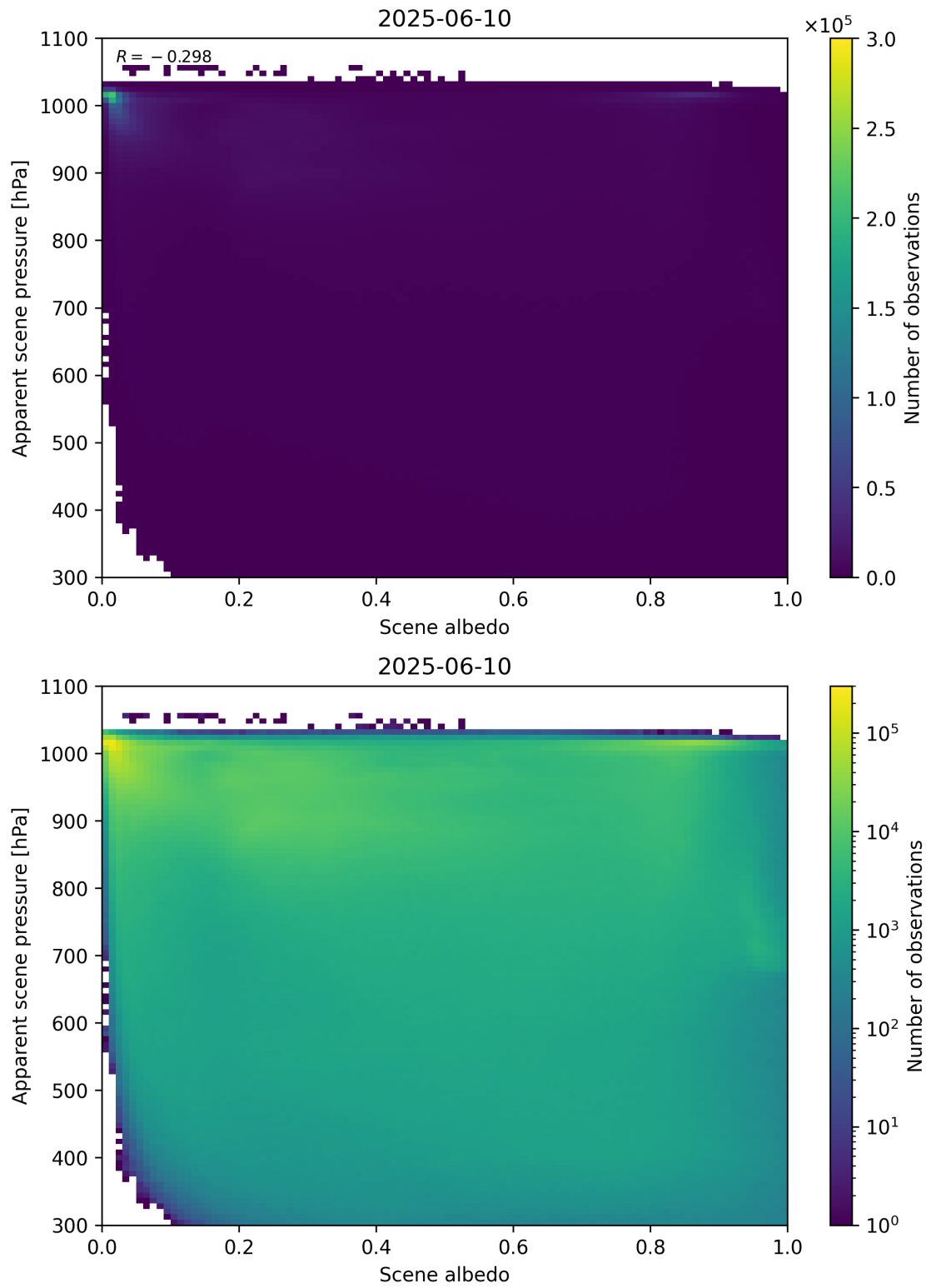
Figure 102: Scatter density plot of “Scene albedo” against “Apparent scene pressure” for 2025-06-09 to 2025-06-11.
