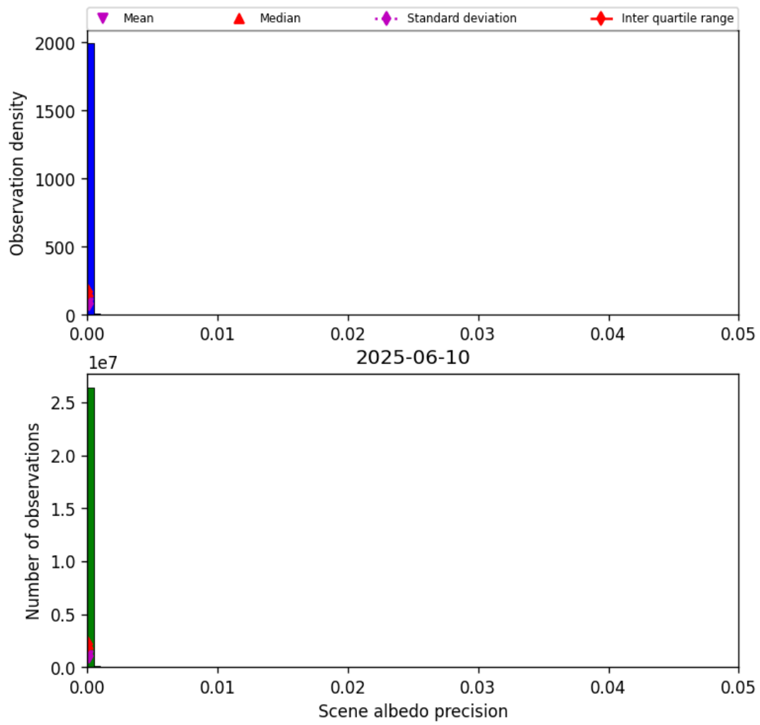
Figure 35: Histogram of “Scene albedo precision” for 2025-06-09 to 2025-06-11
