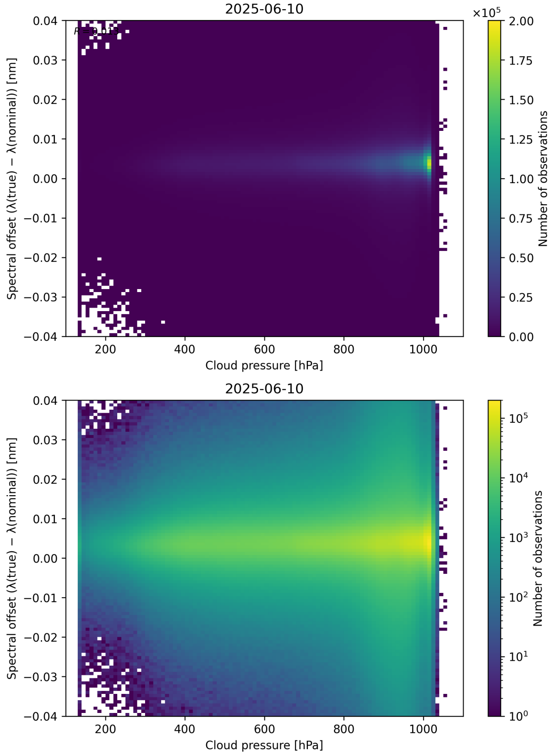
Figure 84: Scatter density plot of “Cloud pressure” against “Spectral offset ( \lambda_{\text{true}} - \lambda_{\text{nominal}} )” for 2025-06-09 to 2025-06-11.
