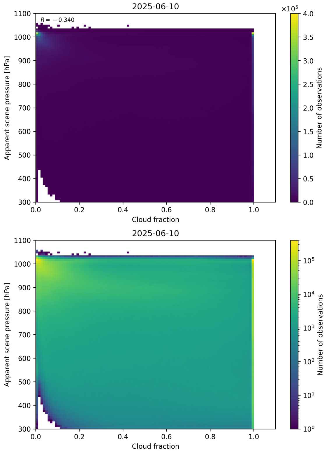
Figure 70: Scatter density plot of “Cloud fraction” against “Apparent scene pressure” for 2025-06-09 to 2025-06-11.
