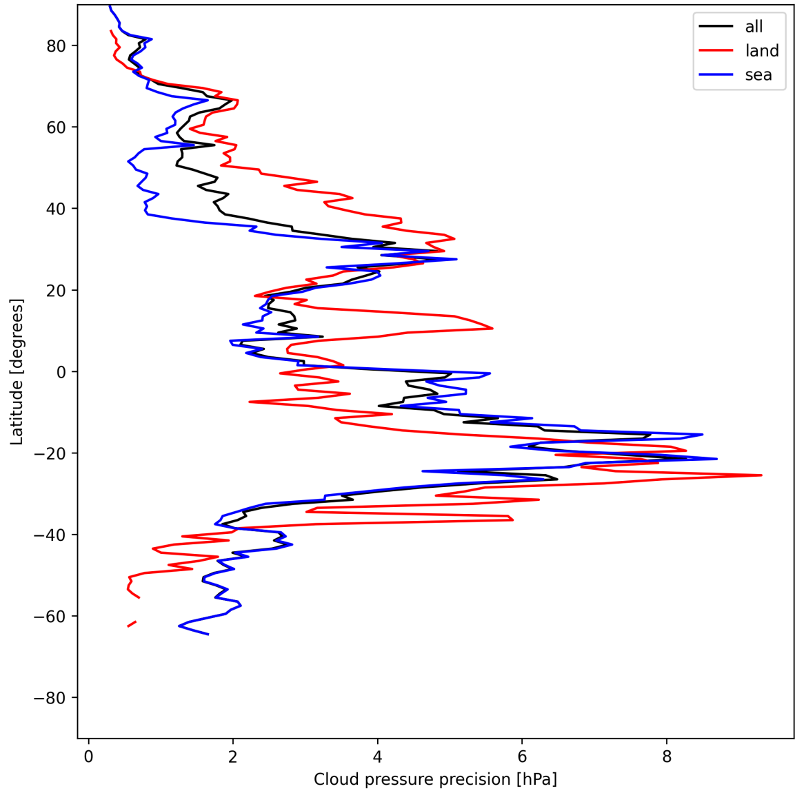
Figure 14: Zonal average of “Cloud pressure precision” for 2025-06-09 to 2025-06-11.
