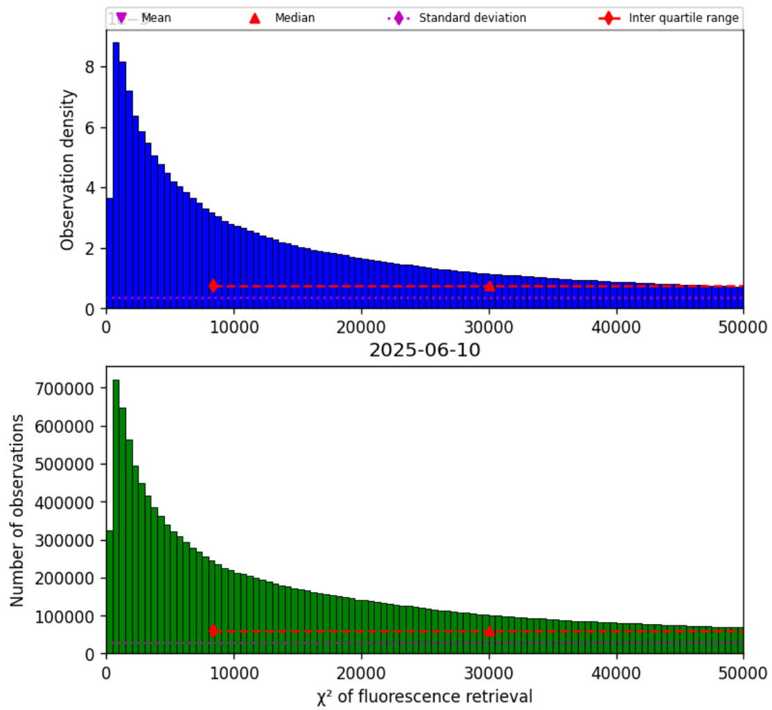
Figure 42: Histogram of “ \chi^2 of fluorescence retrieval” for 2025-06-09 to 2025-06-11
