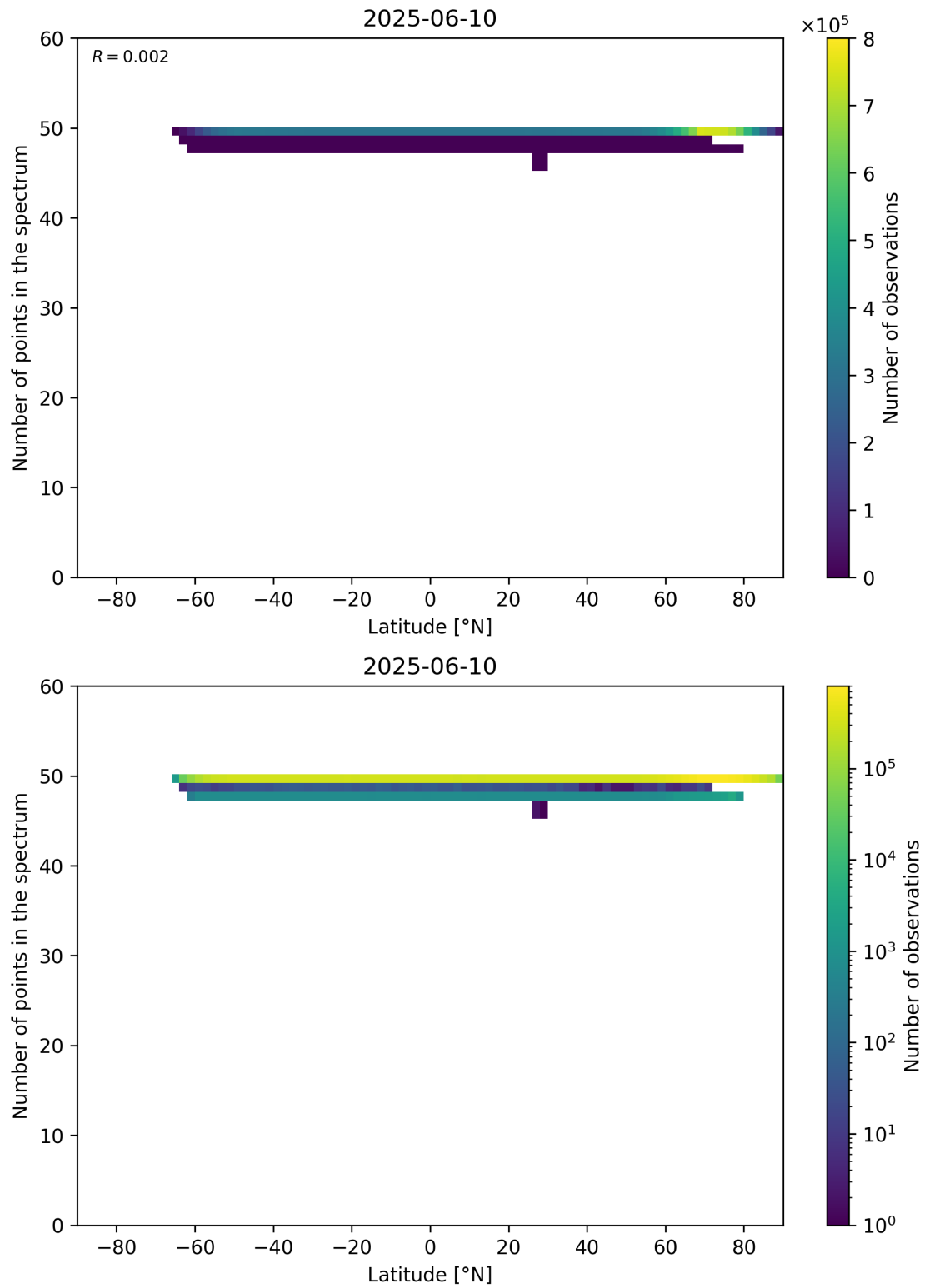
Figure 94: Scatter density plot of “Latitude” against “Number of points in the spectrum” for 2025-06-09 to 2025-06-11.
