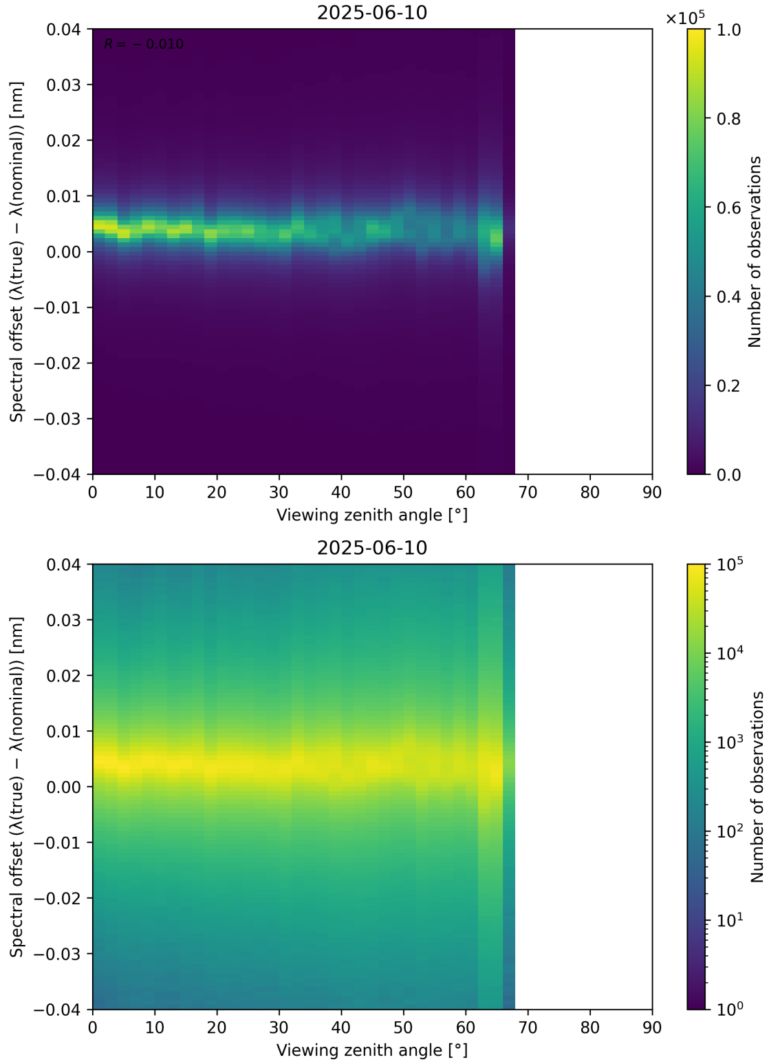
Figure 128: Scatter density plot of “Viewing zenith angle” against “Spectral offset ( \lambda_{\text{true}} - \lambda_{\text{nominal}} )” for 2025-06-09 to 2025-06-11.
