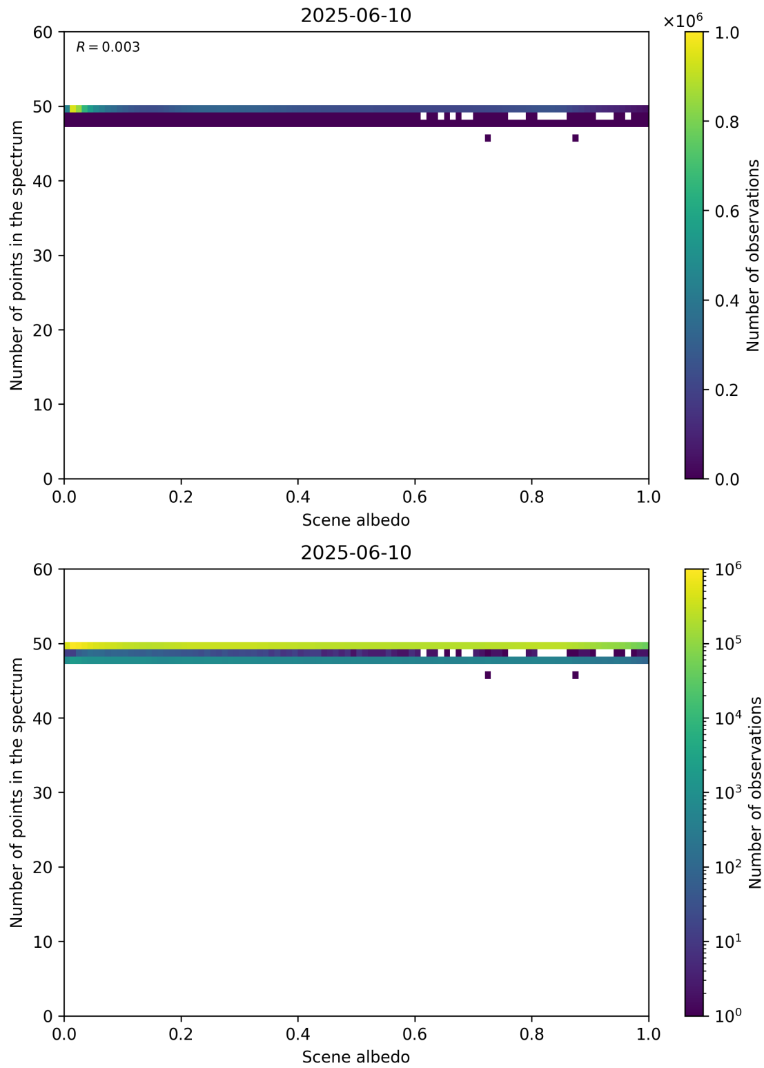
Figure 106: Scatter density plot of “Scene albedo” against “Number of points in the spectrum” for 2025-06-09 to 2025-06-11.
