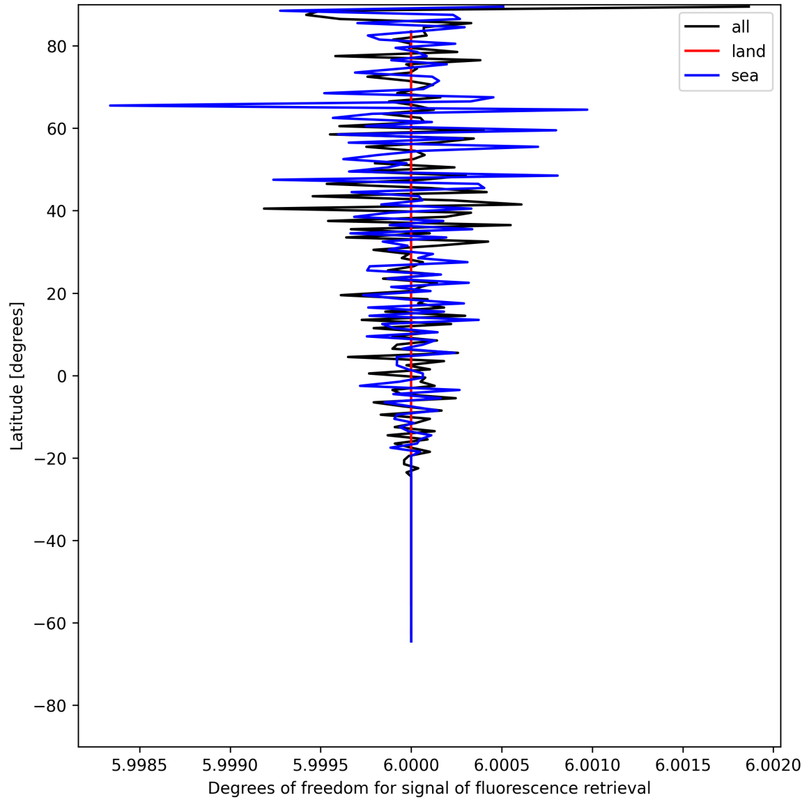
Figure 26: Zonal average of “Degrees of freedom for signal of fluorescence retrieval” for 2025-06-09 to 2025-06-11.
