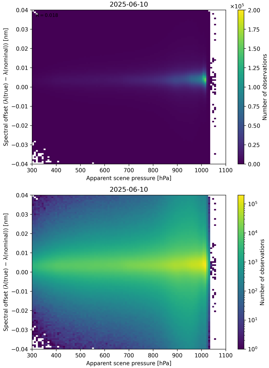
Figure 67: Scatter density plot of “Apparent scene pressure” against “Spectral offset ( \lambda_{\text{true}} - \lambda_{\text{nominal}} )” for 2025-06-09 to 2025-06-11.
