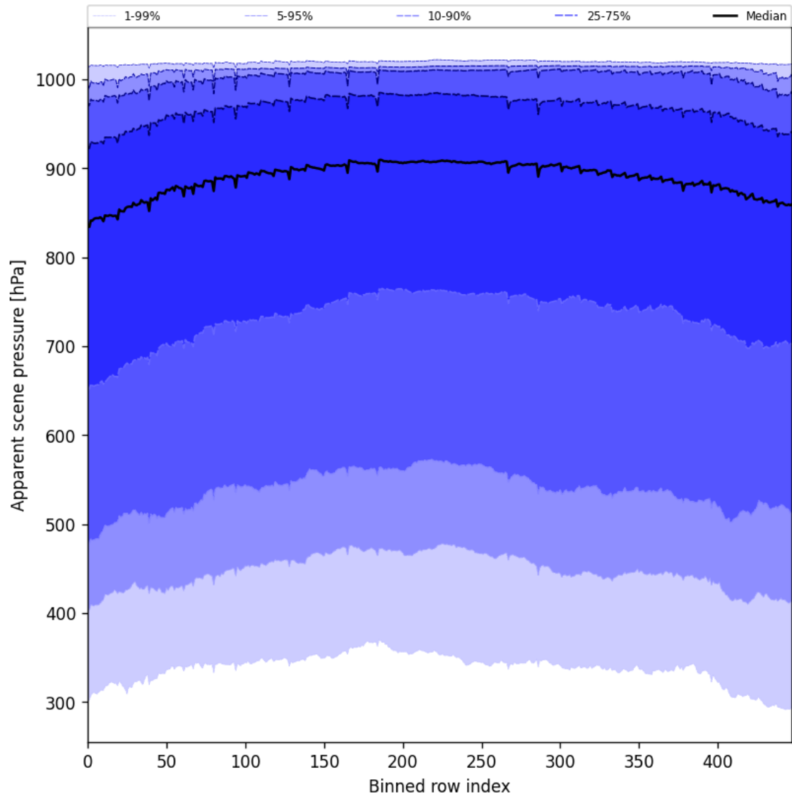
Figure 53: Along track statistics of “Apparent scene pressure” for 2025-06-09 to 2025-06-11
