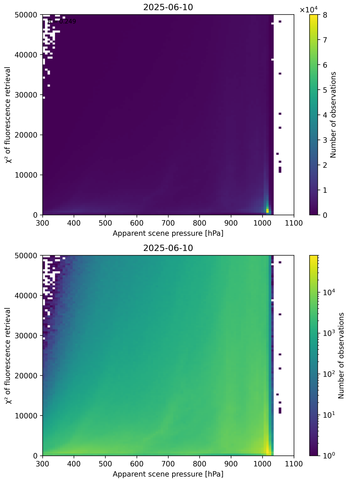
Figure 63: Scatter density plot of “Apparent scene pressure” against “ \chi^2 of fluorescence retrieval” for 2025-06-09 to 2025-06-11.
