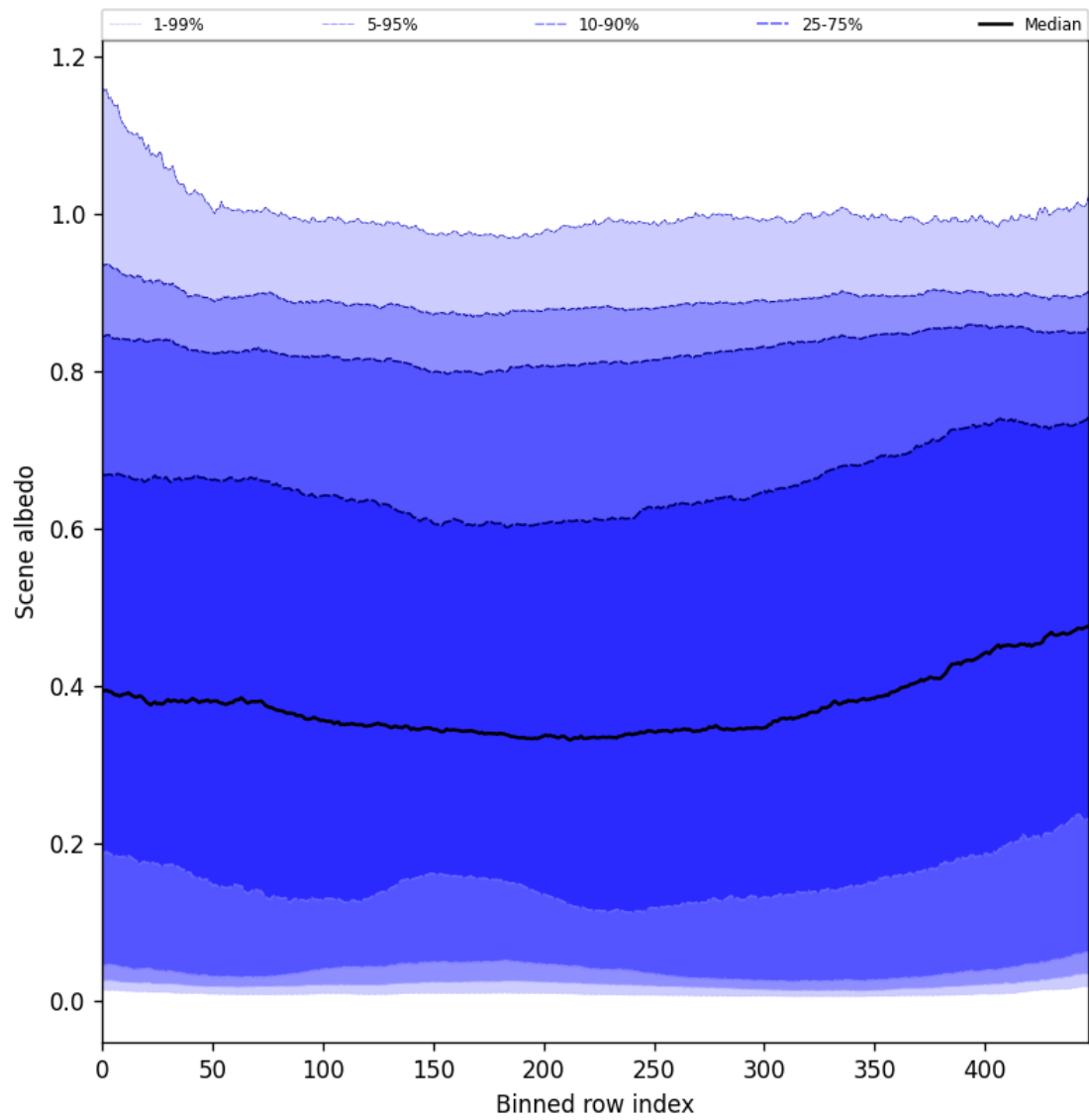
Figure 51: Along track statistics of “Scene albedo” for 2025-06-09 to 2025-06-11
