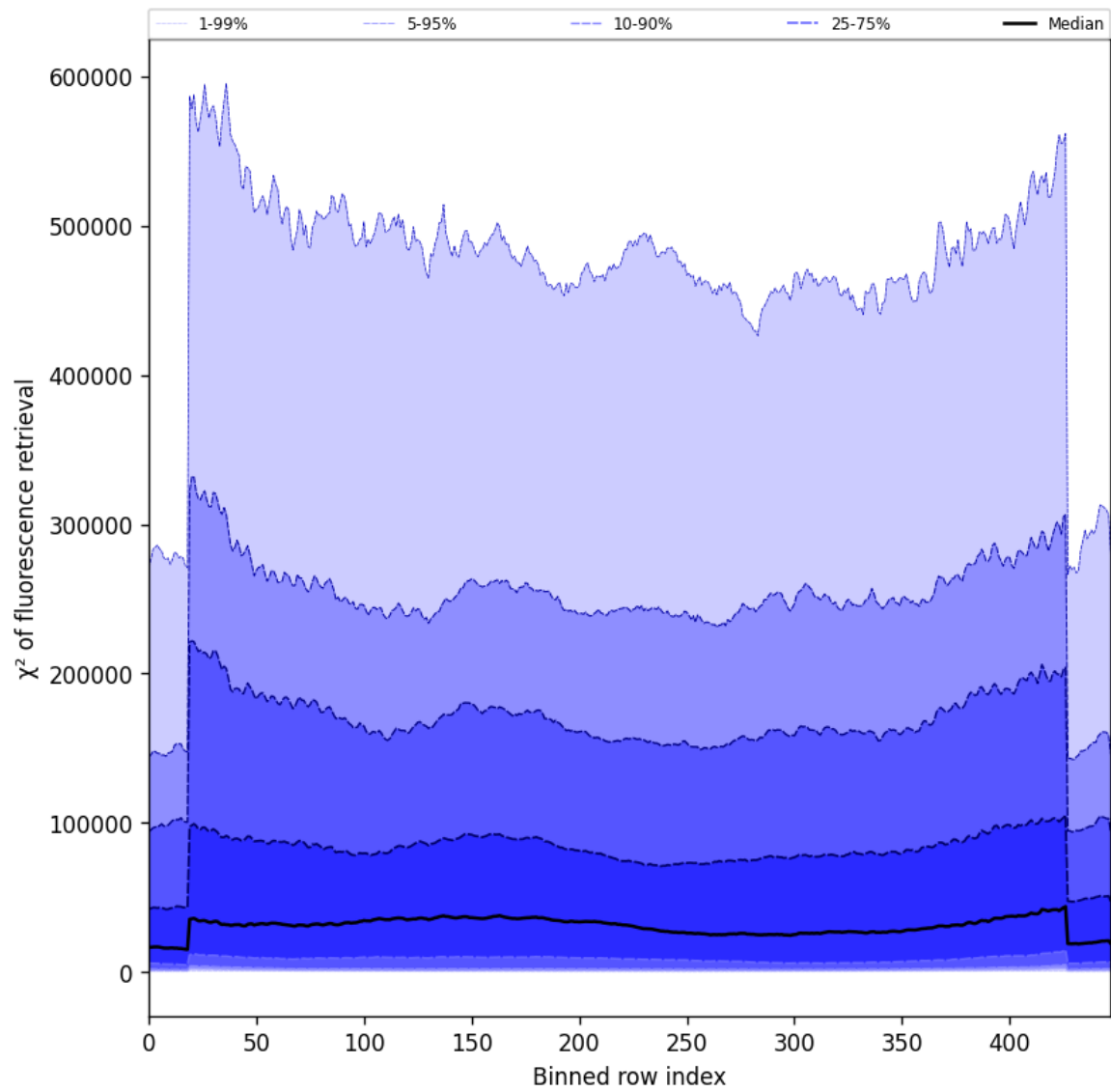
Figure 59: Along track statistics of “ \chi^2 of fluorescence retrieval” for 2025-06-09 to 2025-06-11
