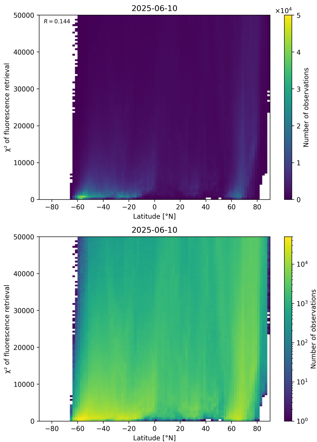
Figure 89: Scatter density plot of “Latitude” against “ \chi^2 of fluorescence retrieval” for 2025-06-09 to 2025-06-11.
