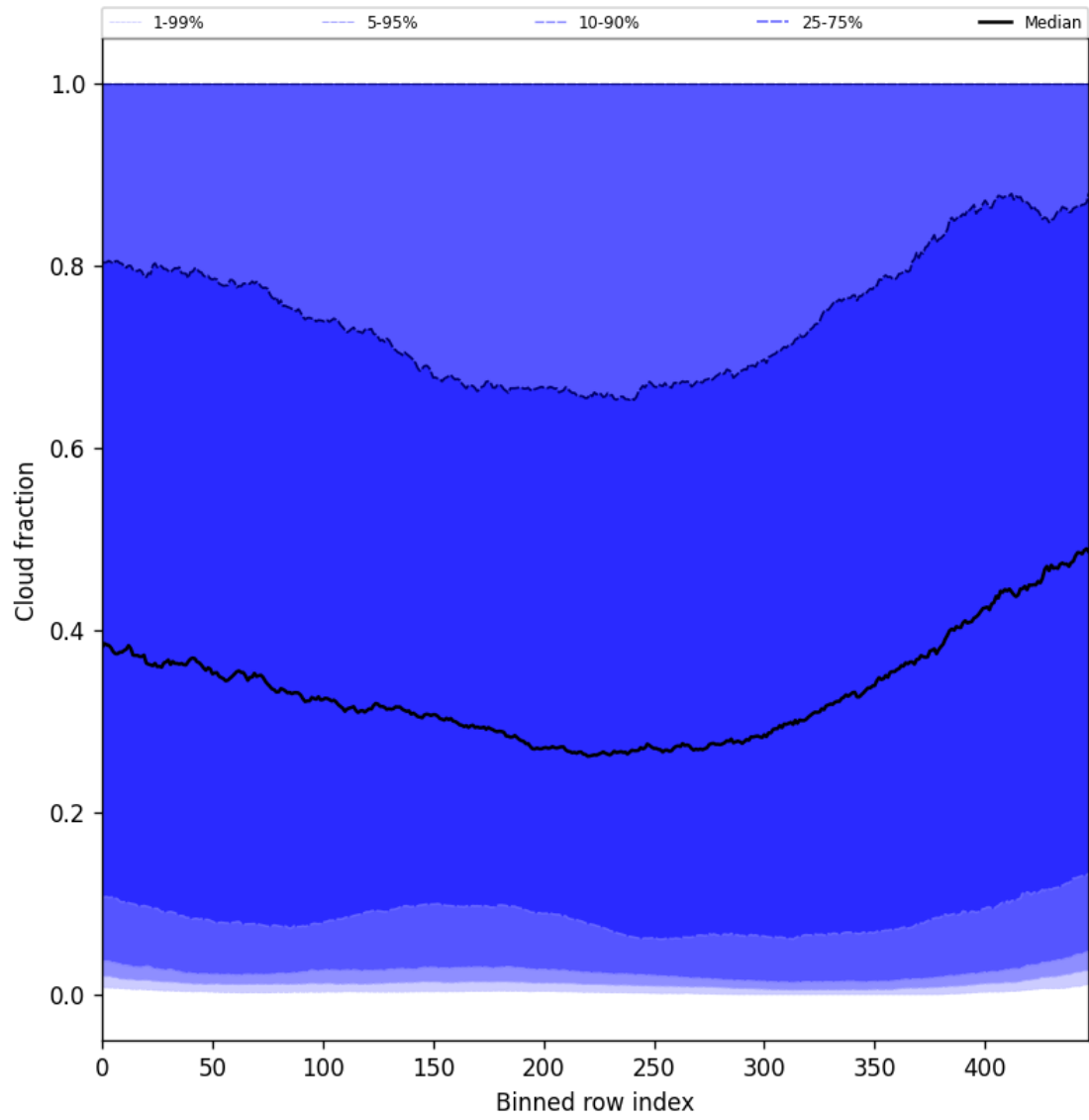
Figure 49: Along track statistics of “Cloud fraction” for 2025-06-09 to 2025-06-11
