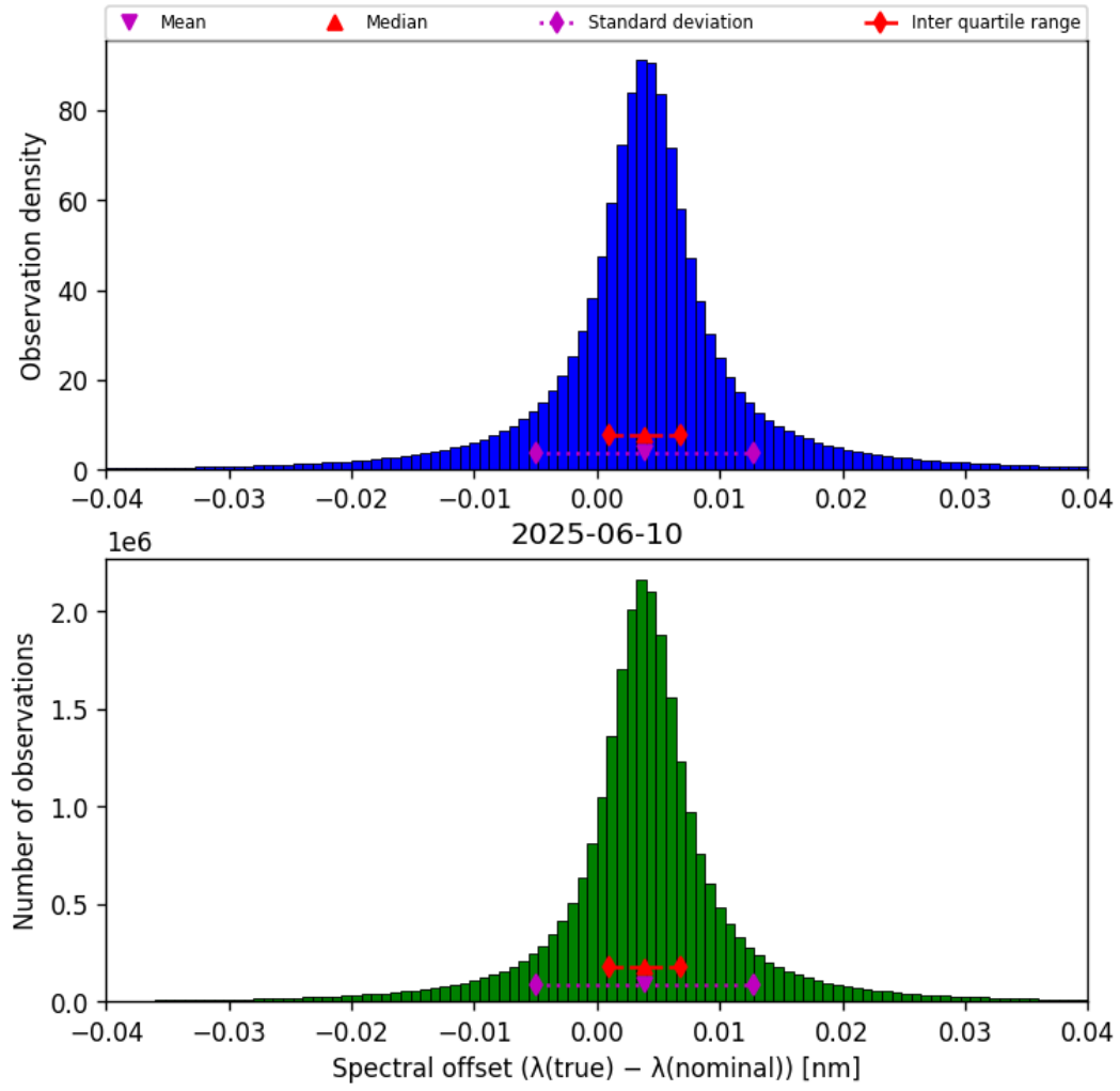
Figure 45: Histogram of “Spectral offset ( \lambda_{\text{true}} - \lambda_{\text{nominal}} )” for 2025-06-09 to 2025-06-11
