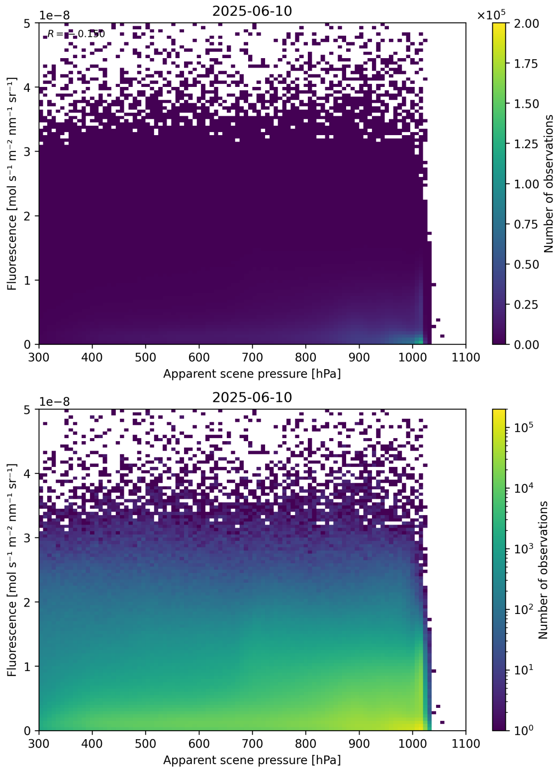
Figure 64: Scatter density plot of “Apparent scene pressure” against “Fluorescence” for 2025-06-09 to 2025-06-11.
