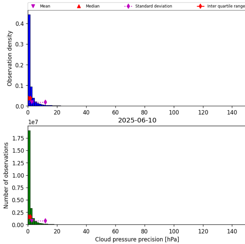
Figure 31: Histogram of “Cloud pressure precision” for 2025-06-09 to 2025-06-11
