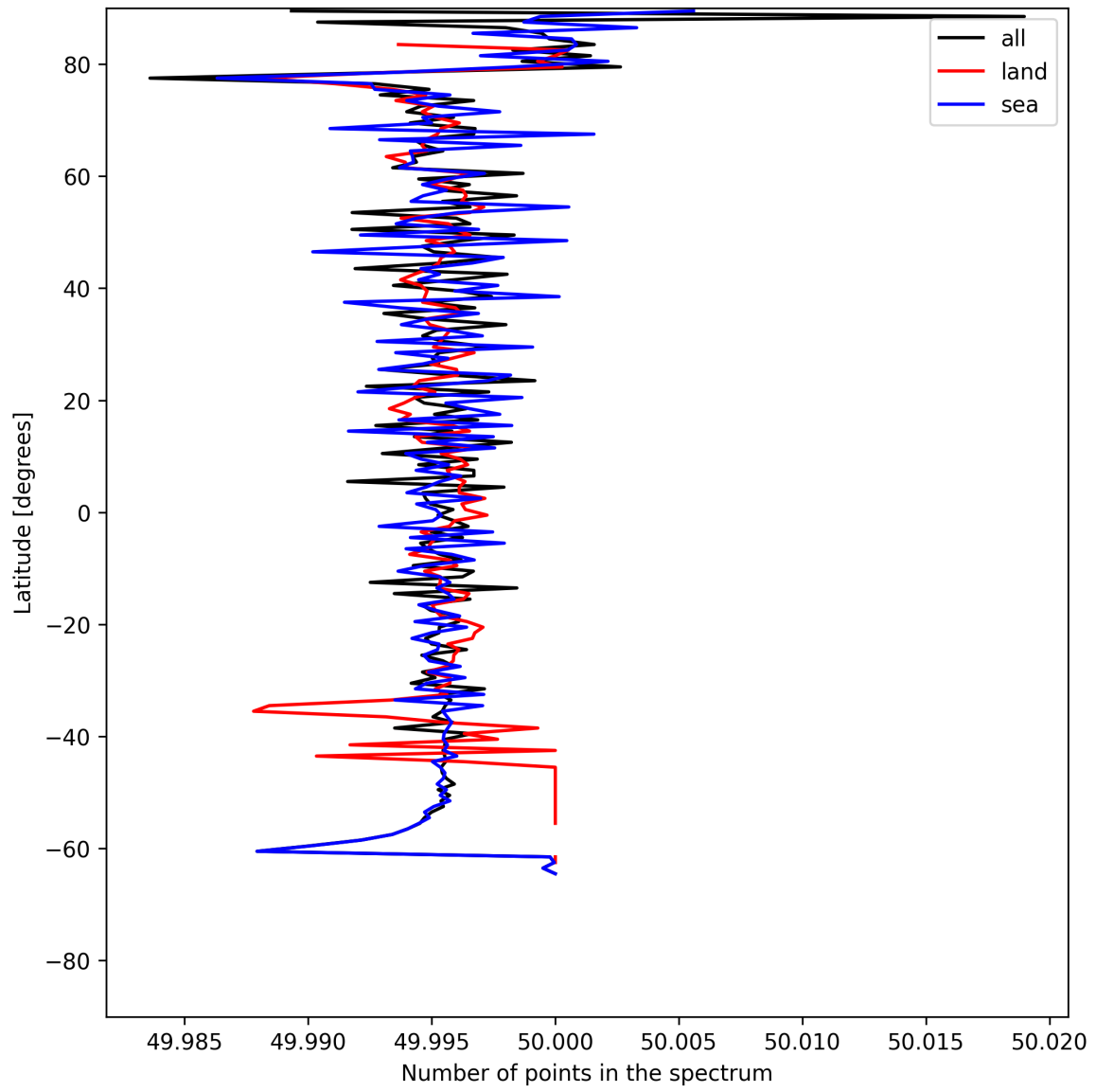
Figure 27: Zonal average of “Number of points in the spectrum” for 2025-06-09 to 2025-06-11.
