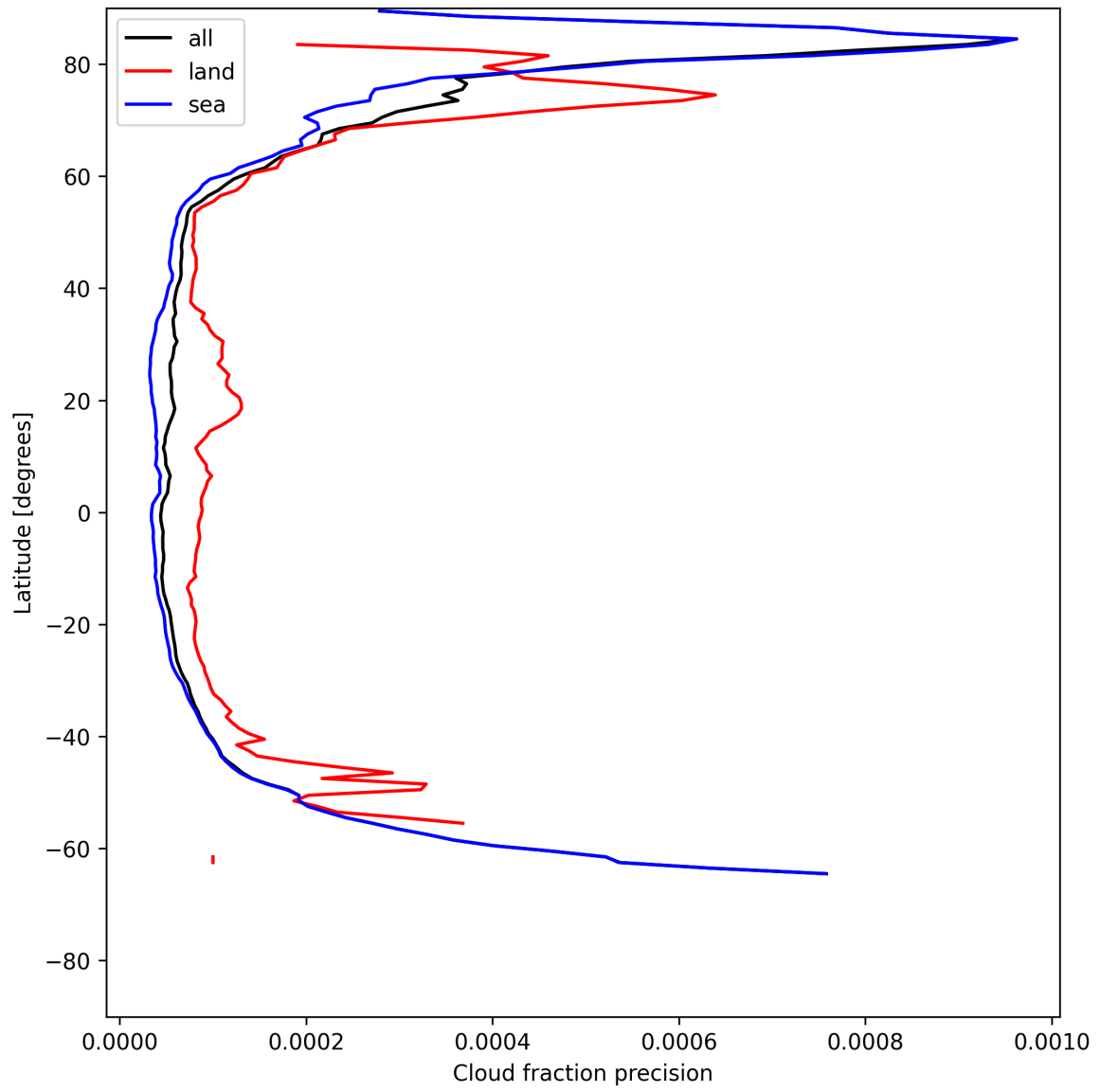
Figure 16: Zonal average of “Cloud fraction precision” for 2025-06-09 to 2025-06-11.
