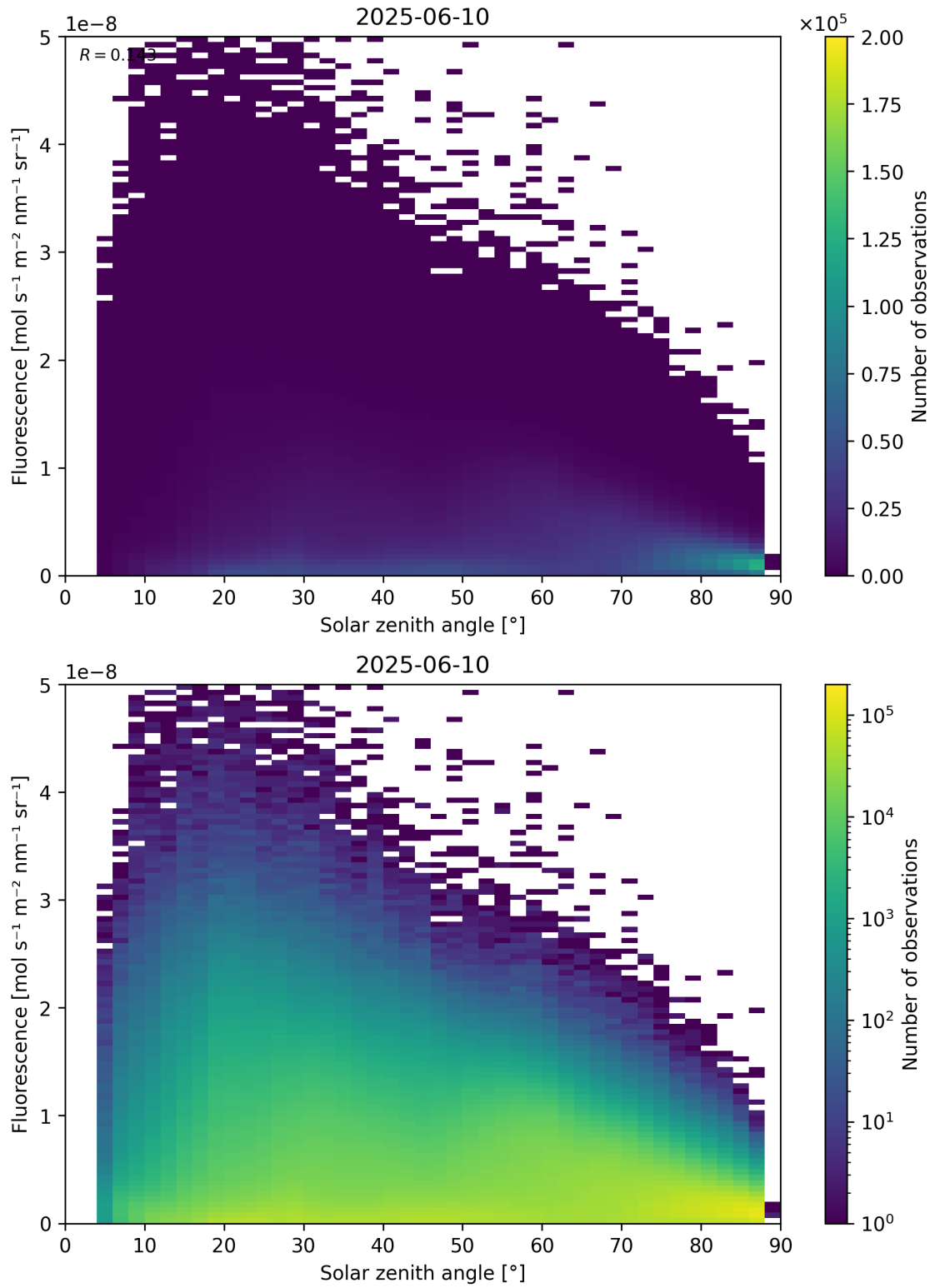
Figure 112: Scatter density plot of “Solar zenith angle” against “Fluorescence” for 2025-06-09 to 2025-06-11.
