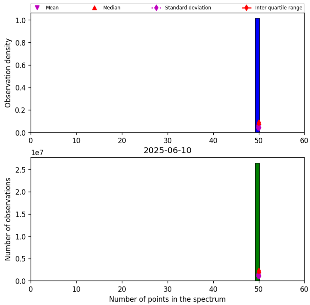
Figure 44: Histogram of “Number of points in the spectrum” for 2025-06-09 to 2025-06-11
