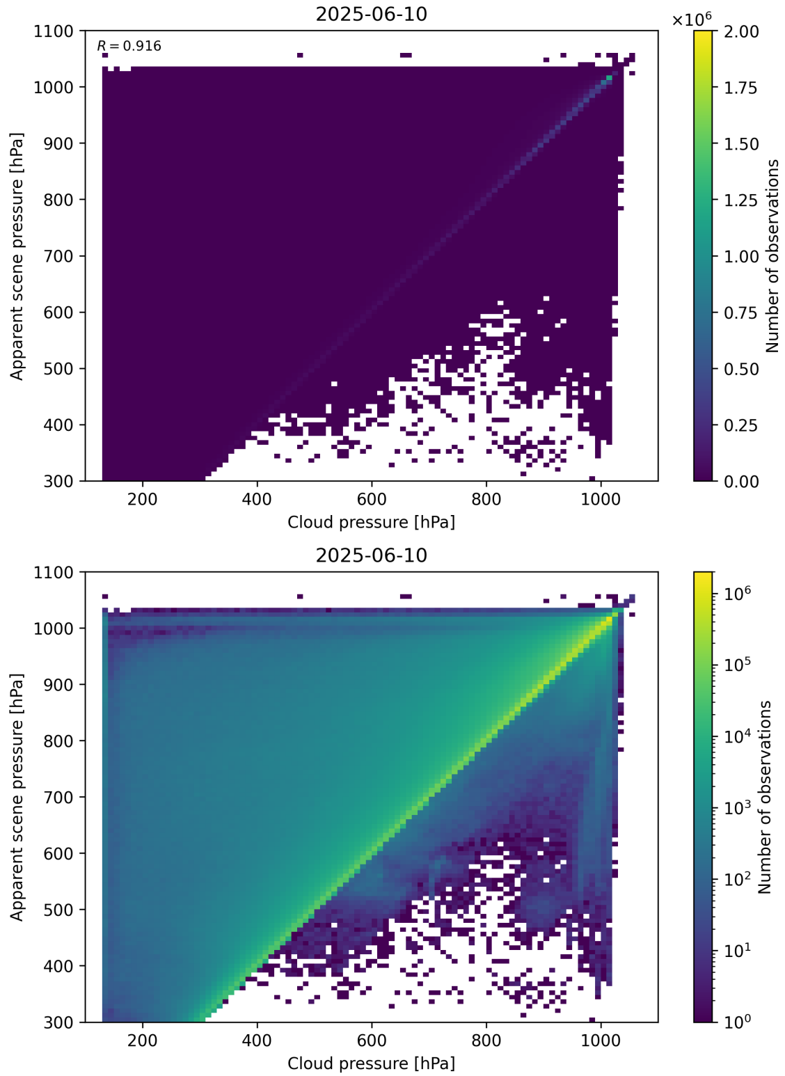
Figure 77: Scatter density plot of “Cloud pressure” against “Apparent scene pressure” for 2025-06-09 to 2025-06-11.
