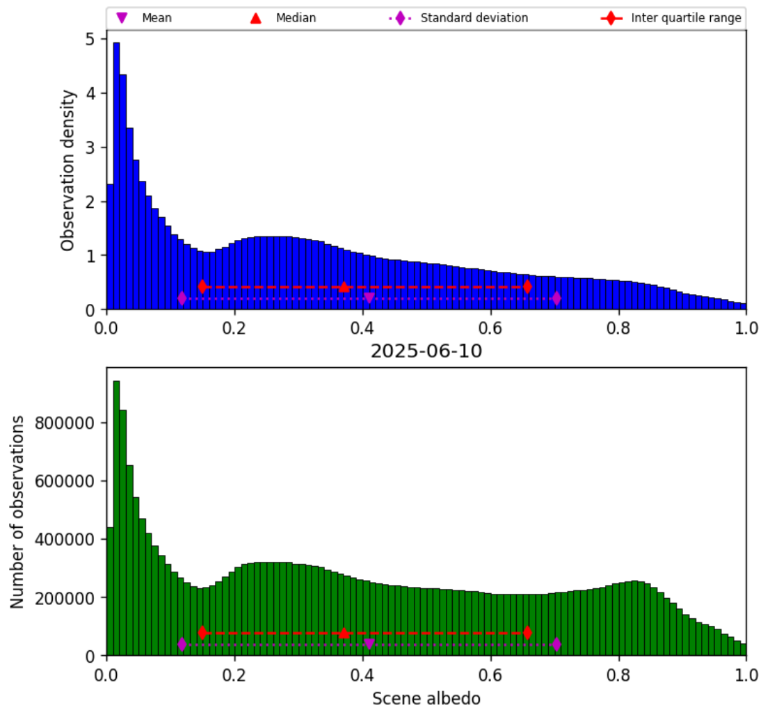
Figure 34: Histogram of “Scene albedo” for 2025-06-09 to 2025-06-11
