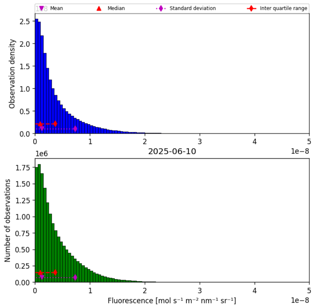
Figure 40: Histogram of “Fluorescence” for 2025-06-09 to 2025-06-11
