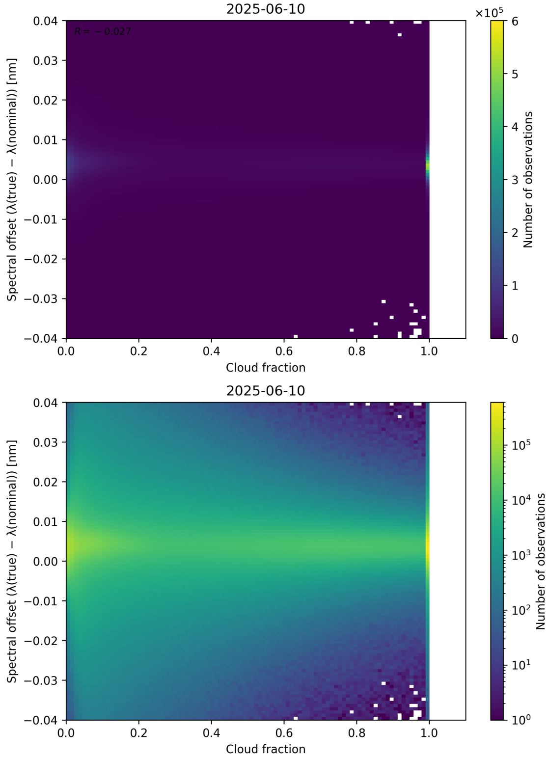
Figure 76: Scatter density plot of “Cloud fraction” against “Spectral offset ( \lambda_{\text{true}} - \lambda_{\text{nominal}} )” for 2025-06-09 to 2025-06-11.
