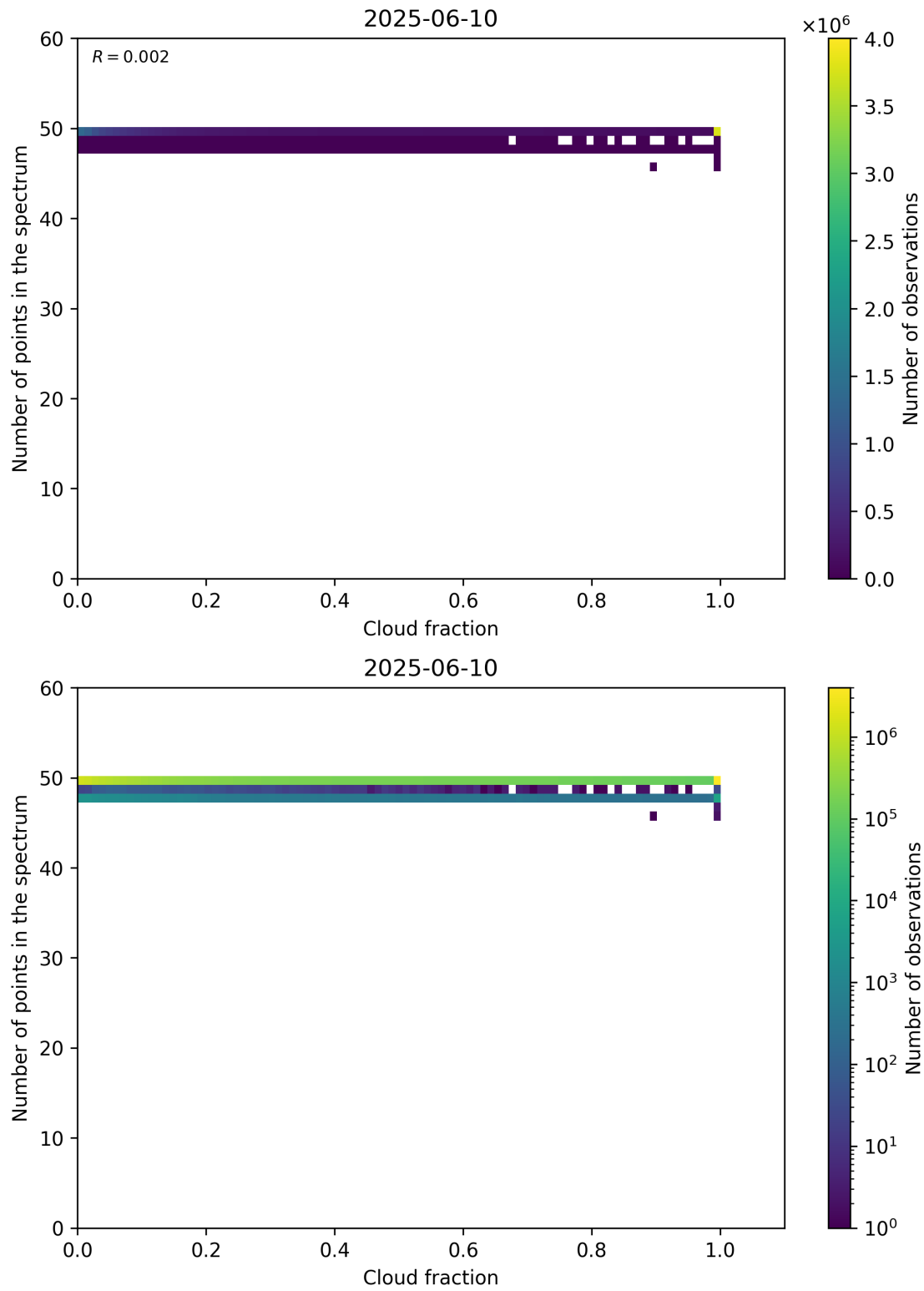
Figure 74: Scatter density plot of “Cloud fraction” against “Number of points in the spectrum” for 2025-06-09 to 2025-06-11.
