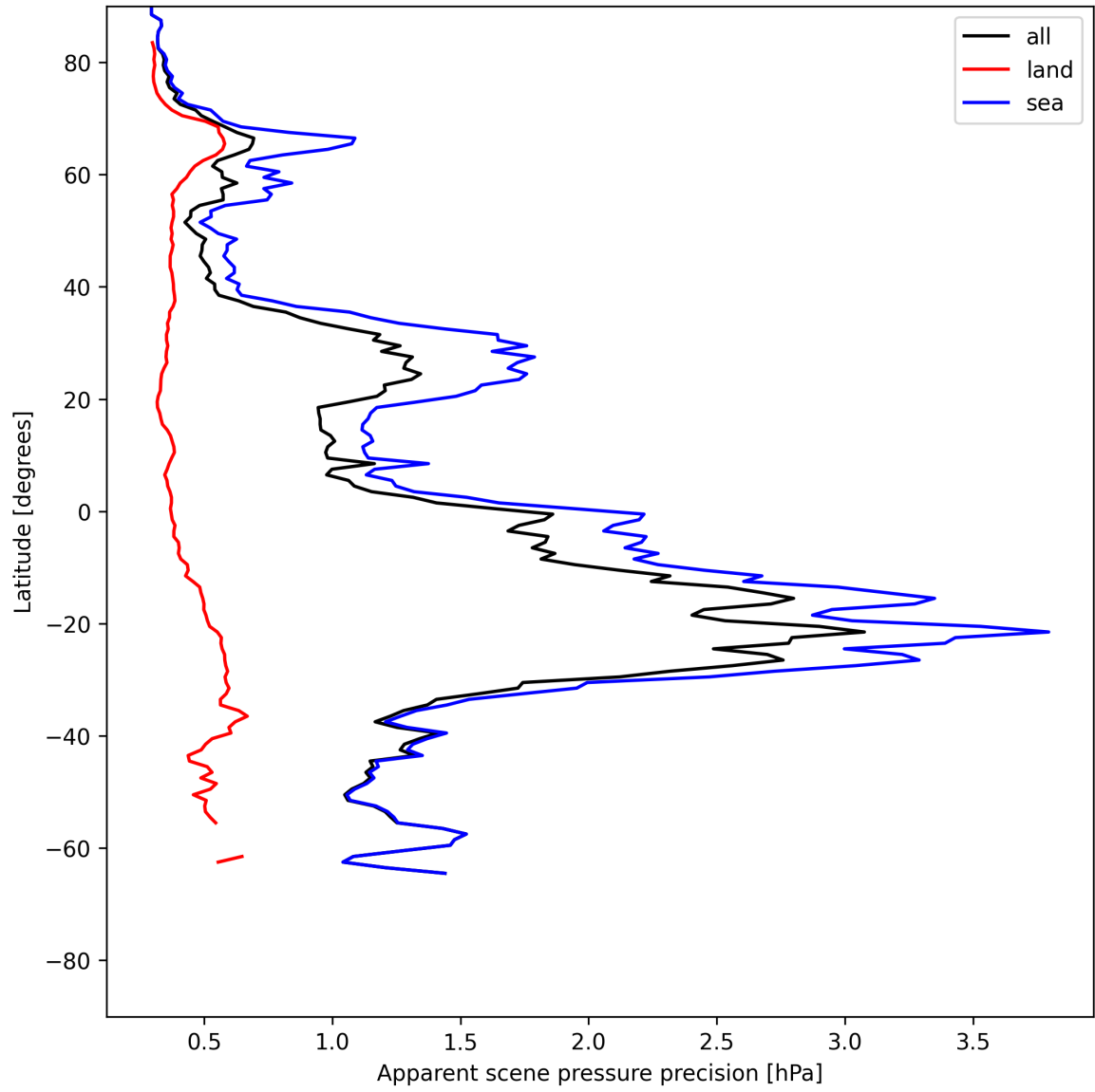
Figure 20: Zonal average of “Apparent scene pressure precision” for 2025-06-09 to 2025-06-11.
