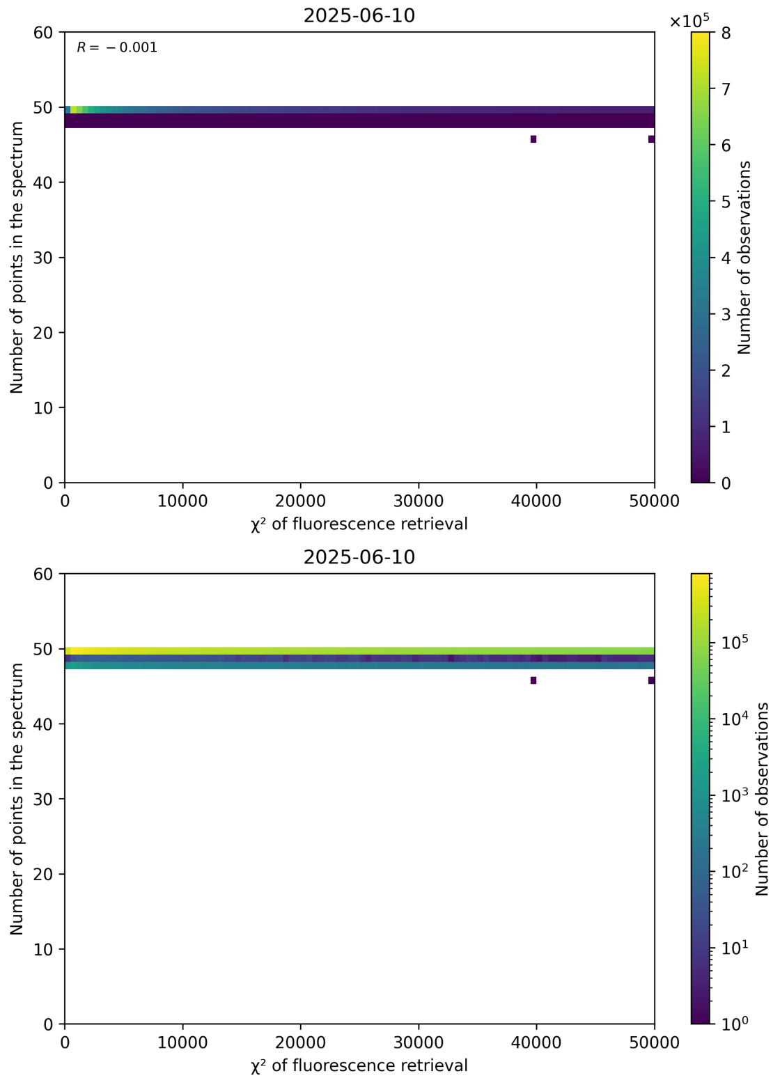
Figure 68: Scatter density plot of “ \chi^2 of fluorescence retrieval” against “Number of points in the spectrum” for 2025-06-09 to 2025-06-11.
