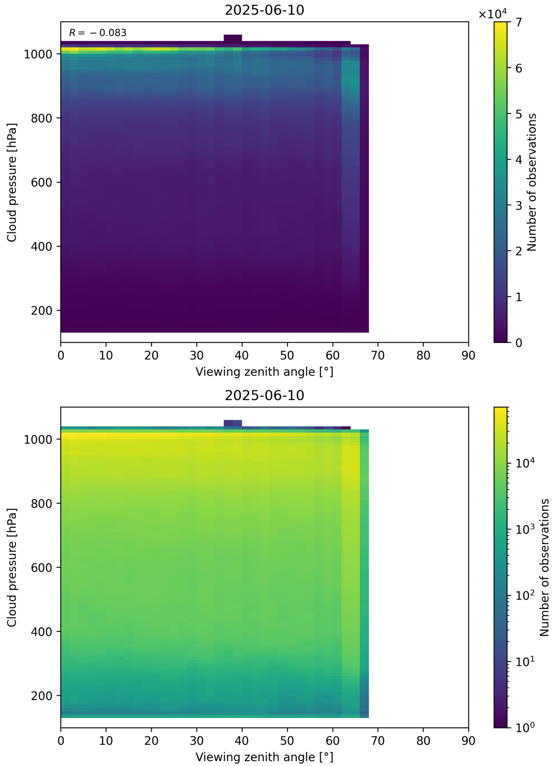
Figure 121: Scatter density plot of “Viewing zenith angle” against “Cloud pressure” for 2025-06-09 to 2025-06-11.
