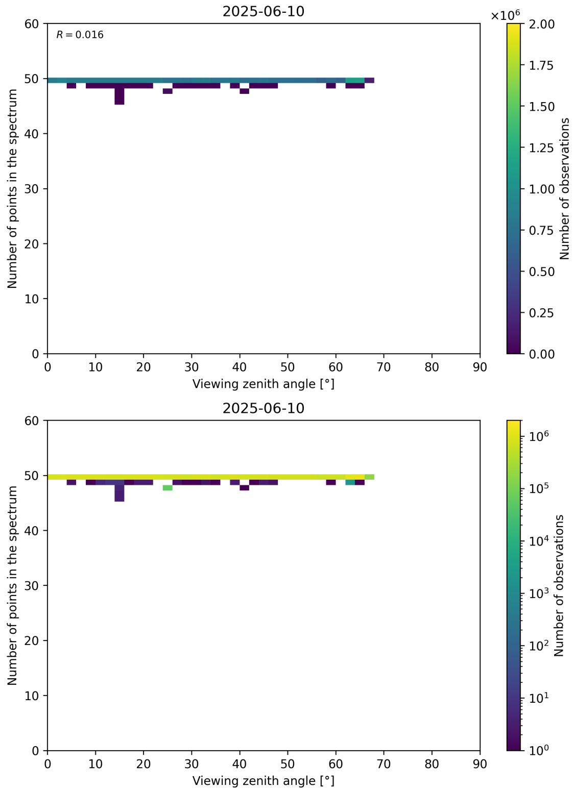
Figure 125: Scatter density plot of “Viewing zenith angle” against “Number of points in the spectrum” for 2025-06-09 to 2025-06-11.
