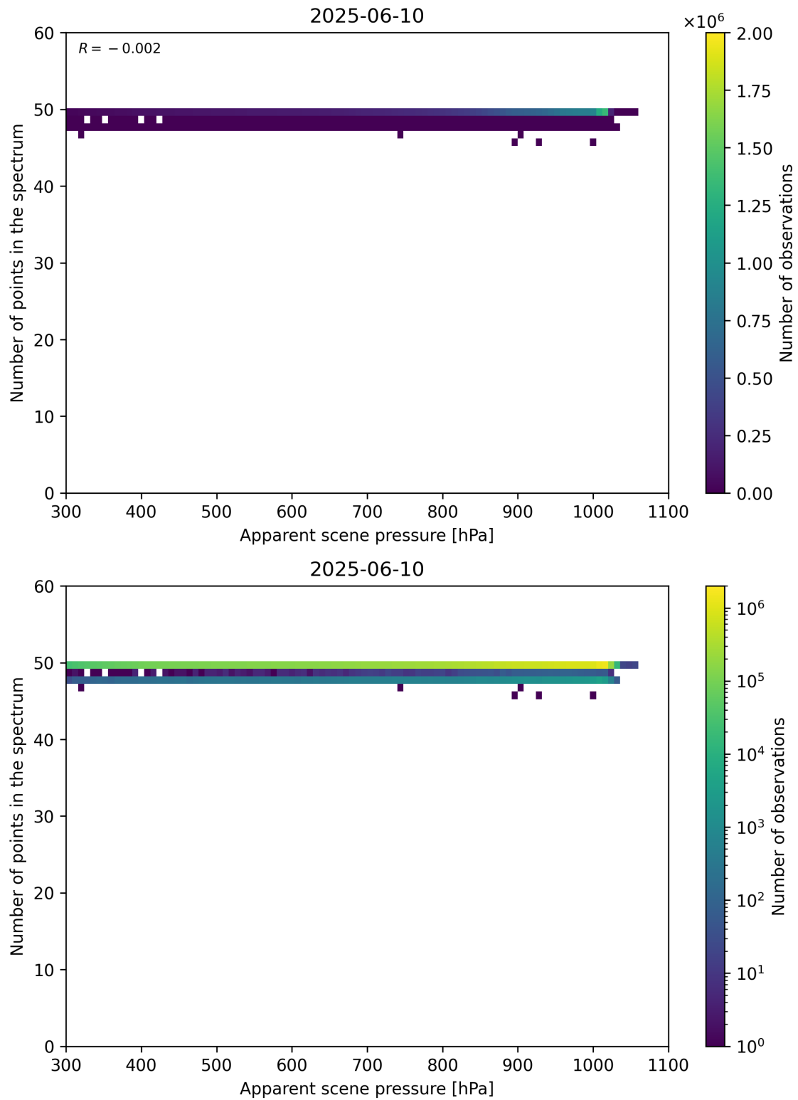
Figure 66: Scatter density plot of “Apparent scene pressure” against “Number of points in the spectrum” for 2025-06-09 to 2025-06-11.
