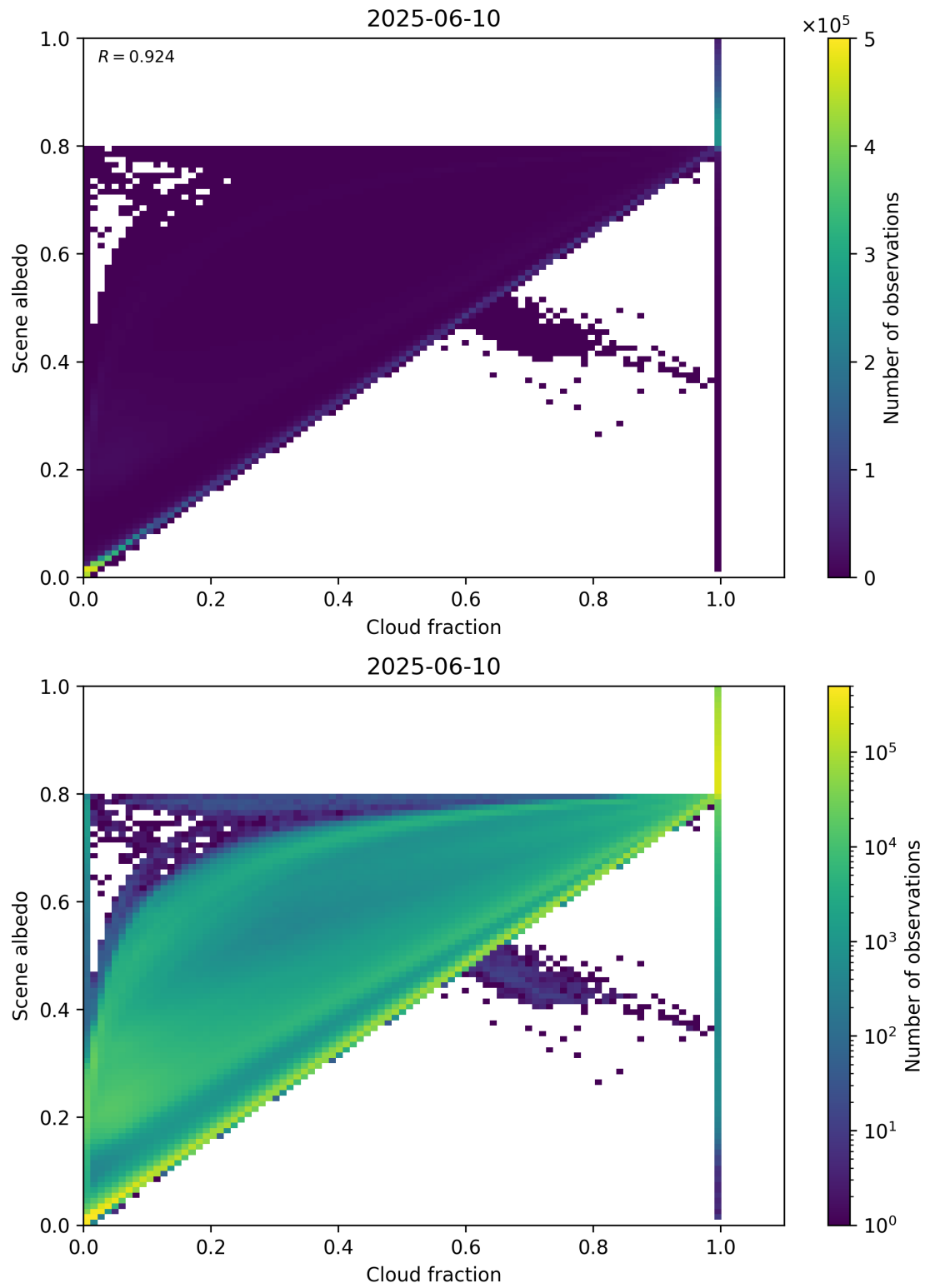
Figure 75: Scatter density plot of “Cloud fraction” against “Scene albedo” for 2025-06-09 to 2025-06-11.
