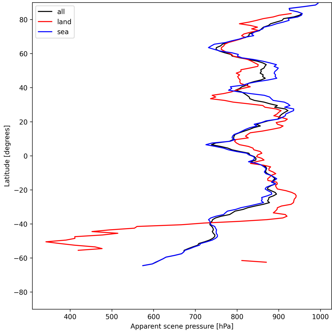
Figure 19: Zonal average of “Apparent scene pressure” for 2025-06-09 to 2025-06-11.
