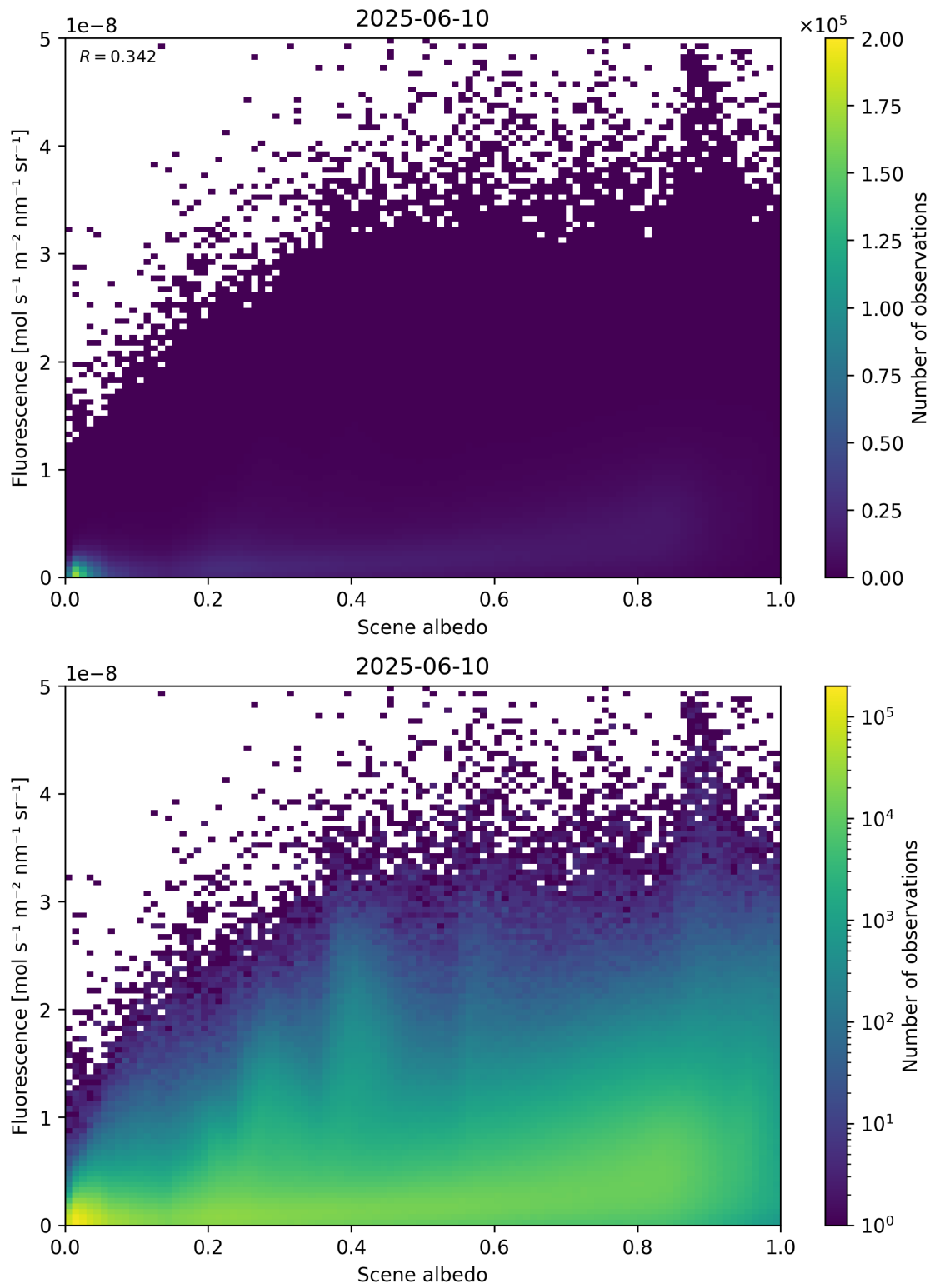
Figure 104: Scatter density plot of “Scene albedo” against “Fluorescence” for 2025-06-09 to 2025-06-11.
