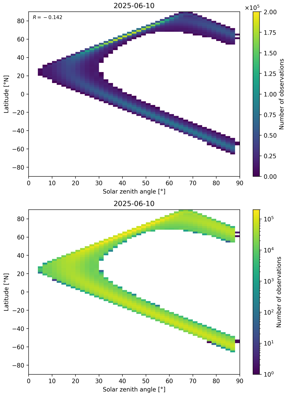
Figure 113: Scatter density plot of “Solar zenith angle” against “Latitude” for 2025-06-09 to 2025-06-11.
