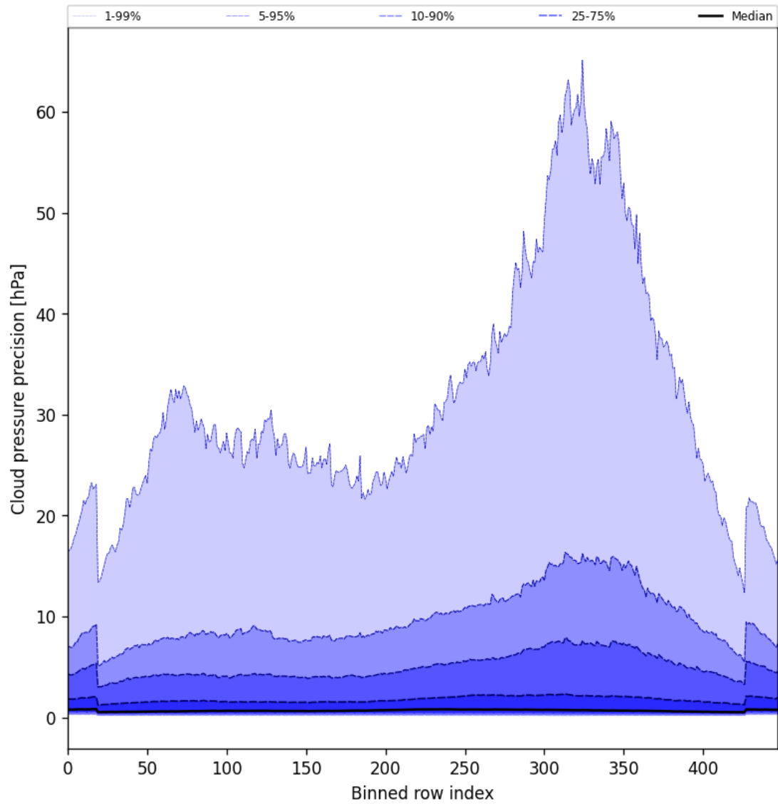
Figure 48: Along track statistics of “Cloud pressure precision” for 2025-06-09 to 2025-06-11
