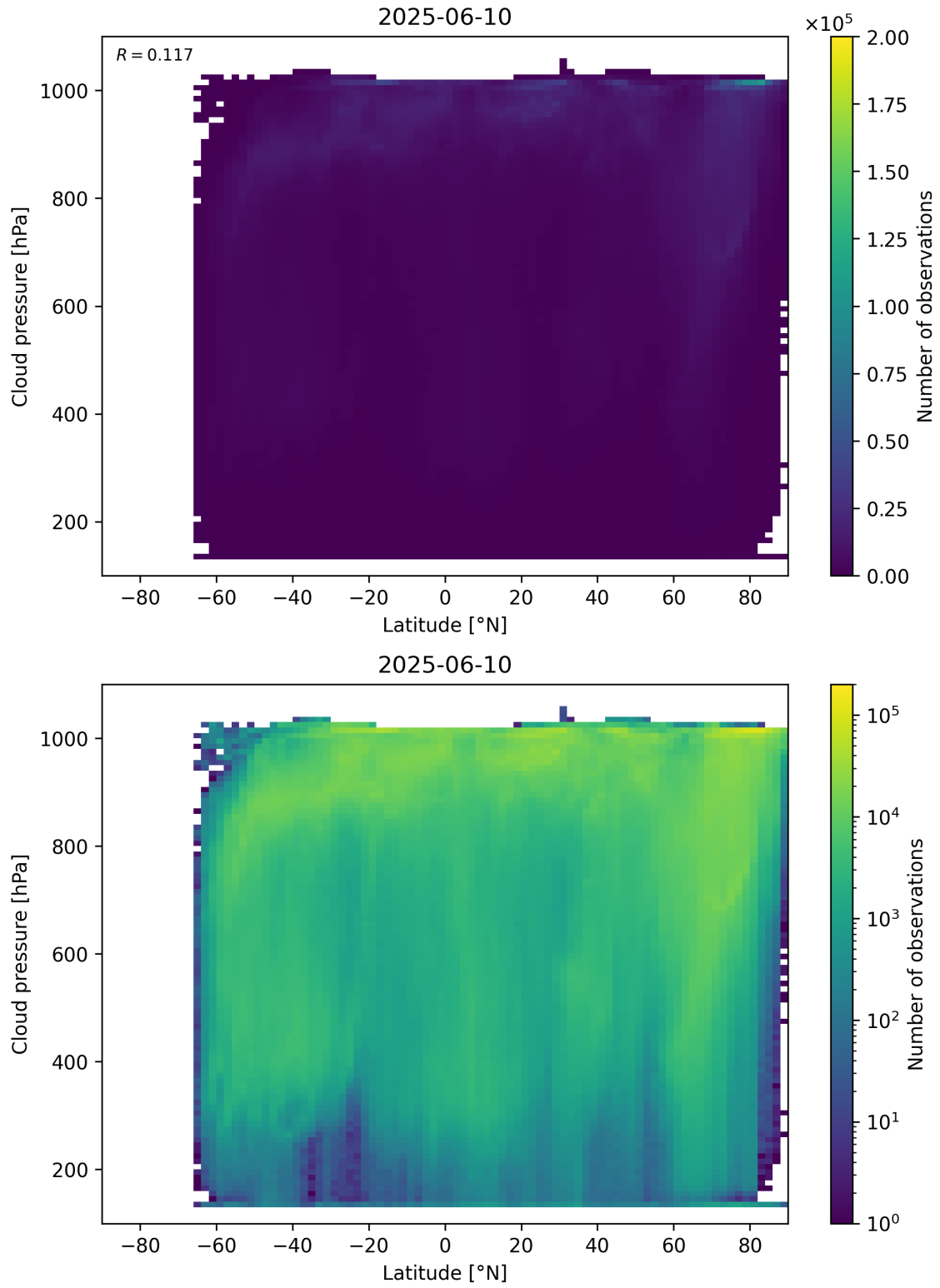
Figure 91: Scatter density plot of “Latitude” against “Cloud pressure” for 2025-06-09 to 2025-06-11.
