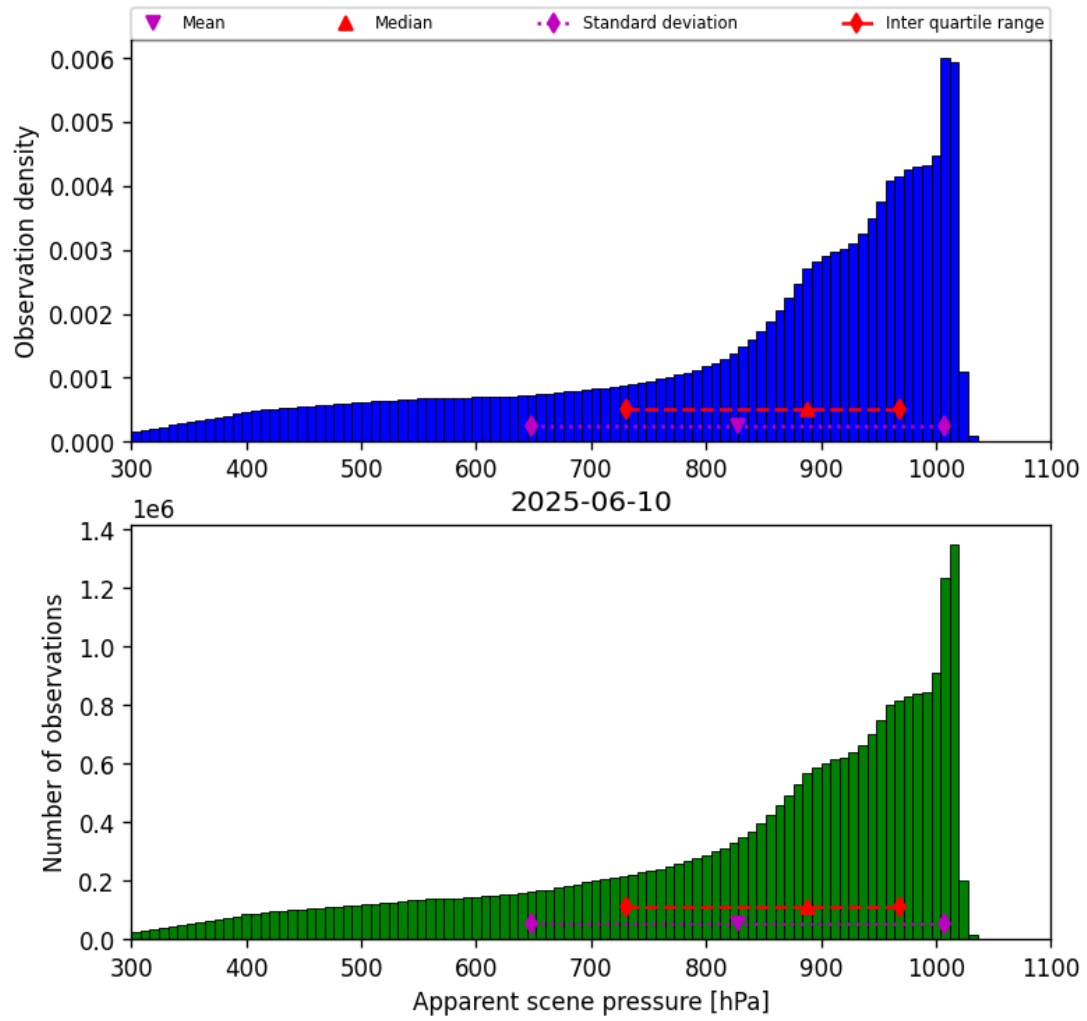
Figure 36: Histogram of “Apparent scene pressure” for 2025-06-09 to 2025-06-11
