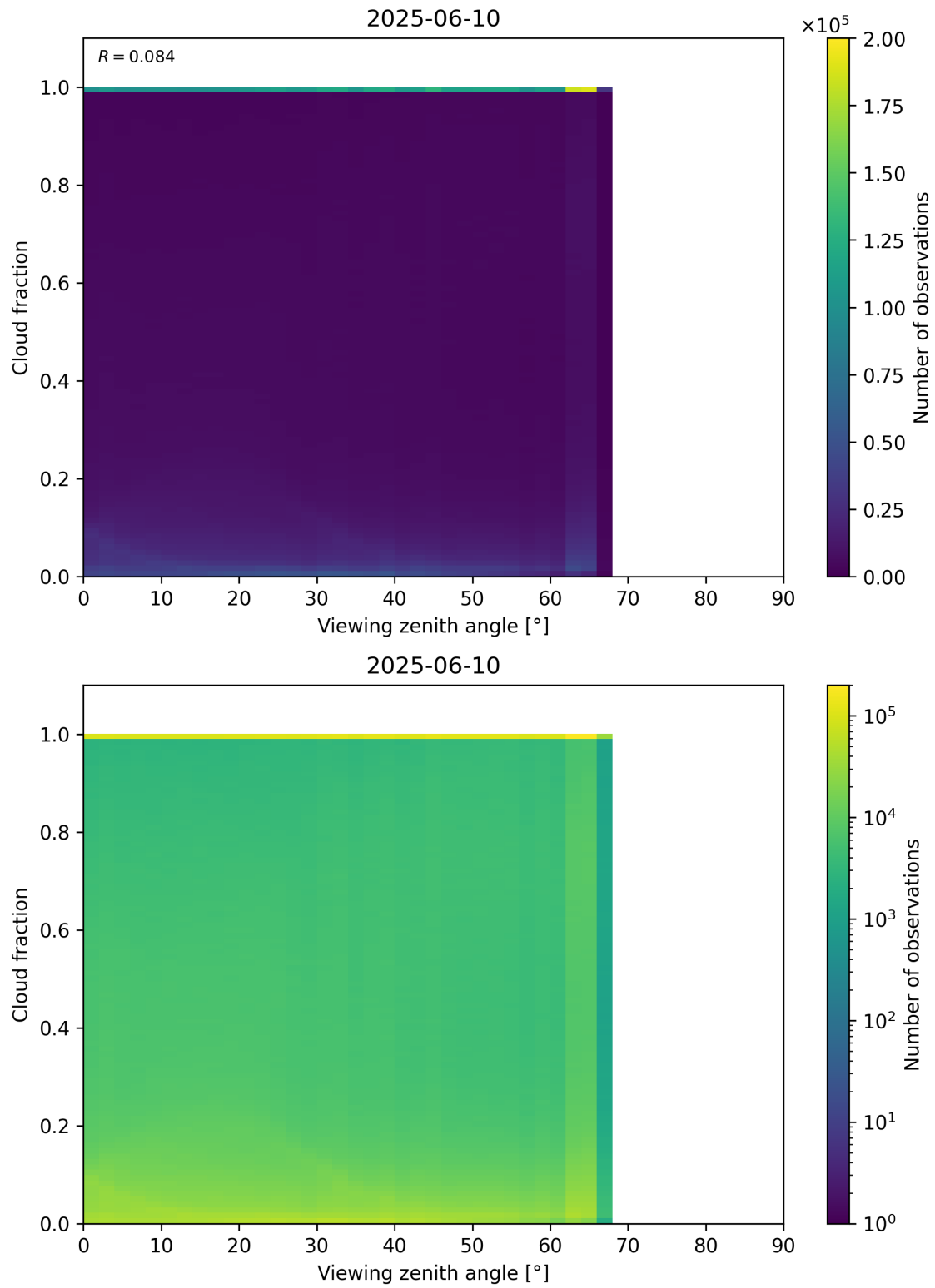
Figure 120: Scatter density plot of “Viewing zenith angle” against “Cloud fraction” for 2025-06-09 to 2025-06-11.
