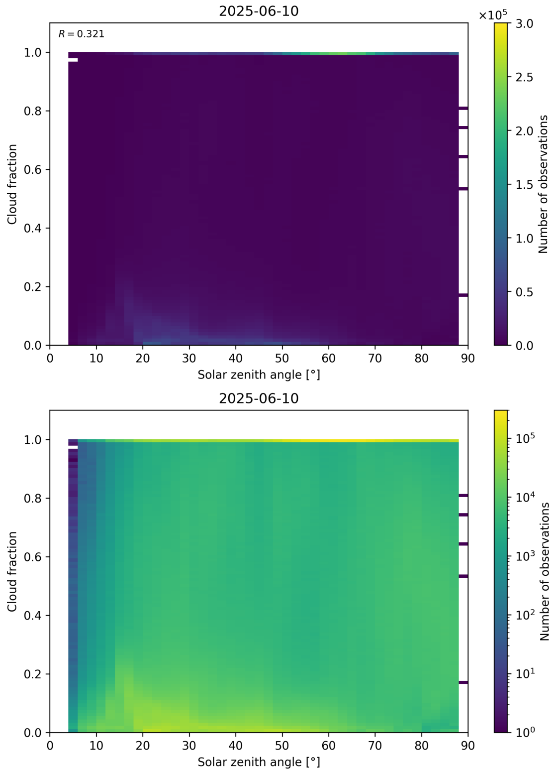
Figure 110: Scatter density plot of “Solar zenith angle” against “Cloud fraction” for 2025-06-09 to 2025-06-11.
