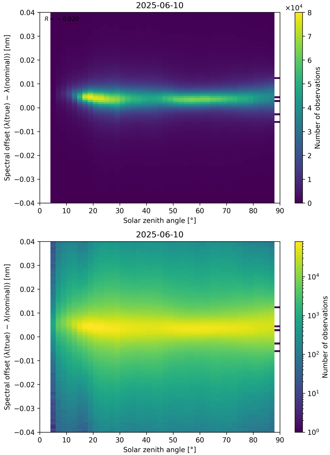
Figure 117: Scatter density plot of “Solar zenith angle” against “Spectral offset ( \lambda_{\text{true}} - \lambda_{\text{nominal}} )” for 2025-06-09 to 2025-06-11.
