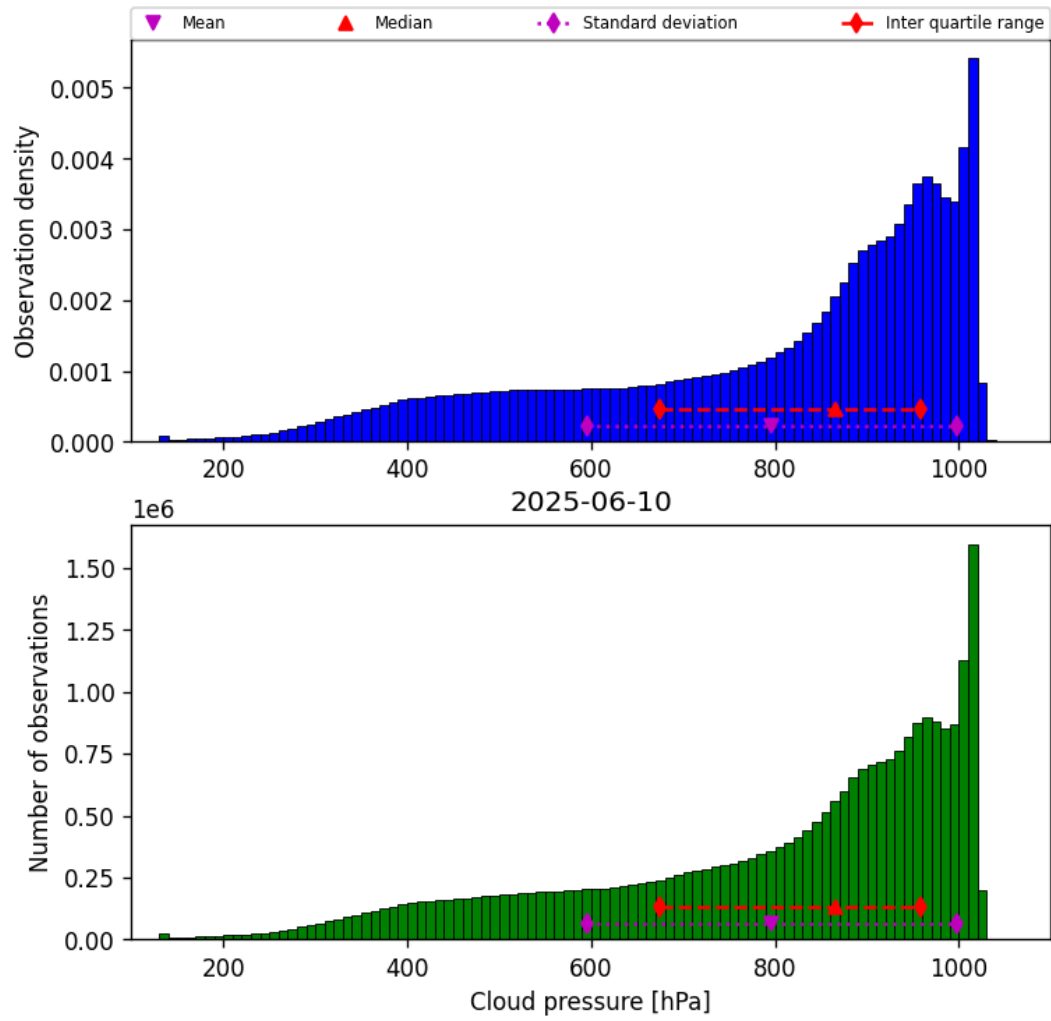
Figure 30: Histogram of “Cloud pressure” for 2025-06-09 to 2025-06-11
