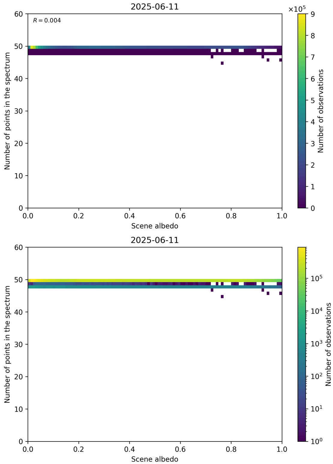
Figure 106: Scatter density plot of “Scene albedo” against “Number of points in the spectrum” for 2025-06-11 to 2025-06-12.
