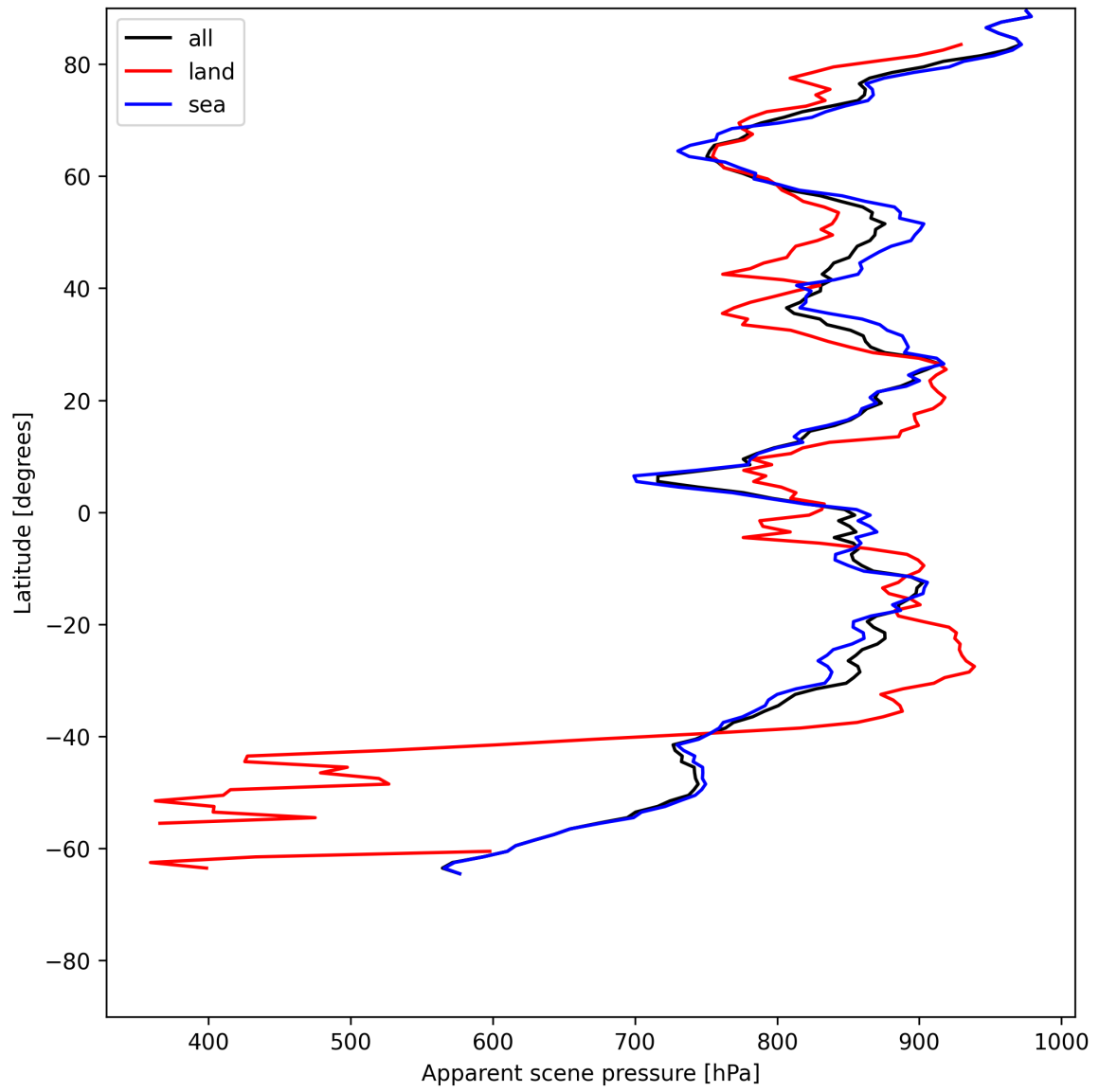
Figure 19: Zonal average of “Apparent scene pressure” for 2025-06-11 to 2025-06-12.
