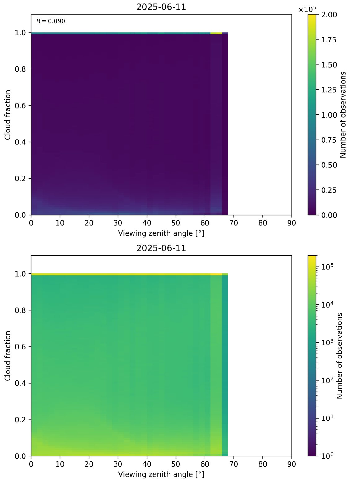
Figure 120: Scatter density plot of “Viewing zenith angle” against “Cloud fraction” for 2025-06-11 to 2025-06-12.
