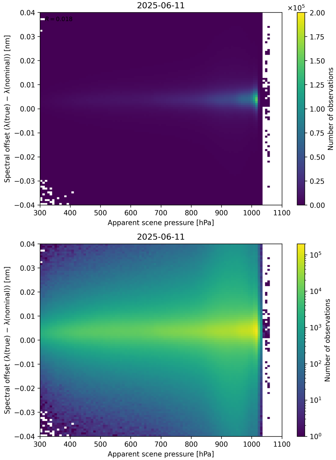
Figure 67: Scatter density plot of “Apparent scene pressure” against “Spectral offset ( \lambda_{\text{true}} - \lambda_{\text{nominal}} )” for 2025-06-11 to 2025-06-12.
