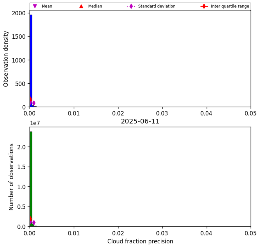
Figure 33: Histogram of “Cloud fraction precision” for 2025-06-11 to 2025-06-12
