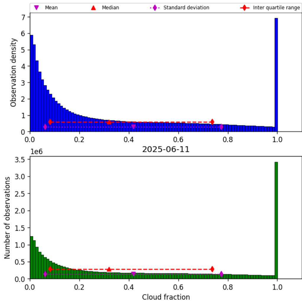
Figure 32: Histogram of “Cloud fraction” for 2025-06-11 to 2025-06-12
