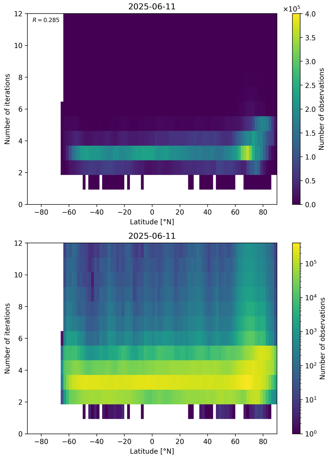
Figure 93: Scatter density plot of “Latitude” against “Number of iterations” for 2025-06-11 to 2025-06-12.
