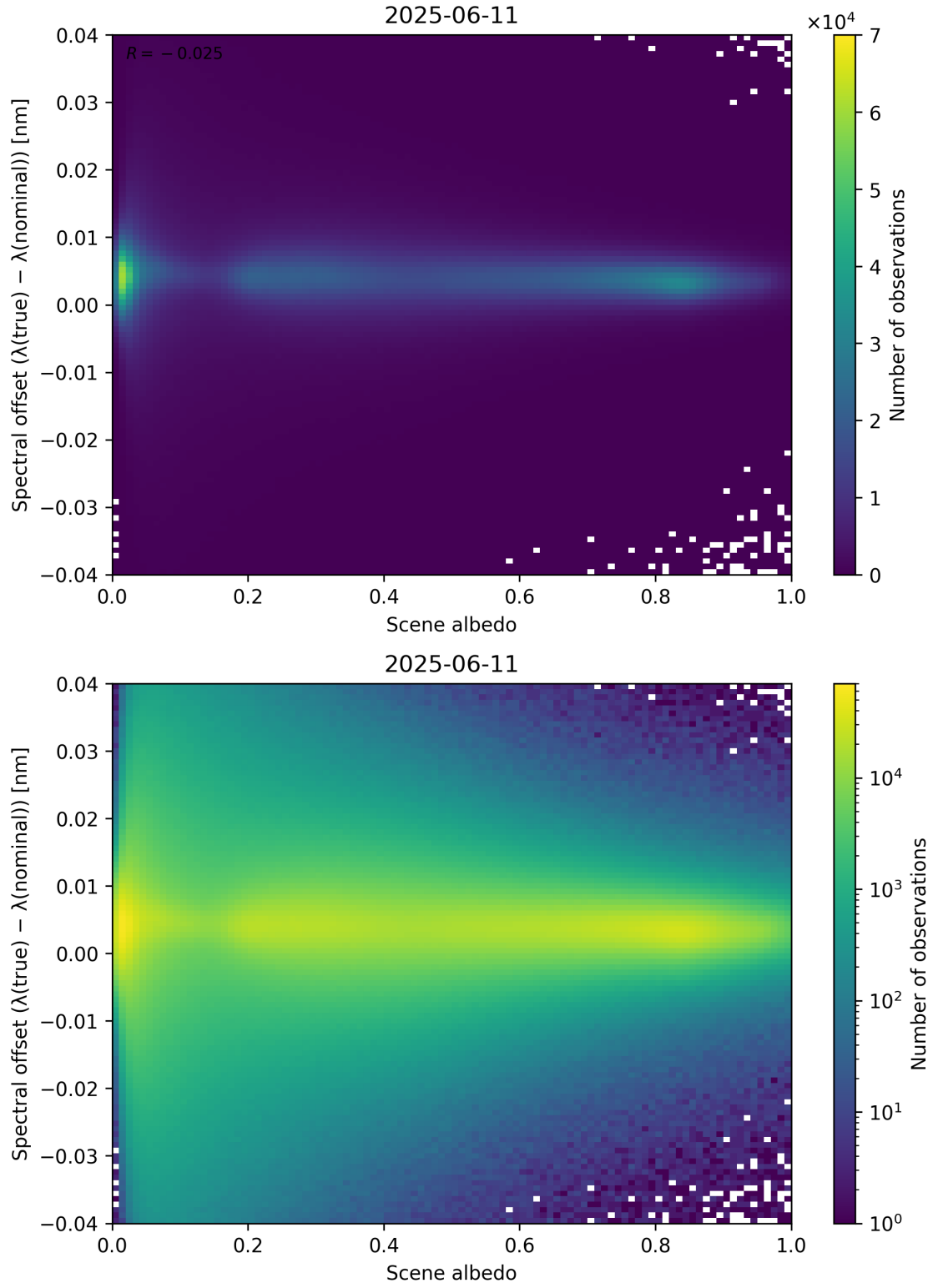
Figure 107: Scatter density plot of “Scene albedo” against “Spectral offset ( \lambda_{\text{true}} - \lambda_{\text{nominal}} )” for 2025-06-11 to 2025-06-12.
