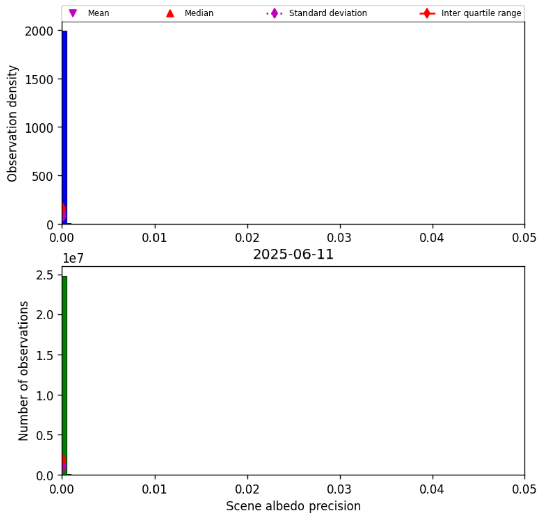
Figure 35: Histogram of “Scene albedo precision” for 2025-06-11 to 2025-06-12
