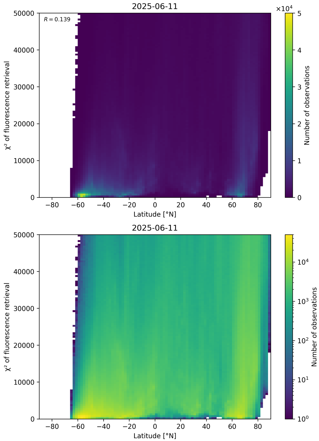
Figure 89: Scatter density plot of “Latitude” against “ \chi^2 of fluorescence retrieval” for 2025-06-11 to 2025-06-12.
