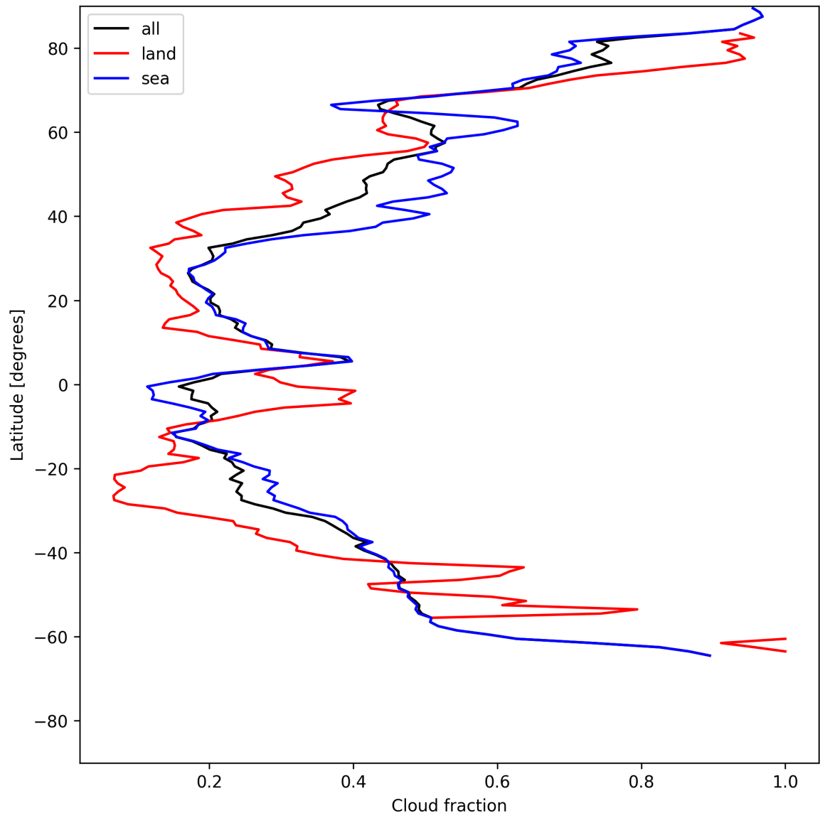
Figure 15: Zonal average of “Cloud fraction” for 2025-06-11 to 2025-06-12.
