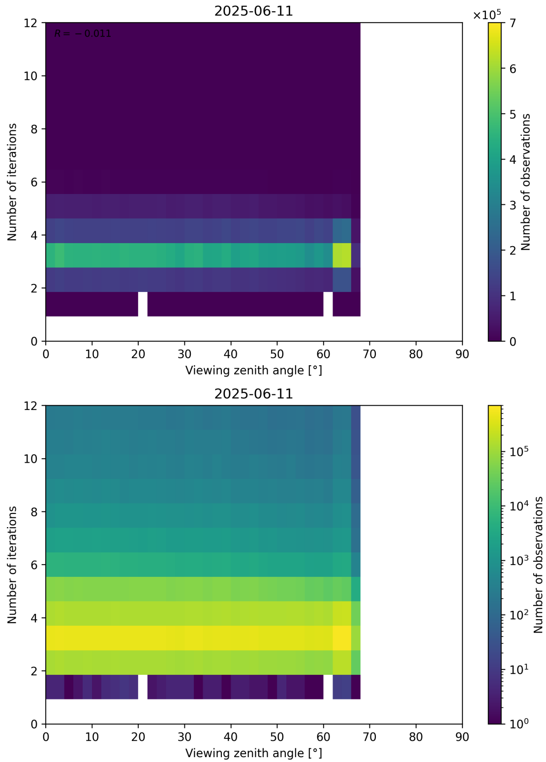
Figure 124: Scatter density plot of “Viewing zenith angle” against “Number of iterations” for 2025-06-11 to 2025-06-12.
