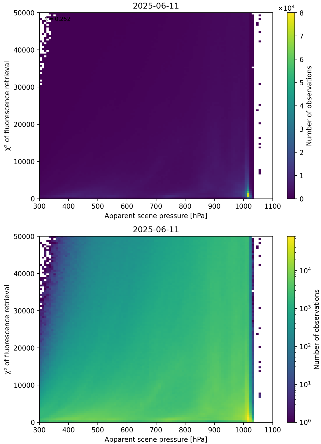
Figure 63: Scatter density plot of “Apparent scene pressure” against “ \chi^2 of fluorescence retrieval” for 2025-06-11 to 2025-06-12.
