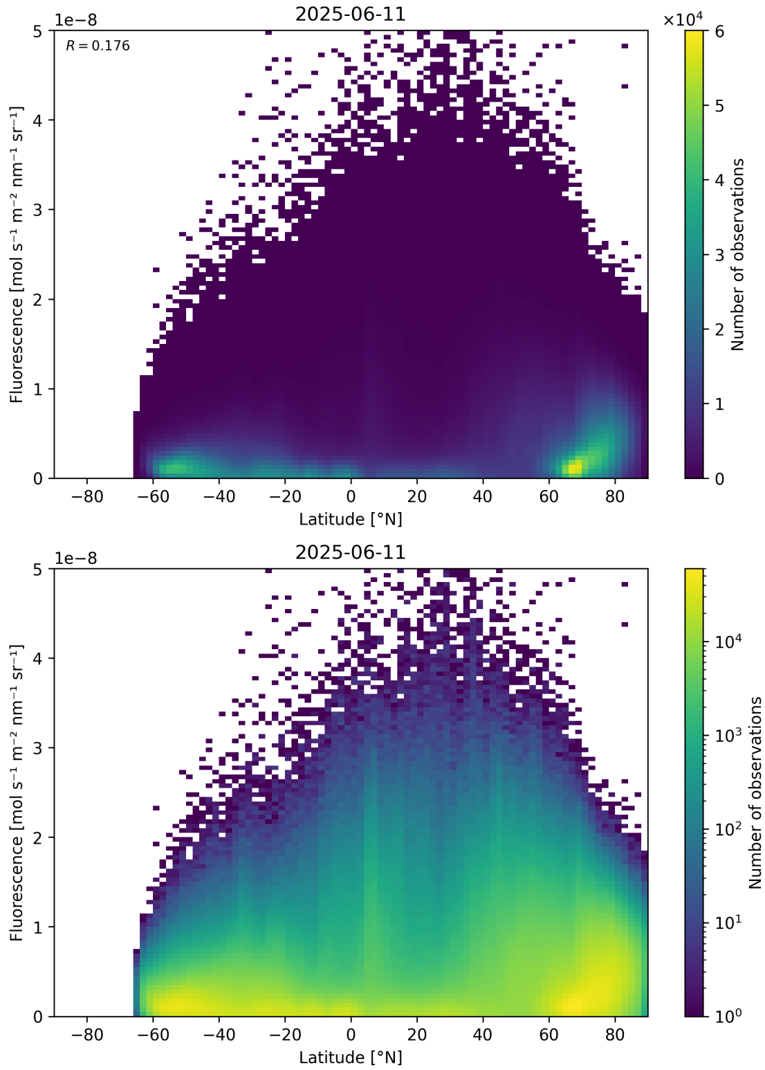
Figure 92: Scatter density plot of “Latitude” against “Fluorescence” for 2025-06-11 to 2025-06-12.
