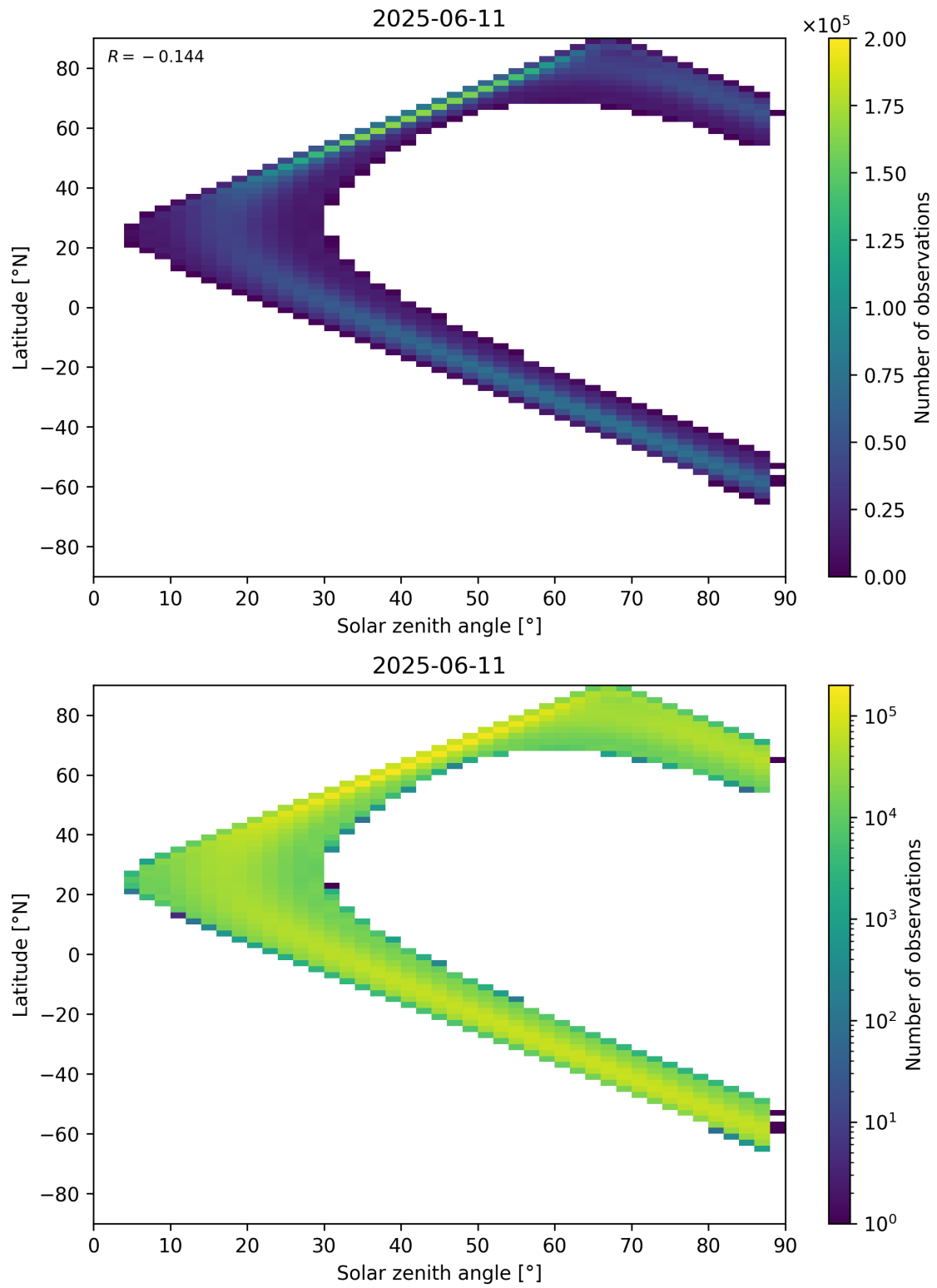
Figure 113: Scatter density plot of “Solar zenith angle” against “Latitude” for 2025-06-11 to 2025-06-12.
