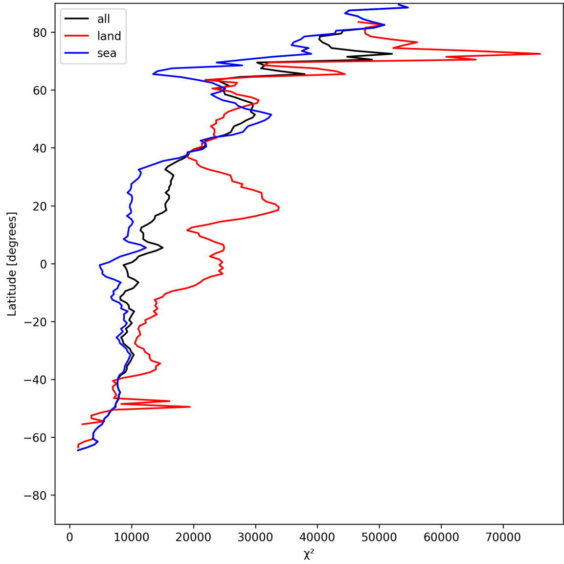
Figure 21: Zonal average of “ \chi^2 ” for 2025-06-11 to 2025-06-12.
