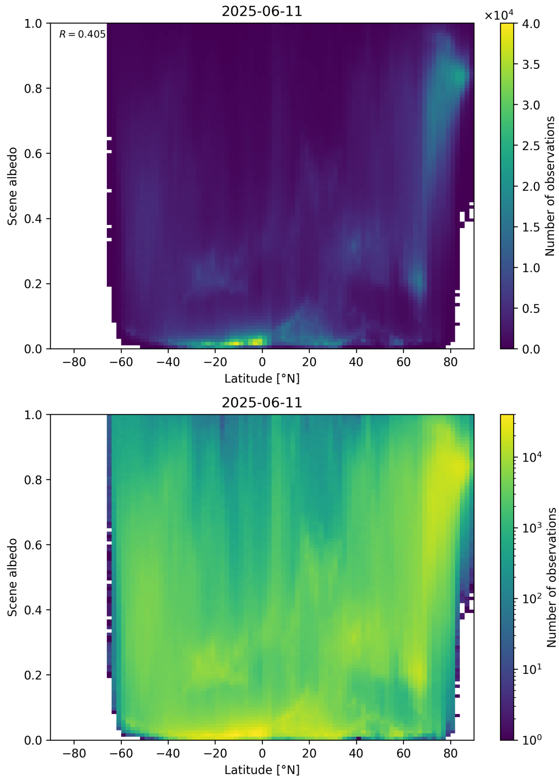
Figure 95: Scatter density plot of “Latitude” against “Scene albedo” for 2025-06-11 to 2025-06-12.
