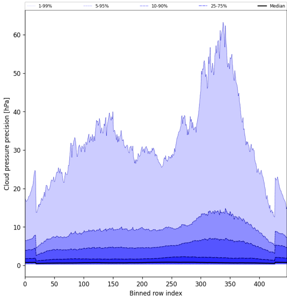
Figure 48: Along track statistics of “Cloud pressure precision” for 2025-06-11 to 2025-06-12
