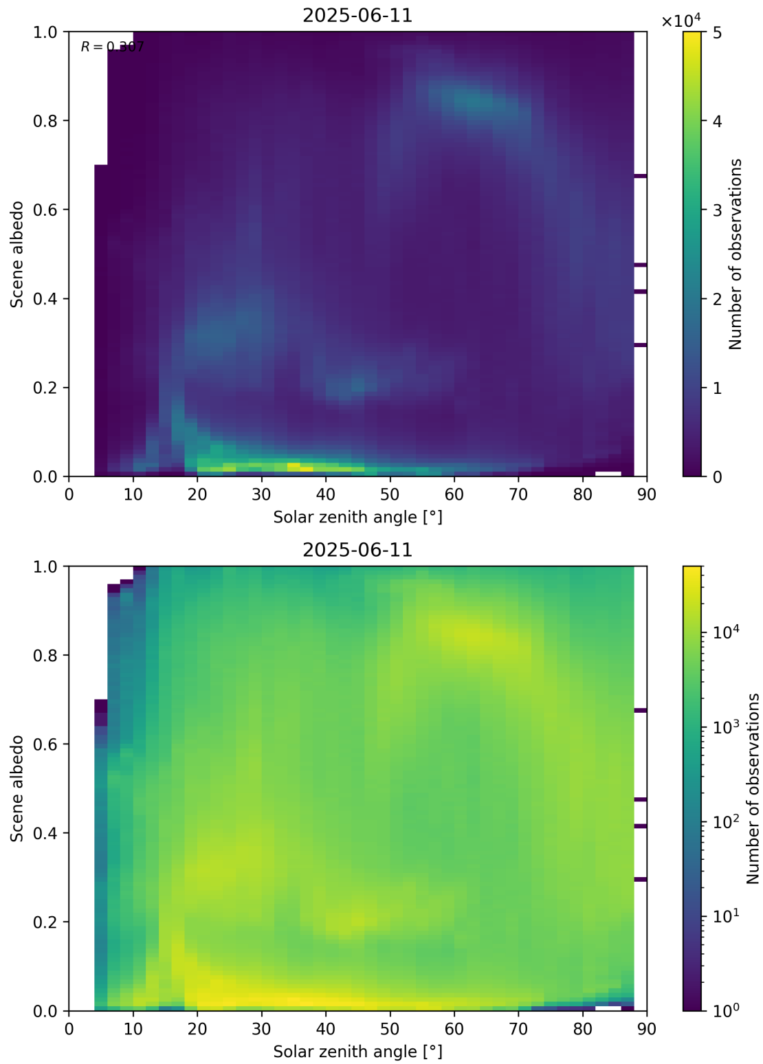
Figure 116: Scatter density plot of “Solar zenith angle” against “Scene albedo” for 2025-06-11 to 2025-06-12.
