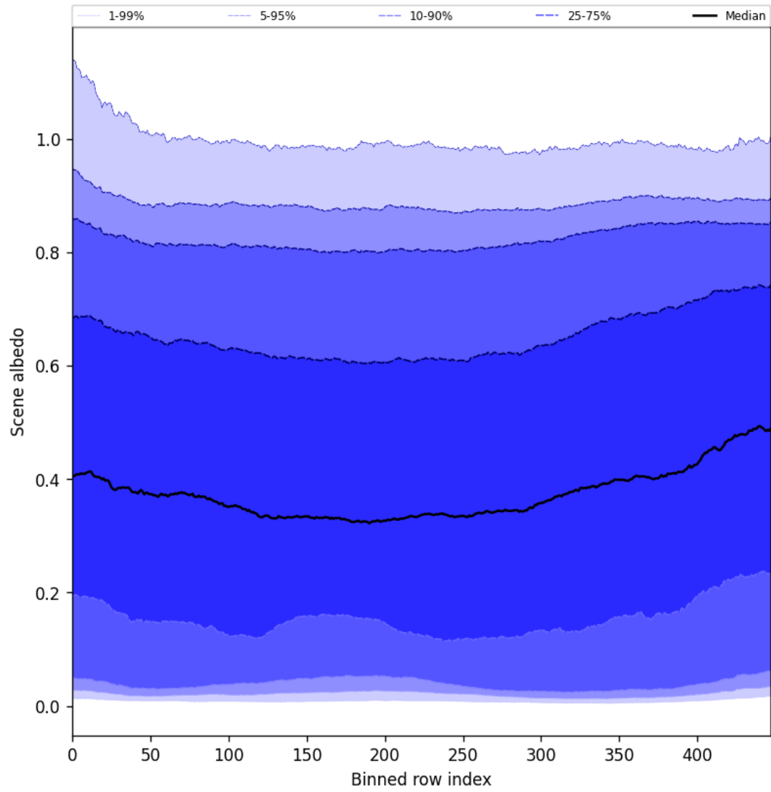
Figure 51: Along track statistics of “Scene albedo” for 2025-06-11 to 2025-06-12
