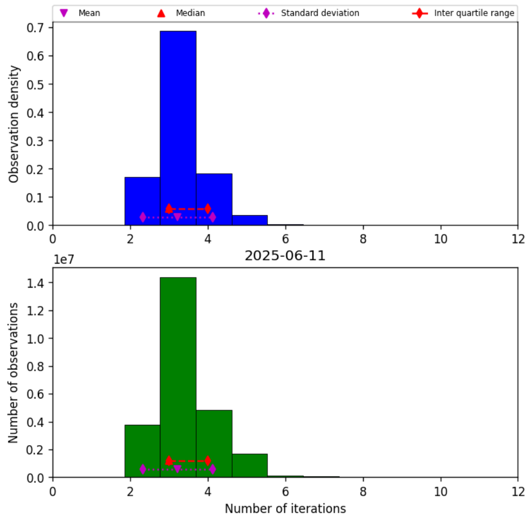
Figure 39: Histogram of “Number of iterations” for 2025-06-11 to 2025-06-12
