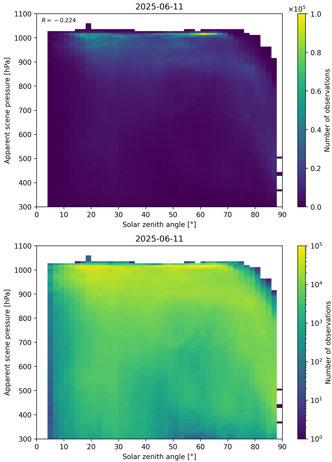
Figure 108: Scatter density plot of “Solar zenith angle” against “Apparent scene pressure” for 2025-06-11 to 2025-06-12.
