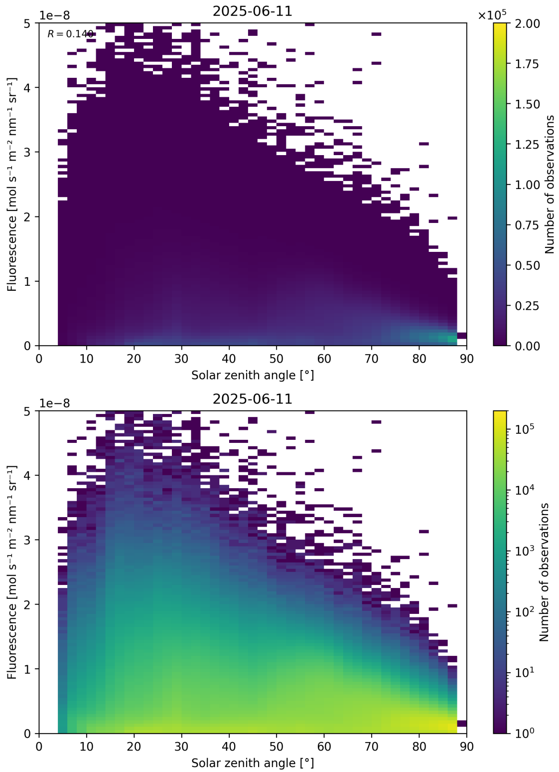
Figure 112: Scatter density plot of “Solar zenith angle” against “Fluorescence” for 2025-06-11 to 2025-06-12.
