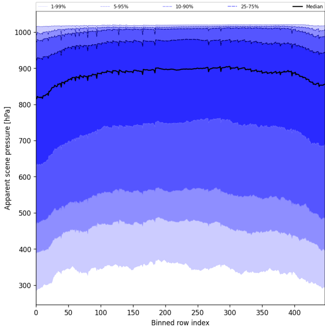
Figure 53: Along track statistics of “Apparent scene pressure” for 2025-06-11 to 2025-06-12
