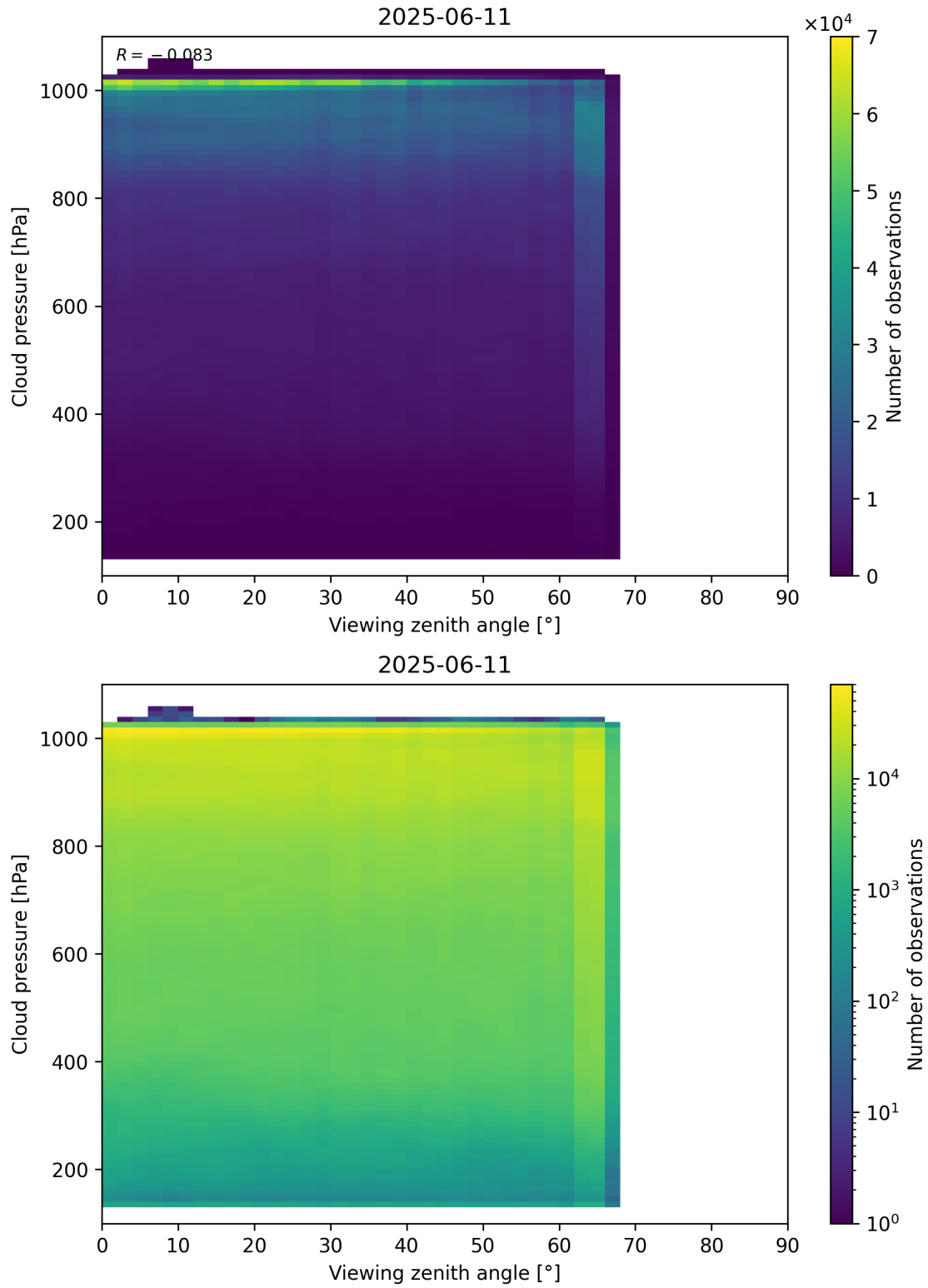
Figure 121: Scatter density plot of “Viewing zenith angle” against “Cloud pressure” for 2025-06-11 to 2025-06-12.
