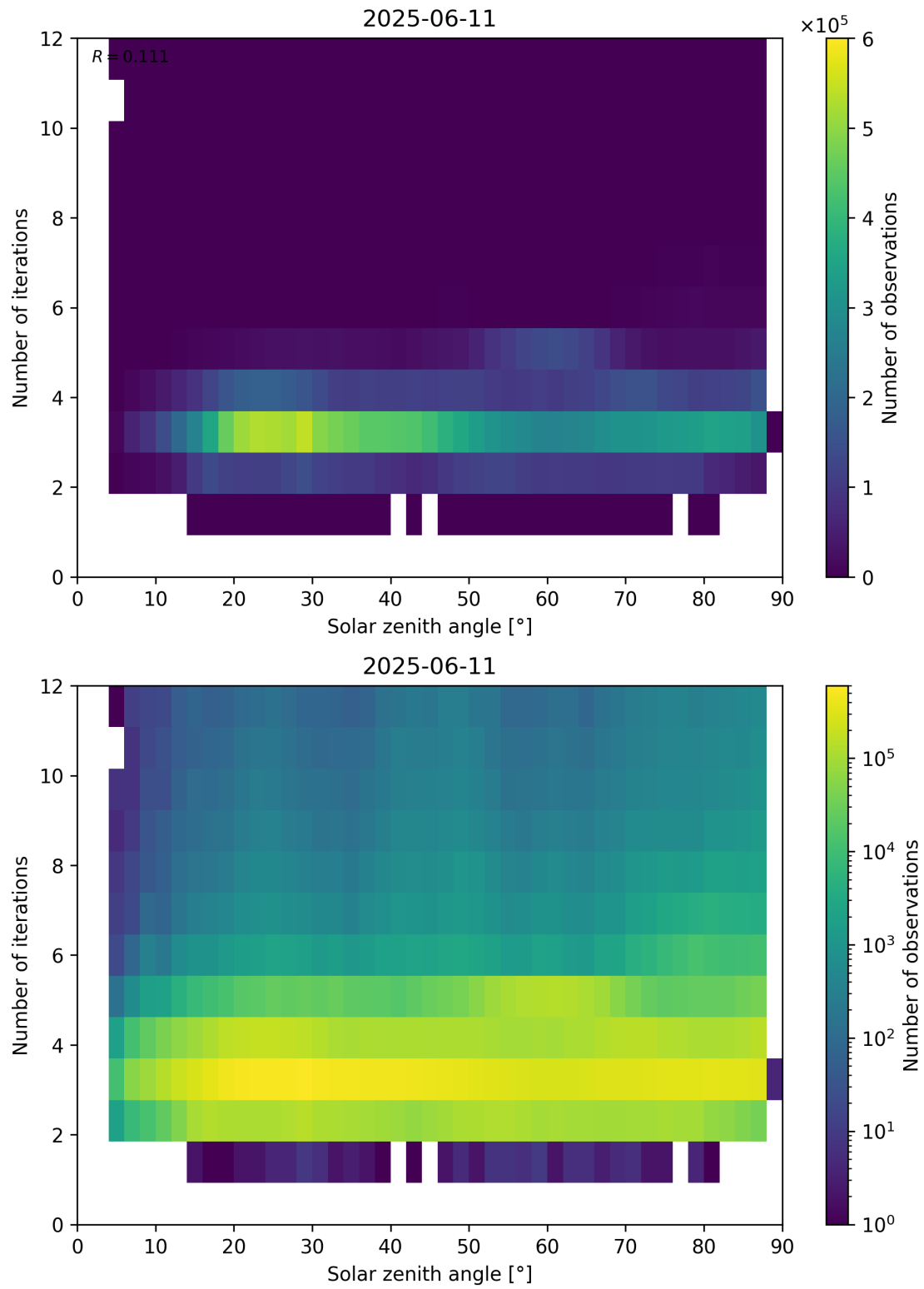
Figure 114: Scatter density plot of “Solar zenith angle” against “Number of iterations” for 2025-06-11 to 2025-06-12.
