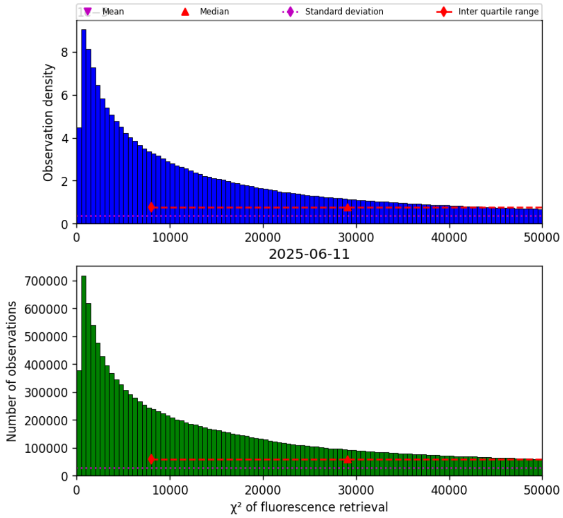
Figure 42: Histogram of “ \chi^2 of fluorescence retrieval” for 2025-06-11 to 2025-06-12
