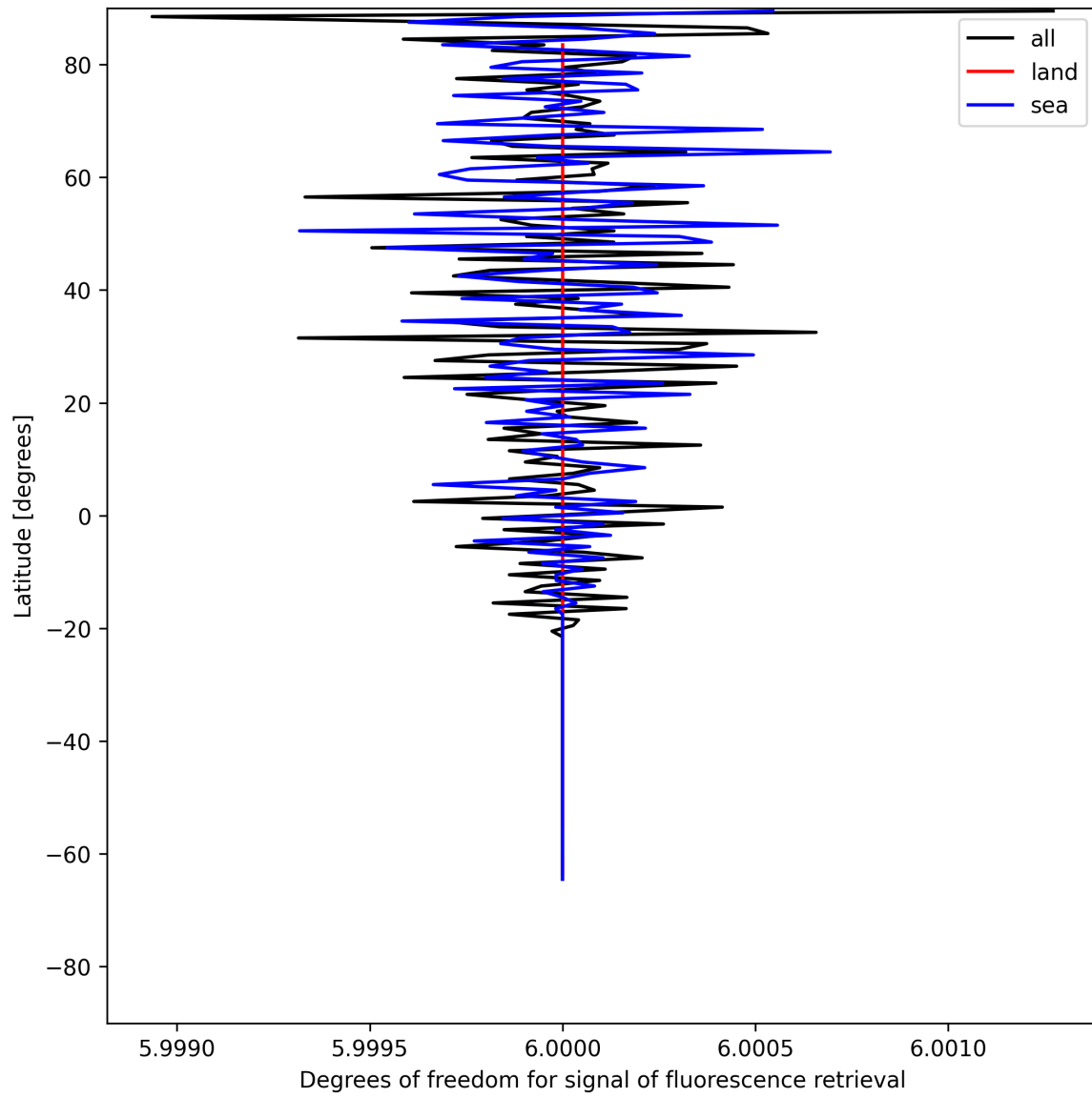
Figure 26: Zonal average of “Degrees of freedom for signal of fluorescence retrieval” for 2025-06-11 to 2025-06-12.
