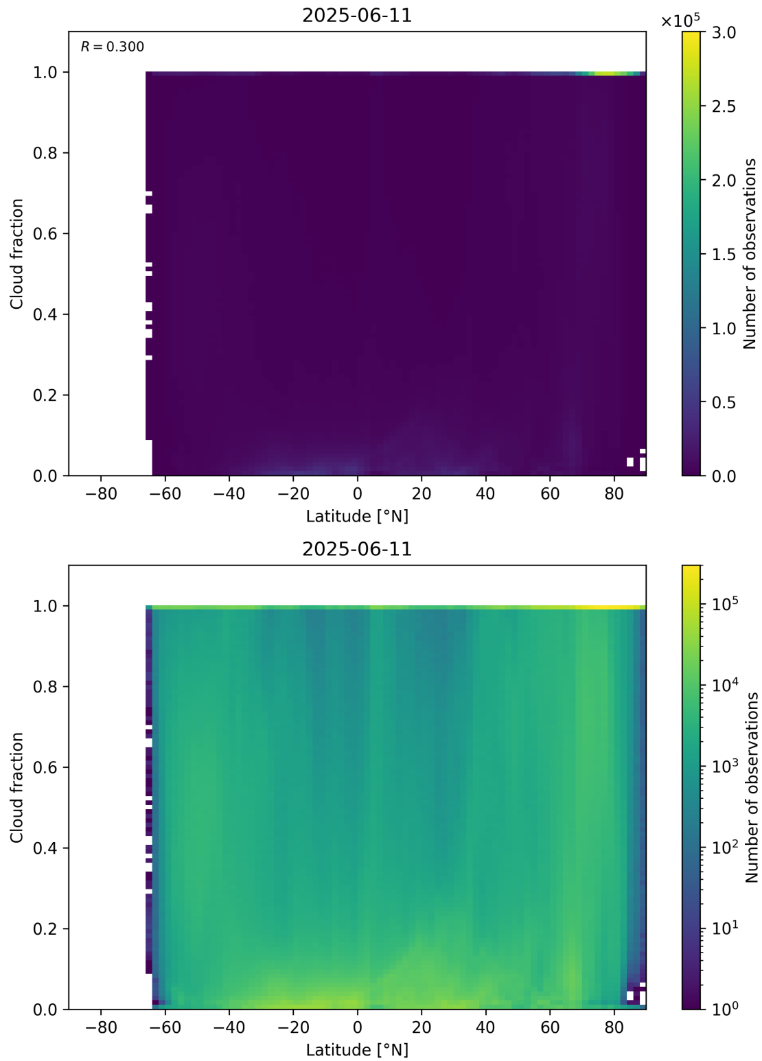
Figure 90: Scatter density plot of “Latitude” against “Cloud fraction” for 2025-06-11 to 2025-06-12.
