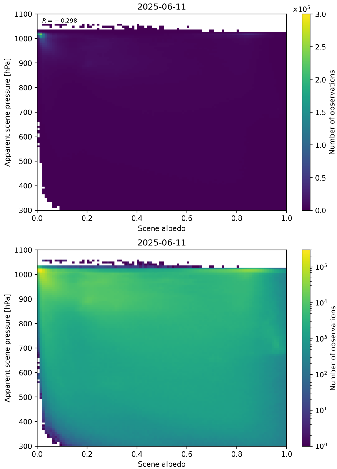
Figure 102: Scatter density plot of “Scene albedo” against “Apparent scene pressure” for 2025-06-11 to 2025-06-12.
