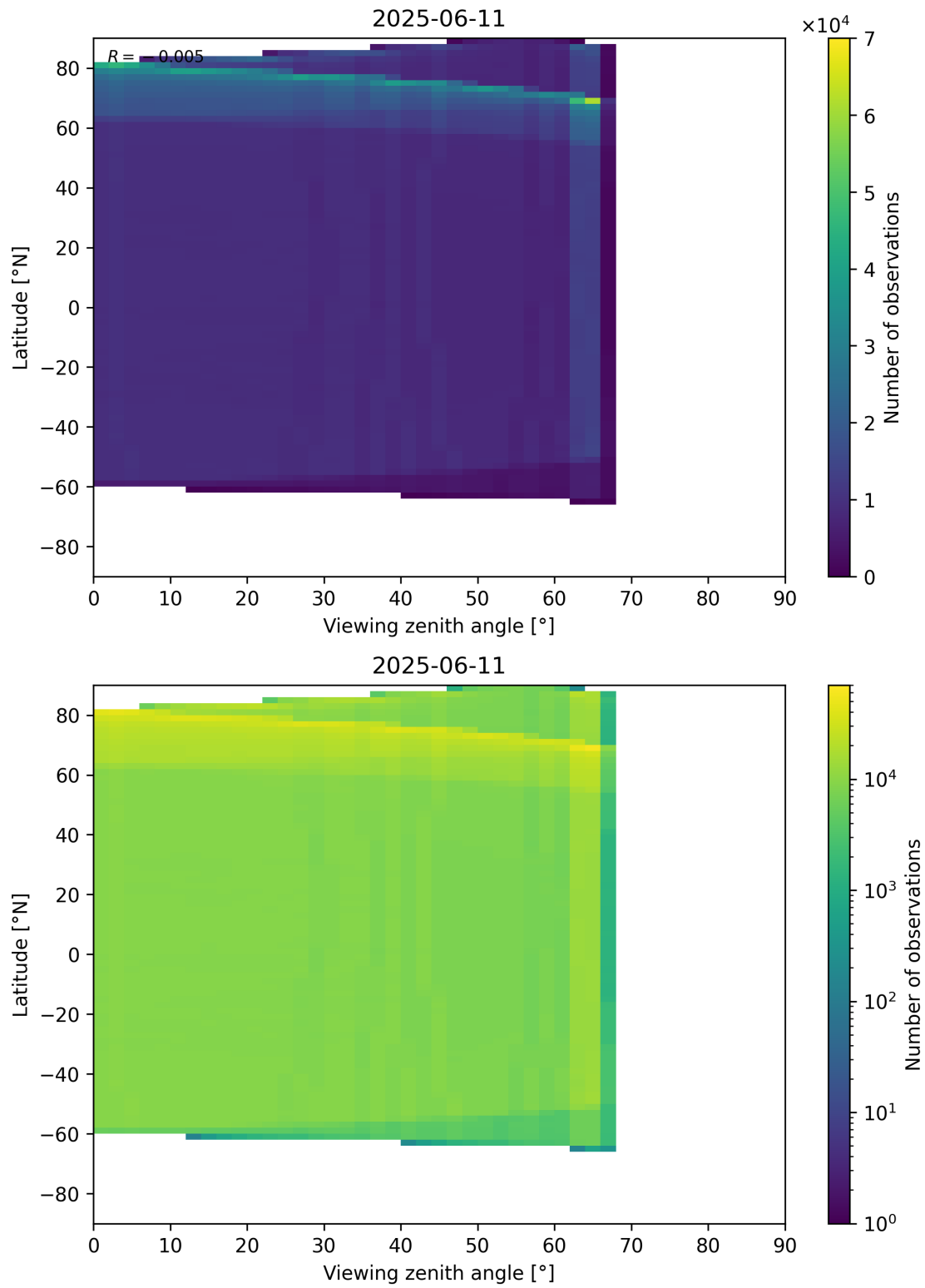
Figure 123: Scatter density plot of “Viewing zenith angle” against “Latitude” for 2025-06-11 to 2025-06-12.
