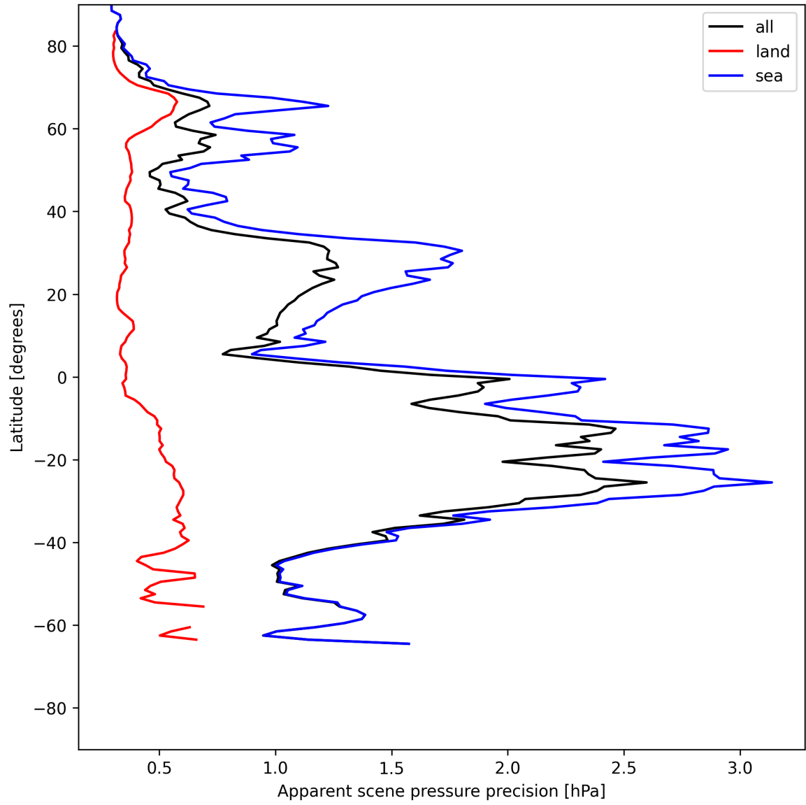
Figure 20: Zonal average of “Apparent scene pressure precision” for 2025-06-11 to 2025-06-12.
