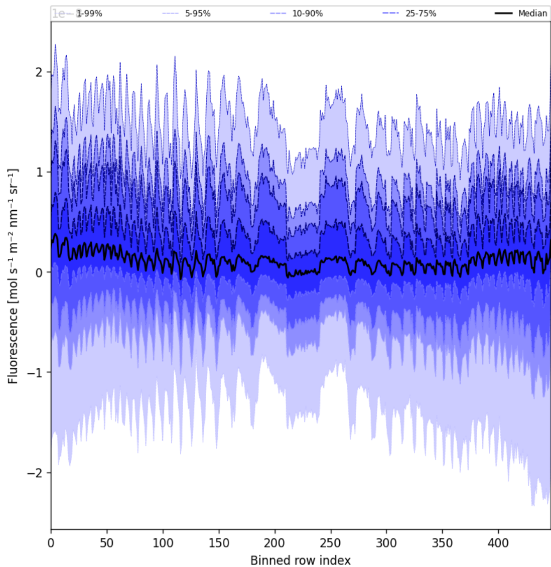
Figure 57: Along track statistics of “Fluorescence” for 2025-06-11 to 2025-06-12
