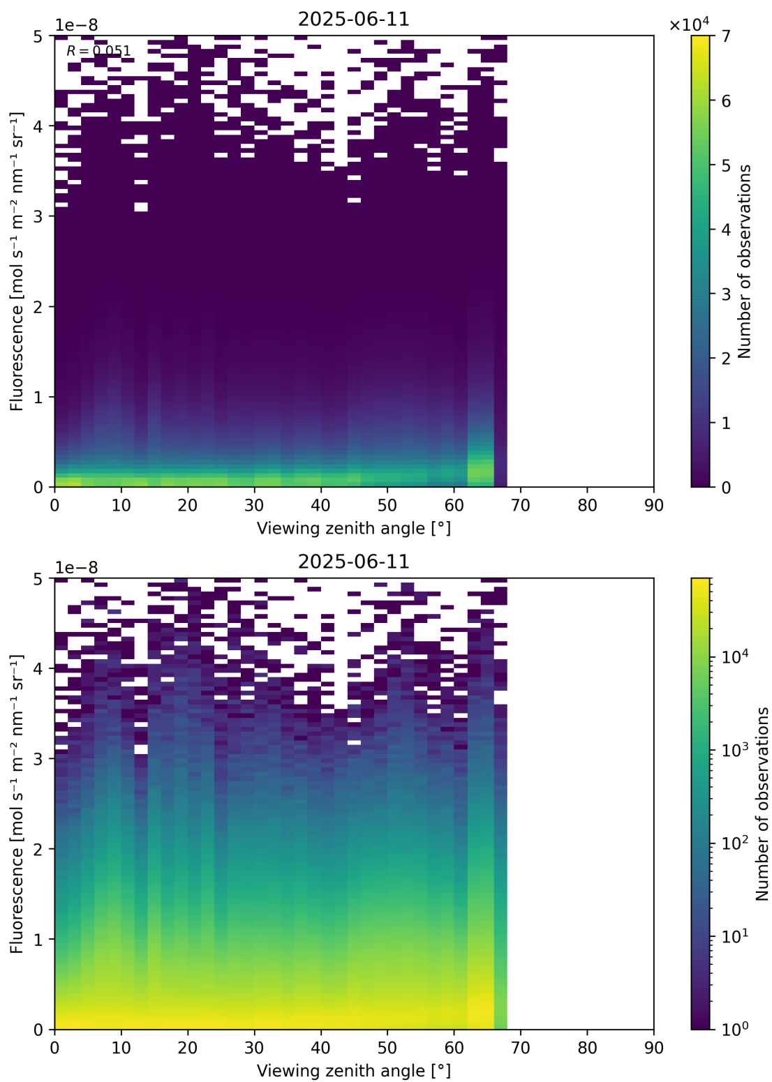
Figure 122: Scatter density plot of “Viewing zenith angle” against “Fluorescence” for 2025-06-11 to 2025-06-12.
