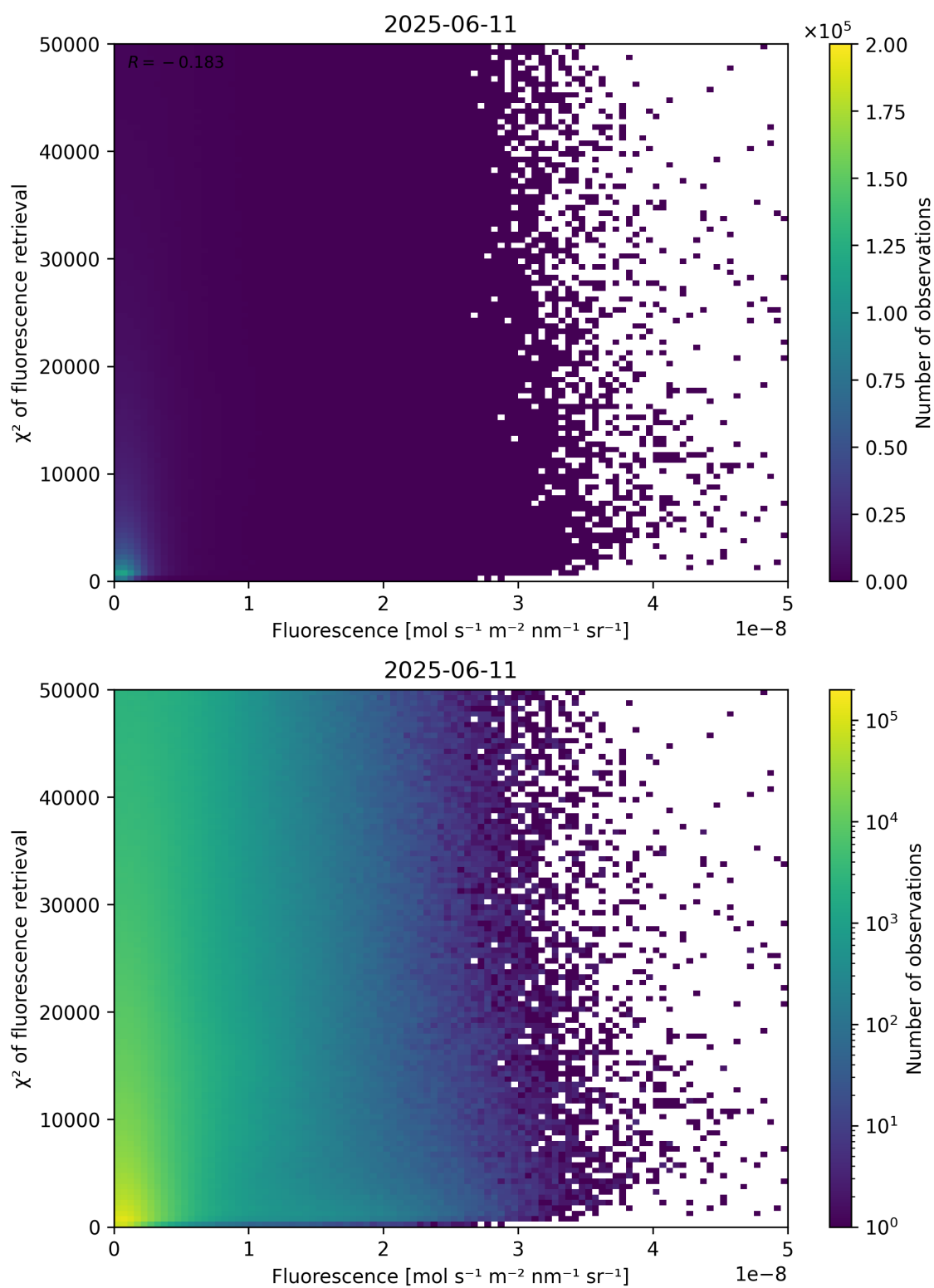
Figure 85: Scatter density plot of “Fluorescence” against “ \chi^2 of fluorescence retrieval” for 2025-06-11 to 2025-06-12.
