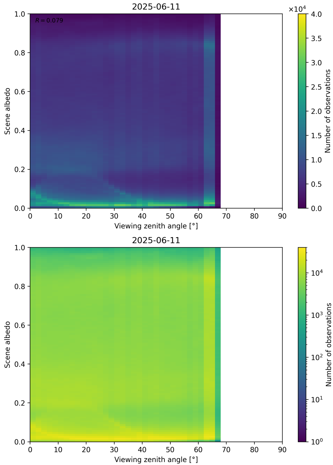
Figure 126: Scatter density plot of “Viewing zenith angle” against “Scene albedo” for 2025-06-11 to 2025-06-12.
