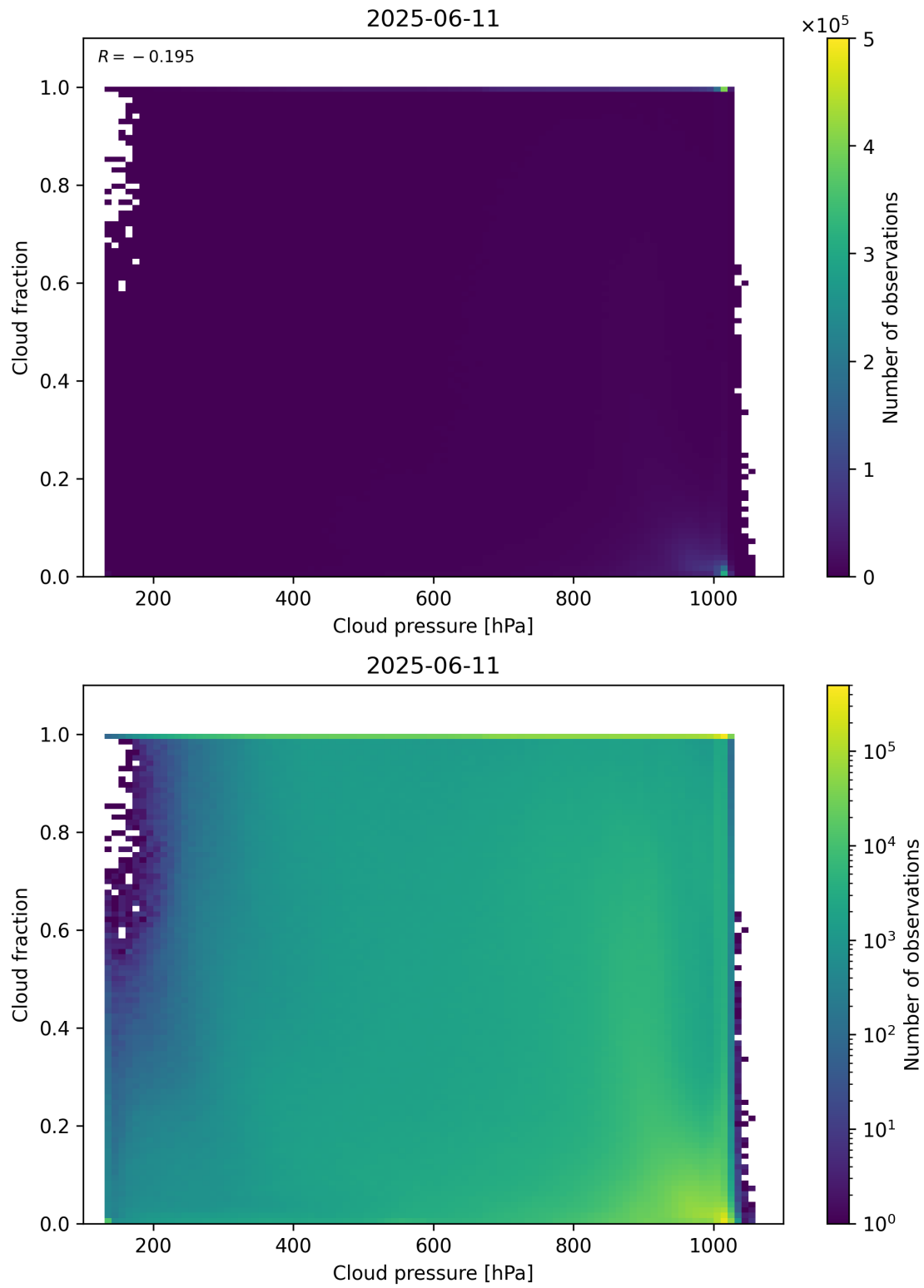
Figure 79: Scatter density plot of “Cloud pressure” against “Cloud fraction” for 2025-06-11 to 2025-06-12.
