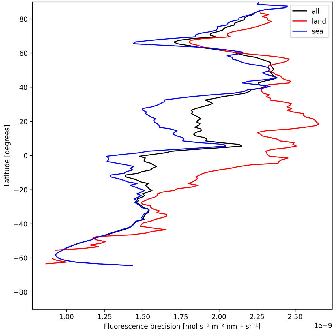
Figure 24: Zonal average of “Fluorescence precision” for 2025-06-11 to 2025-06-12.
