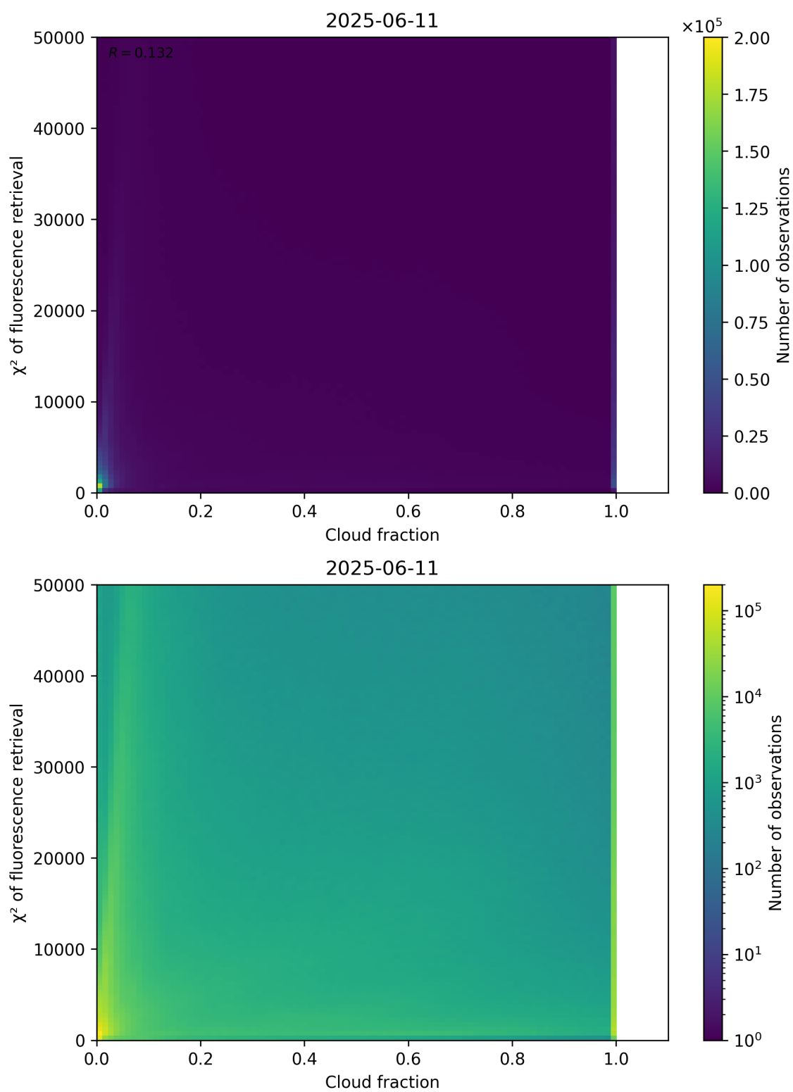
Figure 71: Scatter density plot of “Cloud fraction” against “ \chi^2 of fluorescence retrieval” for 2025-06-11 to 2025-06-12.
