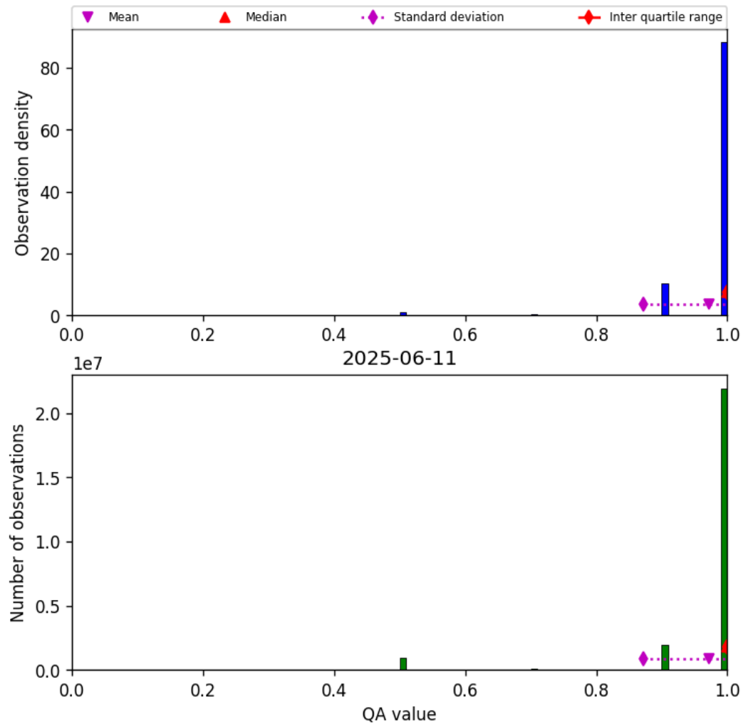
Figure 29: Histogram of “QA value” for 2025-06-11 to 2025-06-12
