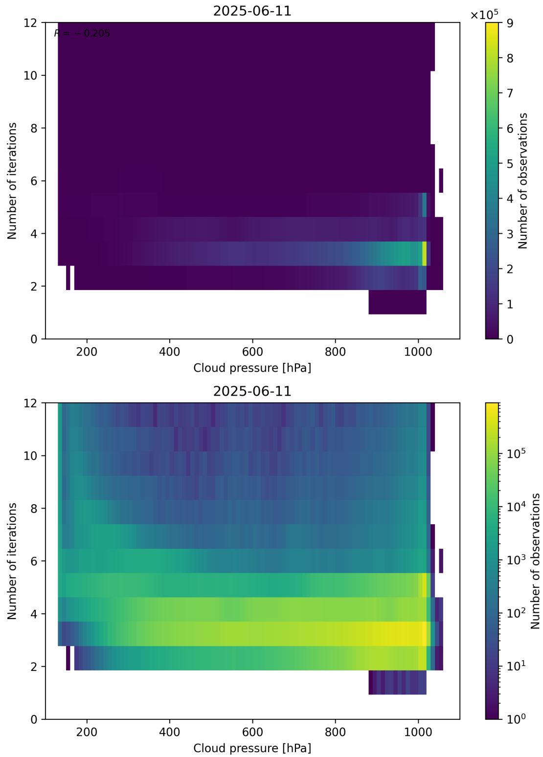
Figure 81: Scatter density plot of “Cloud pressure” against “Number of iterations” for 2025-06-11 to 2025-06-12.
