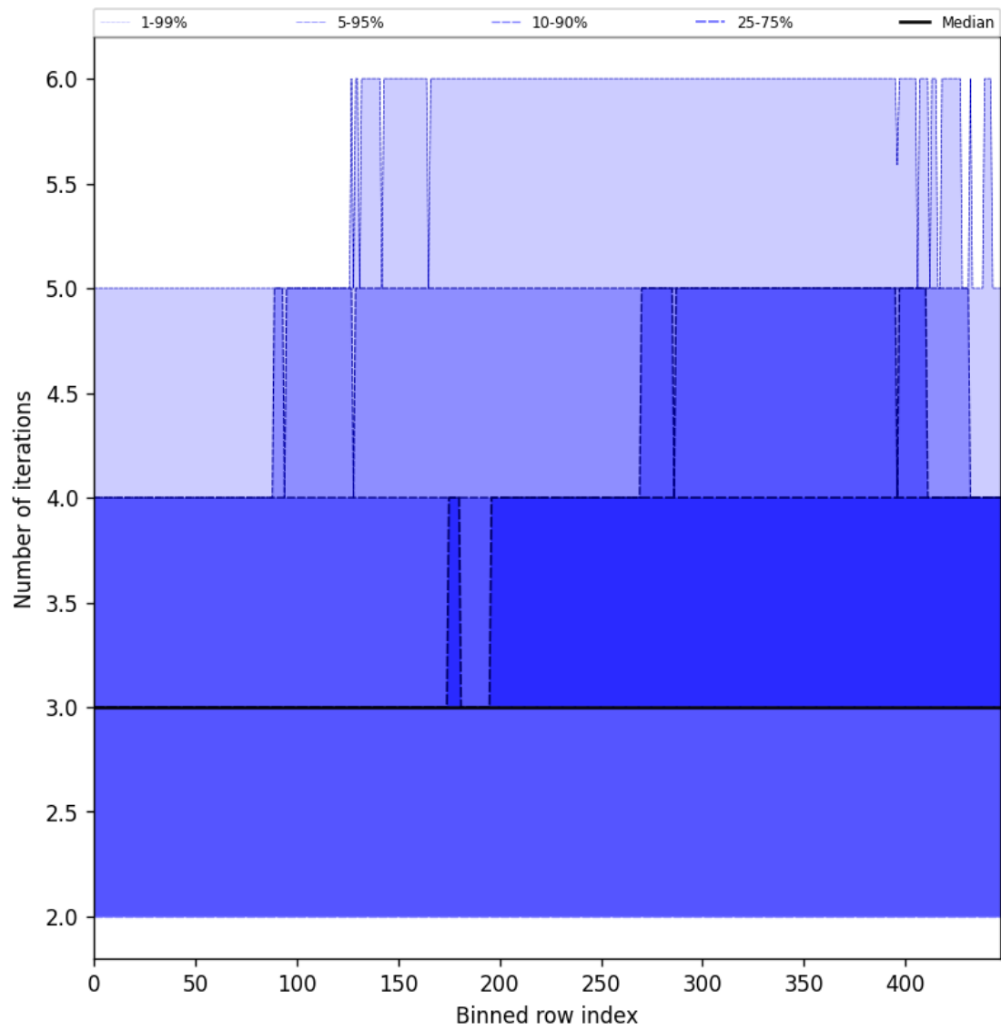
Figure 56: Along track statistics of “Number of iterations” for 2025-06-11 to 2025-06-12
