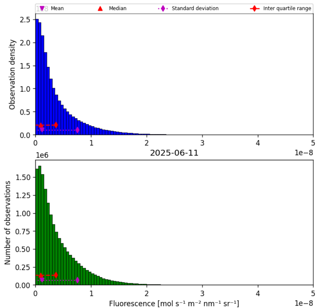
Figure 40: Histogram of “Fluorescence” for 2025-06-11 to 2025-06-12
