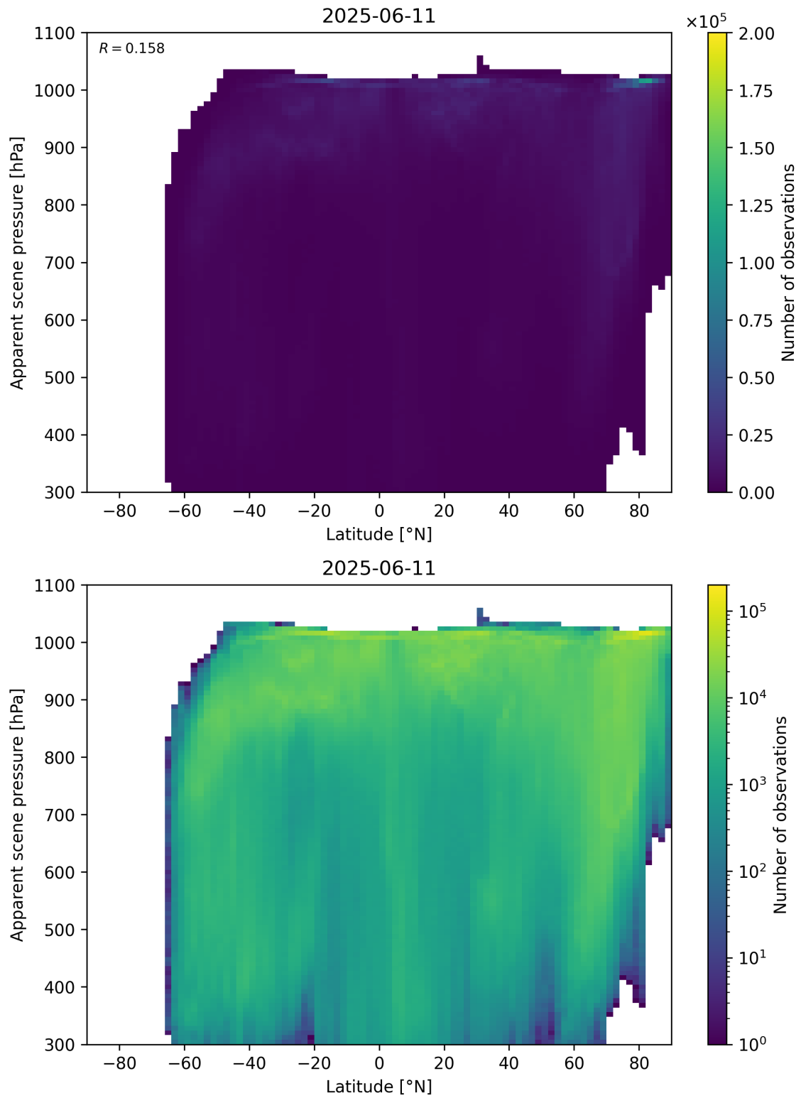
Figure 88: Scatter density plot of “Latitude” against “Apparent scene pressure” for 2025-06-11 to 2025-06-12.
