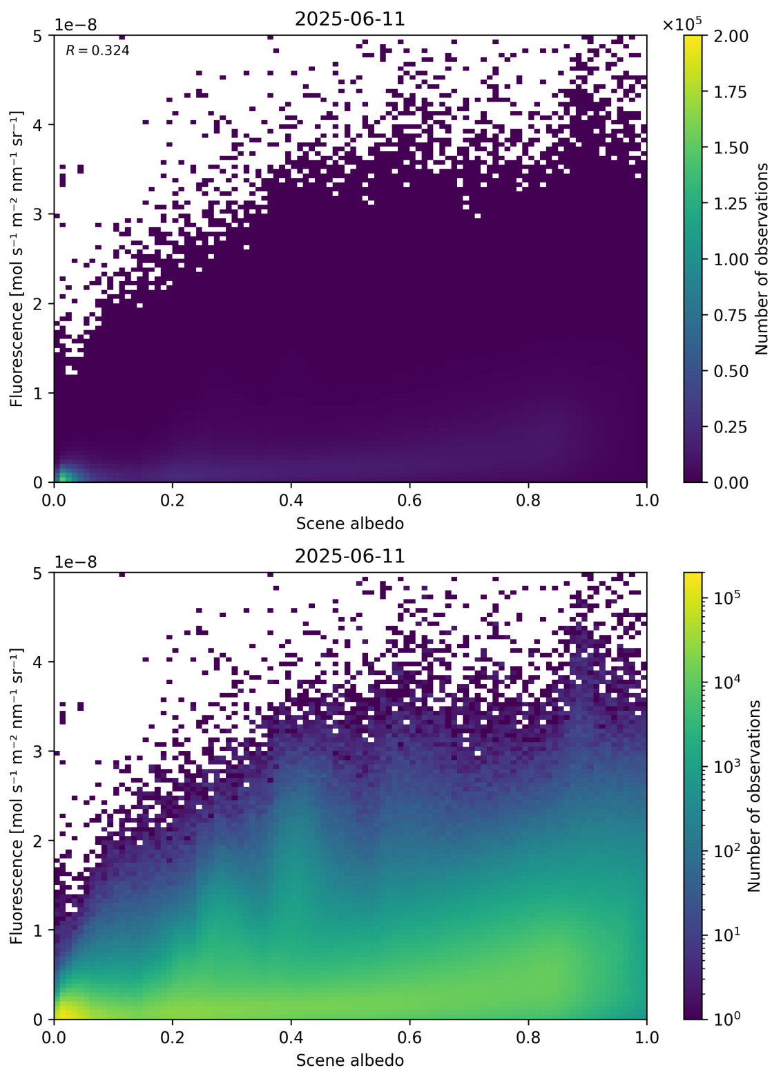
Figure 104: Scatter density plot of “Scene albedo” against “Fluorescence” for 2025-06-11 to 2025-06-12.
