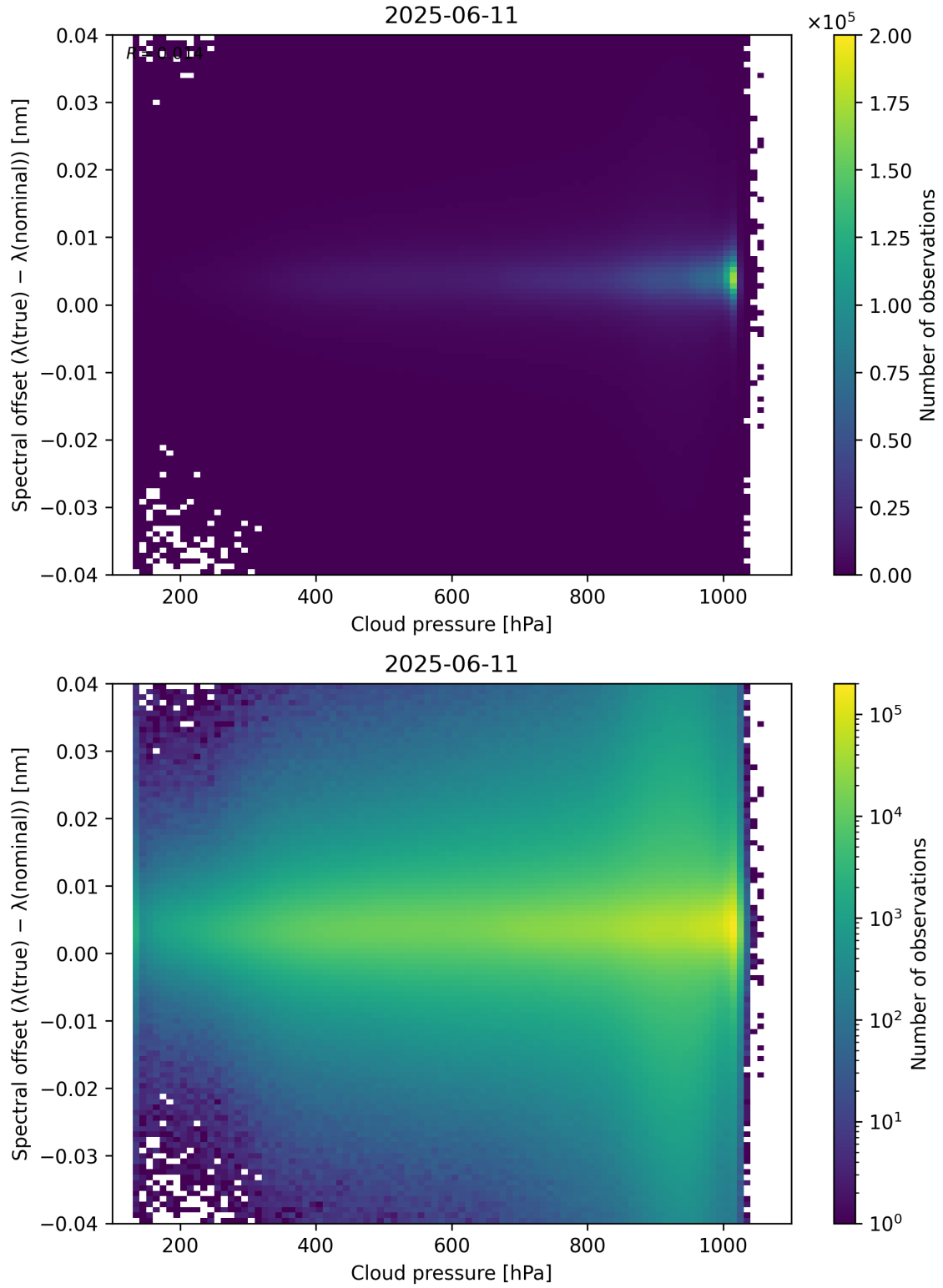
Figure 84: Scatter density plot of “Cloud pressure” against “Spectral offset ( \lambda_{\text{true}} - \lambda_{\text{nominal}} )” for 2025-06-11 to 2025-06-12.
