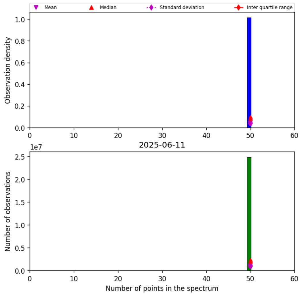
Figure 44: Histogram of “Number of points in the spectrum” for 2025-06-11 to 2025-06-12
