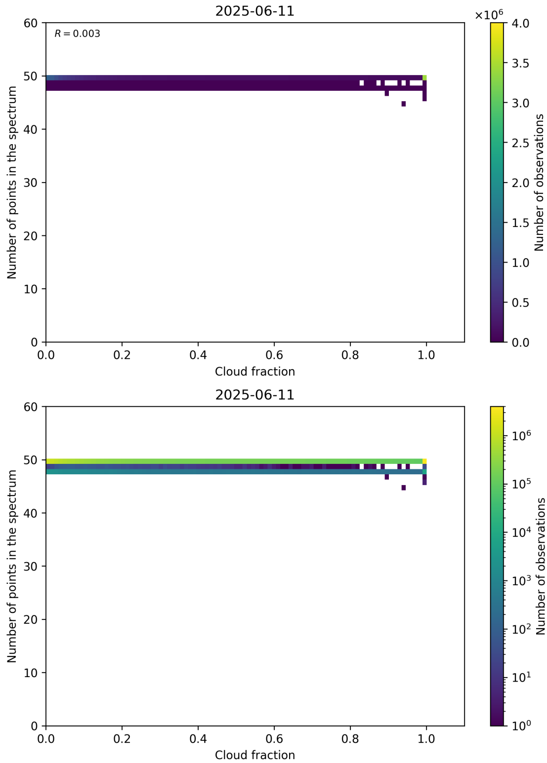
Figure 74: Scatter density plot of “Cloud fraction” against “Number of points in the spectrum” for 2025-06-11 to 2025-06-12.
