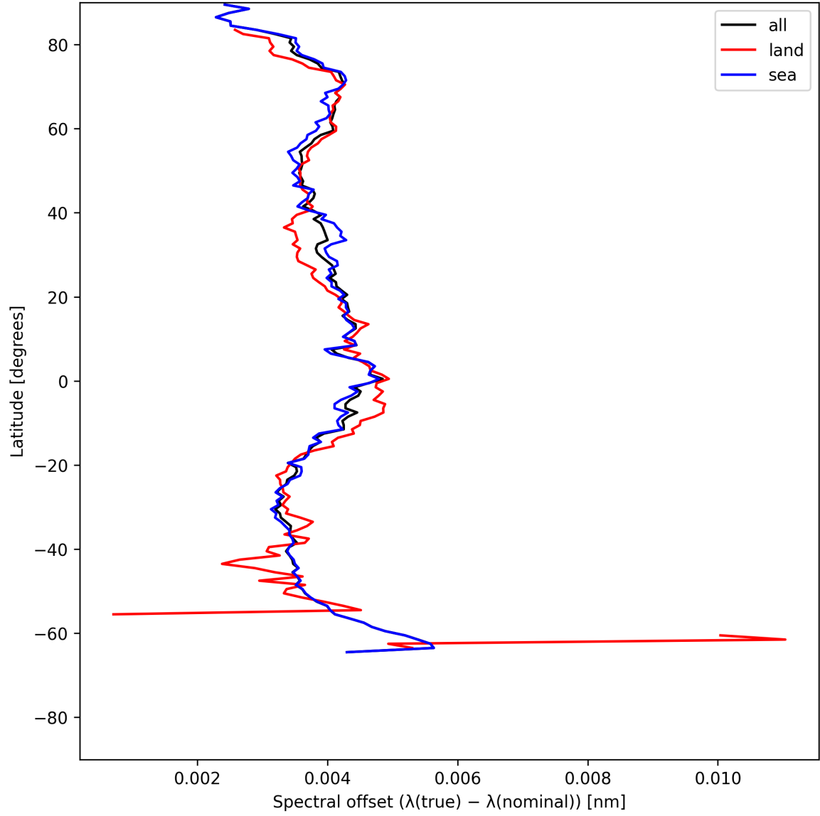
Figure 28: Zonal average of “Spectral offset ( \lambda_{\text{true}} - \lambda_{\text{nominal}} )” for 2025-06-11 to 2025-06-12.
