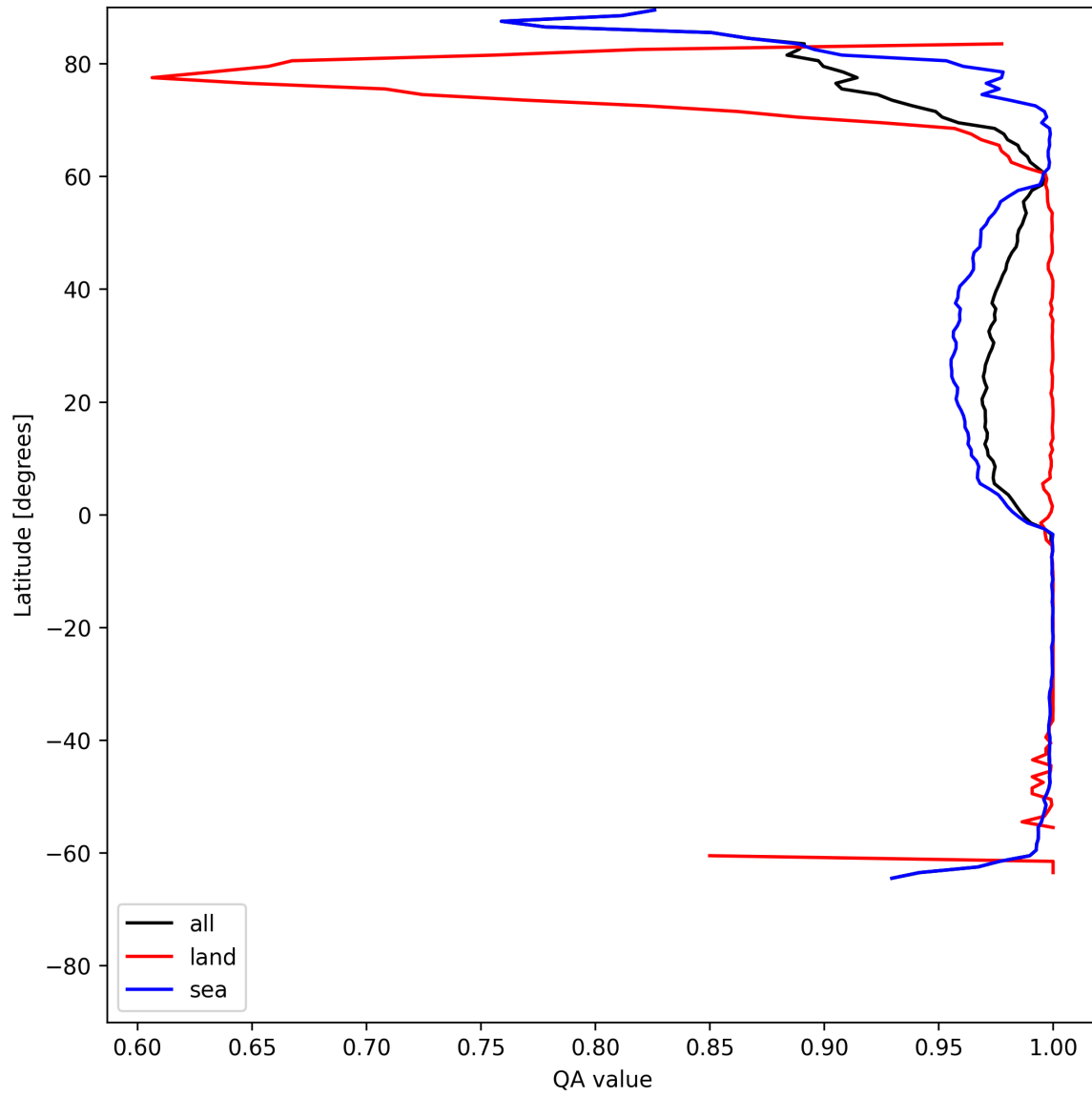
Figure 12: Zonal average of “QA value” for 2025-06-11 to 2025-06-12.
