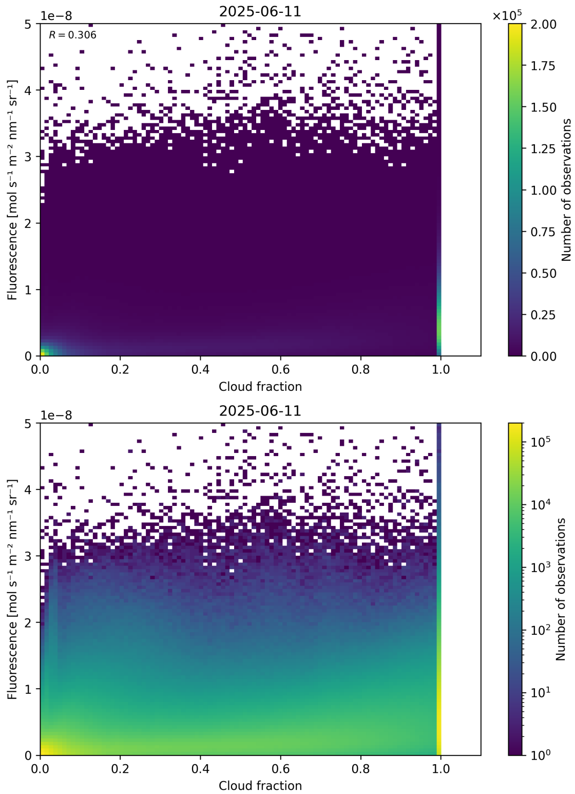
Figure 72: Scatter density plot of “Cloud fraction” against “Fluorescence” for 2025-06-11 to 2025-06-12.
