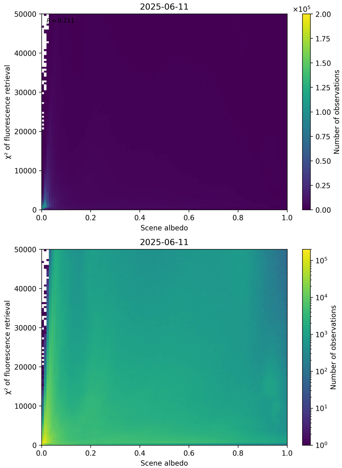
Figure 103: Scatter density plot of “Scene albedo” against “ \chi^2 of fluorescence retrieval” for 2025-06-11 to 2025-06-12.
