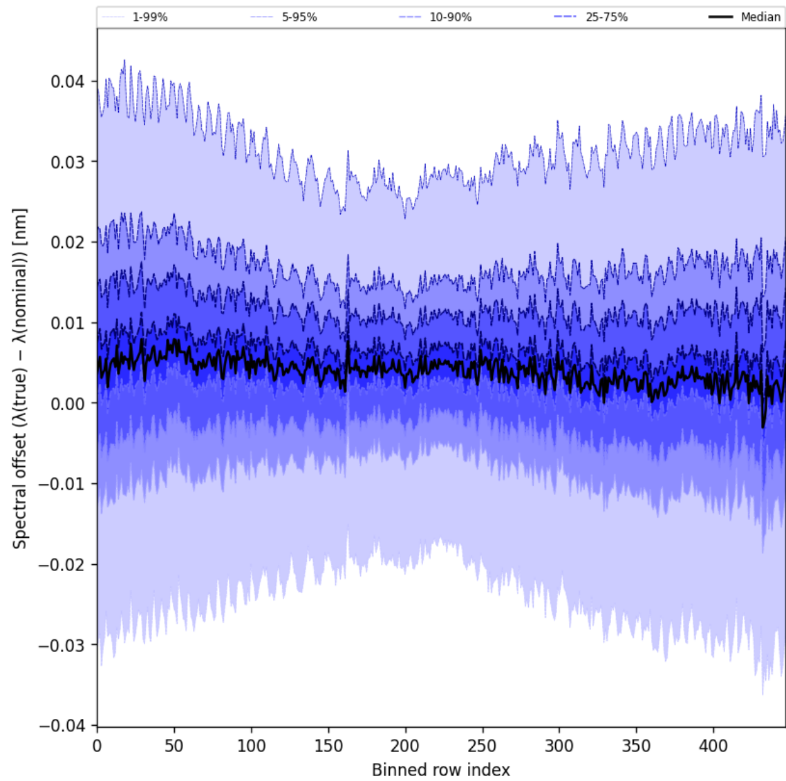
Figure 62: Along track statistics of “Spectral offset ( \lambda_{\text{true}} - \lambda_{\text{nominal}} )” for 2025-06-11 to 2025-06-12
