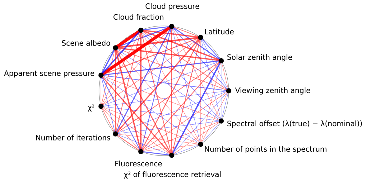
Figure 1: Map of correlation graph for 2025-06-11 to 2025-06-12.
