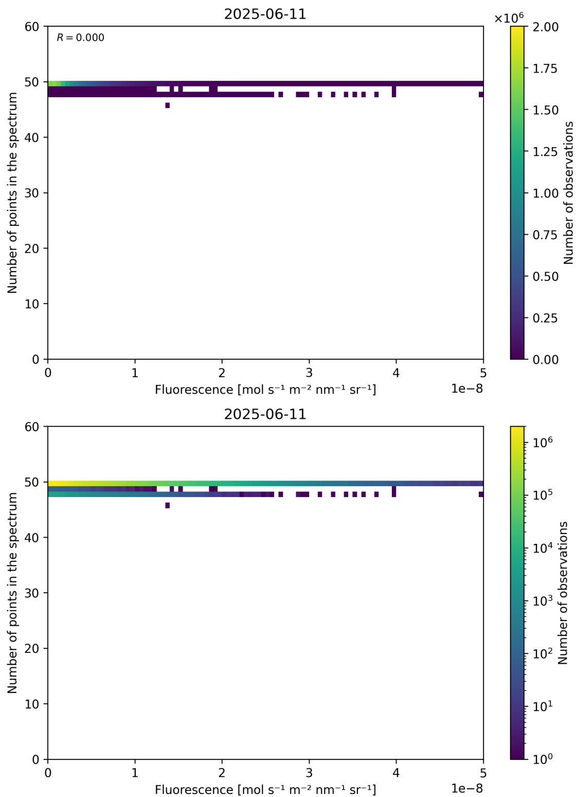
Figure 86: Scatter density plot of “Fluorescence” against “Number of points in the spectrum” for 2025-06-11 to 2025-06-12.
