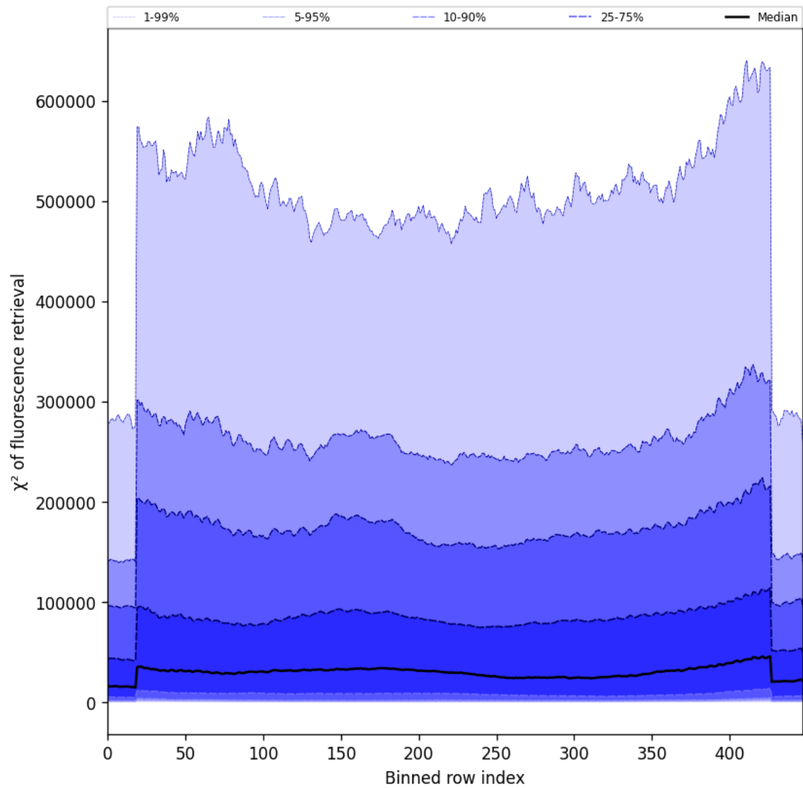
Figure 59: Along track statistics of “ \chi^2 of fluorescence retrieval” for 2025-06-11 to 2025-06-12
