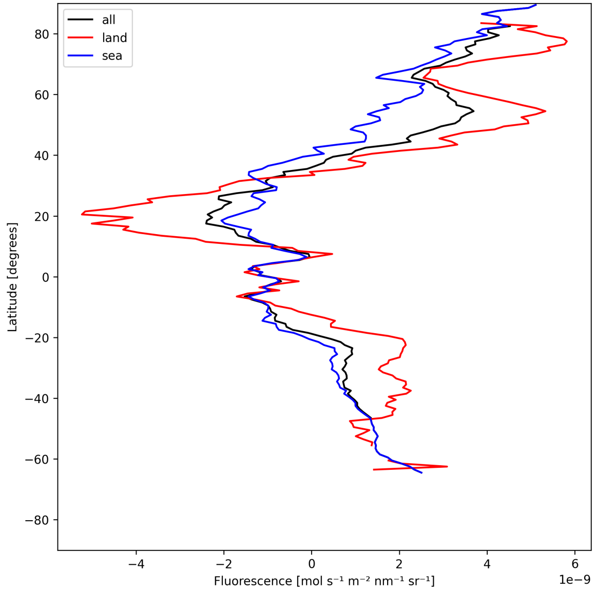
Figure 23: Zonal average of “Fluorescence” for 2025-06-11 to 2025-06-12.
