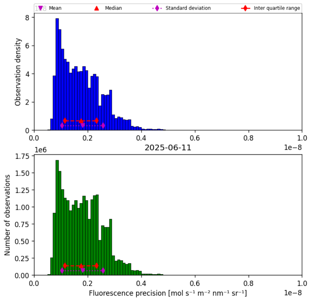
Figure 41: Histogram of “Fluorescence precision” for 2025-06-11 to 2025-06-12
