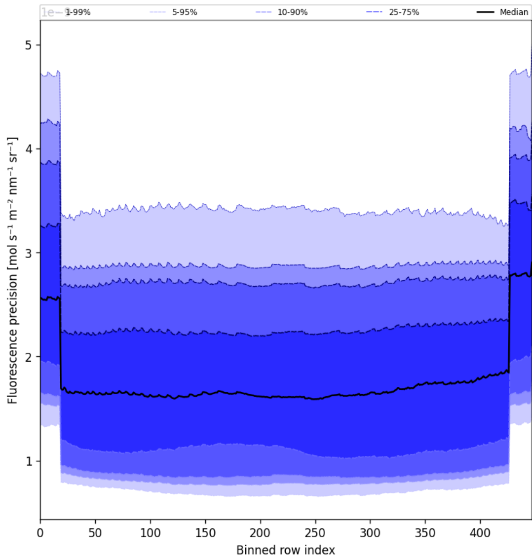
Figure 58: Along track statistics of "Fluorescence precision" for 2025-06-11 to 2025-06-12
