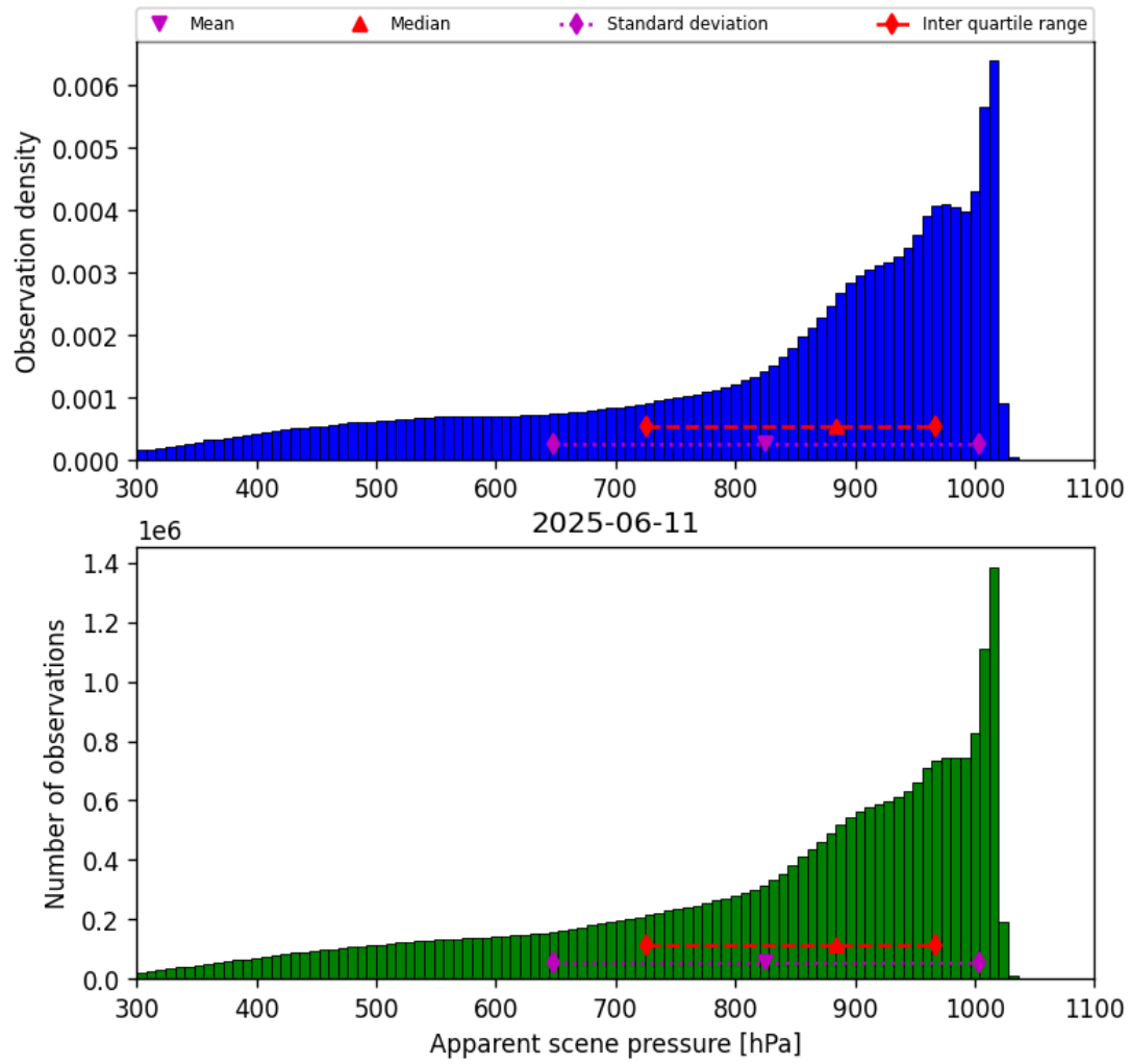
Figure 36: Histogram of “Apparent scene pressure” for 2025-06-11 to 2025-06-12
