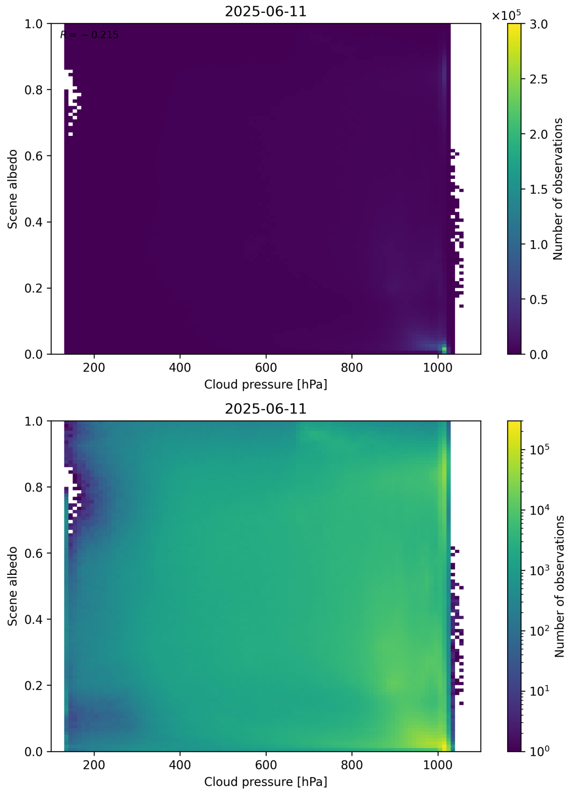
Figure 83: Scatter density plot of “Cloud pressure” against “Scene albedo” for 2025-06-11 to 2025-06-12.
