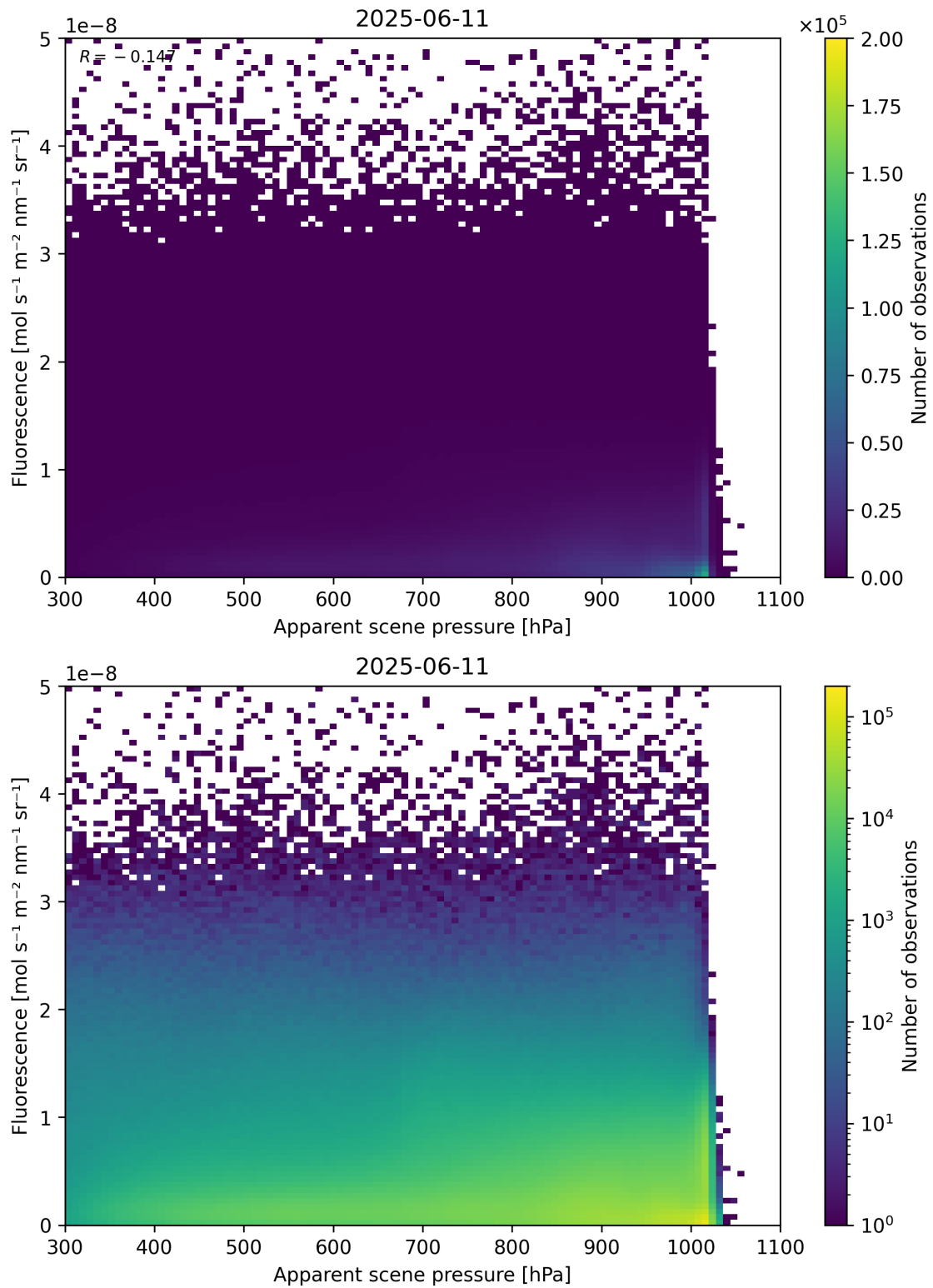
Figure 64: Scatter density plot of “Apparent scene pressure” against “Fluorescence” for 2025-06-11 to 2025-06-12.
