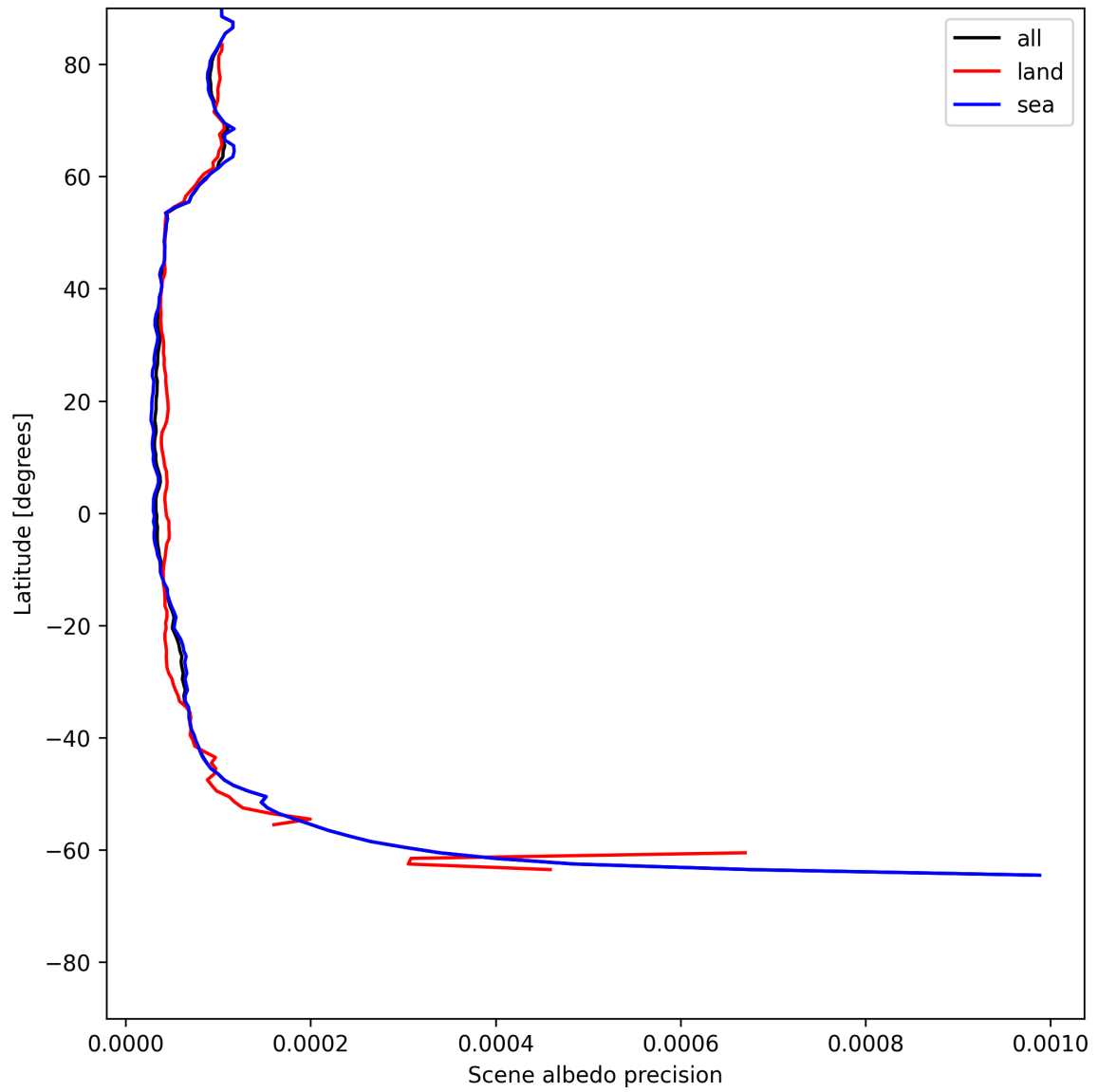
Figure 18: Zonal average of “Scene albedo precision” for 2025-06-11 to 2025-06-12.
