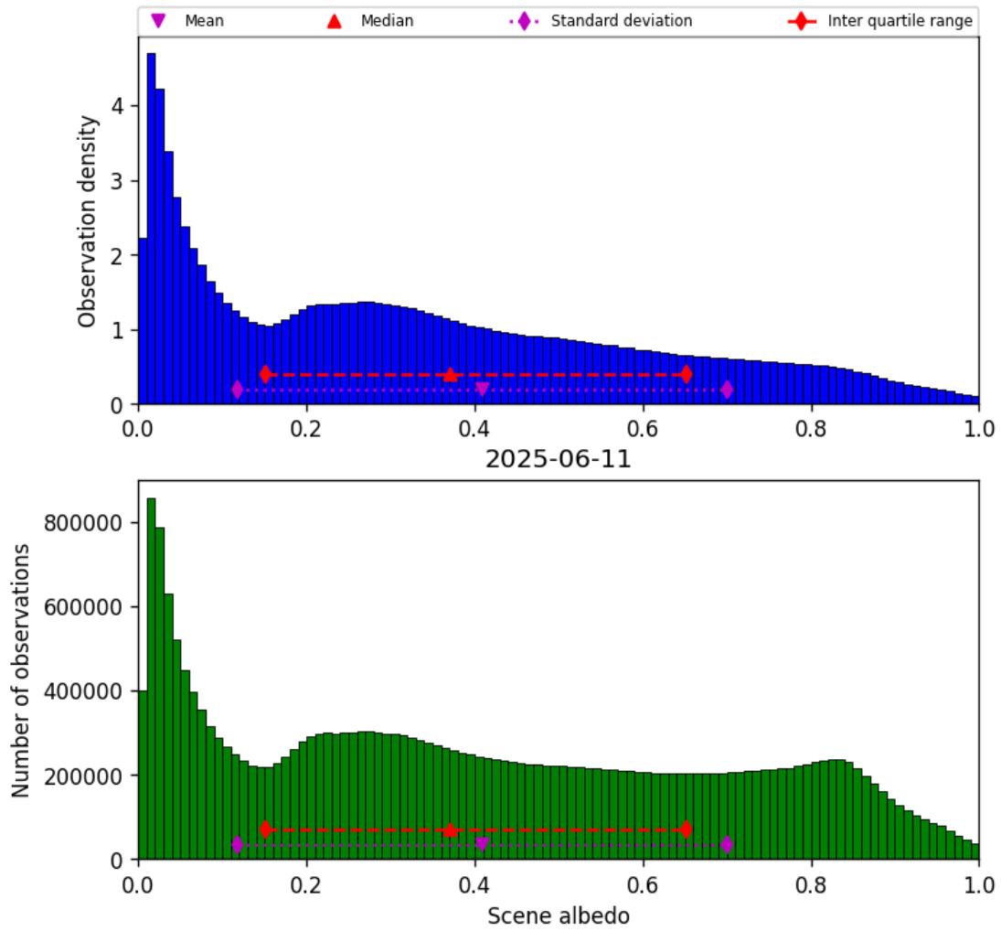
Figure 34: Histogram of “Scene albedo” for 2025-06-11 to 2025-06-12
