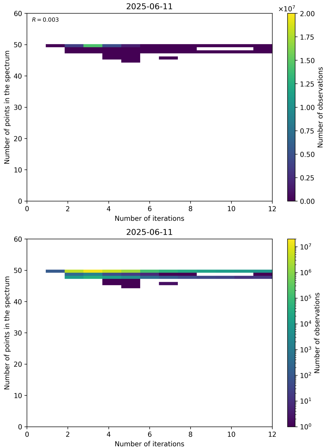
Figure 99: Scatter density plot of “Number of iterations” against “Number of points in the spectrum” for 2025-06-11 to 2025-06-12.
