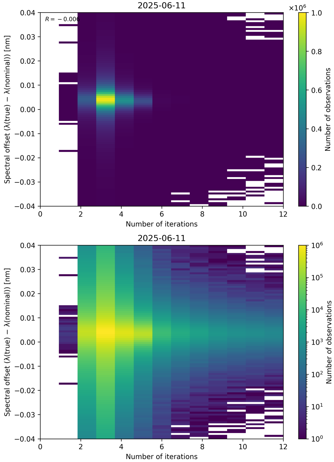
Figure 100: Scatter density plot of “Number of iterations” against “Spectral offset ( \lambda_{\text{true}} - \lambda_{\text{nominal}} )” for 2025-06-11 to 2025-06-12.
