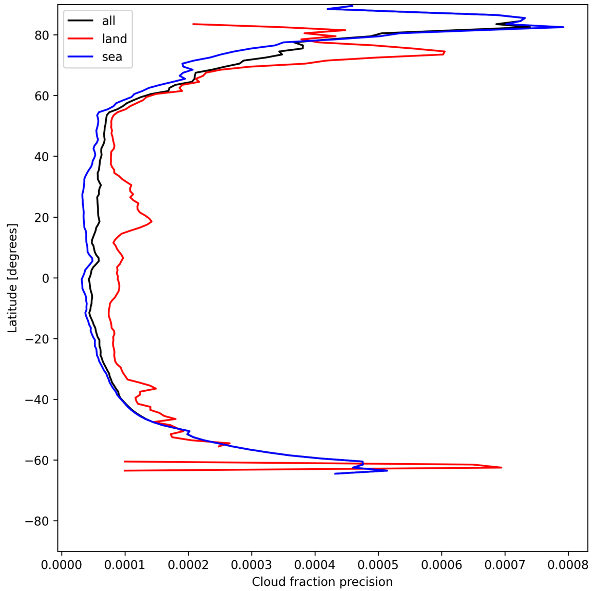
Figure 16: Zonal average of “Cloud fraction precision” for 2025-06-11 to 2025-06-12.
