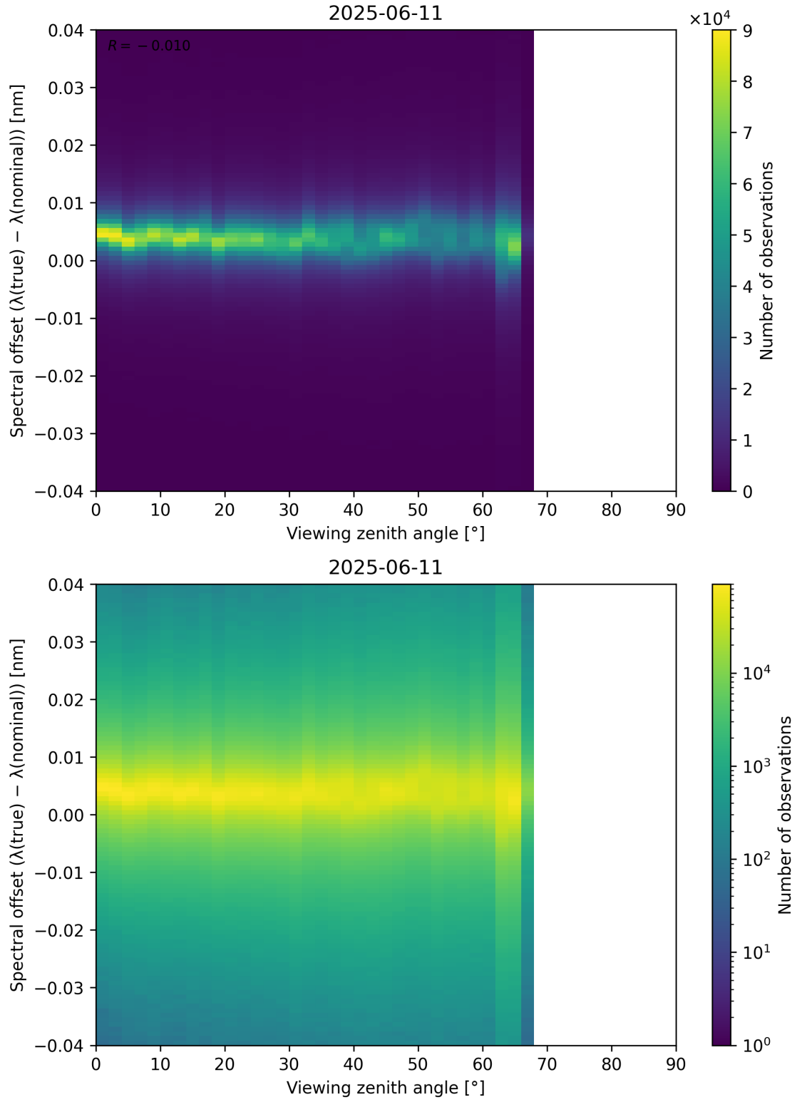
Figure 128: Scatter density plot of “Viewing zenith angle” against “Spectral offset ( \lambda_{\text{true}} - \lambda_{\text{nominal}} )” for 2025-06-11 to 2025-06-12.
