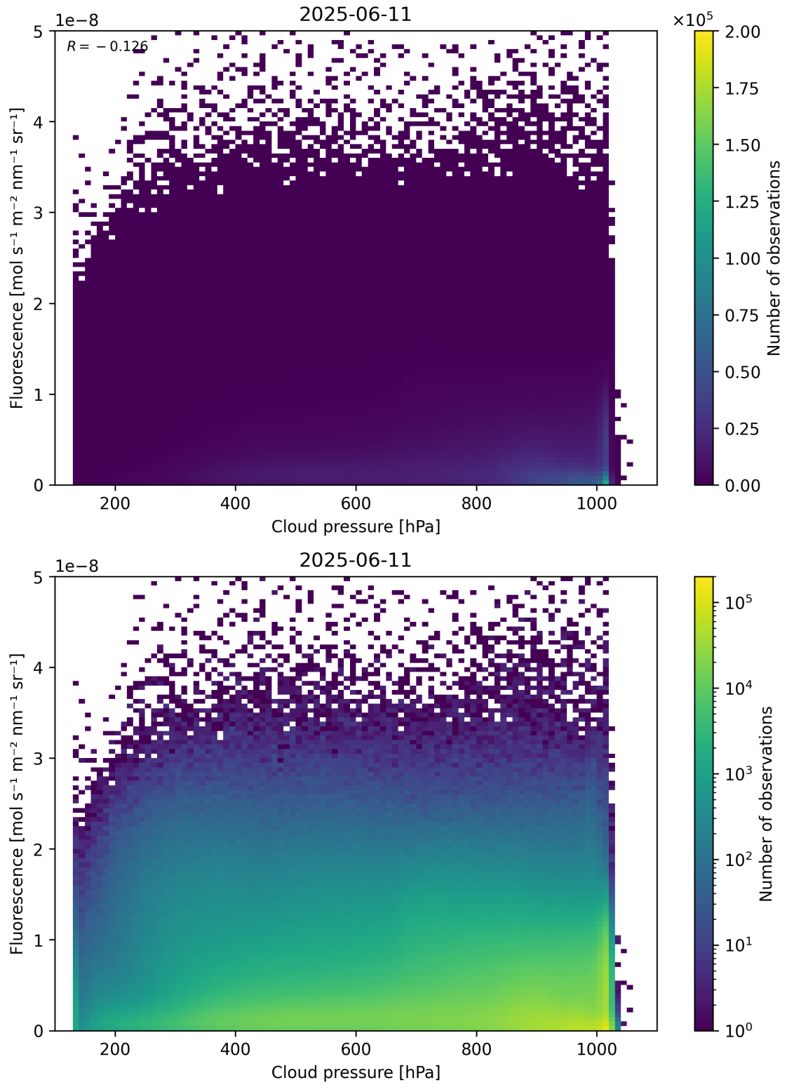
Figure 80: Scatter density plot of “Cloud pressure” against “Fluorescence” for 2025-06-11 to 2025-06-12.
