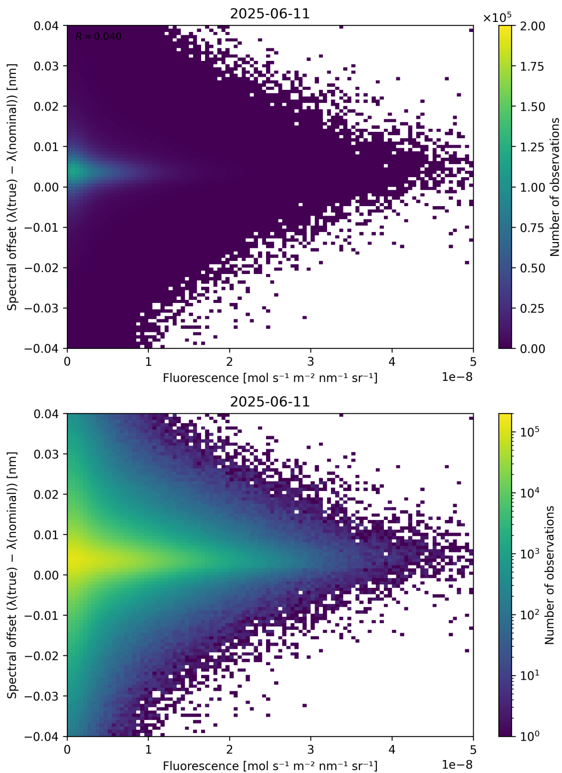
Figure 87: Scatter density plot of “Fluorescence” against “Spectral offset ( \lambda_{\text{true}} - \lambda_{\text{nominal}} )” for 2025-06-11 to 2025-06-12.
