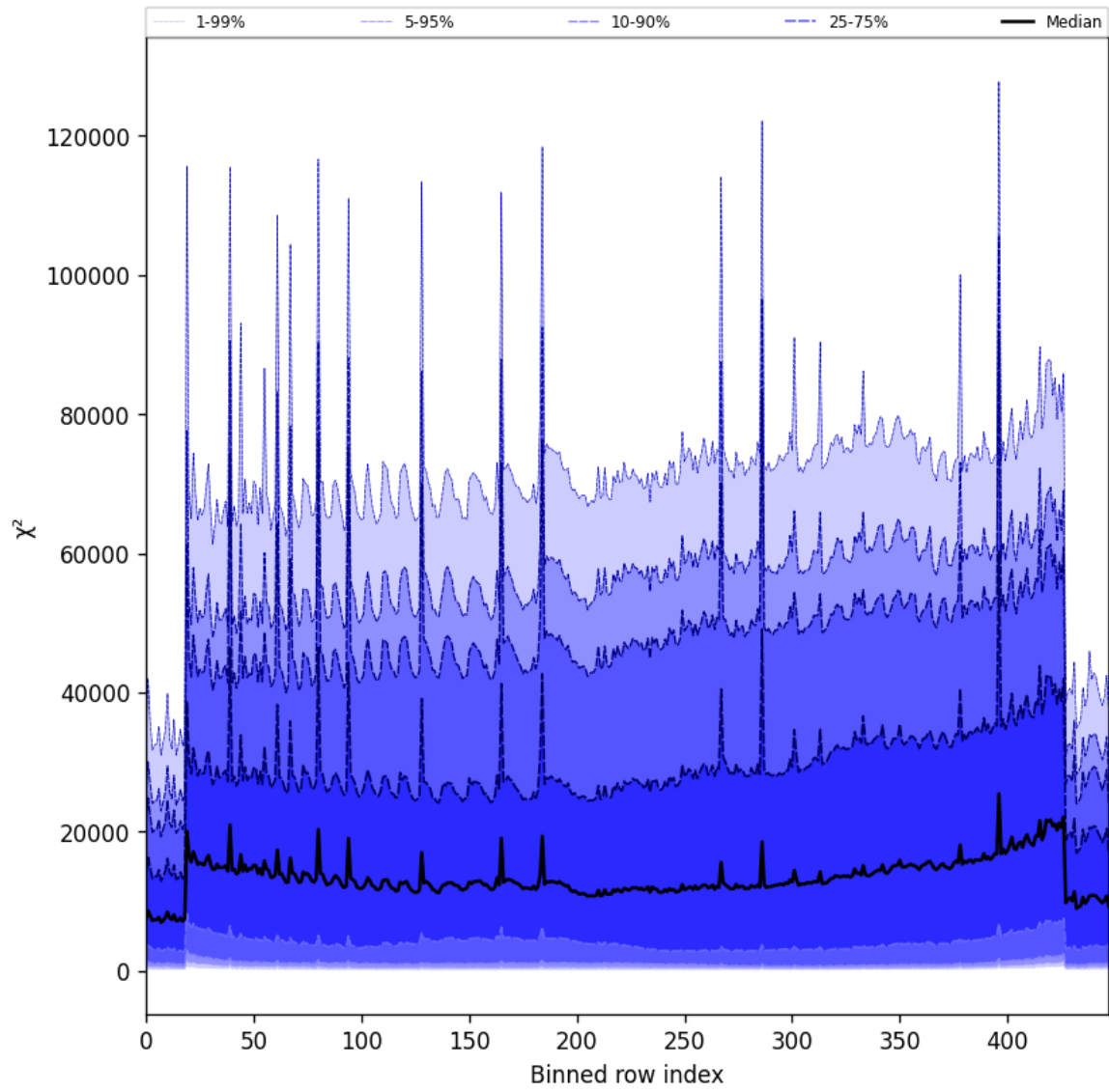
Figure 55: Along track statistics of “ \chi^2 ” for 2025-06-11 to 2025-06-12
