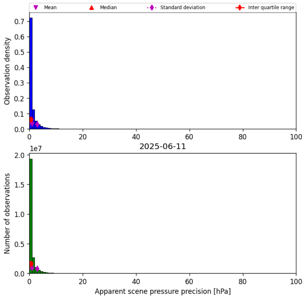
Figure 37: Histogram of “Apparent scene pressure precision” for 2025-06-11 to 2025-06-12
