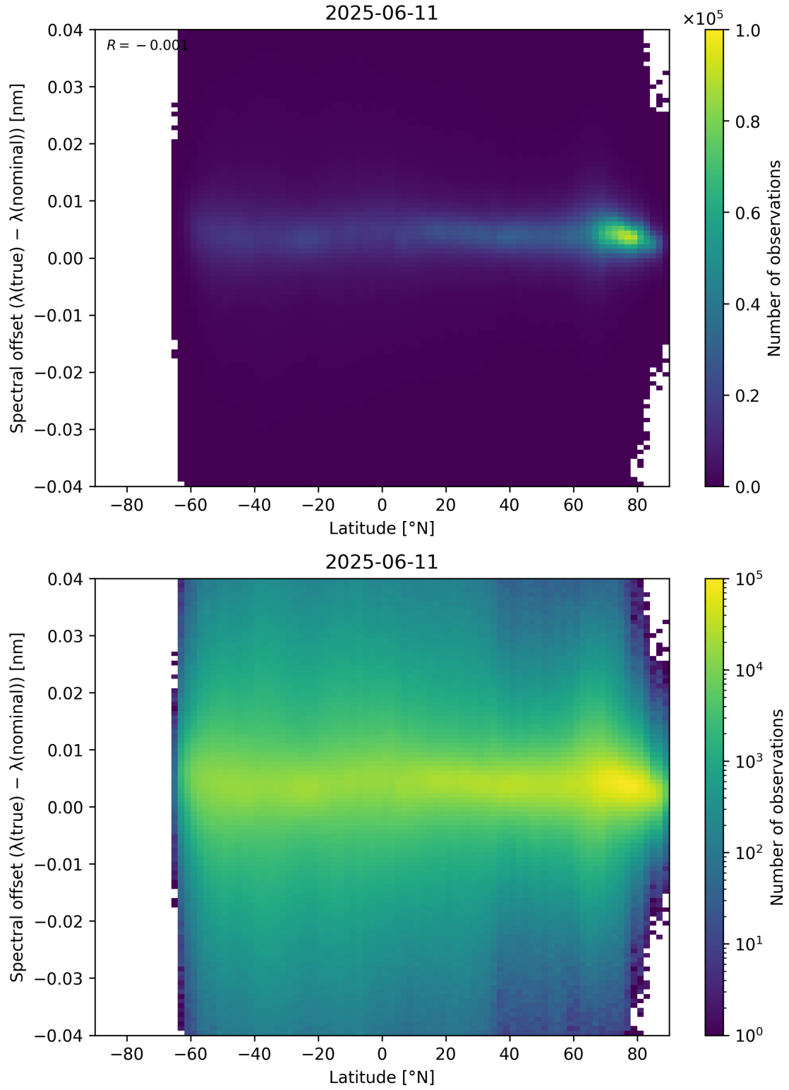
Figure 96: Scatter density plot of “Latitude” against “Spectral offset ( \lambda_{\text{true}} - \lambda_{\text{nominal}} )” for 2025-06-11 to 2025-06-12.
