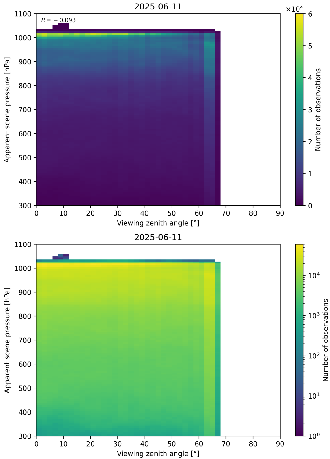
Figure 118: Scatter density plot of “Viewing zenith angle” against “Apparent scene pressure” for 2025-06-11 to 2025-06-12.
