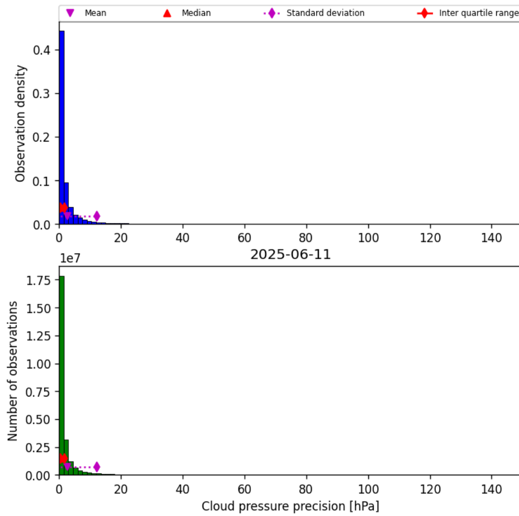
Figure 31: Histogram of “Cloud pressure precision” for 2025-06-11 to 2025-06-12
