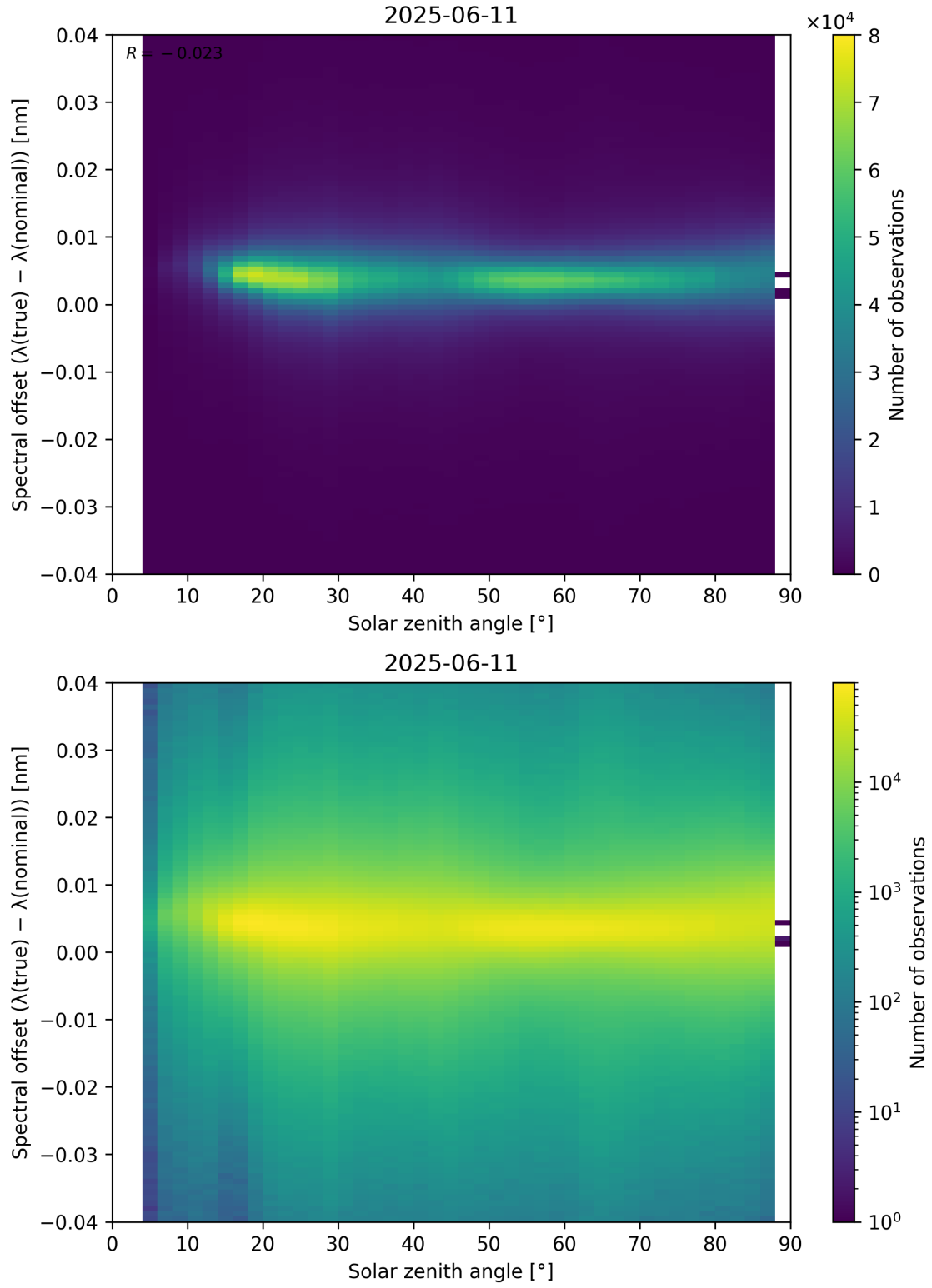
Figure 117: Scatter density plot of “Solar zenith angle” against “Spectral offset ( \lambda_{\text{true}} - \lambda_{\text{nominal}} )” for 2025-06-11 to 2025-06-12.
