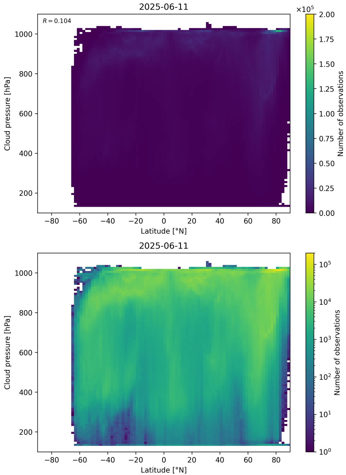
Figure 91: Scatter density plot of “Latitude” against “Cloud pressure” for 2025-06-11 to 2025-06-12.
