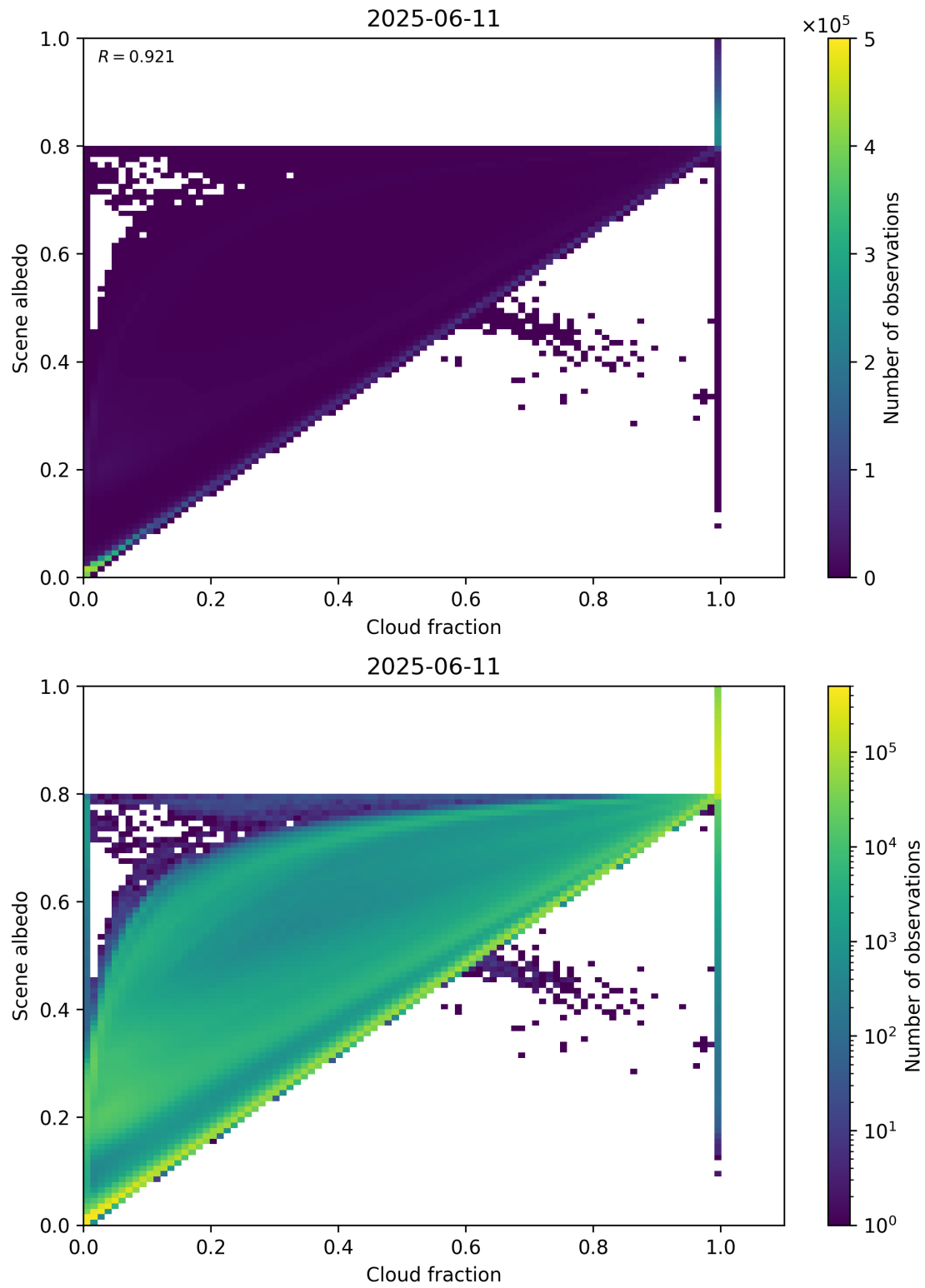
Figure 75: Scatter density plot of “Cloud fraction” against “Scene albedo” for 2025-06-11 to 2025-06-12.
