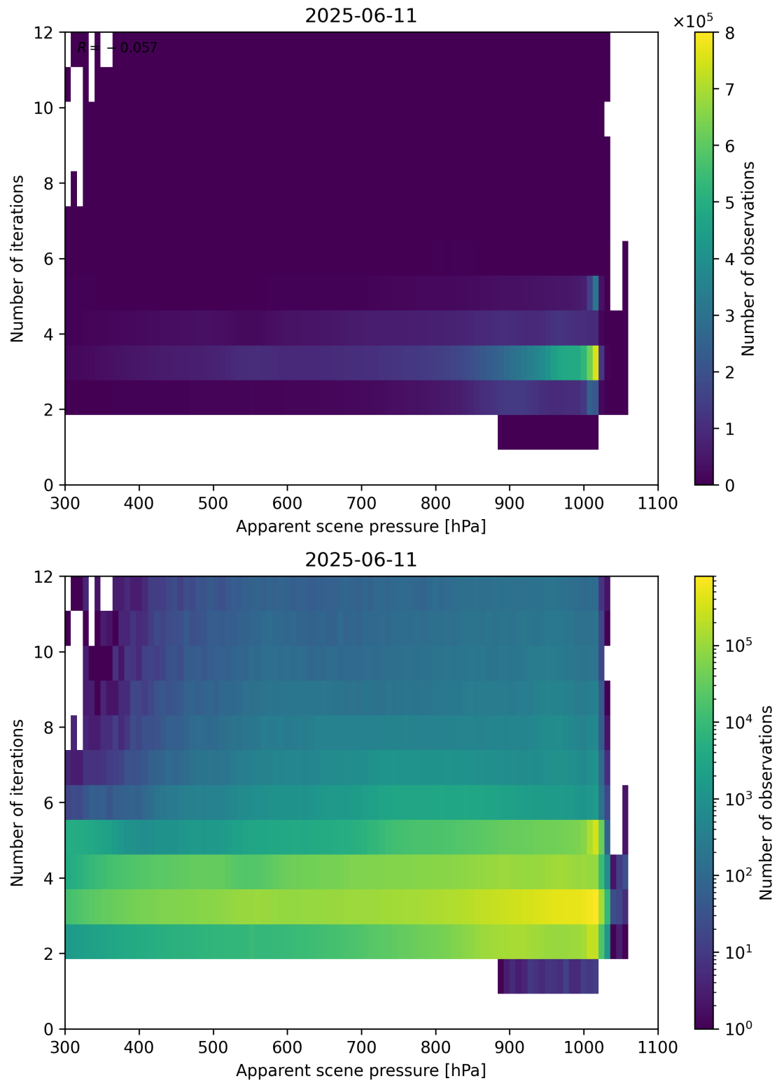
Figure 65: Scatter density plot of “Apparent scene pressure” against “Number of iterations” for 2025-06-11 to 2025-06-12.
