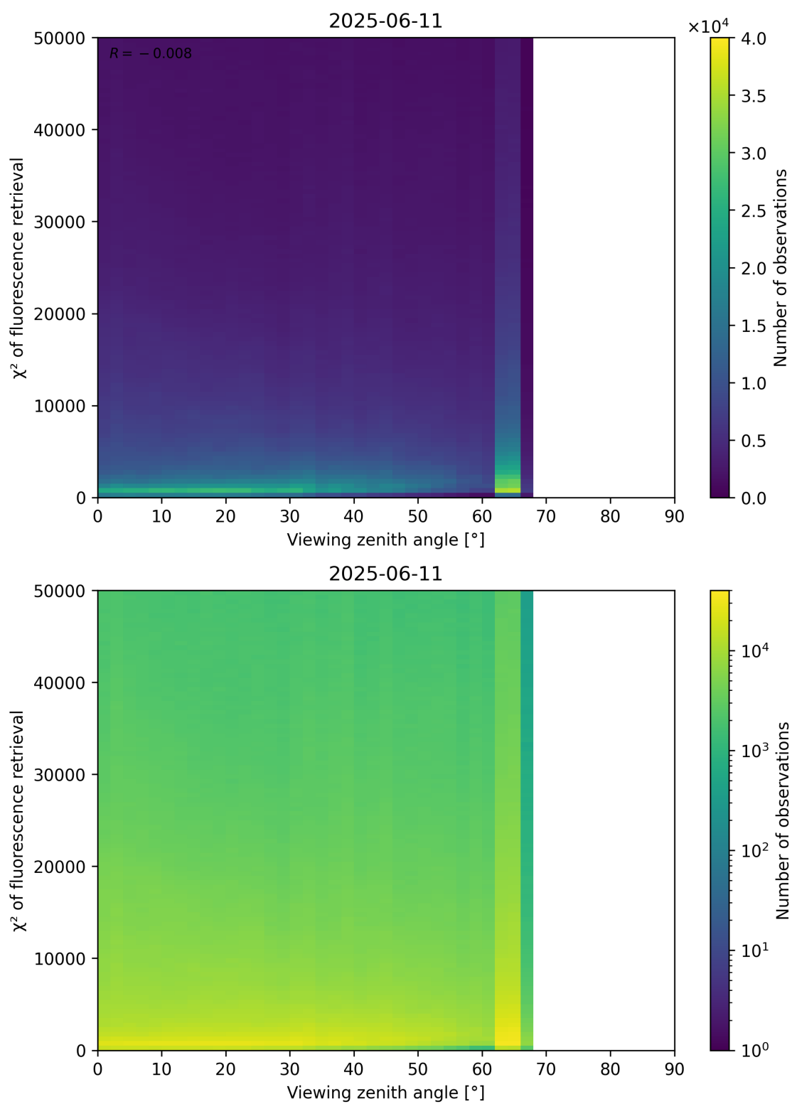
Figure 119: Scatter density plot of “Viewing zenith angle” against “ \chi^2 of fluorescence retrieval” for 2025-06-11 to 2025-06-12.
