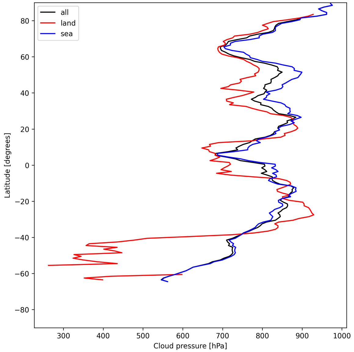
Figure 13: Zonal average of “Cloud pressure” for 2025-06-11 to 2025-06-12.
