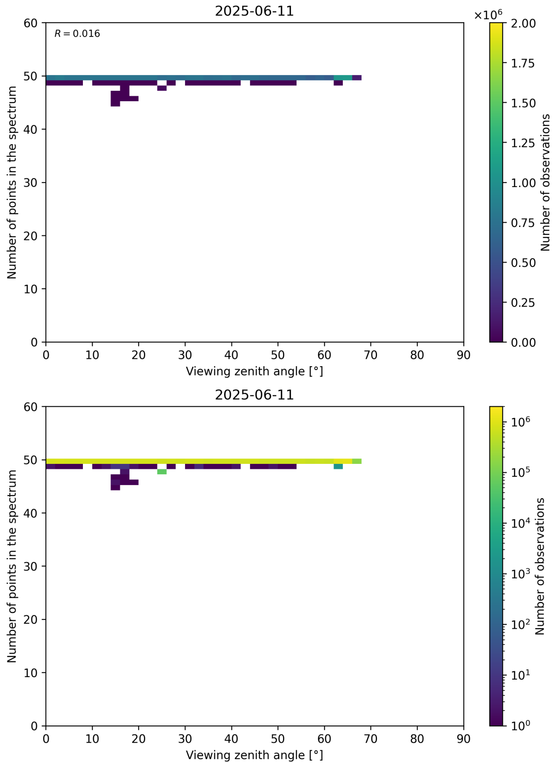
Figure 125: Scatter density plot of “Viewing zenith angle” against “Number of points in the spectrum” for 2025-06-11 to 2025-06-12.
