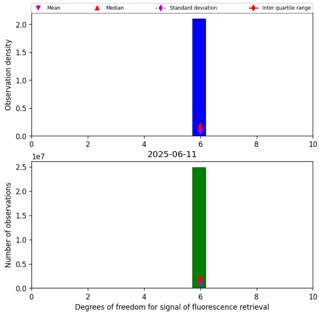
Figure 43: Histogram of “Degrees of freedom for signal of fluorescence retrieval” for 2025-06-11 to 2025-06-12
