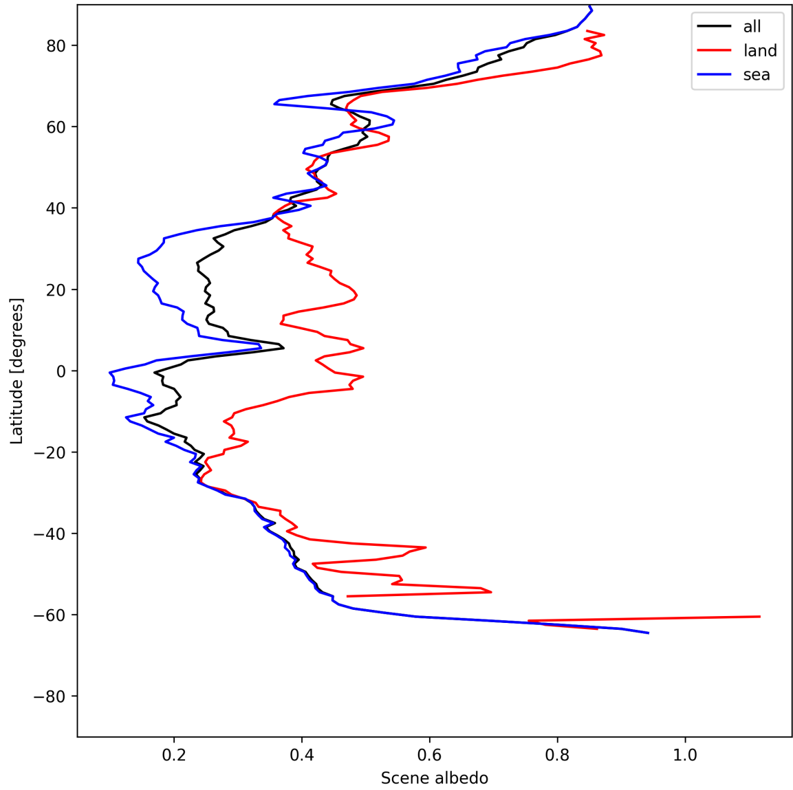
Figure 17: Zonal average of “Scene albedo” for 2025-06-11 to 2025-06-12.
