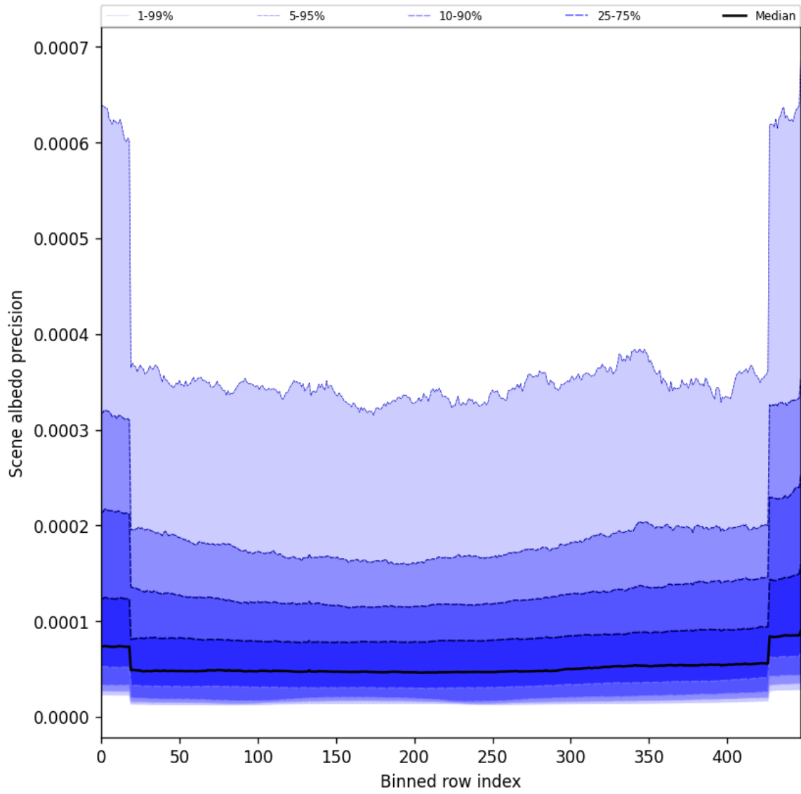
Figure 52: Along track statistics of “Scene albedo precision” for 2025-06-11 to 2025-06-12
