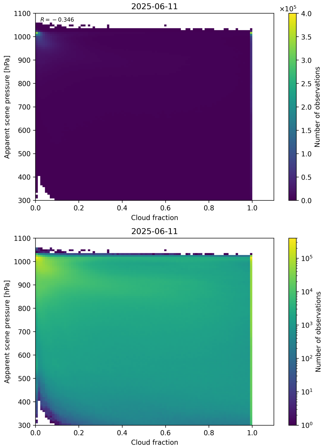
Figure 70: Scatter density plot of “Cloud fraction” against “Apparent scene pressure” for 2025-06-11 to 2025-06-12.
