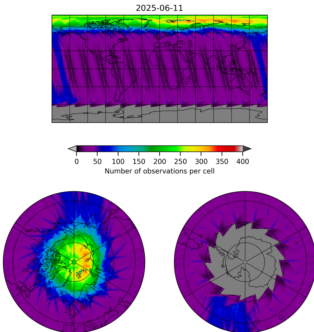
Figure 11: Map of the number of observations for 2025-06-11 to 2025-06-12
