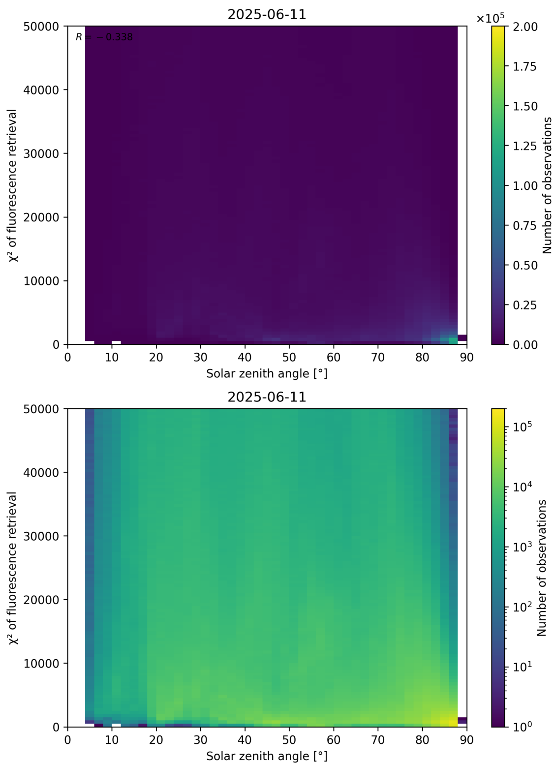
Figure 109: Scatter density plot of “Solar zenith angle” against “ \chi^2 of fluorescence retrieval” for 2025-06-11 to 2025-06-12.
