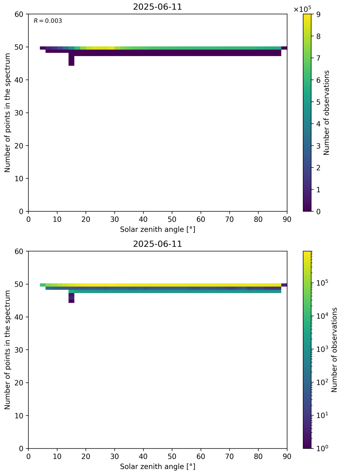
Figure 115: Scatter density plot of “Solar zenith angle” against “Number of points in the spectrum” for 2025-06-11 to 2025-06-12.
