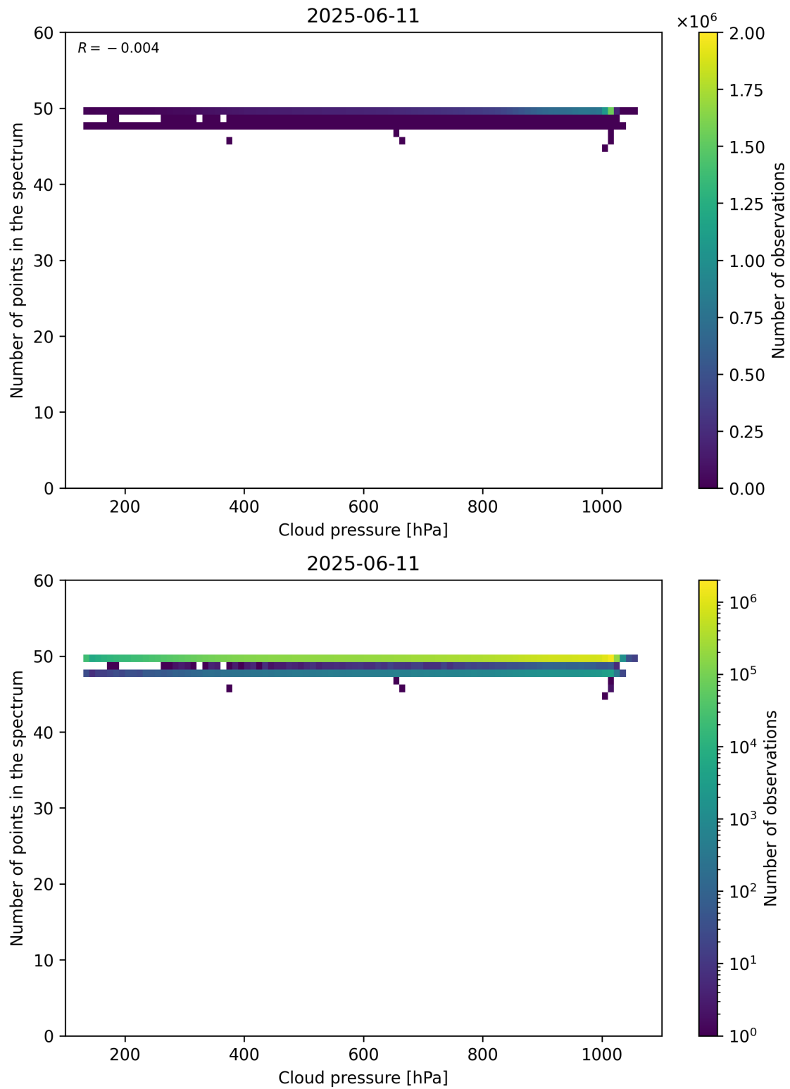
Figure 82: Scatter density plot of “Cloud pressure” against “Number of points in the spectrum” for 2025-06-11 to 2025-06-12.
