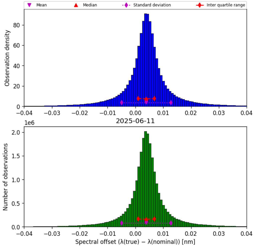
Figure 45: Histogram of “Spectral offset ( \lambda_{\text{true}} - \lambda_{\text{nominal}} )” for 2025-06-11 to 2025-06-12
