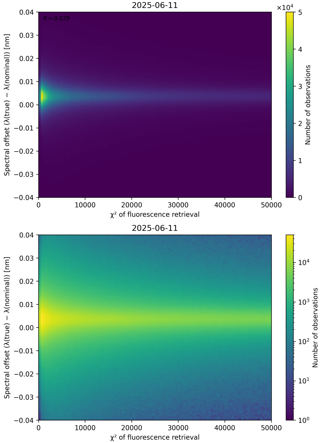
Figure 69: Scatter density plot of “ \chi^2 of fluorescence retrieval” against “Spectral offset ( \lambda_{\text{true}} - \lambda_{\text{nominal}} )” for 2025-06-11 to 2025-06-12.
