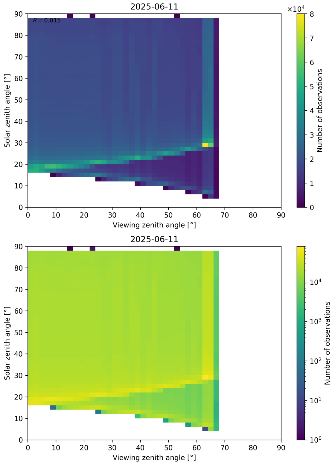
Figure 127: Scatter density plot of “Viewing zenith angle” against “Solar zenith angle” for 2025-06-11 to 2025-06-12.
