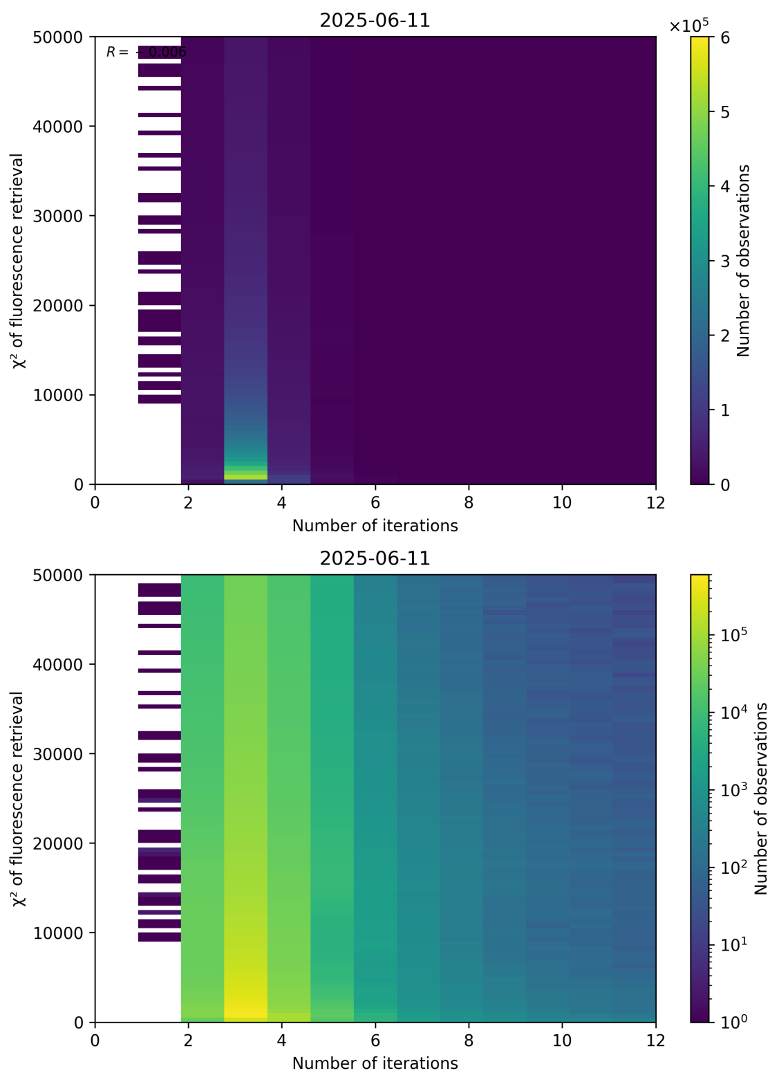
Figure 97: Scatter density plot of “Number of iterations” against “ \chi^2 of fluorescence retrieval” for 2025-06-11 to 2025-06-12.
