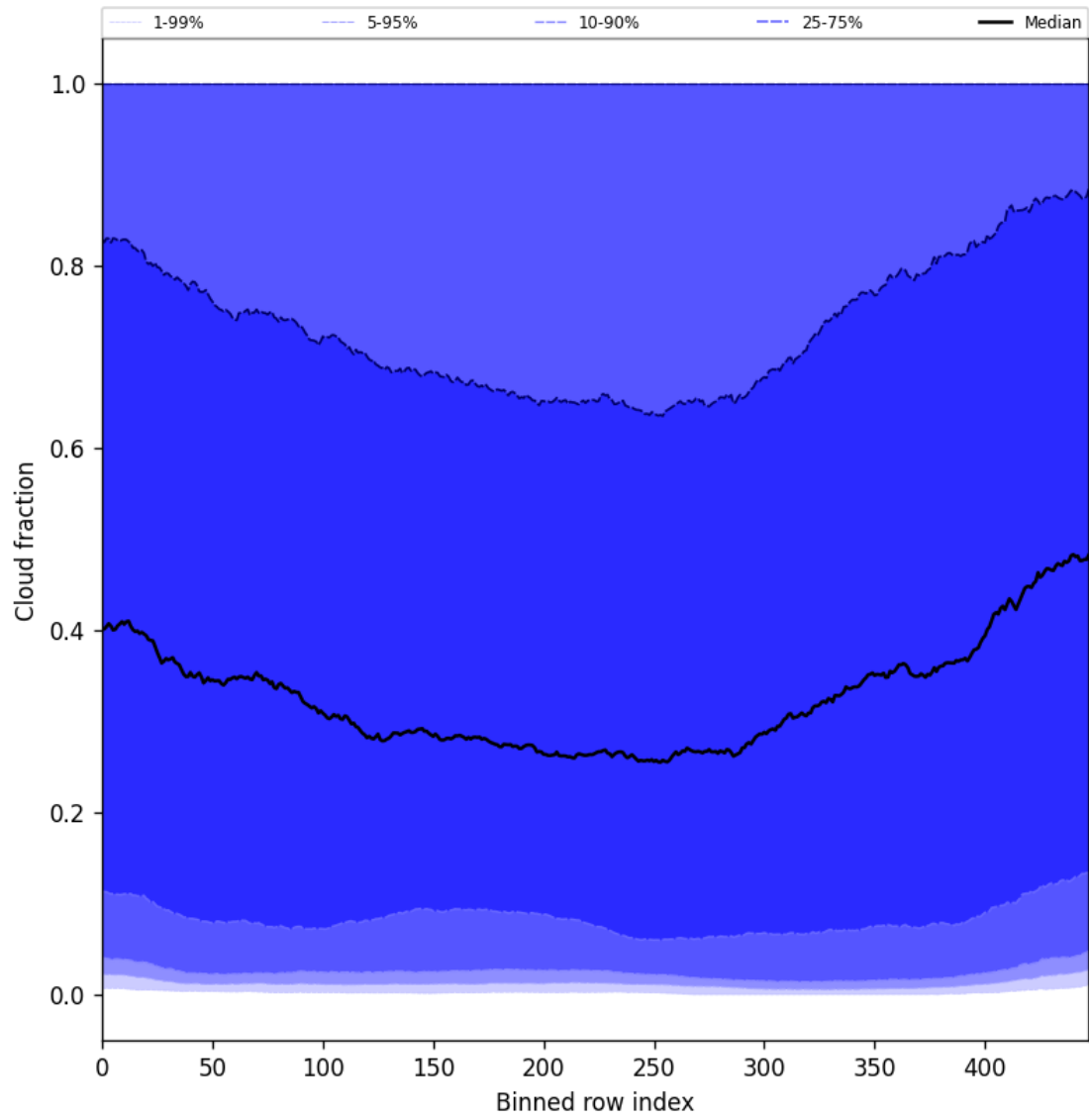
Figure 49: Along track statistics of “Cloud fraction” for 2025-06-11 to 2025-06-12
