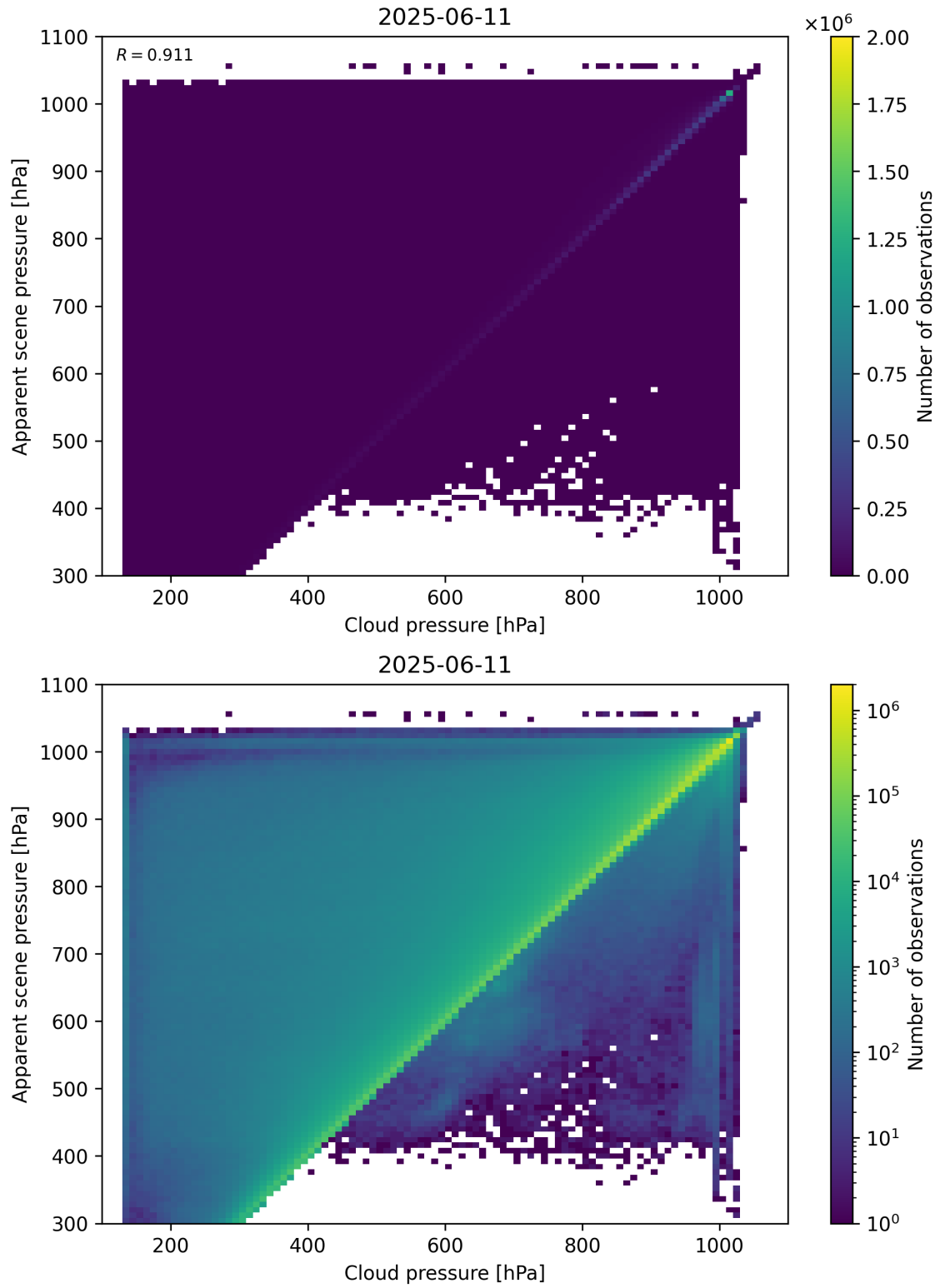
Figure 77: Scatter density plot of “Cloud pressure” against “Apparent scene pressure” for 2025-06-11 to 2025-06-12.
