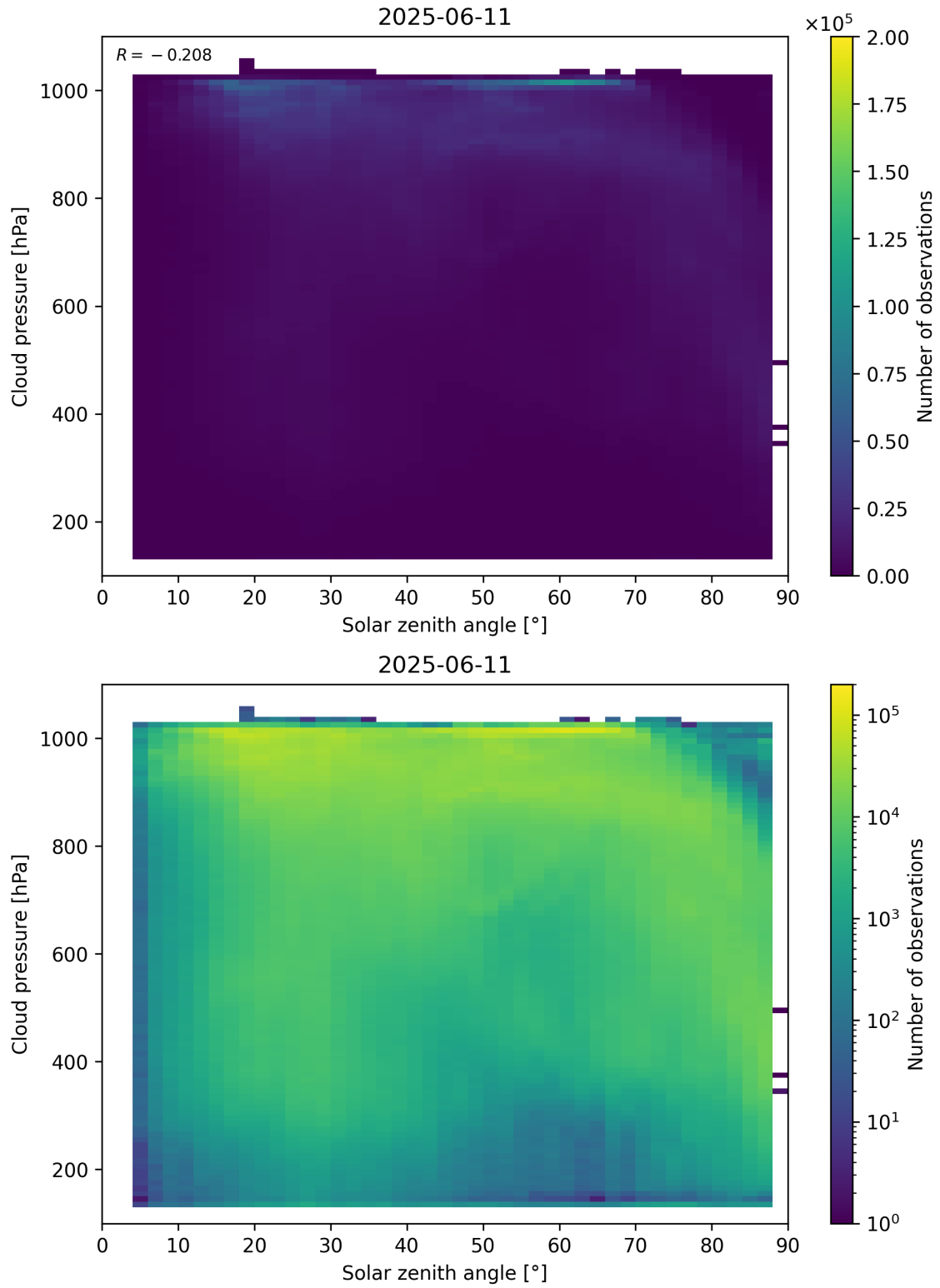
Figure 111: Scatter density plot of “Solar zenith angle” against “Cloud pressure” for 2025-06-11 to 2025-06-12.
