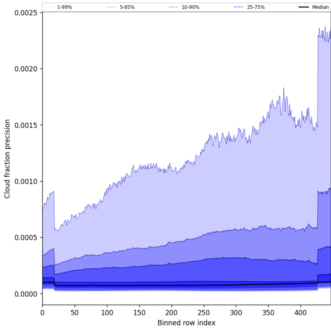
Figure 50: Along track statistics of “Cloud fraction precision” for 2025-06-11 to 2025-06-12
