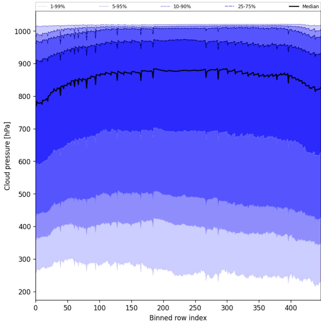
Figure 47: Along track statistics of “Cloud pressure” for 2025-06-11 to 2025-06-12
