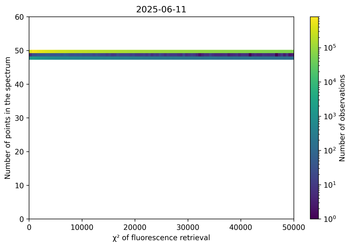
Figure 68: Scatter density plot of “ \chi^2 of fluorescence retrieval” against “Number of points in the spectrum” for 2025-06-11 to 2025-06-12.
