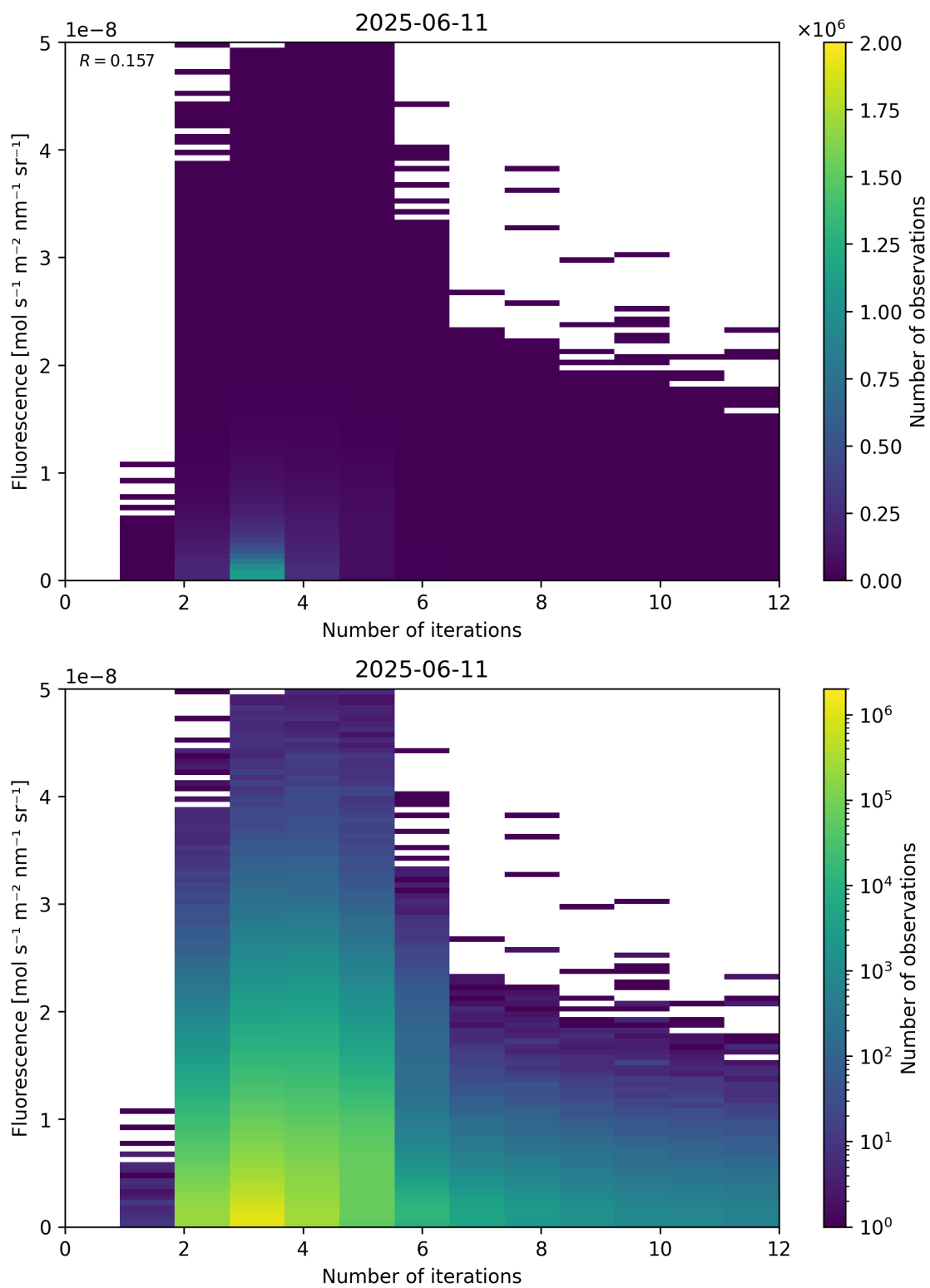
Figure 98: Scatter density plot of “Number of iterations” against “Fluorescence” for 2025-06-11 to 2025-06-12.
