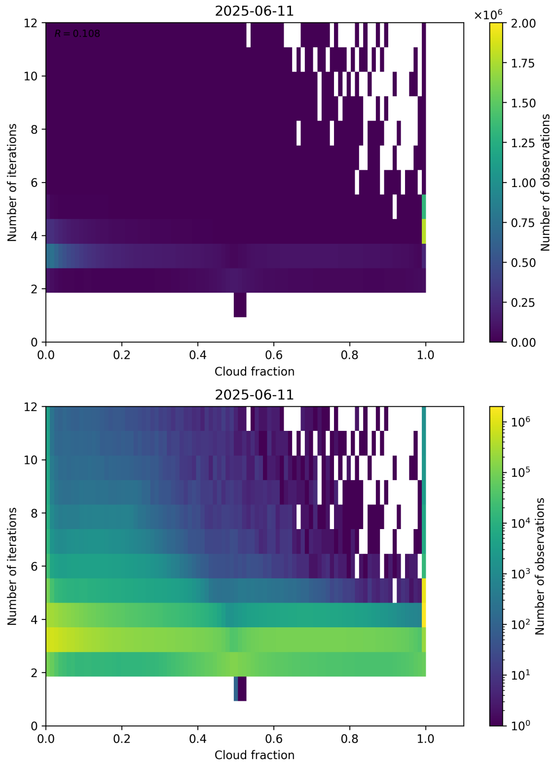
Figure 73: Scatter density plot of “Cloud fraction” against “Number of iterations” for 2025-06-11 to 2025-06-12.
