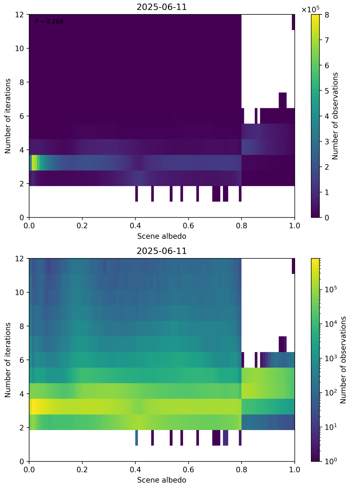
Figure 105: Scatter density plot of “Scene albedo” against “Number of iterations” for 2025-06-11 to 2025-06-12.
