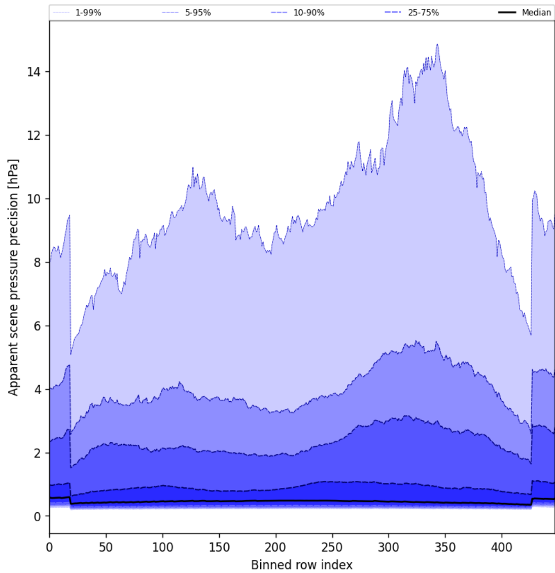
Figure 54: Along track statistics of “Apparent scene pressure precision” for 2025-06-11 to 2025-06-12
