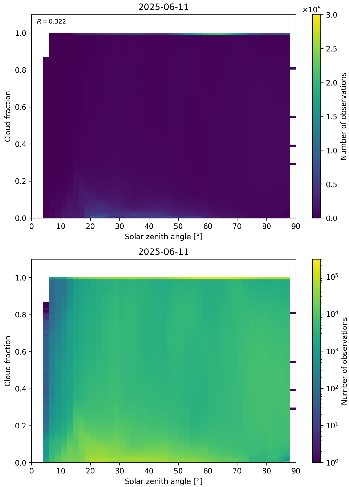
Figure 110: Scatter density plot of “Solar zenith angle” against “Cloud fraction” for 2025-06-11 to 2025-06-12.
