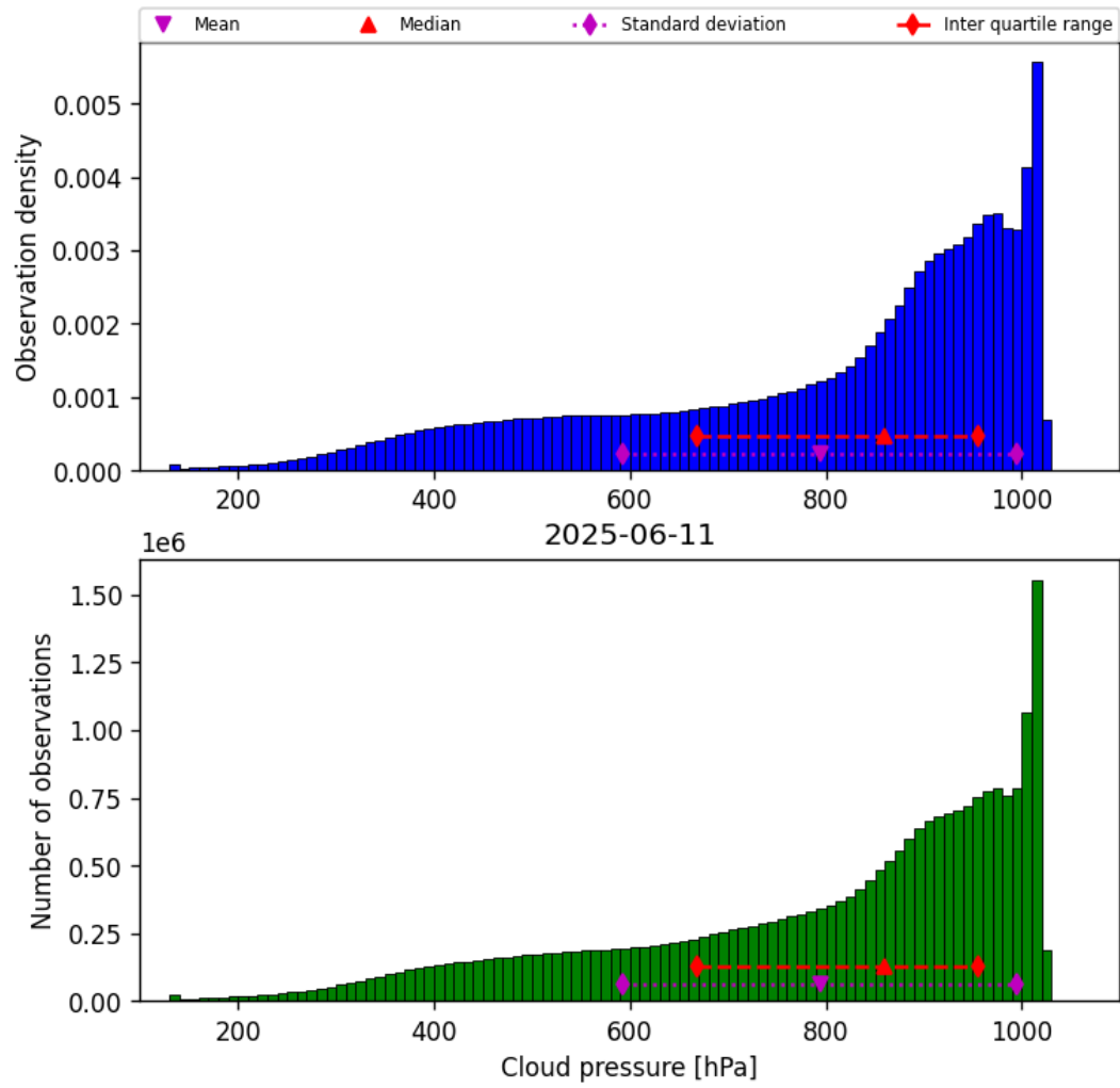
Figure 30: Histogram of “Cloud pressure” for 2025-06-11 to 2025-06-12
