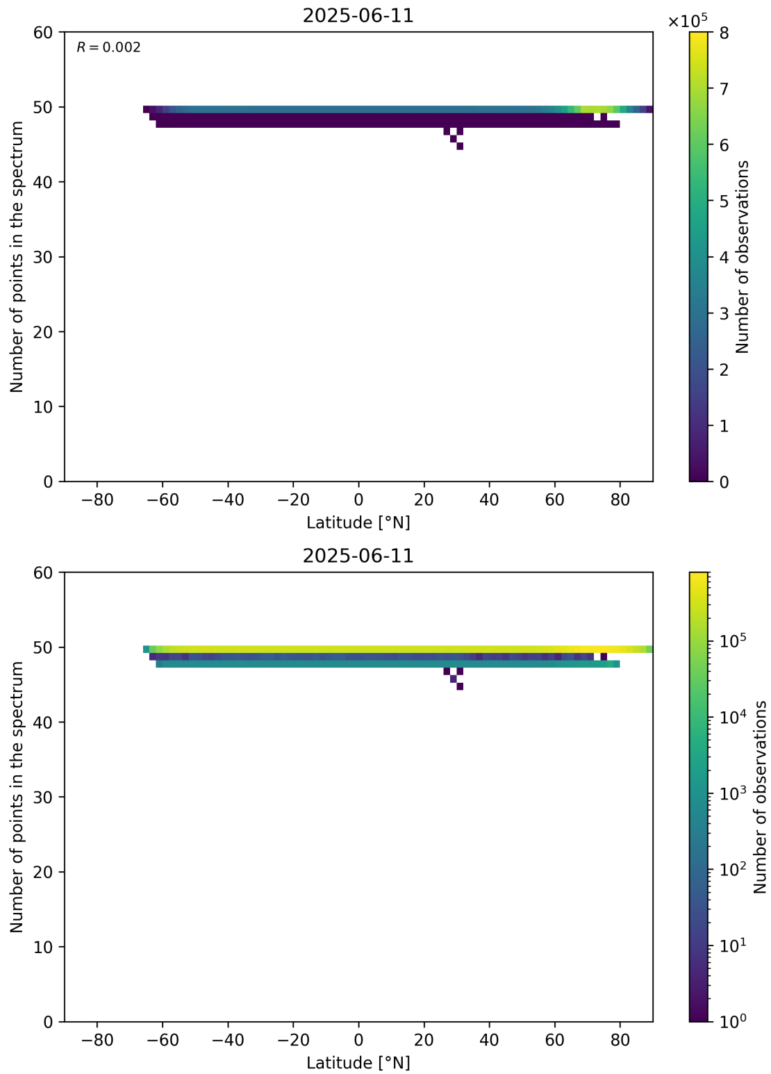
Figure 94: Scatter density plot of “Latitude” against “Number of points in the spectrum” for 2025-06-11 to 2025-06-12.
