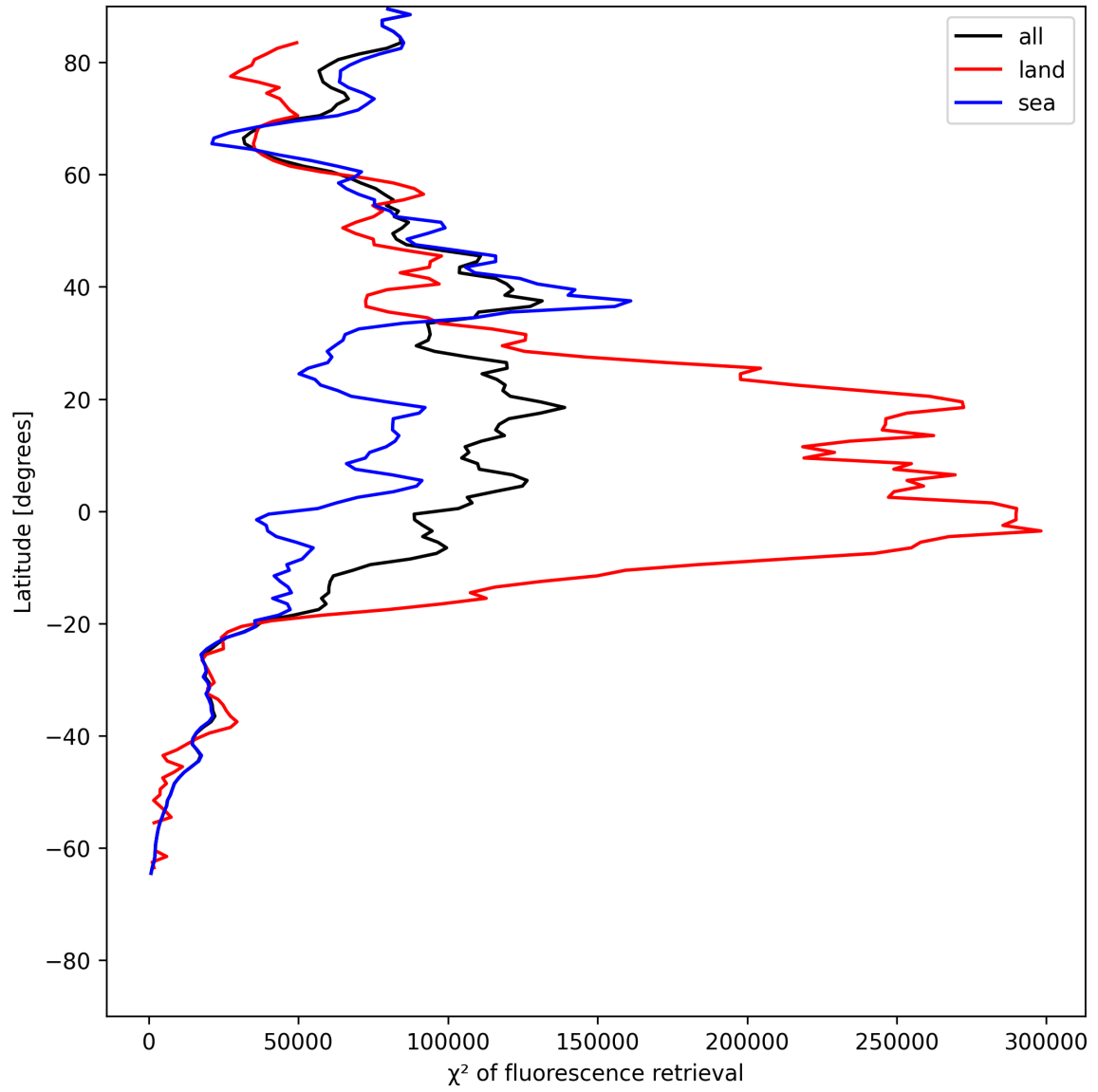
Figure 25: Zonal average of “ \chi^2 of fluorescence retrieval” for 2025-06-11 to 2025-06-12.
