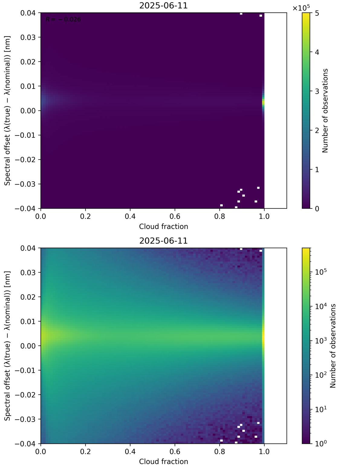
Figure 76: Scatter density plot of “Cloud fraction” against “Spectral offset ( \lambda_{\text{true}} - \lambda_{\text{nominal}} )” for 2025-06-11 to 2025-06-12.
