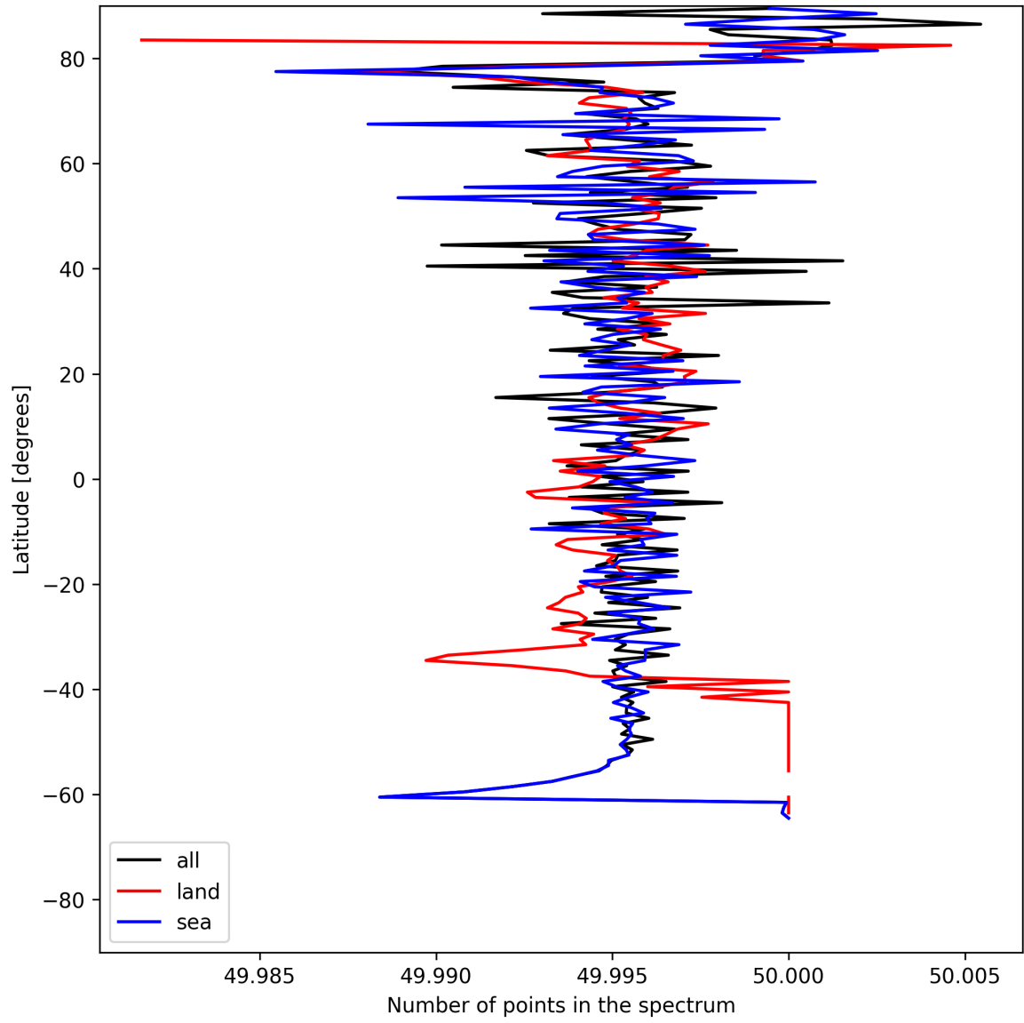
Figure 27: Zonal average of “Number of points in the spectrum” for 2025-06-11 to 2025-06-12.
