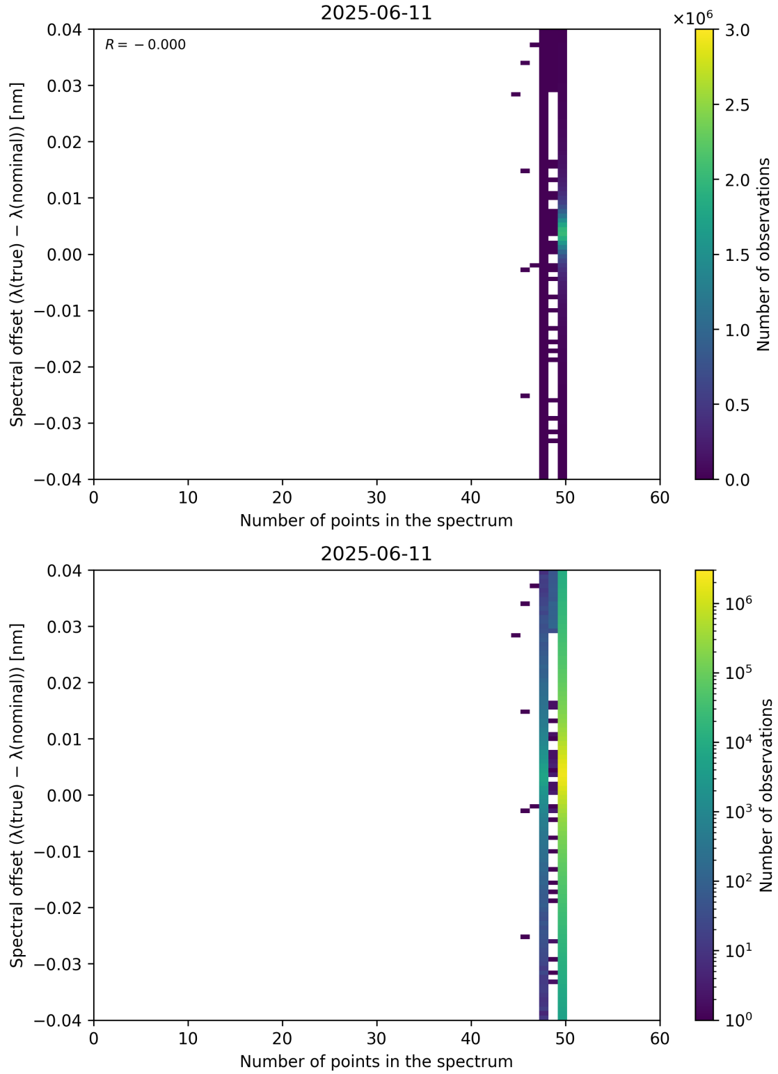
Figure 101: Scatter density plot of “Number of points in the spectrum” against “Spectral offset ( \lambda_{\text{true}} - \lambda_{\text{nominal}} )” for 2025-06-11 to 2025-06-12.
