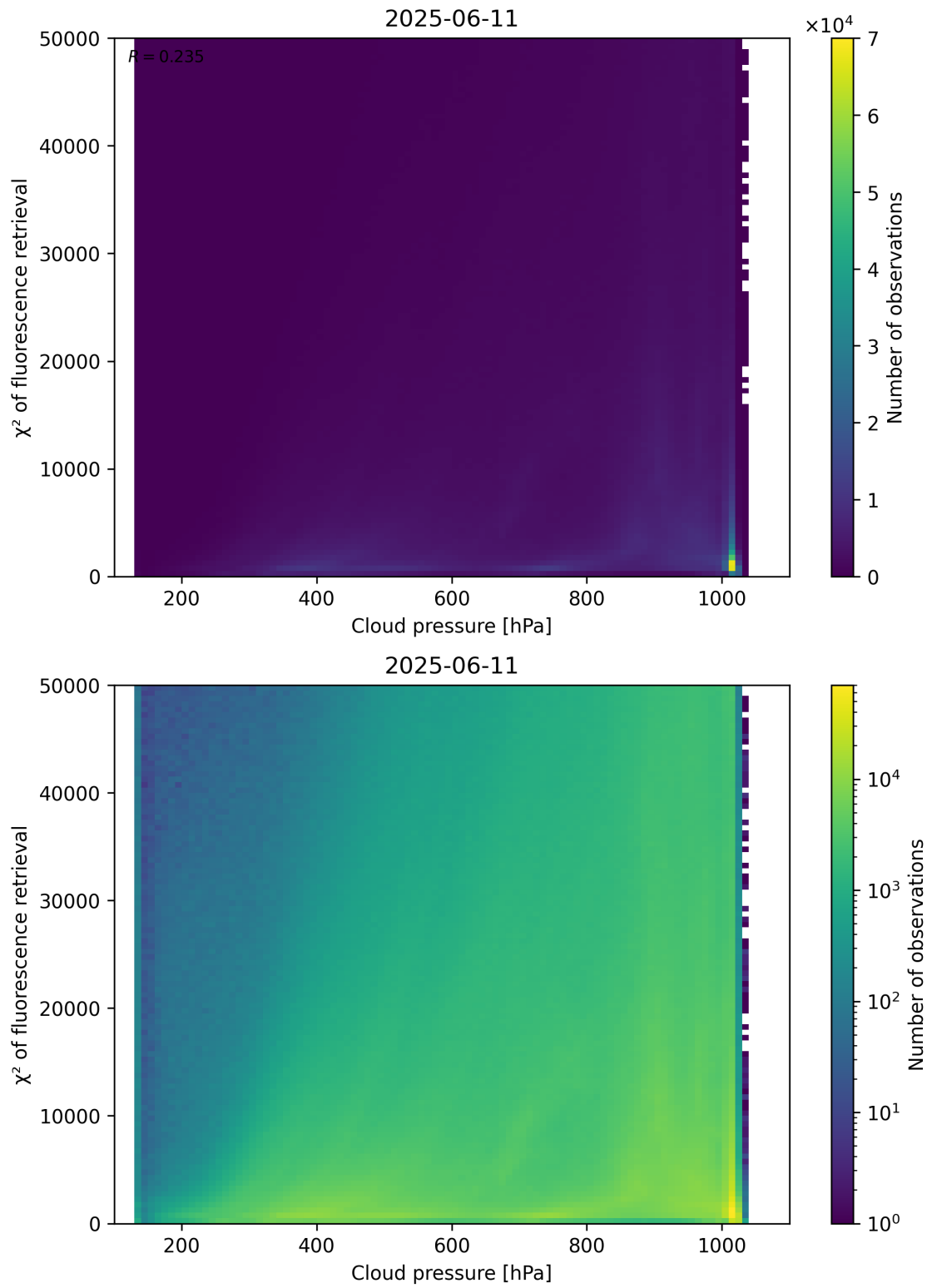
Figure 78: Scatter density plot of “Cloud pressure” against “ \chi^2 of fluorescence retrieval” for 2025-06-11 to 2025-06-12.
