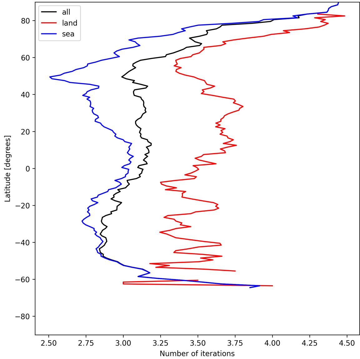
Figure 22: Zonal average of “Number of iterations” for 2025-06-11 to 2025-06-12.
