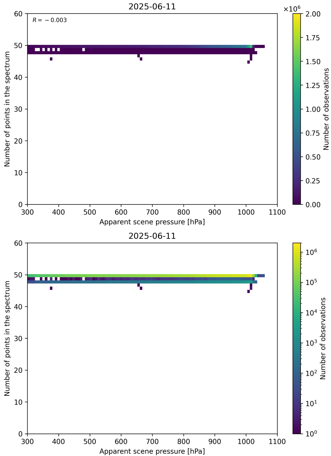
Figure 66: Scatter density plot of “Apparent scene pressure” against “Number of points in the spectrum” for 2025-06-11 to 2025-06-12.
