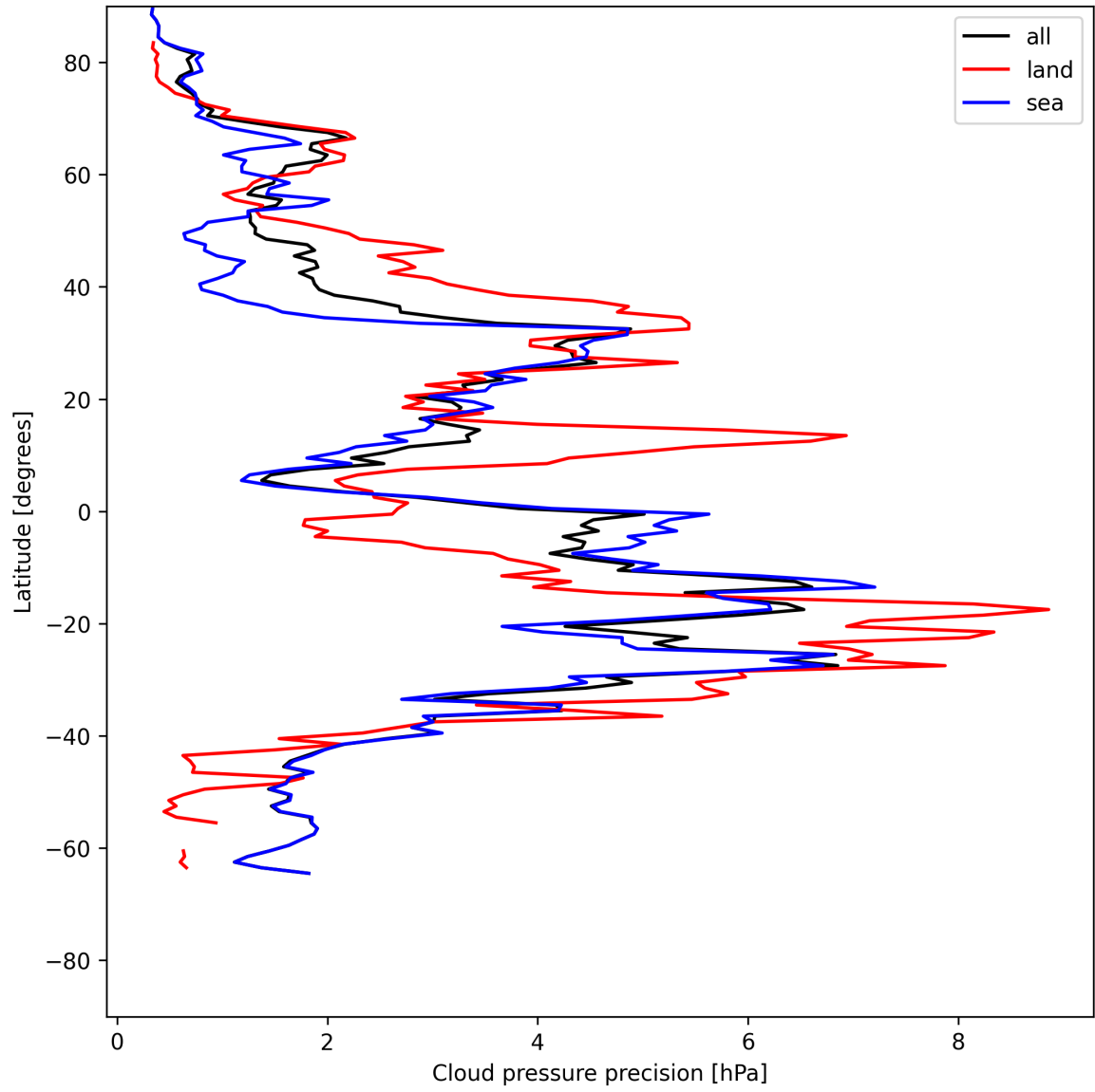
Figure 14: Zonal average of “Cloud pressure precision” for 2025-06-11 to 2025-06-12.
