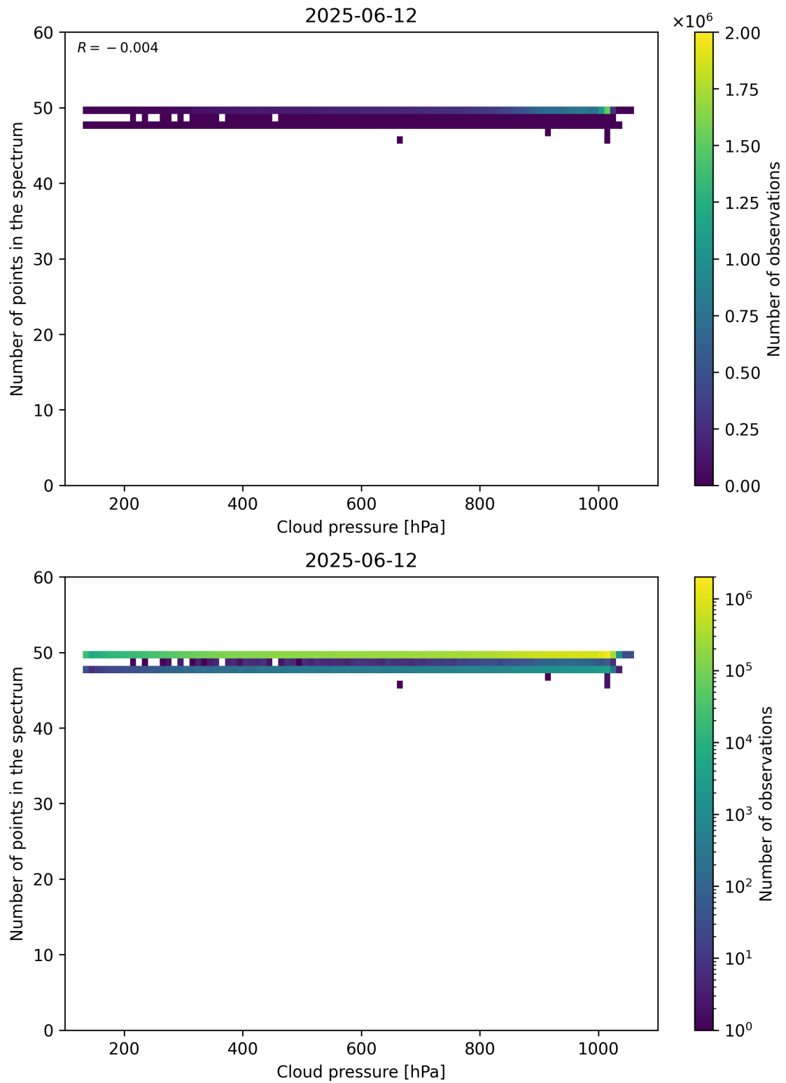
Figure 82: Scatter density plot of “Cloud pressure” against “Number of points in the spectrum” for 2025-06-11 to 2025-06-13.
