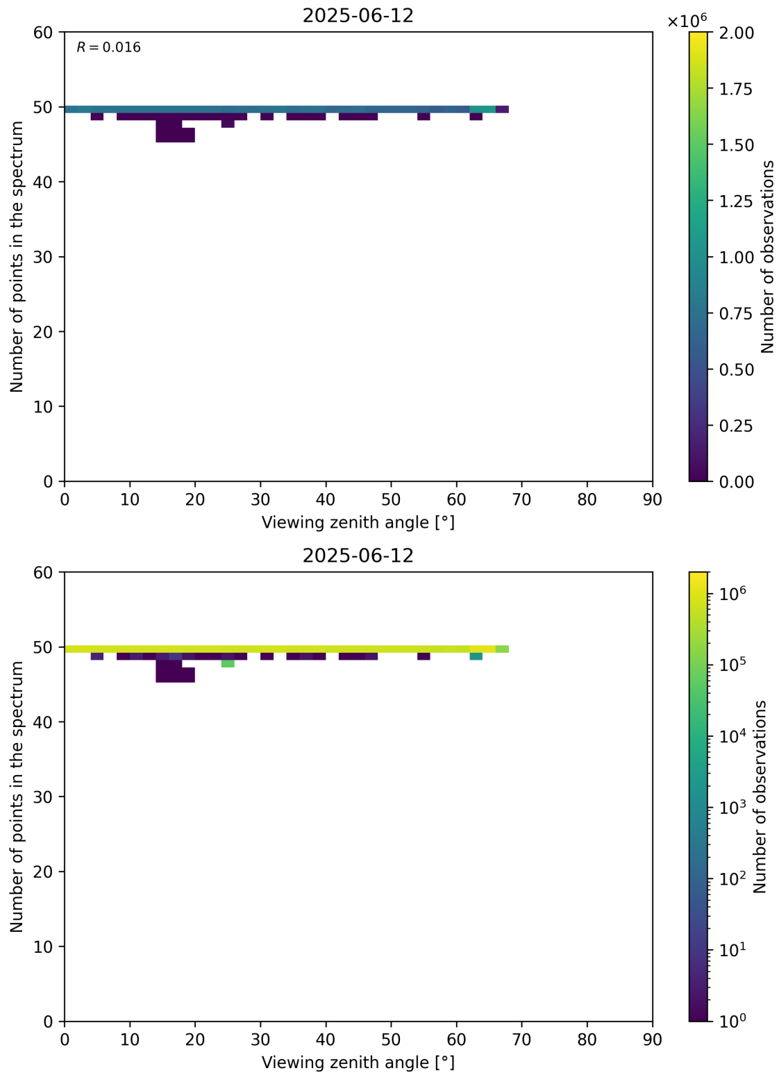
Figure 125: Scatter density plot of “Viewing zenith angle” against “Number of points in the spectrum” for 2025-06-11 to 2025-06-13.
