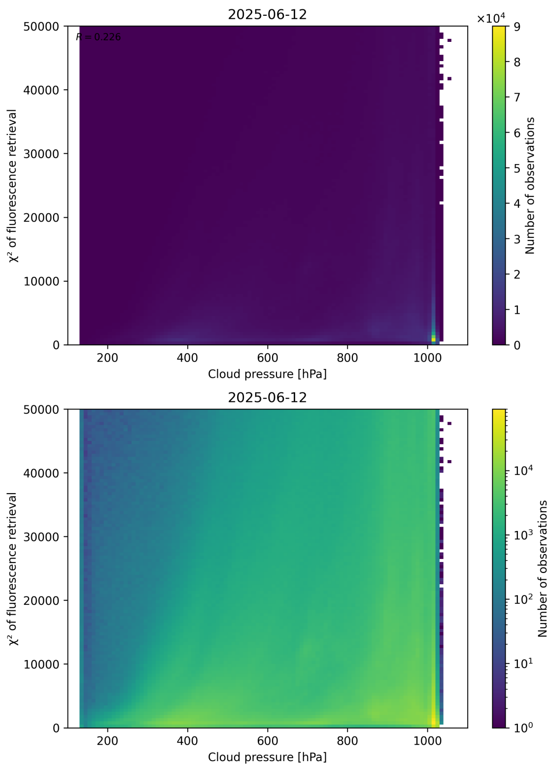
Figure 78: Scatter density plot of “Cloud pressure” against “ \chi^2 of fluorescence retrieval” for 2025-06-11 to 2025-06-13.
