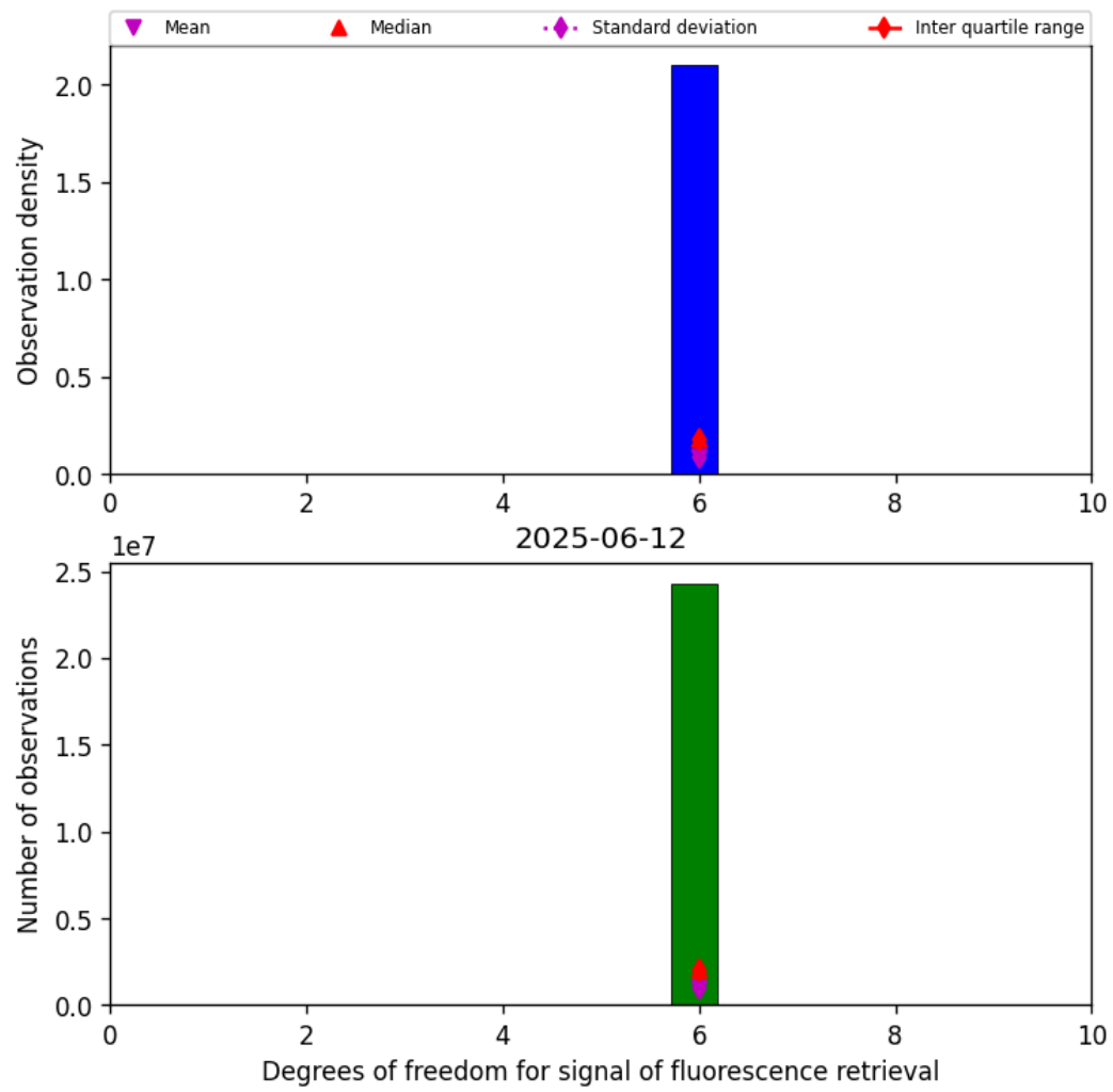
Figure 43: Histogram of “Degrees of freedom for signal of fluorescence retrieval” for 2025-06-11 to 2025-06-13
