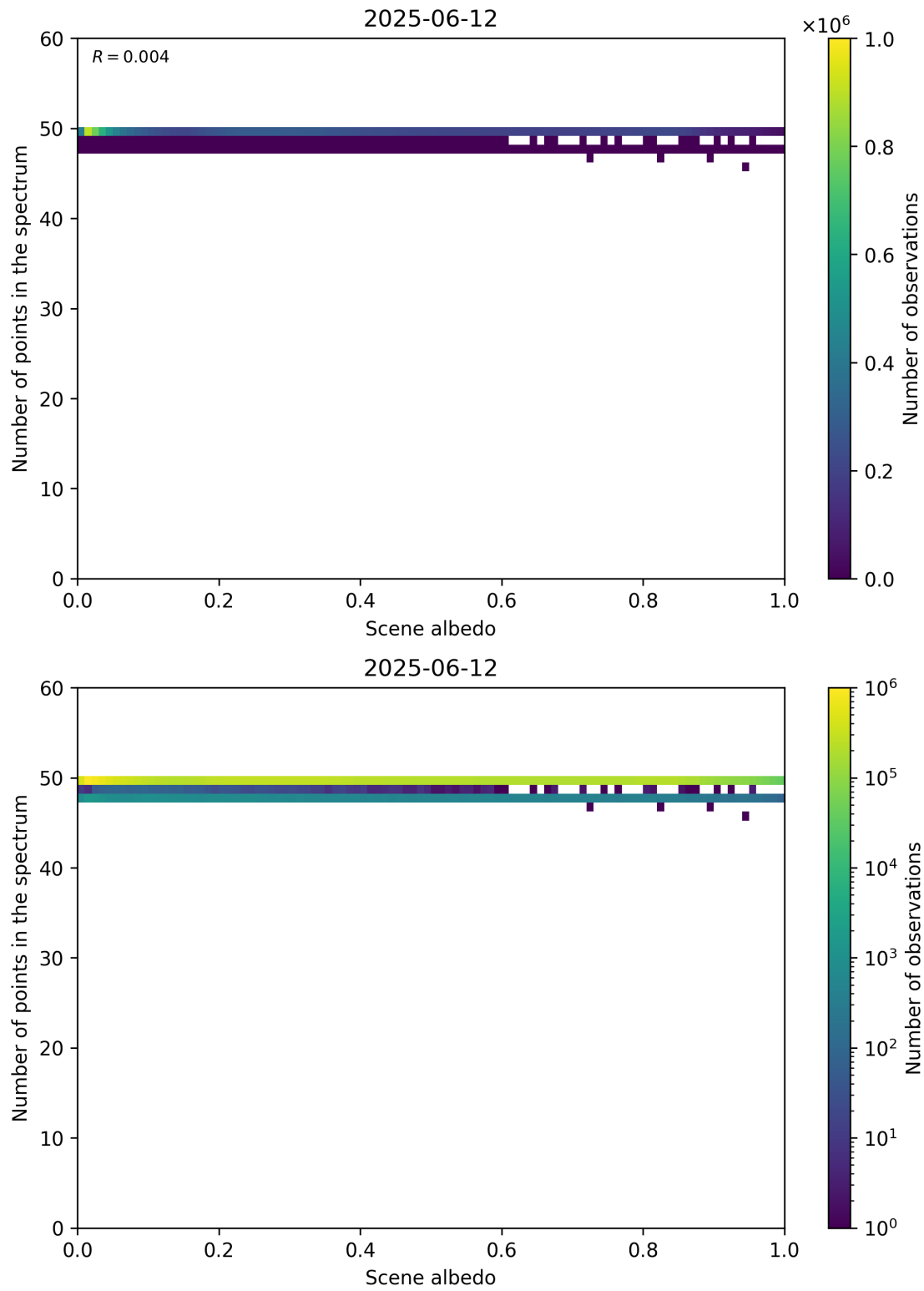
Figure 106: Scatter density plot of “Scene albedo” against “Number of points in the spectrum” for 2025-06-11 to 2025-06-13.
