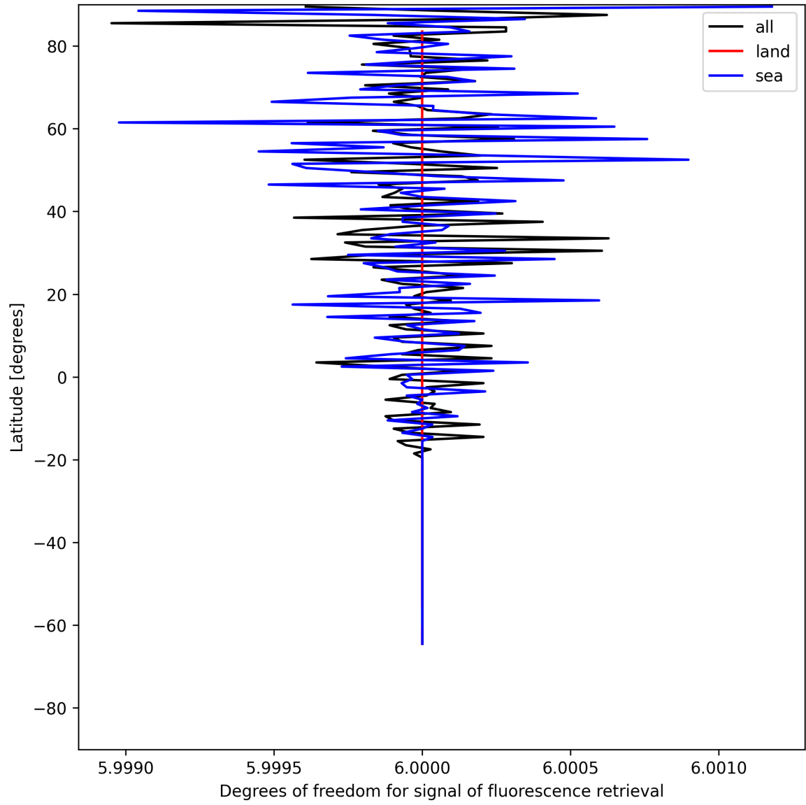
Figure 26: Zonal average of “Degrees of freedom for signal of fluorescence retrieval” for 2025-06-11 to 2025-06-13.
