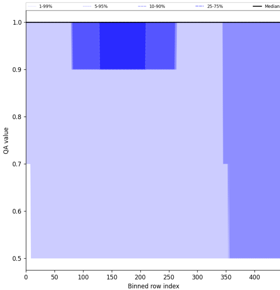
Figure 46: Along track statistics of “QA value” for 2025-06-11 to 2025-06-13
