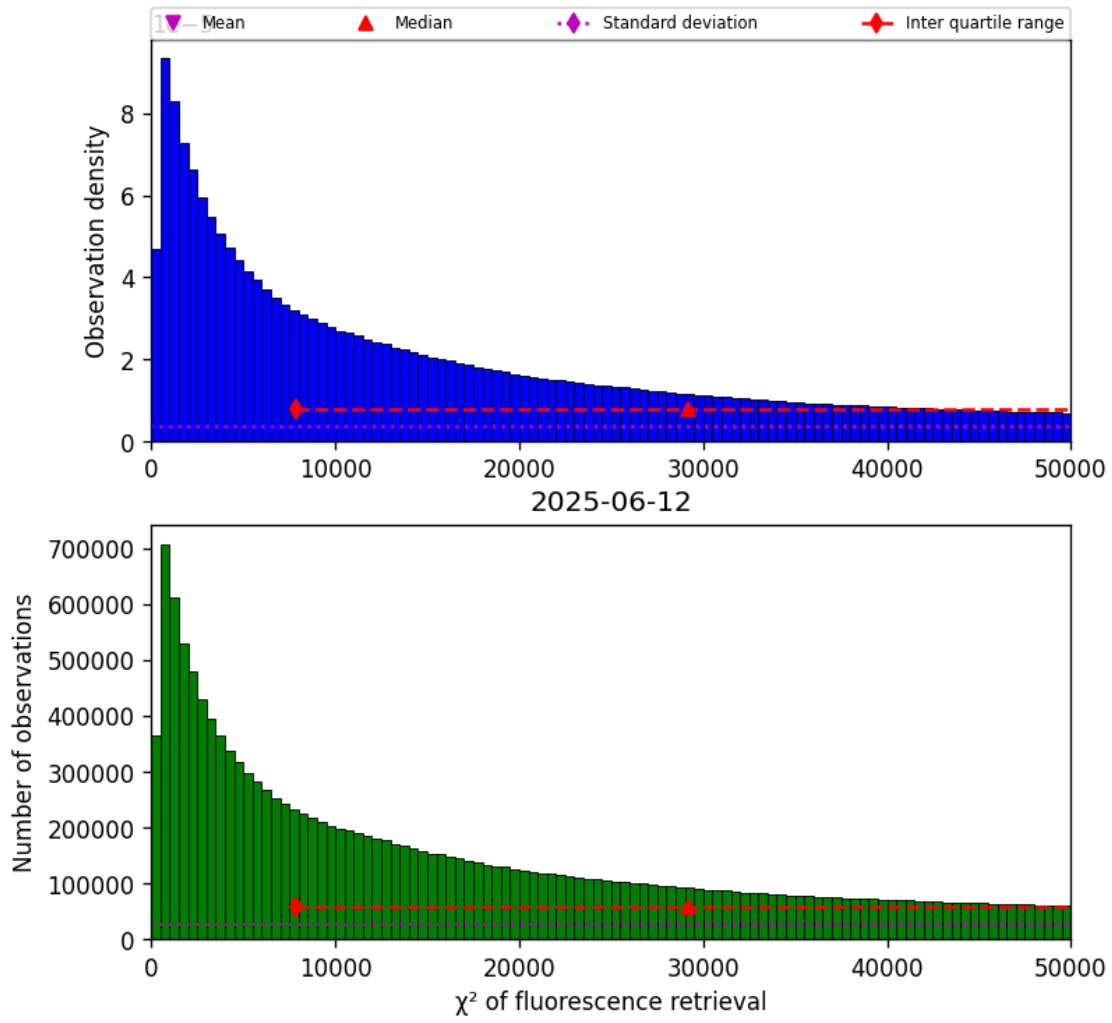
Figure 42: Histogram of “ \chi^2 of fluorescence retrieval” for 2025-06-11 to 2025-06-13
