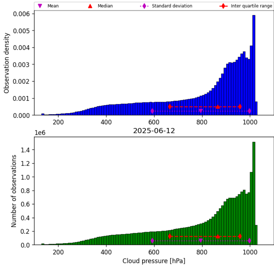
Figure 30: Histogram of “Cloud pressure” for 2025-06-11 to 2025-06-13
