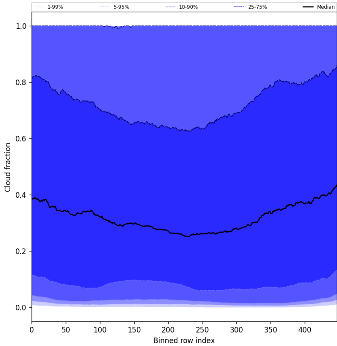
Figure 49: Along track statistics of “Cloud fraction” for 2025-06-11 to 2025-06-13
