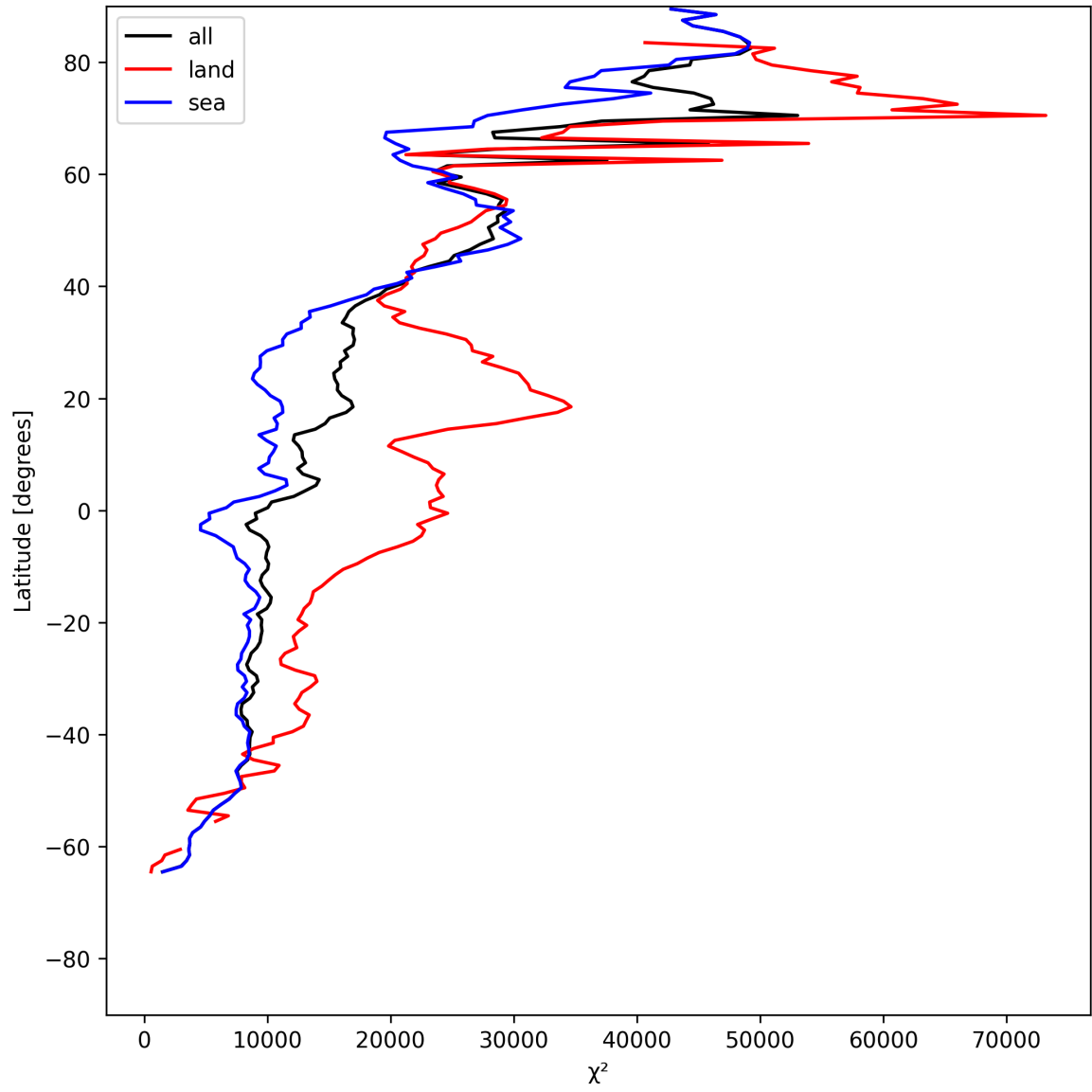
Figure 21: Zonal average of “ \chi^2 ” for 2025-06-11 to 2025-06-13.
