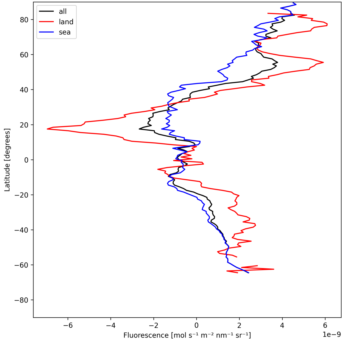
Figure 23: Zonal average of “Fluorescence” for 2025-06-11 to 2025-06-13.
