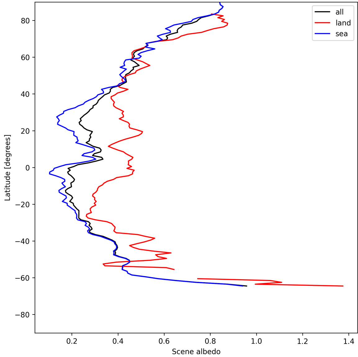
Figure 17: Zonal average of “Scene albedo” for 2025-06-11 to 2025-06-13.
