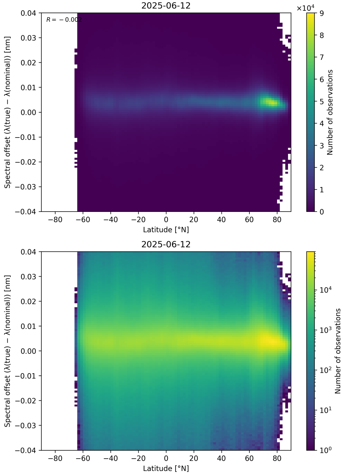
Figure 96: Scatter density plot of “Latitude” against “Spectral offset ( \lambda_{\text{true}} - \lambda_{\text{nominal}} )” for 2025-06-11 to 2025-06-13.
