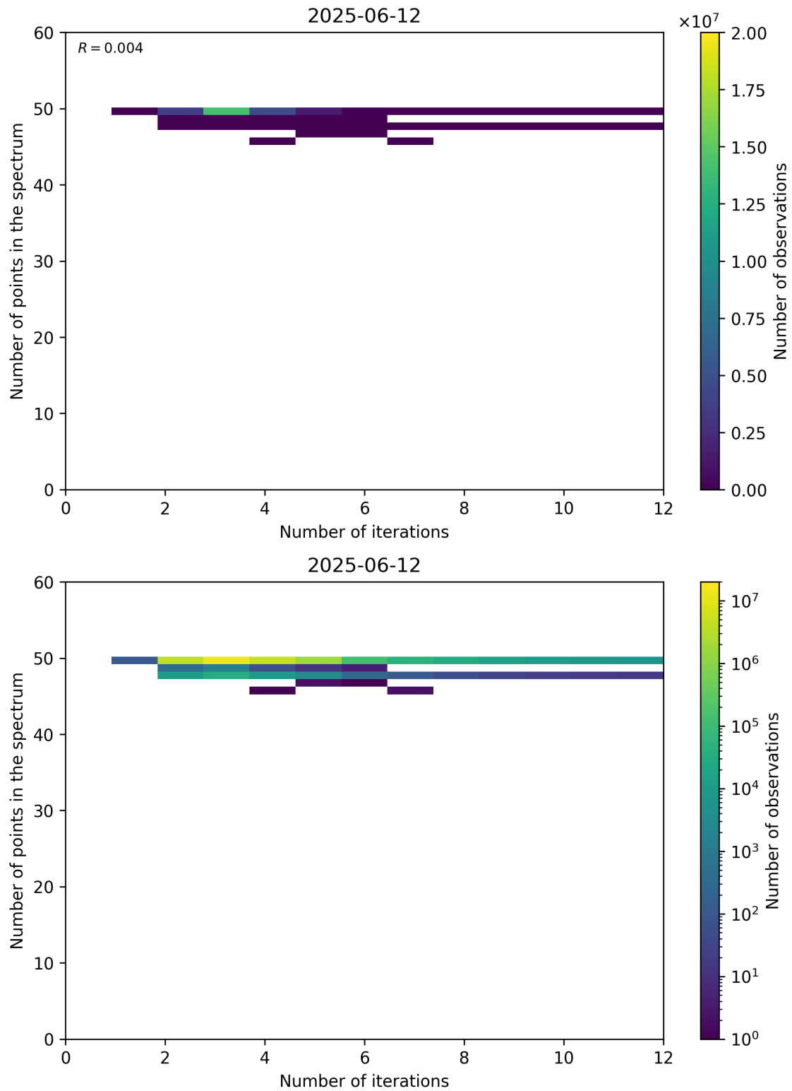
Figure 99: Scatter density plot of “Number of iterations” against “Number of points in the spectrum” for 2025-06-11 to 2025-06-13.
