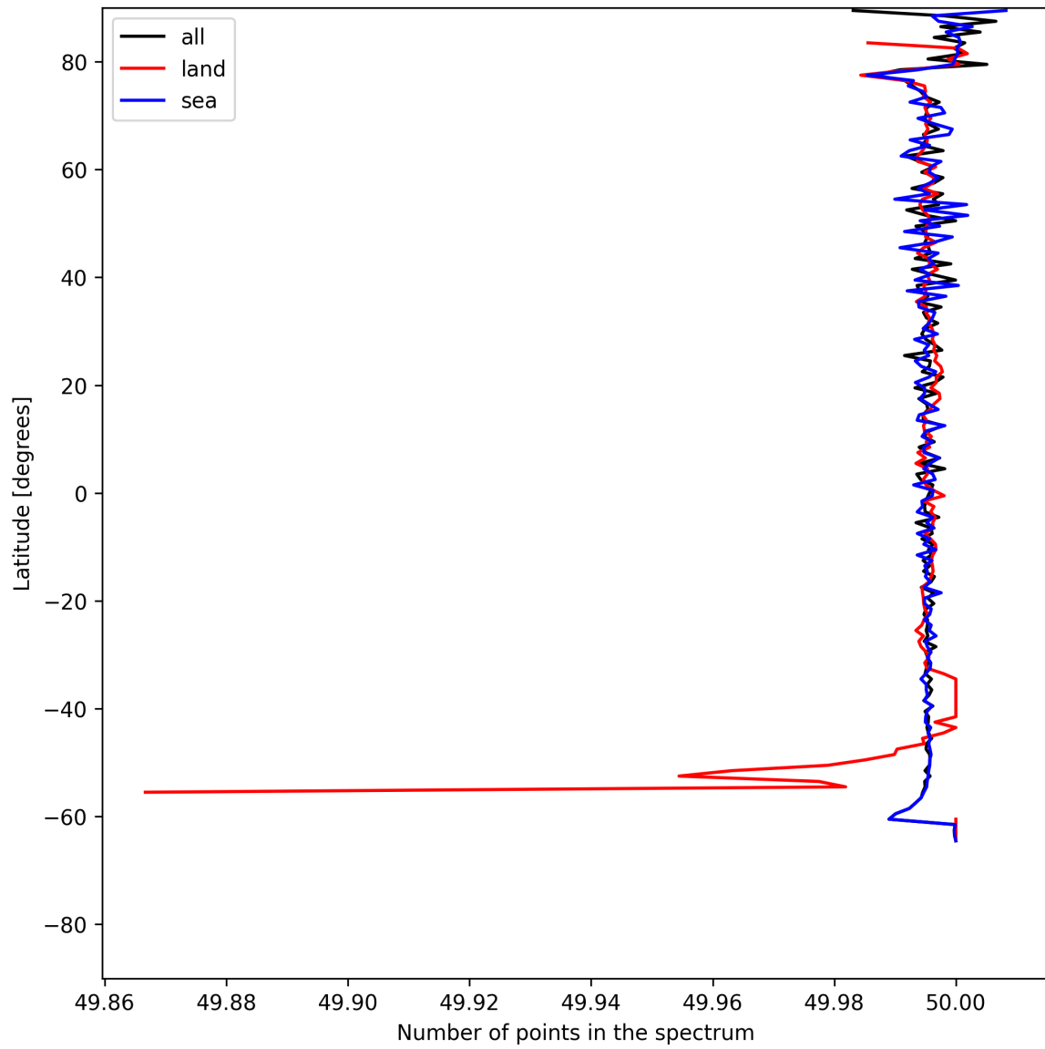
Figure 27: Zonal average of “Number of points in the spectrum” for 2025-06-11 to 2025-06-13.
