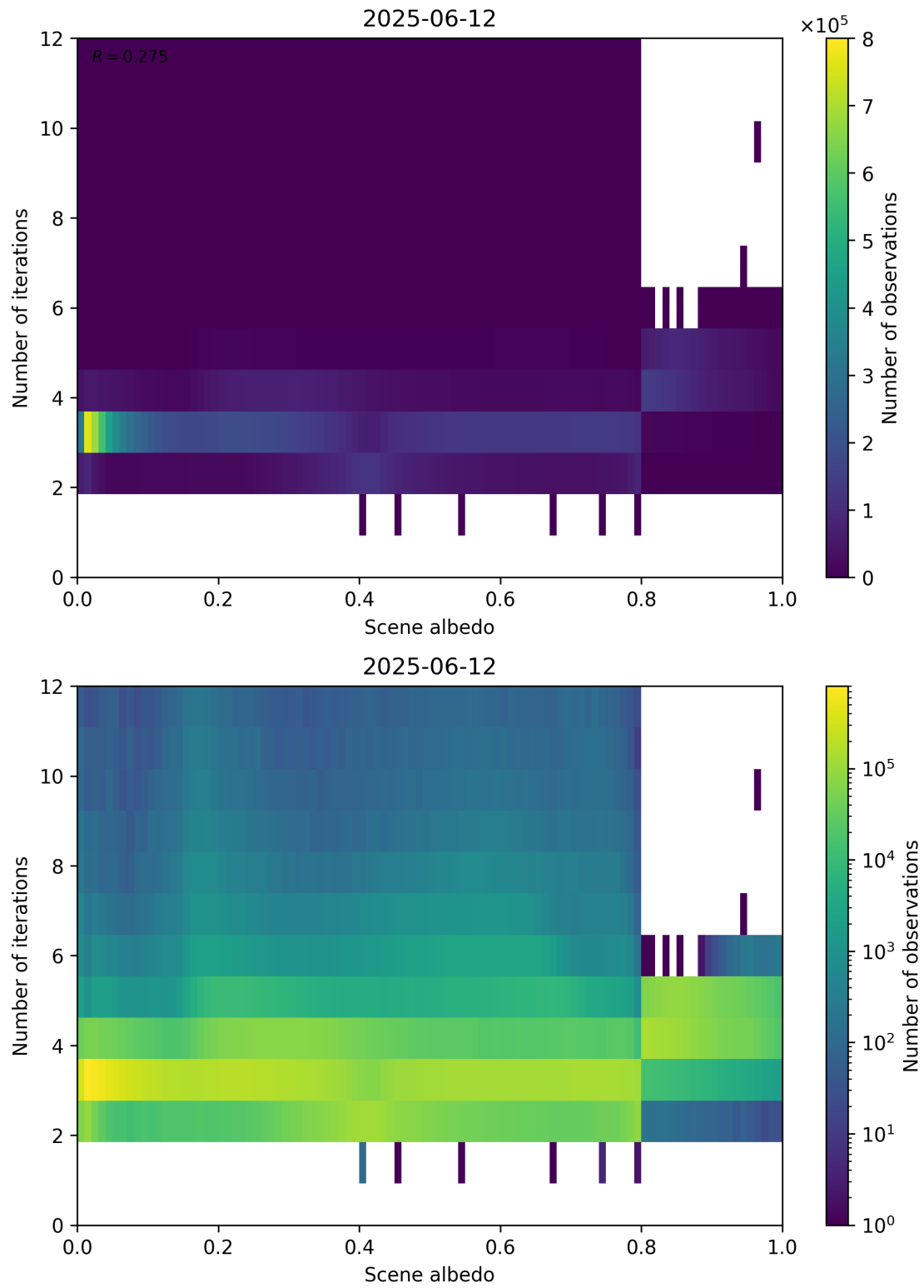
Figure 105: Scatter density plot of “Scene albedo” against “Number of iterations” for 2025-06-11 to 2025-06-13.
