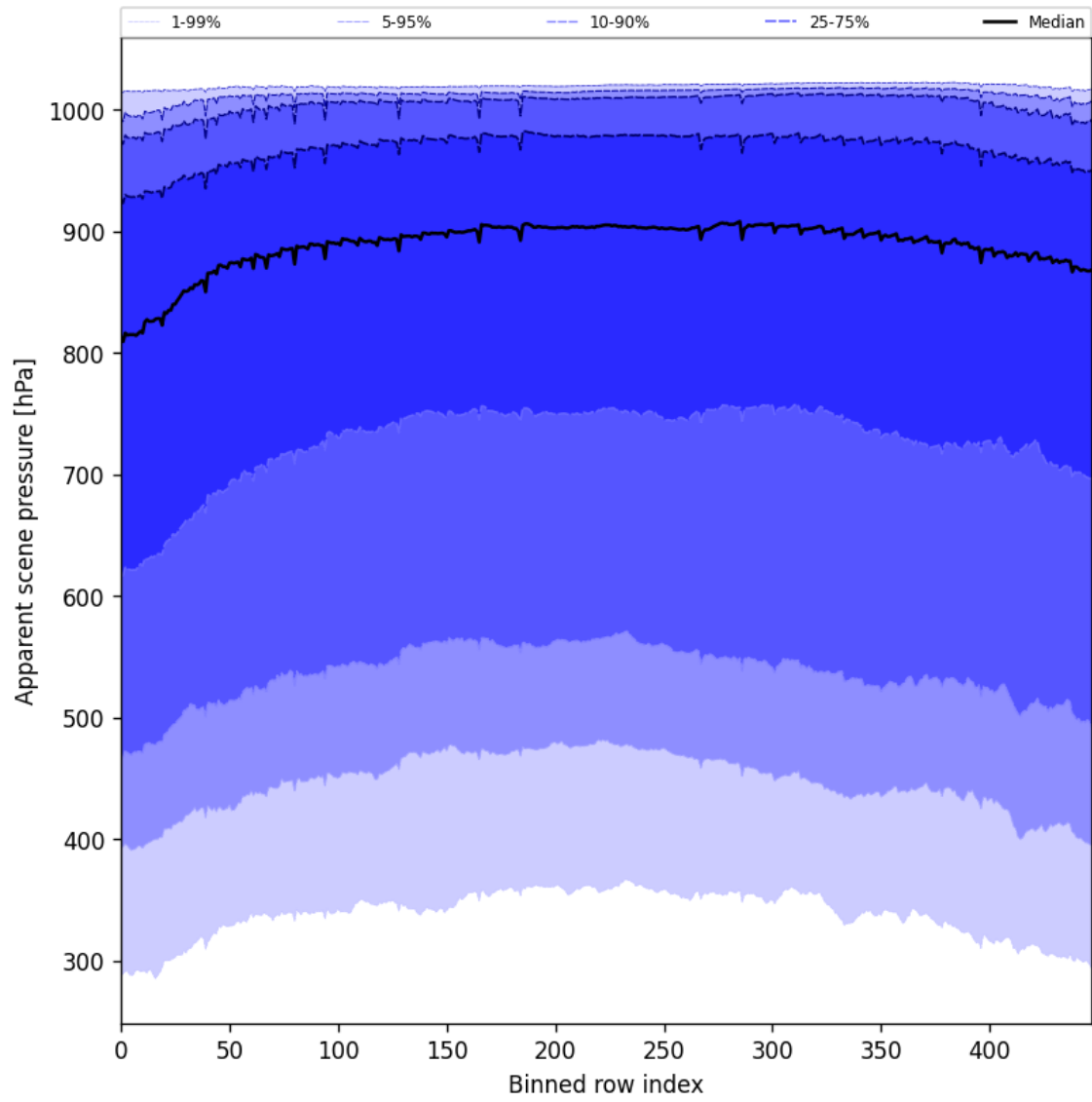
Figure 53: Along track statistics of “Apparent scene pressure” for 2025-06-11 to 2025-06-13
