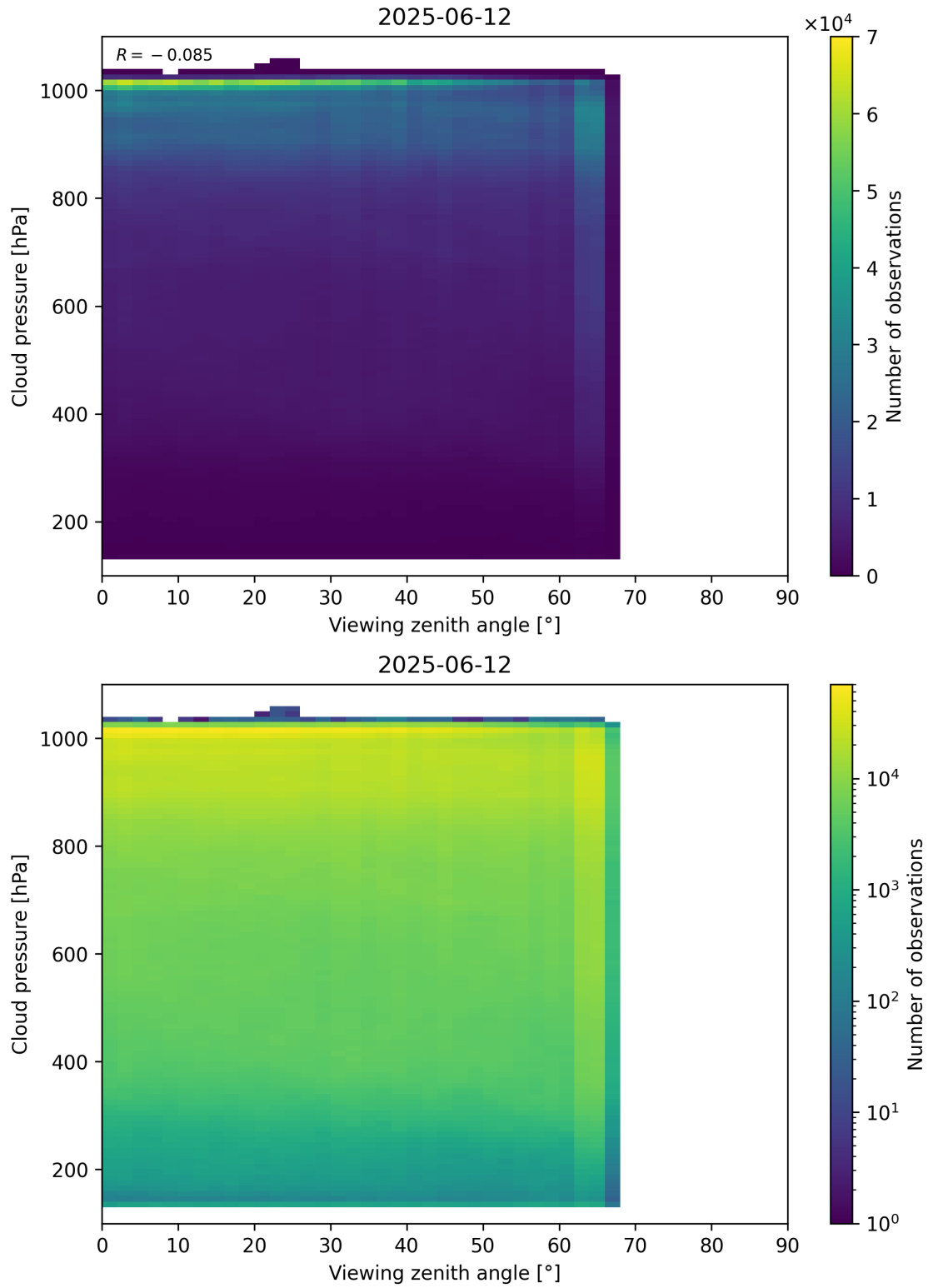
Figure 121: Scatter density plot of “Viewing zenith angle” against “Cloud pressure” for 2025-06-11 to 2025-06-13.
