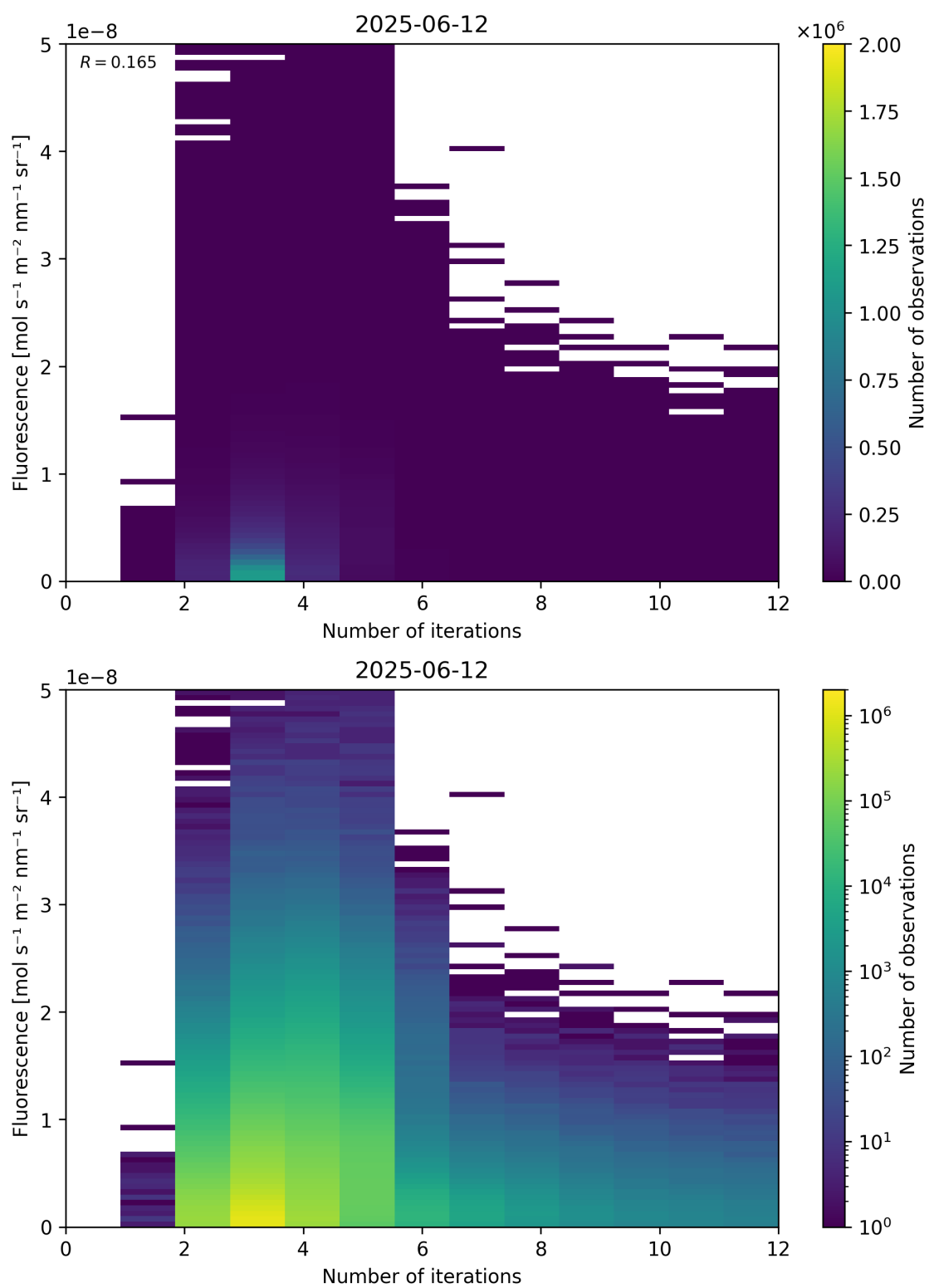
Figure 98: Scatter density plot of “Number of iterations” against “Fluorescence” for 2025-06-11 to 2025-06-13.
