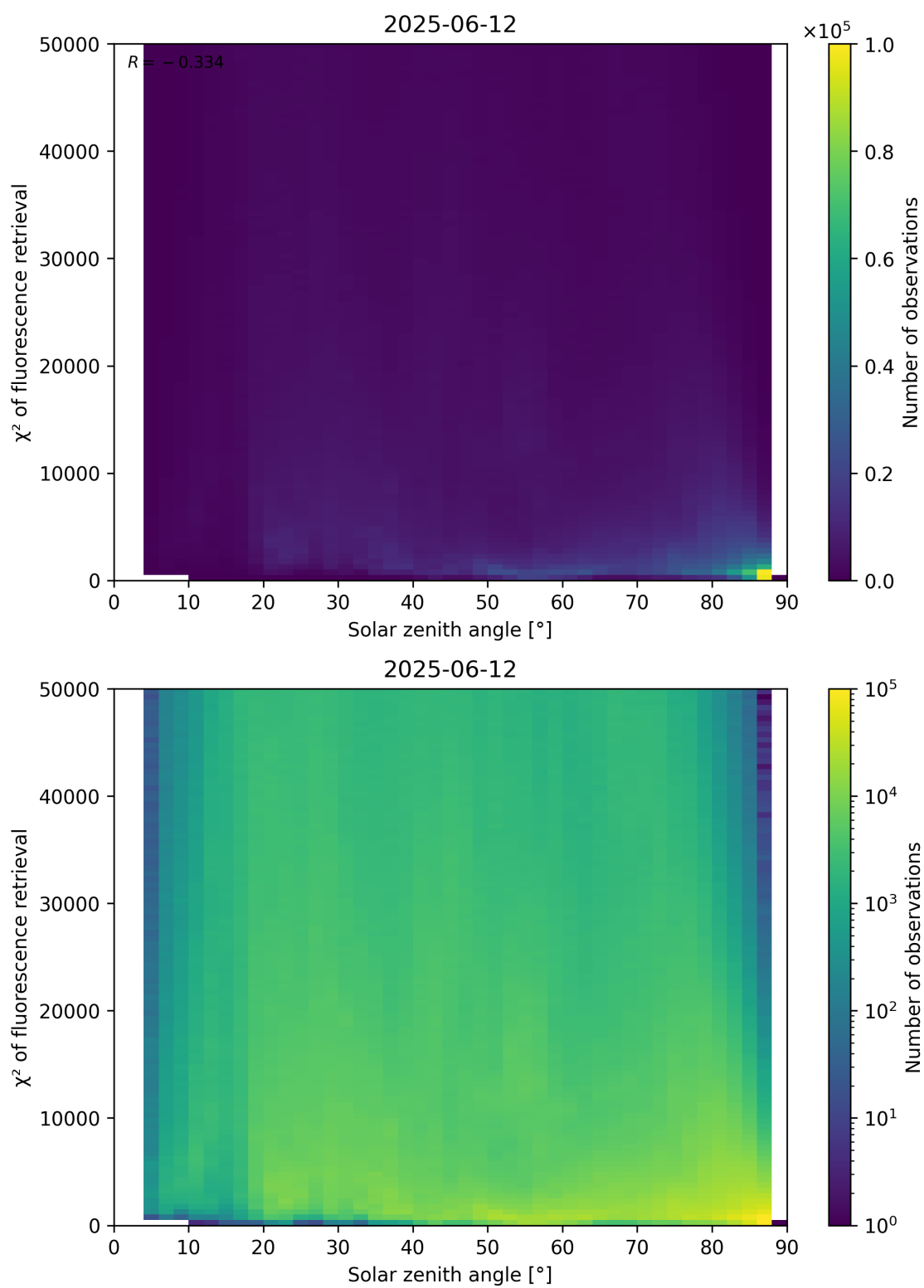
Figure 109: Scatter density plot of “Solar zenith angle” against “ \chi^2 of fluorescence retrieval” for 2025-06-11 to 2025-06-13.
