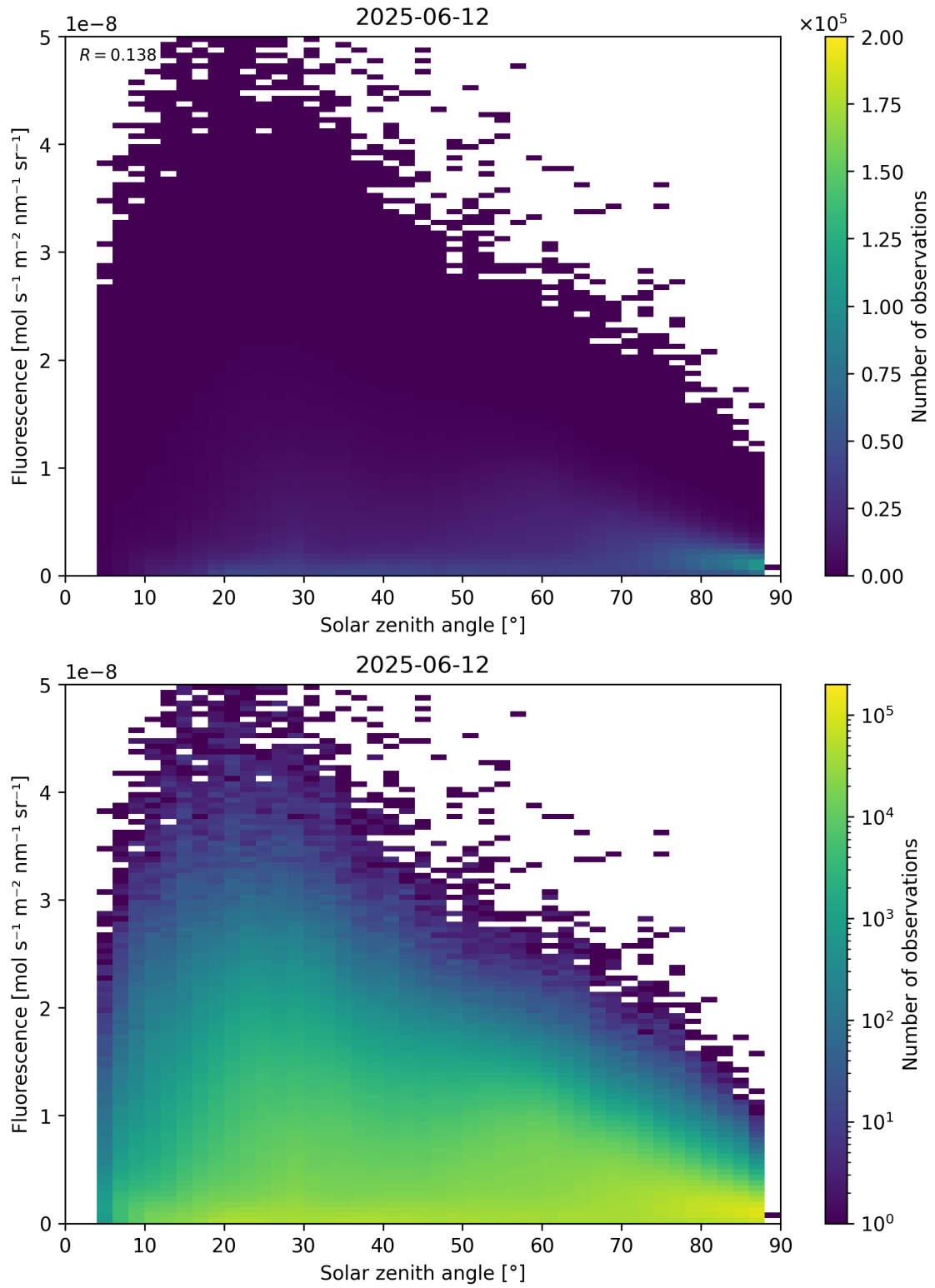
Figure 112: Scatter density plot of “Solar zenith angle” against “Fluorescence” for 2025-06-11 to 2025-06-13.
