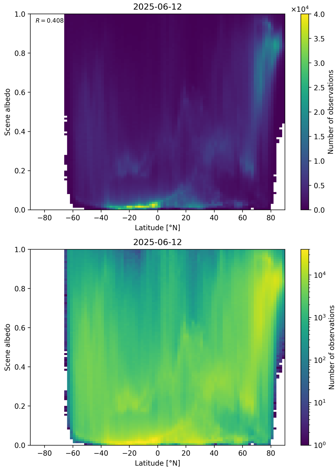
Figure 95: Scatter density plot of “Latitude” against “Scene albedo” for 2025-06-11 to 2025-06-13.
