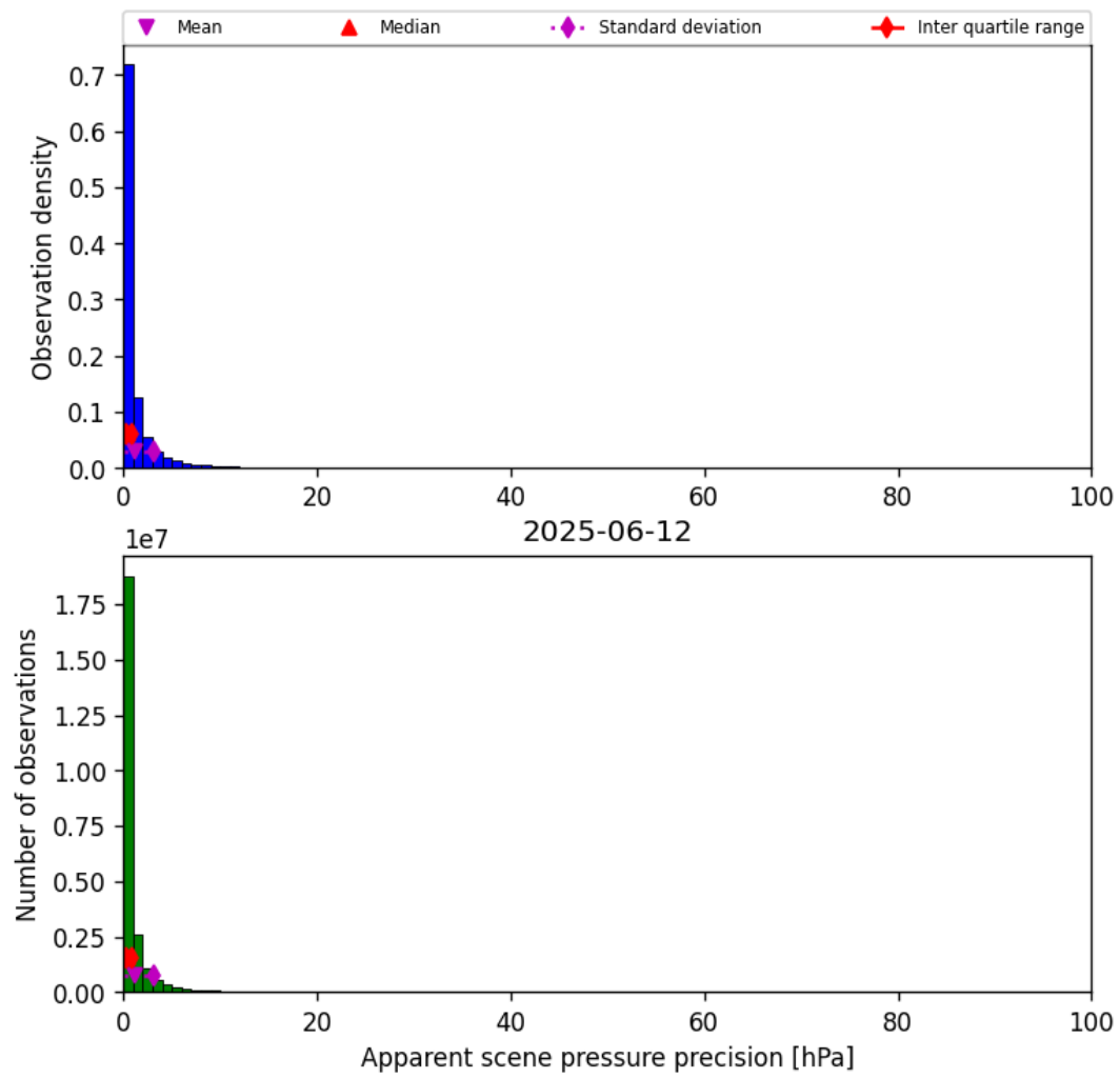
Figure 37: Histogram of “Apparent scene pressure precision” for 2025-06-11 to 2025-06-13
