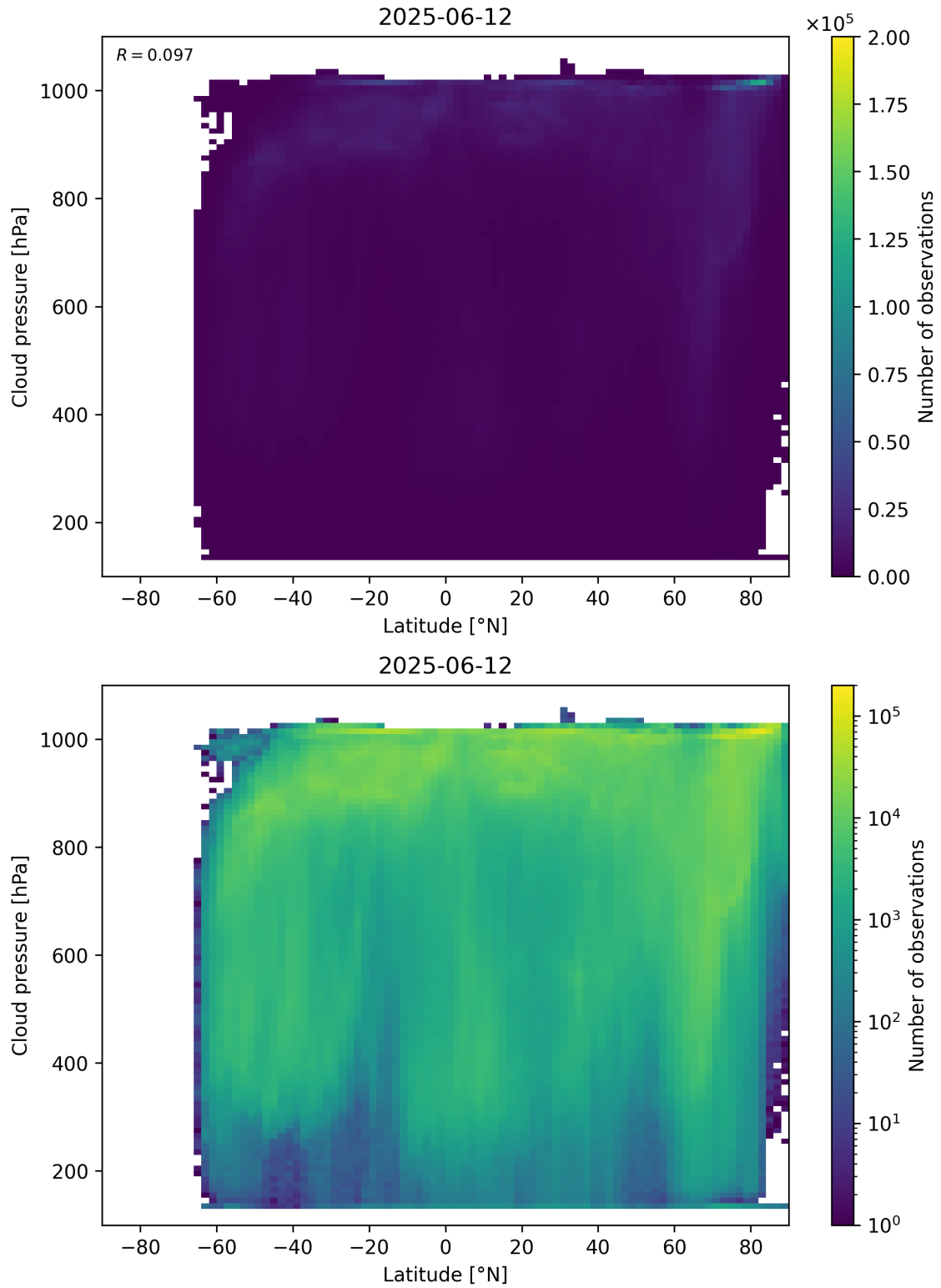
Figure 91: Scatter density plot of “Latitude” against “Cloud pressure” for 2025-06-11 to 2025-06-13.
