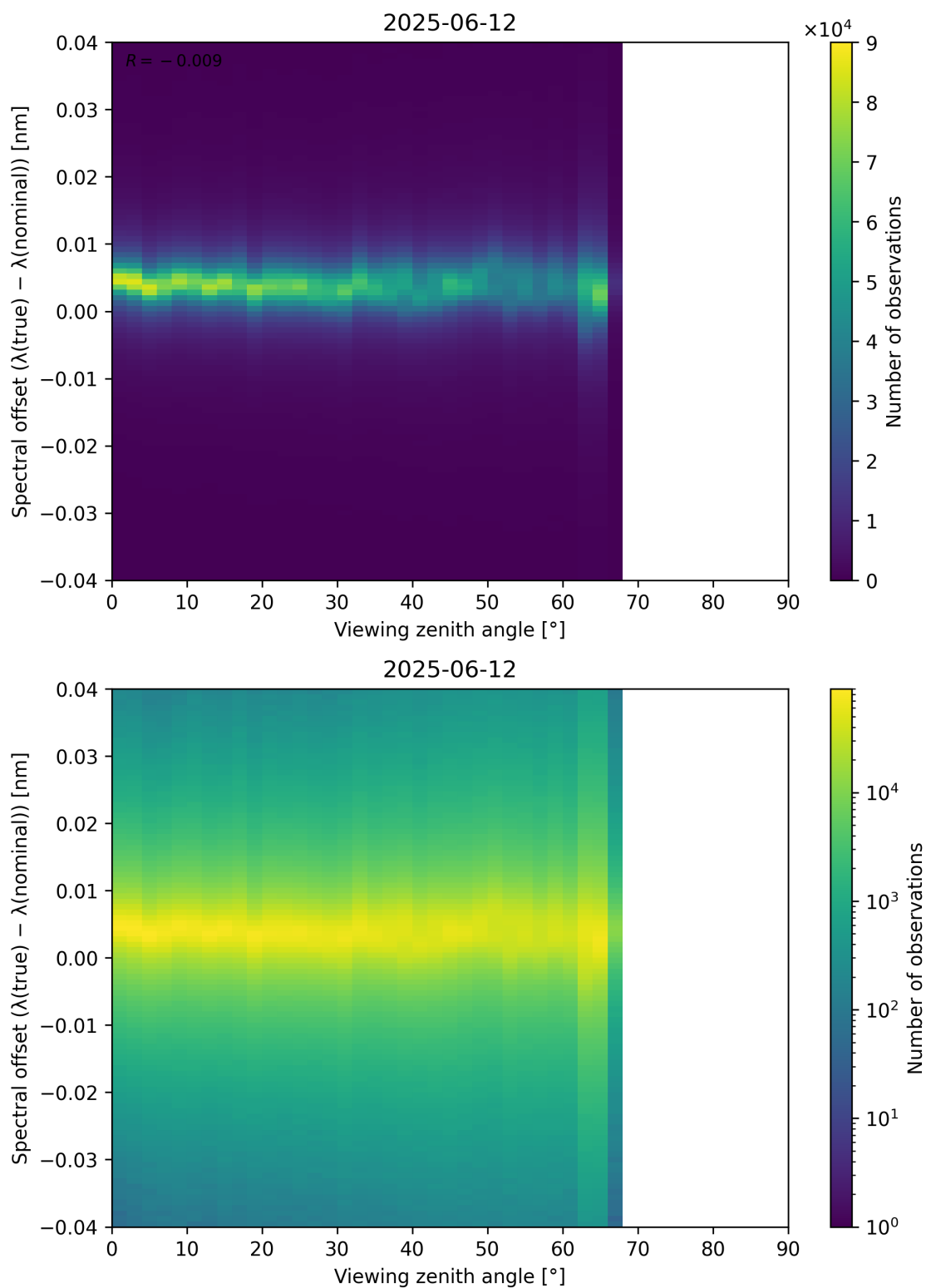
Figure 128: Scatter density plot of “Viewing zenith angle” against “Spectral offset ( \lambda_{\text{true}} - \lambda_{\text{nominal}} )” for 2025-06-11 to 2025-06-13.
