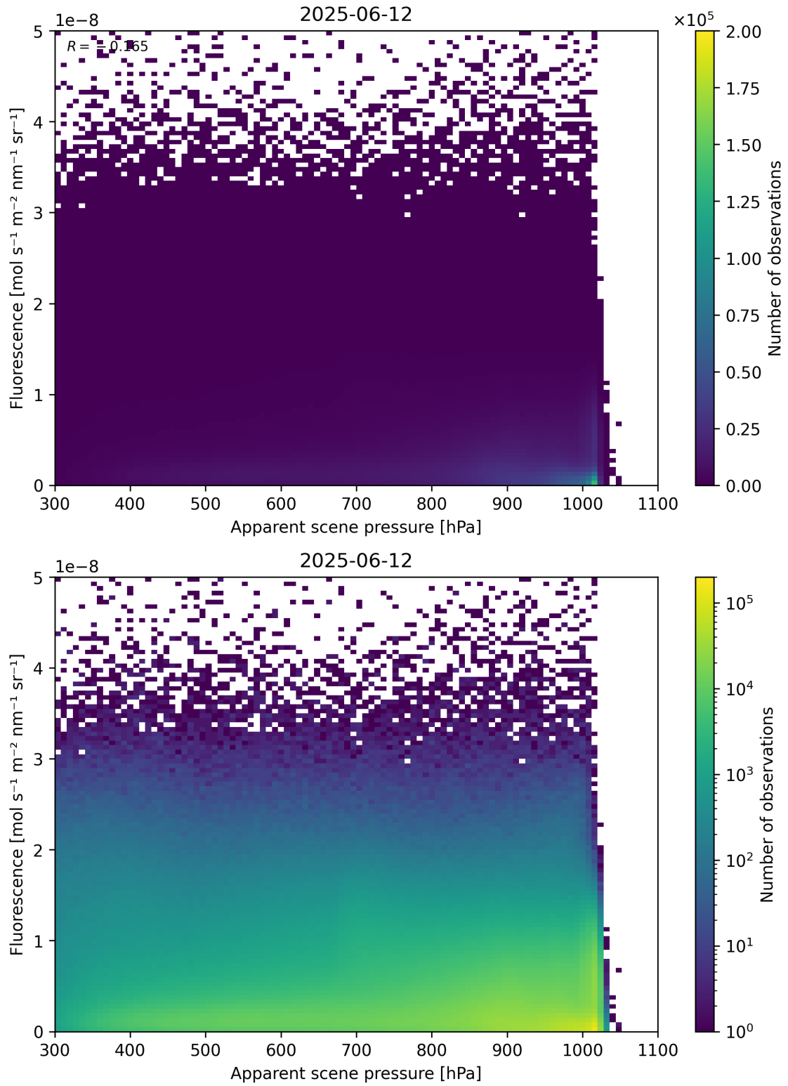
Figure 64: Scatter density plot of “Apparent scene pressure” against “Fluorescence” for 2025-06-11 to 2025-06-13.
