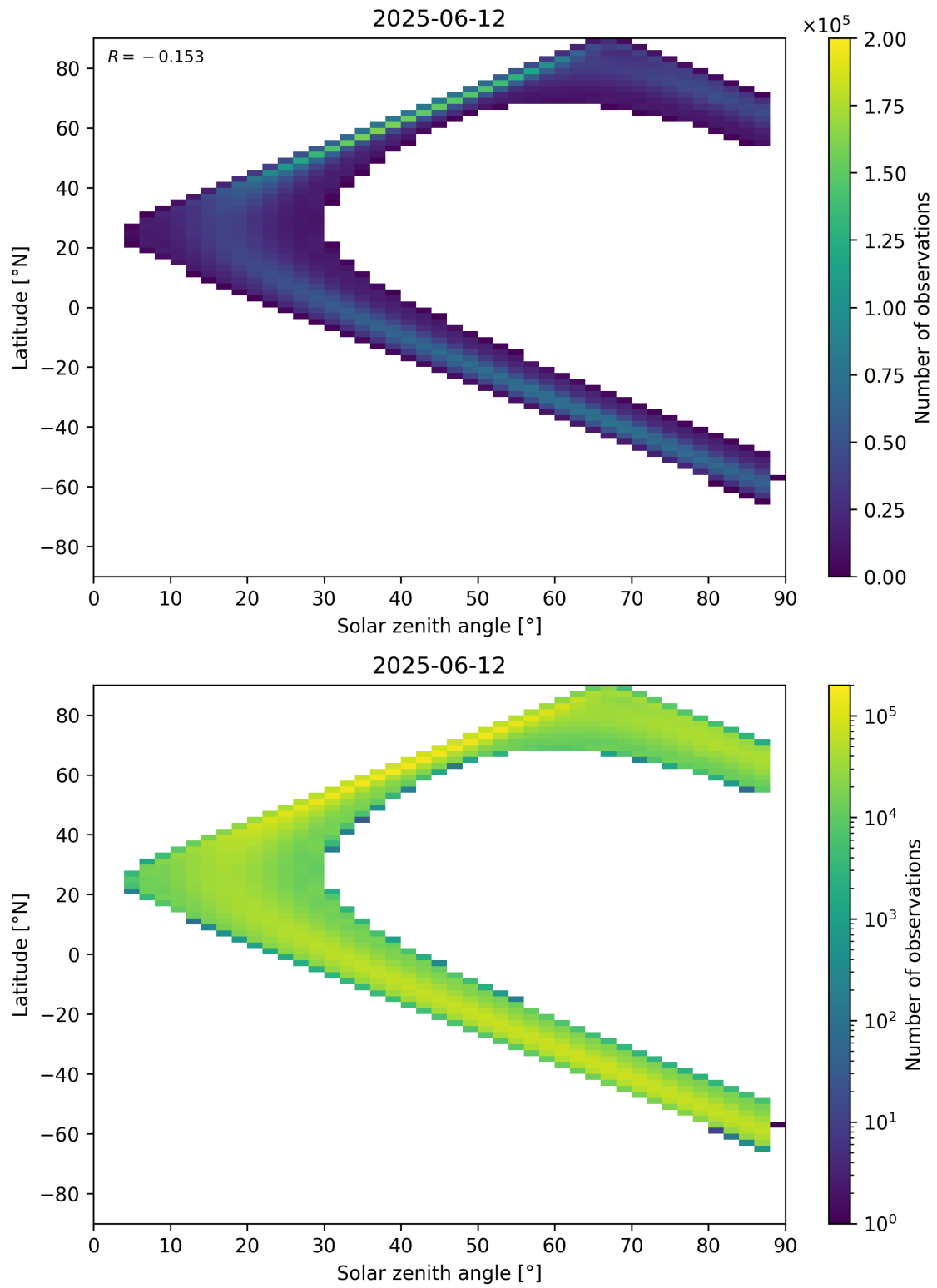
Figure 113: Scatter density plot of “Solar zenith angle” against “Latitude” for 2025-06-11 to 2025-06-13.
