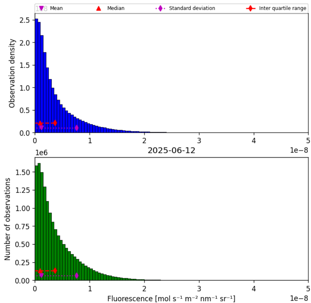
Figure 40: Histogram of “Fluorescence” for 2025-06-11 to 2025-06-13
