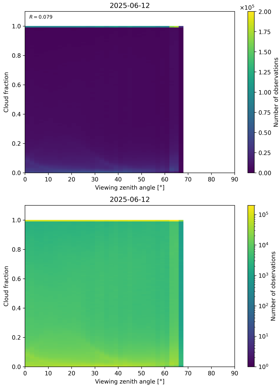
Figure 120: Scatter density plot of “Viewing zenith angle” against “Cloud fraction” for 2025-06-11 to 2025-06-13.
