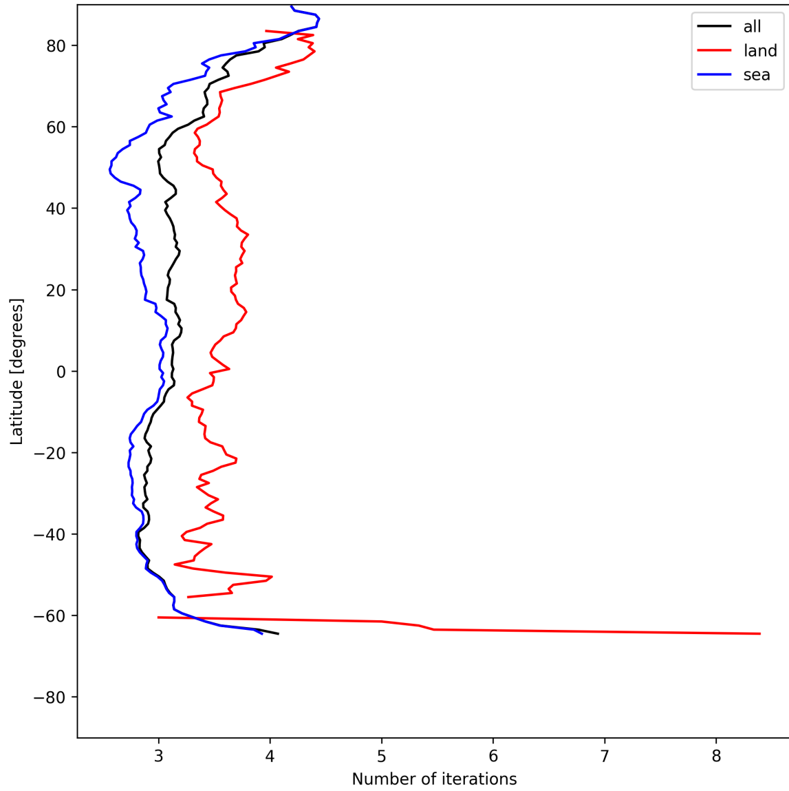
Figure 22: Zonal average of “Number of iterations” for 2025-06-11 to 2025-06-13.
