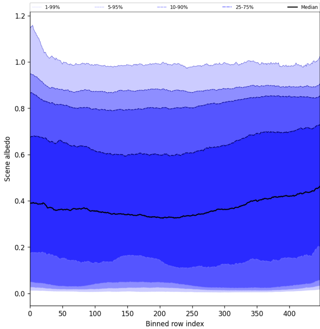
Figure 51: Along track statistics of “Scene albedo” for 2025-06-11 to 2025-06-13
