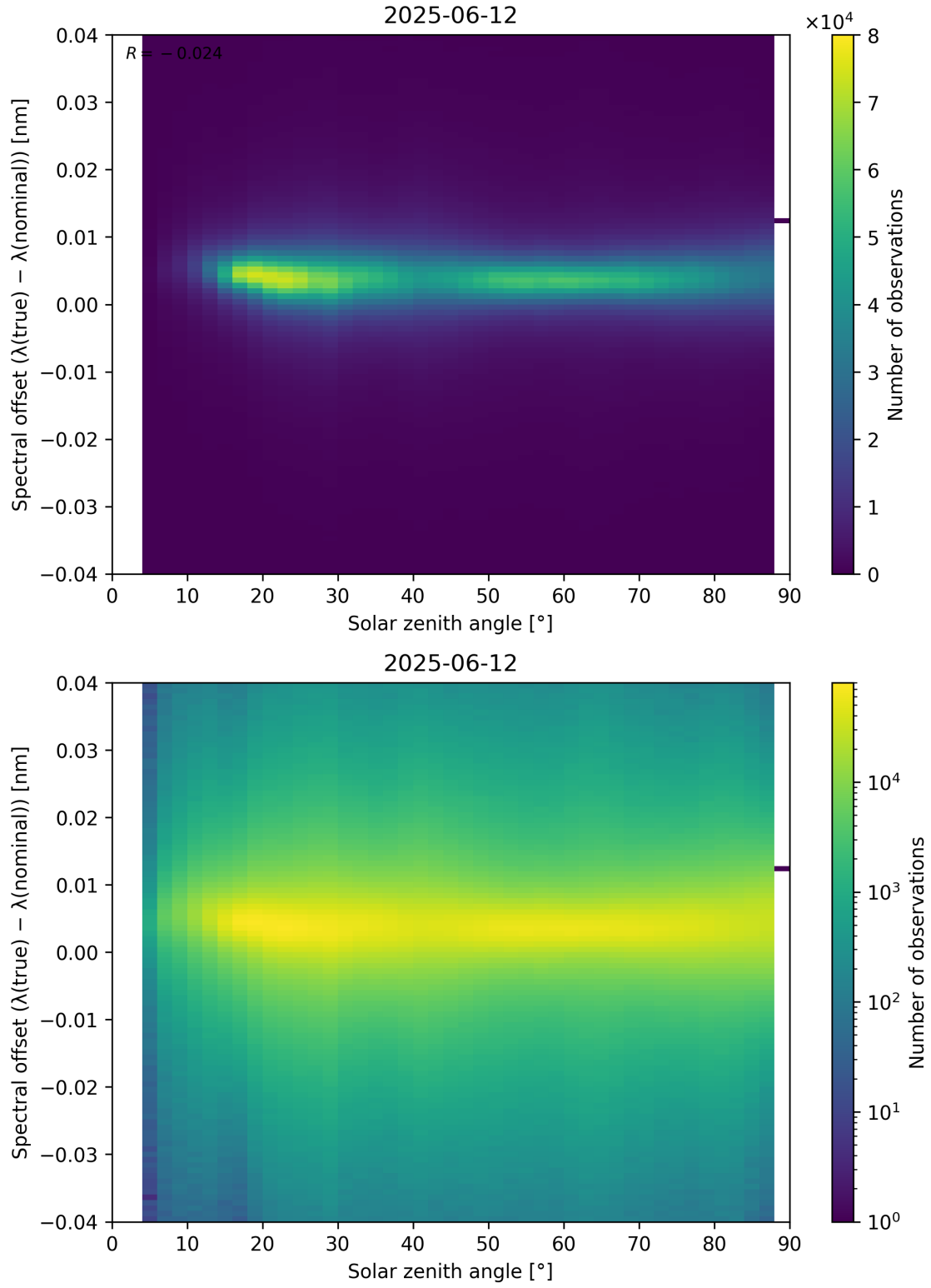
Figure 117: Scatter density plot of “Solar zenith angle” against “Spectral offset ( \lambda_{\text{true}} - \lambda_{\text{nominal}} )” for 2025-06-11 to 2025-06-13.
