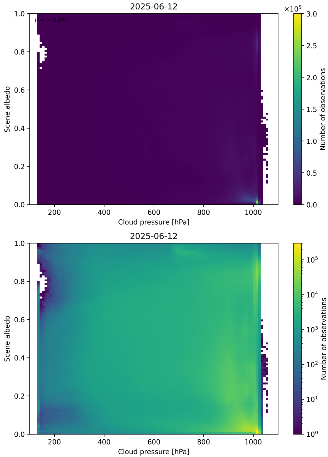
Figure 83: Scatter density plot of “Cloud pressure” against “Scene albedo” for 2025-06-11 to 2025-06-13.
