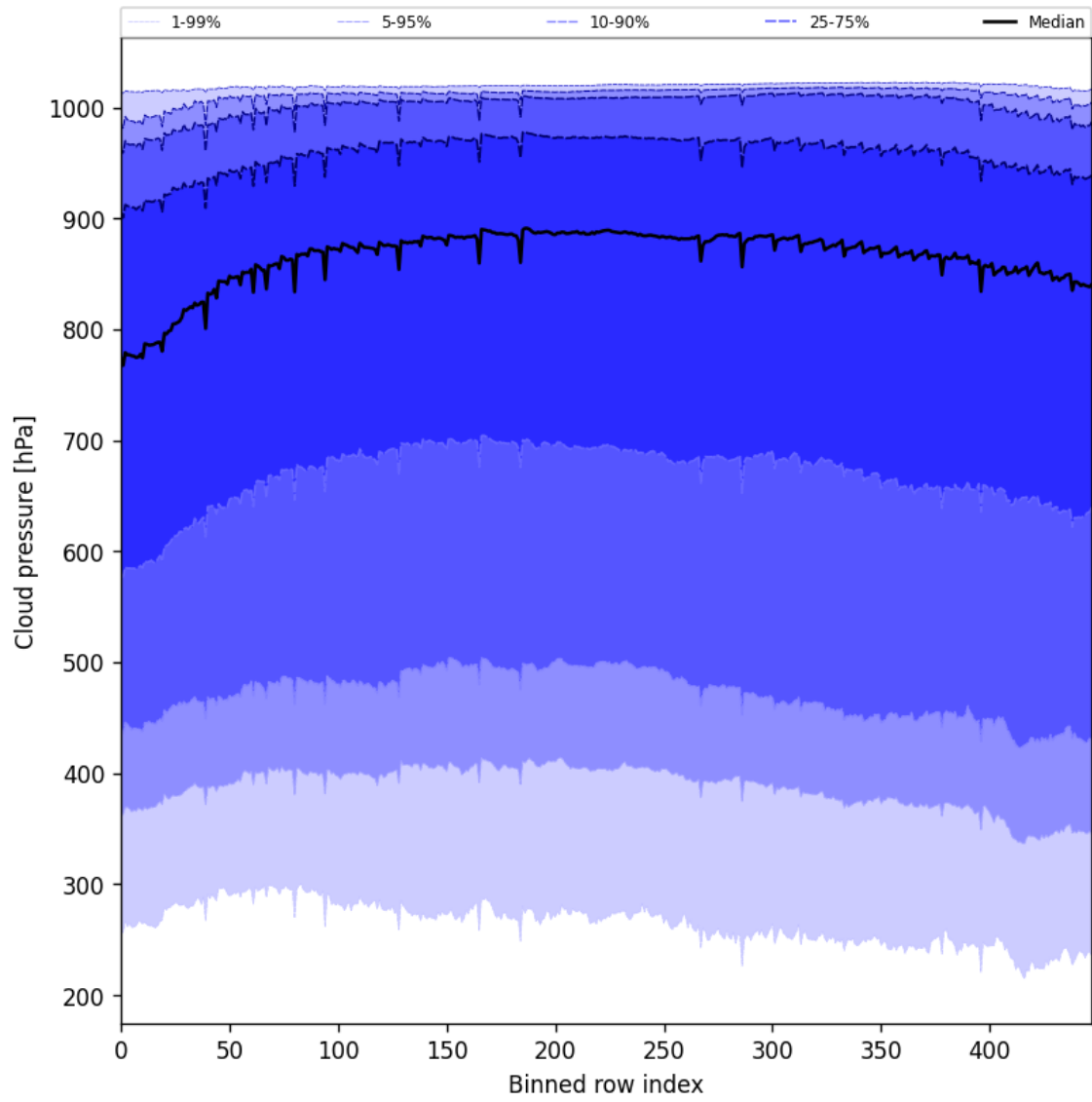
Figure 47: Along track statistics of “Cloud pressure” for 2025-06-11 to 2025-06-13
