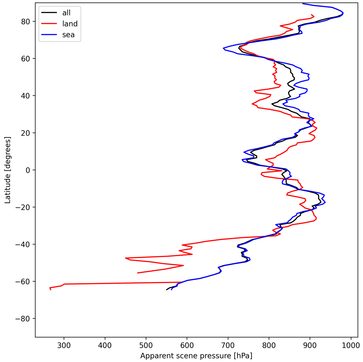
Figure 19: Zonal average of “Apparent scene pressure” for 2025-06-11 to 2025-06-13.
