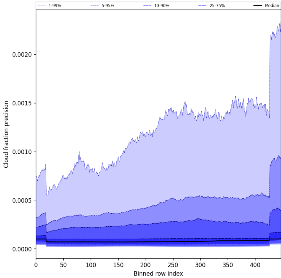
Figure 50: Along track statistics of “Cloud fraction precision” for 2025-06-11 to 2025-06-13
