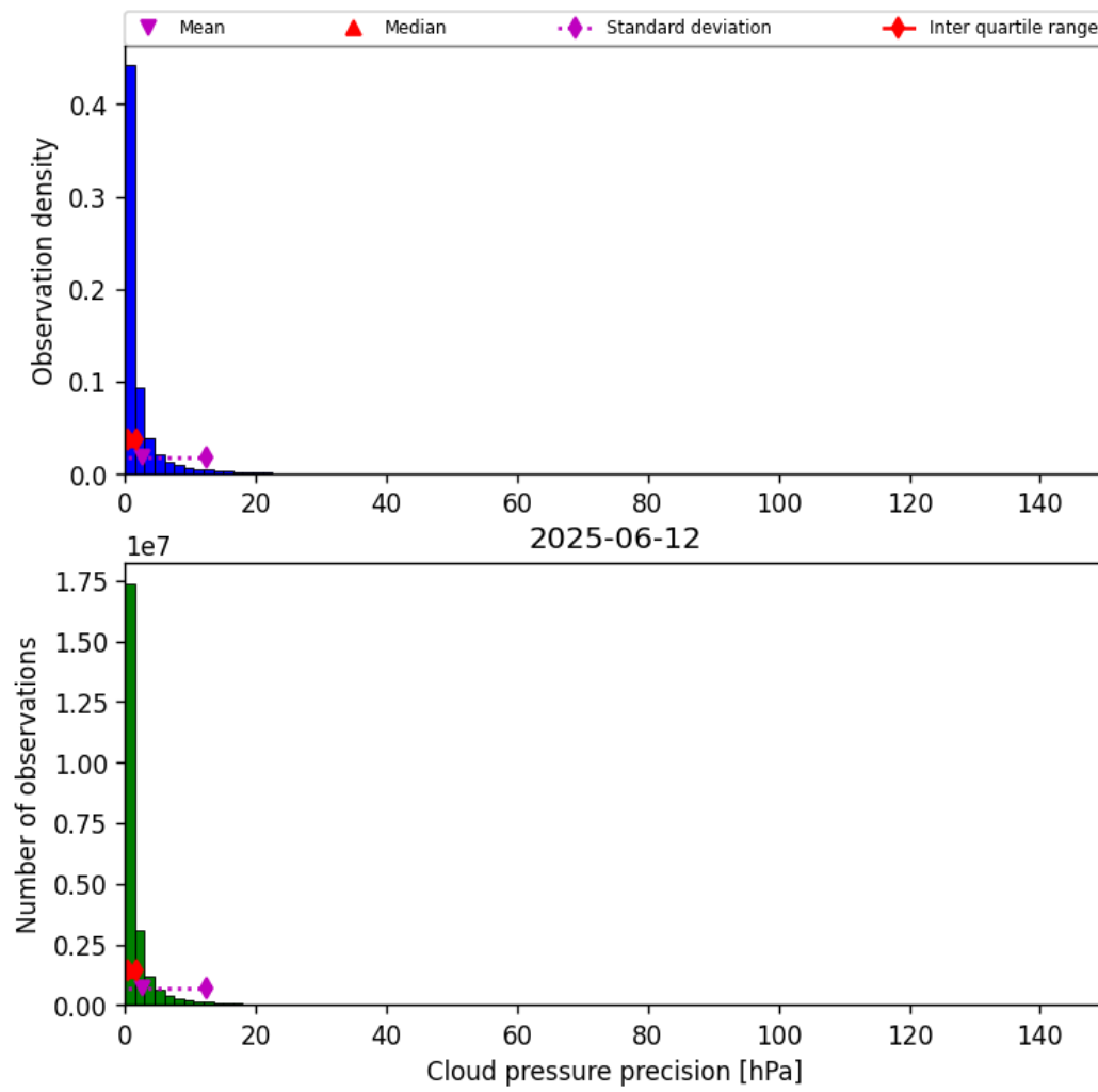
Figure 31: Histogram of “Cloud pressure precision” for 2025-06-11 to 2025-06-13
