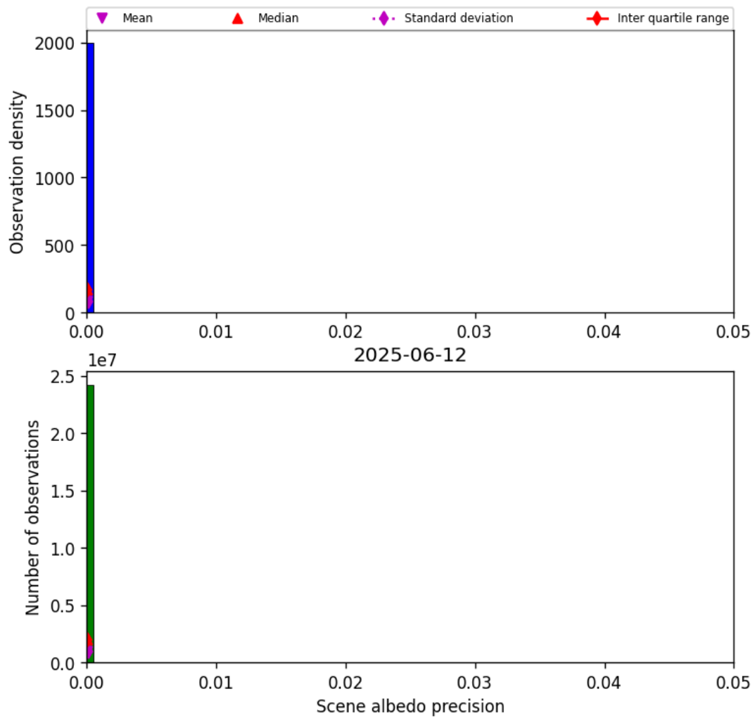
Figure 35: Histogram of “Scene albedo precision” for 2025-06-11 to 2025-06-13
