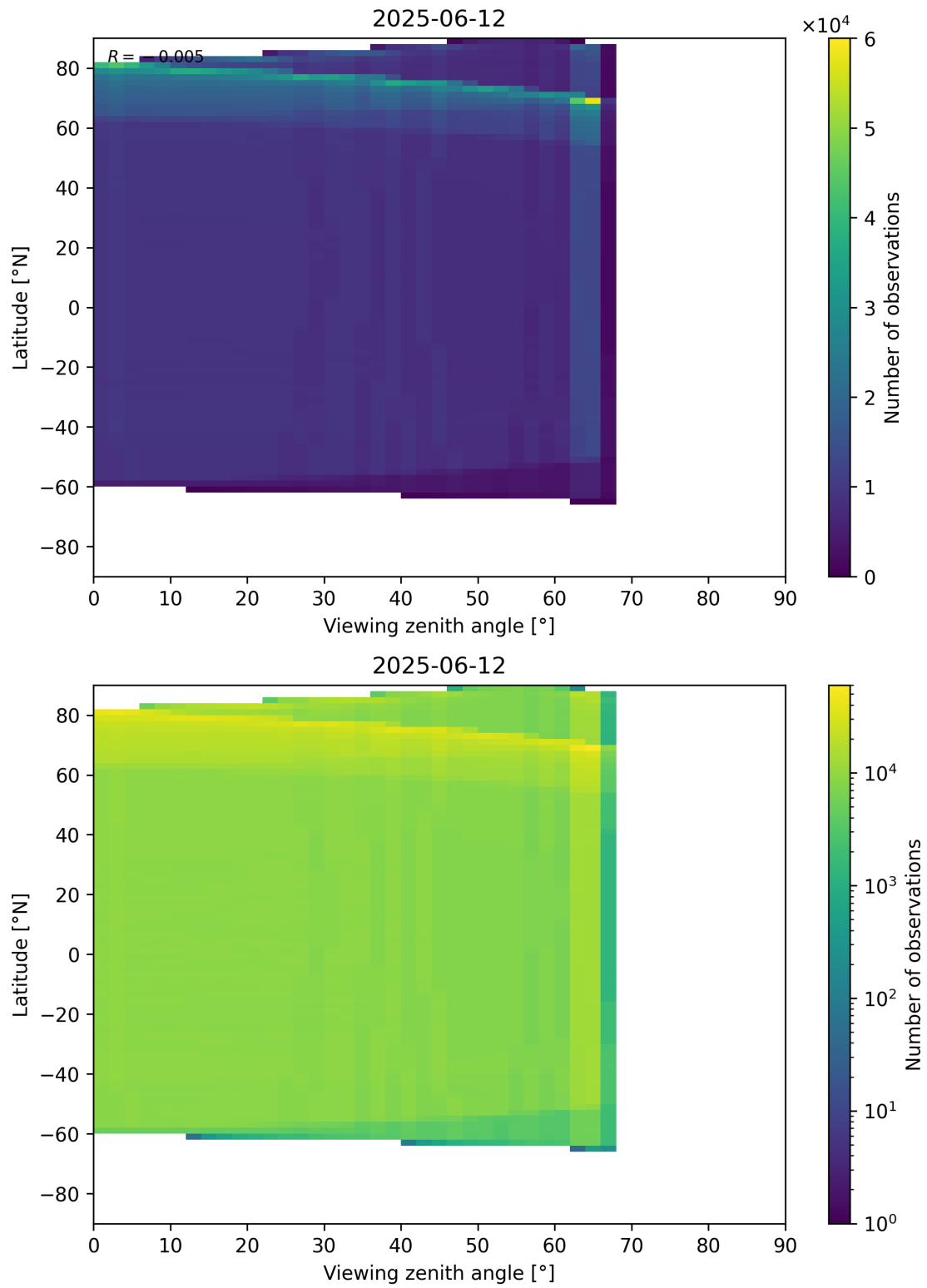
Figure 123: Scatter density plot of “Viewing zenith angle” against “Latitude” for 2025-06-11 to 2025-06-13.
