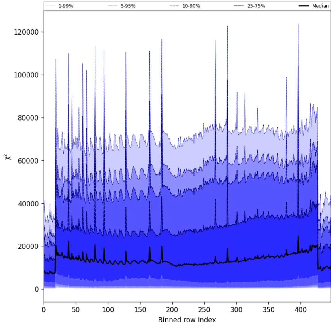
Figure 55: Along track statistics of “ \chi^2 ” for 2025-06-11 to 2025-06-13
