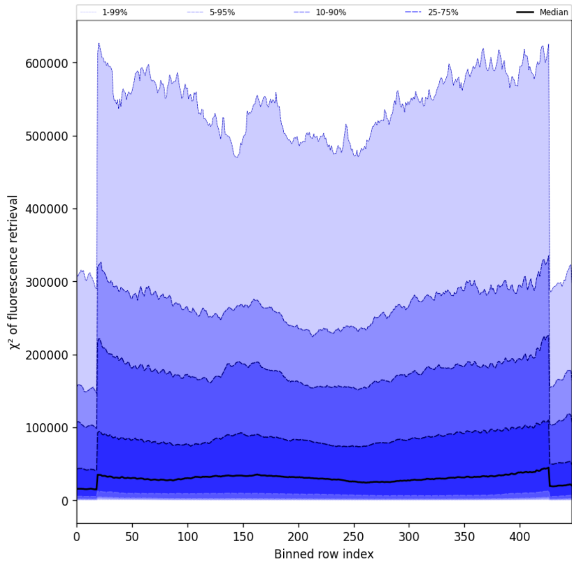
Figure 59: Along track statistics of “ \chi^2 of fluorescence retrieval” for 2025-06-11 to 2025-06-13
