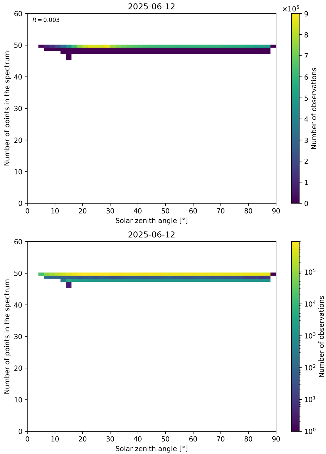
Figure 115: Scatter density plot of “Solar zenith angle” against “Number of points in the spectrum” for 2025-06-11 to 2025-06-13.
