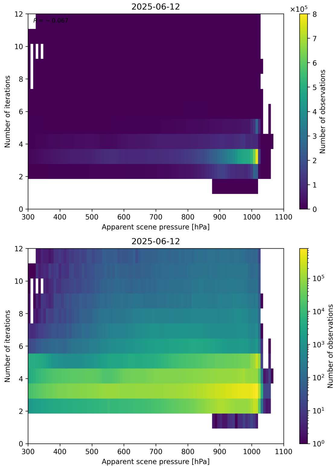
Figure 65: Scatter density plot of “Apparent scene pressure” against “Number of iterations” for 2025-06-11 to 2025-06-13.
