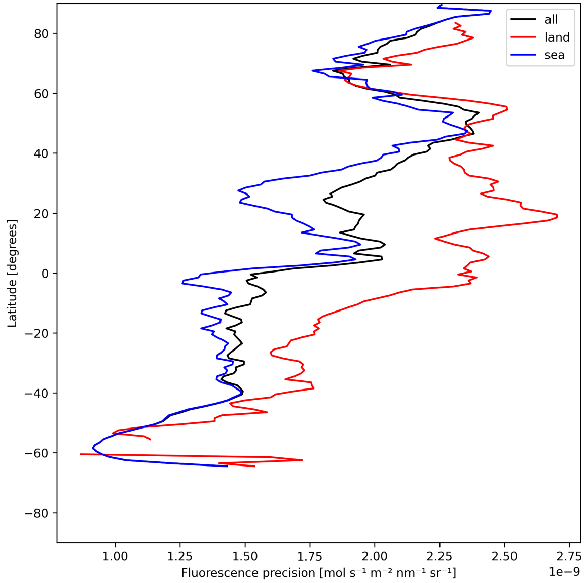
Figure 24: Zonal average of “Fluorescence precision” for 2025-06-11 to 2025-06-13.
