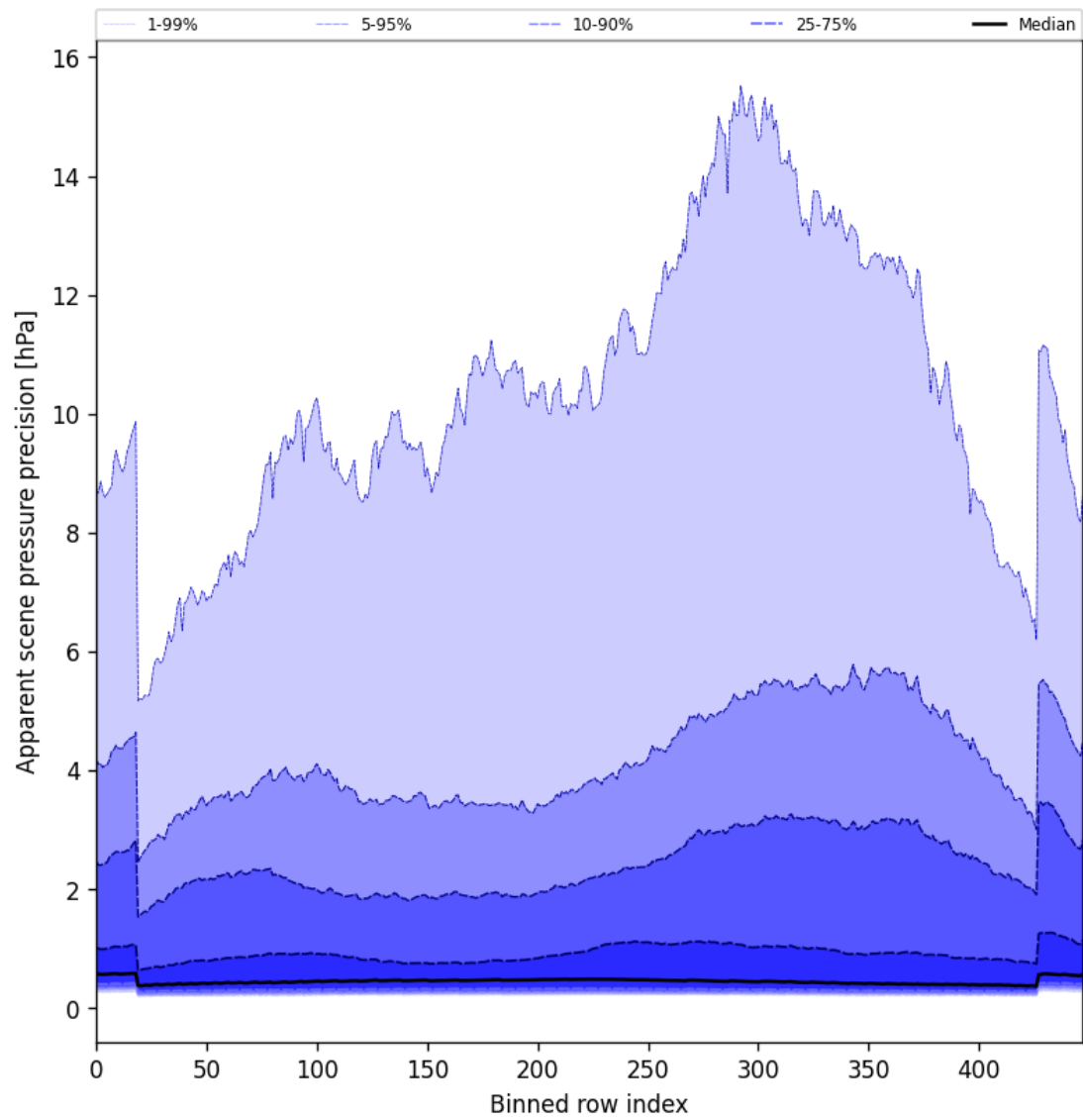
Figure 54: Along track statistics of “Apparent scene pressure precision” for 2025-06-11 to 2025-06-13
