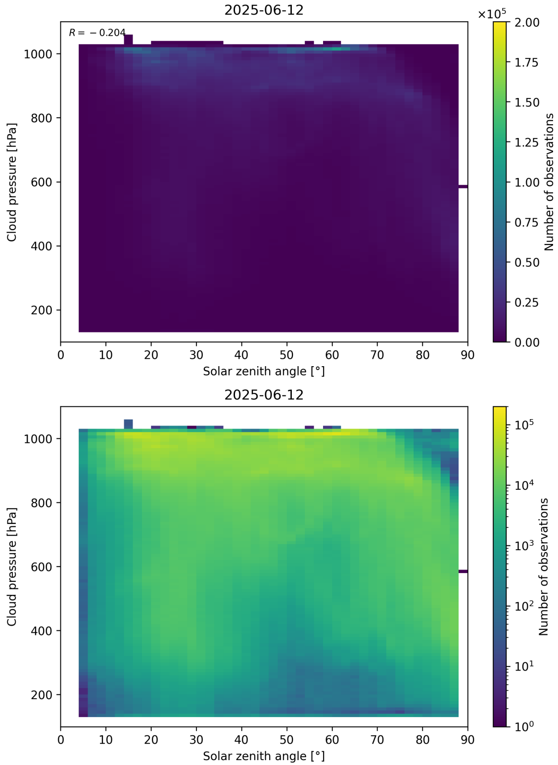
Figure 111: Scatter density plot of “Solar zenith angle” against “Cloud pressure” for 2025-06-11 to 2025-06-13.
