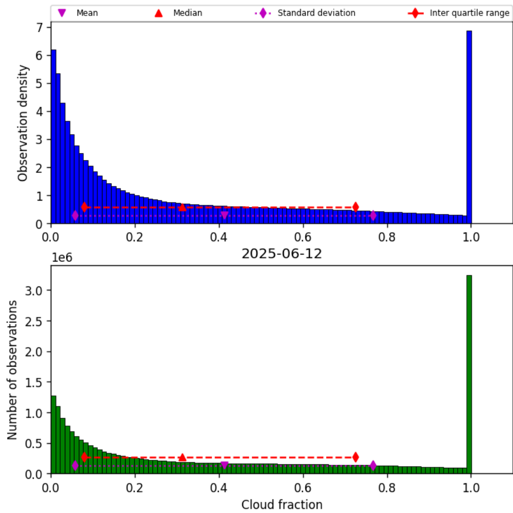
Figure 32: Histogram of “Cloud fraction” for 2025-06-11 to 2025-06-13
