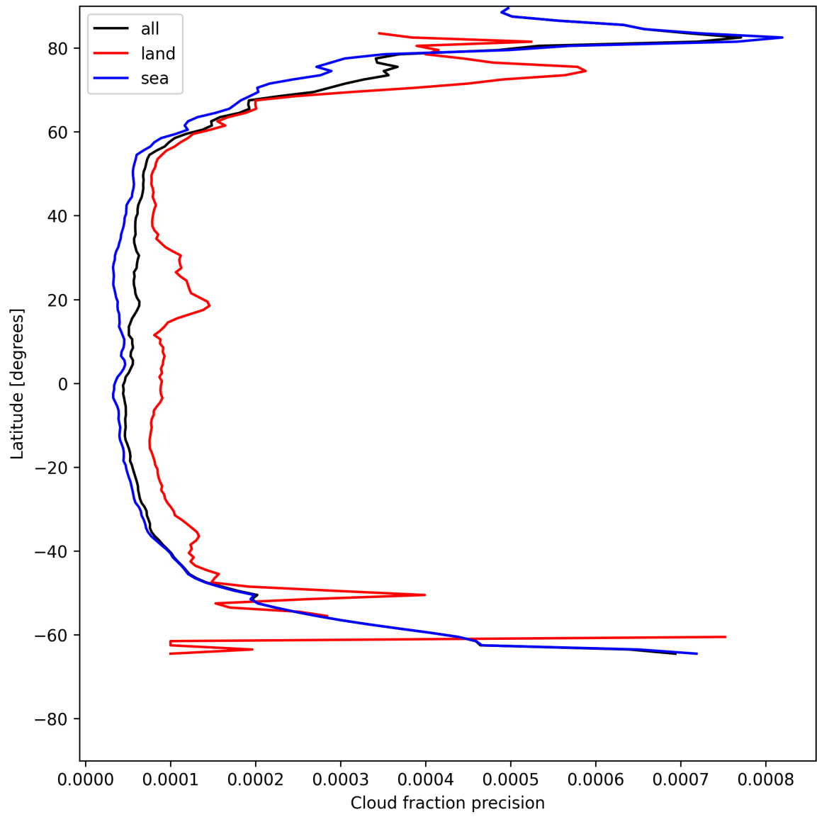
Figure 16: Zonal average of “Cloud fraction precision” for 2025-06-11 to 2025-06-13.
