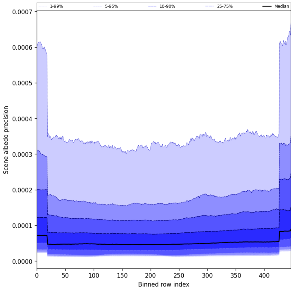
Figure 52: Along track statistics of “Scene albedo precision” for 2025-06-11 to 2025-06-13
