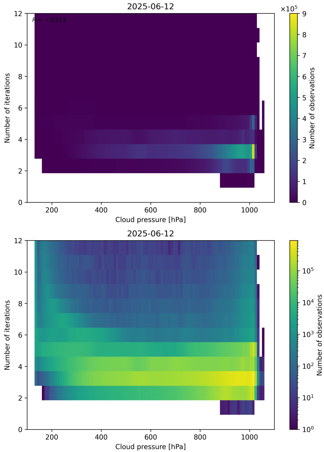
Figure 81: Scatter density plot of “Cloud pressure” against “Number of iterations” for 2025-06-11 to 2025-06-13.
