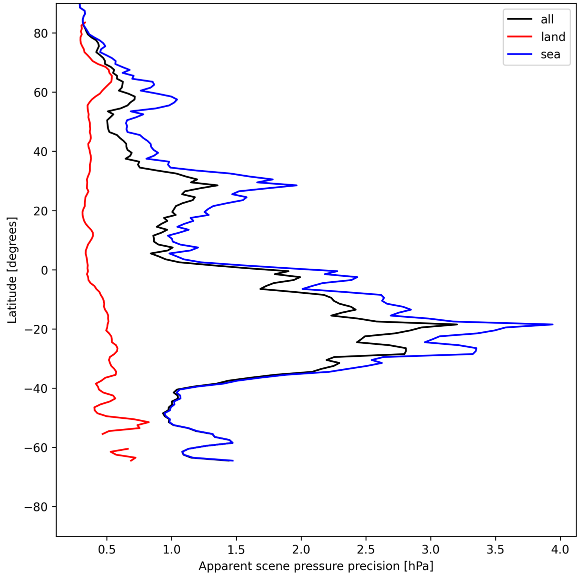
Figure 20: Zonal average of “Apparent scene pressure precision” for 2025-06-11 to 2025-06-13.
