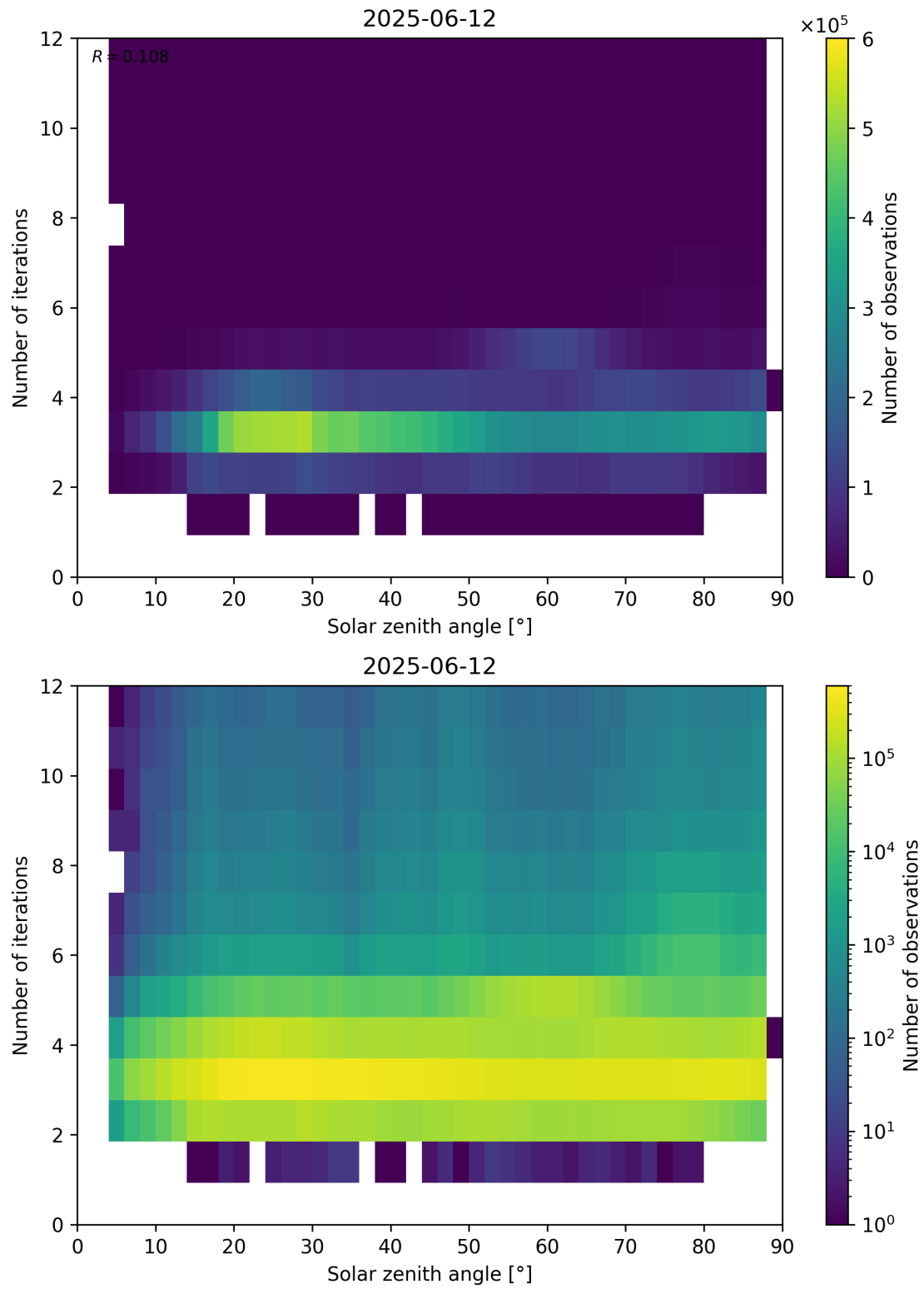
Figure 114: Scatter density plot of “Solar zenith angle” against “Number of iterations” for 2025-06-11 to 2025-06-13.
