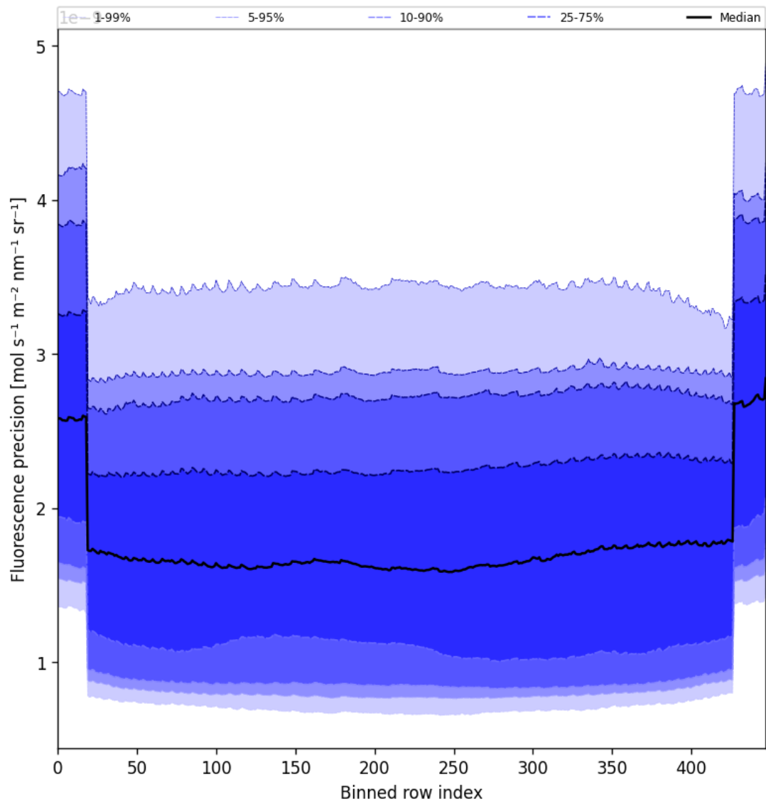
Figure 58: Along track statistics of “Fluorescence precision” for 2025-06-11 to 2025-06-13
