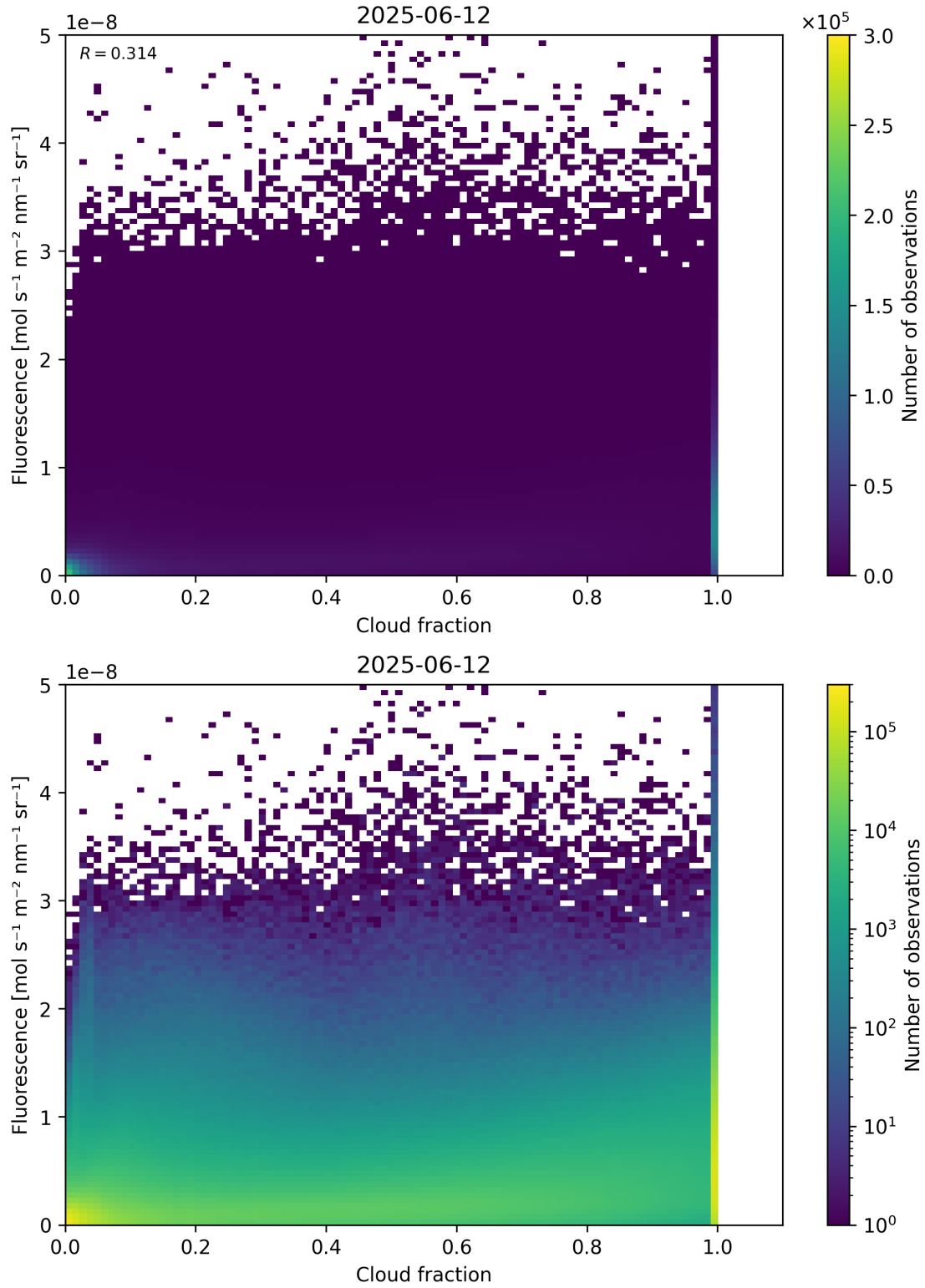
Figure 72: Scatter density plot of “Cloud fraction” against “Fluorescence” for 2025-06-11 to 2025-06-13.
