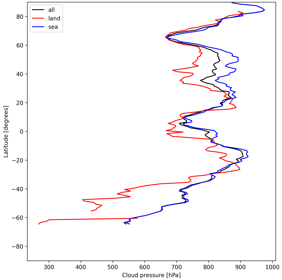
Figure 13: Zonal average of “Cloud pressure” for 2025-06-11 to 2025-06-13.
