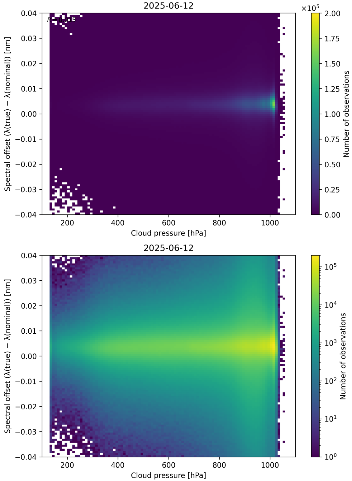
Figure 84: Scatter density plot of “Cloud pressure” against “Spectral offset ( \lambda_{\text{true}} - \lambda_{\text{nominal}} )” for 2025-06-11 to 2025-06-13.
