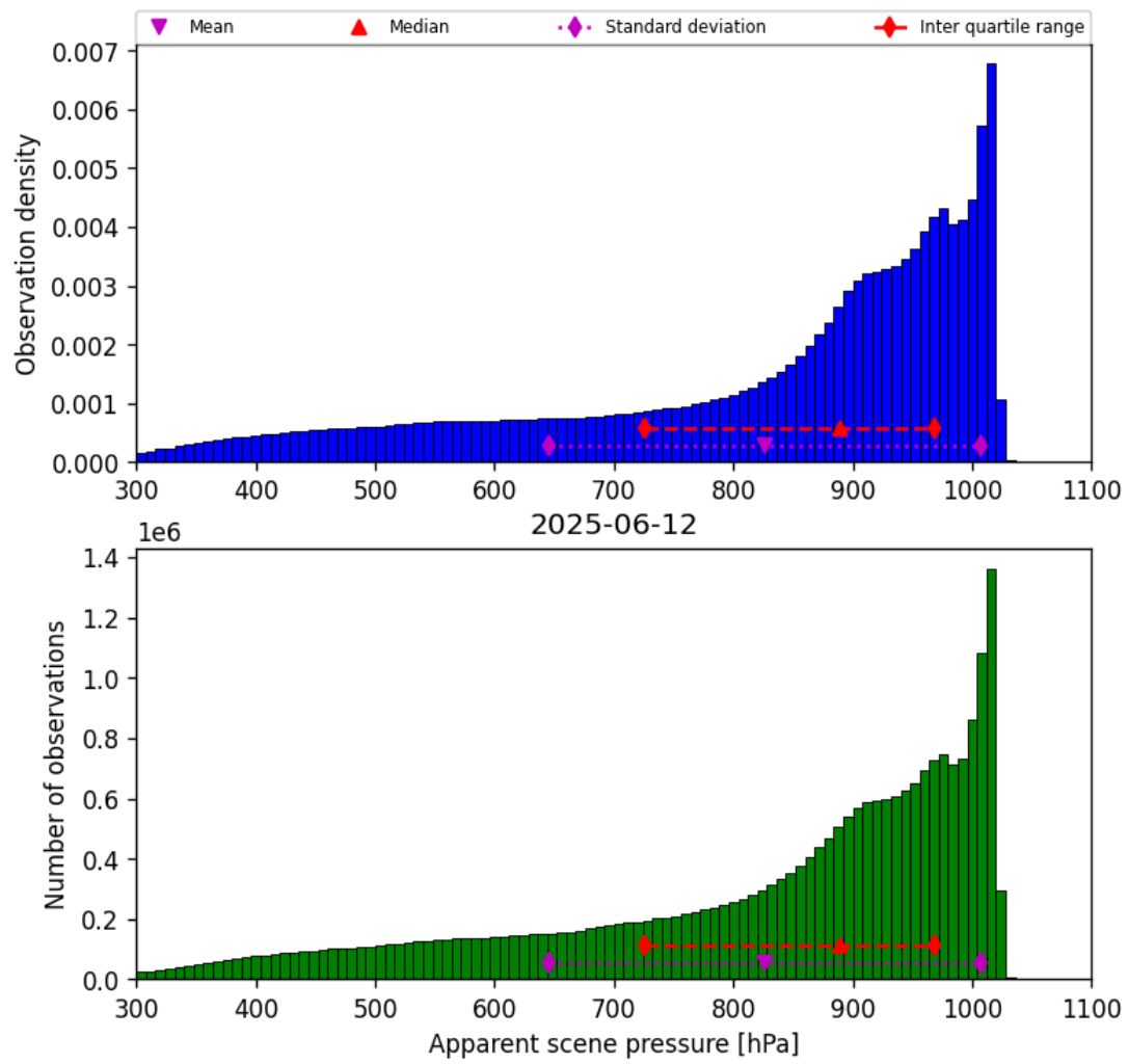
Figure 36: Histogram of “Apparent scene pressure” for 2025-06-11 to 2025-06-13
