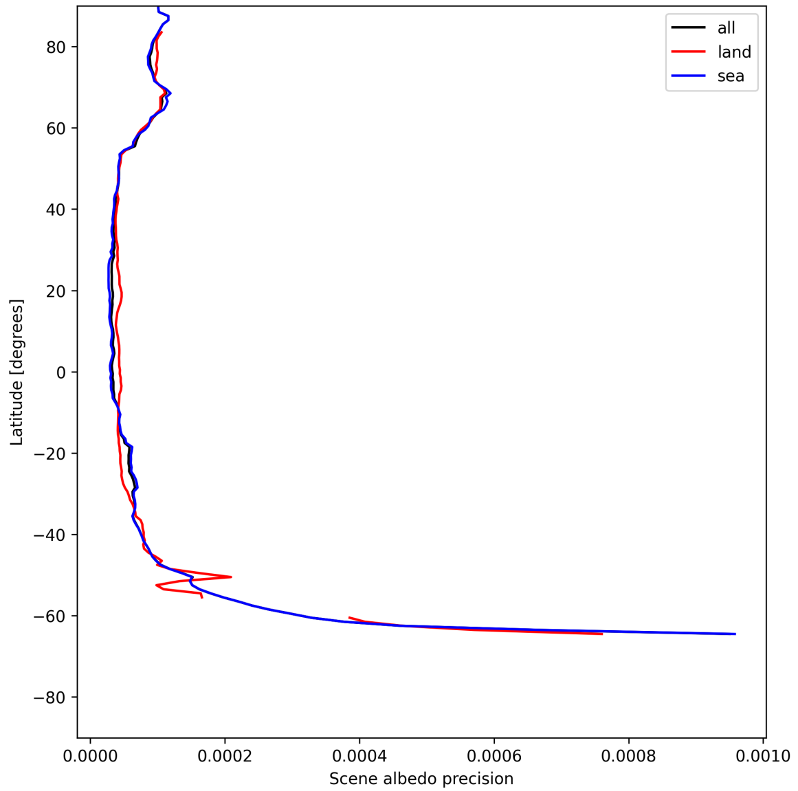
Figure 18: Zonal average of “Scene albedo precision” for 2025-06-11 to 2025-06-13.
