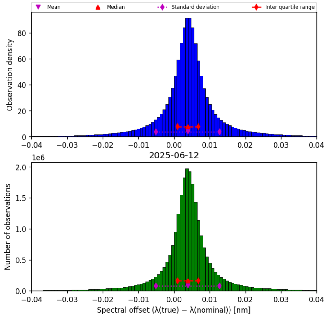
Figure 45: Histogram of “Spectral offset ( \lambda_{\text{true}} - \lambda_{\text{nominal}} )” for 2025-06-11 to 2025-06-13
