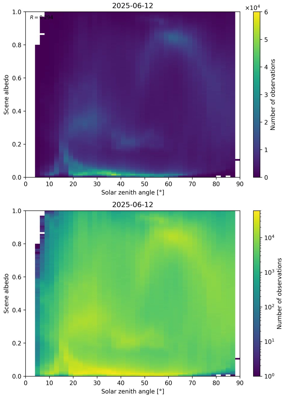
Figure 116: Scatter density plot of “Solar zenith angle” against “Scene albedo” for 2025-06-11 to 2025-06-13.
