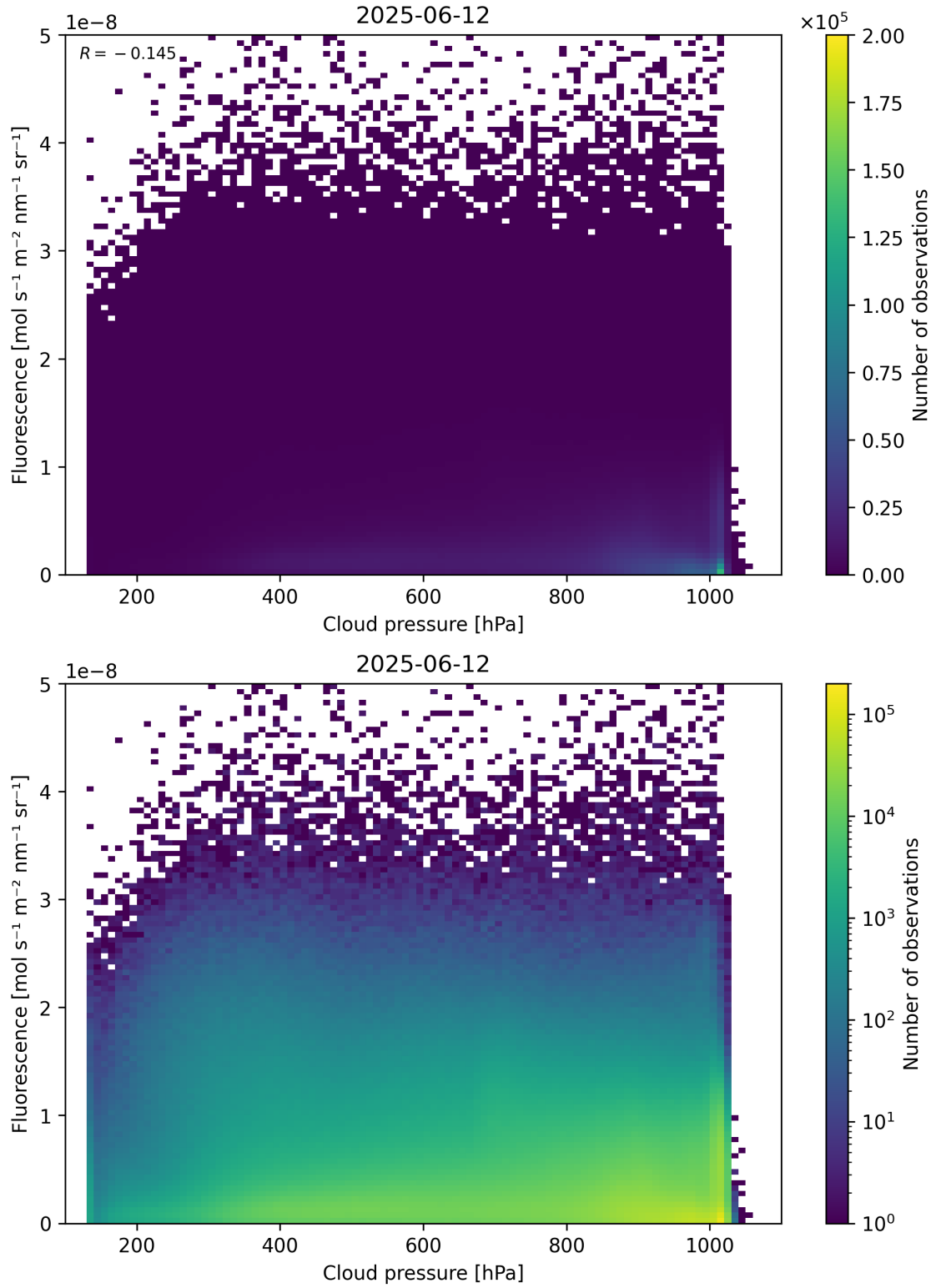
Figure 80: Scatter density plot of “Cloud pressure” against “Fluorescence” for 2025-06-11 to 2025-06-13.
