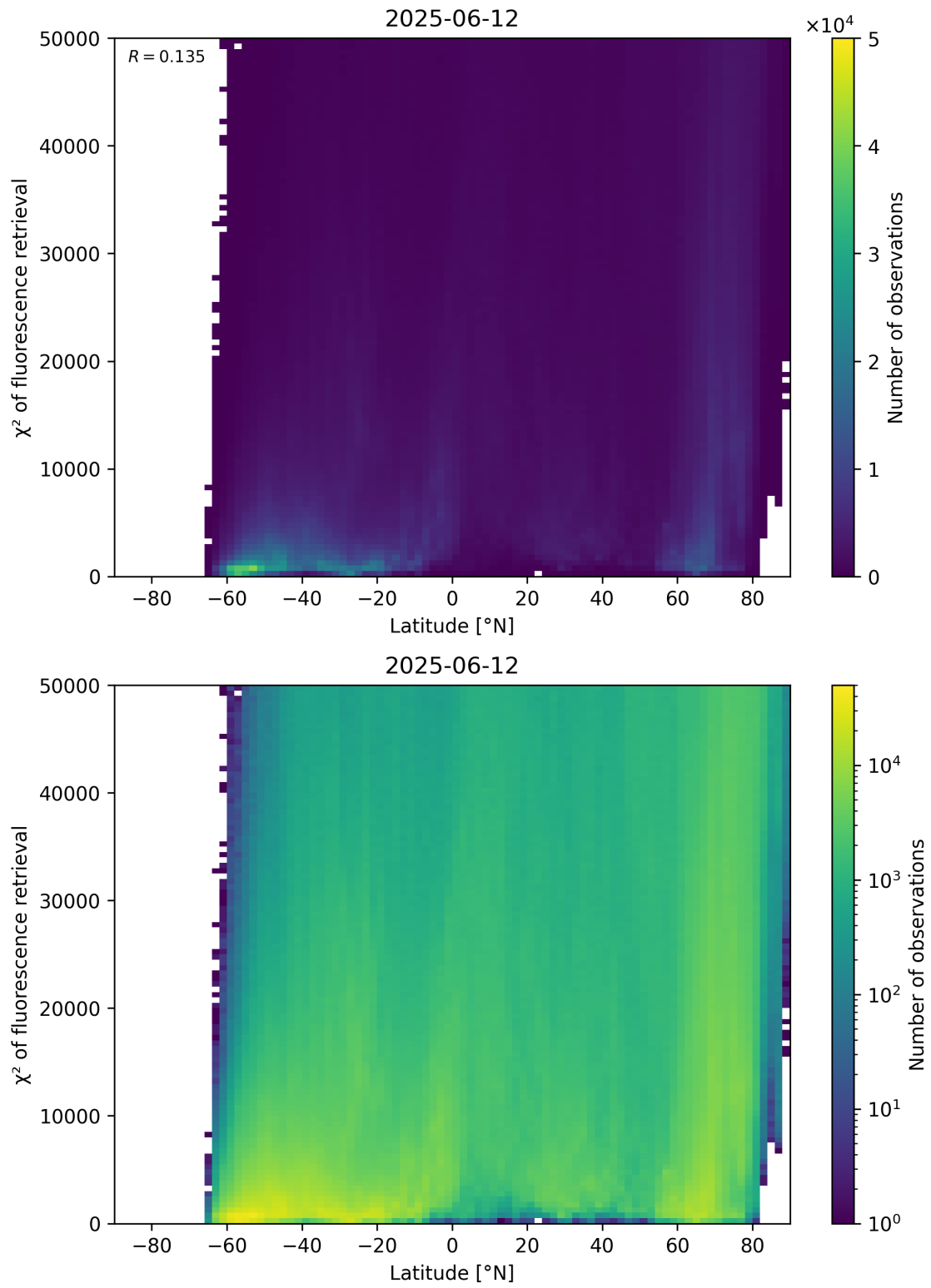
Figure 89: Scatter density plot of “Latitude” against “ \chi^2 of fluorescence retrieval” for 2025-06-11 to 2025-06-13.
