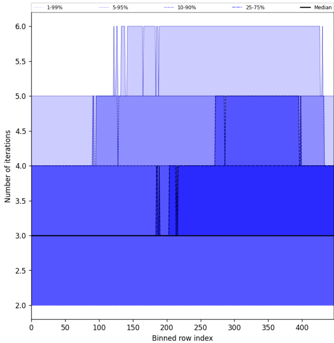
Figure 56: Along track statistics of “Number of iterations” for 2025-06-11 to 2025-06-13
