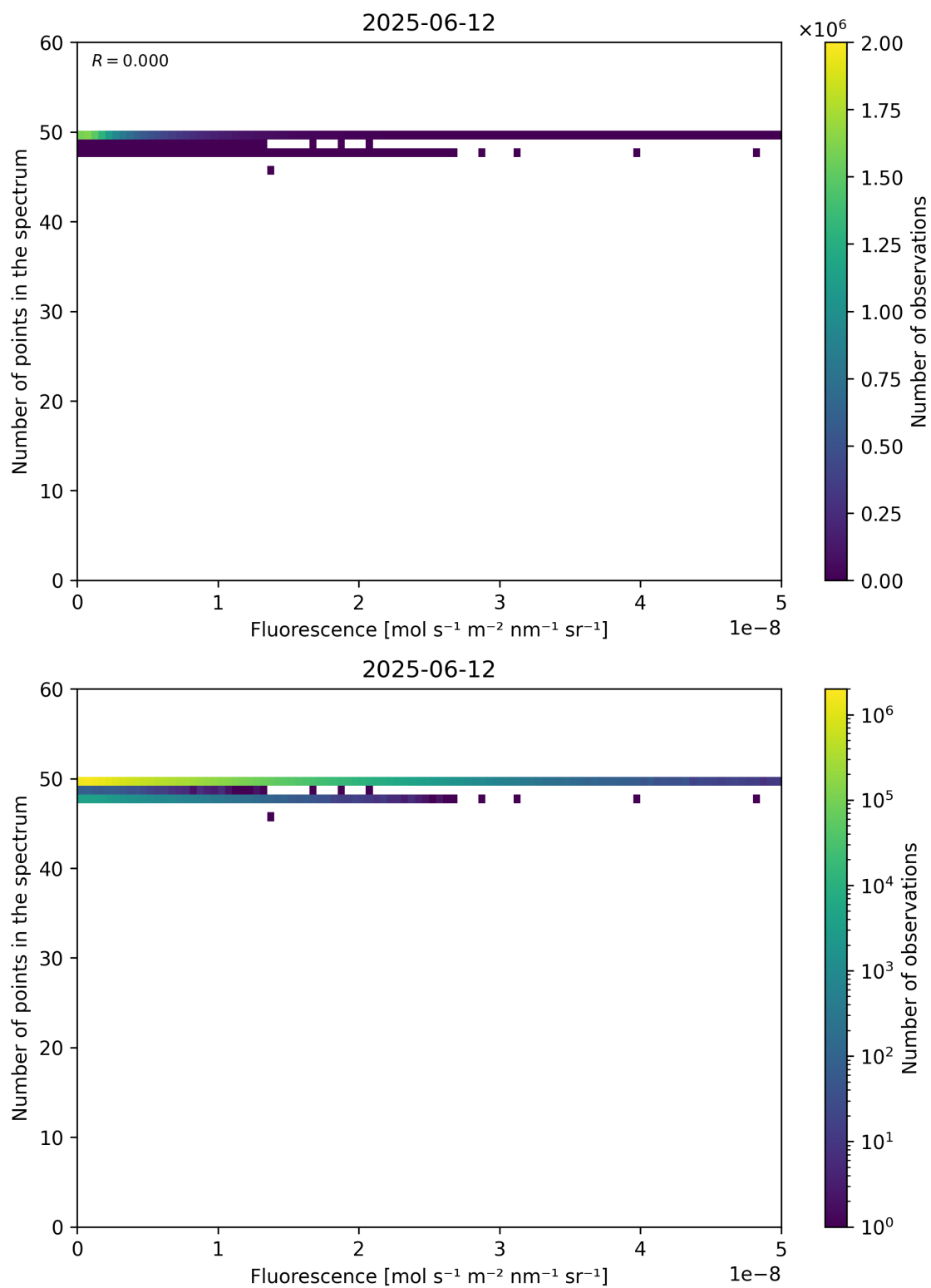
Figure 86: Scatter density plot of “Fluorescence” against “Number of points in the spectrum” for 2025-06-11 to 2025-06-13.
