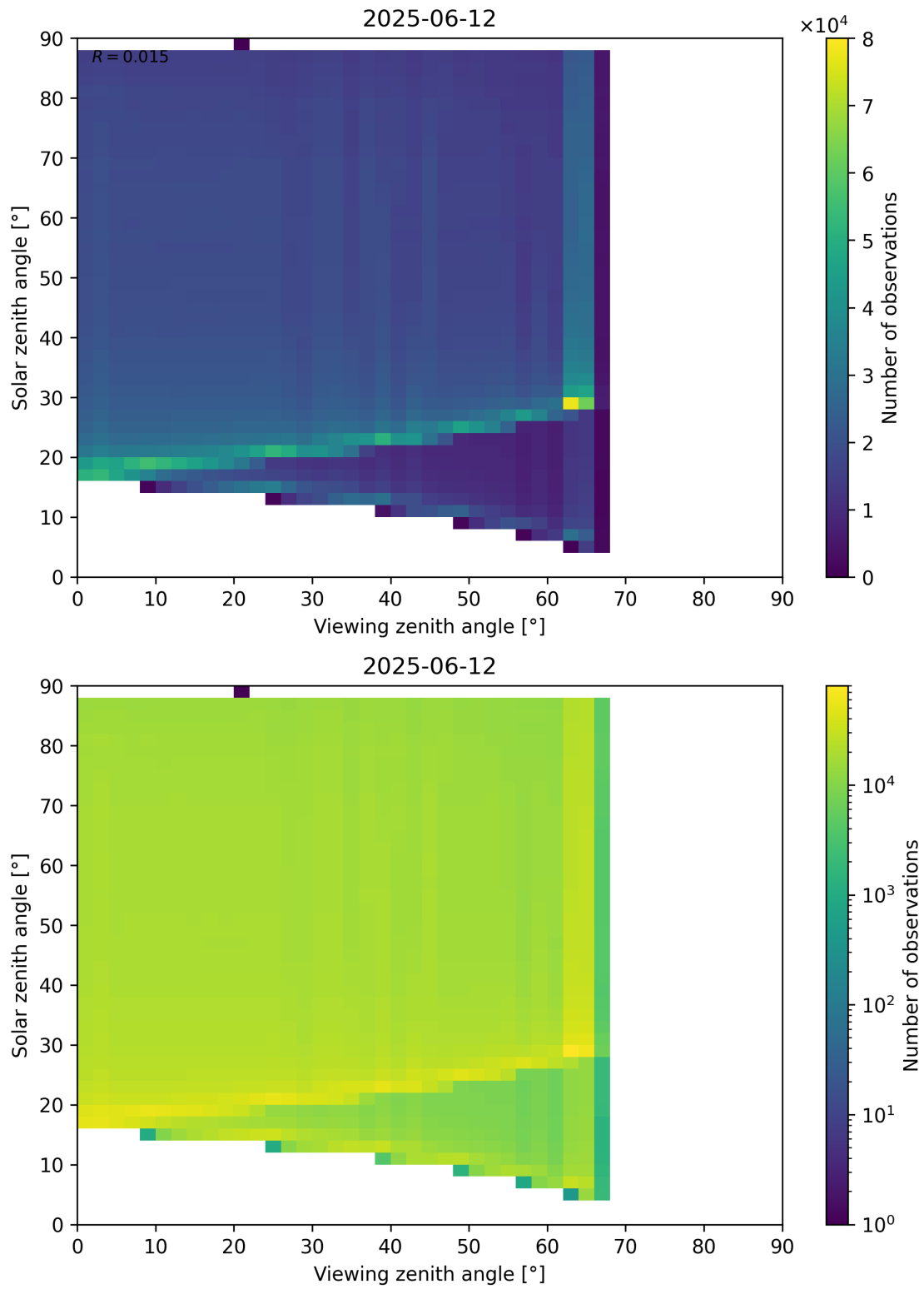
Figure 127: Scatter density plot of “Viewing zenith angle” against “Solar zenith angle” for 2025-06-11 to 2025-06-13.
