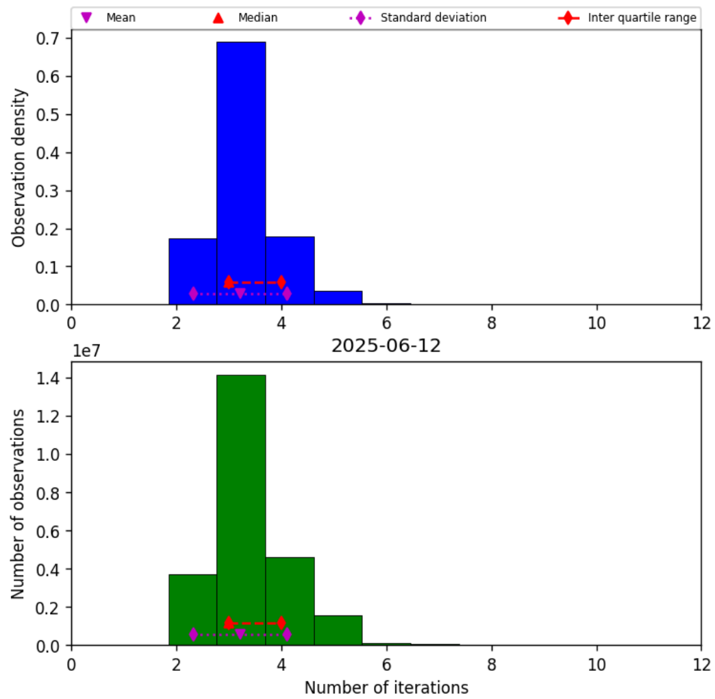
Figure 39: Histogram of “Number of iterations” for 2025-06-11 to 2025-06-13
