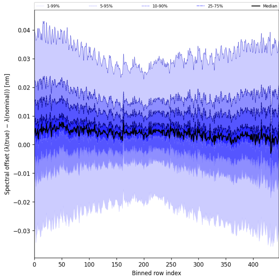
Figure 62: Along track statistics of “Spectral offset ( \lambda_{\text{true}} - \lambda_{\text{nominal}} )” for 2025-06-11 to 2025-06-13
