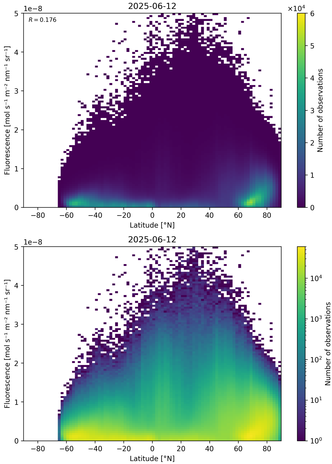
Figure 92: Scatter density plot of “Latitude” against “Fluorescence” for 2025-06-11 to 2025-06-13.
