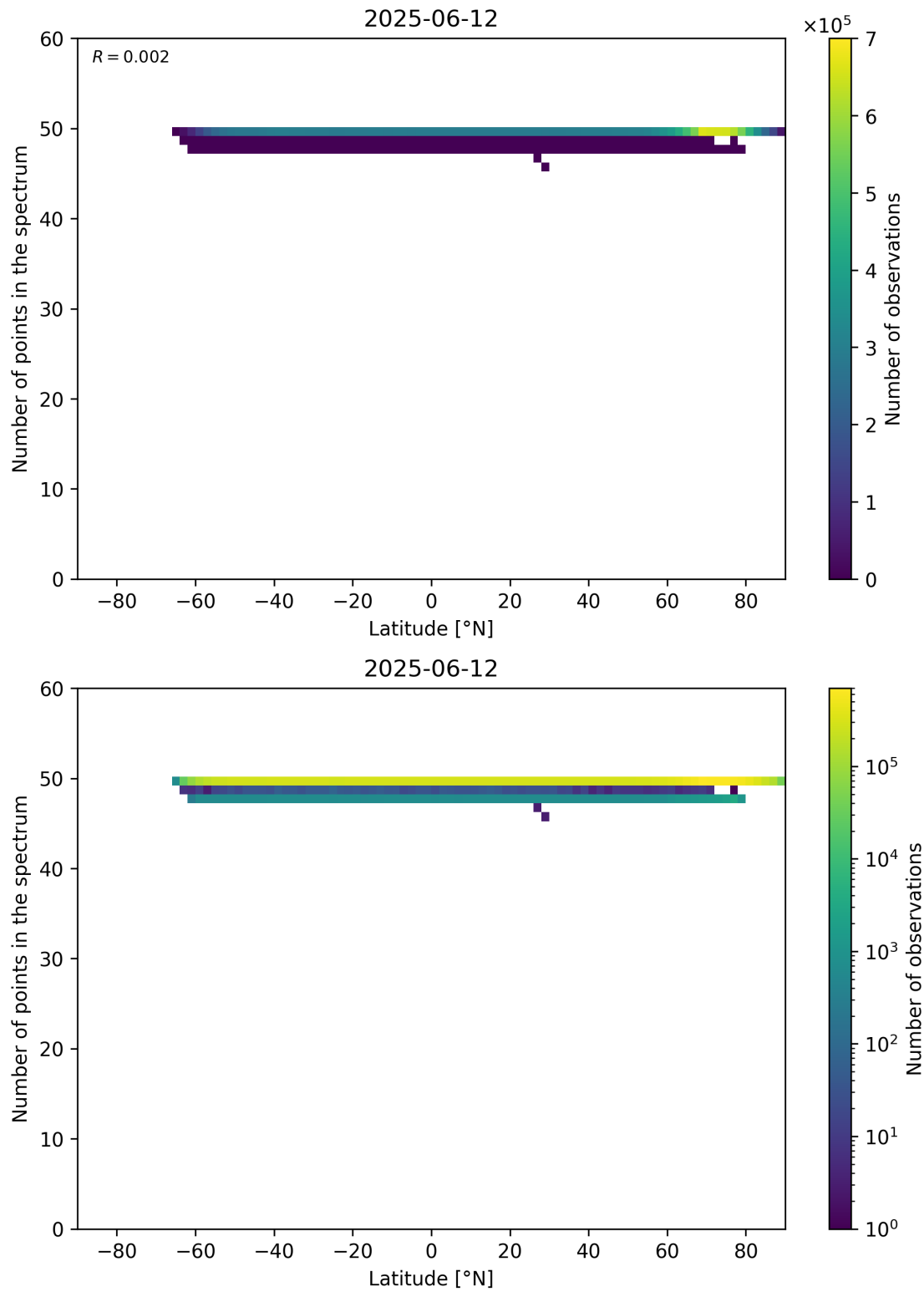
Figure 94: Scatter density plot of “Latitude” against “Number of points in the spectrum” for 2025-06-11 to 2025-06-13.
