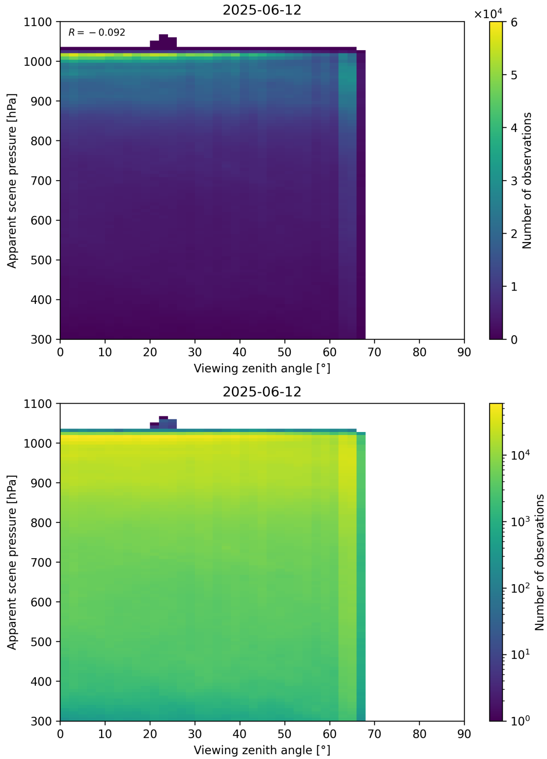
Figure 118: Scatter density plot of “Viewing zenith angle” against “Apparent scene pressure” for 2025-06-11 to 2025-06-13.
