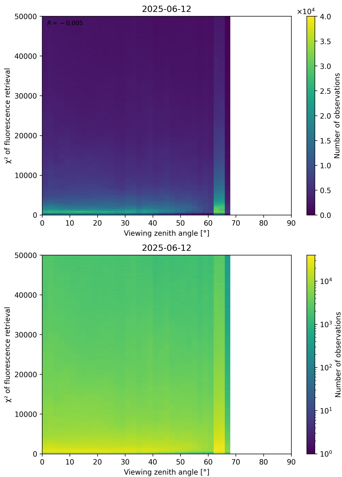
Figure 119: Scatter density plot of “Viewing zenith angle” against “ \chi^2 of fluorescence retrieval” for 2025-06-11 to 2025-06-13.
