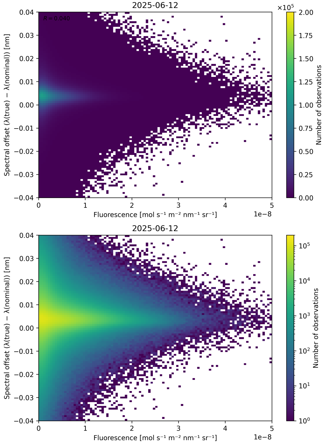
Figure 87: Scatter density plot of “Fluorescence” against “Spectral offset ( \lambda_{\text{true}} - \lambda_{\text{nominal}} )” for 2025-06-11 to 2025-06-13.
