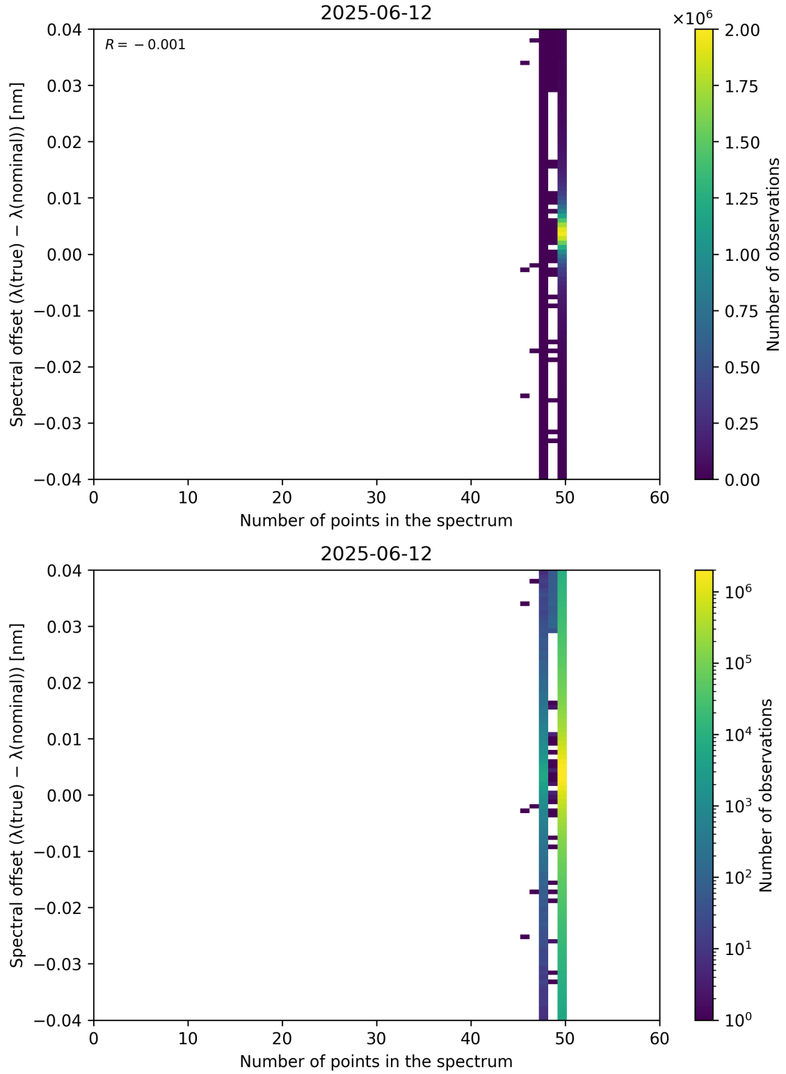
Figure 101: Scatter density plot of “Number of points in the spectrum” against “Spectral offset ( \lambda_{\text{true}} - \lambda_{\text{nominal}} )” for 2025-06-11 to 2025-06-13.
