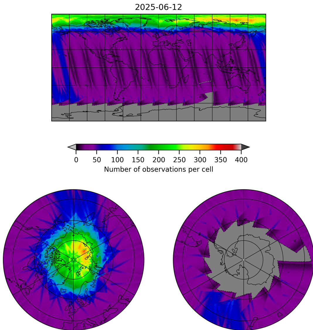
Figure 11: Map of the number of observations for 2025-06-11 to 2025-06-13
