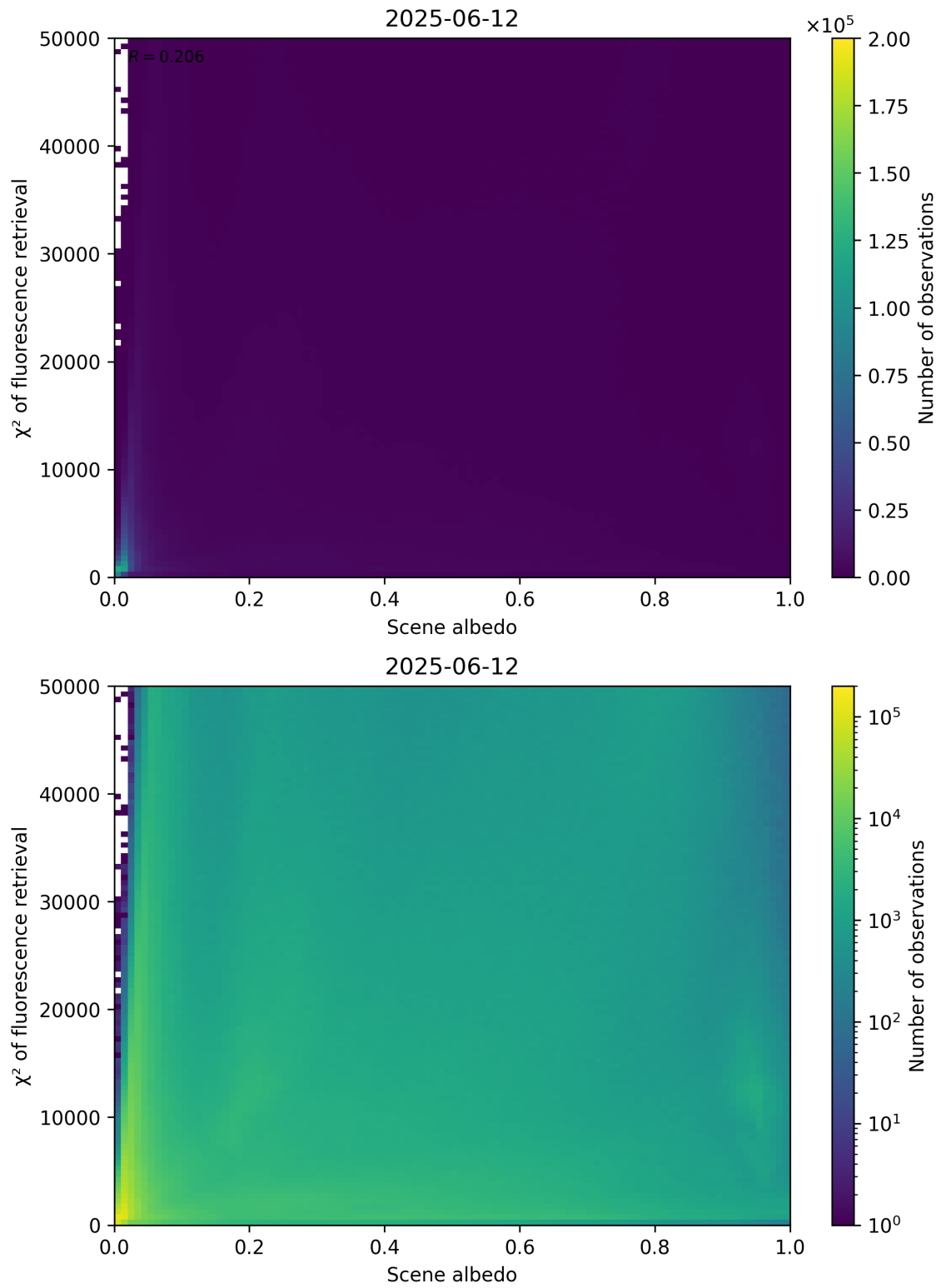
Figure 103: Scatter density plot of “Scene albedo” against “ \chi^2 of fluorescence retrieval” for 2025-06-11 to 2025-06-13.
