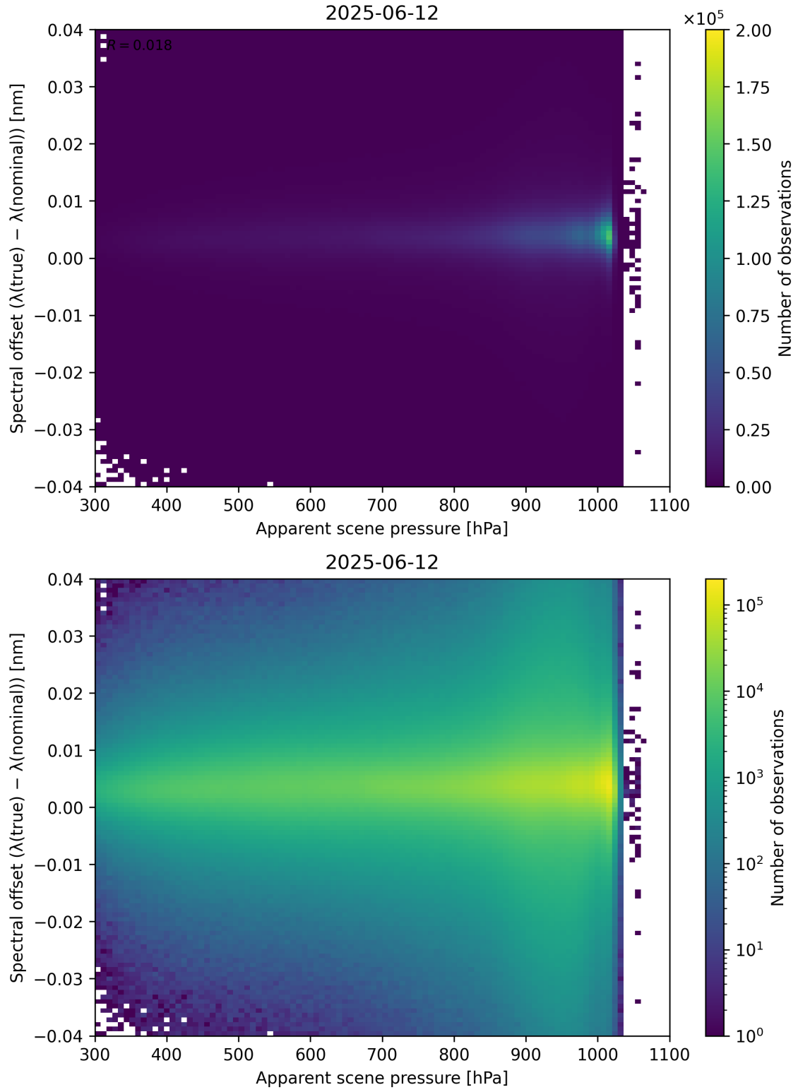
Figure 67: Scatter density plot of “Apparent scene pressure” against “Spectral offset ( \lambda_{\text{true}} - \lambda_{\text{nominal}} )” for 2025-06-11 to 2025-06-13.
