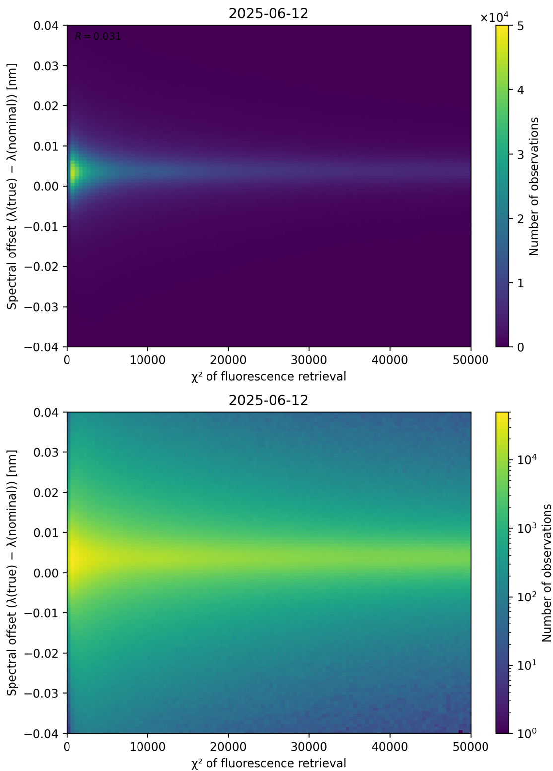
Figure 69: Scatter density plot of “ \chi^2 of fluorescence retrieval” against “Spectral offset ( \lambda_{\text{true}} - \lambda_{\text{nominal}} )” for 2025-06-11 to 2025-06-13.
