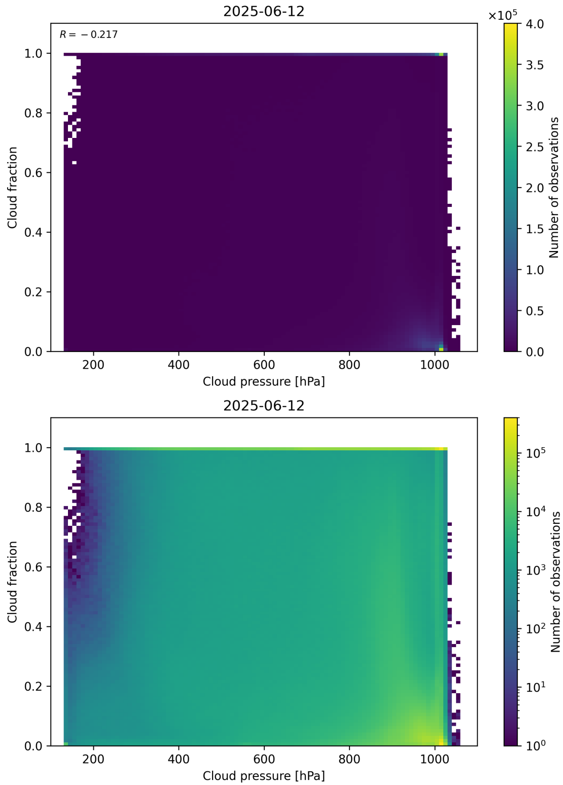
Figure 79: Scatter density plot of “Cloud pressure” against “Cloud fraction” for 2025-06-11 to 2025-06-13.
