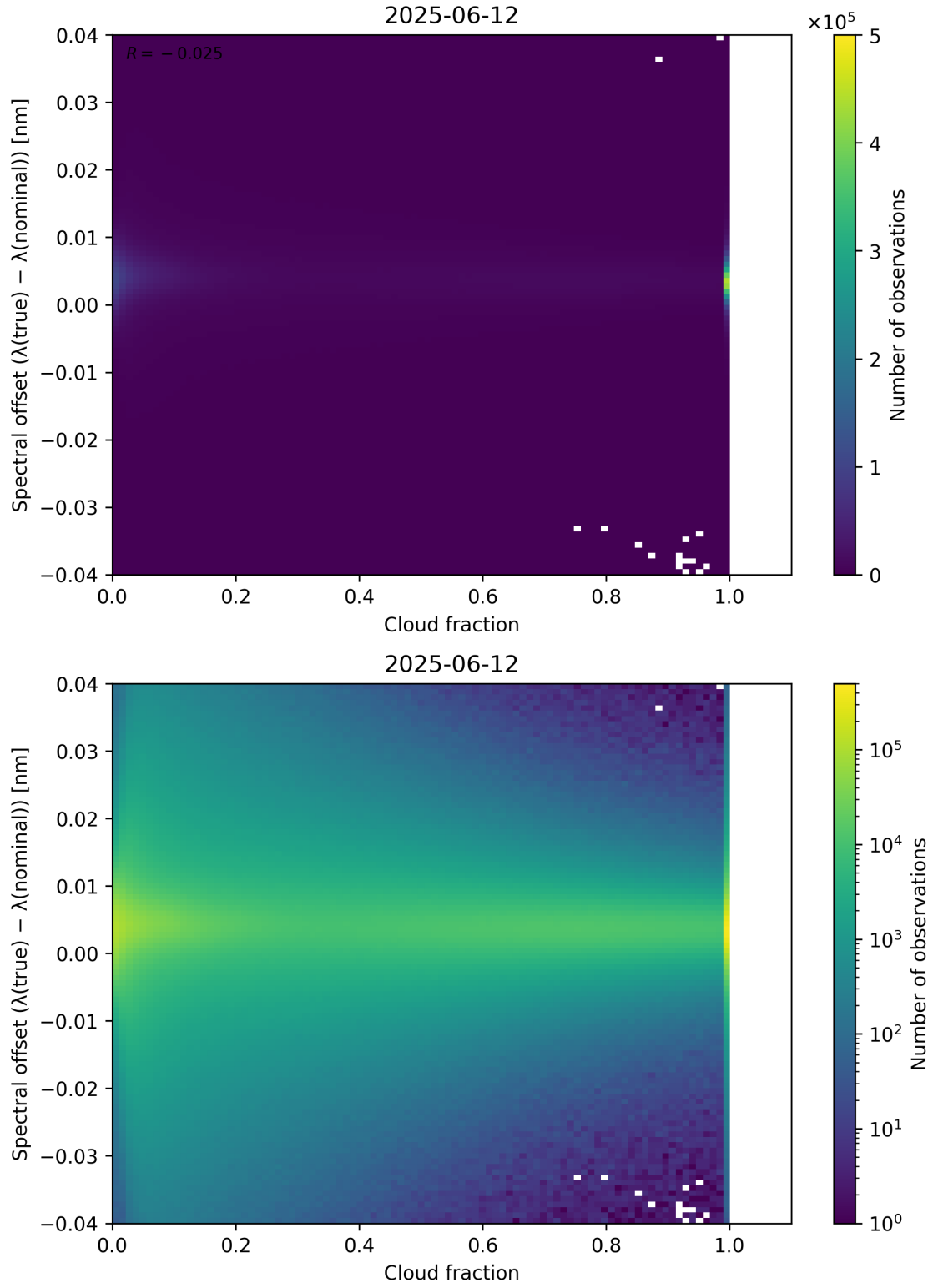
Figure 76: Scatter density plot of “Cloud fraction” against “Spectral offset ( \lambda_{\text{true}} - \lambda_{\text{nominal}} )” for 2025-06-11 to 2025-06-13.
