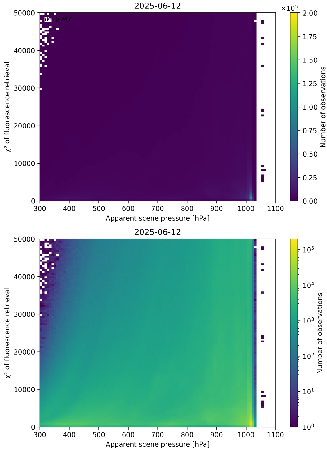
Figure 63: Scatter density plot of “Apparent scene pressure” against “ \chi^2 of fluorescence retrieval” for 2025-06-11 to 2025-06-13.
