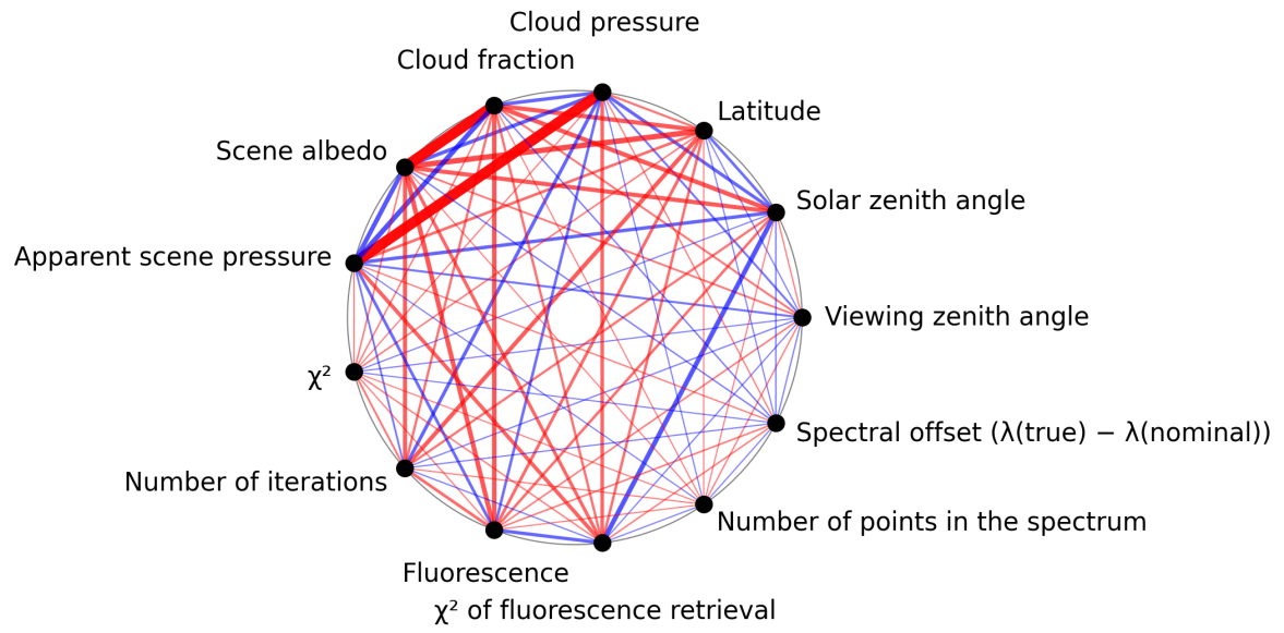
Figure 1: Map of correlation graph for 2025-06-11 to 2025-06-13.
