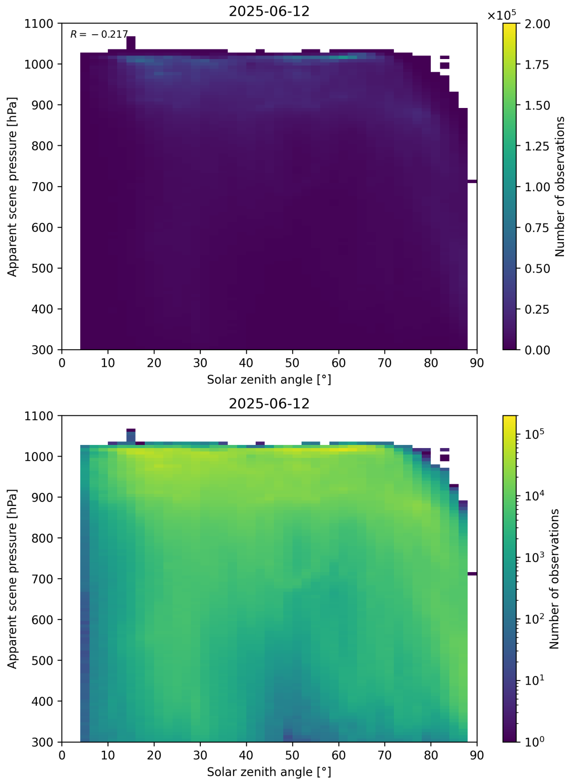
Figure 108: Scatter density plot of “Solar zenith angle” against “Apparent scene pressure” for 2025-06-11 to 2025-06-13.
