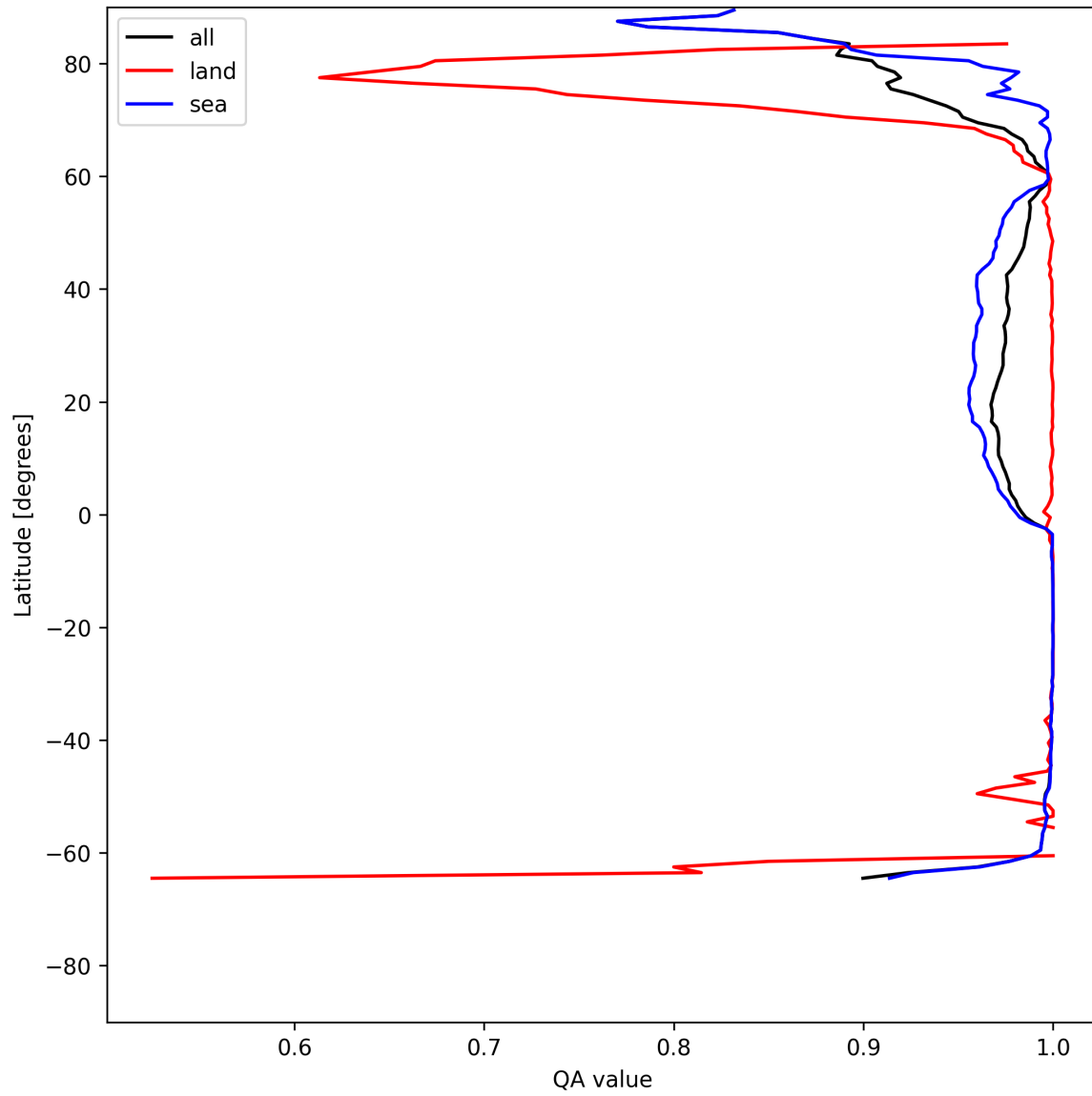
Figure 12: Zonal average of “QA value” for 2025-06-11 to 2025-06-13.
