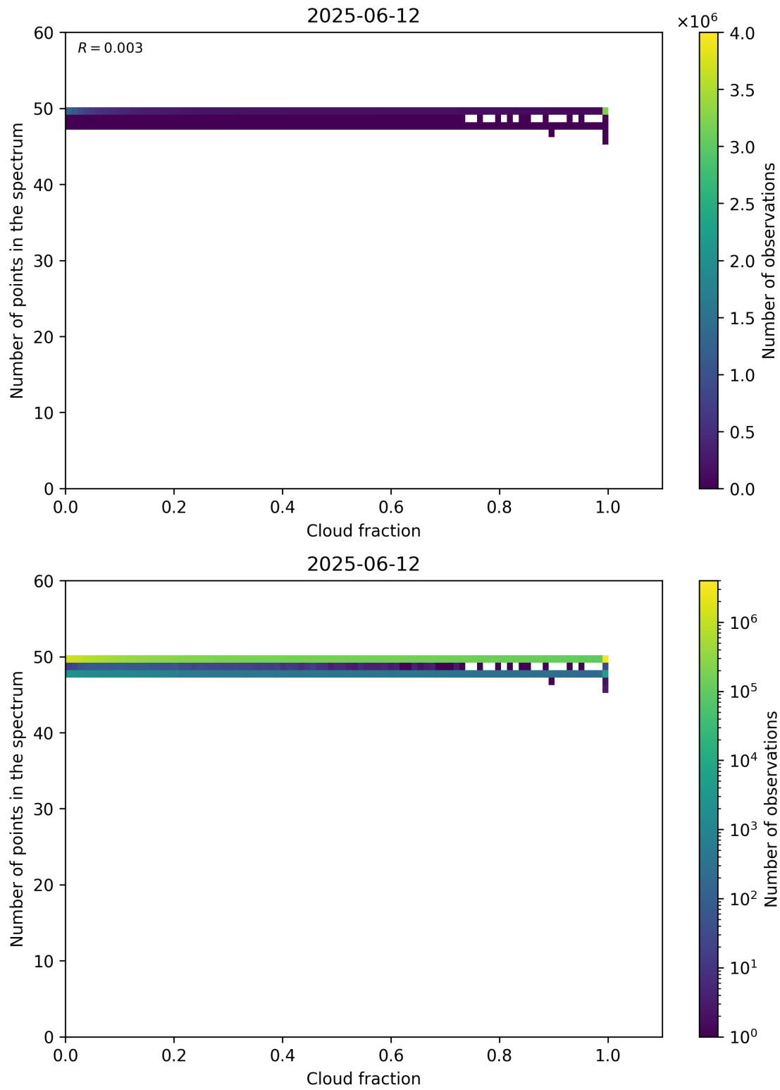
Figure 74: Scatter density plot of “Cloud fraction” against “Number of points in the spectrum” for 2025-06-11 to 2025-06-13.
