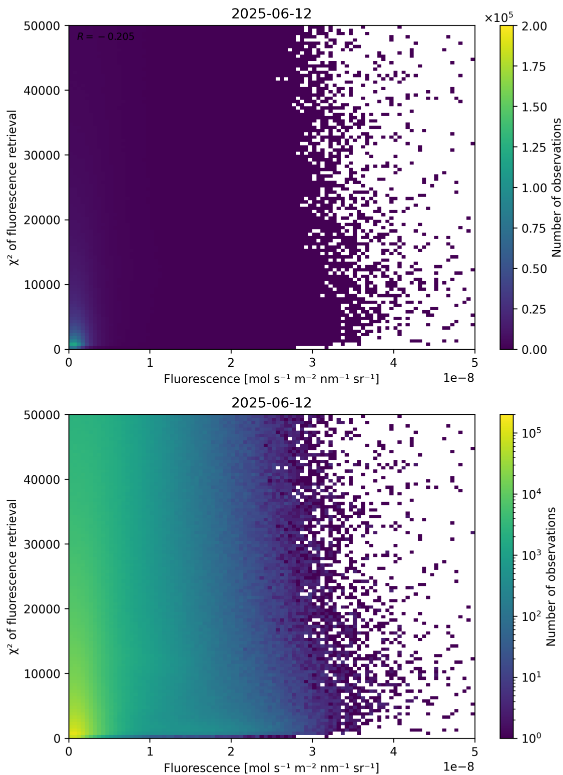
Figure 85: Scatter density plot of “Fluorescence” against “ \chi^2 of fluorescence retrieval” for 2025-06-11 to 2025-06-13.
