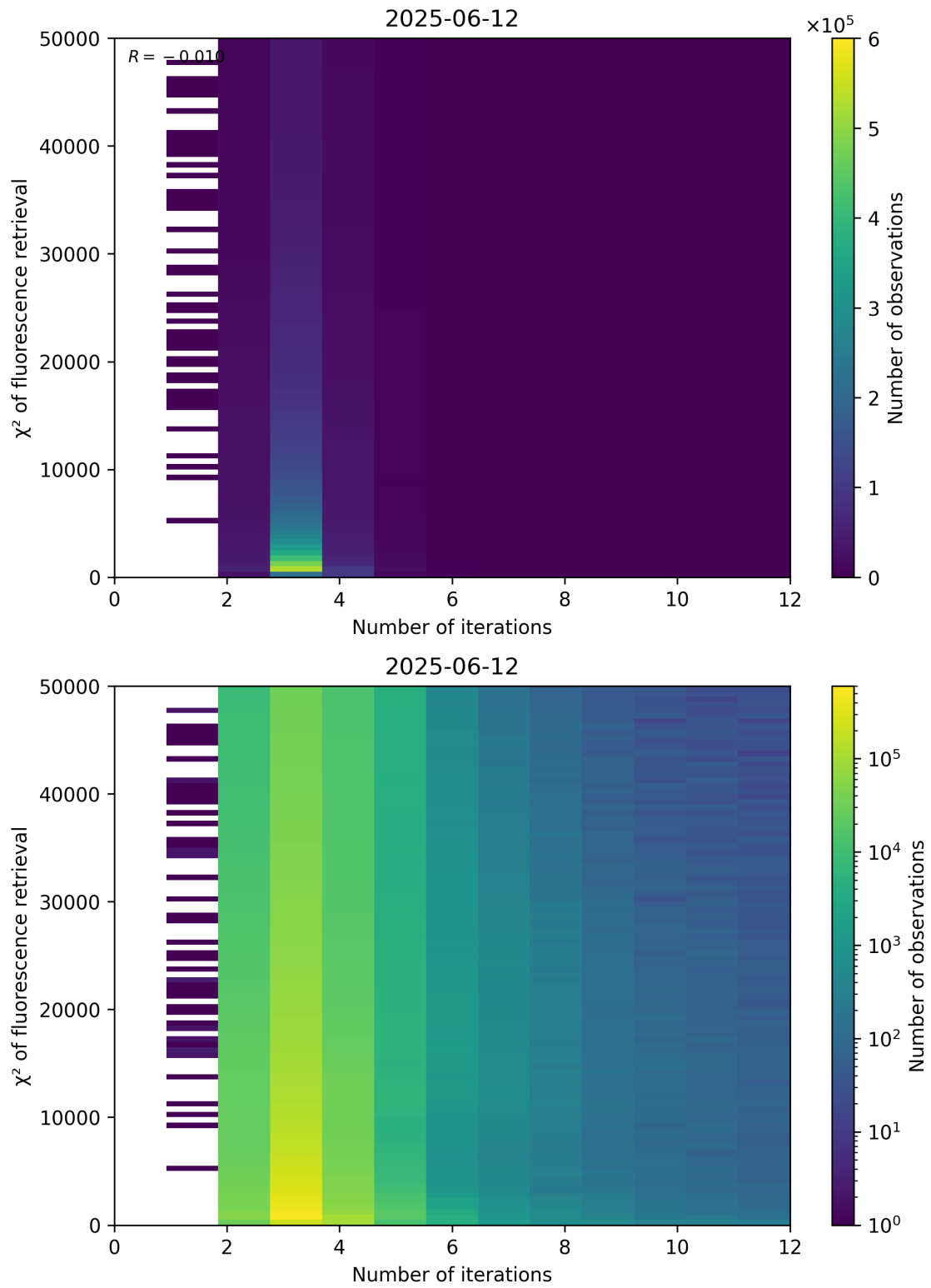
Figure 97: Scatter density plot of “Number of iterations” against “ \chi^2 of fluorescence retrieval” for 2025-06-11 to 2025-06-13.
