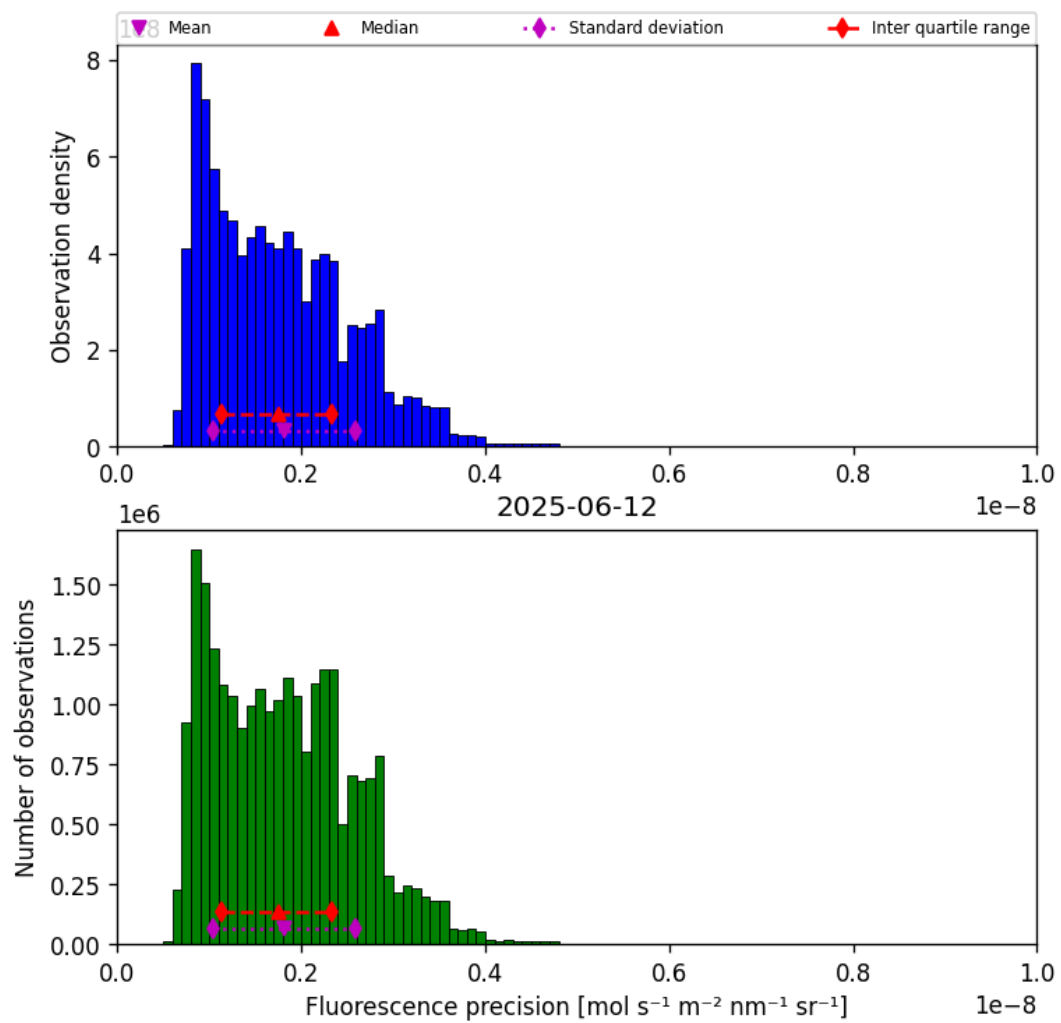
Figure 41: Histogram of “Fluorescence precision” for 2025-06-11 to 2025-06-13
