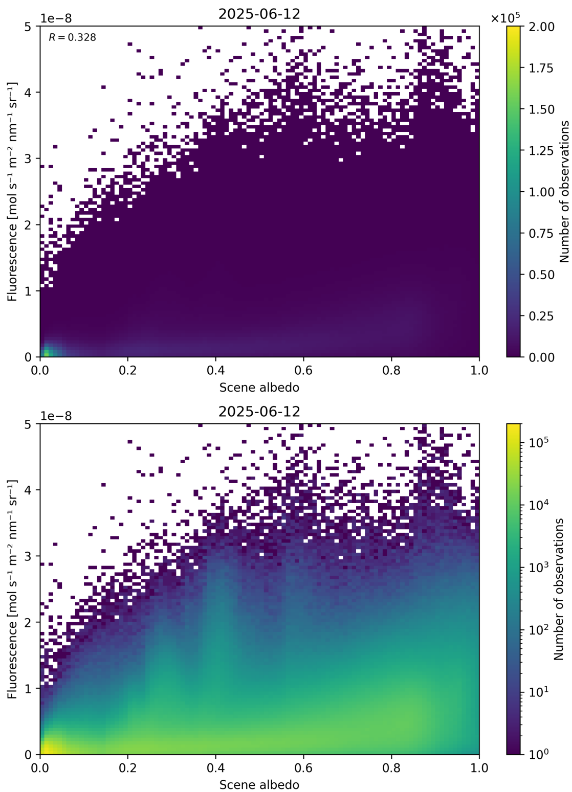
Figure 104: Scatter density plot of “Scene albedo” against “Fluorescence” for 2025-06-11 to 2025-06-13.
