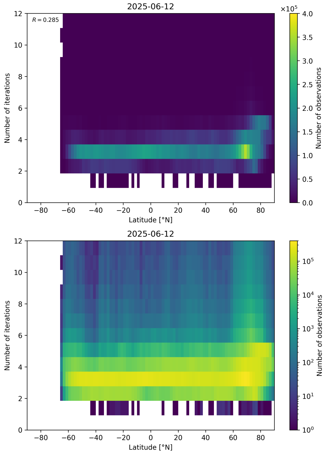
Figure 93: Scatter density plot of “Latitude” against “Number of iterations” for 2025-06-11 to 2025-06-13.
