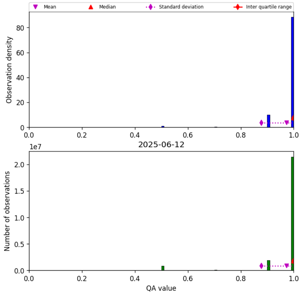
Figure 29: Histogram of “QA value” for 2025-06-11 to 2025-06-13
