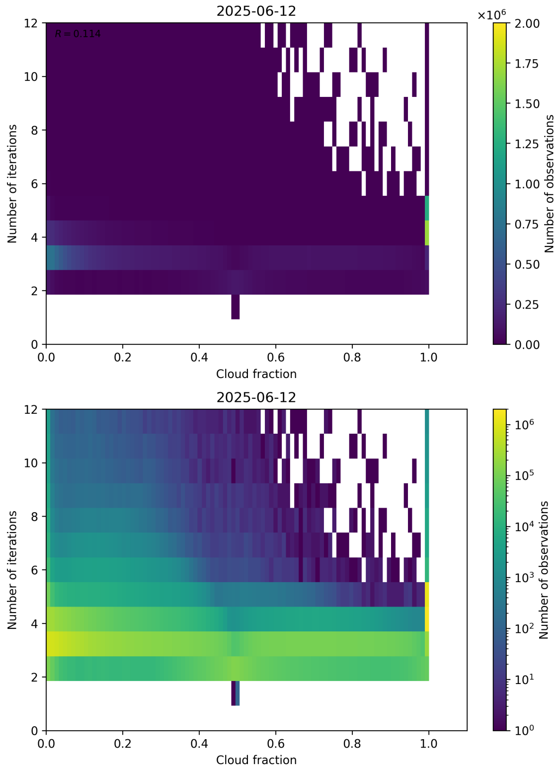
Figure 73: Scatter density plot of “Cloud fraction” against “Number of iterations” for 2025-06-11 to 2025-06-13.
