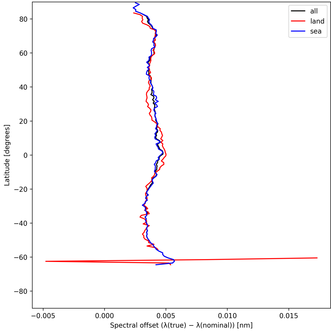
Figure 28: Zonal average of “Spectral offset ( \lambda_{\text{true}} - \lambda_{\text{nominal}} )” for 2025-06-11 to 2025-06-13.
