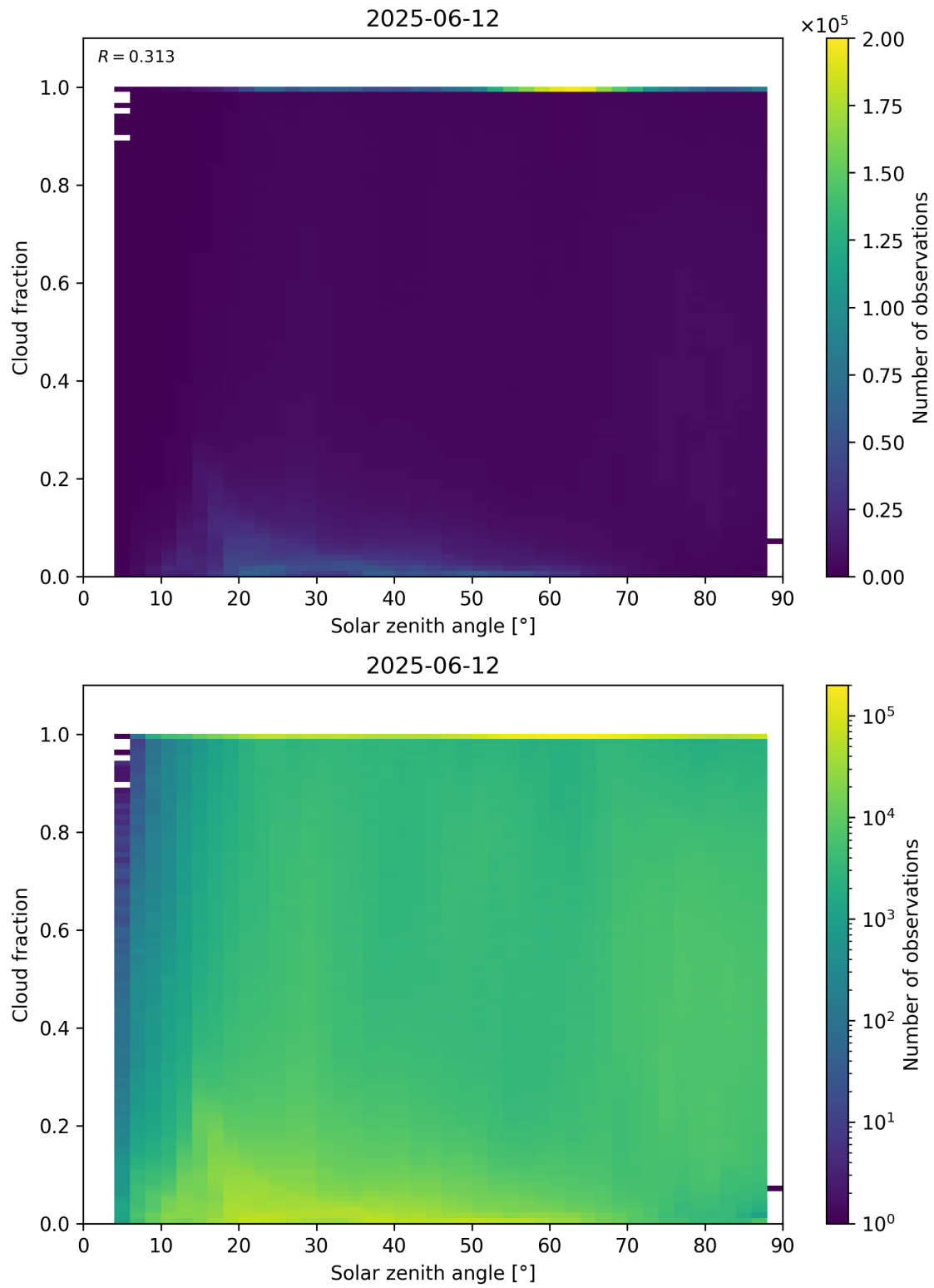
Figure 110: Scatter density plot of “Solar zenith angle” against “Cloud fraction” for 2025-06-11 to 2025-06-13.
