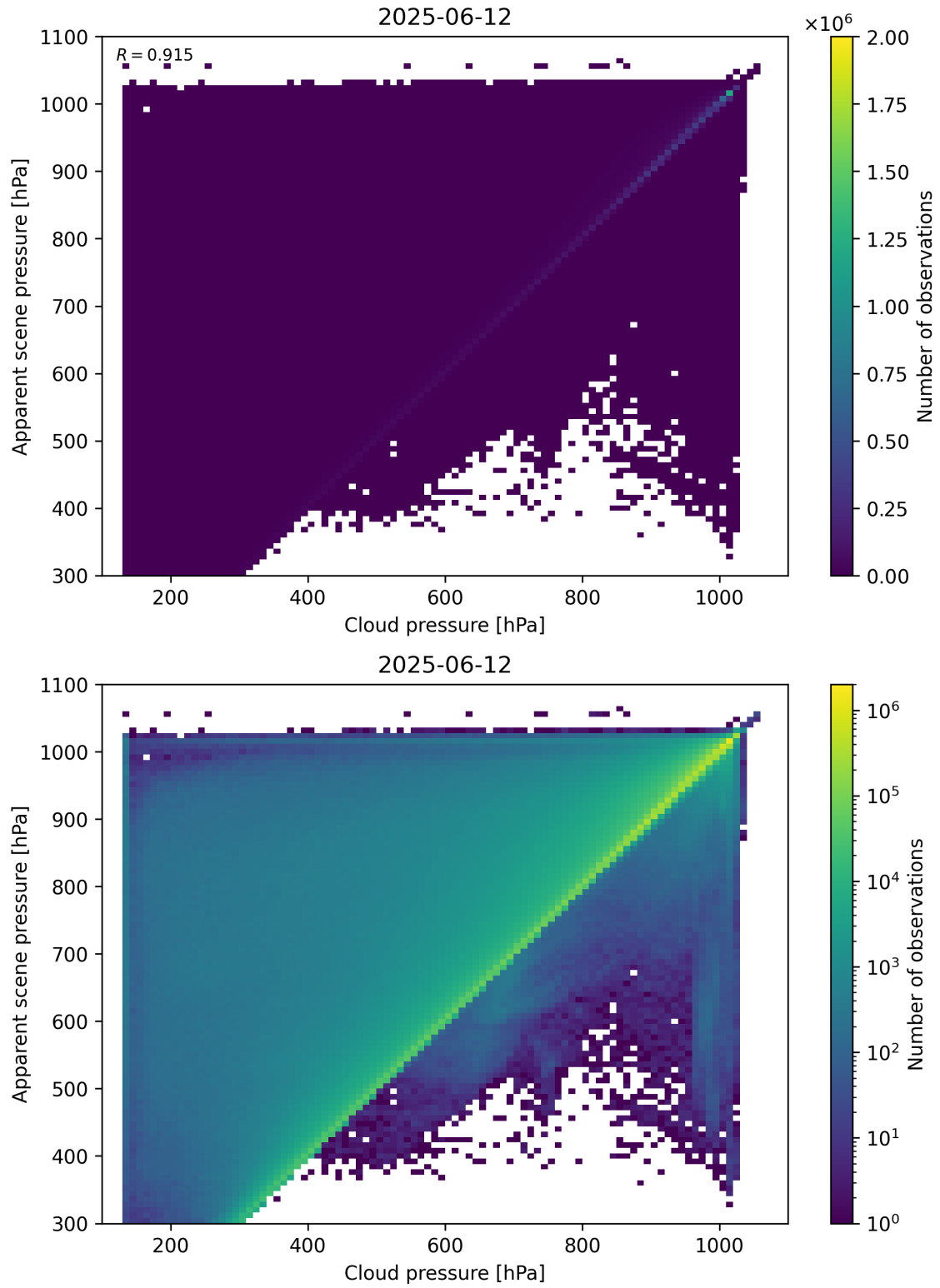
Figure 77: Scatter density plot of “Cloud pressure” against “Apparent scene pressure” for 2025-06-11 to 2025-06-13.
