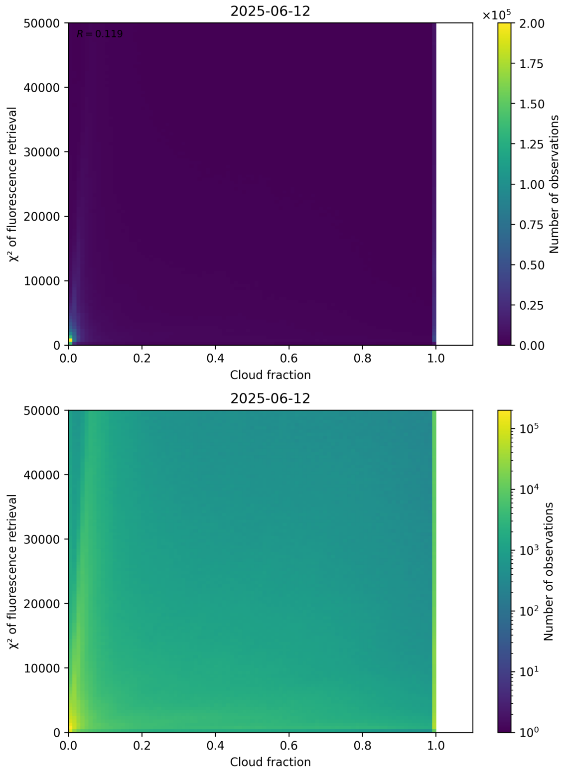
Figure 71: Scatter density plot of “Cloud fraction” against “ \chi^2 of fluorescence retrieval” for 2025-06-11 to 2025-06-13.
