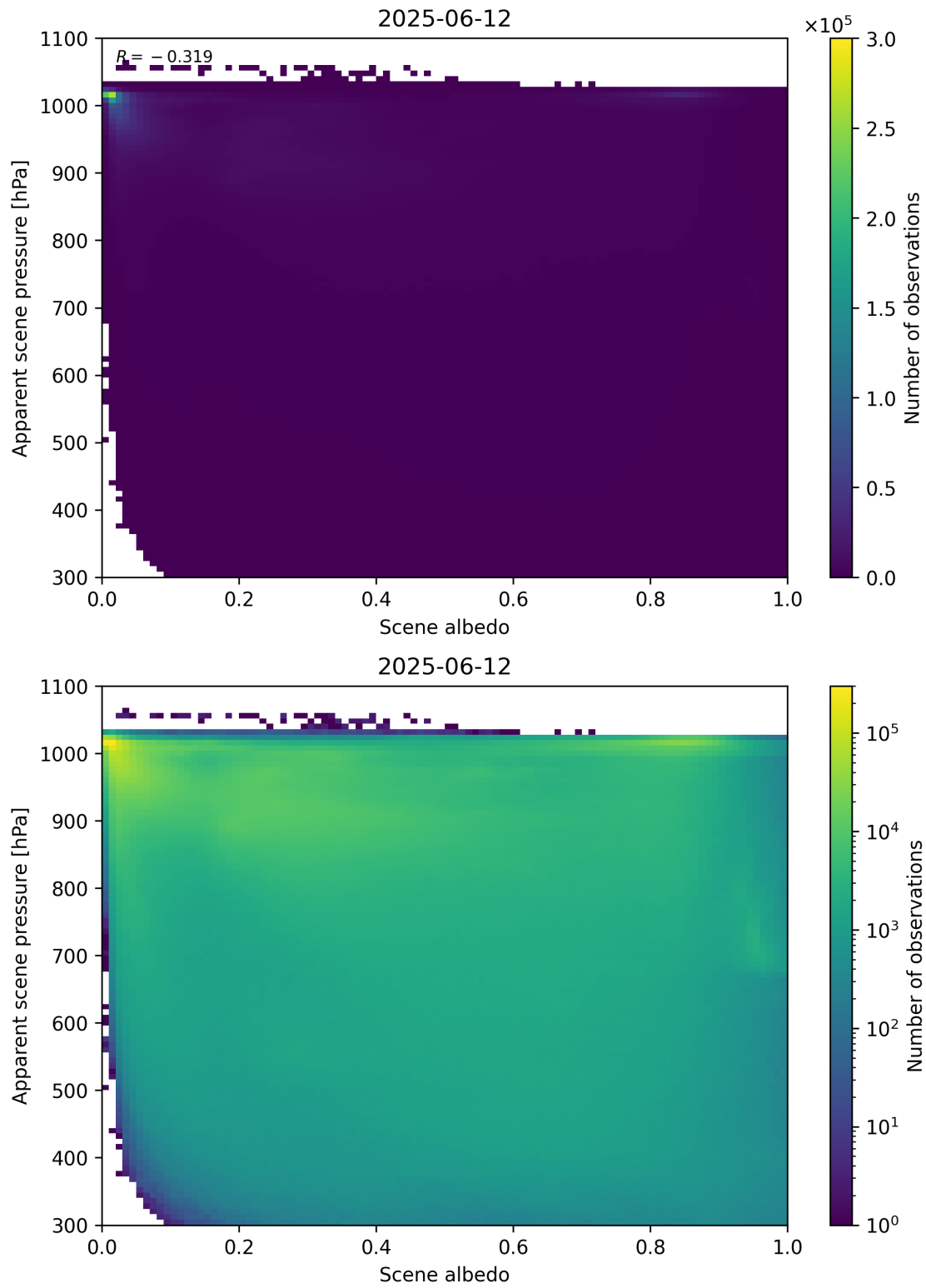
Figure 102: Scatter density plot of “Scene albedo” against “Apparent scene pressure” for 2025-06-11 to 2025-06-13.
