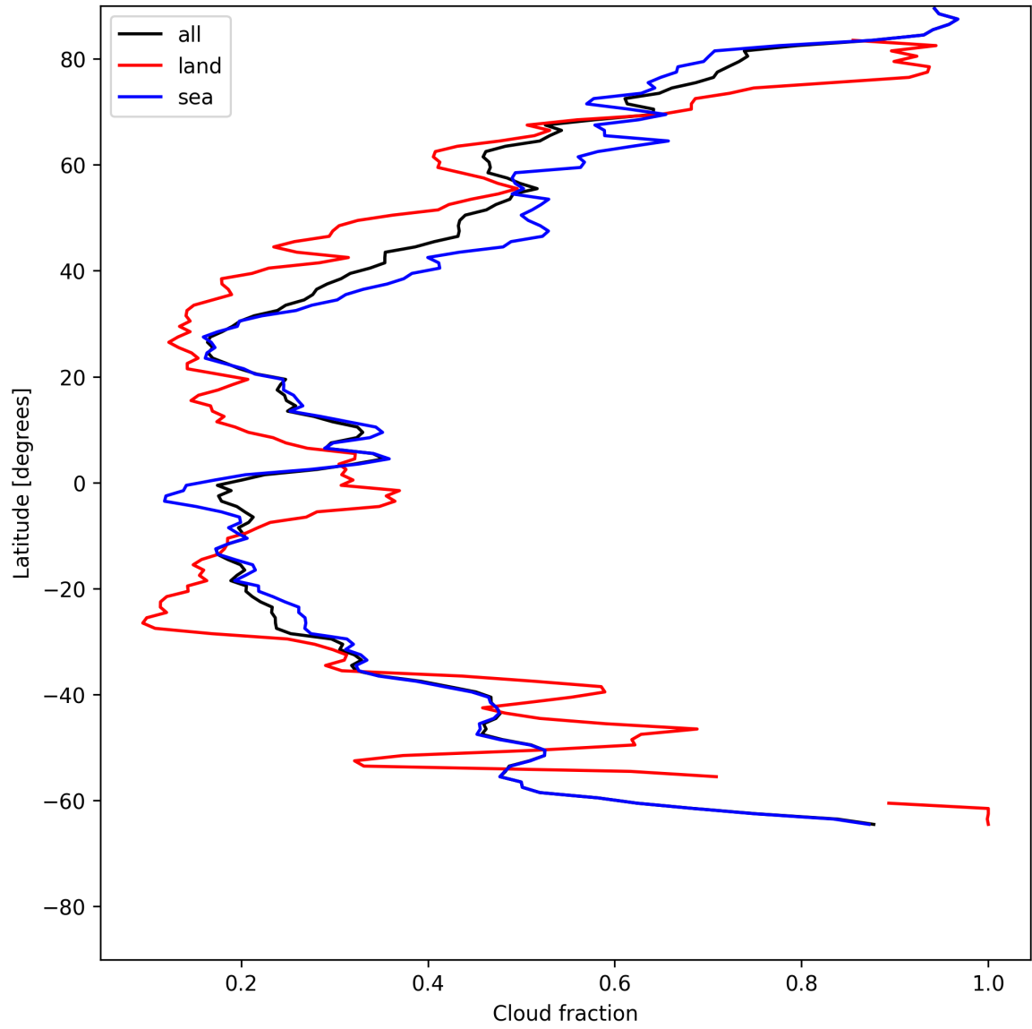
Figure 15: Zonal average of “Cloud fraction” for 2025-06-11 to 2025-06-13.
