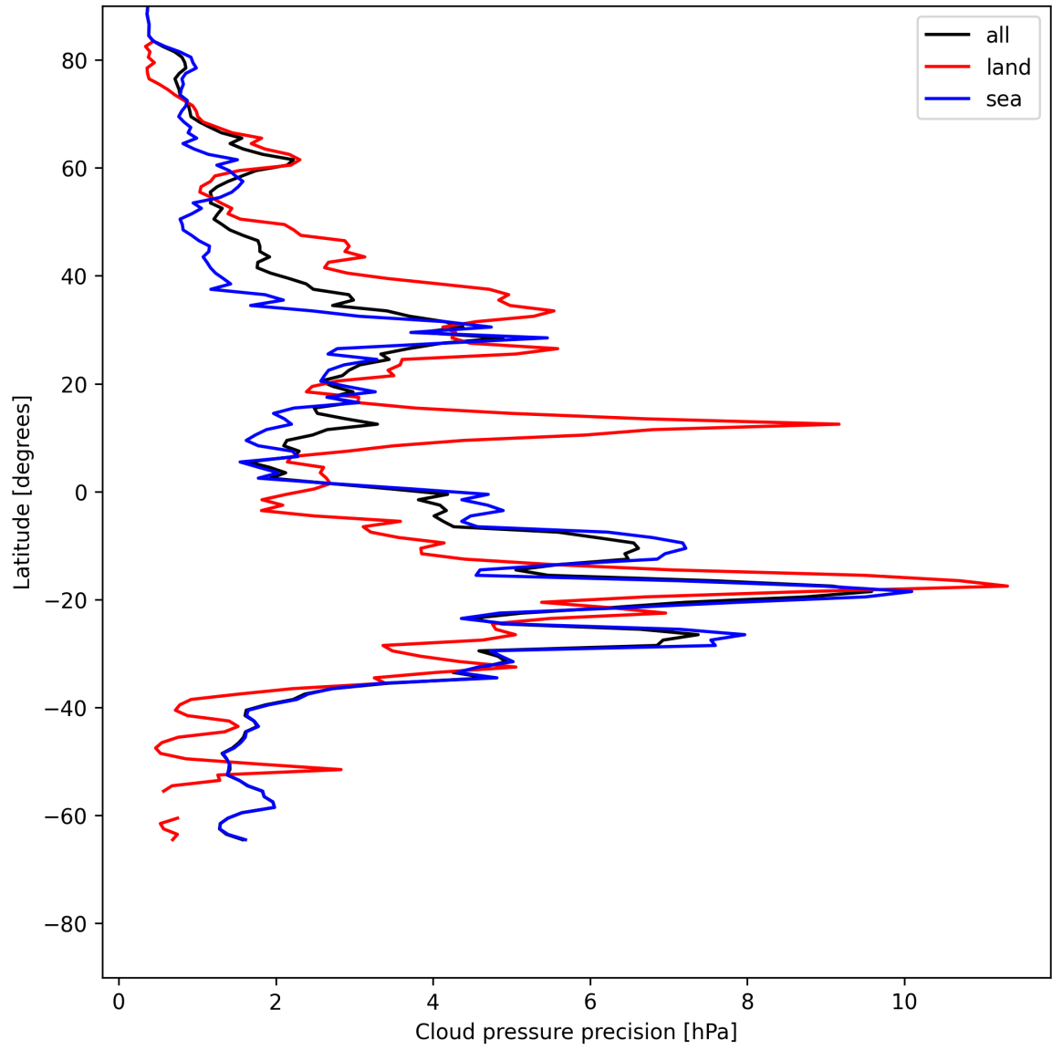
Figure 14: Zonal average of “Cloud pressure precision” for 2025-06-11 to 2025-06-13.
