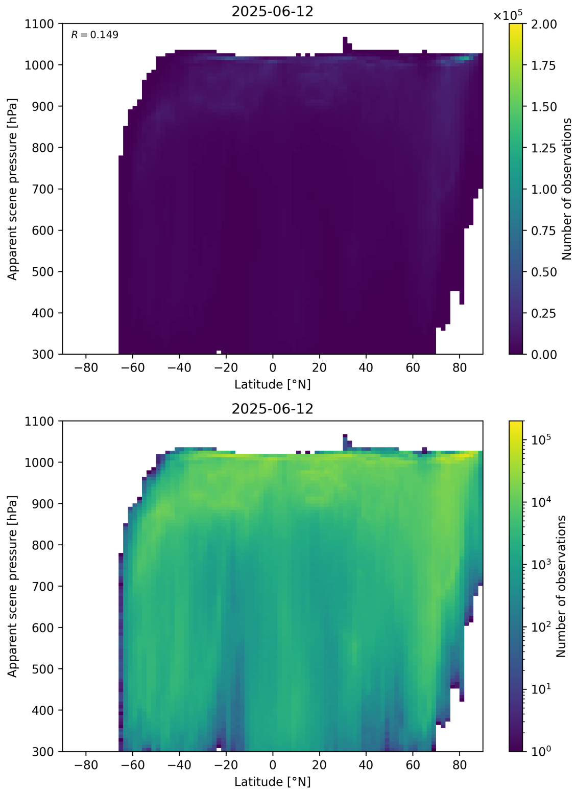
Figure 88: Scatter density plot of “Latitude” against “Apparent scene pressure” for 2025-06-11 to 2025-06-13.
