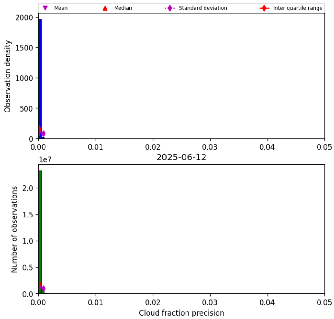
Figure 33: Histogram of “Cloud fraction precision” for 2025-06-11 to 2025-06-13
