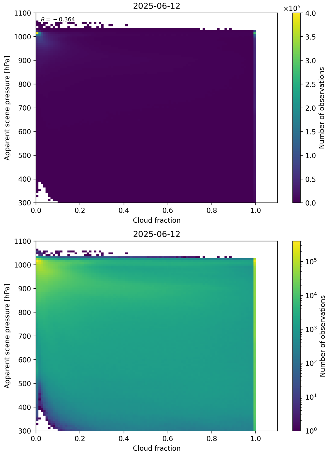
Figure 70: Scatter density plot of “Cloud fraction” against “Apparent scene pressure” for 2025-06-11 to 2025-06-13.
