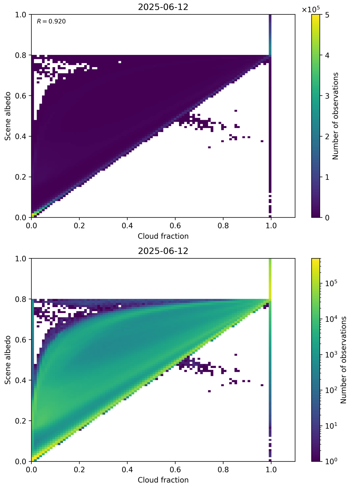
Figure 75: Scatter density plot of “Cloud fraction” against “Scene albedo” for 2025-06-11 to 2025-06-13.
