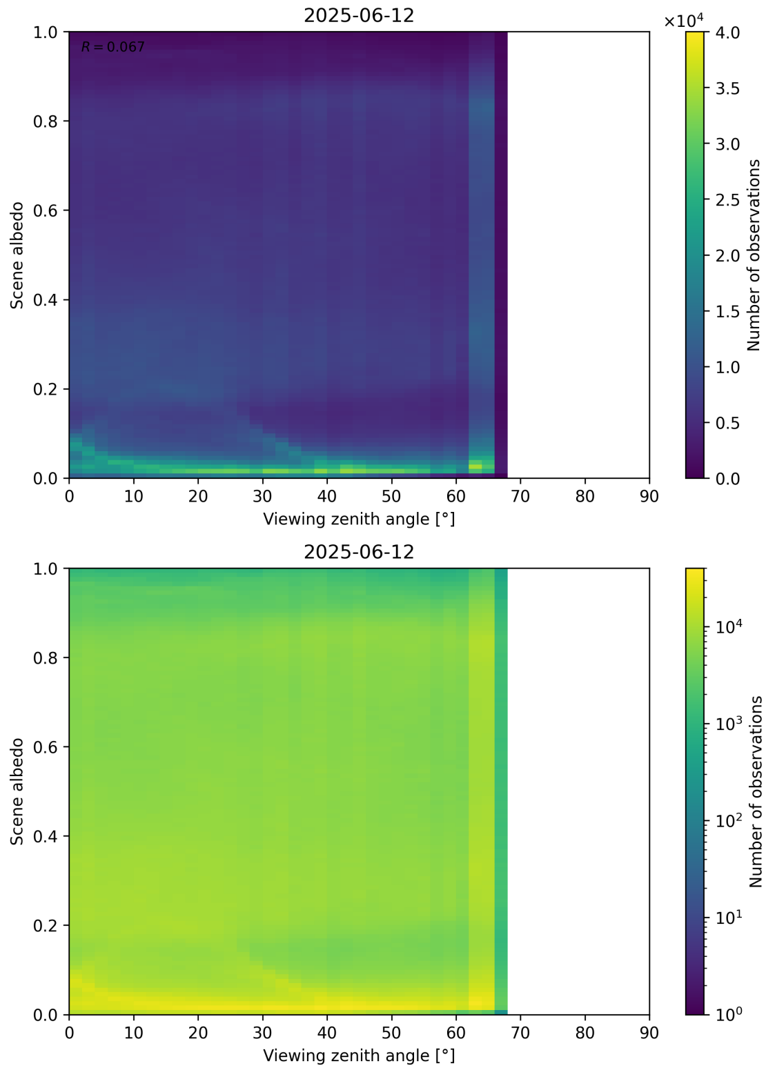
Figure 126: Scatter density plot of “Viewing zenith angle” against “Scene albedo” for 2025-06-11 to 2025-06-13.
