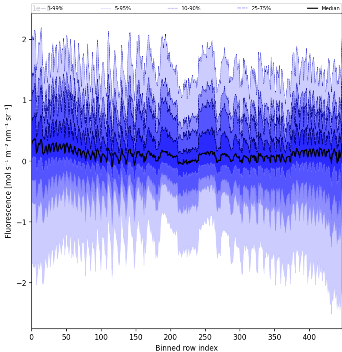
Figure 57: Along track statistics of “Fluorescence” for 2025-06-11 to 2025-06-13
