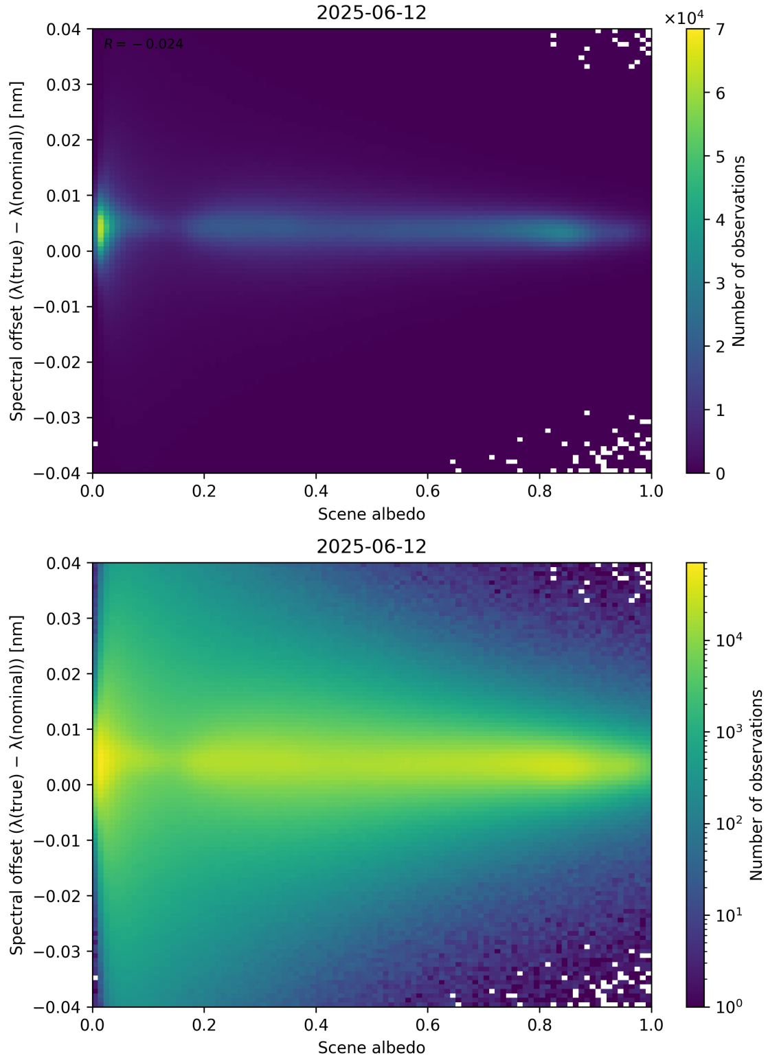
Figure 107: Scatter density plot of “Scene albedo” against “Spectral offset ( \lambda_{\text{true}} - \lambda_{\text{nominal}} )” for 2025-06-11 to 2025-06-13.
