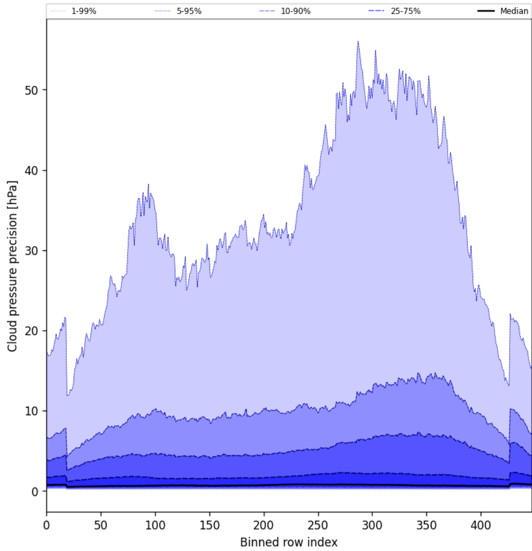
Figure 48: Along track statistics of “Cloud pressure precision” for 2025-06-11 to 2025-06-13
