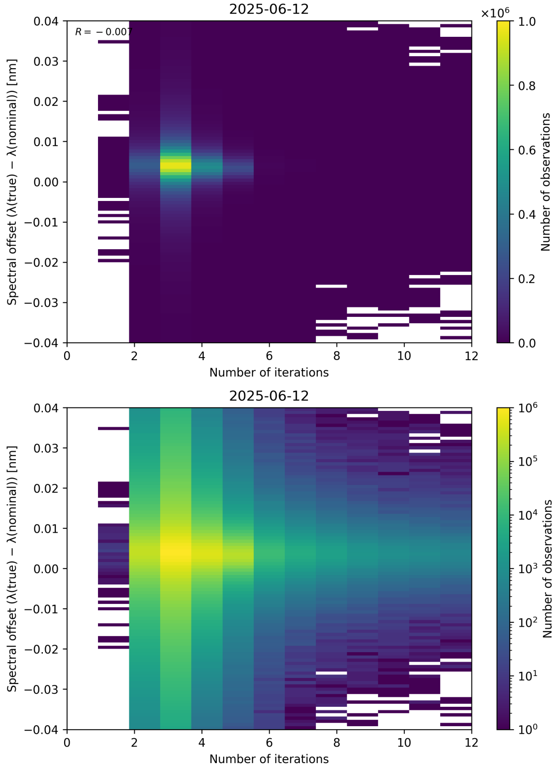
Figure 100: Scatter density plot of “Number of iterations” against “Spectral offset ( \lambda_{\text{true}} - \lambda_{\text{nominal}} )” for 2025-06-11 to 2025-06-13.
