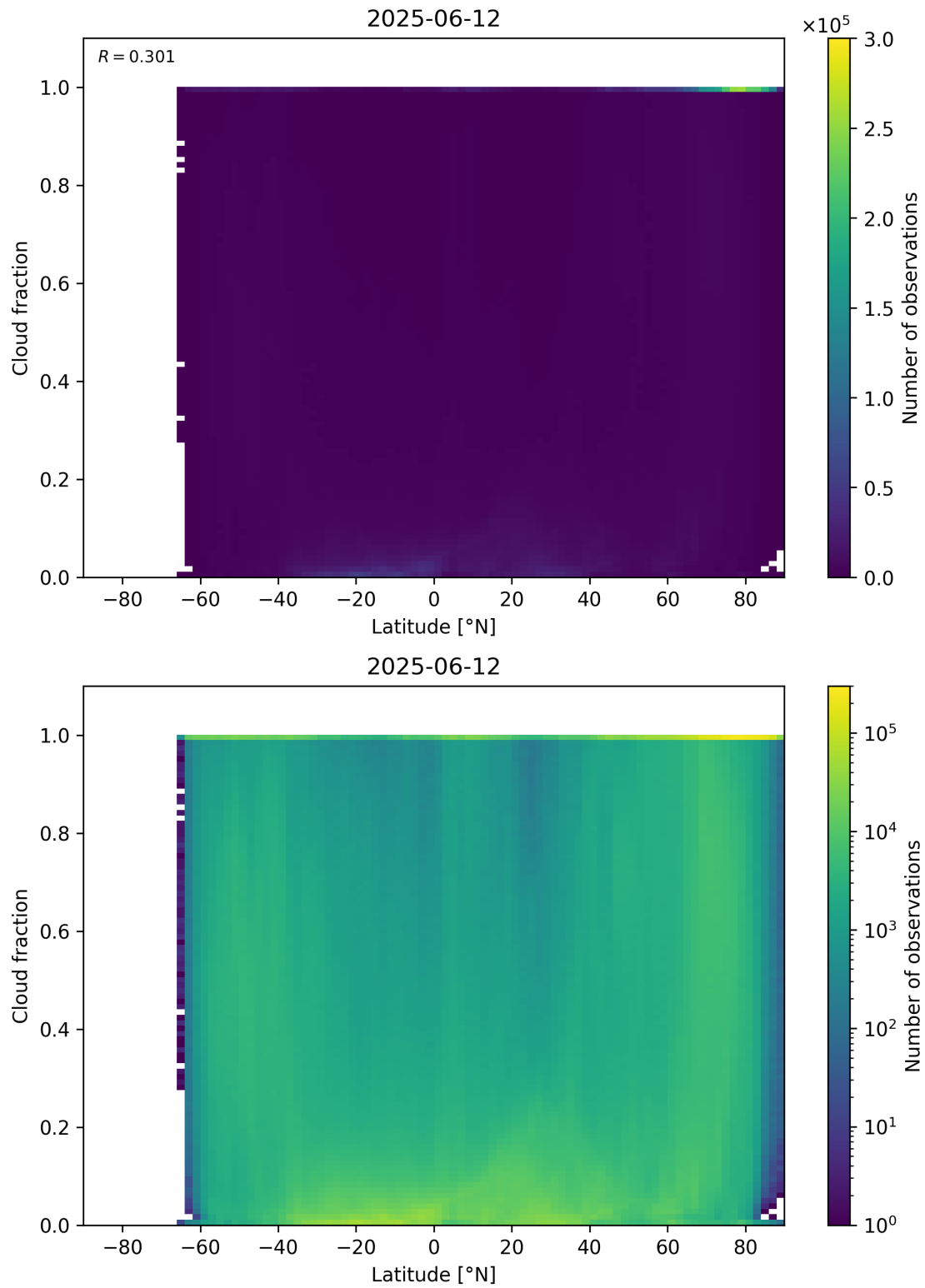
Figure 90: Scatter density plot of “Latitude” against “Cloud fraction” for 2025-06-11 to 2025-06-13.
