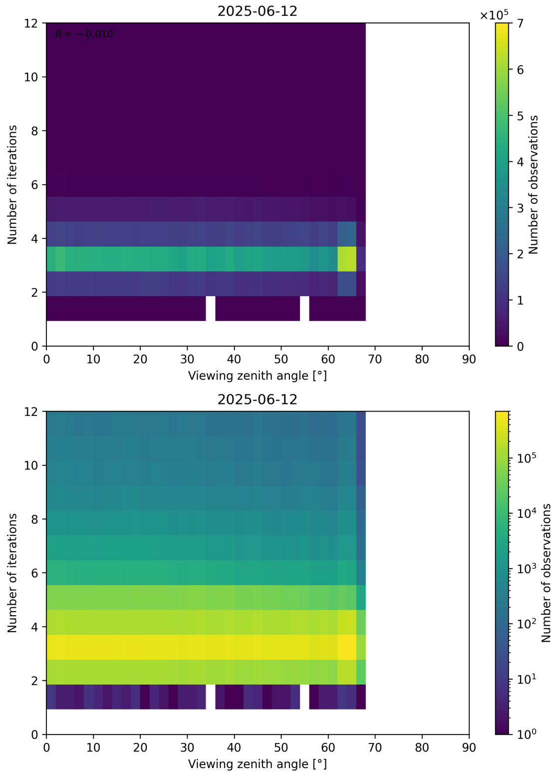
Figure 124: Scatter density plot of “Viewing zenith angle” against “Number of iterations” for 2025-06-11 to 2025-06-13.
