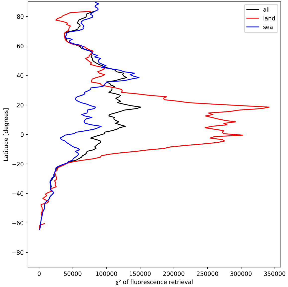
Figure 25: Zonal average of “ \chi^2 of fluorescence retrieval” for 2025-06-11 to 2025-06-13.
