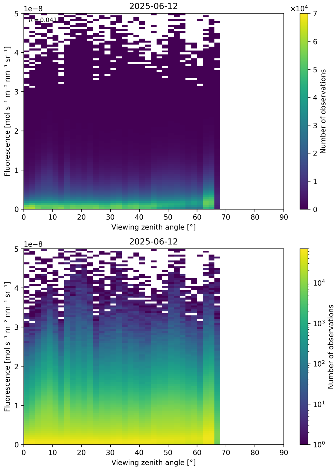
Figure 122: Scatter density plot of “Viewing zenith angle” against “Fluorescence” for 2025-06-11 to 2025-06-13.
