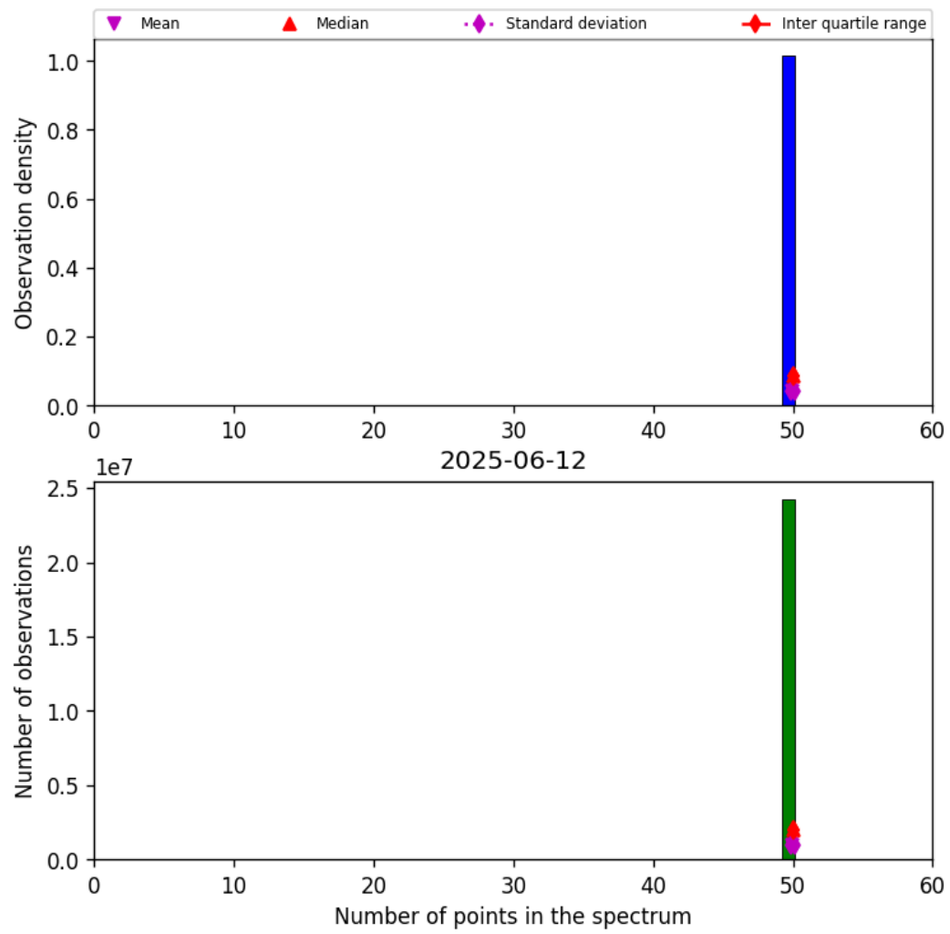
Figure 44: Histogram of “Number of points in the spectrum” for 2025-06-11 to 2025-06-13
