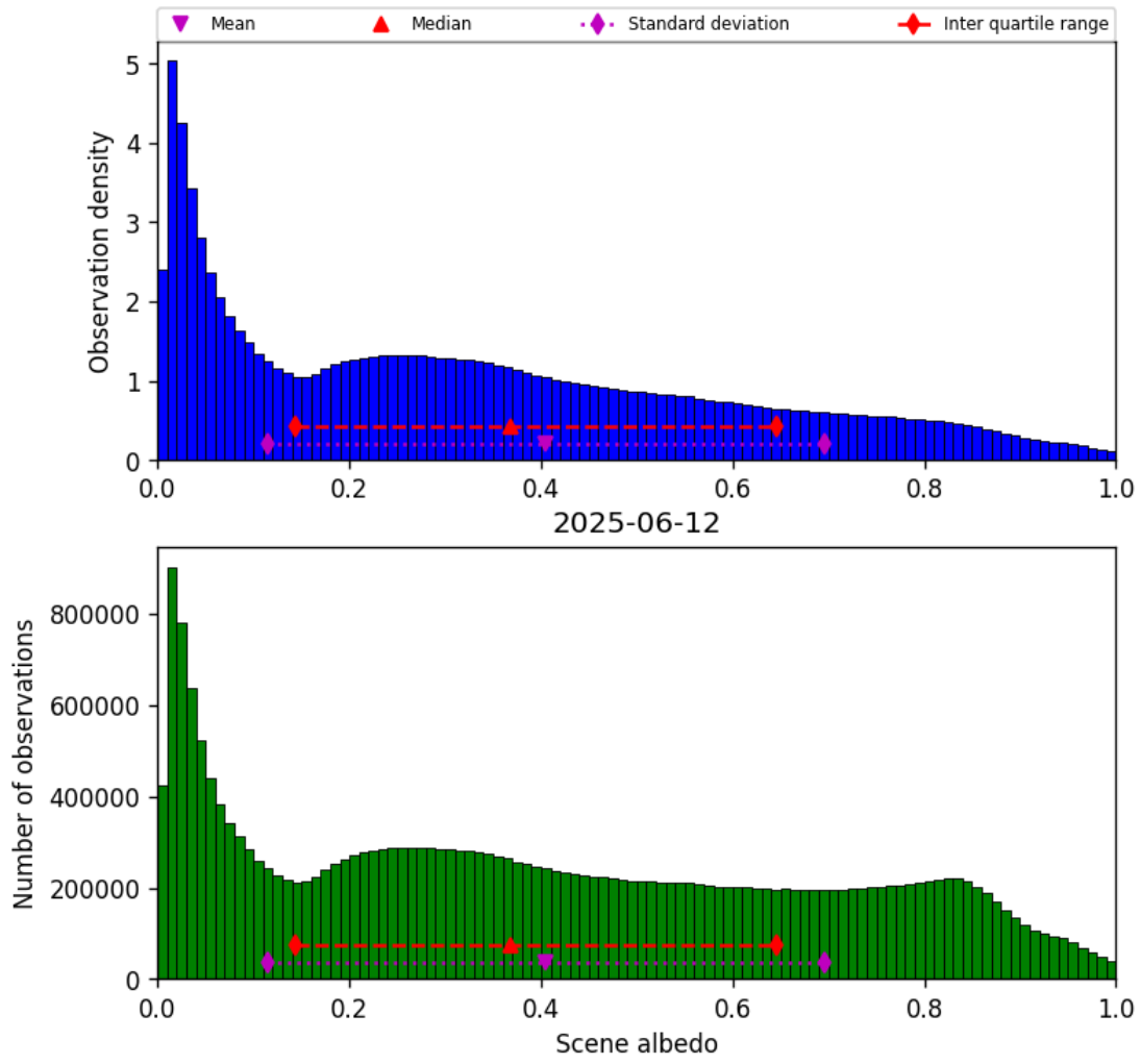
Figure 34: Histogram of “Scene albedo” for 2025-06-11 to 2025-06-13
