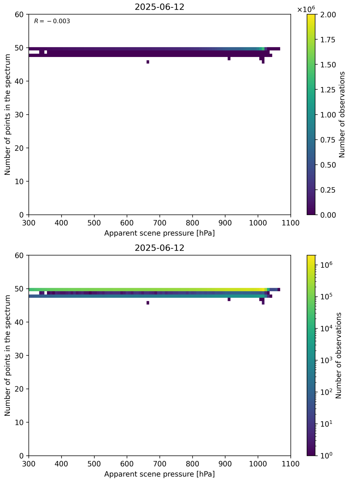
Figure 66: Scatter density plot of “Apparent scene pressure” against “Number of points in the spectrum” for 2025-06-11 to 2025-06-13.
