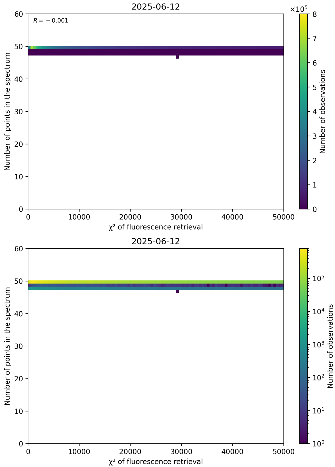
Figure 68: Scatter density plot of " \chi^2 of fluorescence retrieval" against "Number of points in the spectrum" for 2025-06-11 to 2025-06-13.
