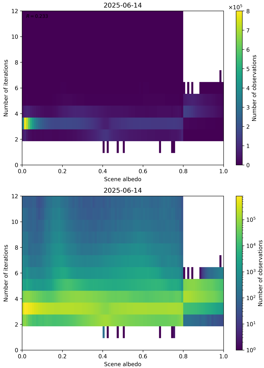
Figure 105: Scatter density plot of “Scene albedo” against “Number of iterations” for 2025-06-13 to 2025-06-15.
