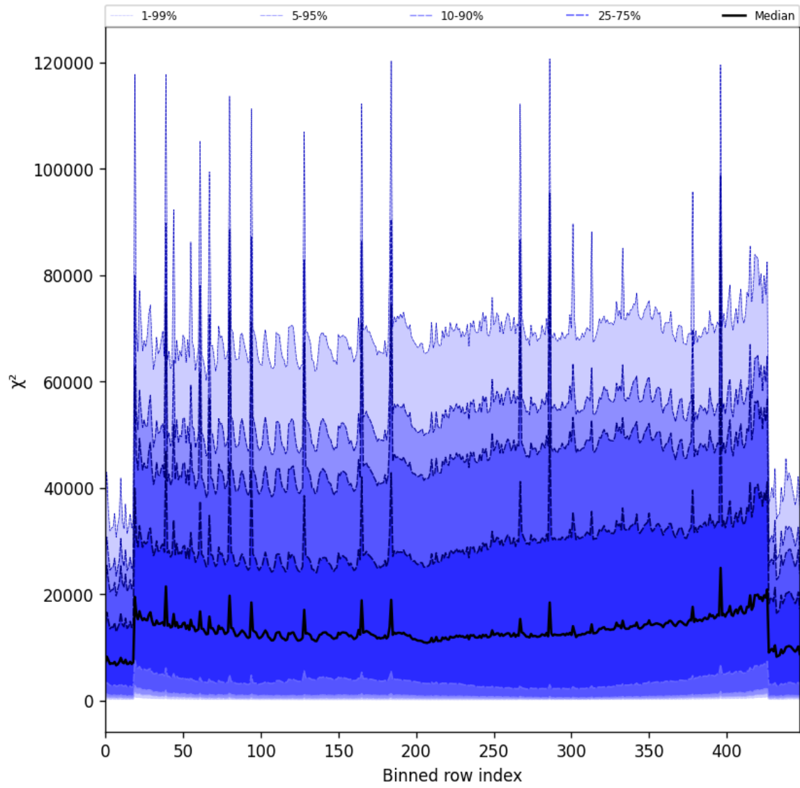
Figure 55: Along track statistics of “ \chi^2 ” for 2025-06-13 to 2025-06-15
