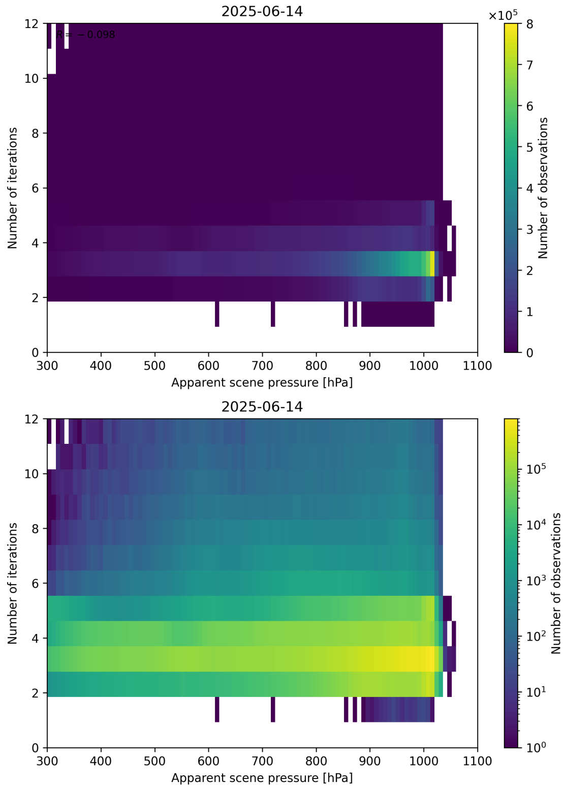
Figure 65: Scatter density plot of “Apparent scene pressure” against “Number of iterations” for 2025-06-13 to 2025-06-15.
