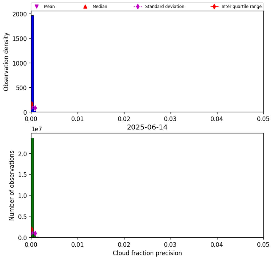
Figure 33: Histogram of “Cloud fraction precision” for 2025-06-13 to 2025-06-15
