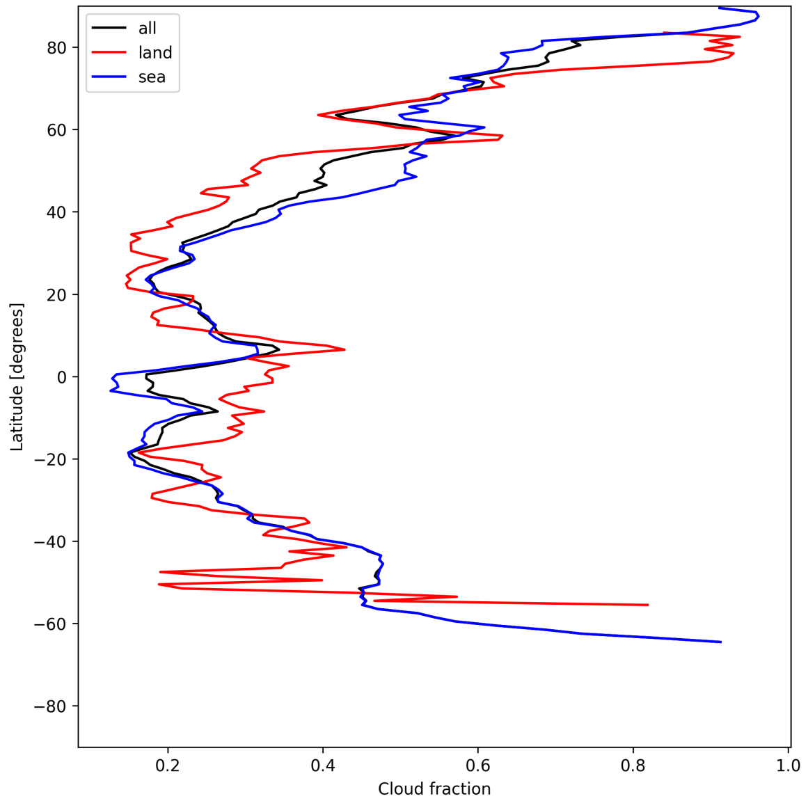
Figure 15: Zonal average of “Cloud fraction” for 2025-06-13 to 2025-06-15.
