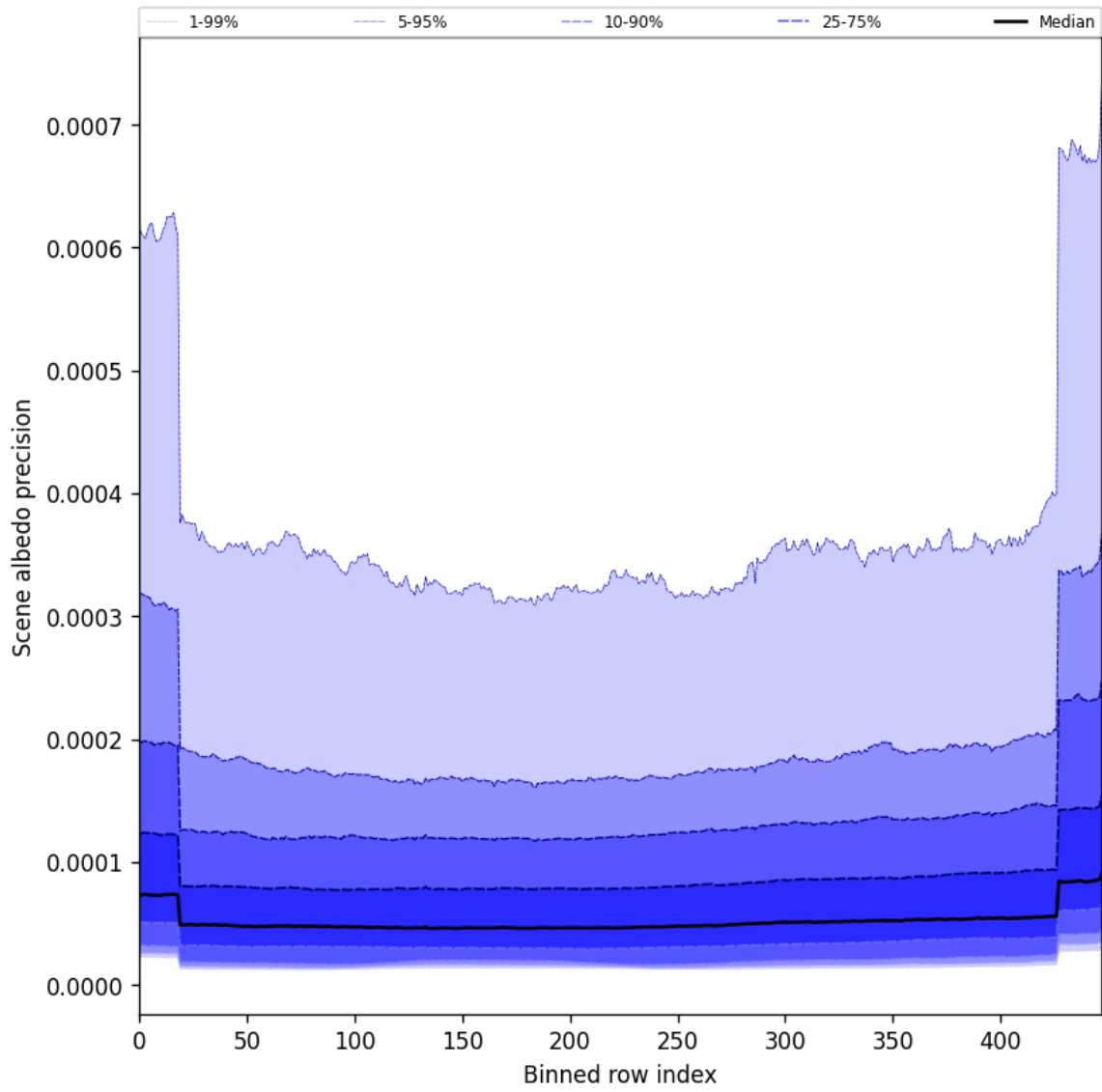
Figure 52: Along track statistics of “Scene albedo precision” for 2025-06-13 to 2025-06-15
