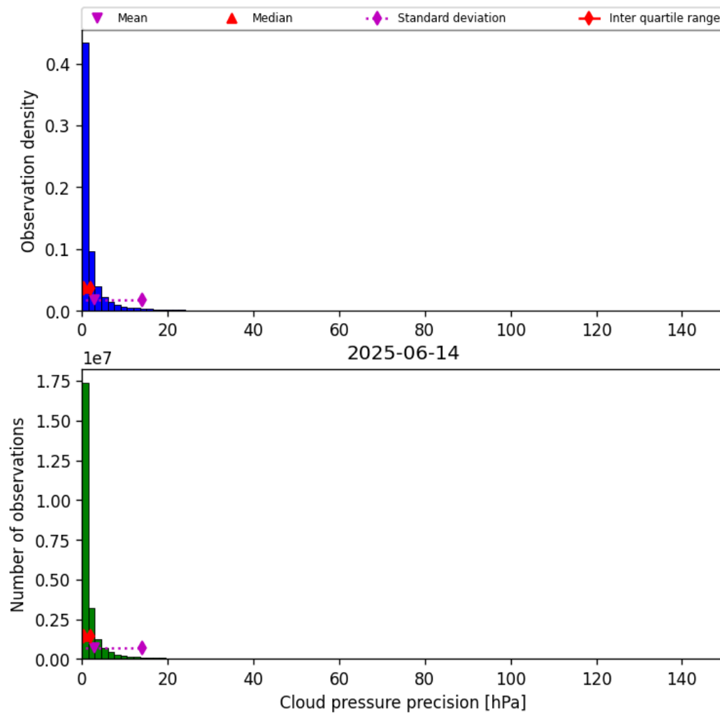
Figure 31: Histogram of “Cloud pressure precision” for 2025-06-13 to 2025-06-15
