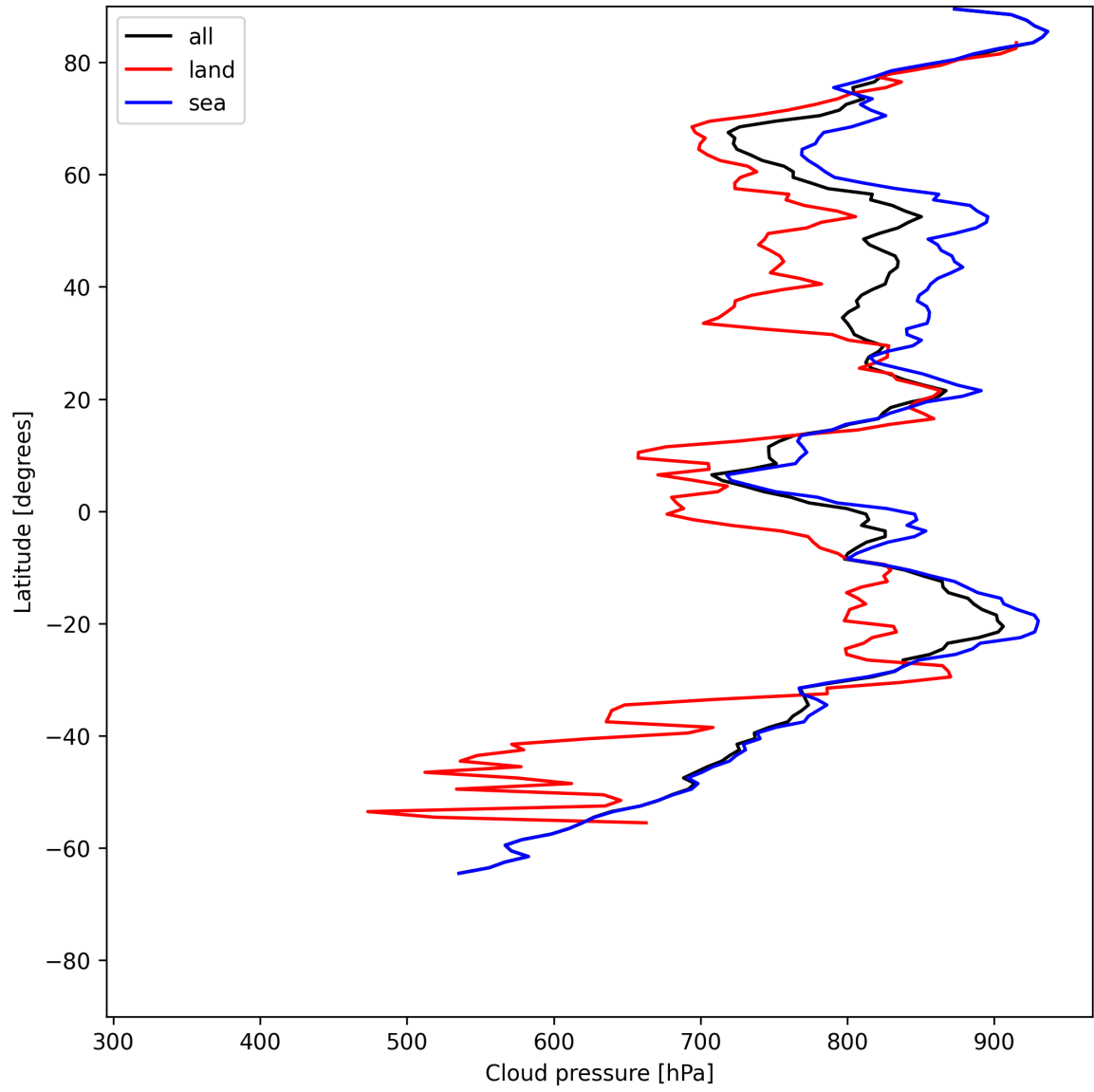
Figure 13: Zonal average of “Cloud pressure” for 2025-06-13 to 2025-06-15.
