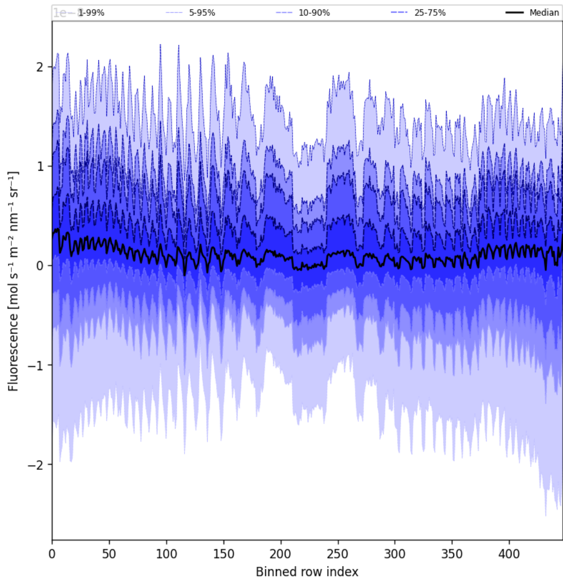
Figure 57: Along track statistics of “Fluorescence” for 2025-06-13 to 2025-06-15
