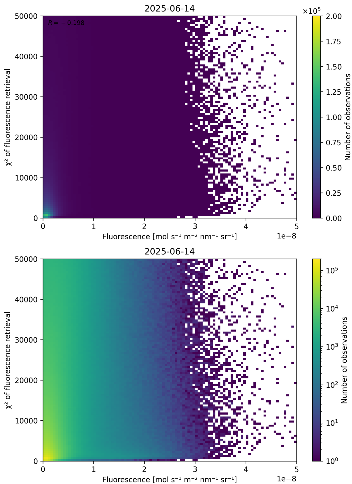
Figure 85: Scatter density plot of “Fluorescence” against “ \chi^2 of fluorescence retrieval” for 2025-06-13 to 2025-06-15.
