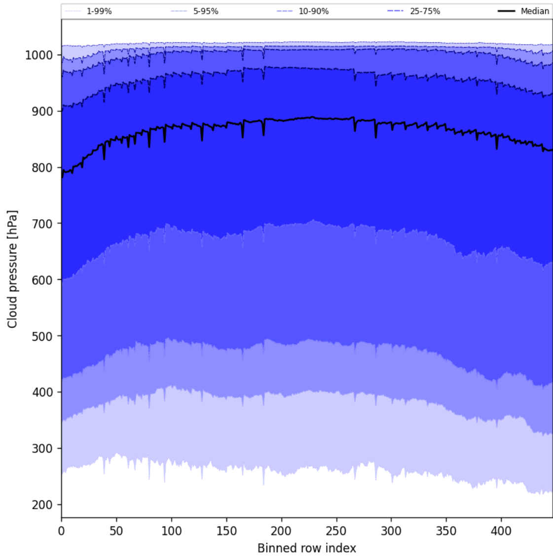
Figure 47: Along track statistics of “Cloud pressure” for 2025-06-13 to 2025-06-15
