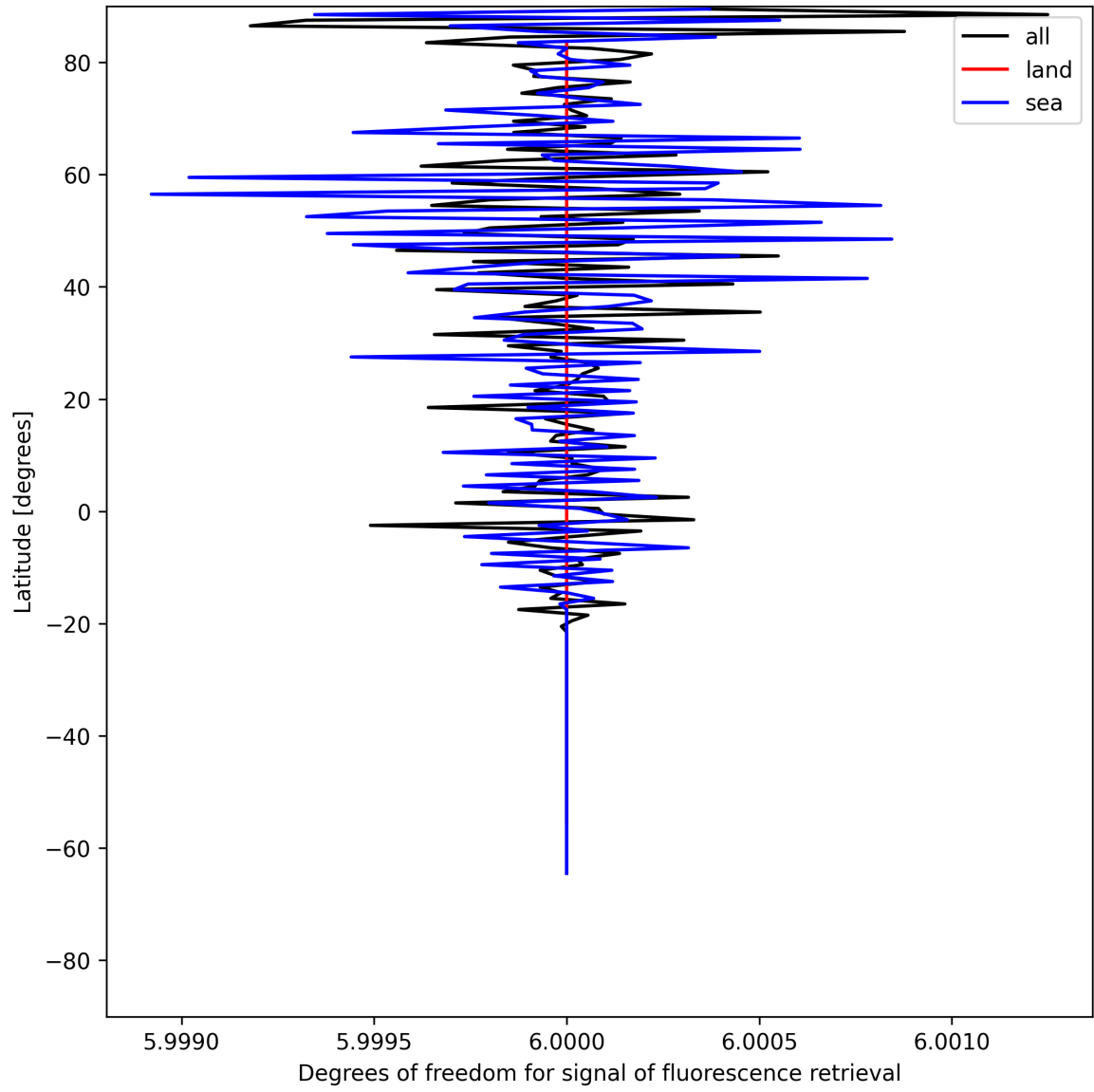
Figure 26: Zonal average of “Degrees of freedom for signal of fluorescence retrieval” for 2025-06-13 to 2025-06-15.
