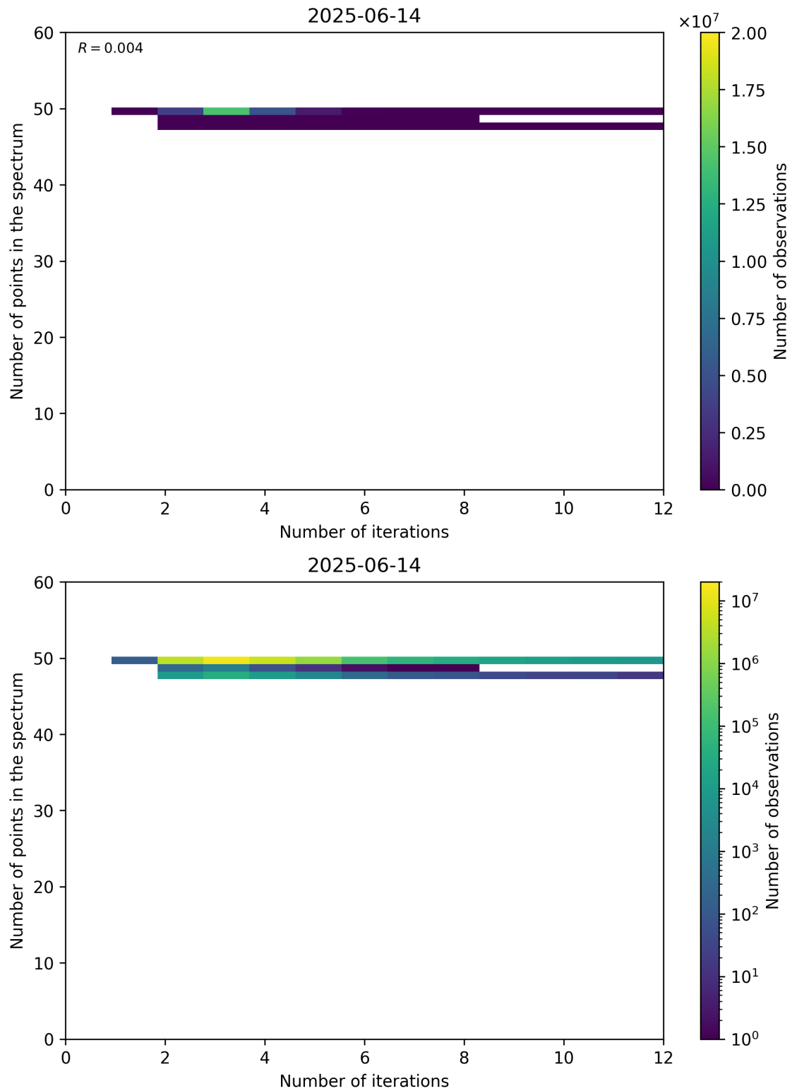
Figure 99: Scatter density plot of “Number of iterations” against “Number of points in the spectrum” for 2025-06-13 to 2025-06-15.
