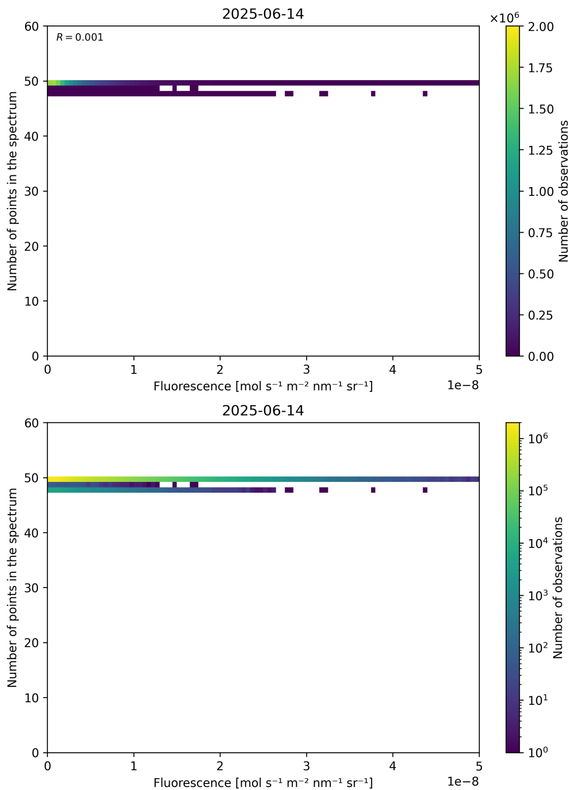
Figure 86: Scatter density plot of “Fluorescence” against “Number of points in the spectrum” for 2025-06-13 to 2025-06-15.
