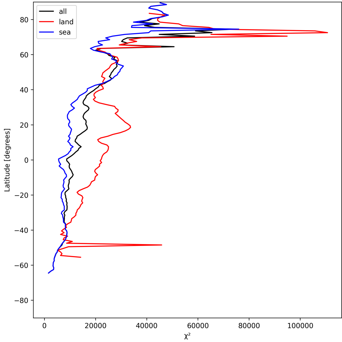
Figure 21: Zonal average of “ \chi^2 ” for 2025-06-13 to 2025-06-15.
