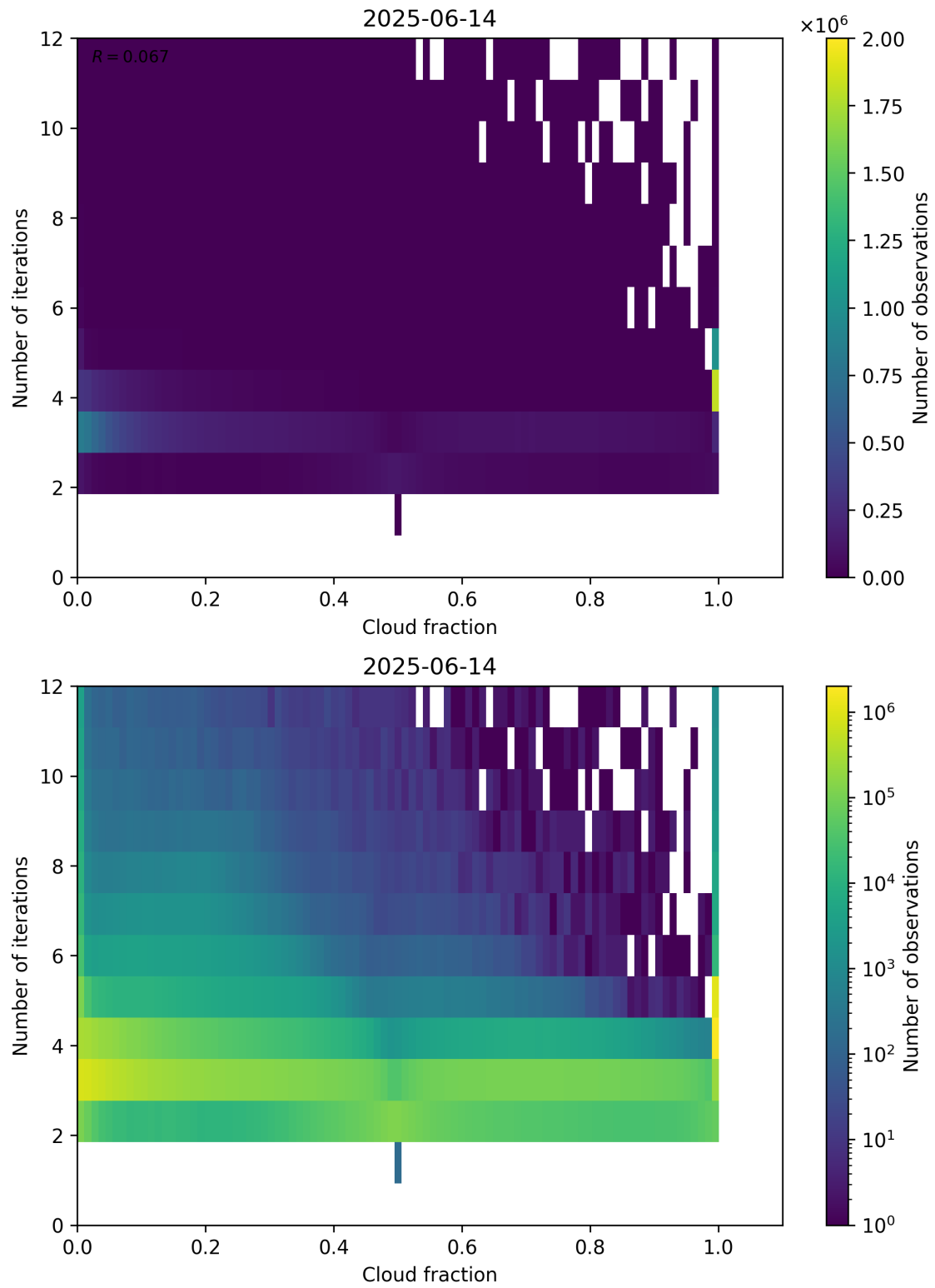
Figure 73: Scatter density plot of “Cloud fraction” against “Number of iterations” for 2025-06-13 to 2025-06-15.
