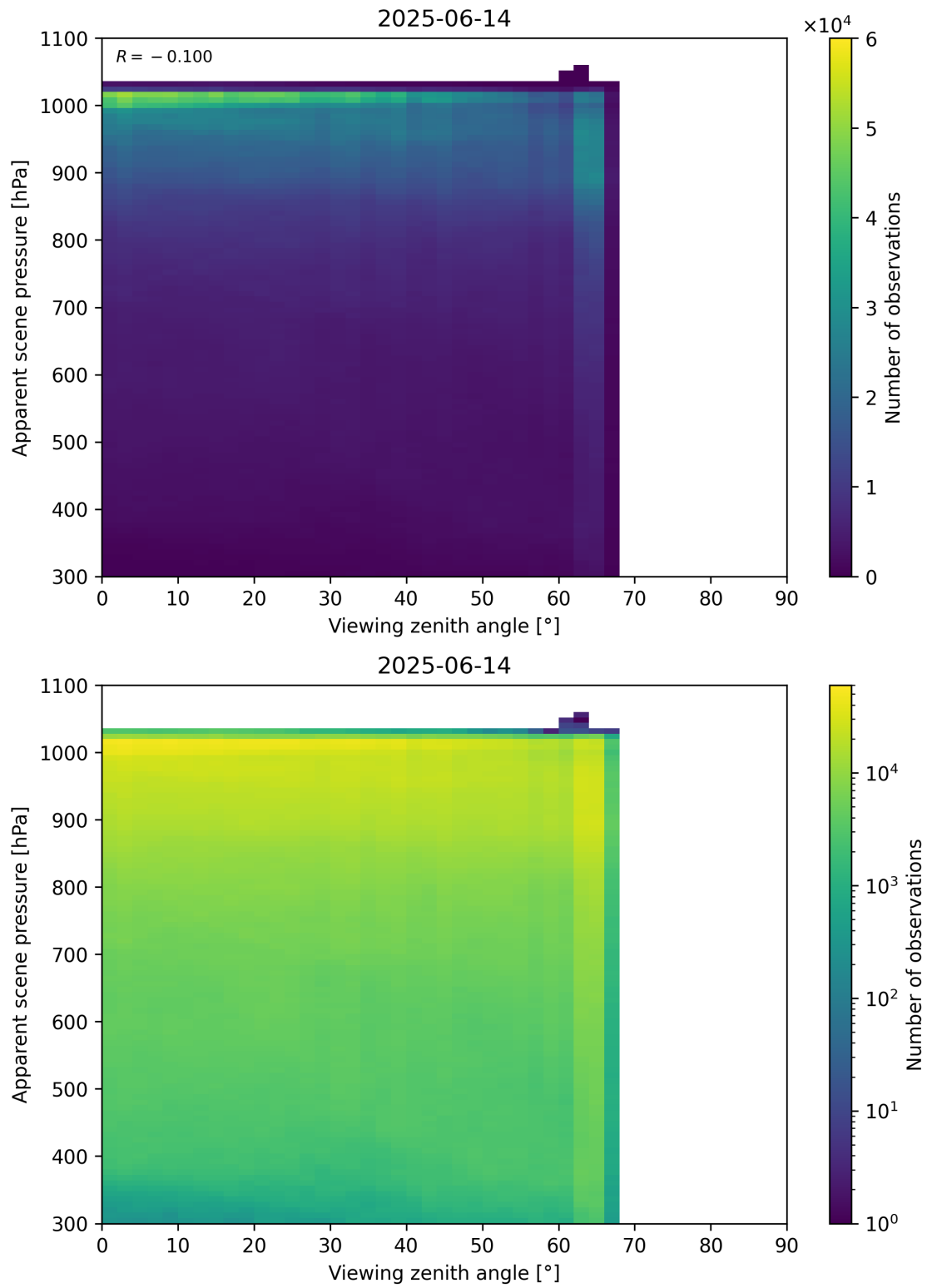
Figure 118: Scatter density plot of “Viewing zenith angle” against “Apparent scene pressure” for 2025-06-13 to 2025-06-15.
