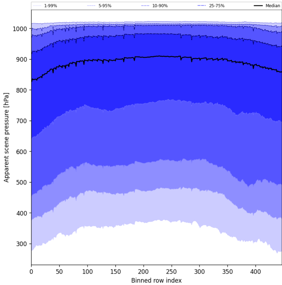
Figure 53: Along track statistics of “Apparent scene pressure” for 2025-06-13 to 2025-06-15
