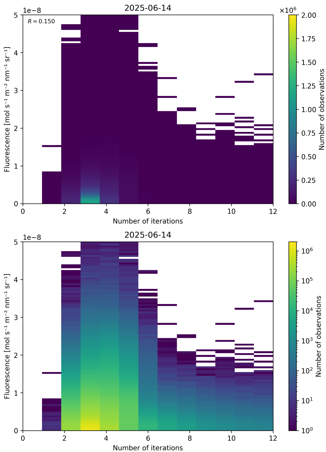
Figure 98: Scatter density plot of “Number of iterations” against “Fluorescence” for 2025-06-13 to 2025-06-15.
