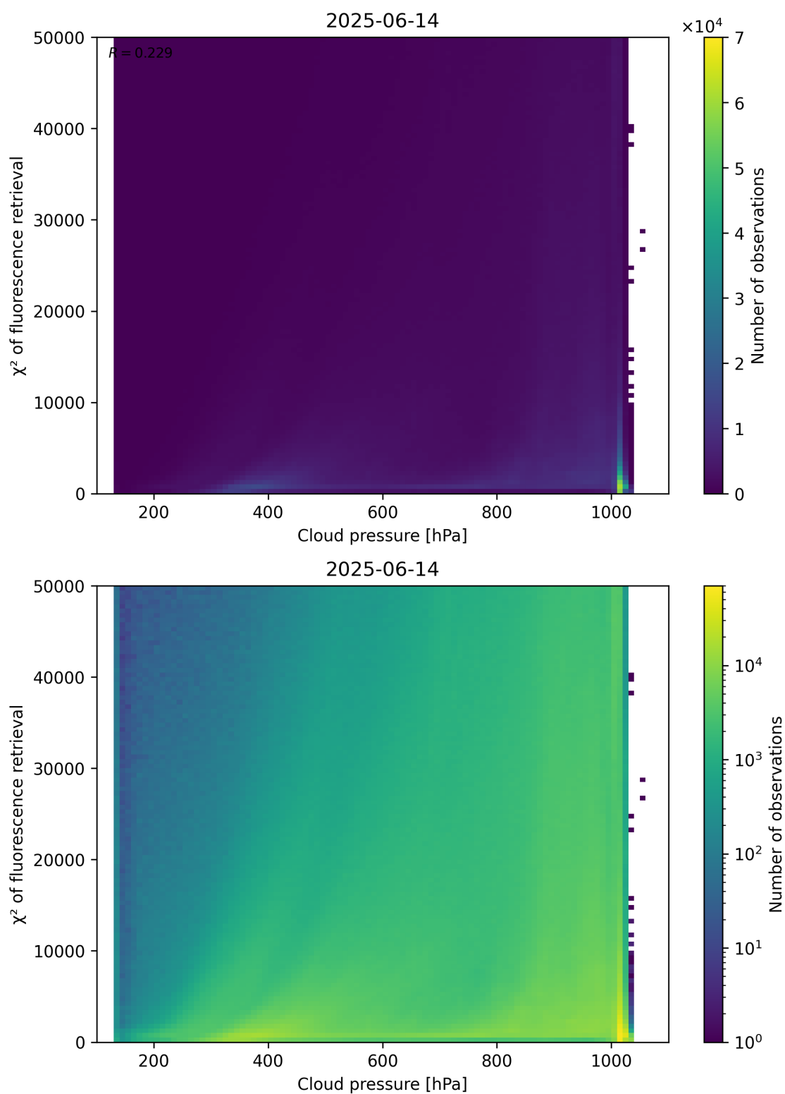
Figure 78: Scatter density plot of “Cloud pressure” against “ \chi^2 of fluorescence retrieval” for 2025-06-13 to 2025-06-15.
