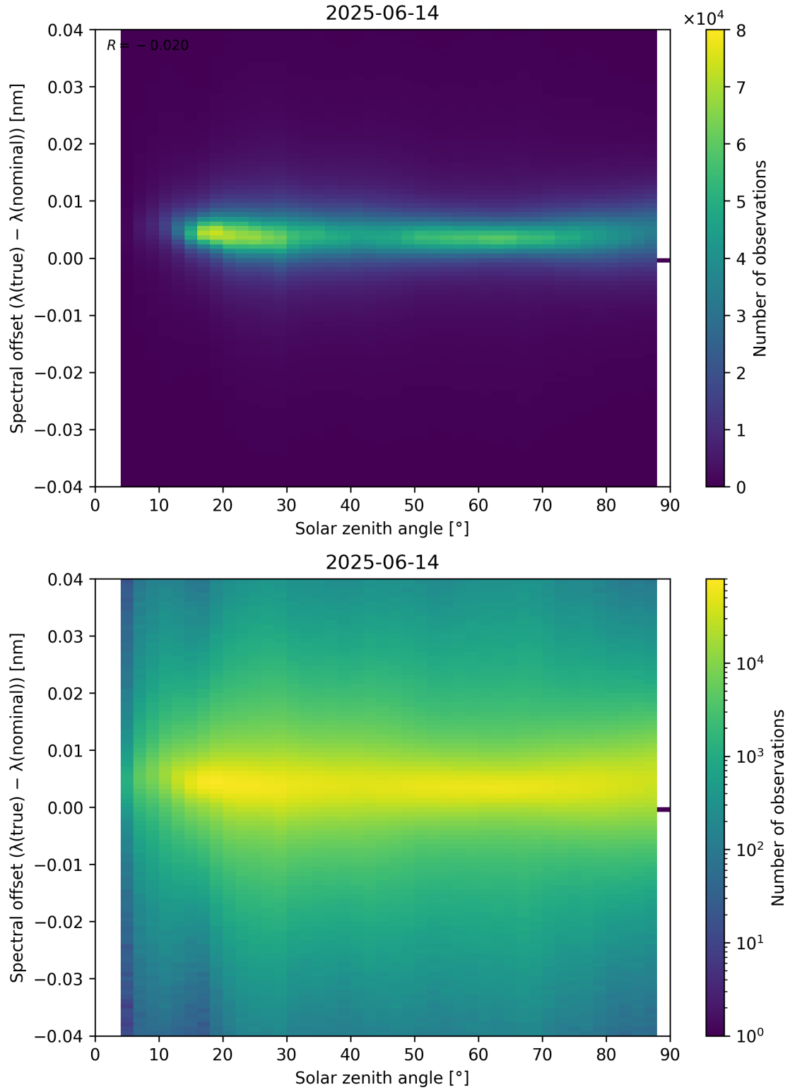
Figure 117: Scatter density plot of “Solar zenith angle” against “Spectral offset ( \lambda_{\text{true}} - \lambda_{\text{nominal}} )” for 2025-06-13 to 2025-06-15.
