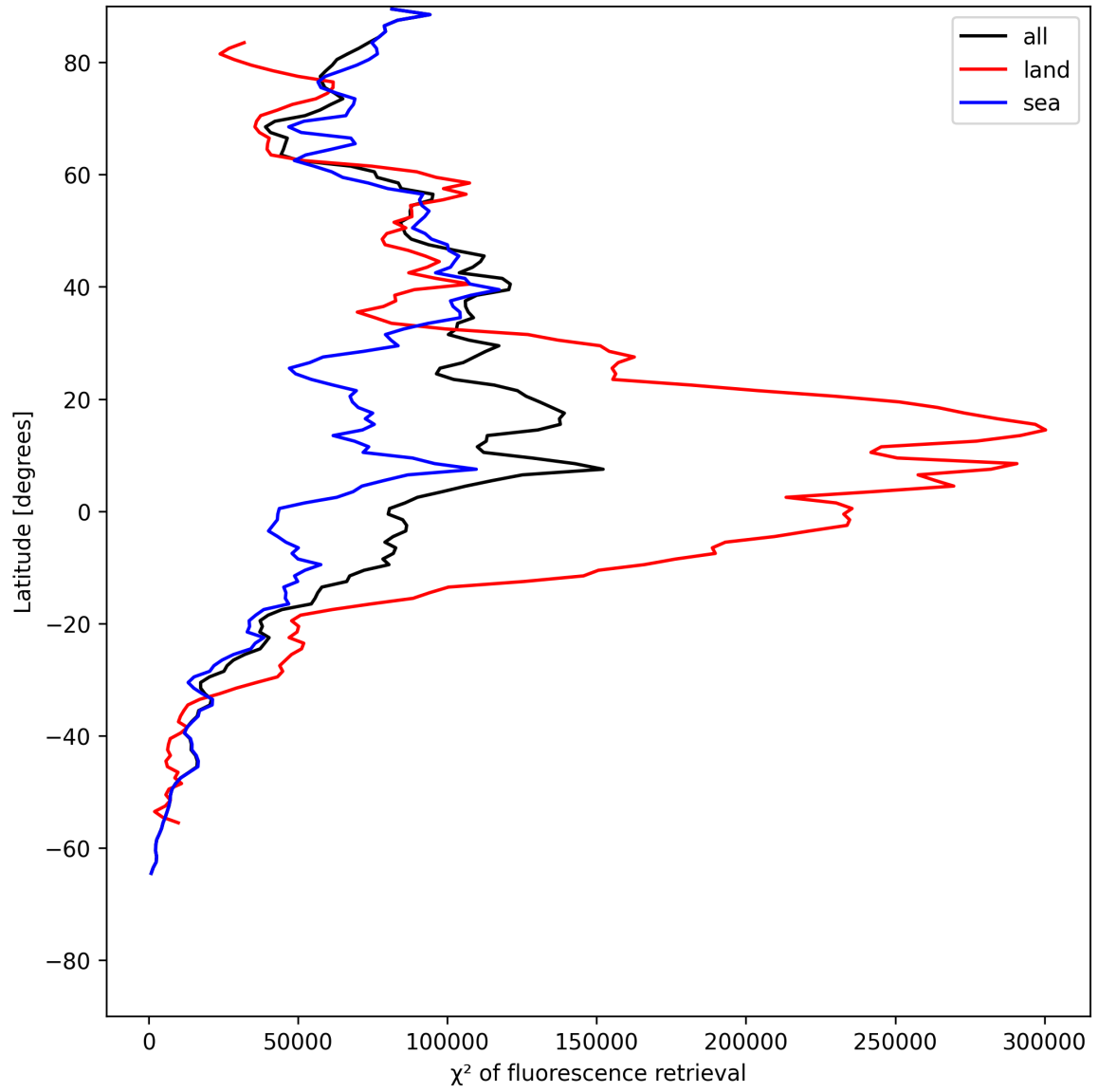
Figure 25: Zonal average of “ \chi^2 of fluorescence retrieval” for 2025-06-13 to 2025-06-15.
