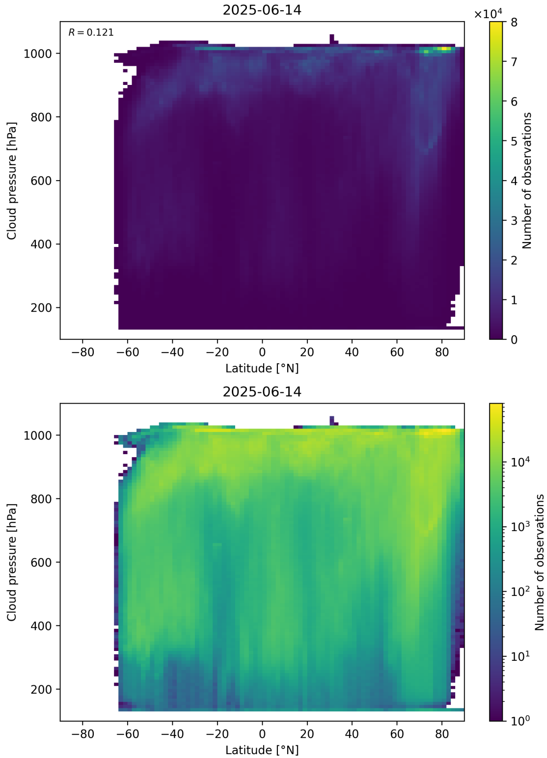
Figure 91: Scatter density plot of “Latitude” against “Cloud pressure” for 2025-06-13 to 2025-06-15.
