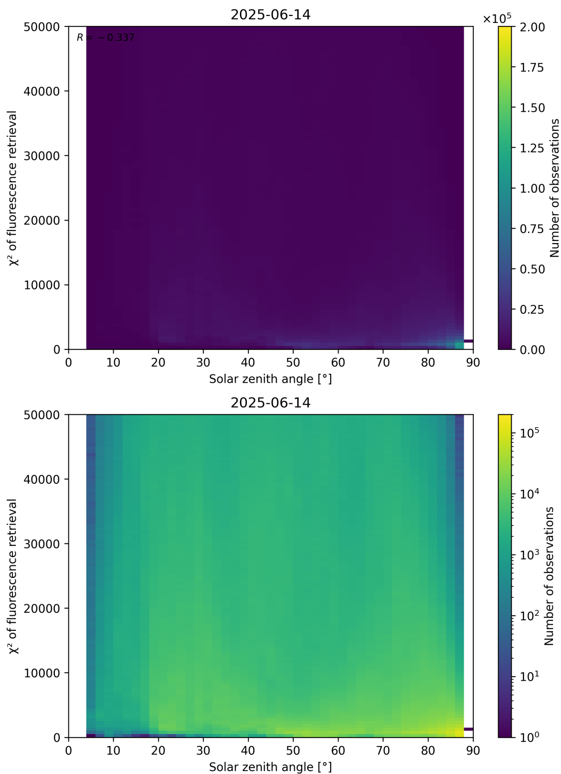
Figure 109: Scatter density plot of “Solar zenith angle” against “ \chi^2 of fluorescence retrieval” for 2025-06-13 to 2025-06-15.
