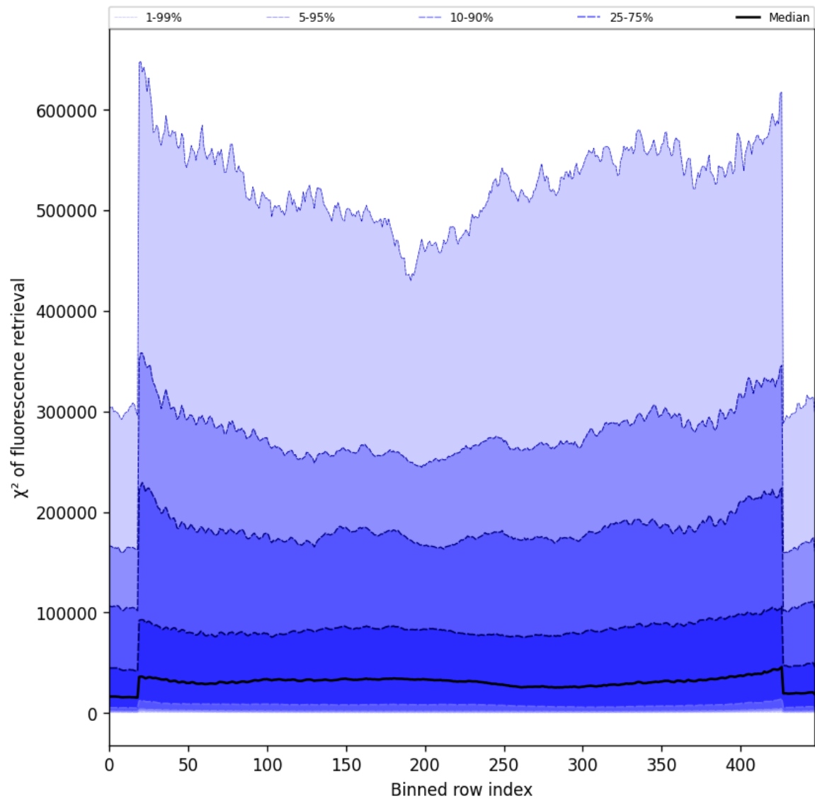
Figure 59: Along track statistics of “ \chi^2 of fluorescence retrieval” for 2025-06-13 to 2025-06-15
