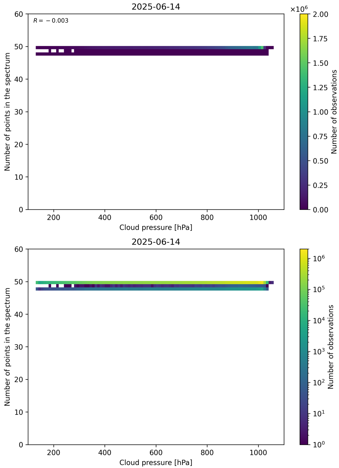
Figure 82: Scatter density plot of “Cloud pressure” against “Number of points in the spectrum” for 2025-06-13 to 2025-06-15.
