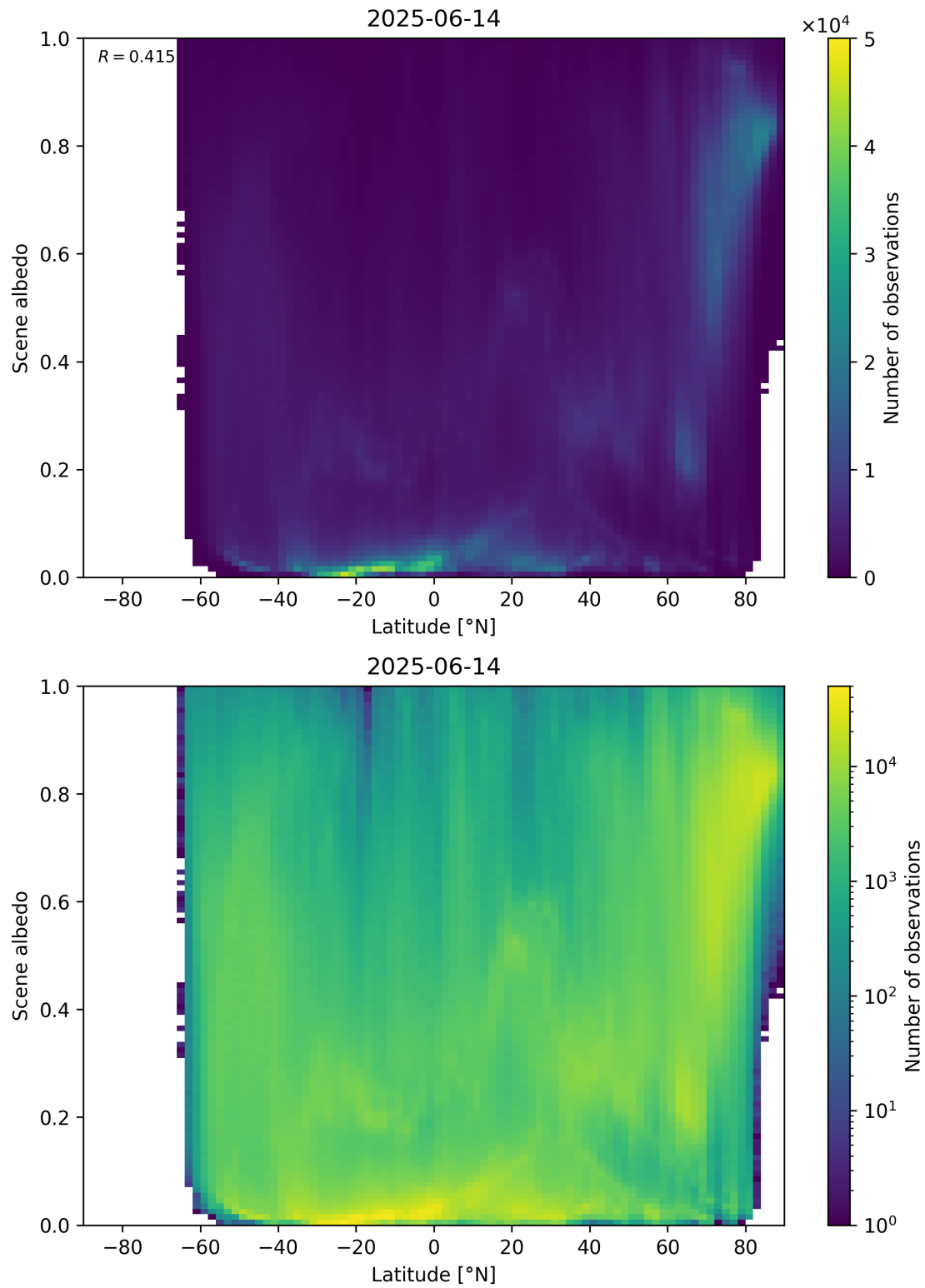
Figure 95: Scatter density plot of “Latitude” against “Scene albedo” for 2025-06-13 to 2025-06-15.
