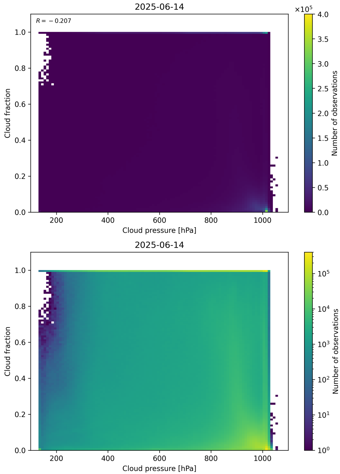
Figure 79: Scatter density plot of “Cloud pressure” against “Cloud fraction” for 2025-06-13 to 2025-06-15.
