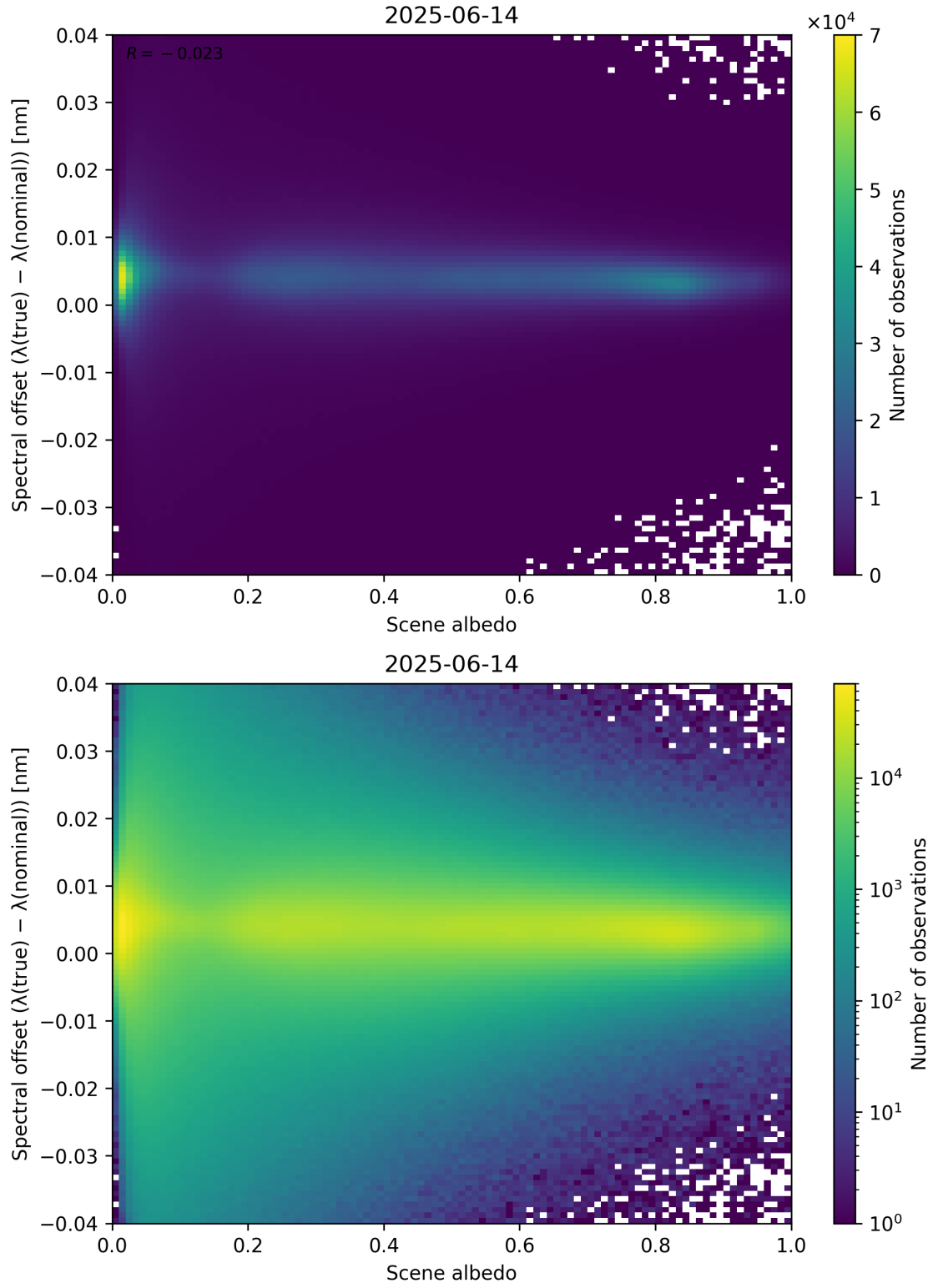
Figure 107: Scatter density plot of “Scene albedo” against “Spectral offset ( \lambda_{\text{true}} - \lambda_{\text{nominal}} )” for 2025-06-13 to 2025-06-15.
