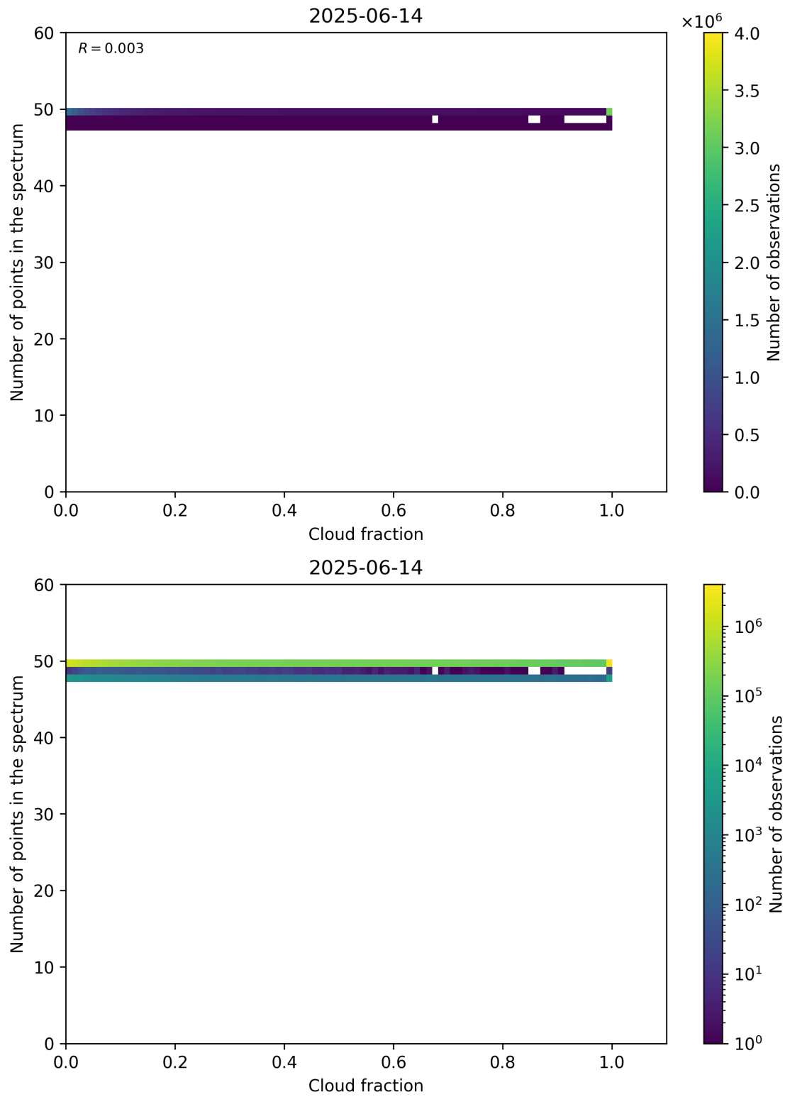
Figure 74: Scatter density plot of “Cloud fraction” against “Number of points in the spectrum” for 2025-06-13 to 2025-06-15.
