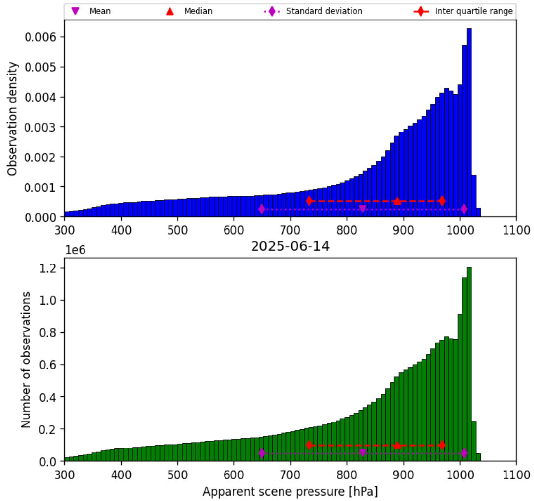
Figure 36: Histogram of “Apparent scene pressure” for 2025-06-13 to 2025-06-15
