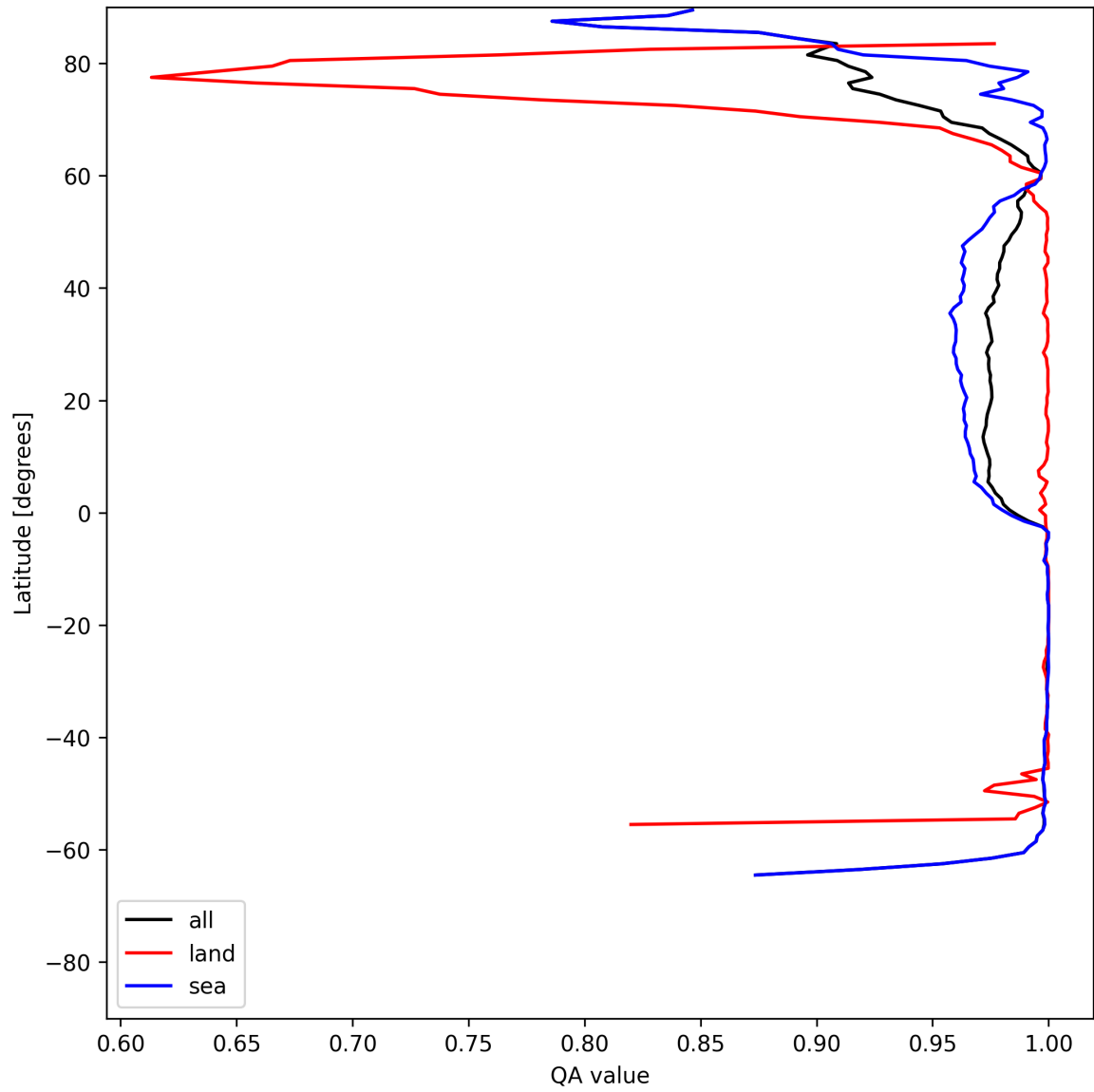
Figure 12: Zonal average of “QA value” for 2025-06-13 to 2025-06-15.
