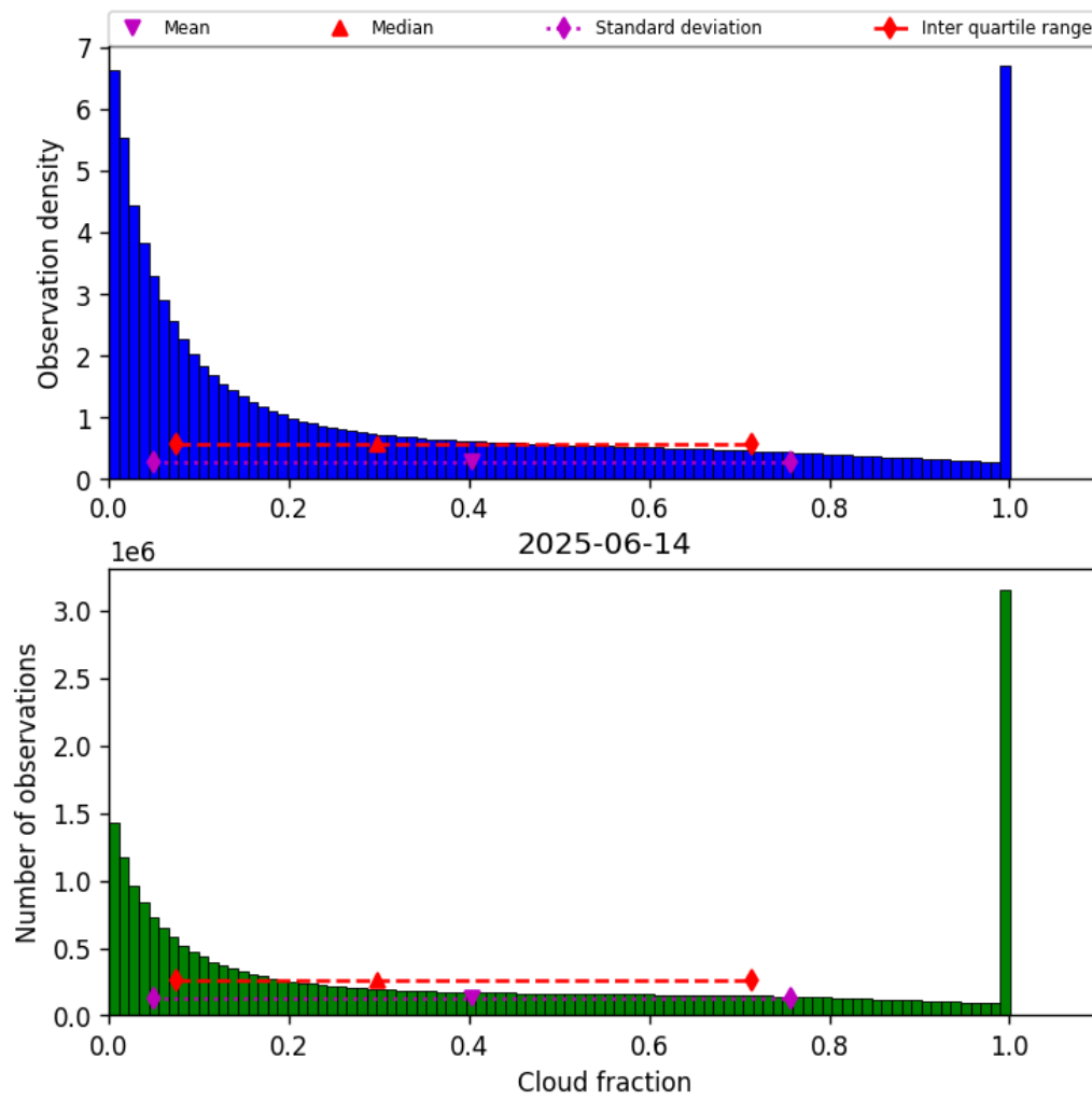
Figure 32: Histogram of “Cloud fraction” for 2025-06-13 to 2025-06-15
