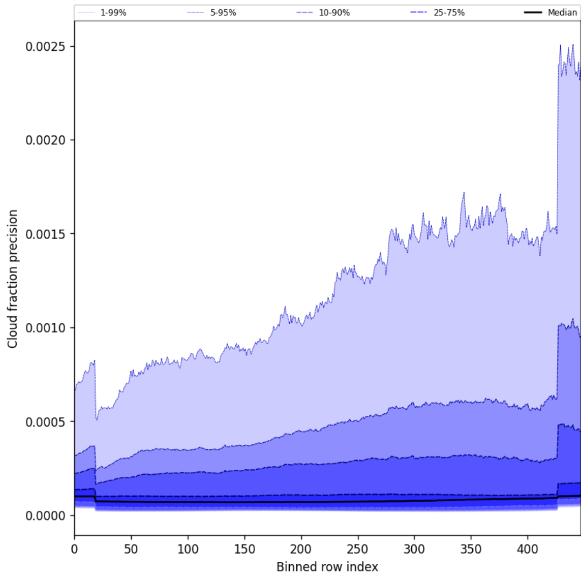
Figure 50: Along track statistics of “Cloud fraction precision” for 2025-06-13 to 2025-06-15
