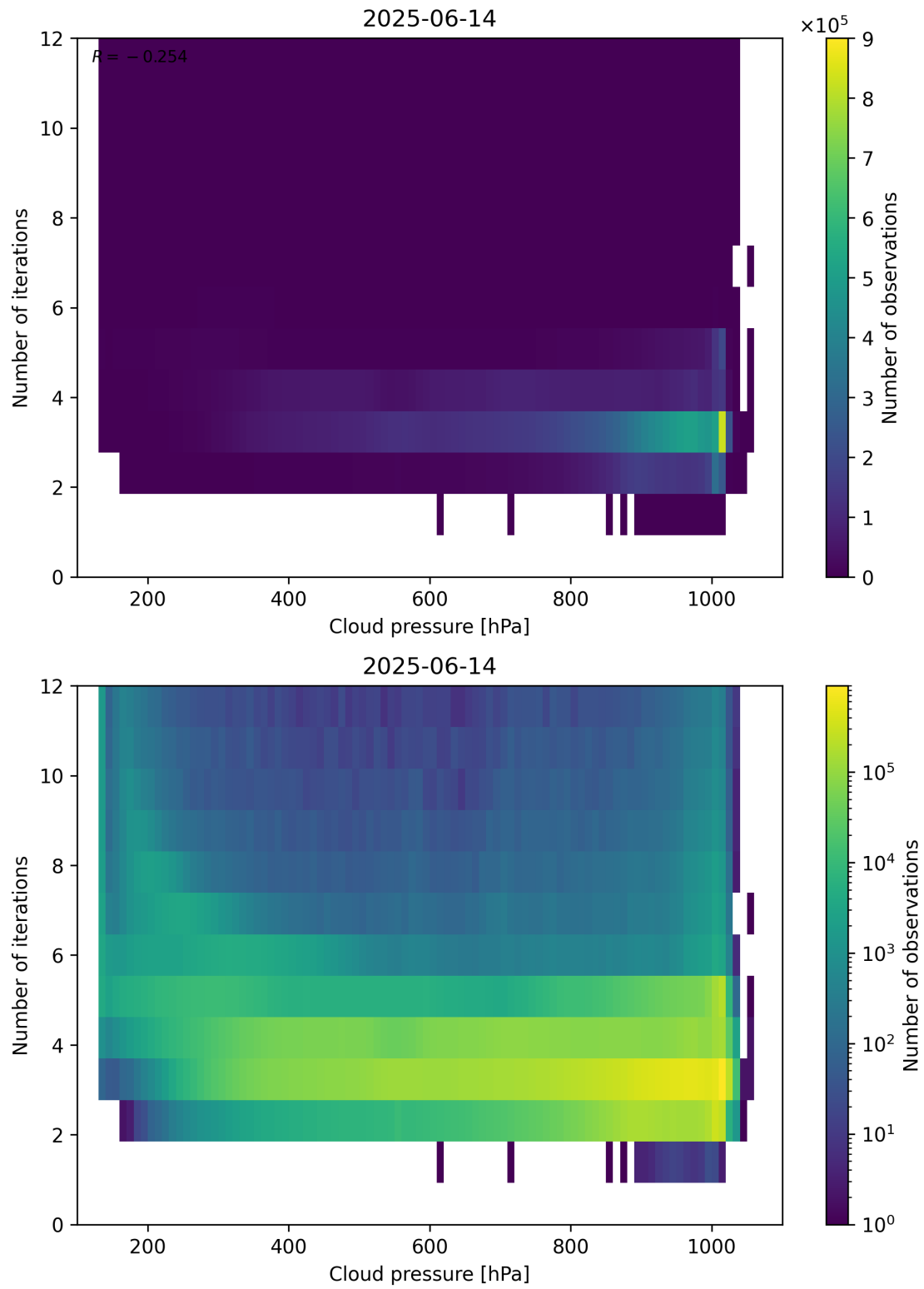
Figure 81: Scatter density plot of “Cloud pressure” against “Number of iterations” for 2025-06-13 to 2025-06-15.
