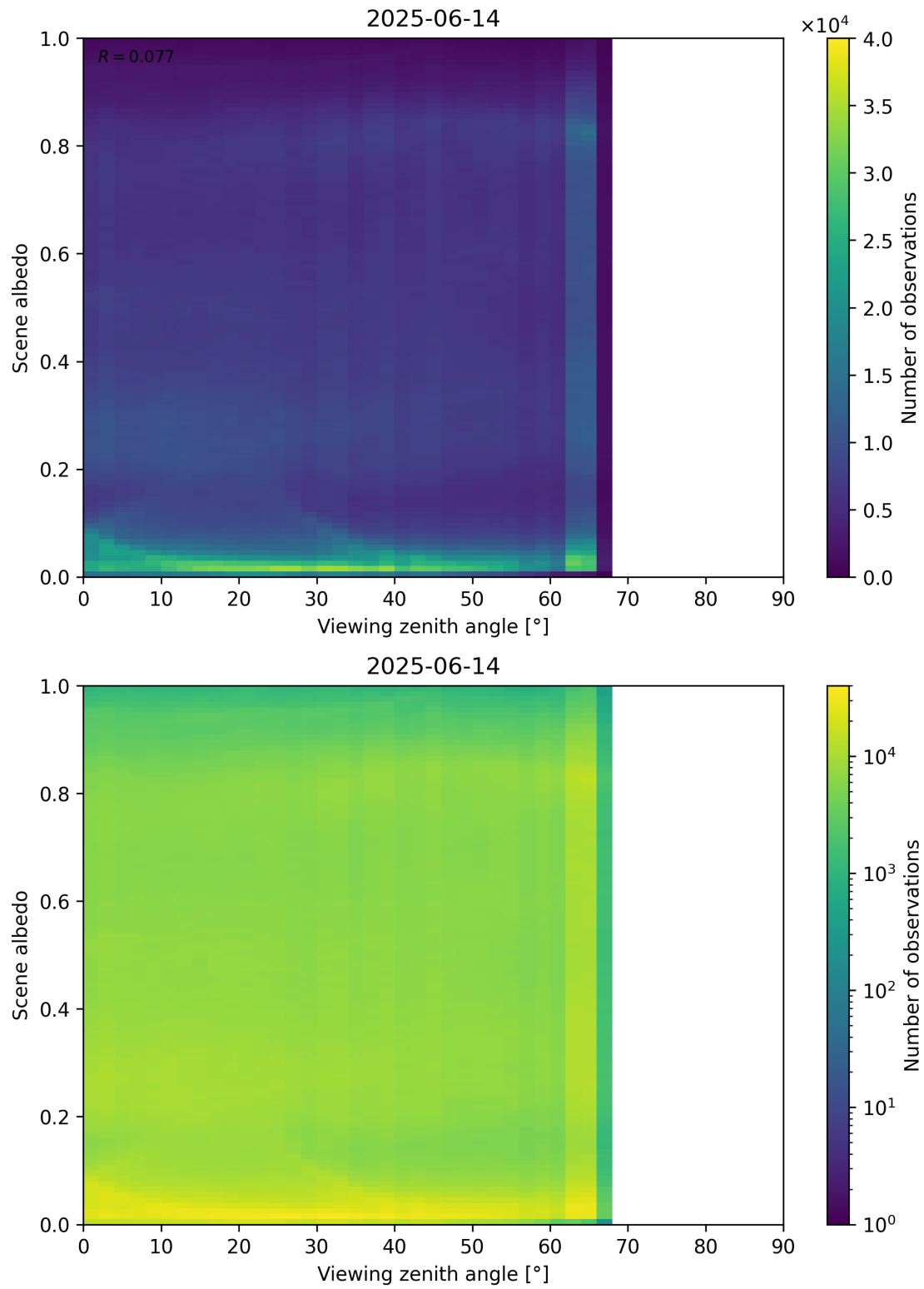
Figure 126: Scatter density plot of “Viewing zenith angle” against “Scene albedo” for 2025-06-13 to 2025-06-15.
