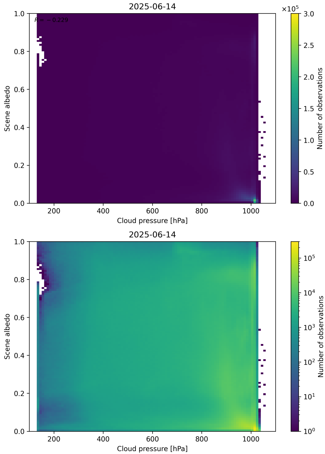
Figure 83: Scatter density plot of “Cloud pressure” against “Scene albedo” for 2025-06-13 to 2025-06-15.
