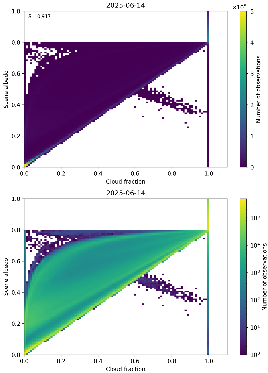
Figure 75: Scatter density plot of “Cloud fraction” against “Scene albedo” for 2025-06-13 to 2025-06-15.
