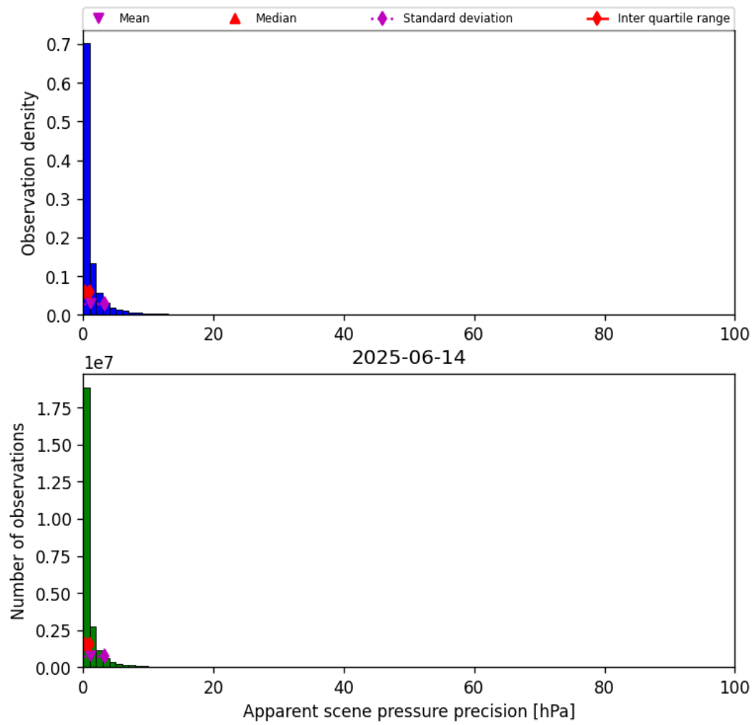
Figure 37: Histogram of “Apparent scene pressure precision” for 2025-06-13 to 2025-06-15
