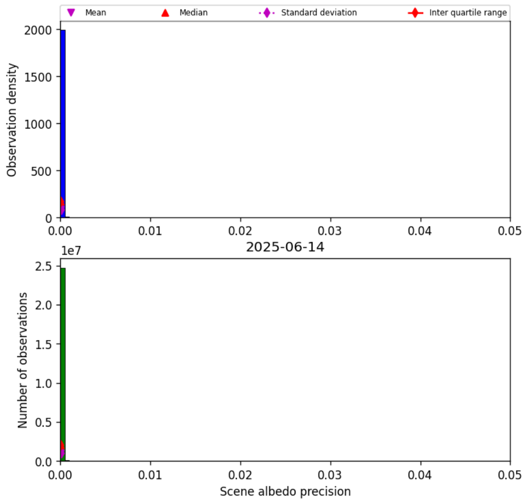
Figure 35: Histogram of “Scene albedo precision” for 2025-06-13 to 2025-06-15
