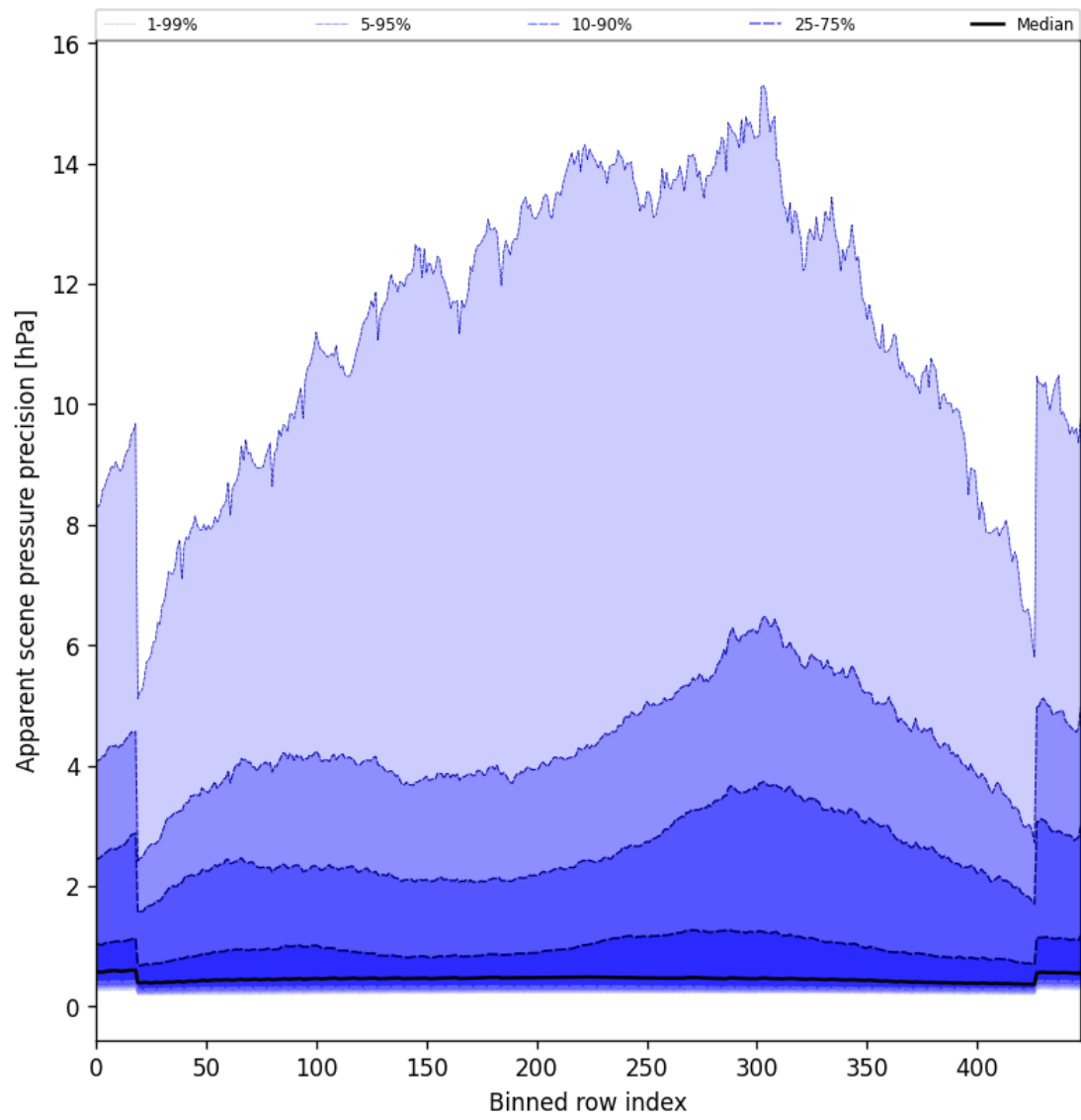
Figure 54: Along track statistics of “Apparent scene pressure precision” for 2025-06-13 to 2025-06-15
