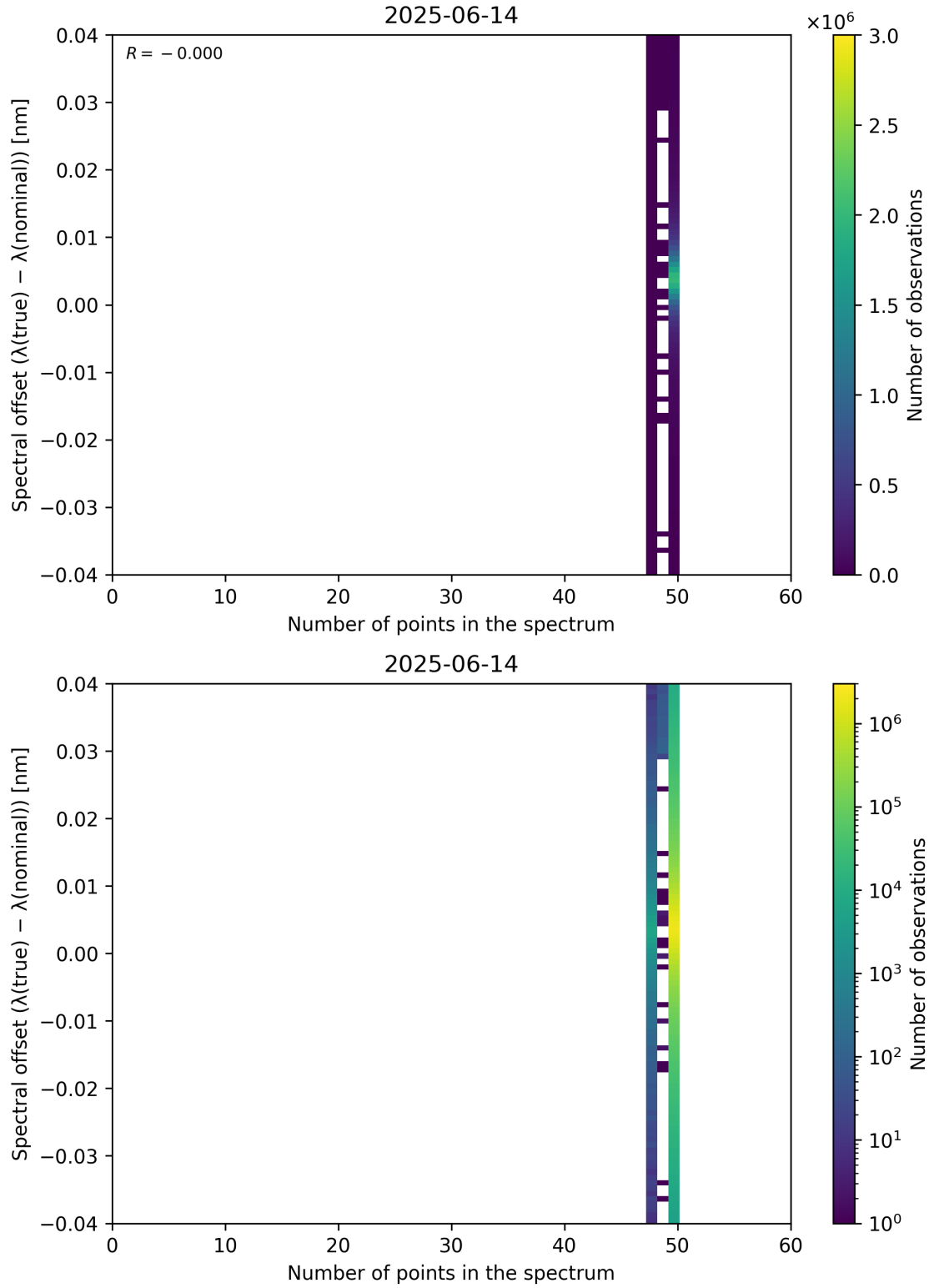
Figure 101: Scatter density plot of “Number of points in the spectrum” against “Spectral offset ( \lambda_{\text{true}} - \lambda_{\text{nominal}} )” for 2025-06-13 to 2025-06-15.
