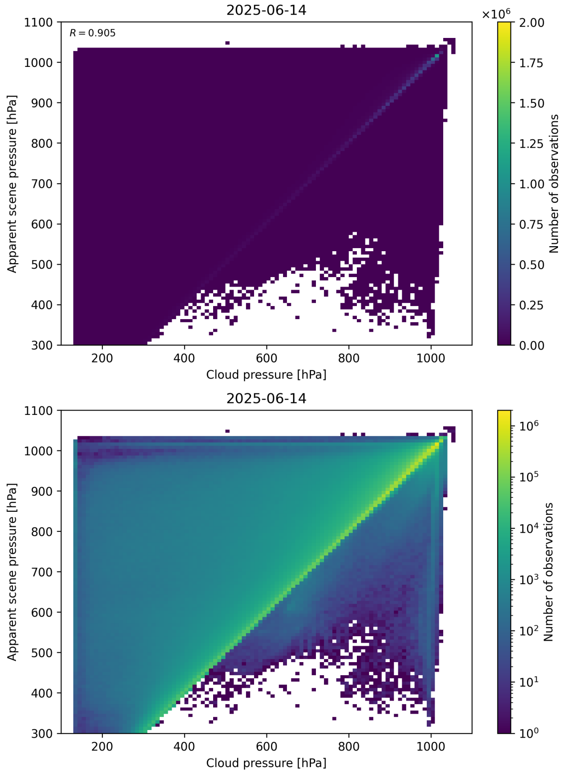
Figure 77: Scatter density plot of “Cloud pressure” against “Apparent scene pressure” for 2025-06-13 to 2025-06-15.
