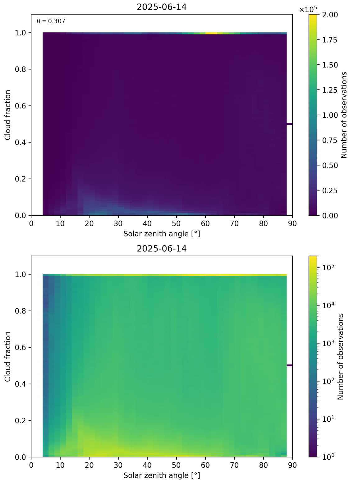
Figure 110: Scatter density plot of “Solar zenith angle” against “Cloud fraction” for 2025-06-13 to 2025-06-15.
