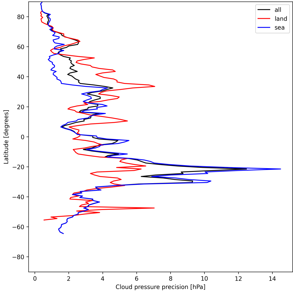
Figure 14: Zonal average of “Cloud pressure precision” for 2025-06-13 to 2025-06-15.
