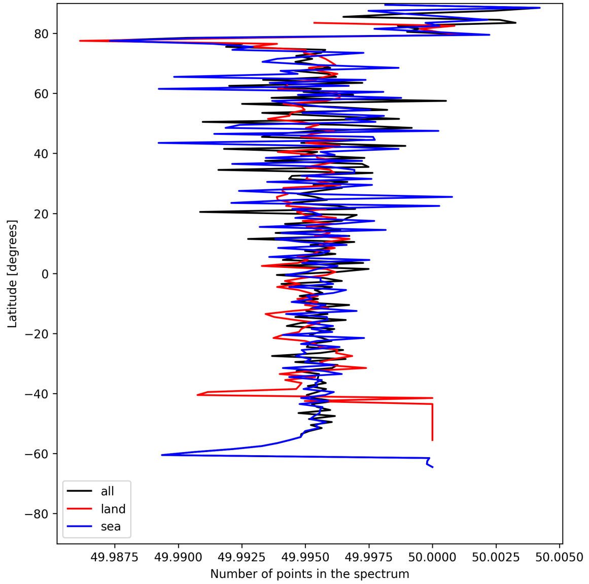
Figure 27: Zonal average of “Number of points in the spectrum” for 2025-06-13 to 2025-06-15.
