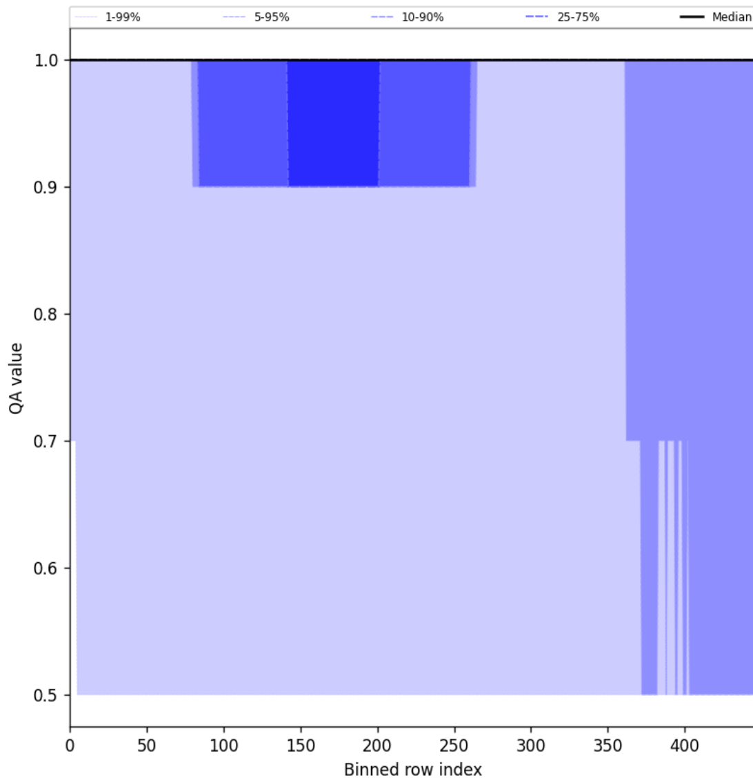
Figure 46: Along track statistics of “QA value” for 2025-06-13 to 2025-06-15
