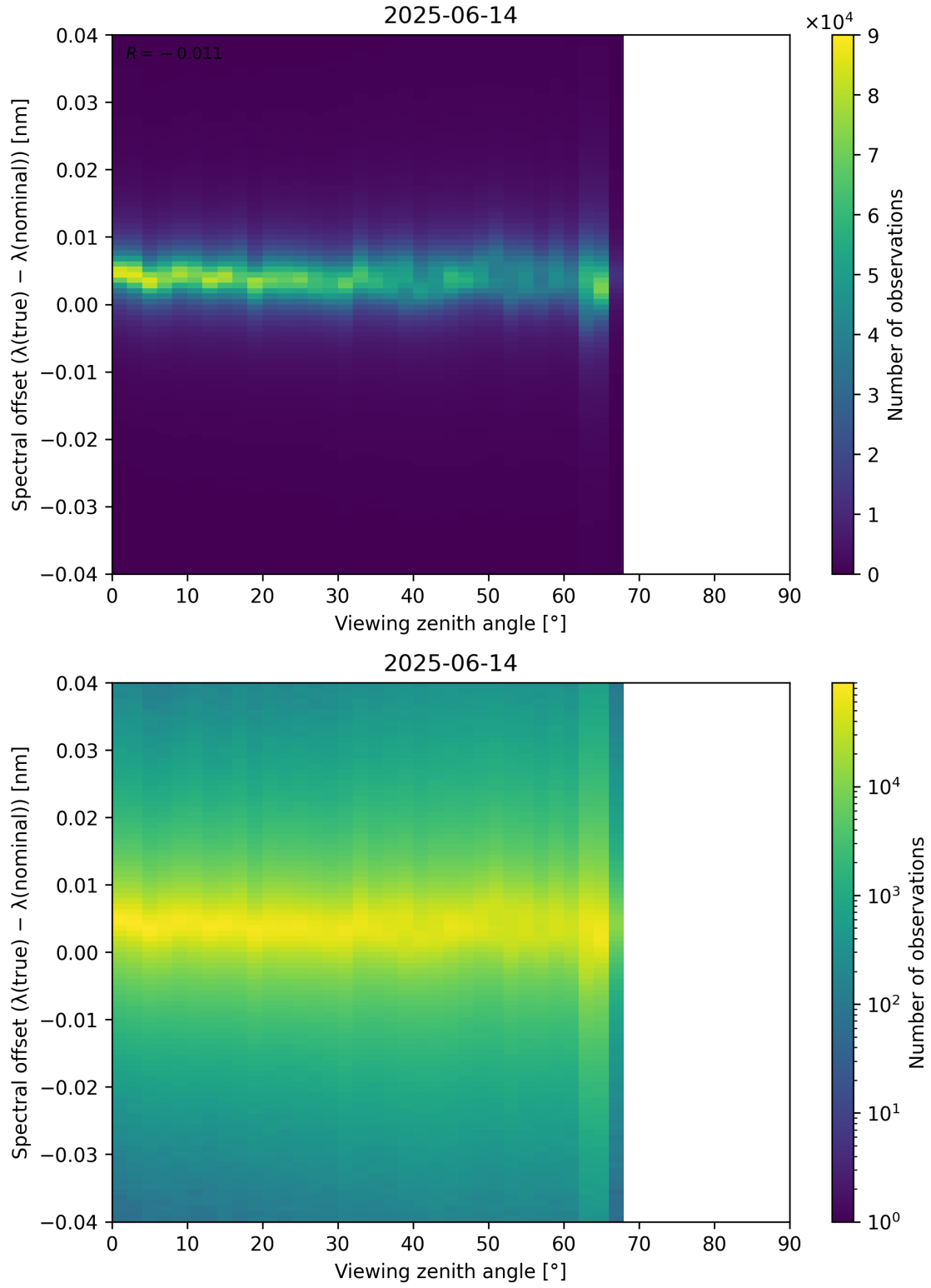
Figure 128: Scatter density plot of “Viewing zenith angle” against “Spectral offset ( \lambda_{\text{true}} - \lambda_{\text{nominal}} )” for 2025-06-13 to 2025-06-15.
