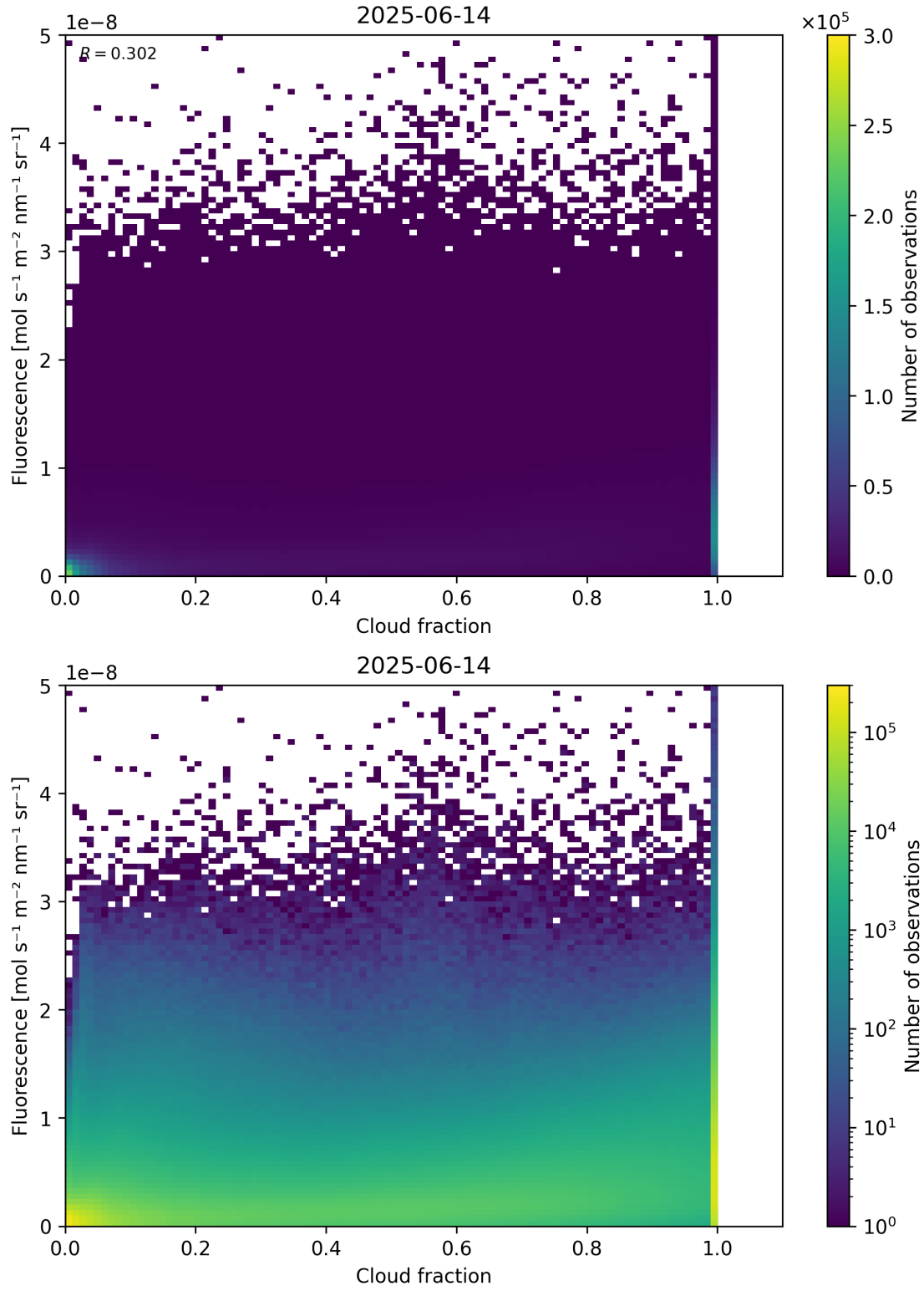
Figure 72: Scatter density plot of “Cloud fraction” against “Fluorescence” for 2025-06-13 to 2025-06-15.
