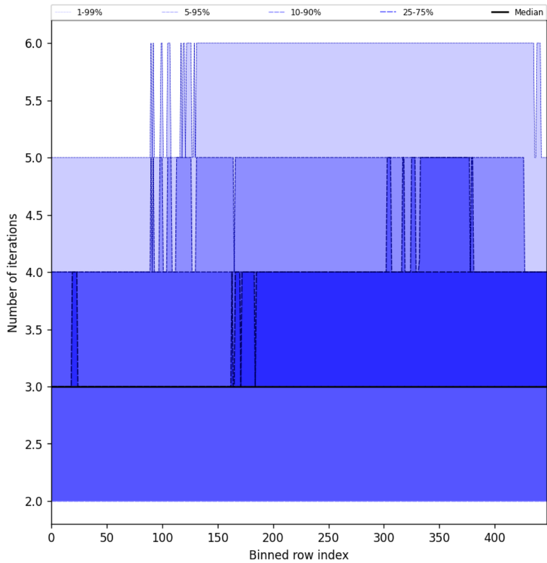
Figure 56: Along track statistics of “Number of iterations” for 2025-06-13 to 2025-06-15
