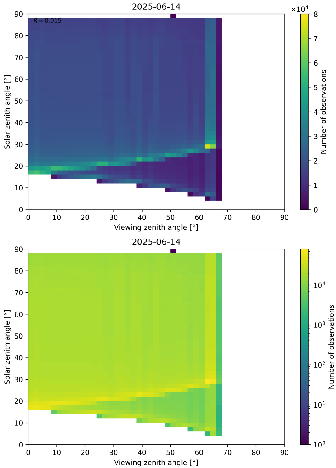
Figure 127: Scatter density plot of “Viewing zenith angle” against “Solar zenith angle” for 2025-06-13 to 2025-06-15.
