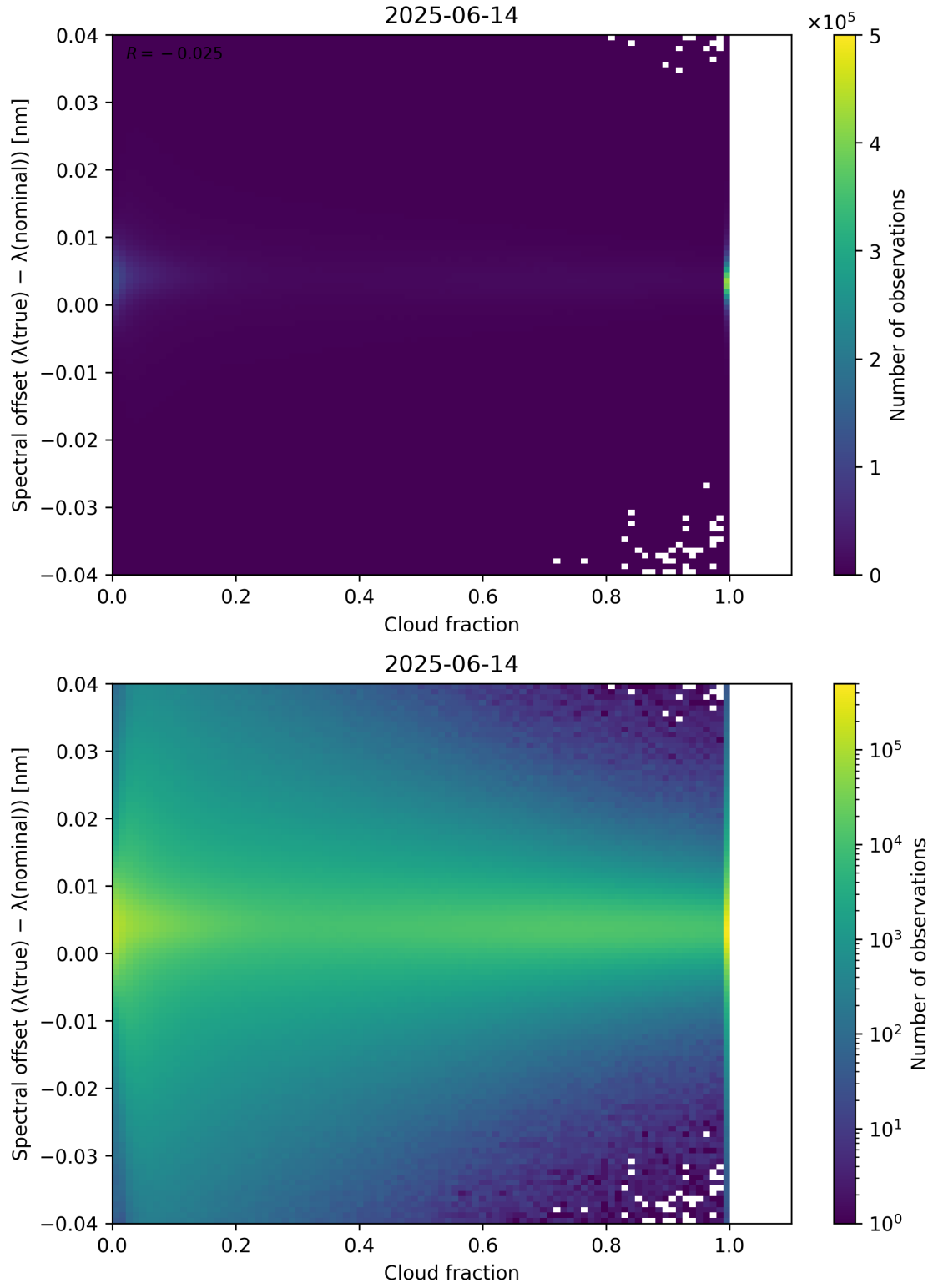
Figure 76: Scatter density plot of “Cloud fraction” against “Spectral offset ( \lambda_{\text{true}} - \lambda_{\text{nominal}} )” for 2025-06-13 to 2025-06-15.
