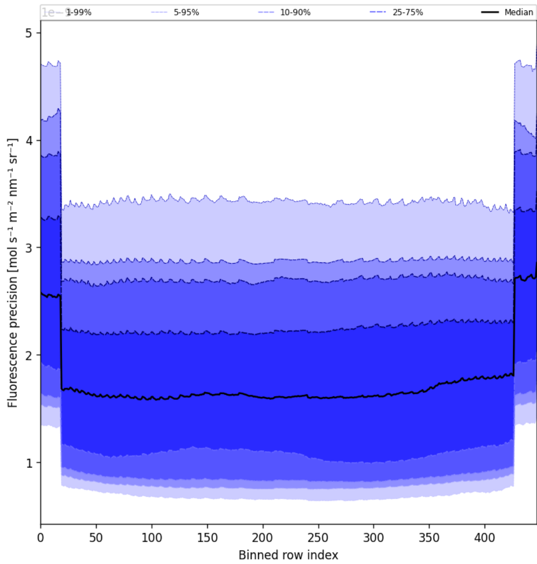
Figure 58: Along track statistics of "Fluorescence precision" for 2025-06-13 to 2025-06-15
