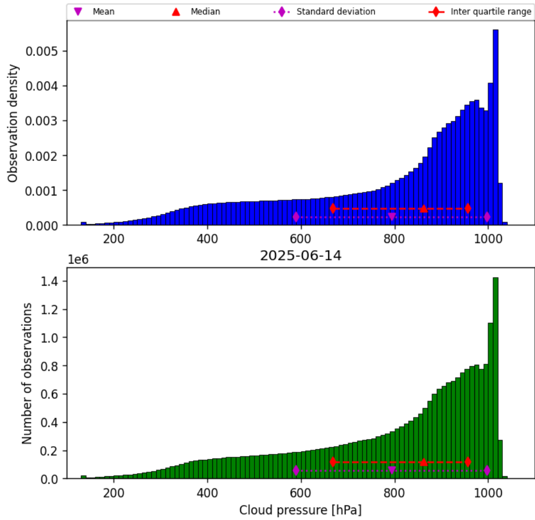
Figure 30: Histogram of “Cloud pressure” for 2025-06-13 to 2025-06-15
