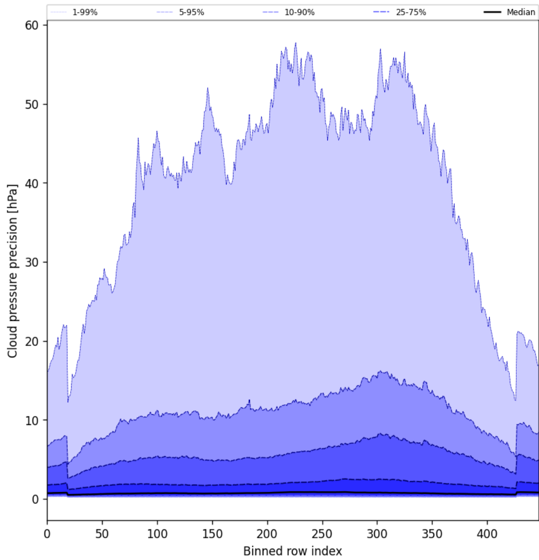
Figure 48: Along track statistics of “Cloud pressure precision” for 2025-06-13 to 2025-06-15
