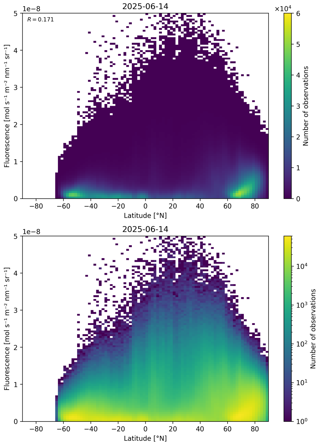
Figure 92: Scatter density plot of “Latitude” against “Fluorescence” for 2025-06-13 to 2025-06-15.
