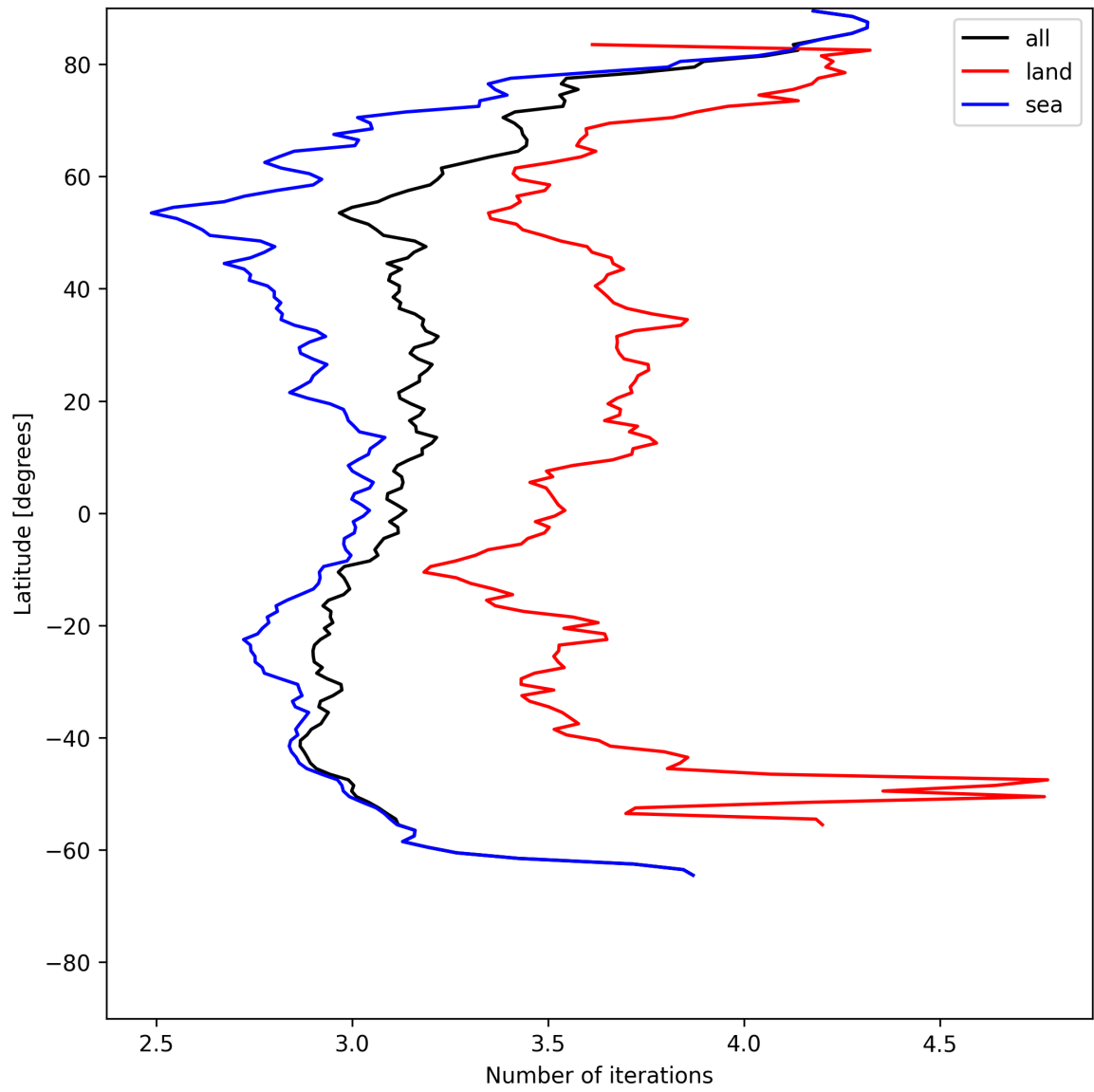
Figure 22: Zonal average of “Number of iterations” for 2025-06-13 to 2025-06-15.
