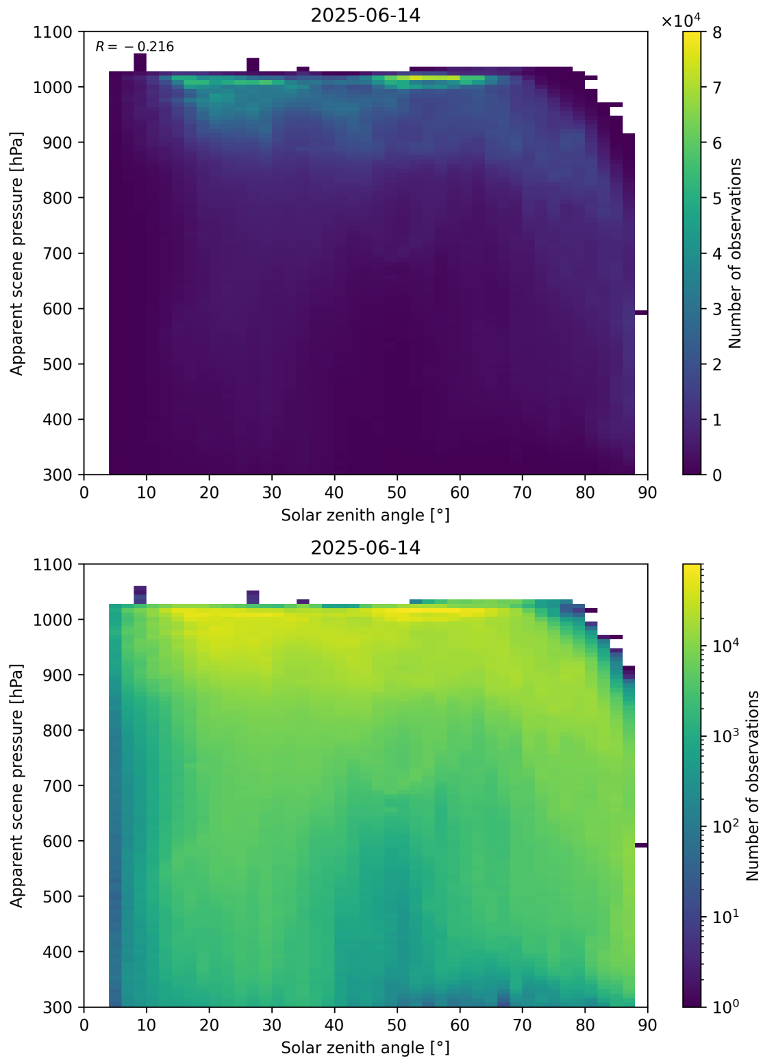
Figure 108: Scatter density plot of “Solar zenith angle” against “Apparent scene pressure” for 2025-06-13 to 2025-06-15.
