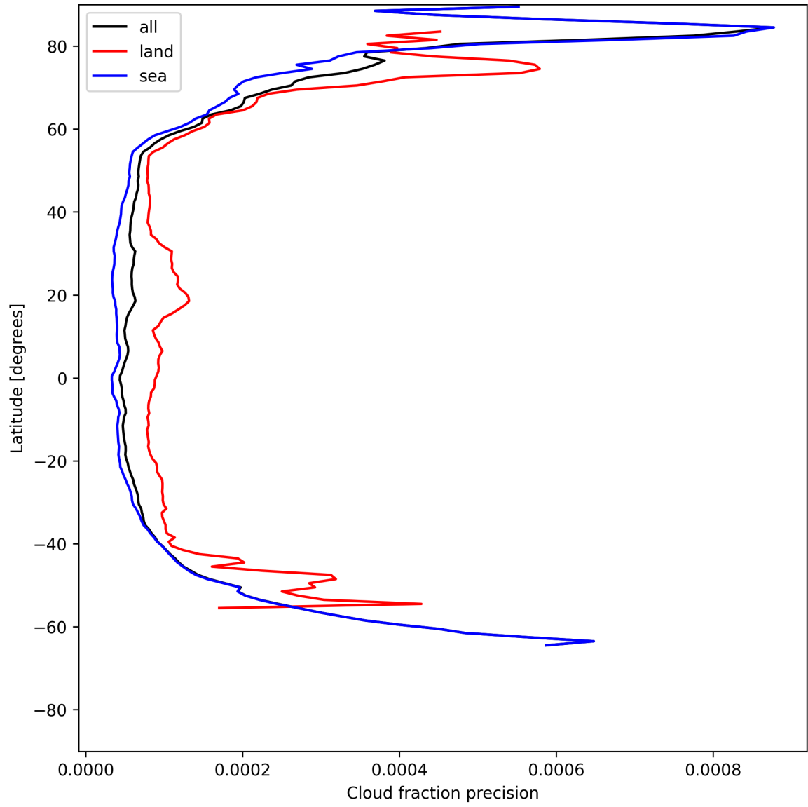
Figure 16: Zonal average of “Cloud fraction precision” for 2025-06-13 to 2025-06-15.
