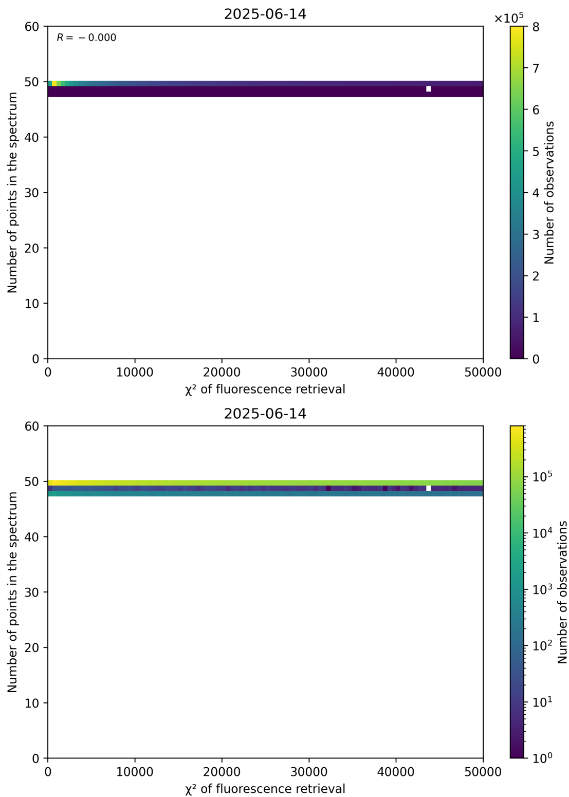
Figure 68: Scatter density plot of “ \chi^2 of fluorescence retrieval” against “Number of points in the spectrum” for 2025-06-13 to 2025-06-15.
