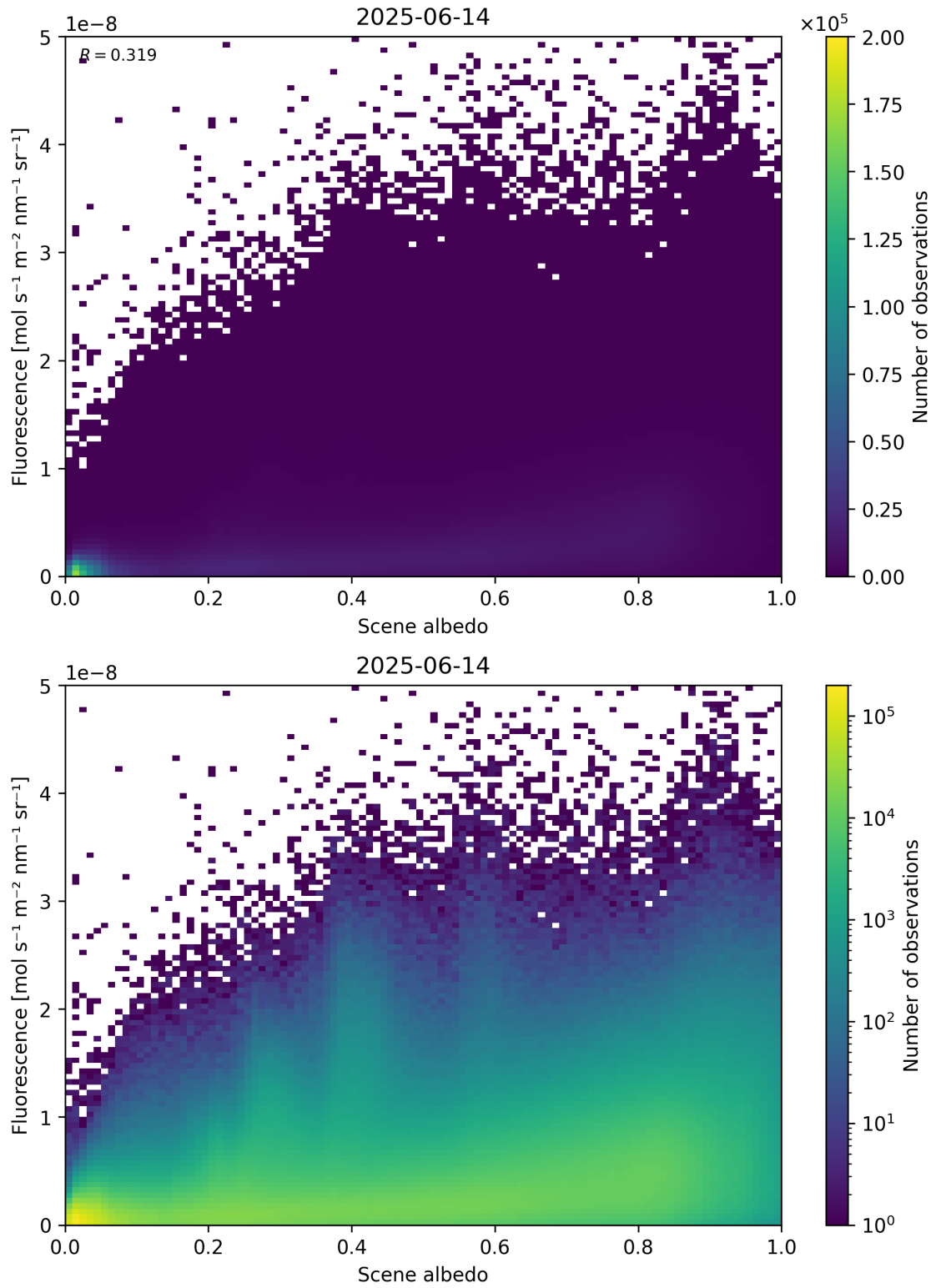
Figure 104: Scatter density plot of “Scene albedo” against “Fluorescence” for 2025-06-13 to 2025-06-15.
