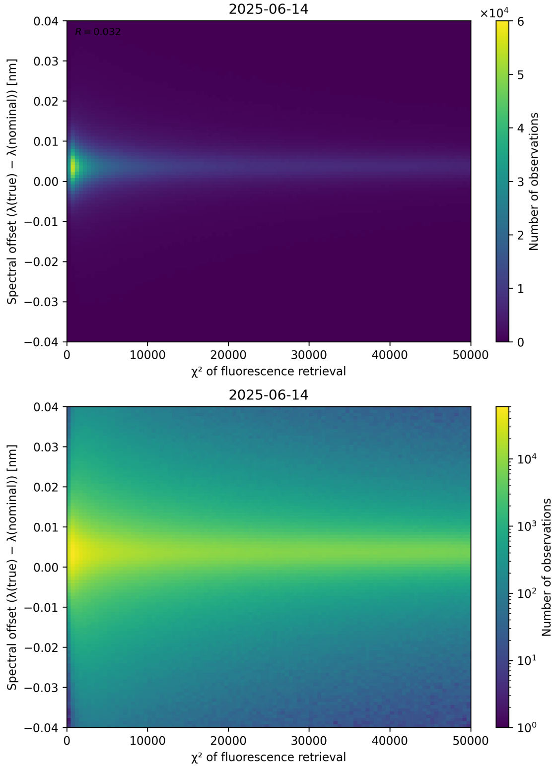
Figure 69: Scatter density plot of “ \chi^2 of fluorescence retrieval” against “Spectral offset ( \lambda_{\text{true}} - \lambda_{\text{nominal}} )” for 2025-06-13 to 2025-06-15.
