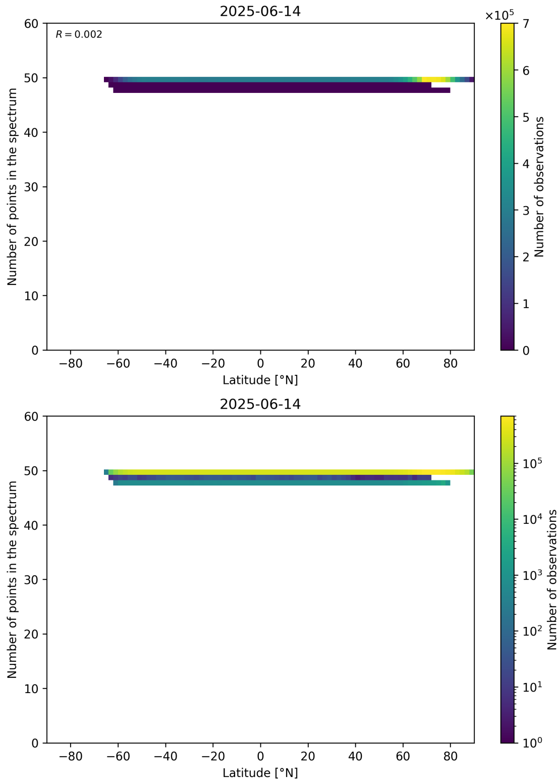
Figure 94: Scatter density plot of “Latitude” against “Number of points in the spectrum” for 2025-06-13 to 2025-06-15.
