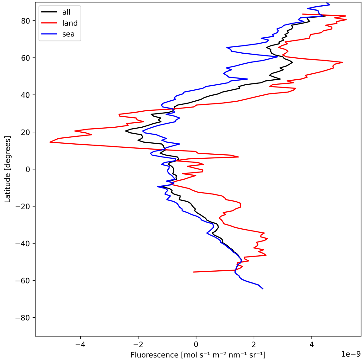
Figure 23: Zonal average of “Fluorescence” for 2025-06-13 to 2025-06-15.
