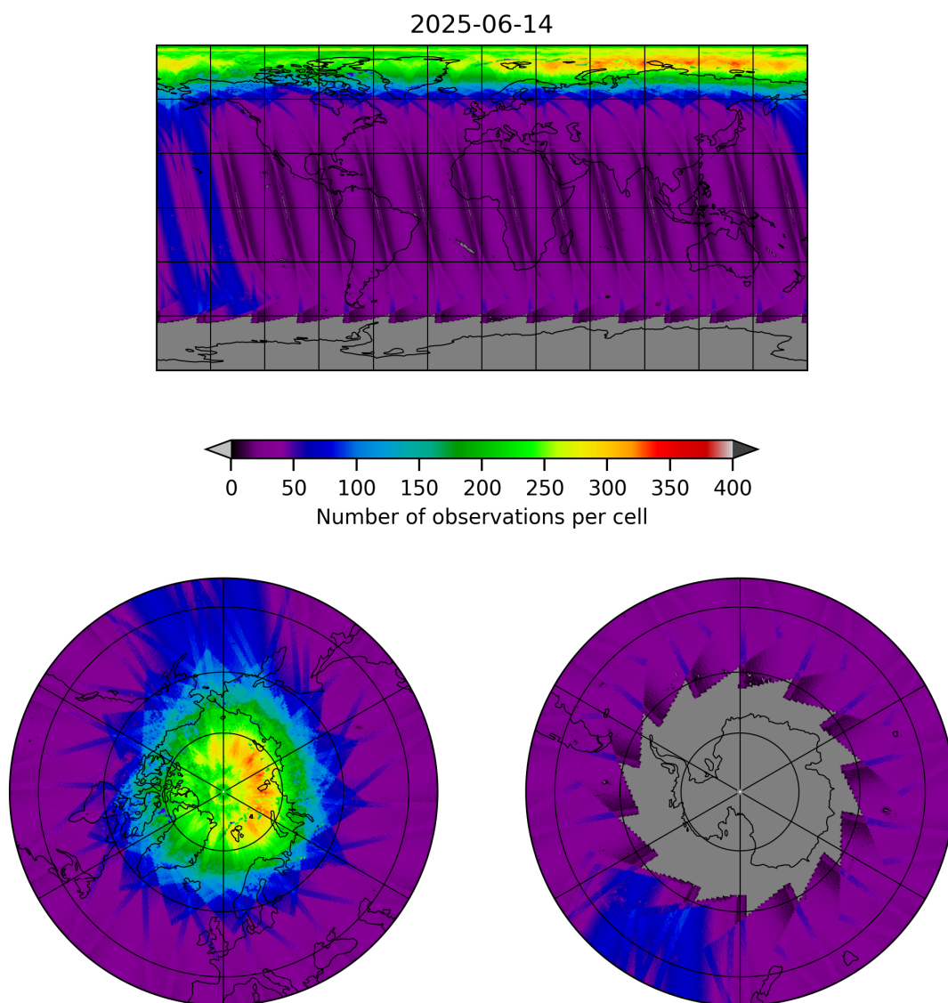
Figure 11: Map of the number of observations for 2025-06-13 to 2025-06-15
