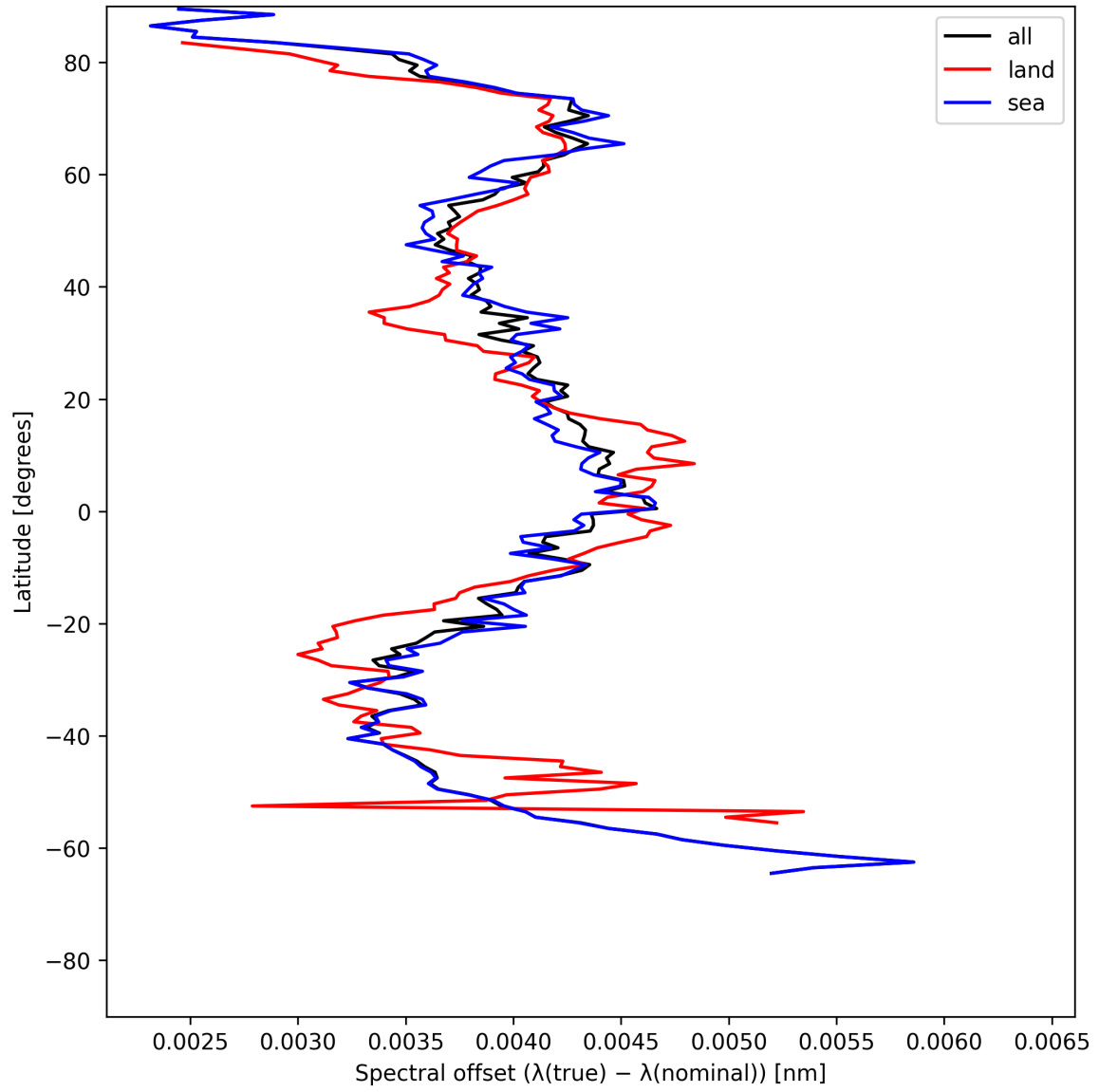
Figure 28: Zonal average of “Spectral offset ( \lambda_{\text{true}} - \lambda_{\text{nominal}} )” for 2025-06-13 to 2025-06-15.
