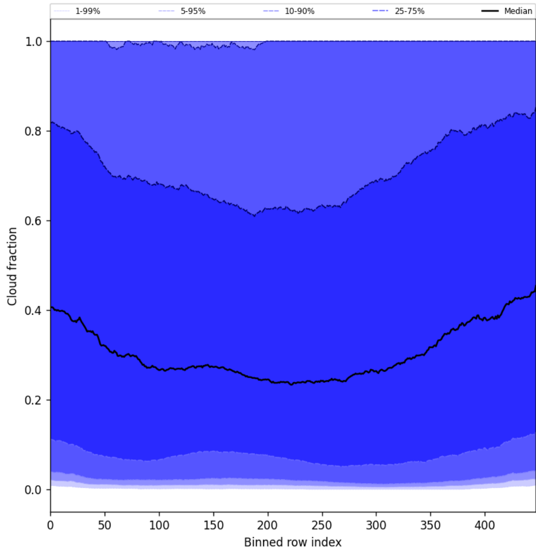
Figure 49: Along track statistics of “Cloud fraction” for 2025-06-13 to 2025-06-15
