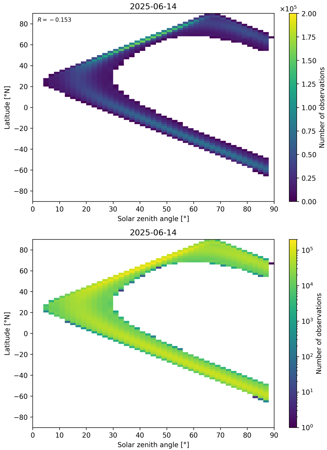
Figure 113: Scatter density plot of “Solar zenith angle” against “Latitude” for 2025-06-13 to 2025-06-15.
