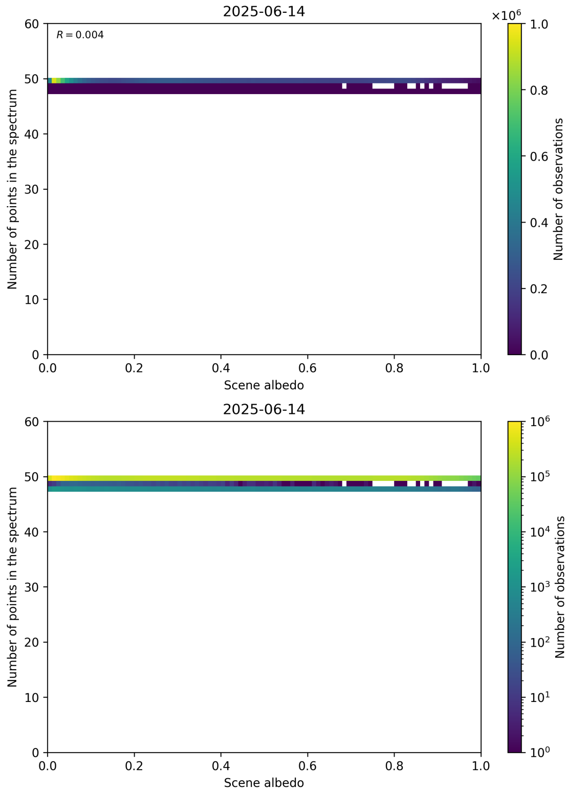
Figure 106: Scatter density plot of “Scene albedo” against “Number of points in the spectrum” for 2025-06-13 to 2025-06-15.
