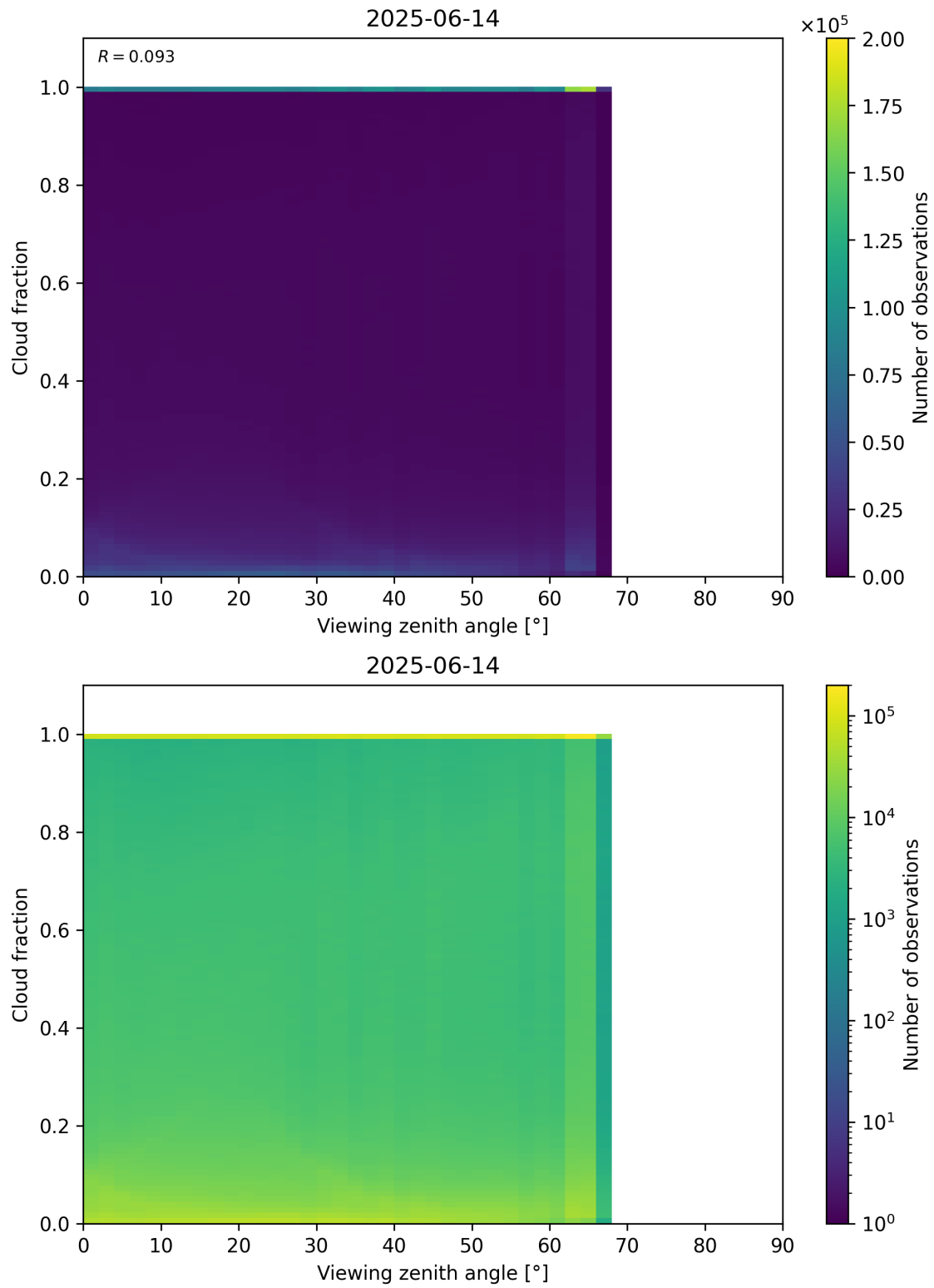
Figure 120: Scatter density plot of “Viewing zenith angle” against “Cloud fraction” for 2025-06-13 to 2025-06-15.
