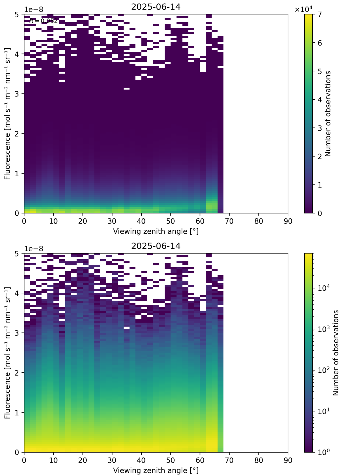
Figure 122: Scatter density plot of “Viewing zenith angle” against “Fluorescence” for 2025-06-13 to 2025-06-15.
