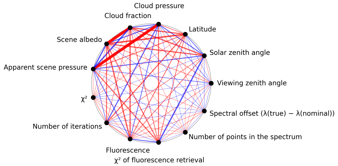
Figure 1: Map of correlation graph for 2025-06-13 to 2025-06-15.
