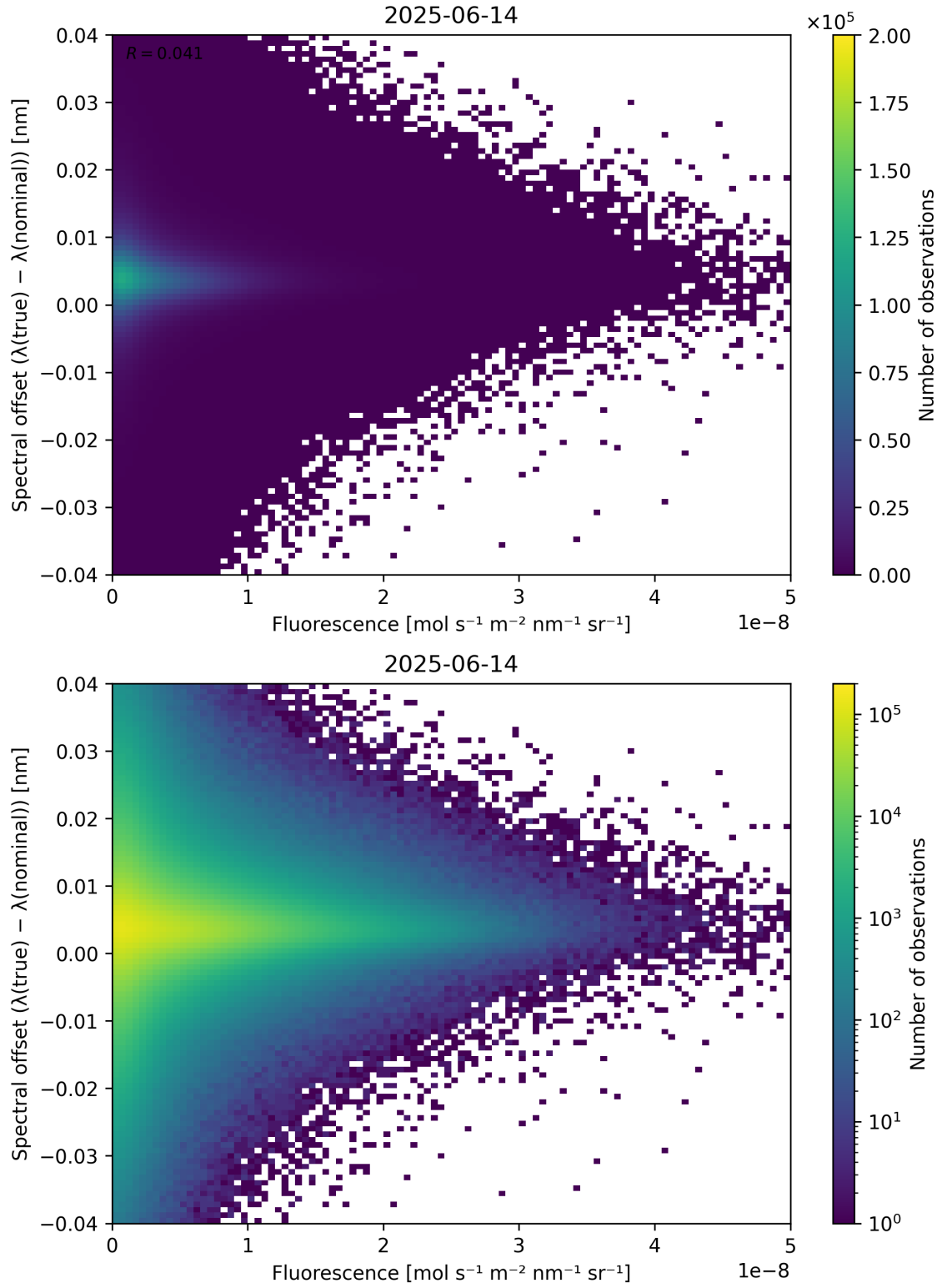
Figure 87: Scatter density plot of “Fluorescence” against “Spectral offset ( \lambda_{\text{true}} - \lambda_{\text{nominal}} )” for 2025-06-13 to 2025-06-15.
