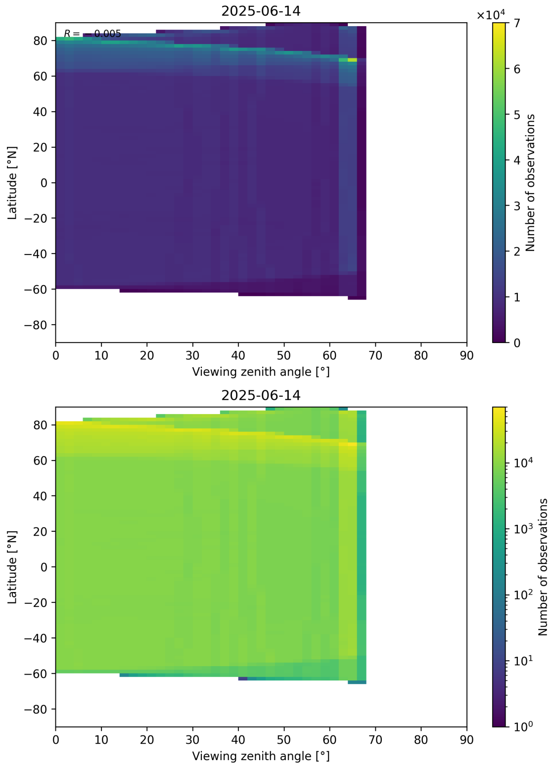
Figure 123: Scatter density plot of “Viewing zenith angle” against “Latitude” for 2025-06-13 to 2025-06-15.
