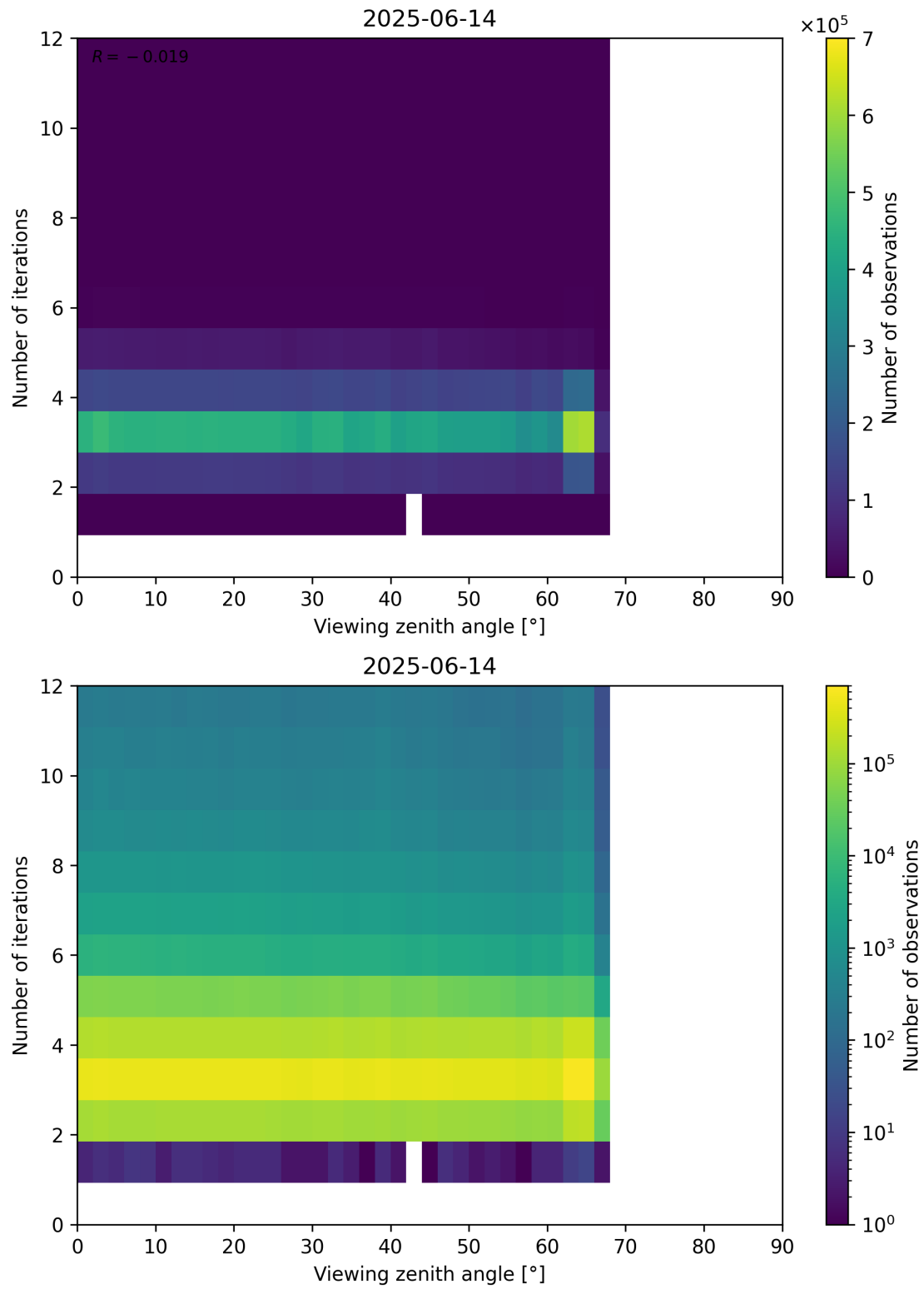
Figure 124: Scatter density plot of “Viewing zenith angle” against “Number of iterations” for 2025-06-13 to 2025-06-15.
