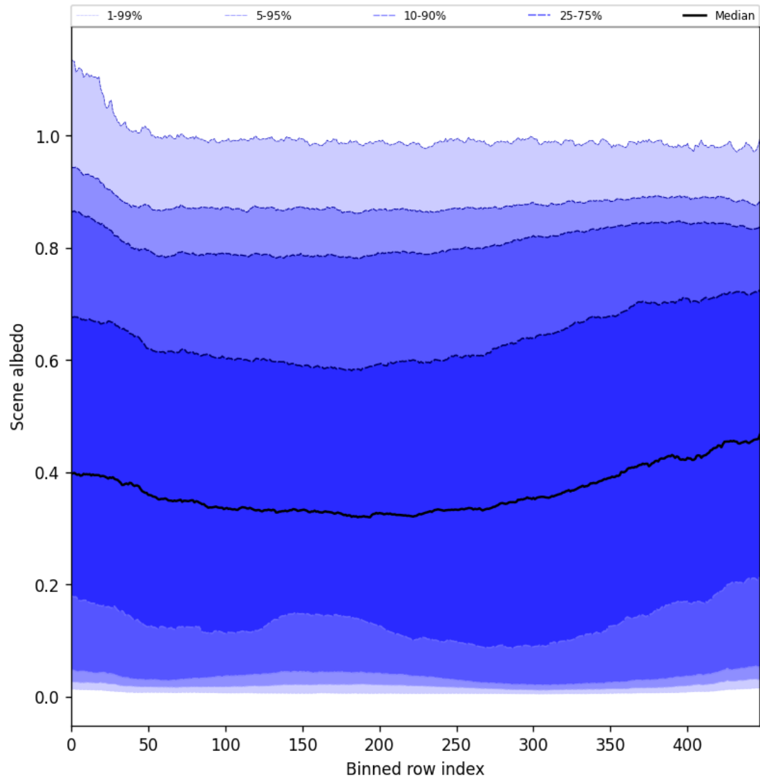
Figure 51: Along track statistics of “Scene albedo” for 2025-06-13 to 2025-06-15
