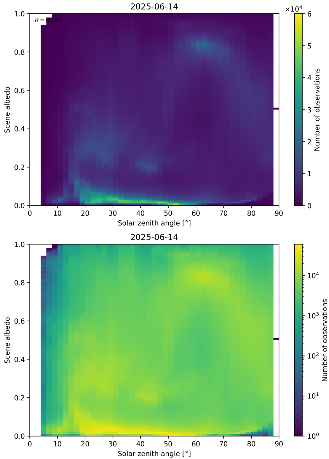
Figure 116: Scatter density plot of “Solar zenith angle” against “Scene albedo” for 2025-06-13 to 2025-06-15.
