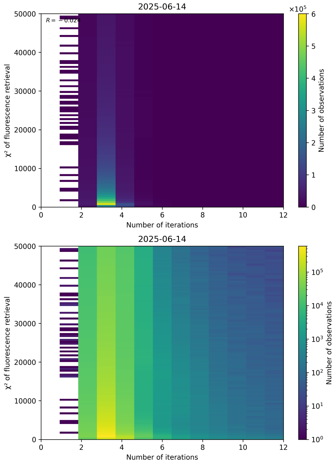
Figure 97: Scatter density plot of “Number of iterations” against “ \chi^2 of fluorescence retrieval” for 2025-06-13 to 2025-06-15.
