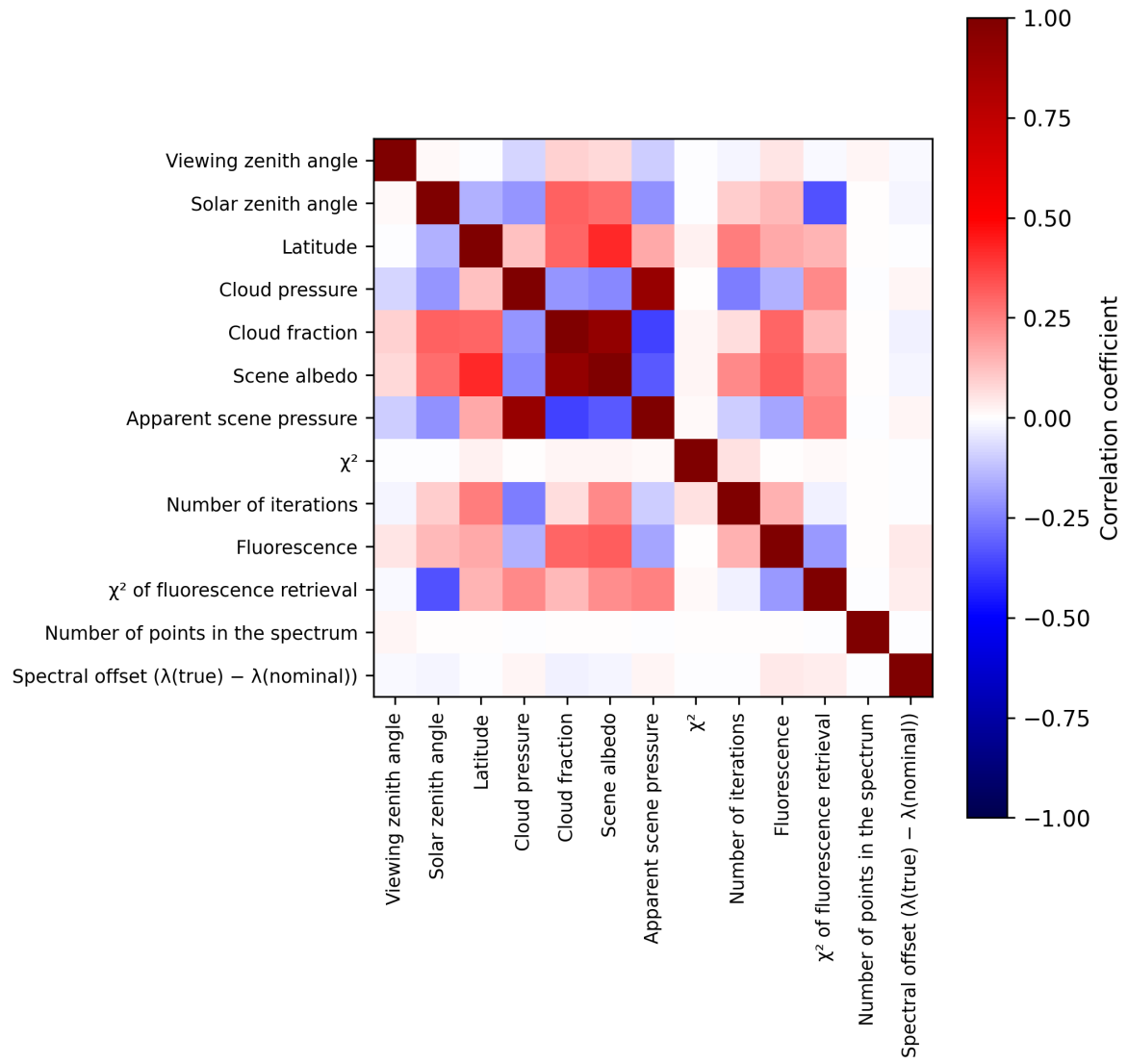
Figure 2: Map of correlation matrix for 2025-06-13 to 2025-06-15.
