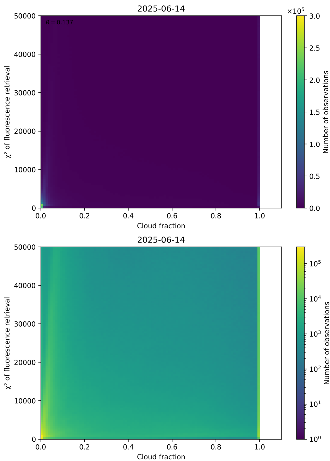
Figure 71: Scatter density plot of “Cloud fraction” against “ \chi^2 of fluorescence retrieval” for 2025-06-13 to 2025-06-15.
