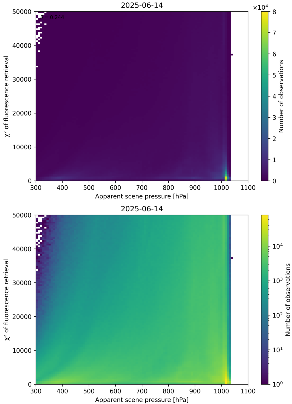
Figure 63: Scatter density plot of “Apparent scene pressure” against “ \chi^2 of fluorescence retrieval” for 2025-06-13 to 2025-06-15.
