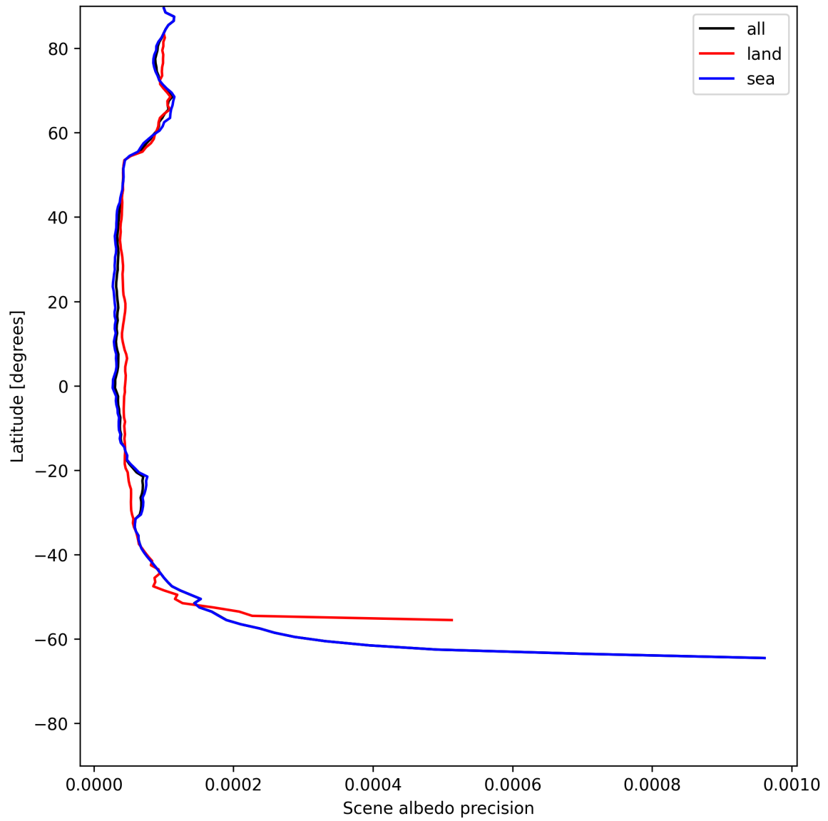
Figure 18: Zonal average of “Scene albedo precision” for 2025-06-13 to 2025-06-15.
