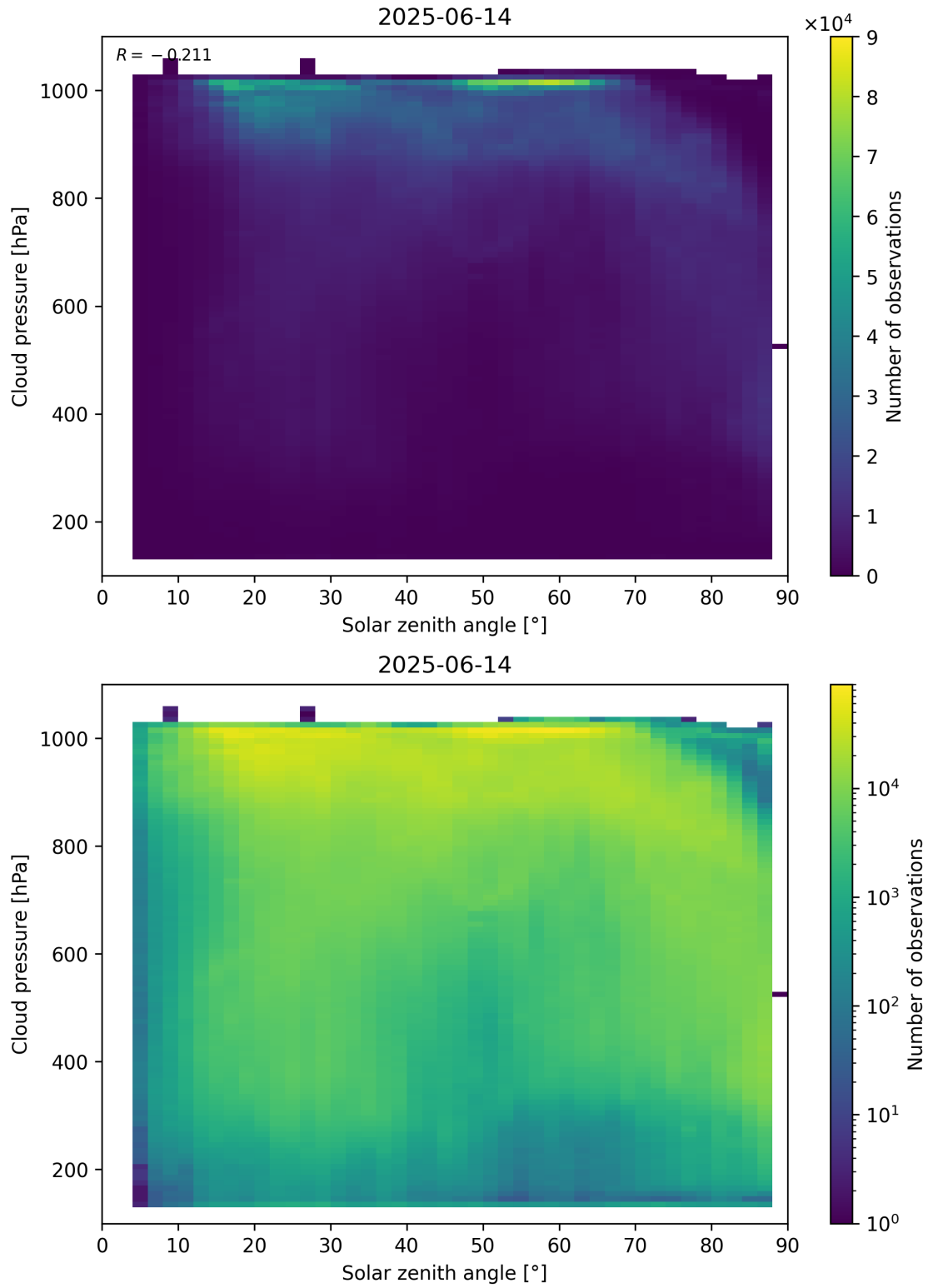
Figure 111: Scatter density plot of “Solar zenith angle” against “Cloud pressure” for 2025-06-13 to 2025-06-15.
