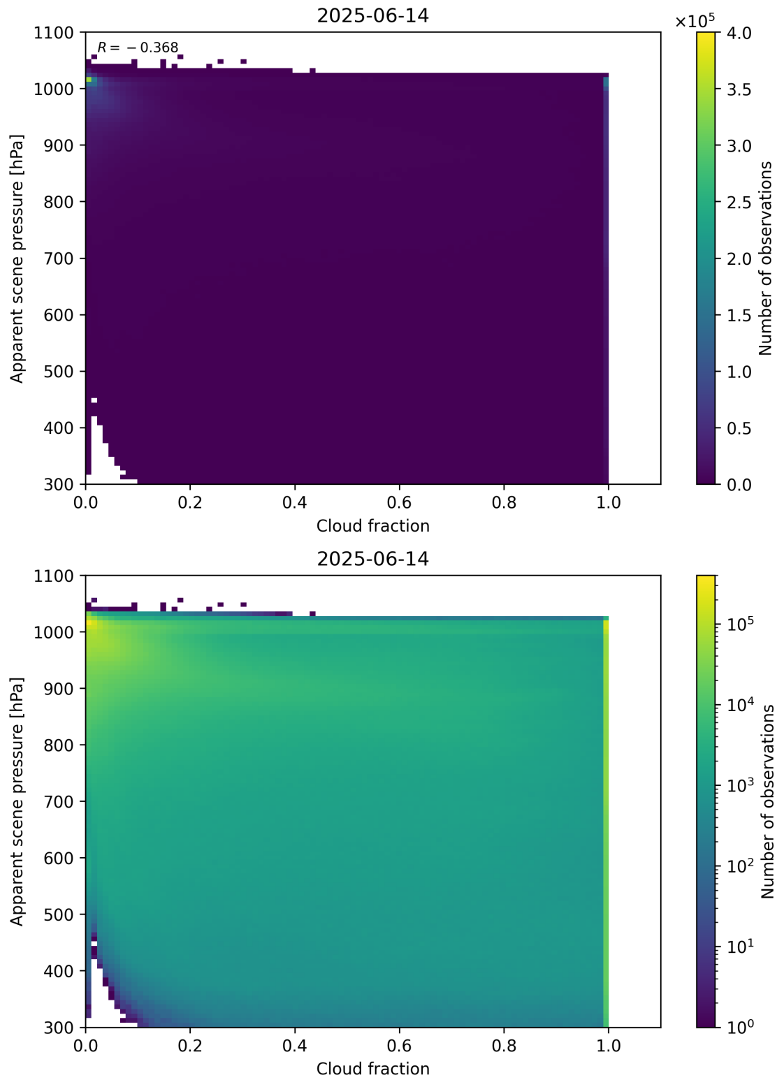
Figure 70: Scatter density plot of “Cloud fraction” against “Apparent scene pressure” for 2025-06-13 to 2025-06-15.
