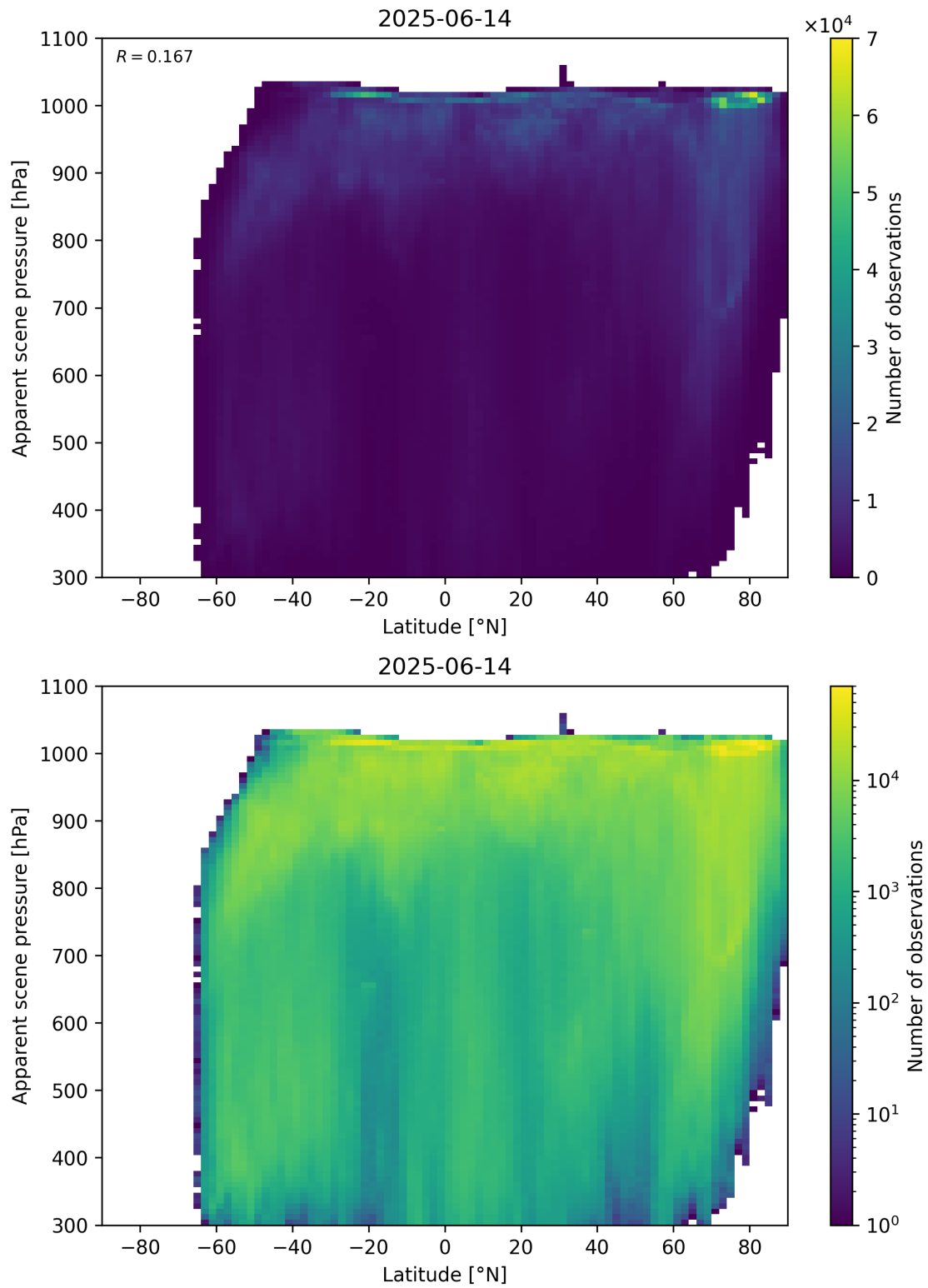
Figure 88: Scatter density plot of “Latitude” against “Apparent scene pressure” for 2025-06-13 to 2025-06-15.
