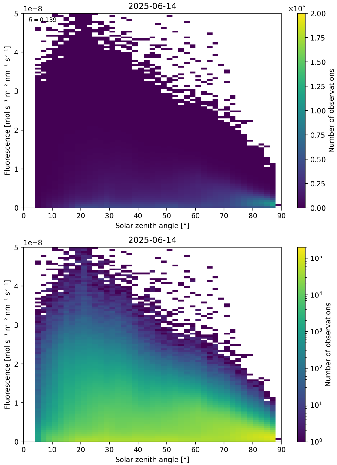
Figure 112: Scatter density plot of “Solar zenith angle” against “Fluorescence” for 2025-06-13 to 2025-06-15.
