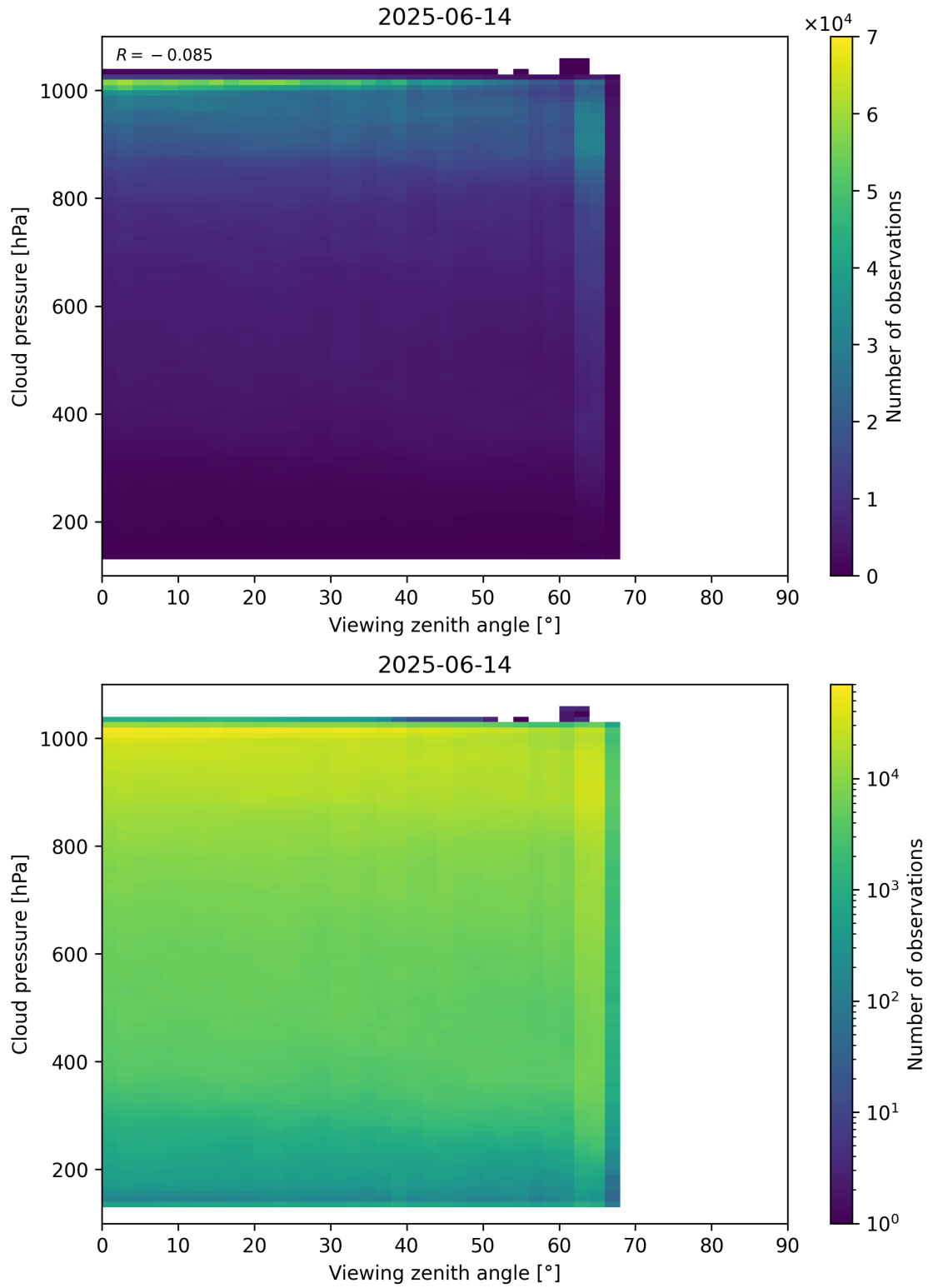
Figure 121: Scatter density plot of “Viewing zenith angle” against “Cloud pressure” for 2025-06-13 to 2025-06-15.
