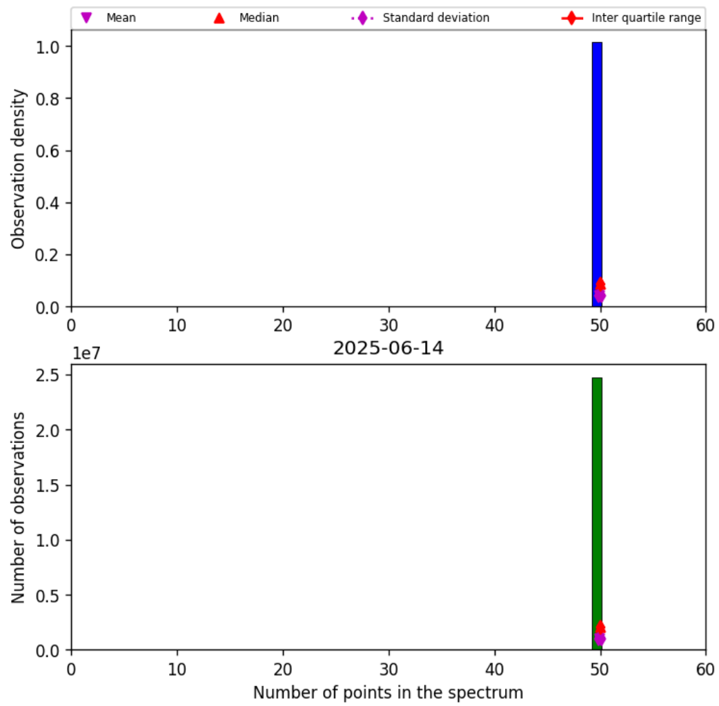
Figure 44: Histogram of “Number of points in the spectrum” for 2025-06-13 to 2025-06-15
