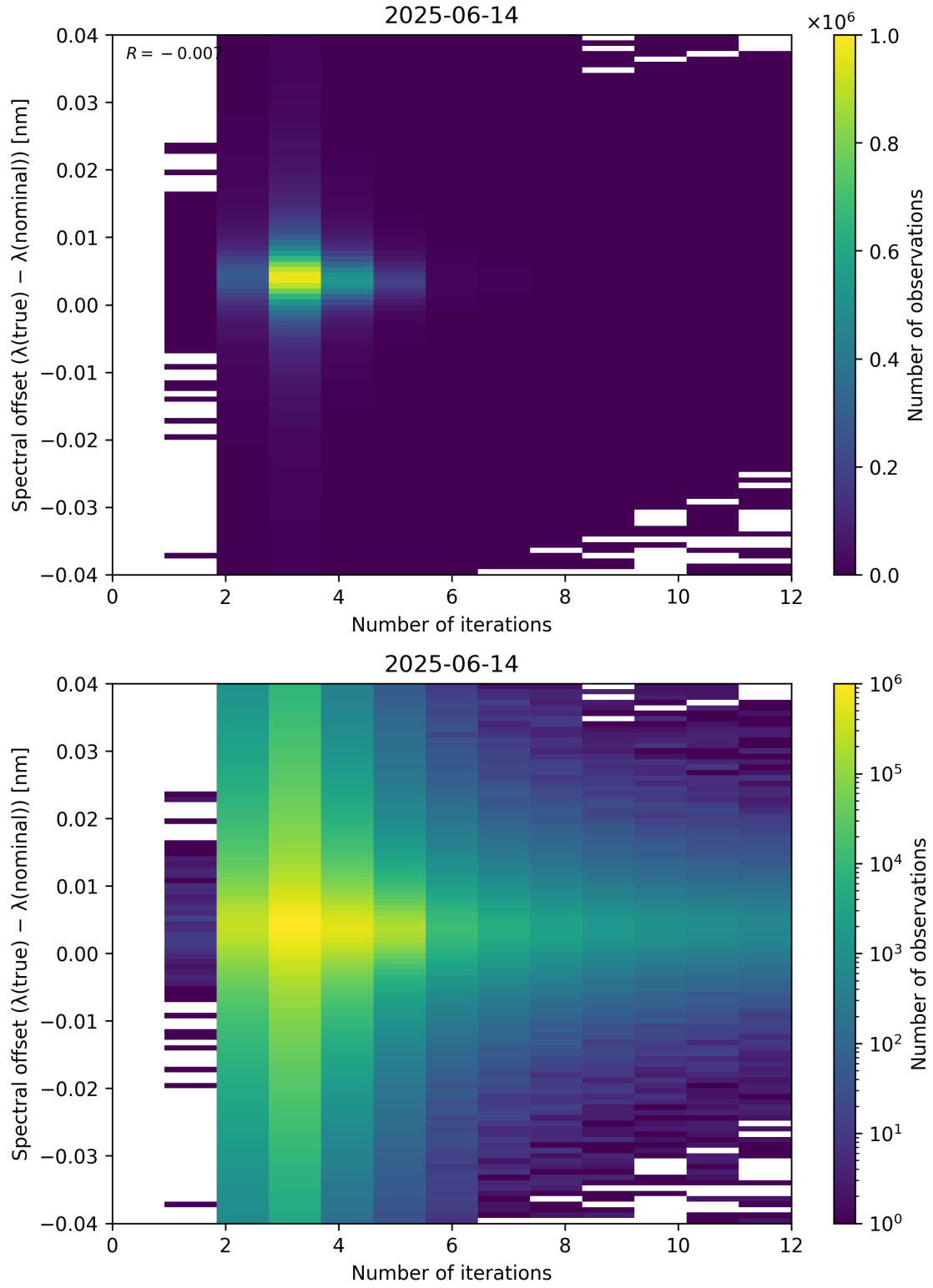
Figure 100: Scatter density plot of “Number of iterations” against “Spectral offset ( \lambda_{\text{true}} - \lambda_{\text{nominal}} )” for 2025-06-13 to 2025-06-15.
