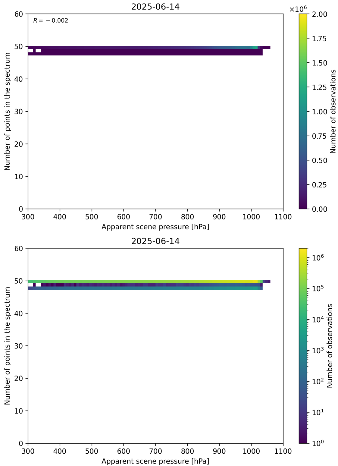
Figure 66: Scatter density plot of “Apparent scene pressure” against “Number of points in the spectrum” for 2025-06-13 to 2025-06-15.
