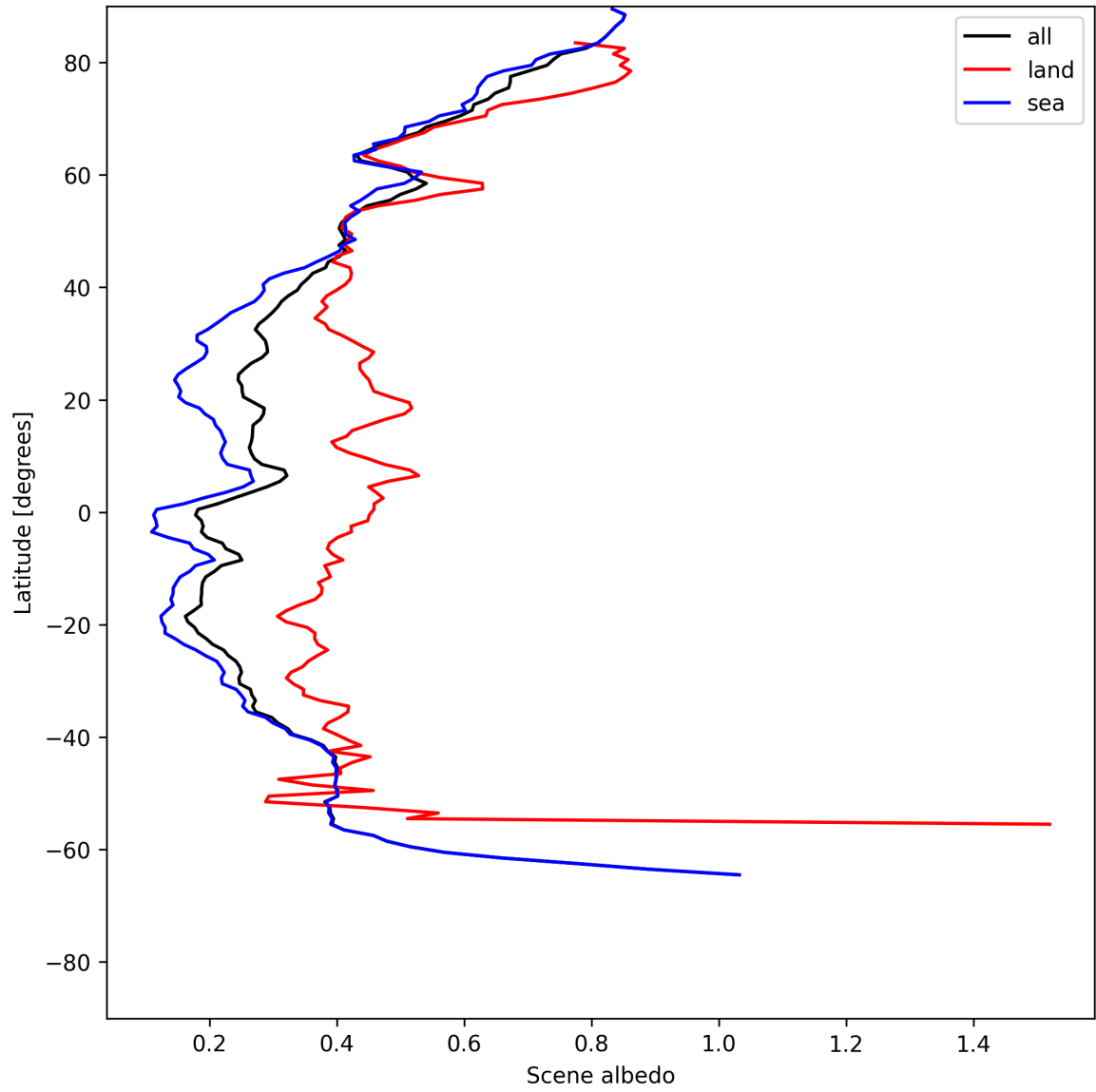
Figure 17: Zonal average of “Scene albedo” for 2025-06-13 to 2025-06-15.
