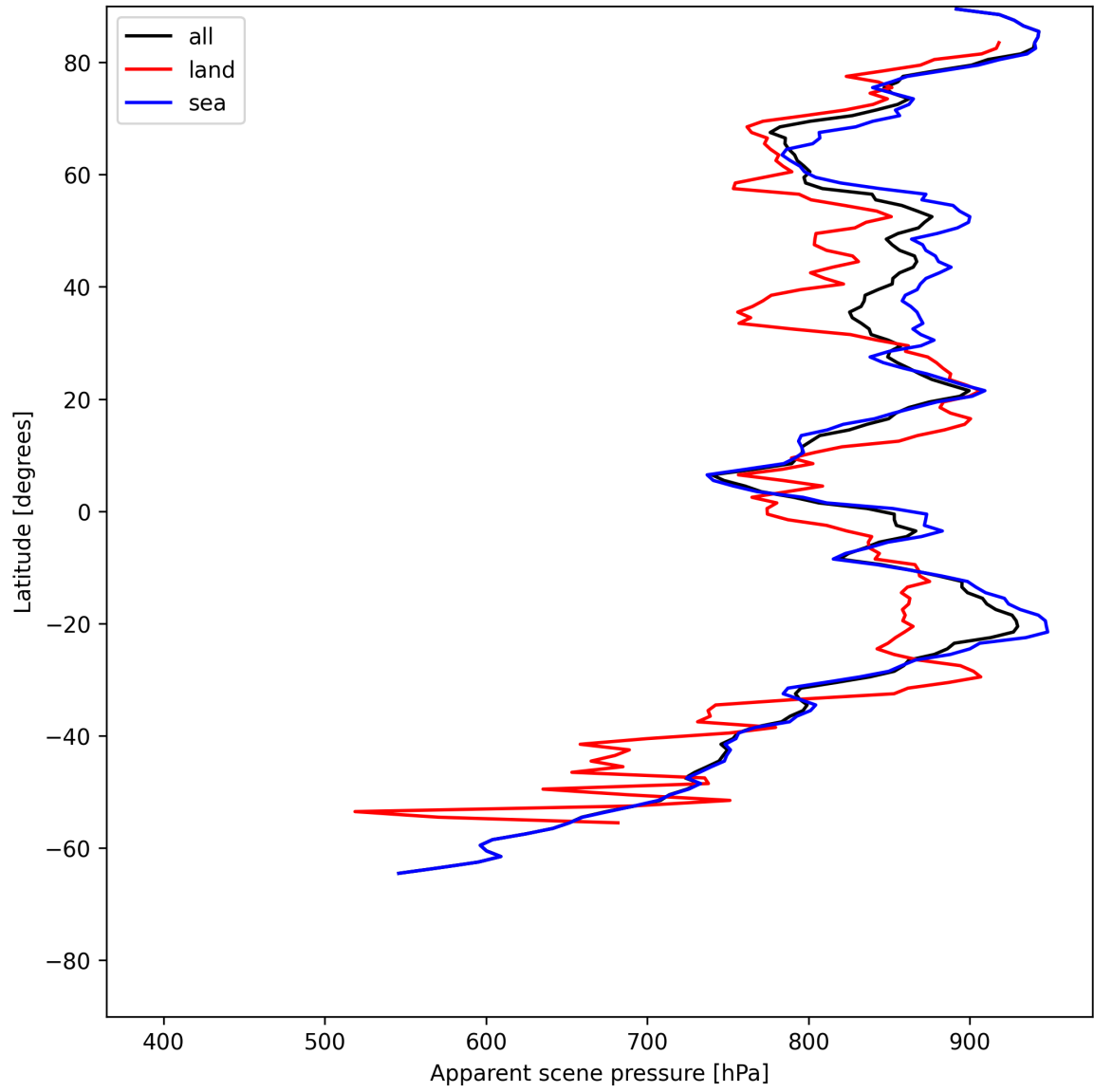
Figure 19: Zonal average of “Apparent scene pressure” for 2025-06-13 to 2025-06-15.
