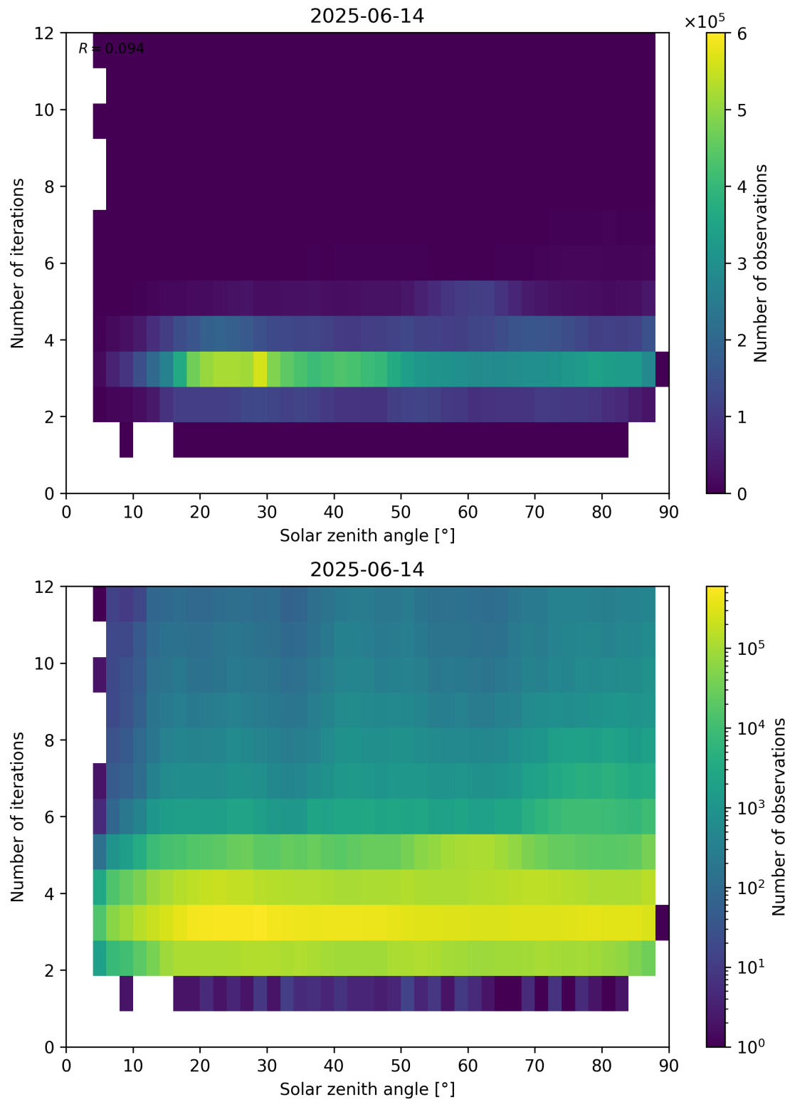
Figure 114: Scatter density plot of “Solar zenith angle” against “Number of iterations” for 2025-06-13 to 2025-06-15.
