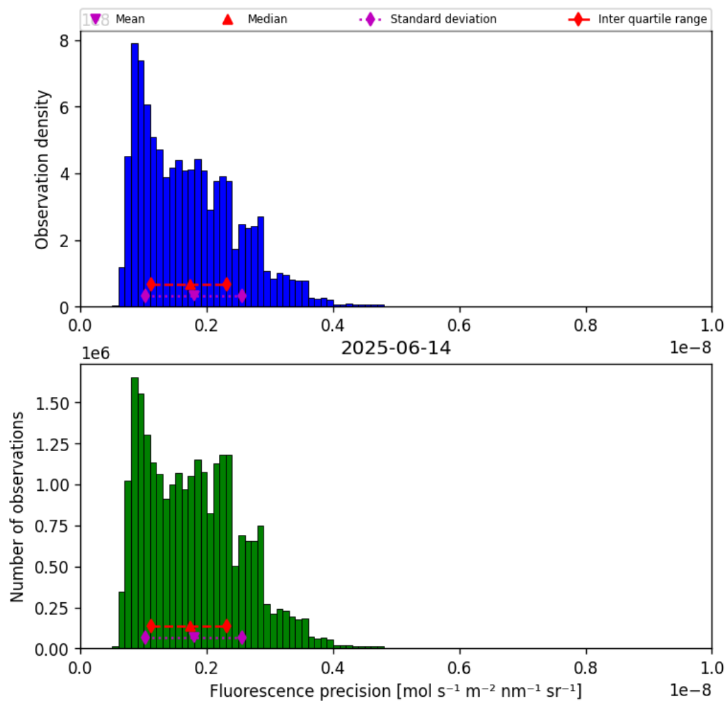
Figure 41: Histogram of “Fluorescence precision” for 2025-06-13 to 2025-06-15
