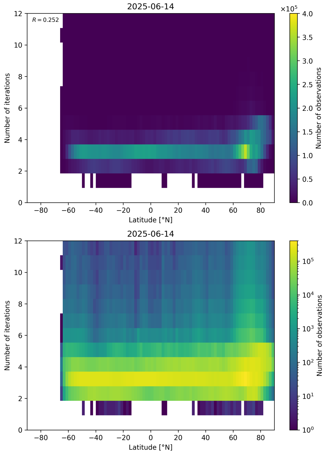
Figure 93: Scatter density plot of “Latitude” against “Number of iterations” for 2025-06-13 to 2025-06-15.
