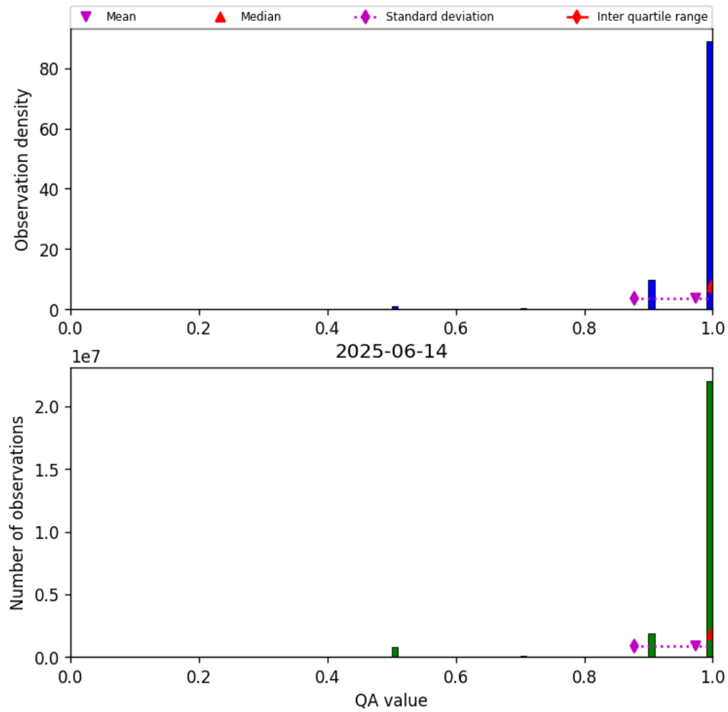
Figure 29: Histogram of “QA value” for 2025-06-13 to 2025-06-15
