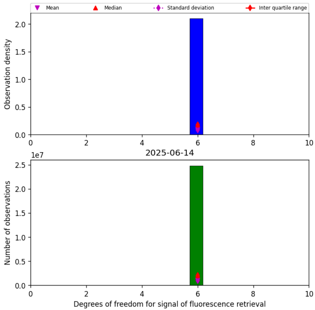
Figure 43: Histogram of "Degrees of freedom for signal of fluorescence retrieval" for 2025-06-13 to 2025-06-15
