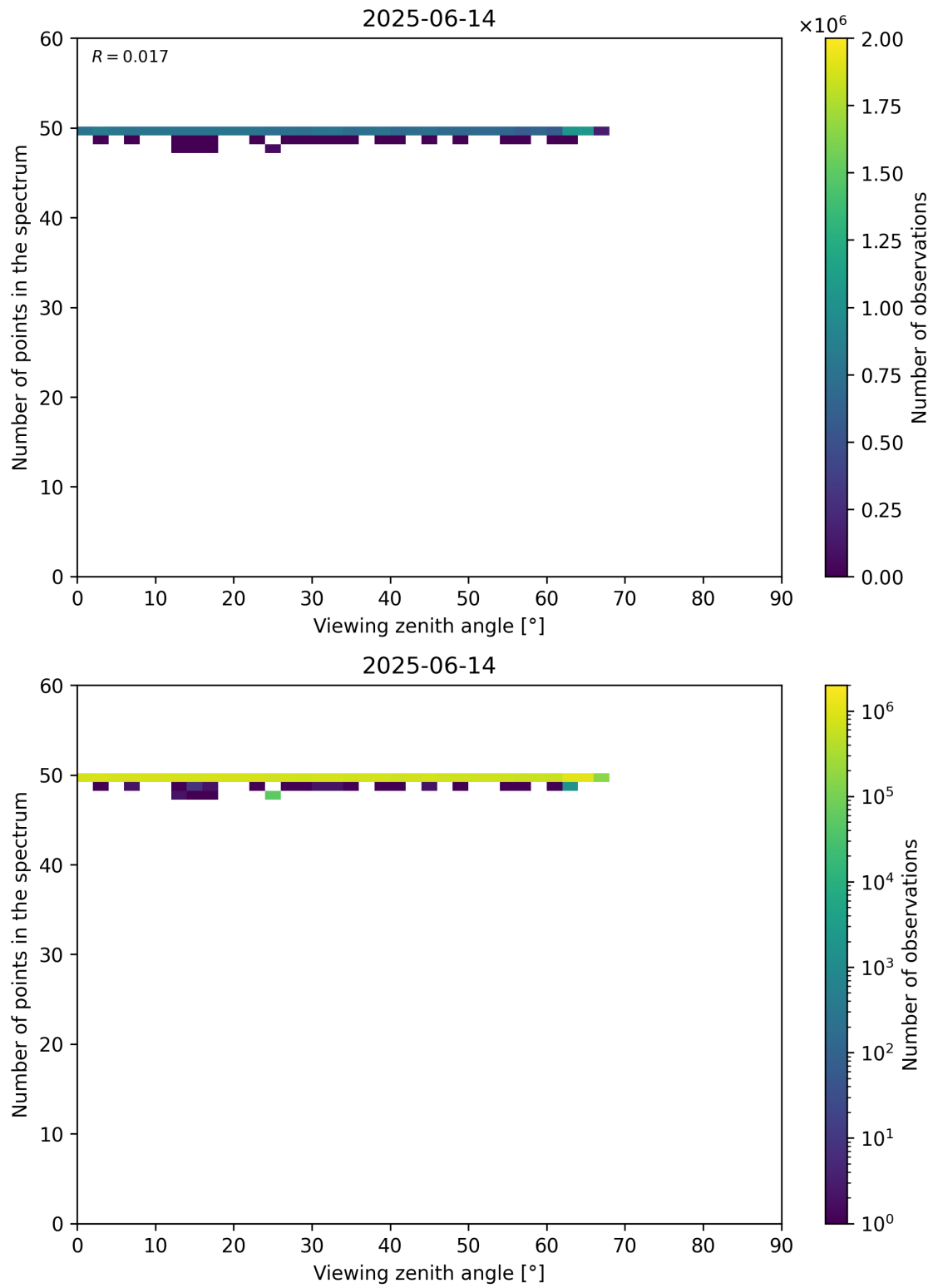
Figure 125: Scatter density plot of “Viewing zenith angle” against “Number of points in the spectrum” for 2025-06-13 to 2025-06-15.
