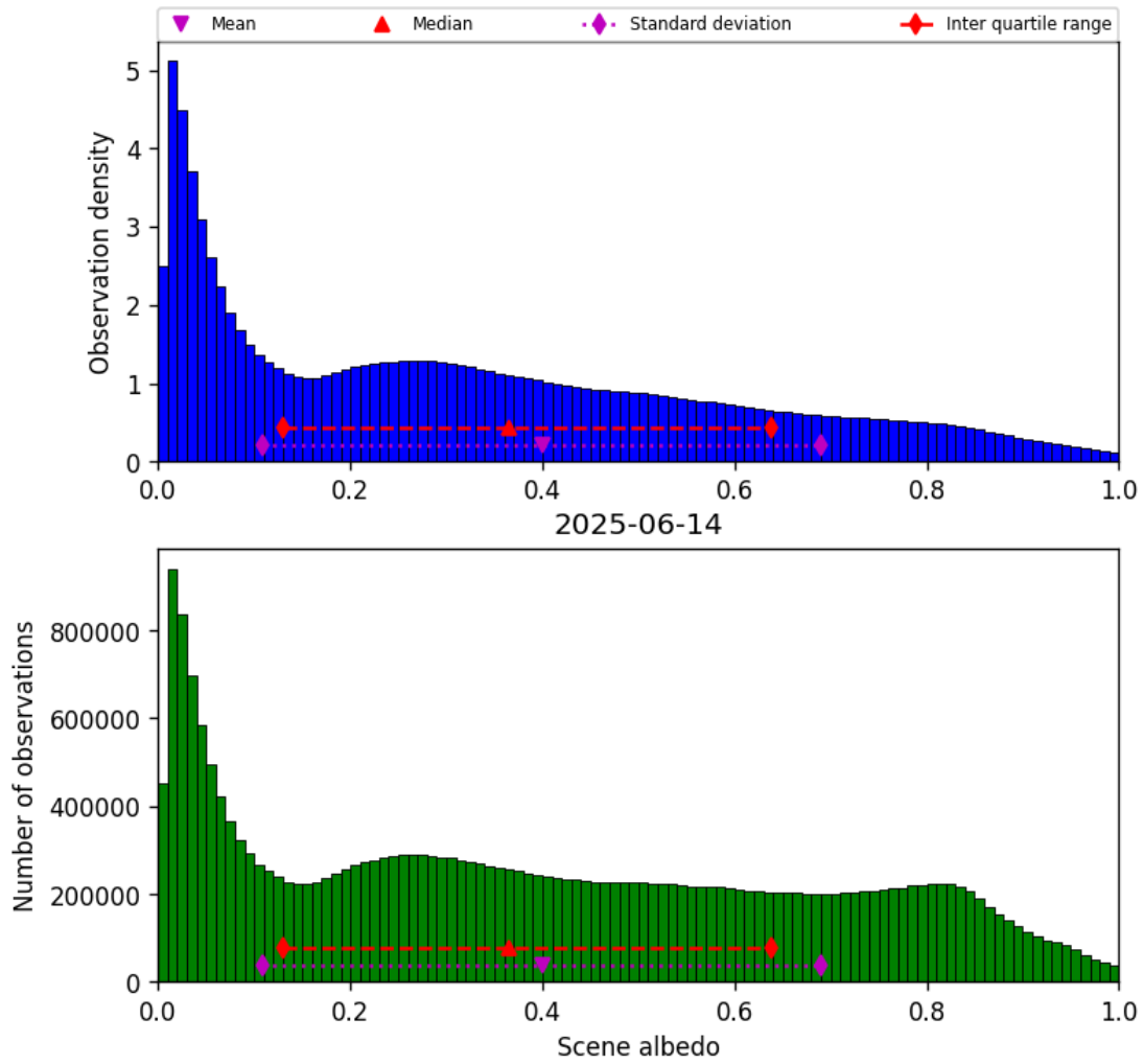
Figure 34: Histogram of “Scene albedo” for 2025-06-13 to 2025-06-15
