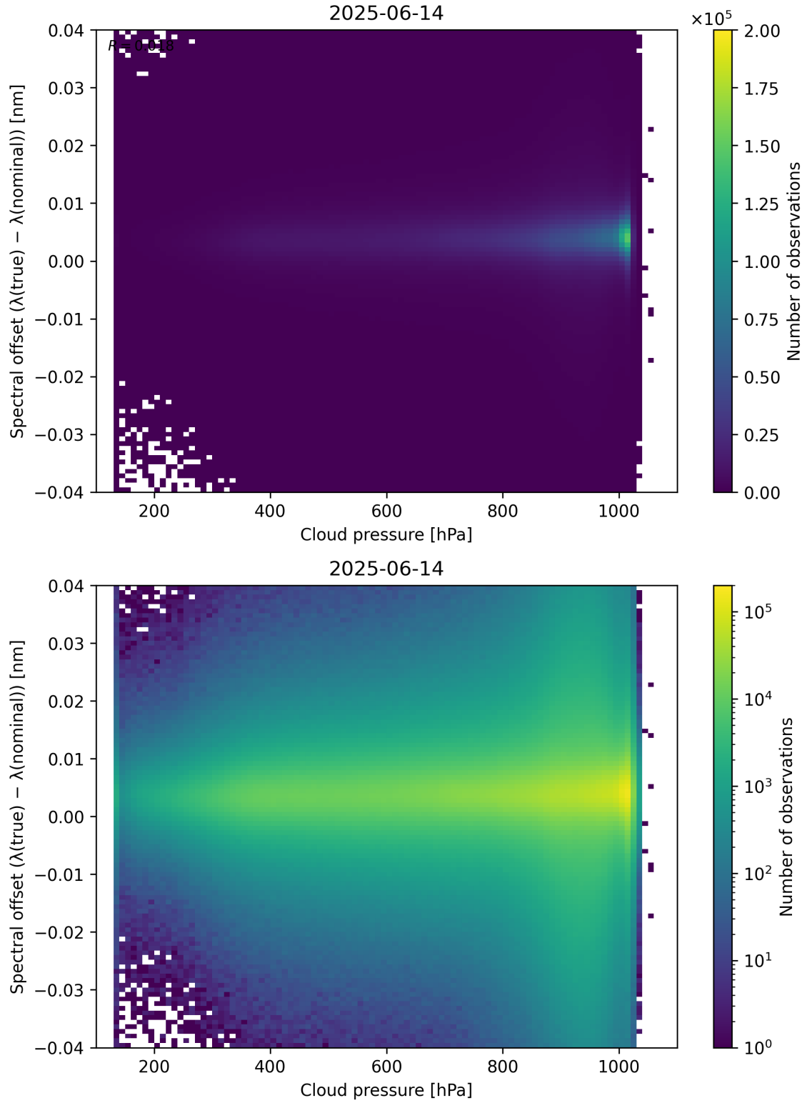
Figure 84: Scatter density plot of “Cloud pressure” against “Spectral offset ( \lambda_{\text{true}} - \lambda_{\text{nominal}} )” for 2025-06-13 to 2025-06-15.
