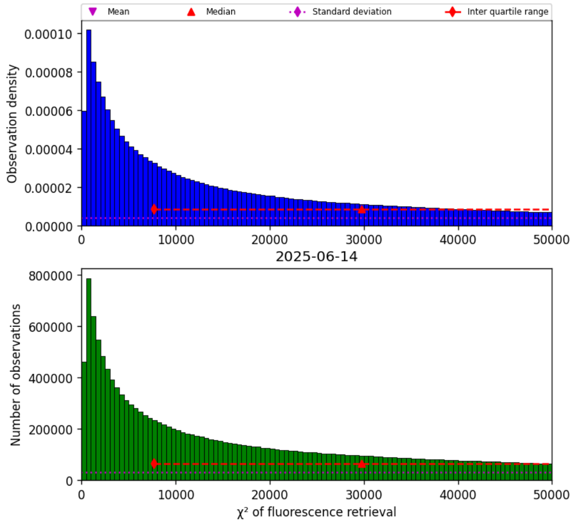
Figure 42: Histogram of “ \chi^2 of fluorescence retrieval” for 2025-06-13 to 2025-06-15
