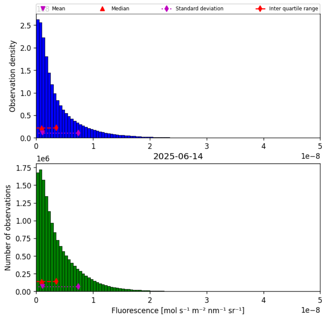
Figure 40: Histogram of “Fluorescence” for 2025-06-13 to 2025-06-15
