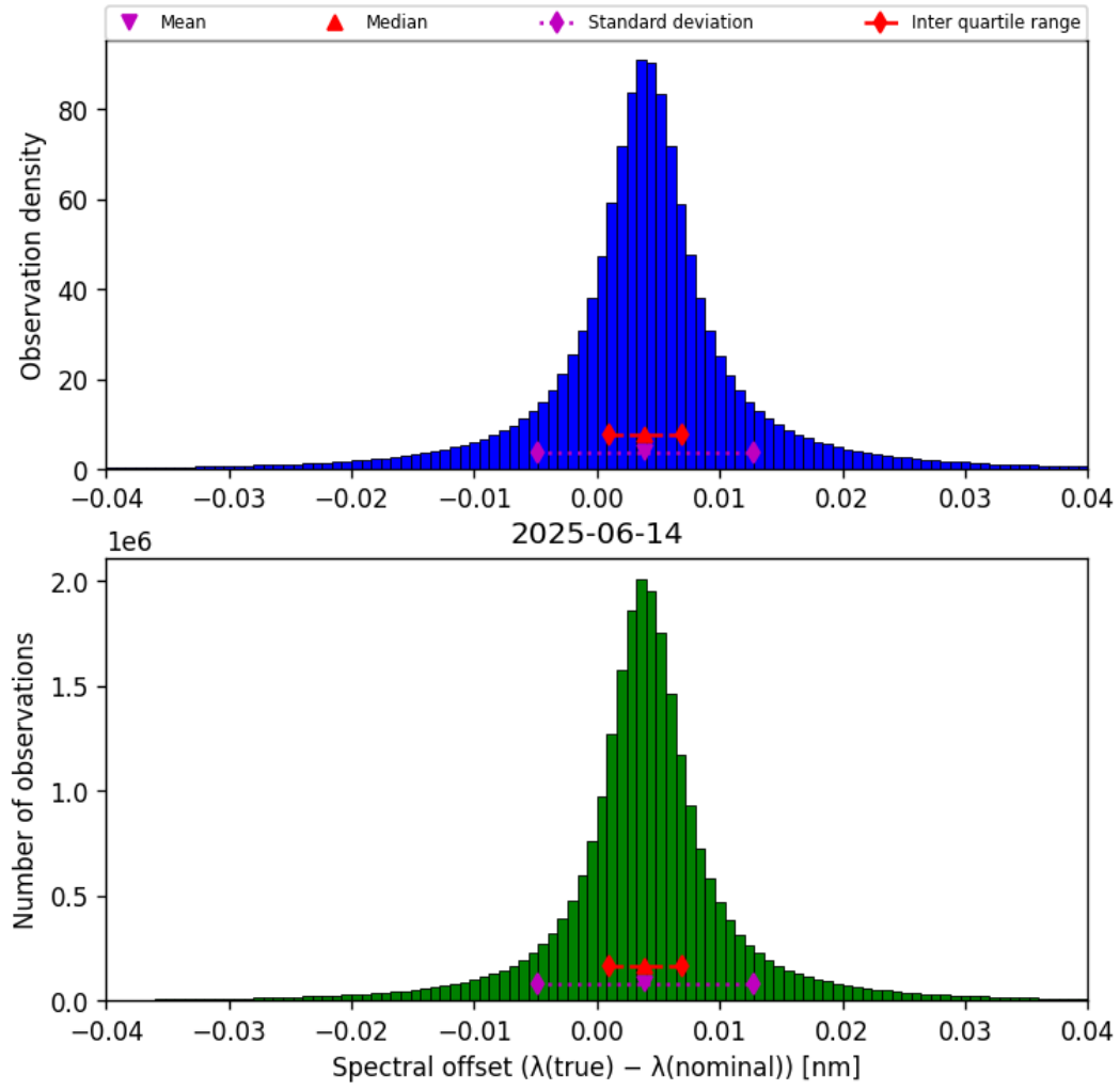
Figure 45: Histogram of “Spectral offset ( \lambda_{\text{true}} - \lambda_{\text{nominal}} )” for 2025-06-13 to 2025-06-15
