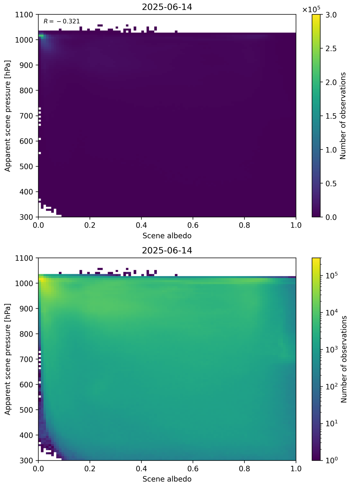
Figure 102: Scatter density plot of “Scene albedo” against “Apparent scene pressure” for 2025-06-13 to 2025-06-15.
