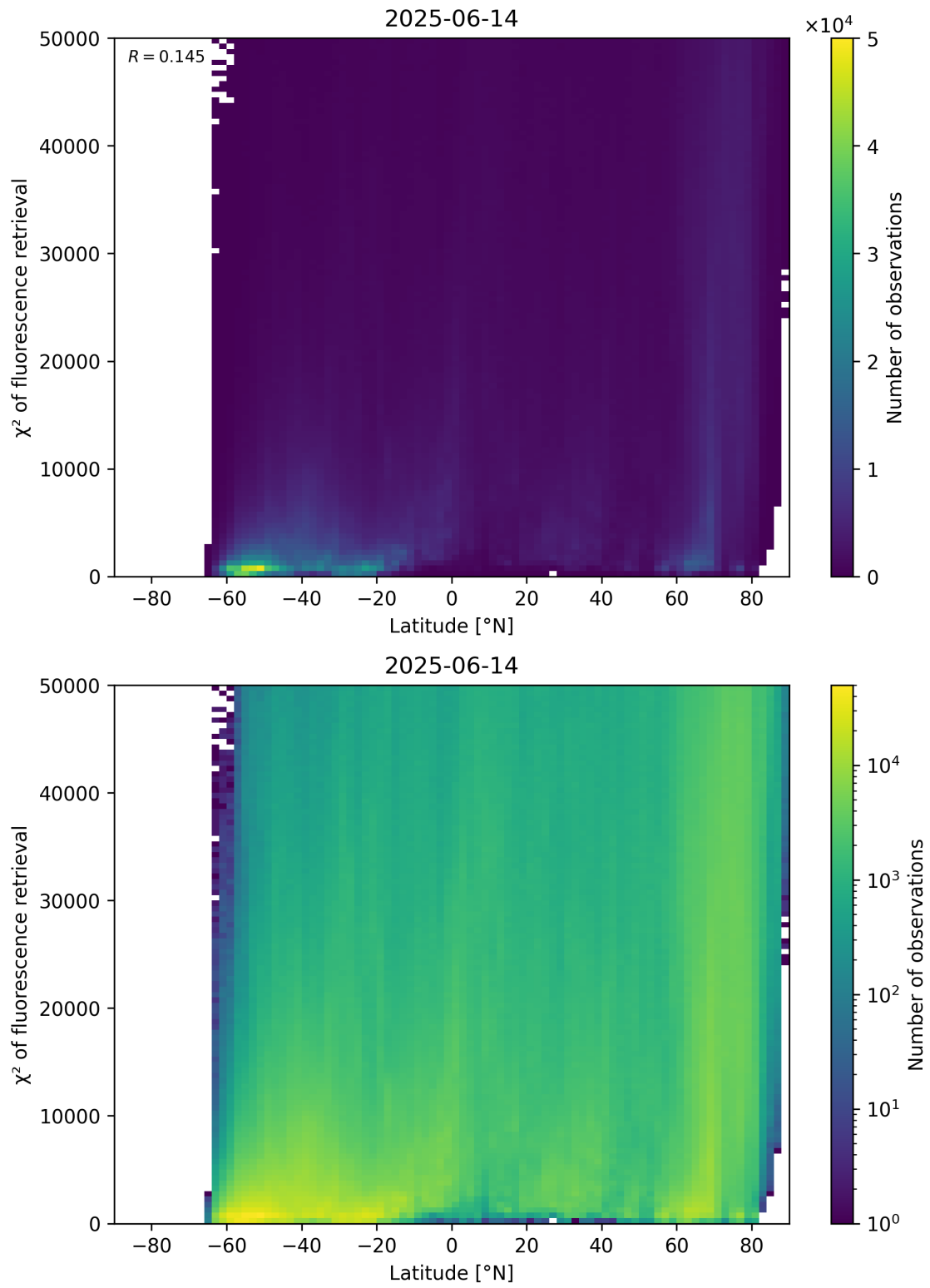
Figure 89: Scatter density plot of “Latitude” against “ \chi^2 of fluorescence retrieval” for 2025-06-13 to 2025-06-15.
