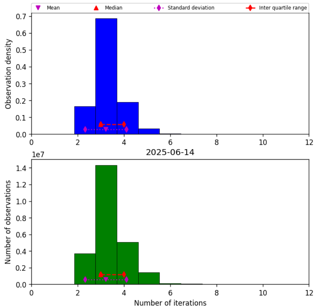
Figure 39: Histogram of “Number of iterations” for 2025-06-13 to 2025-06-15
