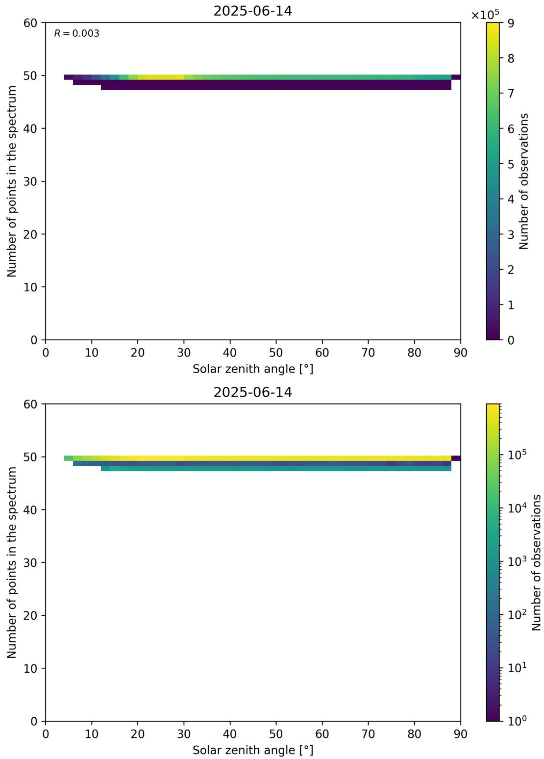
Figure 115: Scatter density plot of “Solar zenith angle” against “Number of points in the spectrum” for 2025-06-13 to 2025-06-15.
