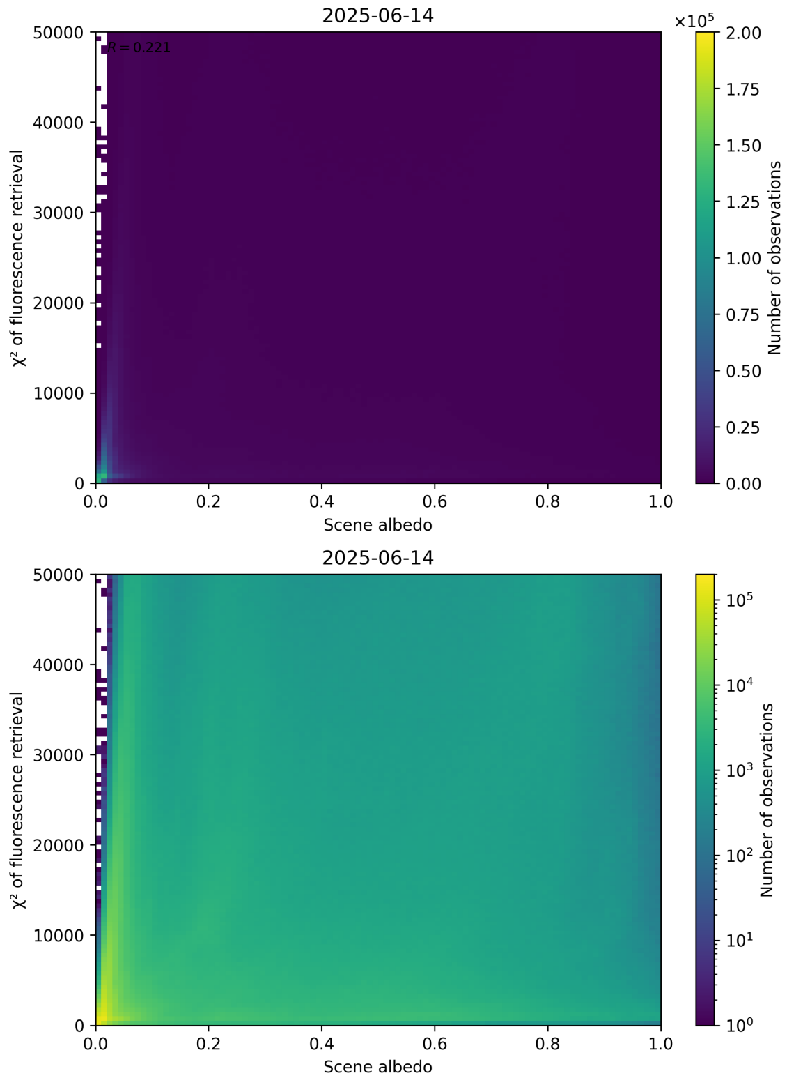
Figure 103: Scatter density plot of “Scene albedo” against “ \chi^2 of fluorescence retrieval” for 2025-06-13 to 2025-06-15.
