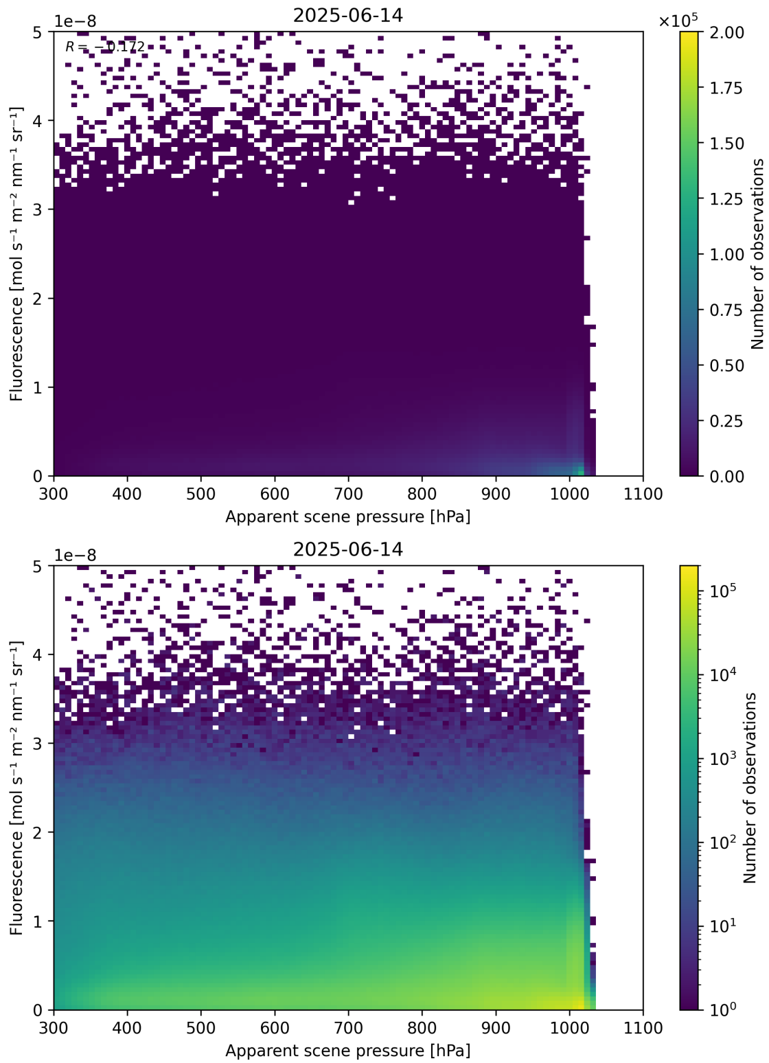
Figure 64: Scatter density plot of “Apparent scene pressure” against “Fluorescence” for 2025-06-13 to 2025-06-15.
