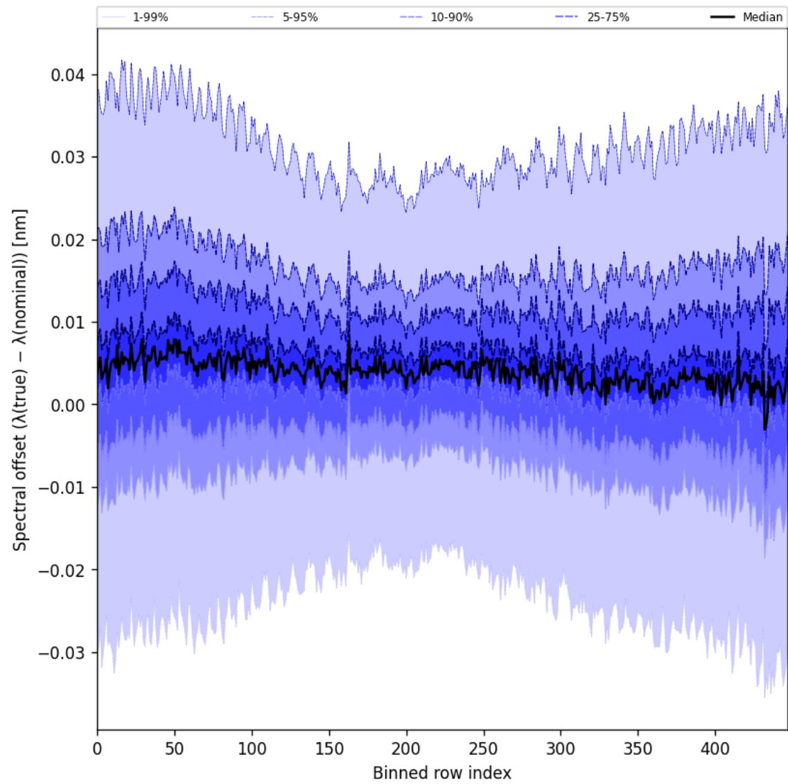
Figure 62: Along track statistics of “Spectral offset ( \lambda_{\text{true}} - \lambda_{\text{nominal}} )” for 2025-06-13 to 2025-06-15
