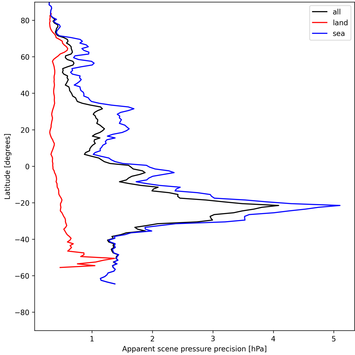
Figure 20: Zonal average of “Apparent scene pressure precision” for 2025-06-13 to 2025-06-15.
