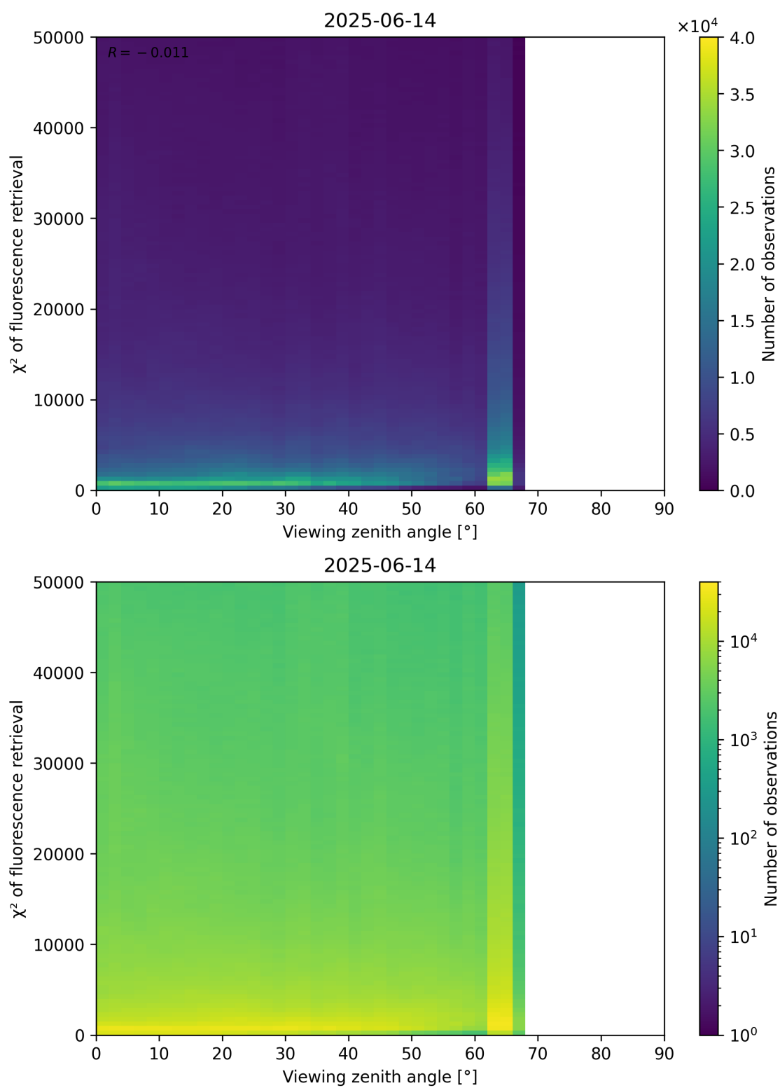
Figure 119: Scatter density plot of “Viewing zenith angle” against “ \chi^2 of fluorescence retrieval” for 2025-06-13 to 2025-06-15.
