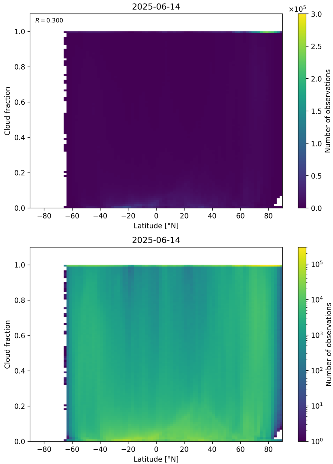
Figure 90: Scatter density plot of “Latitude” against “Cloud fraction” for 2025-06-13 to 2025-06-15.
