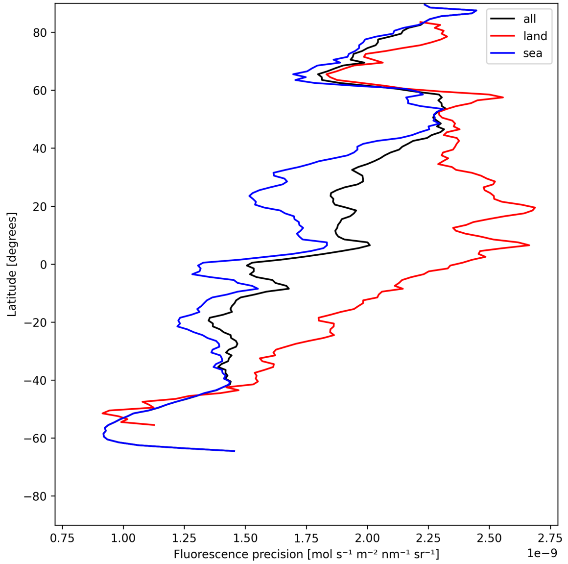
Figure 24: Zonal average of “Fluorescence precision” for 2025-06-13 to 2025-06-15.
