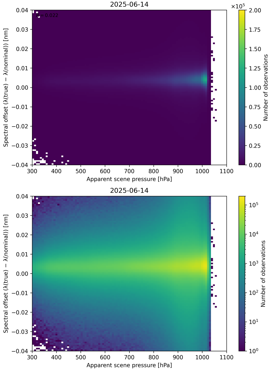
Figure 67: Scatter density plot of “Apparent scene pressure” against “Spectral offset ( \lambda_{\text{true}} - \lambda_{\text{nominal}} )” for 2025-06-13 to 2025-06-15.
