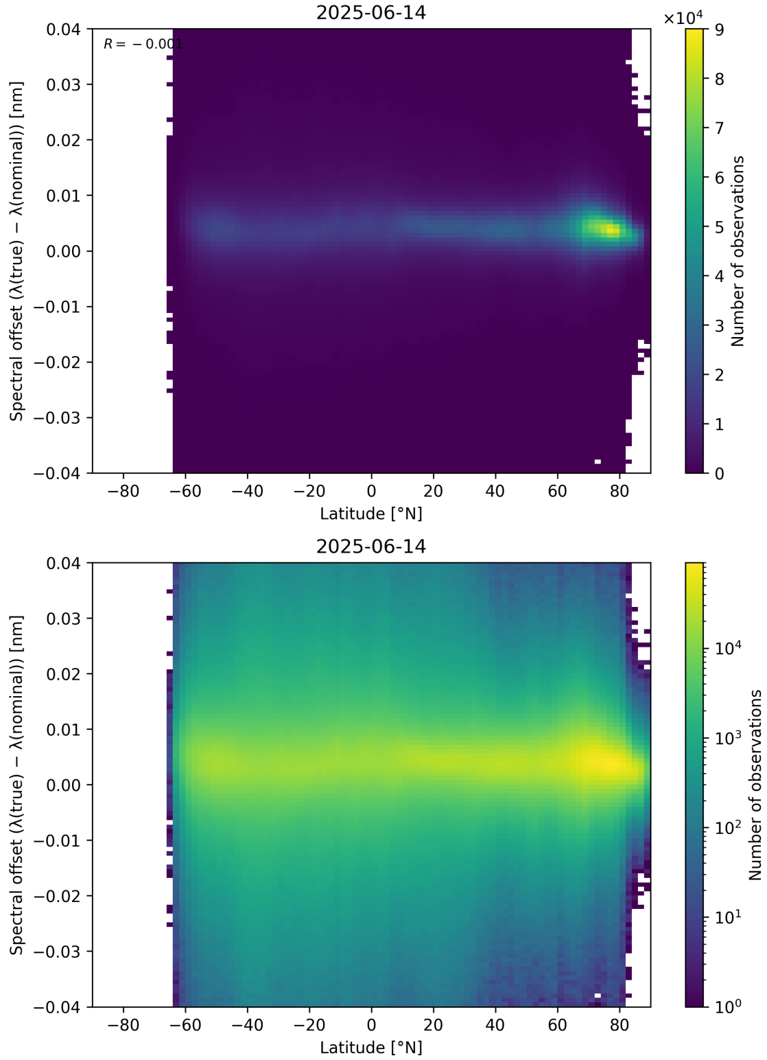
Figure 96: Scatter density plot of “Latitude” against “Spectral offset ( \lambda_{\text{true}} - \lambda_{\text{nominal}} )” for 2025-06-13 to 2025-06-15.
