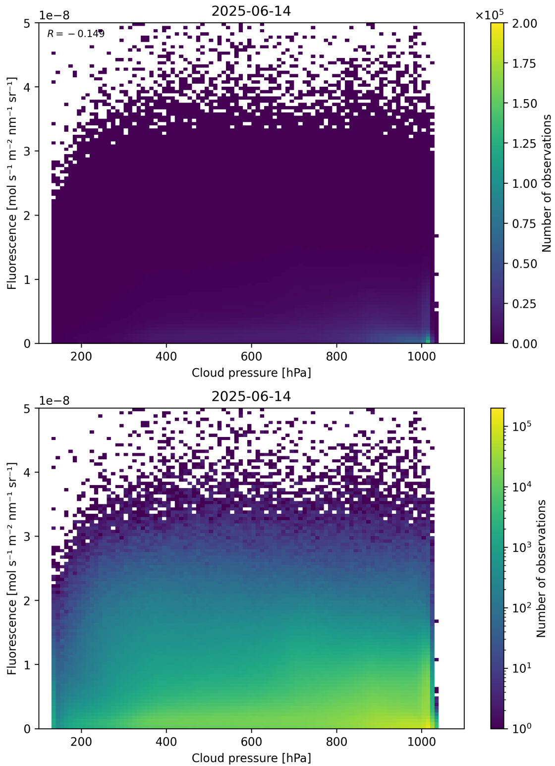
Figure 80: Scatter density plot of “Cloud pressure” against “Fluorescence” for 2025-06-13 to 2025-06-15.
