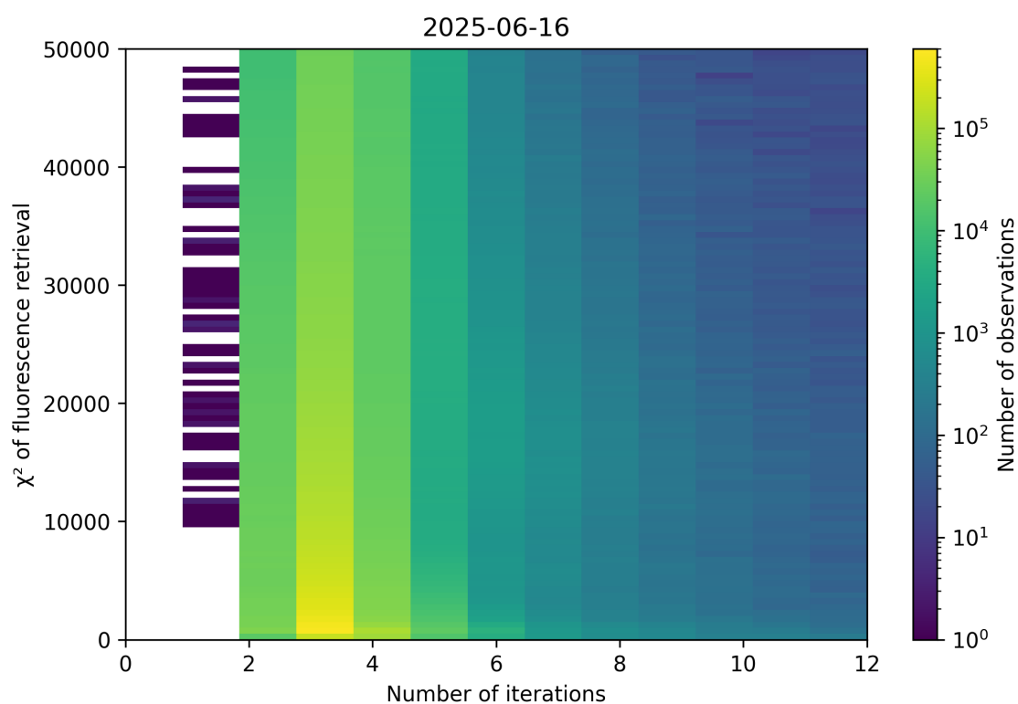
Figure 97: Scatter density plot of “Number of iterations” against “ \chi^2 of fluorescence retrieval” for 2025-06-16 to 2025-06-17.
