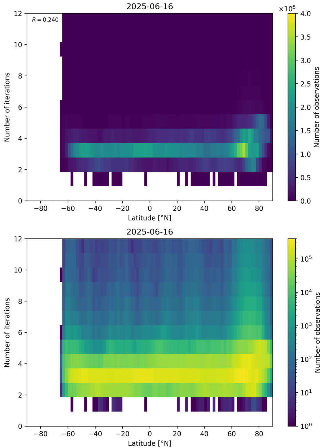
Figure 93: Scatter density plot of “Latitude” against “Number of iterations” for 2025-06-16 to 2025-06-17.
