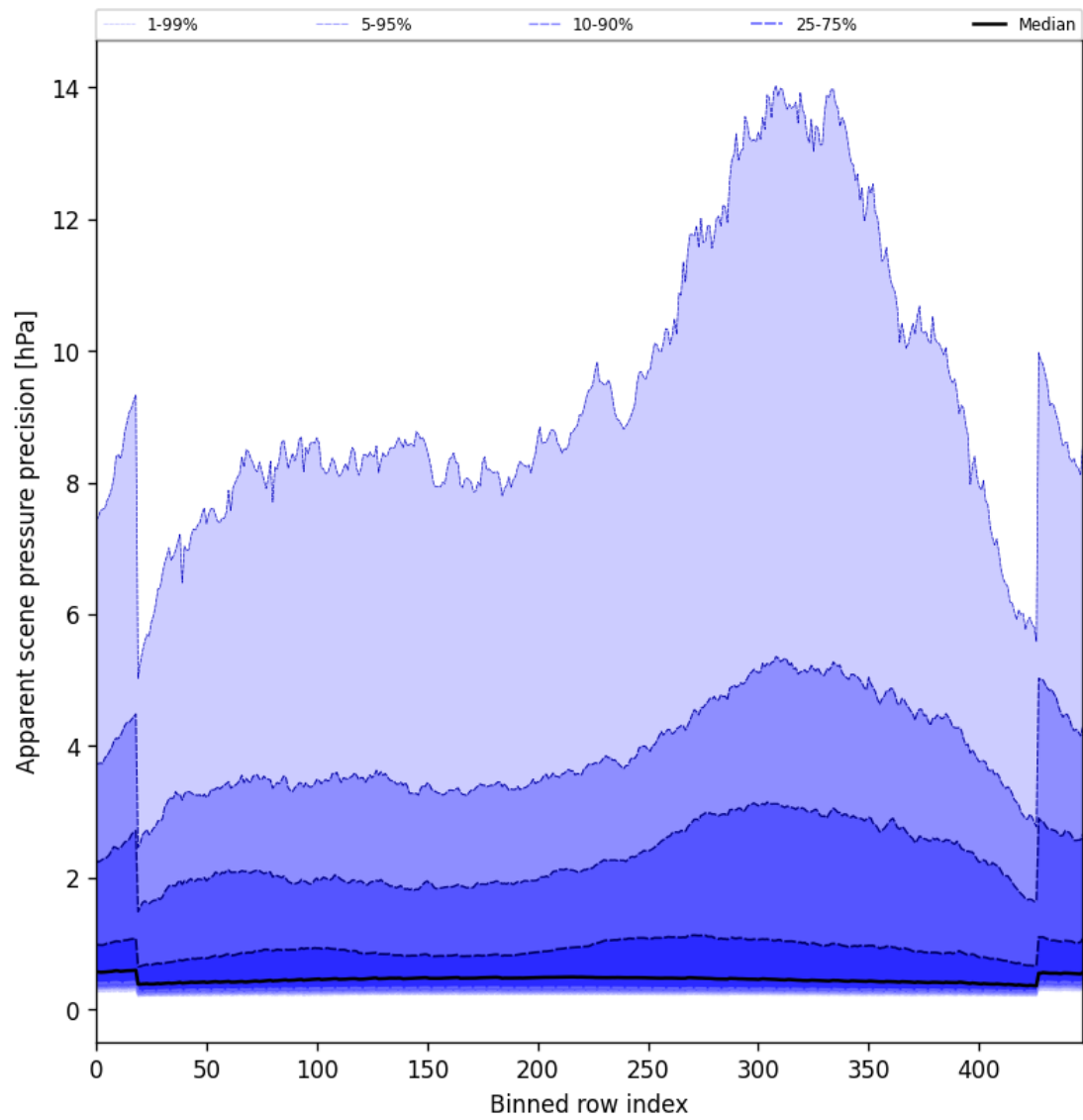
Figure 54: Along track statistics of “Apparent scene pressure precision” for 2025-06-16 to 2025-06-17
