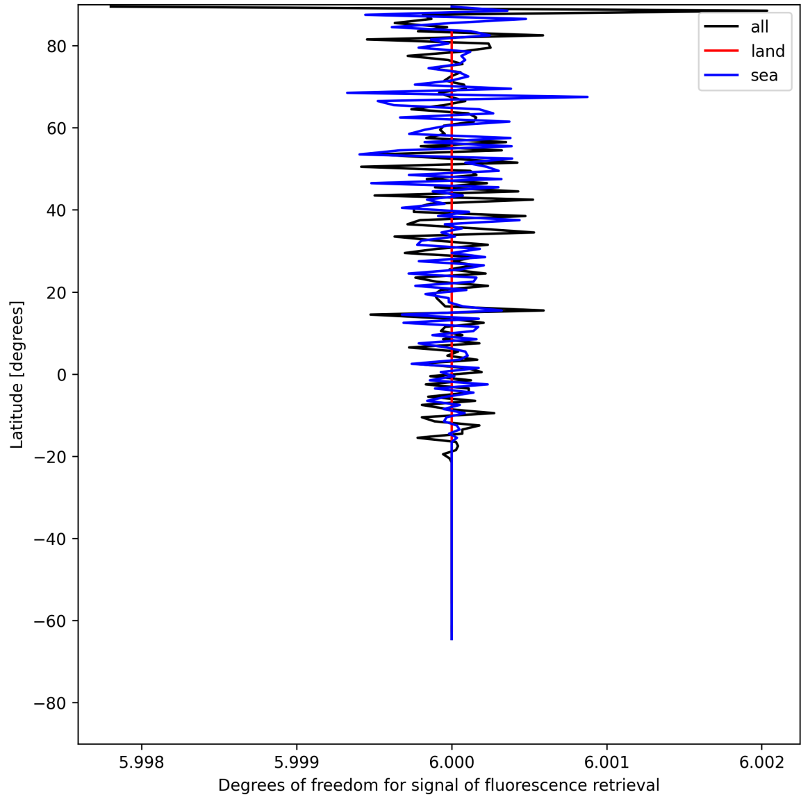
Figure 26: Zonal average of “Degrees of freedom for signal of fluorescence retrieval” for 2025-06-16 to 2025-06-17.
