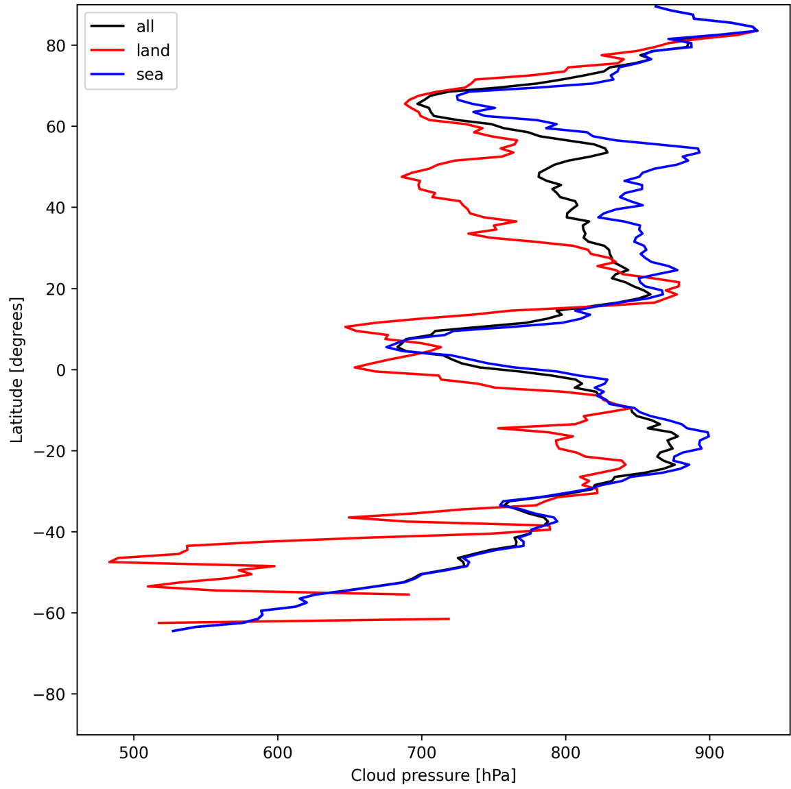
Figure 13: Zonal average of “Cloud pressure” for 2025-06-16 to 2025-06-17.
