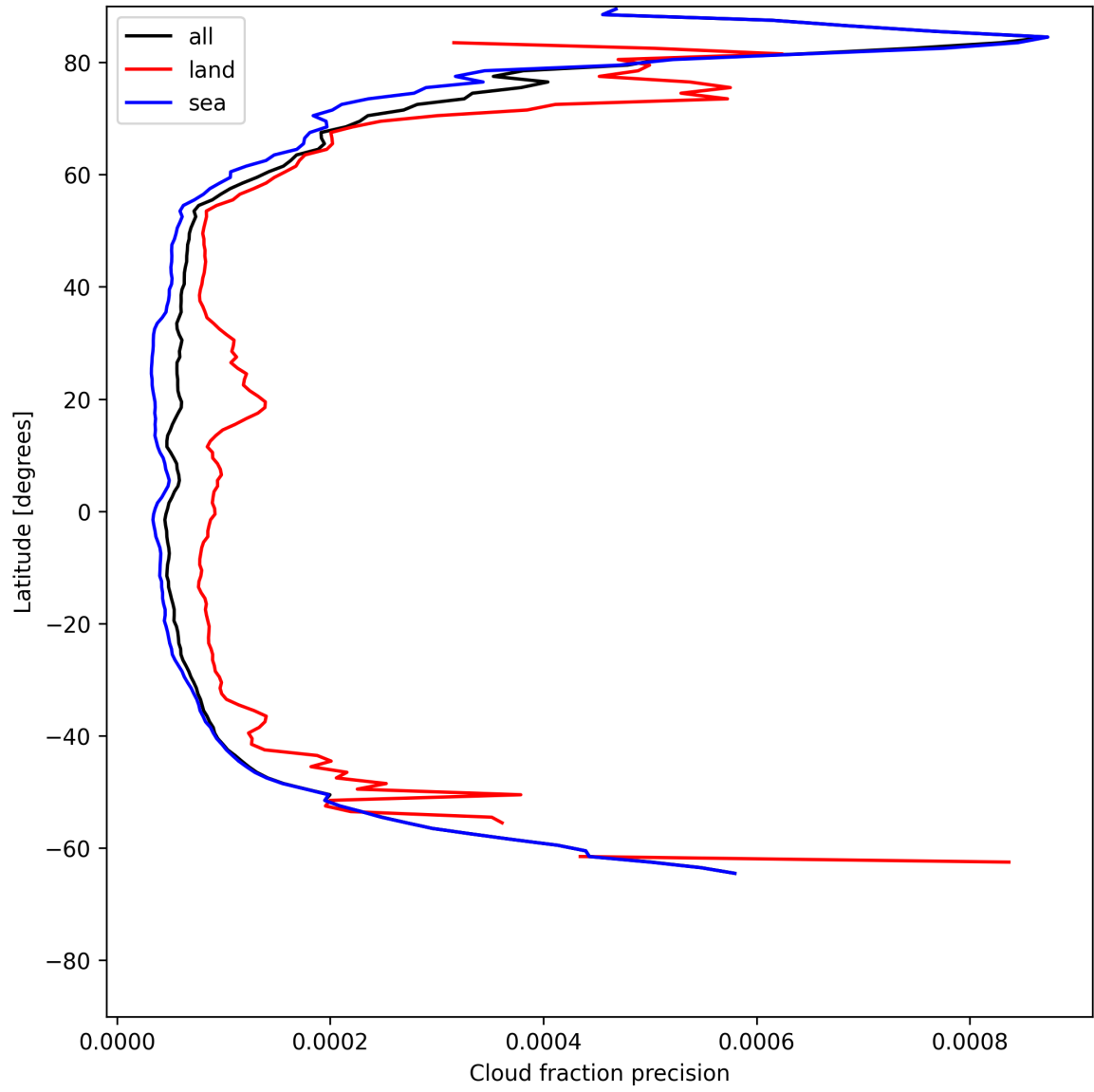
Figure 16: Zonal average of “Cloud fraction precision” for 2025-06-16 to 2025-06-17.
