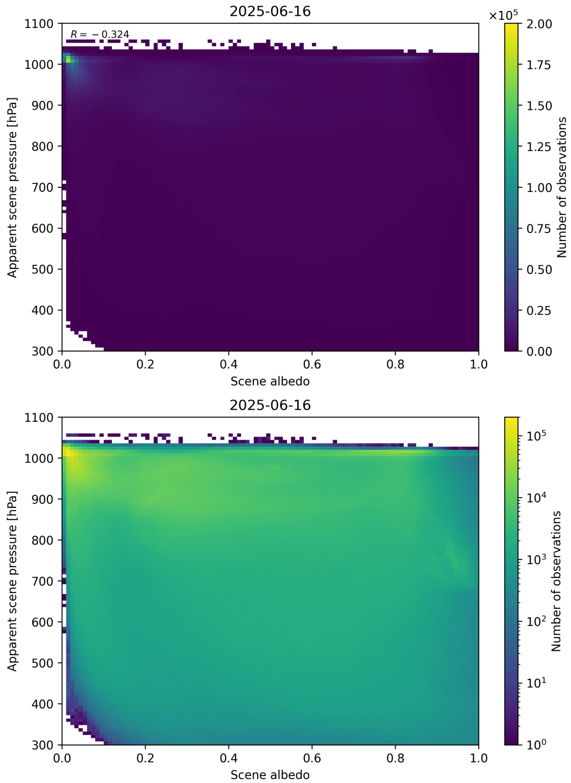
Figure 102: Scatter density plot of “Scene albedo” against “Apparent scene pressure” for 2025-06-16 to 2025-06-17.
