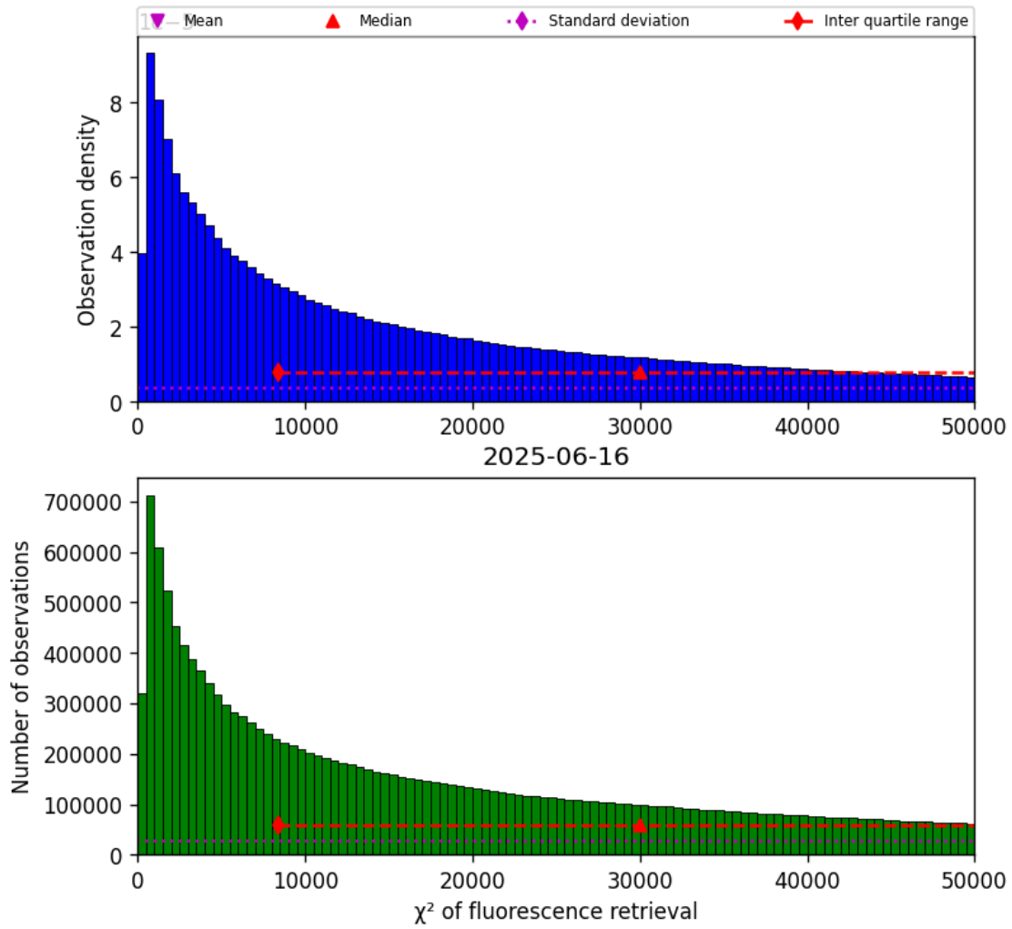
Figure 42: Histogram of “ \chi^2 of fluorescence retrieval” for 2025-06-16 to 2025-06-17
