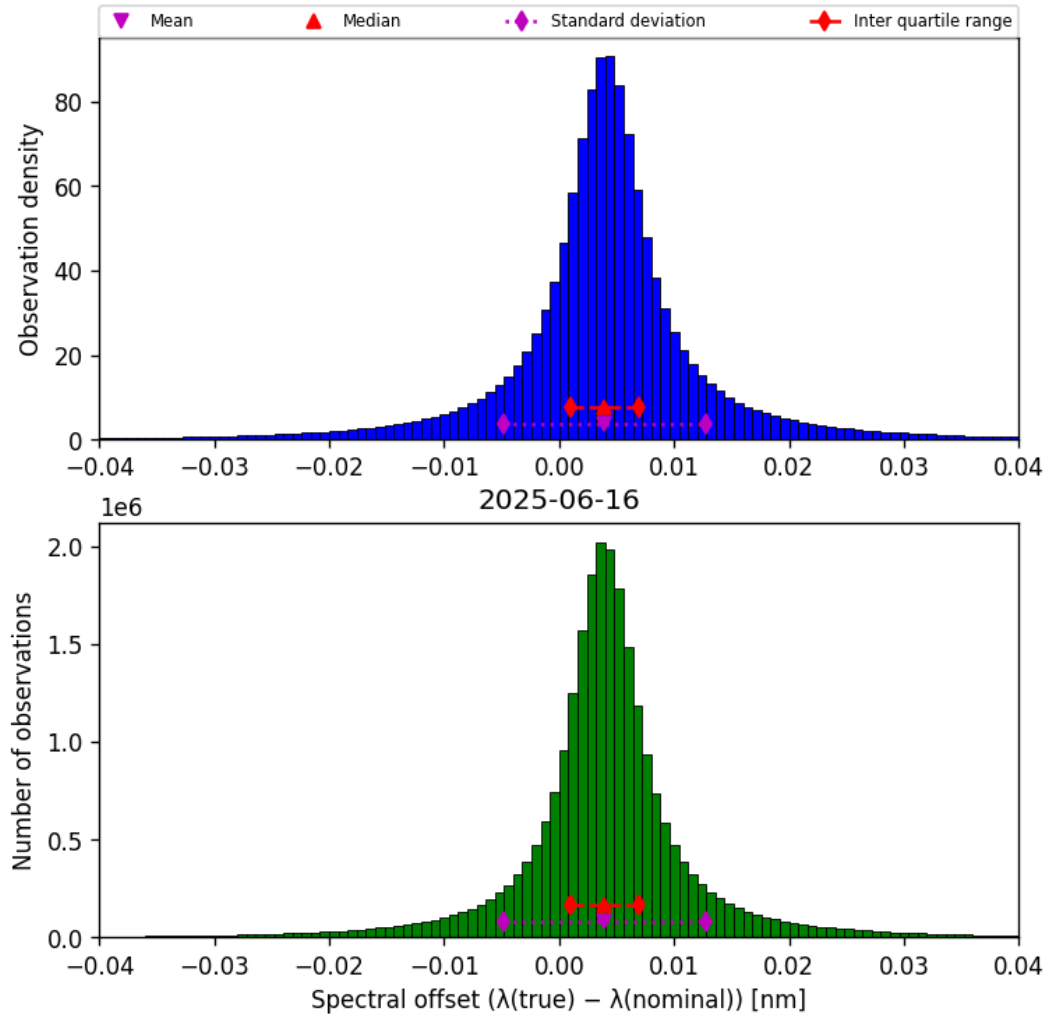
Figure 45: Histogram of “Spectral offset ( \lambda_{\text{true}} - \lambda_{\text{nominal}} )” for 2025-06-16 to 2025-06-17
