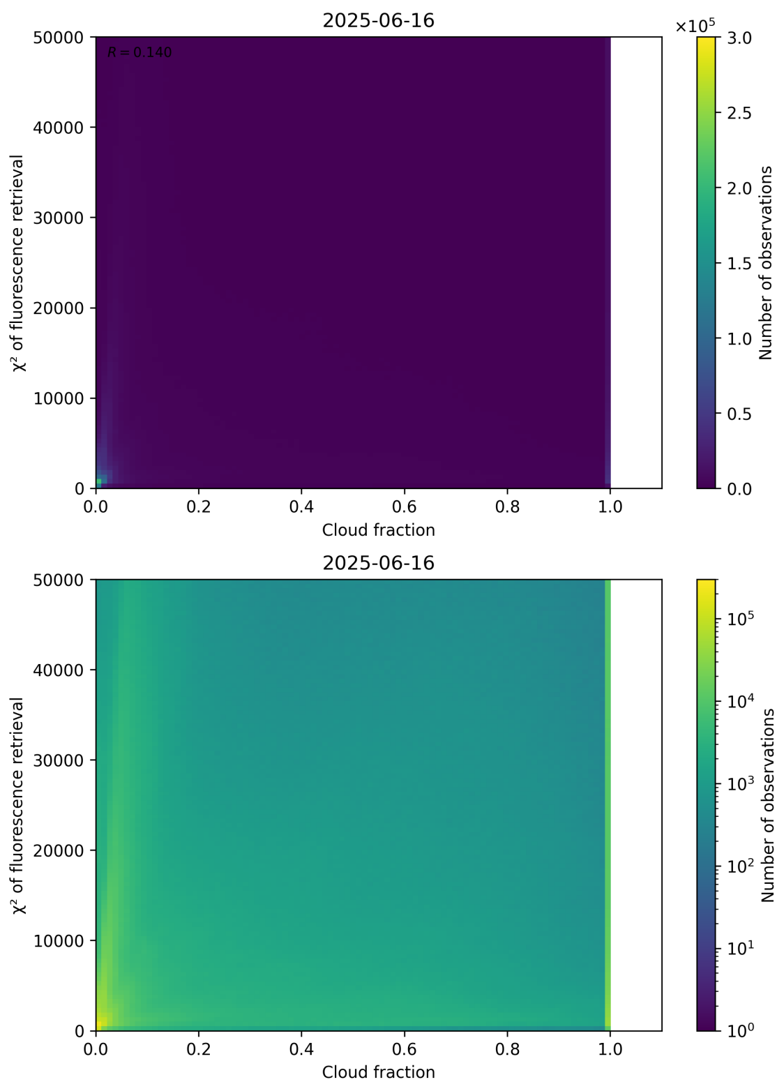
Figure 71: Scatter density plot of “Cloud fraction” against “ \chi^2 of fluorescence retrieval” for 2025-06-16 to 2025-06-17.
