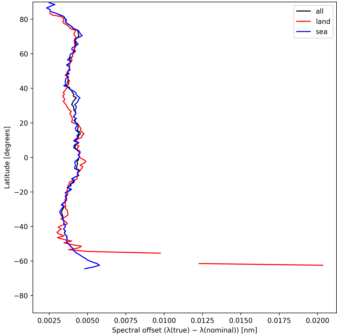
Figure 28: Zonal average of “Spectral offset ( \lambda_{\text{true}} - \lambda_{\text{nominal}} )” for 2025-06-16 to 2025-06-17.
