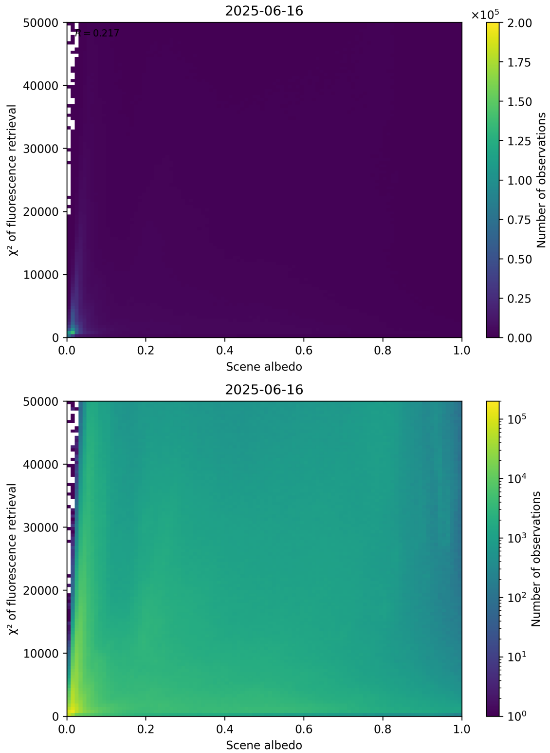
Figure 103: Scatter density plot of “Scene albedo” against “ \chi^2 of fluorescence retrieval” for 2025-06-16 to 2025-06-17.
