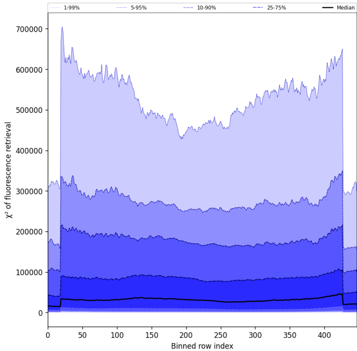
Figure 59: Along track statistics of “ \chi^2 of fluorescence retrieval” for 2025-06-16 to 2025-06-17
