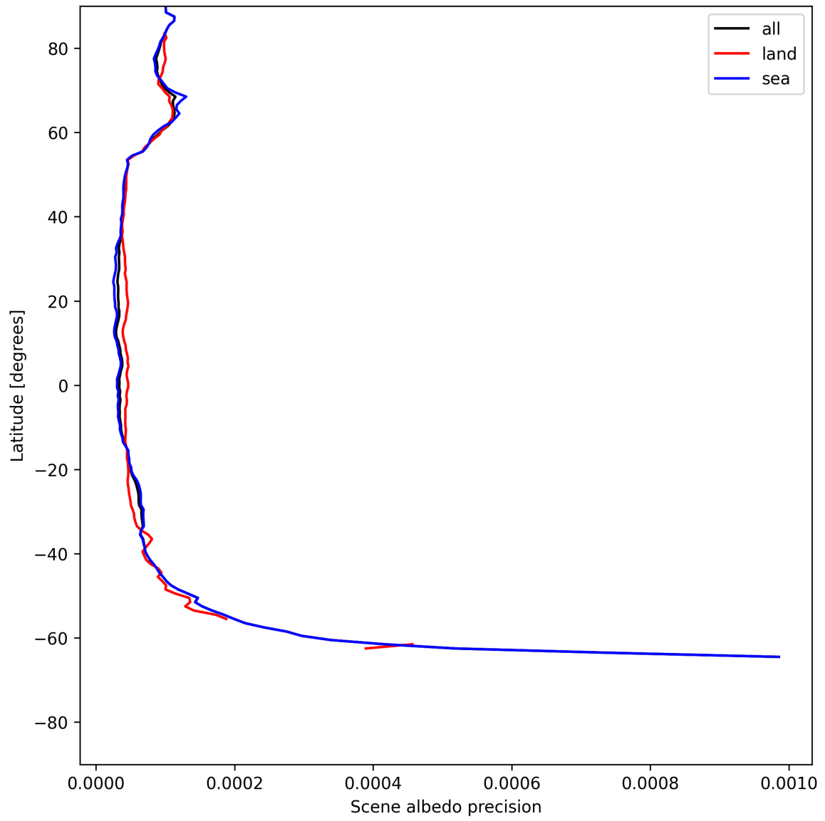
Figure 18: Zonal average of “Scene albedo precision” for 2025-06-16 to 2025-06-17.
