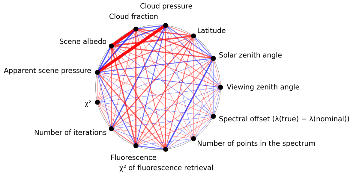
Figure 1: Map of correlation graph for 2025-06-16 to 2025-06-17.
