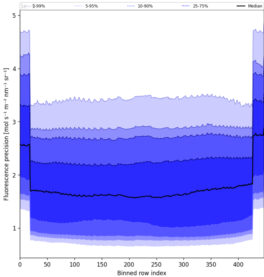
Figure 58: Along track statistics of “Fluorescence precision” for 2025-06-16 to 2025-06-17
