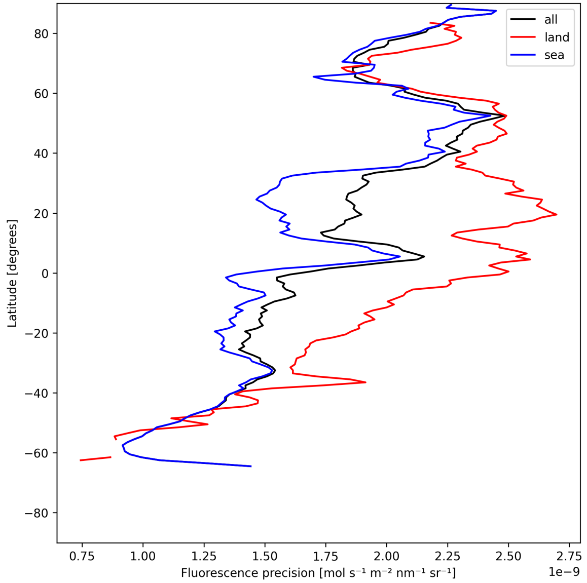
Figure 24: Zonal average of “Fluorescence precision” for 2025-06-16 to 2025-06-17.
