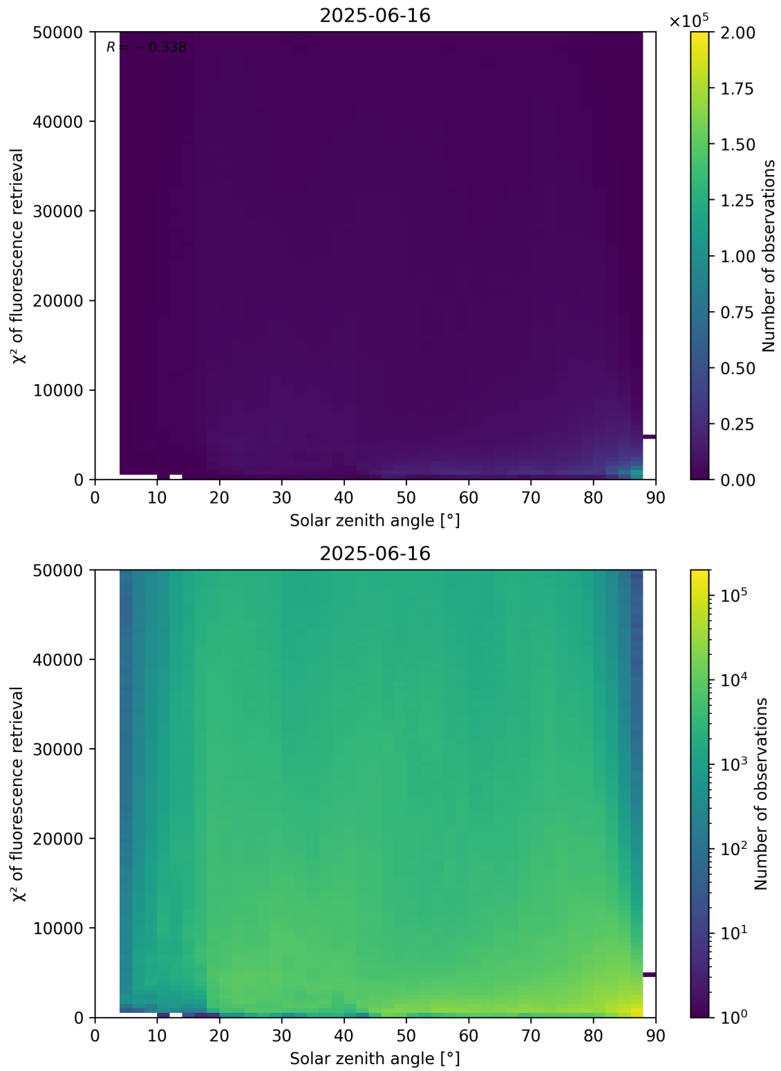
Figure 109: Scatter density plot of “Solar zenith angle” against “ \chi^2 of fluorescence retrieval” for 2025-06-16 to 2025-06-17.
