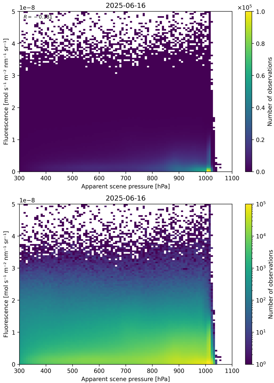
Figure 64: Scatter density plot of “Apparent scene pressure” against “Fluorescence” for 2025-06-16 to 2025-06-17.
