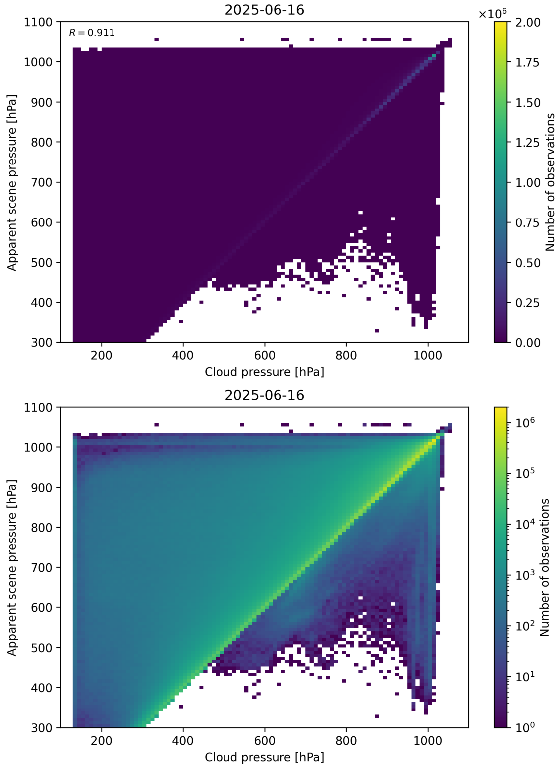
Figure 77: Scatter density plot of “Cloud pressure” against “Apparent scene pressure” for 2025-06-16 to 2025-06-17.
