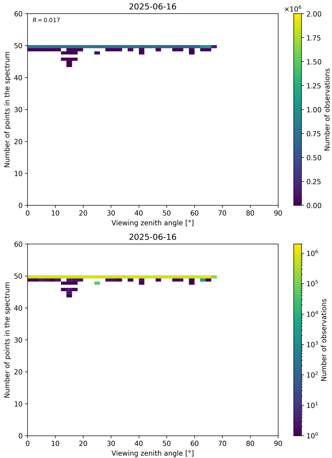
Figure 125: Scatter density plot of “Viewing zenith angle” against “Number of points in the spectrum” for 2025-06-16 to 2025-06-17.
