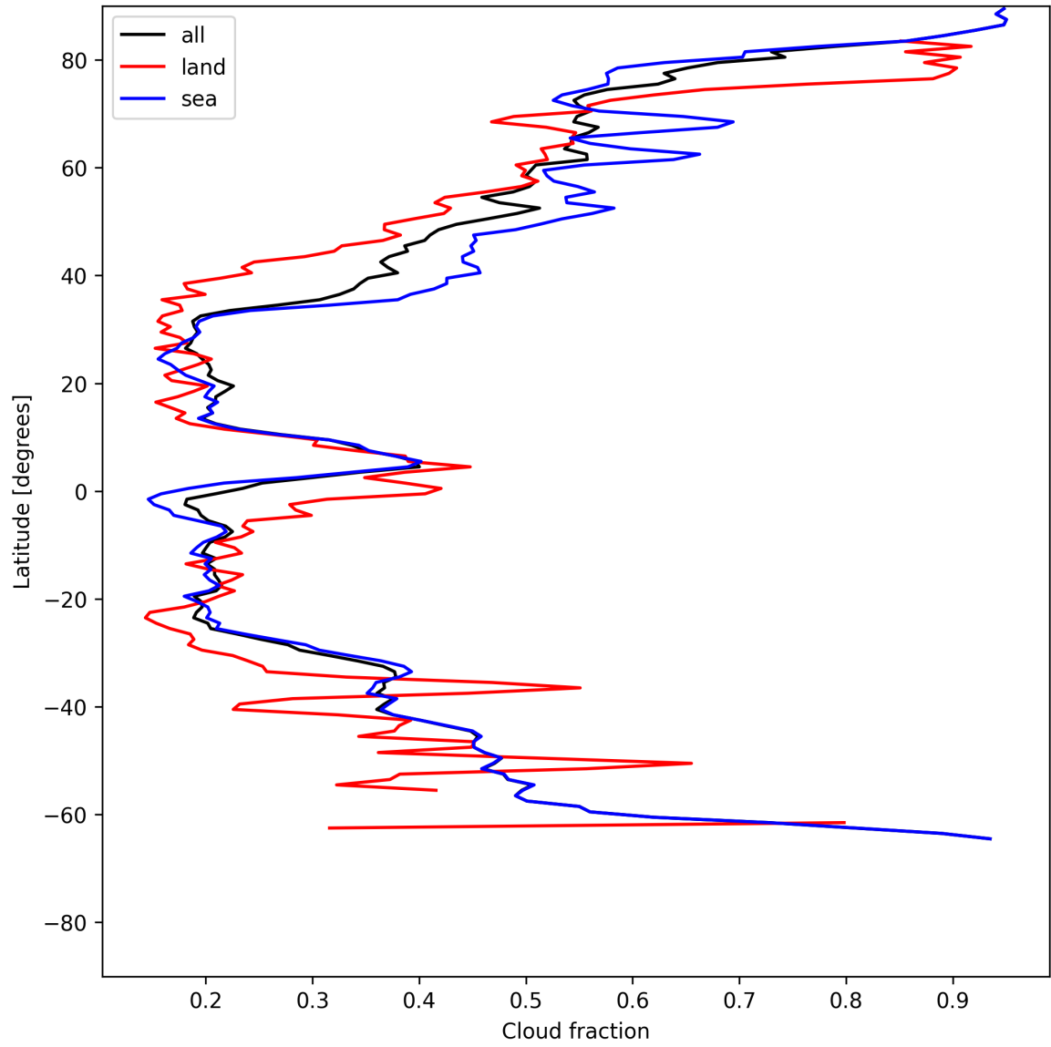
Figure 15: Zonal average of “Cloud fraction” for 2025-06-16 to 2025-06-17.
