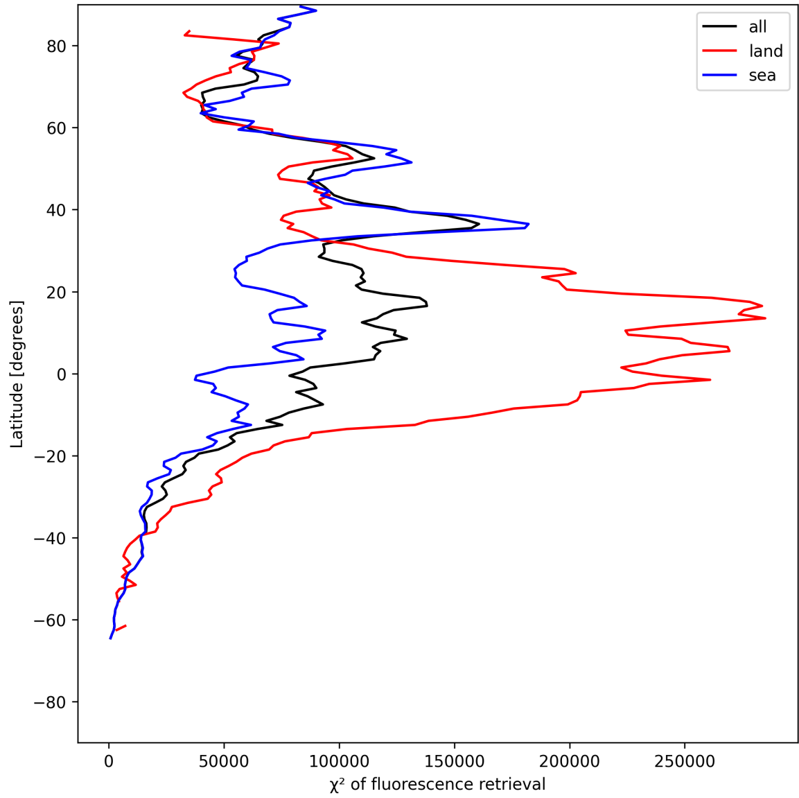
Figure 25: Zonal average of “ \chi^2 of fluorescence retrieval” for 2025-06-16 to 2025-06-17.
