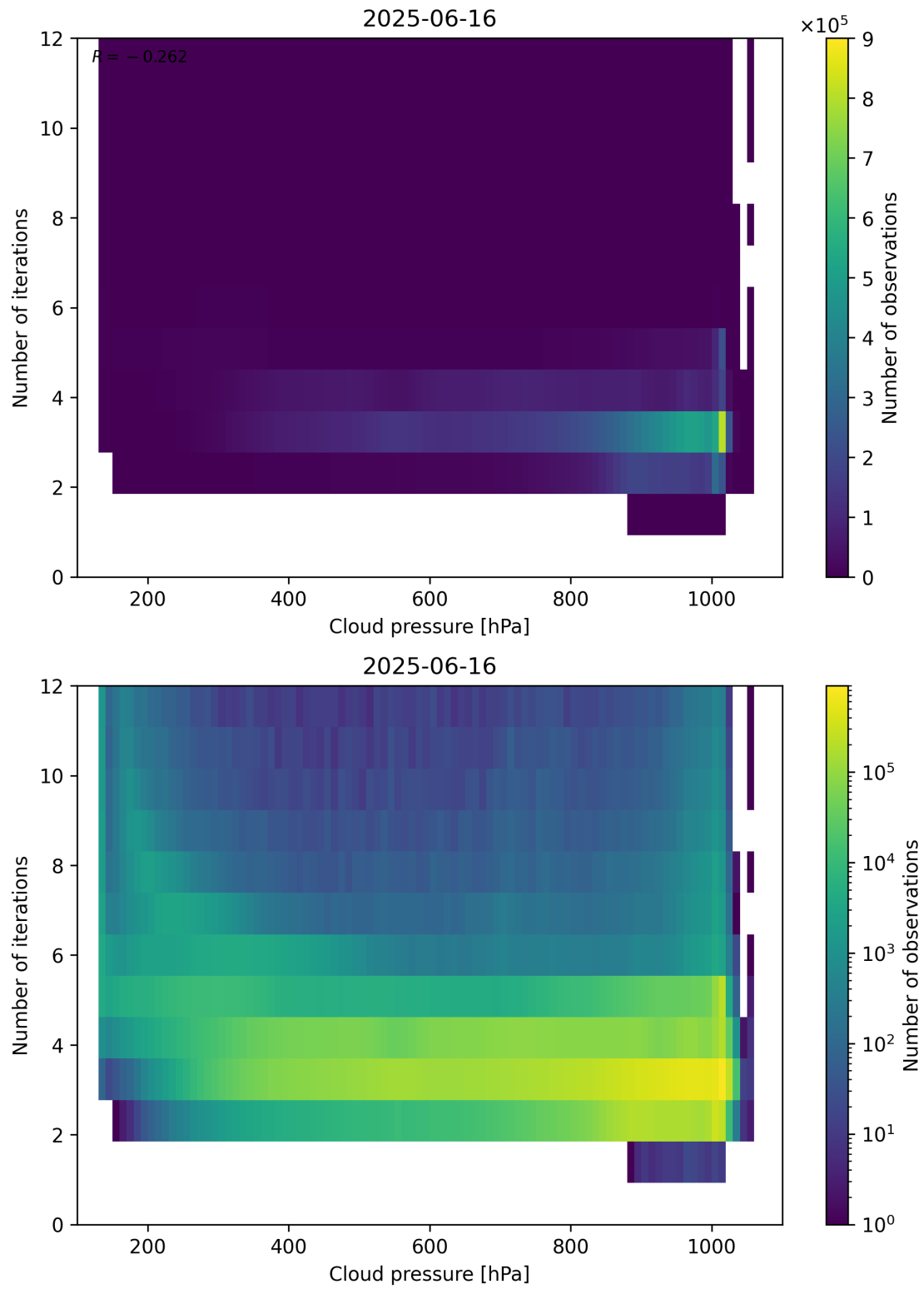
Figure 81: Scatter density plot of “Cloud pressure” against “Number of iterations” for 2025-06-16 to 2025-06-17.
