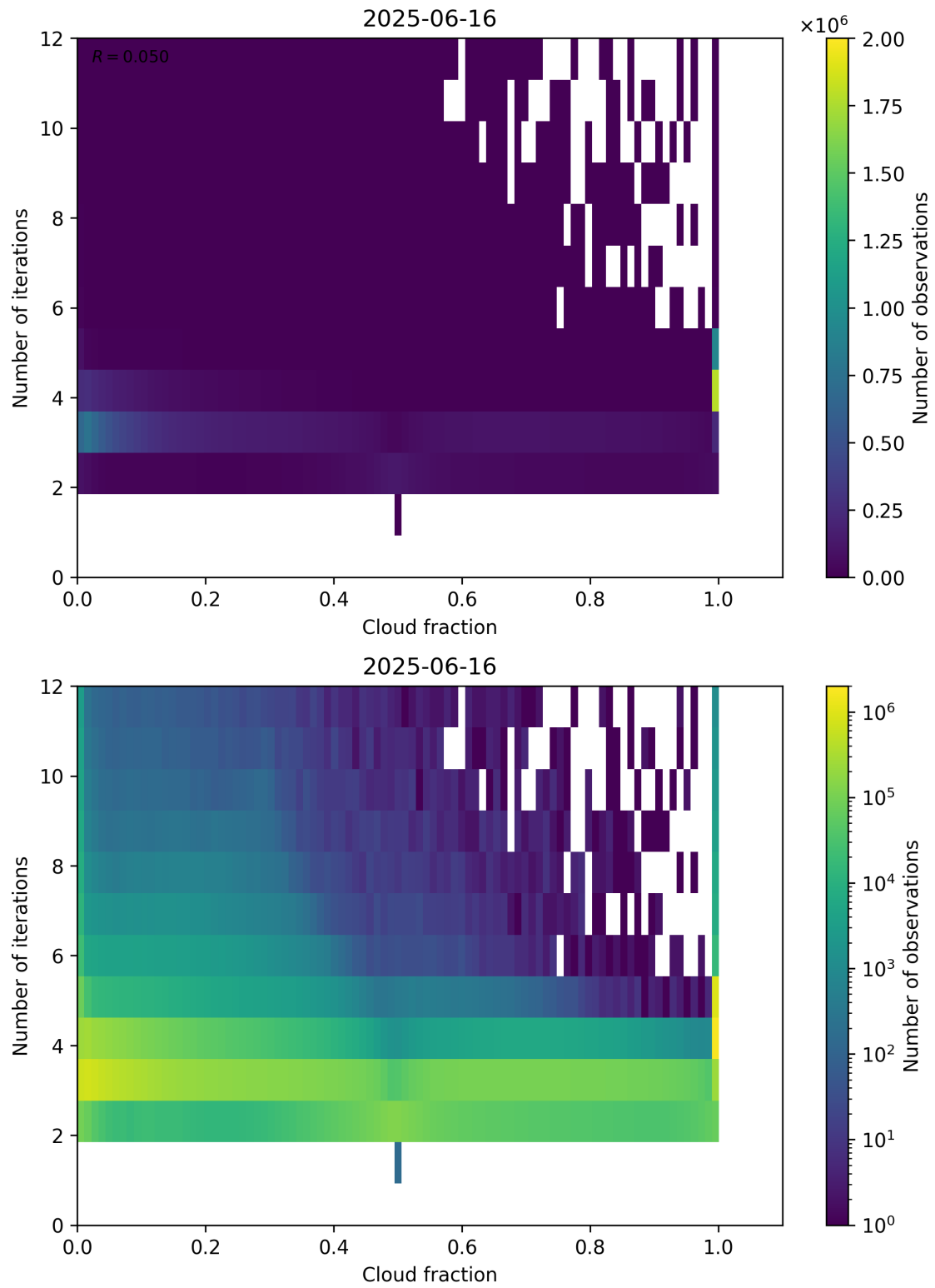
Figure 73: Scatter density plot of “Cloud fraction” against “Number of iterations” for 2025-06-16 to 2025-06-17.
