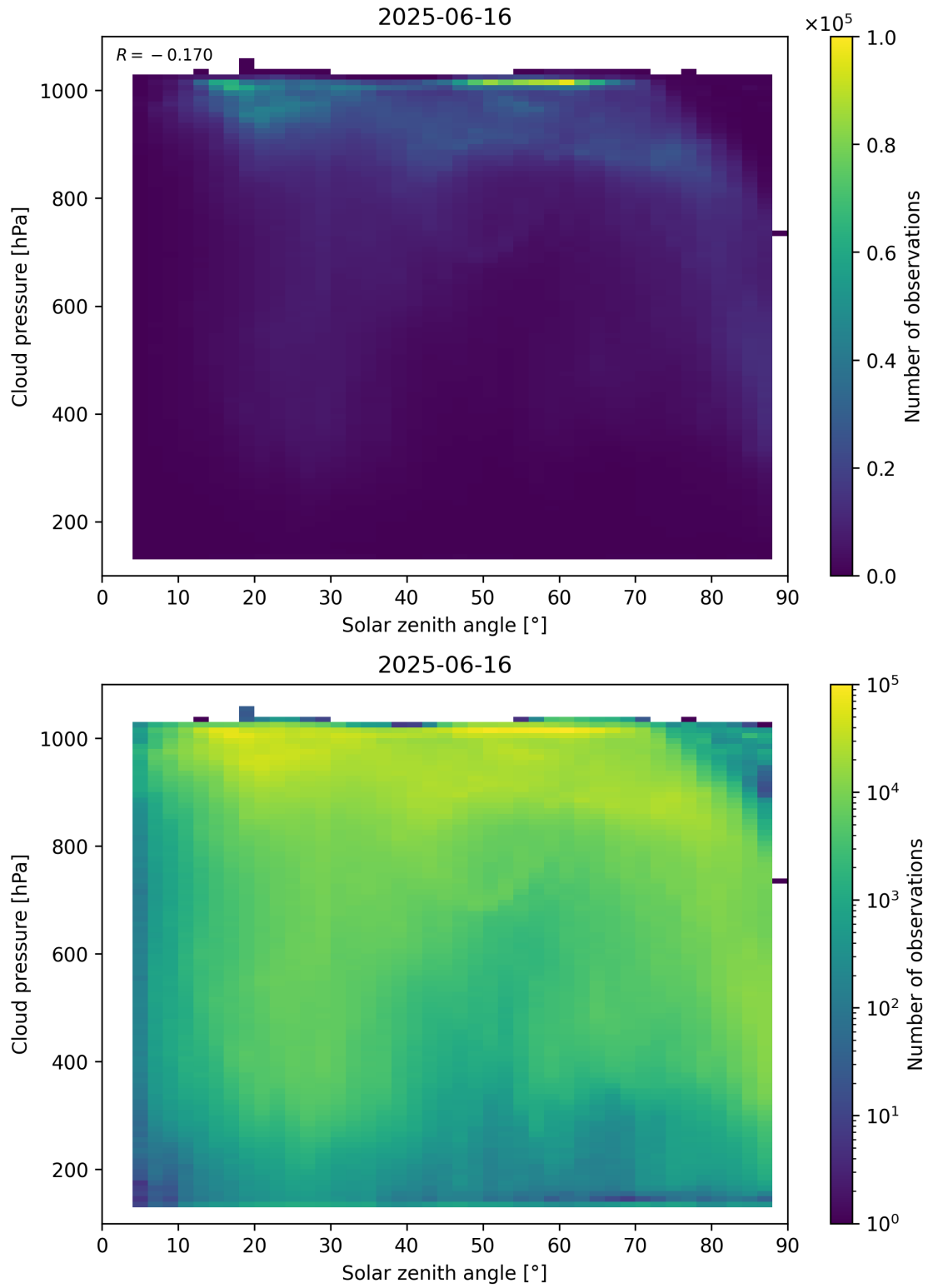
Figure 111: Scatter density plot of “Solar zenith angle” against “Cloud pressure” for 2025-06-16 to 2025-06-17.
