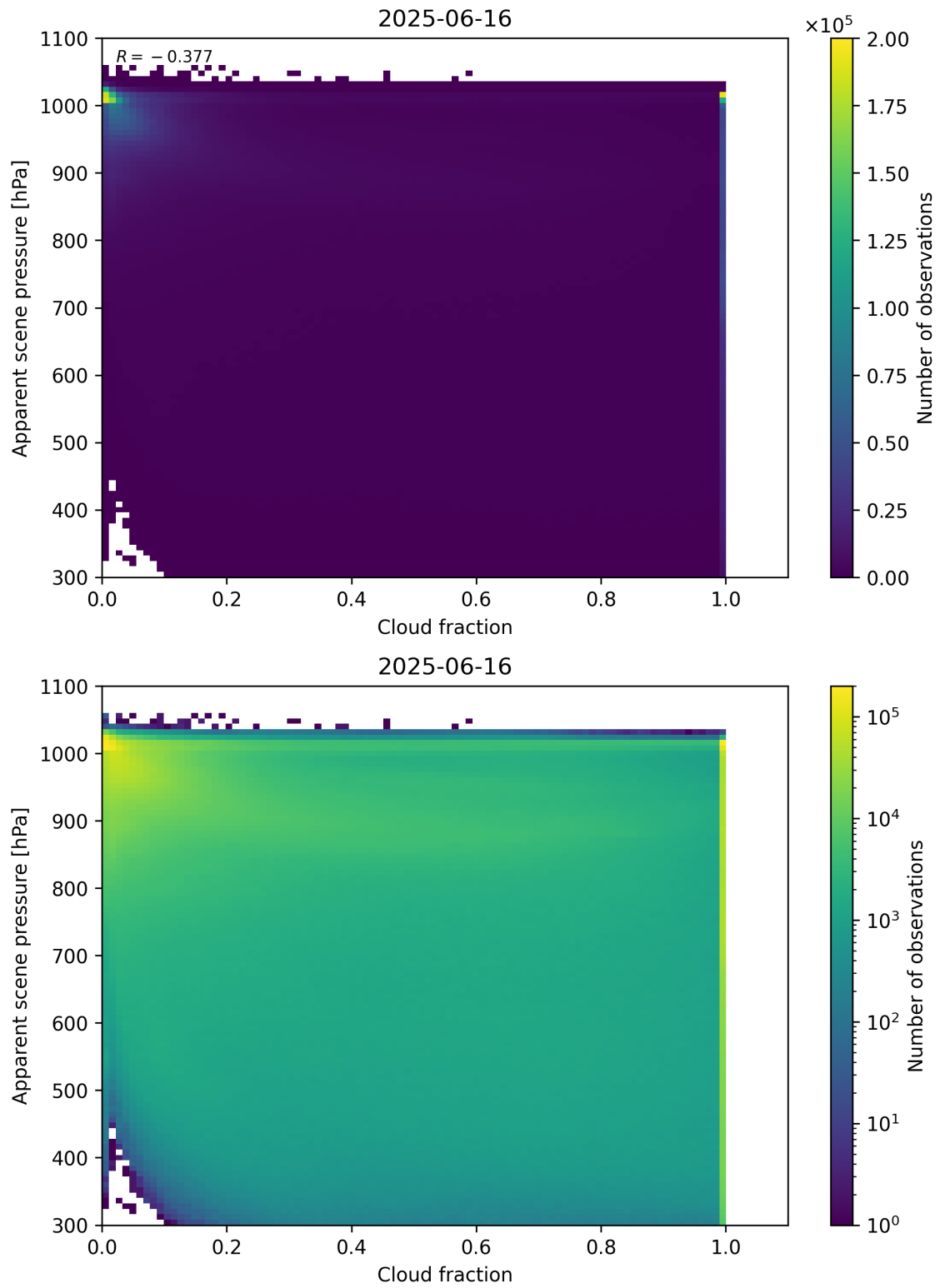
Figure 70: Scatter density plot of “Cloud fraction” against “Apparent scene pressure” for 2025-06-16 to 2025-06-17.
