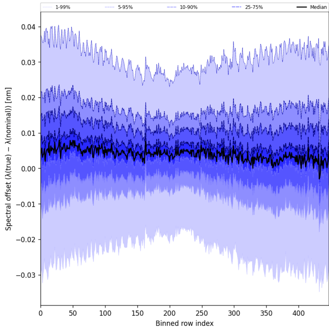
Figure 62: Along track statistics of “Spectral offset ( \lambda_{\text{true}} - \lambda_{\text{nominal}} )” for 2025-06-16 to 2025-06-17
