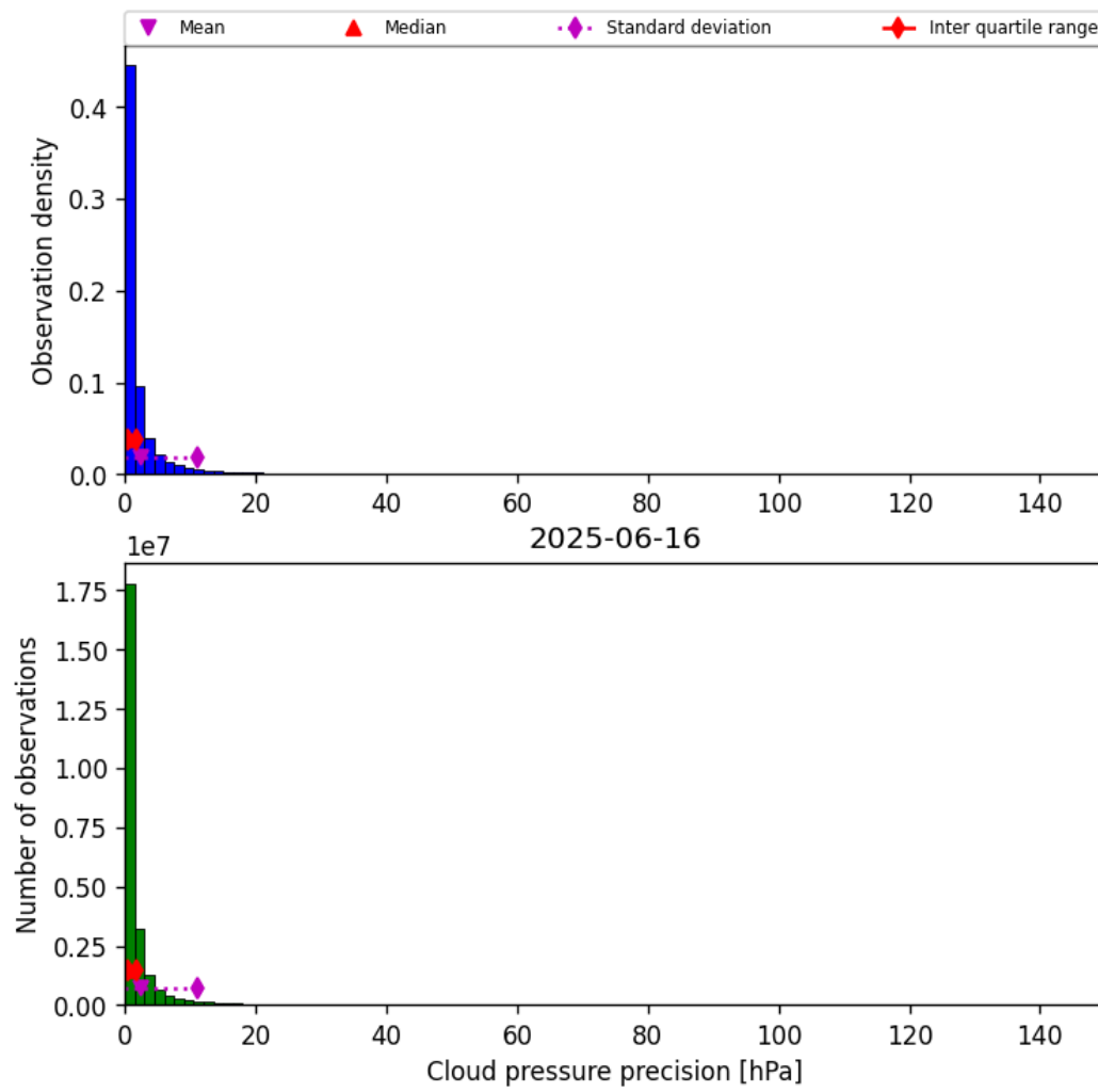
Figure 31: Histogram of “Cloud pressure precision” for 2025-06-16 to 2025-06-17
