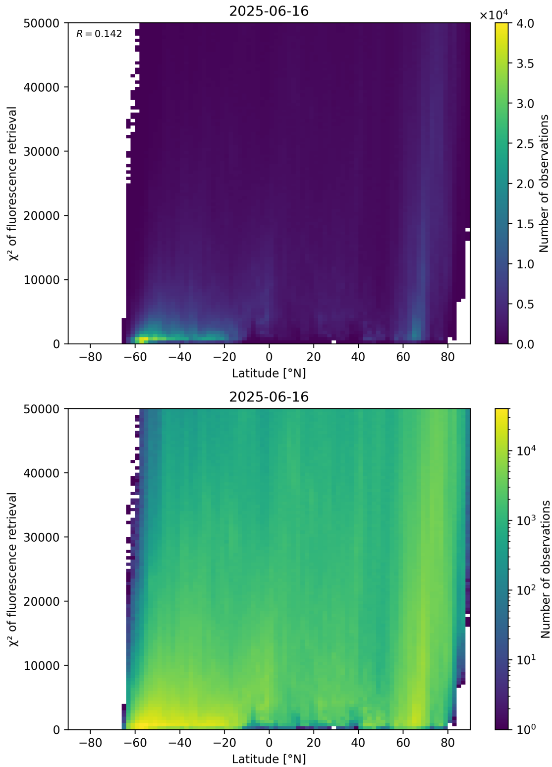
Figure 89: Scatter density plot of “Latitude” against “ \chi^2 of fluorescence retrieval” for 2025-06-16 to 2025-06-17.
