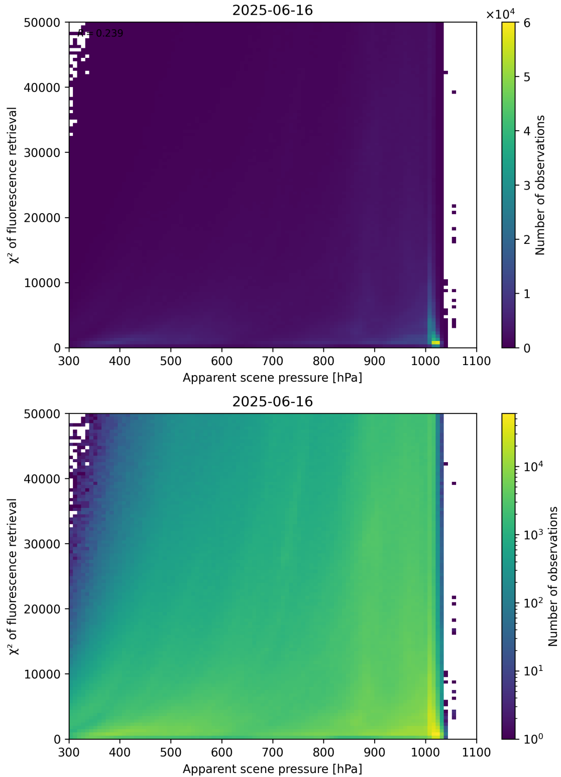
Figure 63: Scatter density plot of “Apparent scene pressure” against “ \chi^2 of fluorescence retrieval” for 2025-06-16 to 2025-06-17.
