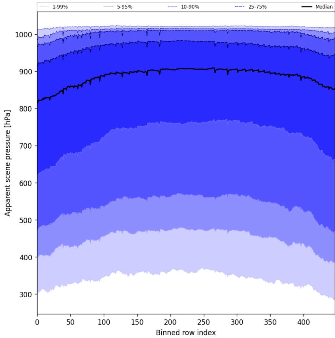
Figure 53: Along track statistics of “Apparent scene pressure” for 2025-06-16 to 2025-06-17
