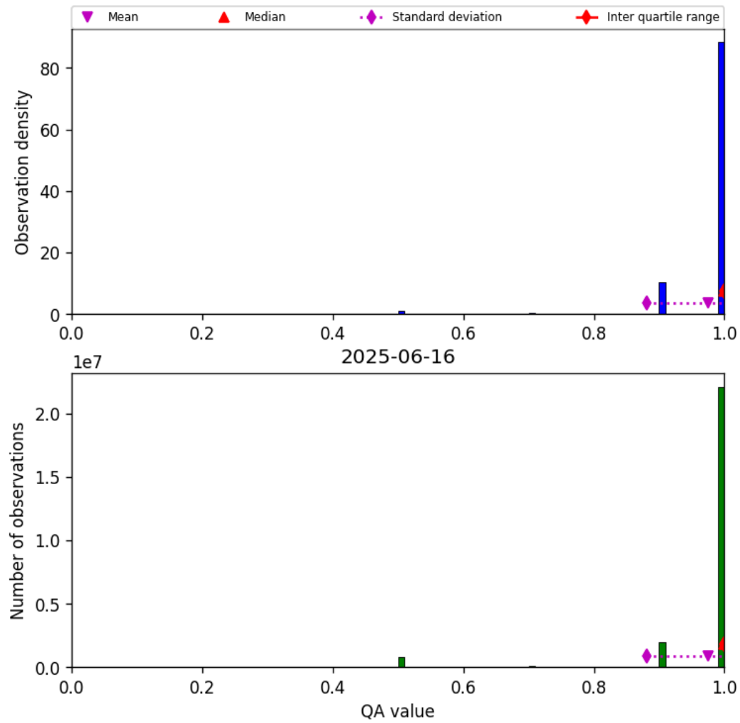
Figure 29: Histogram of “QA value” for 2025-06-16 to 2025-06-17
