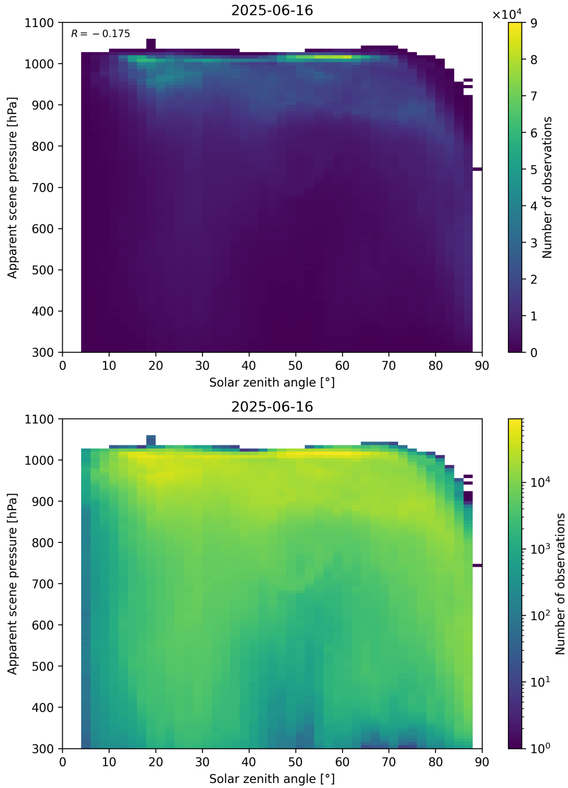
Figure 108: Scatter density plot of “Solar zenith angle” against “Apparent scene pressure” for 2025-06-16 to 2025-06-17.
