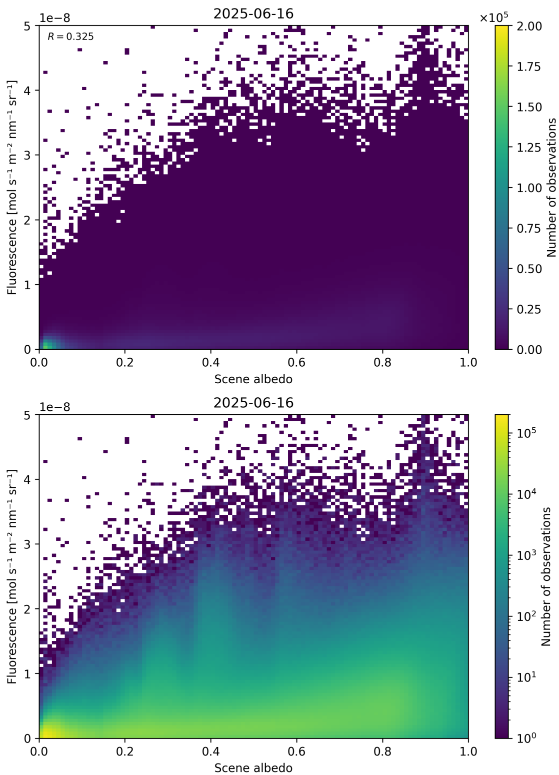
Figure 104: Scatter density plot of “Scene albedo” against “Fluorescence” for 2025-06-16 to 2025-06-17.
