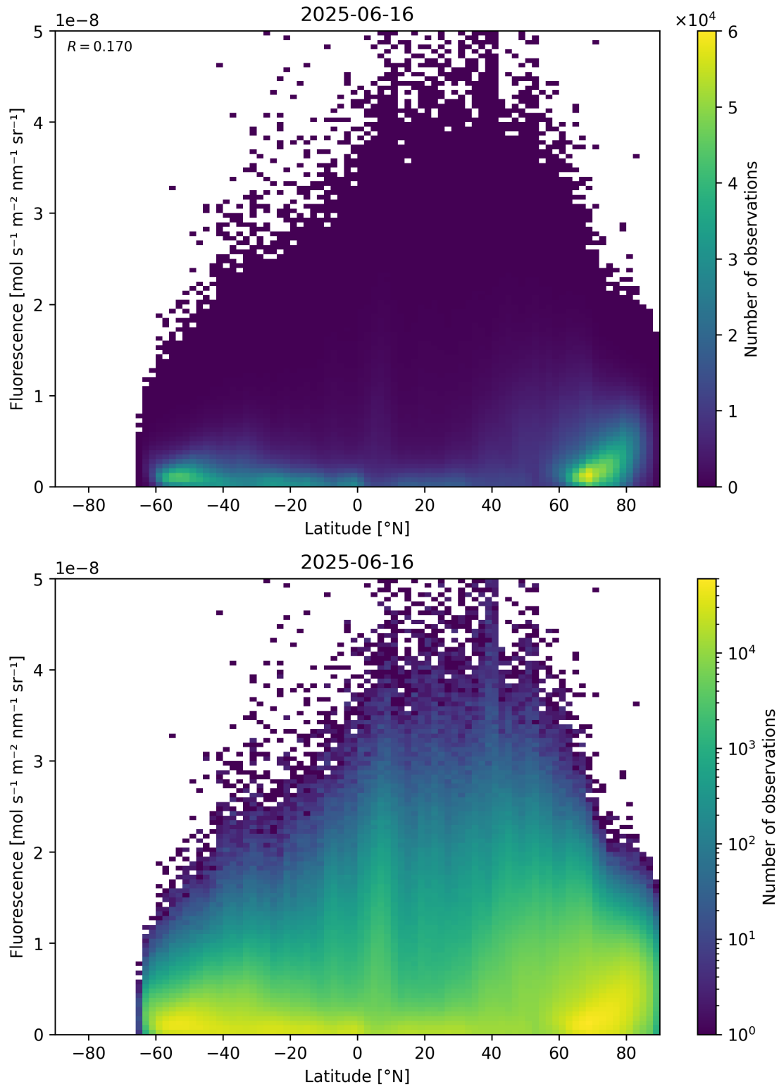
Figure 92: Scatter density plot of “Latitude” against “Fluorescence” for 2025-06-16 to 2025-06-17.
