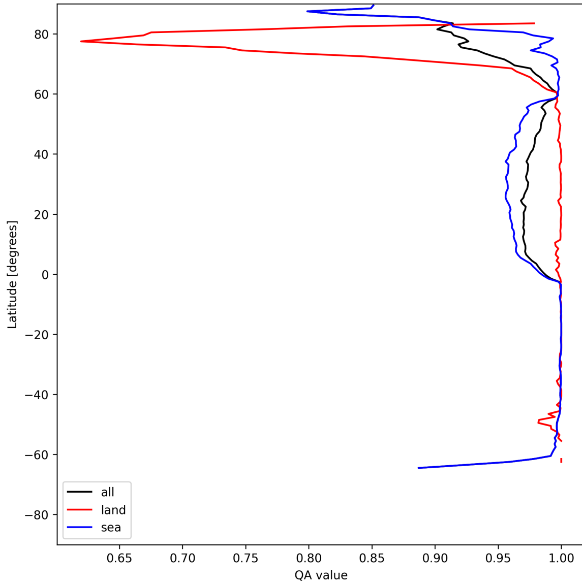
Figure 12: Zonal average of “QA value” for 2025-06-16 to 2025-06-17.
