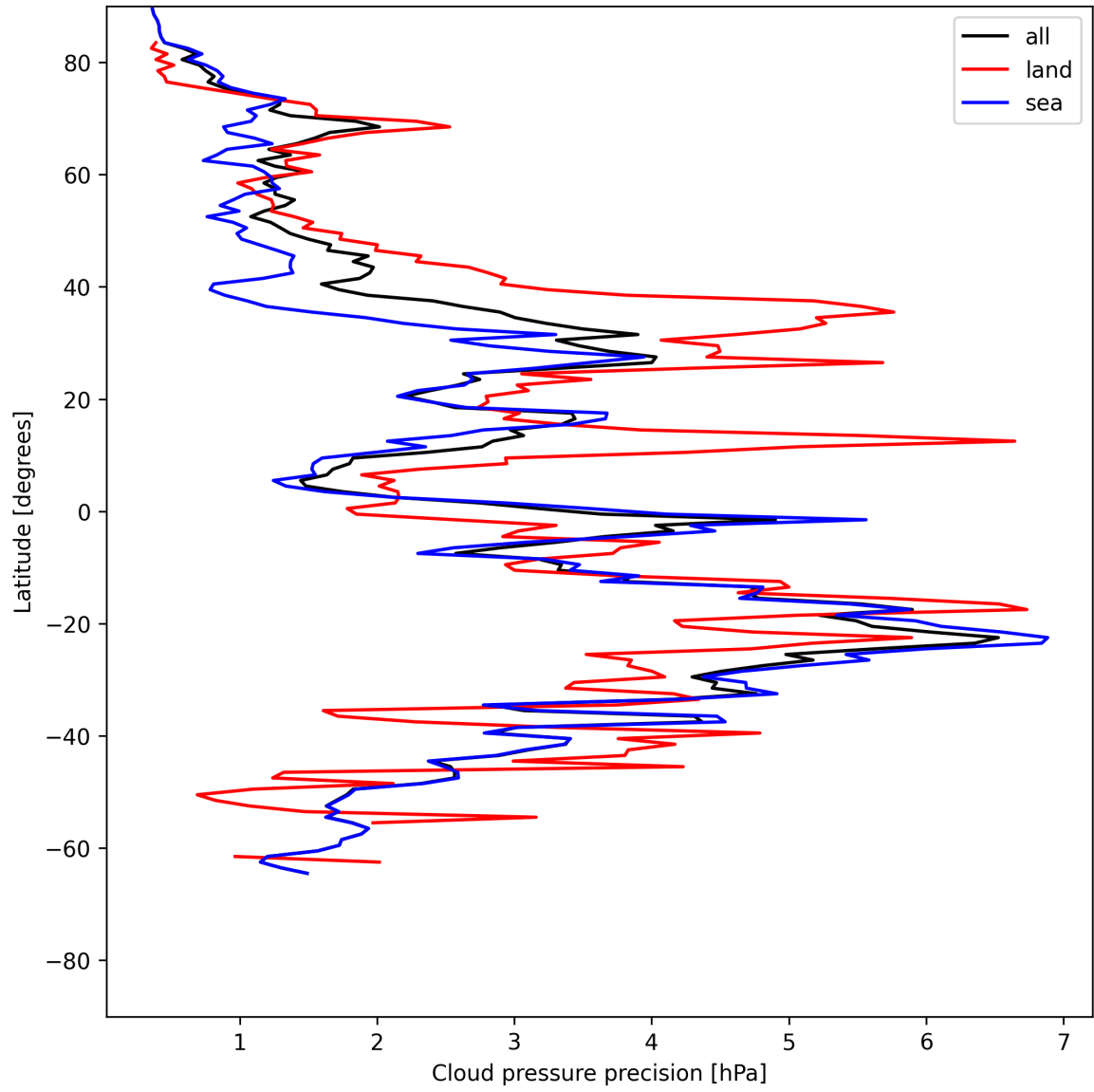
Figure 14: Zonal average of “Cloud pressure precision” for 2025-06-16 to 2025-06-17.
