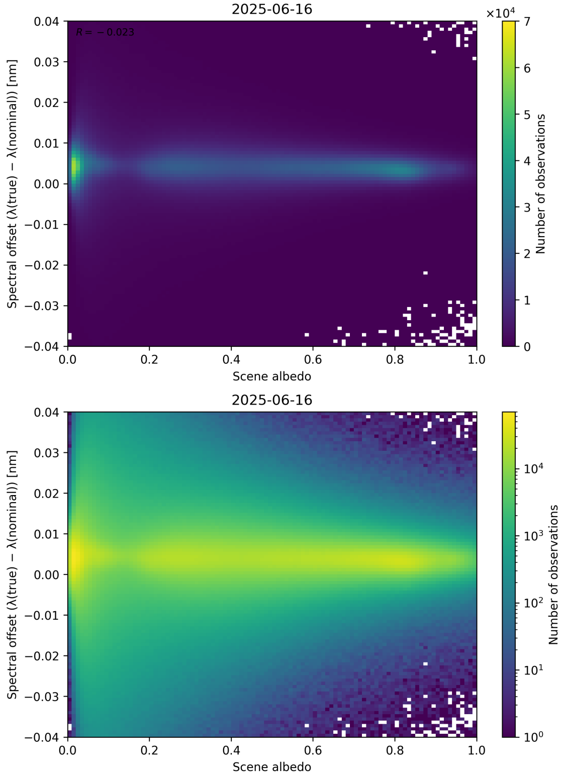
Figure 107: Scatter density plot of “Scene albedo” against “Spectral offset ( \lambda_{\text{true}} - \lambda_{\text{nominal}} )” for 2025-06-16 to 2025-06-17.
