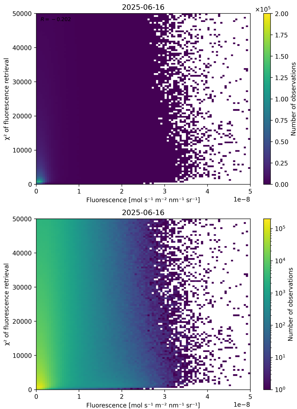
Figure 85: Scatter density plot of “Fluorescence” against “ \chi^2 of fluorescence retrieval” for 2025-06-16 to 2025-06-17.
