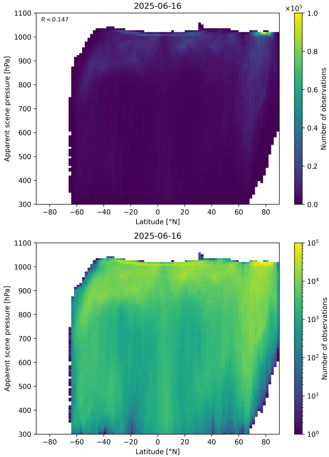
Figure 88: Scatter density plot of “Latitude” against “Apparent scene pressure” for 2025-06-16 to 2025-06-17.
