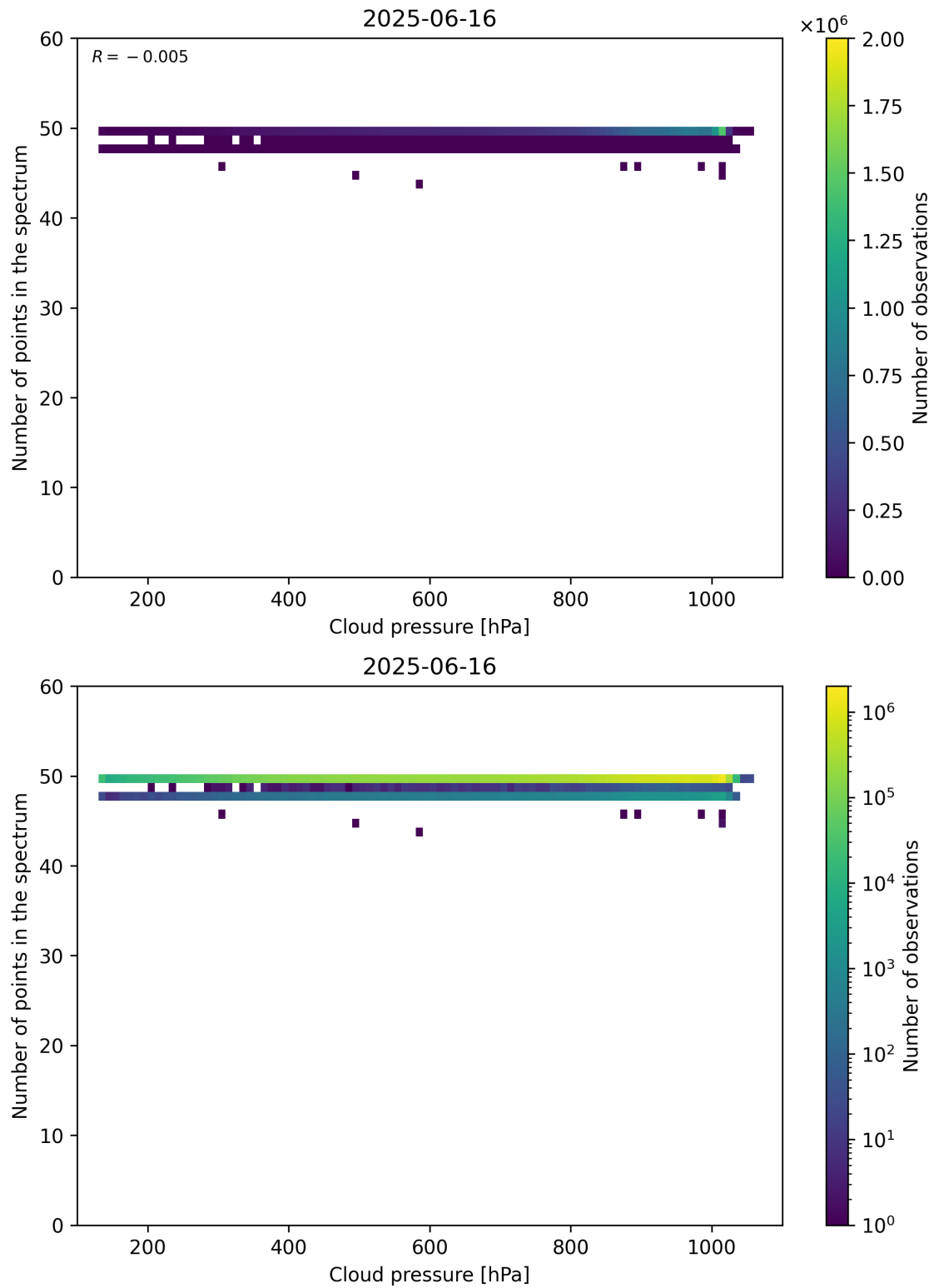
Figure 82: Scatter density plot of “Cloud pressure” against “Number of points in the spectrum” for 2025-06-16 to 2025-06-17.
