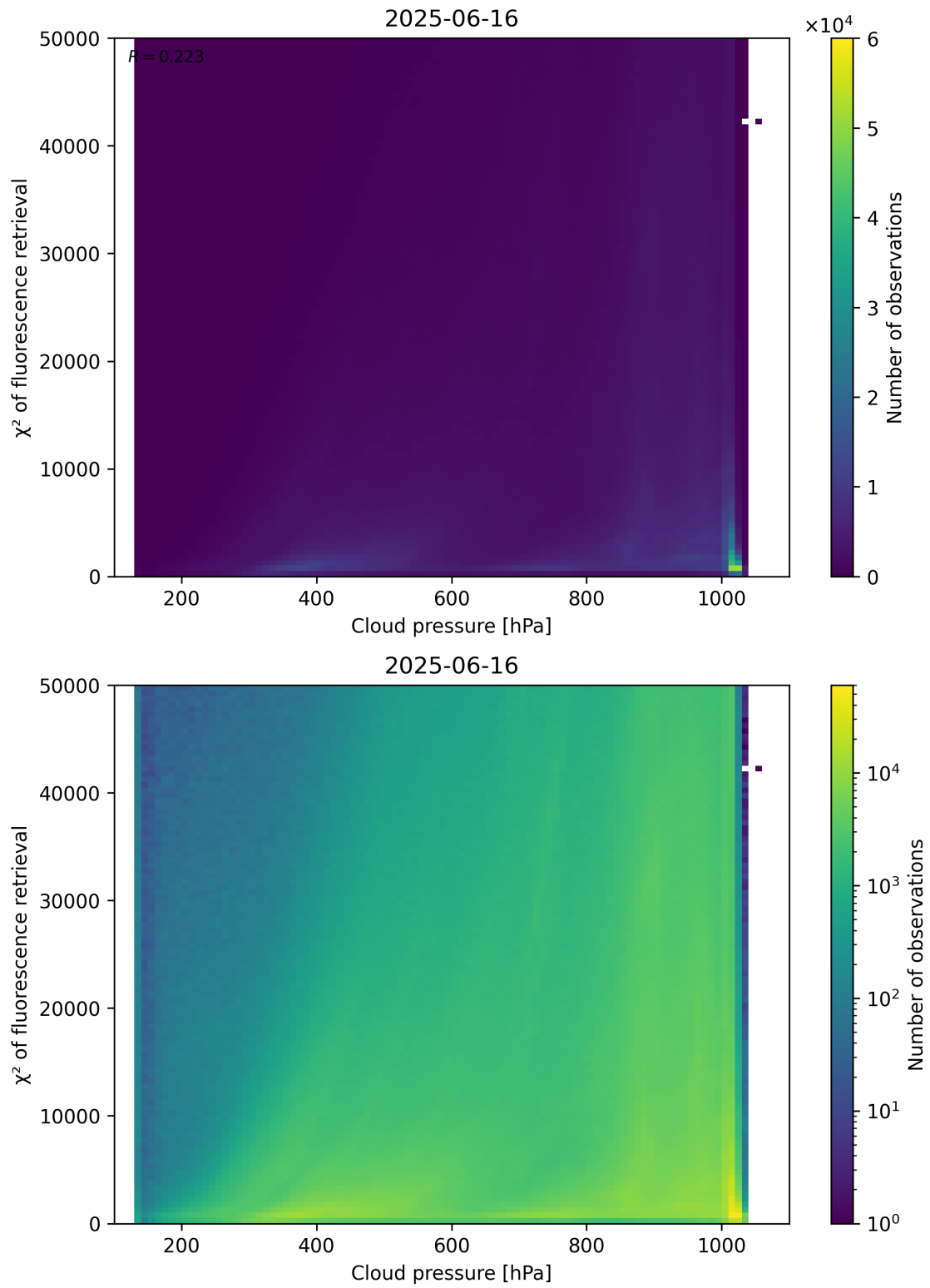
Figure 78: Scatter density plot of “Cloud pressure” against “ \chi^2 of fluorescence retrieval” for 2025-06-16 to 2025-06-17.
