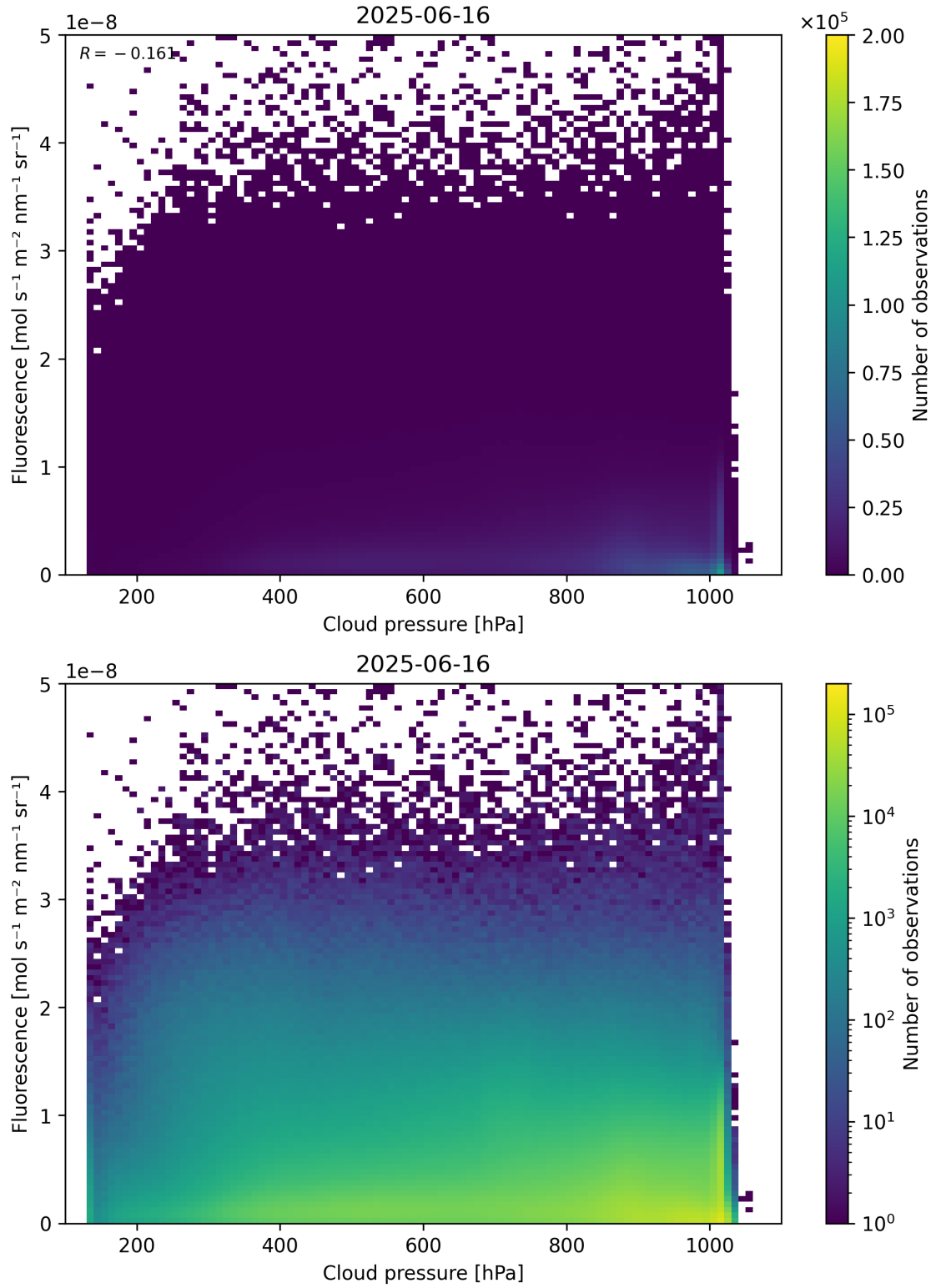
Figure 80: Scatter density plot of “Cloud pressure” against “Fluorescence” for 2025-06-16 to 2025-06-17.
