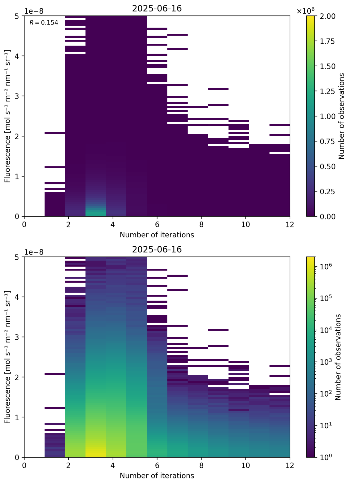
Figure 98: Scatter density plot of “Number of iterations” against “Fluorescence” for 2025-06-16 to 2025-06-17.
