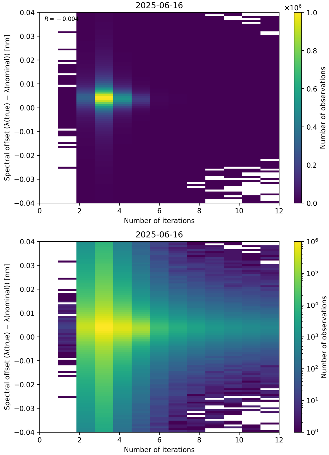
Figure 100: Scatter density plot of “Number of iterations” against “Spectral offset ( \lambda_{\text{true}} - \lambda_{\text{nominal}} )” for 2025-06-16 to 2025-06-17.
