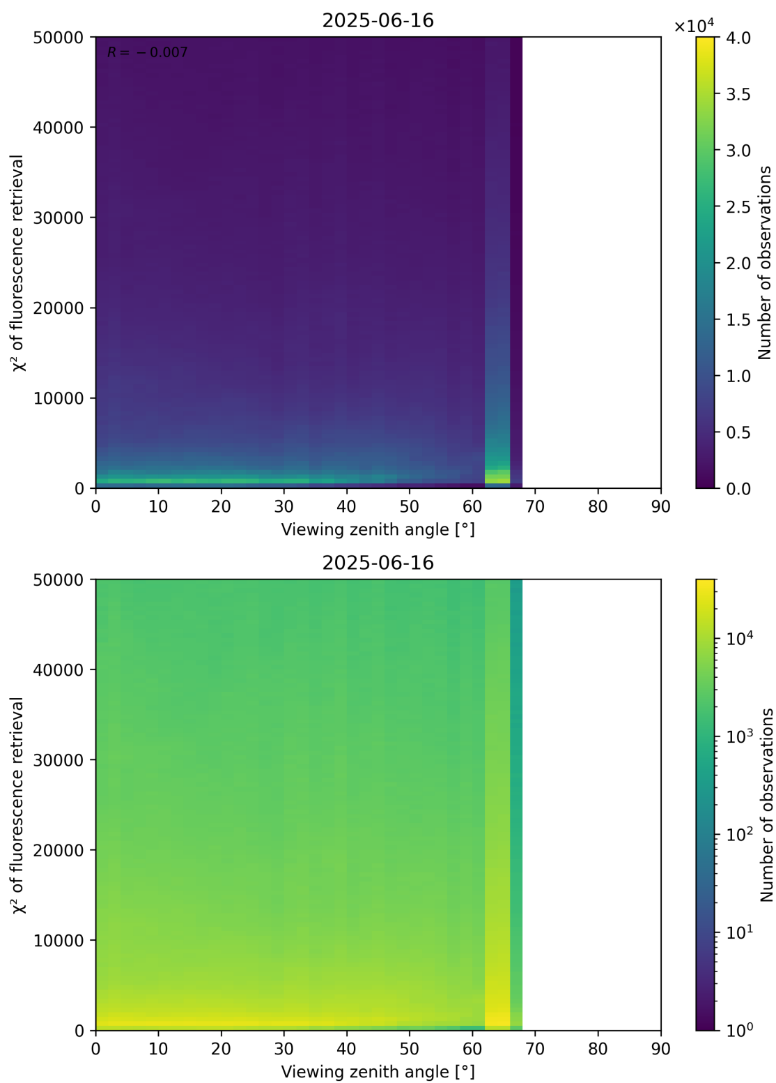
Figure 119: Scatter density plot of “Viewing zenith angle” against “ \chi^2 of fluorescence retrieval” for 2025-06-16 to 2025-06-17.
