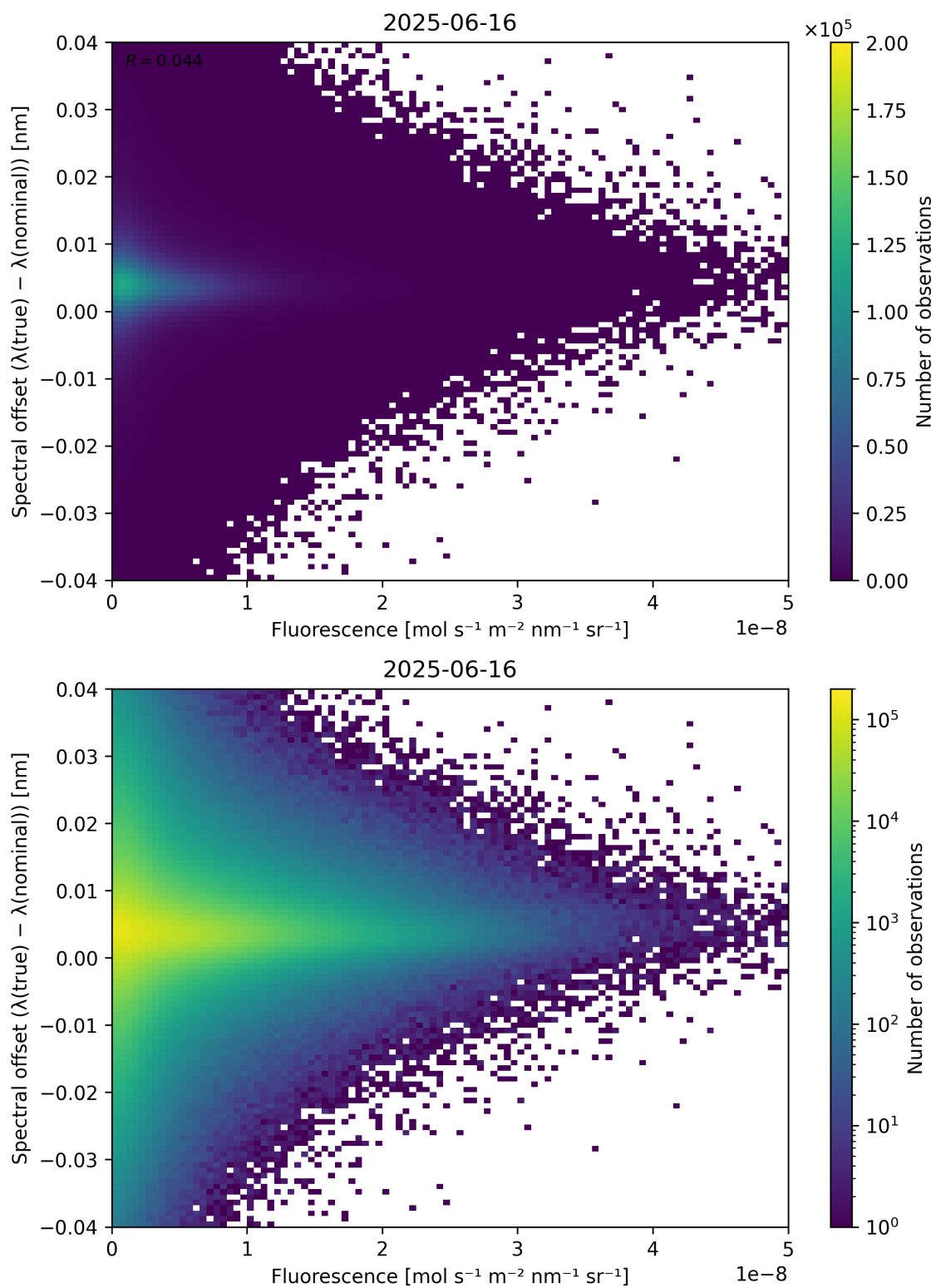
Figure 87: Scatter density plot of “Fluorescence” against “Spectral offset ( \lambda_{\text{true}} - \lambda_{\text{nominal}} )” for 2025-06-16 to 2025-06-17.
