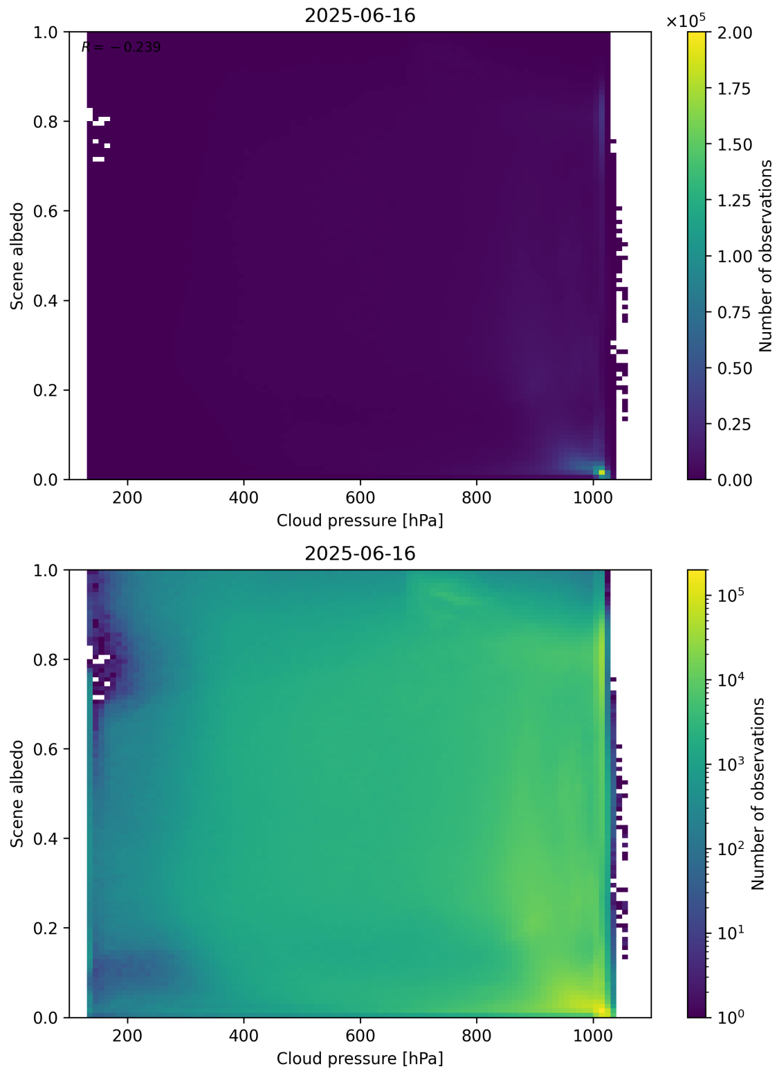
Figure 83: Scatter density plot of “Cloud pressure” against “Scene albedo” for 2025-06-16 to 2025-06-17.
