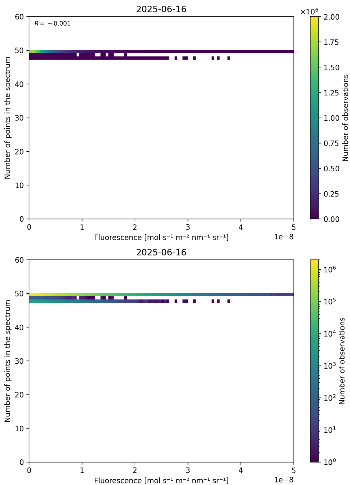
Figure 86: Scatter density plot of “Fluorescence” against “Number of points in the spectrum” for 2025-06-16 to 2025-06-17.
