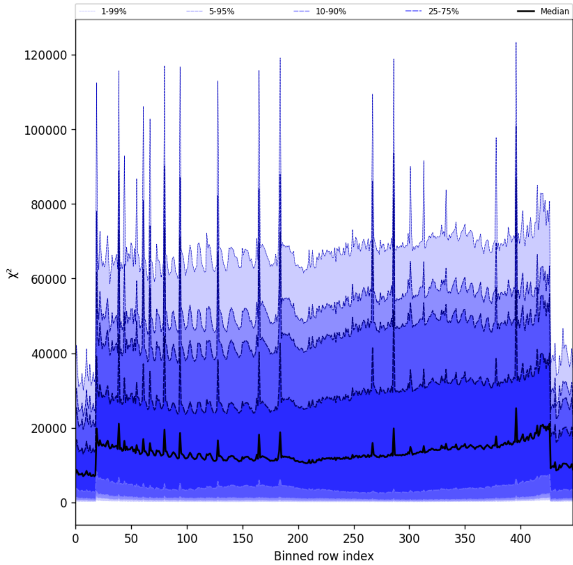
Figure 55: Along track statistics of “ \chi^2 ” for 2025-06-16 to 2025-06-17
