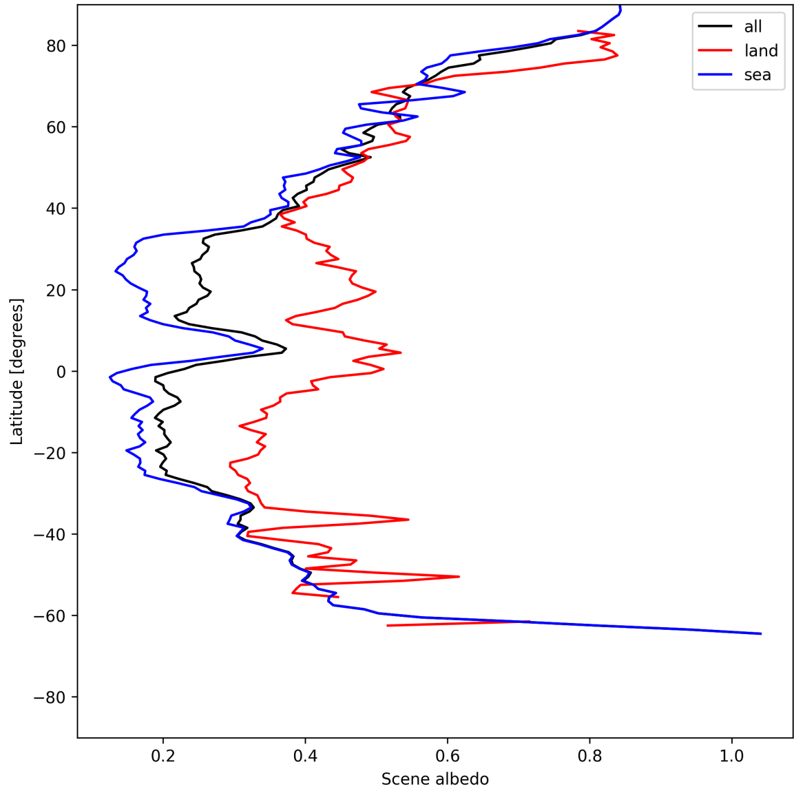
Figure 17: Zonal average of “Scene albedo” for 2025-06-16 to 2025-06-17.
