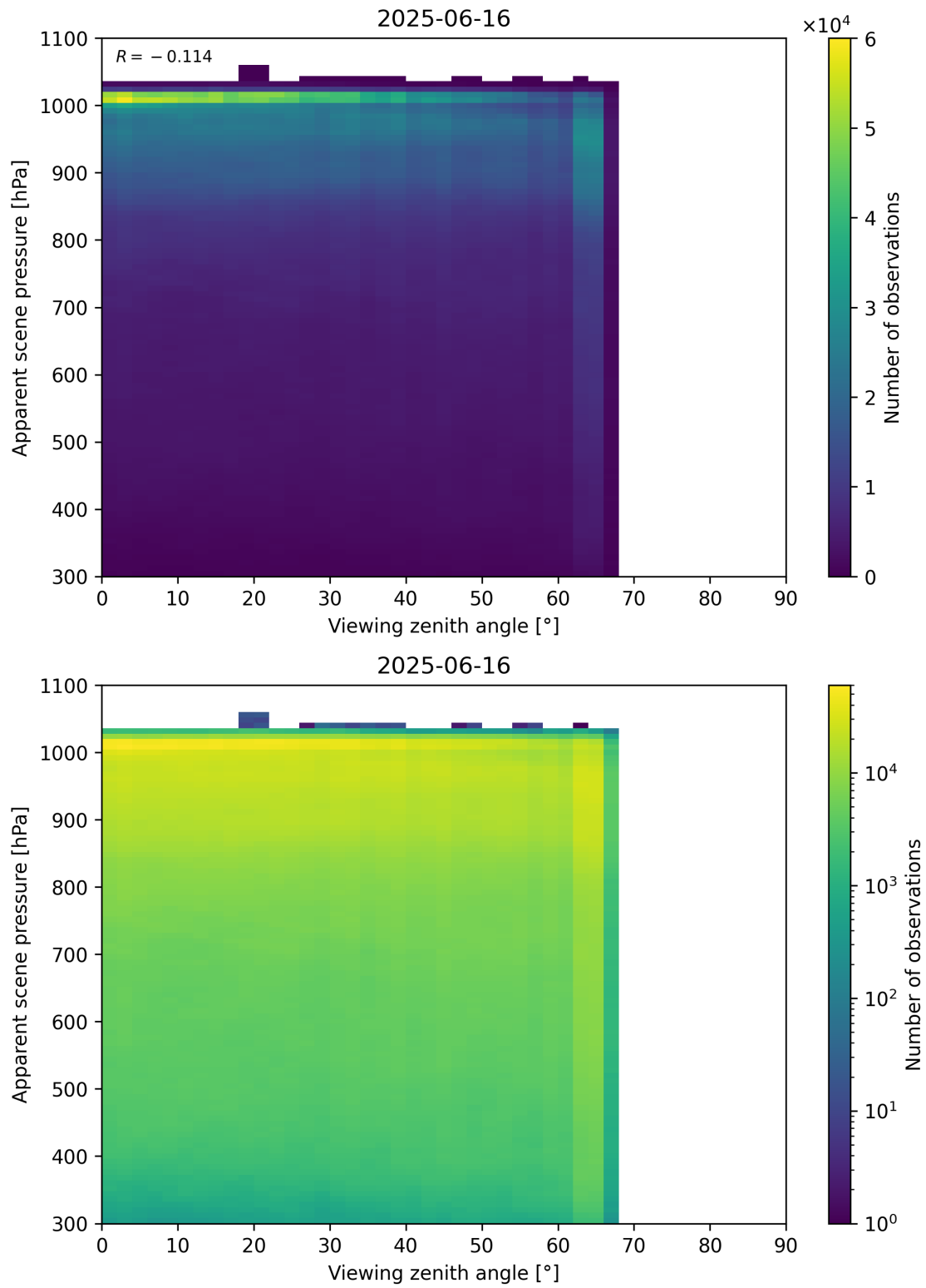
Figure 118: Scatter density plot of “Viewing zenith angle” against “Apparent scene pressure” for 2025-06-16 to 2025-06-17.
