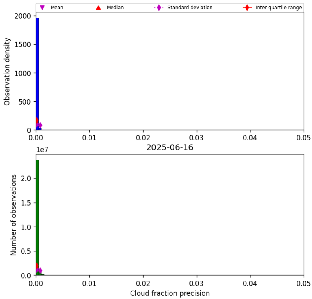
Figure 33: Histogram of “Cloud fraction precision” for 2025-06-16 to 2025-06-17
