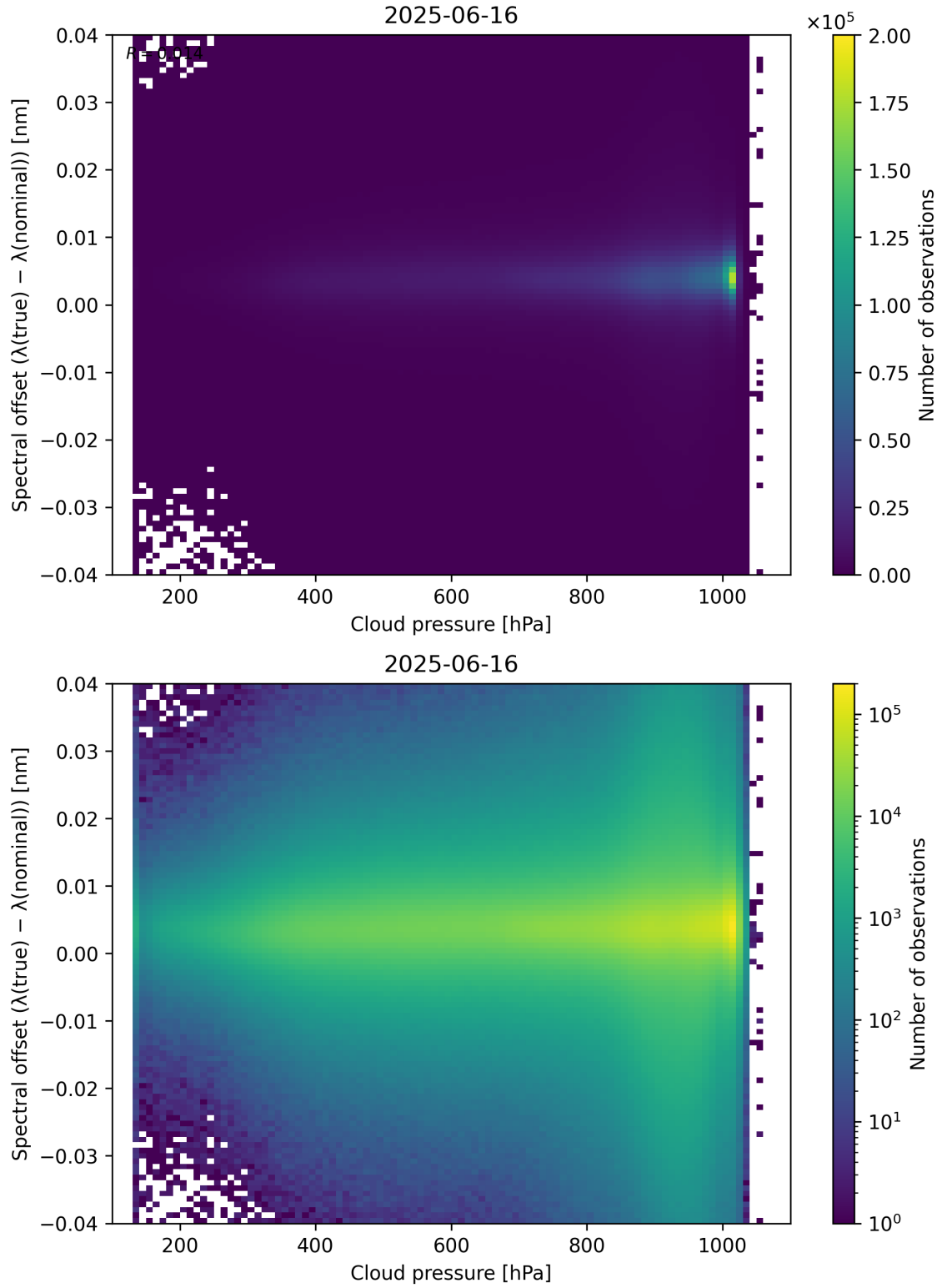
Figure 84: Scatter density plot of “Cloud pressure” against “Spectral offset ( \lambda_{\text{true}} - \lambda_{\text{nominal}} )” for 2025-06-16 to 2025-06-17.
