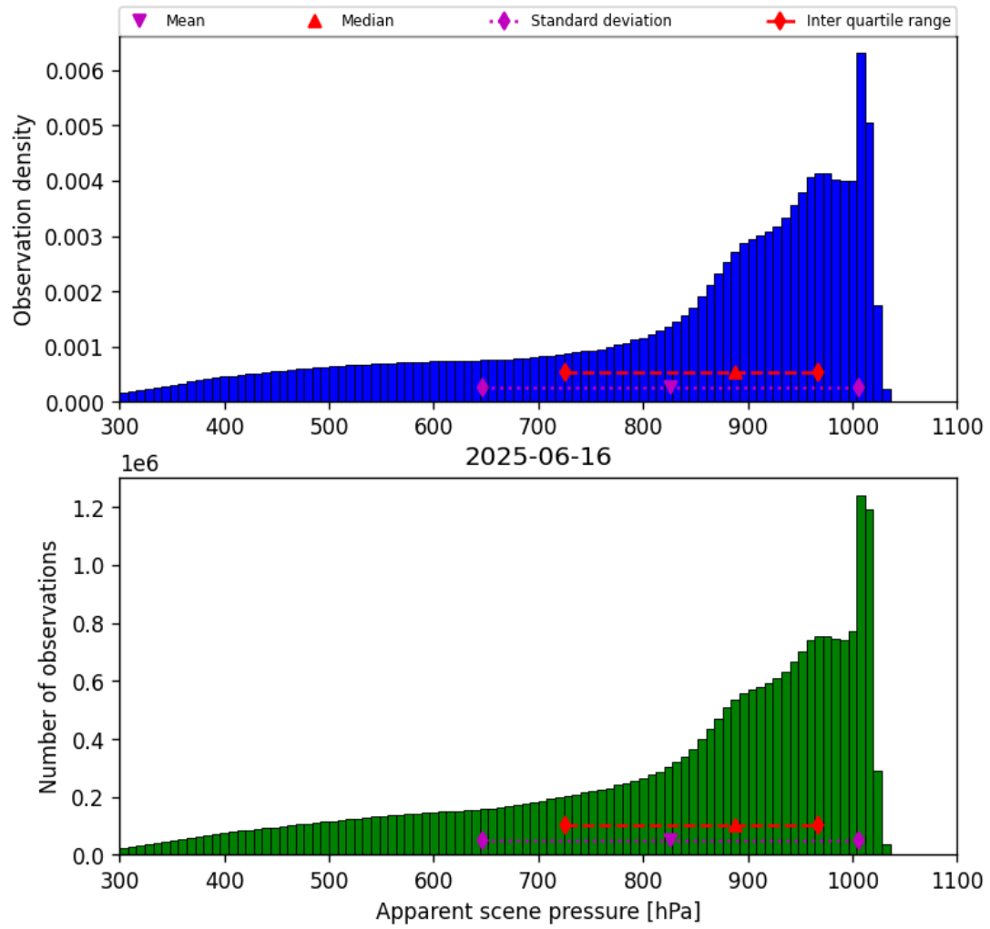
Figure 36: Histogram of “Apparent scene pressure” for 2025-06-16 to 2025-06-17
