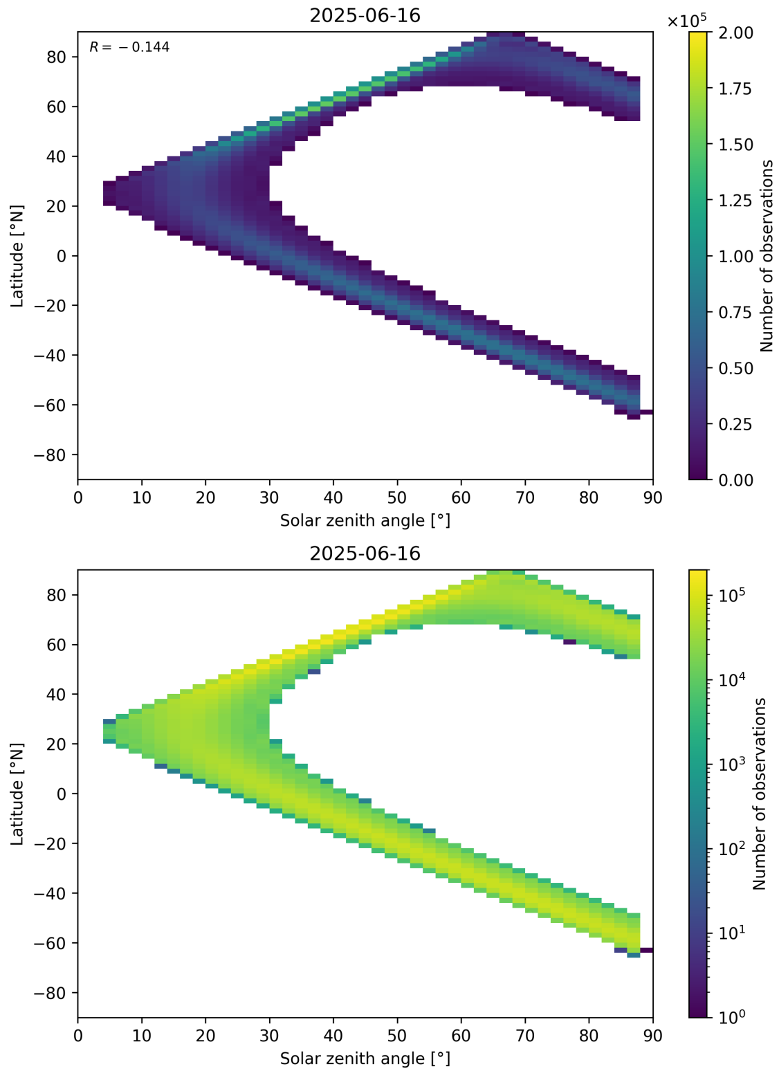
Figure 113: Scatter density plot of “Solar zenith angle” against “Latitude” for 2025-06-16 to 2025-06-17.
