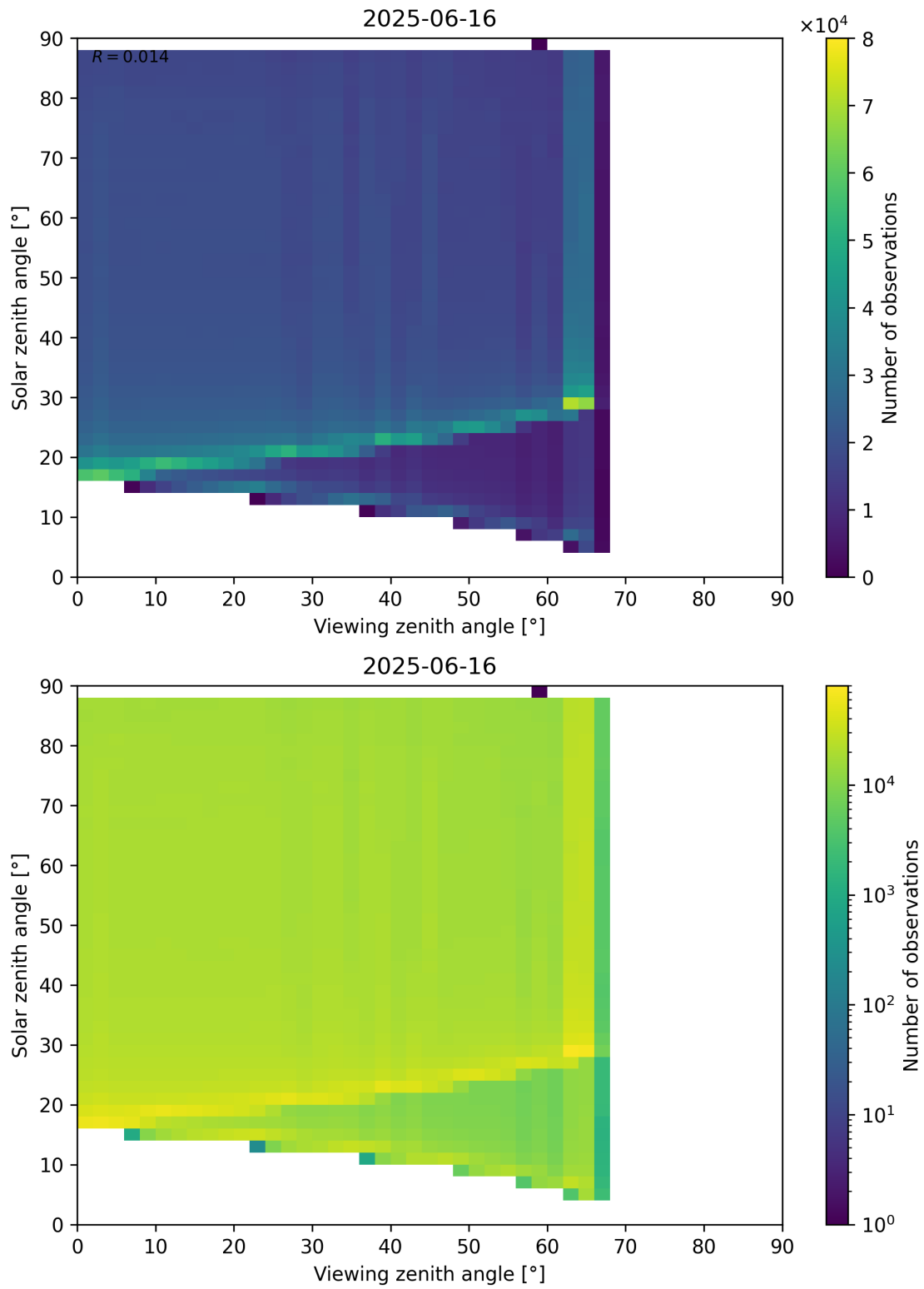
Figure 127: Scatter density plot of “Viewing zenith angle” against “Solar zenith angle” for 2025-06-16 to 2025-06-17.
