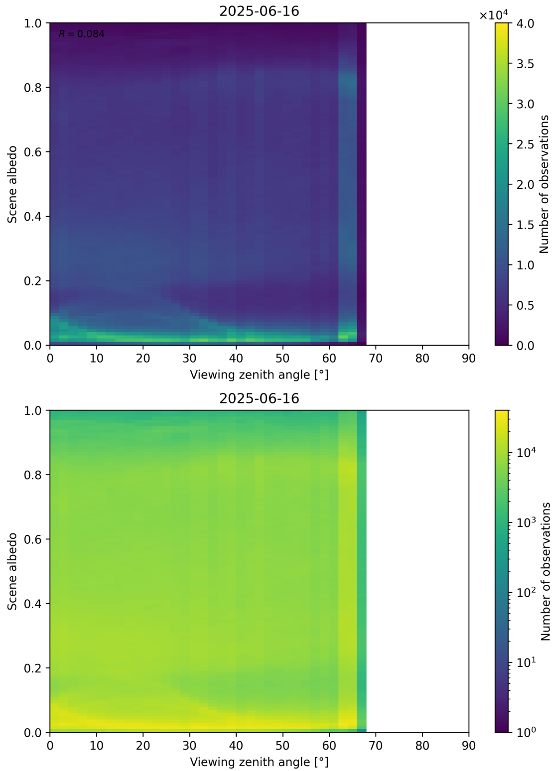
Figure 126: Scatter density plot of “Viewing zenith angle” against “Scene albedo” for 2025-06-16 to 2025-06-17.
