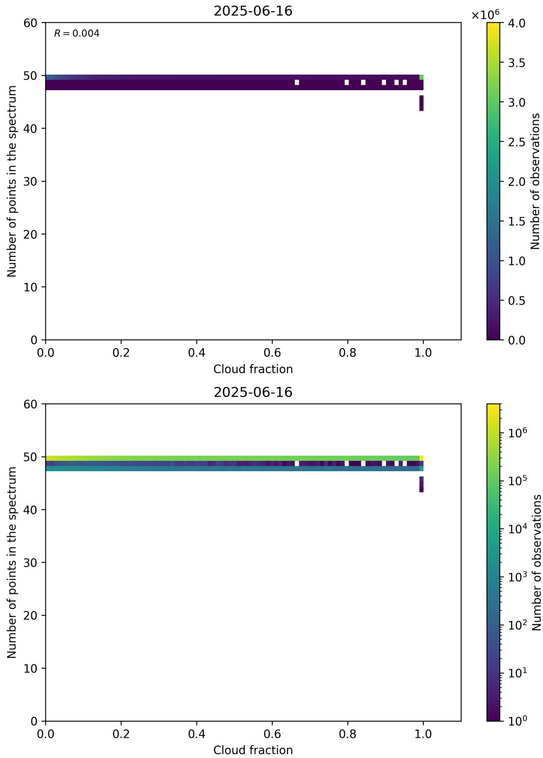
Figure 74: Scatter density plot of “Cloud fraction” against “Number of points in the spectrum” for 2025-06-16 to 2025-06-17.
