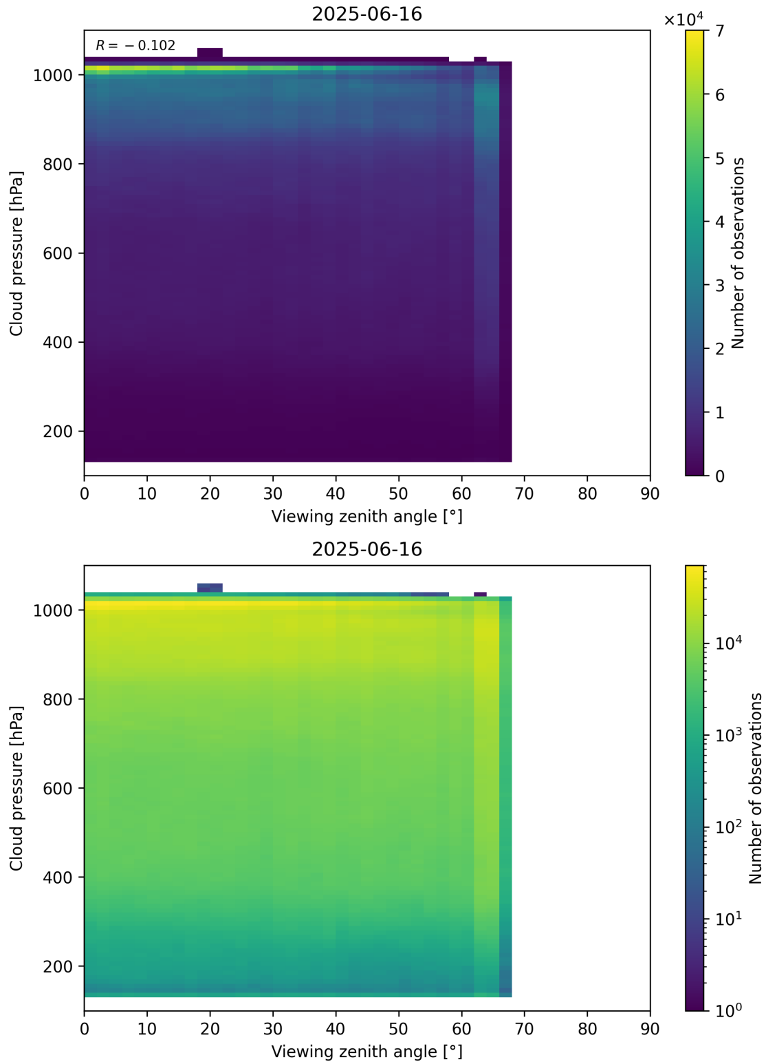
Figure 121: Scatter density plot of “Viewing zenith angle” against “Cloud pressure” for 2025-06-16 to 2025-06-17.
