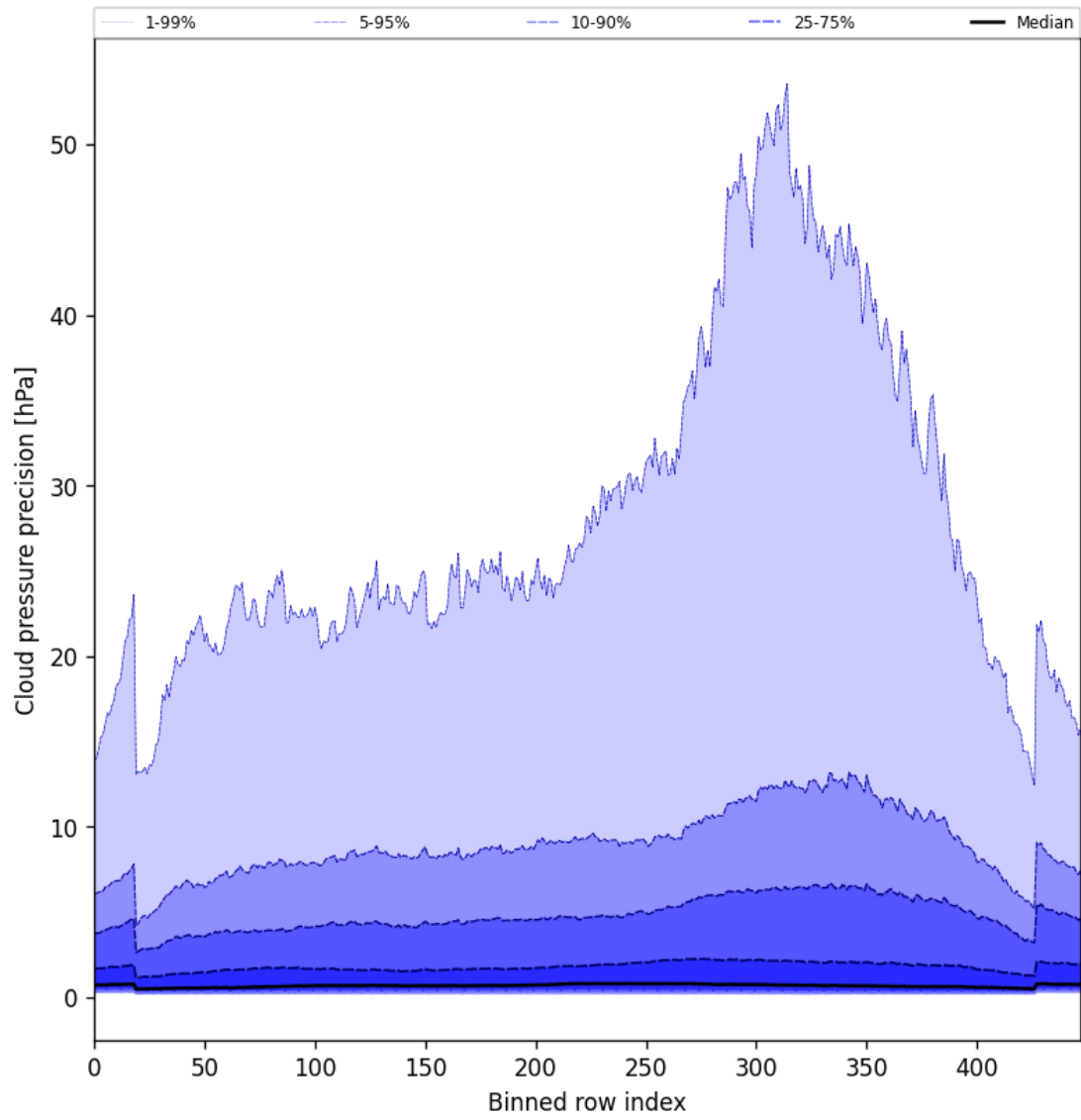
Figure 48: Along track statistics of “Cloud pressure precision” for 2025-06-16 to 2025-06-17
