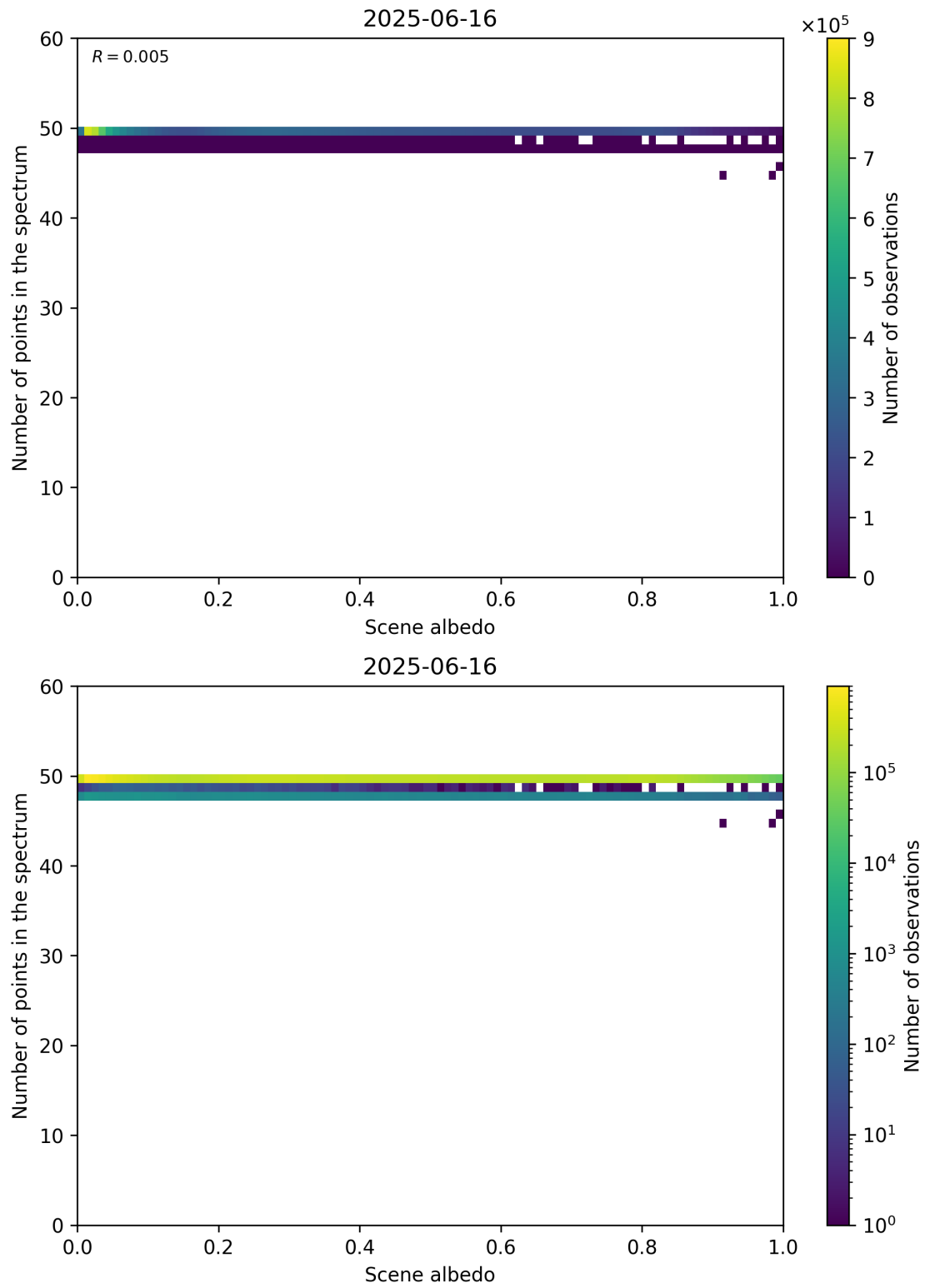
Figure 106: Scatter density plot of “Scene albedo” against “Number of points in the spectrum” for 2025-06-16 to 2025-06-17.
