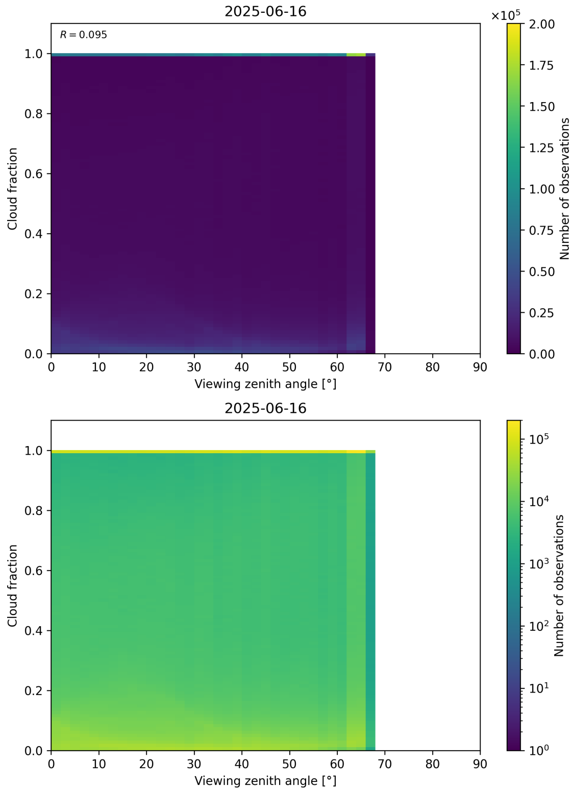
Figure 120: Scatter density plot of “Viewing zenith angle” against “Cloud fraction” for 2025-06-16 to 2025-06-17.
