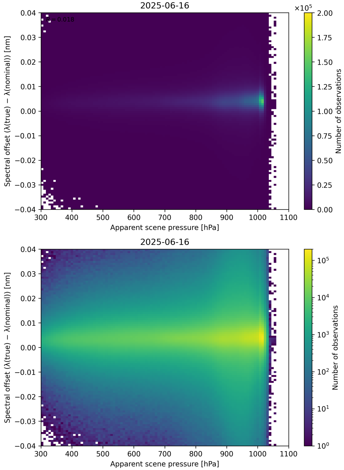
Figure 67: Scatter density plot of “Apparent scene pressure” against “Spectral offset ( \lambda_{\text{true}} - \lambda_{\text{nominal}} )” for 2025-06-16 to 2025-06-17.
