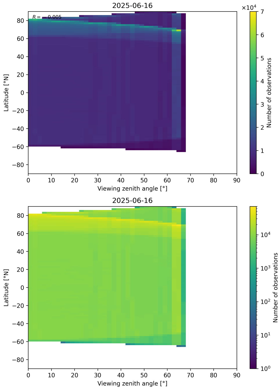
Figure 123: Scatter density plot of “Viewing zenith angle” against “Latitude” for 2025-06-16 to 2025-06-17.
