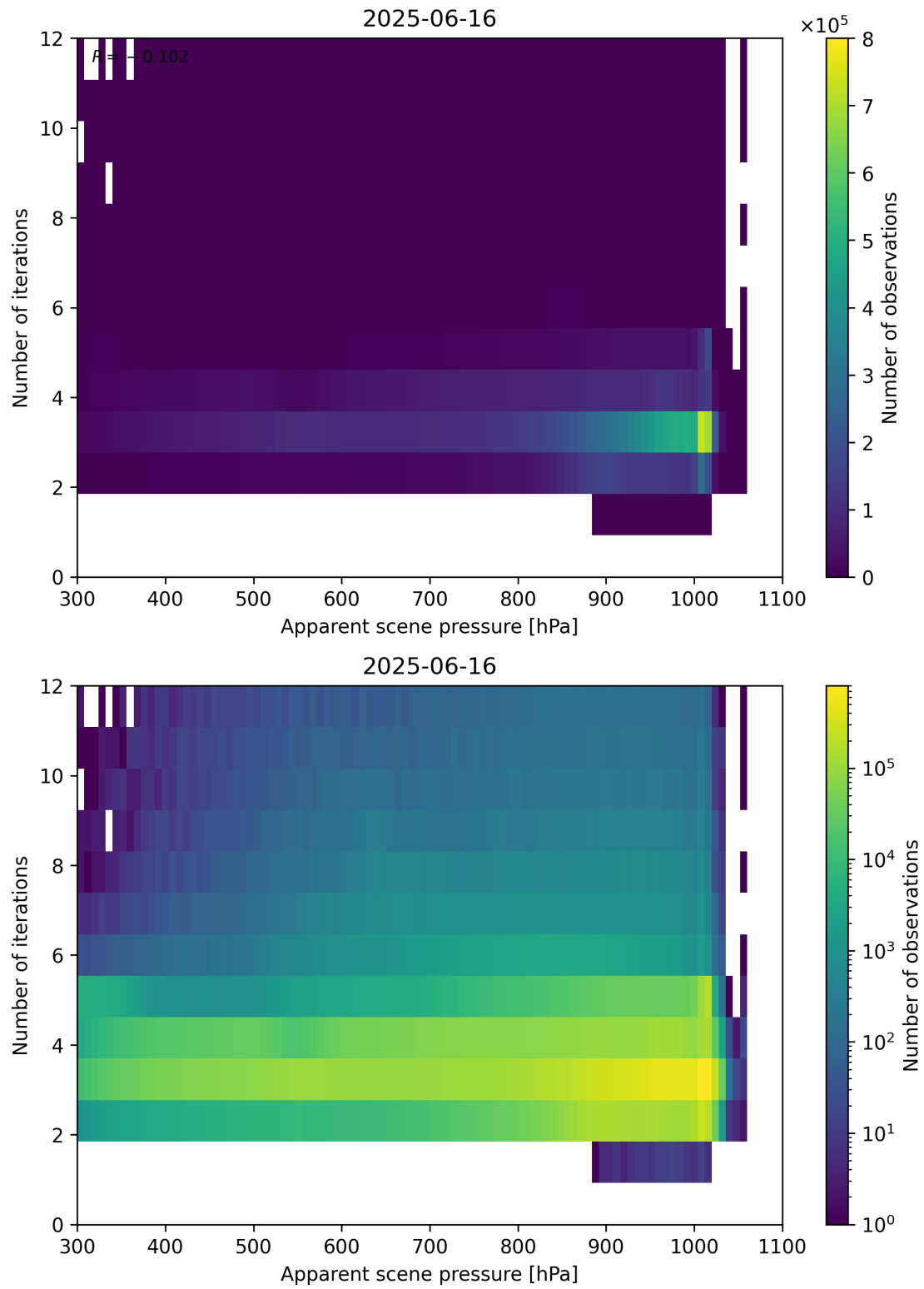
Figure 65: Scatter density plot of “Apparent scene pressure” against “Number of iterations” for 2025-06-16 to 2025-06-17.
