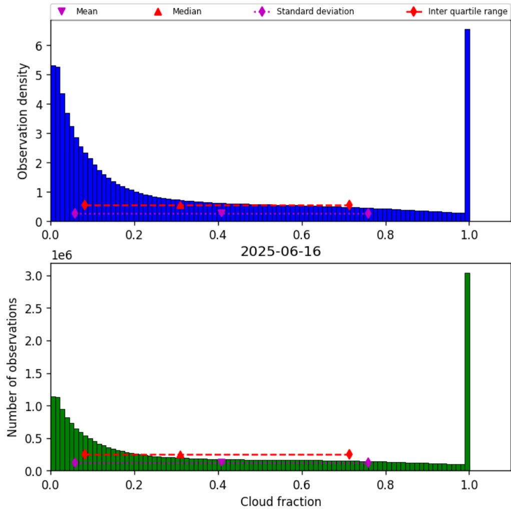
Figure 32: Histogram of “Cloud fraction” for 2025-06-16 to 2025-06-17
