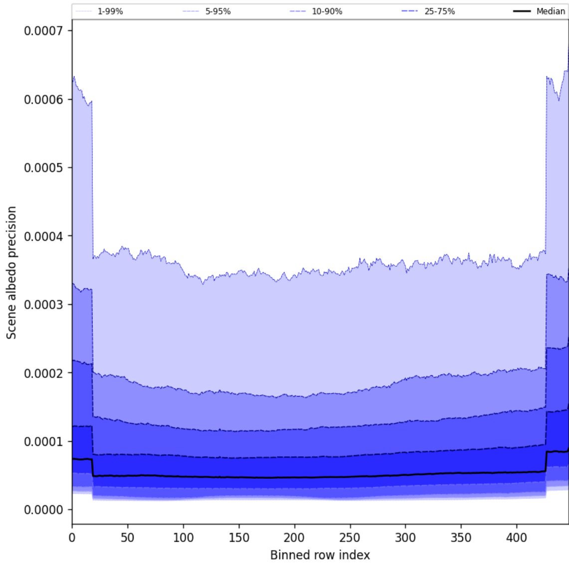
Figure 52: Along track statistics of “Scene albedo precision” for 2025-06-16 to 2025-06-17
