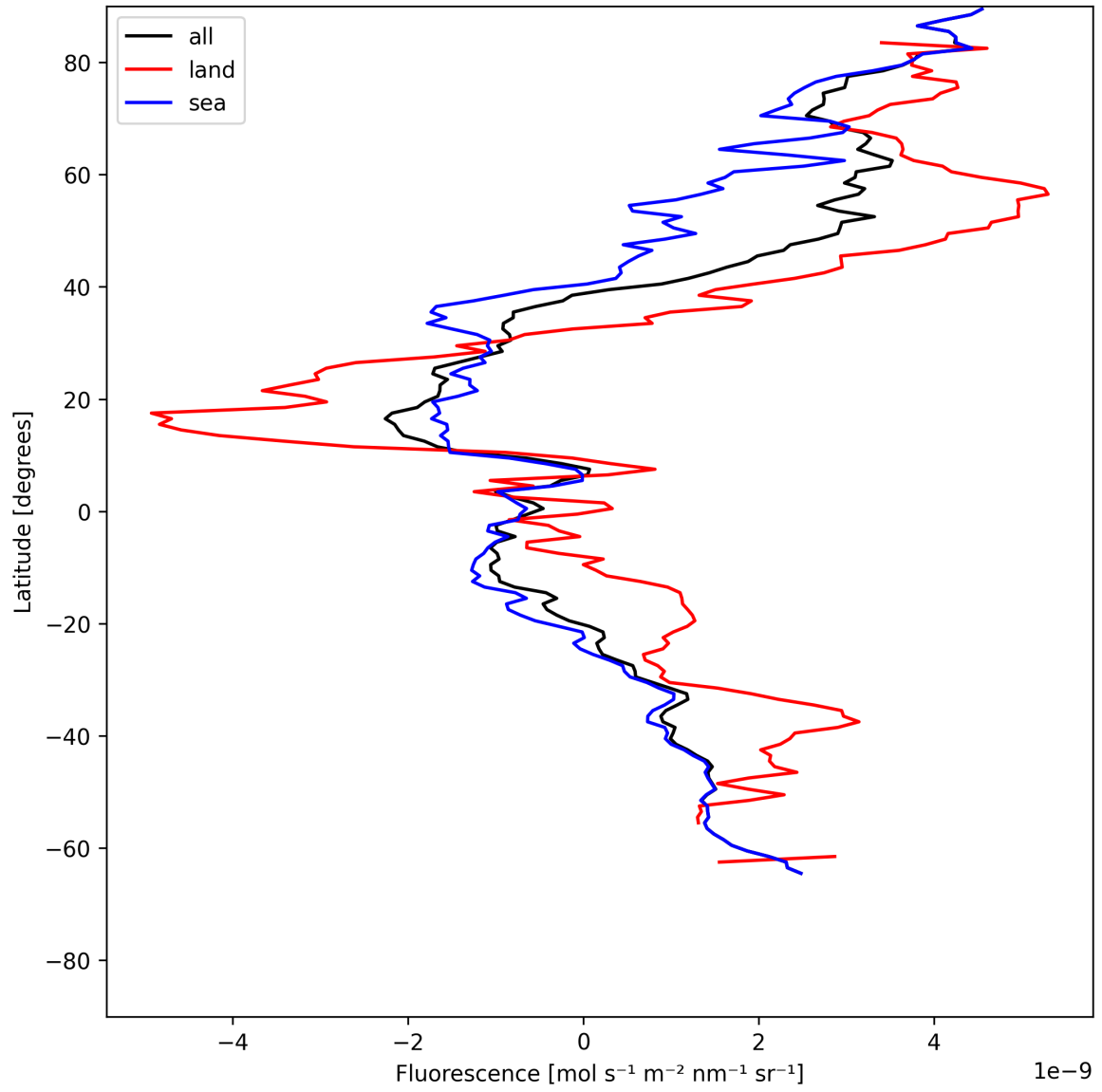
Figure 23: Zonal average of “Fluorescence” for 2025-06-16 to 2025-06-17.
