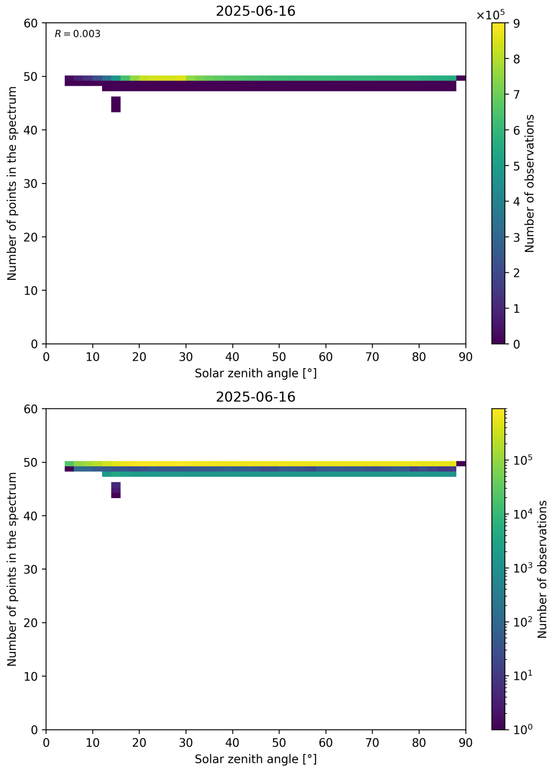
Figure 115: Scatter density plot of “Solar zenith angle” against “Number of points in the spectrum” for 2025-06-16 to 2025-06-17.
