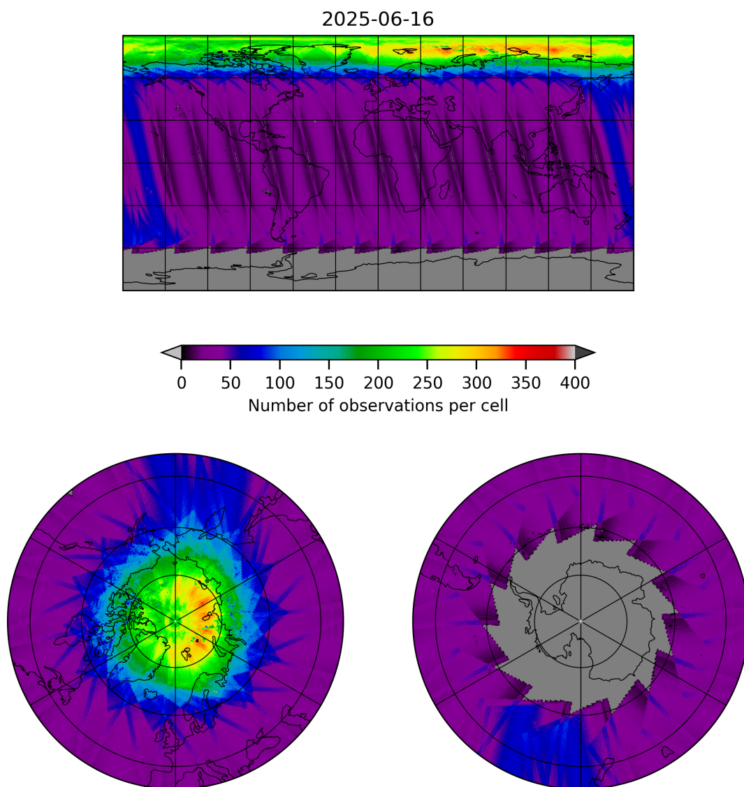
Figure 11: Map of the number of observations for 2025-06-16 to 2025-06-17
