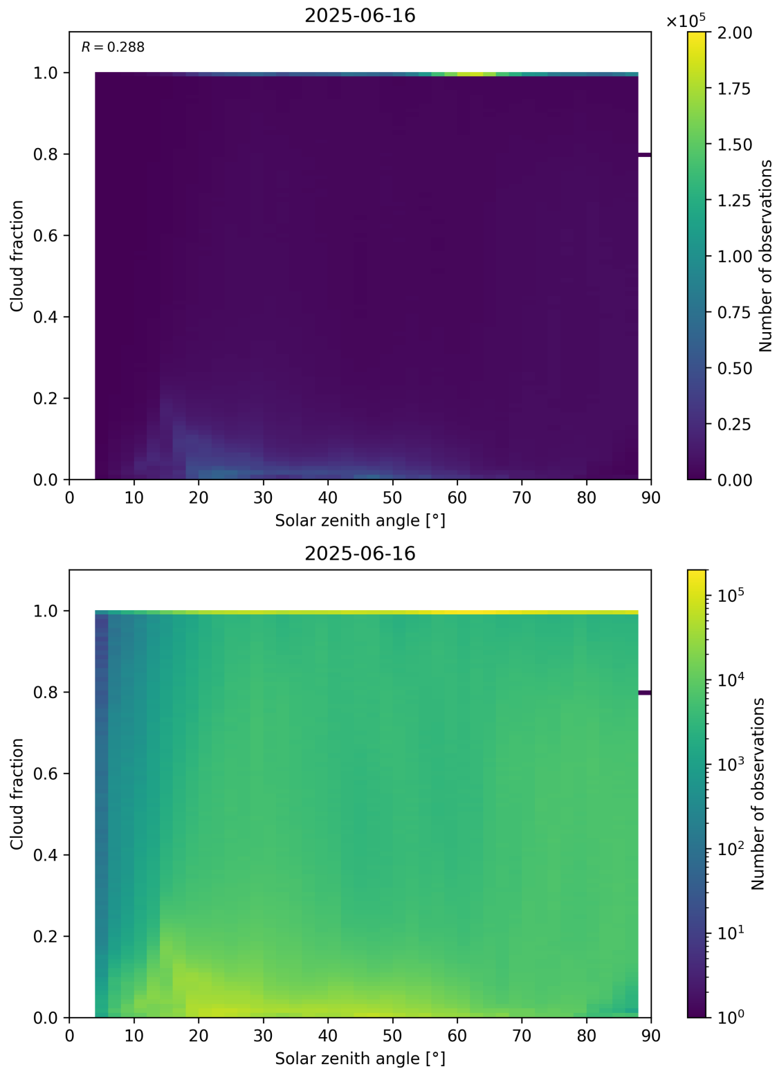
Figure 110: Scatter density plot of “Solar zenith angle” against “Cloud fraction” for 2025-06-16 to 2025-06-17.
