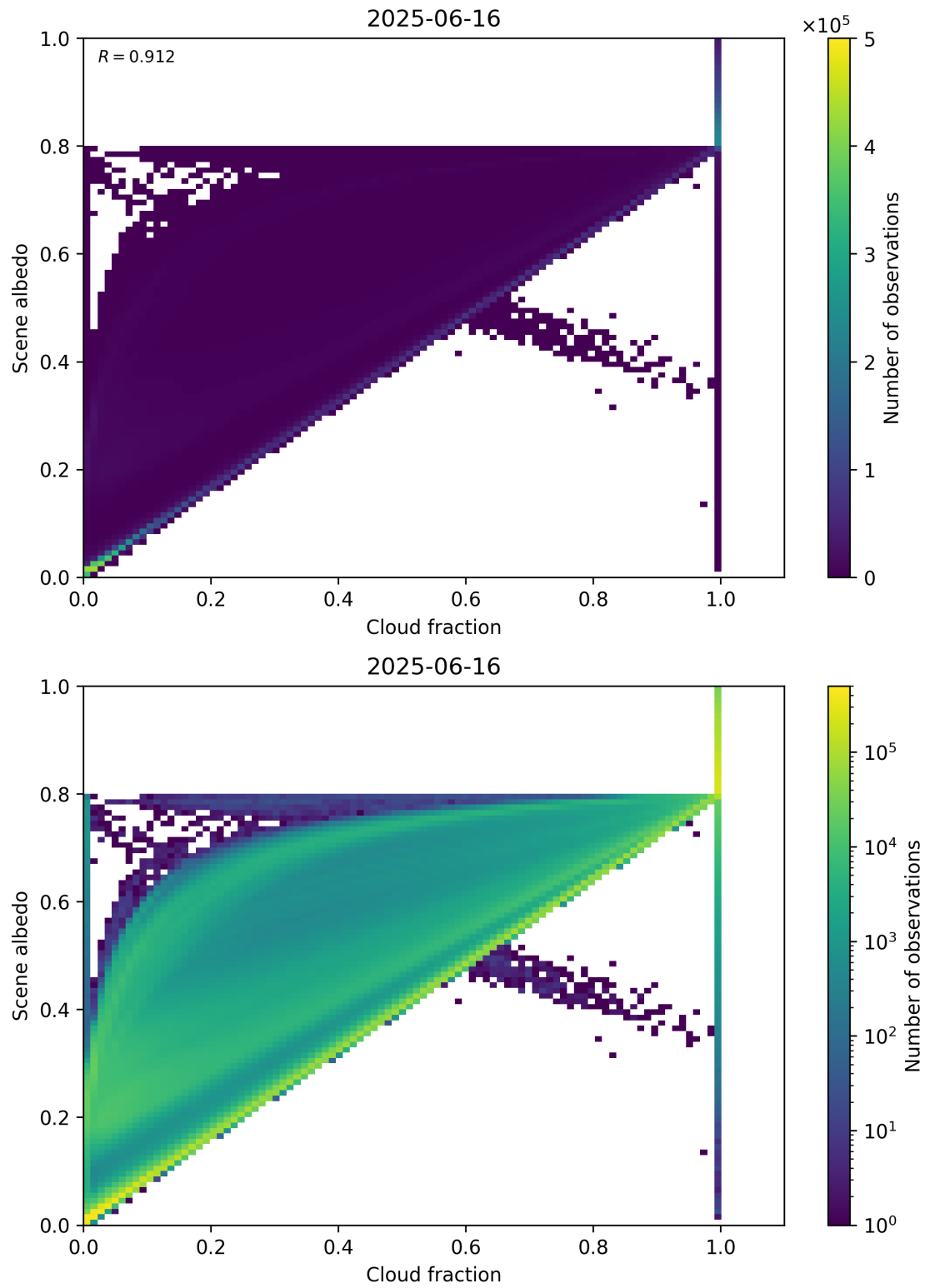
Figure 75: Scatter density plot of “Cloud fraction” against “Scene albedo” for 2025-06-16 to 2025-06-17.
