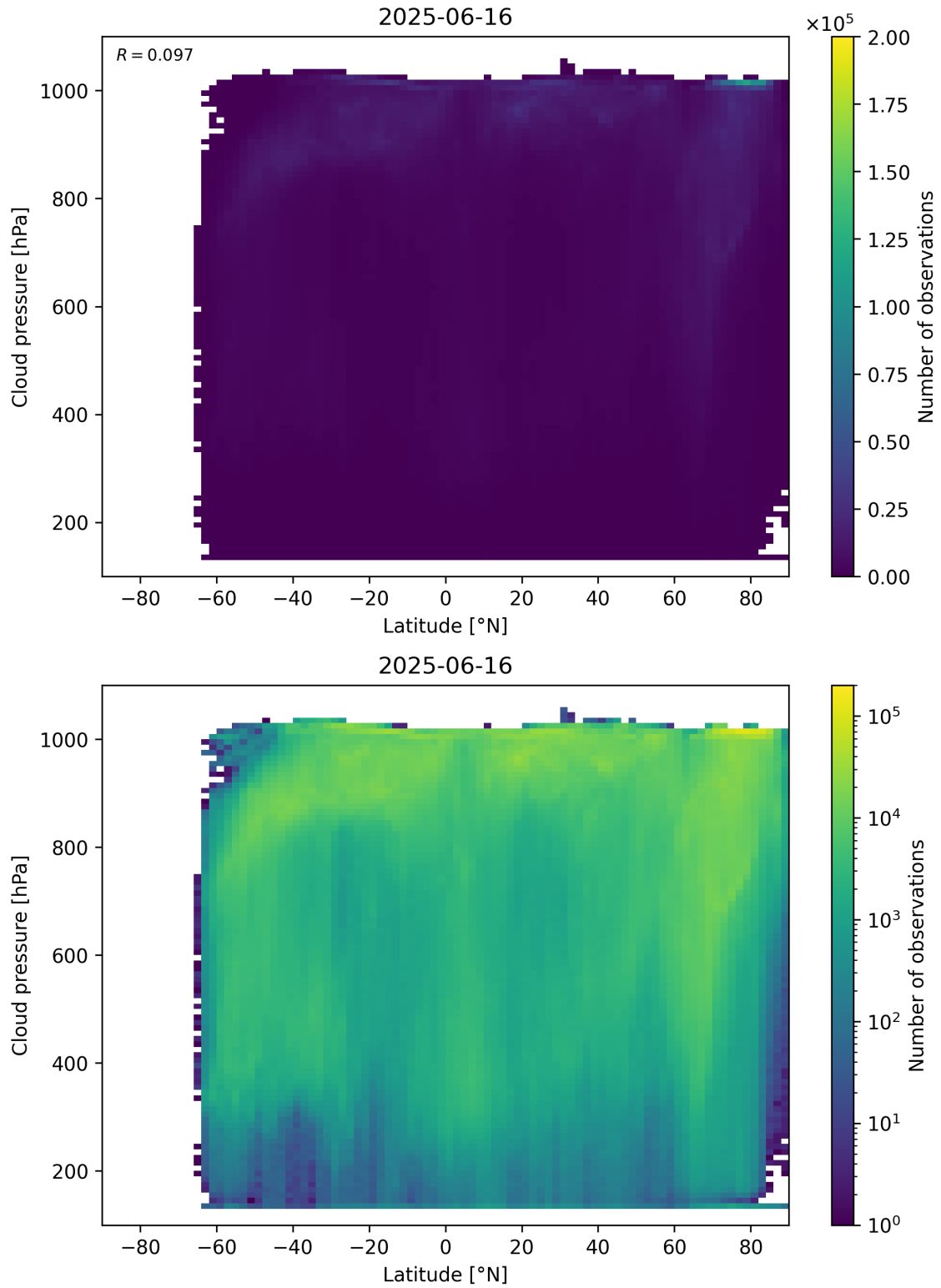
Figure 91: Scatter density plot of “Latitude” against “Cloud pressure” for 2025-06-16 to 2025-06-17.
