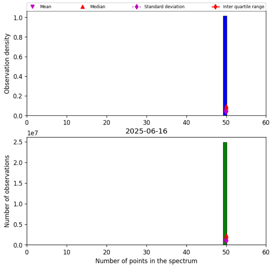
Figure 44: Histogram of “Number of points in the spectrum” for 2025-06-16 to 2025-06-17
