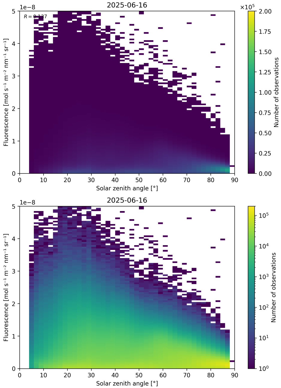
Figure 112: Scatter density plot of “Solar zenith angle” against “Fluorescence” for 2025-06-16 to 2025-06-17.
