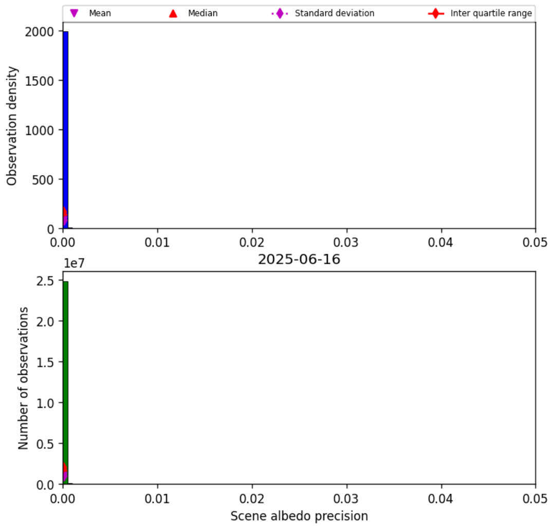
Figure 35: Histogram of “Scene albedo precision” for 2025-06-16 to 2025-06-17
