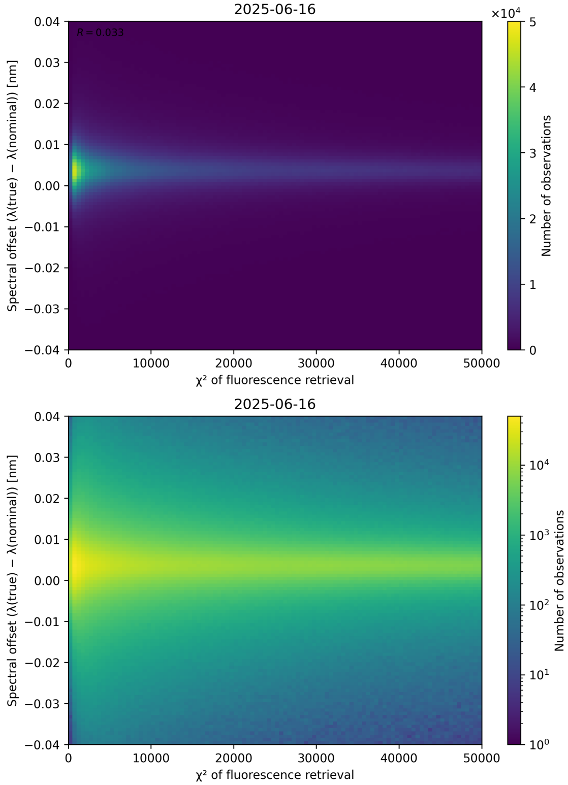
Figure 69: Scatter density plot of “ \chi^2 of fluorescence retrieval” against “Spectral offset ( \lambda_{\text{true}} - \lambda_{\text{nominal}} )” for 2025-06-16 to 2025-06-17.
