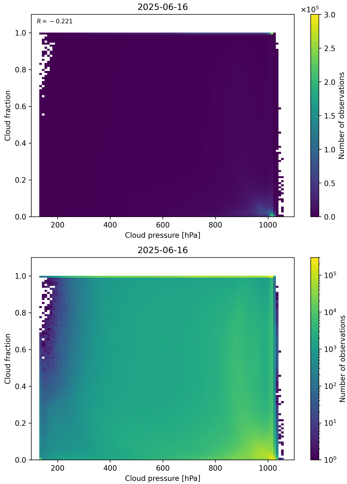
Figure 79: Scatter density plot of “Cloud pressure” against “Cloud fraction” for 2025-06-16 to 2025-06-17.
