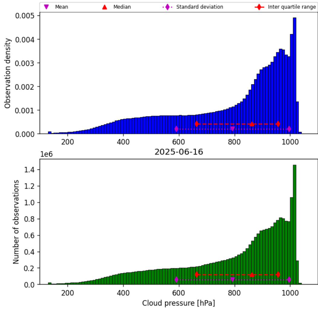
Figure 30: Histogram of “Cloud pressure” for 2025-06-16 to 2025-06-17
