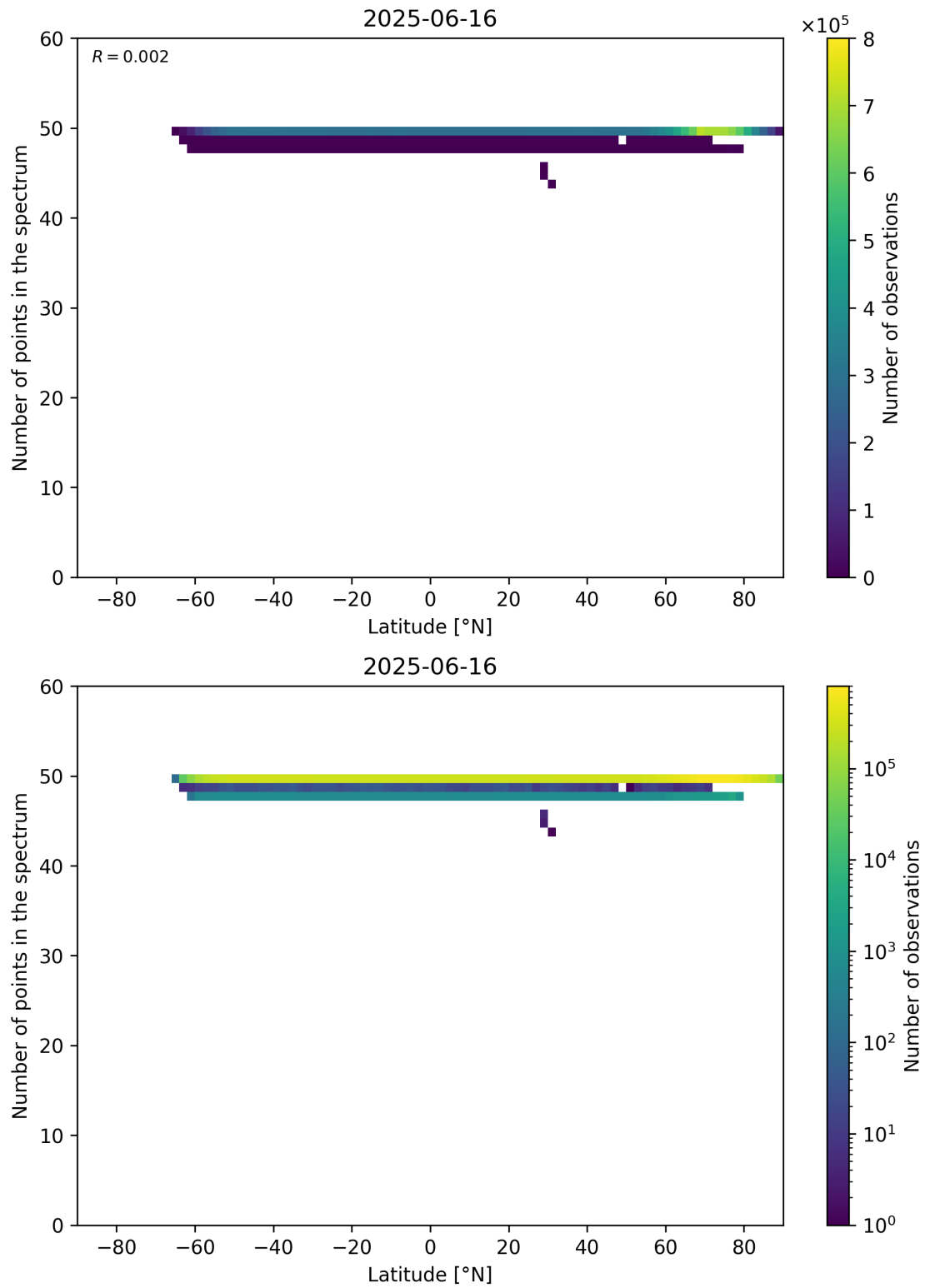
Figure 94: Scatter density plot of “Latitude” against “Number of points in the spectrum” for 2025-06-16 to 2025-06-17.
