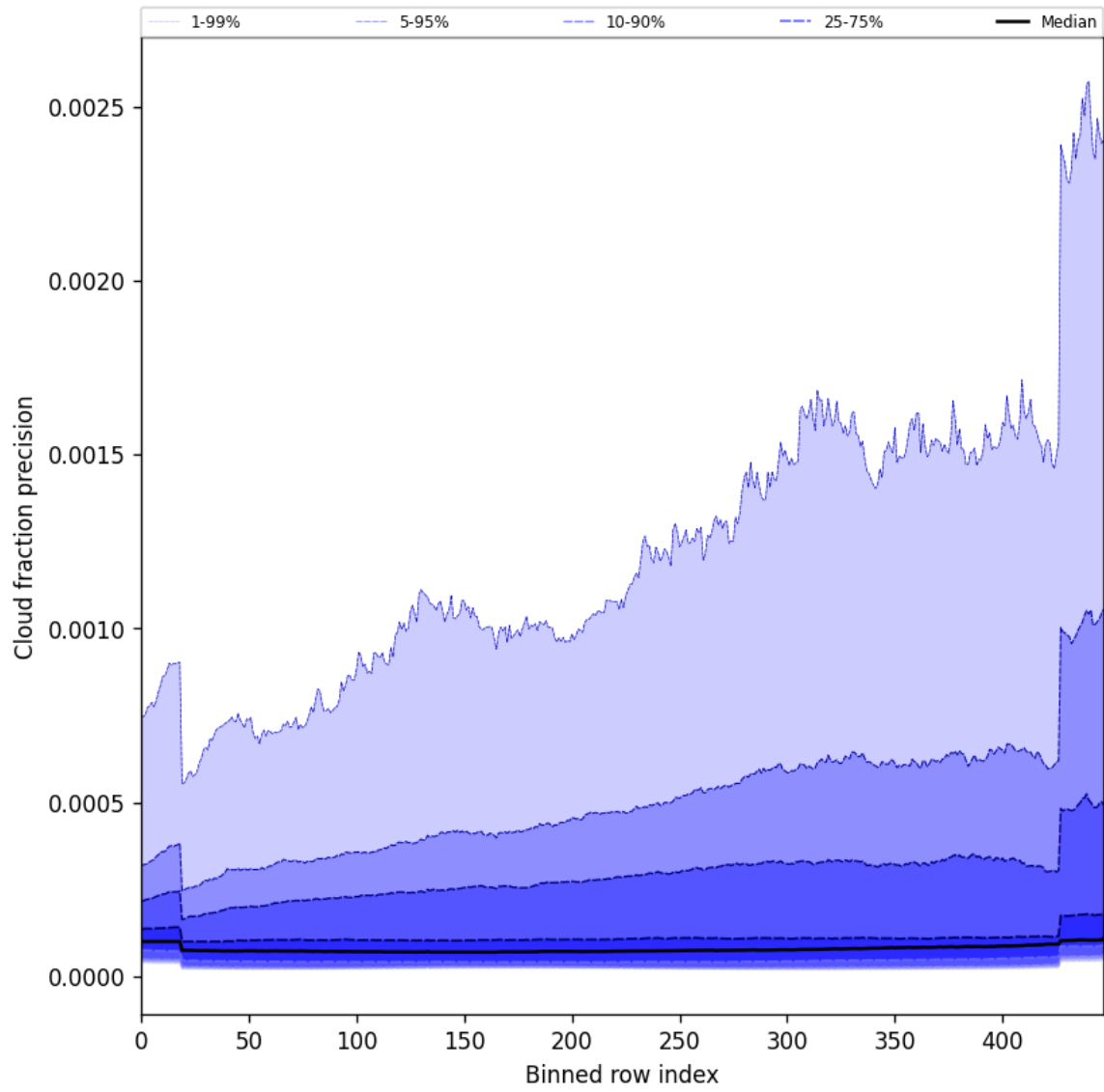
Figure 50: Along track statistics of “Cloud fraction precision” for 2025-06-16 to 2025-06-17
