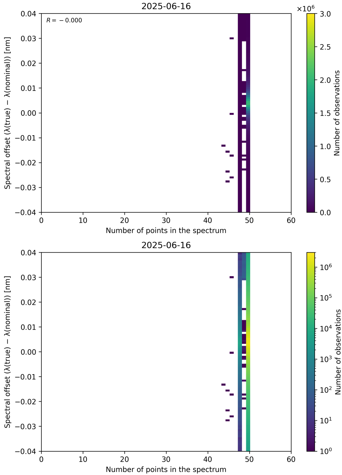
Figure 101: Scatter density plot of “Number of points in the spectrum” against “Spectral offset ( \lambda_{\text{true}} - \lambda_{\text{nominal}} )” for 2025-06-16 to 2025-06-17.
