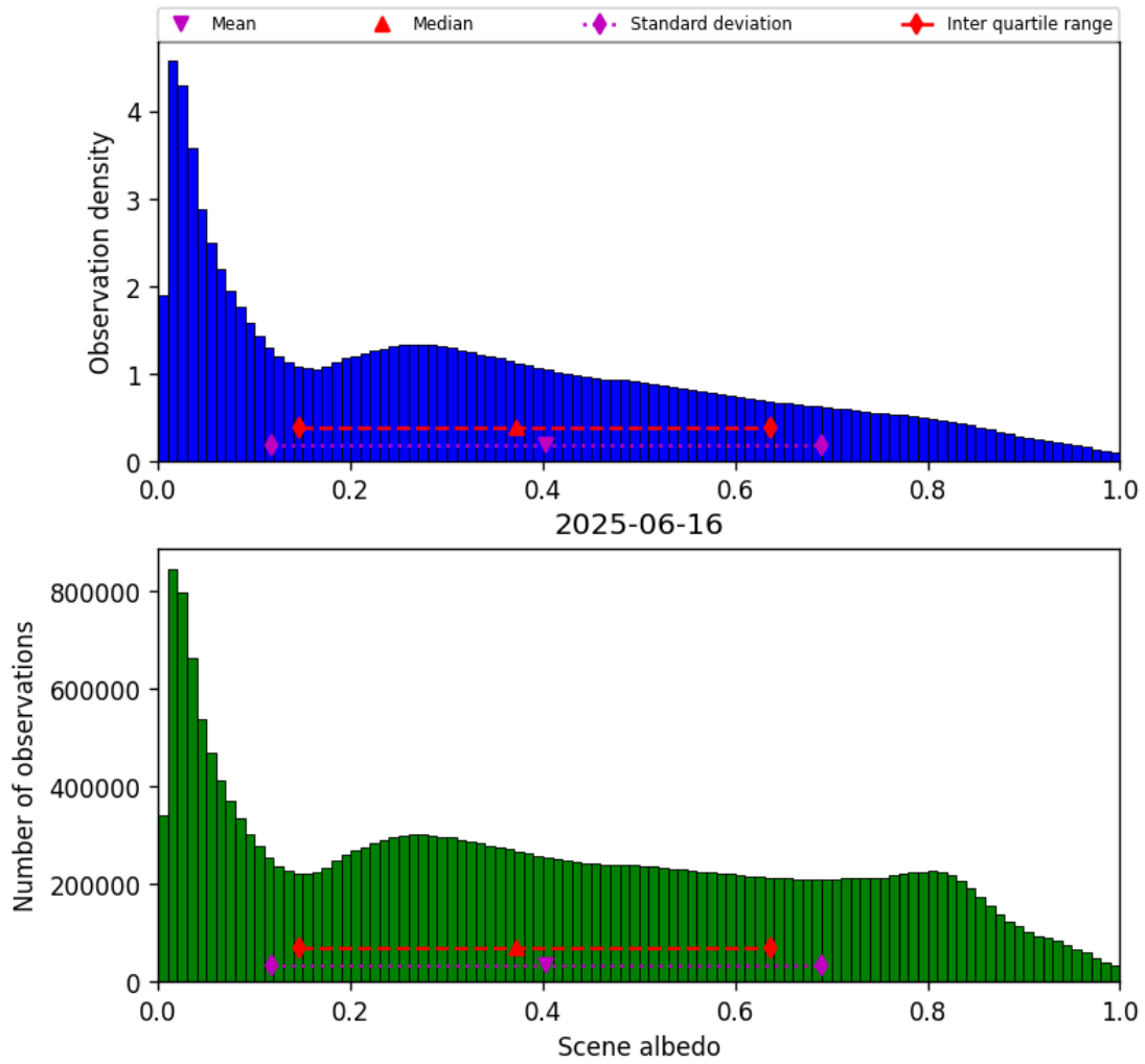
Figure 34: Histogram of “Scene albedo” for 2025-06-16 to 2025-06-17
