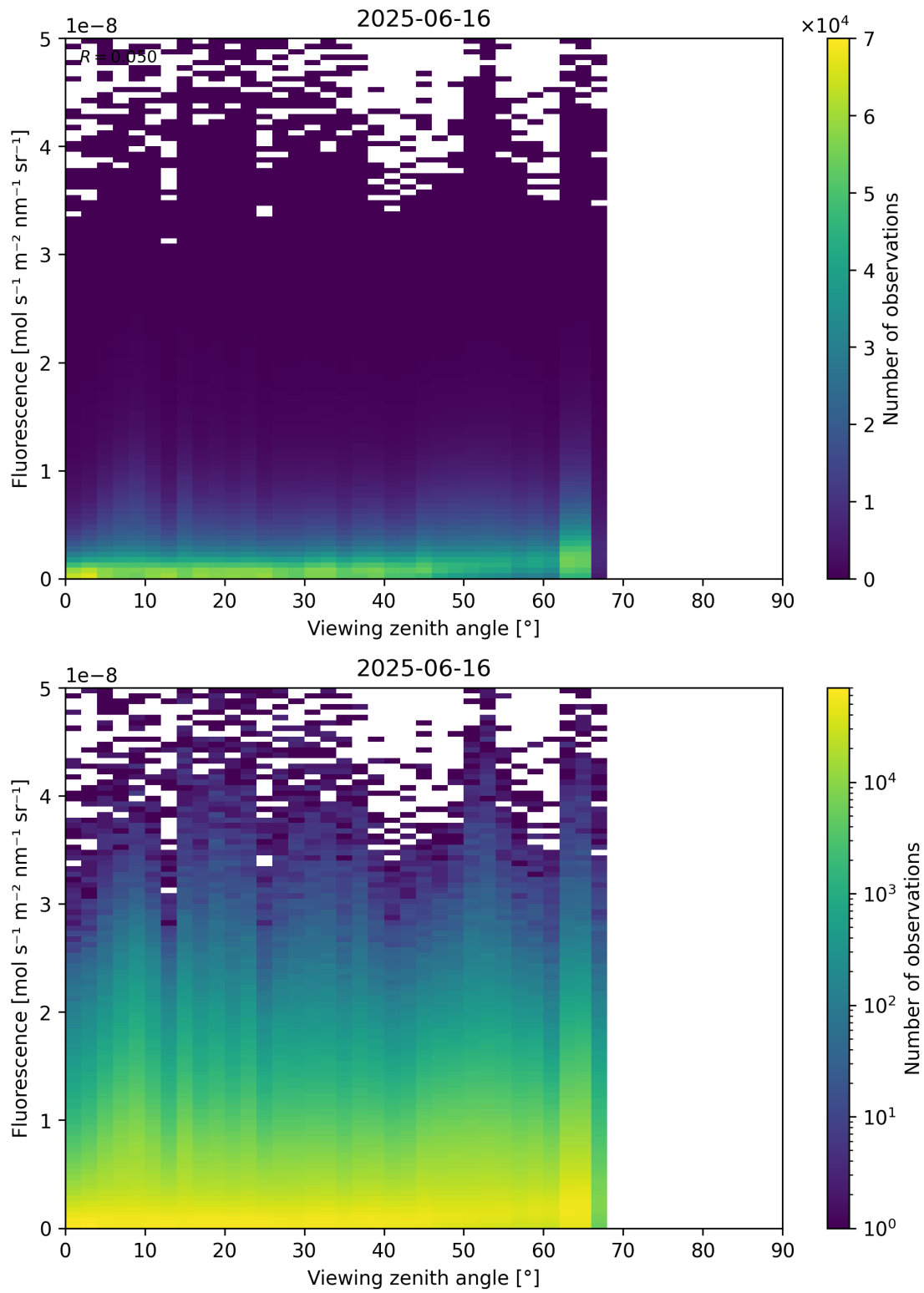
Figure 122: Scatter density plot of “Viewing zenith angle” against “Fluorescence” for 2025-06-16 to 2025-06-17.
