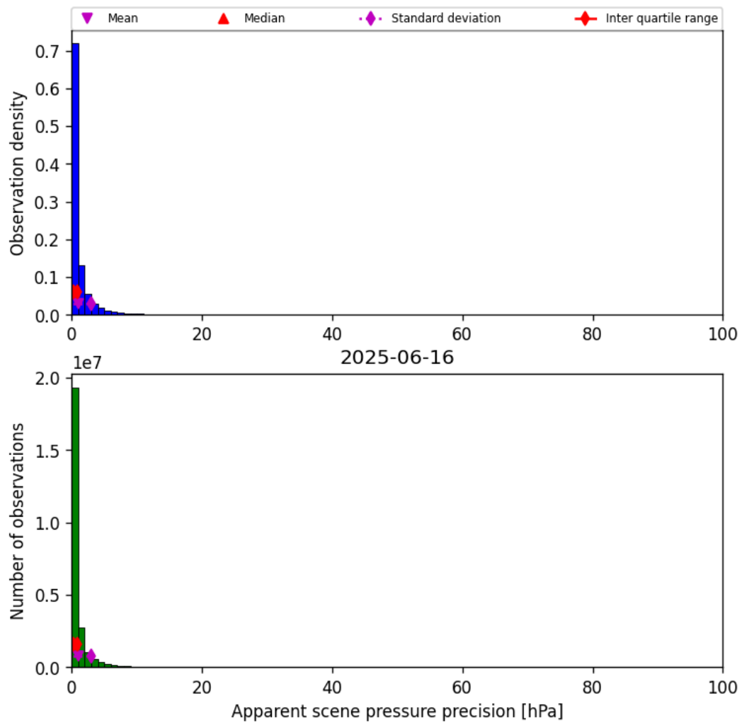
Figure 37: Histogram of “Apparent scene pressure precision” for 2025-06-16 to 2025-06-17
