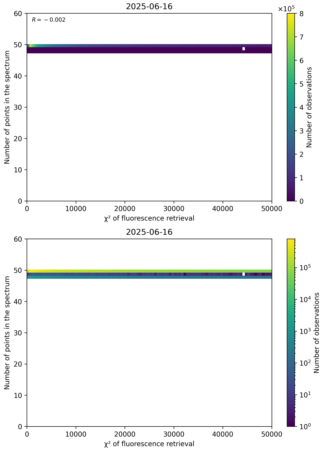
Figure 68: Scatter density plot of “ \chi^2 of fluorescence retrieval” against “Number of points in the spectrum” for 2025-06-16 to 2025-06-17.
