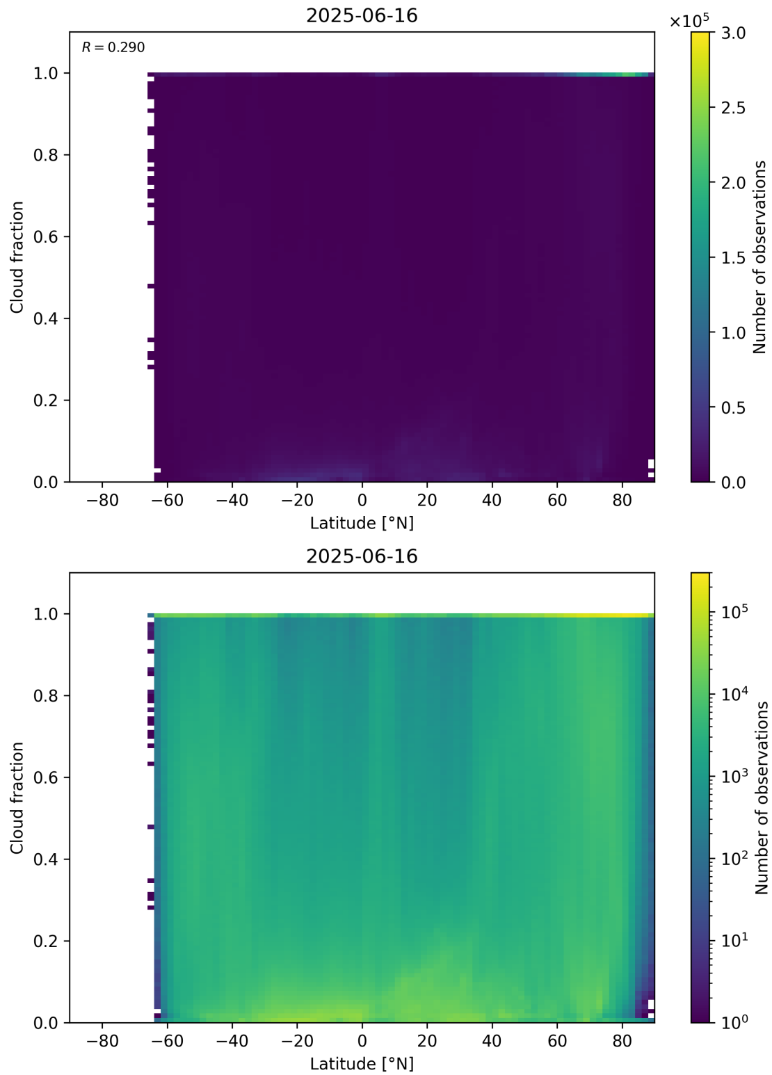
Figure 90: Scatter density plot of “Latitude” against “Cloud fraction” for 2025-06-16 to 2025-06-17.
