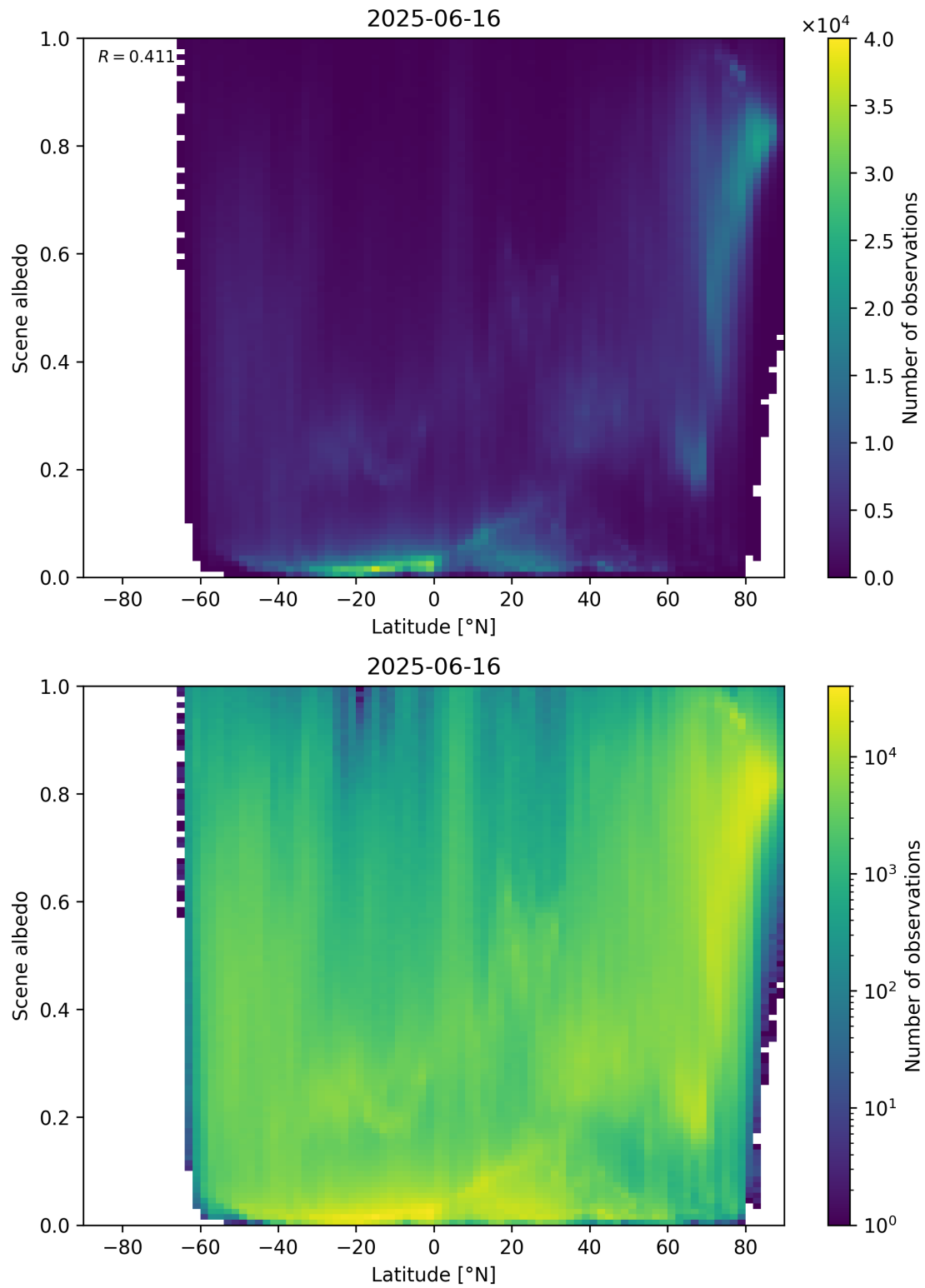
Figure 95: Scatter density plot of “Latitude” against “Scene albedo” for 2025-06-16 to 2025-06-17.
