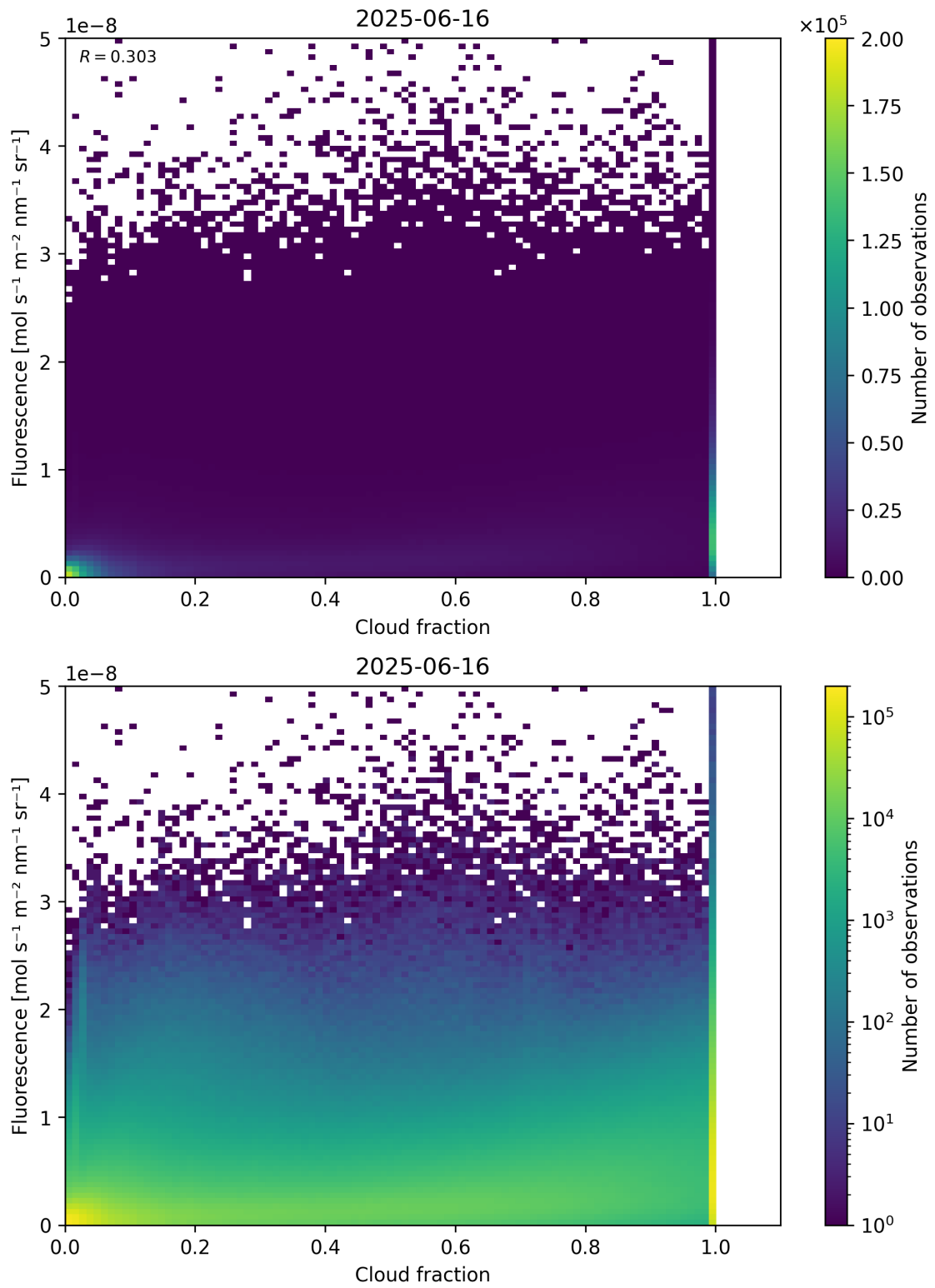
Figure 72: Scatter density plot of “Cloud fraction” against “Fluorescence” for 2025-06-16 to 2025-06-17.
