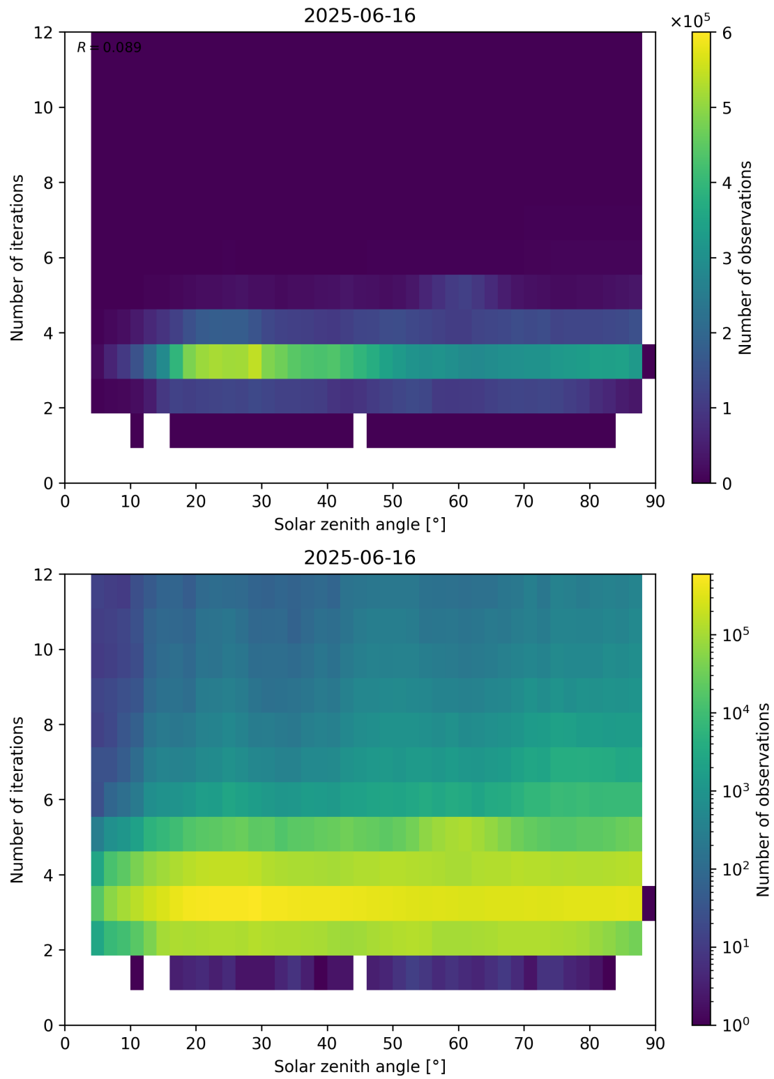
Figure 114: Scatter density plot of “Solar zenith angle” against “Number of iterations” for 2025-06-16 to 2025-06-17.
