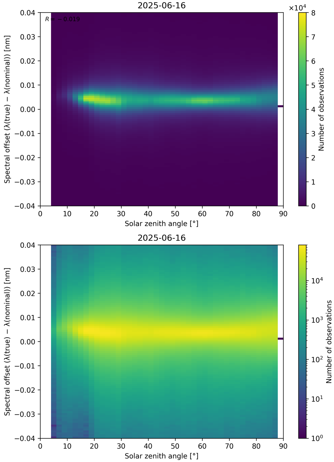
Figure 117: Scatter density plot of “Solar zenith angle” against “Spectral offset ( \lambda_{\text{true}} - \lambda_{\text{nominal}} )” for 2025-06-16 to 2025-06-17.
