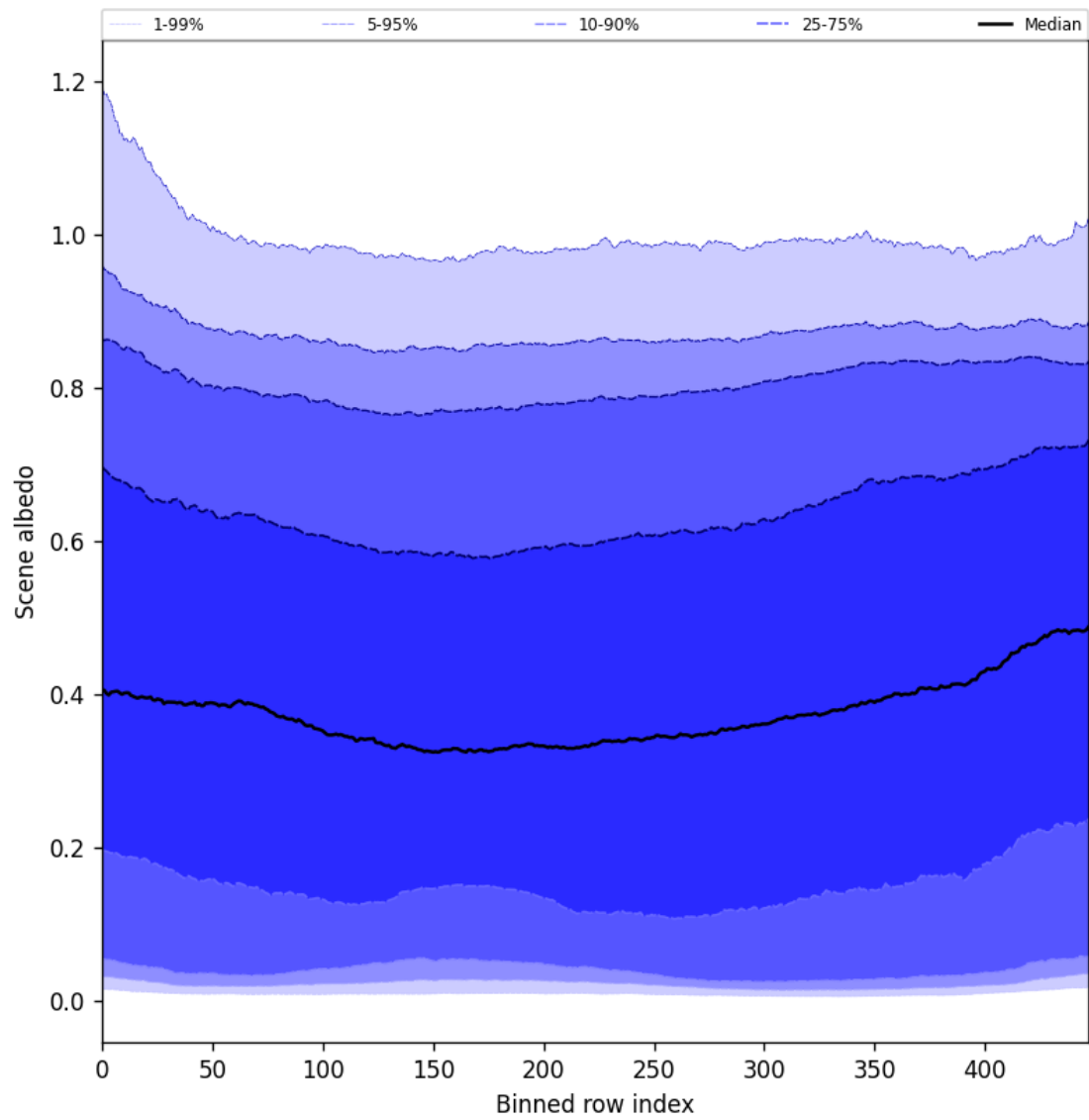
Figure 51: Along track statistics of “Scene albedo” for 2025-06-16 to 2025-06-17
