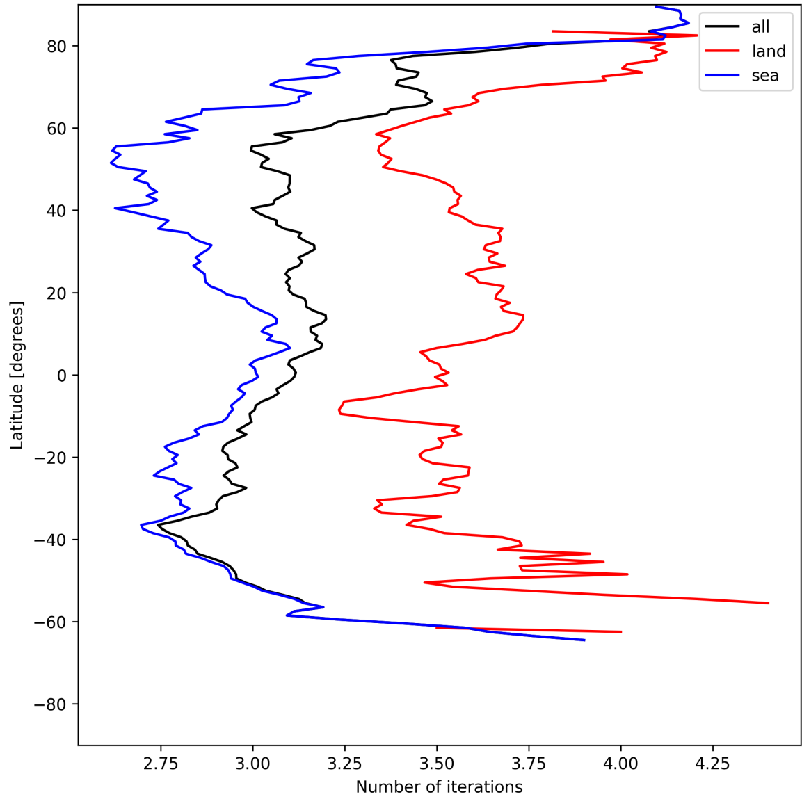
Figure 22: Zonal average of “Number of iterations” for 2025-06-16 to 2025-06-17.
