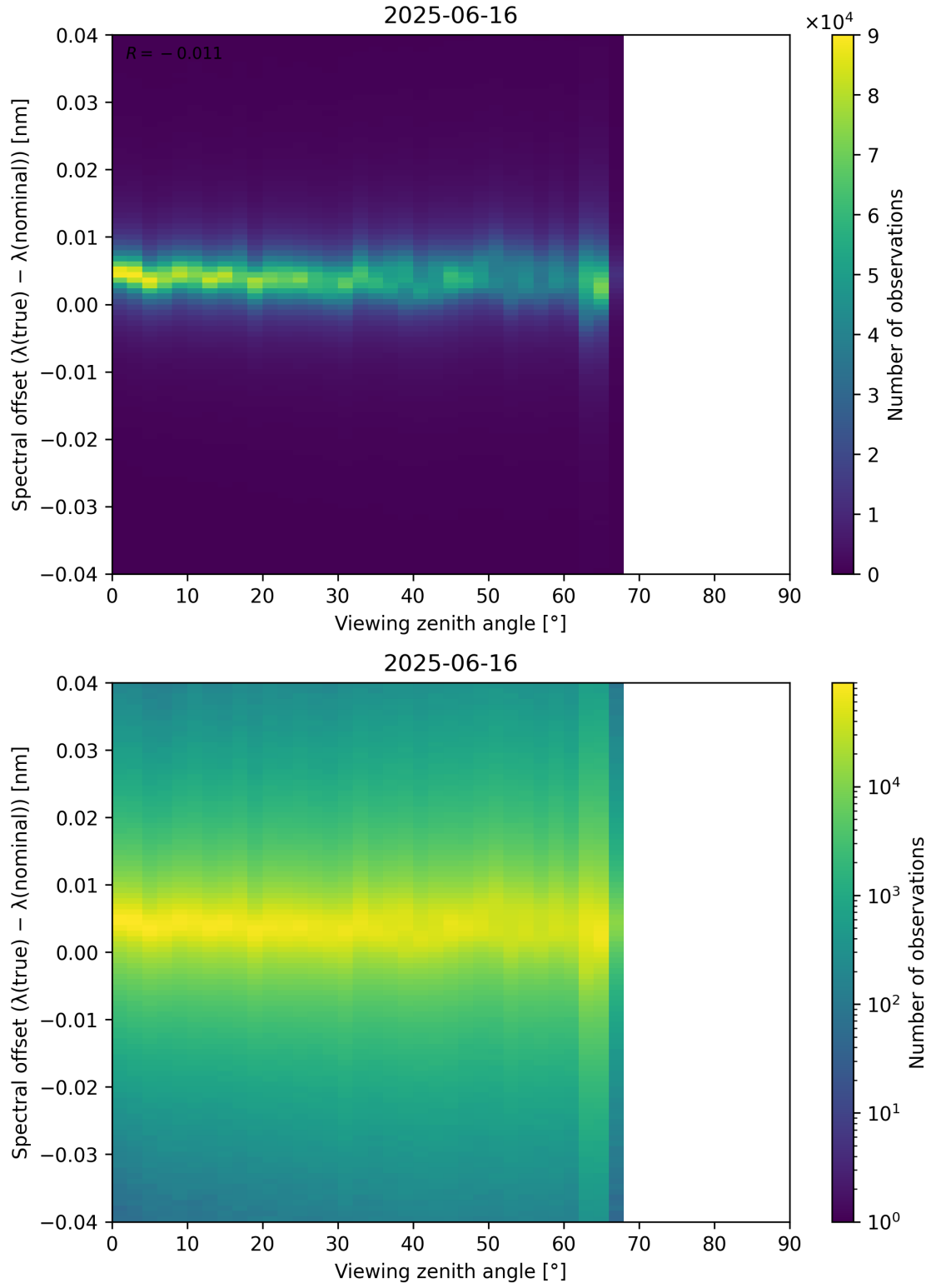
Figure 128: Scatter density plot of “Viewing zenith angle” against “Spectral offset ( \lambda_{\text{true}} - \lambda_{\text{nominal}} )” for 2025-06-16 to 2025-06-17.
