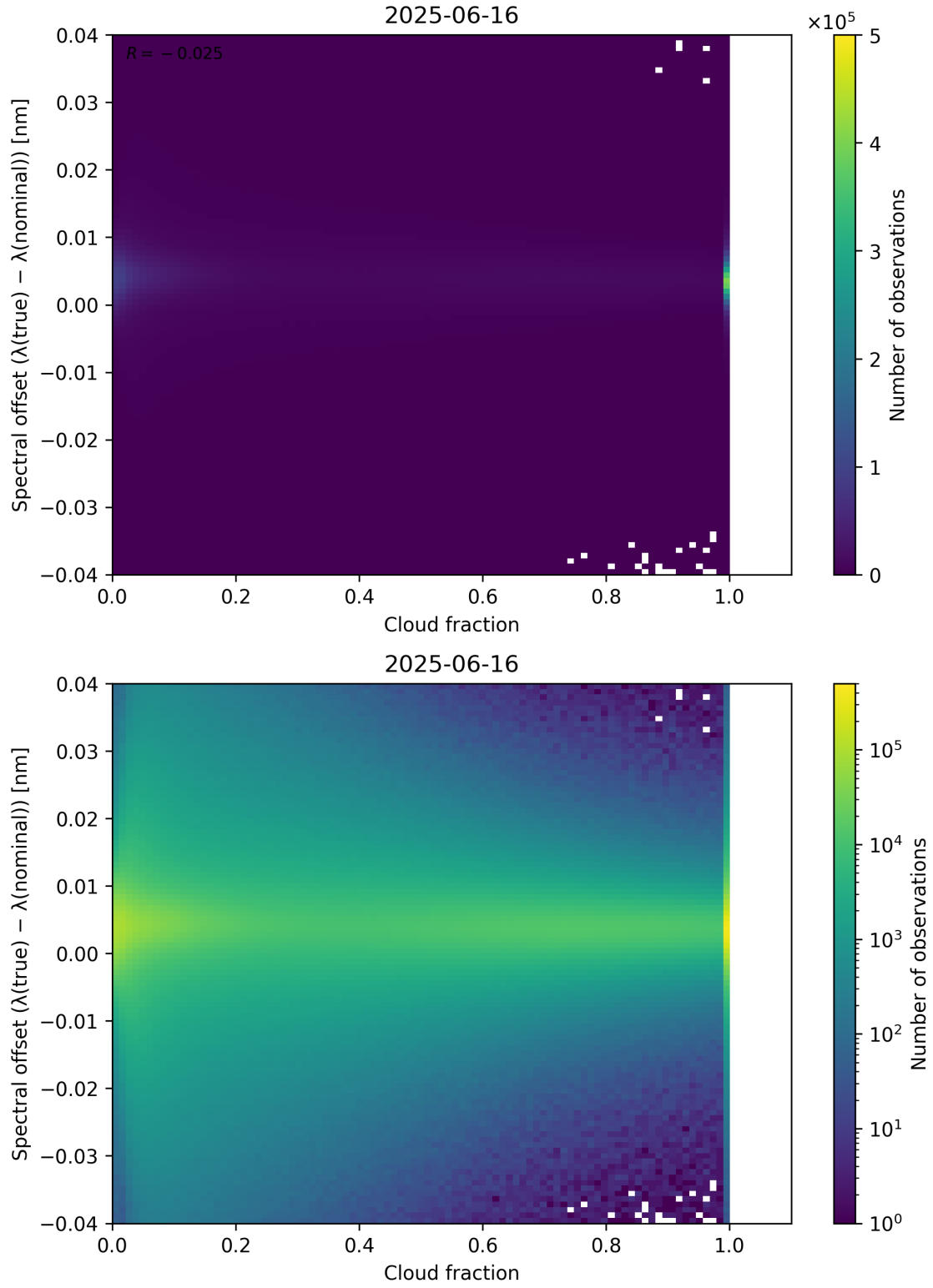
Figure 76: Scatter density plot of “Cloud fraction” against “Spectral offset ( \lambda_{\text{true}} - \lambda_{\text{nominal}} )” for 2025-06-16 to 2025-06-17.
