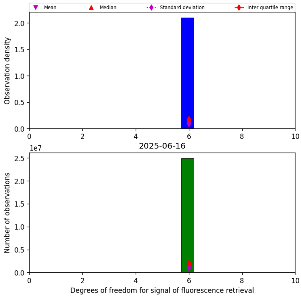
Figure 43: Histogram of “Degrees of freedom for signal of fluorescence retrieval” for 2025-06-16 to 2025-06-17
