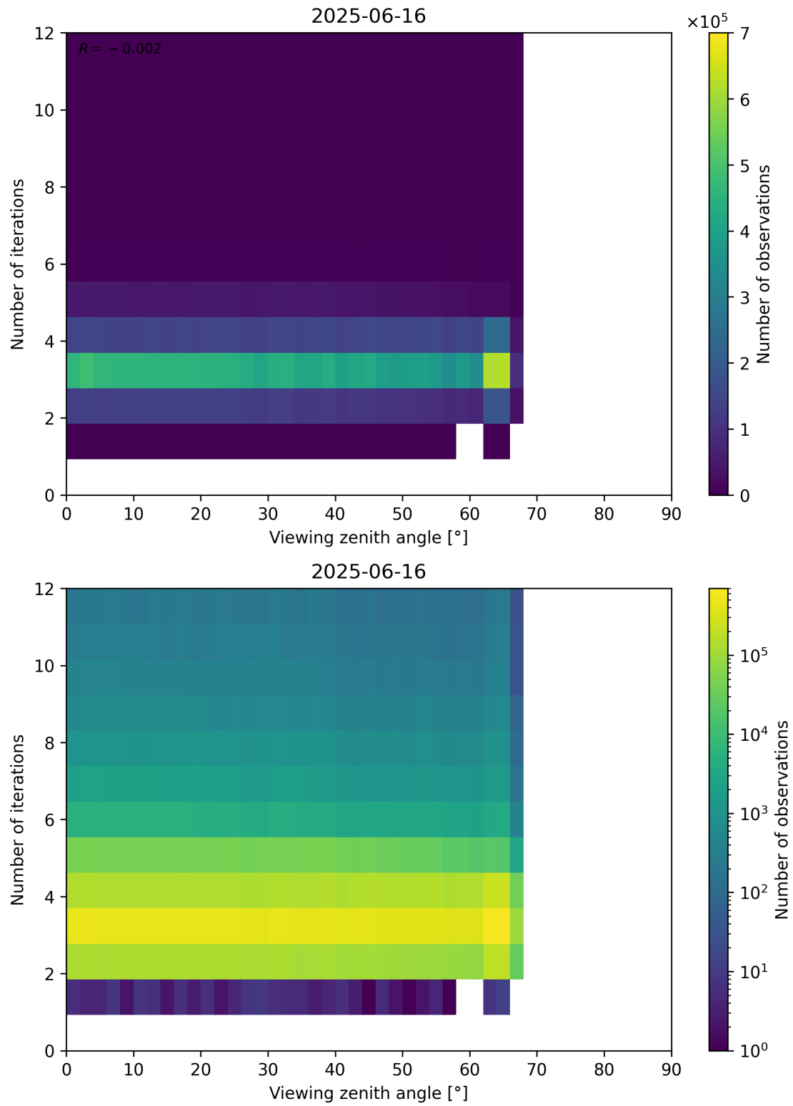
Figure 124: Scatter density plot of “Viewing zenith angle” against “Number of iterations” for 2025-06-16 to 2025-06-17.
