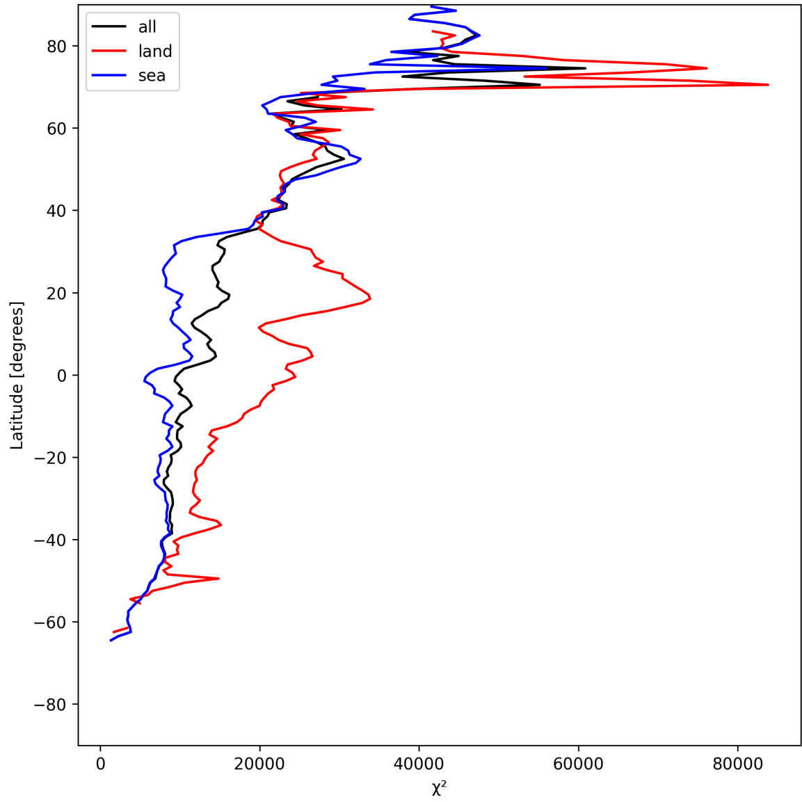
Figure 21: Zonal average of “ \chi^2 ” for 2025-06-16 to 2025-06-17.
