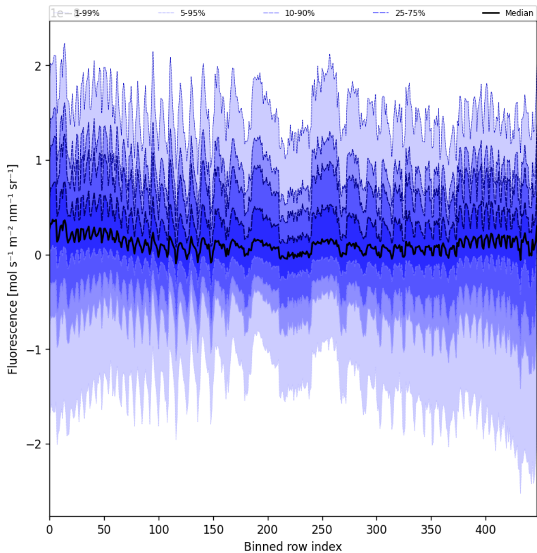
Figure 57: Along track statistics of “Fluorescence” for 2025-06-16 to 2025-06-17
