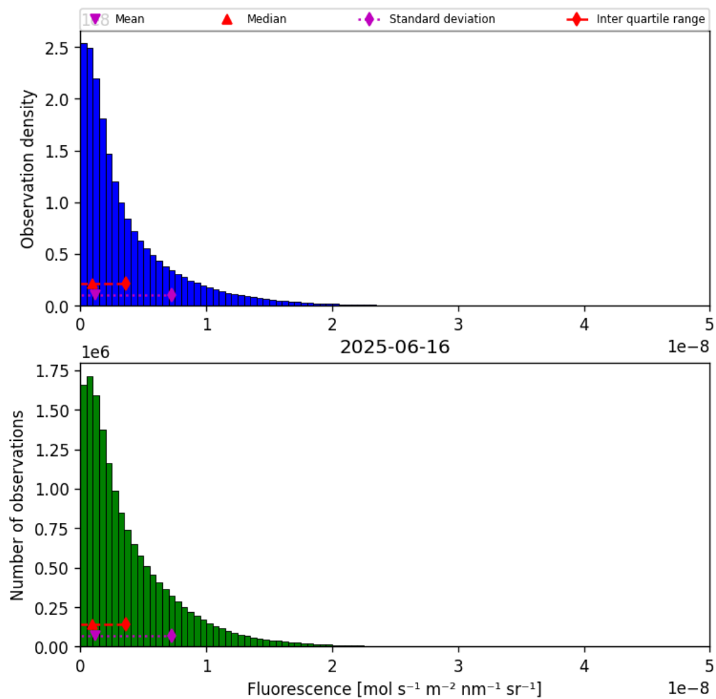
Figure 40: Histogram of “Fluorescence” for 2025-06-16 to 2025-06-17
