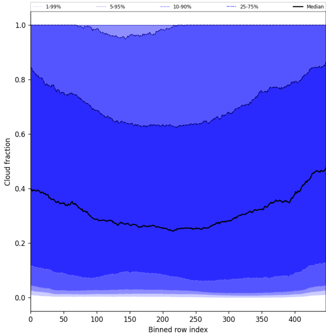
Figure 49: Along track statistics of “Cloud fraction” for 2025-06-16 to 2025-06-17
