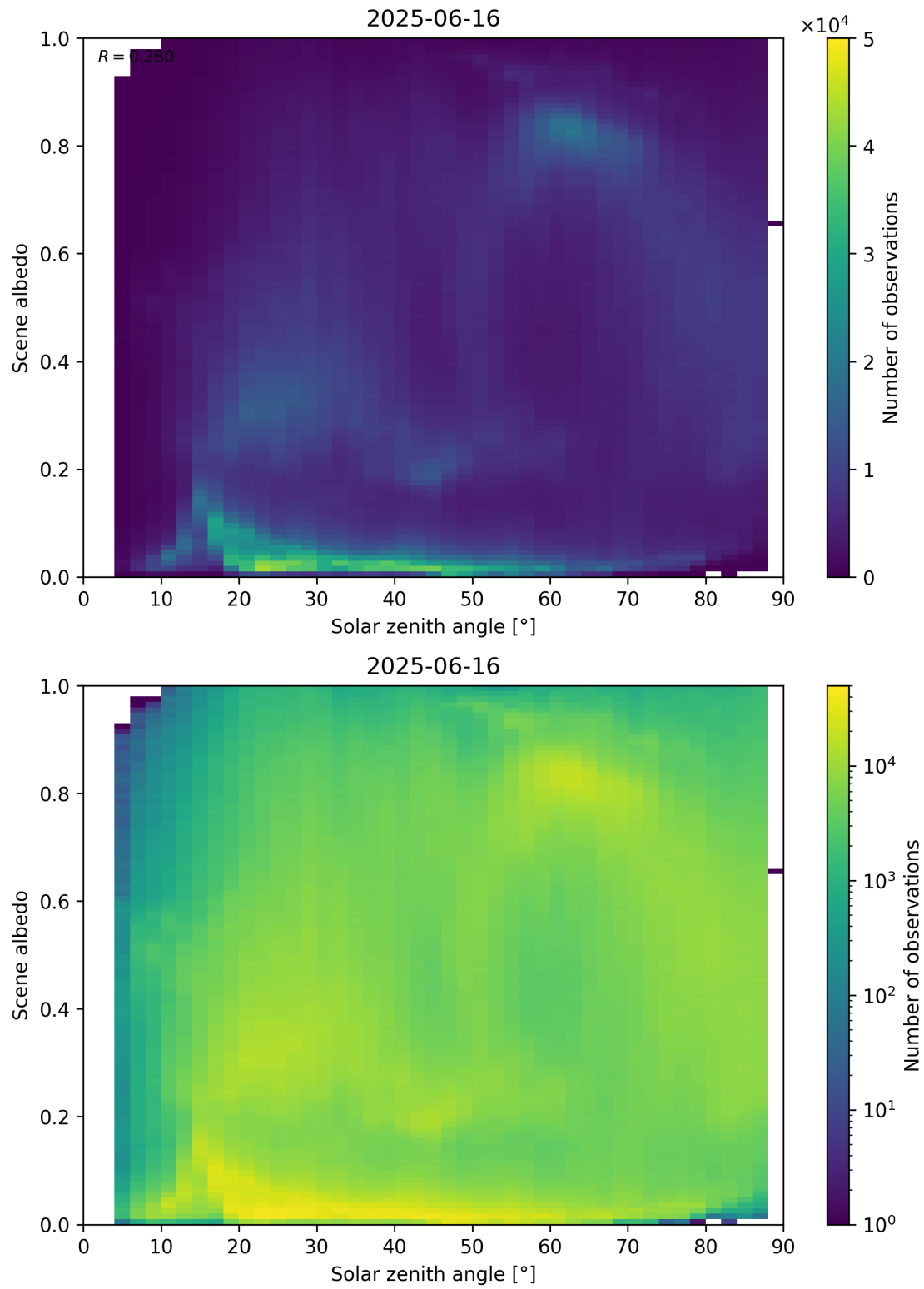
Figure 116: Scatter density plot of “Solar zenith angle” against “Scene albedo” for 2025-06-16 to 2025-06-17.
