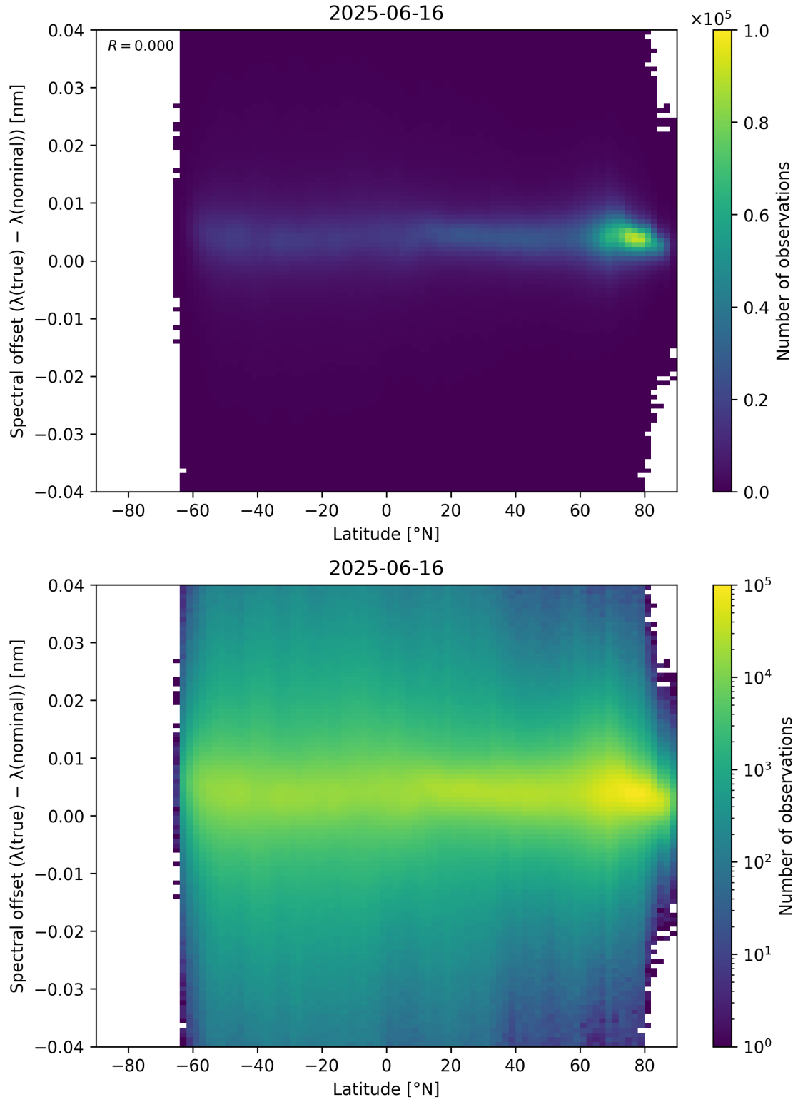
Figure 96: Scatter density plot of “Latitude” against “Spectral offset ( \lambda_{\text{true}} - \lambda_{\text{nominal}} )” for 2025-06-16 to 2025-06-17.
