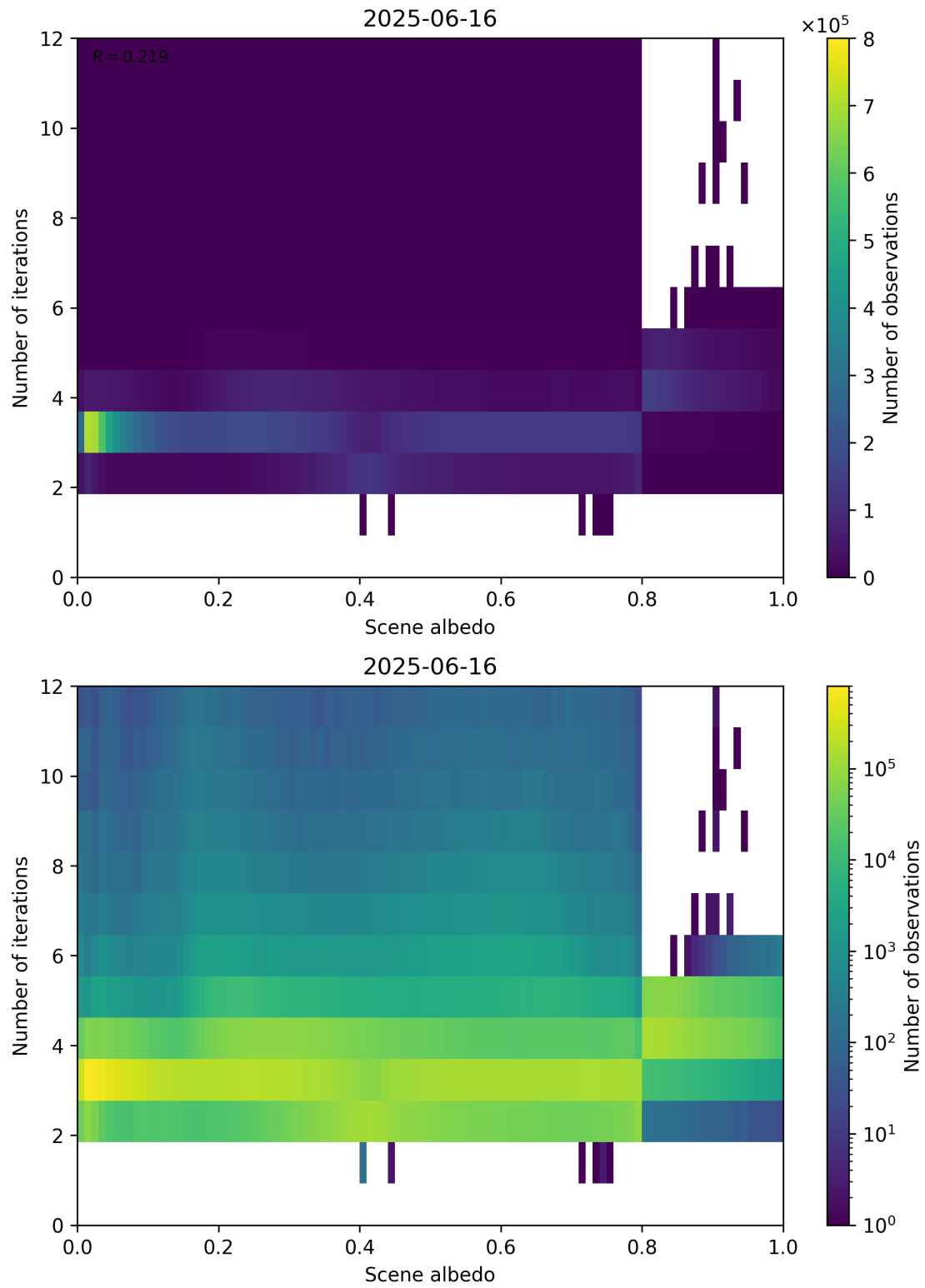
Figure 105: Scatter density plot of “Scene albedo” against “Number of iterations” for 2025-06-16 to 2025-06-17.
