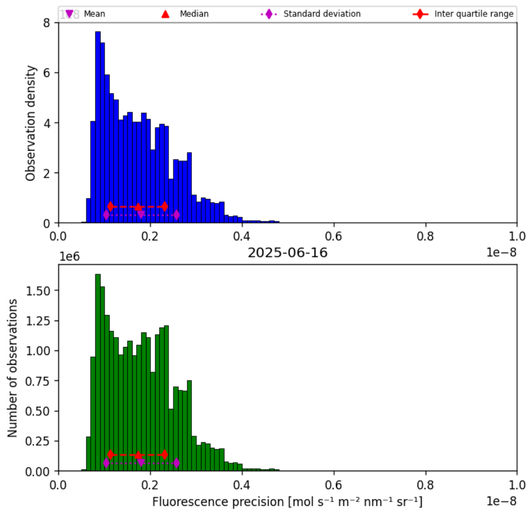
Figure 41: Histogram of “Fluorescence precision” for 2025-06-16 to 2025-06-17
