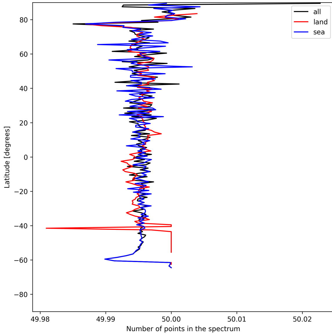
Figure 27: Zonal average of “Number of points in the spectrum” for 2025-06-16 to 2025-06-17.
