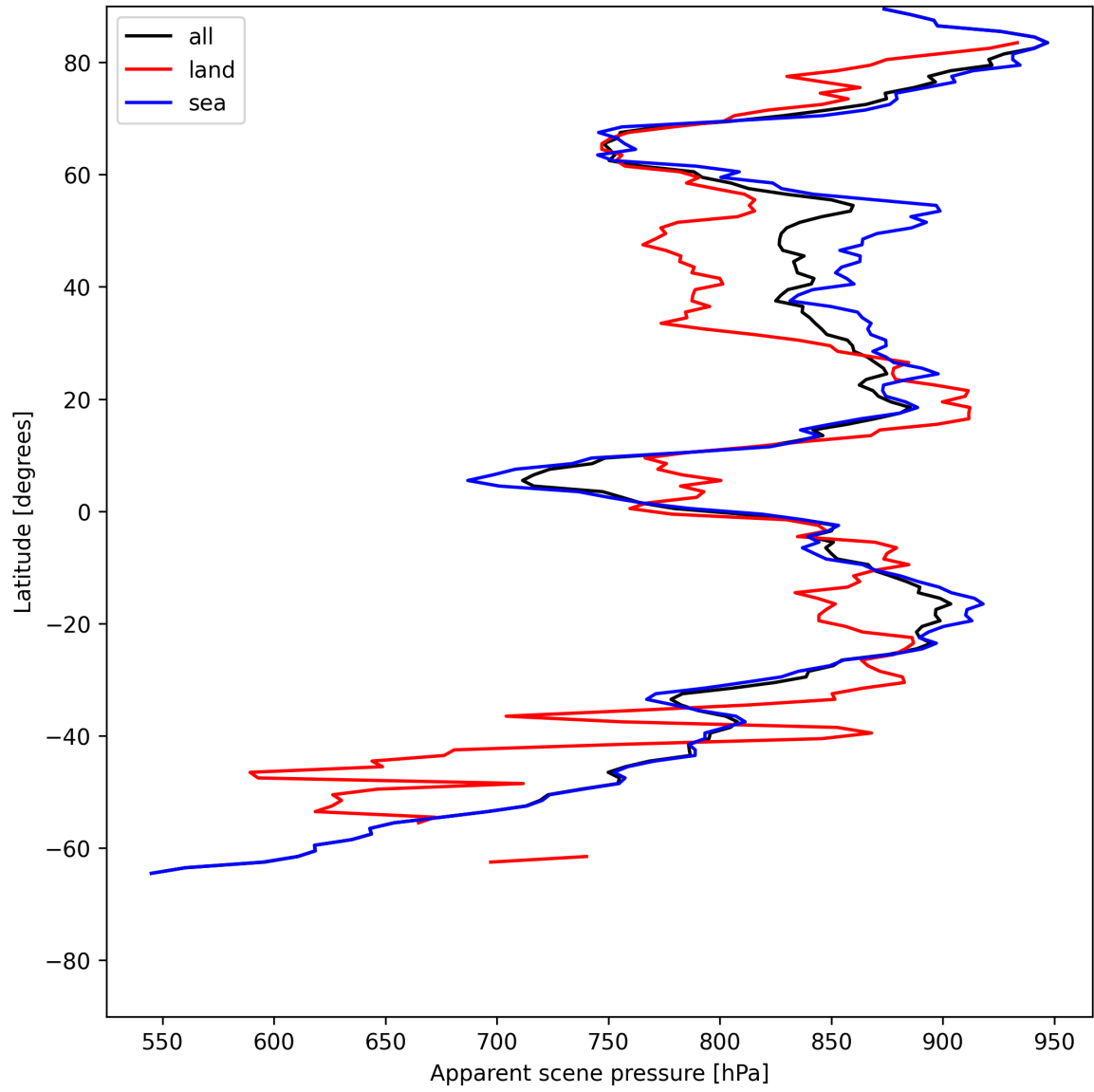
Figure 19: Zonal average of “Apparent scene pressure” for 2025-06-16 to 2025-06-17.
