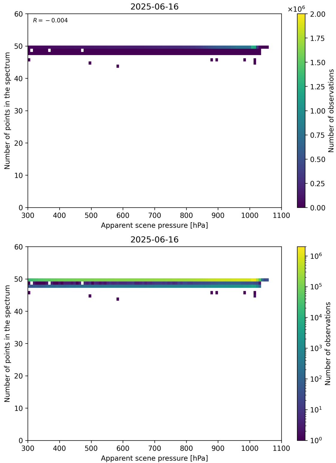
Figure 66: Scatter density plot of “Apparent scene pressure” against “Number of points in the spectrum” for 2025-06-16 to 2025-06-17.
