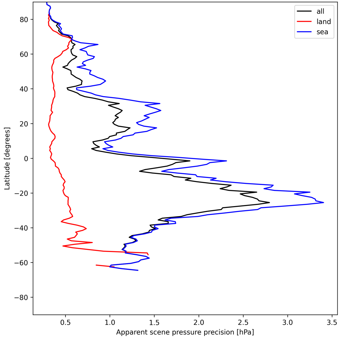
Figure 20: Zonal average of “Apparent scene pressure precision” for 2025-06-16 to 2025-06-17.
