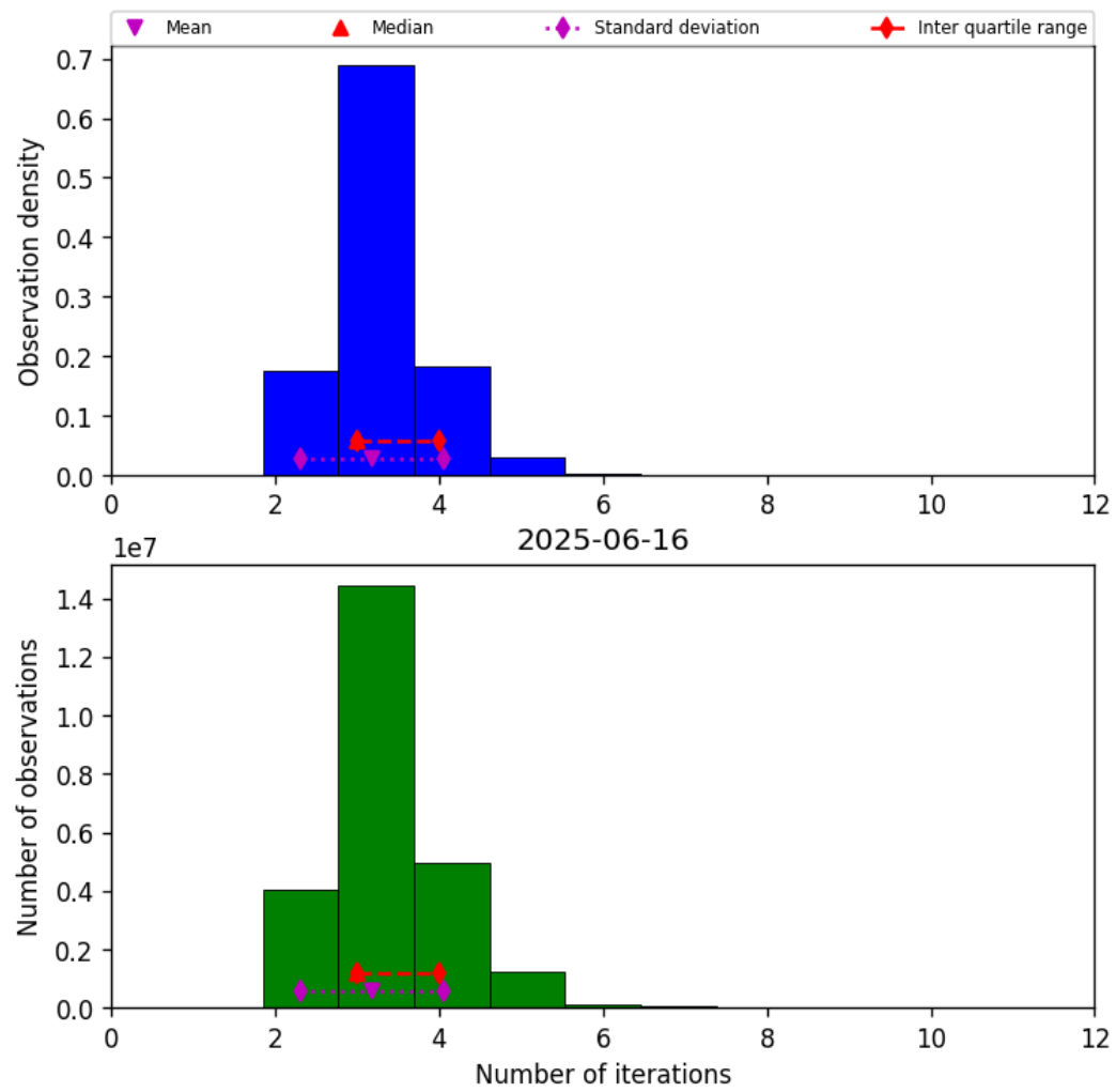
Figure 39: Histogram of “Number of iterations” for 2025-06-16 to 2025-06-17
