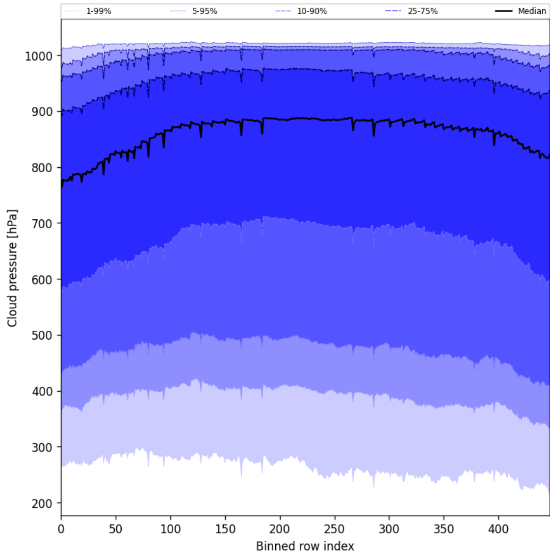
Figure 47: Along track statistics of “Cloud pressure” for 2025-06-16 to 2025-06-17
