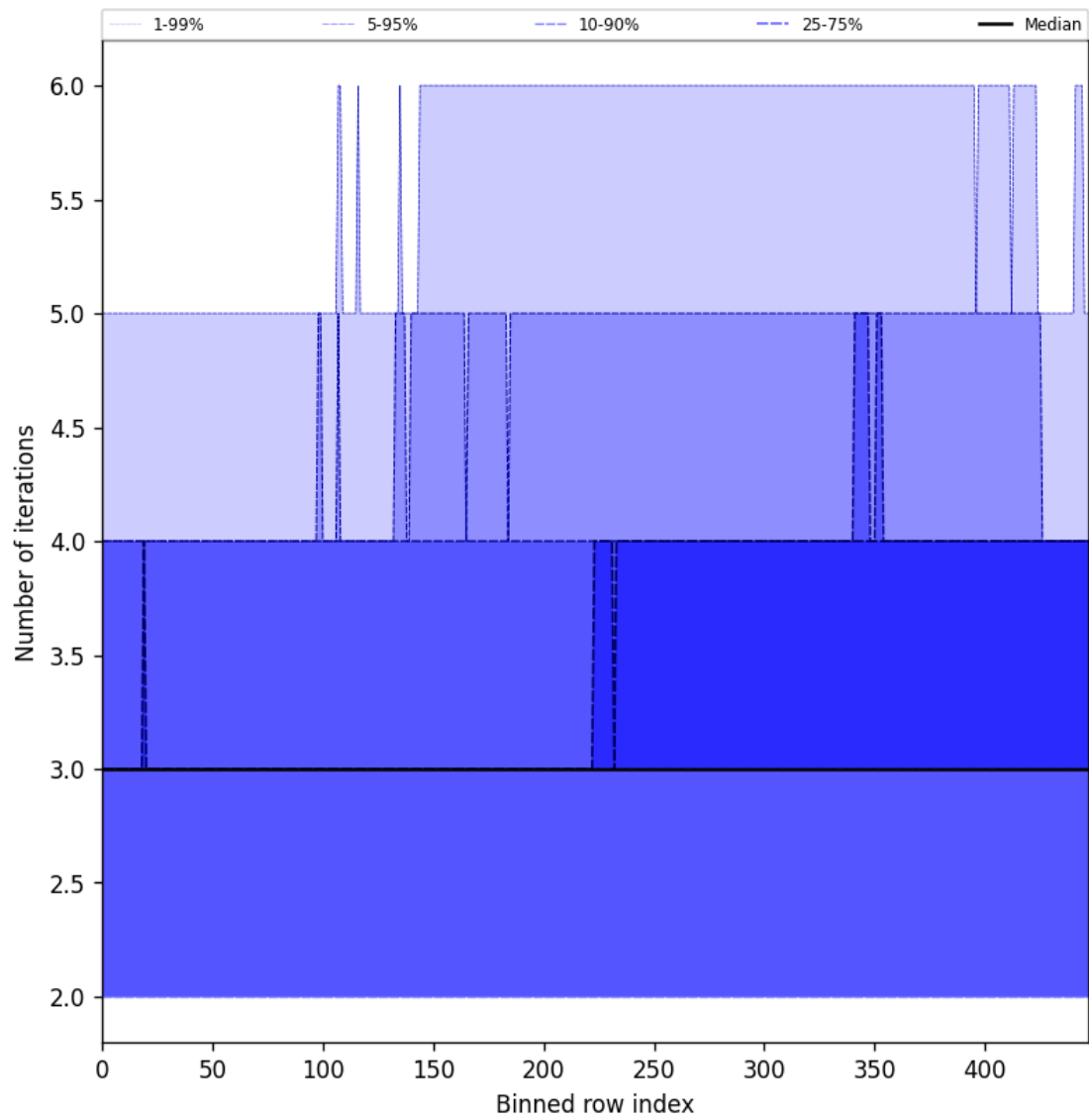
Figure 56: Along track statistics of “Number of iterations” for 2025-06-16 to 2025-06-17
