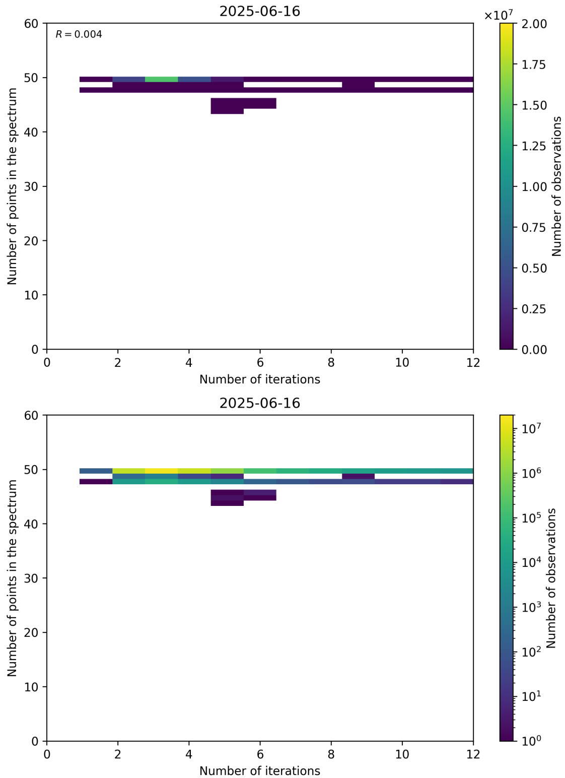
Figure 99: Scatter density plot of “Number of iterations” against “Number of points in the spectrum” for 2025-06-16 to 2025-06-17.
