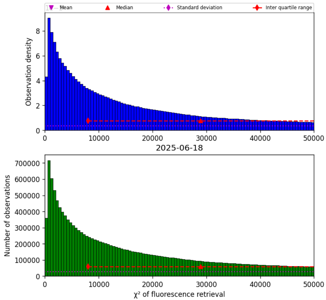
Figure 42: Histogram of “ \chi^2 of fluorescence retrieval” for 2025-06-17 to 2025-06-19
