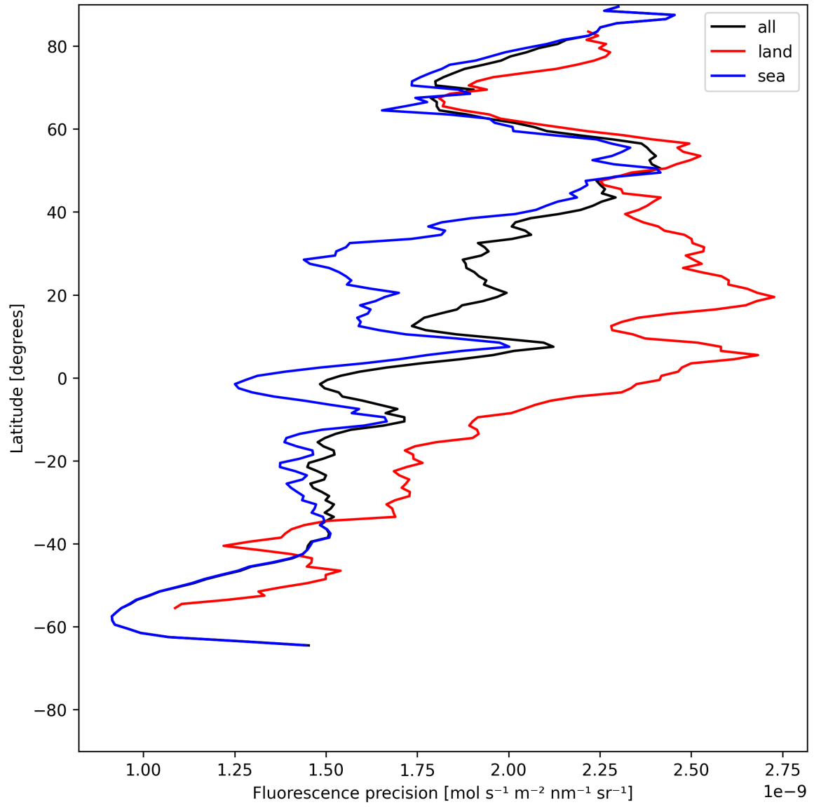
Figure 24: Zonal average of “Fluorescence precision” for 2025-06-17 to 2025-06-19.
