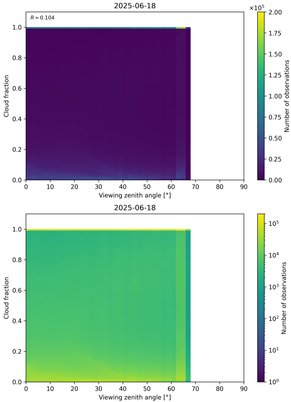
Figure 120: Scatter density plot of “Viewing zenith angle” against “Cloud fraction” for 2025-06-17 to 2025-06-19.
