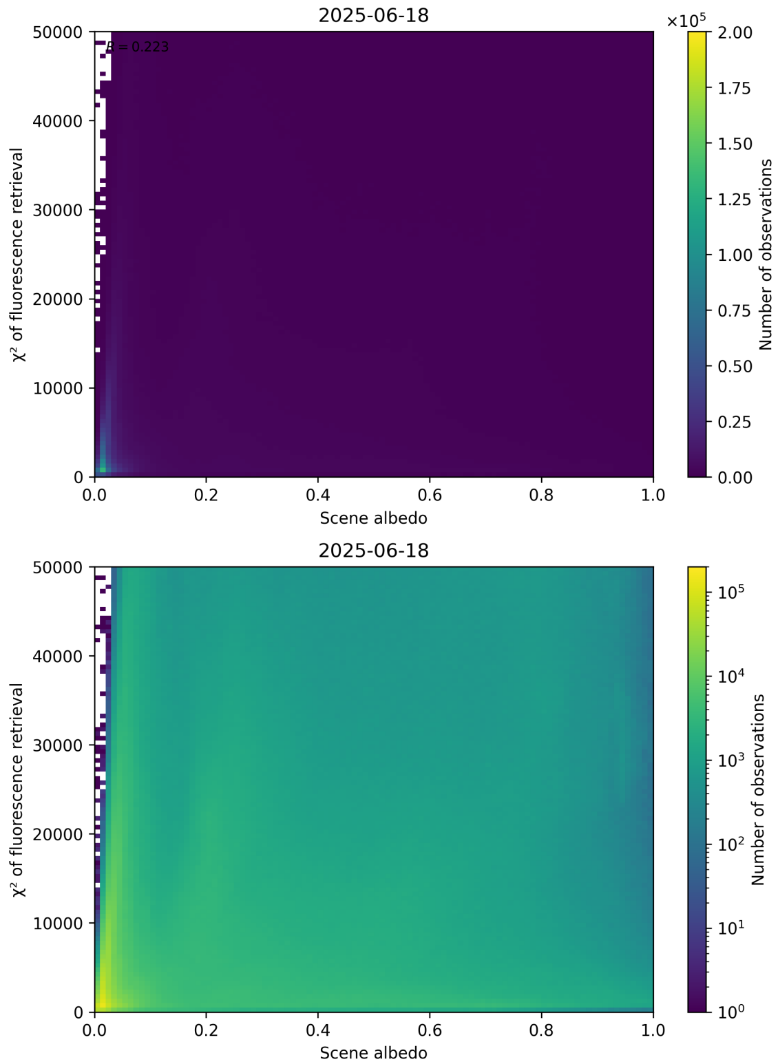
Figure 103: Scatter density plot of “Scene albedo” against “ \chi^2 of fluorescence retrieval” for 2025-06-17 to 2025-06-19.
