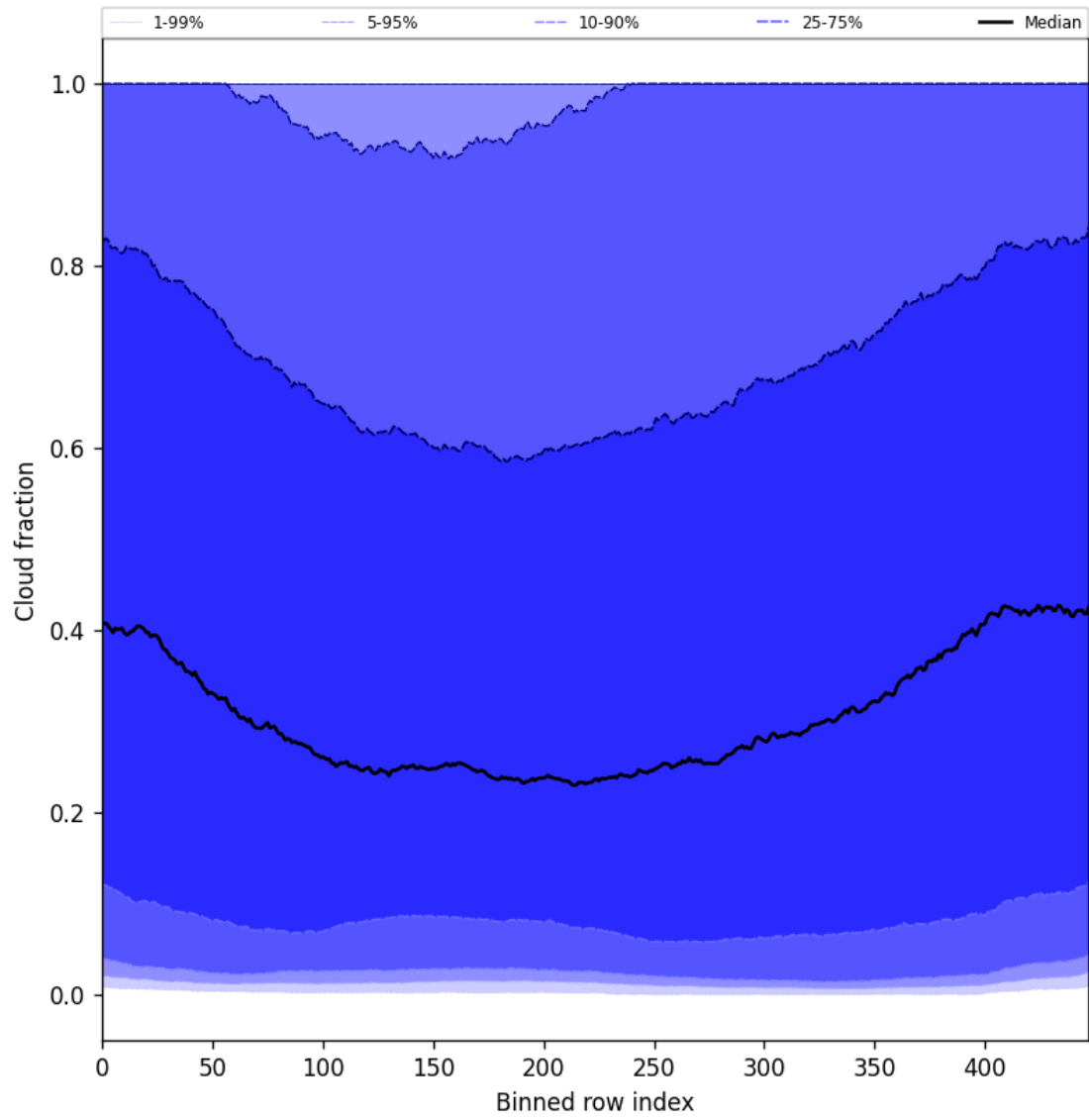
Figure 49: Along track statistics of “Cloud fraction” for 2025-06-17 to 2025-06-19
