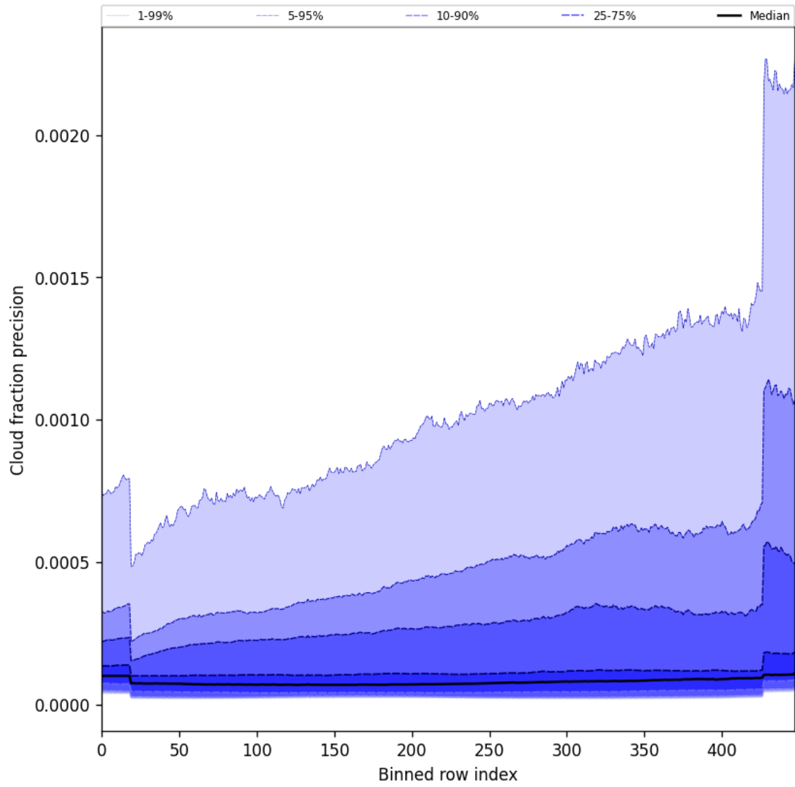
Figure 50: Along track statistics of “Cloud fraction precision” for 2025-06-17 to 2025-06-19
