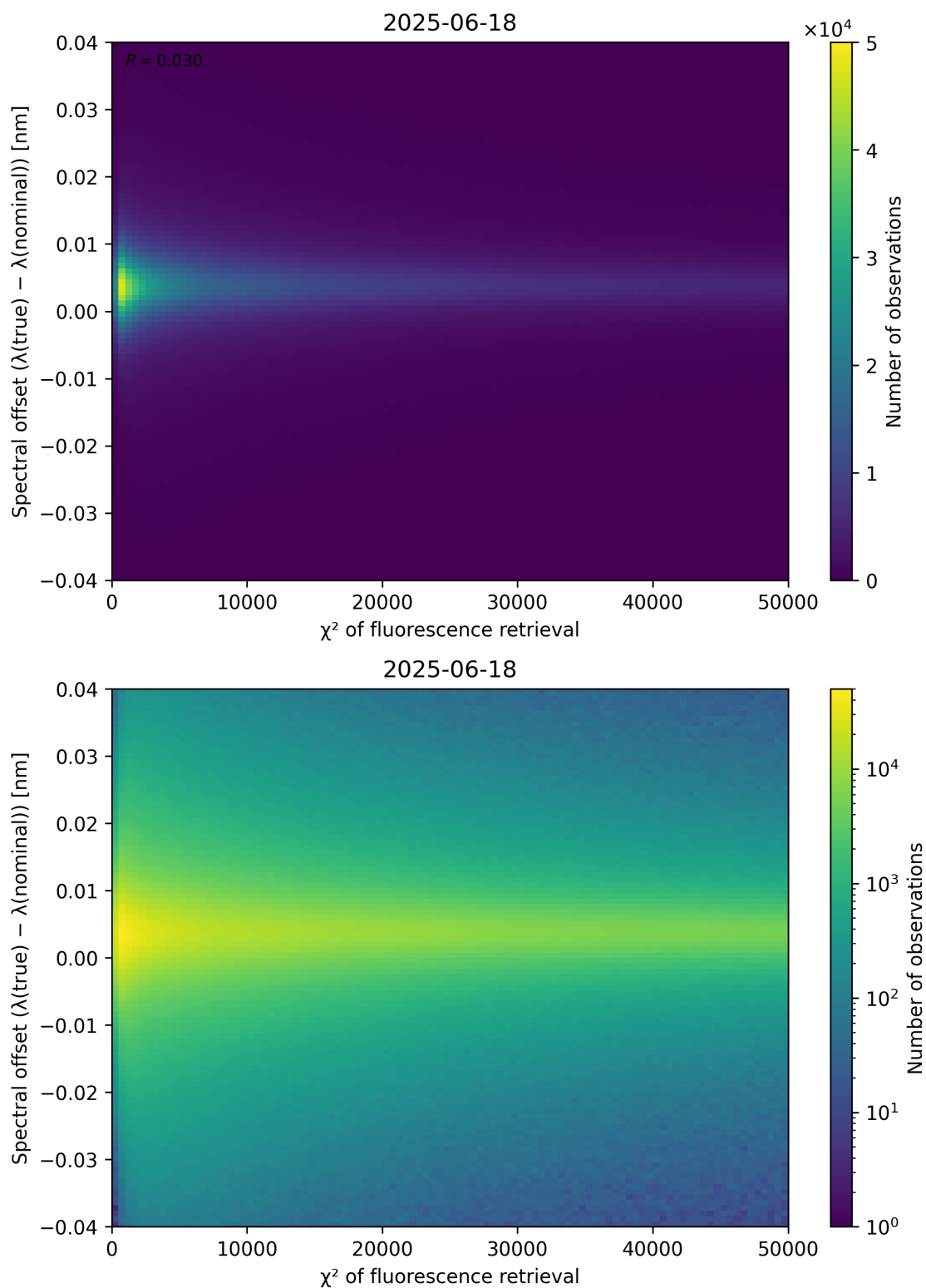
Figure 69: Scatter density plot of “ \chi^2 of fluorescence retrieval” against “Spectral offset ( \lambda_{\text{true}} - \lambda_{\text{nominal}} )” for 2025-06-17 to 2025-06-19.
