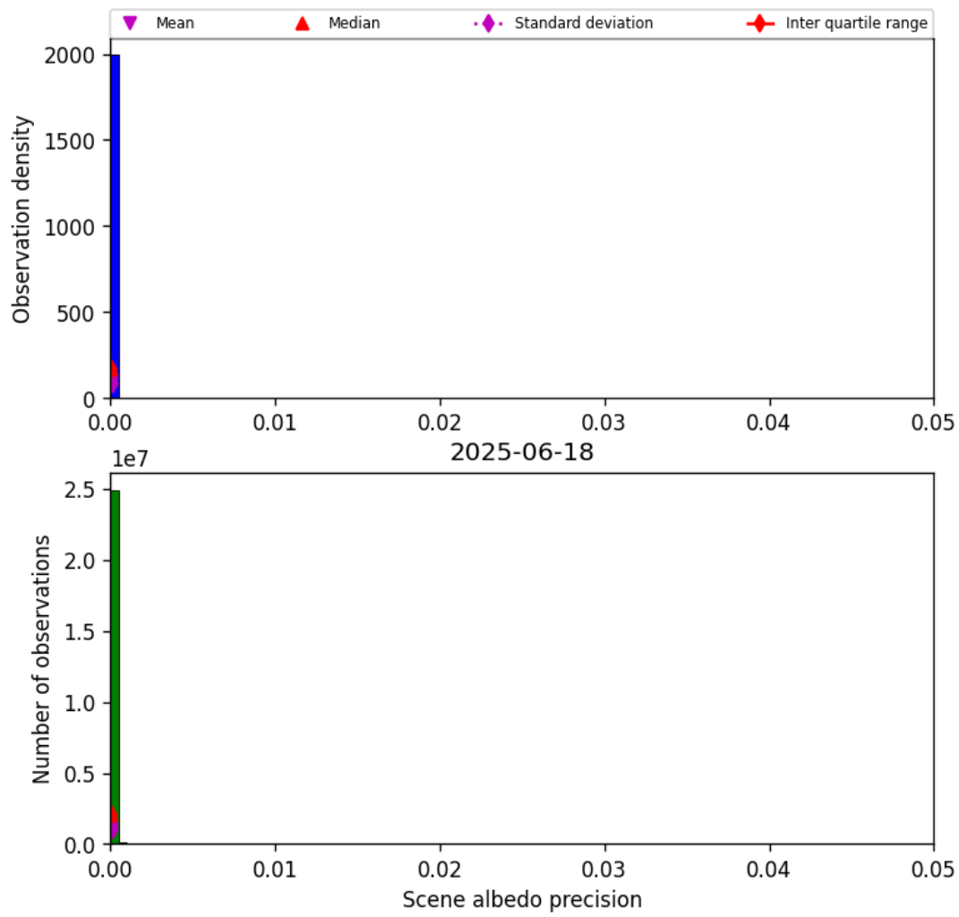
Figure 35: Histogram of “Scene albedo precision” for 2025-06-17 to 2025-06-19
