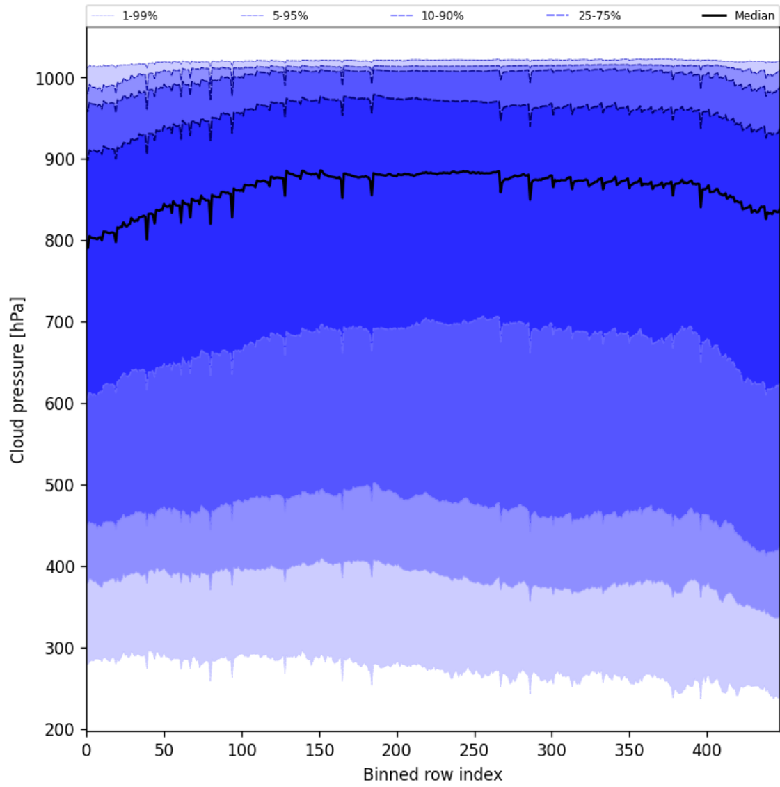
Figure 47: Along track statistics of “Cloud pressure” for 2025-06-17 to 2025-06-19
