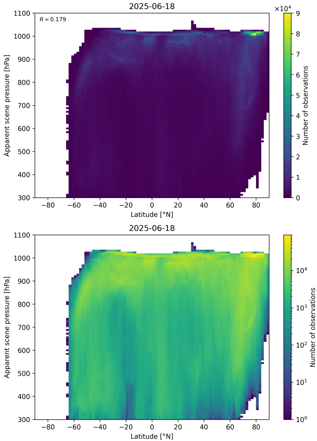
Figure 88: Scatter density plot of “Latitude” against “Apparent scene pressure” for 2025-06-17 to 2025-06-19.
