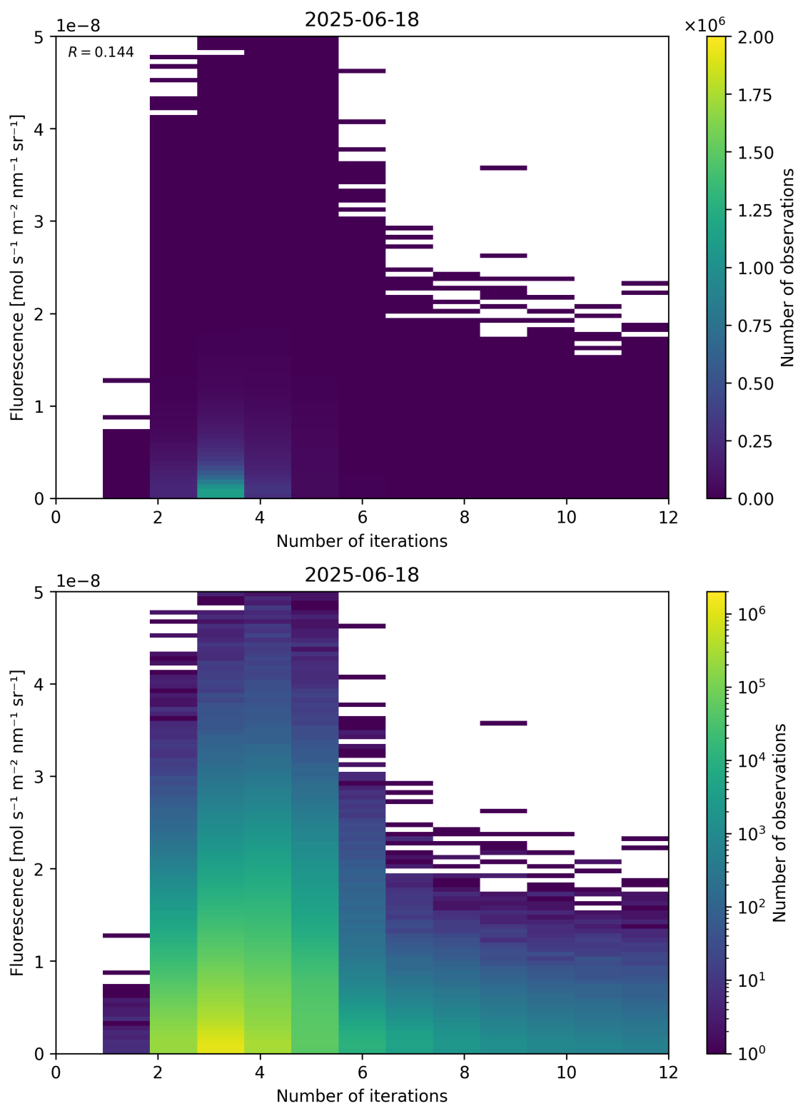
Figure 98: Scatter density plot of “Number of iterations” against “Fluorescence” for 2025-06-17 to 2025-06-19.
