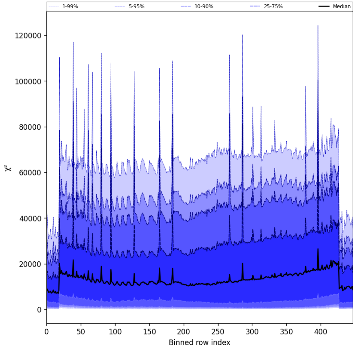
Figure 55: Along track statistics of “ \chi^2 ” for 2025-06-17 to 2025-06-19
