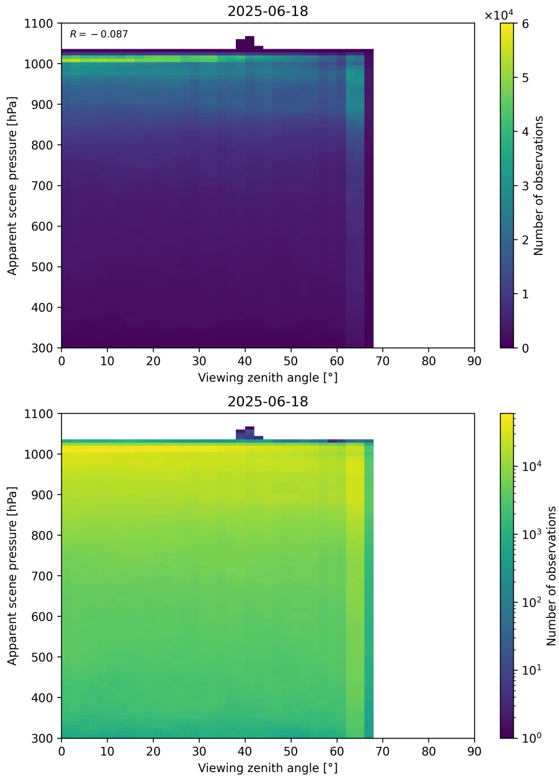
Figure 118: Scatter density plot of “Viewing zenith angle” against “Apparent scene pressure” for 2025-06-17 to 2025-06-19.
