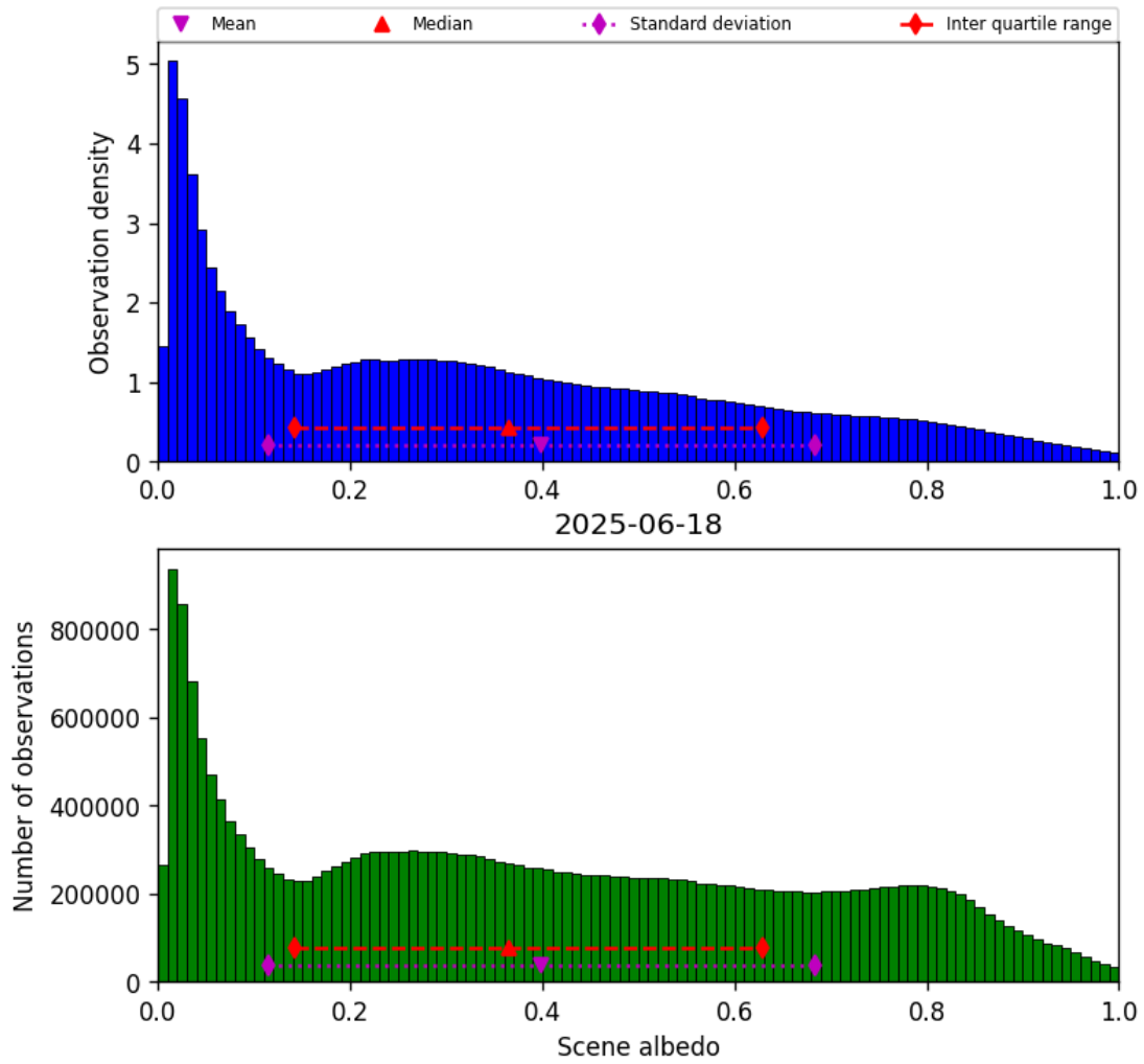
Figure 34: Histogram of “Scene albedo” for 2025-06-17 to 2025-06-19
