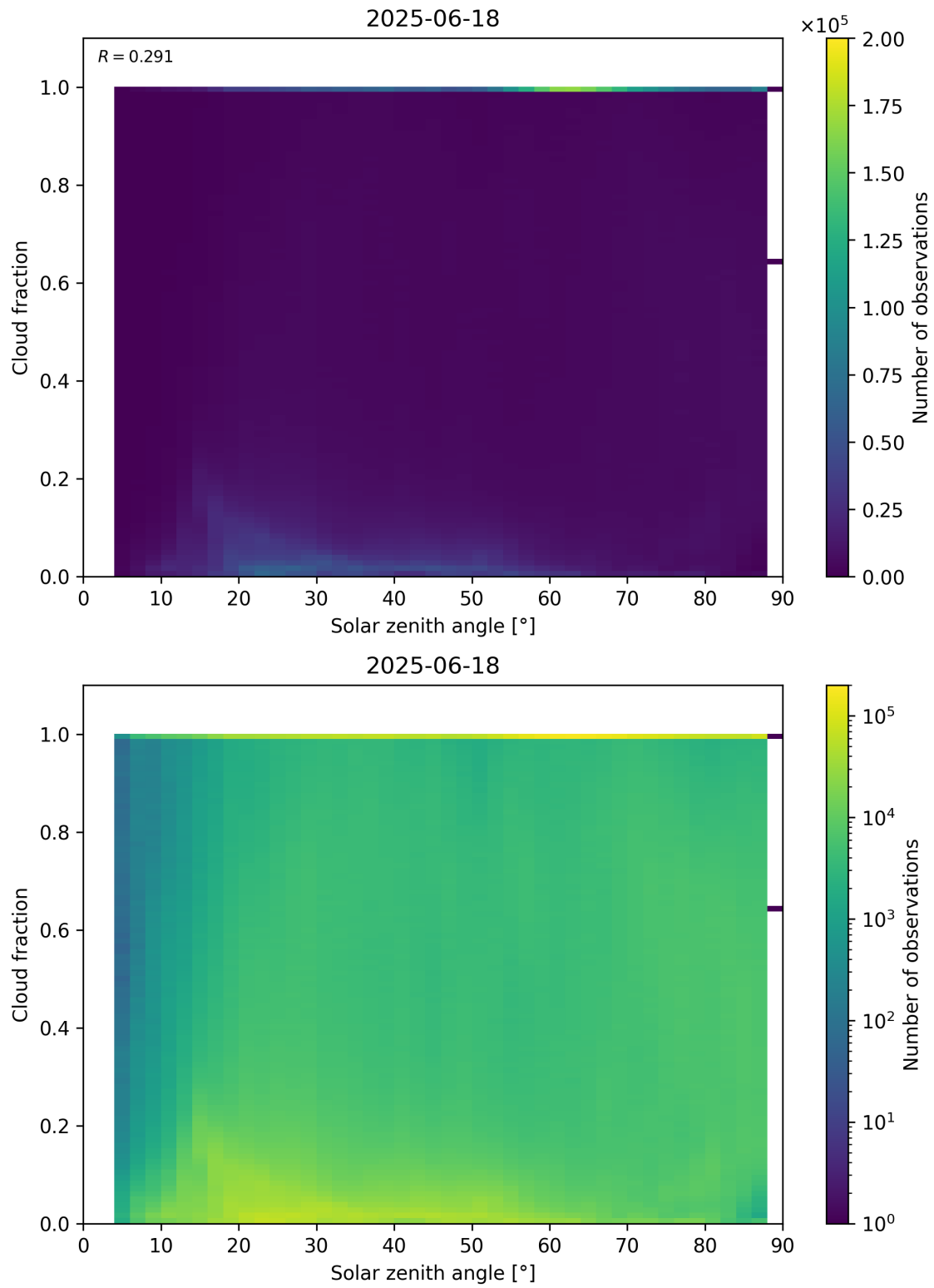
Figure 110: Scatter density plot of “Solar zenith angle” against “Cloud fraction” for 2025-06-17 to 2025-06-19.
