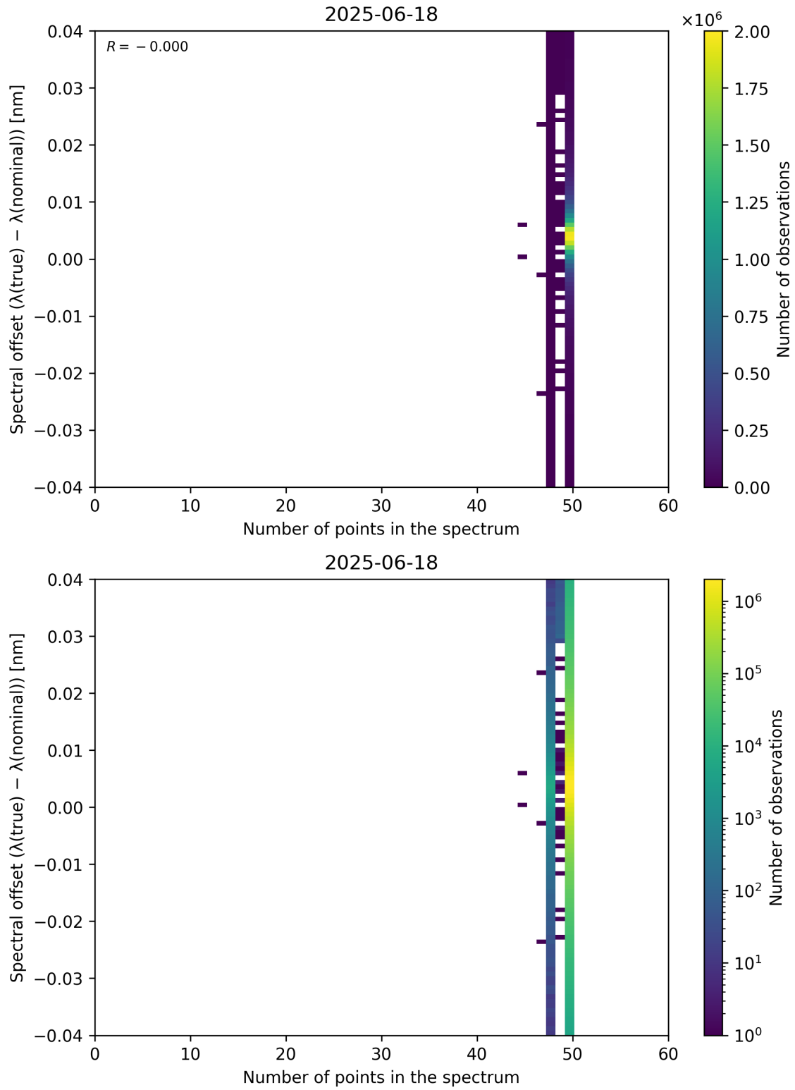
Figure 101: Scatter density plot of “Number of points in the spectrum” against “Spectral offset ( \lambda_{\text{true}} - \lambda_{\text{nominal}} )” for 2025-06-17 to 2025-06-19.
