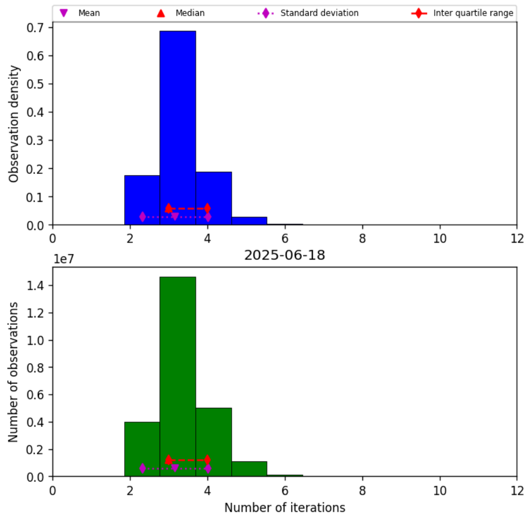
Figure 39: Histogram of “Number of iterations” for 2025-06-17 to 2025-06-19
