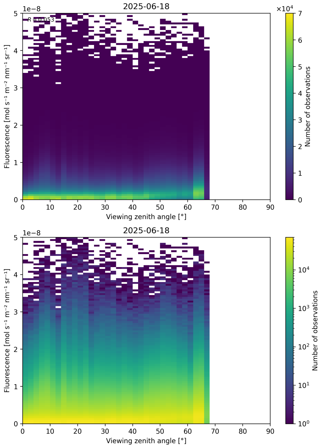
Figure 122: Scatter density plot of “Viewing zenith angle” against “Fluorescence” for 2025-06-17 to 2025-06-19.
