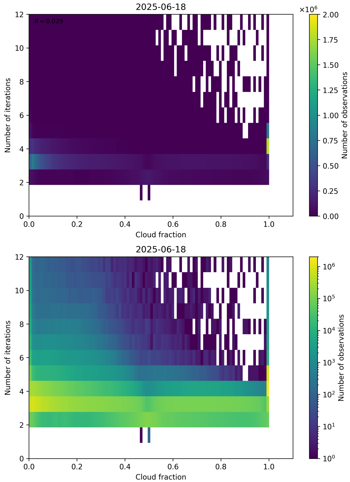
Figure 73: Scatter density plot of “Cloud fraction” against “Number of iterations” for 2025-06-17 to 2025-06-19.
