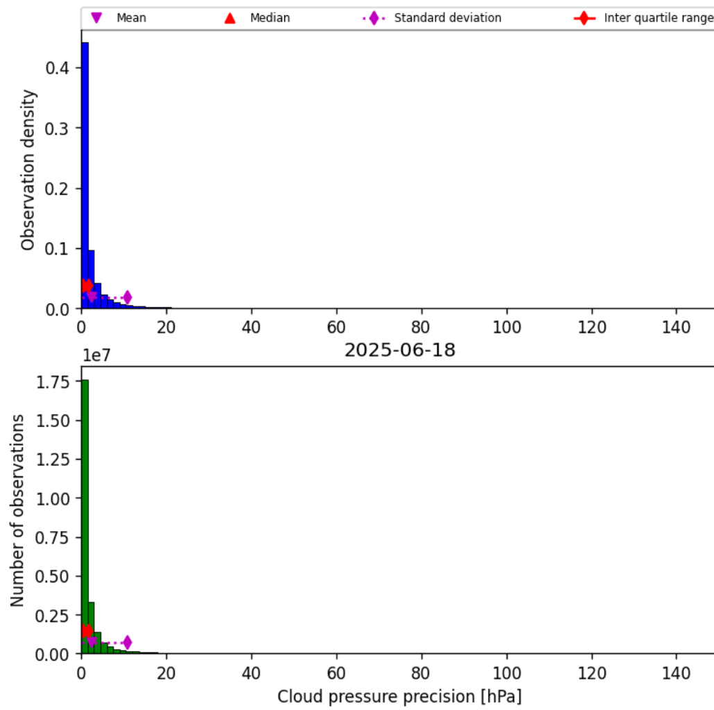
Figure 31: Histogram of “Cloud pressure precision” for 2025-06-17 to 2025-06-19
