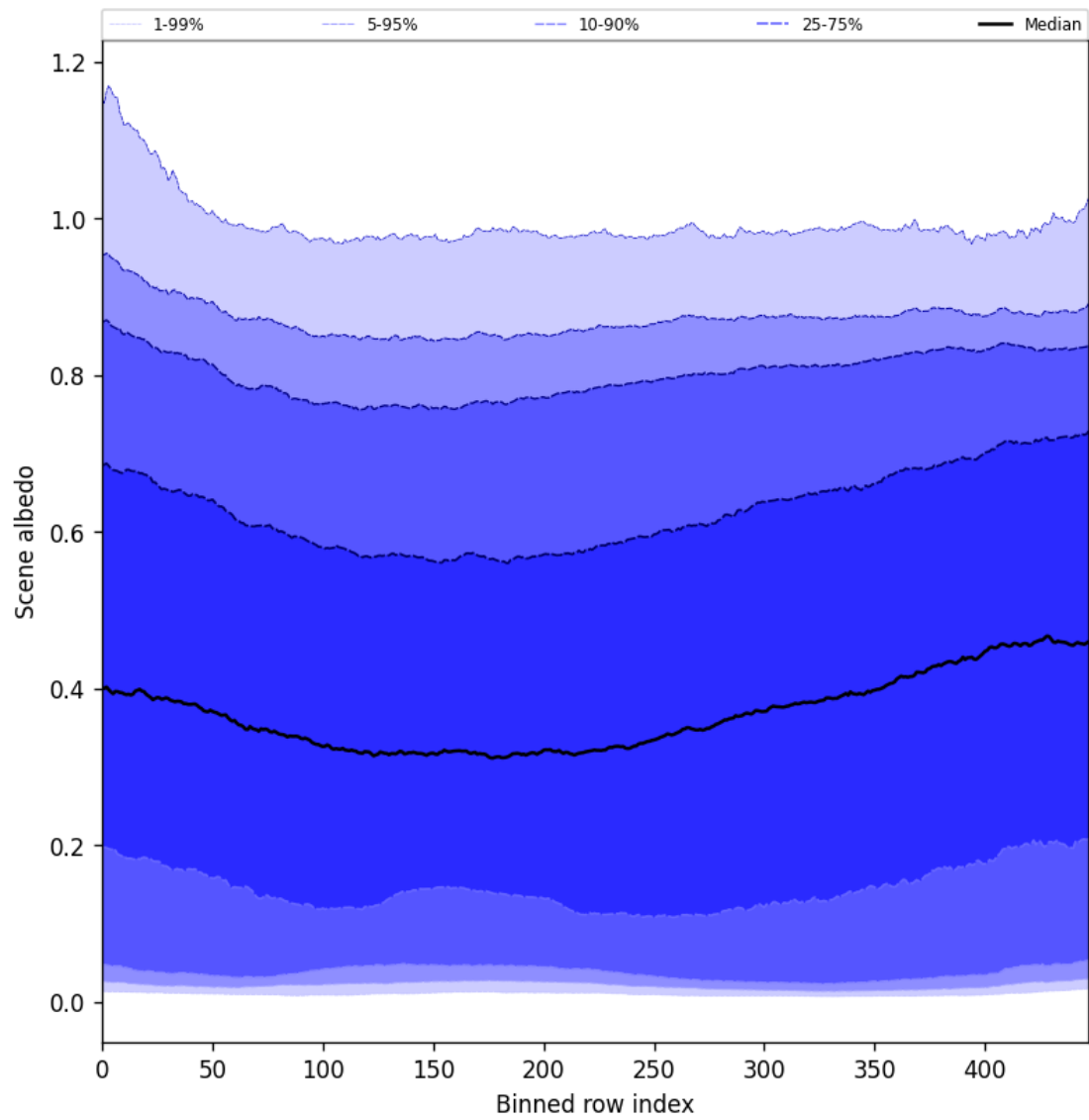
Figure 51: Along track statistics of “Scene albedo” for 2025-06-17 to 2025-06-19
