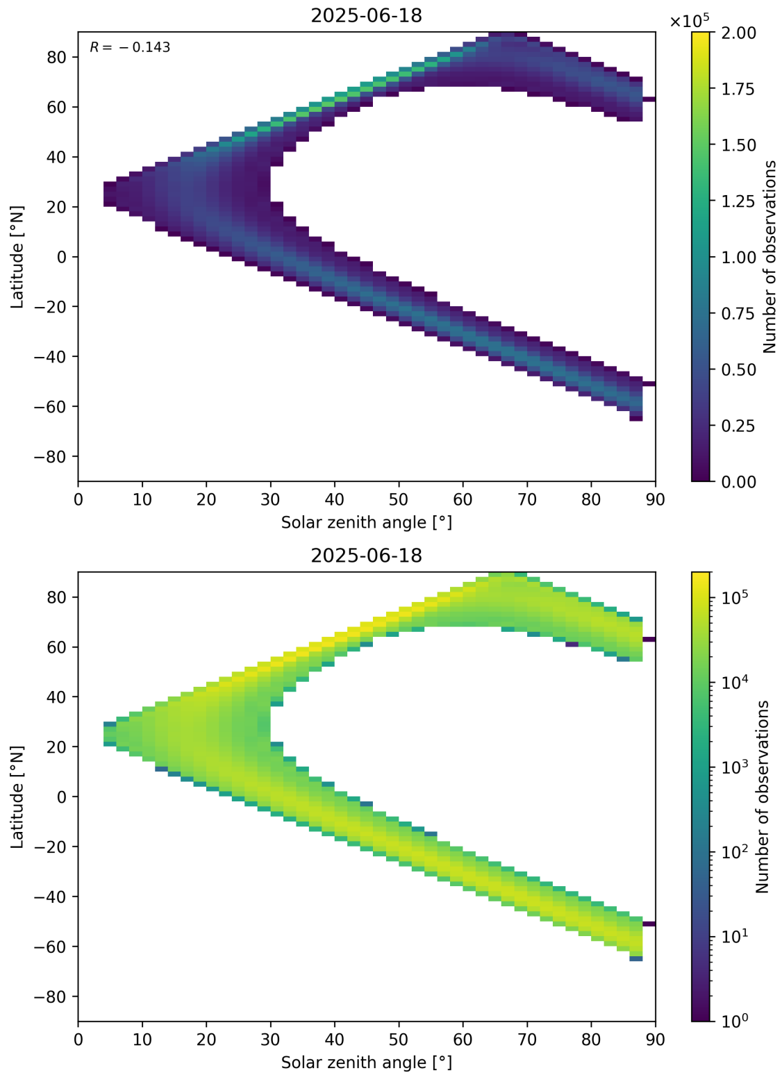
Figure 113: Scatter density plot of “Solar zenith angle” against “Latitude” for 2025-06-17 to 2025-06-19.
