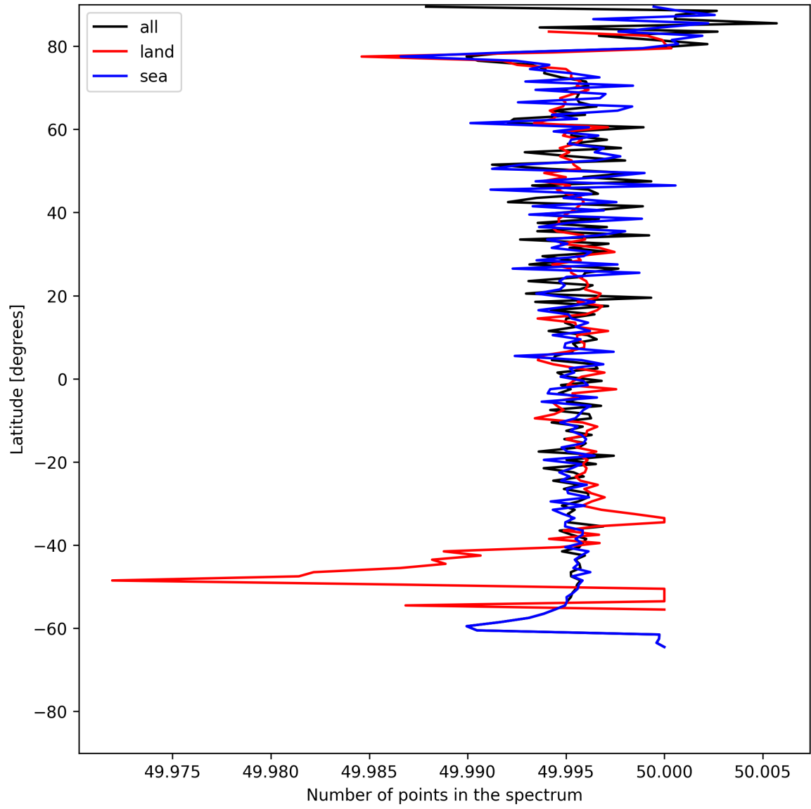
Figure 27: Zonal average of “Number of points in the spectrum” for 2025-06-17 to 2025-06-19.
