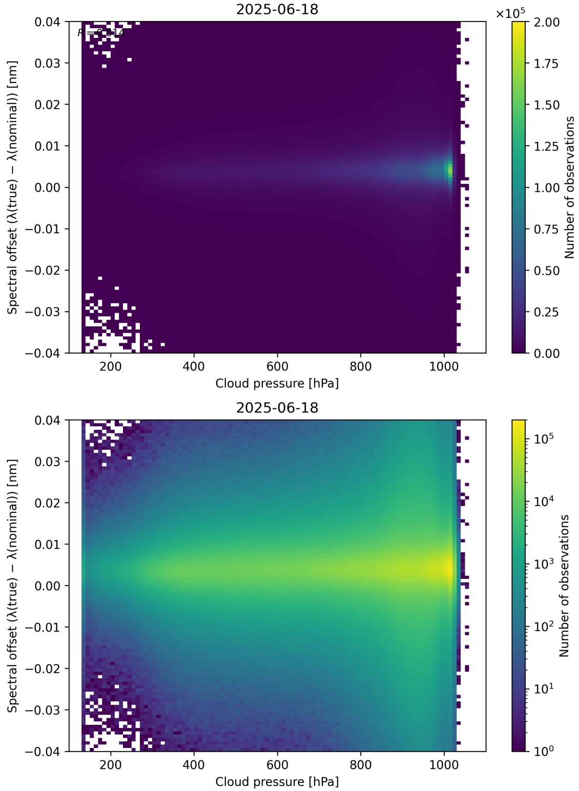
Figure 84: Scatter density plot of “Cloud pressure” against “Spectral offset ( \lambda_{\text{true}} - \lambda_{\text{nominal}} )” for 2025-06-17 to 2025-06-19.
