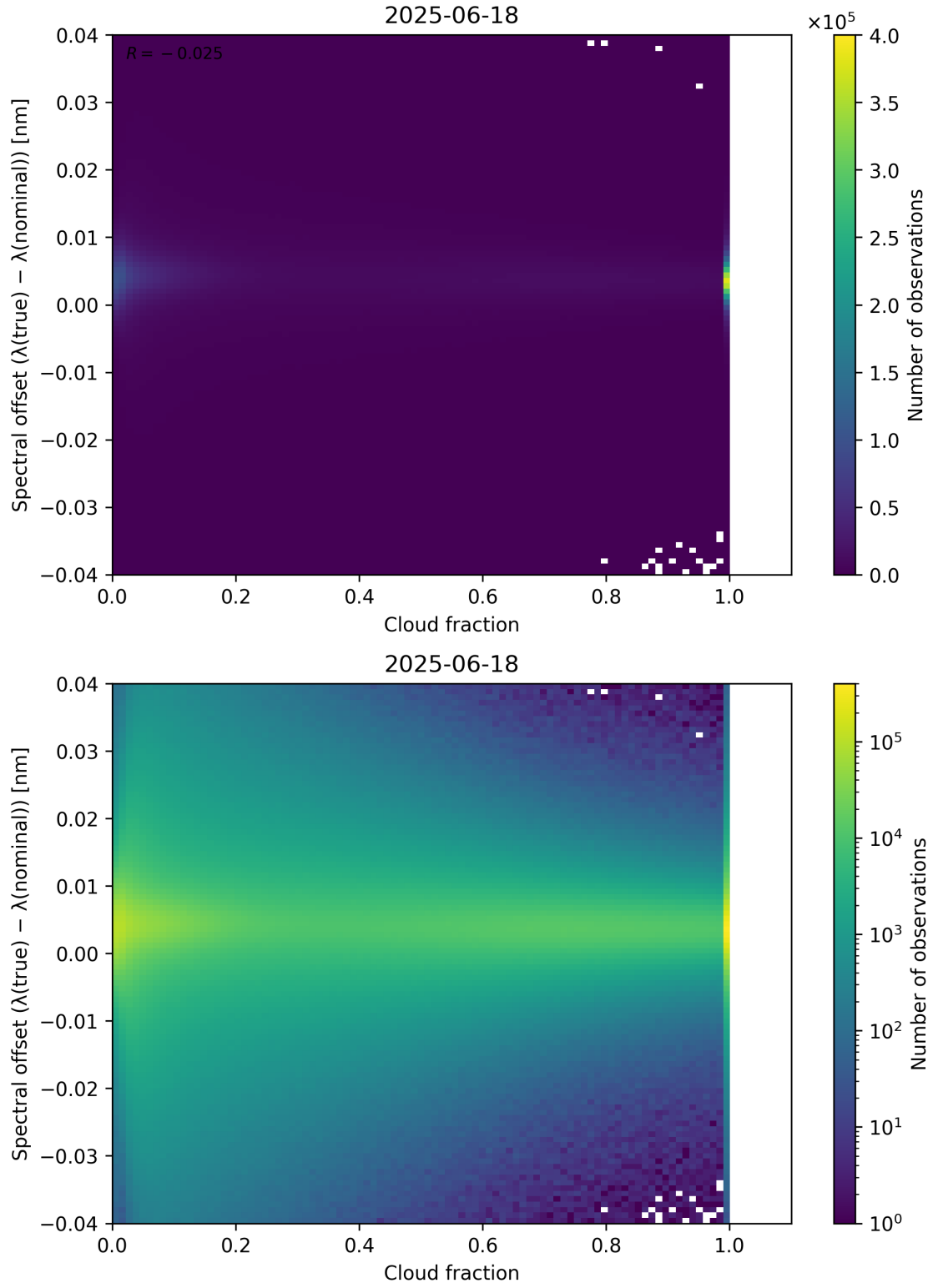
Figure 76: Scatter density plot of “Cloud fraction” against “Spectral offset ( \lambda_{\text{true}} - \lambda_{\text{nominal}} )” for 2025-06-17 to 2025-06-19.
