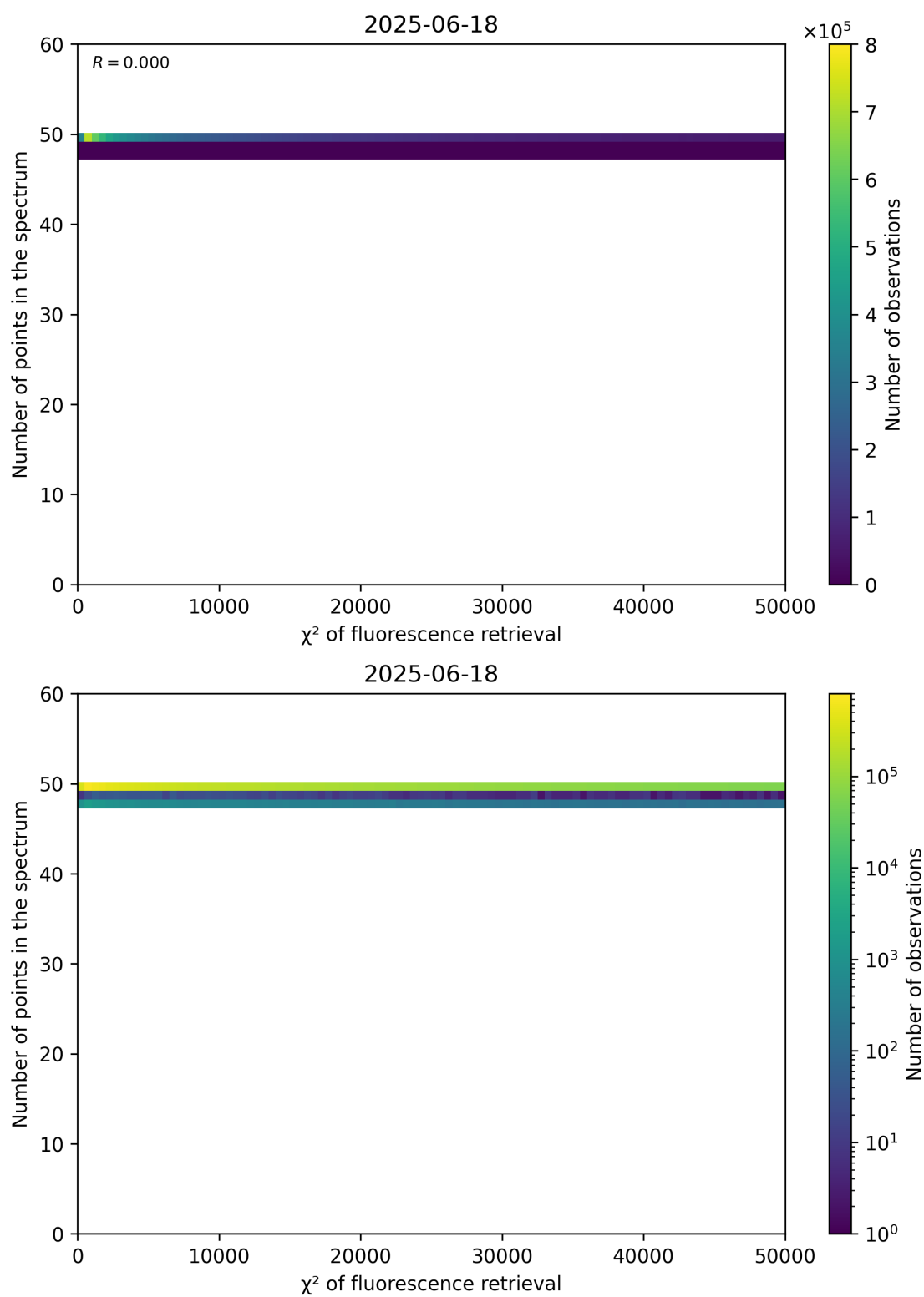
Figure 68: Scatter density plot of " \chi^2 of fluorescence retrieval" against "Number of points in the spectrum" for 2025-06-17 to 2025-06-19.
