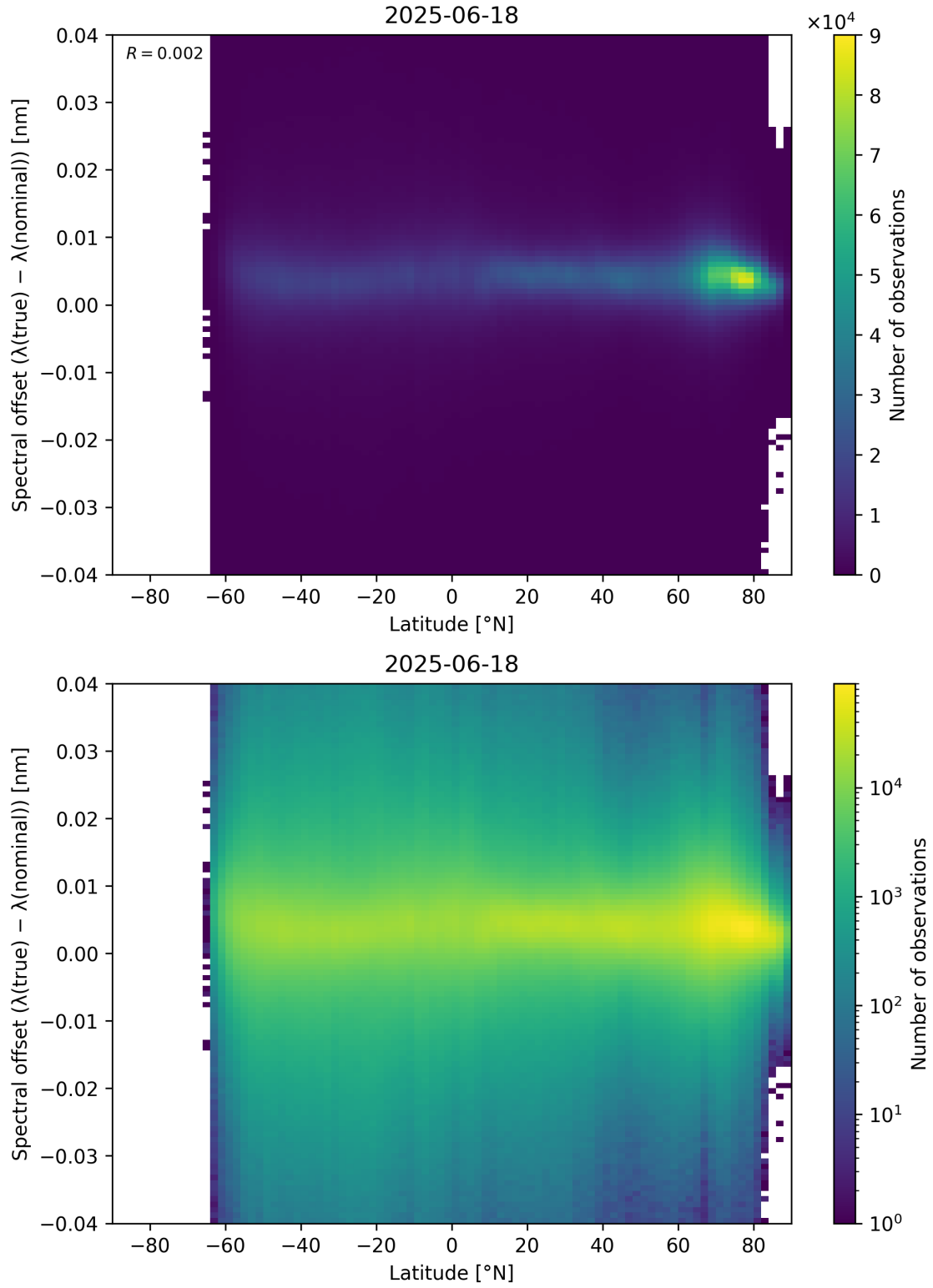
Figure 96: Scatter density plot of “Latitude” against “Spectral offset ( \lambda_{\text{true}} - \lambda_{\text{nominal}} )” for 2025-06-17 to 2025-06-19.
