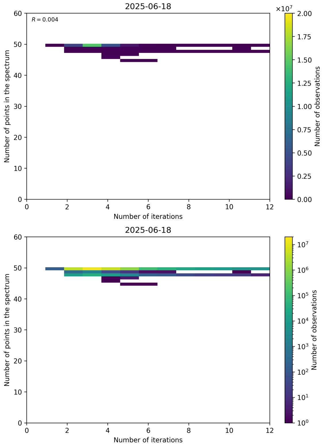
Figure 99: Scatter density plot of “Number of iterations” against “Number of points in the spectrum” for 2025-06-17 to 2025-06-19.
