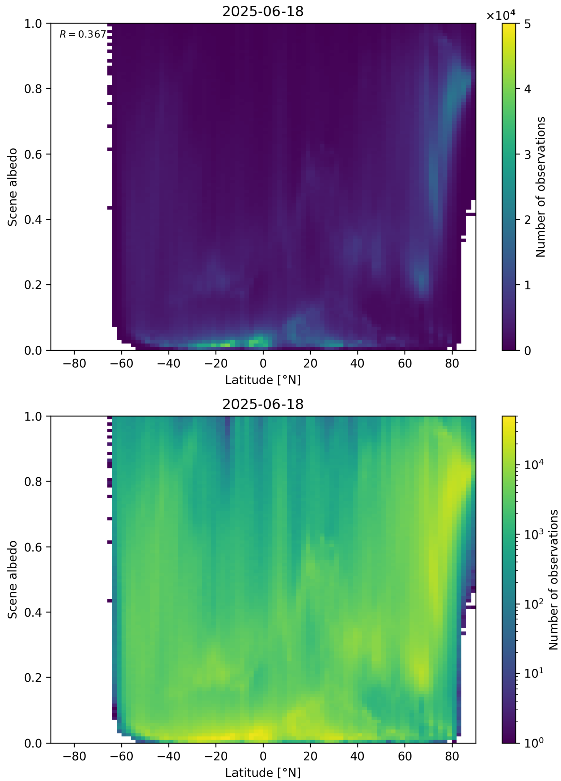
Figure 95: Scatter density plot of “Latitude” against “Scene albedo” for 2025-06-17 to 2025-06-19.
