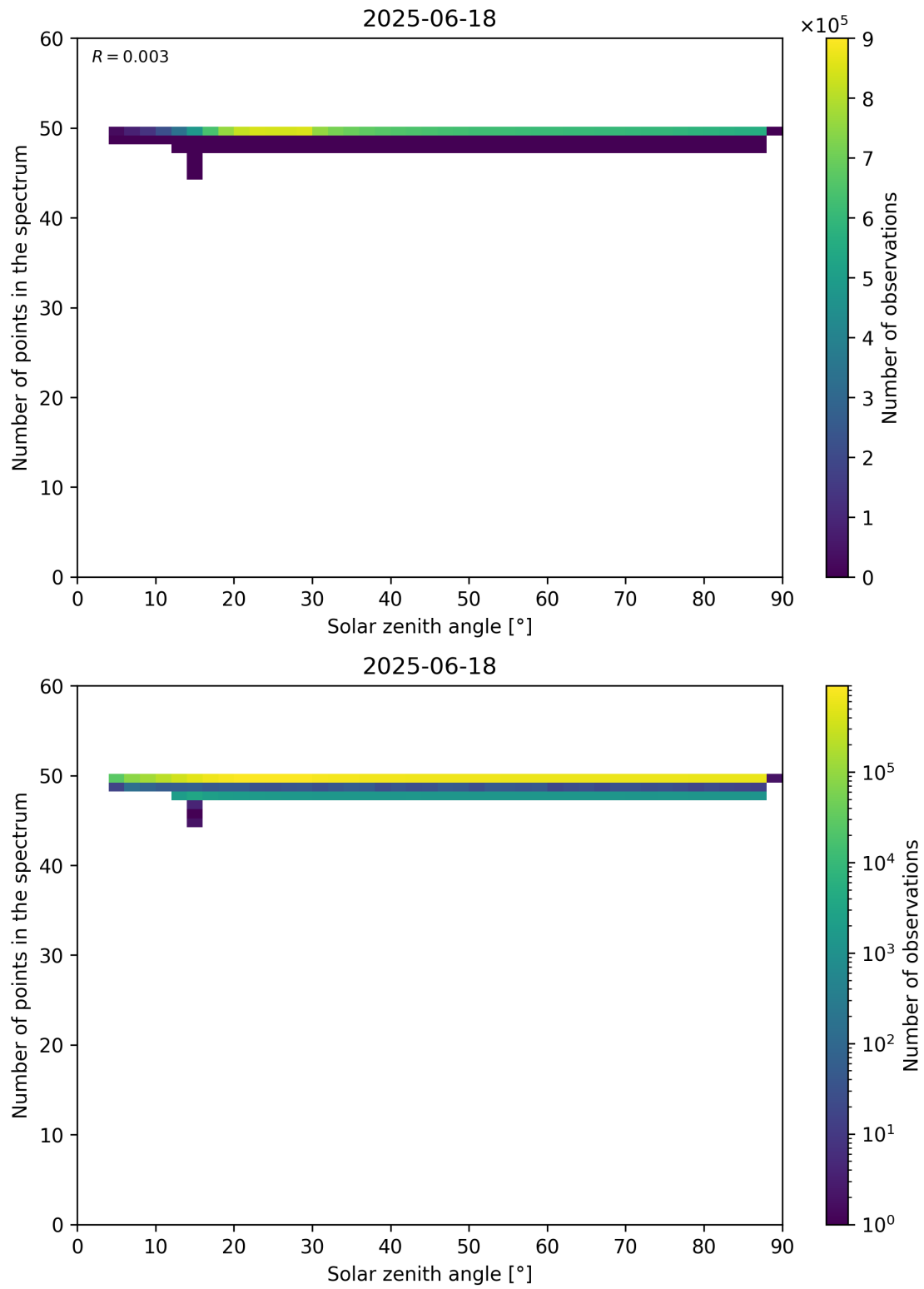
Figure 115: Scatter density plot of “Solar zenith angle” against “Number of points in the spectrum” for 2025-06-17 to 2025-06-19.
