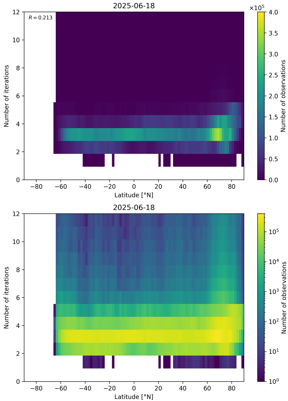
Figure 93: Scatter density plot of “Latitude” against “Number of iterations” for 2025-06-17 to 2025-06-19.
