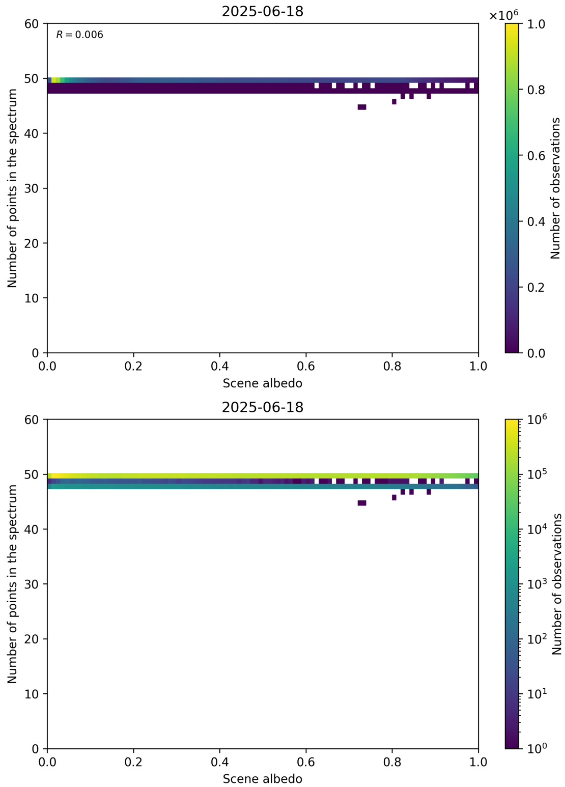
Figure 106: Scatter density plot of “Scene albedo” against “Number of points in the spectrum” for 2025-06-17 to 2025-06-19.
