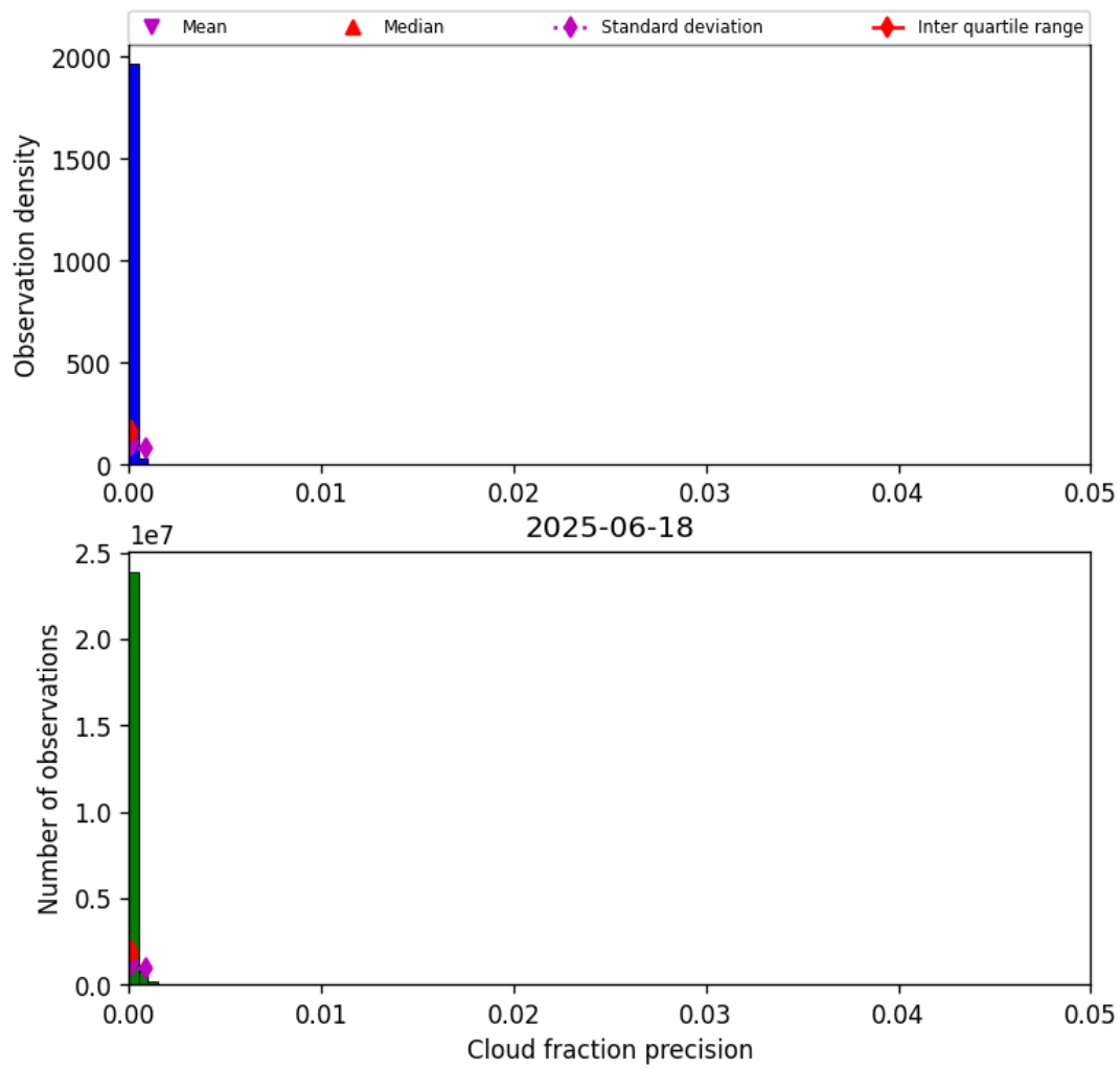
Figure 33: Histogram of “Cloud fraction precision” for 2025-06-17 to 2025-06-19
