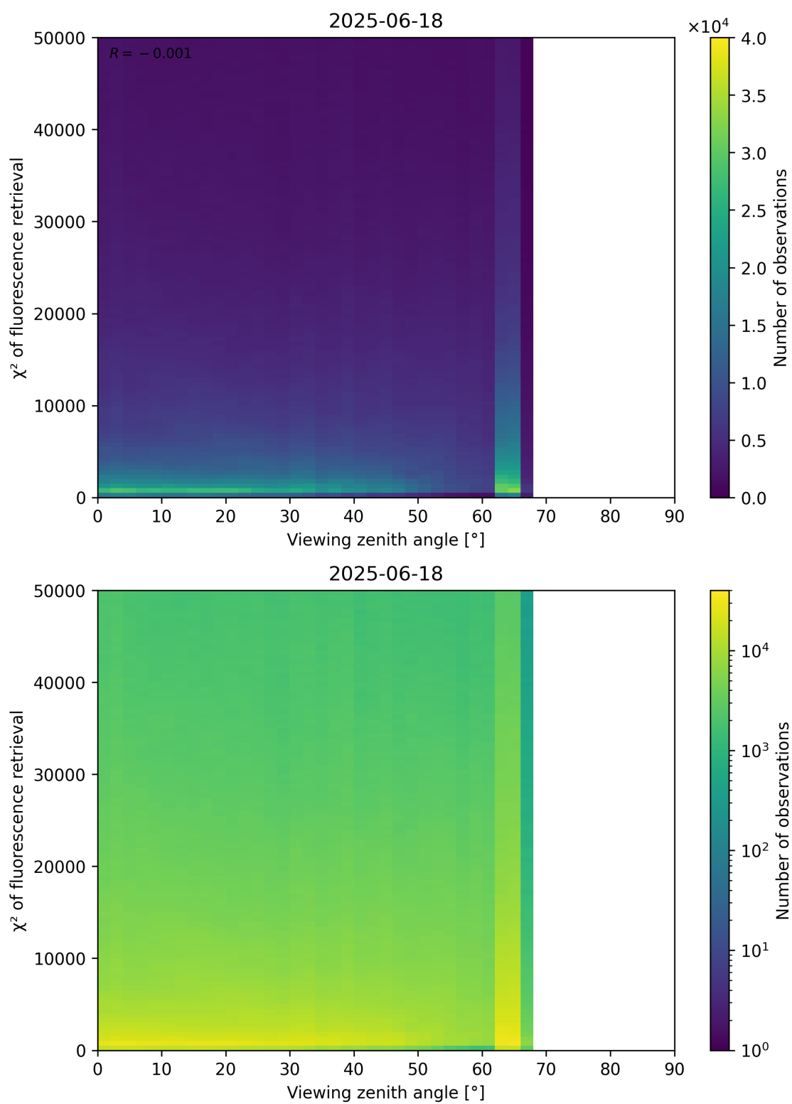
Figure 119: Scatter density plot of “Viewing zenith angle” against “ \chi^2 of fluorescence retrieval” for 2025-06-17 to 2025-06-19.
