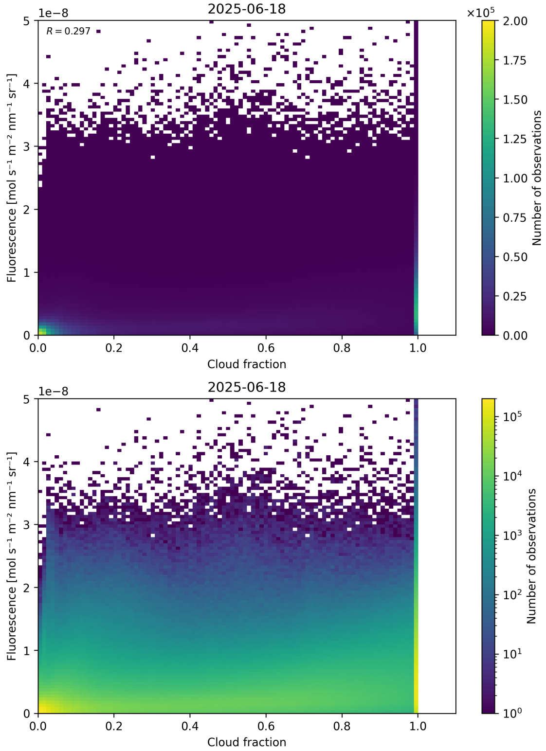
Figure 72: Scatter density plot of “Cloud fraction” against “Fluorescence” for 2025-06-17 to 2025-06-19.
