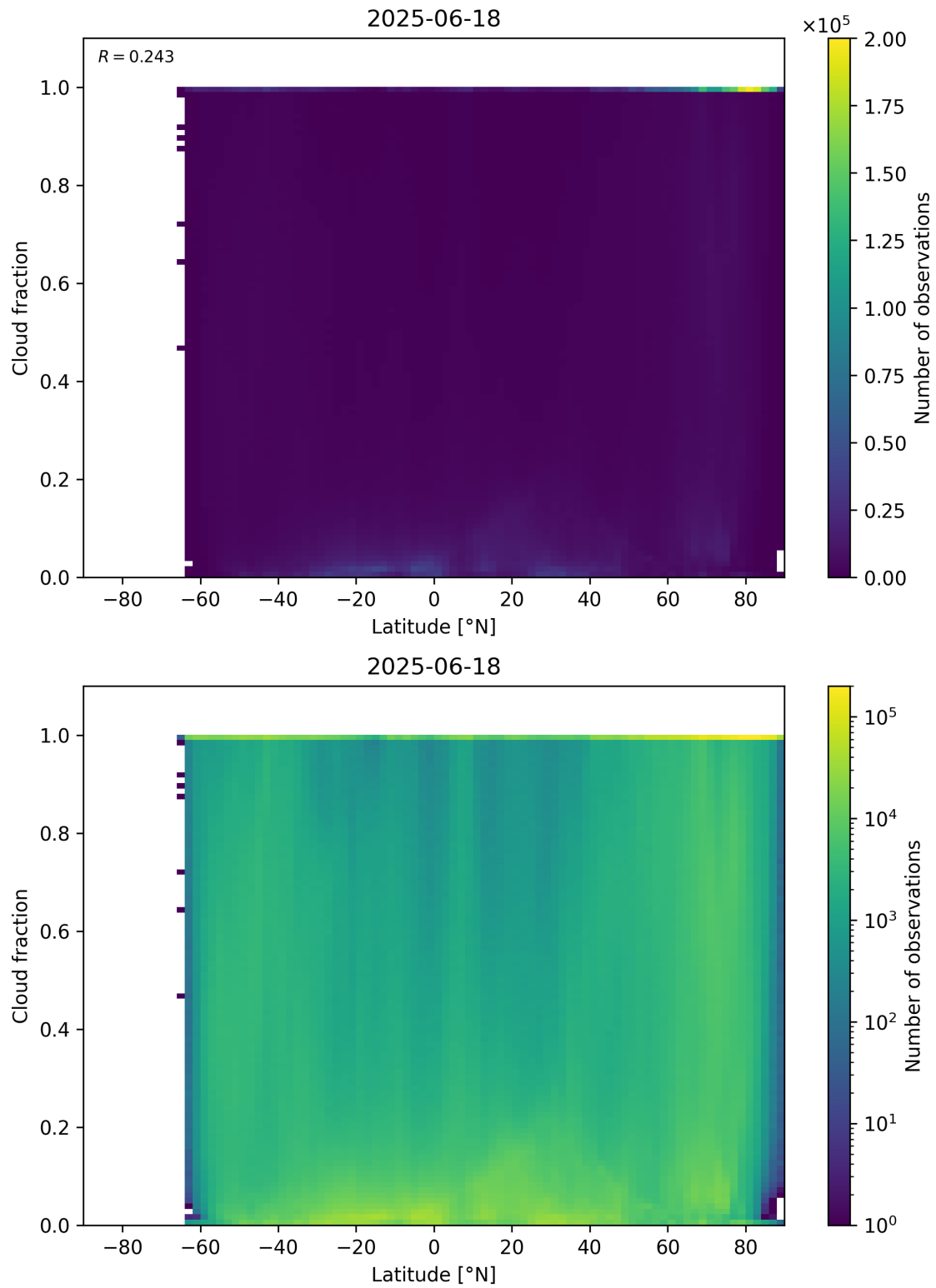
Figure 90: Scatter density plot of “Latitude” against “Cloud fraction” for 2025-06-17 to 2025-06-19.
