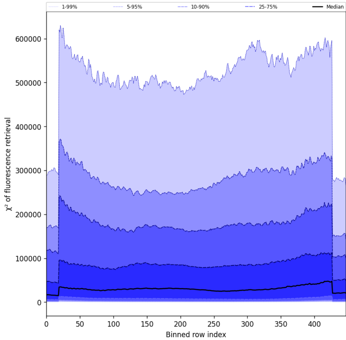
Figure 59: Along track statistics of “ \chi^2 of fluorescence retrieval” for 2025-06-17 to 2025-06-19
