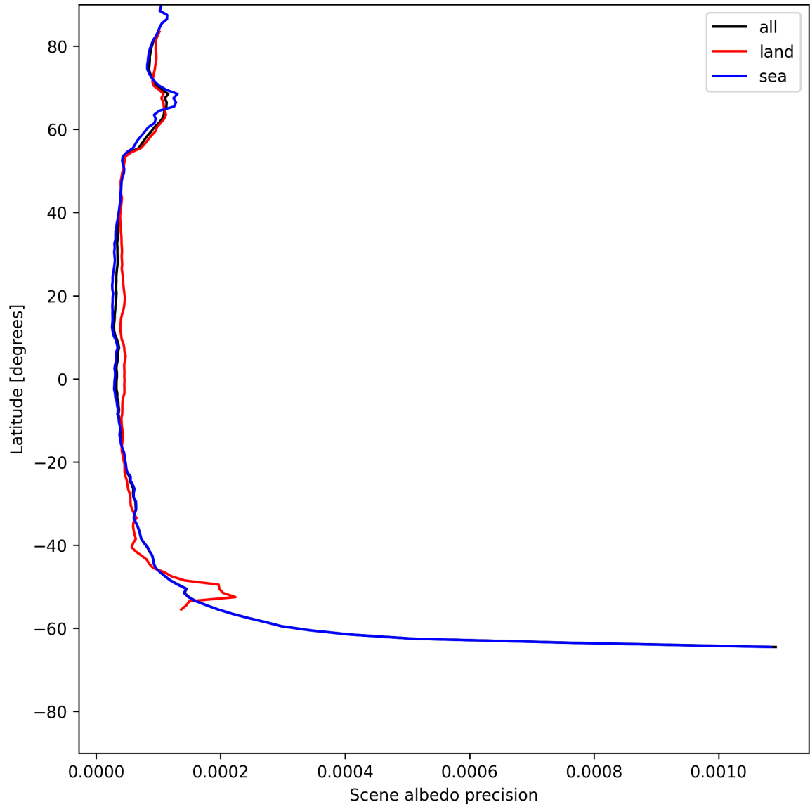
Figure 18: Zonal average of “Scene albedo precision” for 2025-06-17 to 2025-06-19.
