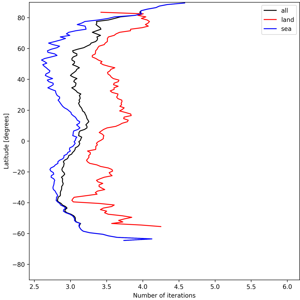
Figure 22: Zonal average of “Number of iterations” for 2025-06-17 to 2025-06-19.
