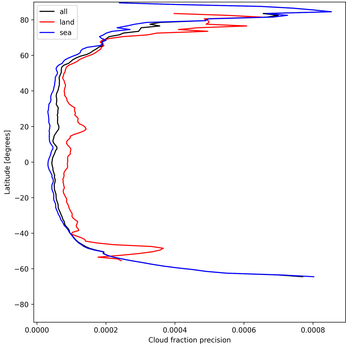
Figure 16: Zonal average of “Cloud fraction precision” for 2025-06-17 to 2025-06-19.
