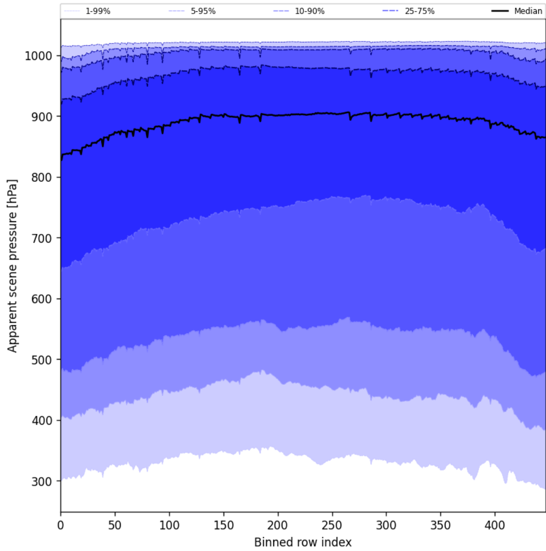
Figure 53: Along track statistics of “Apparent scene pressure” for 2025-06-17 to 2025-06-19
