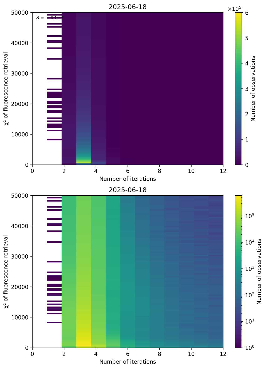
Figure 97: Scatter density plot of “Number of iterations” against “ \chi^2 of fluorescence retrieval” for 2025-06-17 to 2025-06-19.
