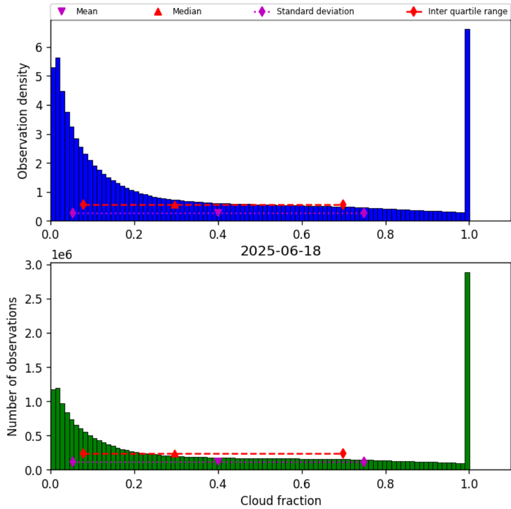
Figure 32: Histogram of “Cloud fraction” for 2025-06-17 to 2025-06-19
