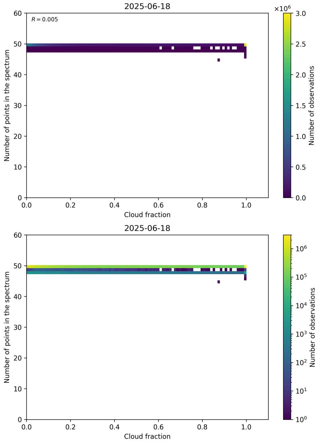
Figure 74: Scatter density plot of “Cloud fraction” against “Number of points in the spectrum” for 2025-06-17 to 2025-06-19.
