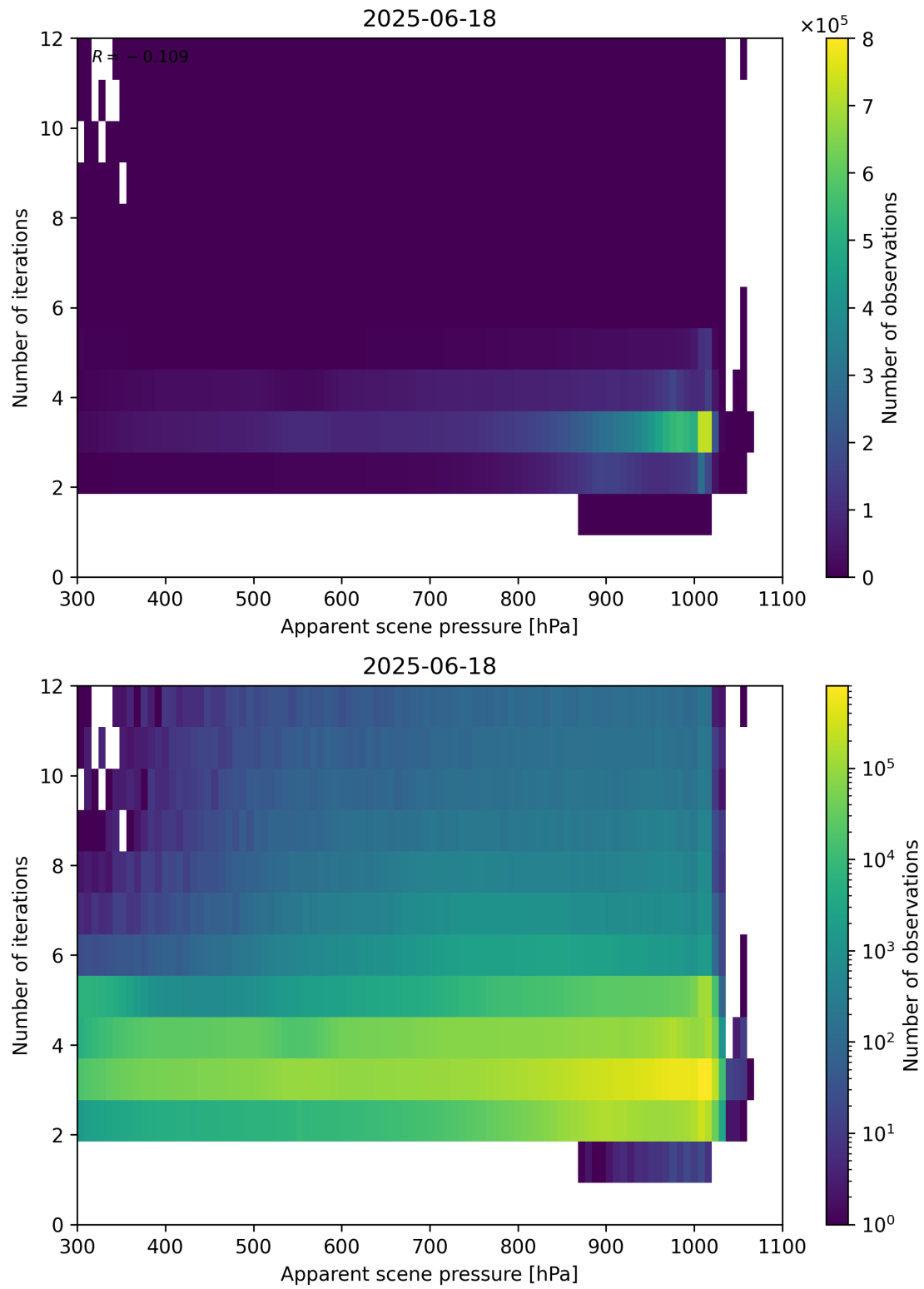
Figure 65: Scatter density plot of “Apparent scene pressure” against “Number of iterations” for 2025-06-17 to 2025-06-19.
