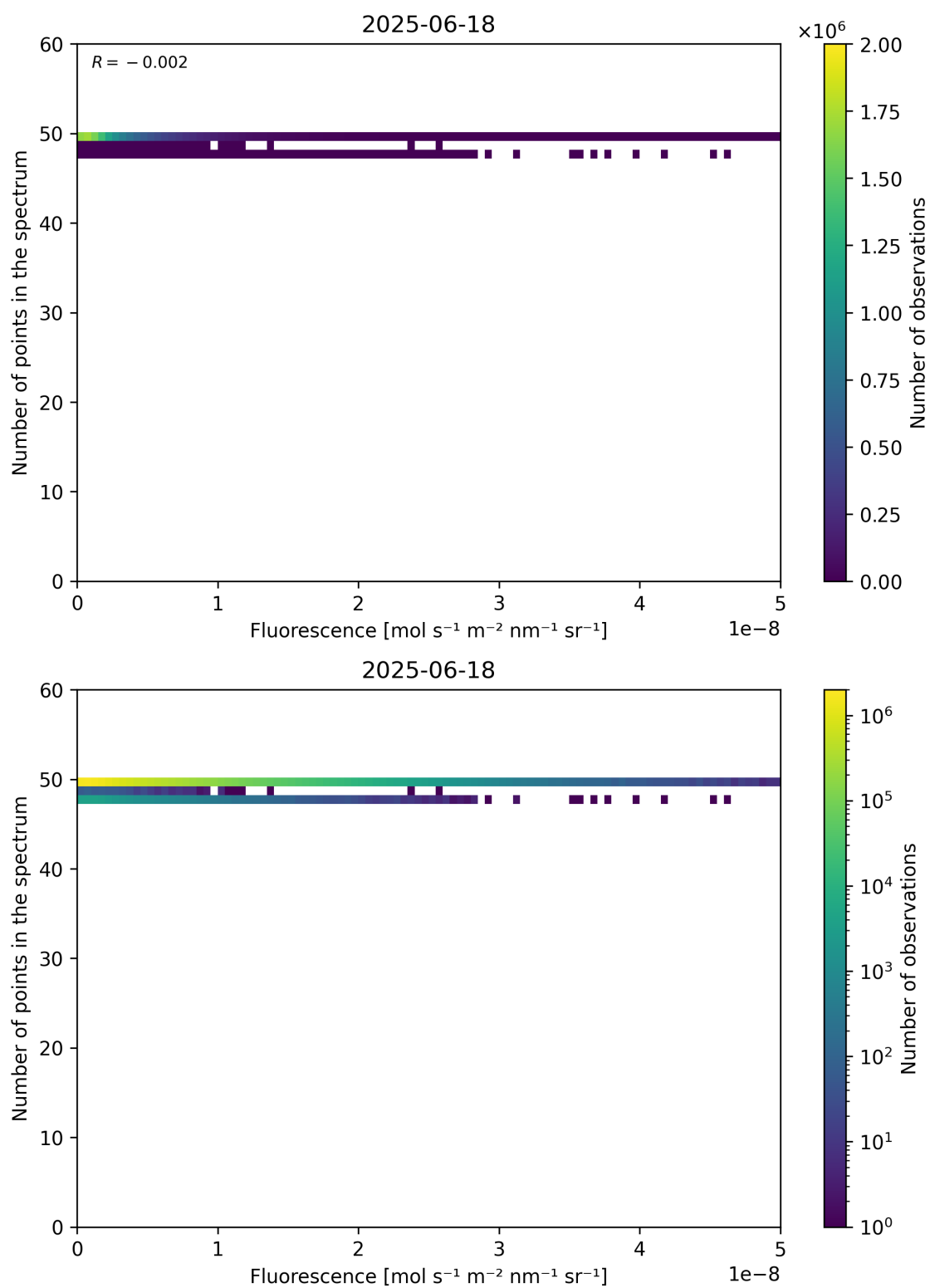
Figure 86: Scatter density plot of “Fluorescence” against “Number of points in the spectrum” for 2025-06-17 to 2025-06-19.
