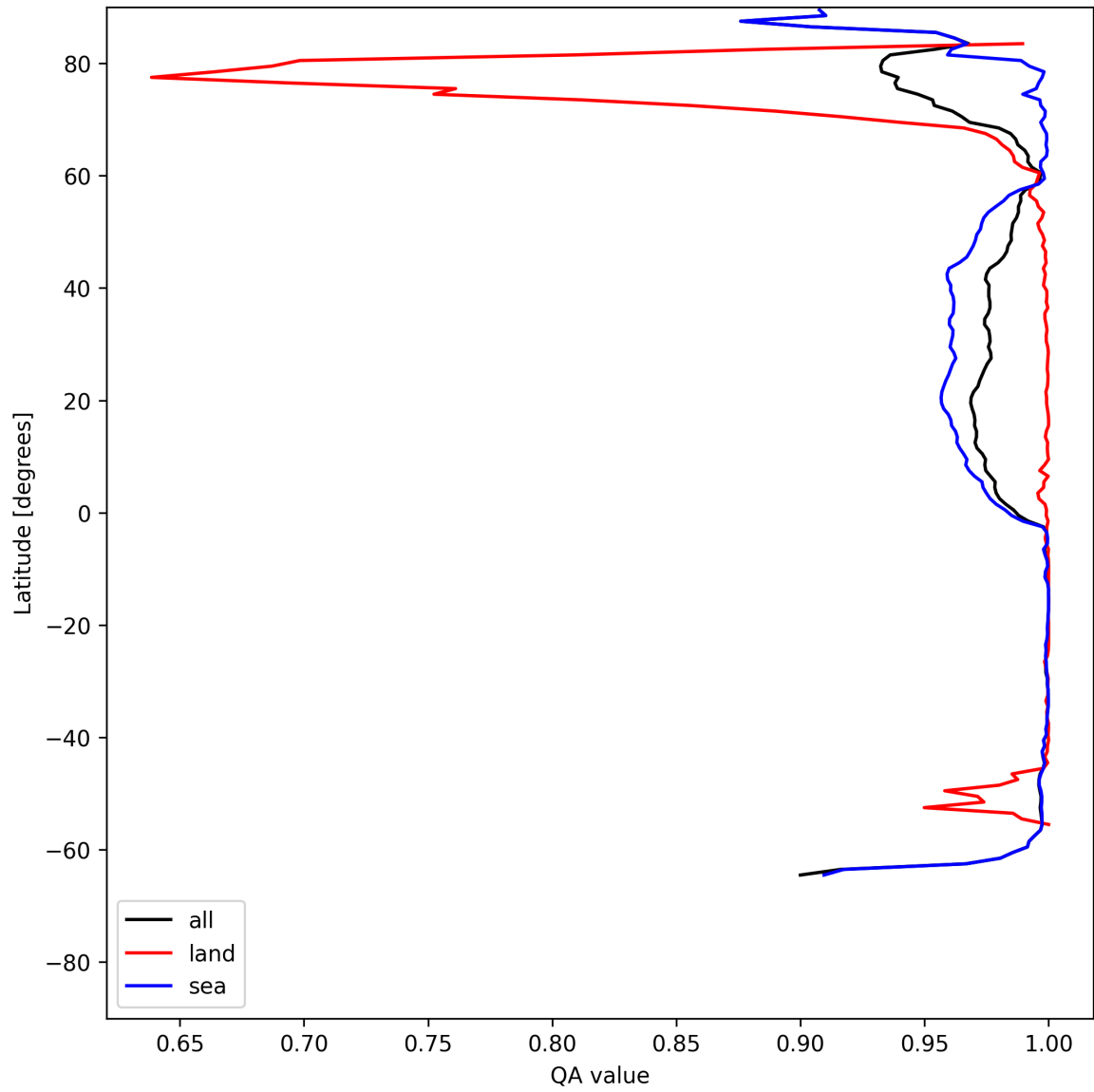
Figure 12: Zonal average of “QA value” for 2025-06-17 to 2025-06-19.
