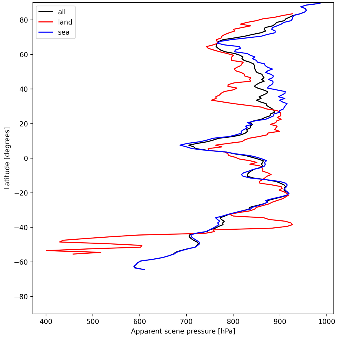
Figure 19: Zonal average of “Apparent scene pressure” for 2025-06-17 to 2025-06-19.
