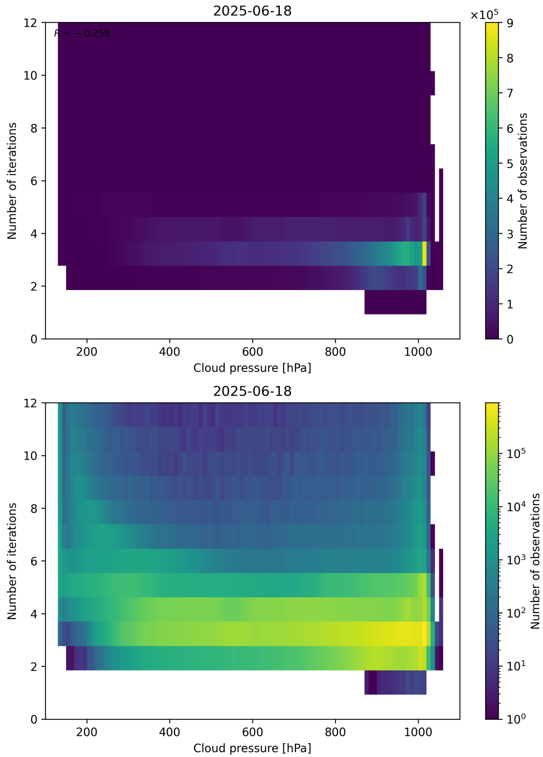
Figure 81: Scatter density plot of “Cloud pressure” against “Number of iterations” for 2025-06-17 to 2025-06-19.
