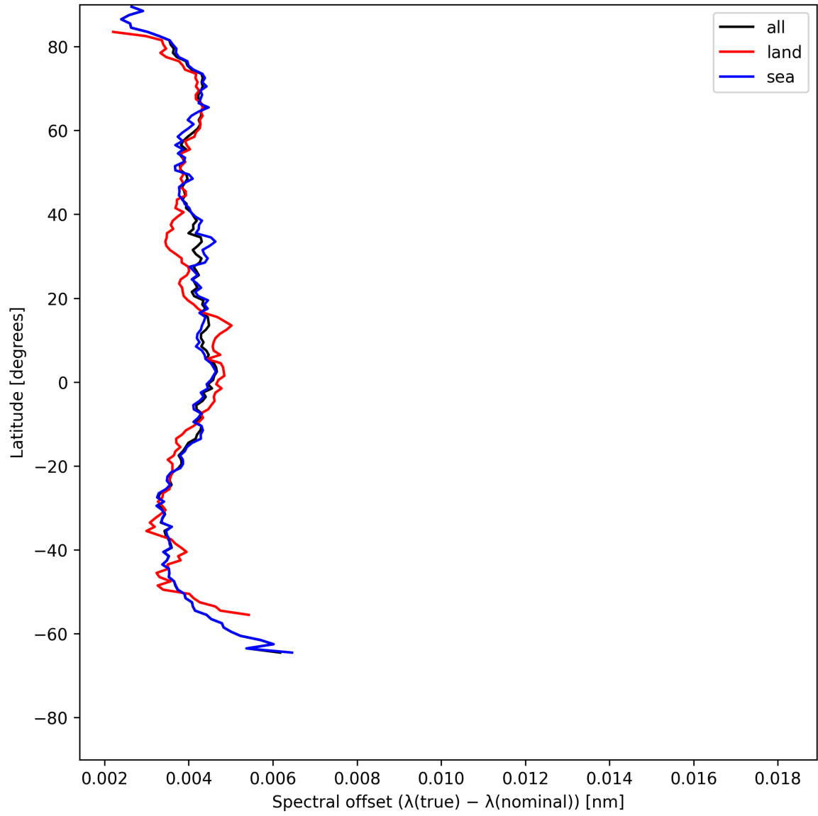
Figure 28: Zonal average of “Spectral offset ( \lambda_{\text{true}} - \lambda_{\text{nominal}} )” for 2025-06-17 to 2025-06-19.
