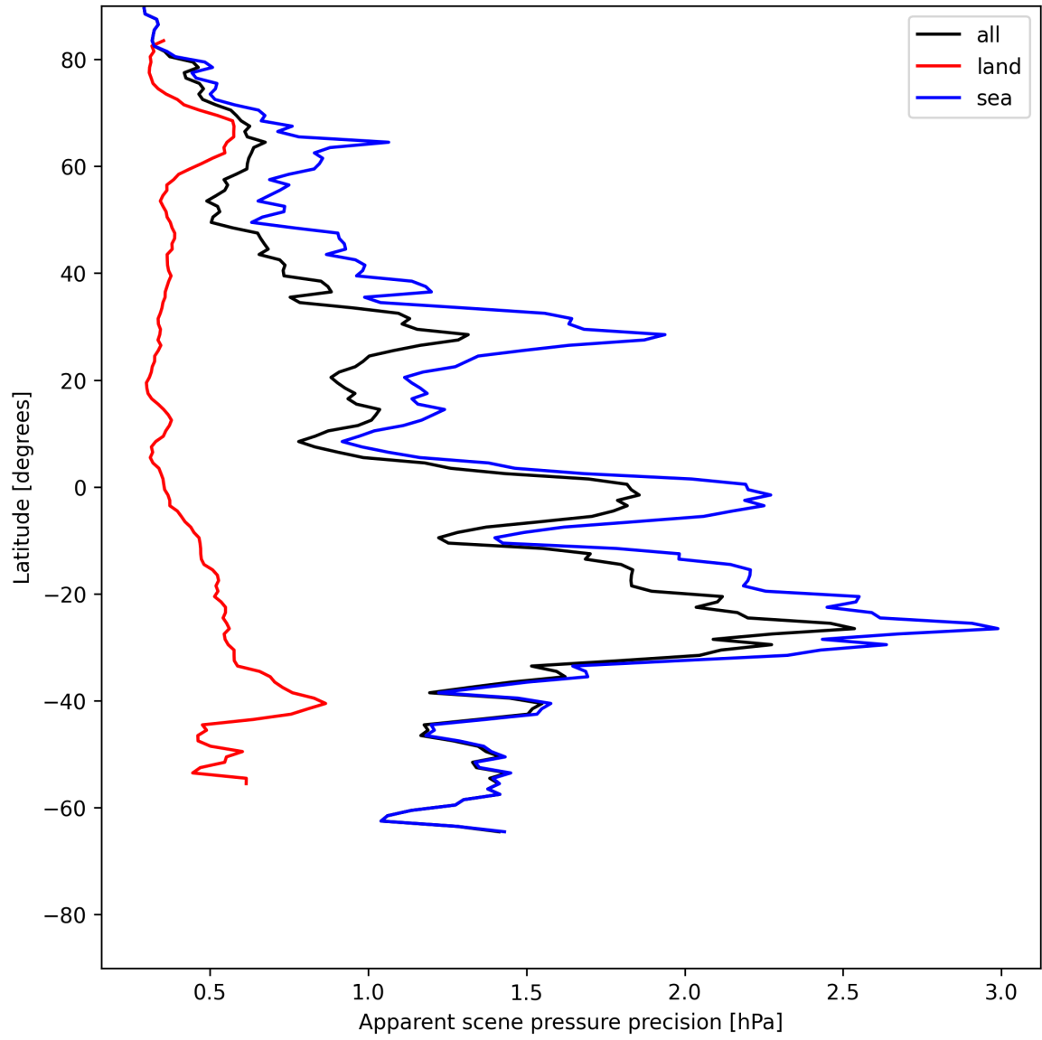
Figure 20: Zonal average of “Apparent scene pressure precision” for 2025-06-17 to 2025-06-19.
