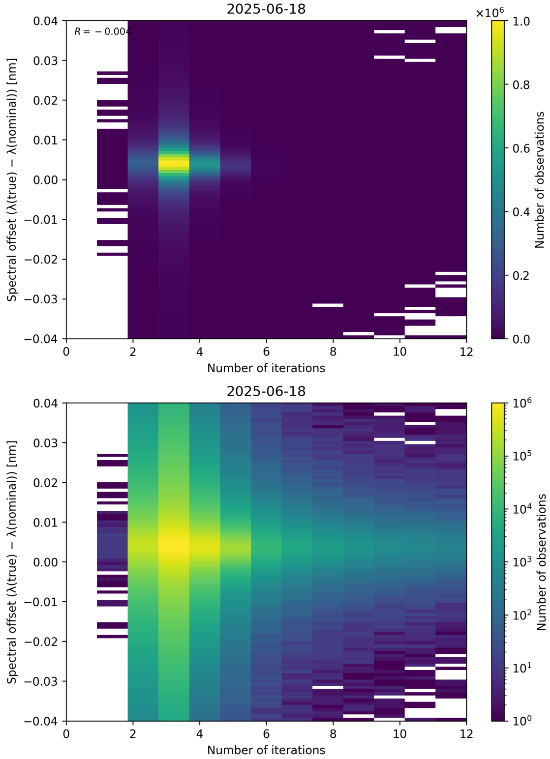
Figure 100: Scatter density plot of “Number of iterations” against “Spectral offset ( \lambda_{\text{true}} - \lambda_{\text{nominal}} )” for 2025-06-17 to 2025-06-19.
