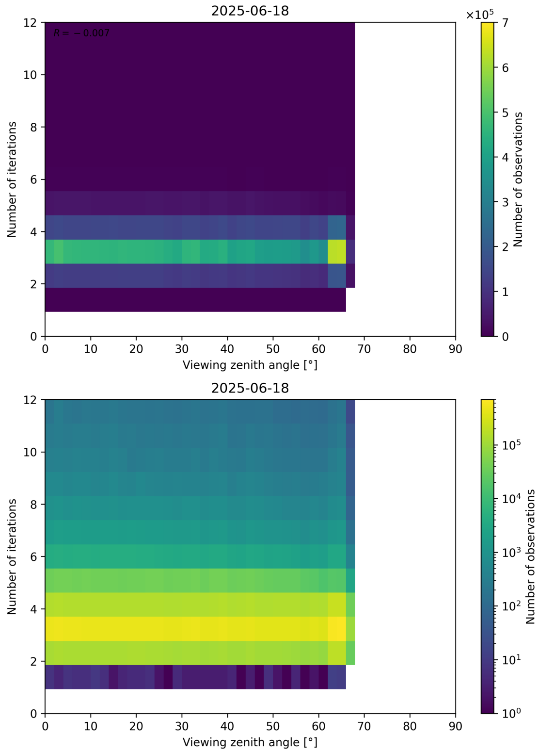
Figure 124: Scatter density plot of “Viewing zenith angle” against “Number of iterations” for 2025-06-17 to 2025-06-19.
