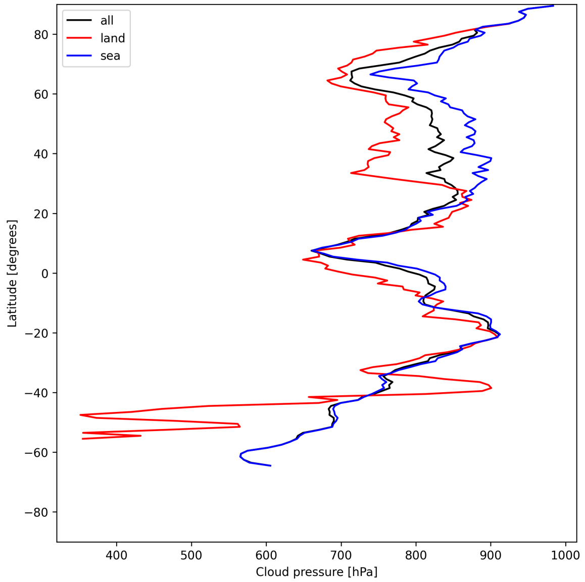
Figure 13: Zonal average of “Cloud pressure” for 2025-06-17 to 2025-06-19.
