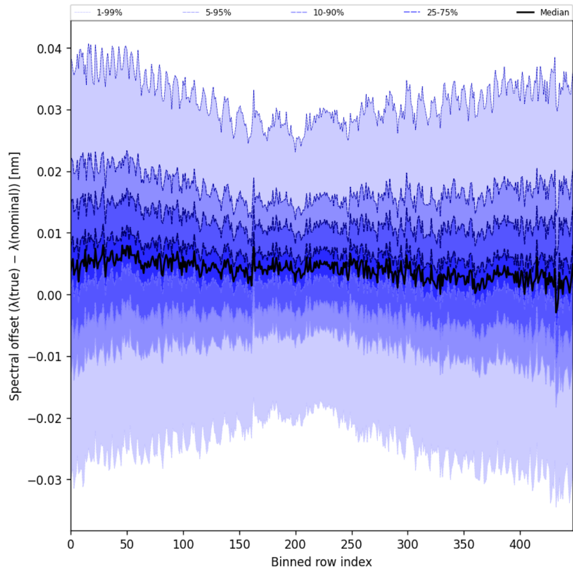
Figure 62: Along track statistics of “Spectral offset ( \lambda_{\text{true}} - \lambda_{\text{nominal}} )” for 2025-06-17 to 2025-06-19
