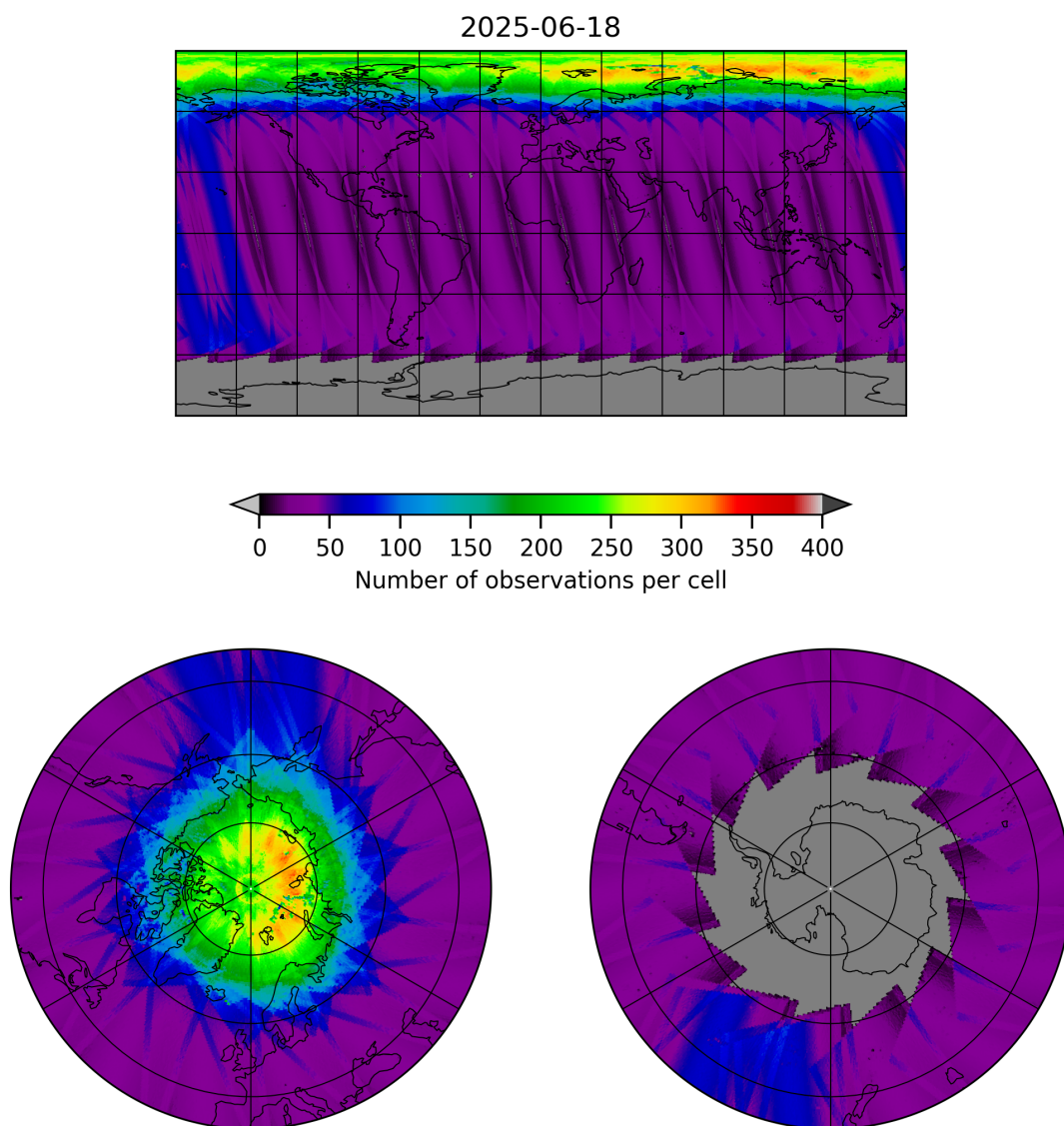
Figure 11: Map of the number of observations for 2025-06-17 to 2025-06-19
