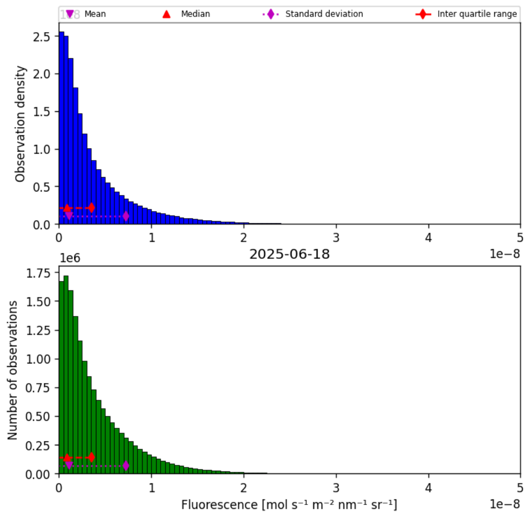
Figure 40: Histogram of “Fluorescence” for 2025-06-17 to 2025-06-19
