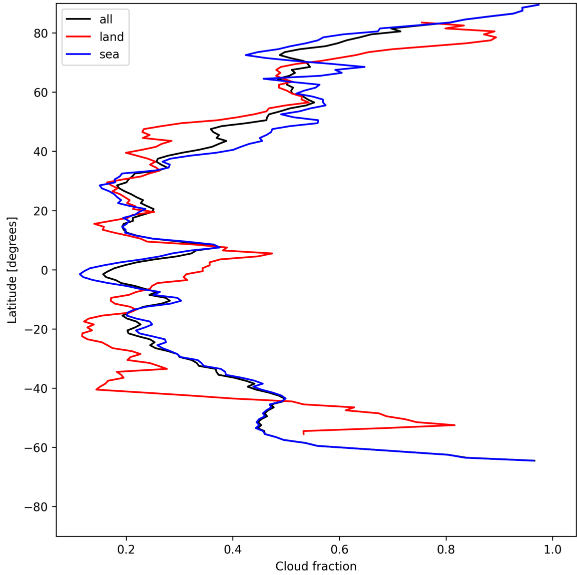
Figure 15: Zonal average of “Cloud fraction” for 2025-06-17 to 2025-06-19.
