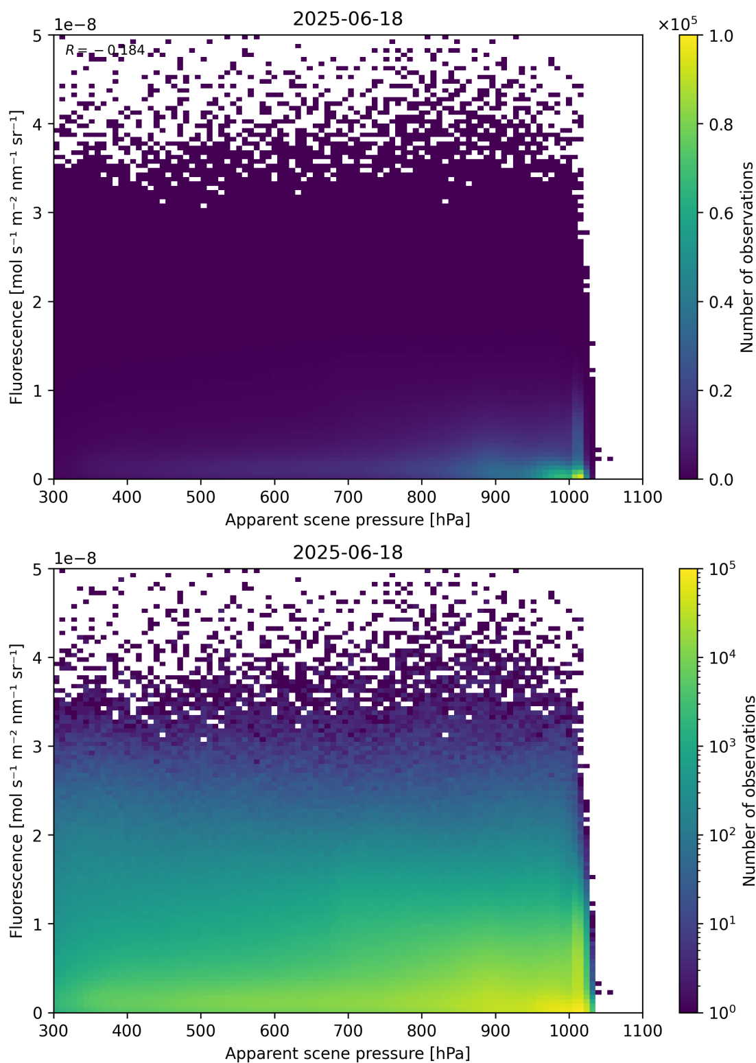
Figure 64: Scatter density plot of “Apparent scene pressure” against “Fluorescence” for 2025-06-17 to 2025-06-19.
