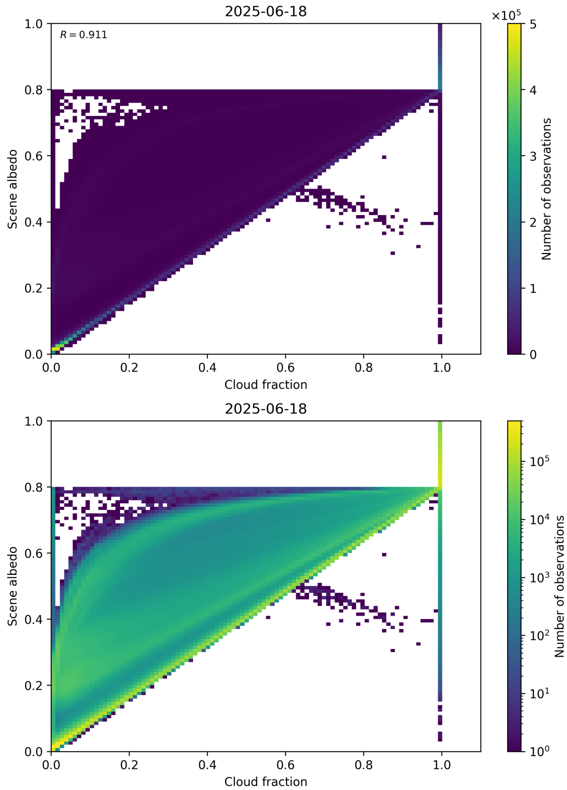
Figure 75: Scatter density plot of “Cloud fraction” against “Scene albedo” for 2025-06-17 to 2025-06-19.
