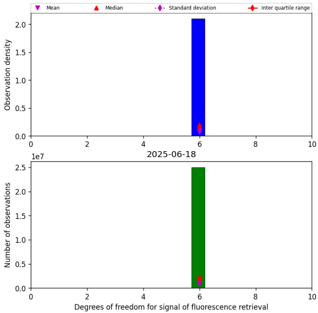
Figure 43: Histogram of “Degrees of freedom for signal of fluorescence retrieval” for 2025-06-17 to 2025-06-19
