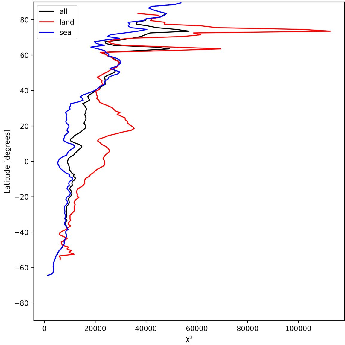
Figure 21: Zonal average of “ \chi^2 ” for 2025-06-17 to 2025-06-19.
