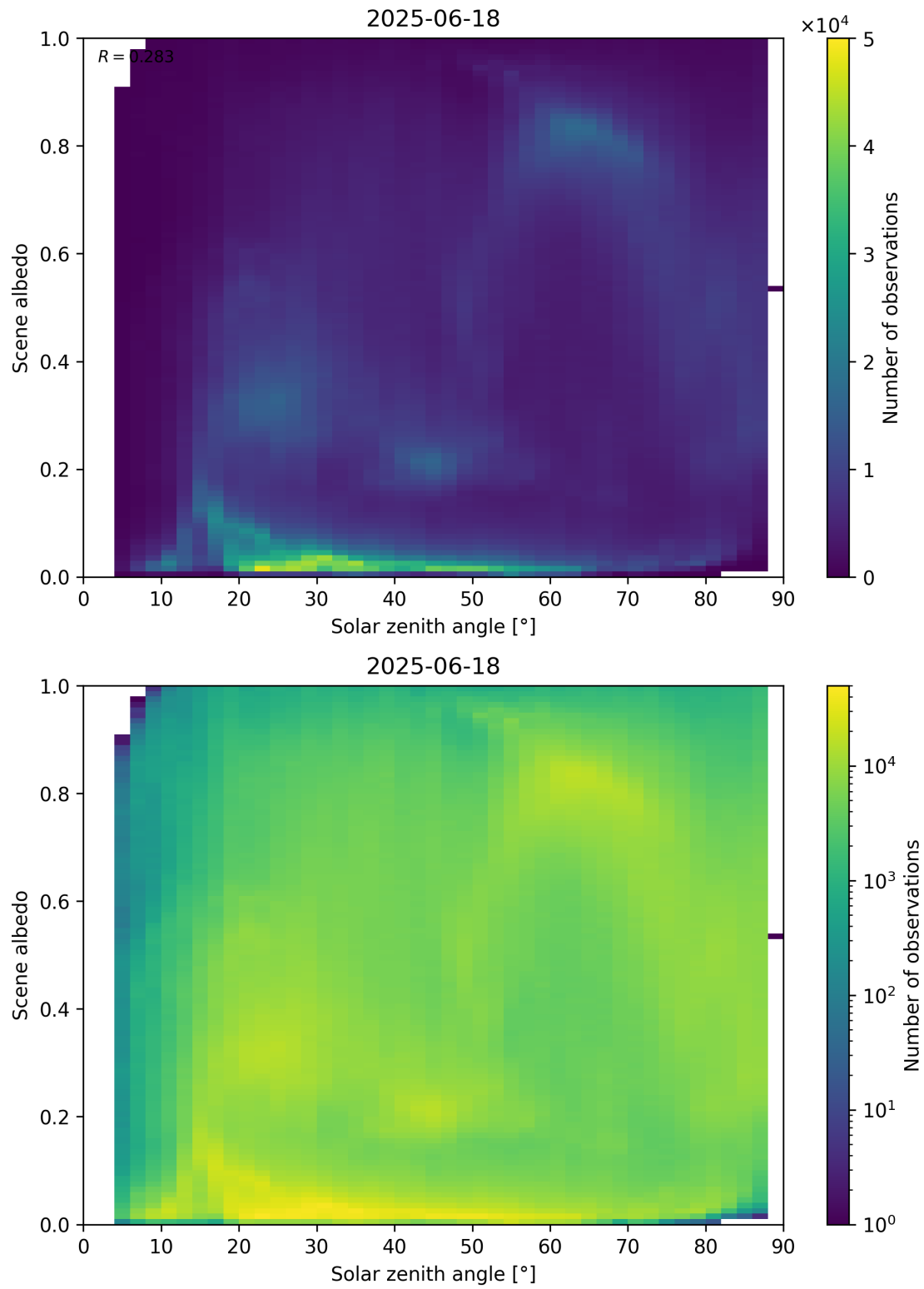
Figure 116: Scatter density plot of “Solar zenith angle” against “Scene albedo” for 2025-06-17 to 2025-06-19.
