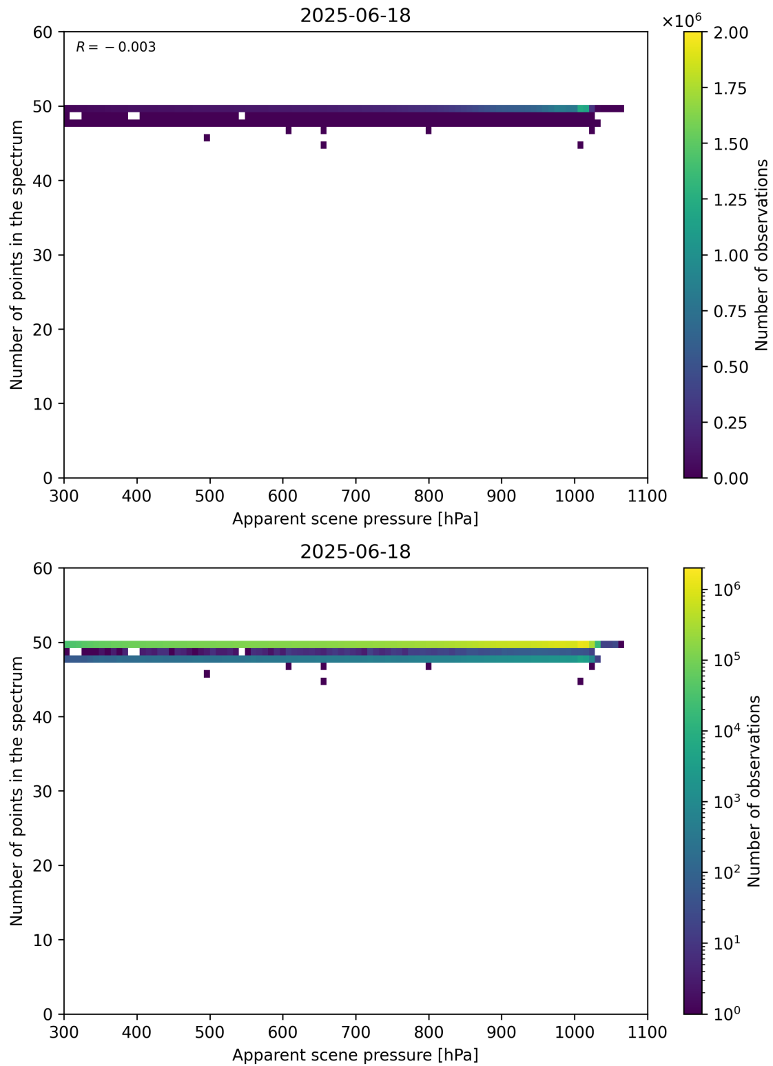
Figure 66: Scatter density plot of “Apparent scene pressure” against “Number of points in the spectrum” for 2025-06-17 to 2025-06-19.
