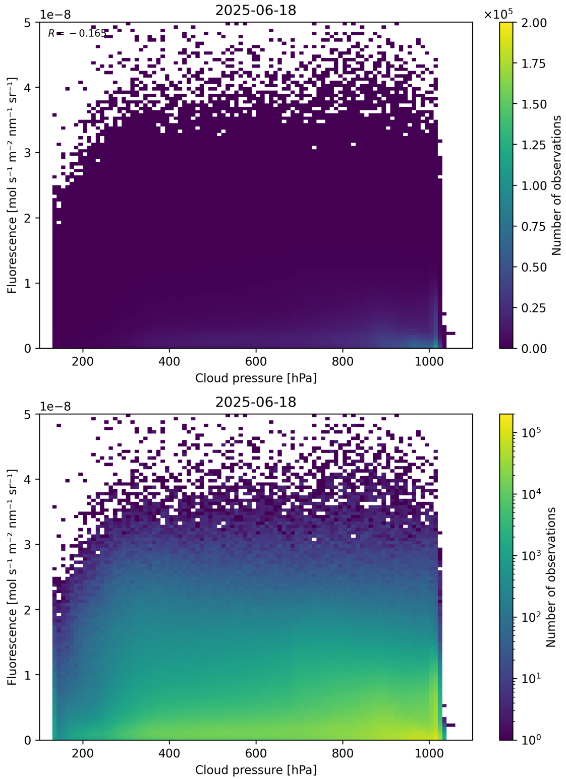
Figure 80: Scatter density plot of “Cloud pressure” against “Fluorescence” for 2025-06-17 to 2025-06-19.
