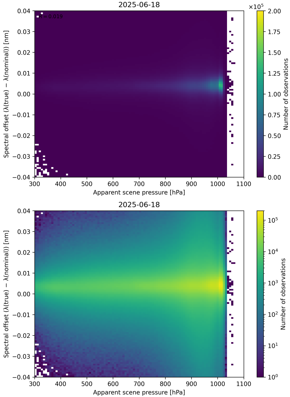
Figure 67: Scatter density plot of “Apparent scene pressure” against “Spectral offset ( \lambda_{\text{true}} - \lambda_{\text{nominal}} )” for 2025-06-17 to 2025-06-19.
