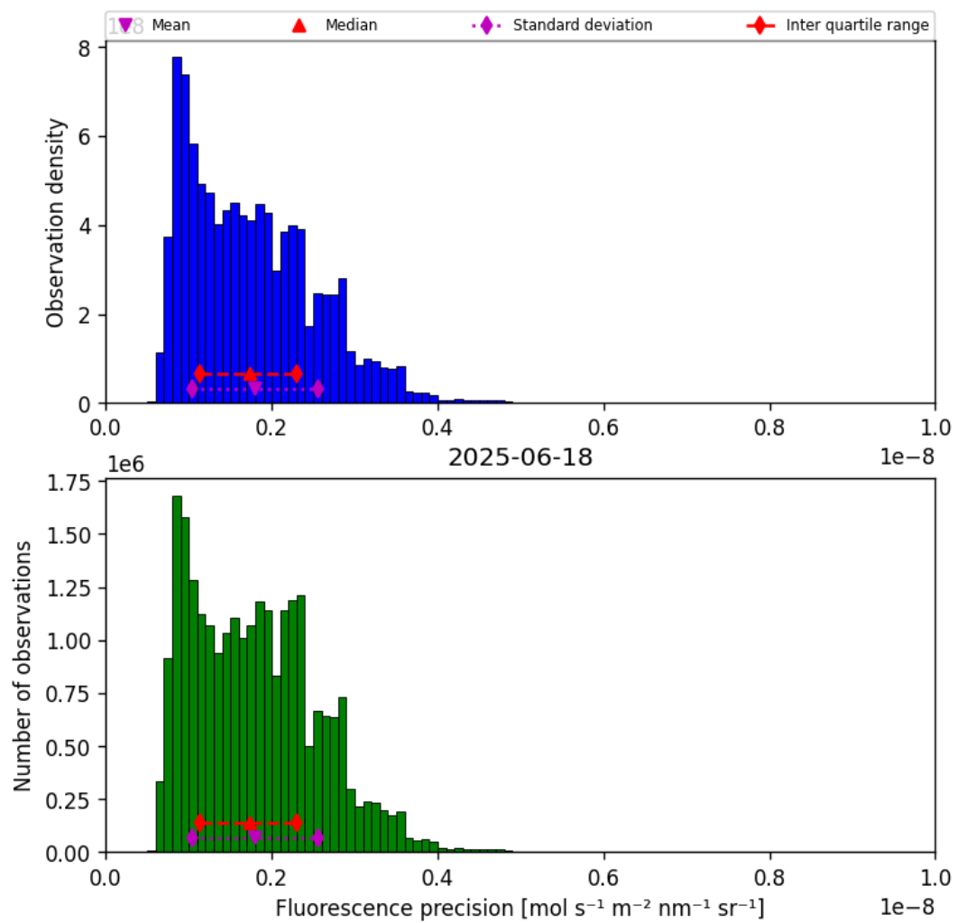
Figure 41: Histogram of “Fluorescence precision” for 2025-06-17 to 2025-06-19
