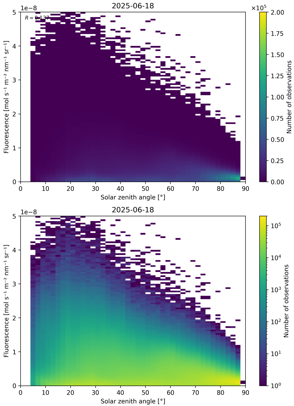
Figure 112: Scatter density plot of “Solar zenith angle” against “Fluorescence” for 2025-06-17 to 2025-06-19.
