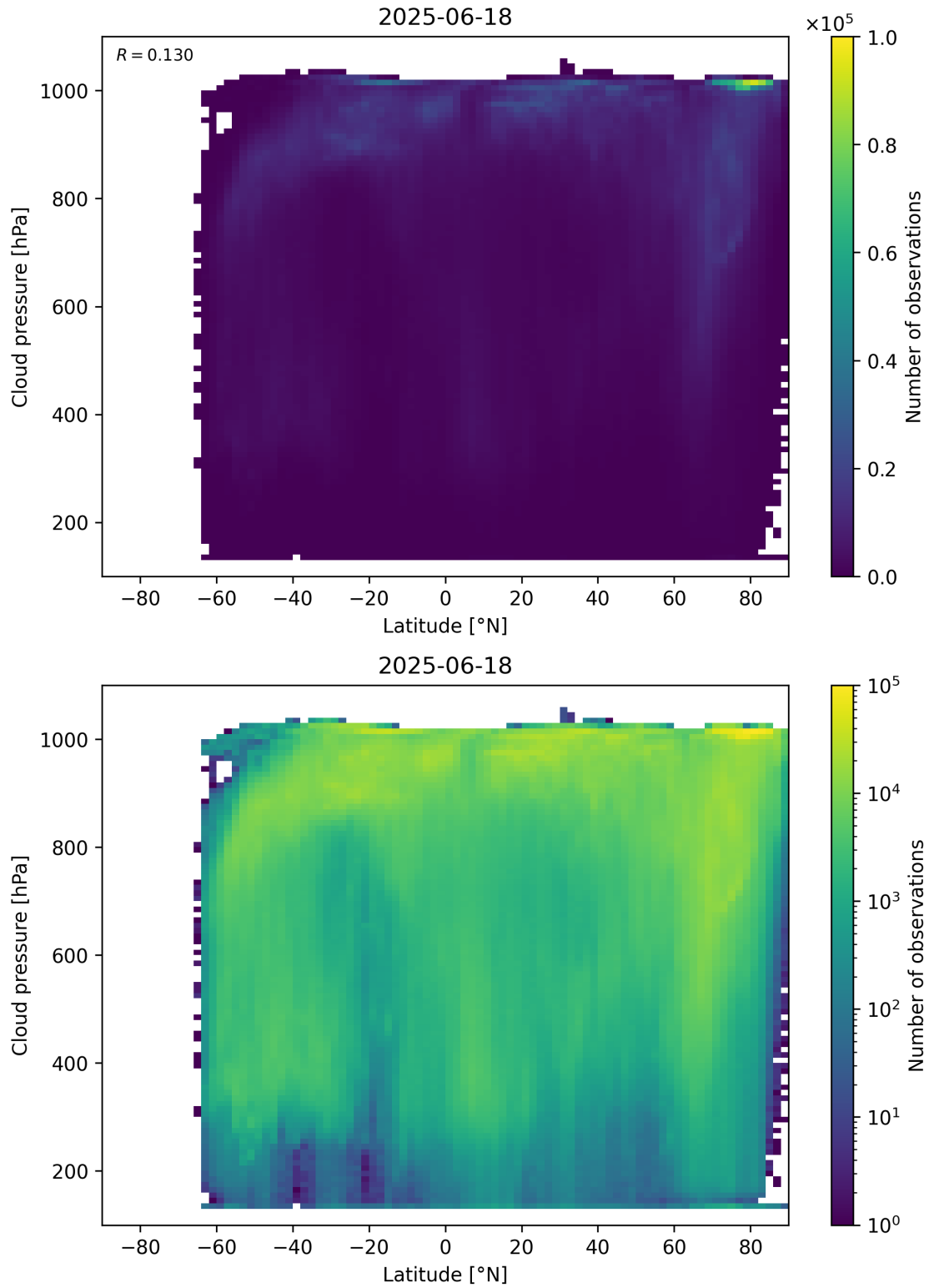
Figure 91: Scatter density plot of “Latitude” against “Cloud pressure” for 2025-06-17 to 2025-06-19.
