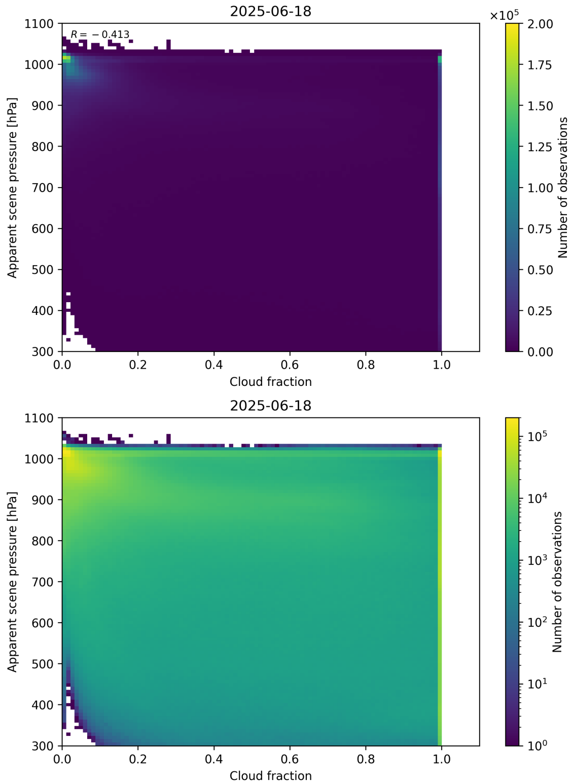
Figure 70: Scatter density plot of “Cloud fraction” against “Apparent scene pressure” for 2025-06-17 to 2025-06-19.
