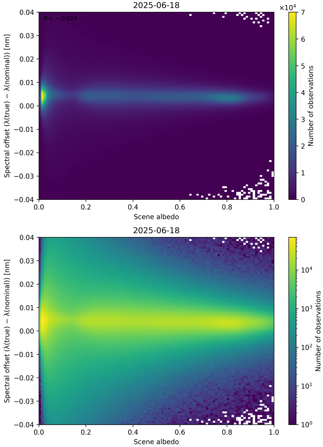
Figure 107: Scatter density plot of “Scene albedo” against “Spectral offset ( \lambda_{\text{true}} - \lambda_{\text{nominal}} )” for 2025-06-17 to 2025-06-19.
