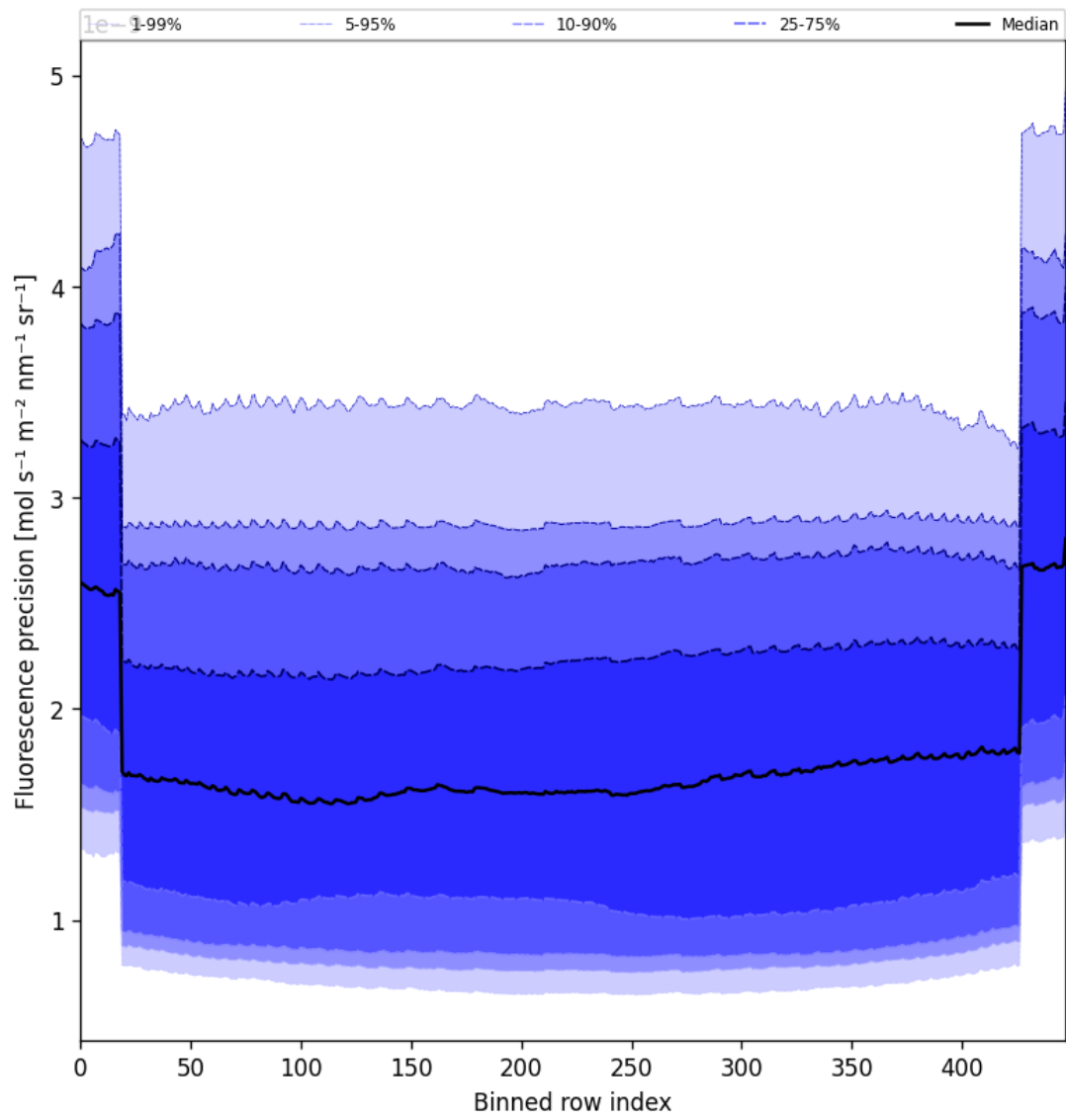
Figure 58: Along track statistics of "Fluorescence precision" for 2025-06-17 to 2025-06-19
