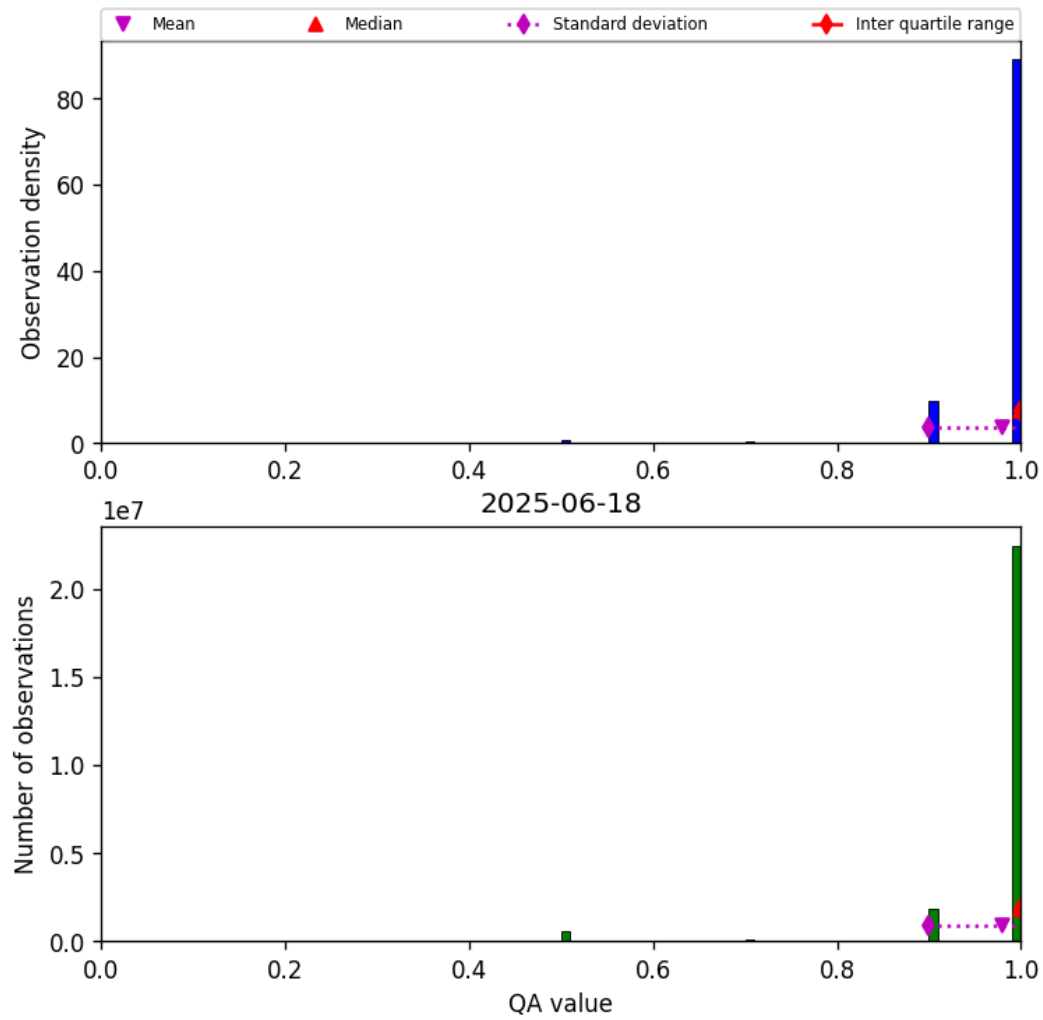
Figure 29: Histogram of “QA value” for 2025-06-17 to 2025-06-19
