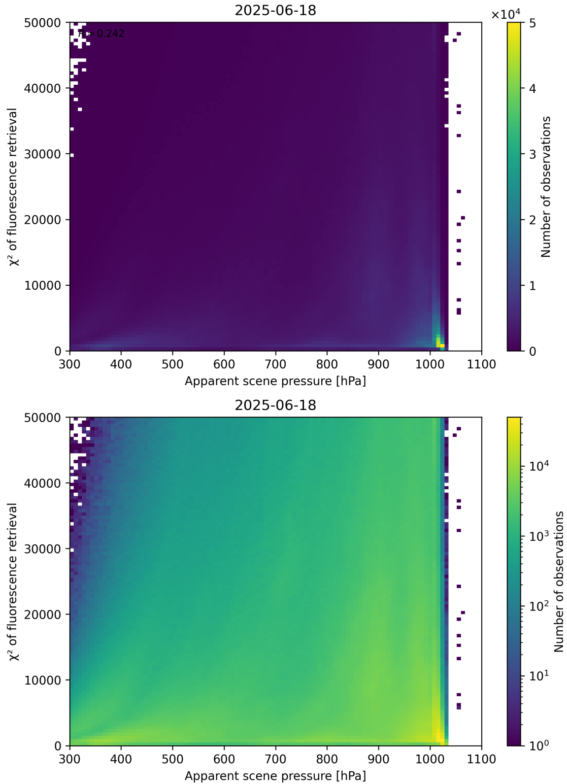
Figure 63: Scatter density plot of “Apparent scene pressure” against “ \chi^2 of fluorescence retrieval” for 2025-06-17 to 2025-06-19.
