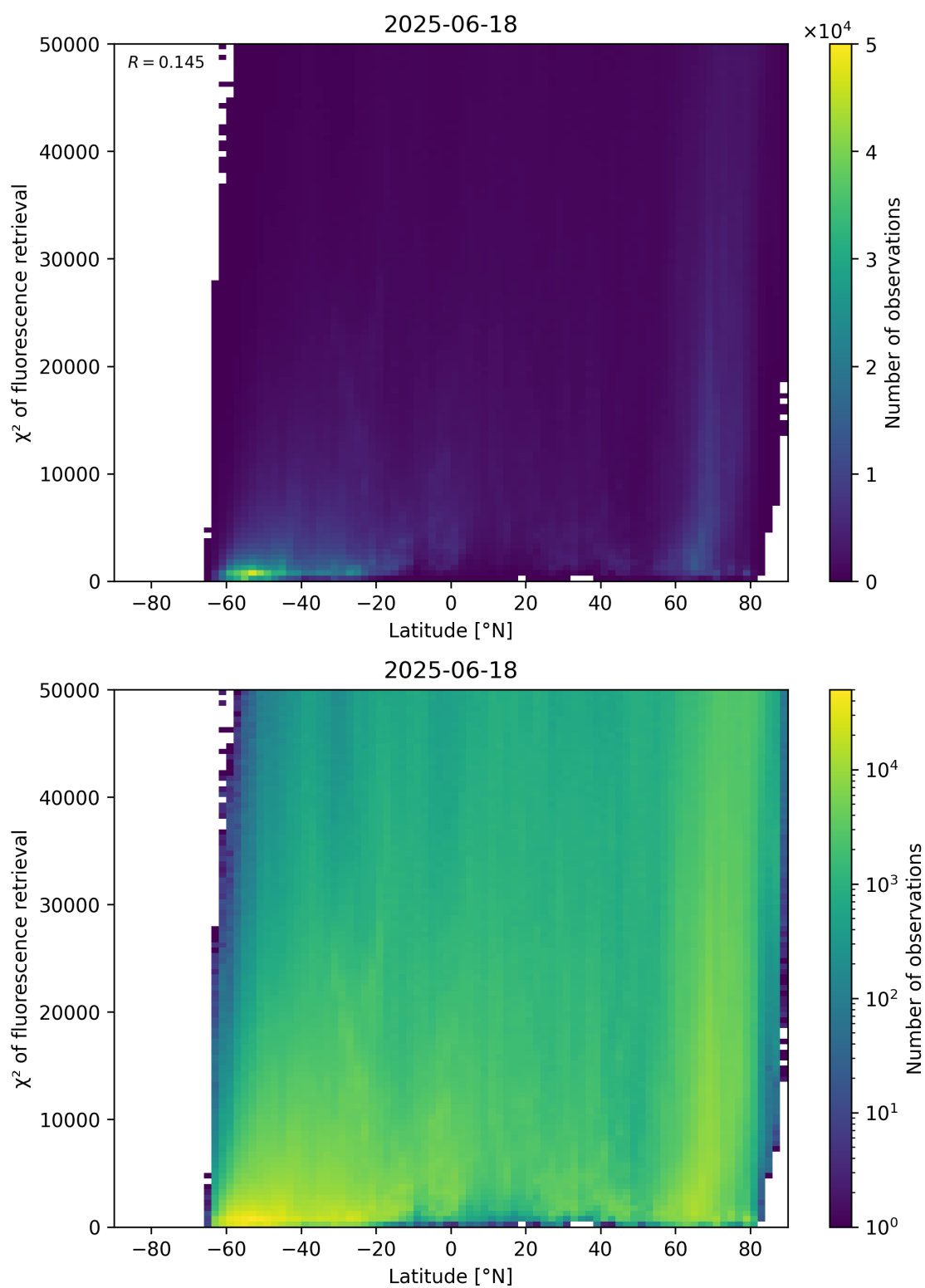
Figure 89: Scatter density plot of “Latitude” against “ \chi^2 of fluorescence retrieval” for 2025-06-17 to 2025-06-19.
