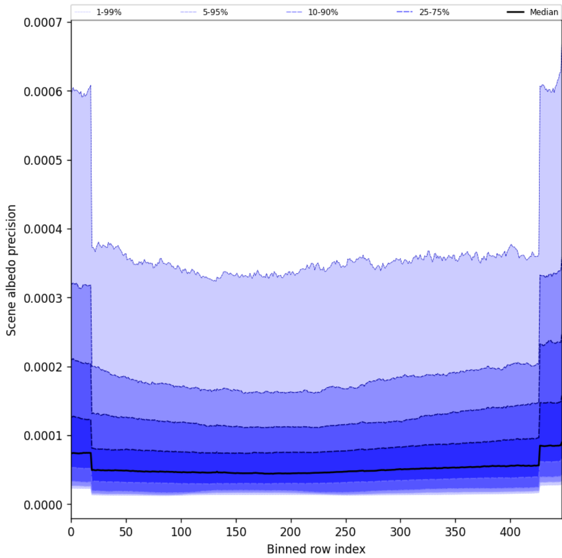
Figure 52: Along track statistics of “Scene albedo precision” for 2025-06-17 to 2025-06-19
