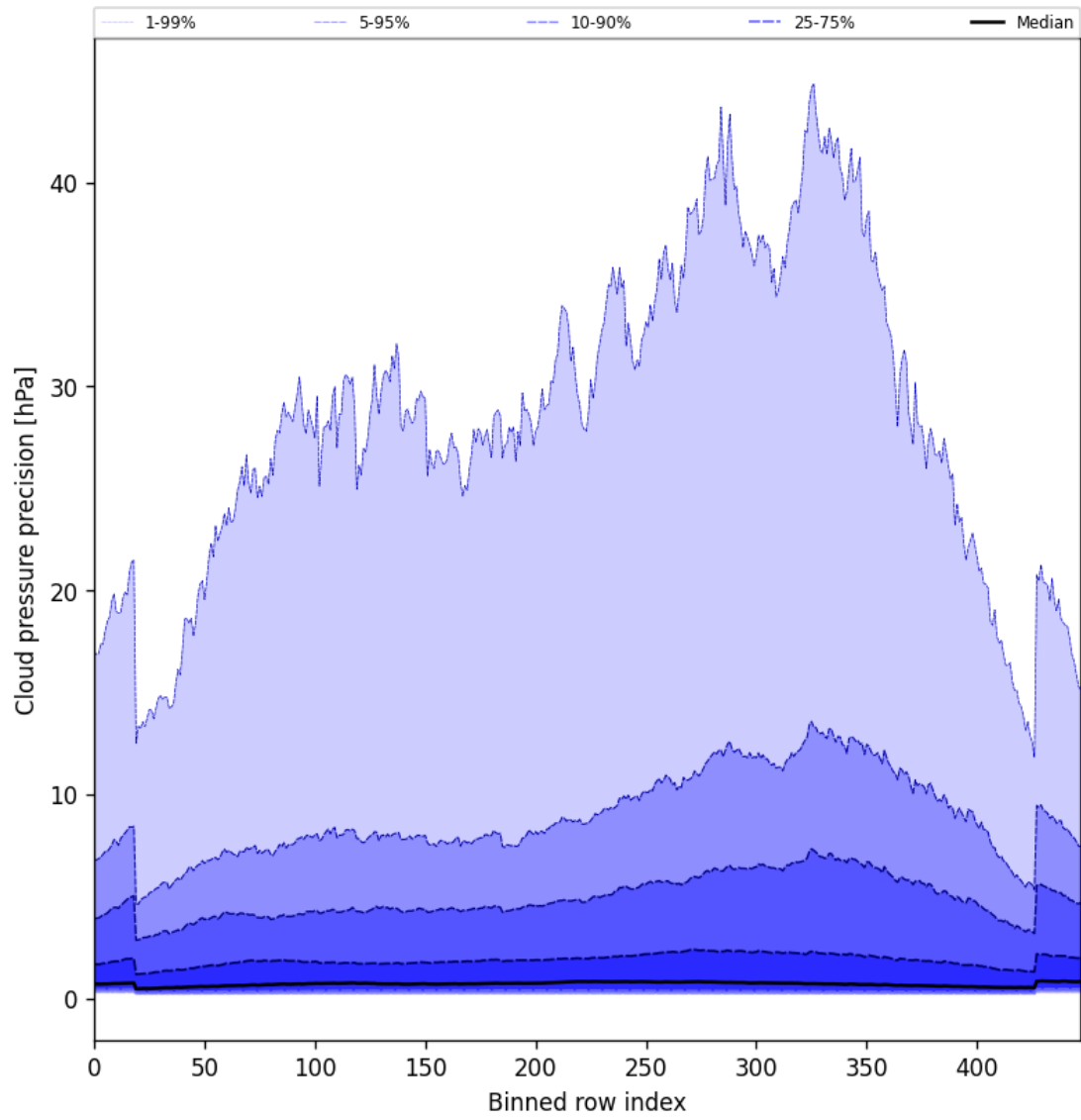
Figure 48: Along track statistics of “Cloud pressure precision” for 2025-06-17 to 2025-06-19
