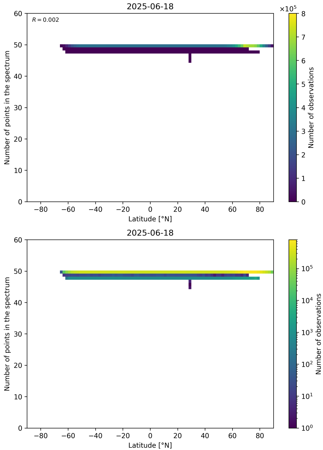
Figure 94: Scatter density plot of “Latitude” against “Number of points in the spectrum” for 2025-06-17 to 2025-06-19.
