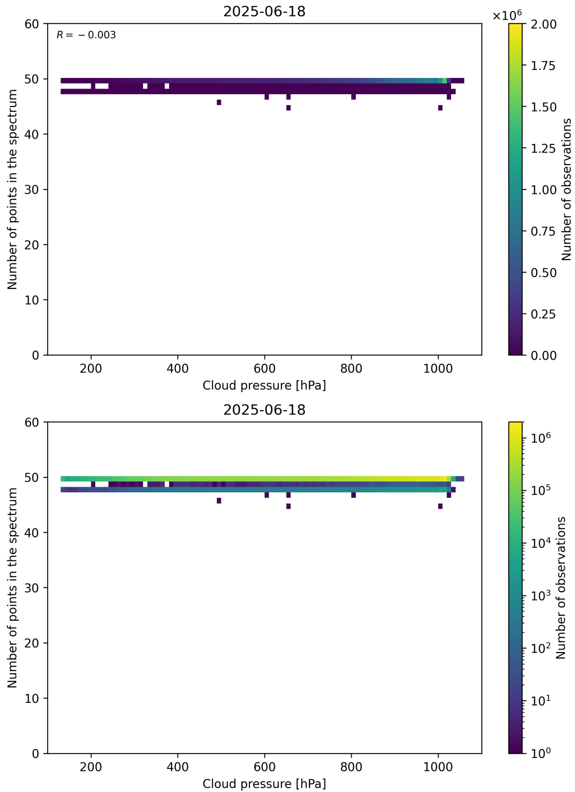
Figure 82: Scatter density plot of “Cloud pressure” against “Number of points in the spectrum” for 2025-06-17 to 2025-06-19.
