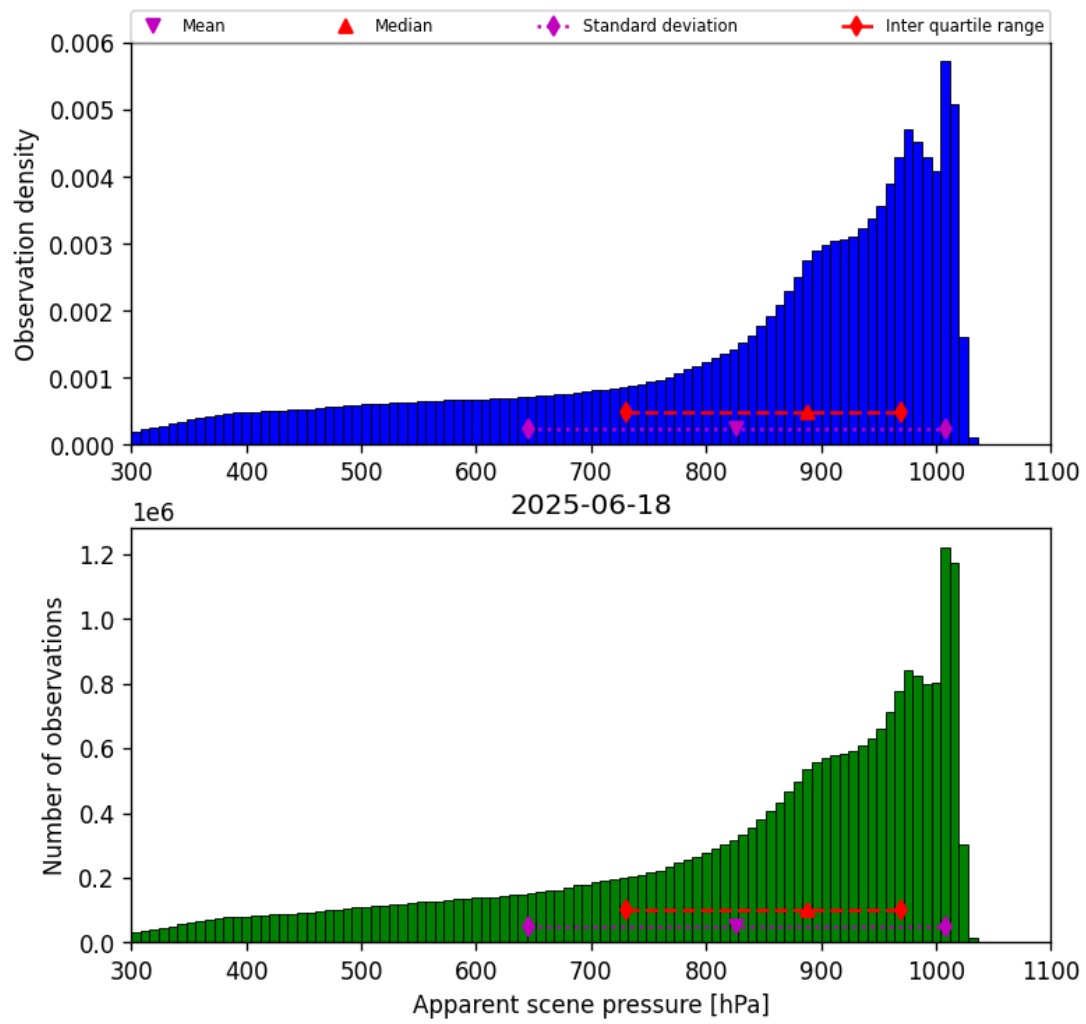
Figure 36: Histogram of “Apparent scene pressure” for 2025-06-17 to 2025-06-19
