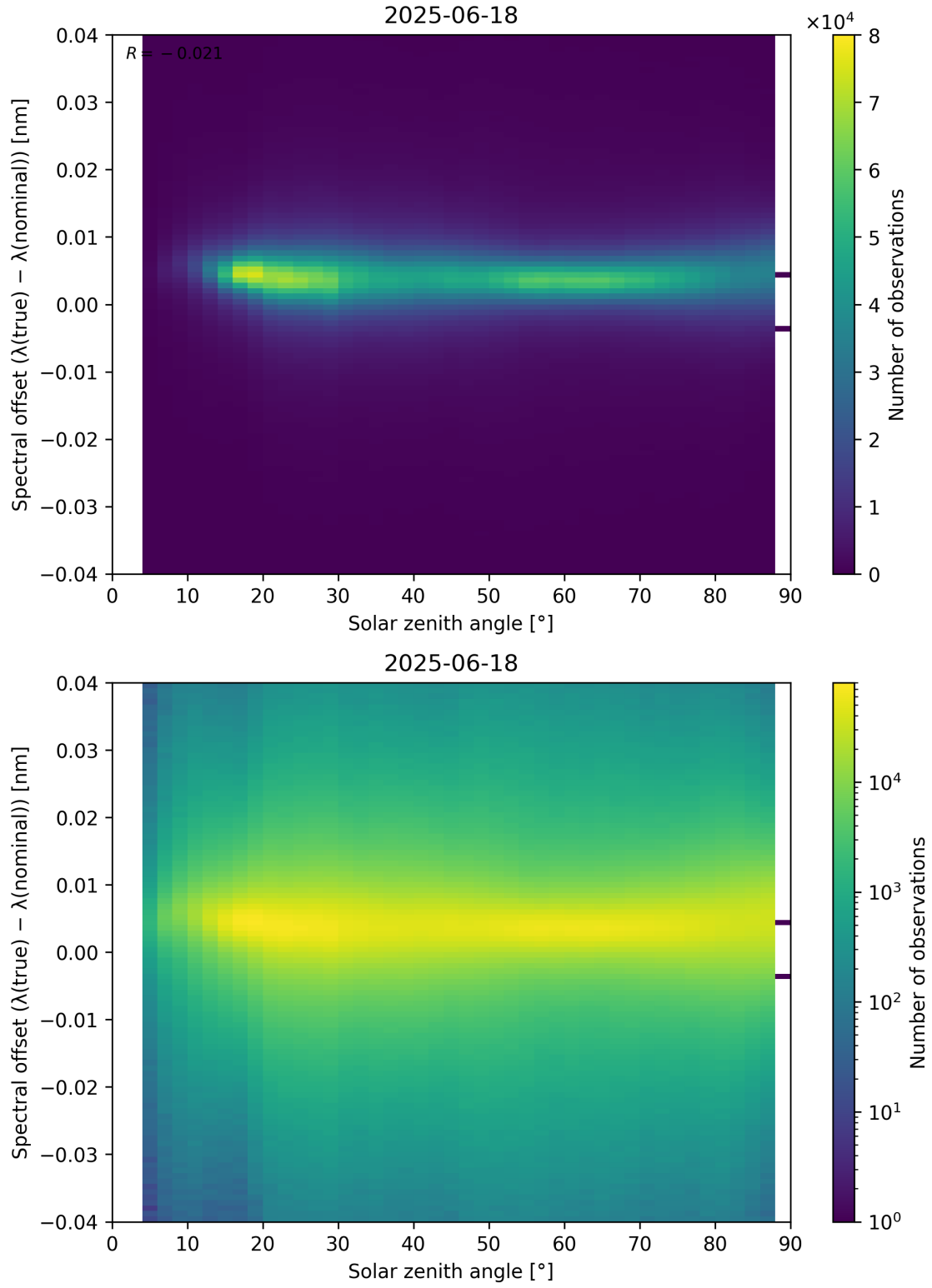
Figure 117: Scatter density plot of “Solar zenith angle” against “Spectral offset ( \lambda_{\text{true}} - \lambda_{\text{nominal}} )” for 2025-06-17 to 2025-06-19.
