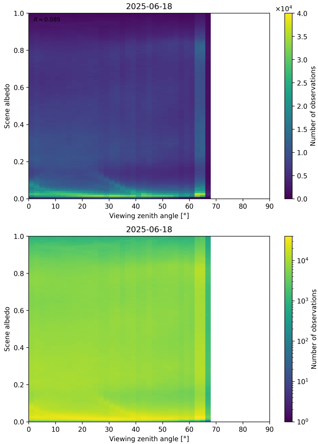
Figure 126: Scatter density plot of “Viewing zenith angle” against “Scene albedo” for 2025-06-17 to 2025-06-19.
