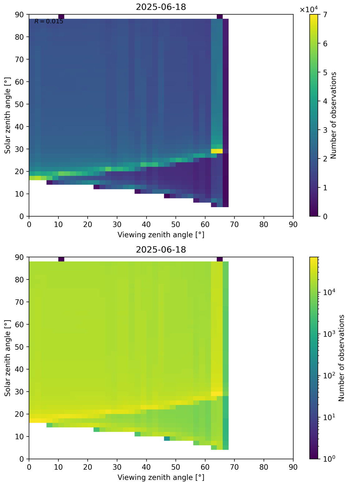
Figure 127: Scatter density plot of “Viewing zenith angle” against “Solar zenith angle” for 2025-06-17 to 2025-06-19.
