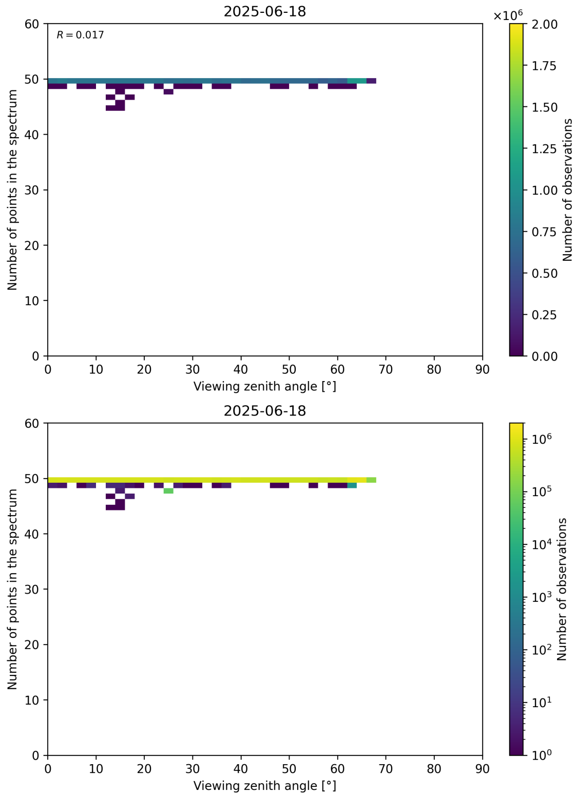
Figure 125: Scatter density plot of “Viewing zenith angle” against “Number of points in the spectrum” for 2025-06-17 to 2025-06-19.
