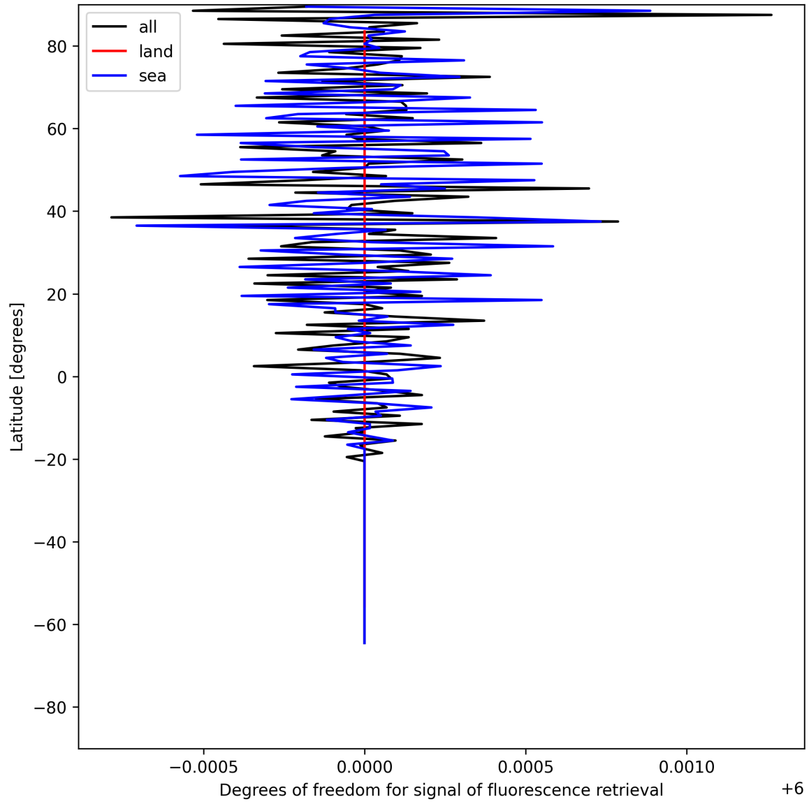
Figure 26: Zonal average of “Degrees of freedom for signal of fluorescence retrieval” for 2025-06-17 to 2025-06-19.
