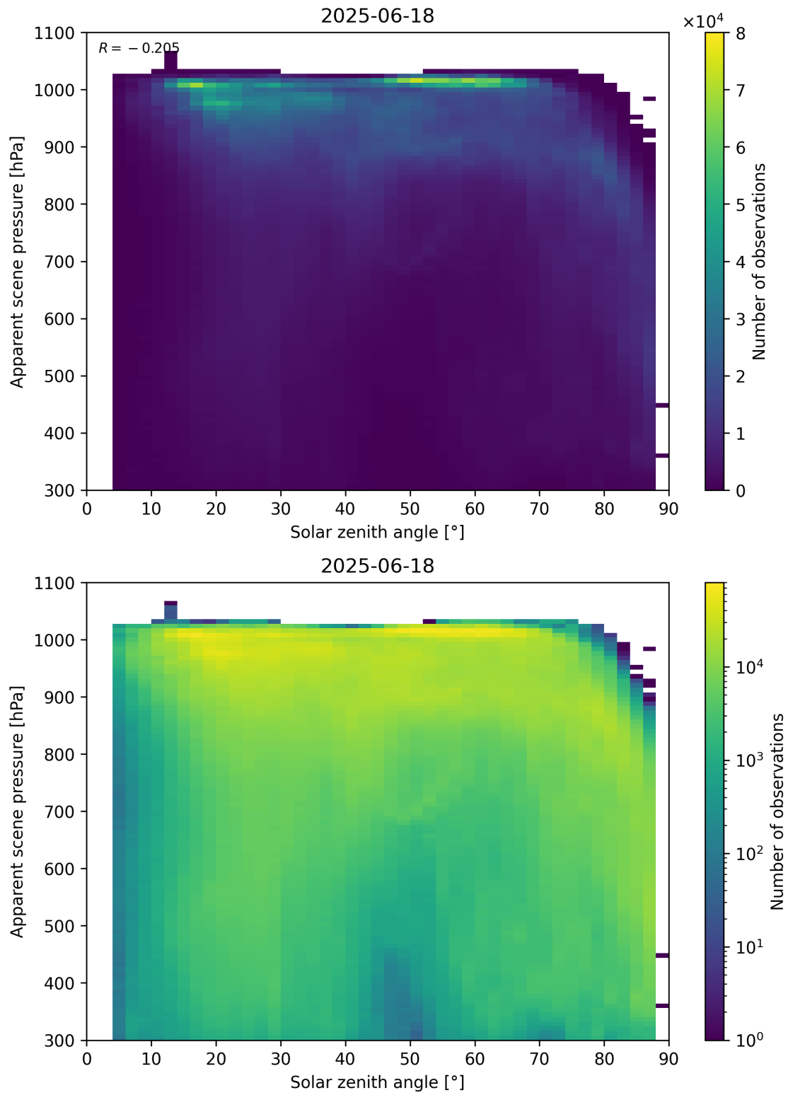
Figure 108: Scatter density plot of “Solar zenith angle” against “Apparent scene pressure” for 2025-06-17 to 2025-06-19.
