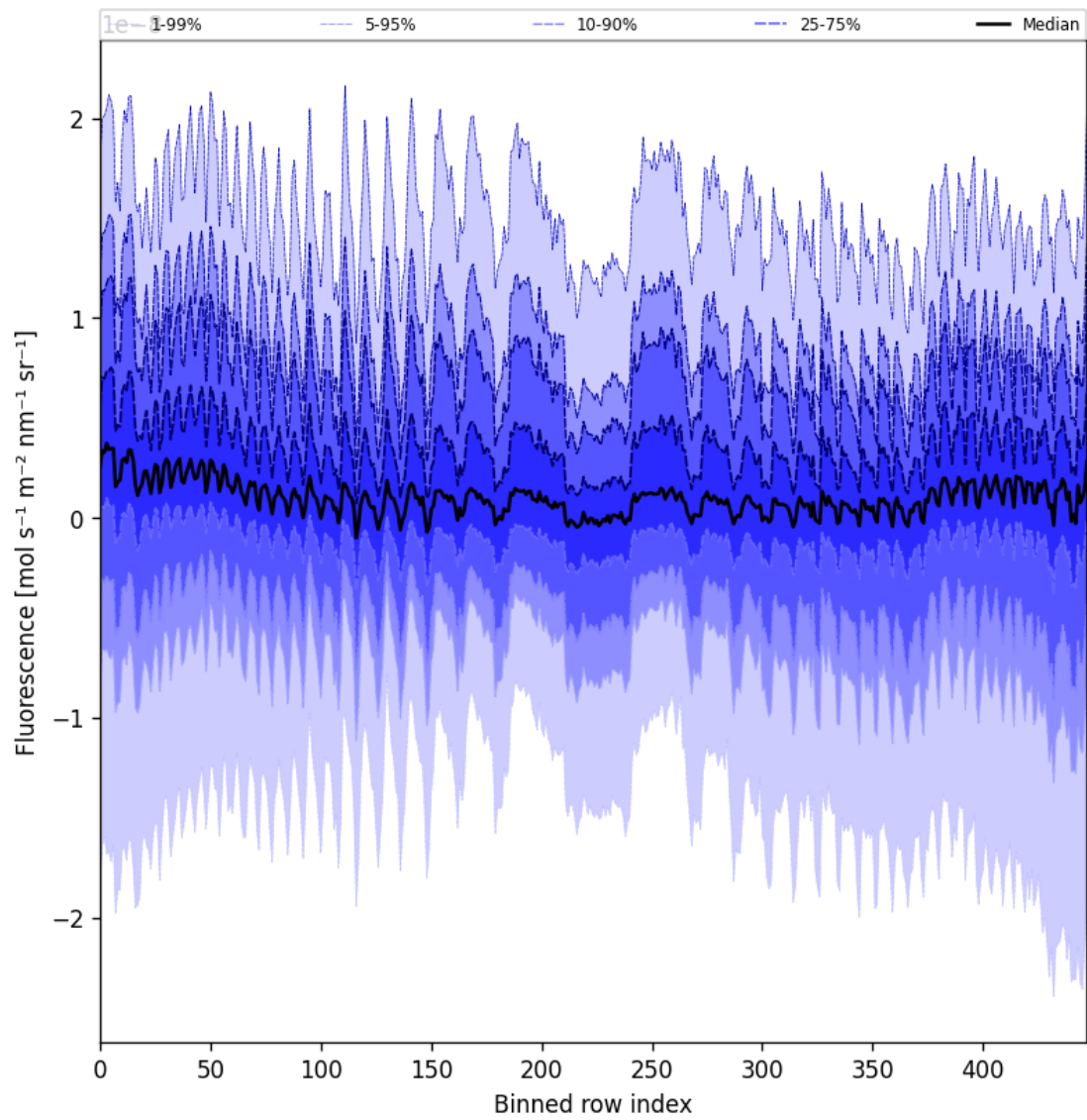
Figure 57: Along track statistics of “Fluorescence” for 2025-06-17 to 2025-06-19
