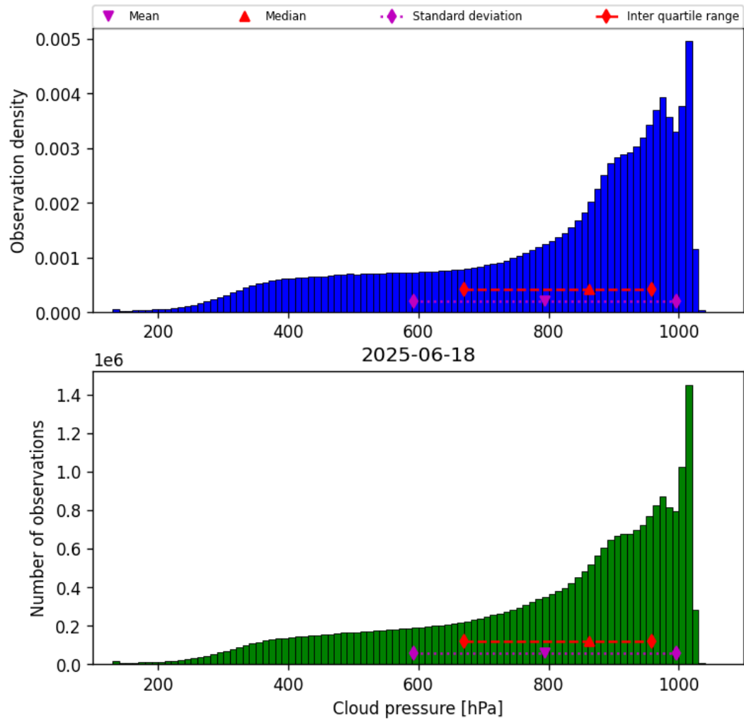
Figure 30: Histogram of “Cloud pressure” for 2025-06-17 to 2025-06-19
