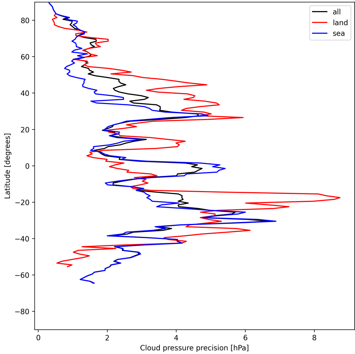
Figure 14: Zonal average of “Cloud pressure precision” for 2025-06-17 to 2025-06-19.
