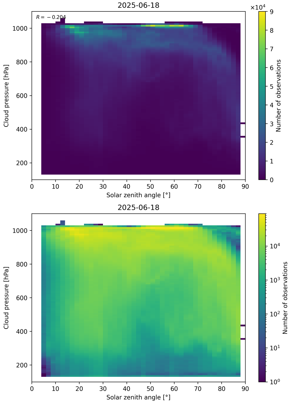
Figure 111: Scatter density plot of “Solar zenith angle” against “Cloud pressure” for 2025-06-17 to 2025-06-19.
