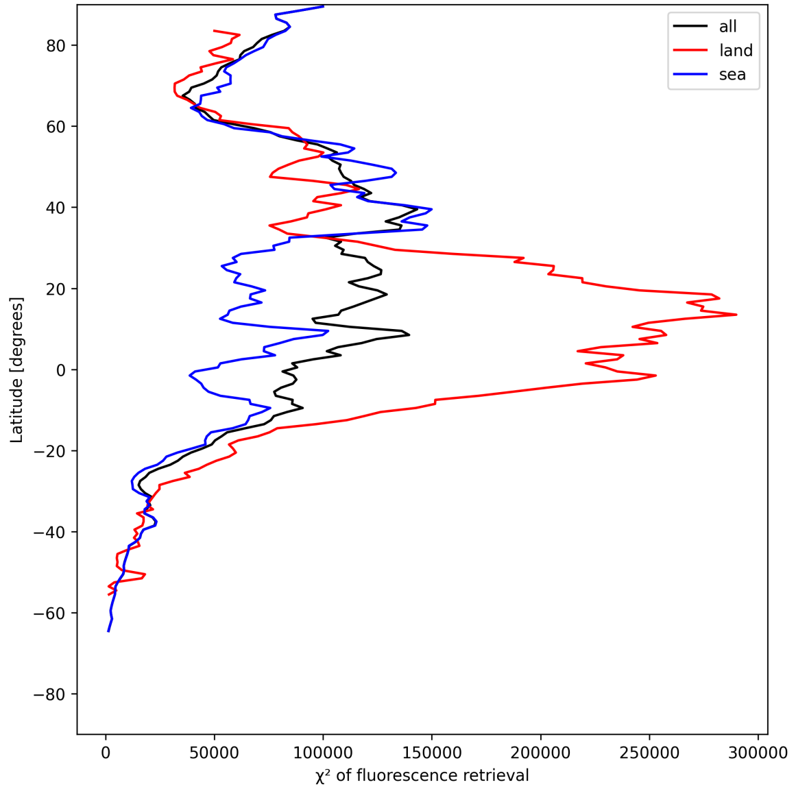
Figure 25: Zonal average of “ \chi^2 of fluorescence retrieval” for 2025-06-17 to 2025-06-19.
