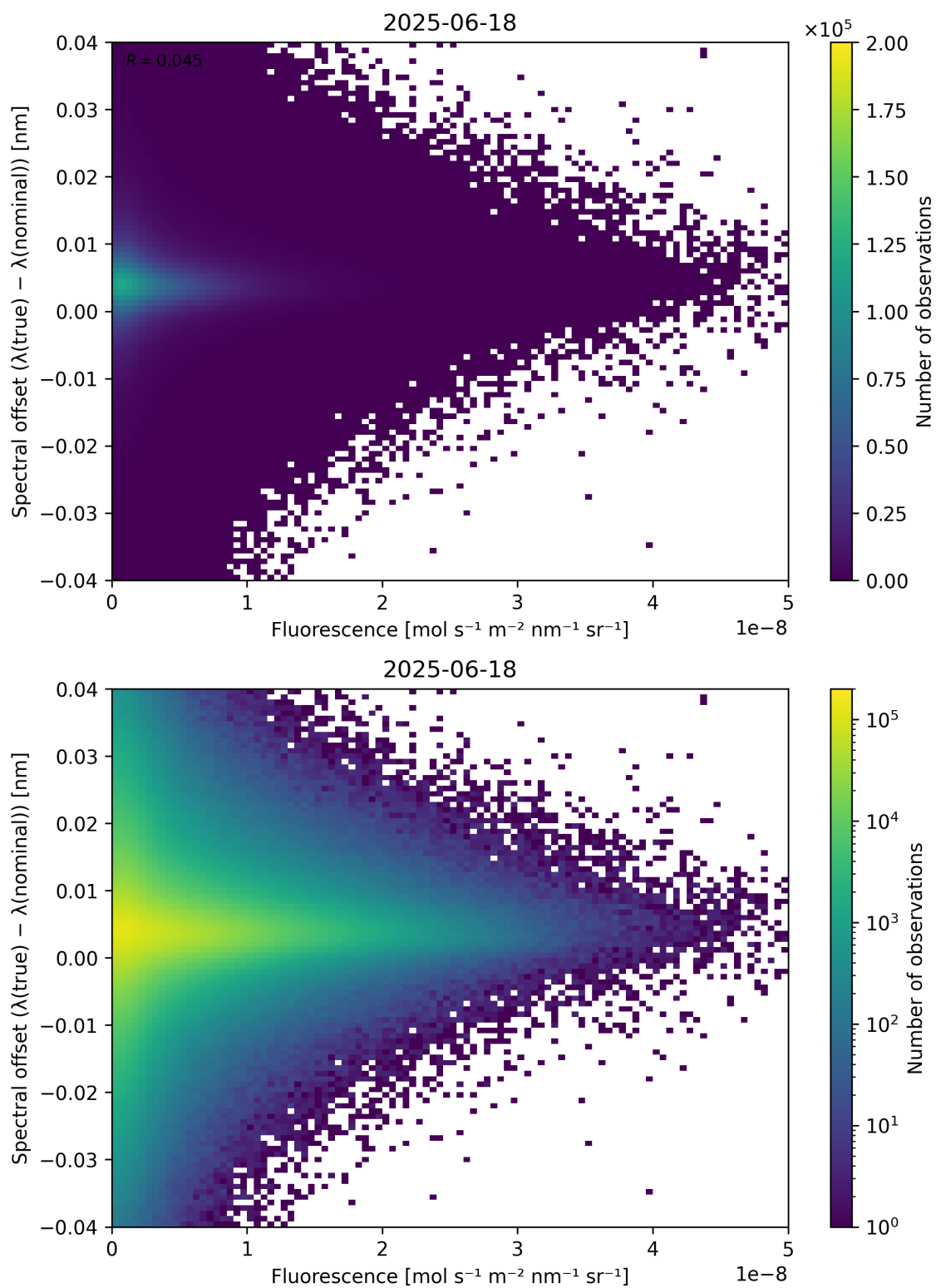
Figure 87: Scatter density plot of “Fluorescence” against “Spectral offset ( \lambda_{\text{true}} - \lambda_{\text{nominal}} )” for 2025-06-17 to 2025-06-19.
