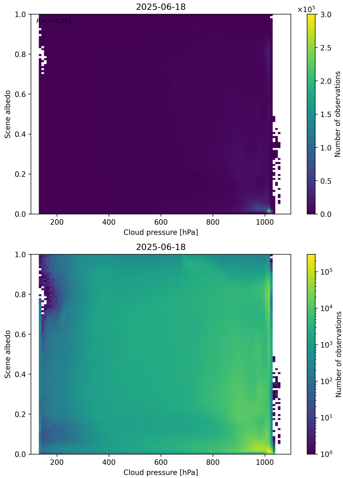
Figure 83: Scatter density plot of “Cloud pressure” against “Scene albedo” for 2025-06-17 to 2025-06-19.
