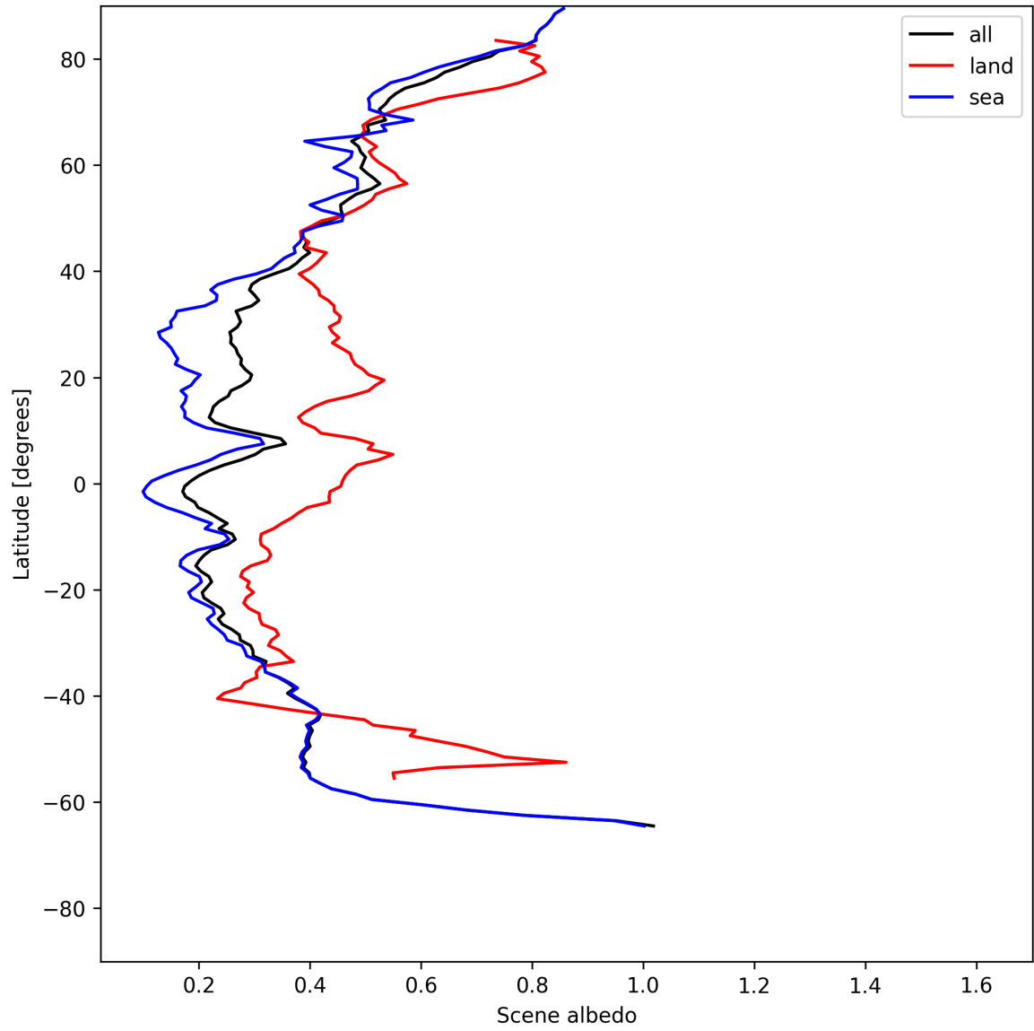
Figure 17: Zonal average of “Scene albedo” for 2025-06-17 to 2025-06-19.
