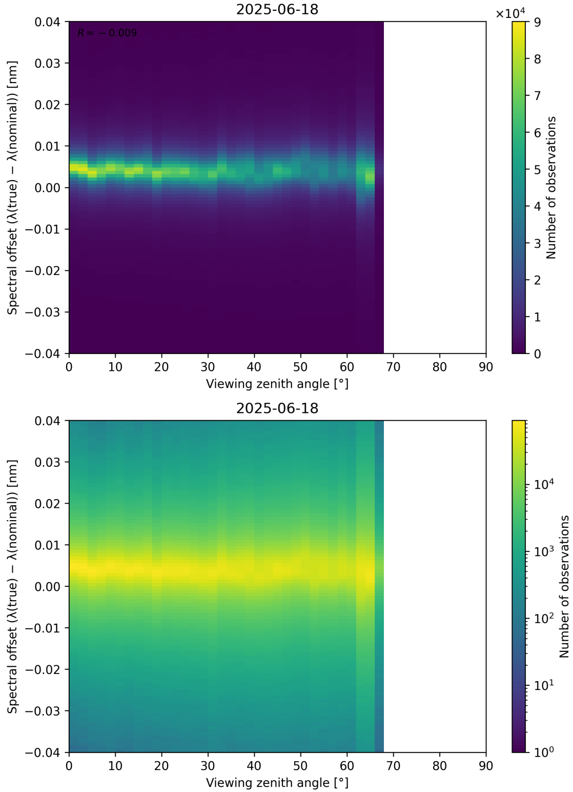
Figure 128: Scatter density plot of “Viewing zenith angle” against “Spectral offset ( \lambda_{\text{true}} - \lambda_{\text{nominal}} )” for 2025-06-17 to 2025-06-19.
