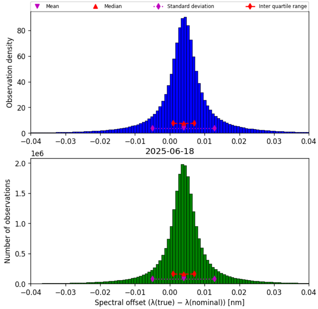
Figure 45: Histogram of “Spectral offset ( \lambda_{\text{true}} - \lambda_{\text{nominal}} )” for 2025-06-17 to 2025-06-19
