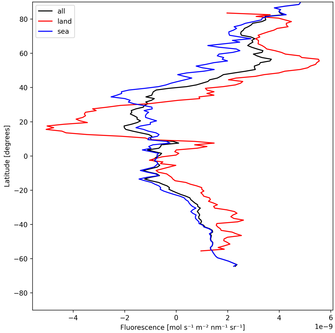
Figure 23: Zonal average of “Fluorescence” for 2025-06-17 to 2025-06-19.
