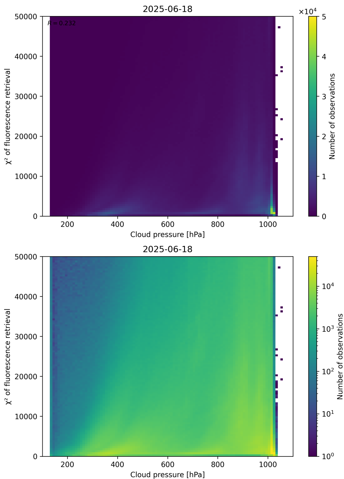
Figure 78: Scatter density plot of “Cloud pressure” against “ \chi^2 of fluorescence retrieval” for 2025-06-17 to 2025-06-19.
