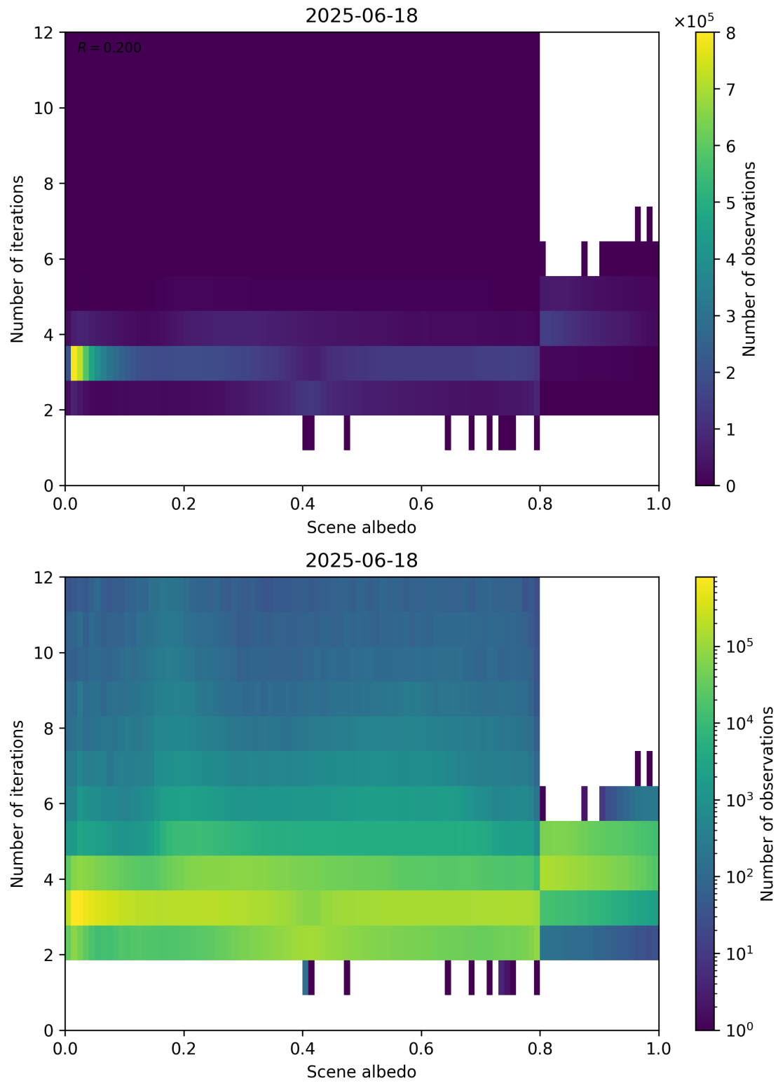
Figure 105: Scatter density plot of “Scene albedo” against “Number of iterations” for 2025-06-17 to 2025-06-19.
