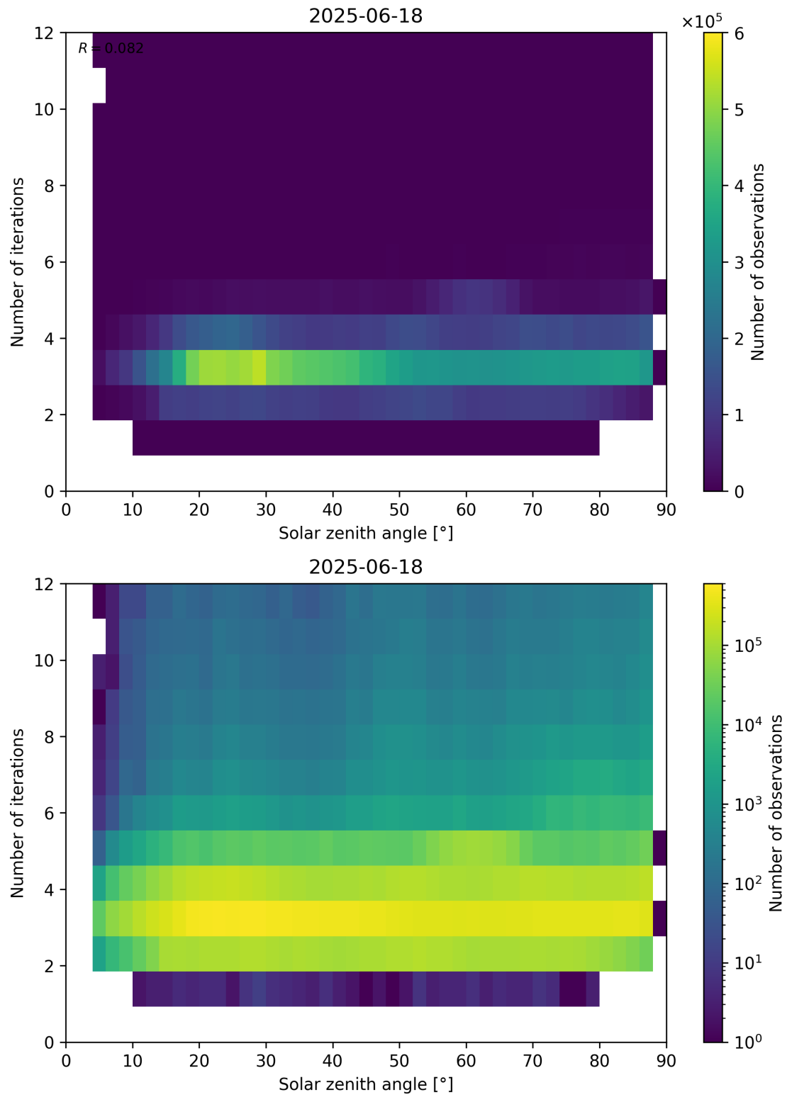
Figure 114: Scatter density plot of “Solar zenith angle” against “Number of iterations” for 2025-06-17 to 2025-06-19.
