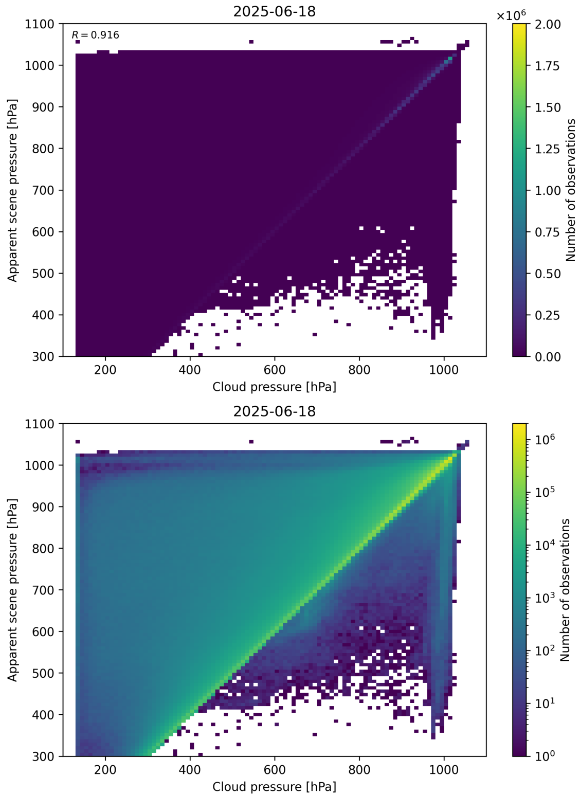
Figure 77: Scatter density plot of “Cloud pressure” against “Apparent scene pressure” for 2025-06-17 to 2025-06-19.
