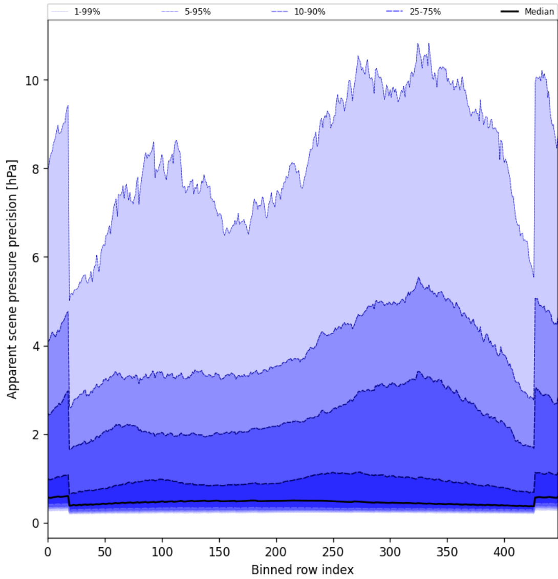
Figure 54: Along track statistics of “Apparent scene pressure precision” for 2025-06-17 to 2025-06-19
