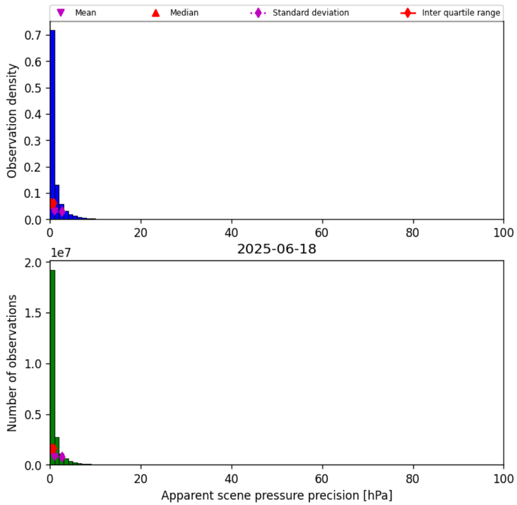
Figure 37: Histogram of "Apparent scene pressure precision" for 2025-06-17 to 2025-06-19
