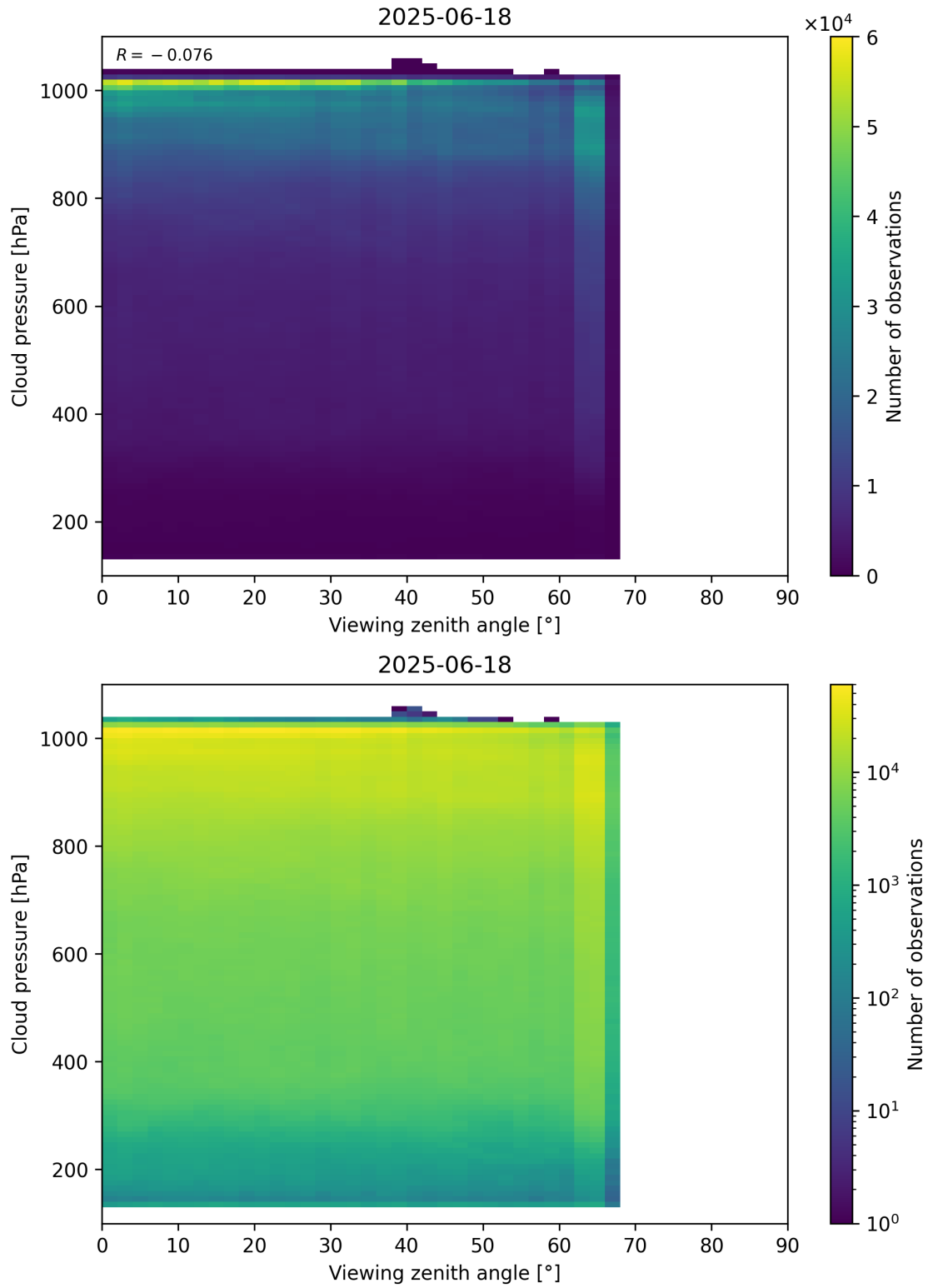
Figure 121: Scatter density plot of “Viewing zenith angle” against “Cloud pressure” for 2025-06-17 to 2025-06-19.
