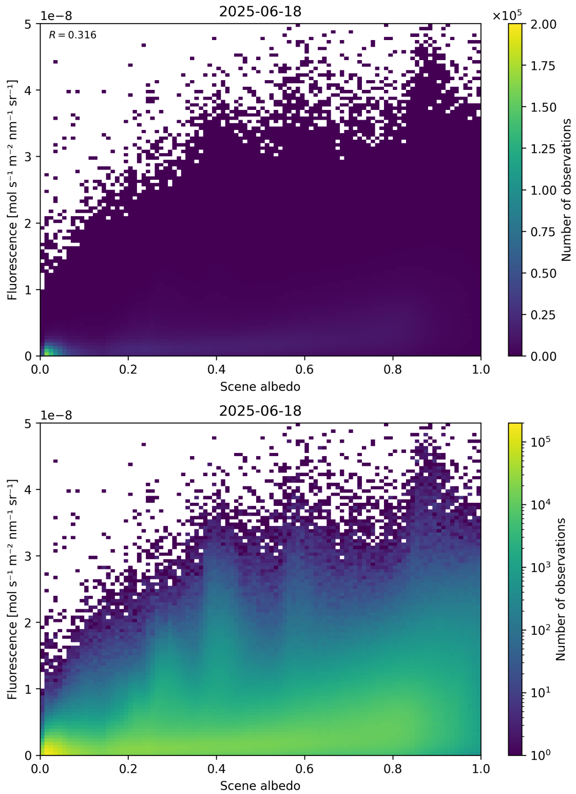
Figure 104: Scatter density plot of “Scene albedo” against “Fluorescence” for 2025-06-17 to 2025-06-19.
