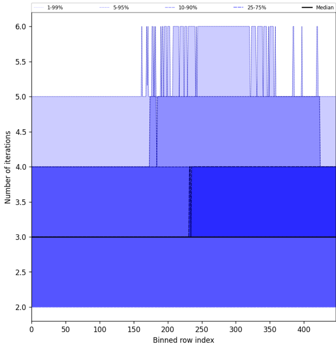
Figure 56: Along track statistics of “Number of iterations” for 2025-06-17 to 2025-06-19
