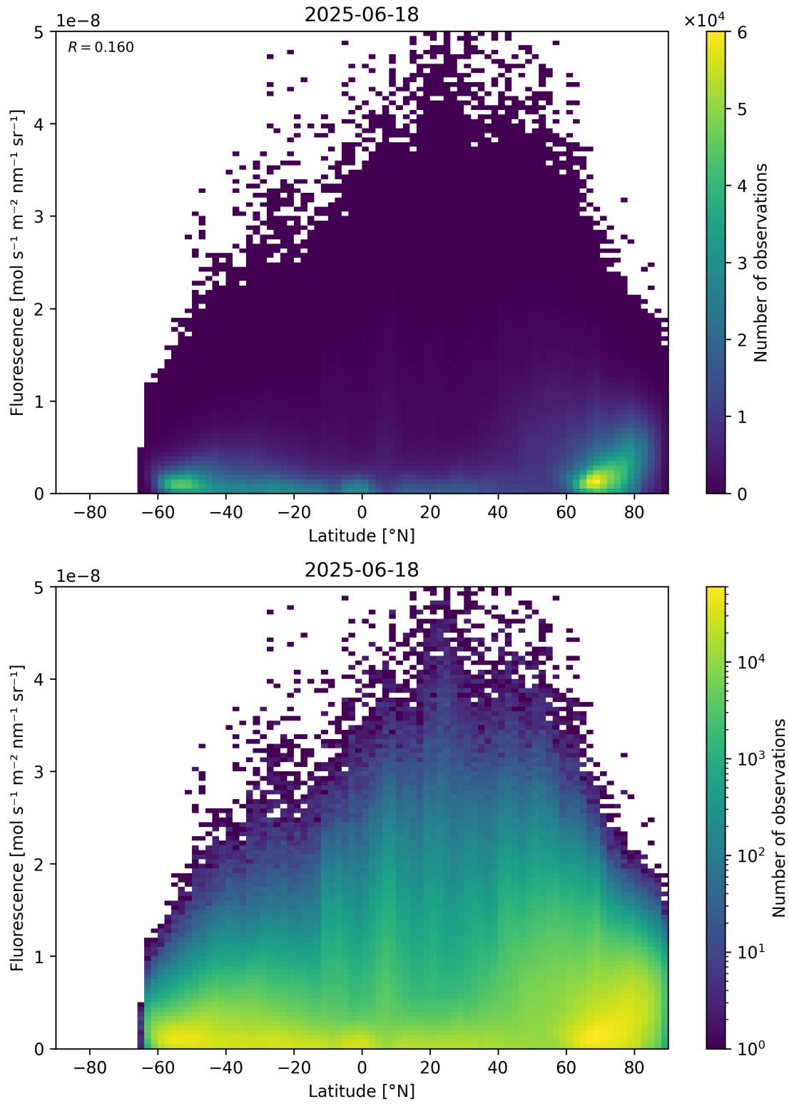
Figure 92: Scatter density plot of “Latitude” against “Fluorescence” for 2025-06-17 to 2025-06-19.
