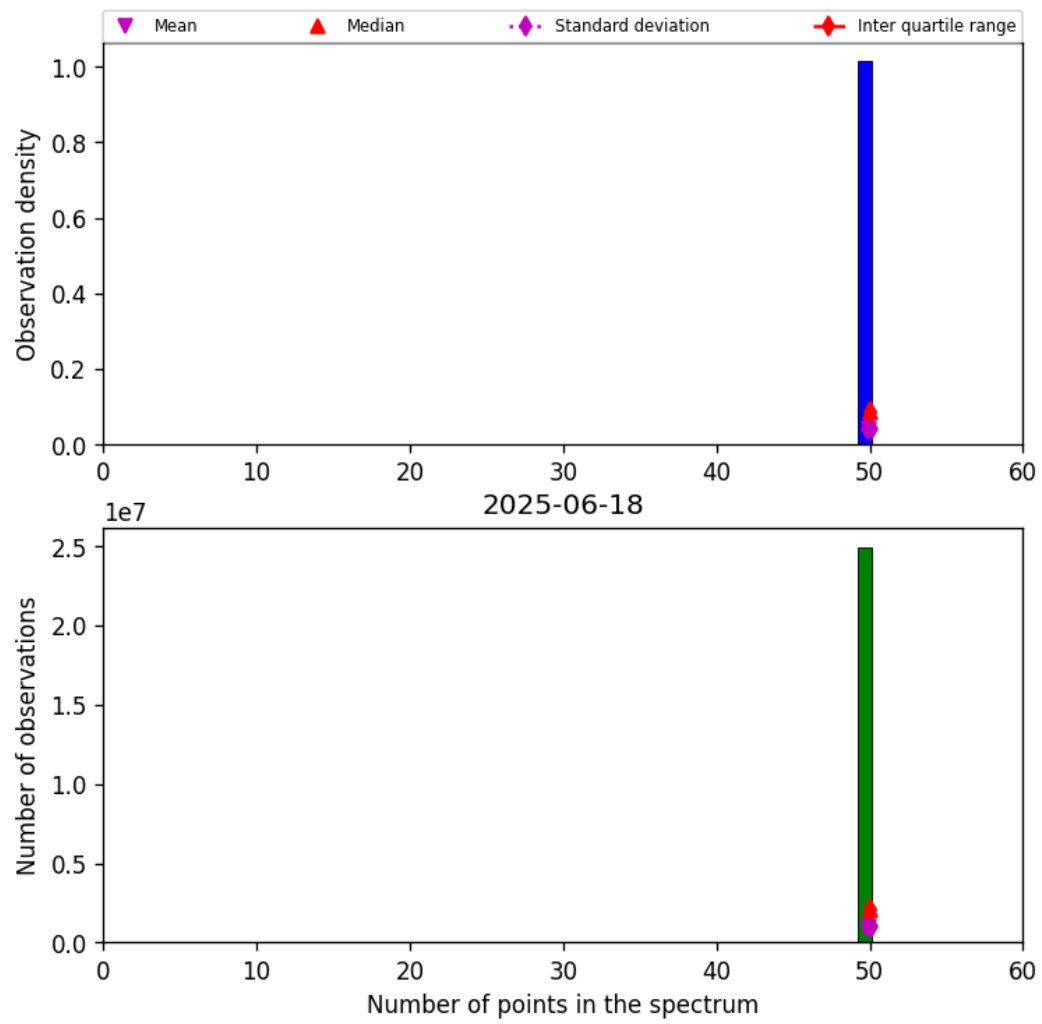
Figure 44: Histogram of “Number of points in the spectrum” for 2025-06-17 to 2025-06-19
