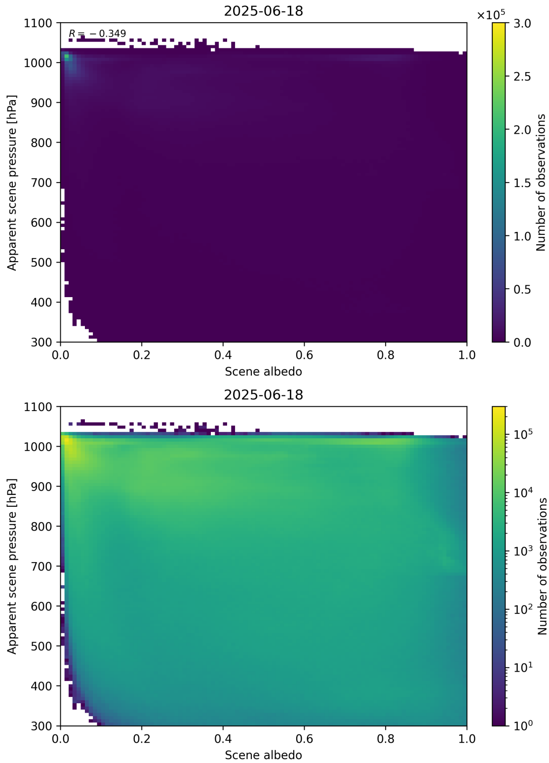
Figure 102: Scatter density plot of “Scene albedo” against “Apparent scene pressure” for 2025-06-17 to 2025-06-19.
