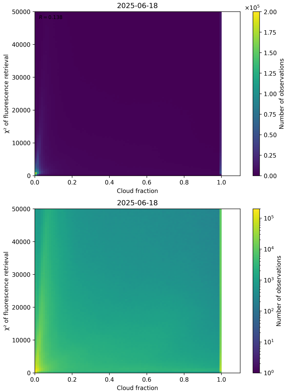
Figure 71: Scatter density plot of “Cloud fraction” against “ \chi^2 of fluorescence retrieval” for 2025-06-17 to 2025-06-19.
