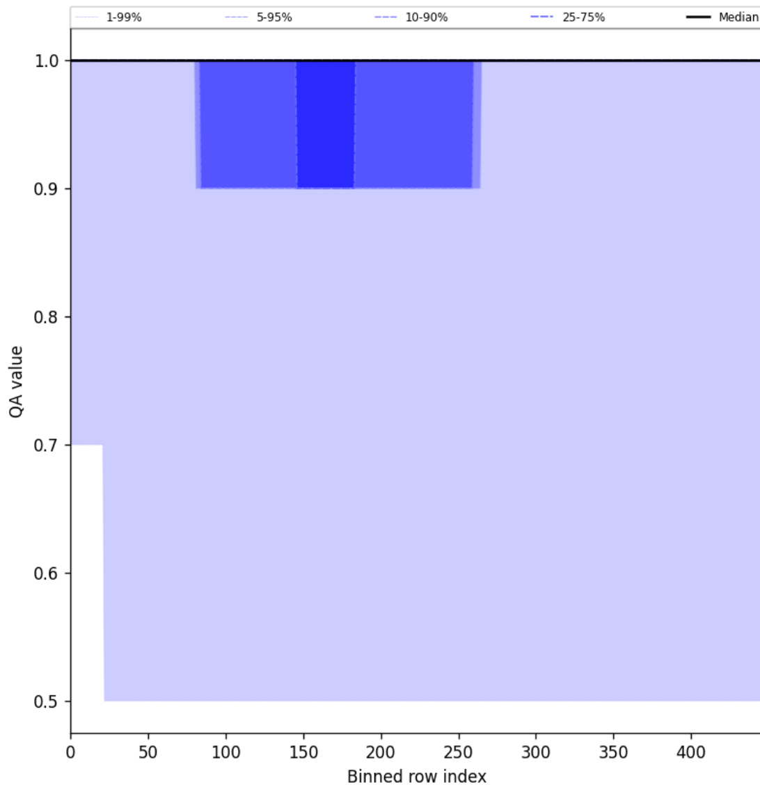
Figure 46: Along track statistics of “QA value” for 2025-06-17 to 2025-06-19
