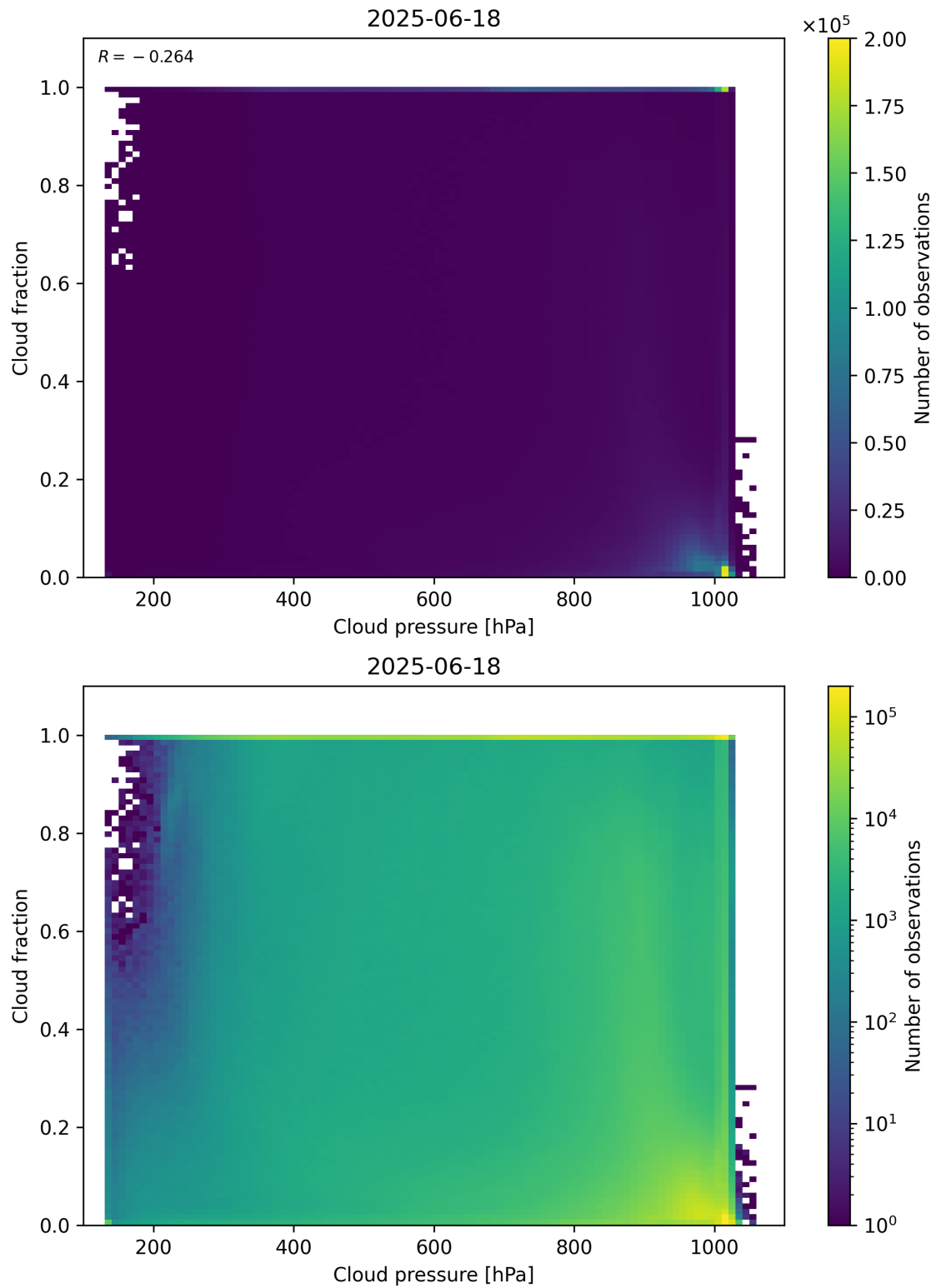
Figure 79: Scatter density plot of “Cloud pressure” against “Cloud fraction” for 2025-06-17 to 2025-06-19.
