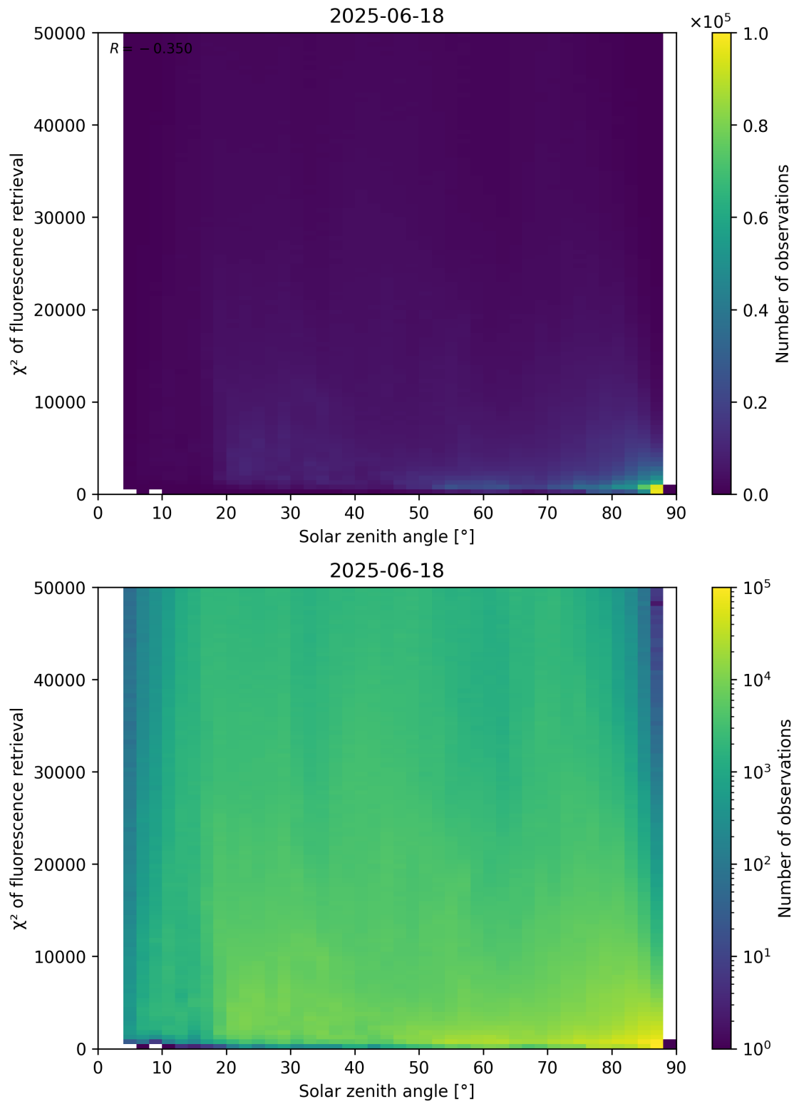
Figure 109: Scatter density plot of “Solar zenith angle” against “ \chi^2 of fluorescence retrieval” for 2025-06-17 to 2025-06-19.
