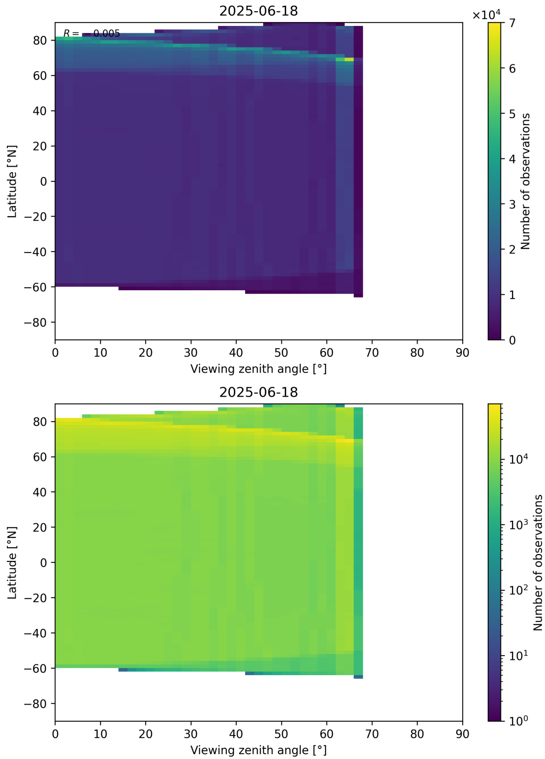
Figure 123: Scatter density plot of “Viewing zenith angle” against “Latitude” for 2025-06-17 to 2025-06-19.
