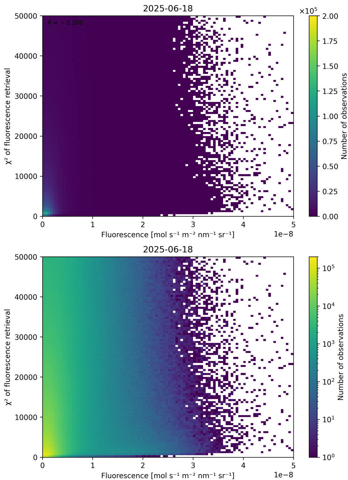
Figure 85: Scatter density plot of “Fluorescence” against “ \chi^2 of fluorescence retrieval” for 2025-06-17 to 2025-06-19.
