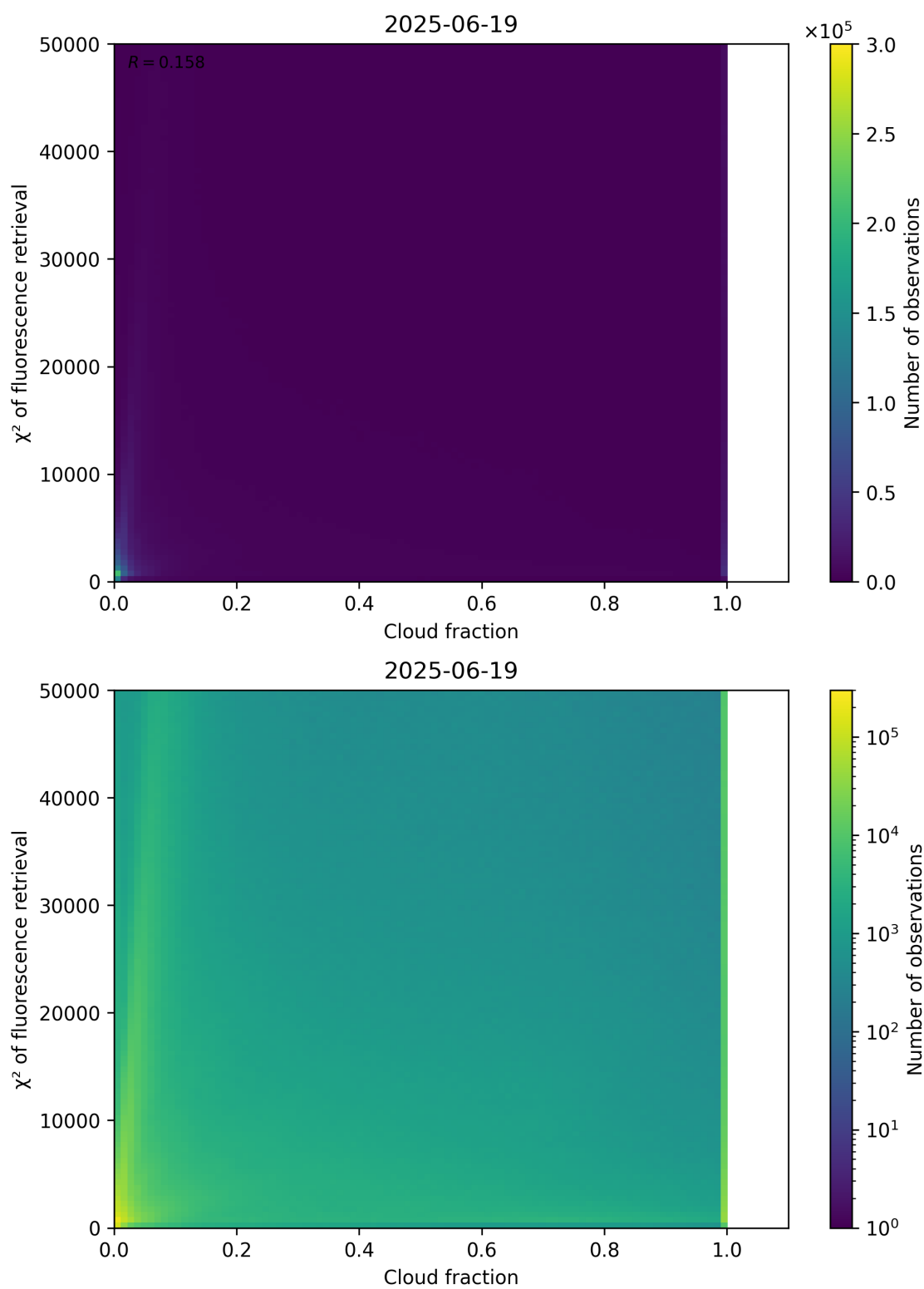
Figure 71: Scatter density plot of “Cloud fraction” against “ \chi^2 of fluorescence retrieval” for 2025-06-18 to 2025-06-20.
