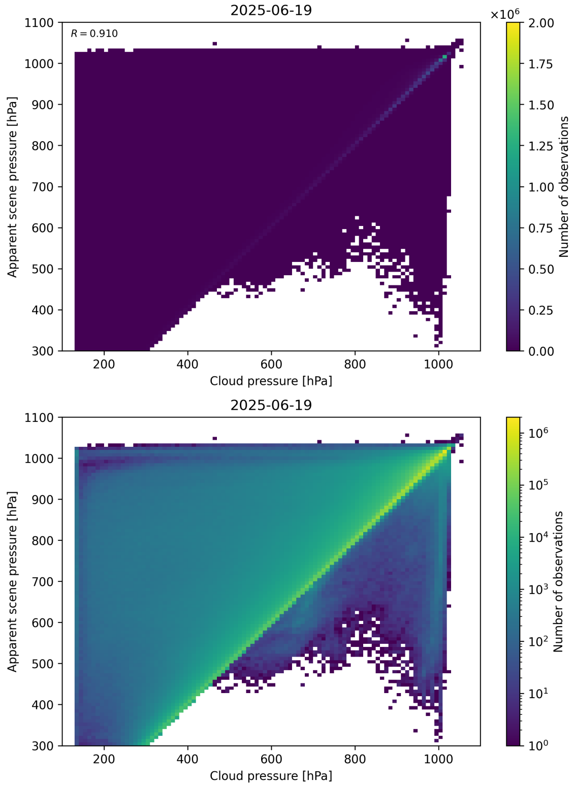
Figure 77: Scatter density plot of “Cloud pressure” against “Apparent scene pressure” for 2025-06-18 to 2025-06-20.
