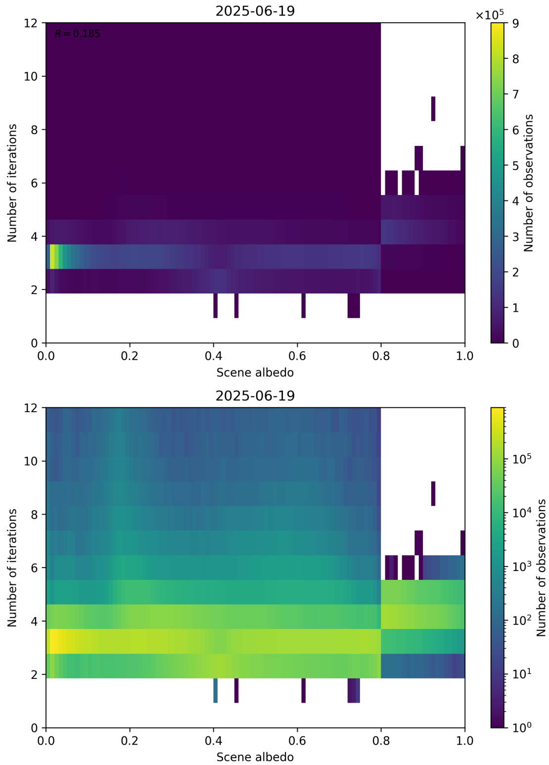
Figure 105: Scatter density plot of “Scene albedo” against “Number of iterations” for 2025-06-18 to 2025-06-20.
