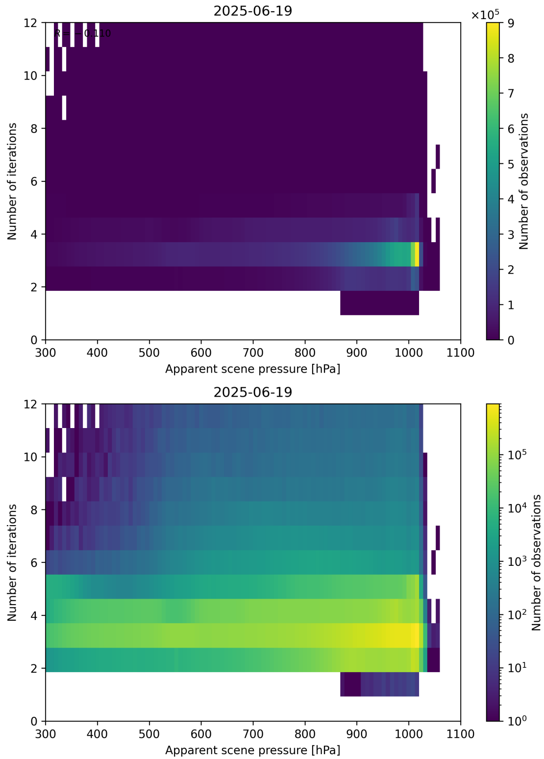
Figure 65: Scatter density plot of “Apparent scene pressure” against “Number of iterations” for 2025-06-18 to 2025-06-20.
