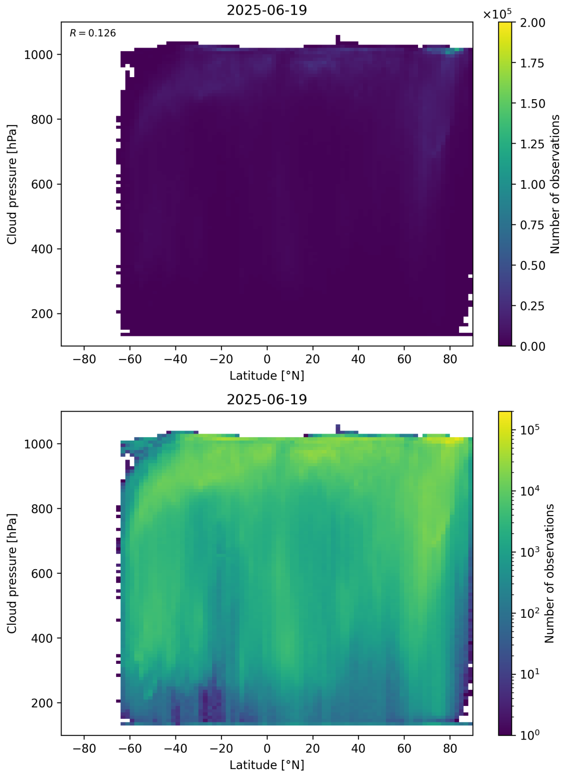
Figure 91: Scatter density plot of “Latitude” against “Cloud pressure” for 2025-06-18 to 2025-06-20.
