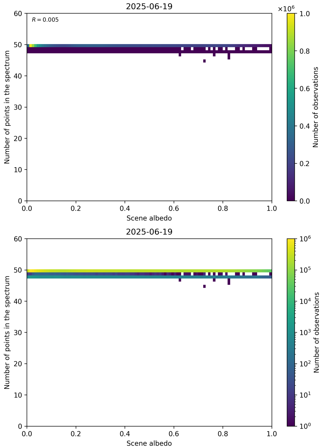
Figure 106: Scatter density plot of “Scene albedo” against “Number of points in the spectrum” for 2025-06-18 to 2025-06-20.
