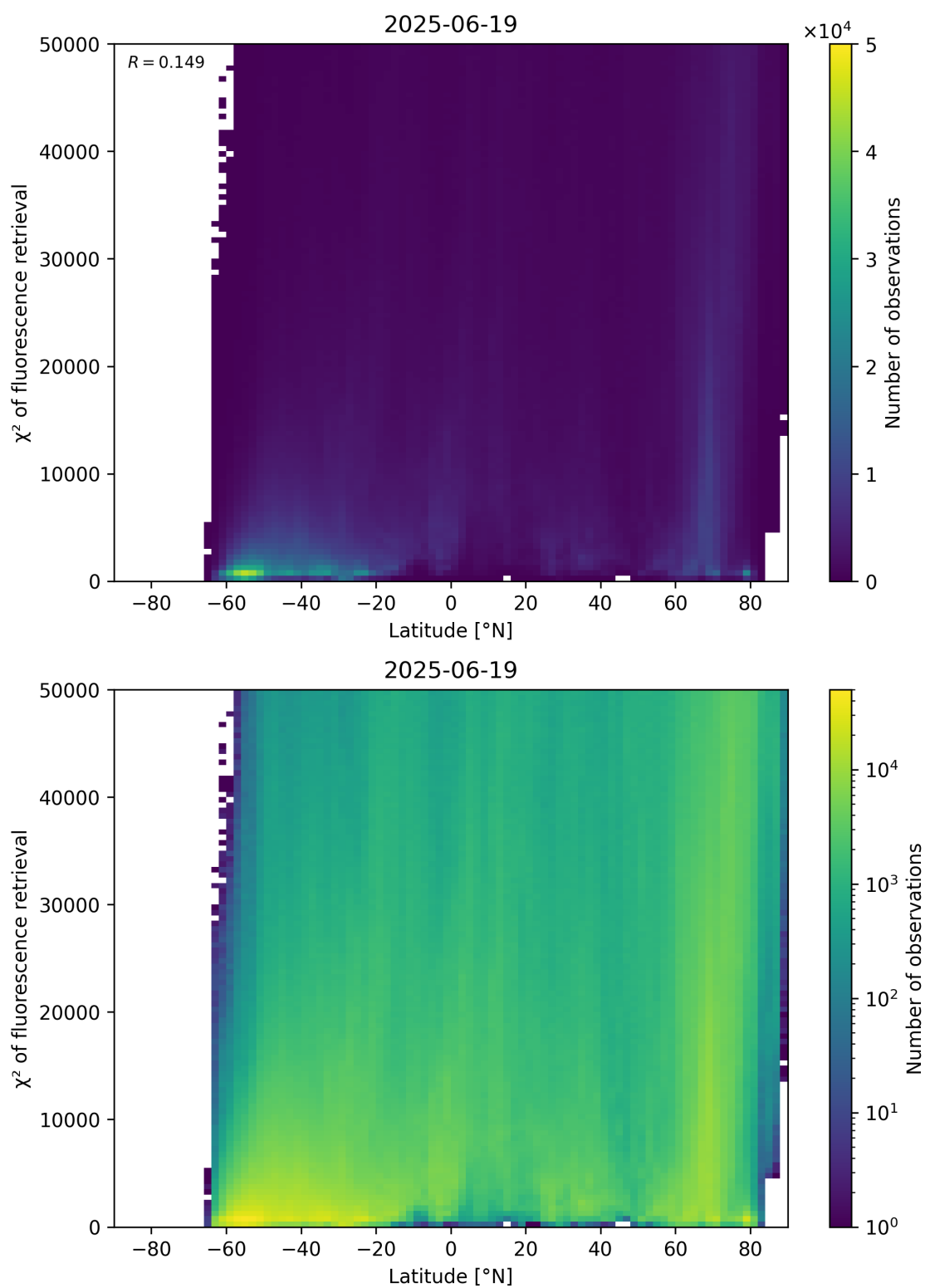
Figure 89: Scatter density plot of “Latitude” against “ \chi^2 of fluorescence retrieval” for 2025-06-18 to 2025-06-20.
