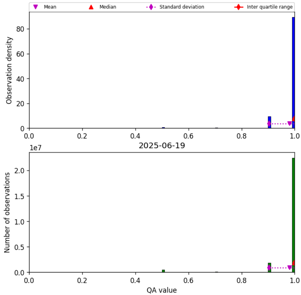
Figure 29: Histogram of “QA value” for 2025-06-18 to 2025-06-20
