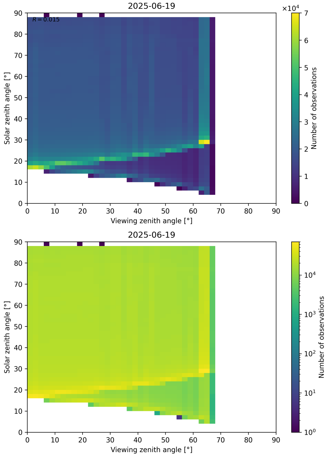
Figure 127: Scatter density plot of “Viewing zenith angle” against “Solar zenith angle” for 2025-06-18 to 2025-06-20.
