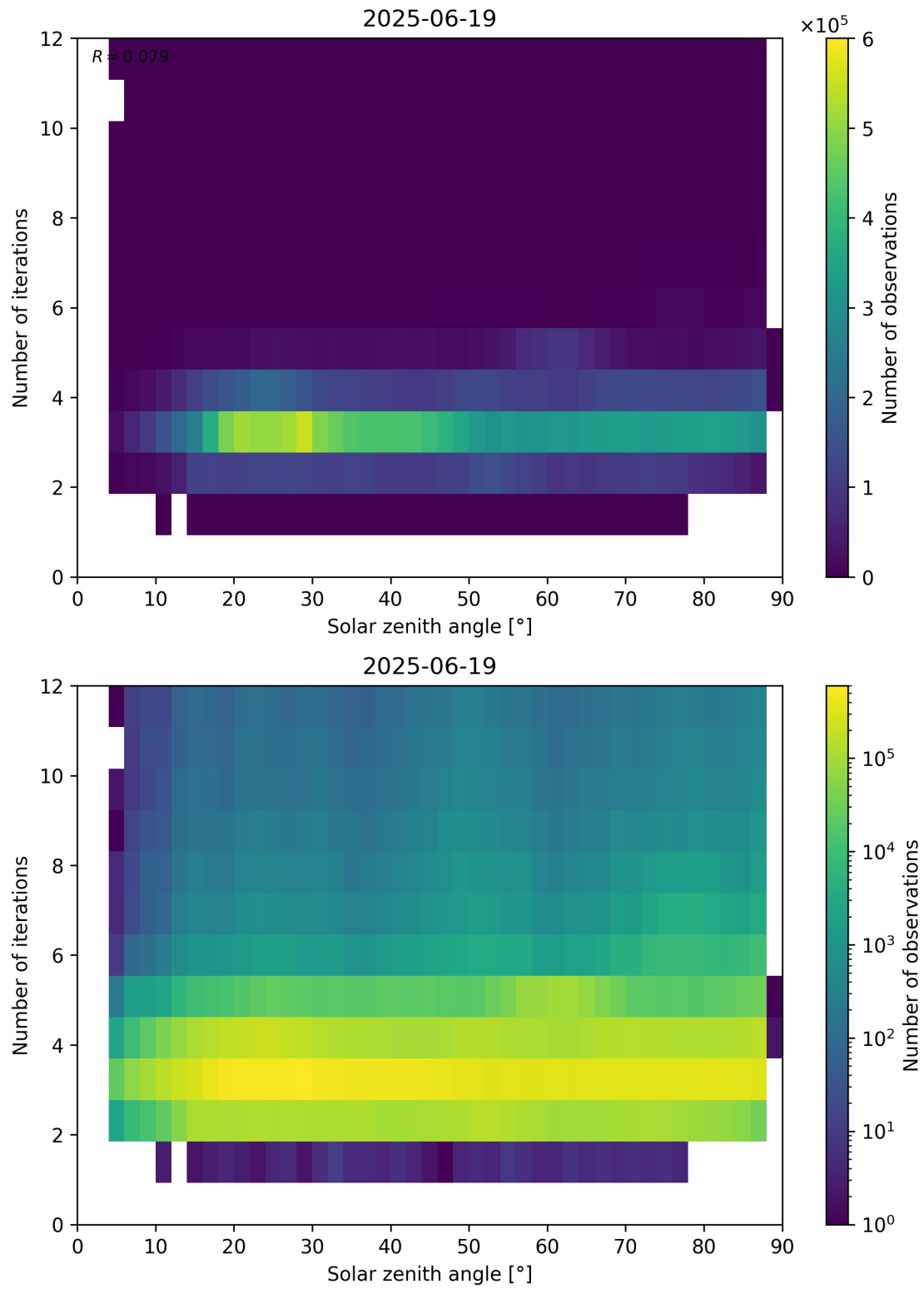
Figure 114: Scatter density plot of “Solar zenith angle” against “Number of iterations” for 2025-06-18 to 2025-06-20.
