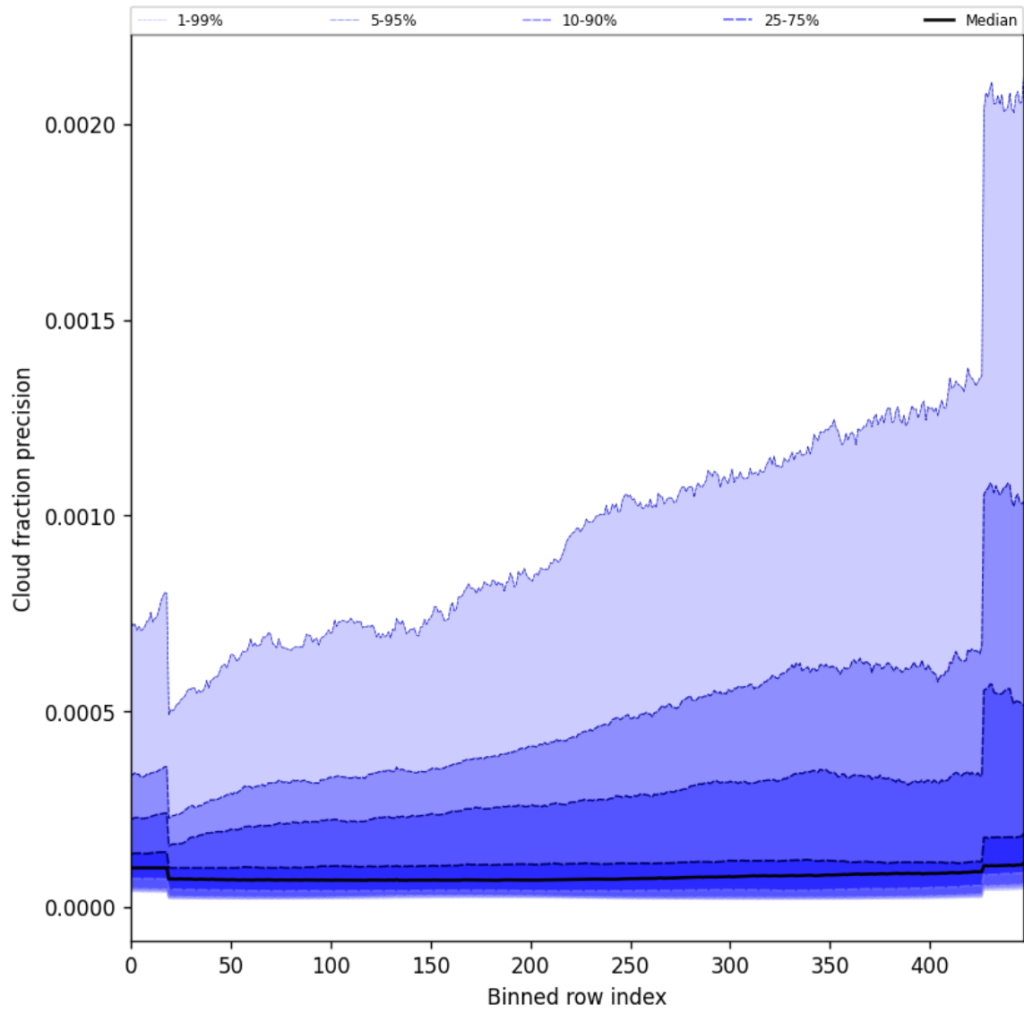
Figure 50: Along track statistics of “Cloud fraction precision” for 2025-06-18 to 2025-06-20
