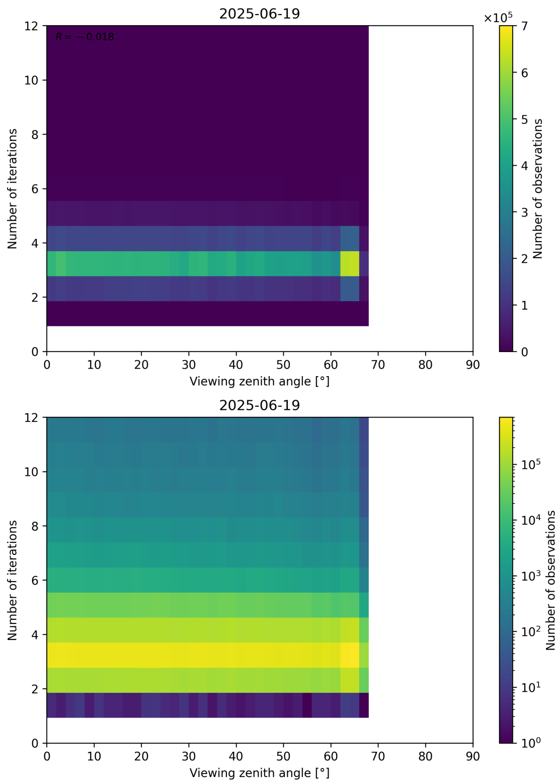
Figure 124: Scatter density plot of “Viewing zenith angle” against “Number of iterations” for 2025-06-18 to 2025-06-20.
