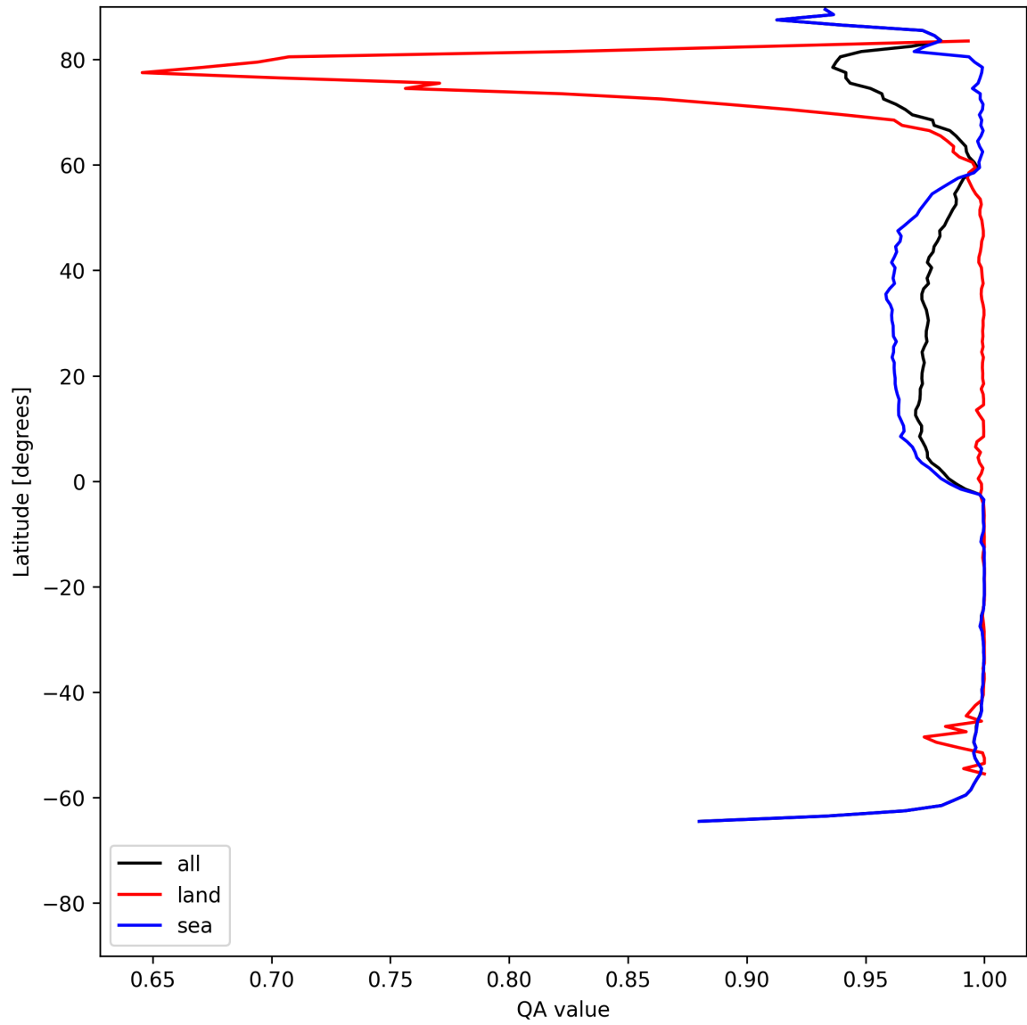
Figure 12: Zonal average of “QA value” for 2025-06-18 to 2025-06-20.
