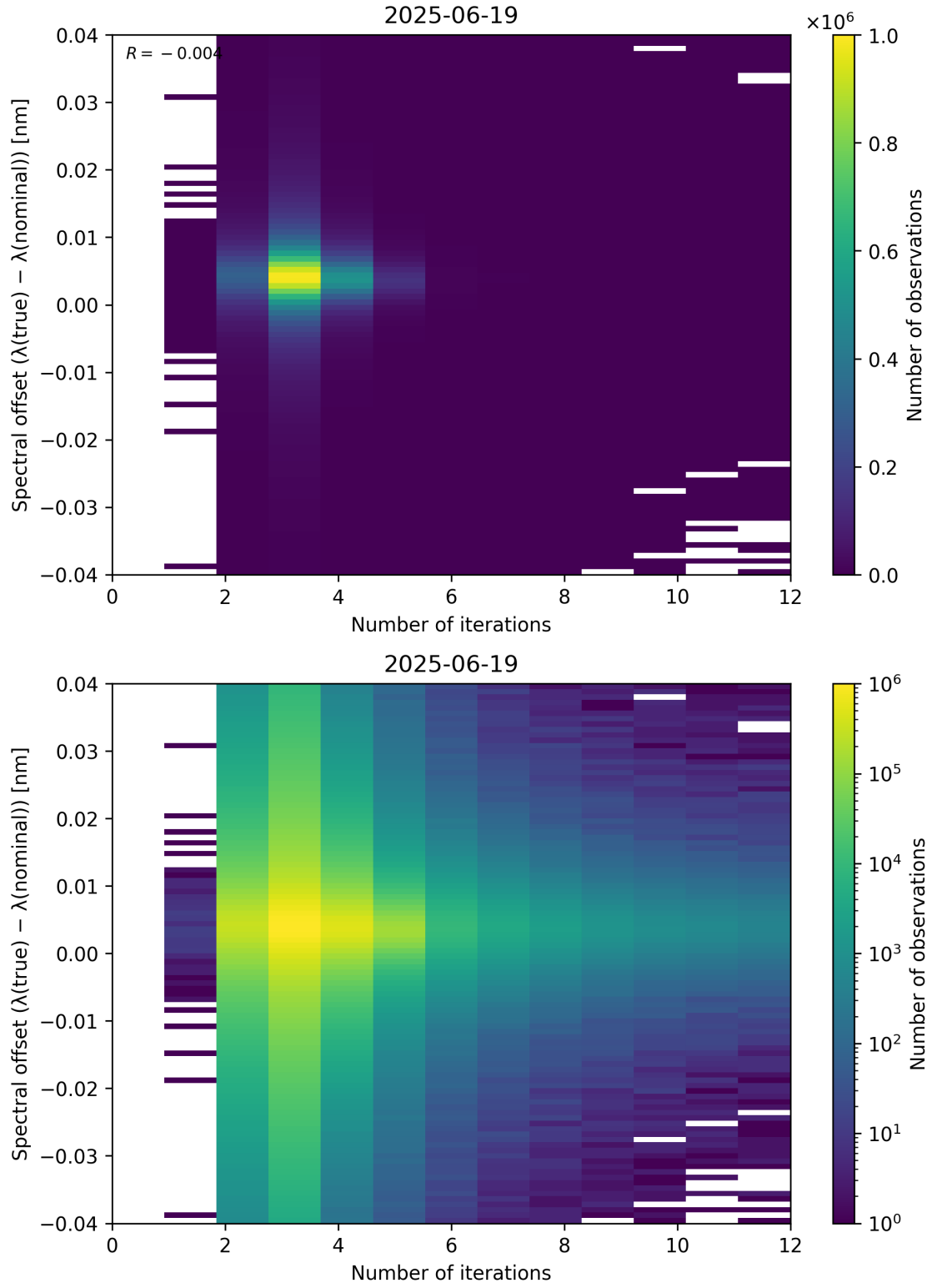
Figure 100: Scatter density plot of “Number of iterations” against “Spectral offset ( \lambda_{\text{true}} - \lambda_{\text{nominal}} )” for 2025-06-18 to 2025-06-20.
