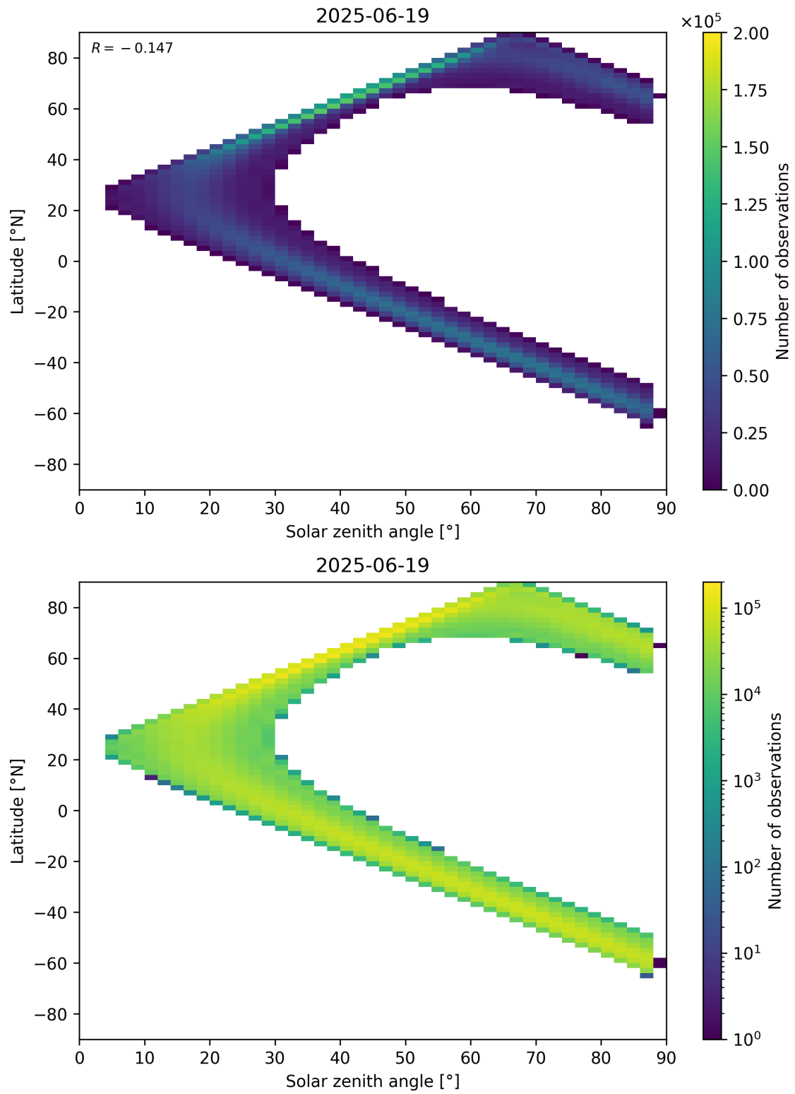
Figure 113: Scatter density plot of “Solar zenith angle” against “Latitude” for 2025-06-18 to 2025-06-20.
