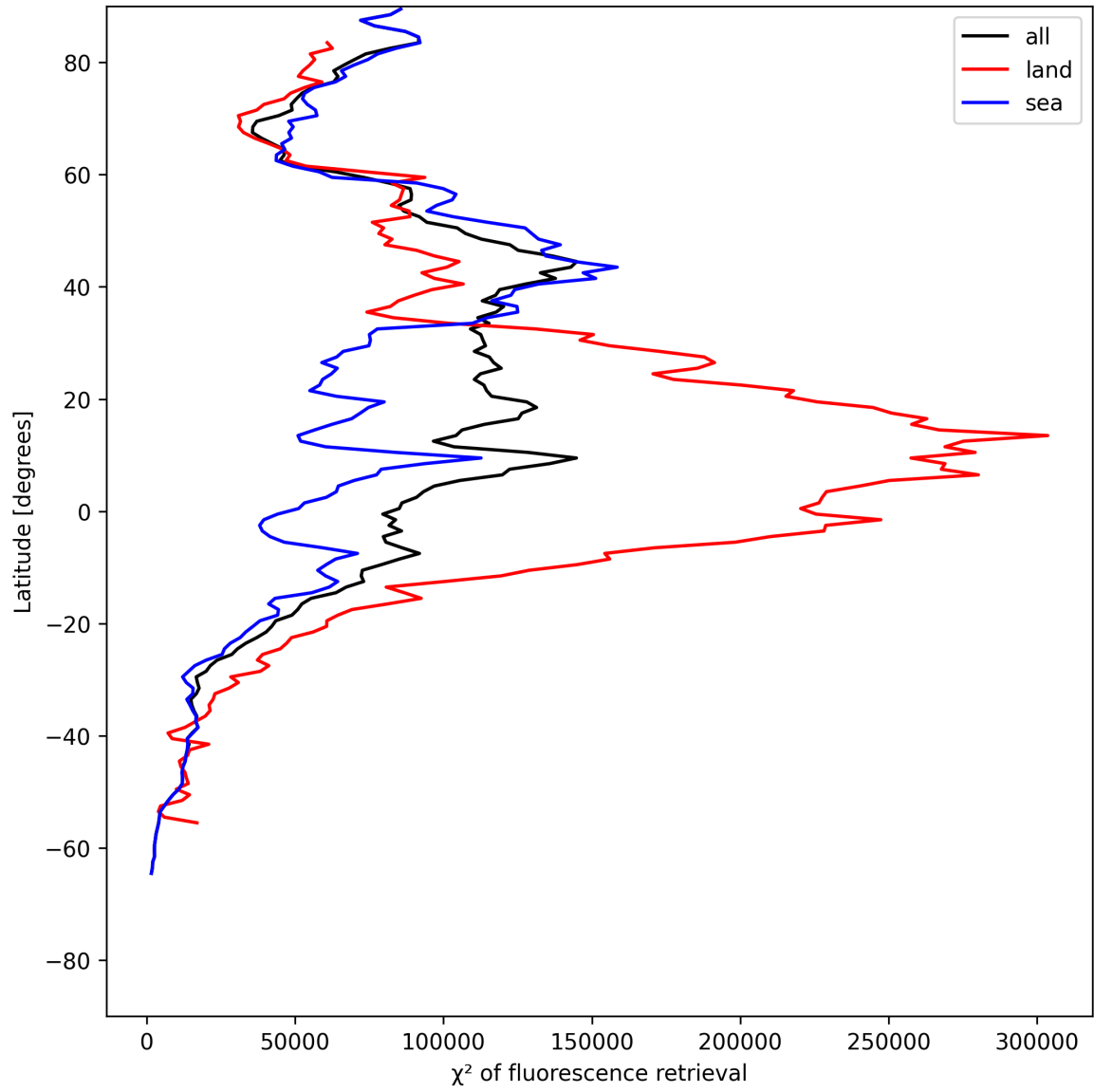
Figure 25: Zonal average of “ \chi^2 of fluorescence retrieval” for 2025-06-18 to 2025-06-20.
