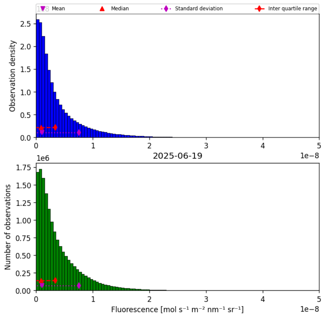
Figure 40: Histogram of “Fluorescence” for 2025-06-18 to 2025-06-20
