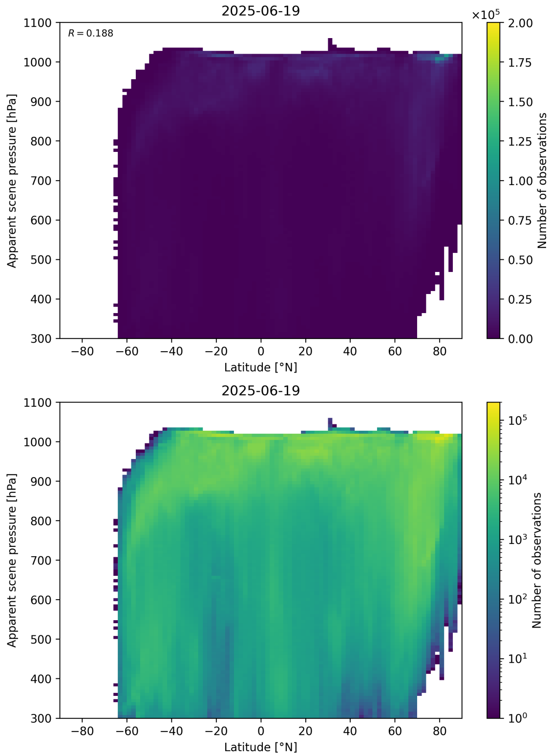
Figure 88: Scatter density plot of “Latitude” against “Apparent scene pressure” for 2025-06-18 to 2025-06-20.
