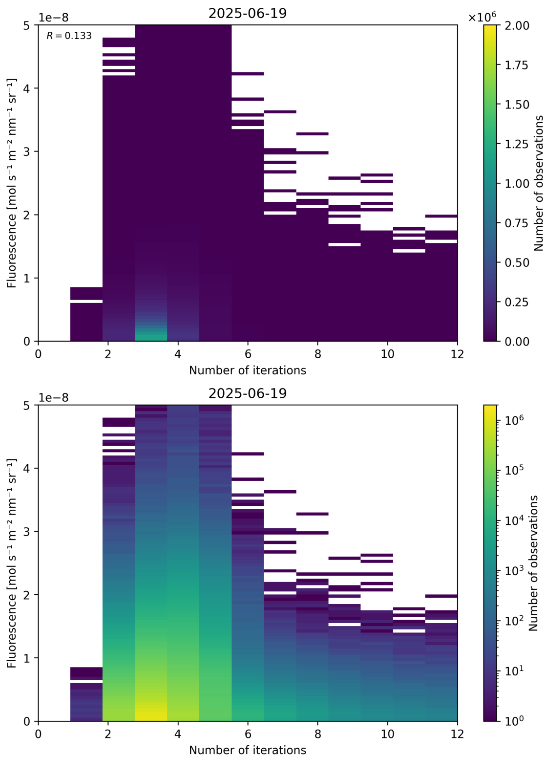
Figure 98: Scatter density plot of “Number of iterations” against “Fluorescence” for 2025-06-18 to 2025-06-20.
