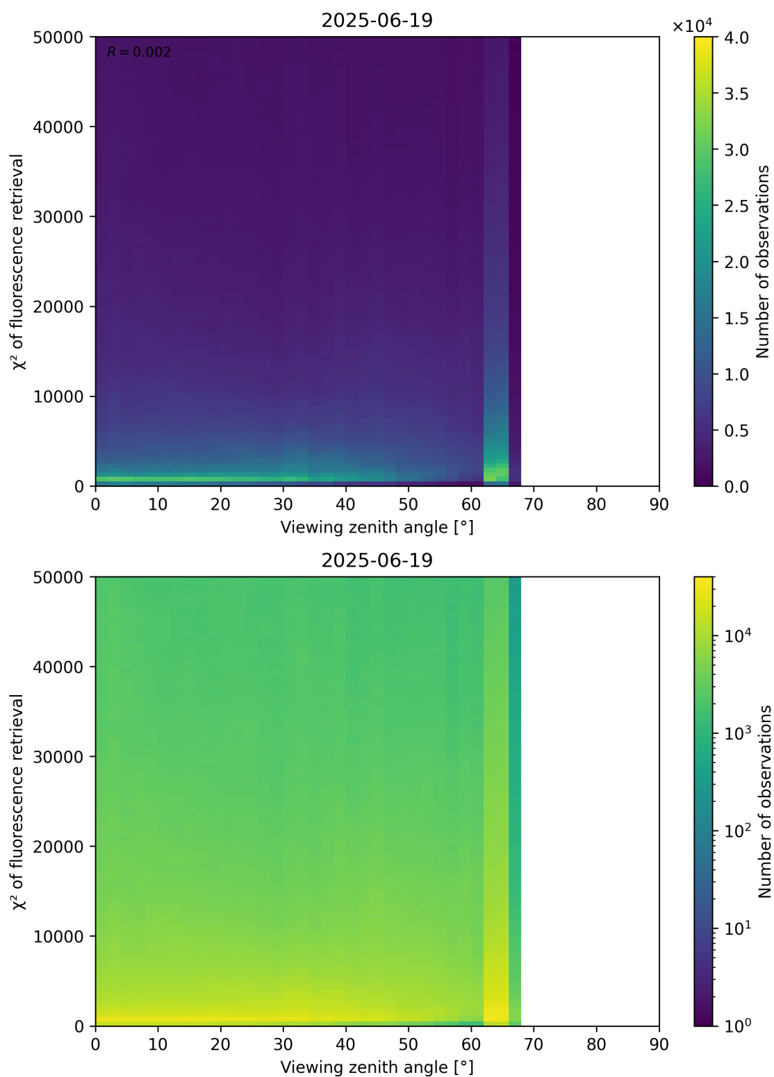
Figure 119: Scatter density plot of “Viewing zenith angle” against “ \chi^2 of fluorescence retrieval” for 2025-06-18 to 2025-06-20.
