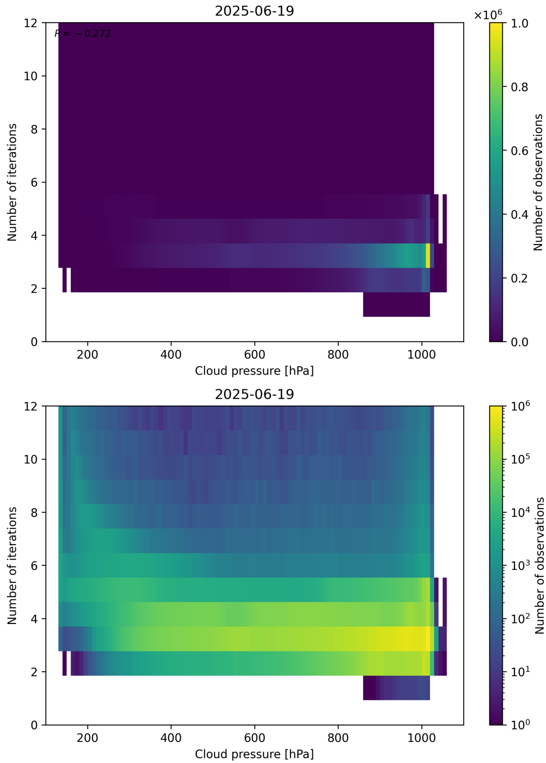
Figure 81: Scatter density plot of “Cloud pressure” against “Number of iterations” for 2025-06-18 to 2025-06-20.
