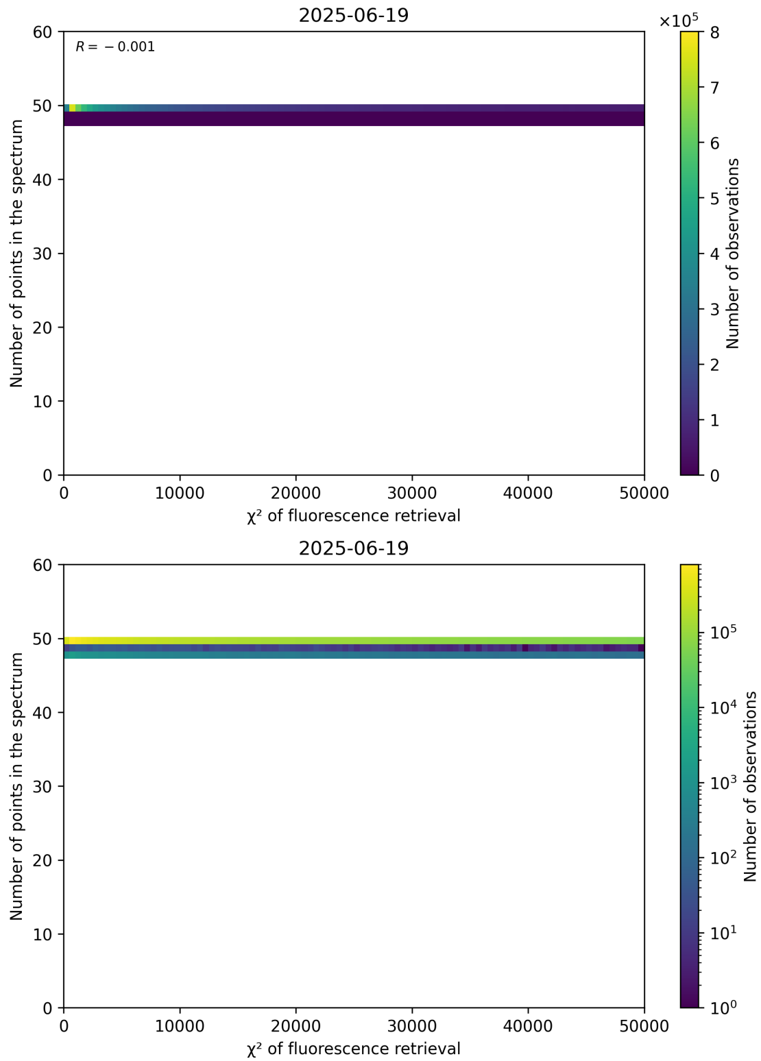
Figure 68: Scatter density plot of “ \chi^2 of fluorescence retrieval” against “Number of points in the spectrum” for 2025-06-18 to 2025-06-20.
