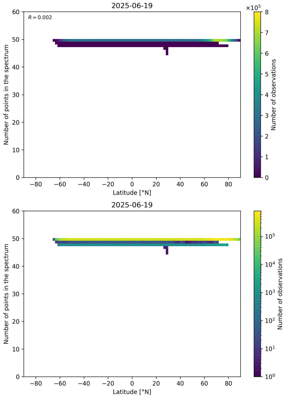
Figure 94: Scatter density plot of “Latitude” against “Number of points in the spectrum” for 2025-06-18 to 2025-06-20.
