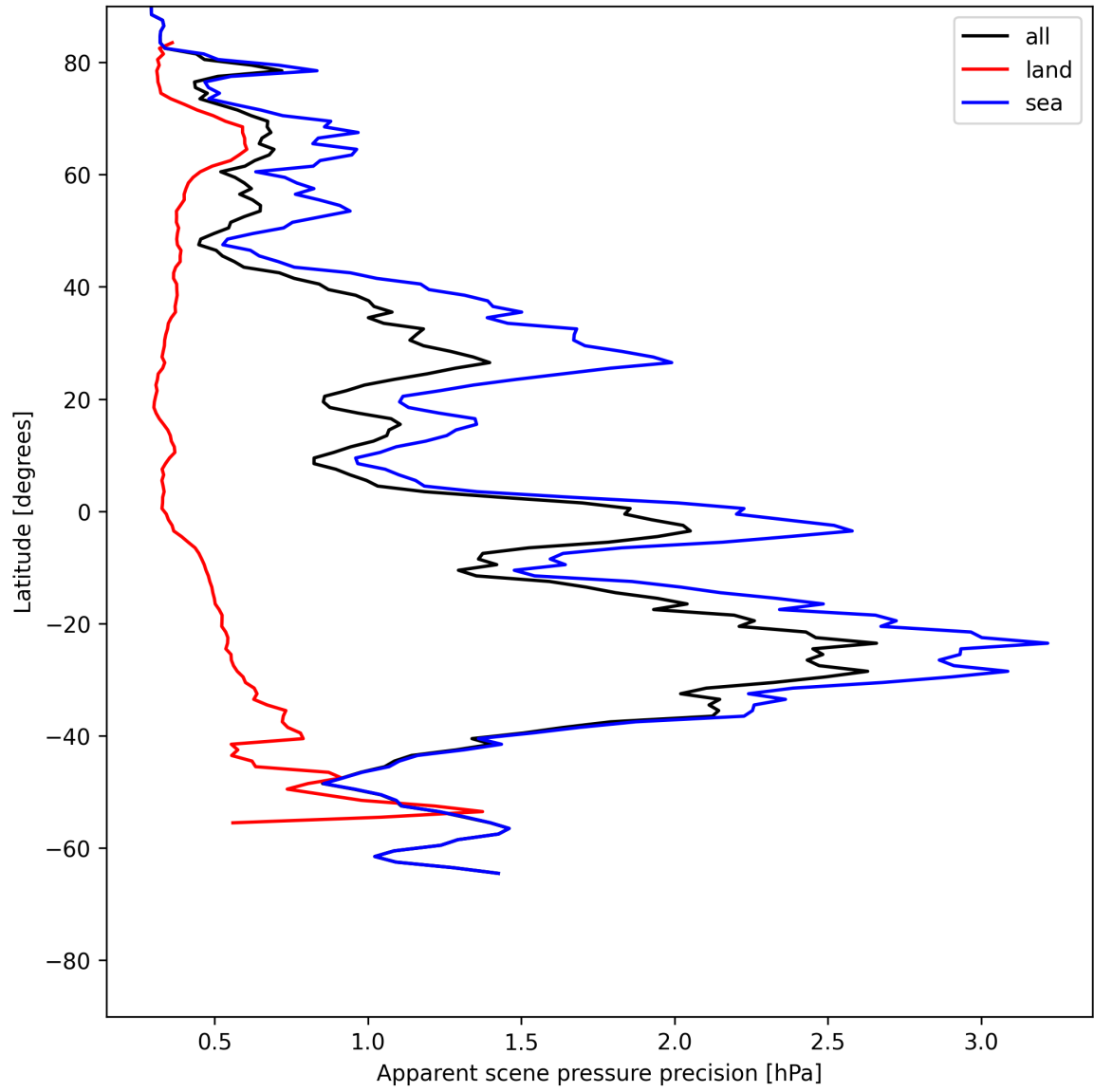
Figure 20: Zonal average of “Apparent scene pressure precision” for 2025-06-18 to 2025-06-20.
