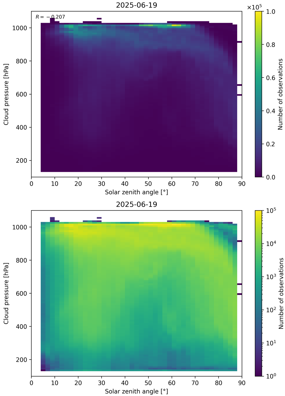
Figure 111: Scatter density plot of “Solar zenith angle” against “Cloud pressure” for 2025-06-18 to 2025-06-20.
