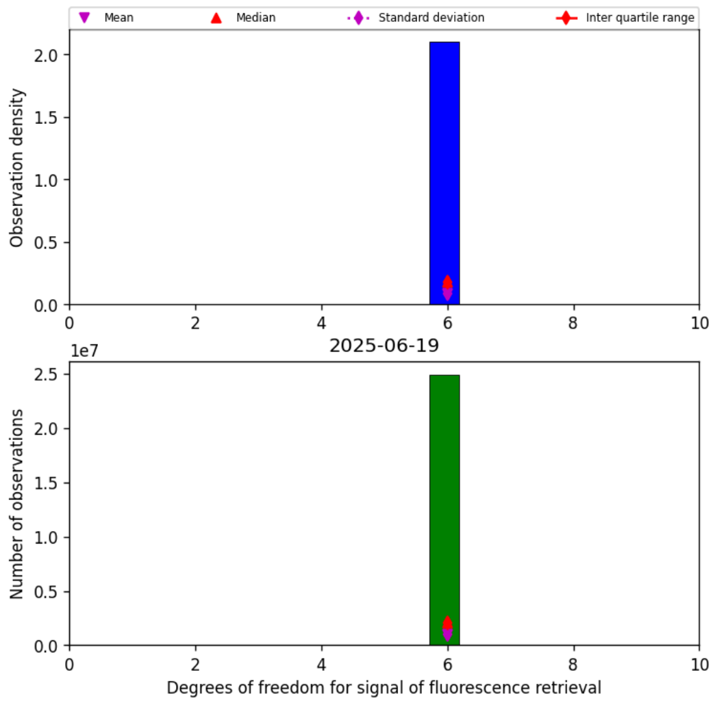
Figure 43: Histogram of "Degrees of freedom for signal of fluorescence retrieval" for 2025-06-18 to 2025-06-20
