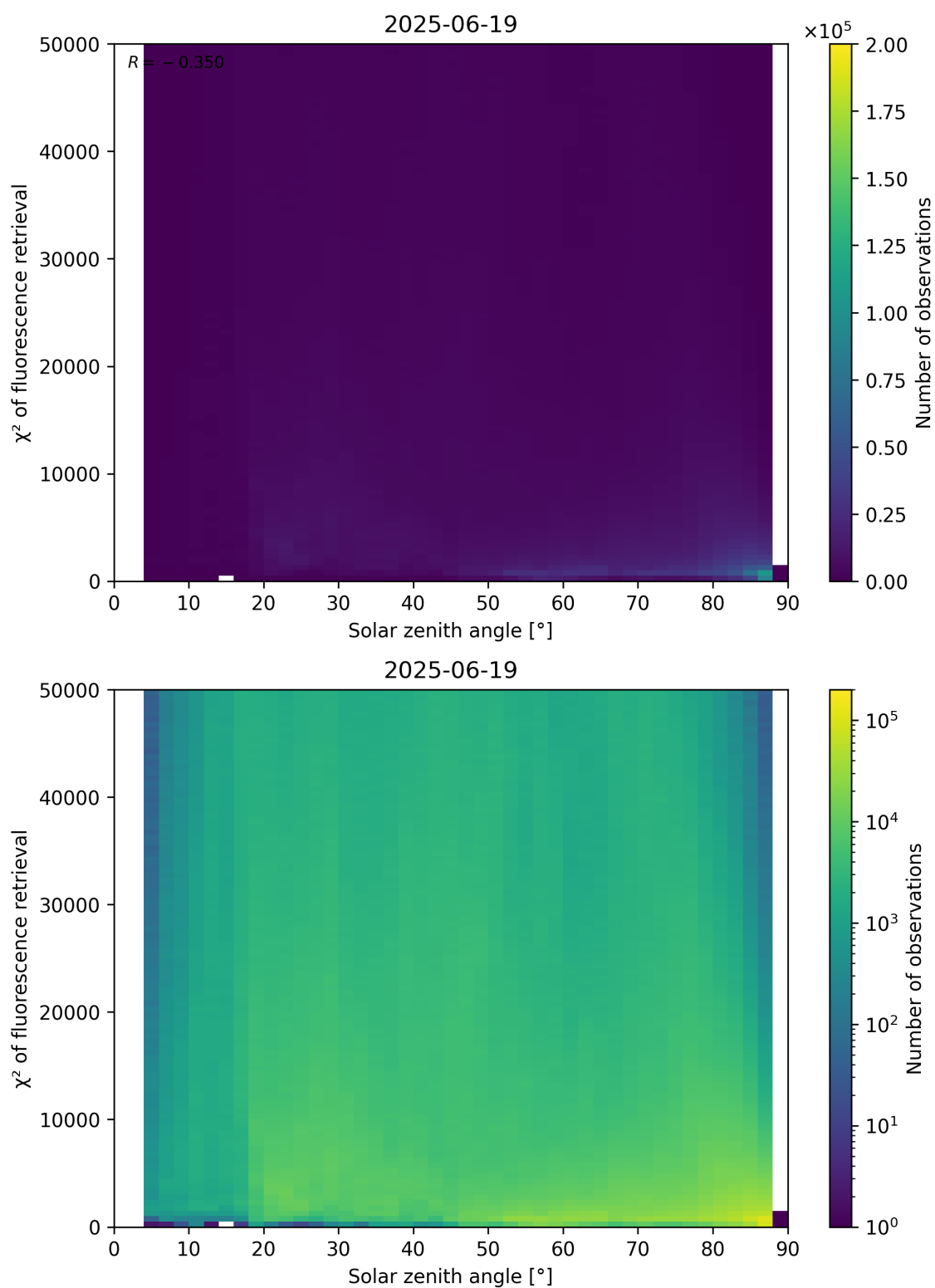
Figure 109: Scatter density plot of “Solar zenith angle” against “ \chi^2 of fluorescence retrieval” for 2025-06-18 to 2025-06-20.
