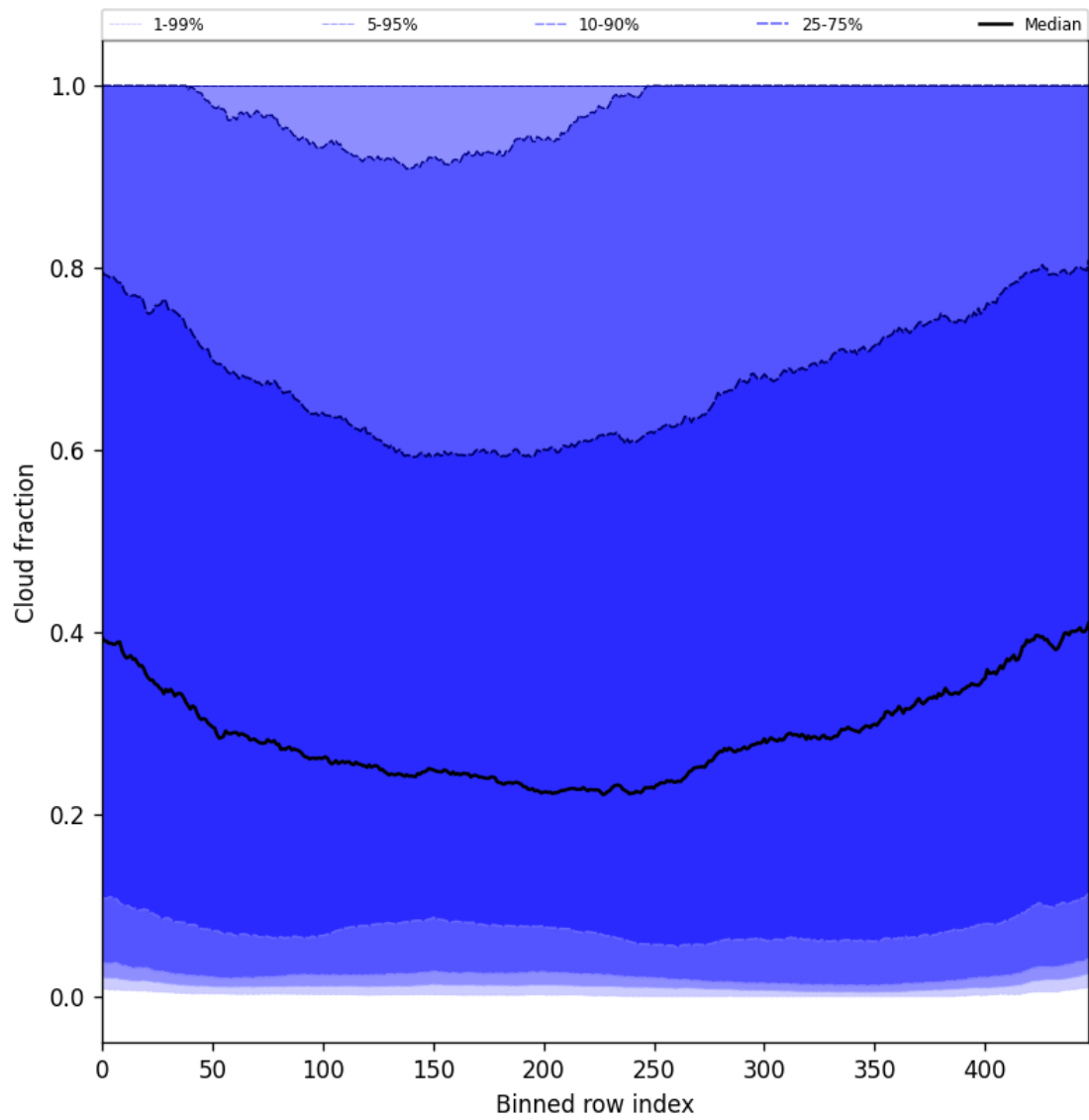
Figure 49: Along track statistics of “Cloud fraction” for 2025-06-18 to 2025-06-20
