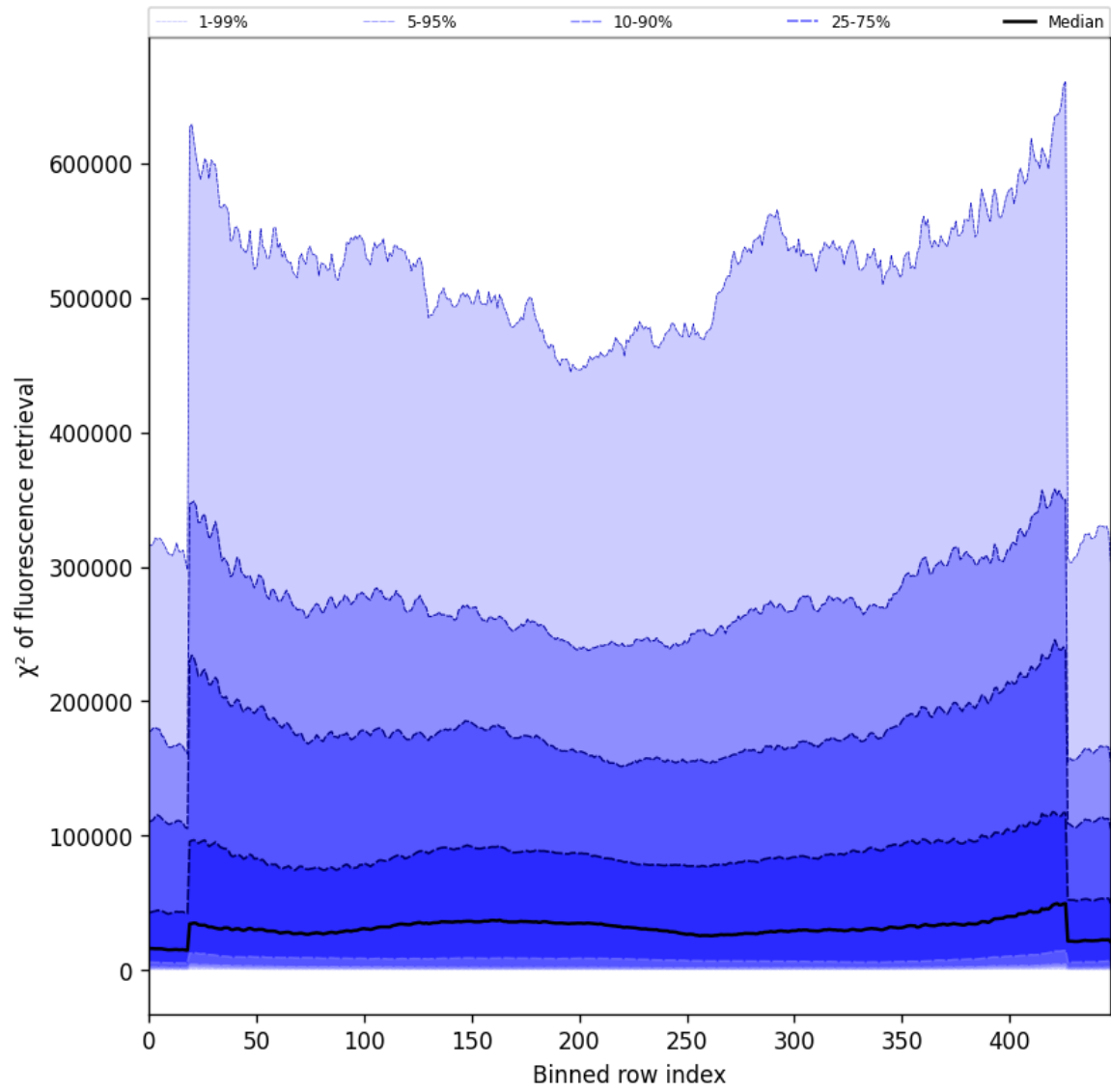
Figure 59: Along track statistics of “ \chi^2 of fluorescence retrieval” for 2025-06-18 to 2025-06-20
