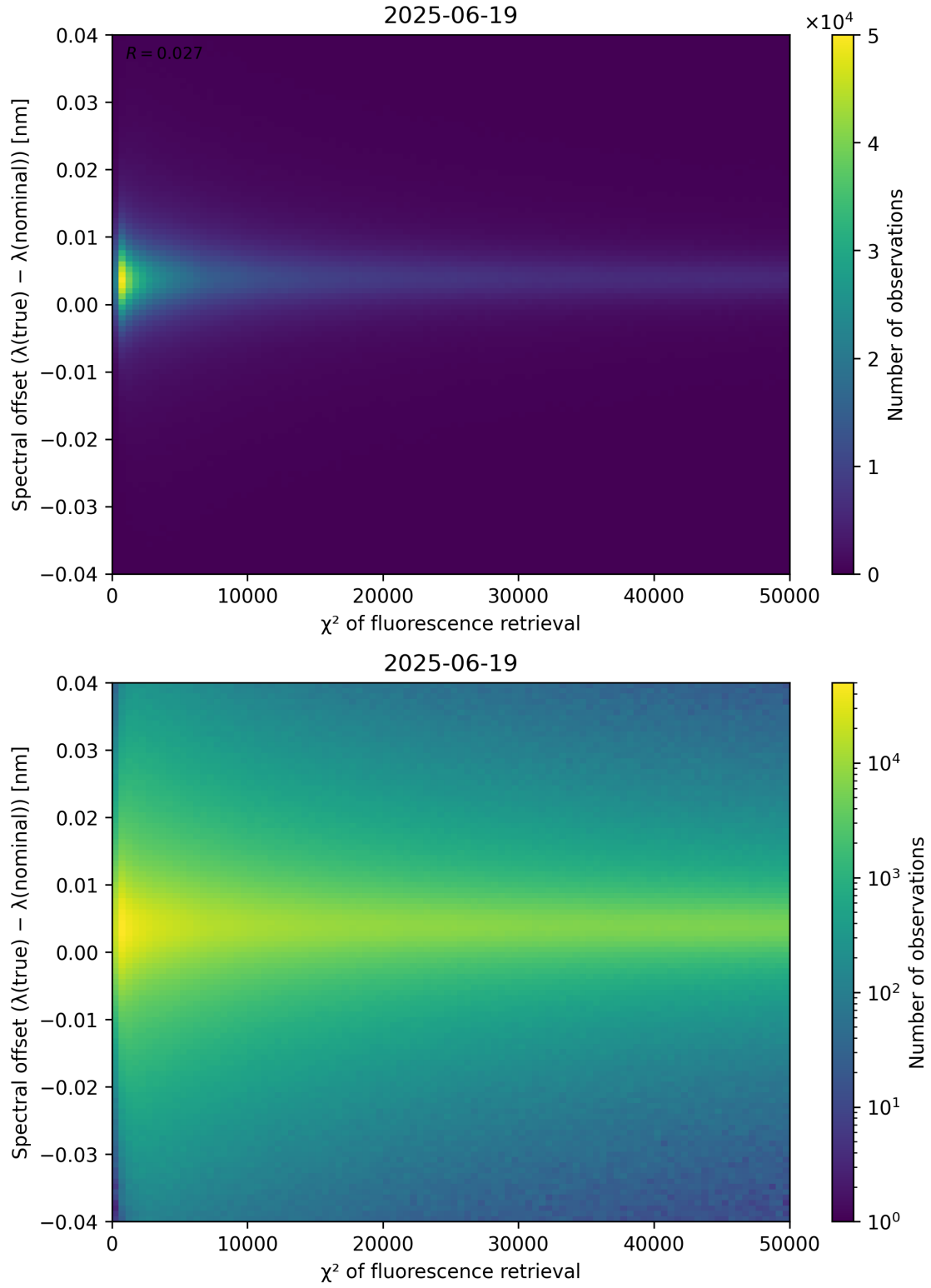
Figure 69: Scatter density plot of “ \chi^2 of fluorescence retrieval” against “Spectral offset ( \lambda_{\text{true}} - \lambda_{\text{nominal}} )” for 2025-06-18 to 2025-06-20.
