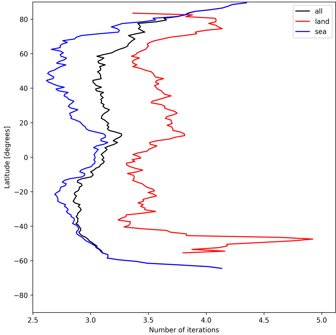
Figure 22: Zonal average of “Number of iterations” for 2025-06-18 to 2025-06-20.
