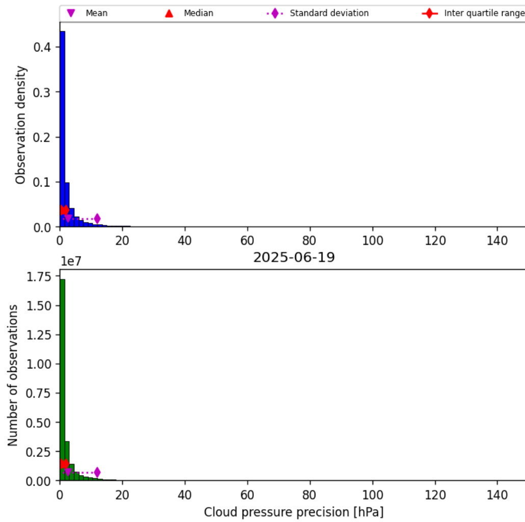
Figure 31: Histogram of “Cloud pressure precision” for 2025-06-18 to 2025-06-20
