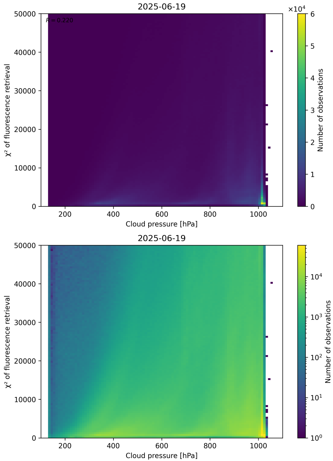
Figure 78: Scatter density plot of “Cloud pressure” against “ \chi^2 of fluorescence retrieval” for 2025-06-18 to 2025-06-20.
