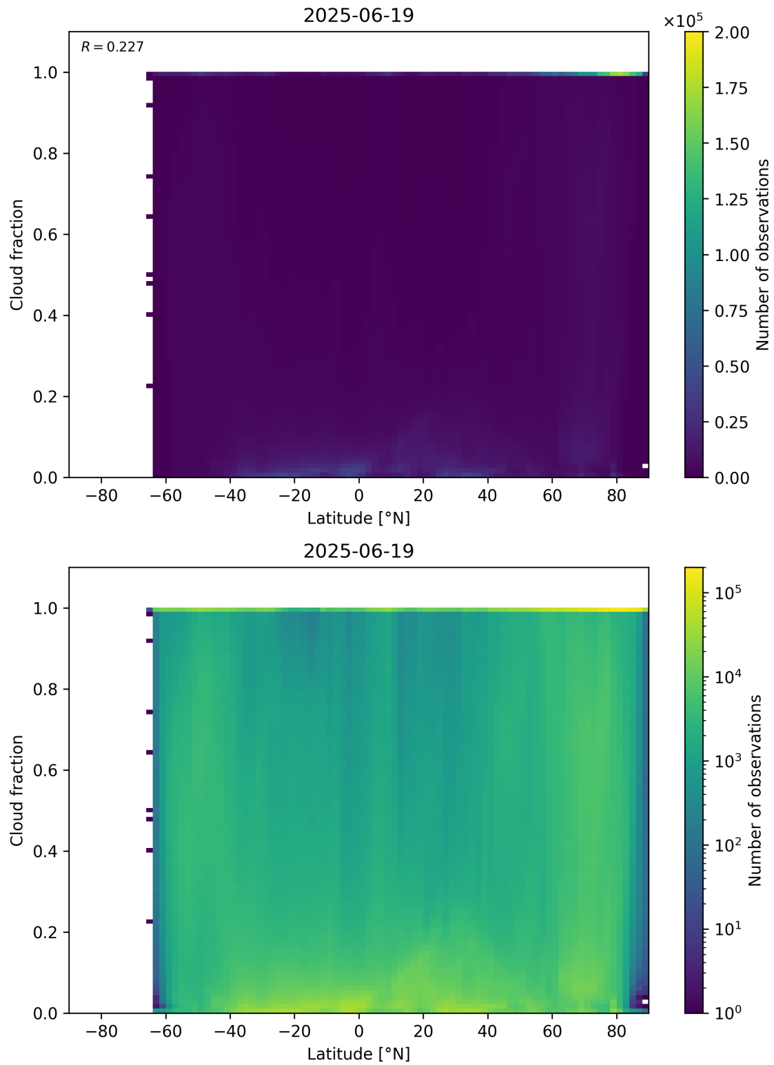
Figure 90: Scatter density plot of “Latitude” against “Cloud fraction” for 2025-06-18 to 2025-06-20.
