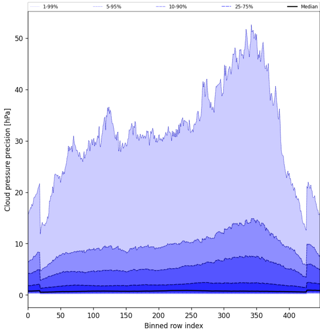
Figure 48: Along track statistics of “Cloud pressure precision” for 2025-06-18 to 2025-06-20
