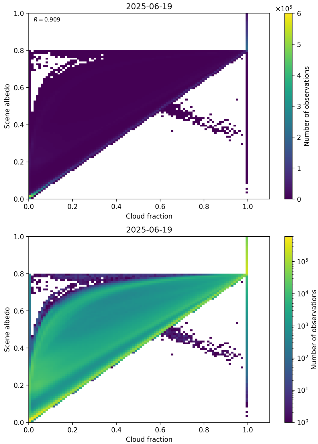
Figure 75: Scatter density plot of “Cloud fraction” against “Scene albedo” for 2025-06-18 to 2025-06-20.
