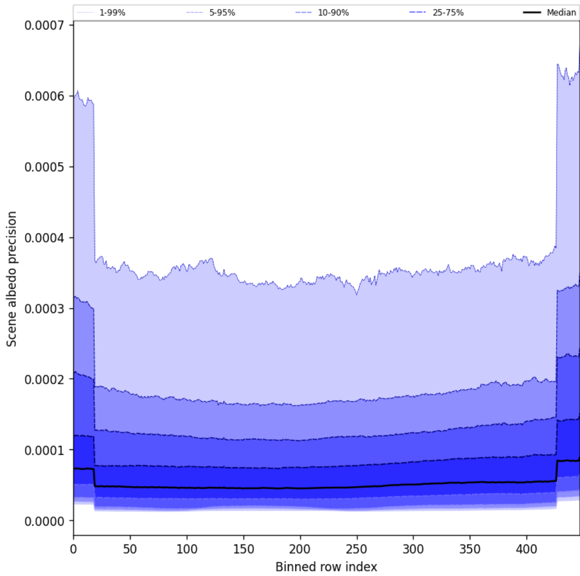
Figure 52: Along track statistics of “Scene albedo precision” for 2025-06-18 to 2025-06-20
