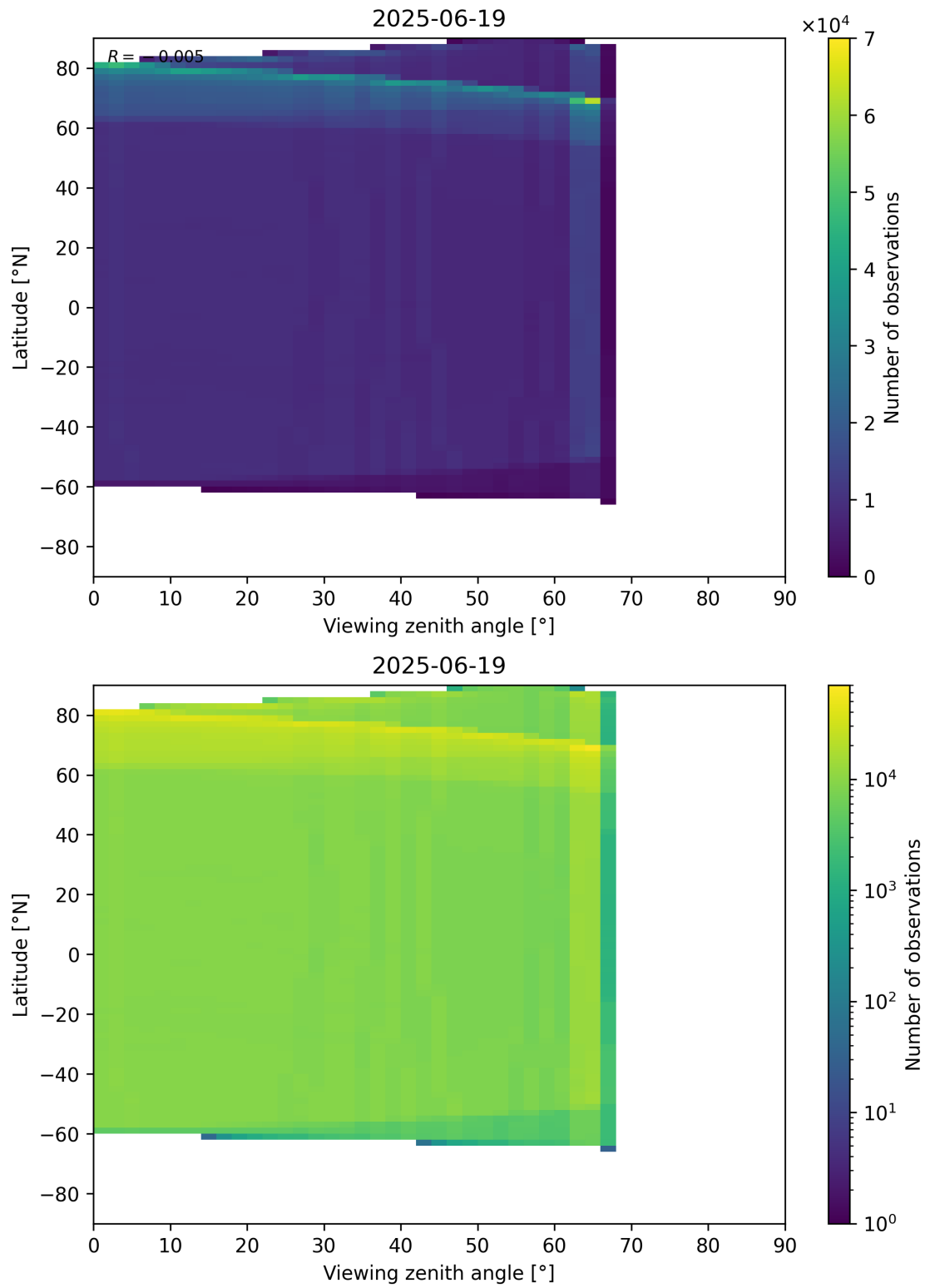
Figure 123: Scatter density plot of “Viewing zenith angle” against “Latitude” for 2025-06-18 to 2025-06-20.
