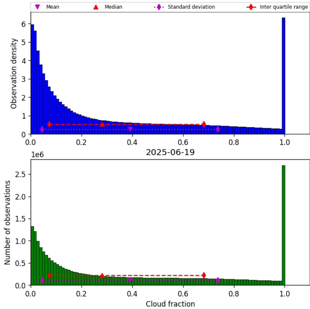
Figure 32: Histogram of “Cloud fraction” for 2025-06-18 to 2025-06-20
