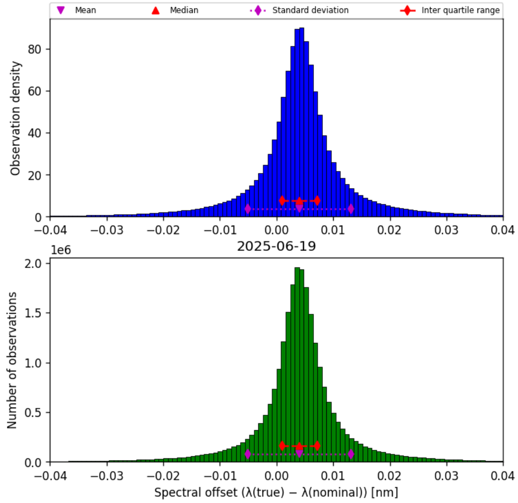
Figure 45: Histogram of “Spectral offset ( \lambda_{\text{true}} - \lambda_{\text{nominal}} )” for 2025-06-18 to 2025-06-20
