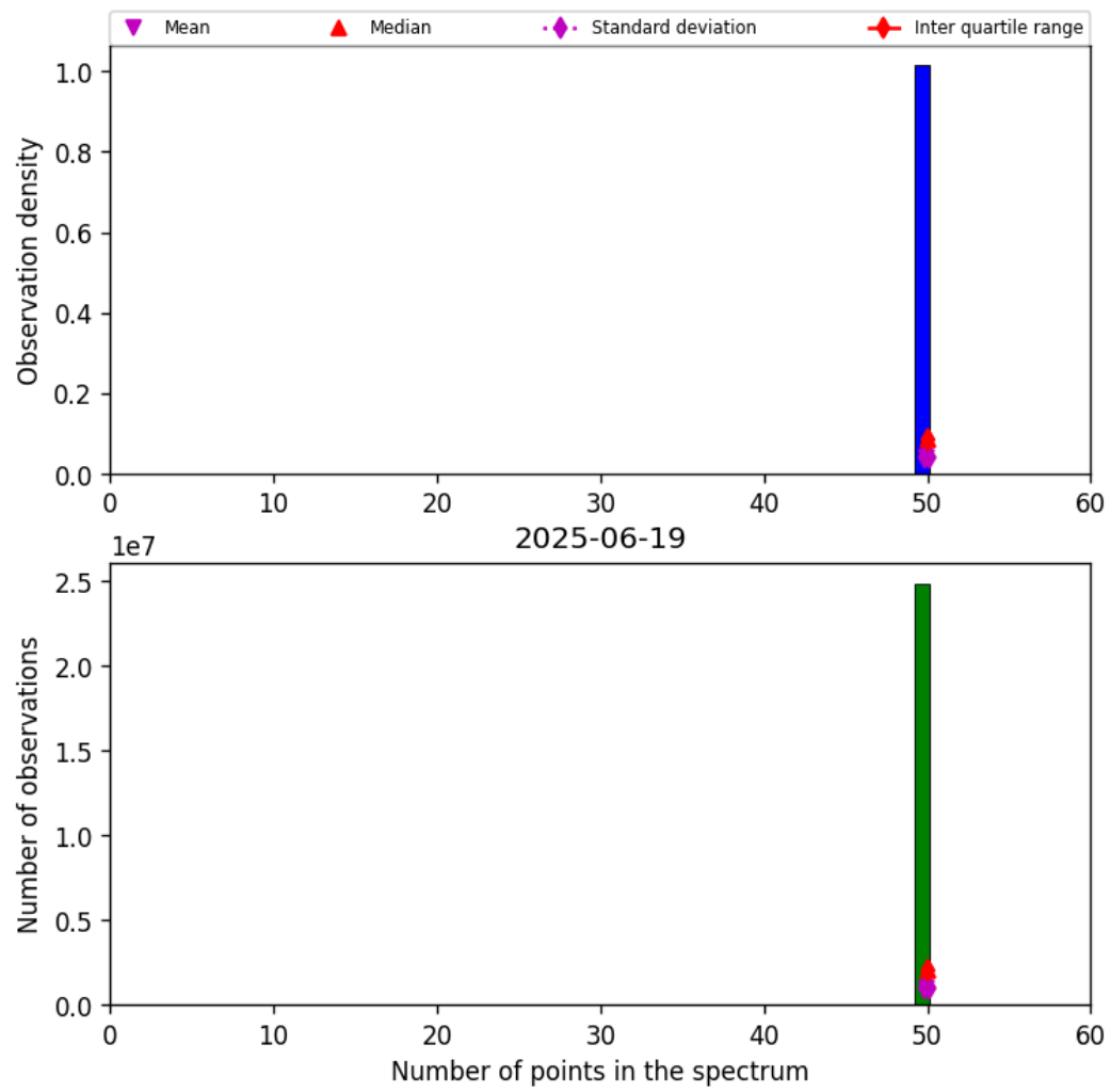
Figure 44: Histogram of “Number of points in the spectrum” for 2025-06-18 to 2025-06-20
