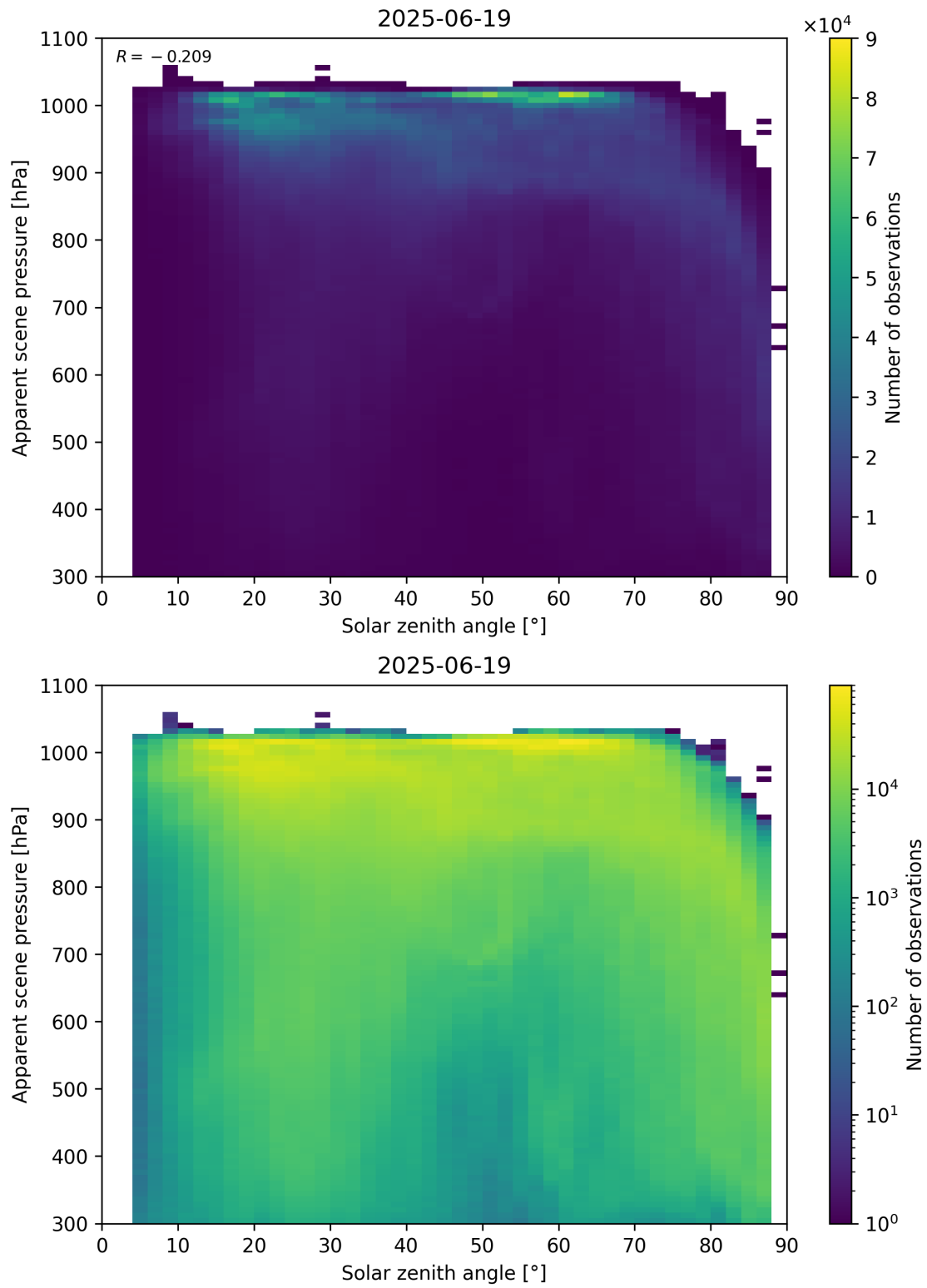
Figure 108: Scatter density plot of “Solar zenith angle” against “Apparent scene pressure” for 2025-06-18 to 2025-06-20.
