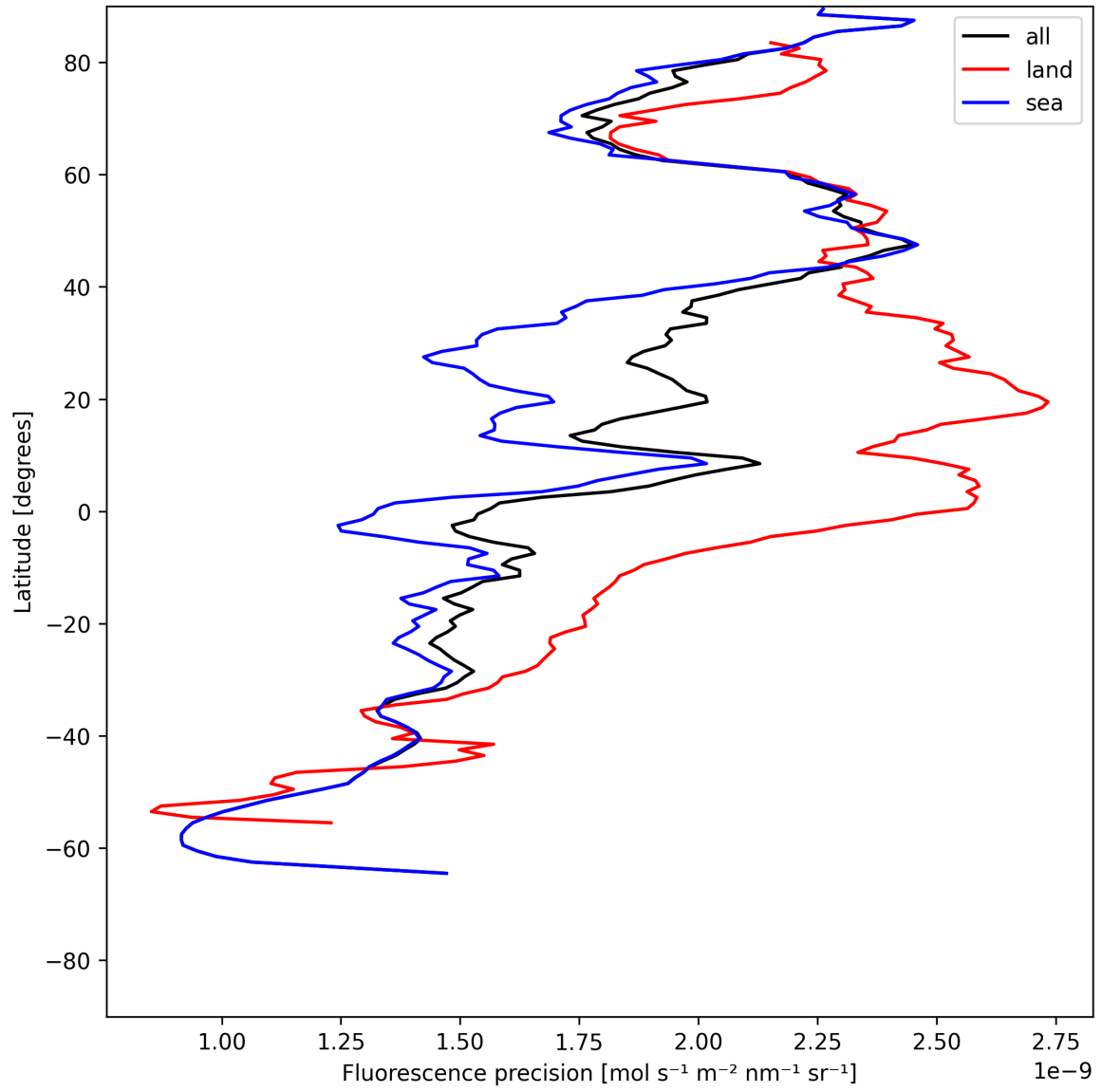
Figure 24: Zonal average of “Fluorescence precision” for 2025-06-18 to 2025-06-20.
