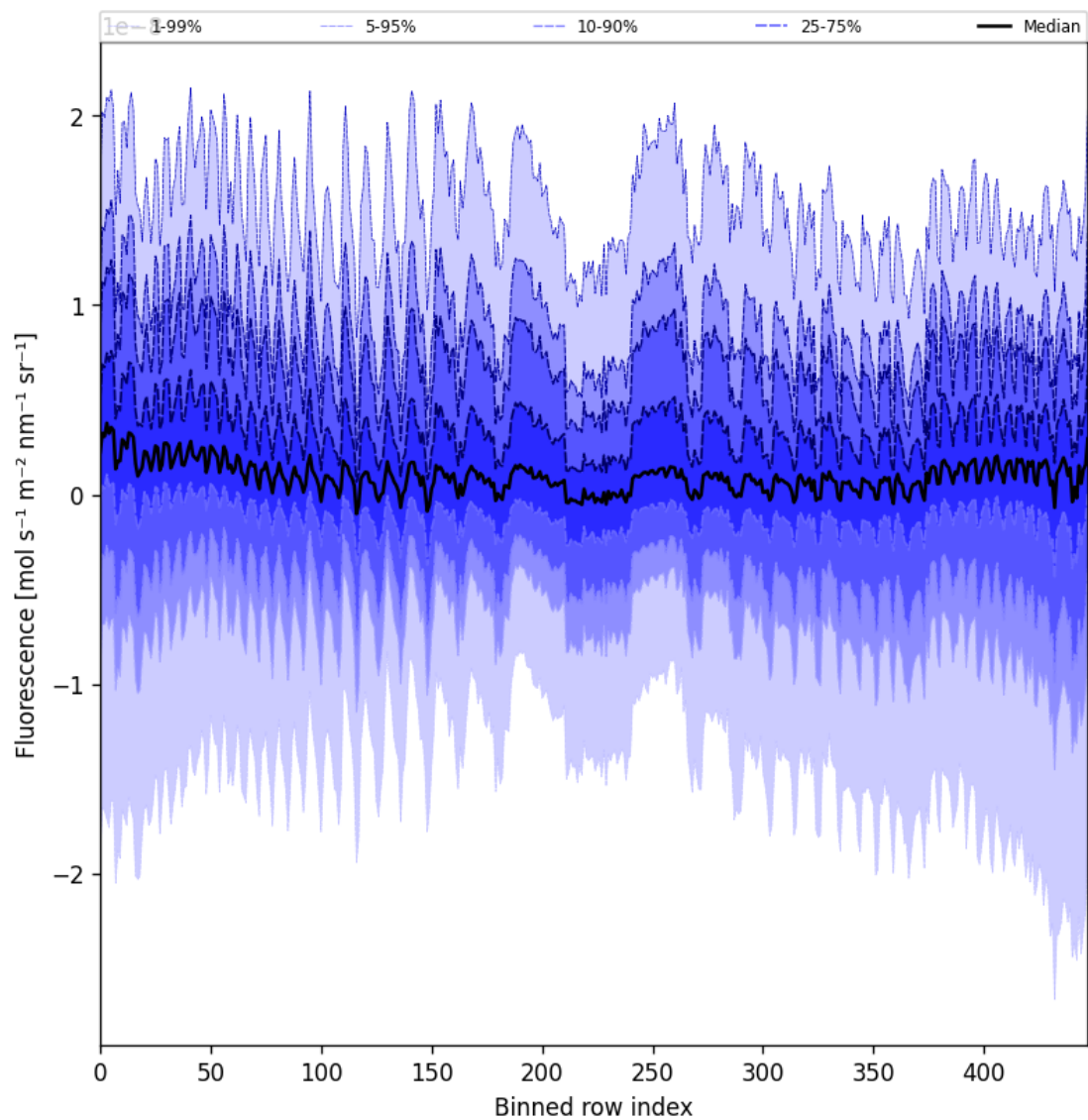
Figure 57: Along track statistics of “Fluorescence” for 2025-06-18 to 2025-06-20
