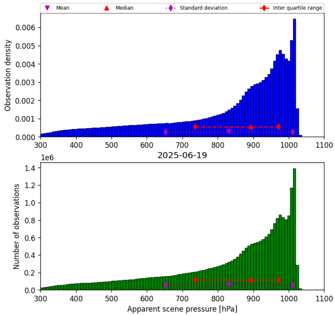
Figure 36: Histogram of “Apparent scene pressure” for 2025-06-18 to 2025-06-20
