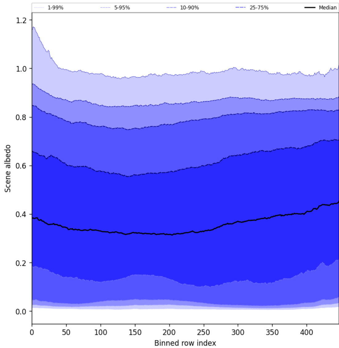
Figure 51: Along track statistics of “Scene albedo” for 2025-06-18 to 2025-06-20
