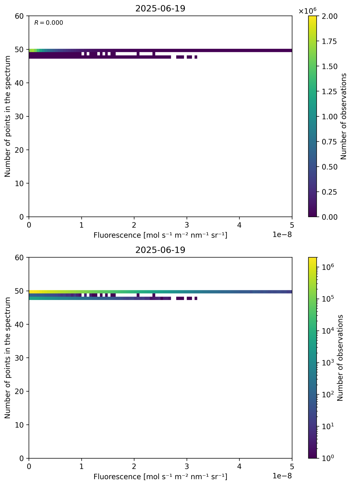
Figure 86: Scatter density plot of “Fluorescence” against “Number of points in the spectrum” for 2025-06-18 to 2025-06-20.
