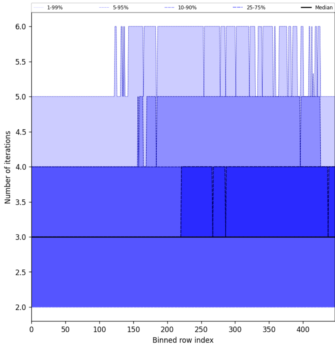
Figure 56: Along track statistics of “Number of iterations” for 2025-06-18 to 2025-06-20
