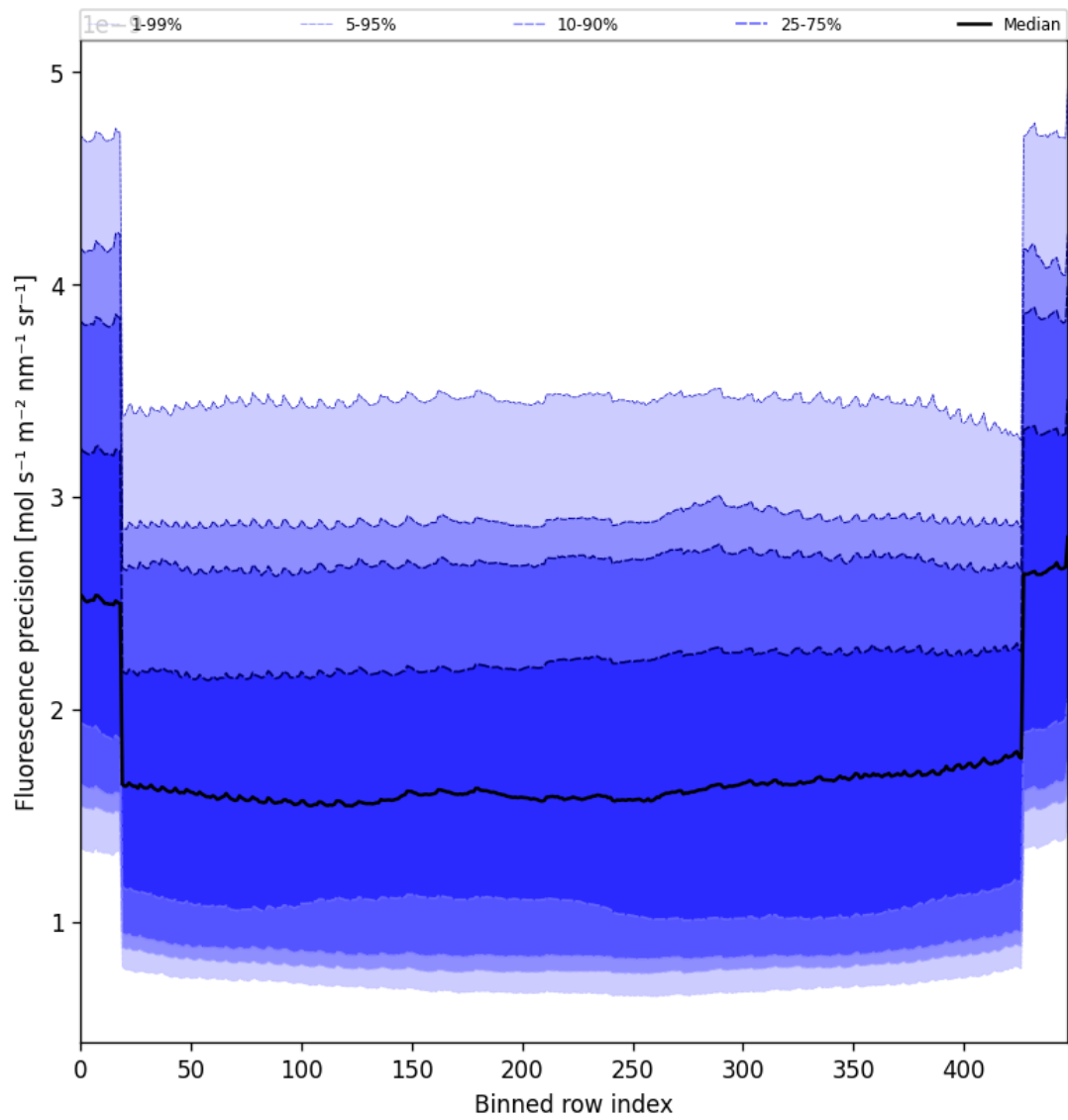
Figure 58: Along track statistics of “Fluorescence precision” for 2025-06-18 to 2025-06-20
