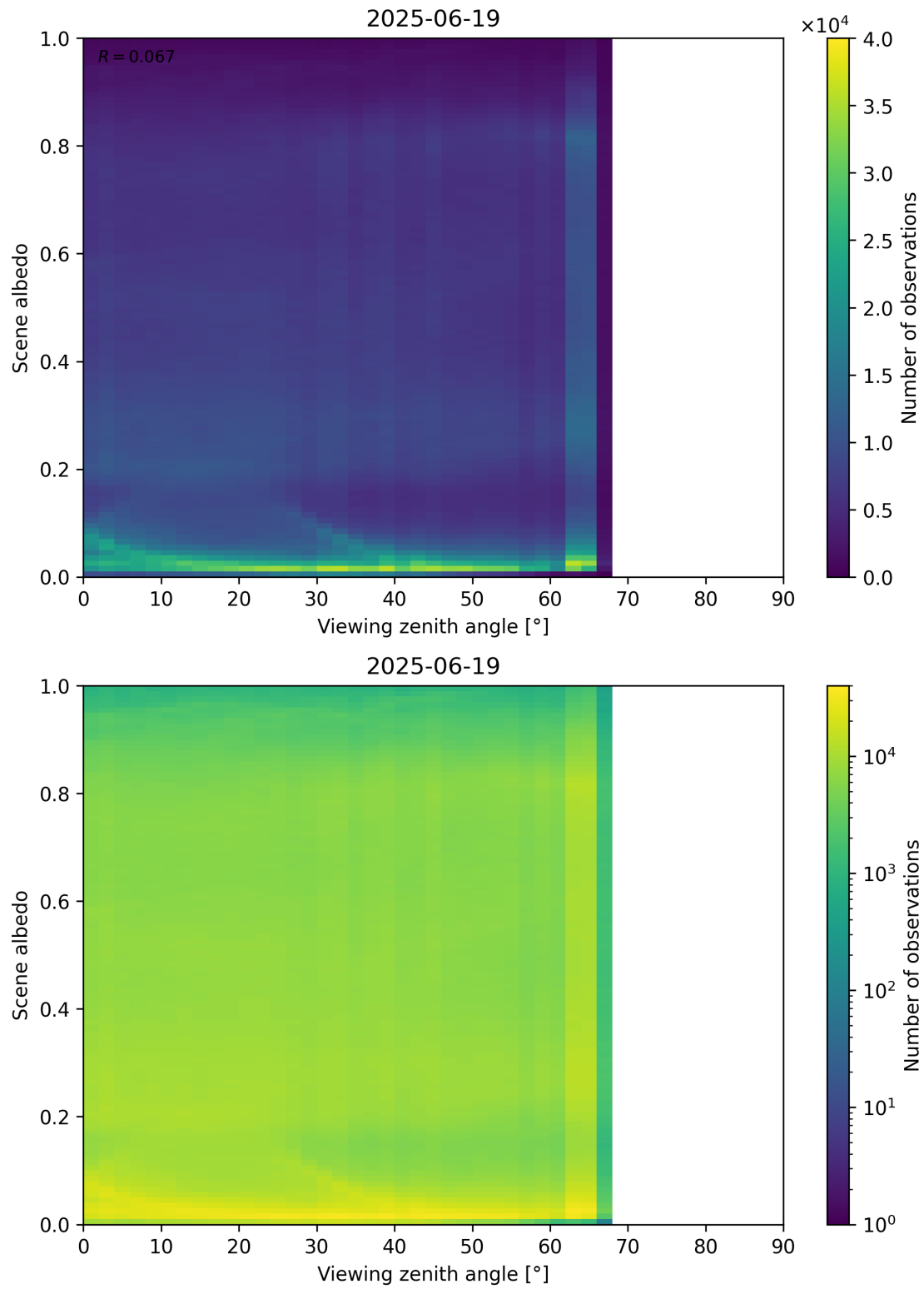
Figure 126: Scatter density plot of “Viewing zenith angle” against “Scene albedo” for 2025-06-18 to 2025-06-20.
