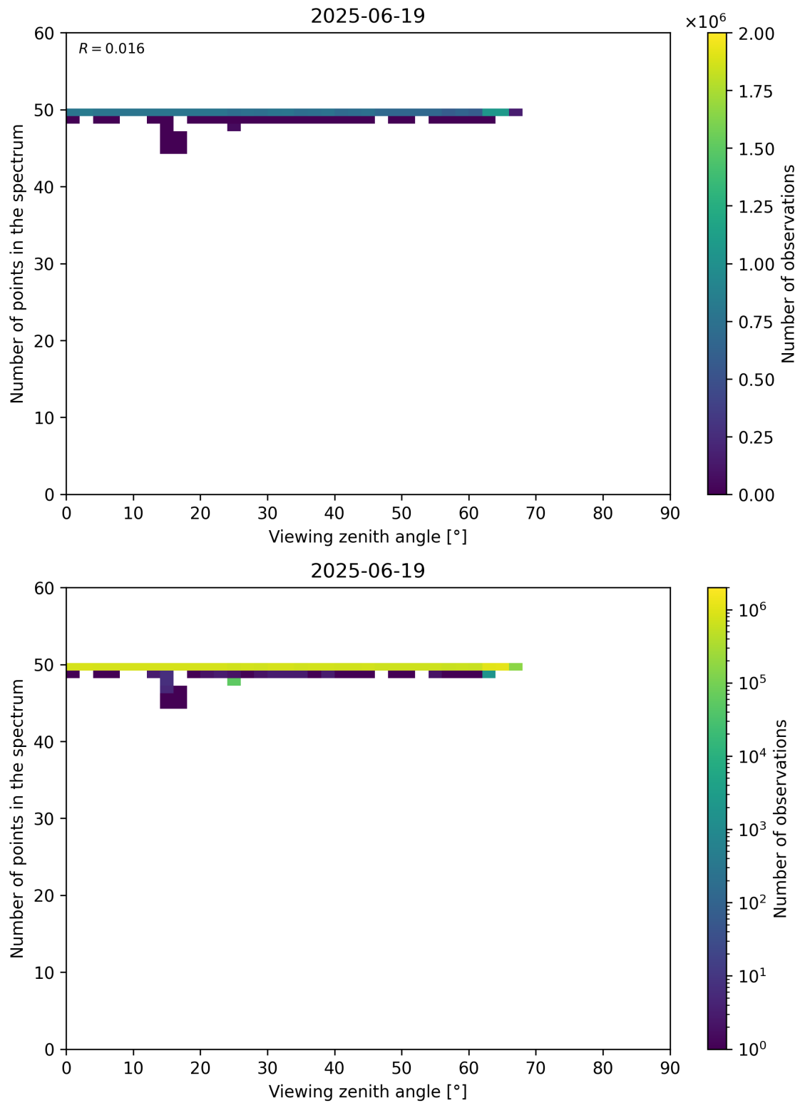
Figure 125: Scatter density plot of “Viewing zenith angle” against “Number of points in the spectrum” for 2025-06-18 to 2025-06-20.
