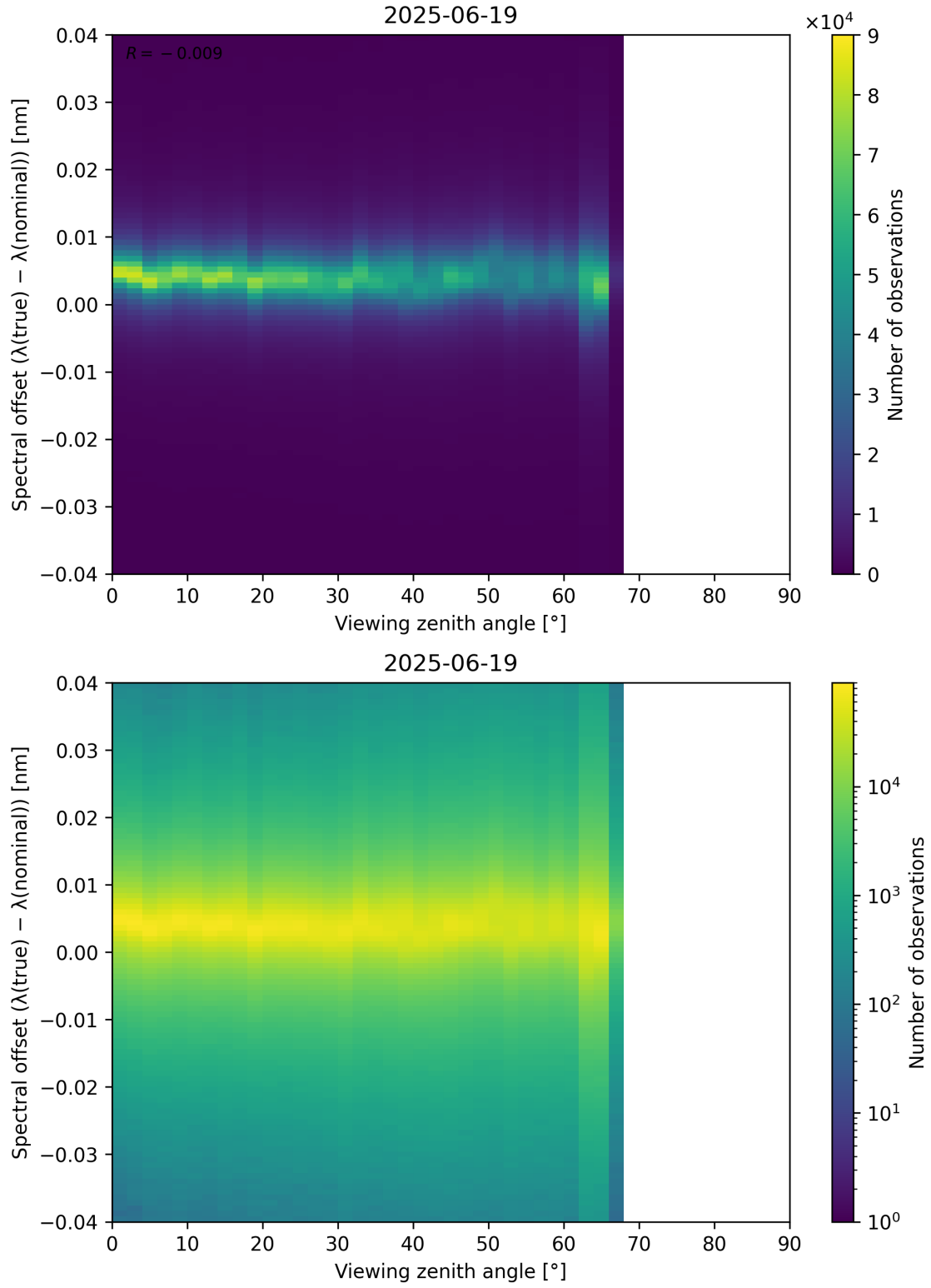
Figure 128: Scatter density plot of “Viewing zenith angle” against “Spectral offset ( \lambda_{\text{true}} - \lambda_{\text{nominal}} )” for 2025-06-18 to 2025-06-20.
