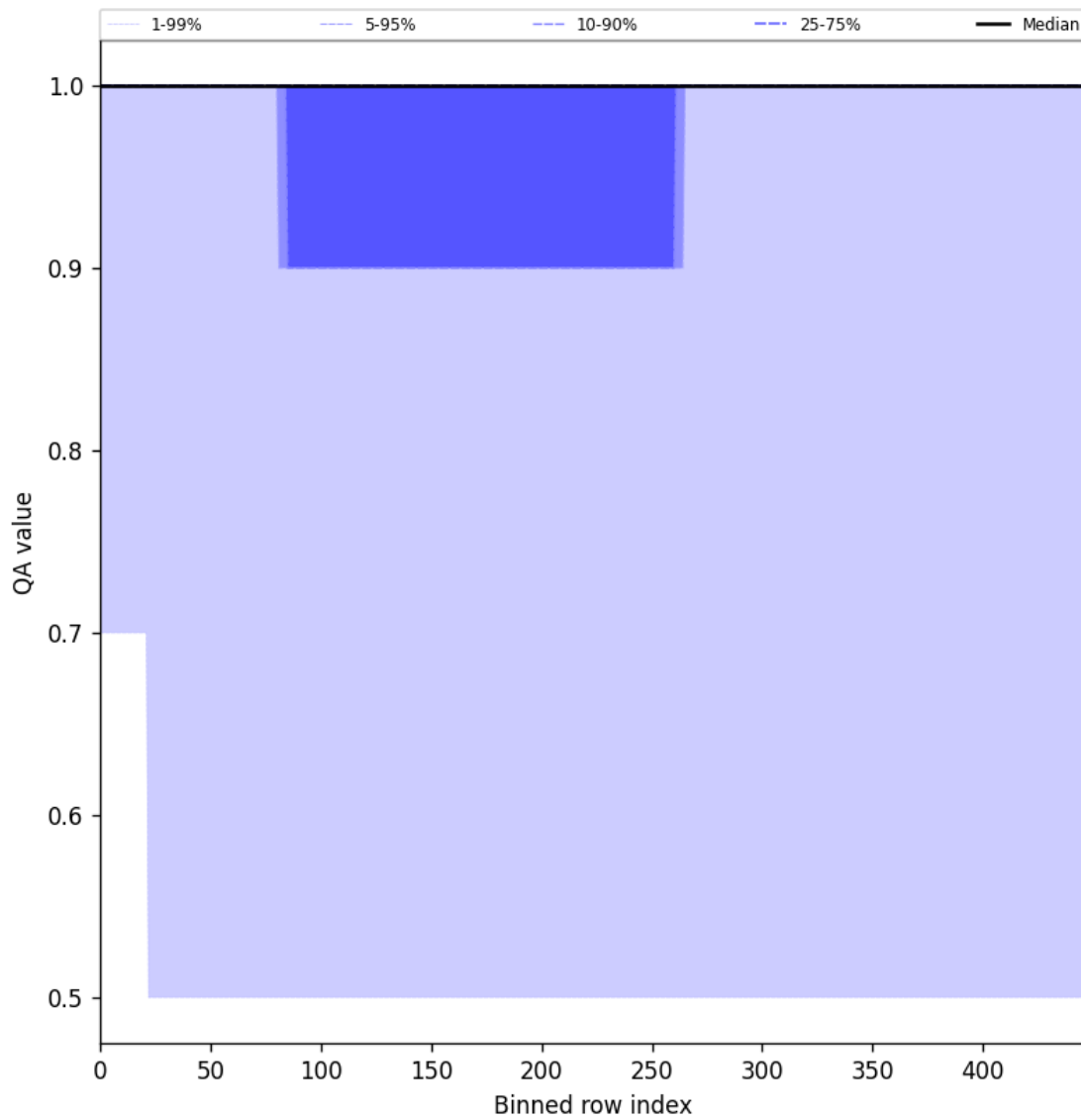
Figure 46: Along track statistics of “QA value” for 2025-06-18 to 2025-06-20
