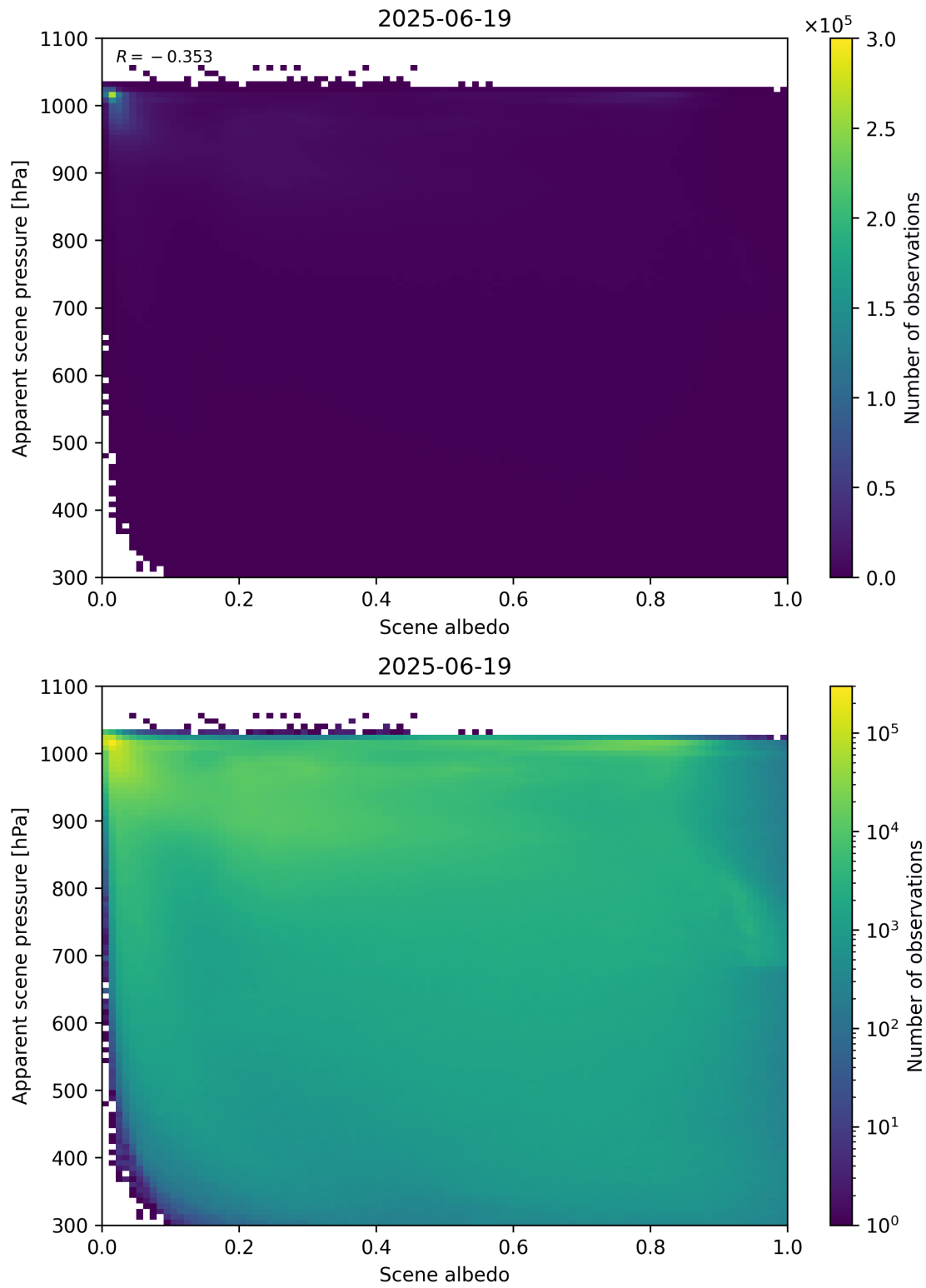
Figure 102: Scatter density plot of “Scene albedo” against “Apparent scene pressure” for 2025-06-18 to 2025-06-20.
