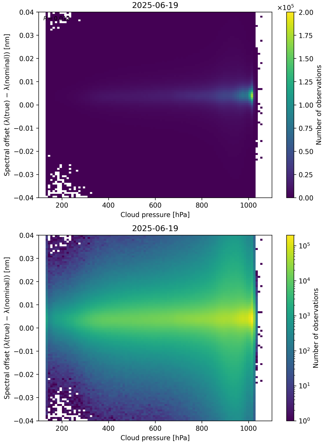
Figure 84: Scatter density plot of “Cloud pressure” against “Spectral offset ( \lambda_{\text{true}} - \lambda_{\text{nominal}} )” for 2025-06-18 to 2025-06-20.
