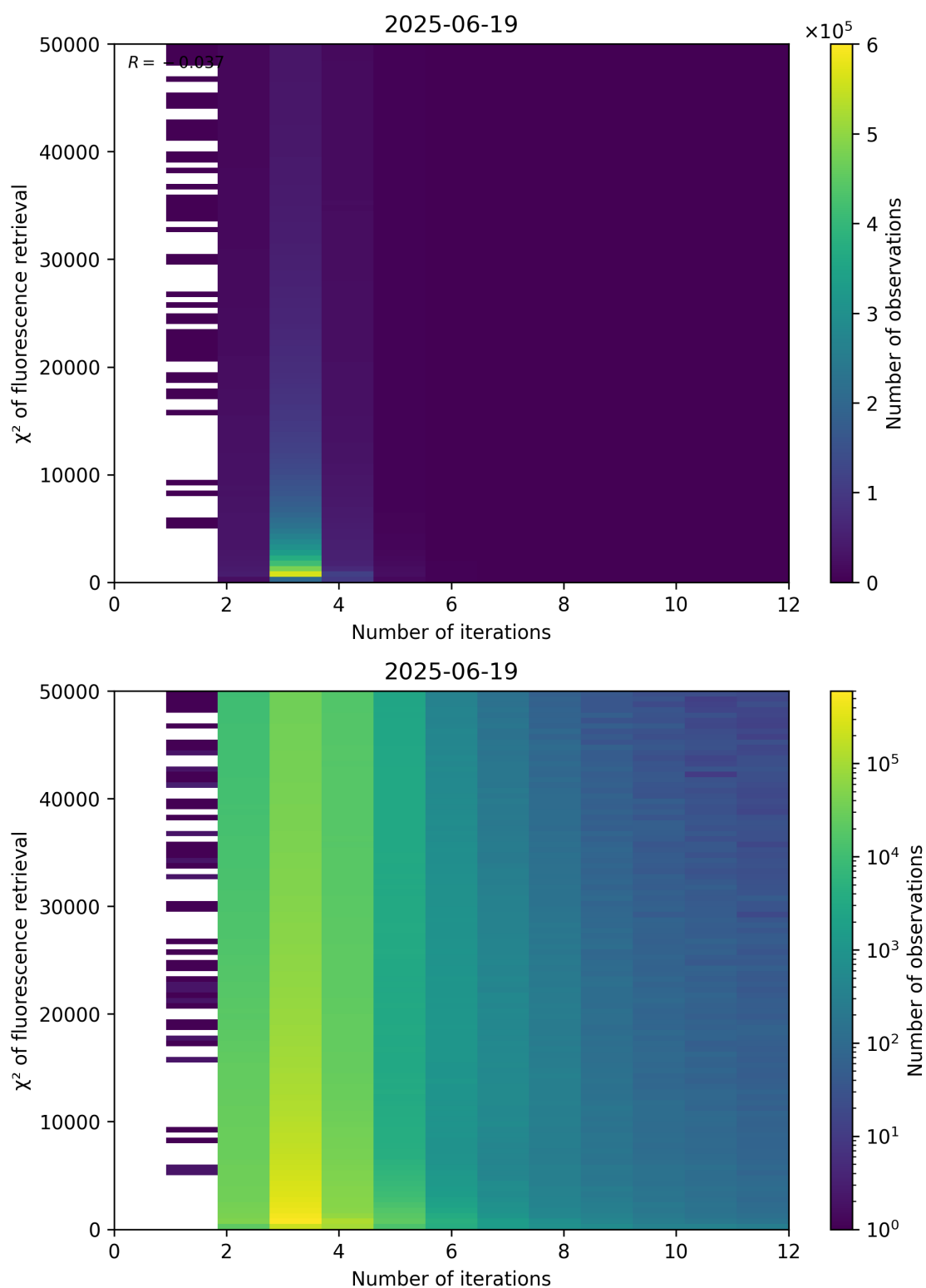
Figure 97: Scatter density plot of “Number of iterations” against “ \chi^2 of fluorescence retrieval” for 2025-06-18 to 2025-06-20.
