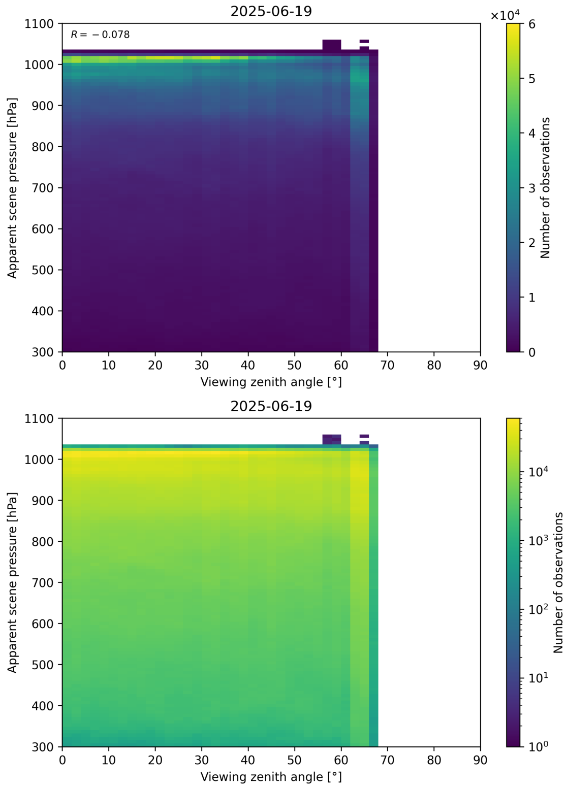
Figure 118: Scatter density plot of “Viewing zenith angle” against “Apparent scene pressure” for 2025-06-18 to 2025-06-20.
