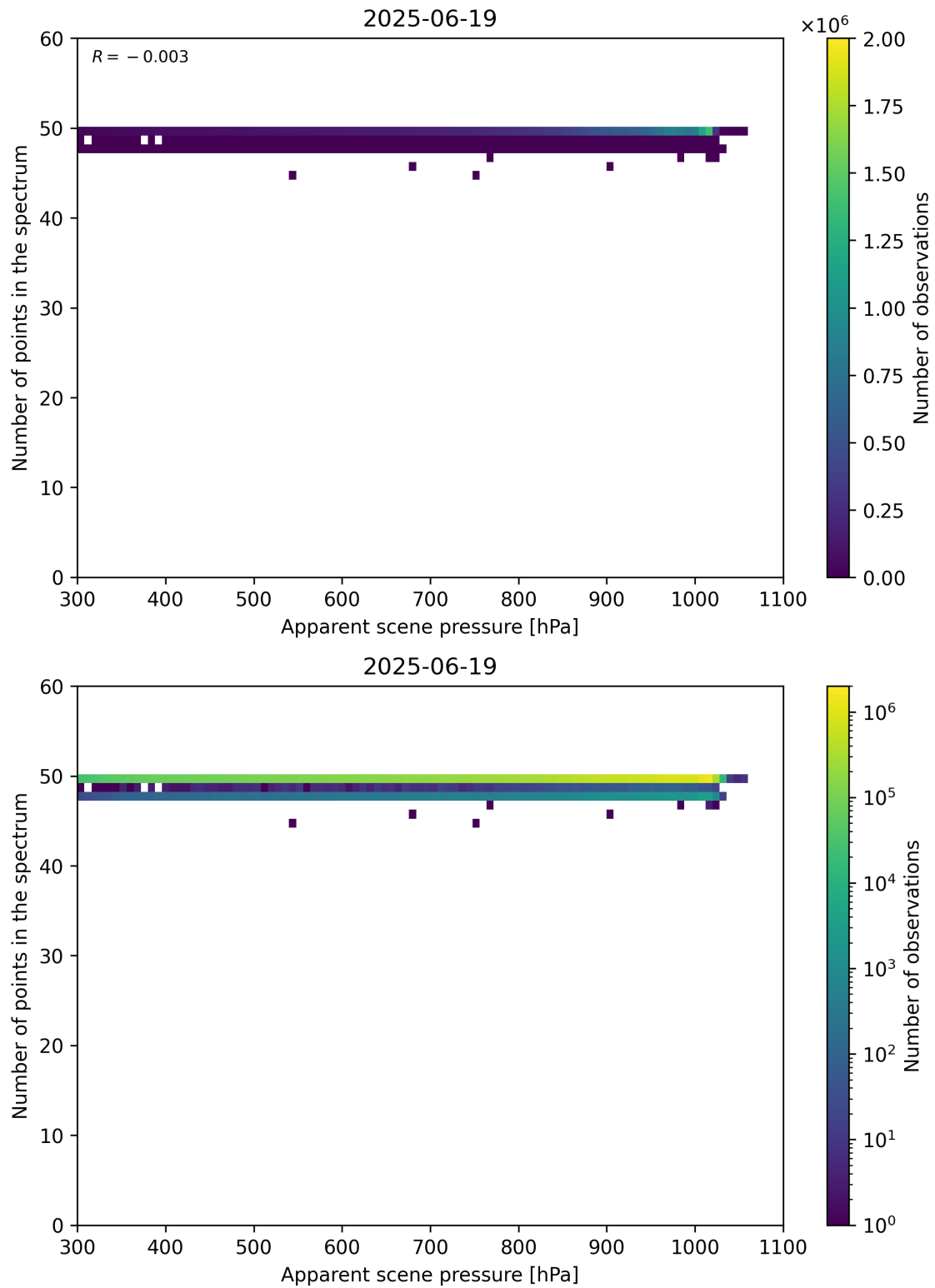
Figure 66: Scatter density plot of “Apparent scene pressure” against “Number of points in the spectrum” for 2025-06-18 to 2025-06-20.
