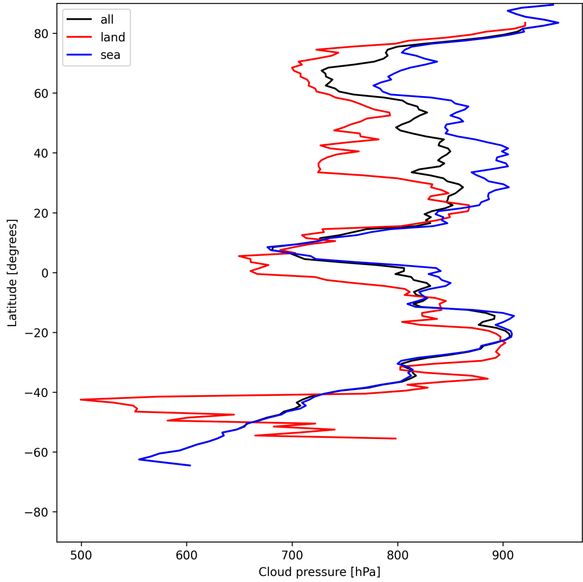
Figure 13: Zonal average of “Cloud pressure” for 2025-06-18 to 2025-06-20.
