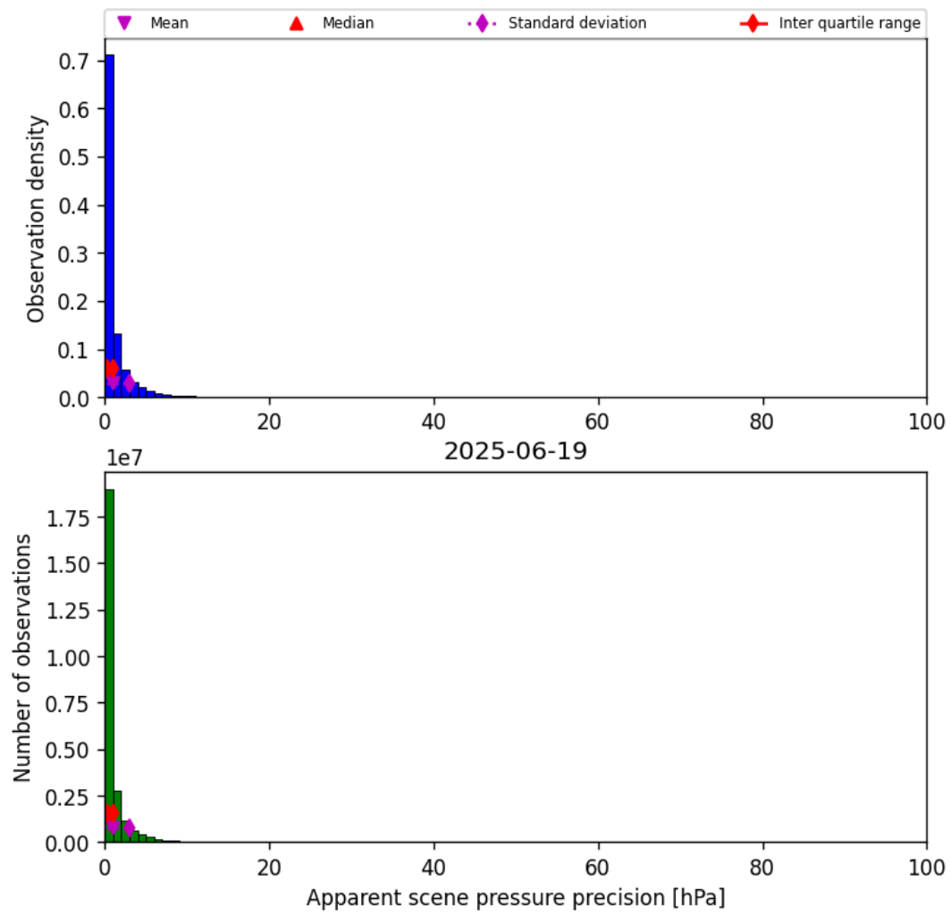
Figure 37: Histogram of “Apparent scene pressure precision” for 2025-06-18 to 2025-06-20
