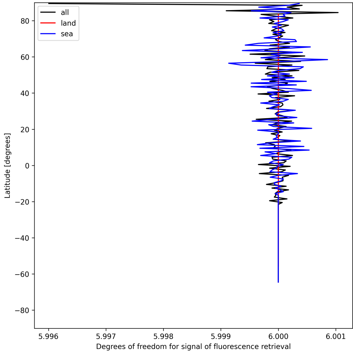
Figure 26: Zonal average of “Degrees of freedom for signal of fluorescence retrieval” for 2025-06-18 to 2025-06-20.
