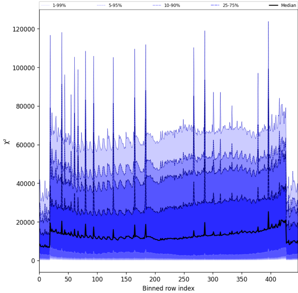
Figure 55: Along track statistics of “ \chi^2 ” for 2025-06-18 to 2025-06-20
