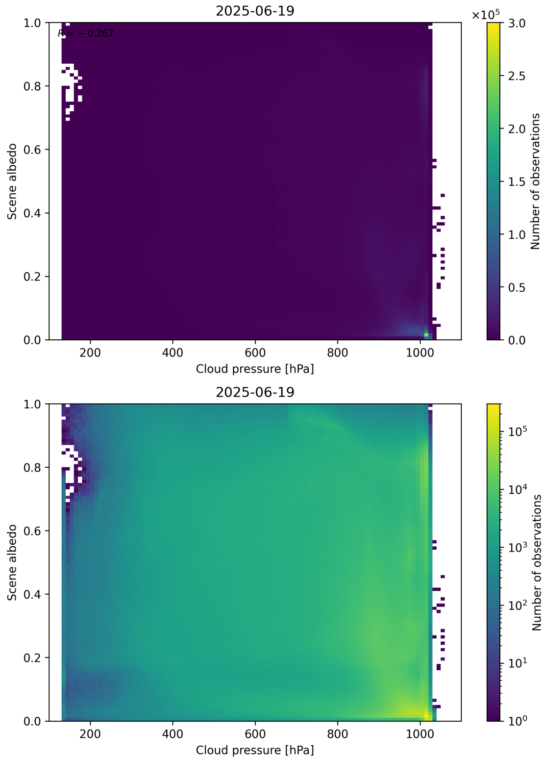
Figure 83: Scatter density plot of “Cloud pressure” against “Scene albedo” for 2025-06-18 to 2025-06-20.
