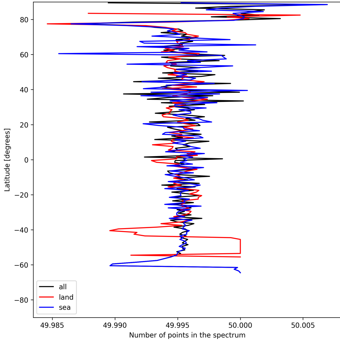
Figure 27: Zonal average of “Number of points in the spectrum” for 2025-06-18 to 2025-06-20.
