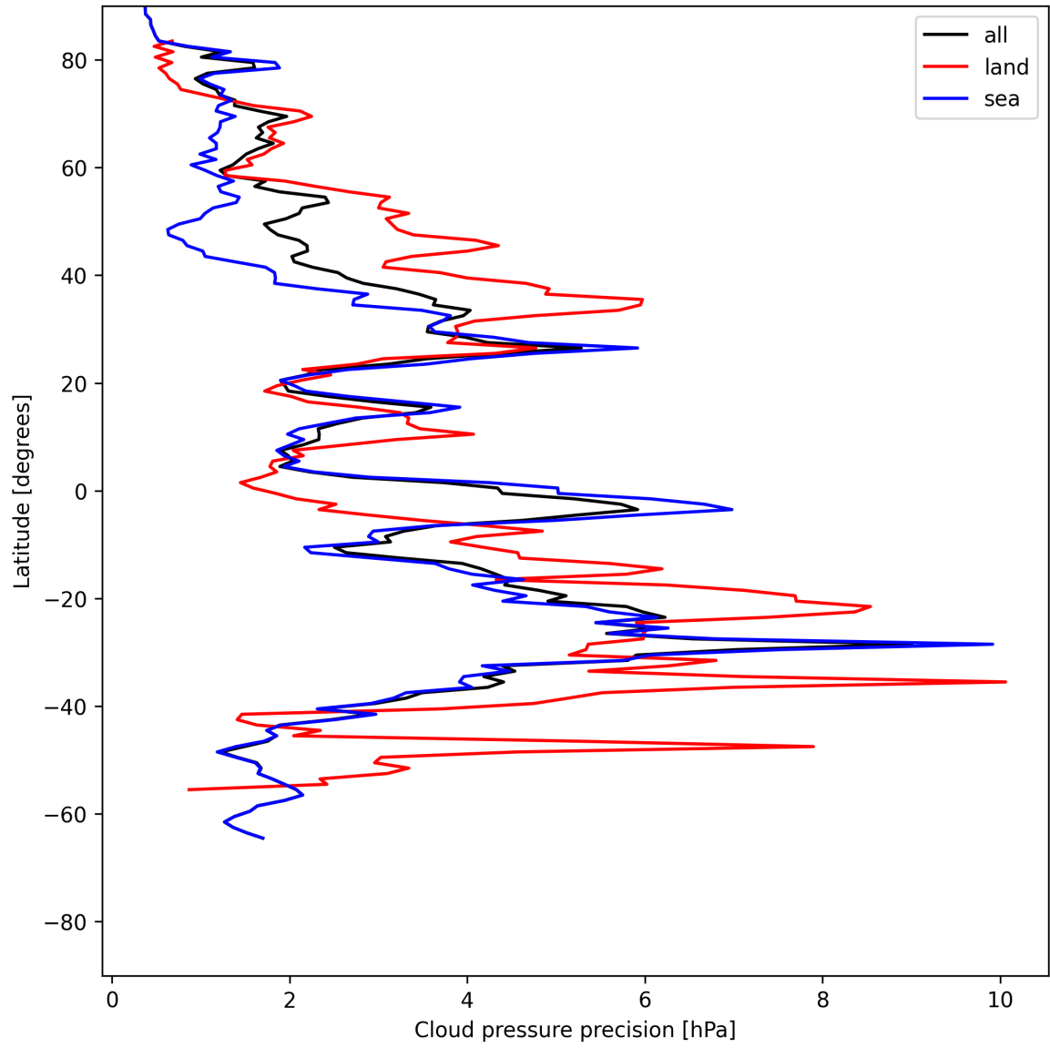
Figure 14: Zonal average of “Cloud pressure precision” for 2025-06-18 to 2025-06-20.
