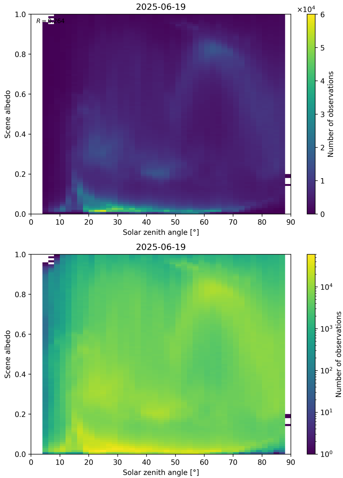
Figure 116: Scatter density plot of “Solar zenith angle” against “Scene albedo” for 2025-06-18 to 2025-06-20.
