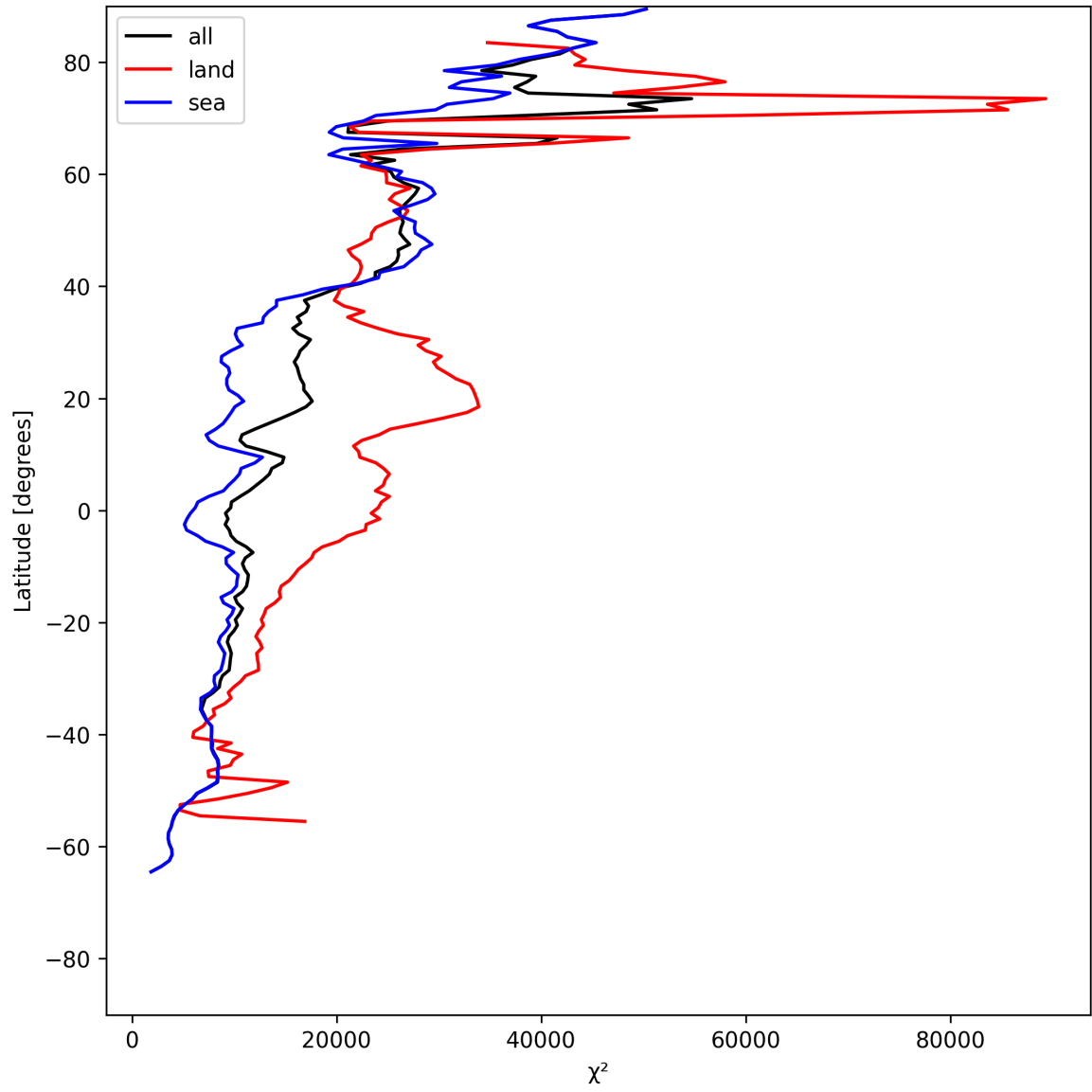
Figure 21: Zonal average of “ \chi^2 ” for 2025-06-18 to 2025-06-20.
