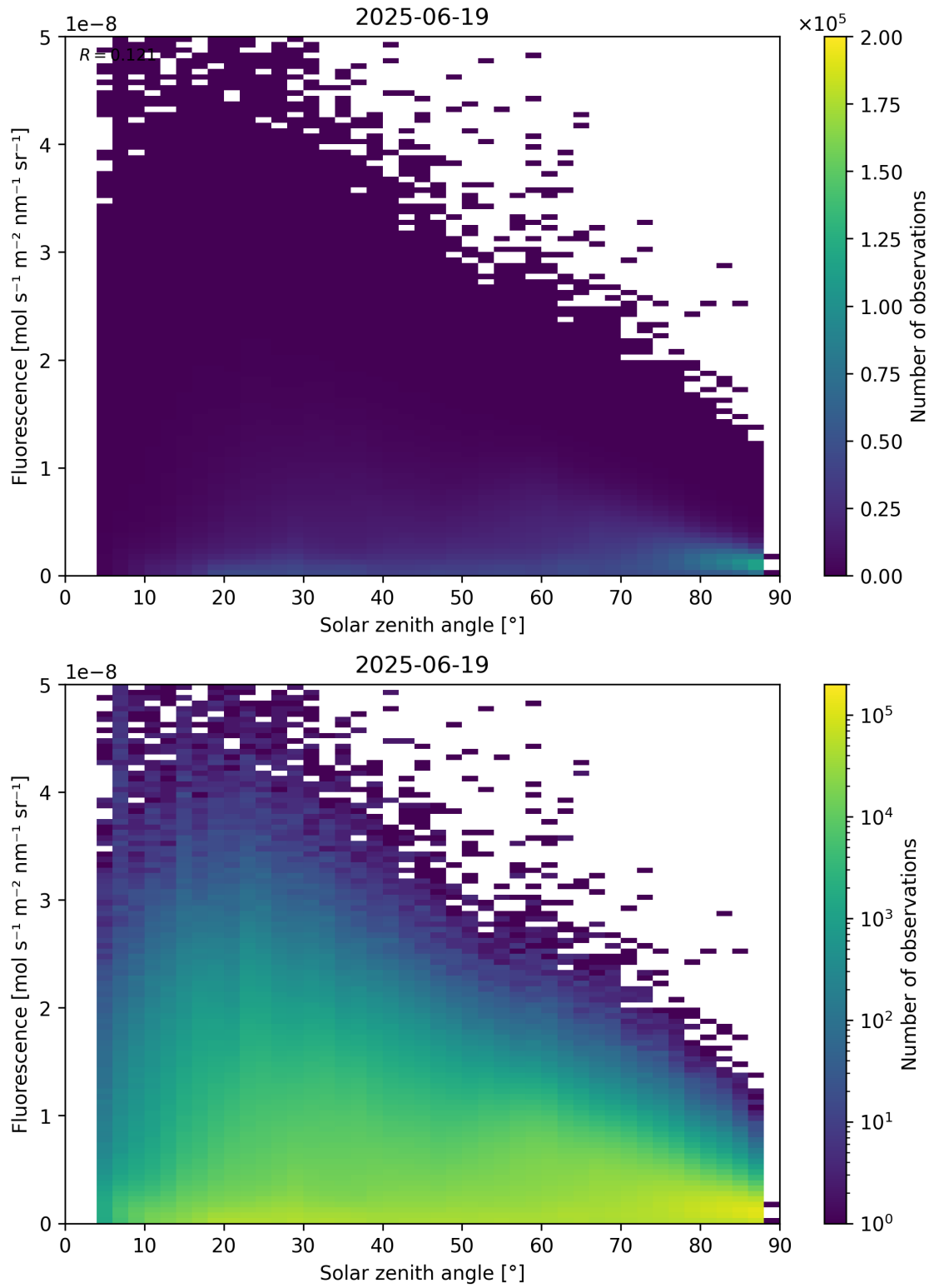
Figure 112: Scatter density plot of “Solar zenith angle” against “Fluorescence” for 2025-06-18 to 2025-06-20.
