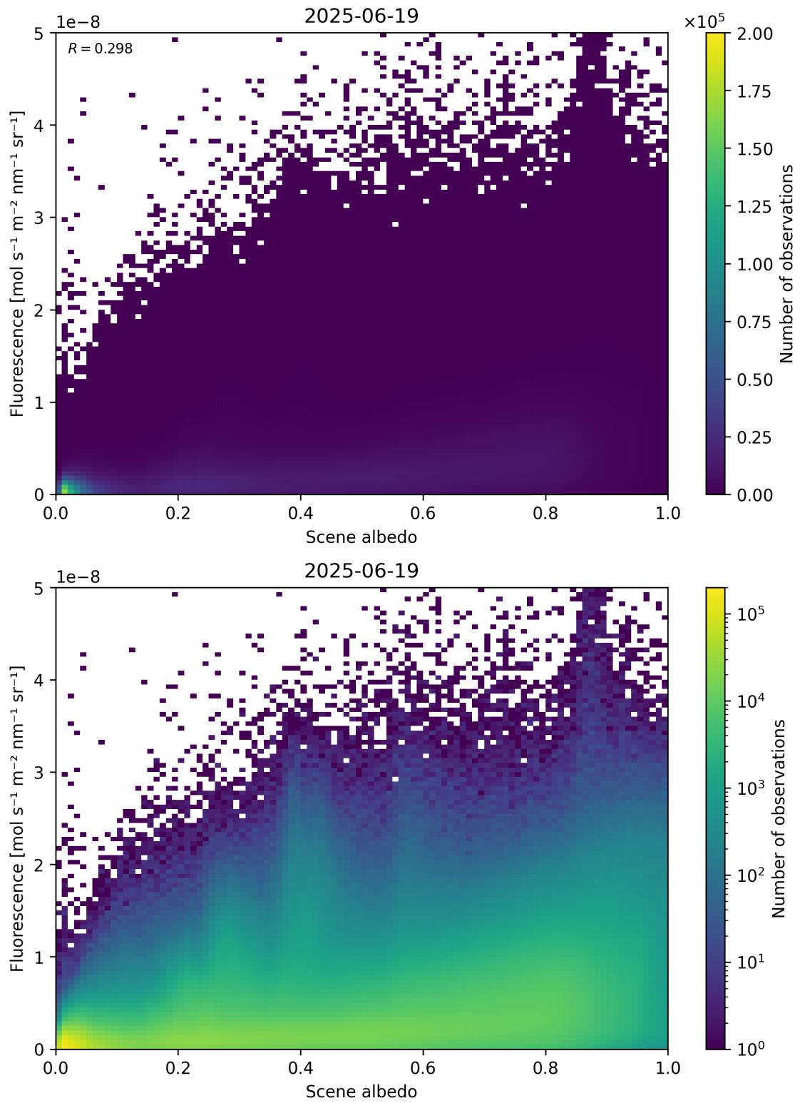
Figure 104: Scatter density plot of “Scene albedo” against “Fluorescence” for 2025-06-18 to 2025-06-20.
