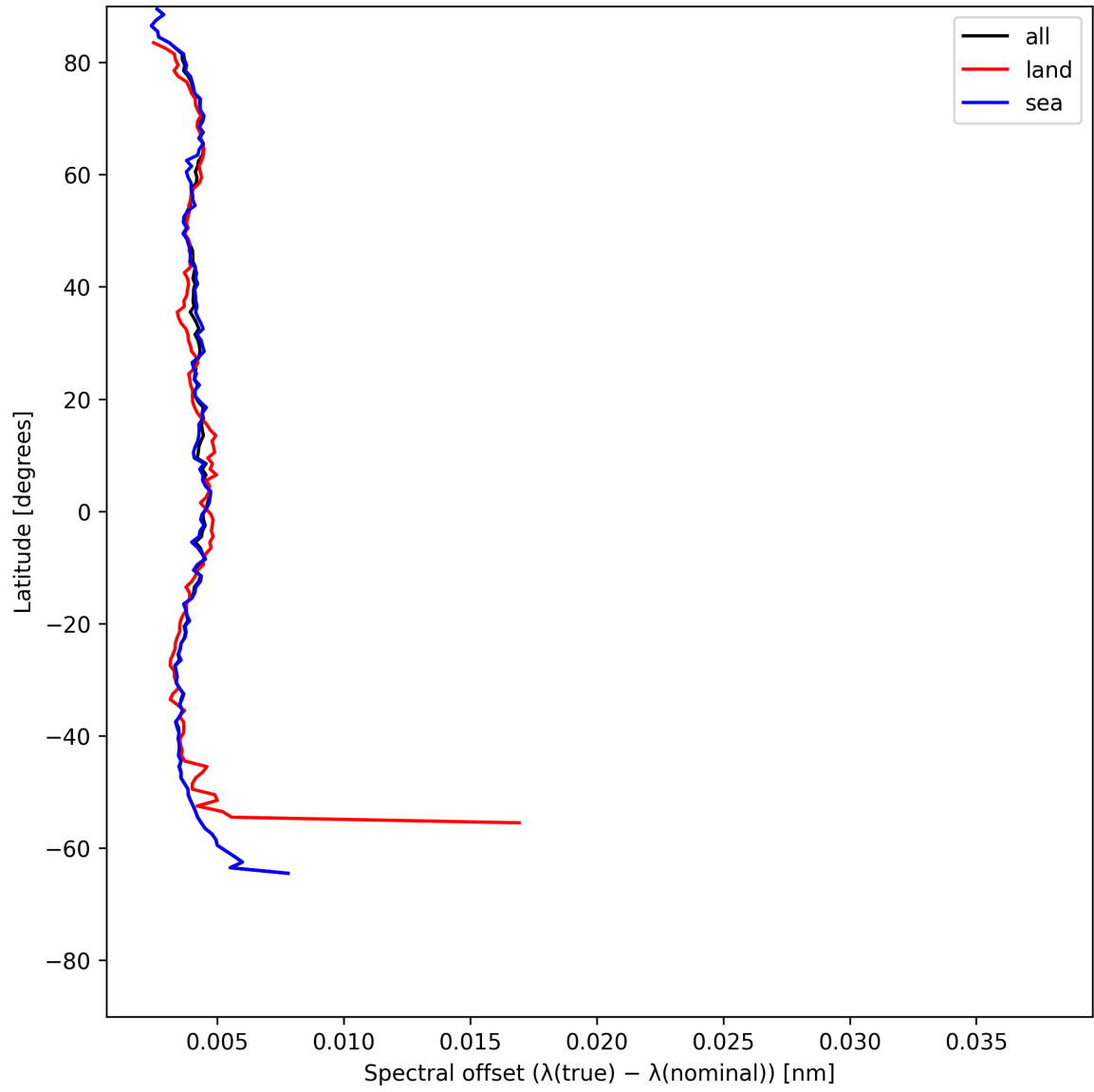
Figure 28: Zonal average of “Spectral offset ( \lambda_{\text{true}} - \lambda_{\text{nominal}} )” for 2025-06-18 to 2025-06-20.
