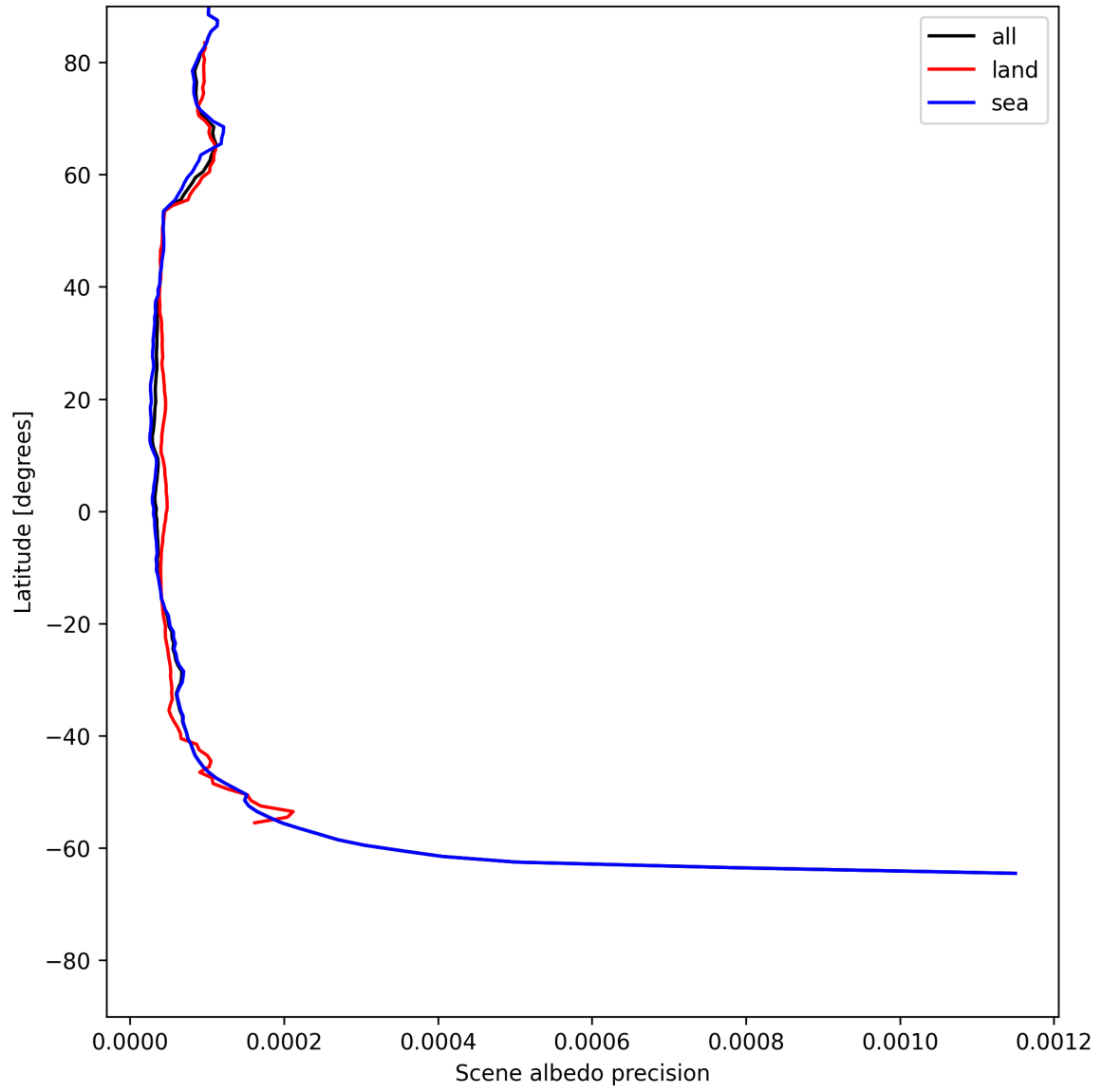
Figure 18: Zonal average of “Scene albedo precision” for 2025-06-18 to 2025-06-20.
