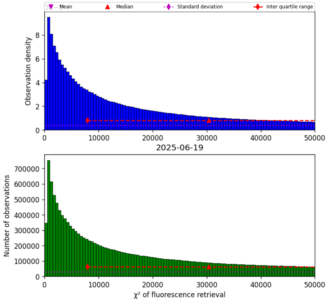
Figure 42: Histogram of “ \chi^2 of fluorescence retrieval” for 2025-06-18 to 2025-06-20
