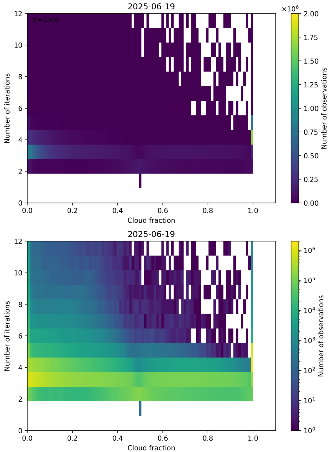
Figure 73: Scatter density plot of “Cloud fraction” against “Number of iterations” for 2025-06-18 to 2025-06-20.
