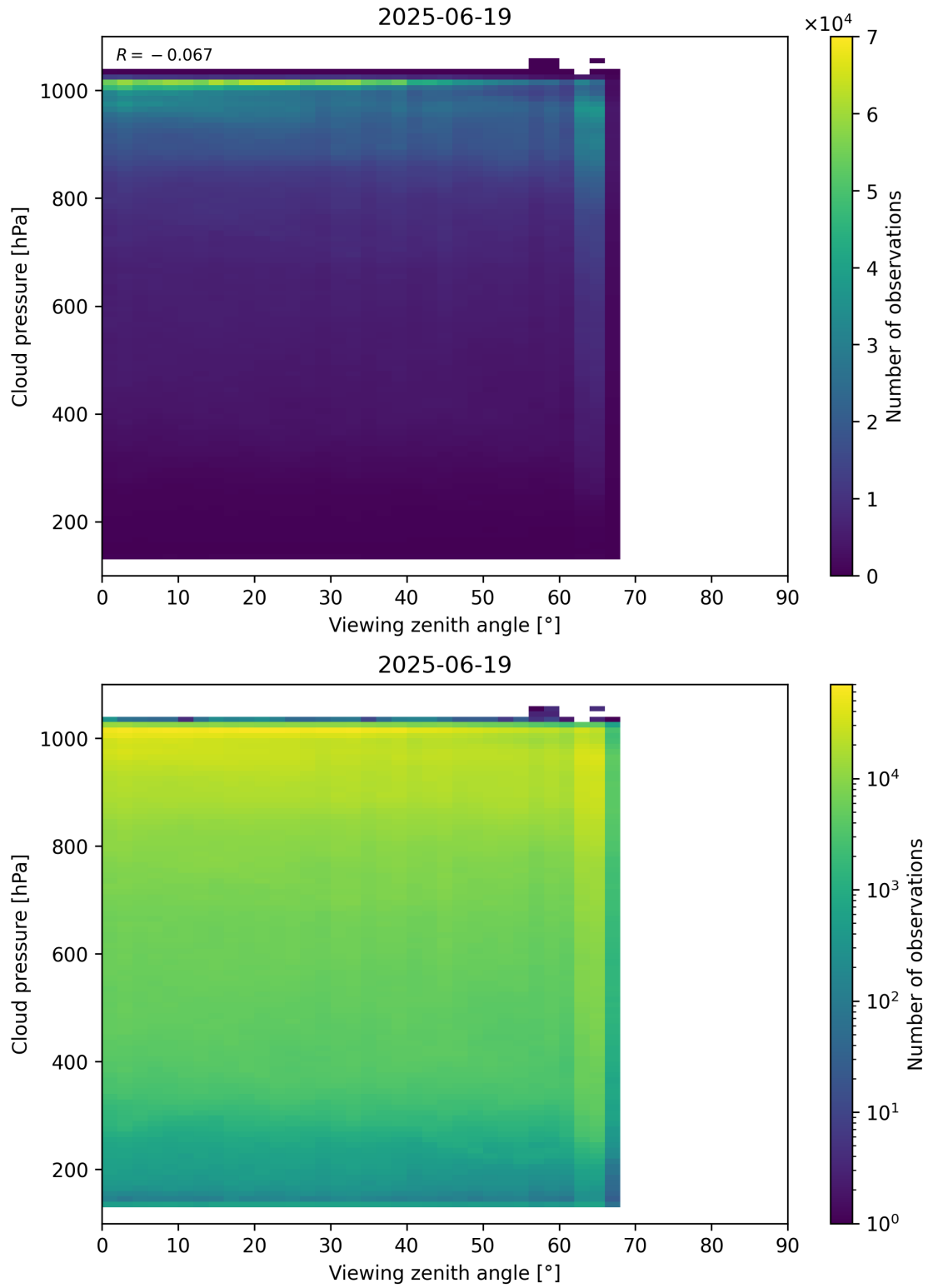
Figure 121: Scatter density plot of “Viewing zenith angle” against “Cloud pressure” for 2025-06-18 to 2025-06-20.
