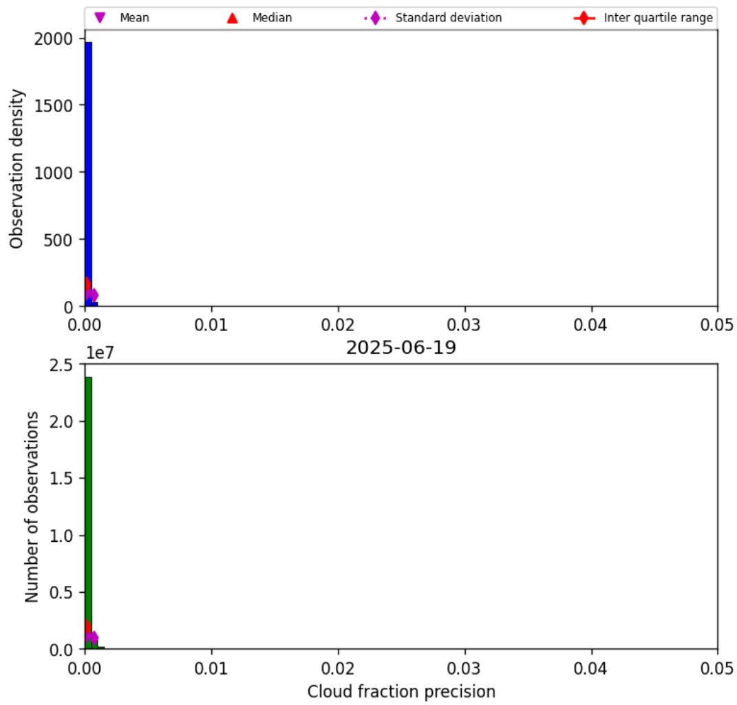
Figure 33: Histogram of “Cloud fraction precision” for 2025-06-18 to 2025-06-20
