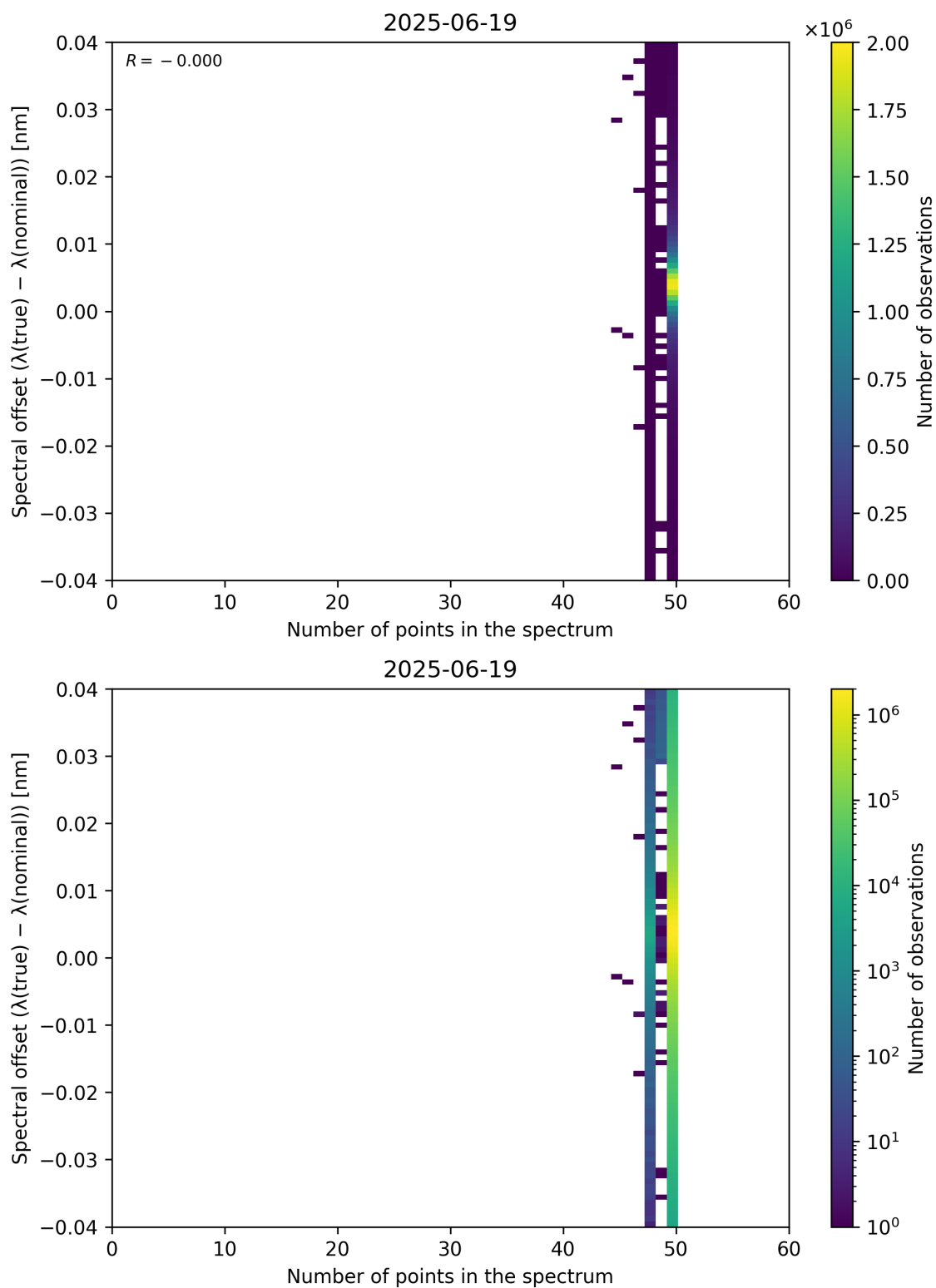
Figure 101: Scatter density plot of “Number of points in the spectrum” against “Spectral offset ( \lambda_{\text{true}} - \lambda_{\text{nominal}} )” for 2025-06-18 to 2025-06-20.
