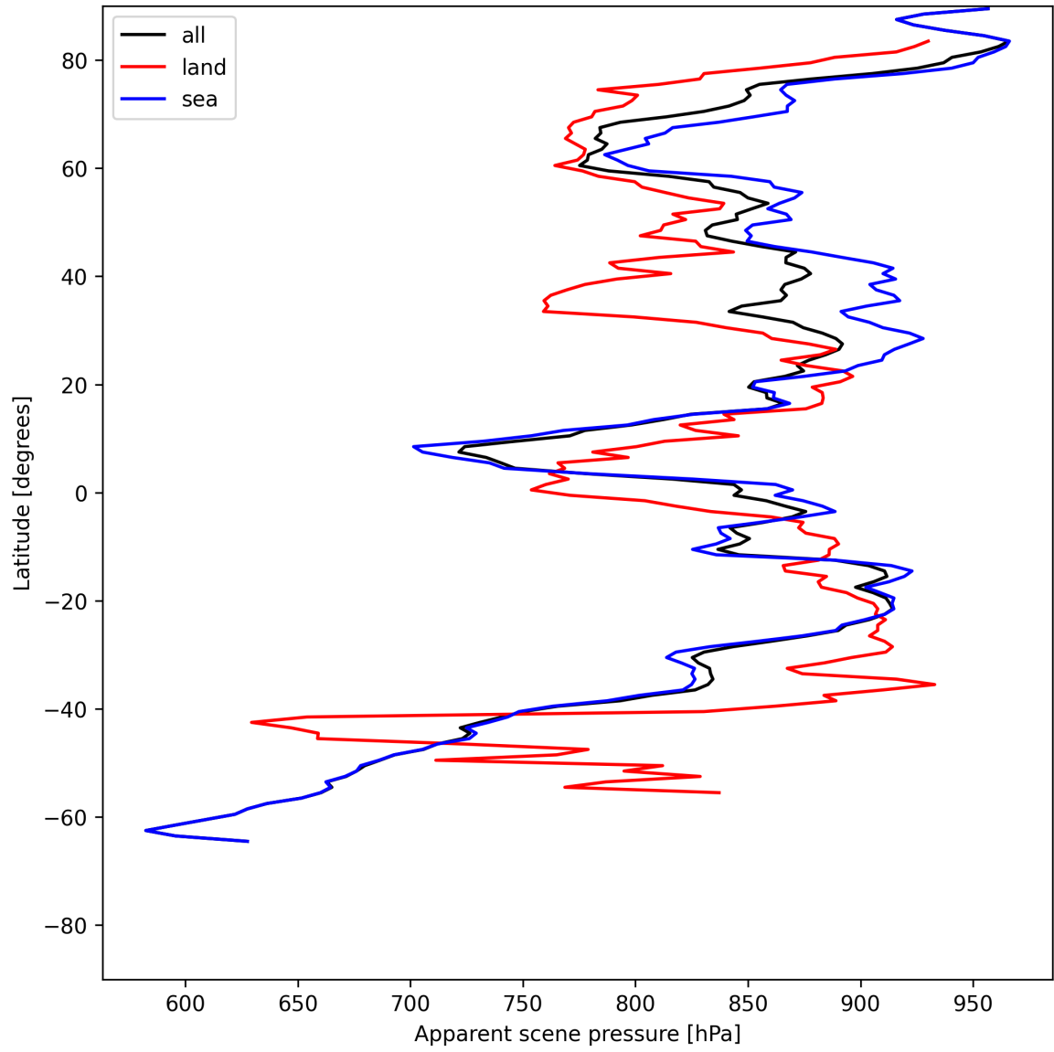
Figure 19: Zonal average of “Apparent scene pressure” for 2025-06-18 to 2025-06-20.
