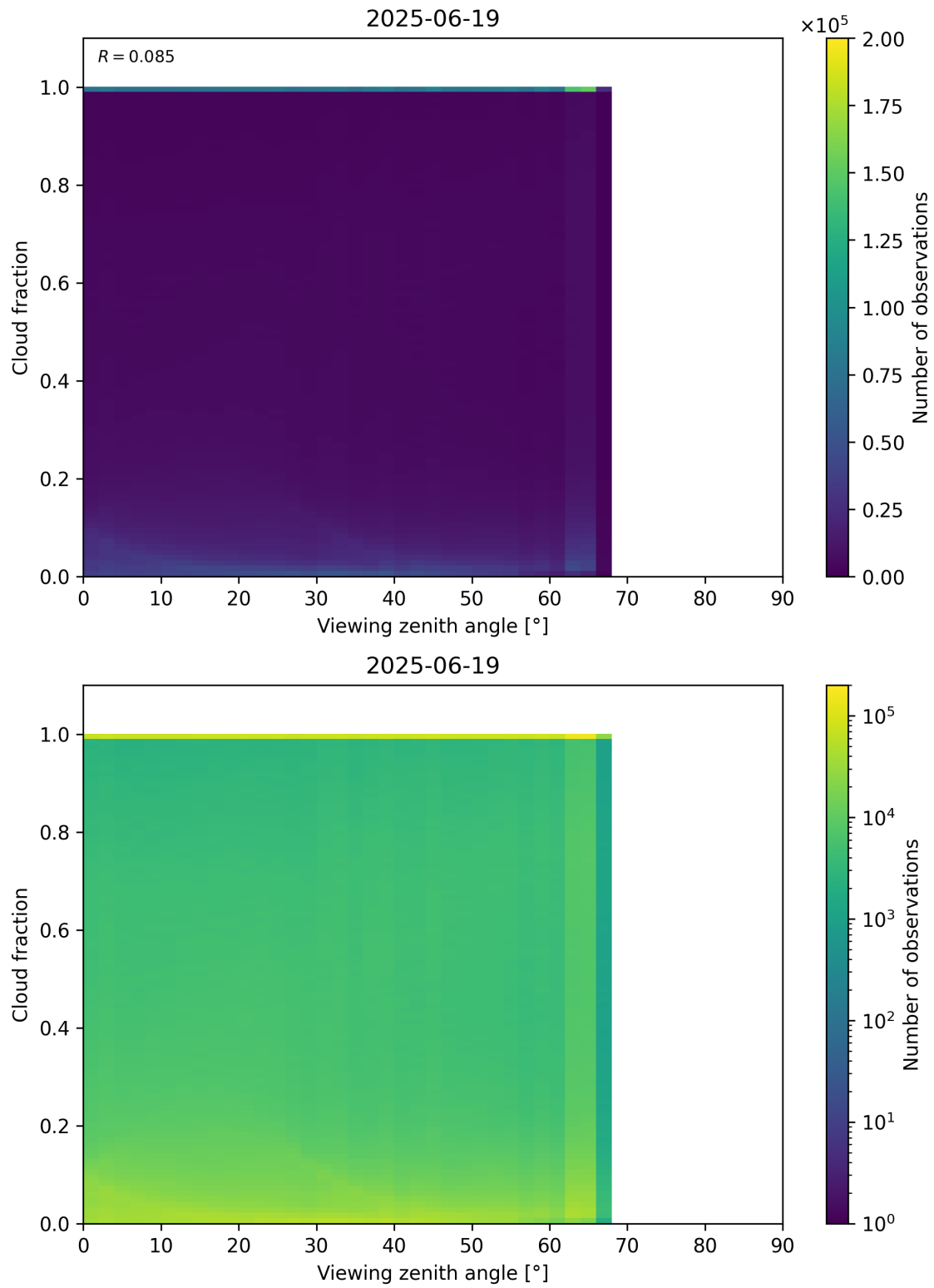
Figure 120: Scatter density plot of “Viewing zenith angle” against “Cloud fraction” for 2025-06-18 to 2025-06-20.
