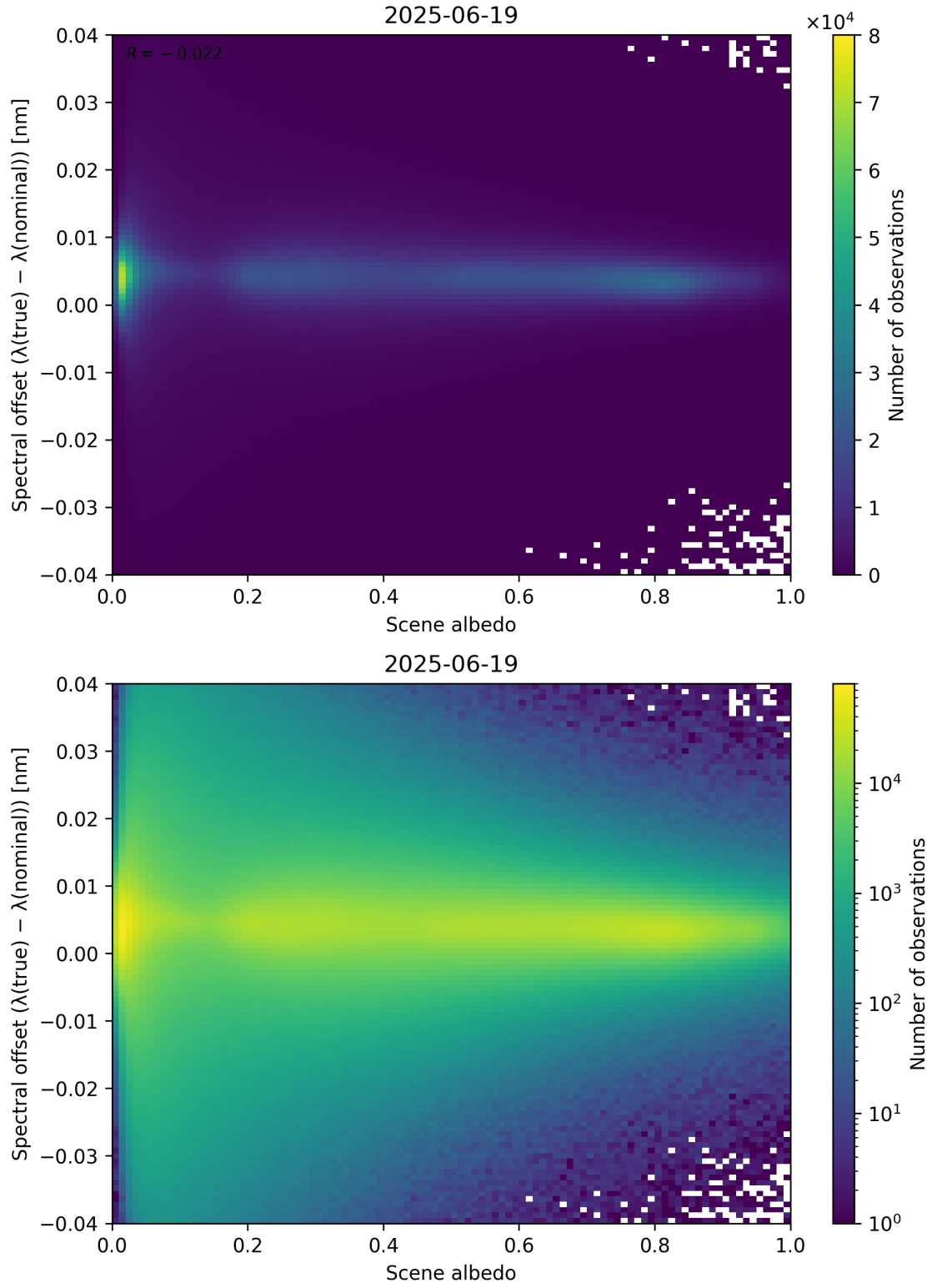
Figure 107: Scatter density plot of “Scene albedo” against “Spectral offset ( \lambda_{\text{true}} - \lambda_{\text{nominal}} )” for 2025-06-18 to 2025-06-20.
