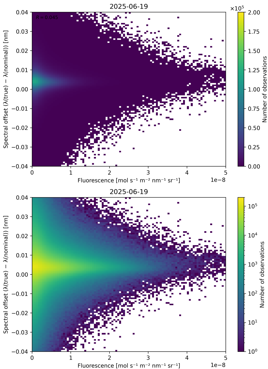
Figure 87: Scatter density plot of “Fluorescence” against “Spectral offset ( \lambda_{\text{true}} - \lambda_{\text{nominal}} )” for 2025-06-18 to 2025-06-20.
