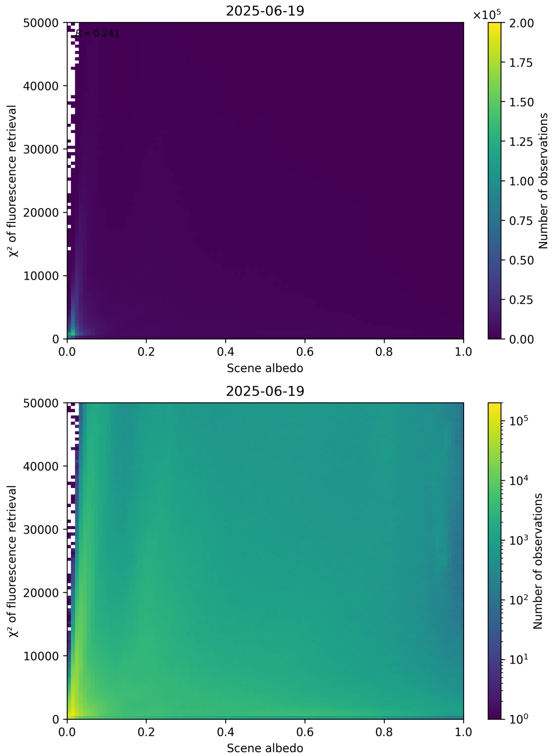
Figure 103: Scatter density plot of “Scene albedo” against “ \chi^2 of fluorescence retrieval” for 2025-06-18 to 2025-06-20.
