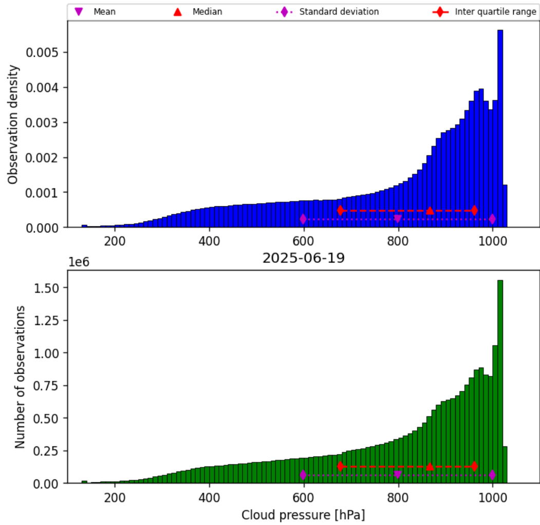
Figure 30: Histogram of “Cloud pressure” for 2025-06-18 to 2025-06-20
