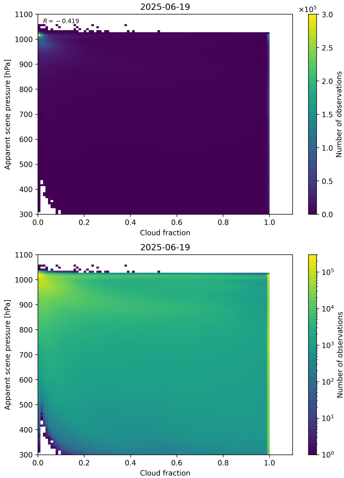
Figure 70: Scatter density plot of “Cloud fraction” against “Apparent scene pressure” for 2025-06-18 to 2025-06-20.
