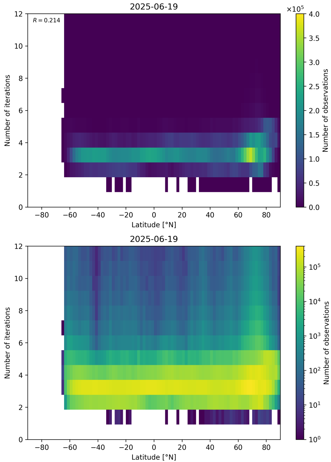
Figure 93: Scatter density plot of “Latitude” against “Number of iterations” for 2025-06-18 to 2025-06-20.
