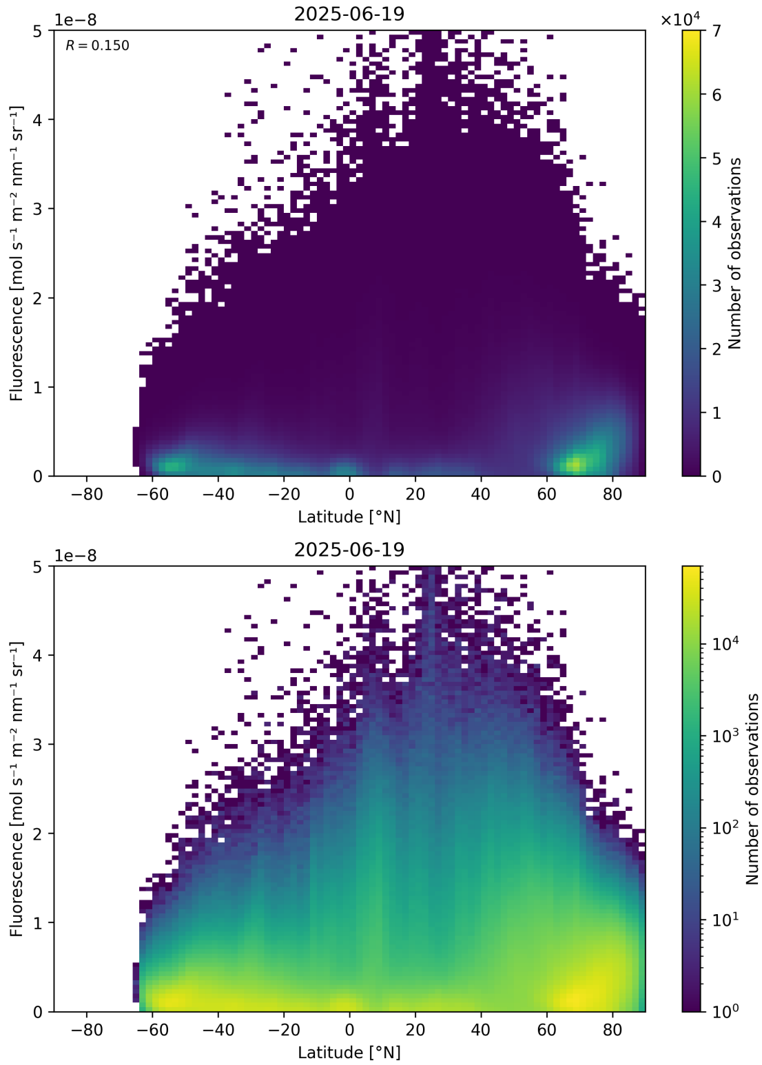
Figure 92: Scatter density plot of “Latitude” against “Fluorescence” for 2025-06-18 to 2025-06-20.
