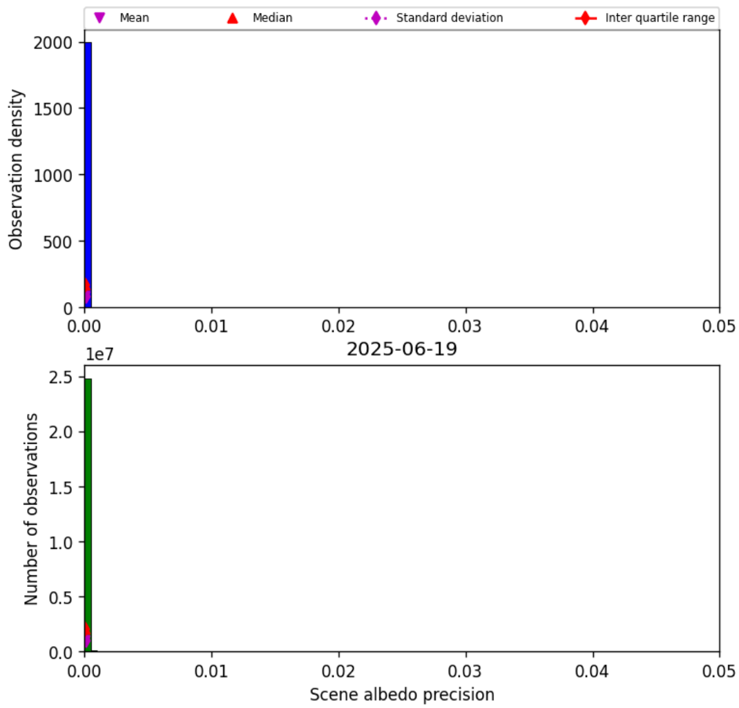
Figure 35: Histogram of “Scene albedo precision” for 2025-06-18 to 2025-06-20
