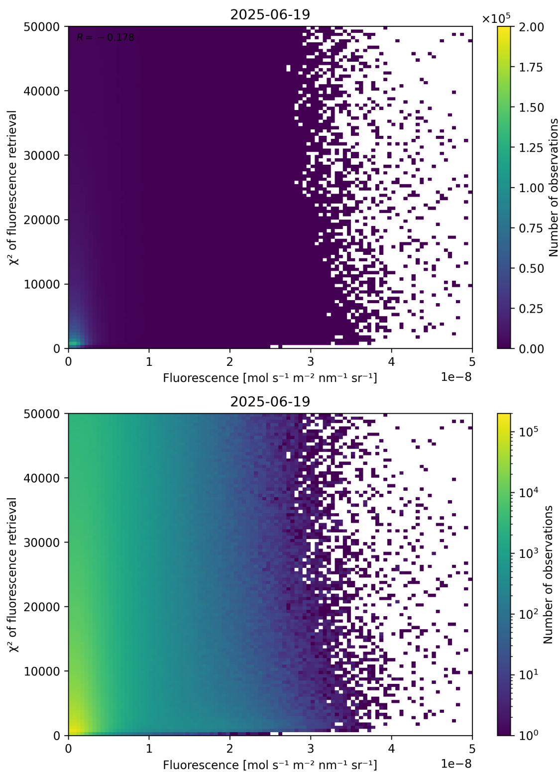
Figure 85: Scatter density plot of “Fluorescence” against “ \chi^2 of fluorescence retrieval” for 2025-06-18 to 2025-06-20.
