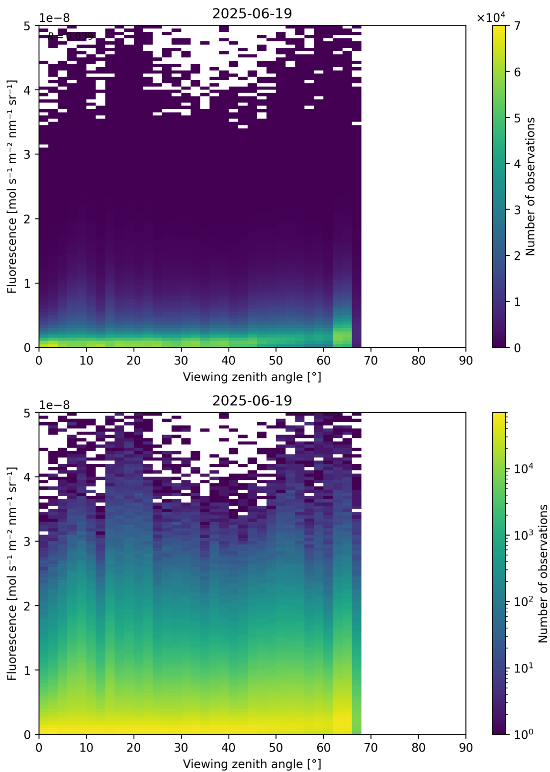
Figure 122: Scatter density plot of “Viewing zenith angle” against “Fluorescence” for 2025-06-18 to 2025-06-20.
