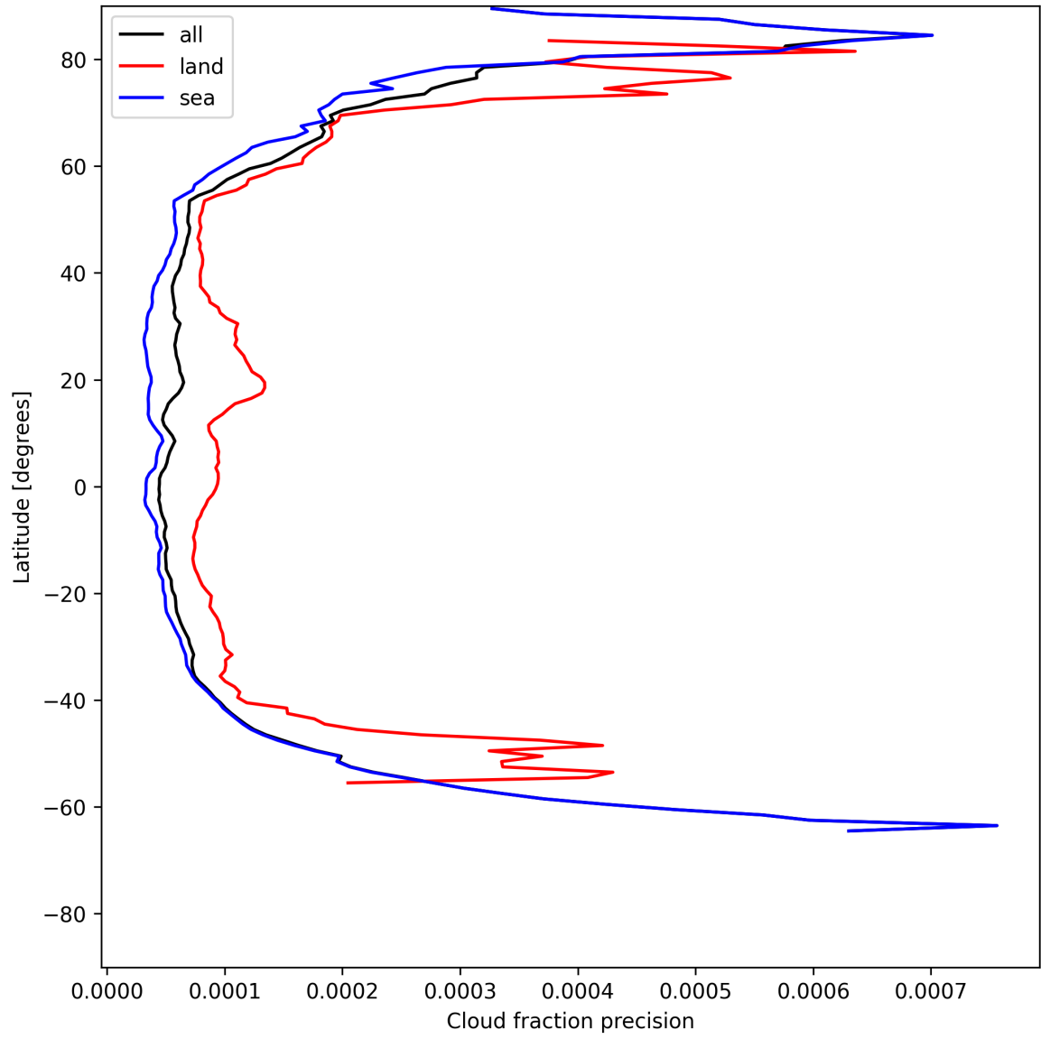
Figure 16: Zonal average of “Cloud fraction precision” for 2025-06-18 to 2025-06-20.
