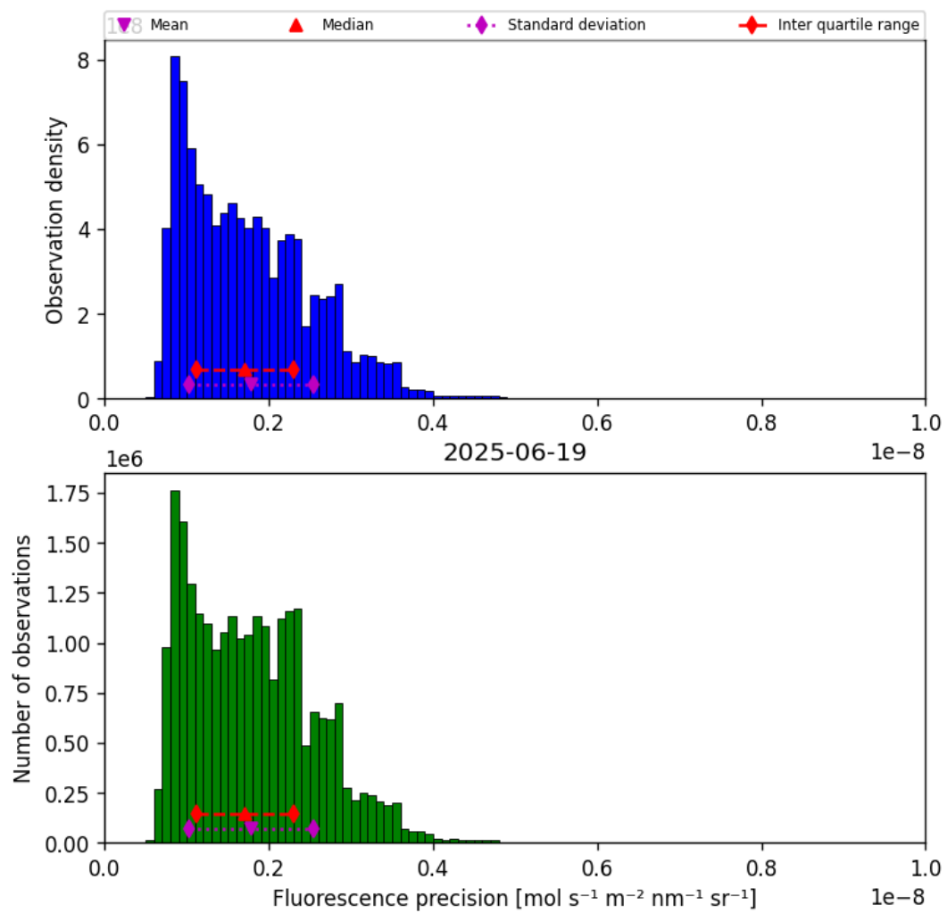
Figure 41: Histogram of “Fluorescence precision” for 2025-06-18 to 2025-06-20
