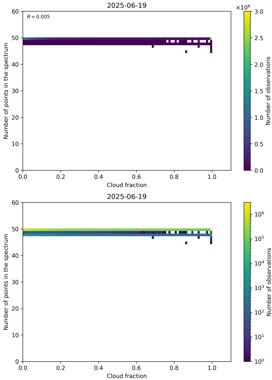
Figure 74: Scatter density plot of “Cloud fraction” against “Number of points in the spectrum” for 2025-06-18 to 2025-06-20.
