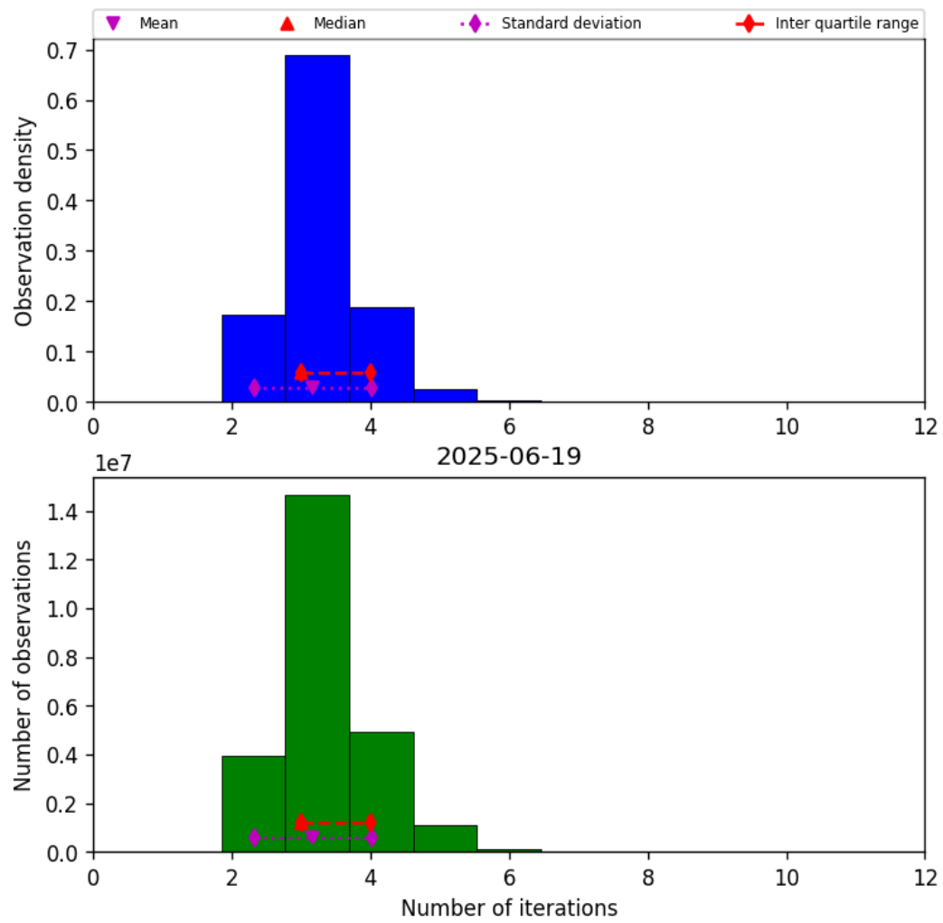
Figure 39: Histogram of “Number of iterations” for 2025-06-18 to 2025-06-20
