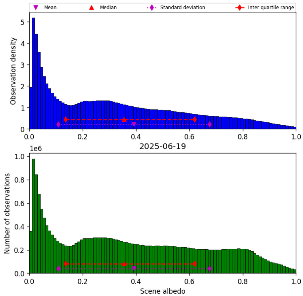
Figure 34: Histogram of “Scene albedo” for 2025-06-18 to 2025-06-20
