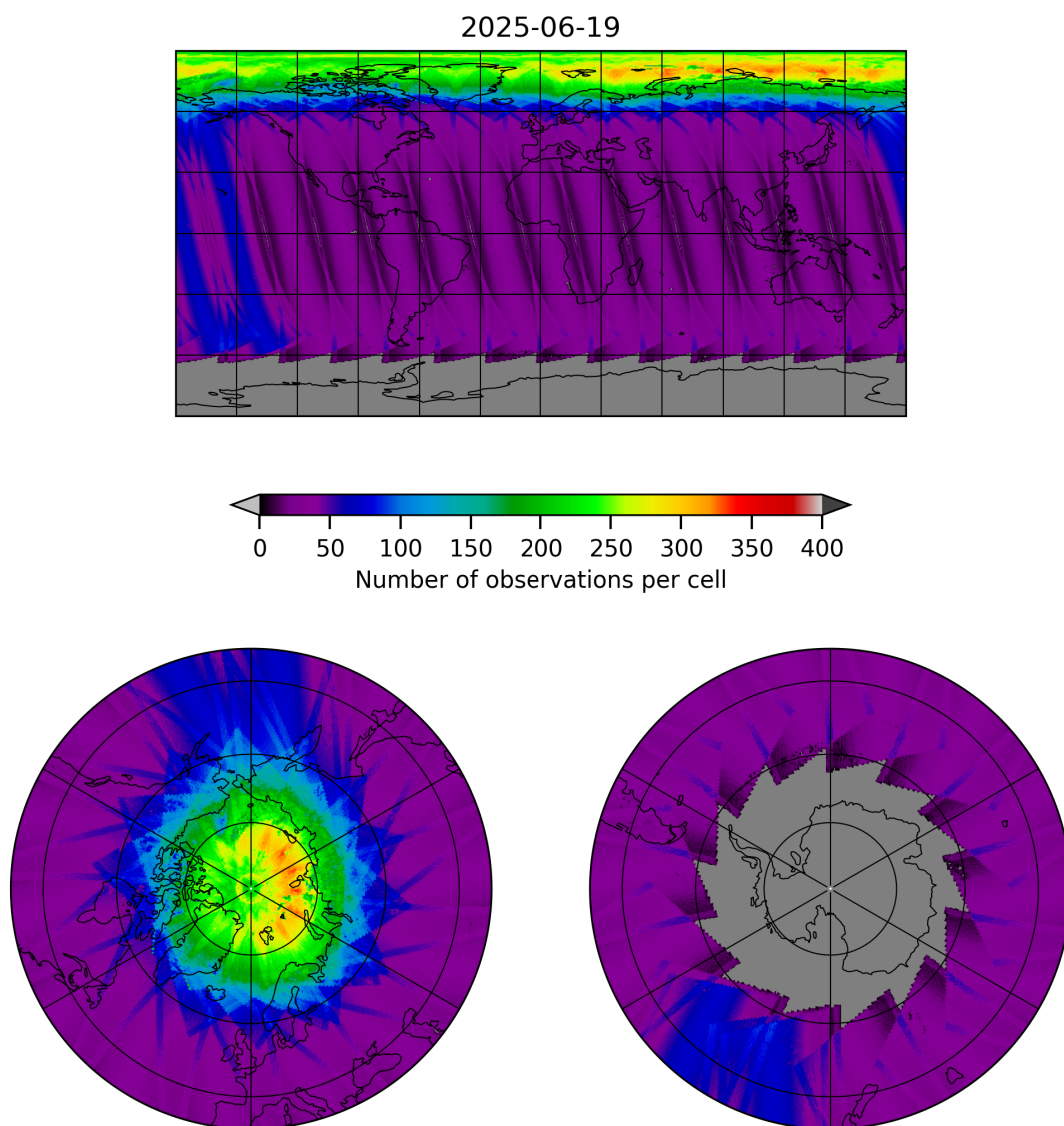
Figure 11: Map of the number of observations for 2025-06-18 to 2025-06-20
