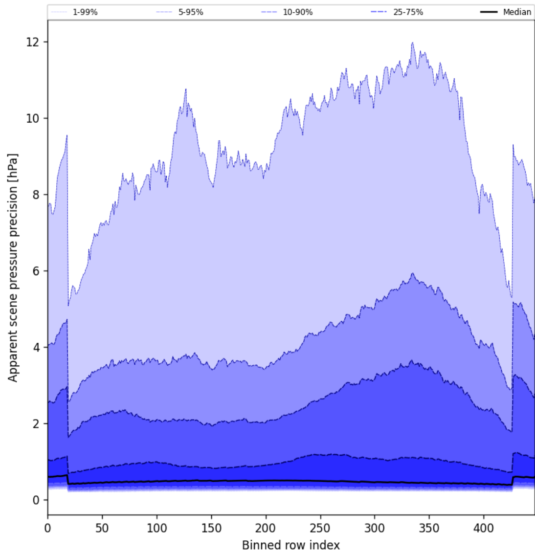
Figure 54: Along track statistics of “Apparent scene pressure precision” for 2025-06-18 to 2025-06-20
