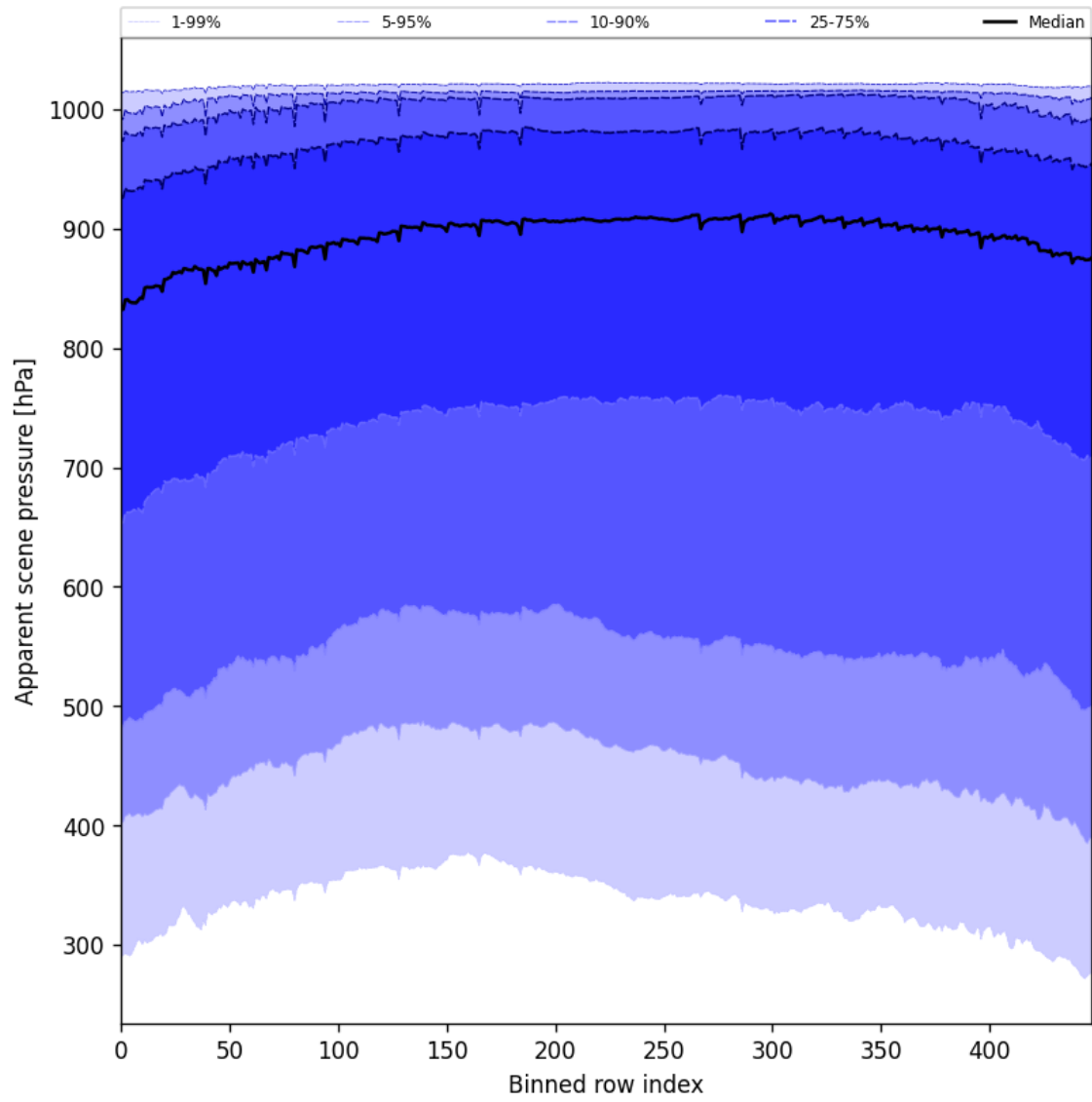
Figure 53: Along track statistics of “Apparent scene pressure” for 2025-06-18 to 2025-06-20
