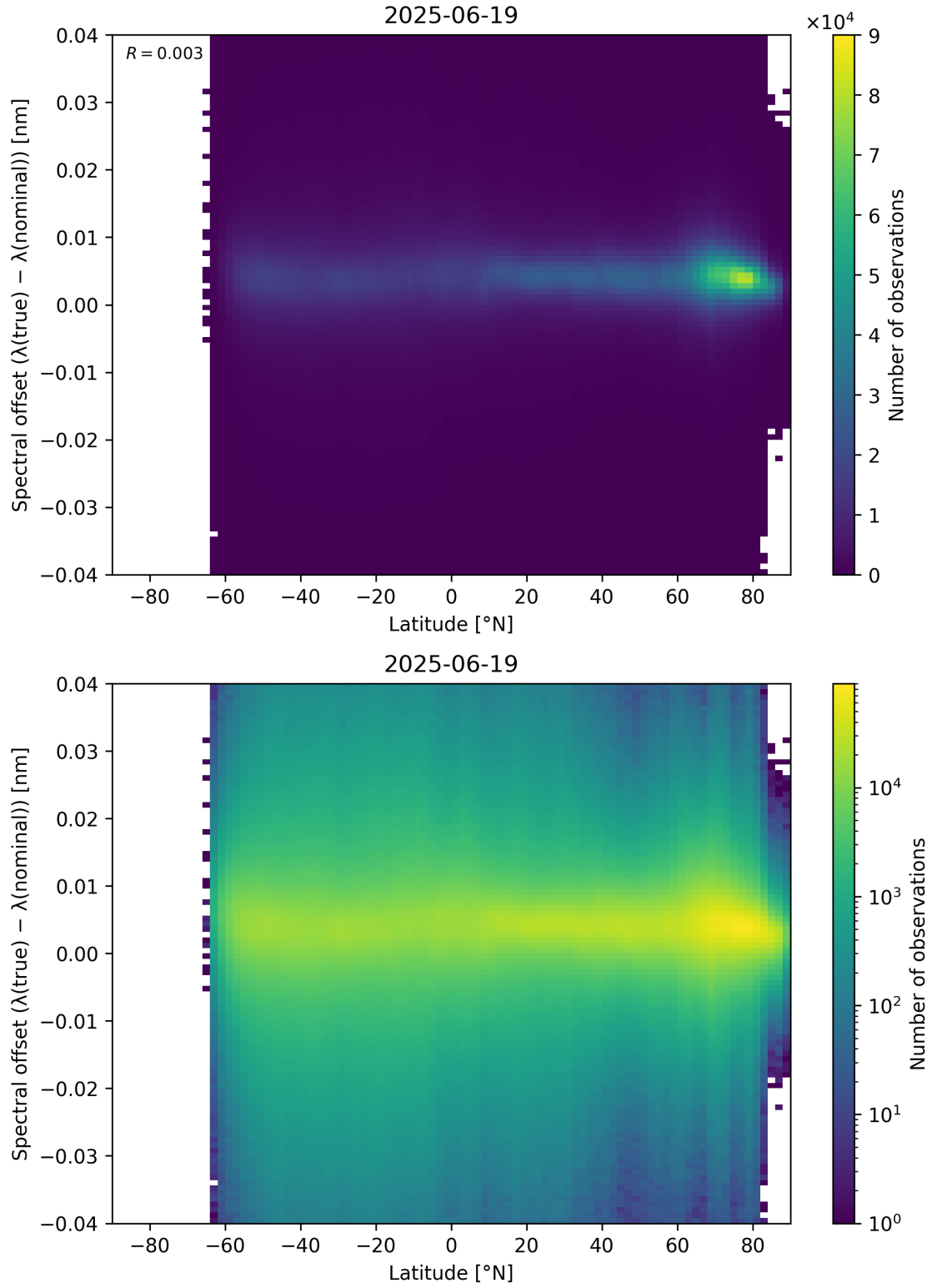
Figure 96: Scatter density plot of “Latitude” against “Spectral offset ( \lambda_{\text{true}} - \lambda_{\text{nominal}} )” for 2025-06-18 to 2025-06-20.
