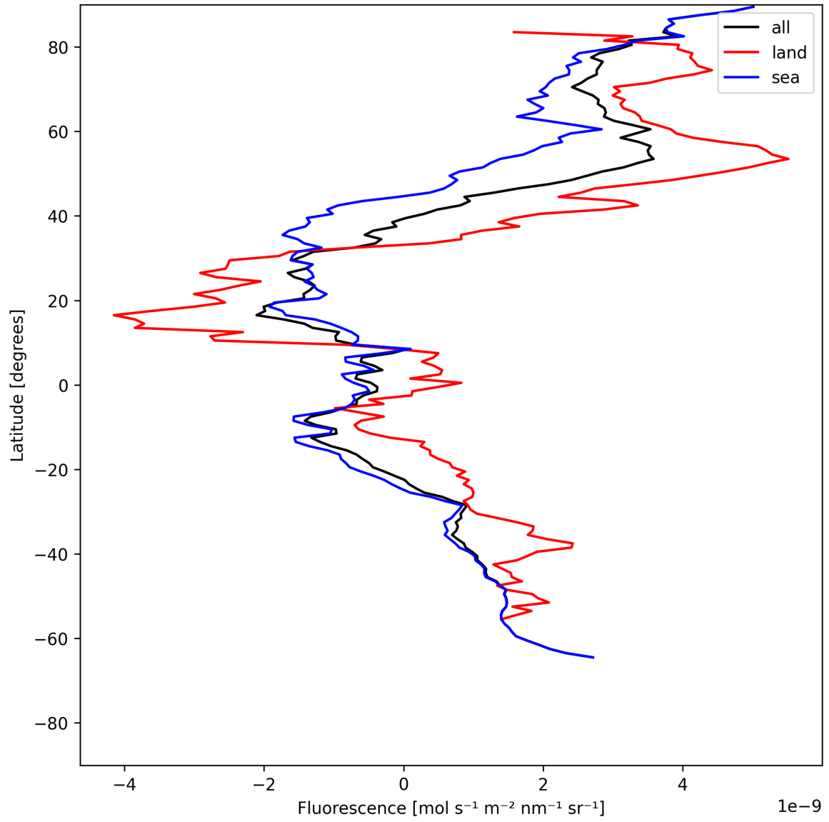
Figure 23: Zonal average of “Fluorescence” for 2025-06-18 to 2025-06-20.
