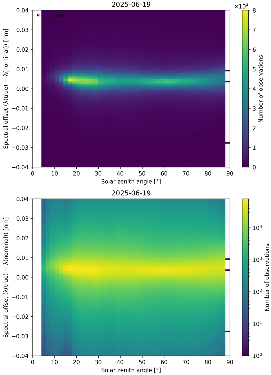
Figure 117: Scatter density plot of “Solar zenith angle” against “Spectral offset ( \lambda_{\text{true}} - \lambda_{\text{nominal}} )” for 2025-06-18 to 2025-06-20.
