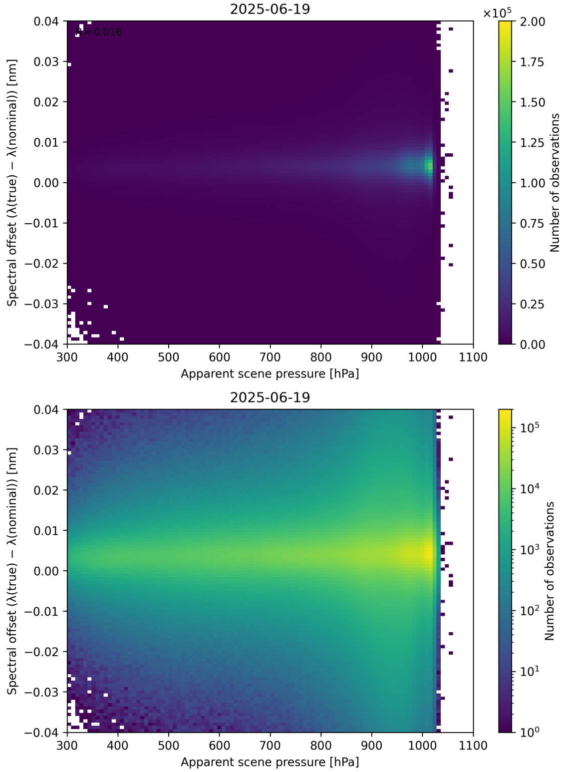
Figure 67: Scatter density plot of “Apparent scene pressure” against “Spectral offset ( \lambda_{\text{true}} - \lambda_{\text{nominal}} )” for 2025-06-18 to 2025-06-20.
