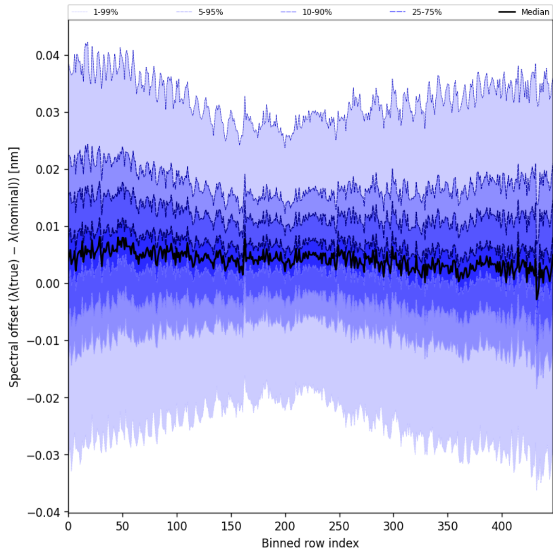
Figure 62: Along track statistics of “Spectral offset ( \lambda_{\text{true}} - \lambda_{\text{nominal}} )” for 2025-06-18 to 2025-06-20
