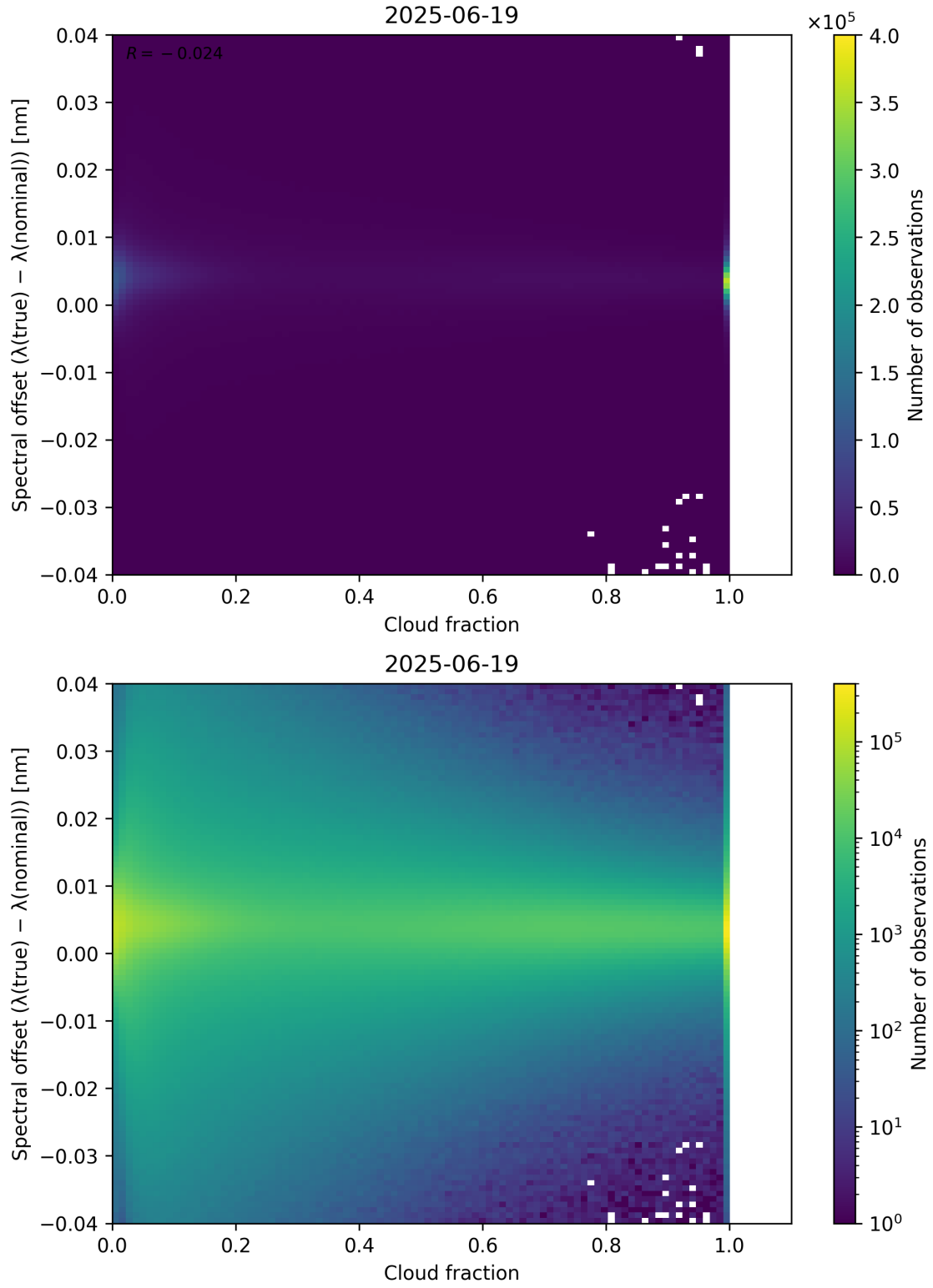
Figure 76: Scatter density plot of “Cloud fraction” against “Spectral offset ( \lambda_{\text{true}} - \lambda_{\text{nominal}} )” for 2025-06-18 to 2025-06-20.
