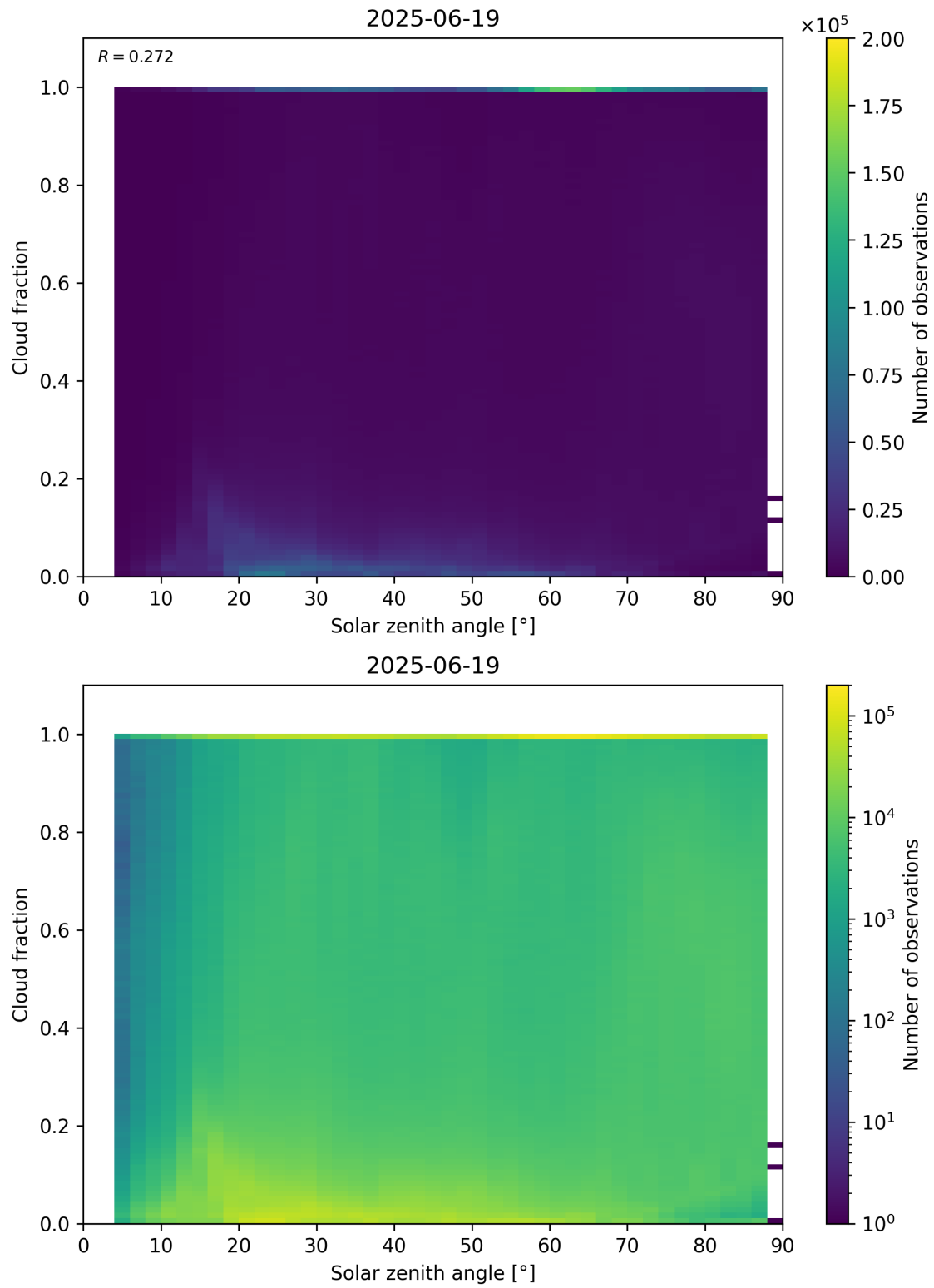
Figure 110: Scatter density plot of “Solar zenith angle” against “Cloud fraction” for 2025-06-18 to 2025-06-20.
