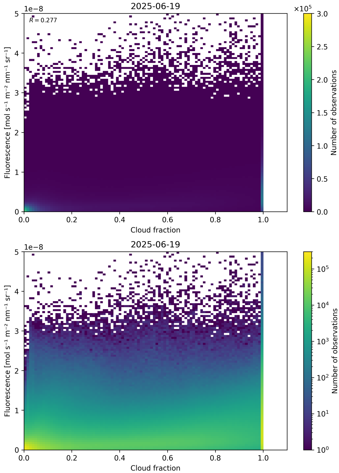
Figure 72: Scatter density plot of “Cloud fraction” against “Fluorescence” for 2025-06-18 to 2025-06-20.
