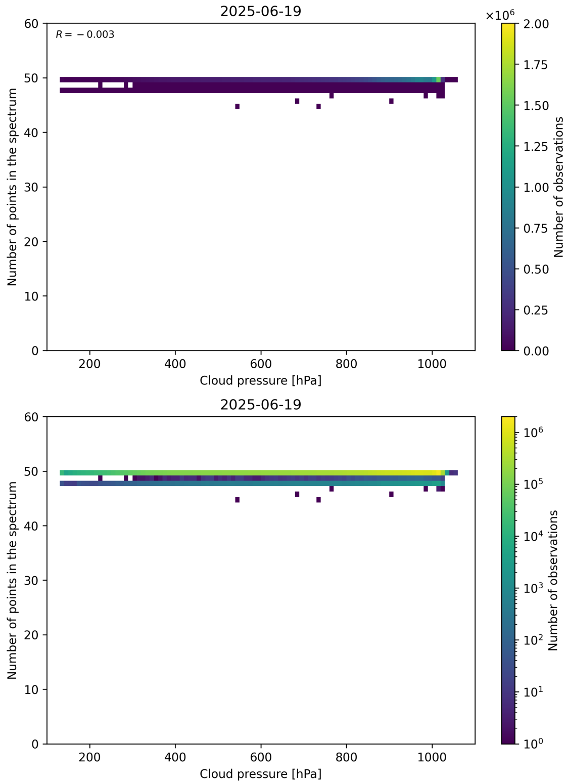
Figure 82: Scatter density plot of “Cloud pressure” against “Number of points in the spectrum” for 2025-06-18 to 2025-06-20.
