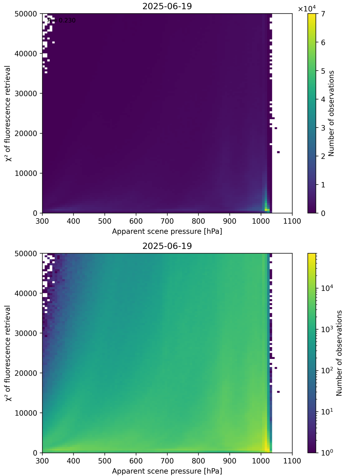
Figure 63: Scatter density plot of “Apparent scene pressure” against “ \chi^2 of fluorescence retrieval” for 2025-06-18 to 2025-06-20.
