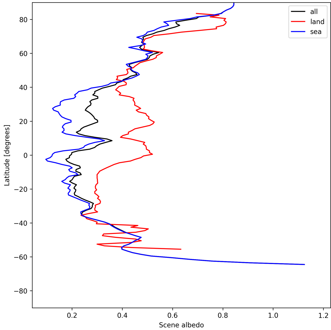
Figure 17: Zonal average of “Scene albedo” for 2025-06-18 to 2025-06-20.
