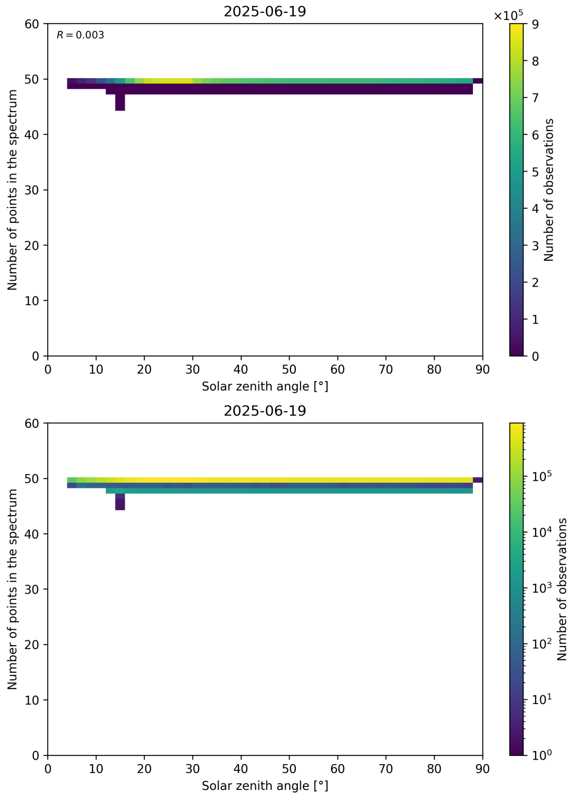
Figure 115: Scatter density plot of “Solar zenith angle” against “Number of points in the spectrum” for 2025-06-18 to 2025-06-20.
