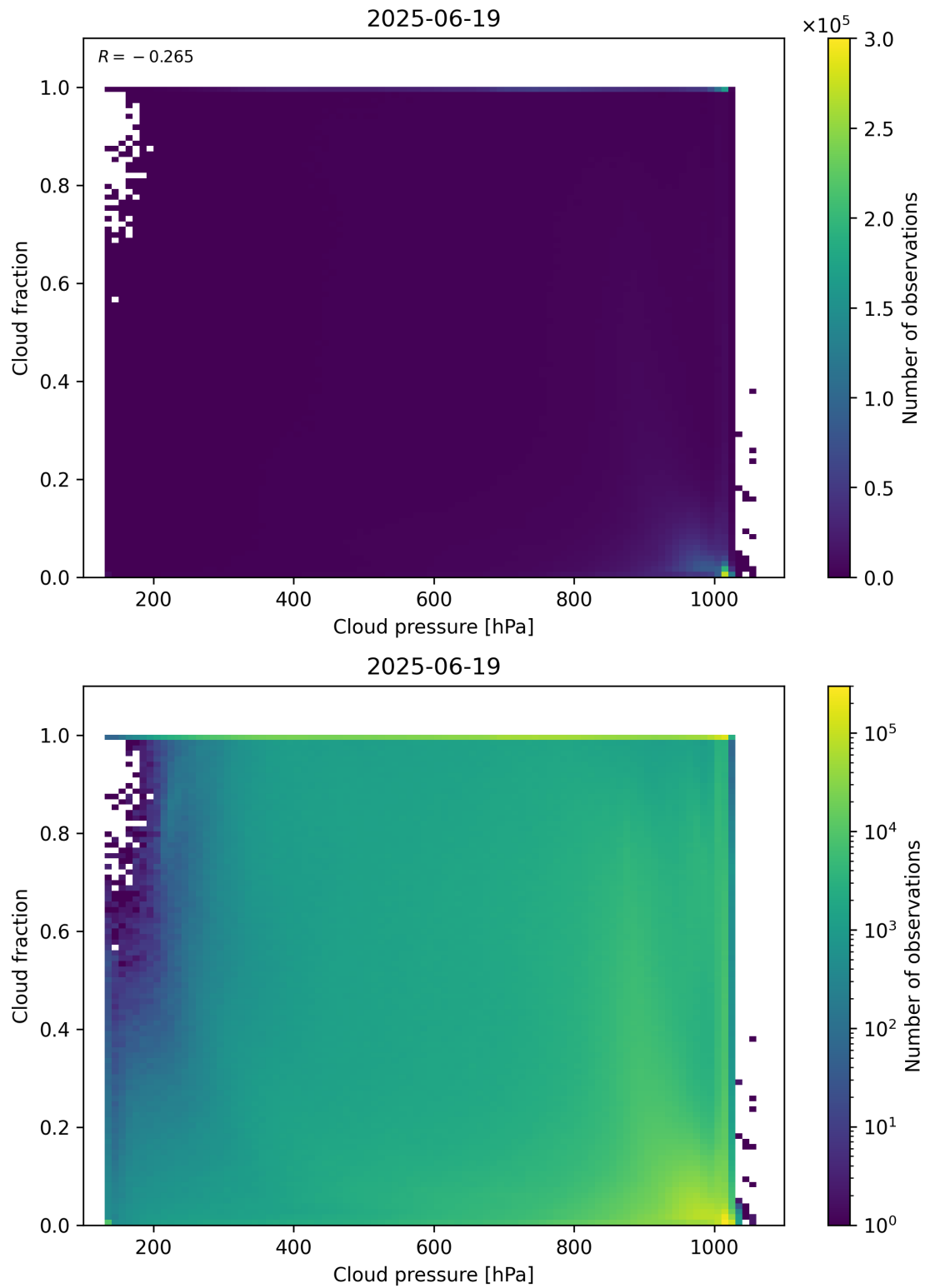
Figure 79: Scatter density plot of “Cloud pressure” against “Cloud fraction” for 2025-06-18 to 2025-06-20.
