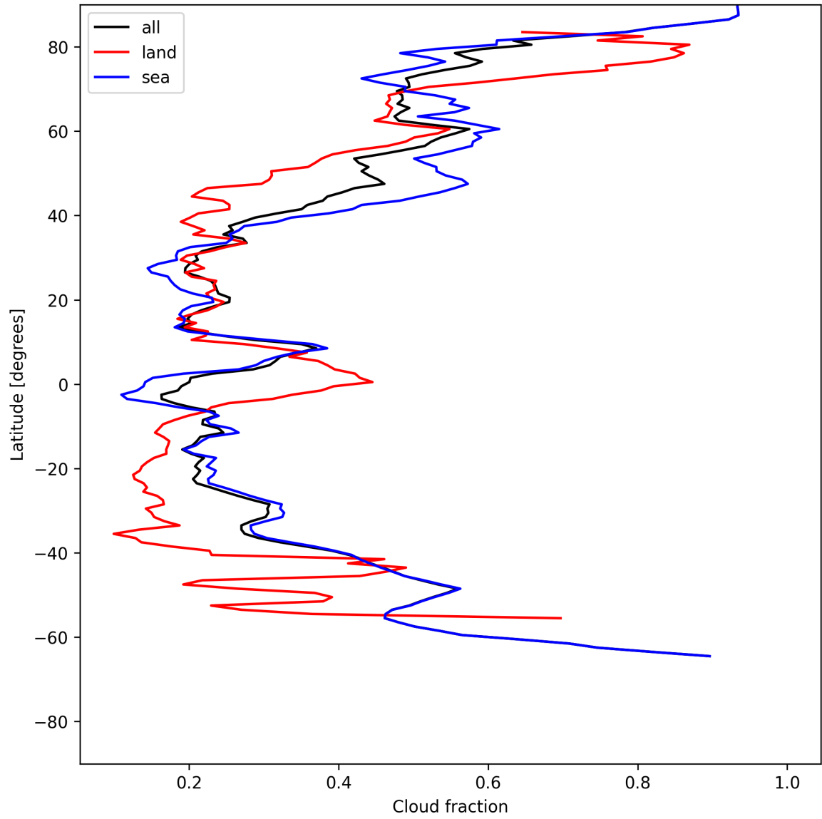
Figure 15: Zonal average of “Cloud fraction” for 2025-06-18 to 2025-06-20.
