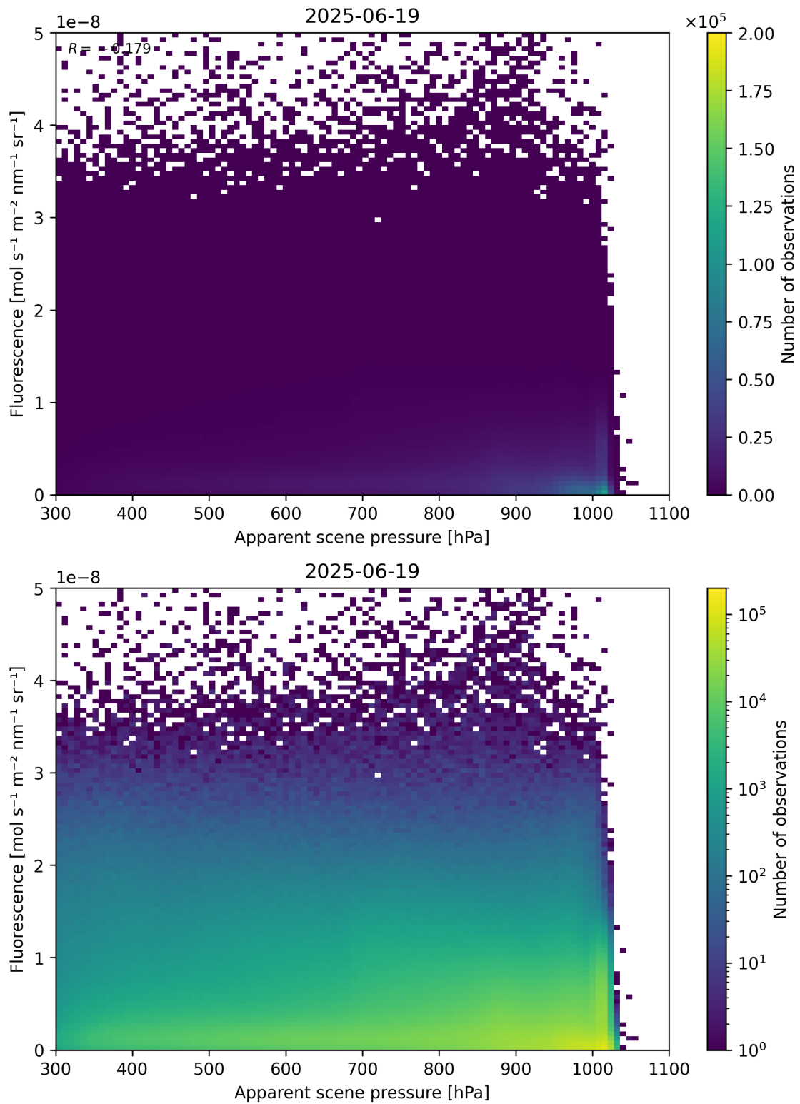
Figure 64: Scatter density plot of “Apparent scene pressure” against “Fluorescence” for 2025-06-18 to 2025-06-20.
