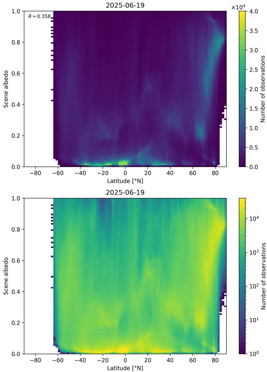
Figure 95: Scatter density plot of “Latitude” against “Scene albedo” for 2025-06-18 to 2025-06-20.
