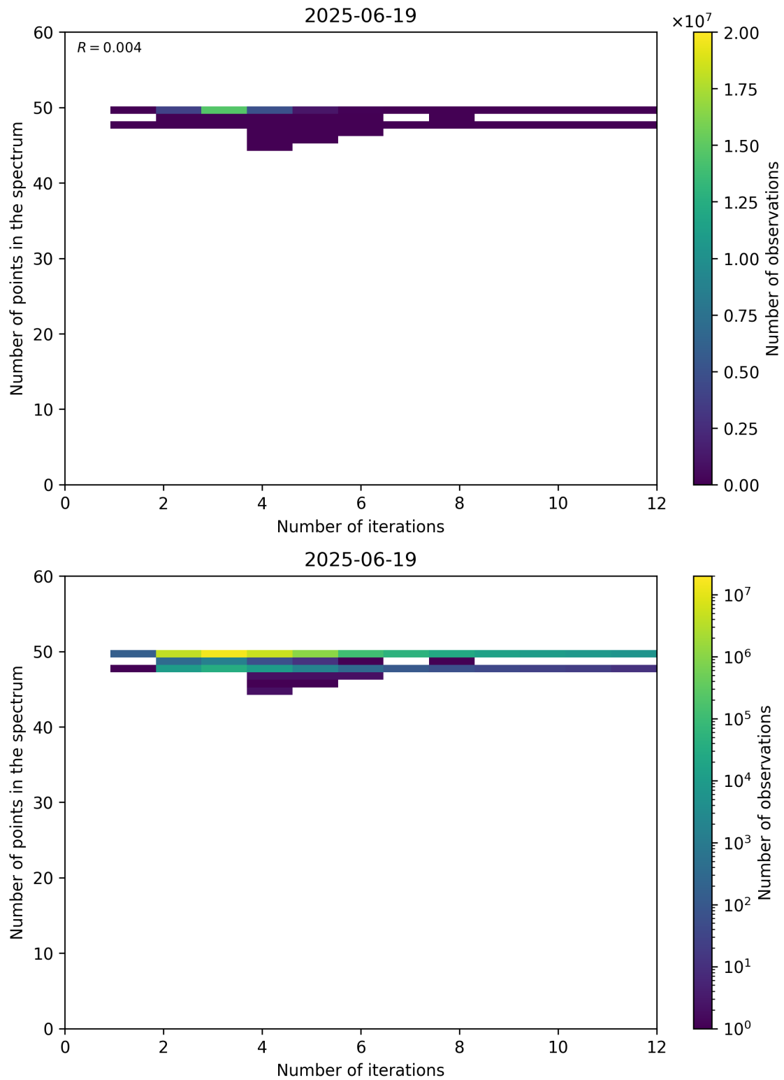
Figure 99: Scatter density plot of “Number of iterations” against “Number of points in the spectrum” for 2025-06-18 to 2025-06-20.
