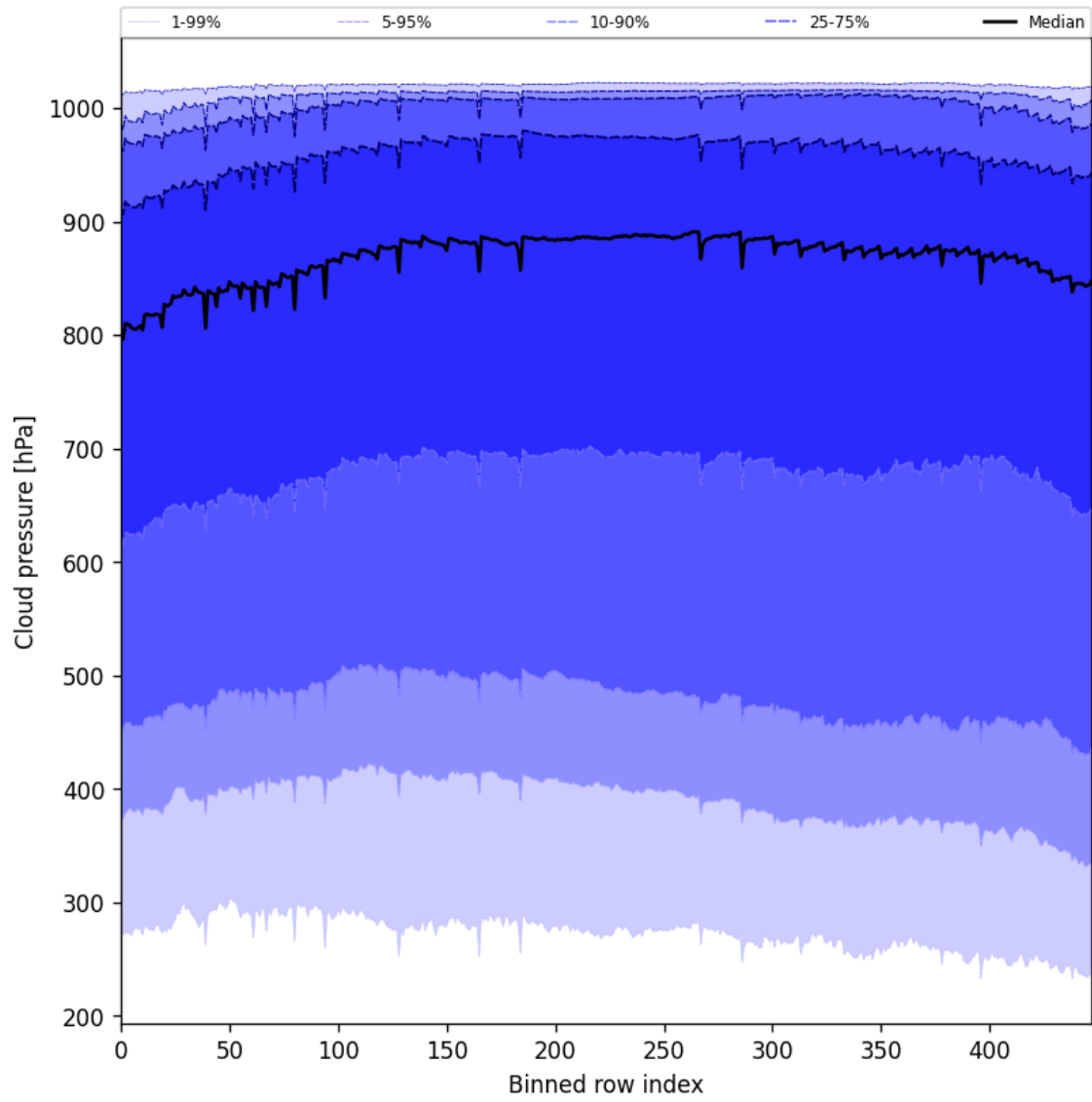
Figure 47: Along track statistics of “Cloud pressure” for 2025-06-18 to 2025-06-20
