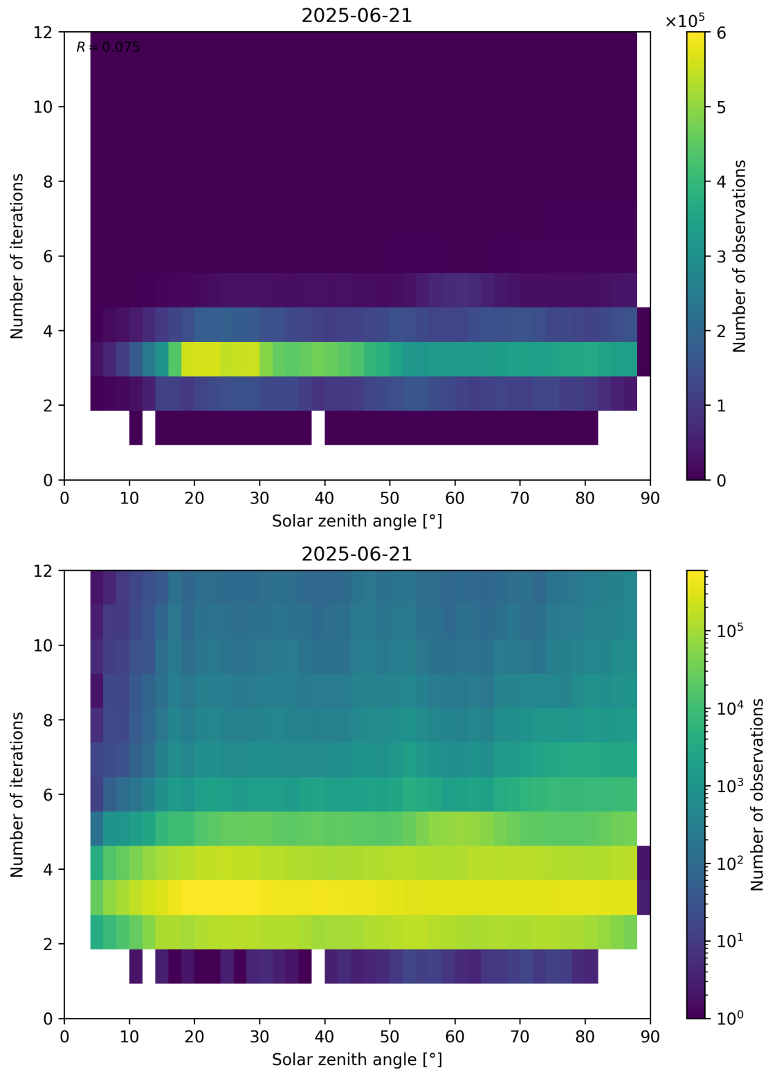
Figure 114: Scatter density plot of “Solar zenith angle” against “Number of iterations” for 2025-06-20 to 2025-06-22.
