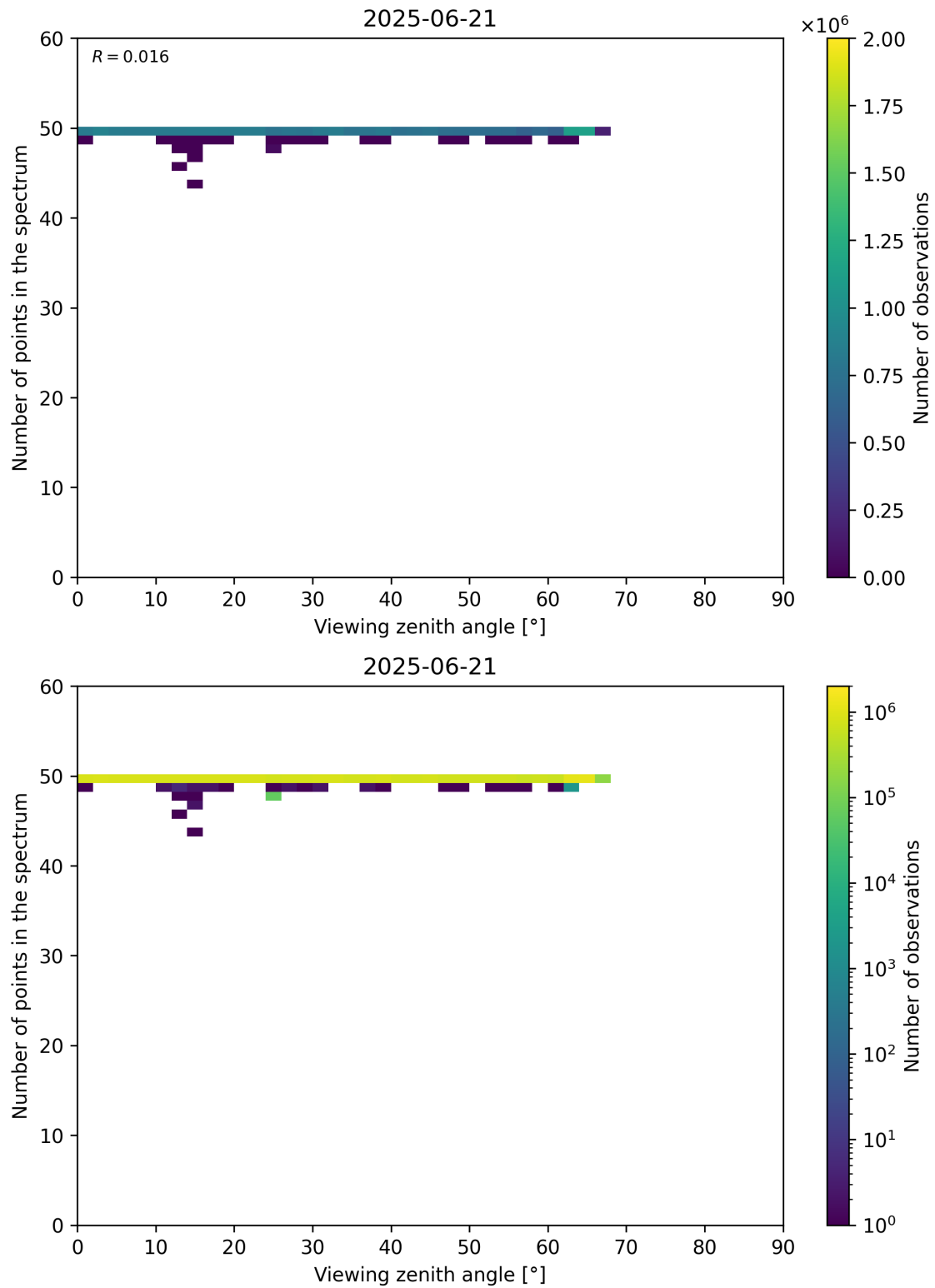
Figure 125: Scatter density plot of “Viewing zenith angle” against “Number of points in the spectrum” for 2025-06-20 to 2025-06-22.
