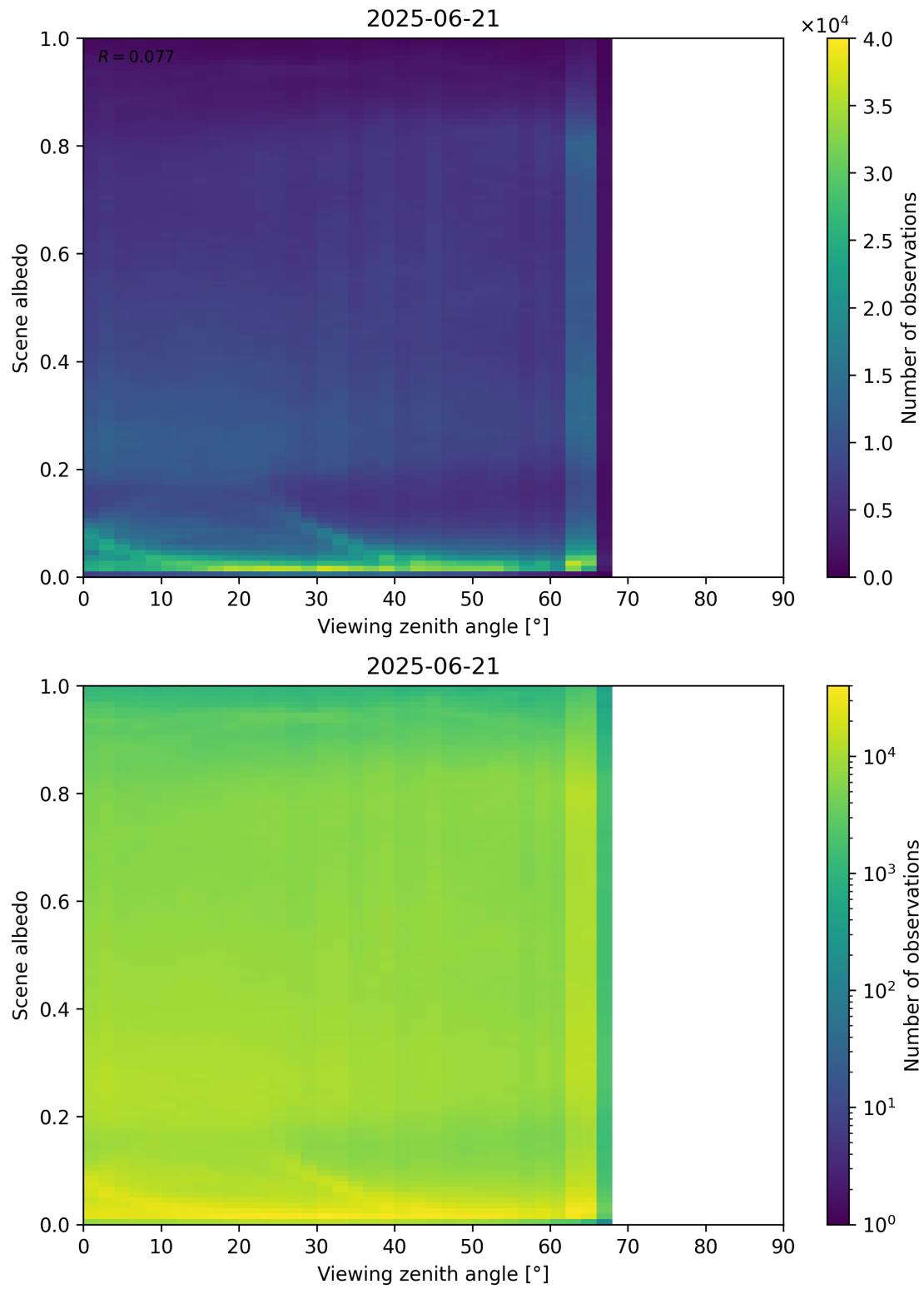
Figure 126: Scatter density plot of “Viewing zenith angle” against “Scene albedo” for 2025-06-20 to 2025-06-22.
