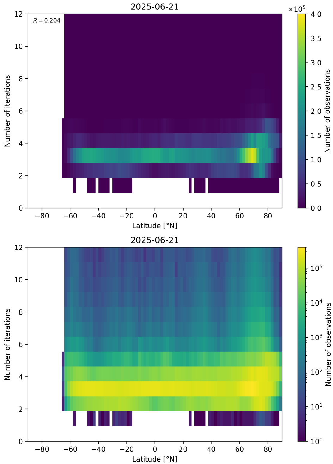
Figure 93: Scatter density plot of “Latitude” against “Number of iterations” for 2025-06-20 to 2025-06-22.
