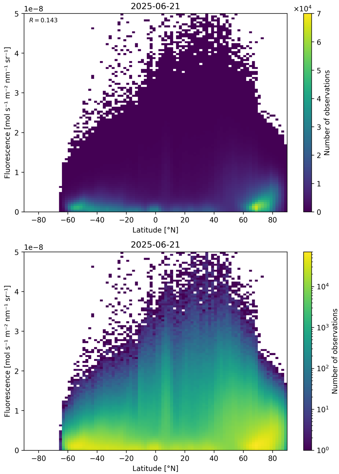
Figure 92: Scatter density plot of “Latitude” against “Fluorescence” for 2025-06-20 to 2025-06-22.
