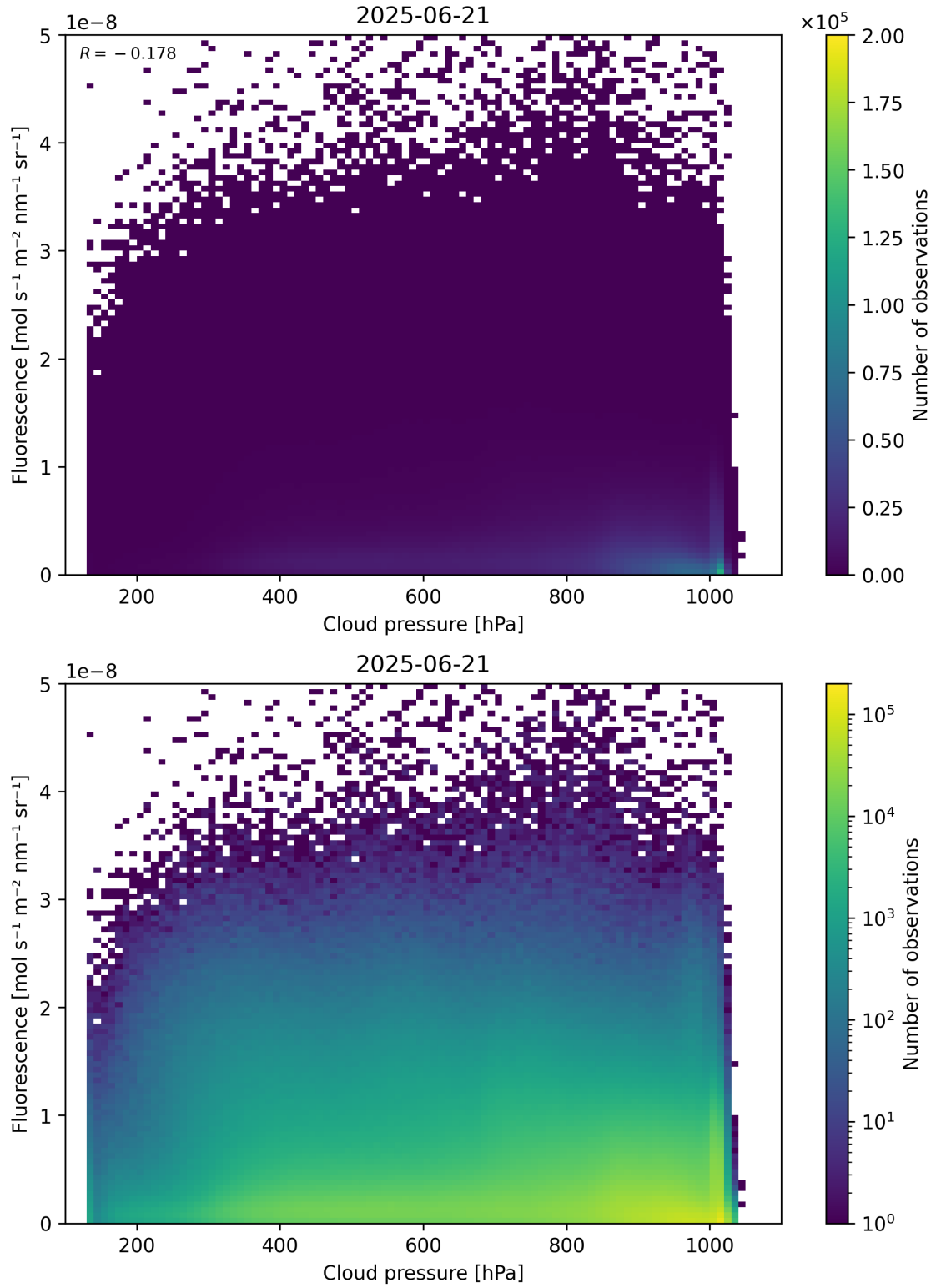
Figure 80: Scatter density plot of “Cloud pressure” against “Fluorescence” for 2025-06-20 to 2025-06-22.
