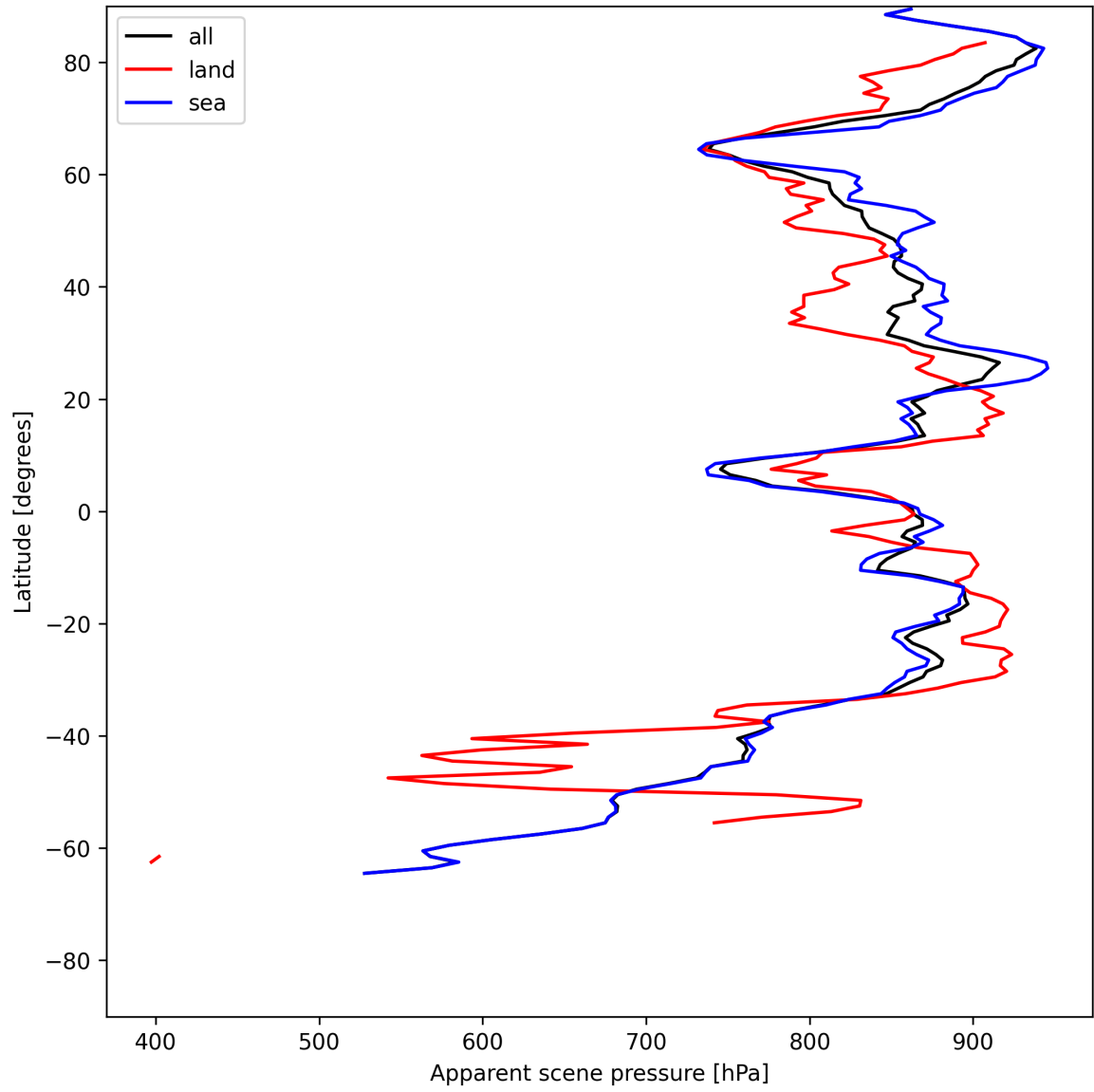
Figure 19: Zonal average of “Apparent scene pressure” for 2025-06-20 to 2025-06-22.
