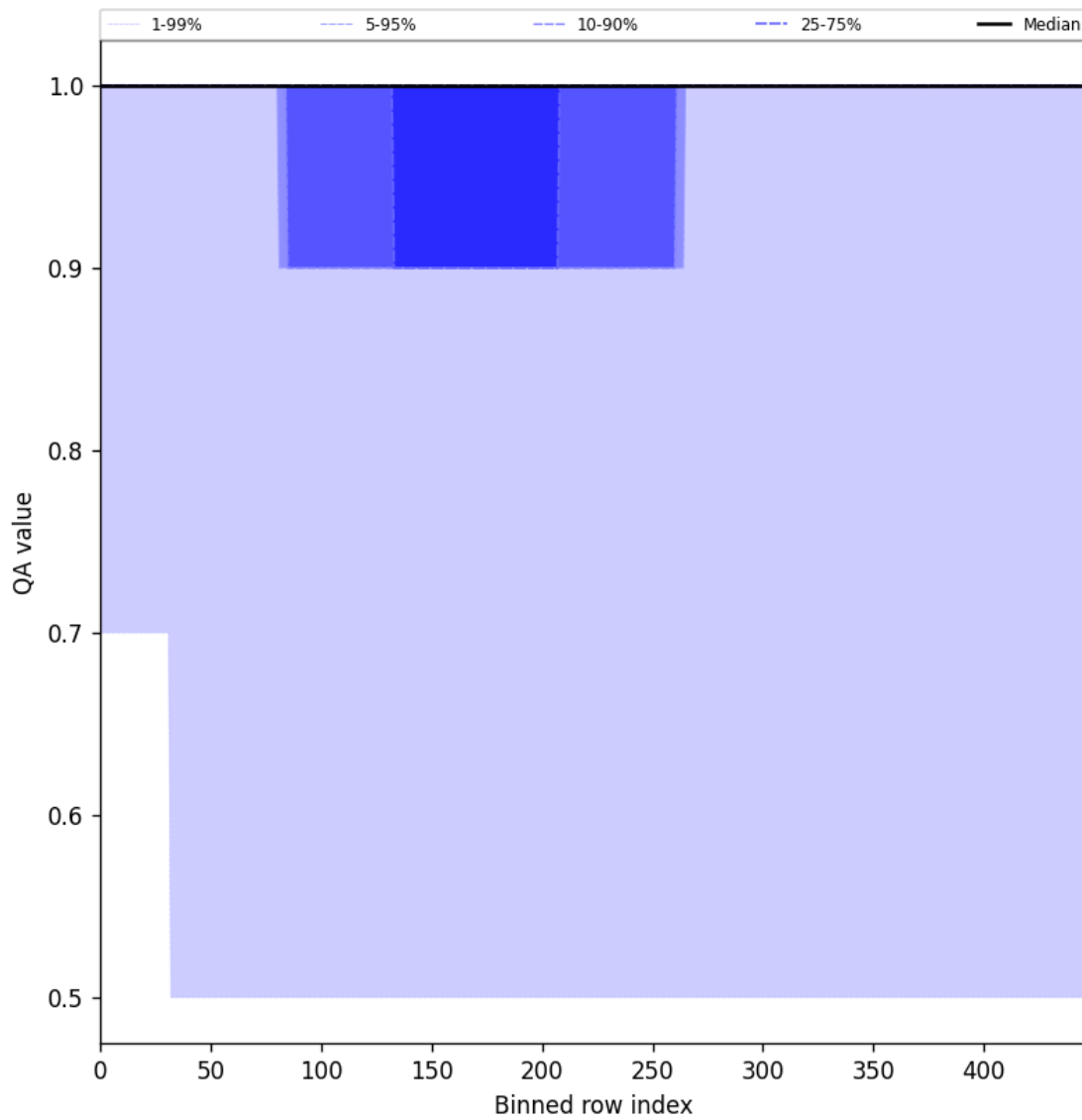
Figure 46: Along track statistics of “QA value” for 2025-06-20 to 2025-06-22
