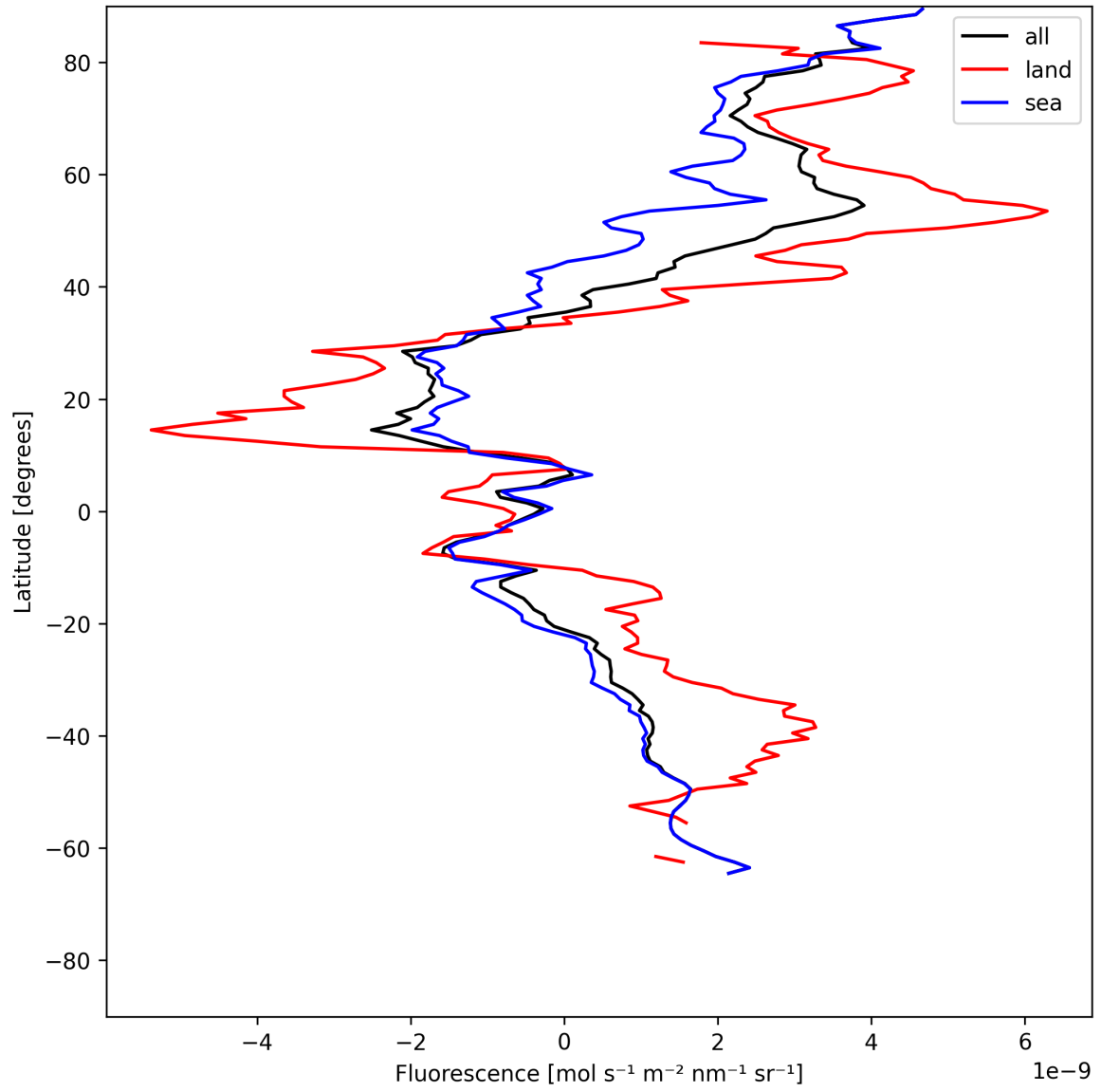
Figure 23: Zonal average of “Fluorescence” for 2025-06-20 to 2025-06-22.
