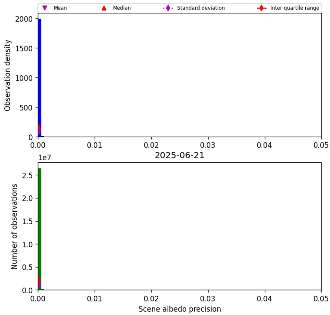
Figure 35: Histogram of “Scene albedo precision” for 2025-06-20 to 2025-06-22
