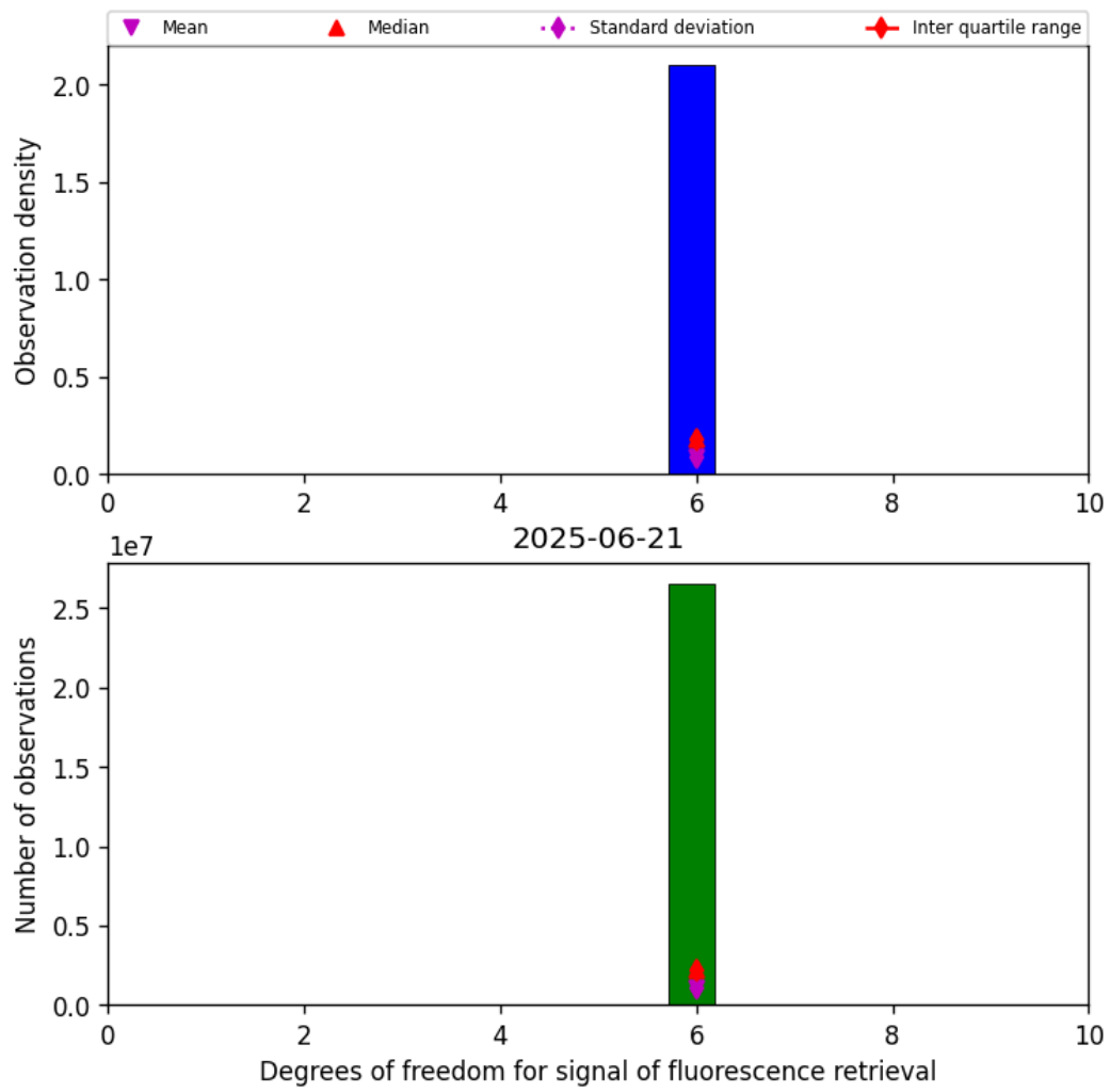
Figure 43: Histogram of "Degrees of freedom for signal of fluorescence retrieval" for 2025-06-20 to 2025-06-22
