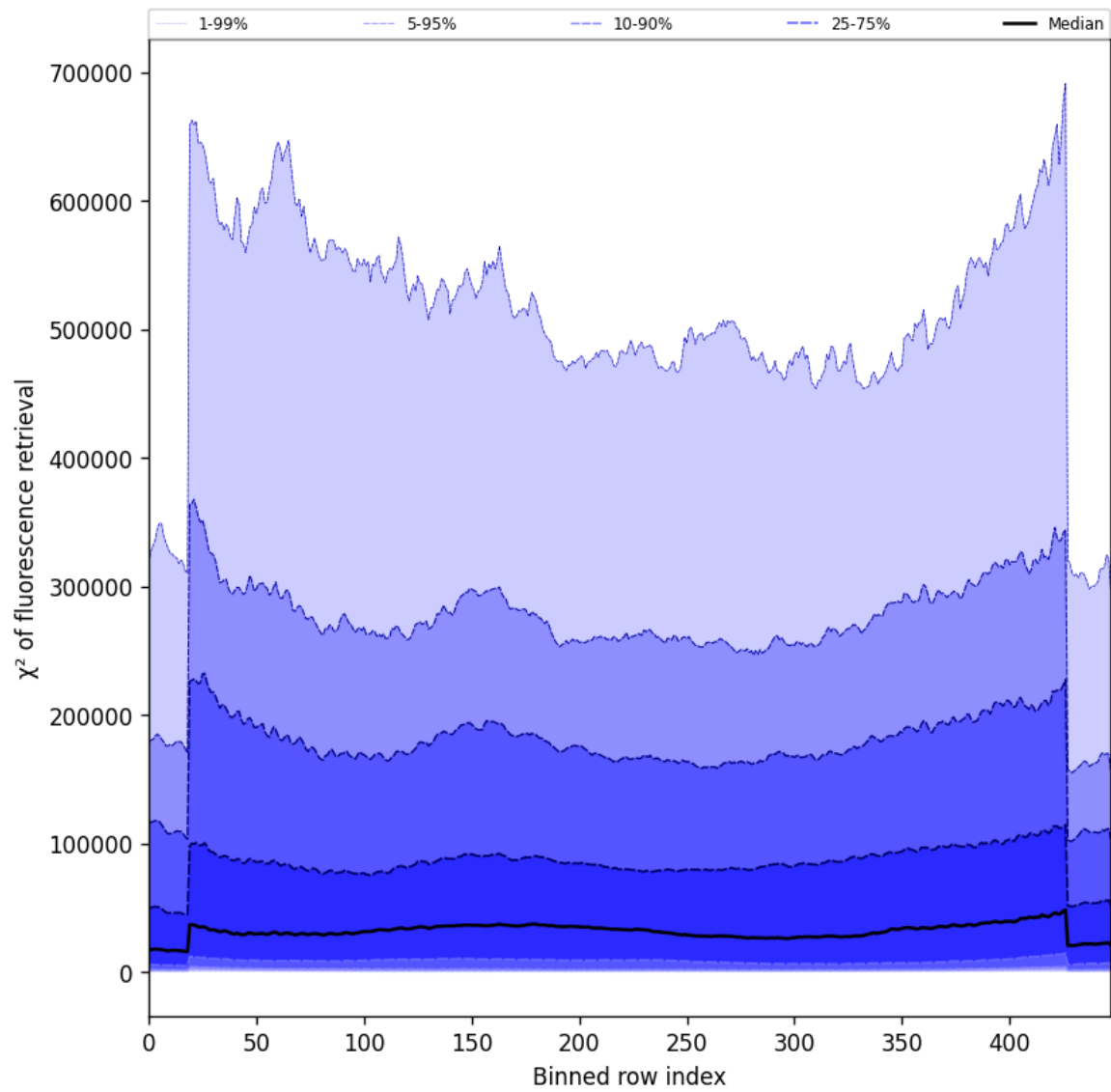
Figure 59: Along track statistics of “ \chi^2 of fluorescence retrieval” for 2025-06-20 to 2025-06-22
