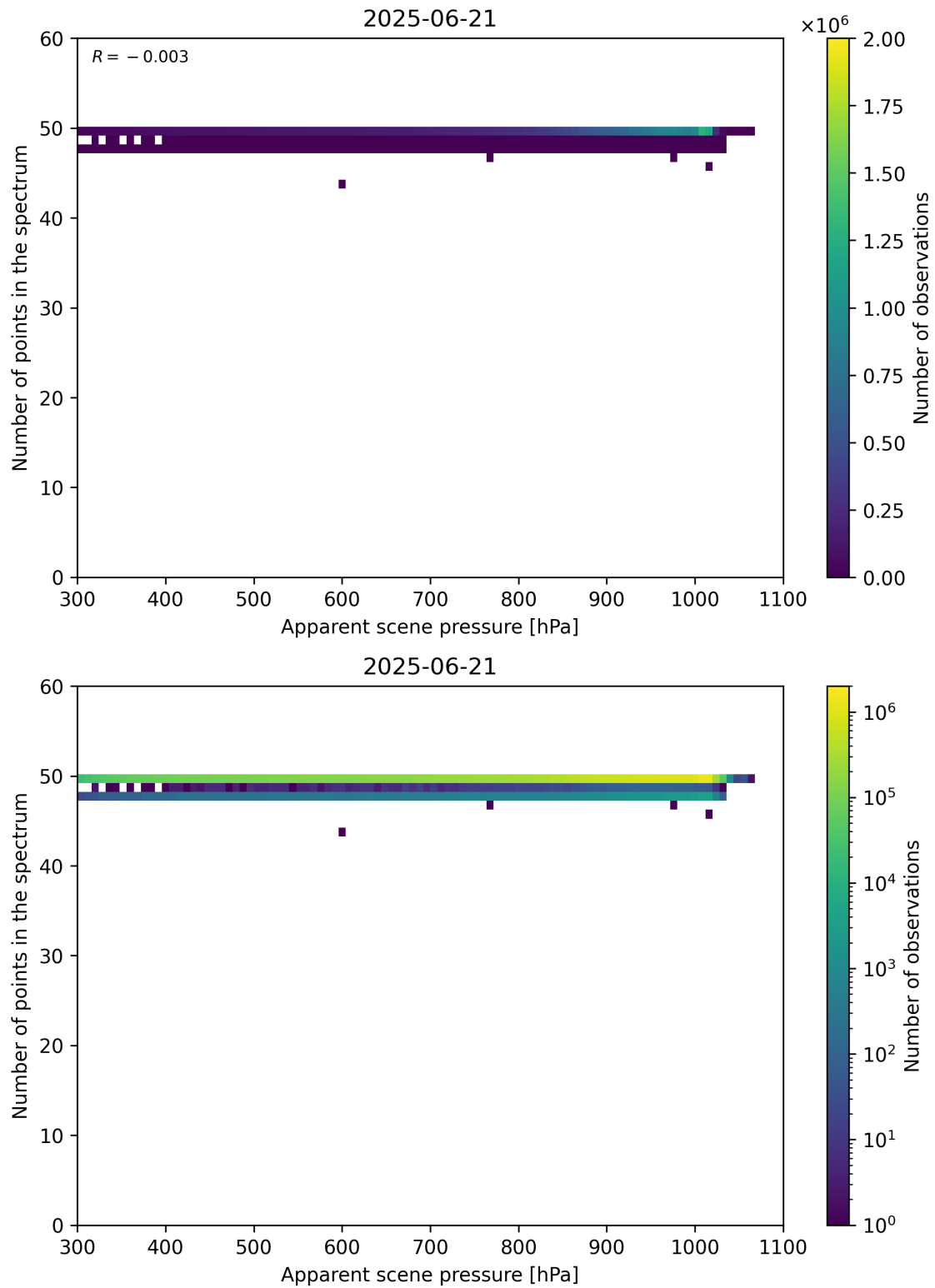
Figure 66: Scatter density plot of “Apparent scene pressure” against “Number of points in the spectrum” for 2025-06-20 to 2025-06-22.
