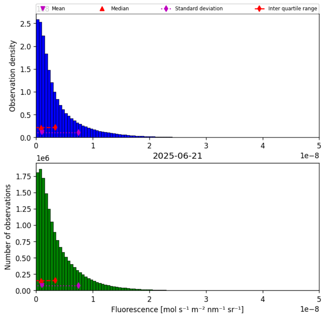
Figure 40: Histogram of “Fluorescence” for 2025-06-20 to 2025-06-22
