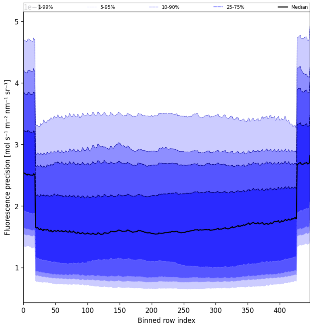
Figure 58: Along track statistics of “Fluorescence precision” for 2025-06-20 to 2025-06-22
