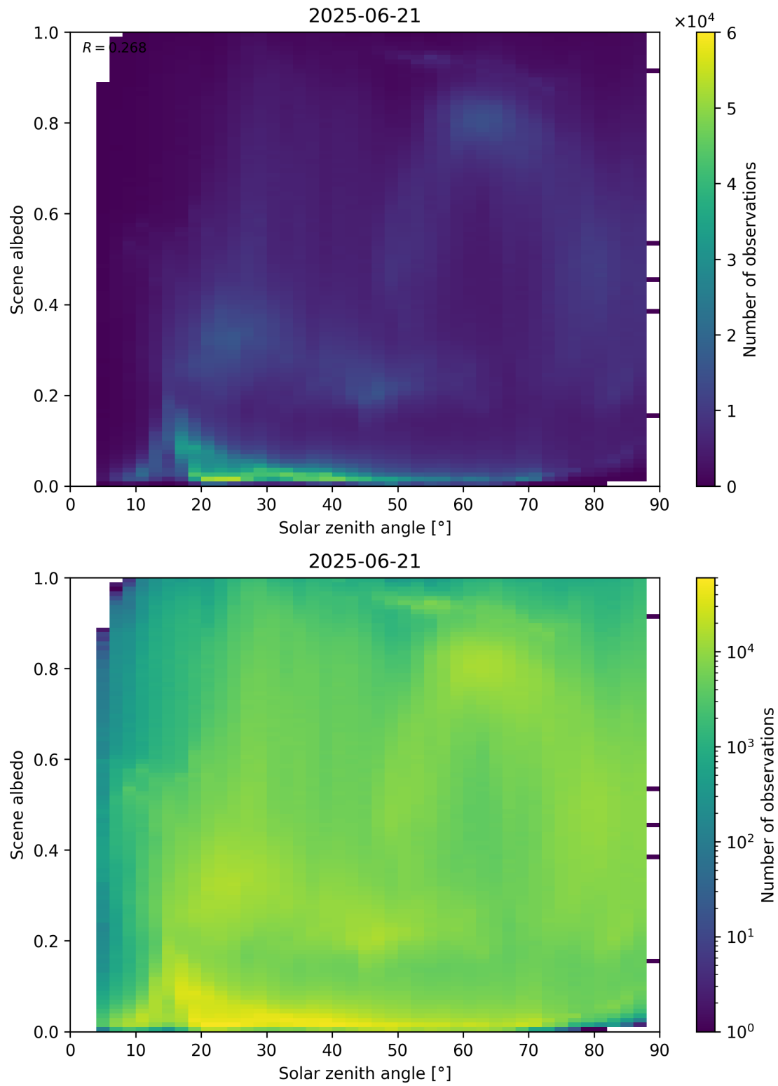
Figure 116: Scatter density plot of “Solar zenith angle” against “Scene albedo” for 2025-06-20 to 2025-06-22.
