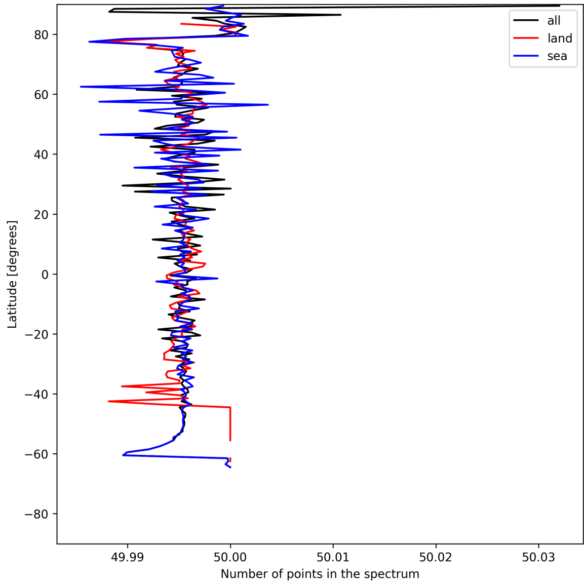
Figure 27: Zonal average of “Number of points in the spectrum” for 2025-06-20 to 2025-06-22.
