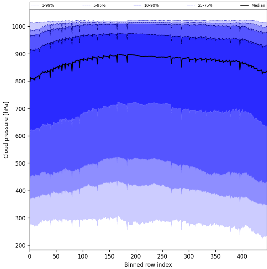
Figure 47: Along track statistics of “Cloud pressure” for 2025-06-20 to 2025-06-22
