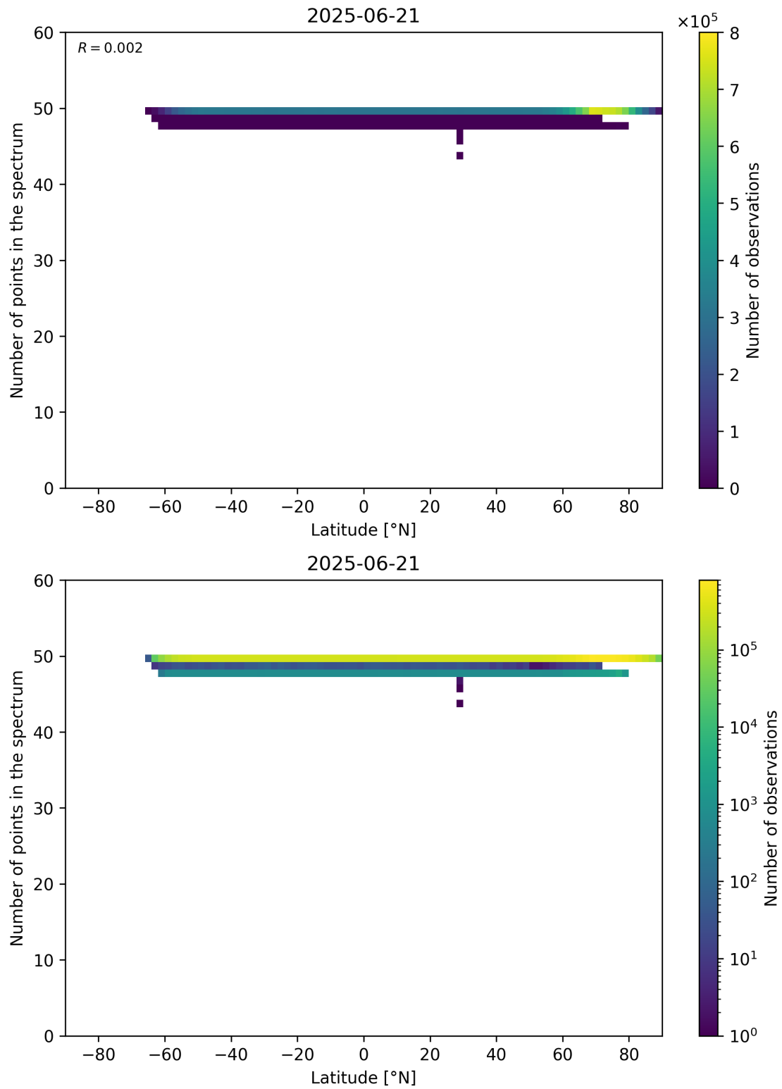
Figure 94: Scatter density plot of “Latitude” against “Number of points in the spectrum” for 2025-06-20 to 2025-06-22.
