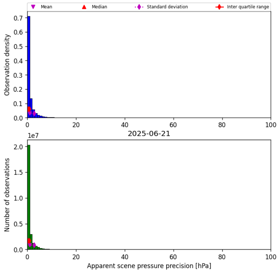
Figure 37: Histogram of “Apparent scene pressure precision” for 2025-06-20 to 2025-06-22
