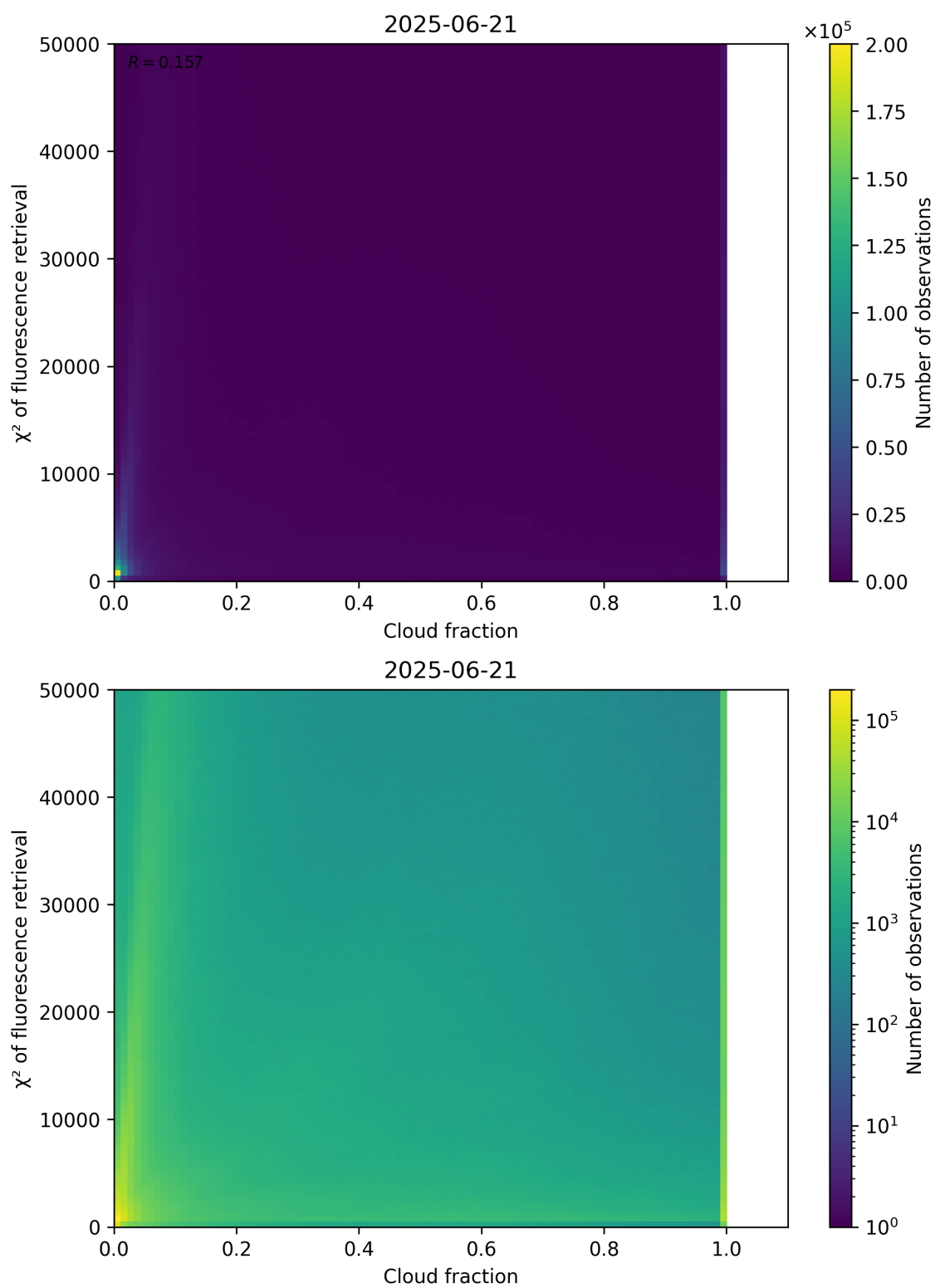
Figure 71: Scatter density plot of “Cloud fraction” against “ \chi^2 of fluorescence retrieval” for 2025-06-20 to 2025-06-22.
