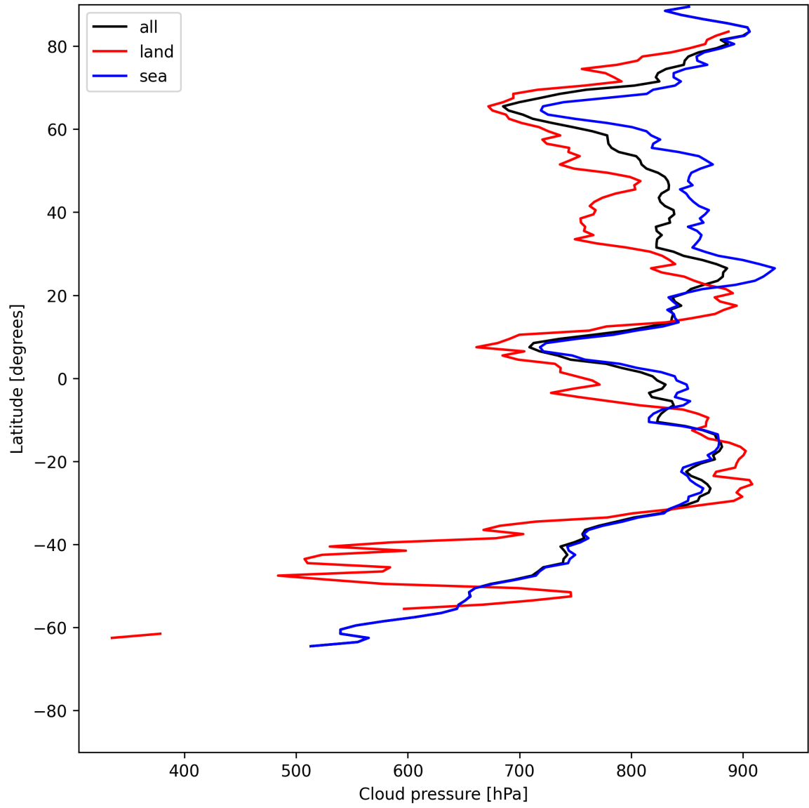
Figure 13: Zonal average of “Cloud pressure” for 2025-06-20 to 2025-06-22.
