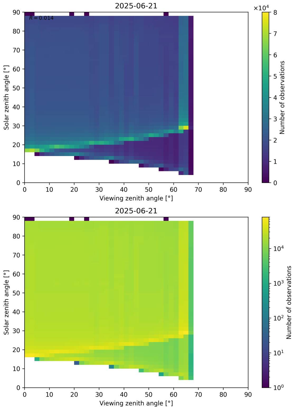
Figure 127: Scatter density plot of “Viewing zenith angle” against “Solar zenith angle” for 2025-06-20 to 2025-06-22.
