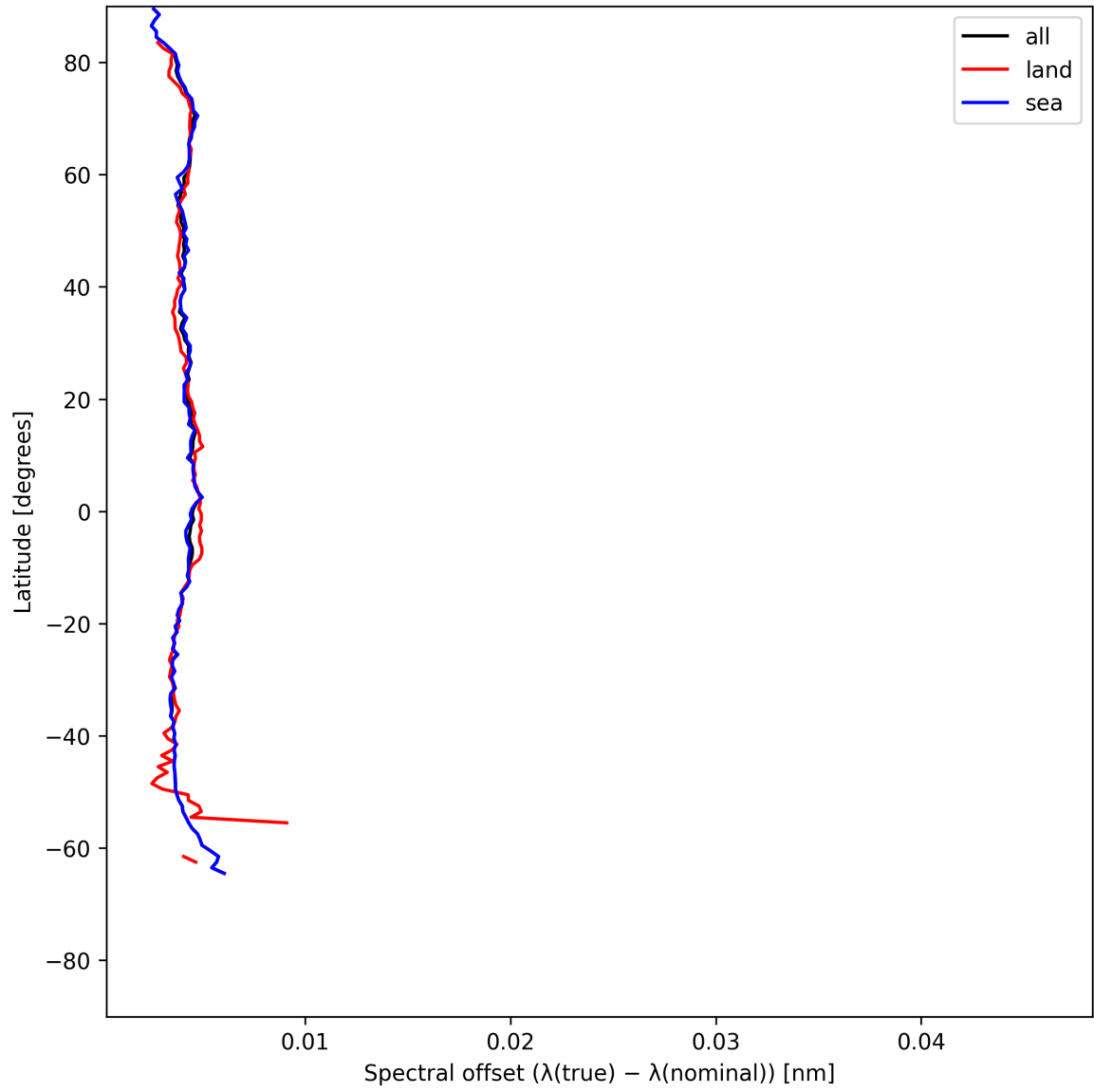
Figure 28: Zonal average of “Spectral offset ( \lambda_{\text{true}} - \lambda_{\text{nominal}} )” for 2025-06-20 to 2025-06-22.
