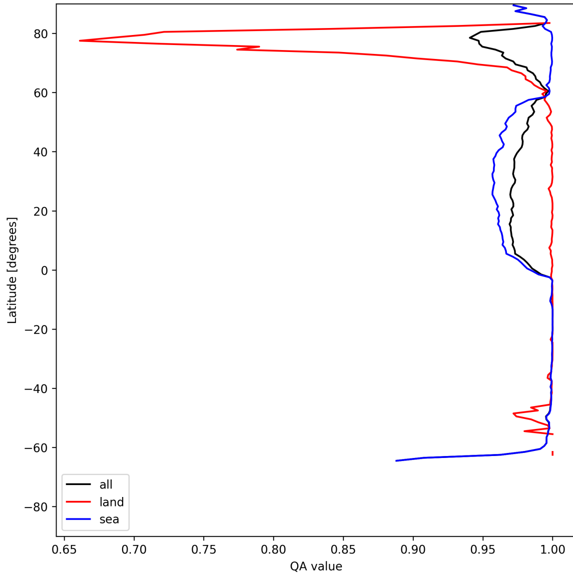
Figure 12: Zonal average of “QA value” for 2025-06-20 to 2025-06-22.
