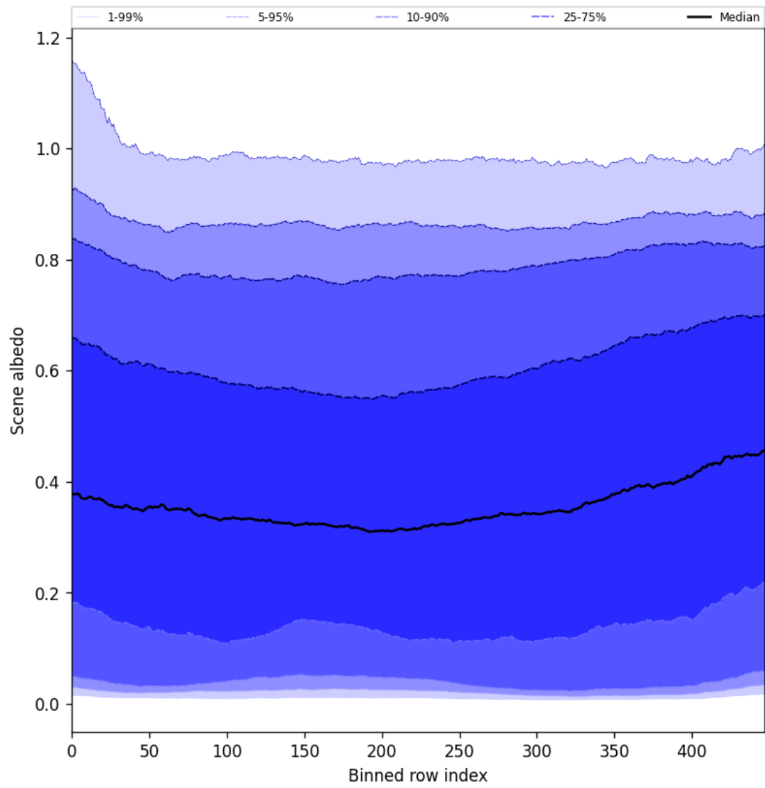
Figure 51: Along track statistics of “Scene albedo” for 2025-06-20 to 2025-06-22
