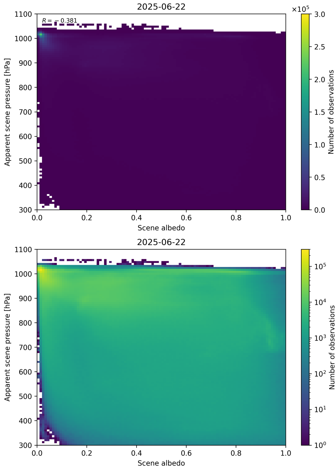
Figure 102: Scatter density plot of “Scene albedo” against “Apparent scene pressure” for 2025-06-22 to 2025-06-23.
