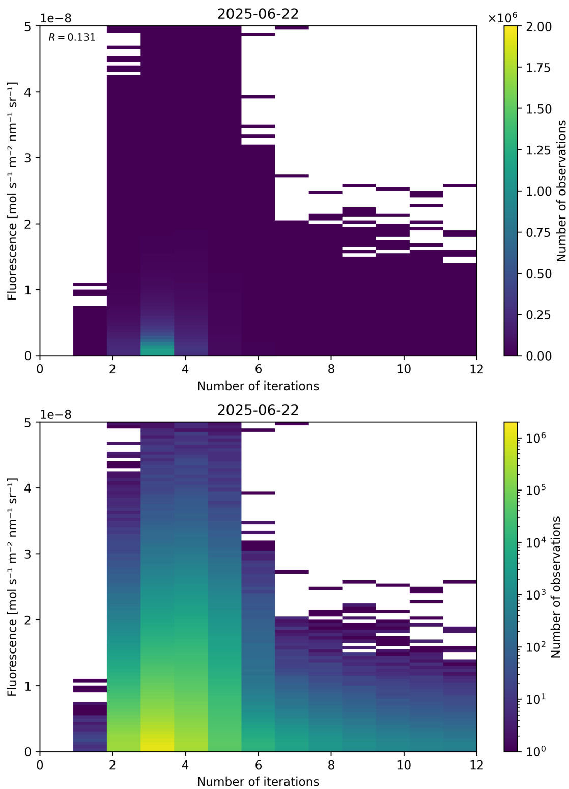
Figure 98: Scatter density plot of “Number of iterations” against “Fluorescence” for 2025-06-22 to 2025-06-23.
