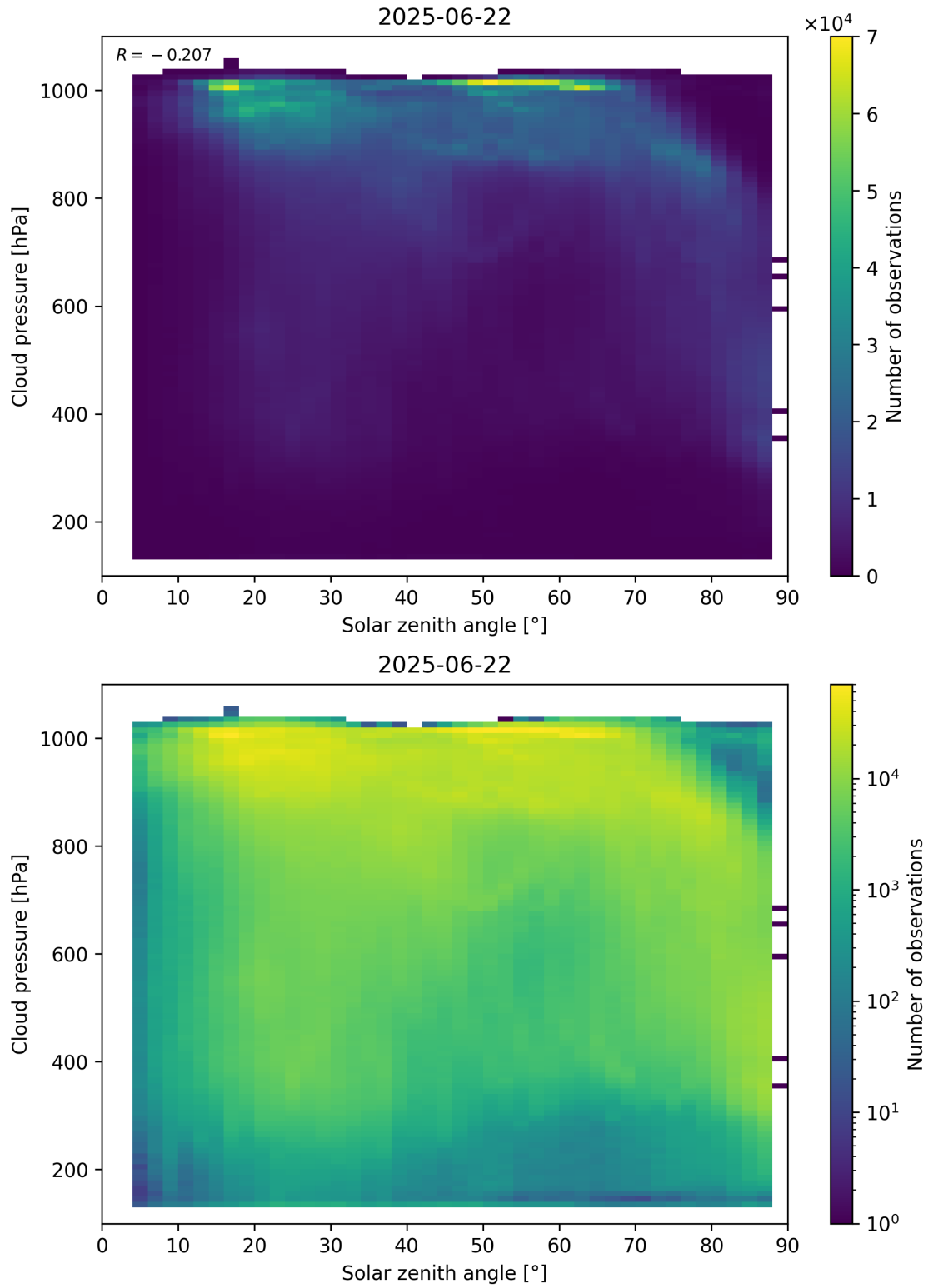
Figure 111: Scatter density plot of “Solar zenith angle” against “Cloud pressure” for 2025-06-22 to 2025-06-23.
