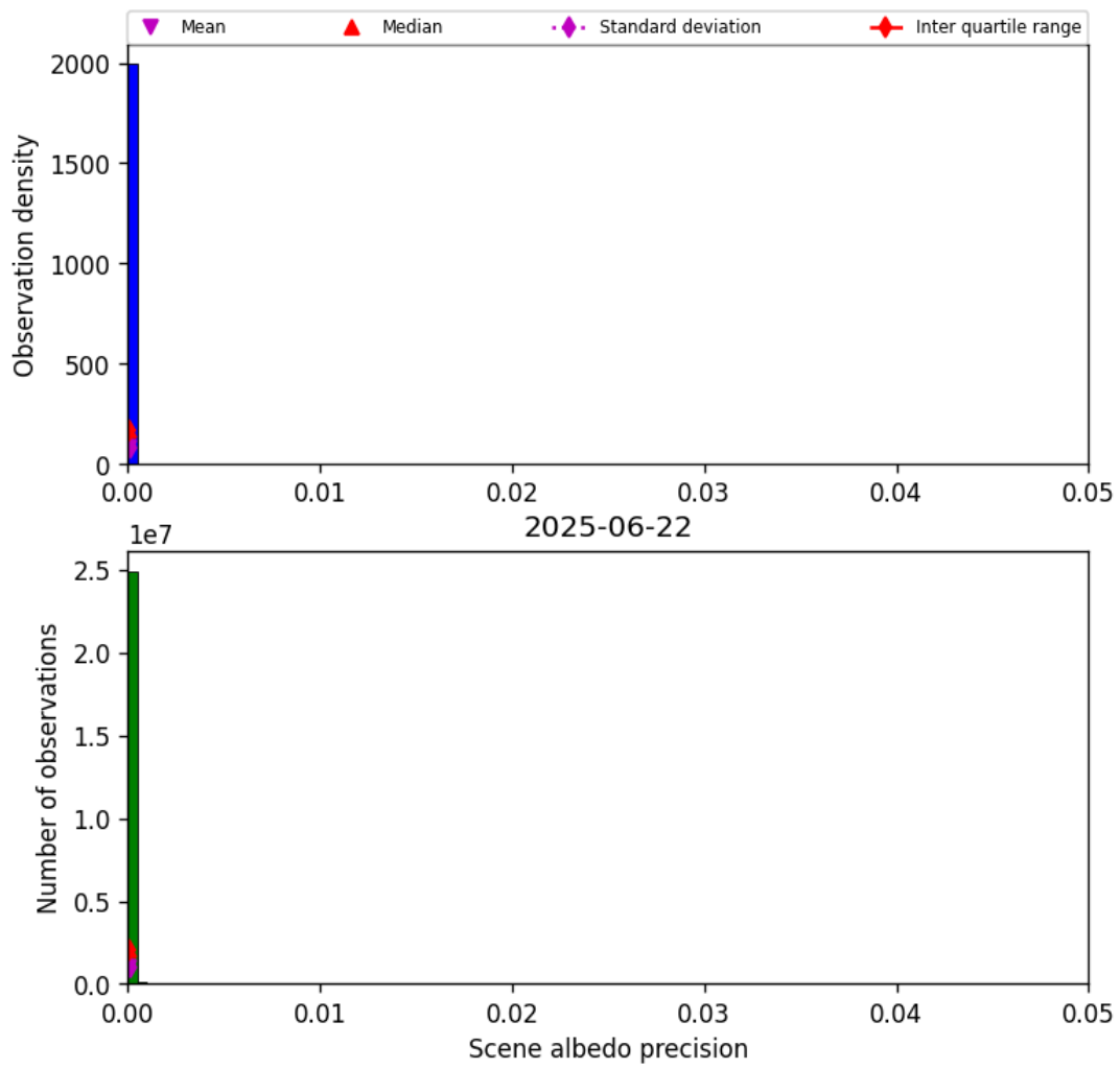
Figure 35: Histogram of “Scene albedo precision” for 2025-06-22 to 2025-06-23
