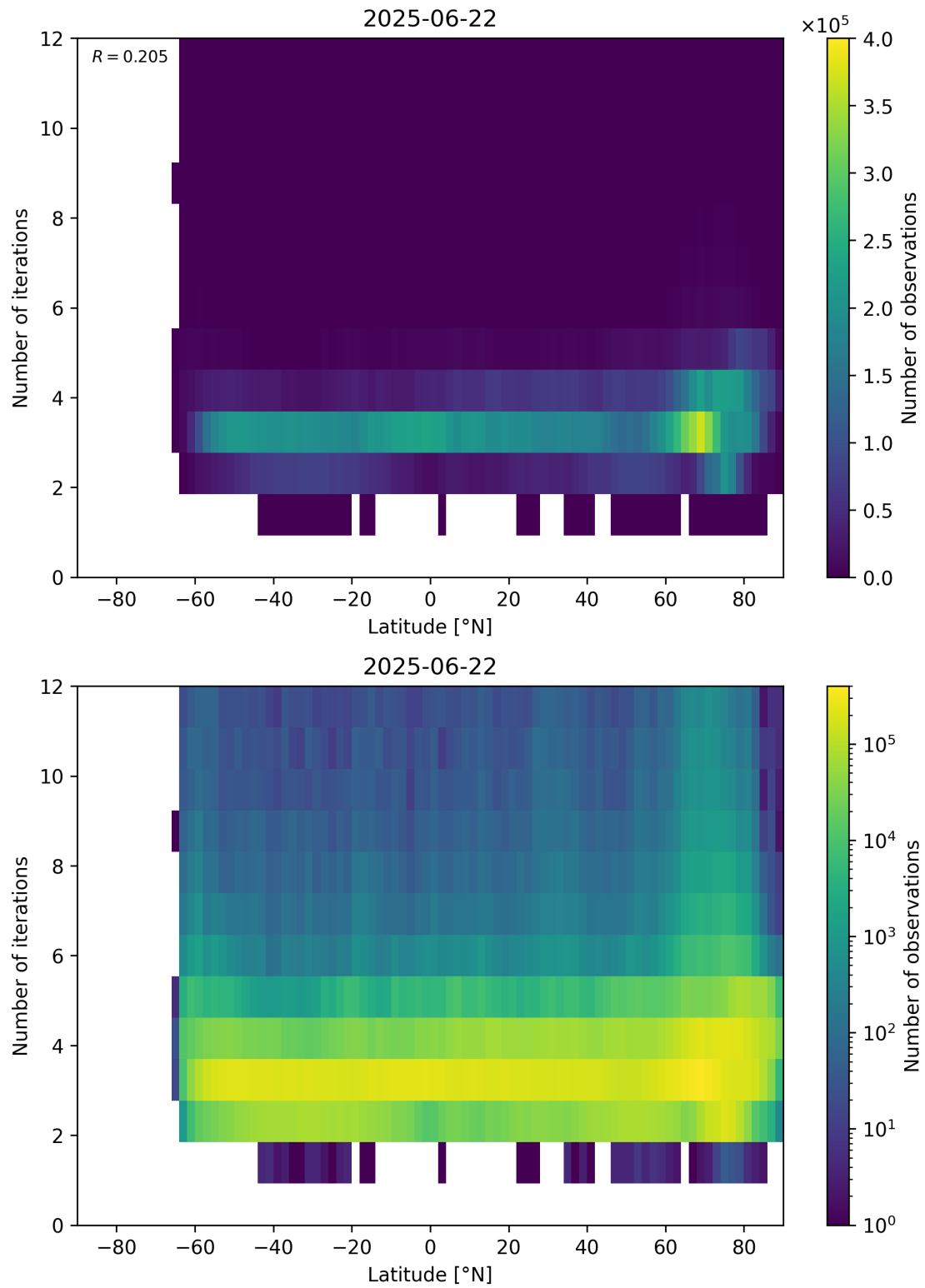
Figure 93: Scatter density plot of “Latitude” against “Number of iterations” for 2025-06-22 to 2025-06-23.
