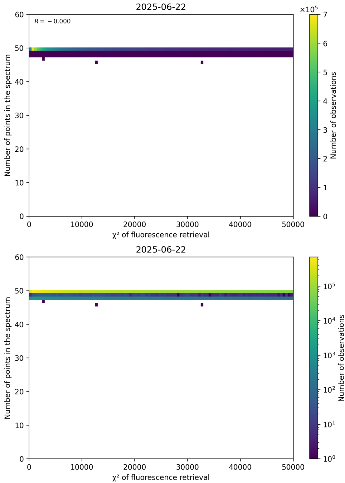
Figure 68: Scatter density plot of “ \chi^2 of fluorescence retrieval” against “Number of points in the spectrum” for 2025-06-22 to 2025-06-23.
