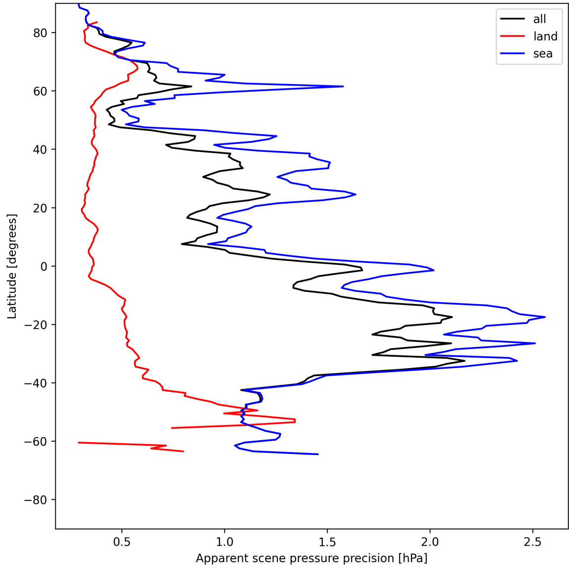
Figure 20: Zonal average of “Apparent scene pressure precision” for 2025-06-22 to 2025-06-23.
