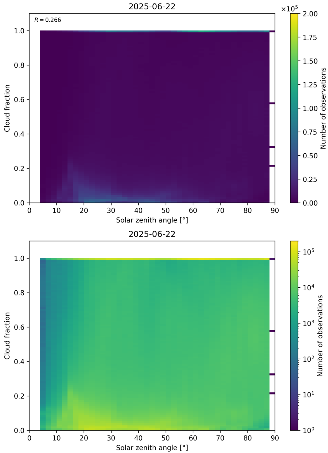
Figure 110: Scatter density plot of “Solar zenith angle” against “Cloud fraction” for 2025-06-22 to 2025-06-23.
