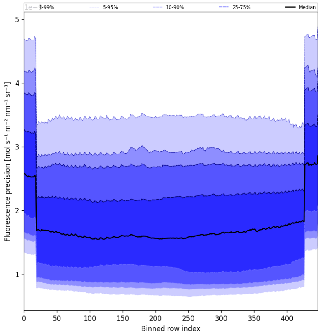
Figure 58: Along track statistics of “Fluorescence precision” for 2025-06-22 to 2025-06-23
