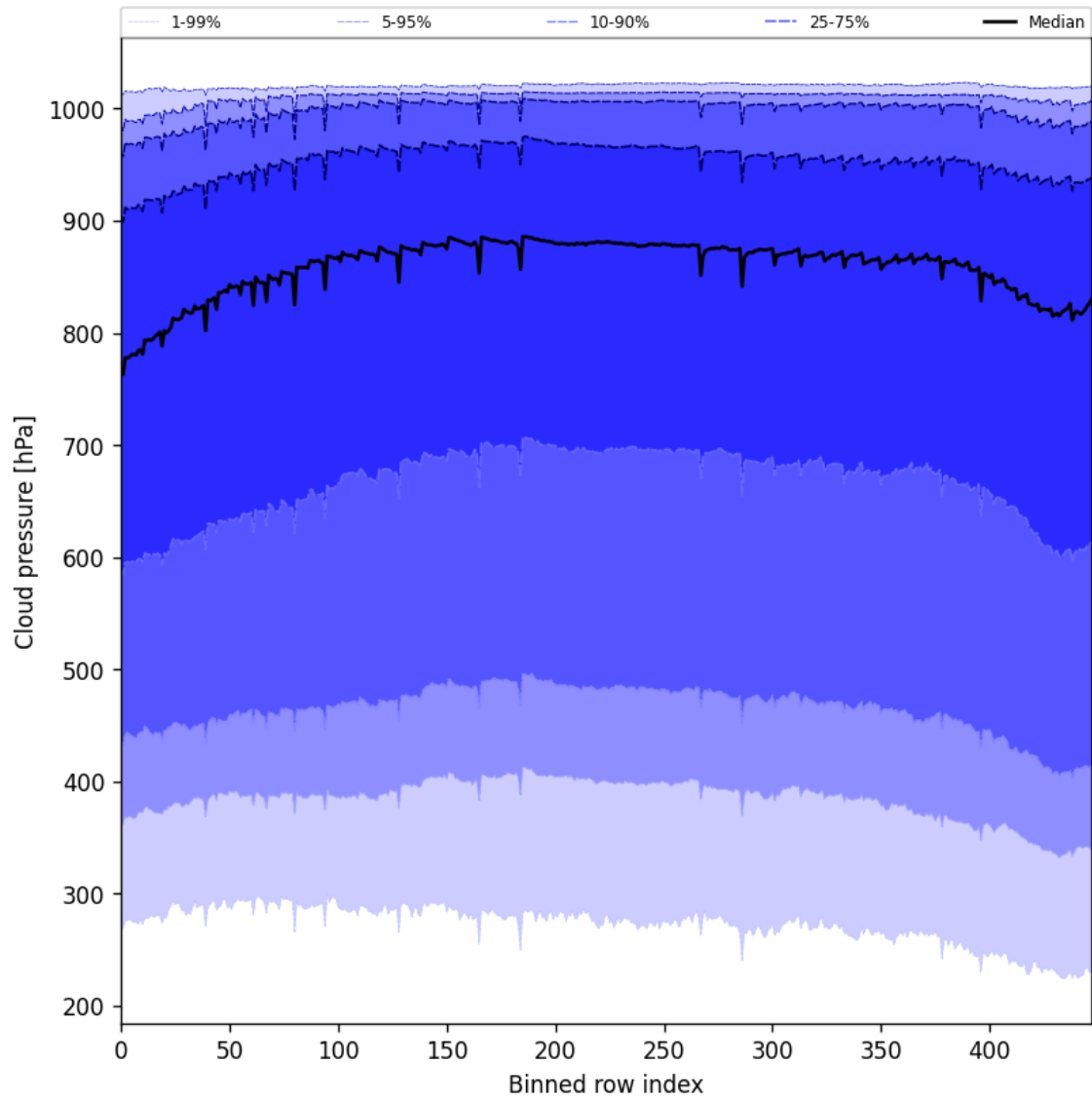
Figure 47: Along track statistics of “Cloud pressure” for 2025-06-22 to 2025-06-23
