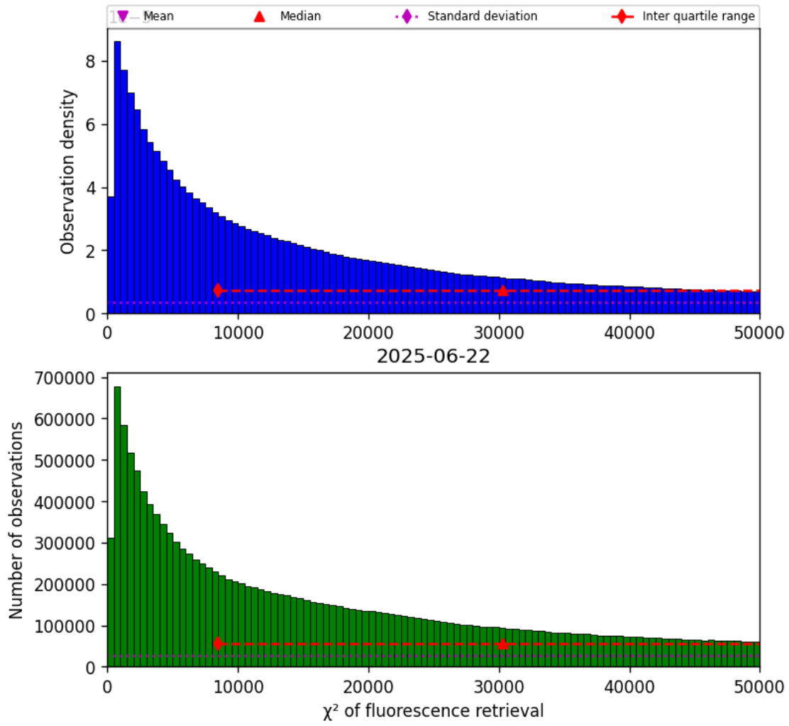
Figure 42: Histogram of “ \chi^2 of fluorescence retrieval” for 2025-06-22 to 2025-06-23
