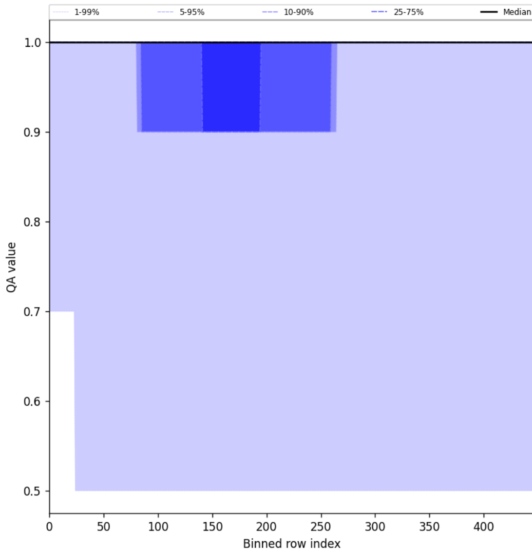
Figure 46: Along track statistics of “QA value” for 2025-06-22 to 2025-06-23
