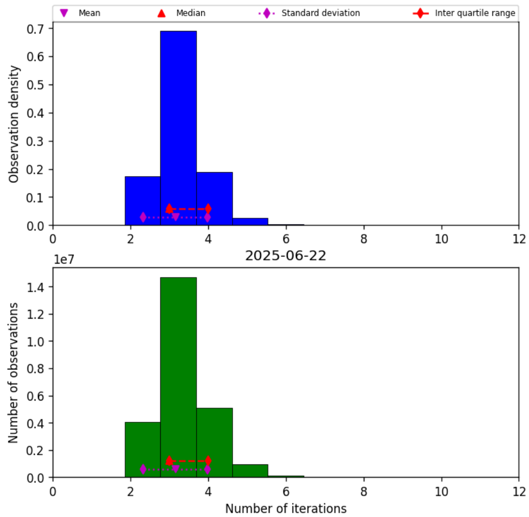
Figure 39: Histogram of “Number of iterations” for 2025-06-22 to 2025-06-23
