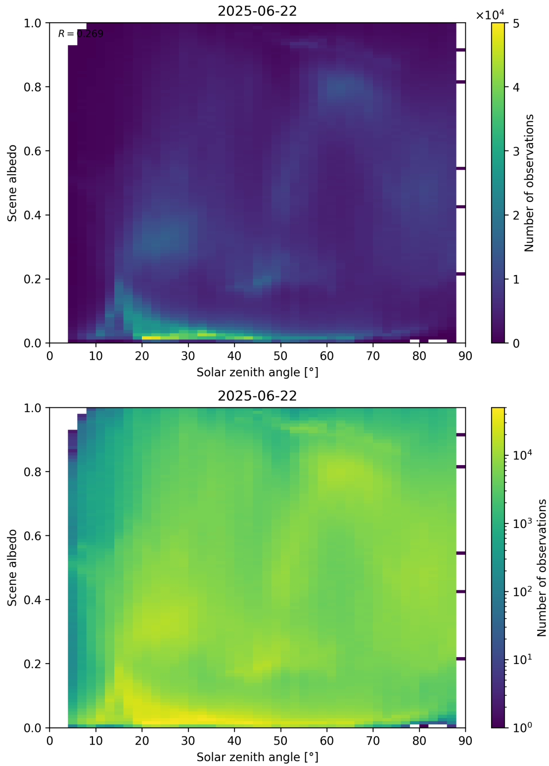
Figure 116: Scatter density plot of “Solar zenith angle” against “Scene albedo” for 2025-06-22 to 2025-06-23.
