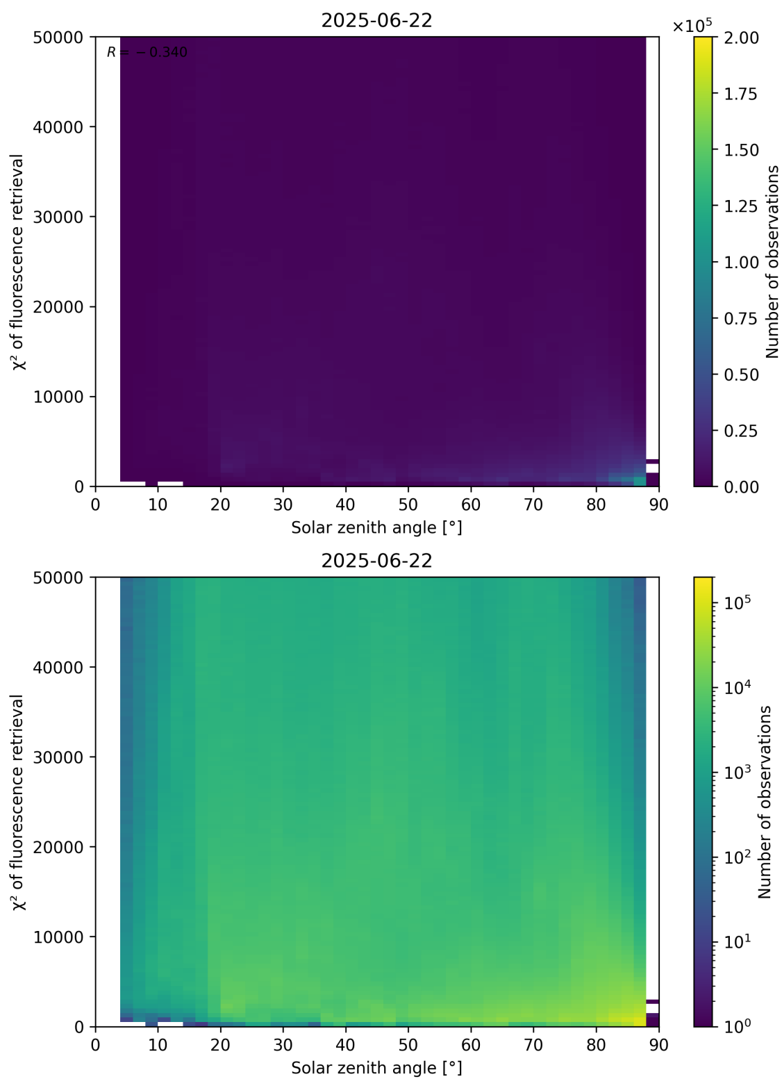
Figure 109: Scatter density plot of “Solar zenith angle” against “ \chi^2 of fluorescence retrieval” for 2025-06-22 to 2025-06-23.
