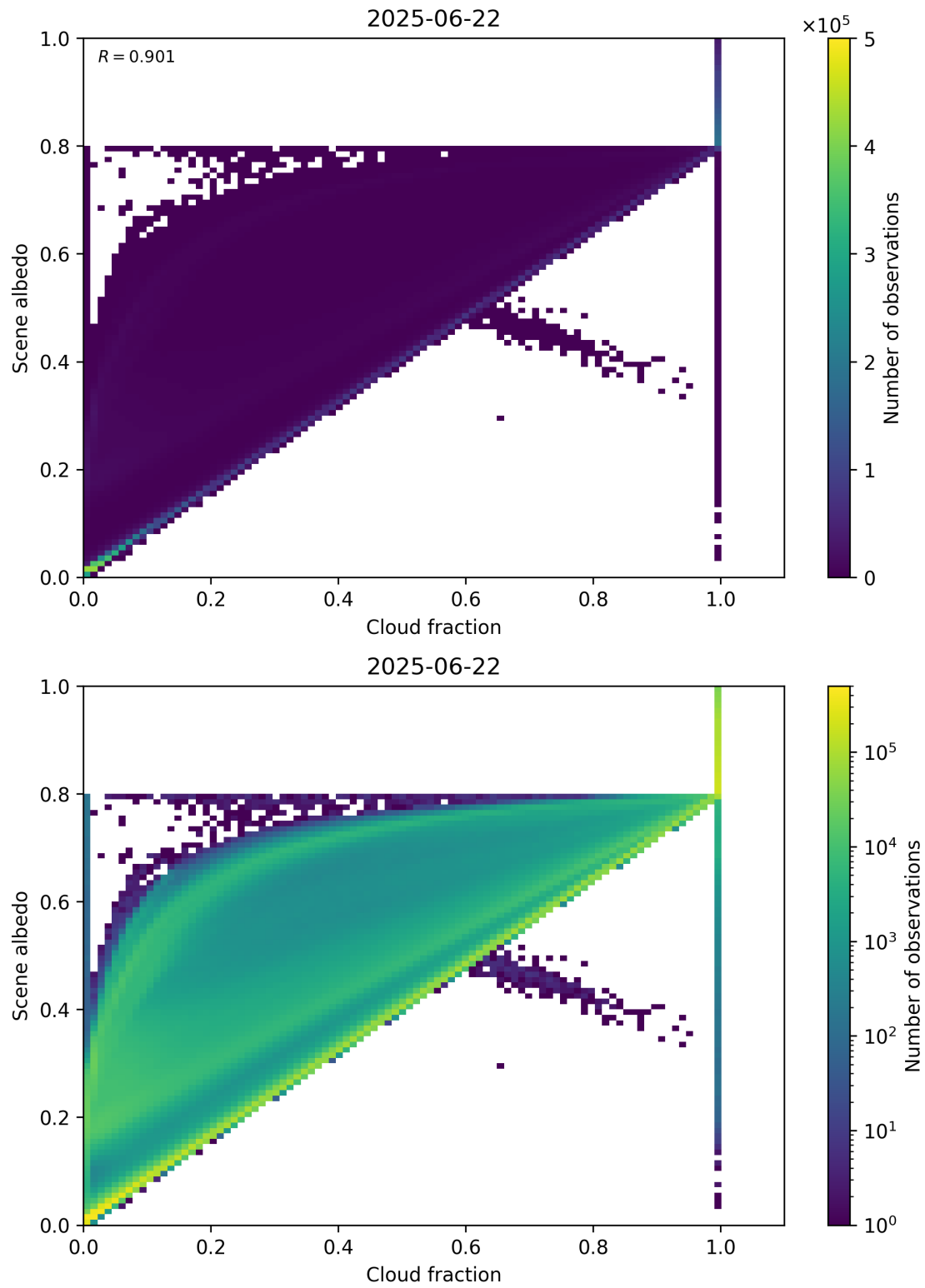
Figure 75: Scatter density plot of “Cloud fraction” against “Scene albedo” for 2025-06-22 to 2025-06-23.
