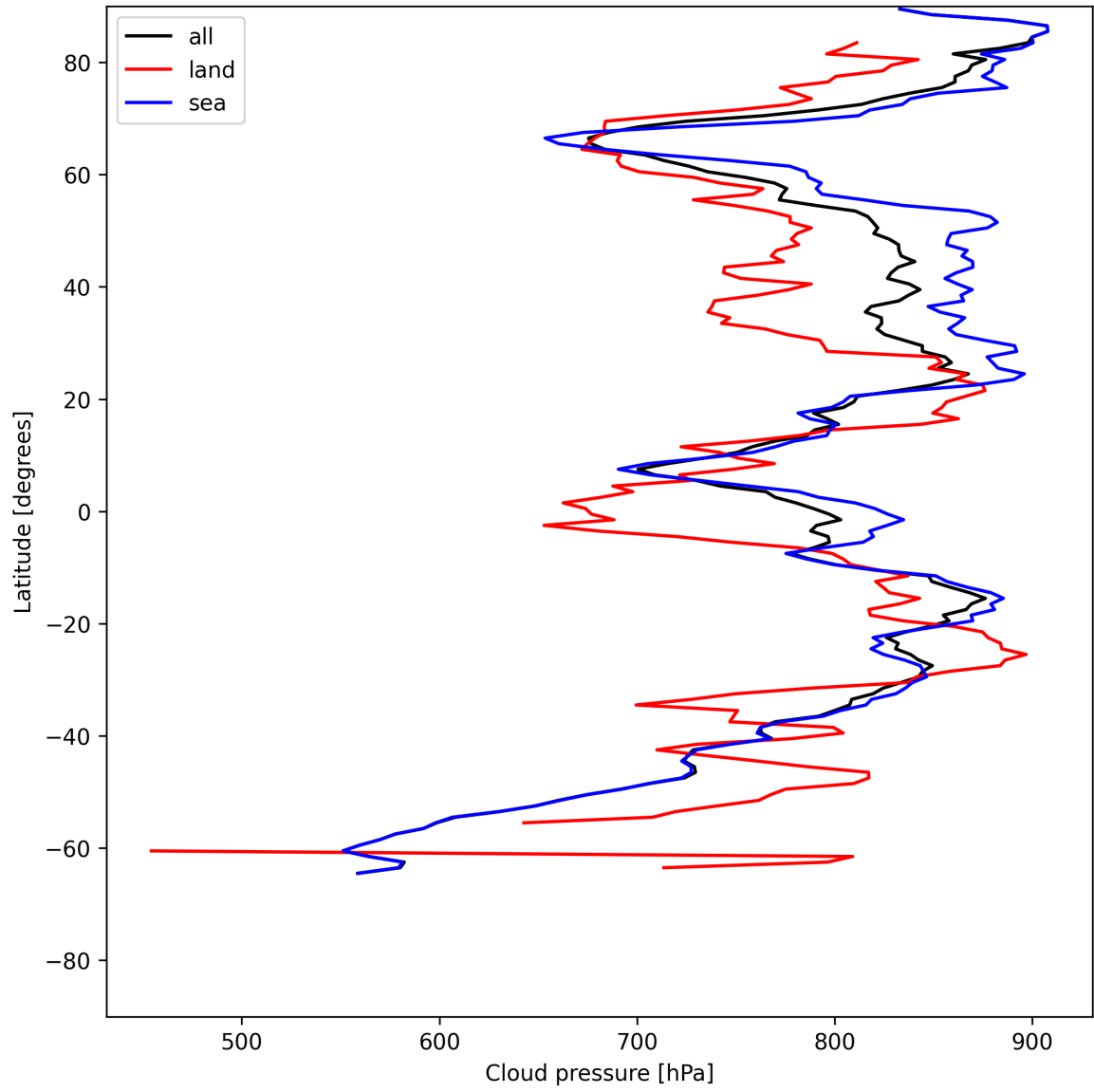
Figure 13: Zonal average of “Cloud pressure” for 2025-06-22 to 2025-06-23.
