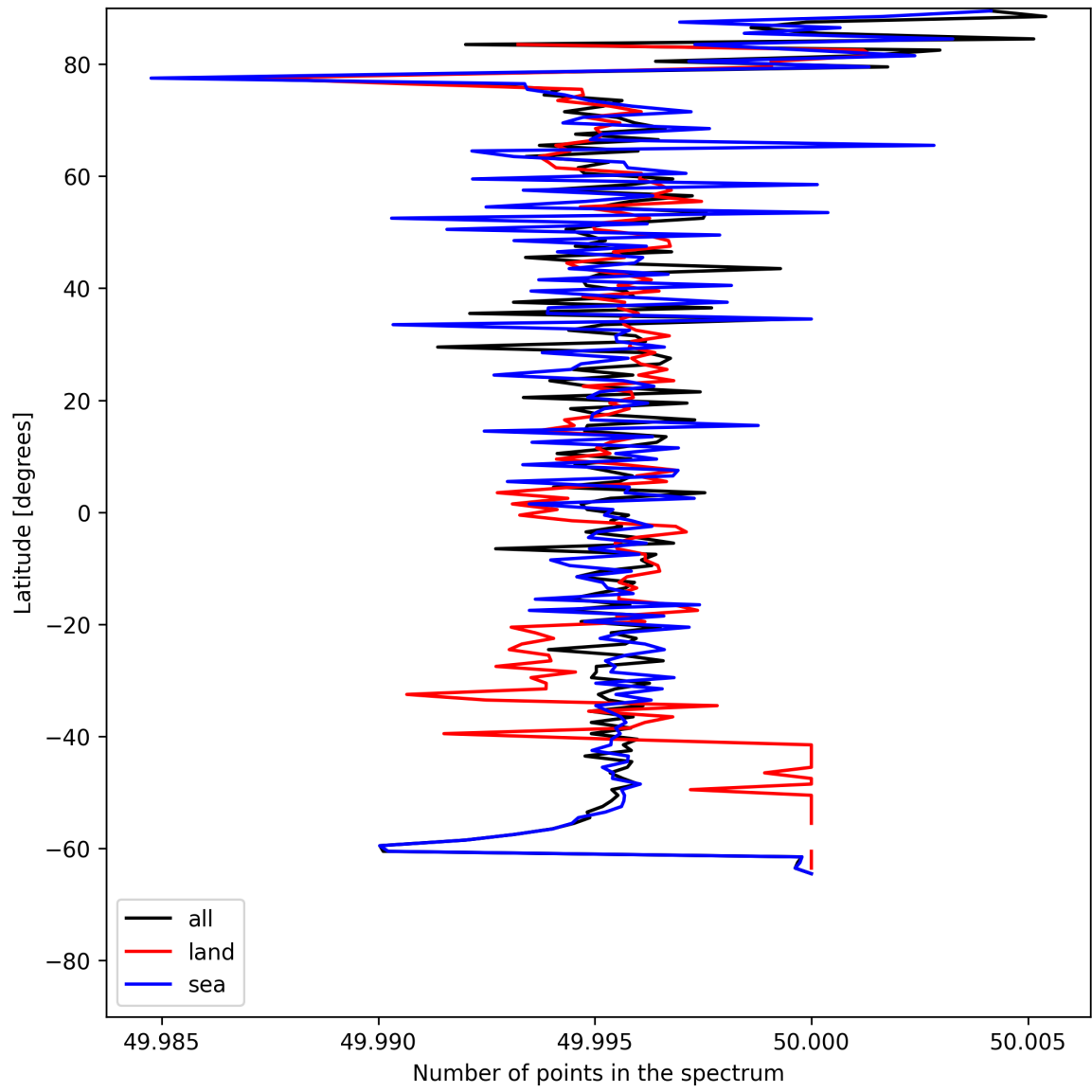
Figure 27: Zonal average of “Number of points in the spectrum” for 2025-06-22 to 2025-06-23.
