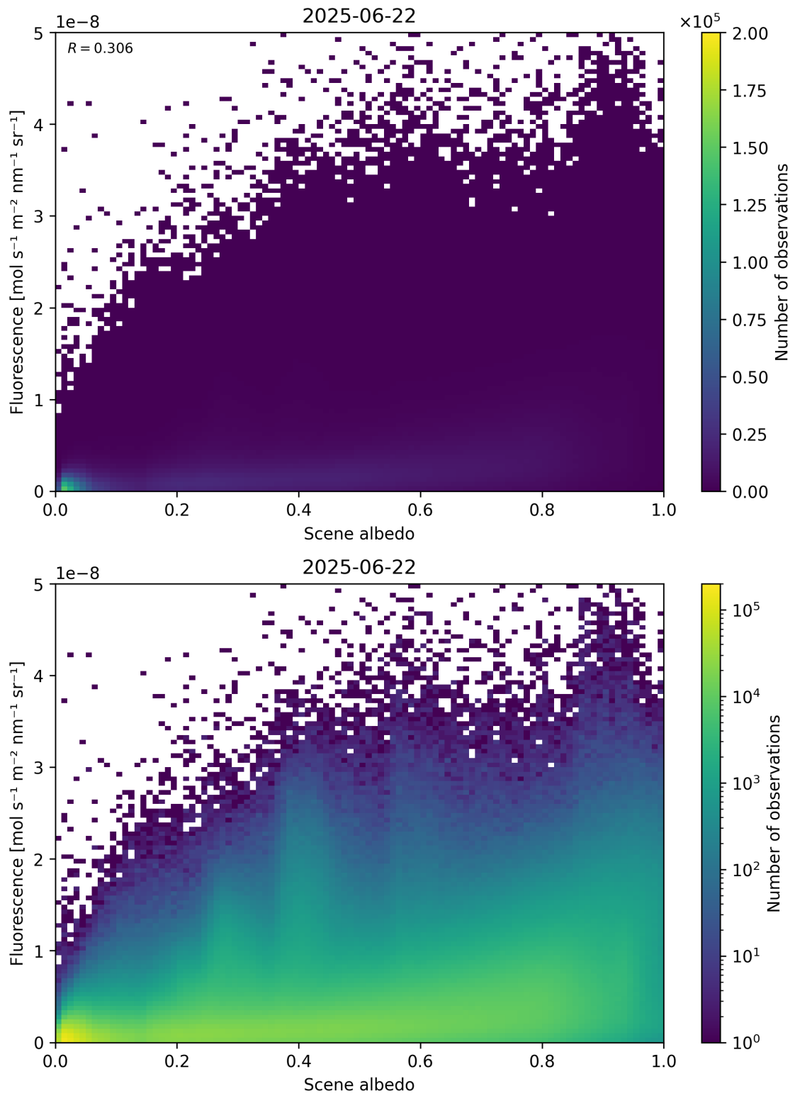
Figure 104: Scatter density plot of “Scene albedo” against “Fluorescence” for 2025-06-22 to 2025-06-23.
