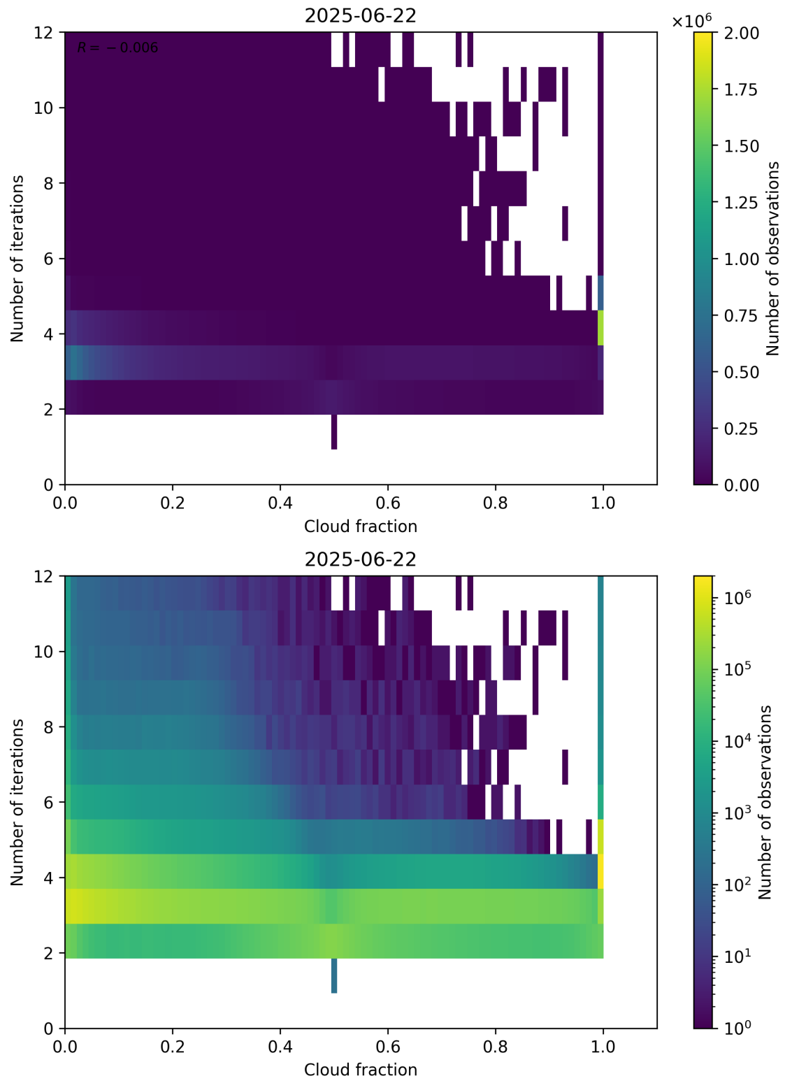
Figure 73: Scatter density plot of “Cloud fraction” against “Number of iterations” for 2025-06-22 to 2025-06-23.
