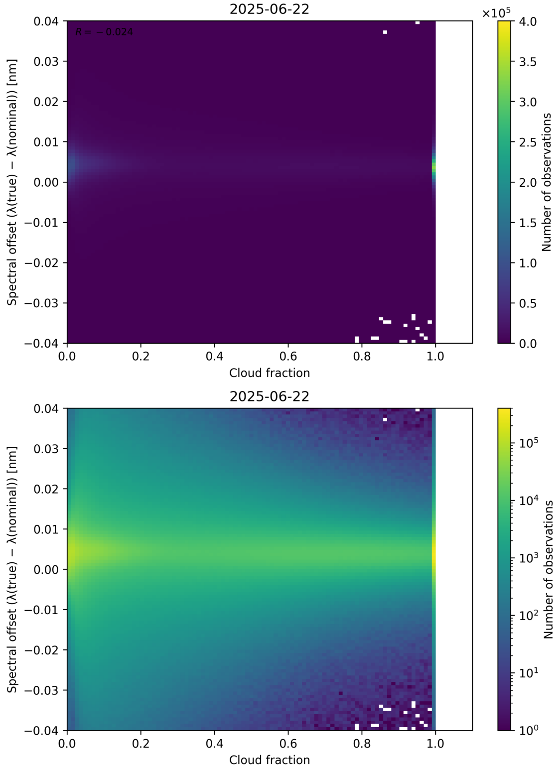
Figure 76: Scatter density plot of “Cloud fraction” against “Spectral offset ( \lambda_{\text{true}} - \lambda_{\text{nominal}} )” for 2025-06-22 to 2025-06-23.
