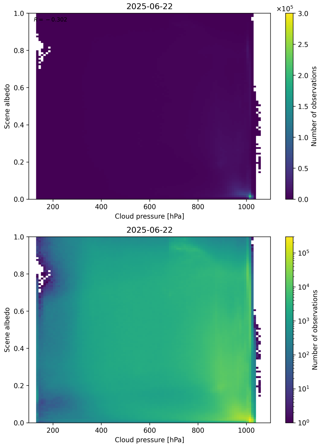
Figure 83: Scatter density plot of “Cloud pressure” against “Scene albedo” for 2025-06-22 to 2025-06-23.
