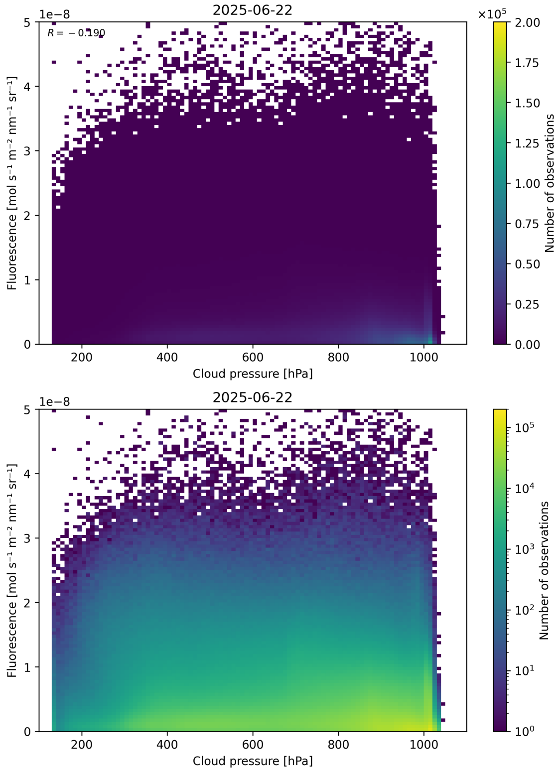
Figure 80: Scatter density plot of “Cloud pressure” against “Fluorescence” for 2025-06-22 to 2025-06-23.
