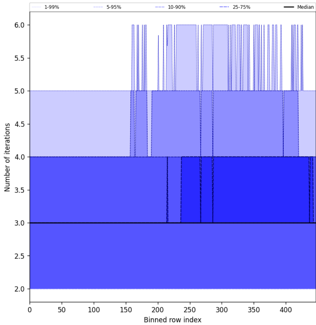
Figure 56: Along track statistics of “Number of iterations” for 2025-06-22 to 2025-06-23
