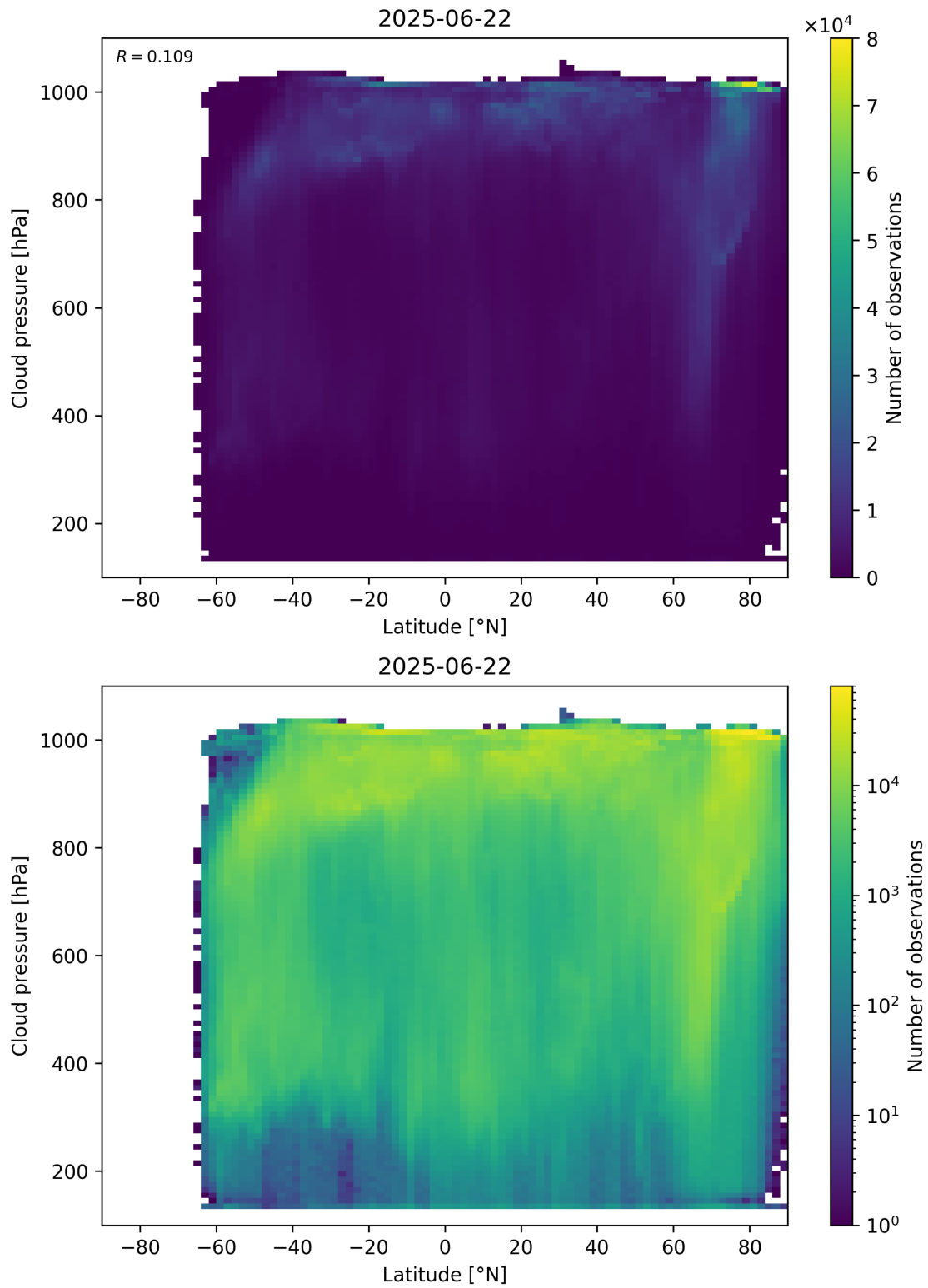
Figure 91: Scatter density plot of “Latitude” against “Cloud pressure” for 2025-06-22 to 2025-06-23.
