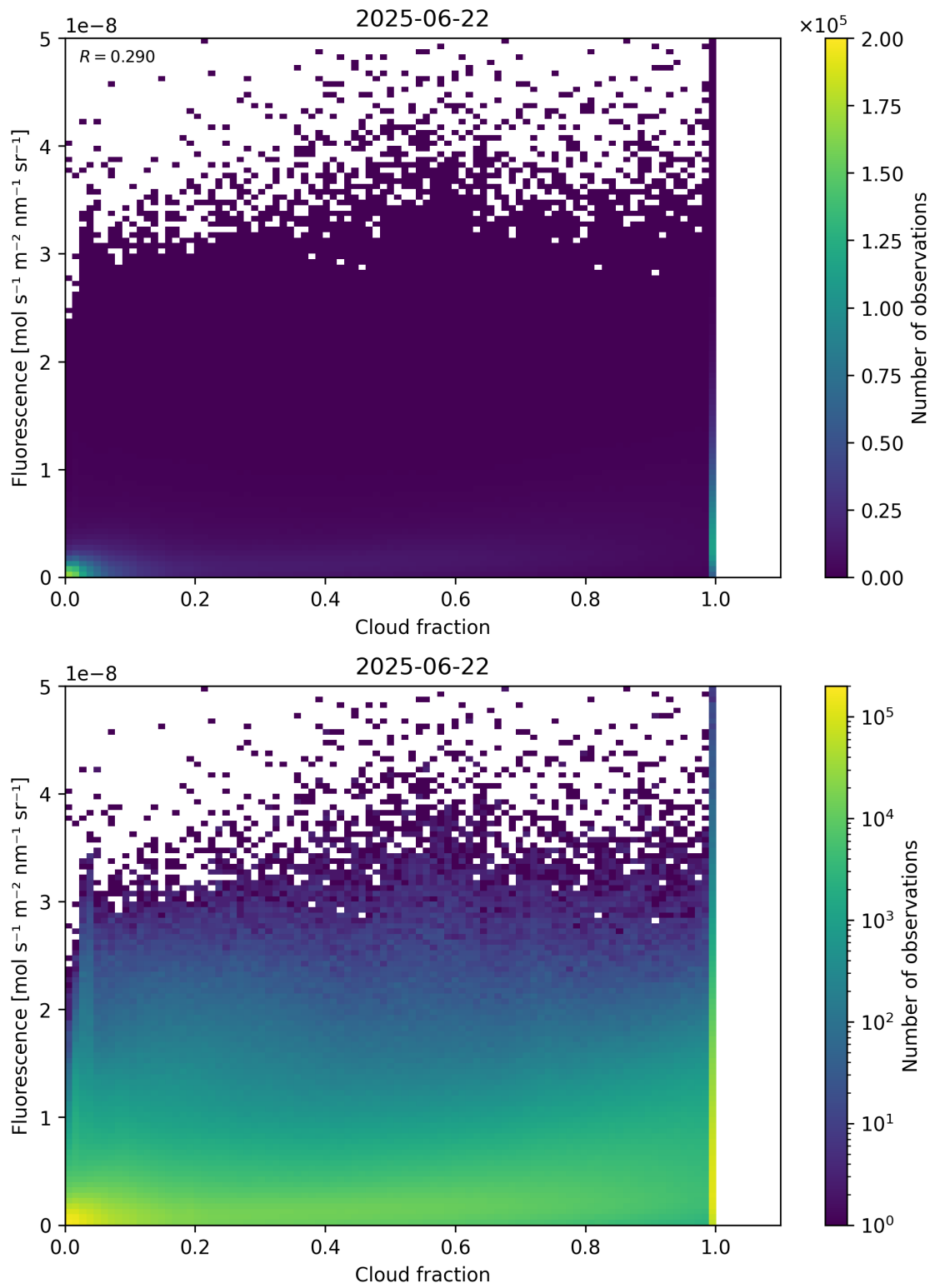
Figure 72: Scatter density plot of “Cloud fraction” against “Fluorescence” for 2025-06-22 to 2025-06-23.
