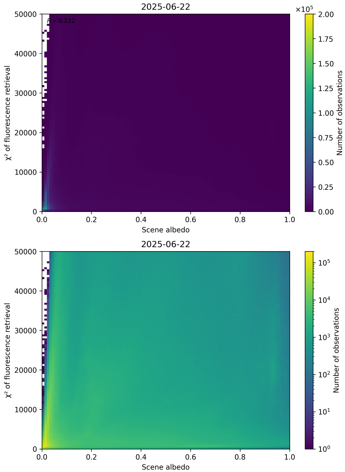
Figure 103: Scatter density plot of “Scene albedo” against “ \chi^2 of fluorescence retrieval” for 2025-06-22 to 2025-06-23.
