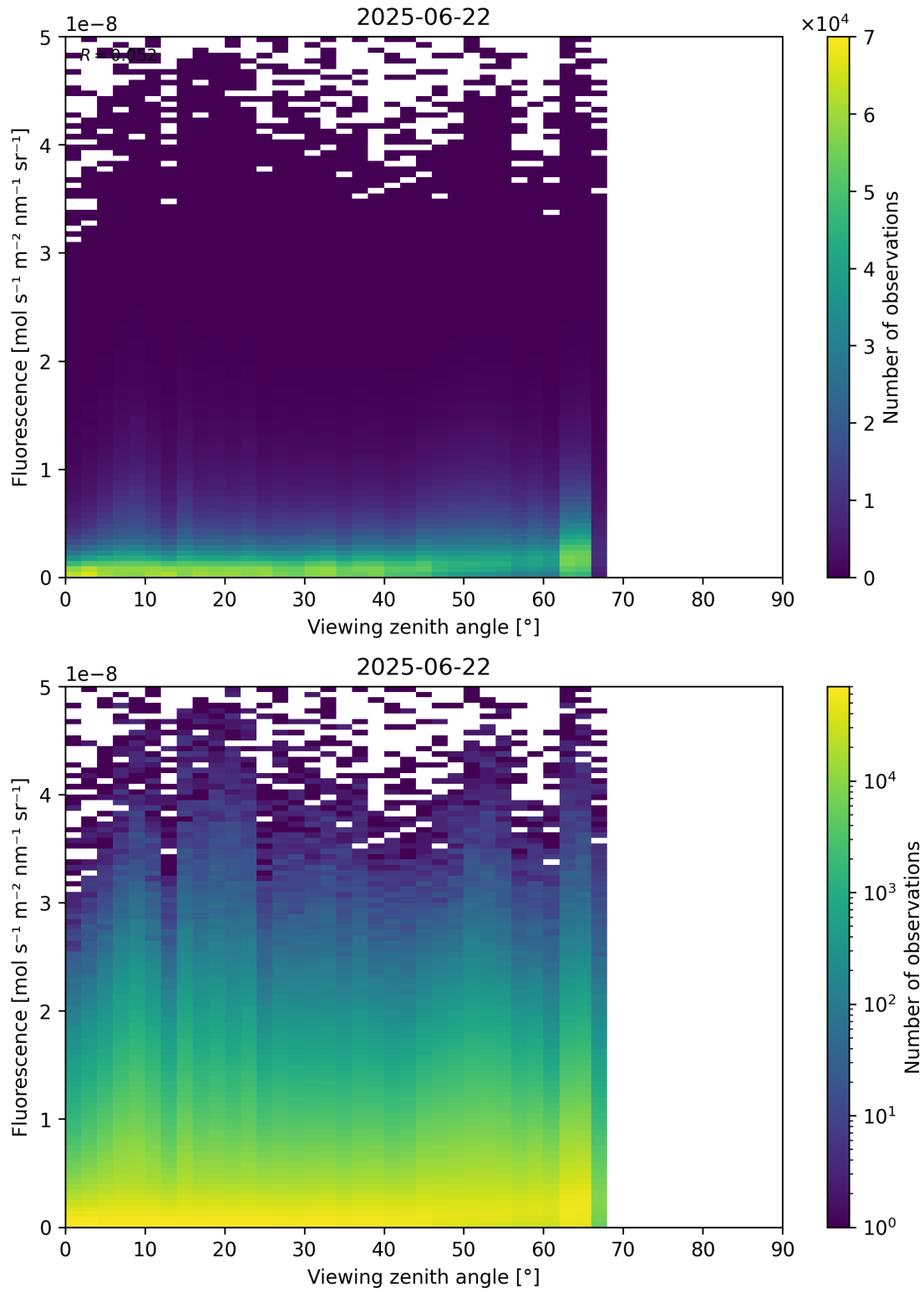
Figure 122: Scatter density plot of “Viewing zenith angle” against “Fluorescence” for 2025-06-22 to 2025-06-23.
