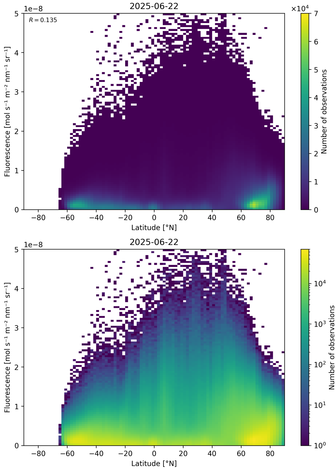
Figure 92: Scatter density plot of “Latitude” against “Fluorescence” for 2025-06-22 to 2025-06-23.
