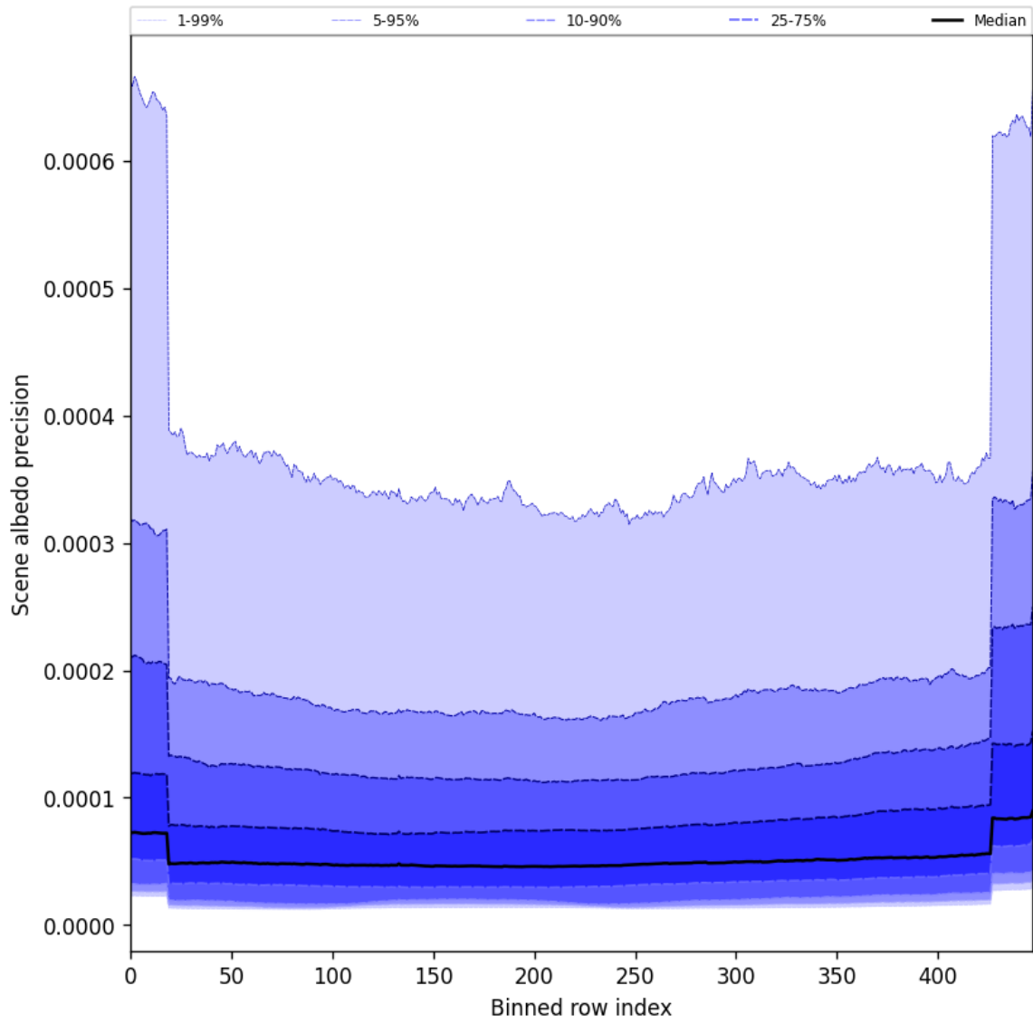
Figure 52: Along track statistics of “Scene albedo precision” for 2025-06-22 to 2025-06-23
