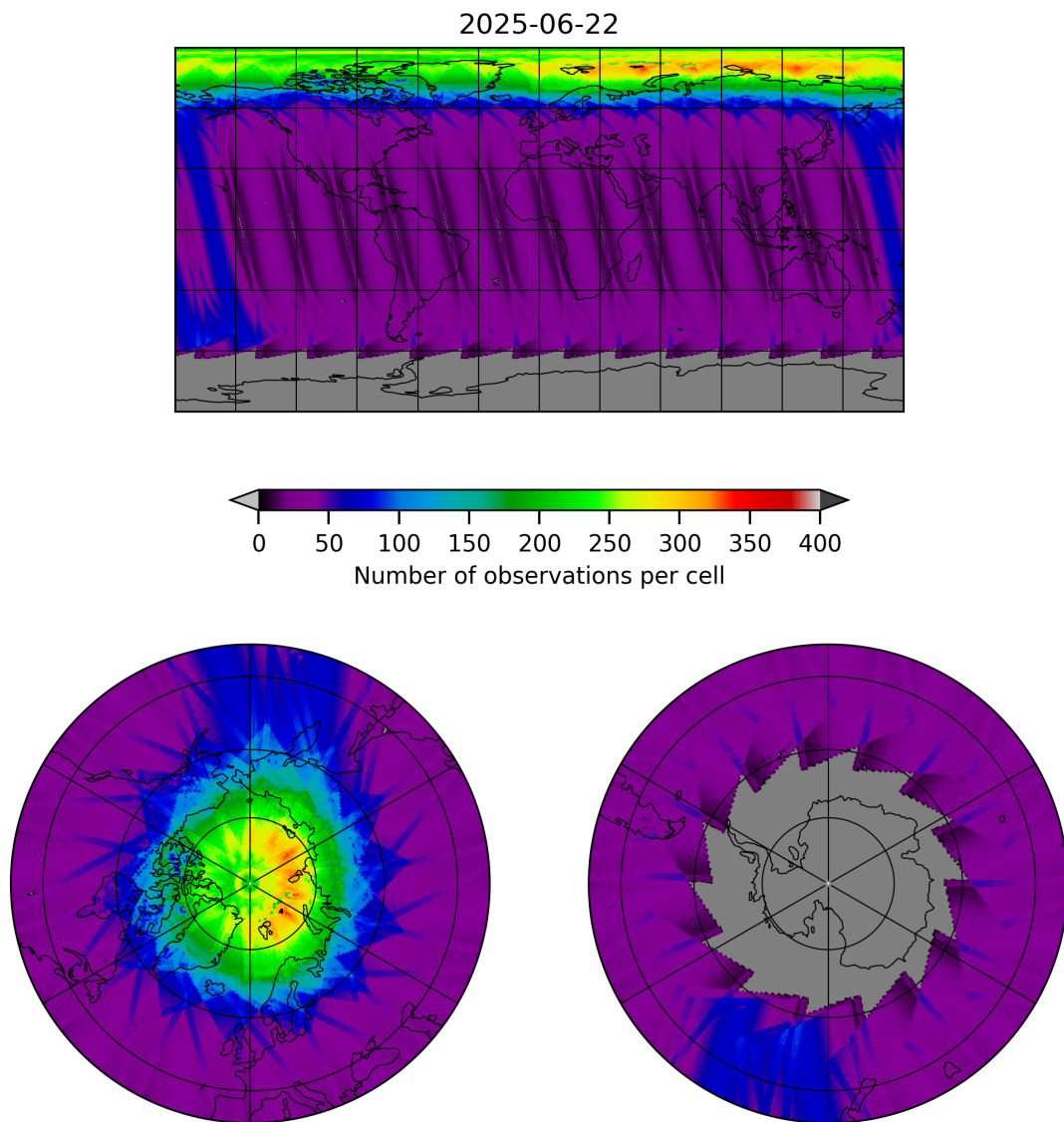
Figure 11: Map of the number of observations for 2025-06-22 to 2025-06-23
