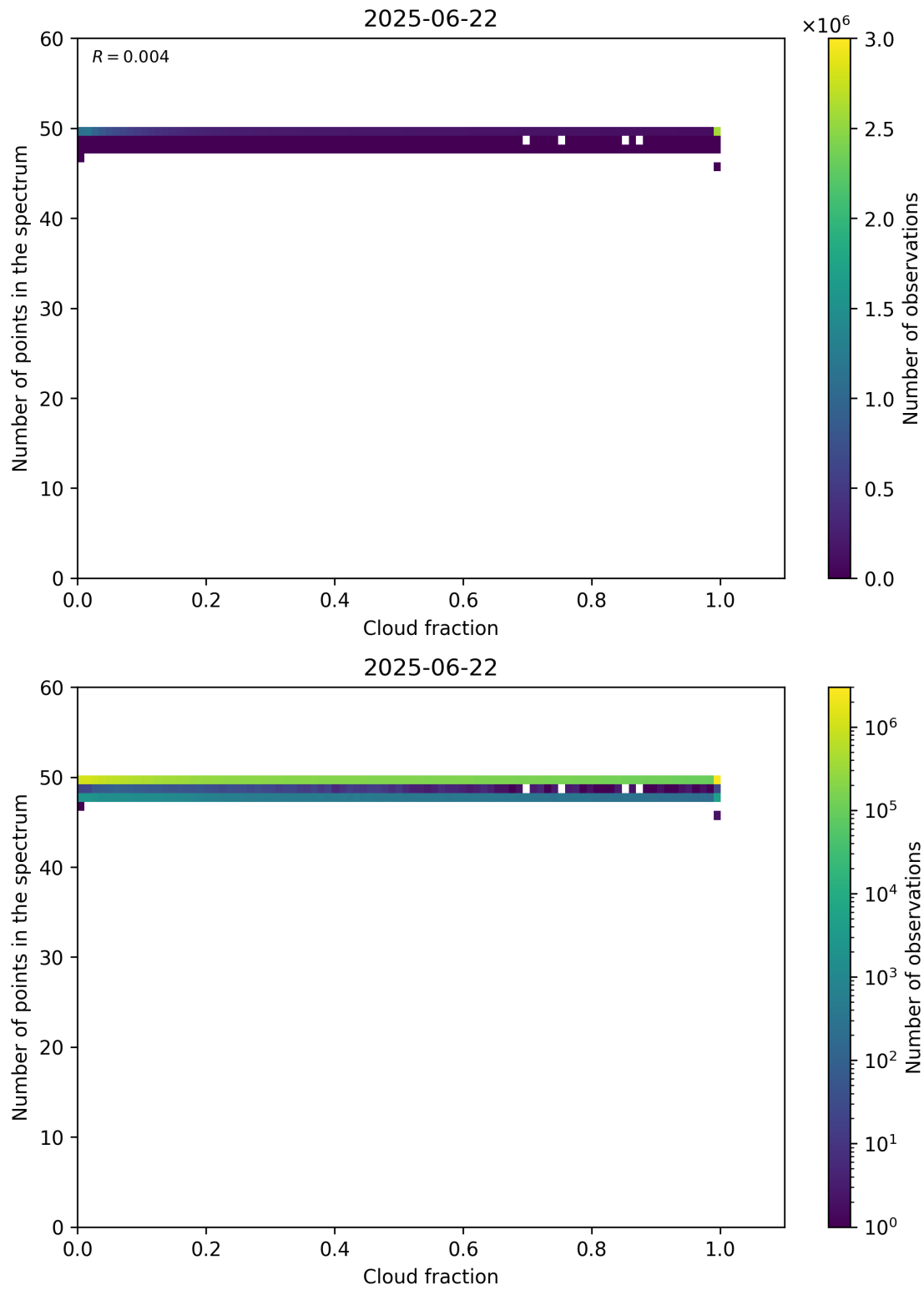
Figure 74: Scatter density plot of “Cloud fraction” against “Number of points in the spectrum” for 2025-06-22 to 2025-06-23.
