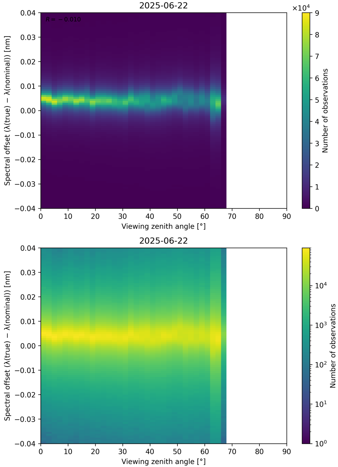
Figure 128: Scatter density plot of “Viewing zenith angle” against “Spectral offset ( \lambda_{\text{true}} - \lambda_{\text{nominal}} )” for 2025-06-22 to 2025-06-23.
