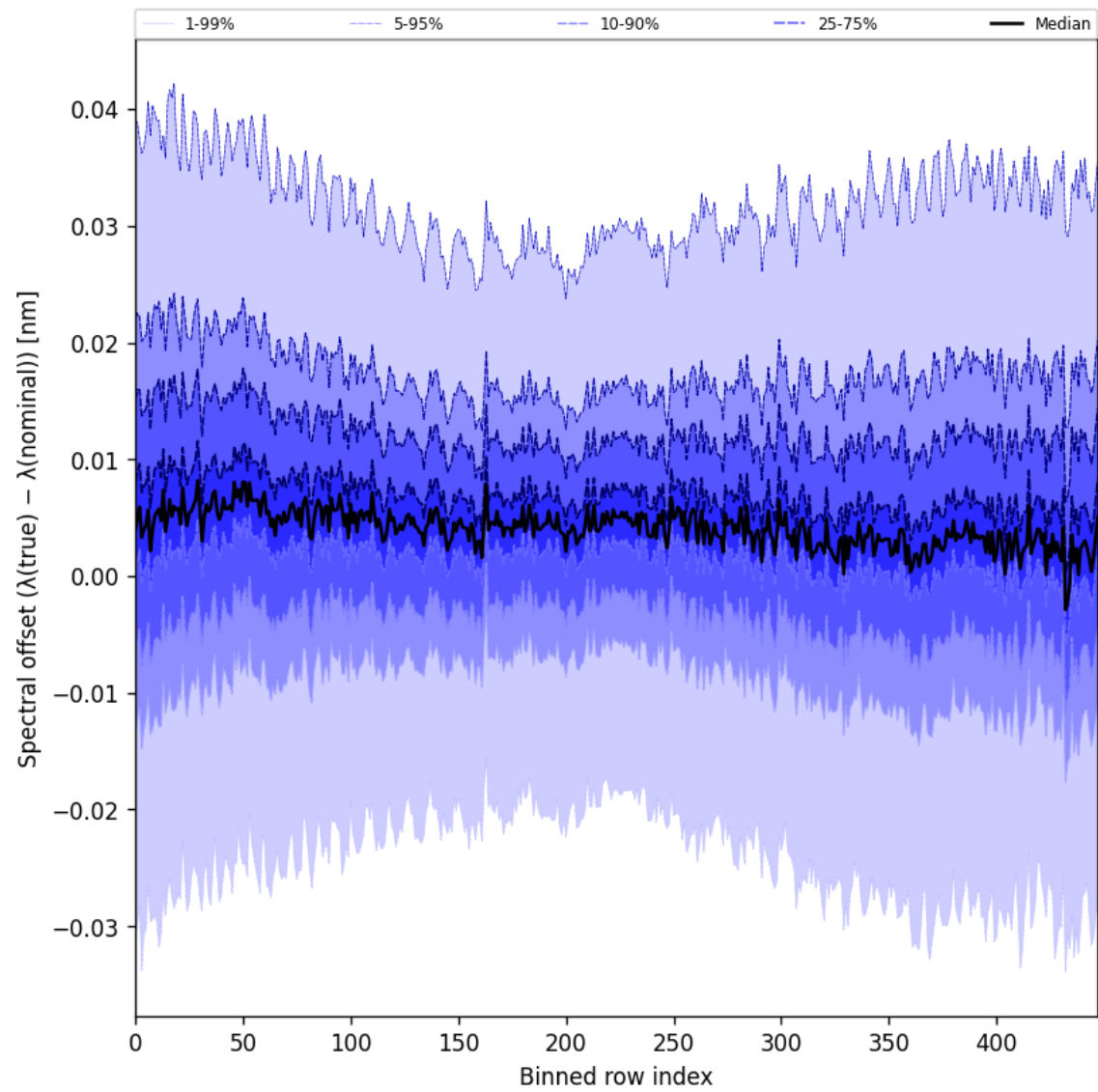
Figure 62: Along track statistics of “Spectral offset ( \lambda_{\text{true}} - \lambda_{\text{nominal}} )” for 2025-06-22 to 2025-06-23
