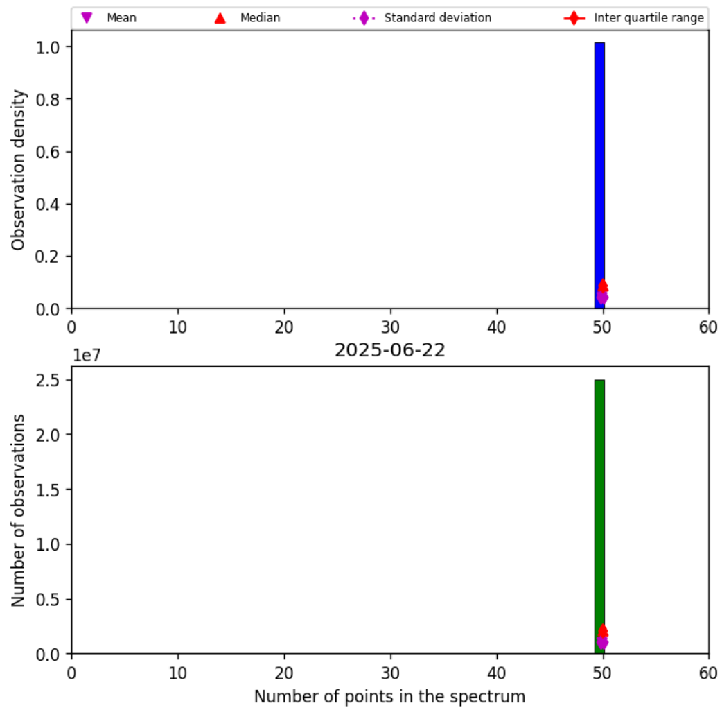
Figure 44: Histogram of “Number of points in the spectrum” for 2025-06-22 to 2025-06-23
