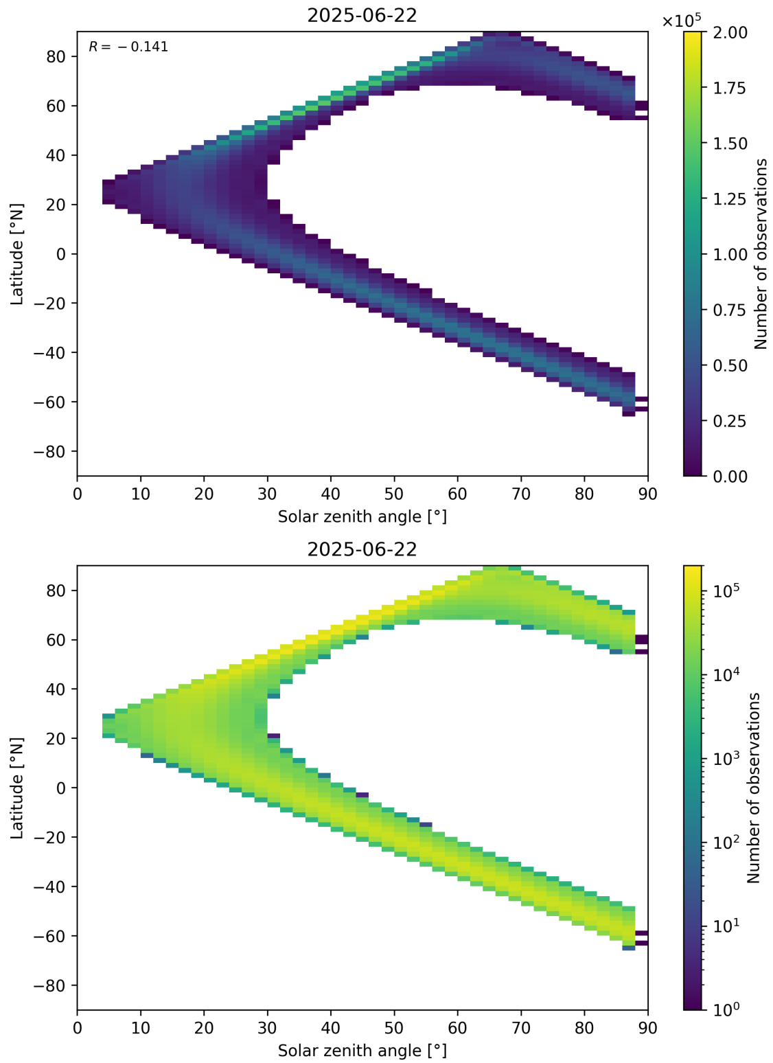
Figure 113: Scatter density plot of “Solar zenith angle” against “Latitude” for 2025-06-22 to 2025-06-23.
