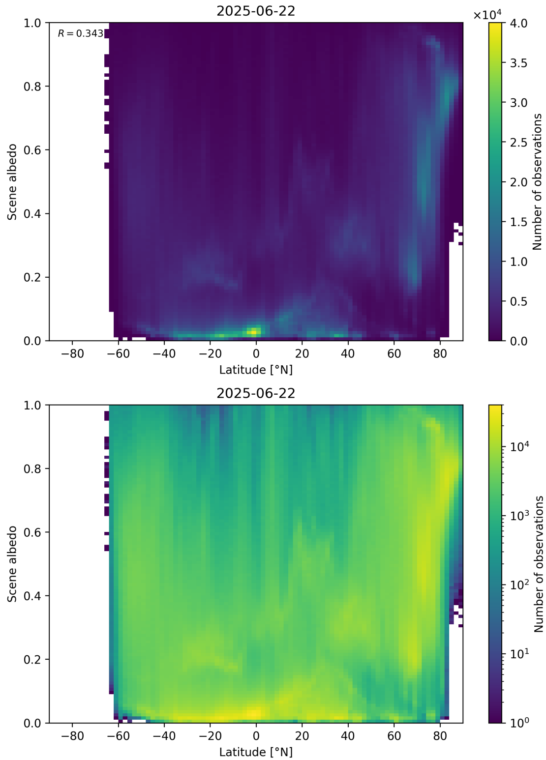
Figure 95: Scatter density plot of “Latitude” against “Scene albedo” for 2025-06-22 to 2025-06-23.
