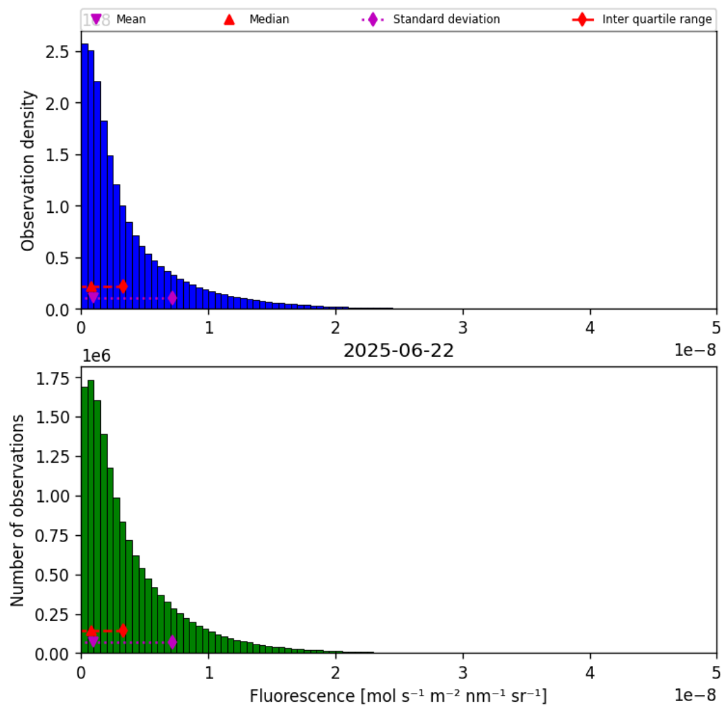
Figure 40: Histogram of “Fluorescence” for 2025-06-22 to 2025-06-23
