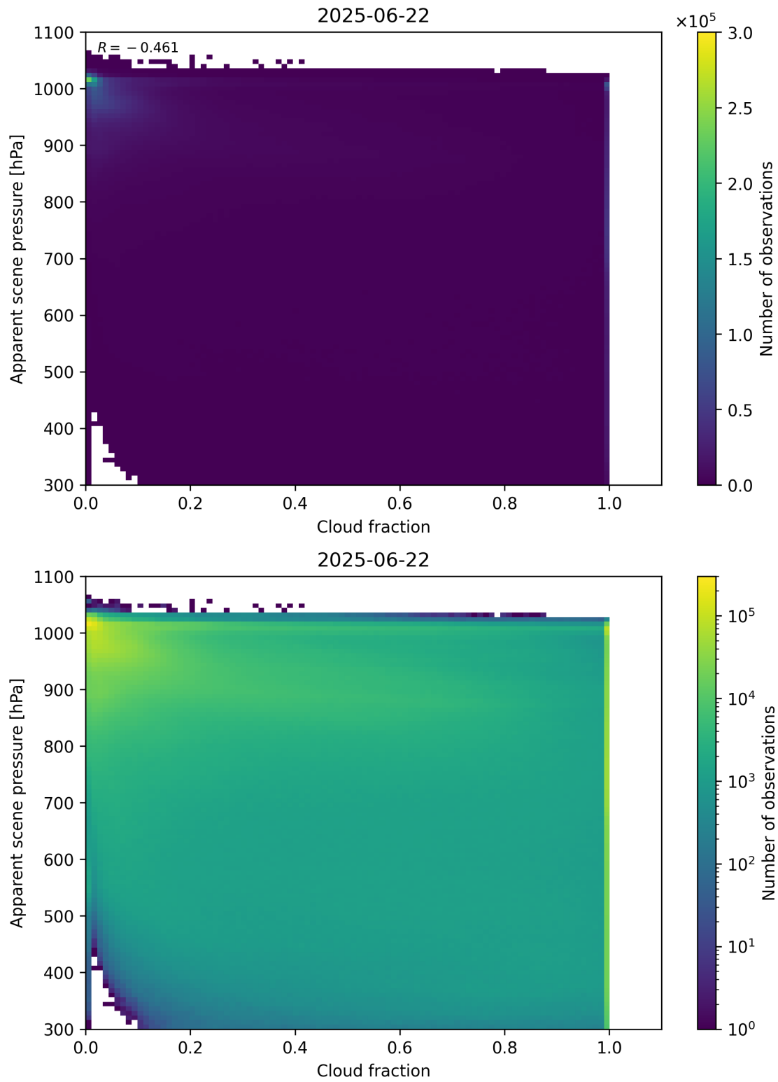
Figure 70: Scatter density plot of “Cloud fraction” against “Apparent scene pressure” for 2025-06-22 to 2025-06-23.
