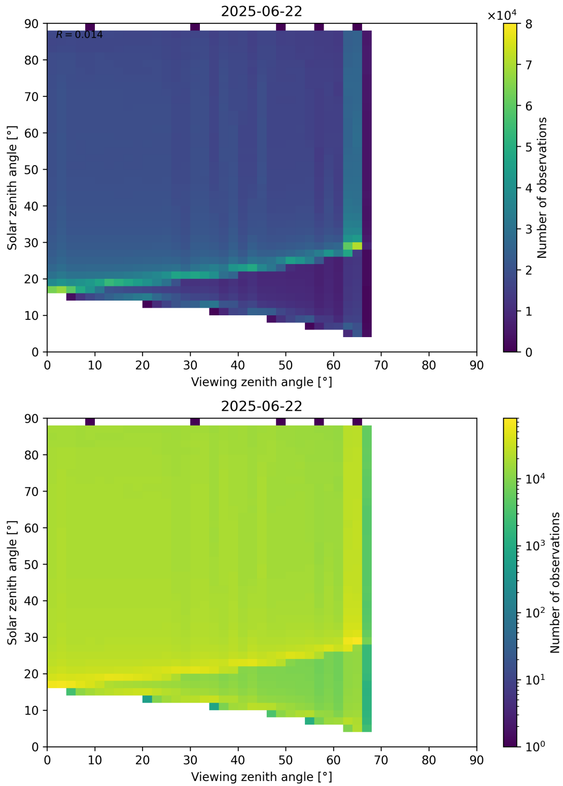
Figure 127: Scatter density plot of “Viewing zenith angle” against “Solar zenith angle” for 2025-06-22 to 2025-06-23.
