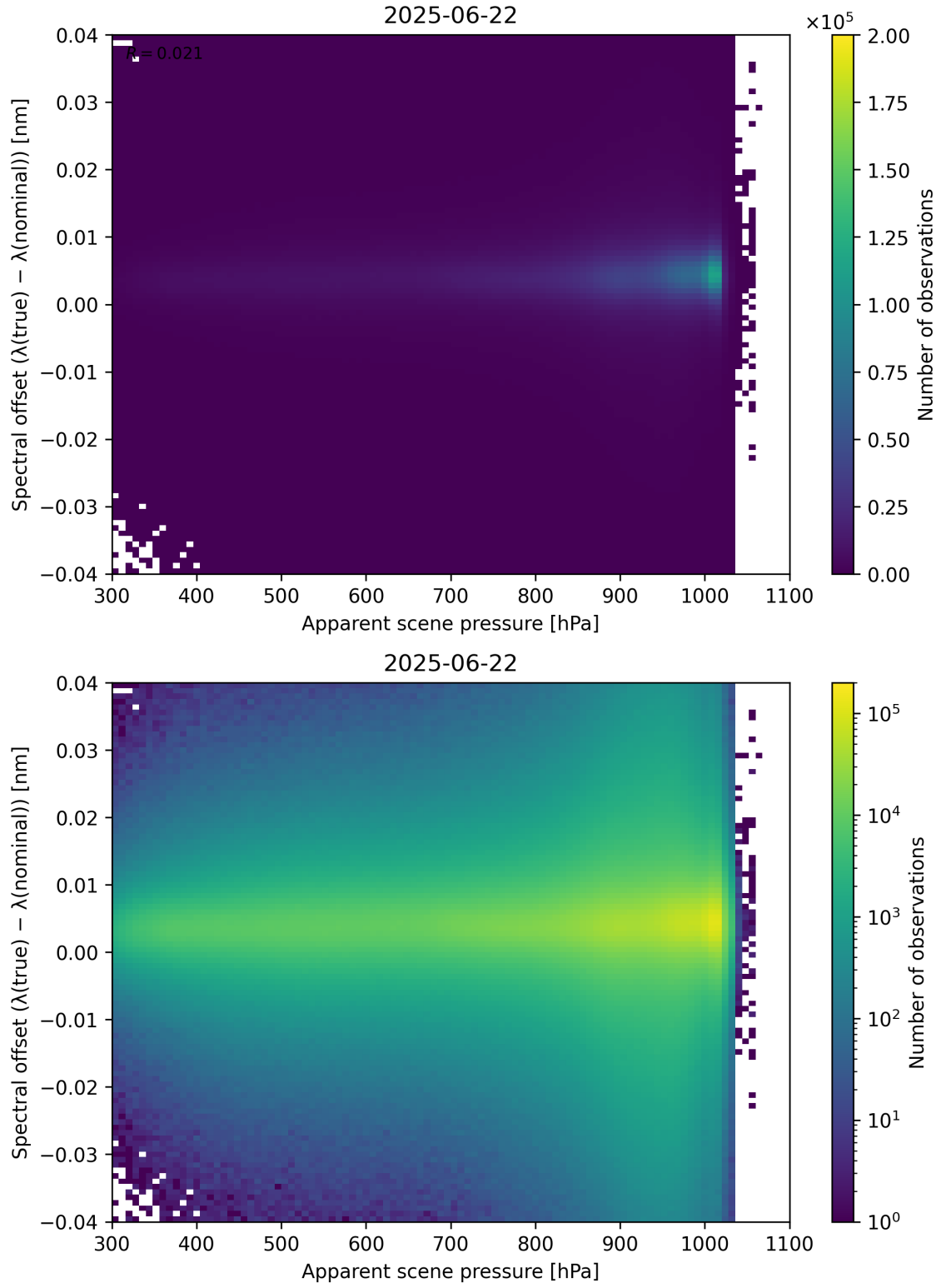
Figure 67: Scatter density plot of “Apparent scene pressure” against “Spectral offset ( \lambda_{\text{true}} - \lambda_{\text{nominal}} )” for 2025-06-22 to 2025-06-23.
