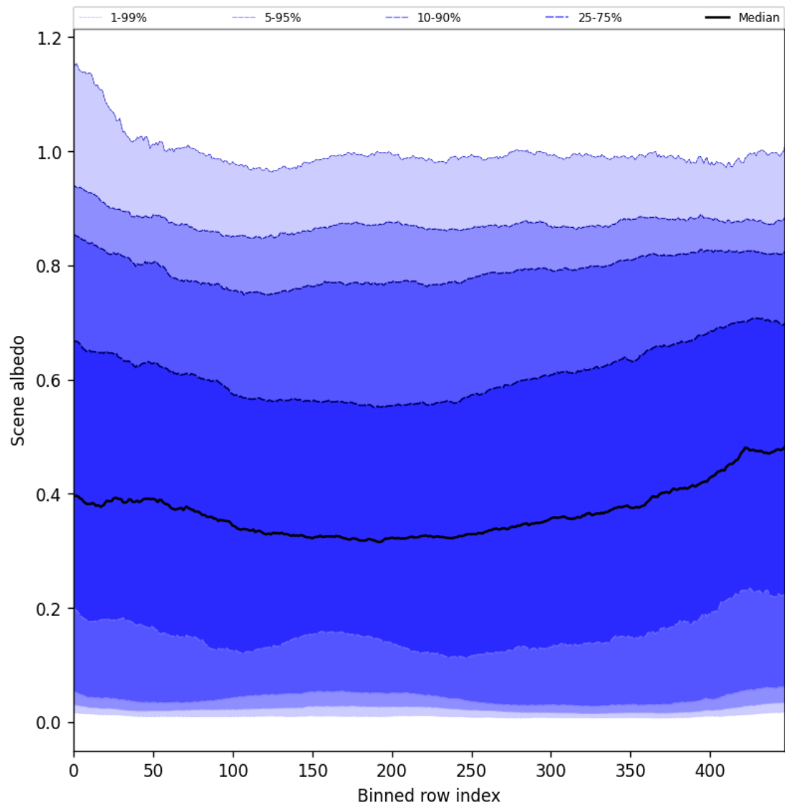
Figure 51: Along track statistics of “Scene albedo” for 2025-06-22 to 2025-06-23
