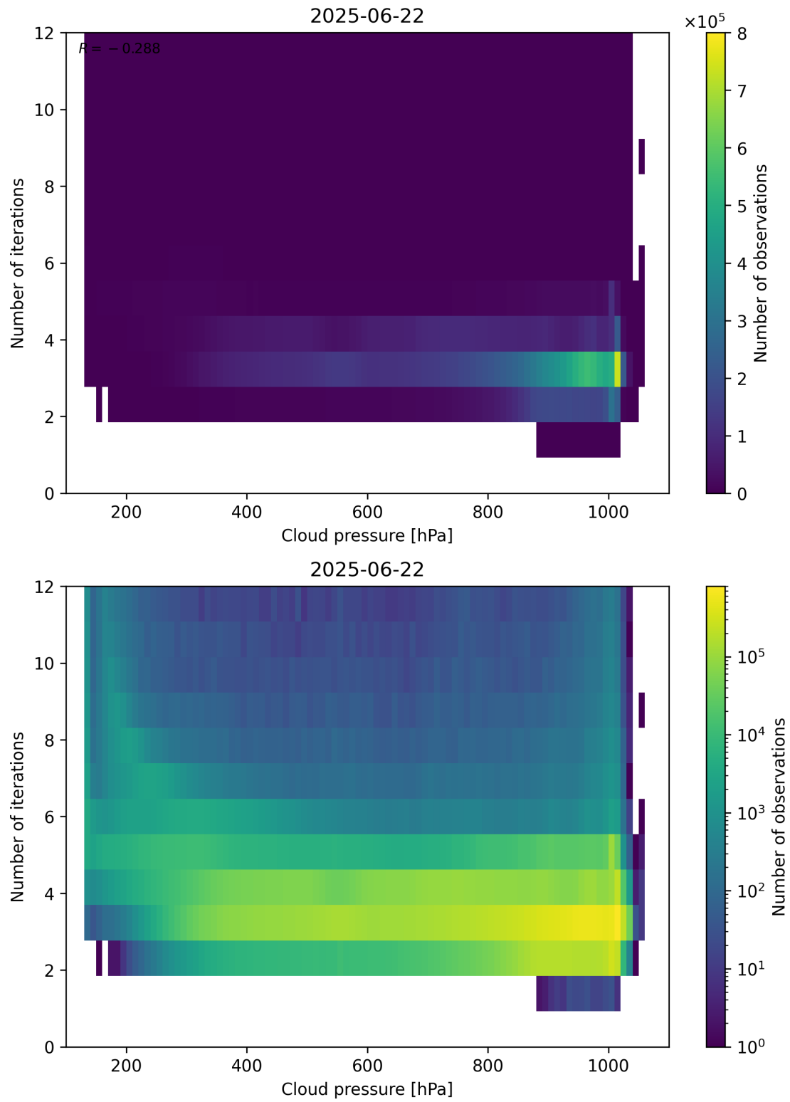
Figure 81: Scatter density plot of “Cloud pressure” against “Number of iterations” for 2025-06-22 to 2025-06-23.
