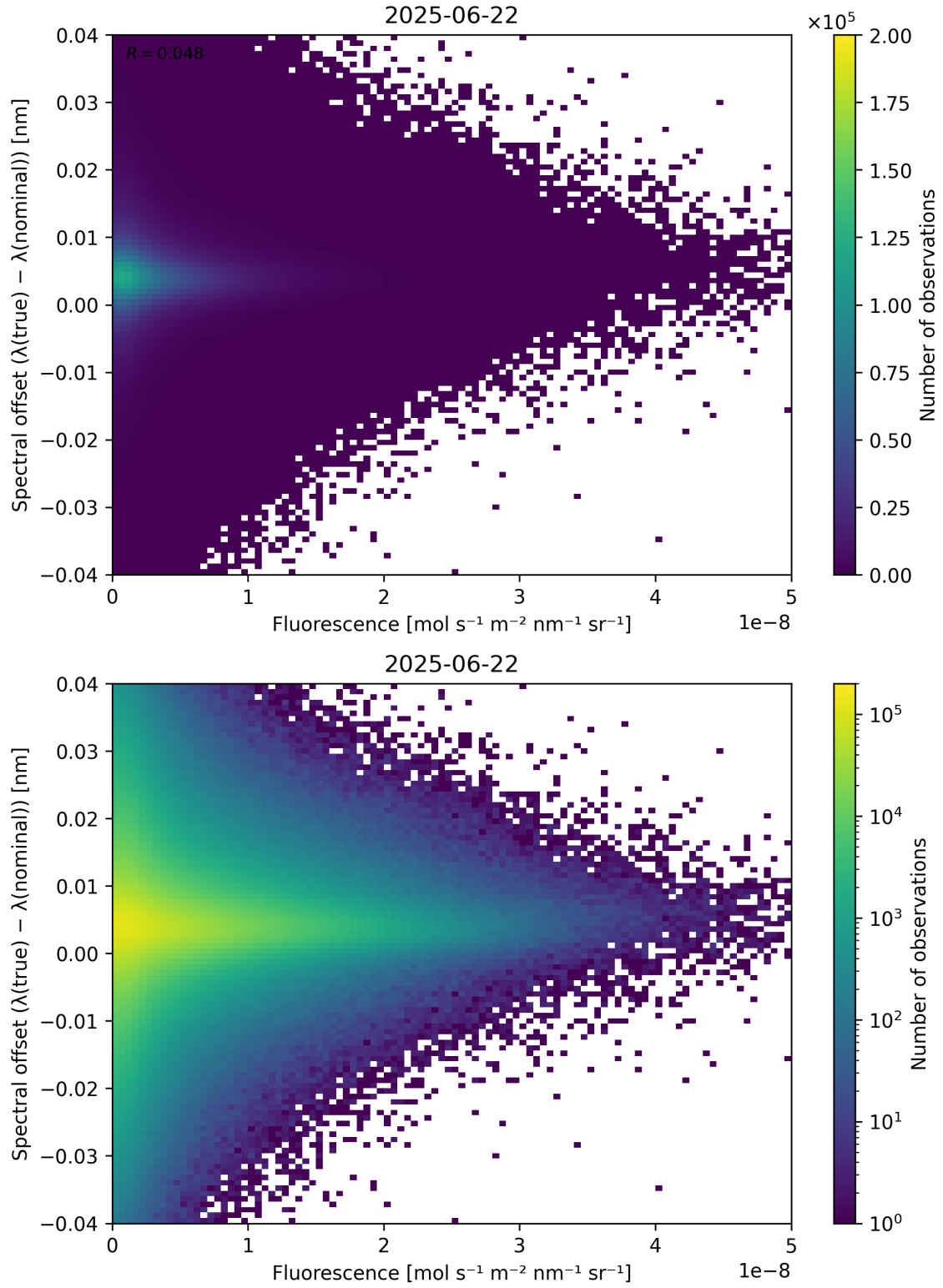
Figure 87: Scatter density plot of “Fluorescence” against “Spectral offset ( \lambda_{\text{true}} - \lambda_{\text{nominal}} )” for 2025-06-22 to 2025-06-23.
