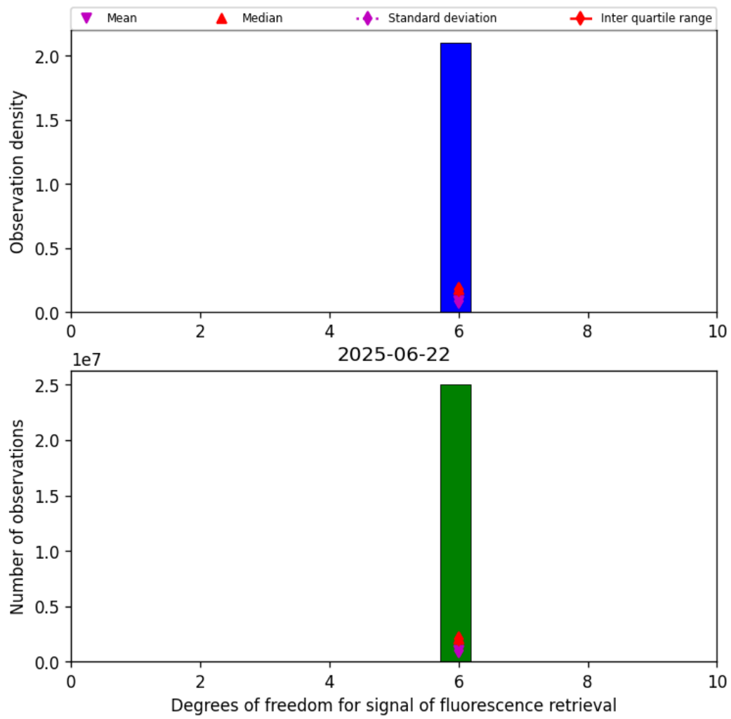
Figure 43: Histogram of “Degrees of freedom for signal of fluorescence retrieval” for 2025-06-22 to 2025-06-23
