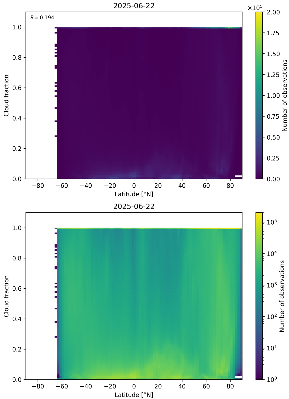
Figure 90: Scatter density plot of “Latitude” against “Cloud fraction” for 2025-06-22 to 2025-06-23.
