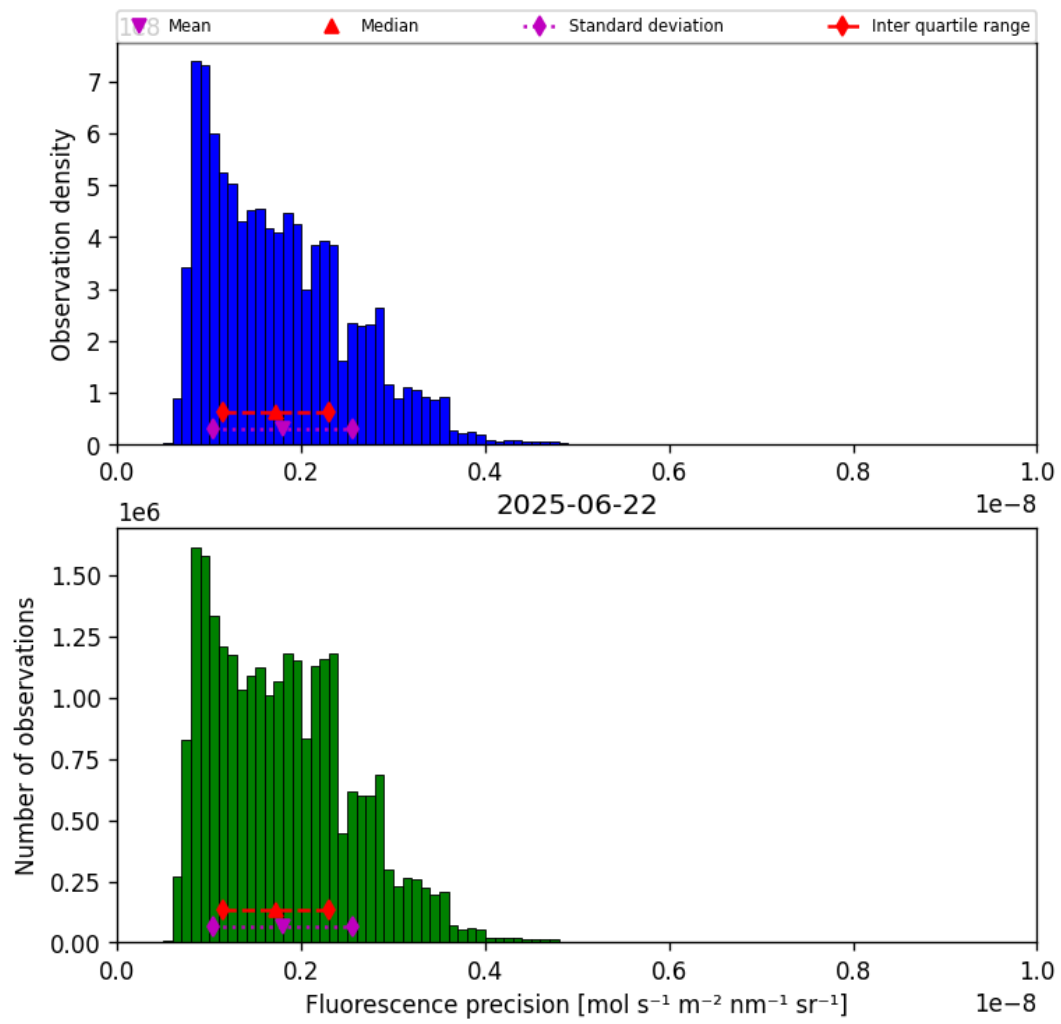
Figure 41: Histogram of “Fluorescence precision” for 2025-06-22 to 2025-06-23
