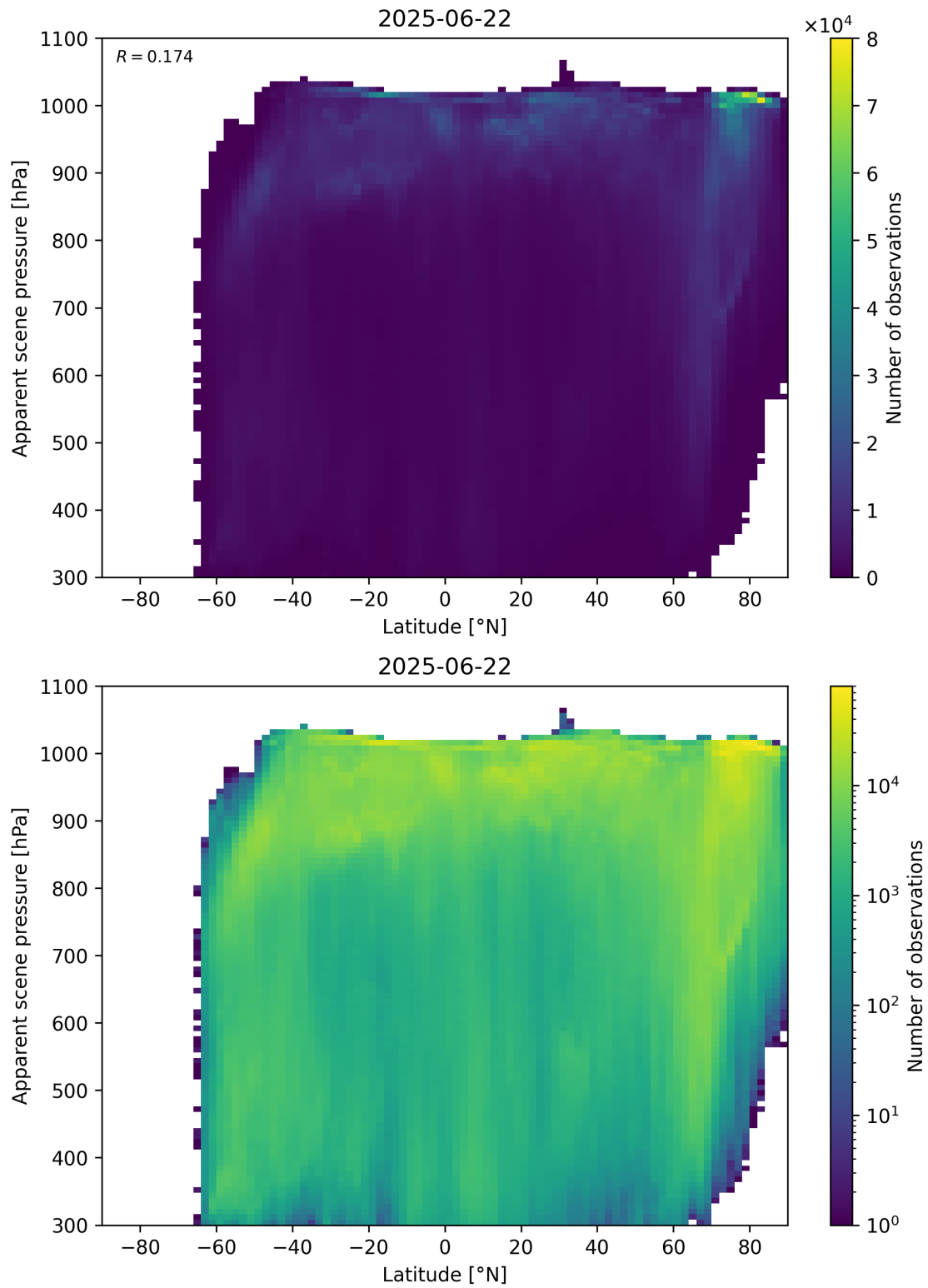
Figure 88: Scatter density plot of “Latitude” against “Apparent scene pressure” for 2025-06-22 to 2025-06-23.
