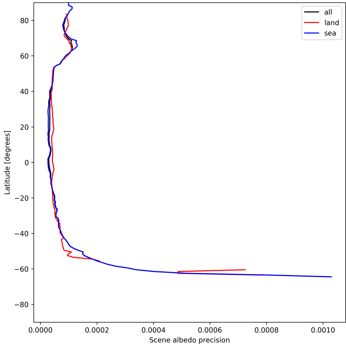
Figure 18: Zonal average of “Scene albedo precision” for 2025-06-22 to 2025-06-23.
