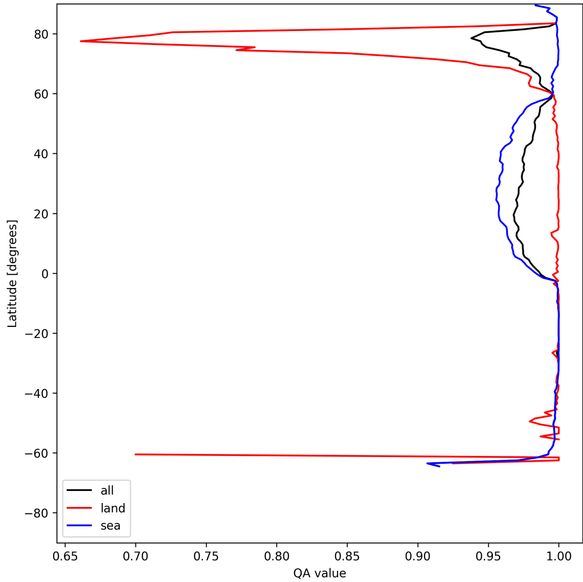
Figure 12: Zonal average of “QA value” for 2025-06-22 to 2025-06-23.
