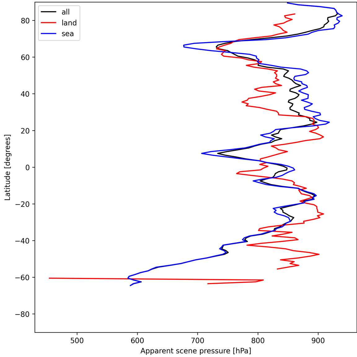
Figure 19: Zonal average of “Apparent scene pressure” for 2025-06-22 to 2025-06-23.
