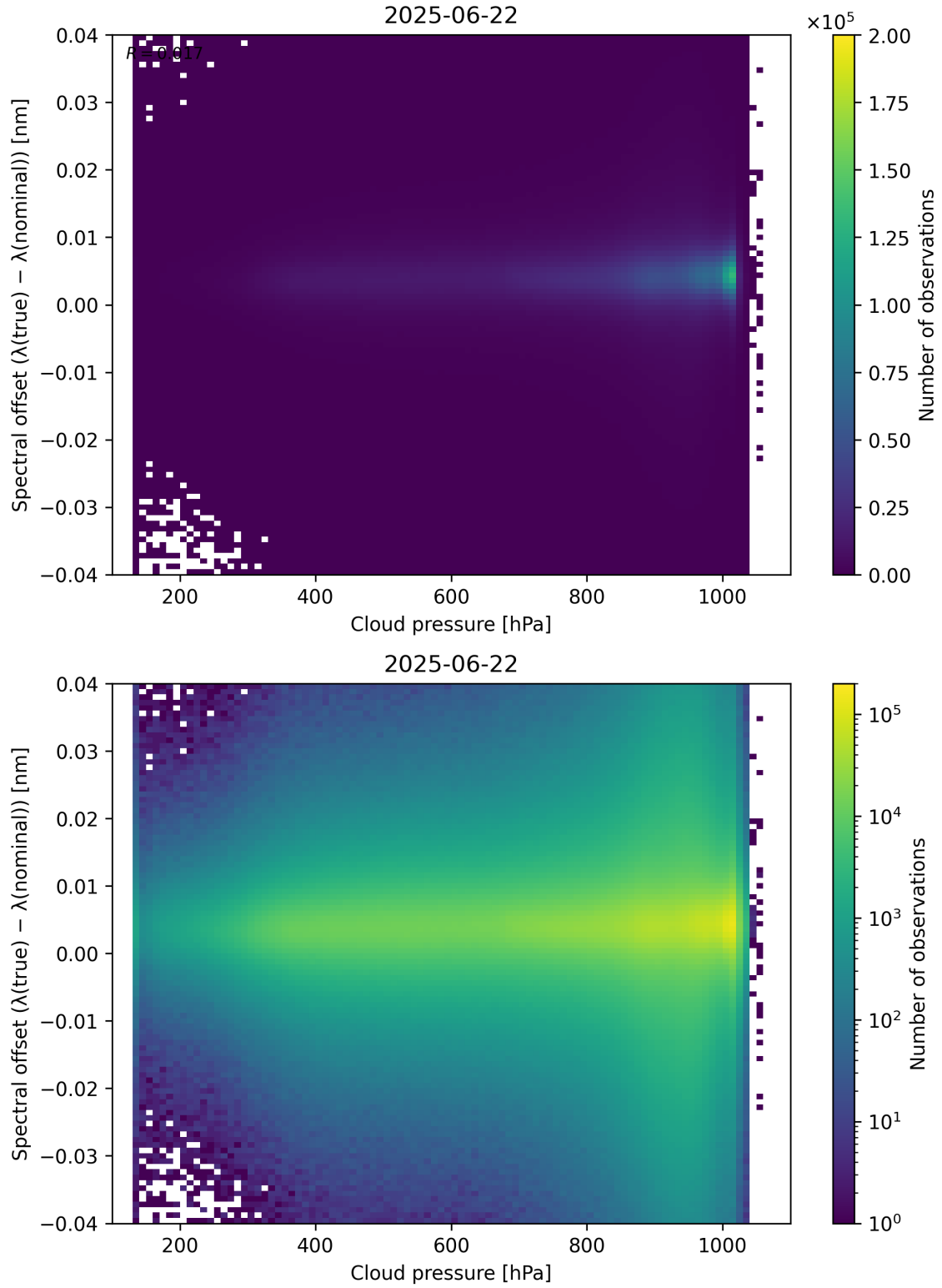
Figure 84: Scatter density plot of “Cloud pressure” against “Spectral offset ( \lambda_{\text{true}} - \lambda_{\text{nominal}} )” for 2025-06-22 to 2025-06-23.
