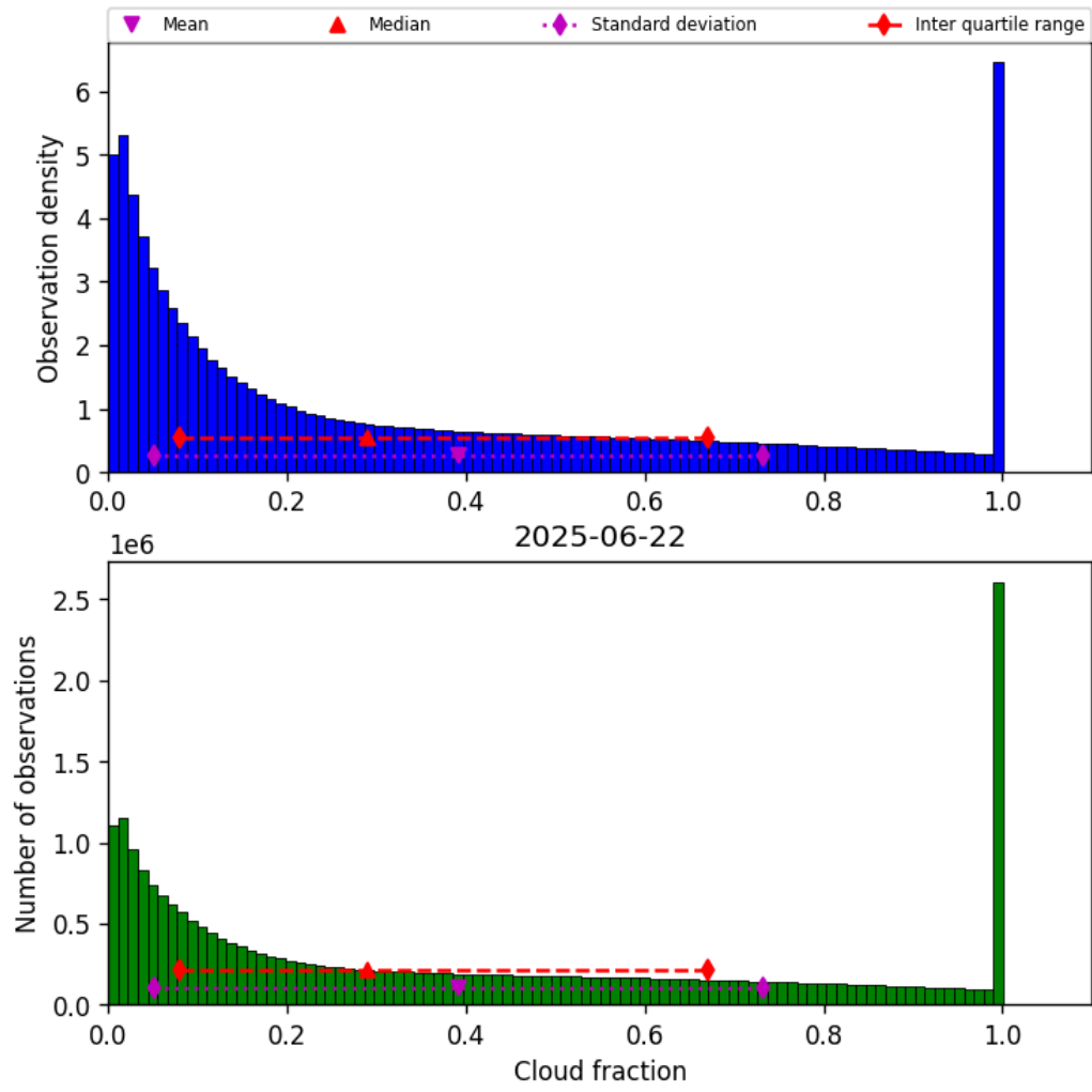
Figure 32: Histogram of “Cloud fraction” for 2025-06-22 to 2025-06-23
