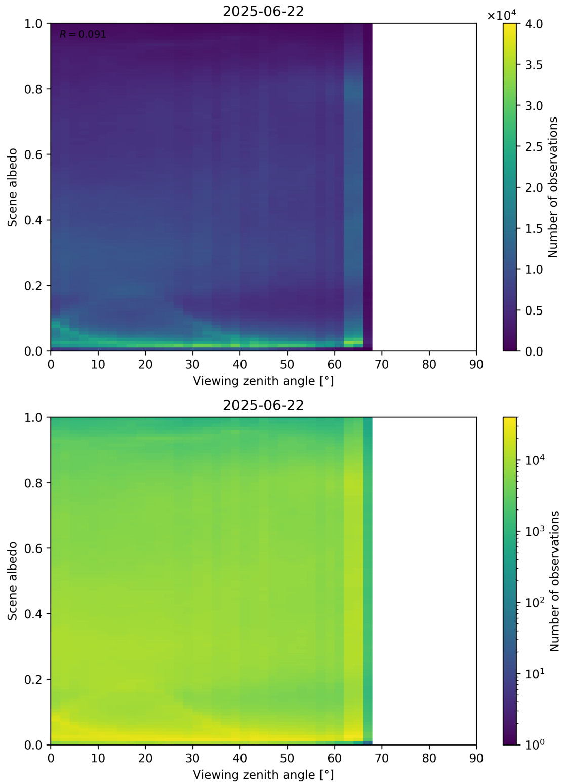
Figure 126: Scatter density plot of “Viewing zenith angle” against “Scene albedo” for 2025-06-22 to 2025-06-23.
