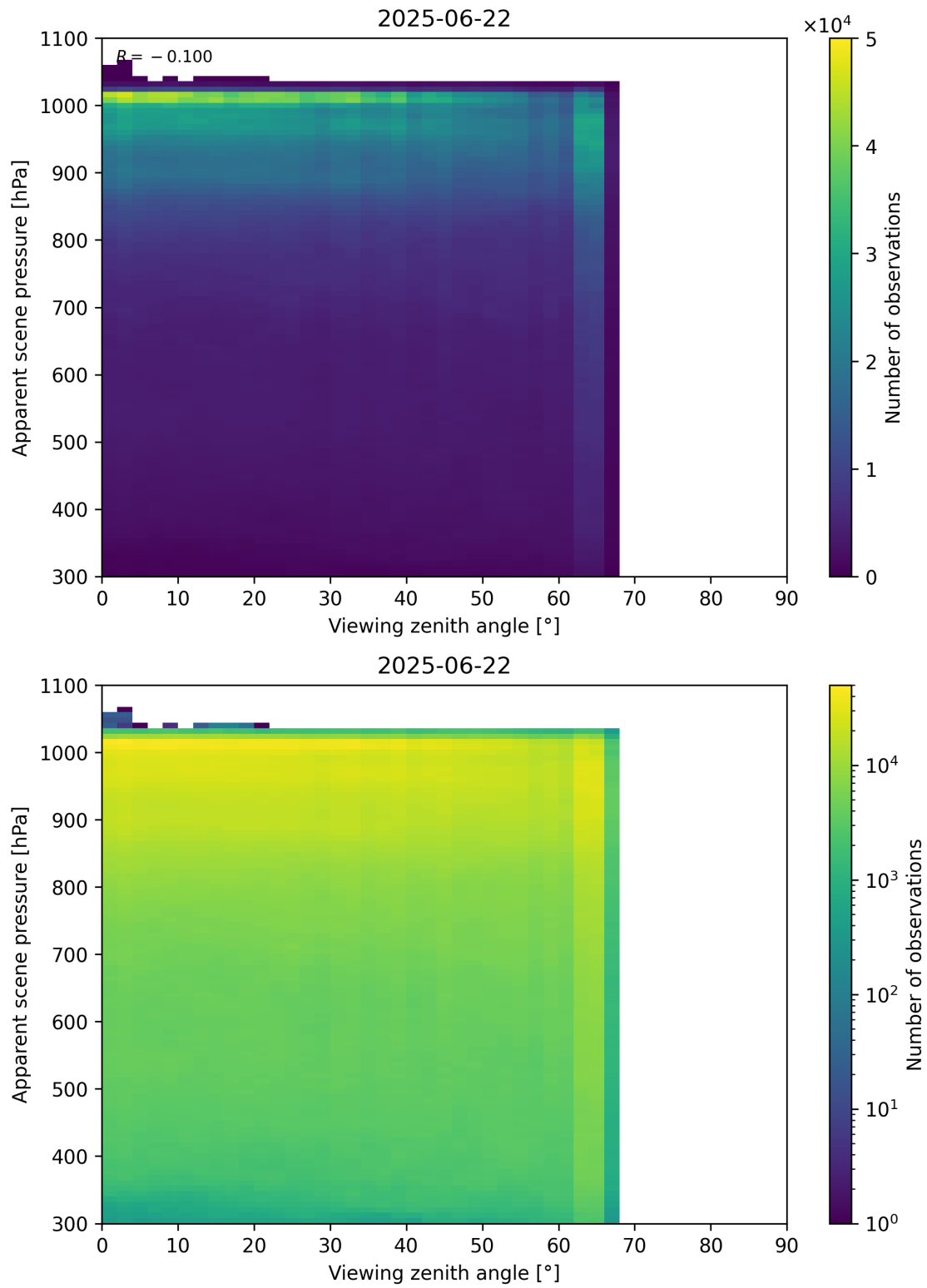
Figure 118: Scatter density plot of “Viewing zenith angle” against “Apparent scene pressure” for 2025-06-22 to 2025-06-23.
