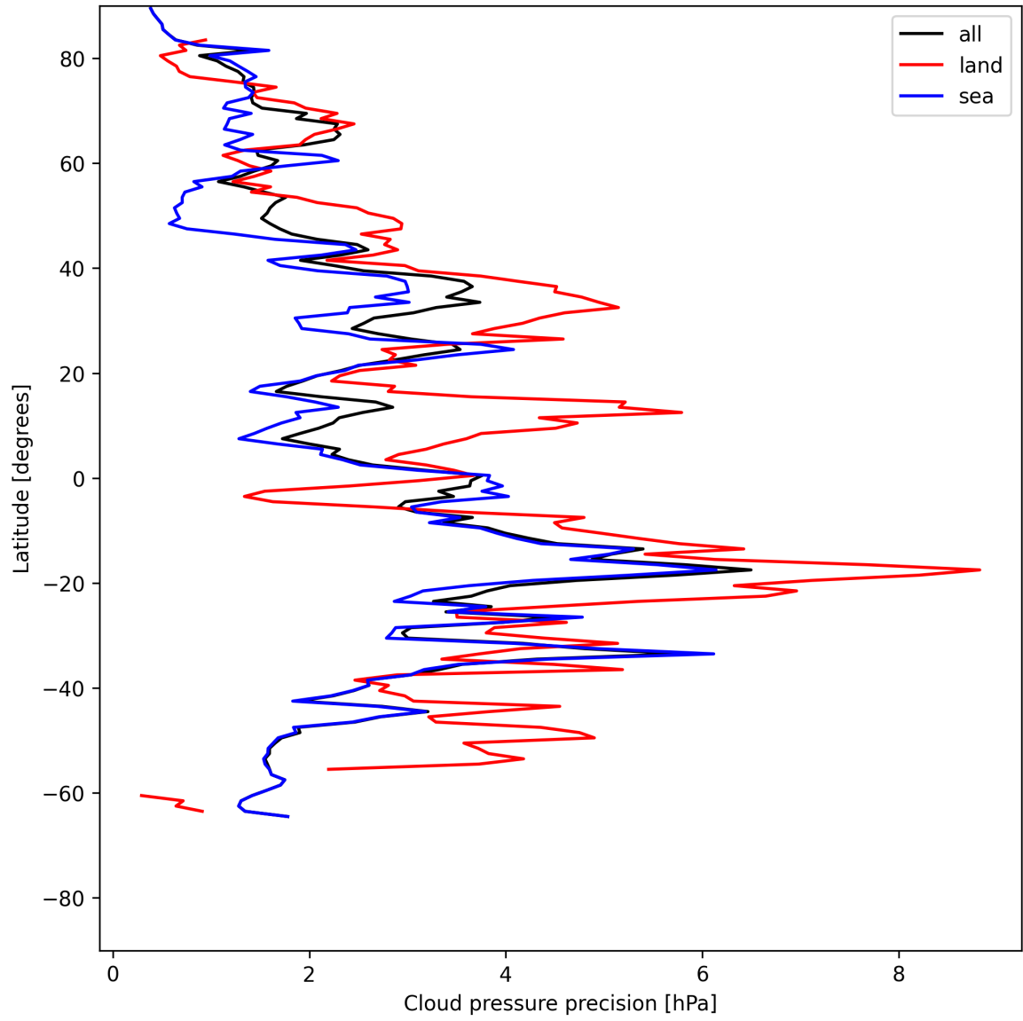
Figure 14: Zonal average of “Cloud pressure precision” for 2025-06-22 to 2025-06-23.
