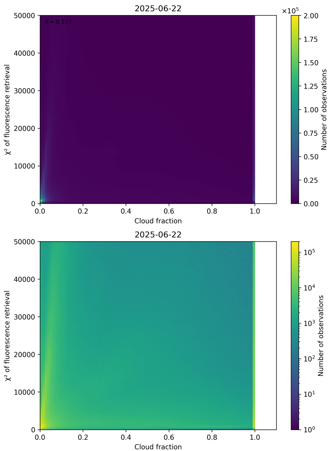
Figure 71: Scatter density plot of “Cloud fraction” against “ \chi^2 of fluorescence retrieval” for 2025-06-22 to 2025-06-23.
