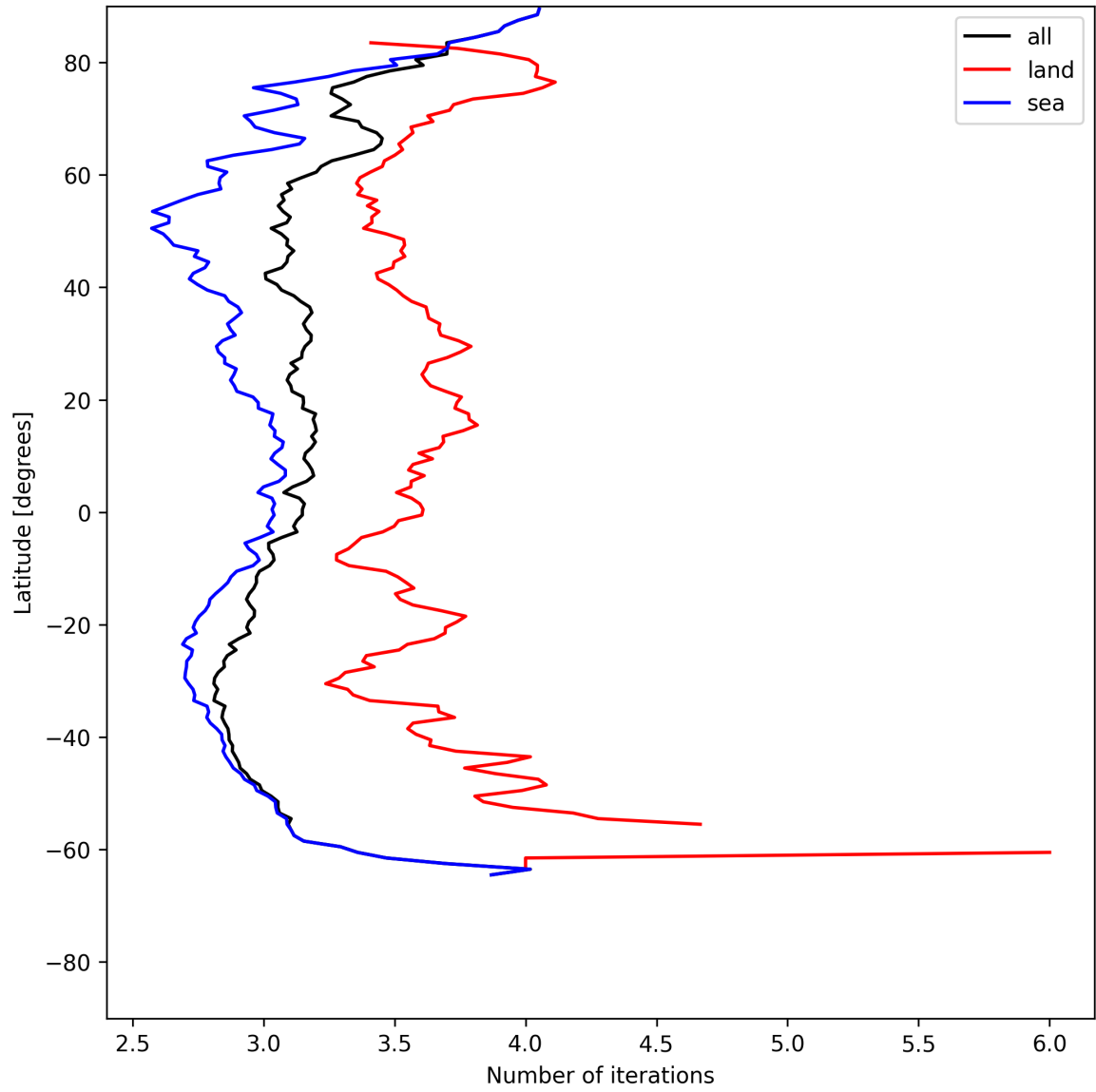
Figure 22: Zonal average of “Number of iterations” for 2025-06-22 to 2025-06-23.
