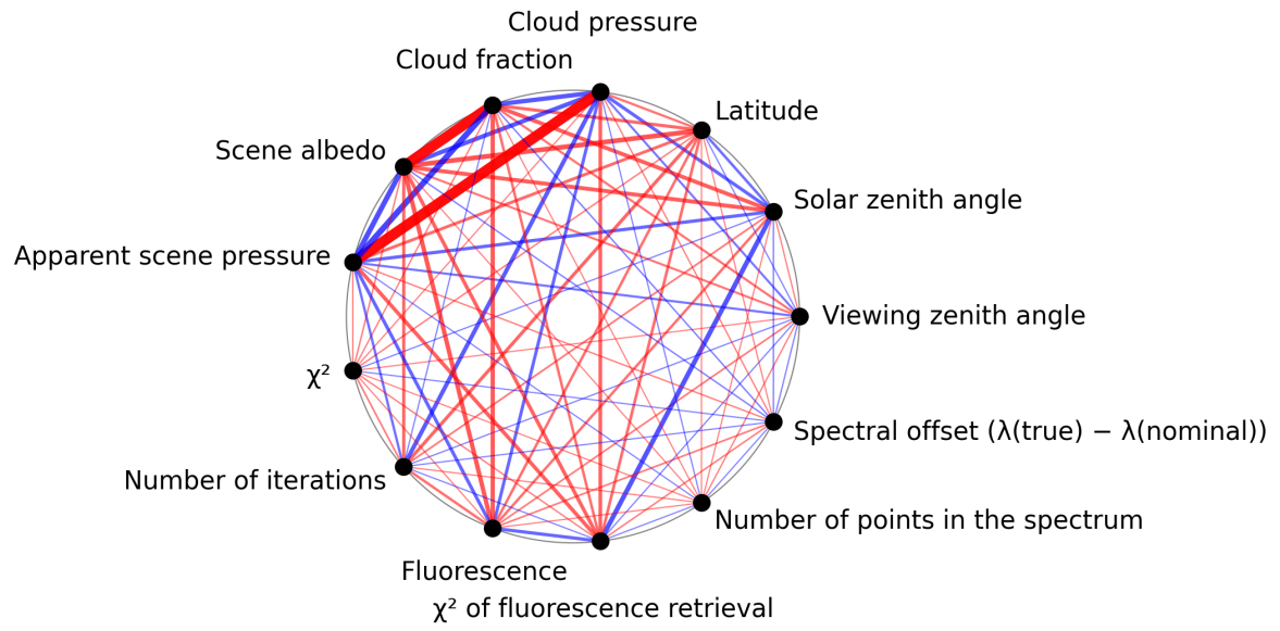
Figure 1: Map of correlation graph for 2025-06-22 to 2025-06-23.
