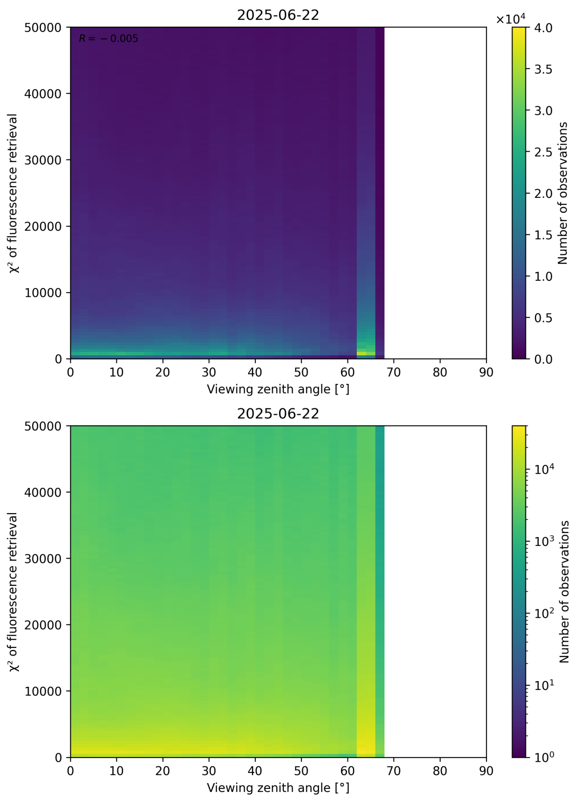
Figure 119: Scatter density plot of “Viewing zenith angle” against “ \chi^2 of fluorescence retrieval” for 2025-06-22 to 2025-06-23.
