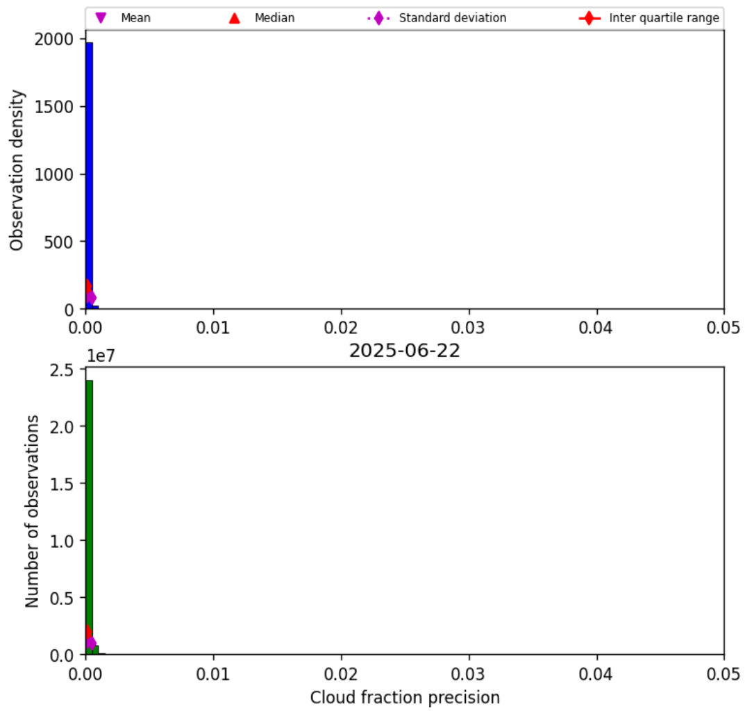
Figure 33: Histogram of “Cloud fraction precision” for 2025-06-22 to 2025-06-23
