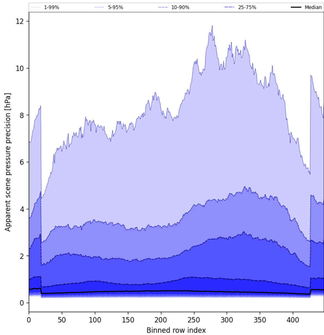
Figure 54: Along track statistics of “Apparent scene pressure precision” for 2025-06-22 to 2025-06-23
