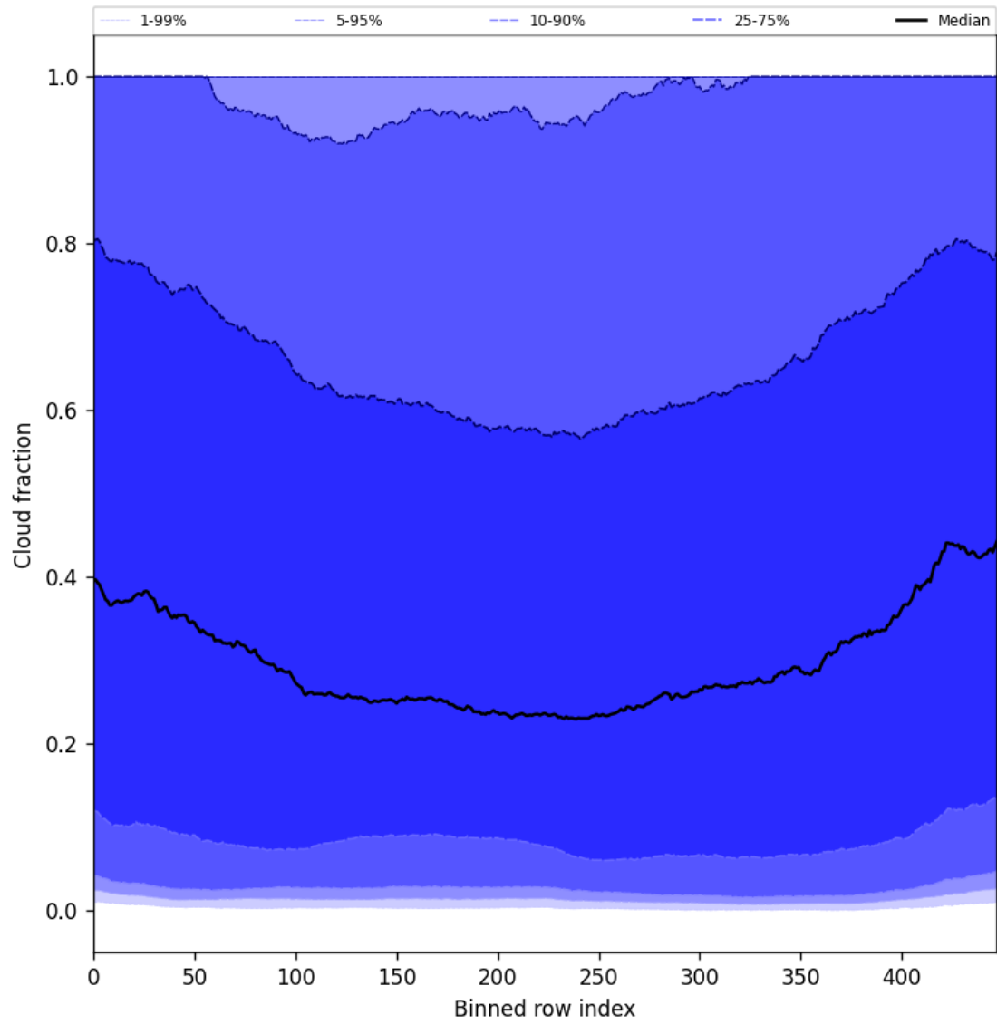
Figure 49: Along track statistics of “Cloud fraction” for 2025-06-22 to 2025-06-23
