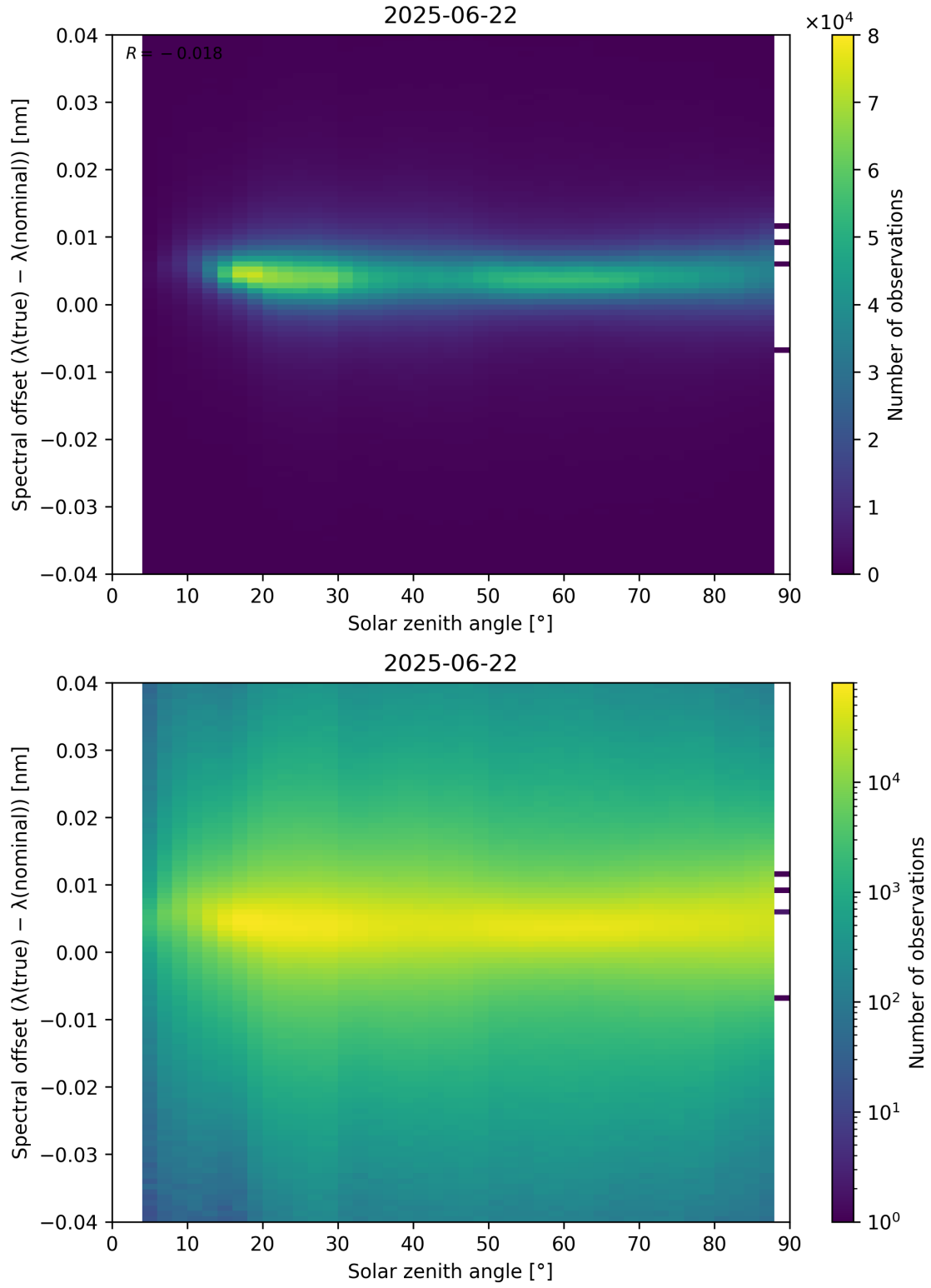
Figure 117: Scatter density plot of “Solar zenith angle” against “Spectral offset ( \lambda_{\text{true}} - \lambda_{\text{nominal}} )” for 2025-06-22 to 2025-06-23.
