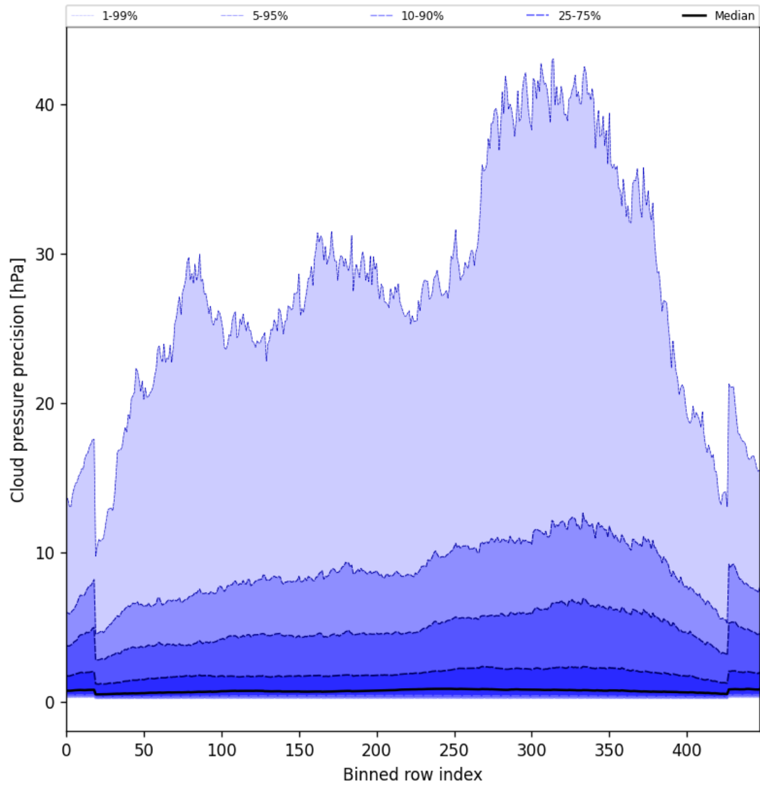
Figure 48: Along track statistics of “Cloud pressure precision” for 2025-06-22 to 2025-06-23
