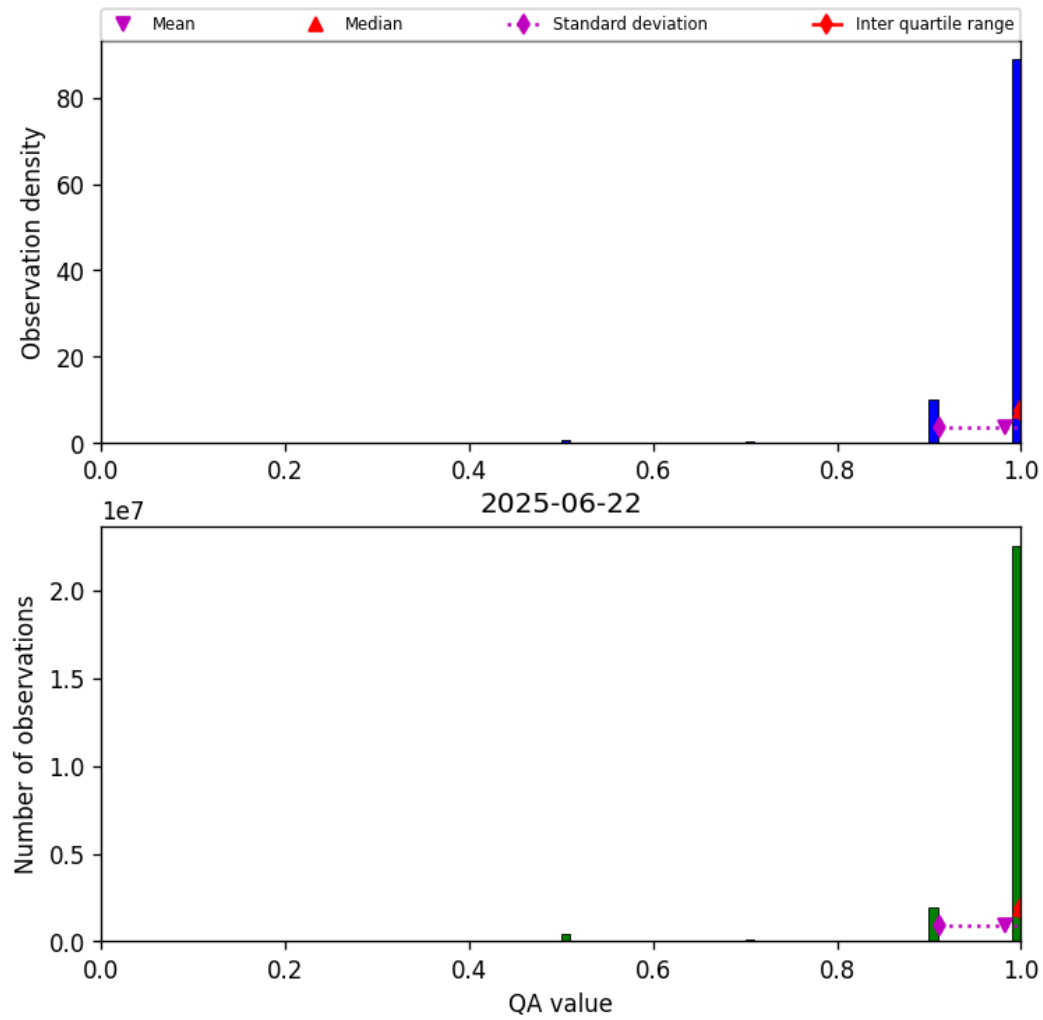
Figure 29: Histogram of “QA value” for 2025-06-22 to 2025-06-23
