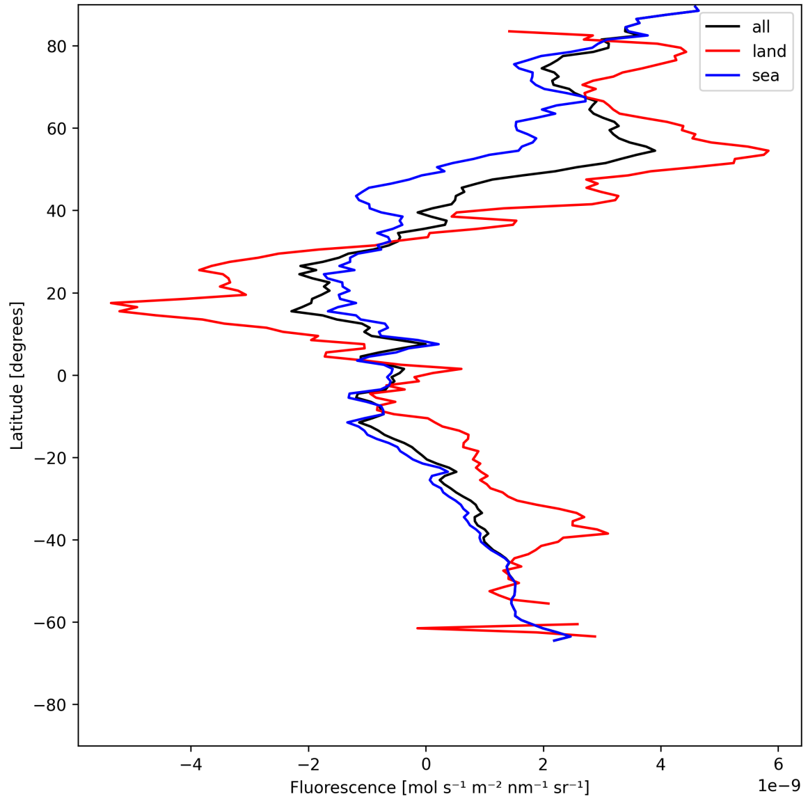
Figure 23: Zonal average of “Fluorescence” for 2025-06-22 to 2025-06-23.
