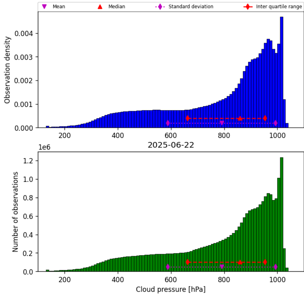
Figure 30: Histogram of “Cloud pressure” for 2025-06-22 to 2025-06-23
