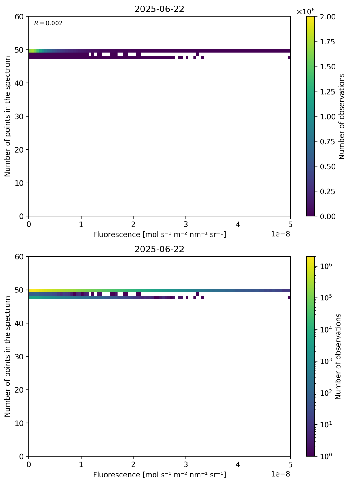
Figure 86: Scatter density plot of “Fluorescence” against “Number of points in the spectrum” for 2025-06-22 to 2025-06-23.
