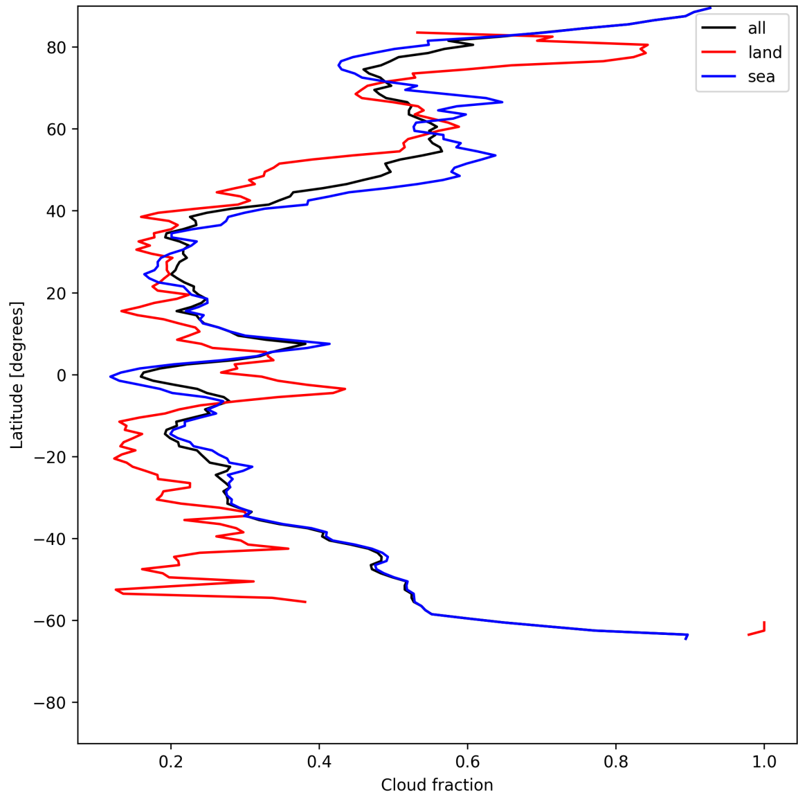
Figure 15: Zonal average of “Cloud fraction” for 2025-06-22 to 2025-06-23.
