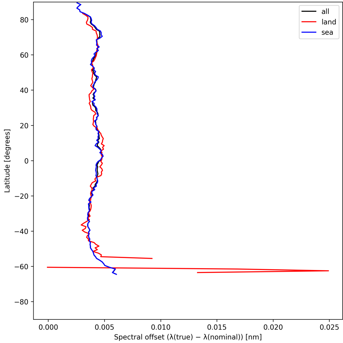
Figure 28: Zonal average of “Spectral offset ( \lambda_{\text{true}} - \lambda_{\text{nominal}} )” for 2025-06-22 to 2025-06-23.
