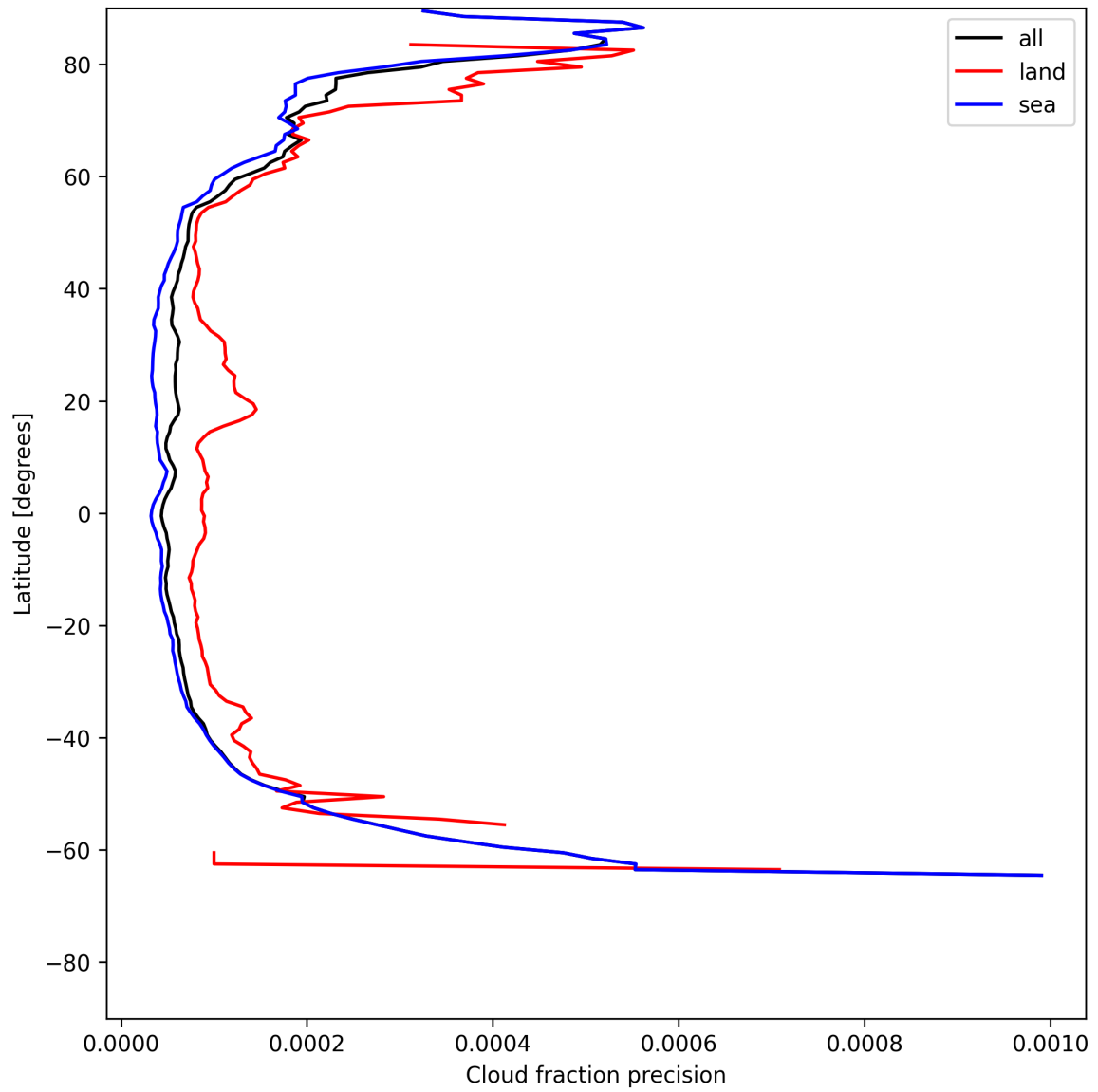
Figure 16: Zonal average of “Cloud fraction precision” for 2025-06-22 to 2025-06-23.
