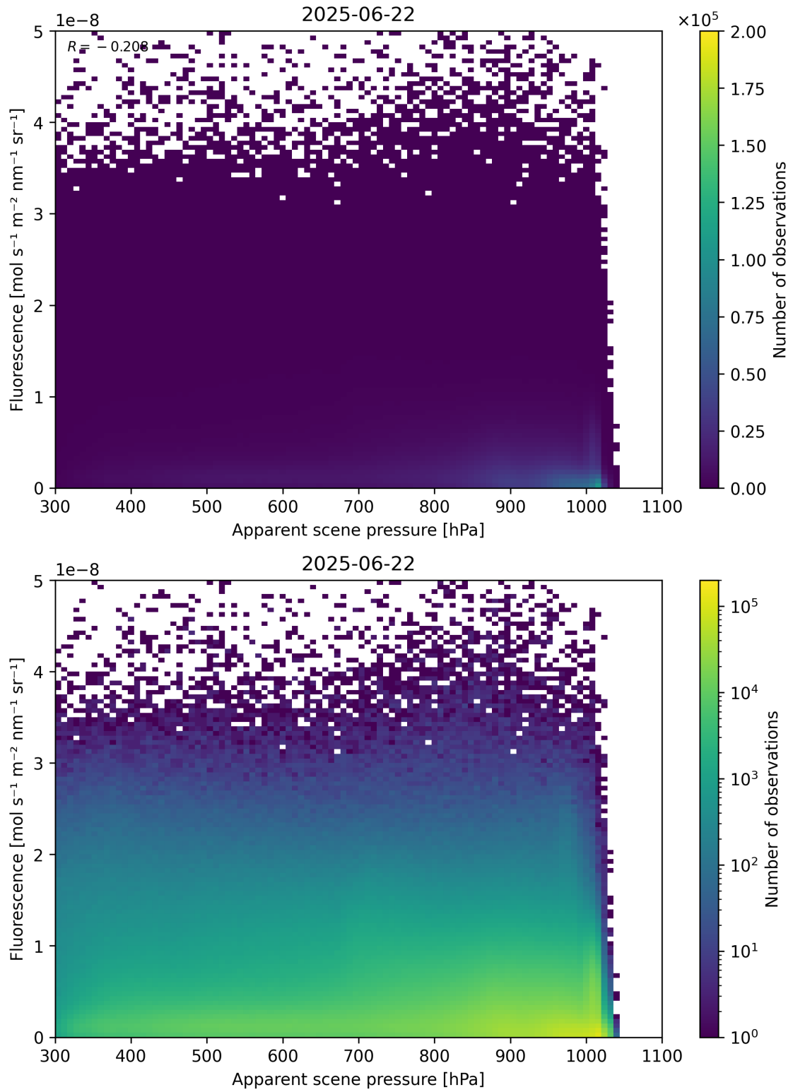
Figure 64: Scatter density plot of “Apparent scene pressure” against “Fluorescence” for 2025-06-22 to 2025-06-23.
