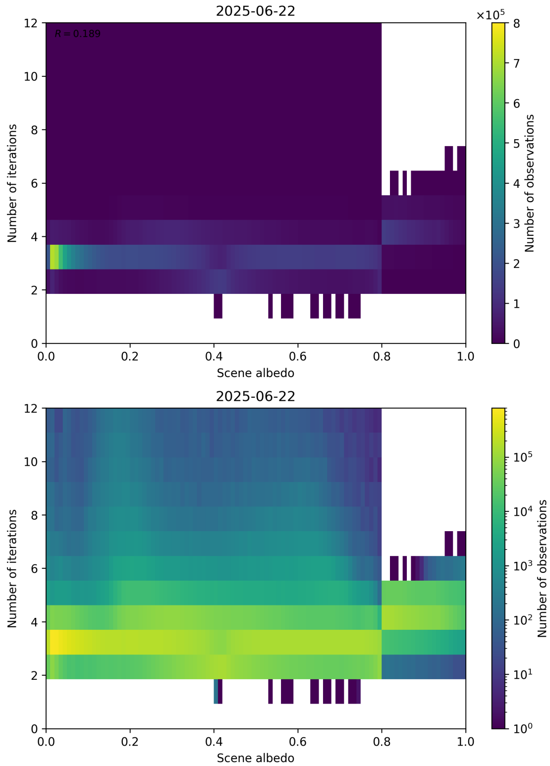
Figure 105: Scatter density plot of “Scene albedo” against “Number of iterations” for 2025-06-22 to 2025-06-23.
