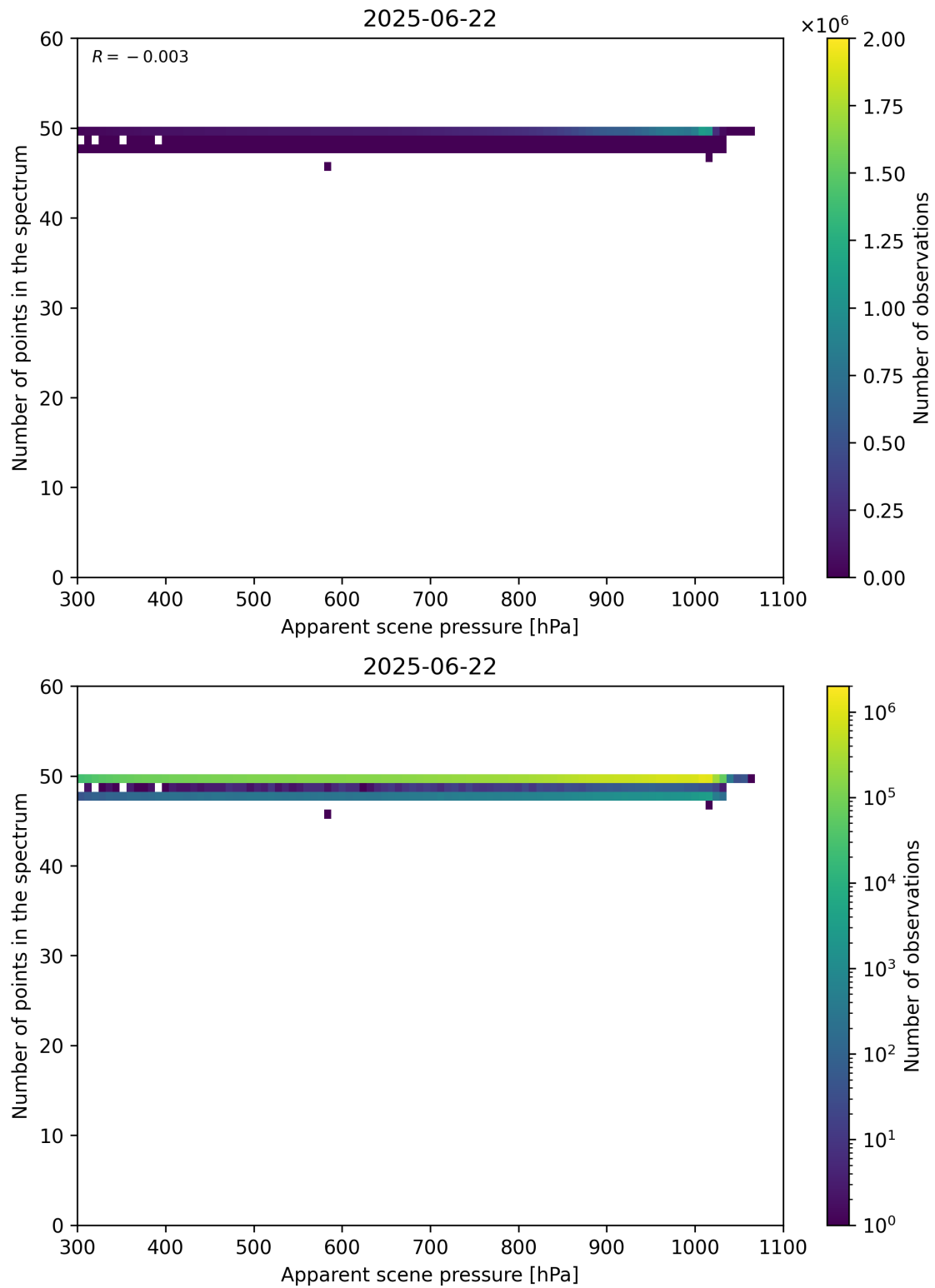
Figure 66: Scatter density plot of “Apparent scene pressure” against “Number of points in the spectrum” for 2025-06-22 to 2025-06-23.
