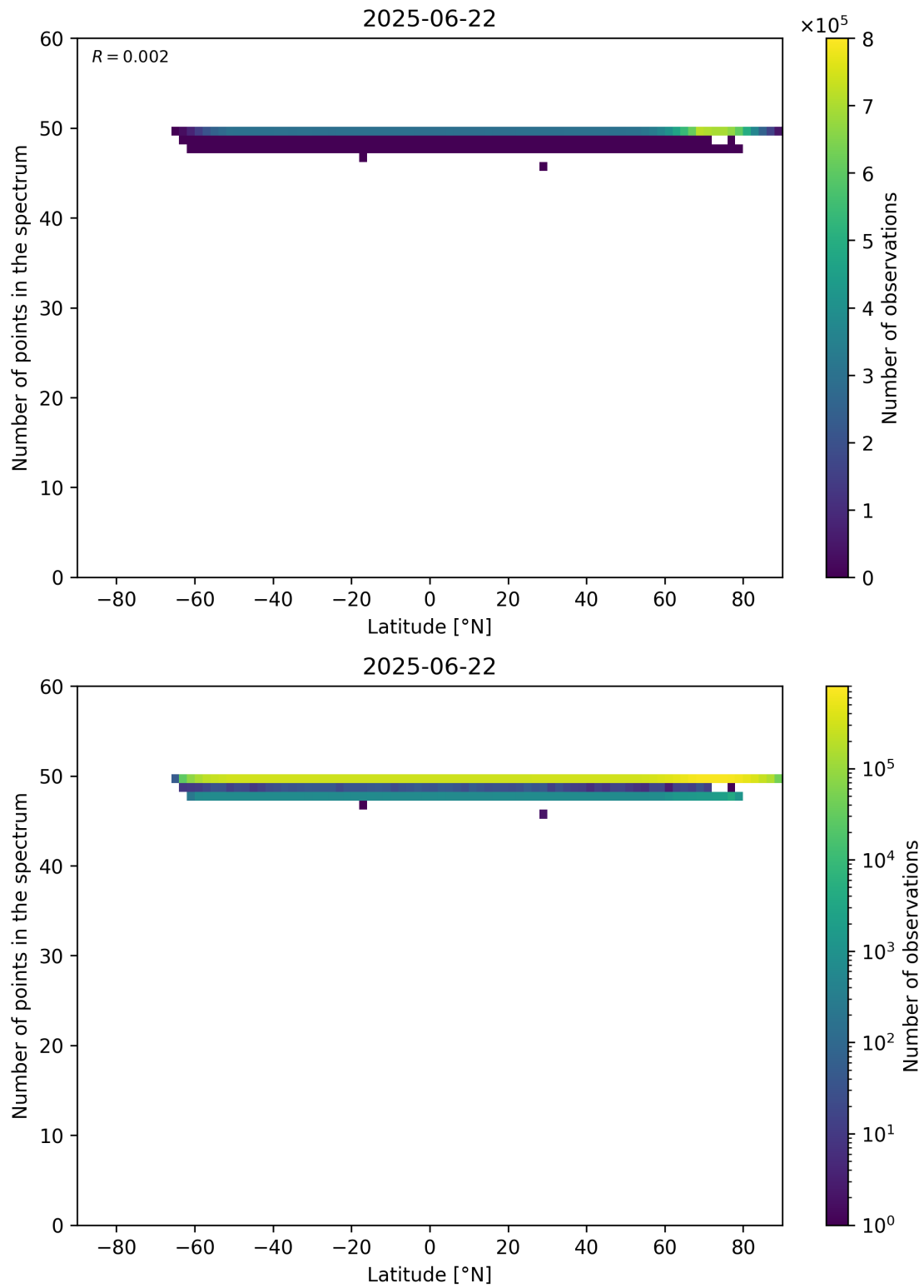
Figure 94: Scatter density plot of “Latitude” against “Number of points in the spectrum” for 2025-06-22 to 2025-06-23.
