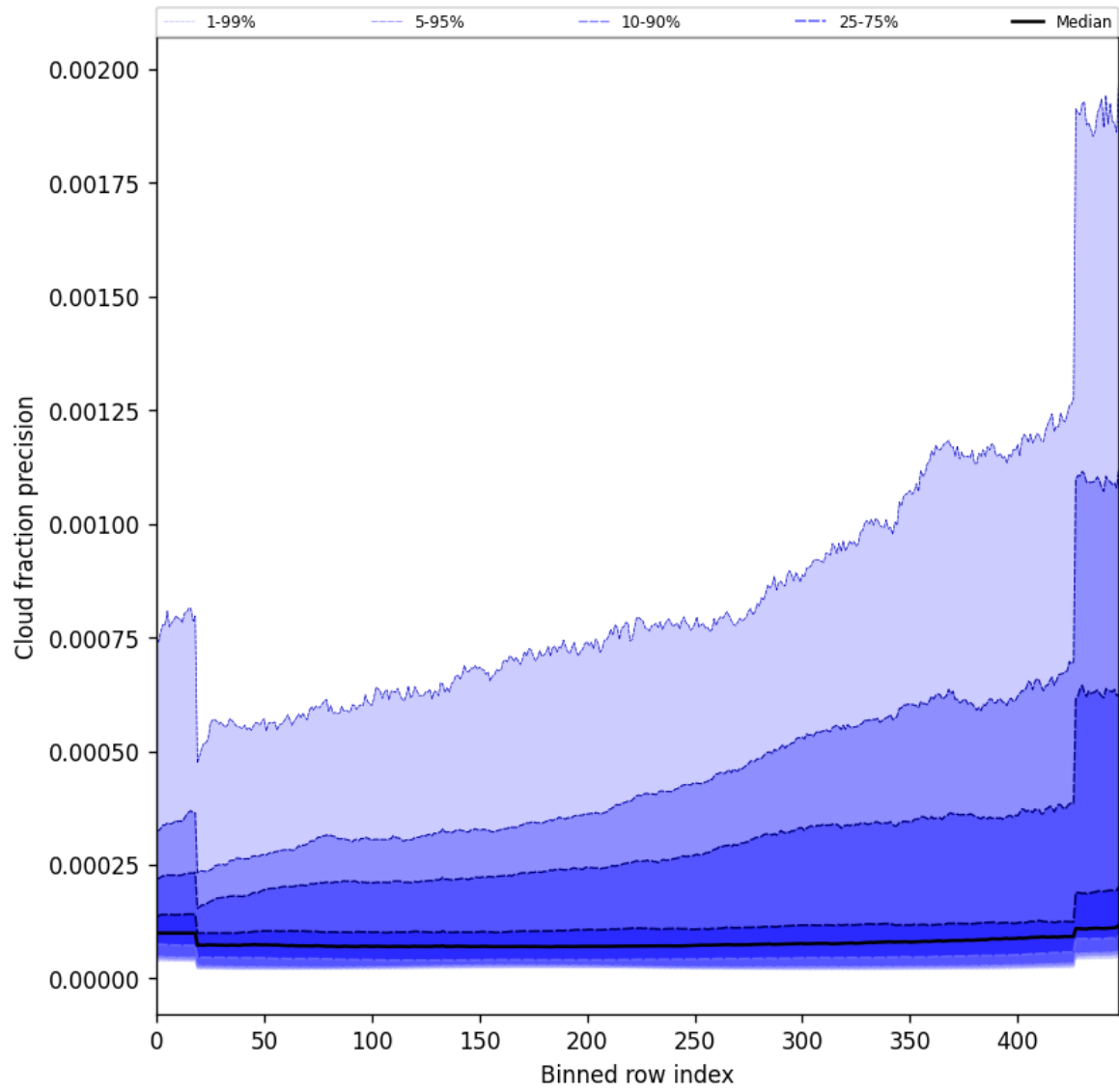
Figure 50: Along track statistics of “Cloud fraction precision” for 2025-06-22 to 2025-06-23
