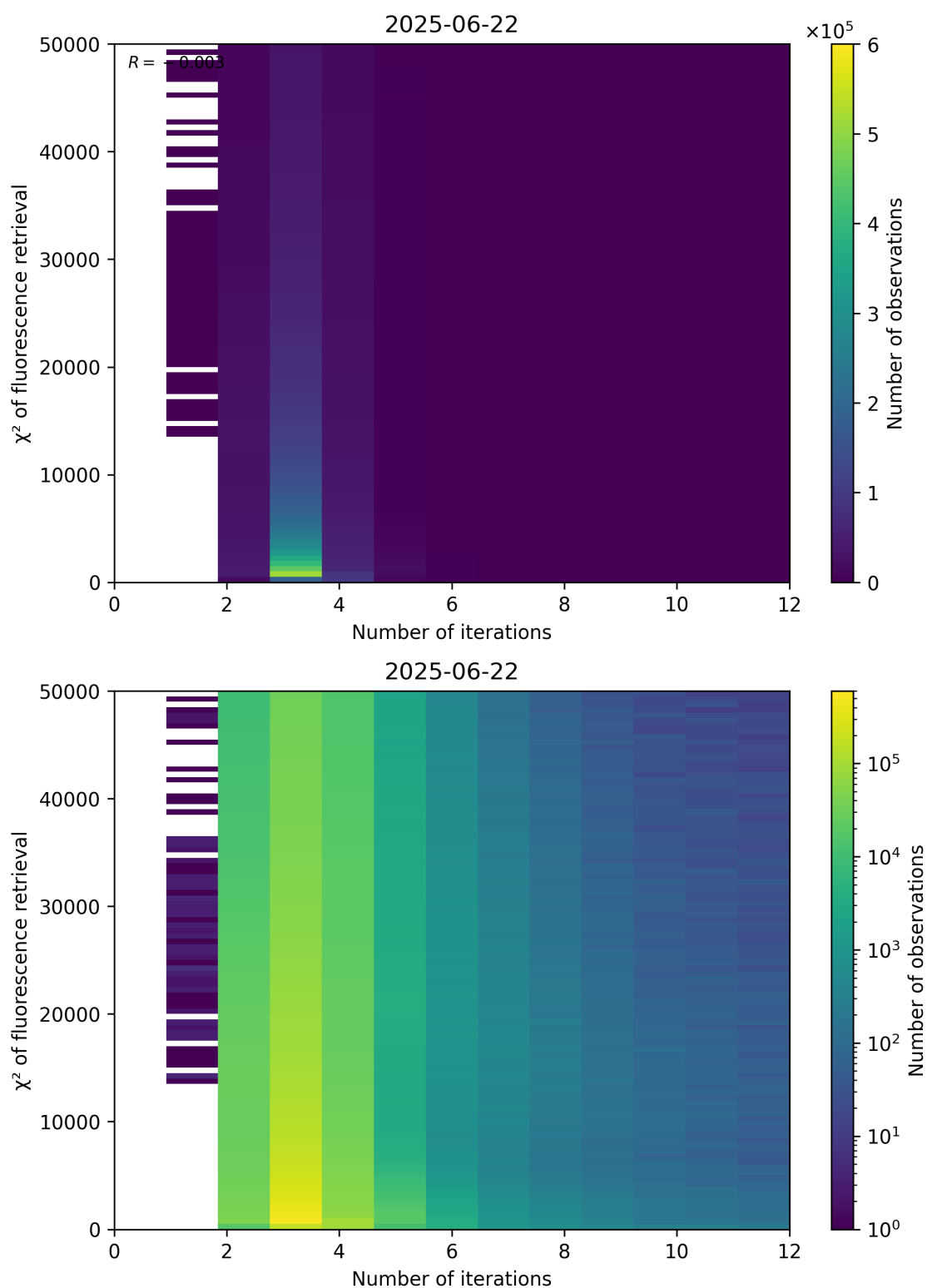
Figure 97: Scatter density plot of “Number of iterations” against “ \chi^2 of fluorescence retrieval” for 2025-06-22 to 2025-06-23.
