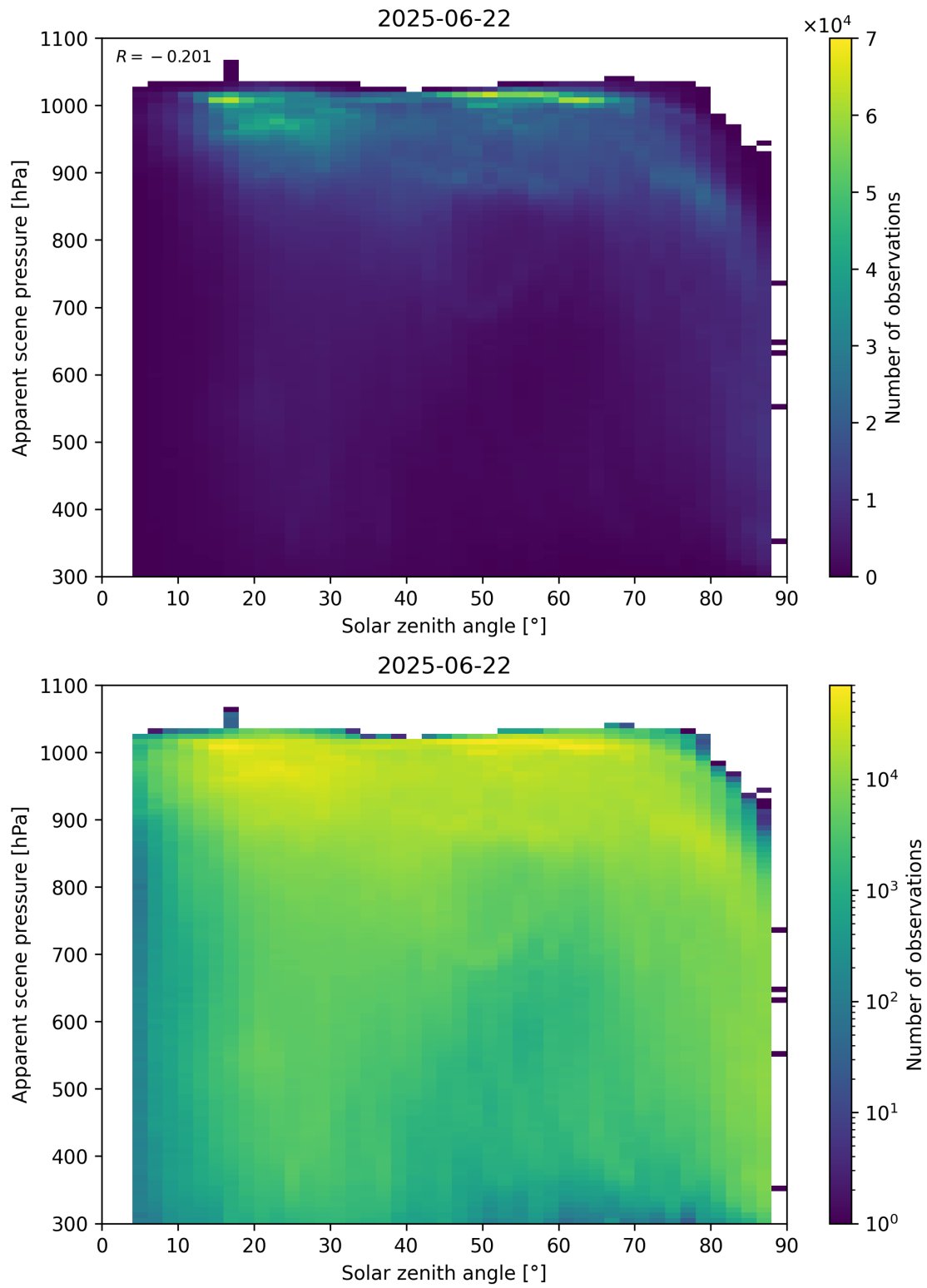
Figure 108: Scatter density plot of “Solar zenith angle” against “Apparent scene pressure” for 2025-06-22 to 2025-06-23.
