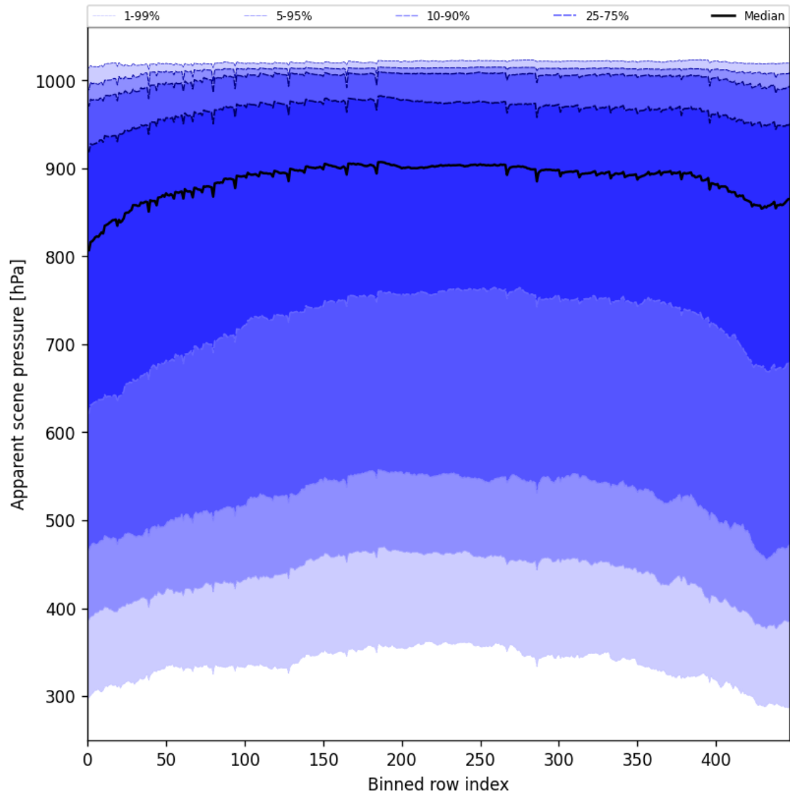
Figure 53: Along track statistics of “Apparent scene pressure” for 2025-06-22 to 2025-06-23
