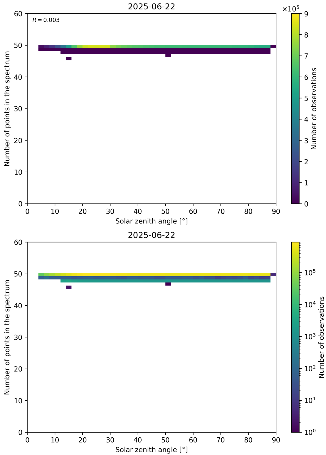
Figure 115: Scatter density plot of “Solar zenith angle” against “Number of points in the spectrum” for 2025-06-22 to 2025-06-23.
