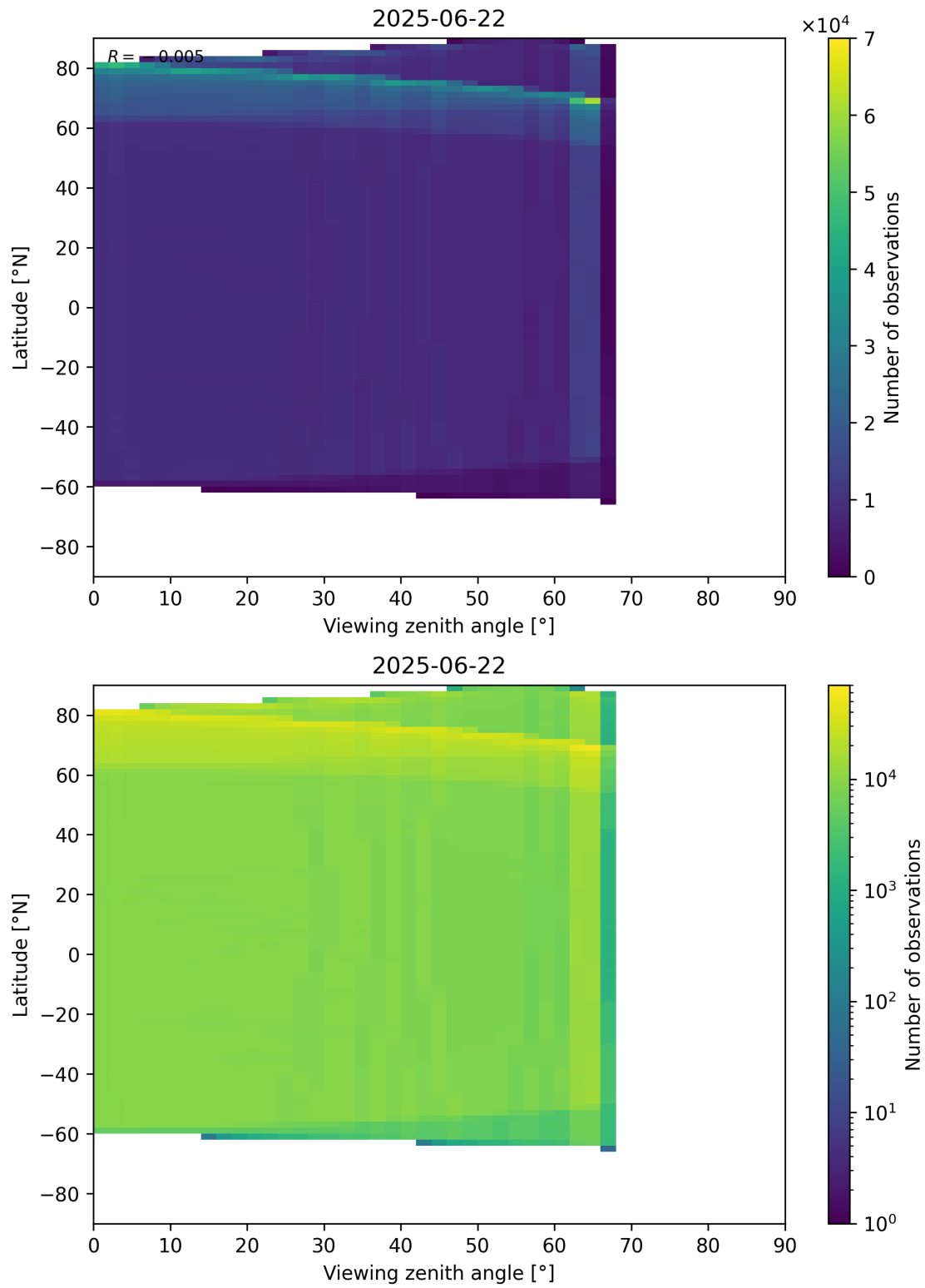
Figure 123: Scatter density plot of “Viewing zenith angle” against “Latitude” for 2025-06-22 to 2025-06-23.
