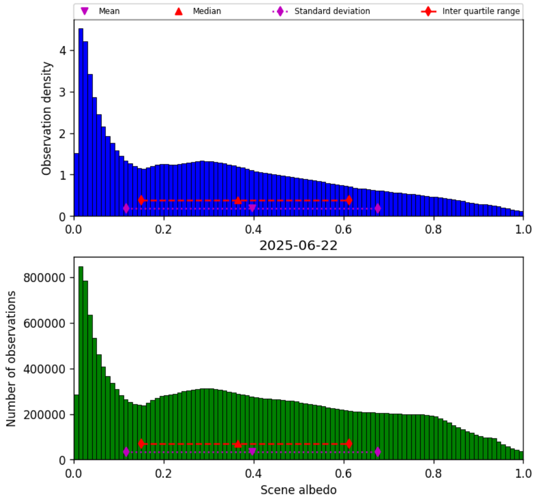
Figure 34: Histogram of “Scene albedo” for 2025-06-22 to 2025-06-23
