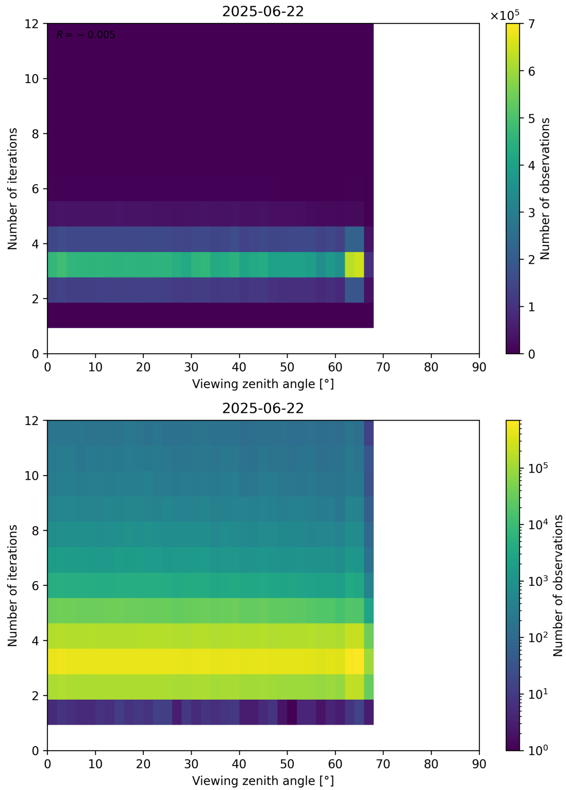
Figure 124: Scatter density plot of “Viewing zenith angle” against “Number of iterations” for 2025-06-22 to 2025-06-23.
