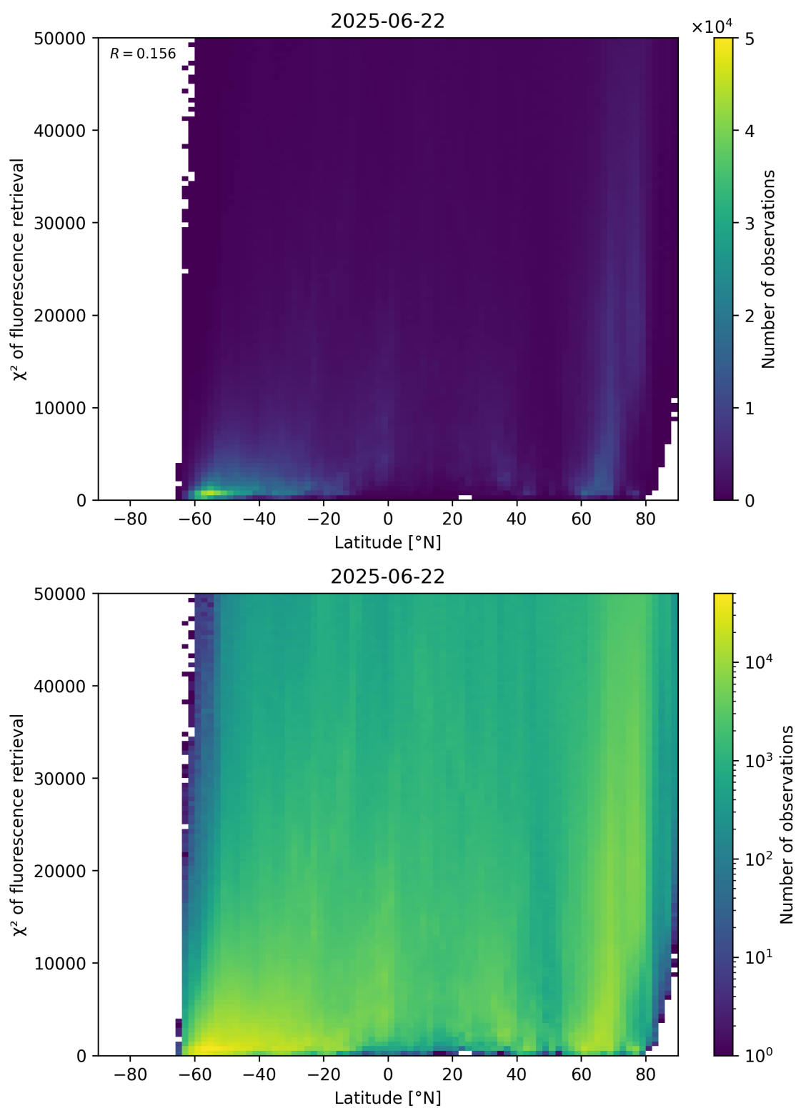
Figure 89: Scatter density plot of “Latitude” against “ \chi^2 of fluorescence retrieval” for 2025-06-22 to 2025-06-23.
