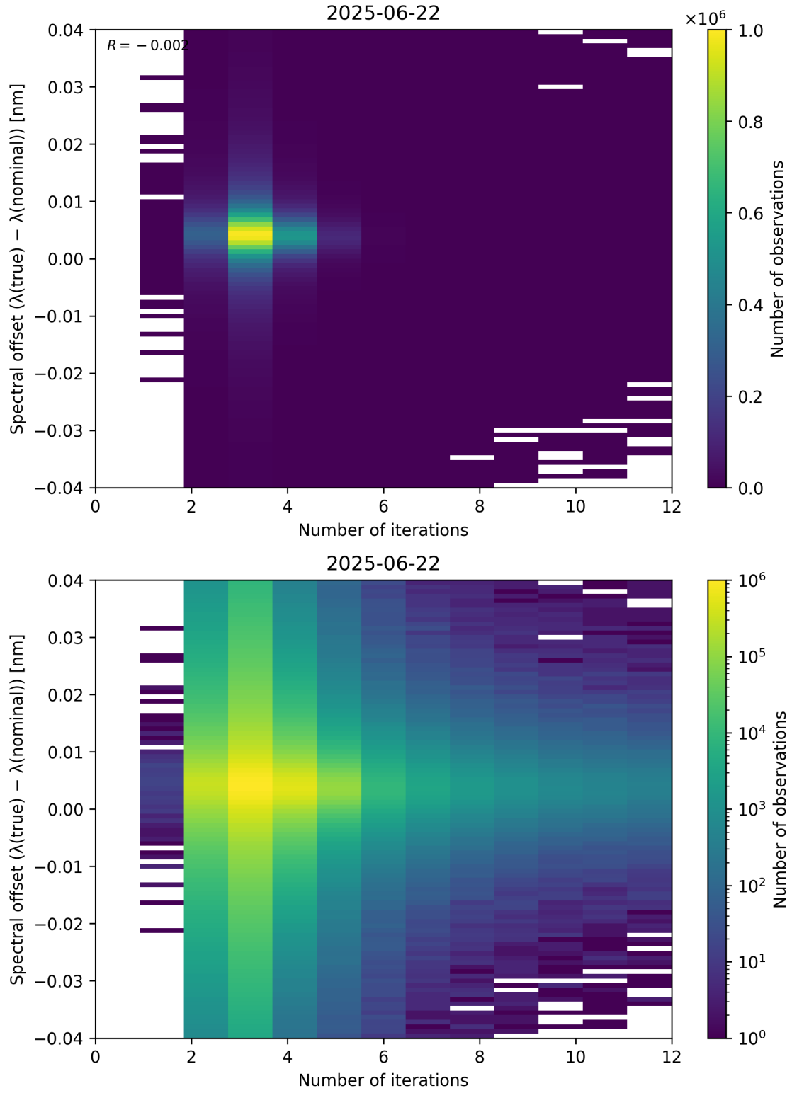
Figure 100: Scatter density plot of “Number of iterations” against “Spectral offset ( \lambda_{\text{true}} - \lambda_{\text{nominal}} )” for 2025-06-22 to 2025-06-23.
