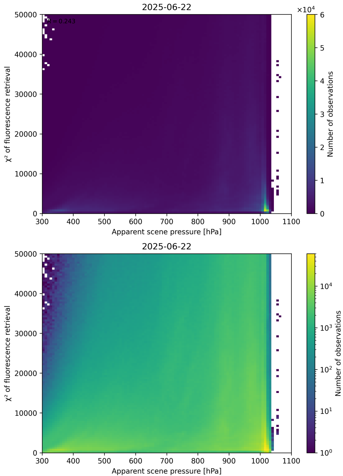
Figure 63: Scatter density plot of “Apparent scene pressure” against “ \chi^2 of fluorescence retrieval” for 2025-06-22 to 2025-06-23.
