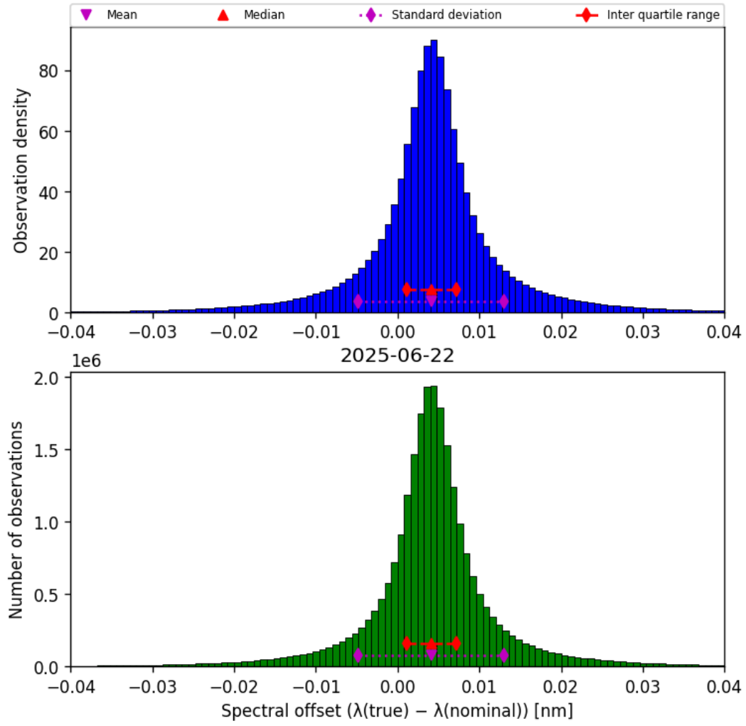
Figure 45: Histogram of “Spectral offset ( \lambda_{\text{true}} - \lambda_{\text{nominal}} )” for 2025-06-22 to 2025-06-23
