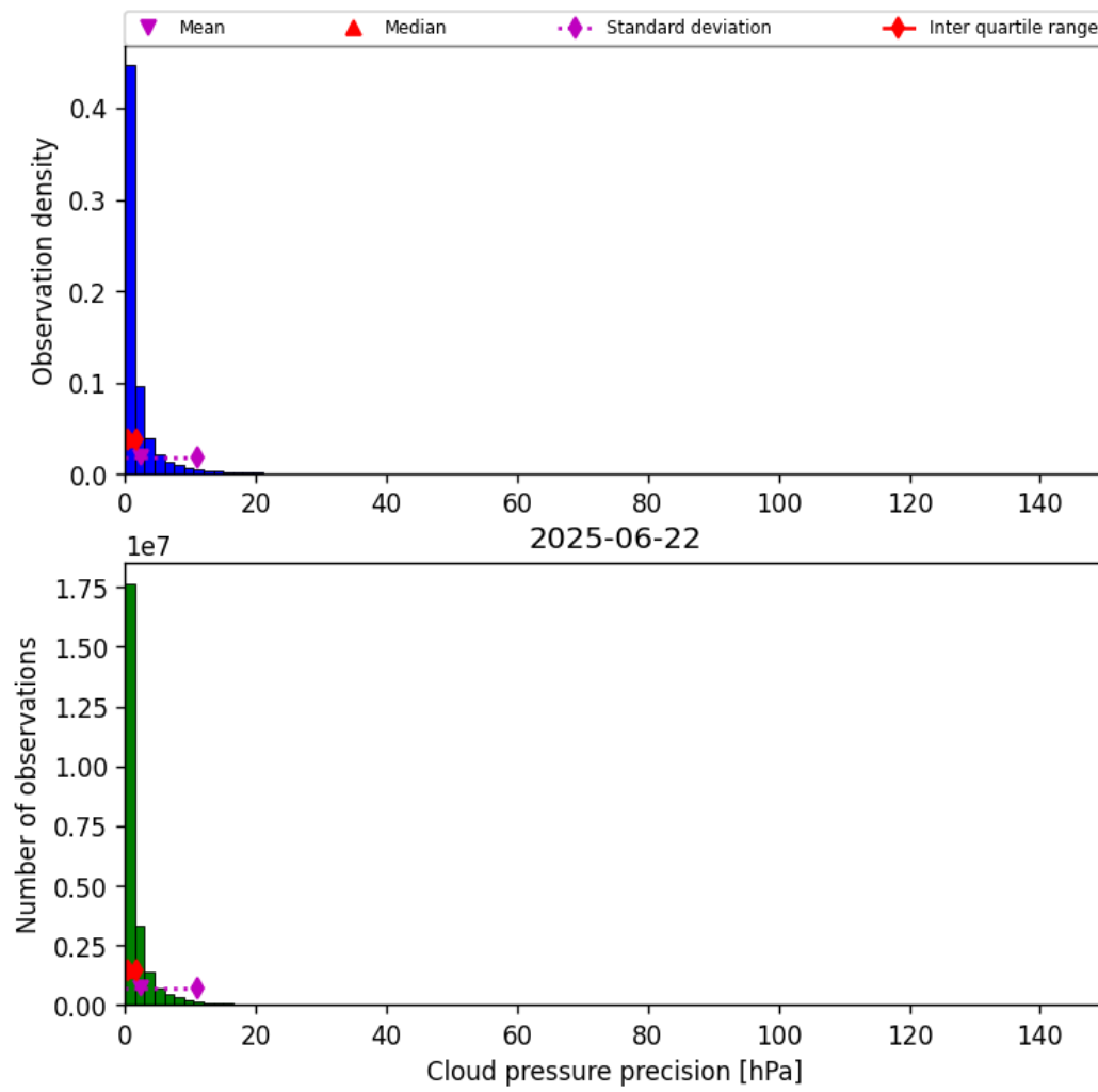
Figure 31: Histogram of “Cloud pressure precision” for 2025-06-22 to 2025-06-23
