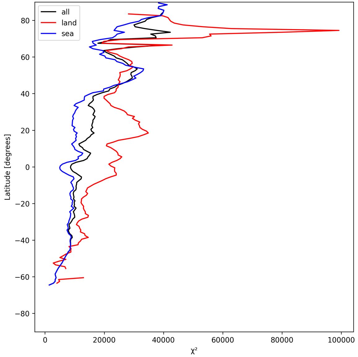
Figure 21: Zonal average of “ \chi^2 ” for 2025-06-22 to 2025-06-23.
