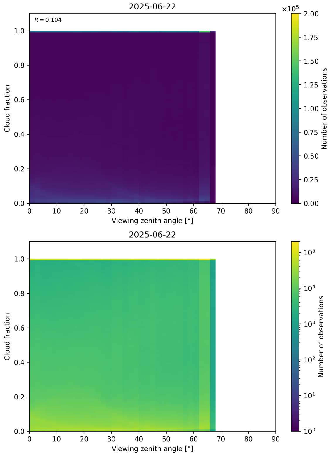
Figure 120: Scatter density plot of “Viewing zenith angle” against “Cloud fraction” for 2025-06-22 to 2025-06-23.
