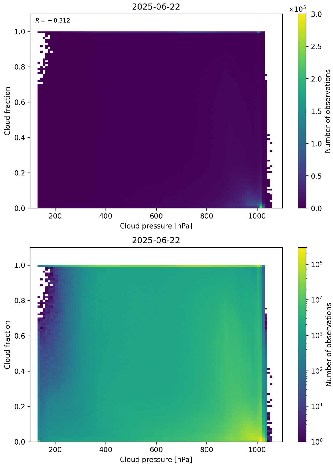
Figure 79: Scatter density plot of “Cloud pressure” against “Cloud fraction” for 2025-06-22 to 2025-06-23.
