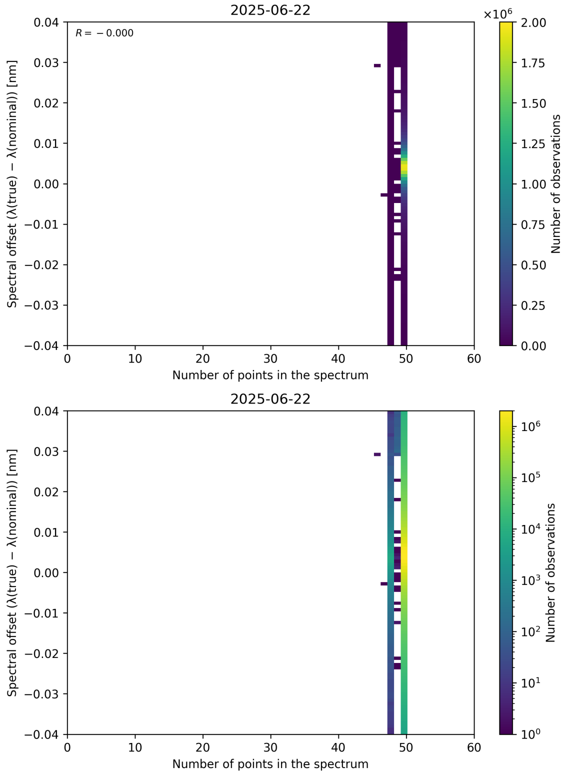
Figure 101: Scatter density plot of “Number of points in the spectrum” against “Spectral offset ( \lambda_{\text{true}} - \lambda_{\text{nominal}} )” for 2025-06-22 to 2025-06-23.
