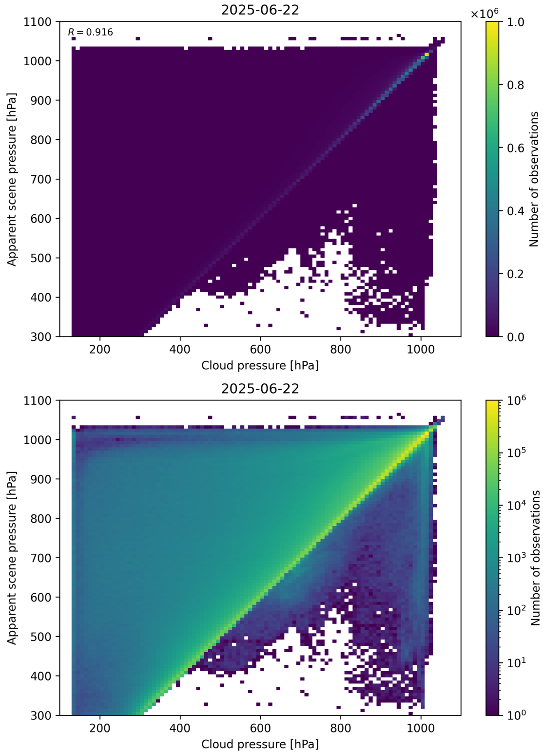
Figure 77: Scatter density plot of “Cloud pressure” against “Apparent scene pressure” for 2025-06-22 to 2025-06-23.
