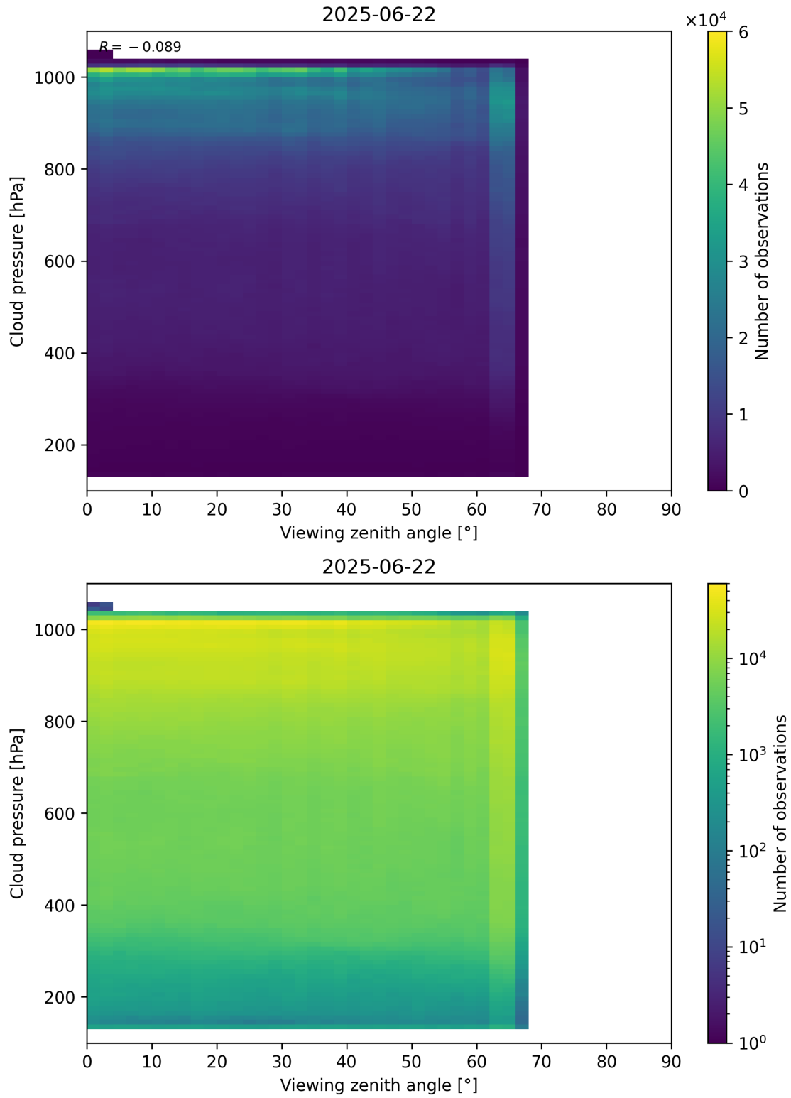
Figure 121: Scatter density plot of “Viewing zenith angle” against “Cloud pressure” for 2025-06-22 to 2025-06-23.
