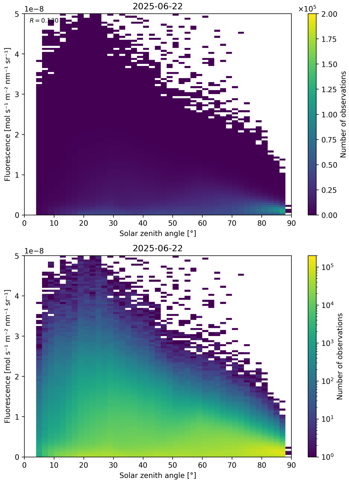
Figure 112: Scatter density plot of “Solar zenith angle” against “Fluorescence” for 2025-06-22 to 2025-06-23.
