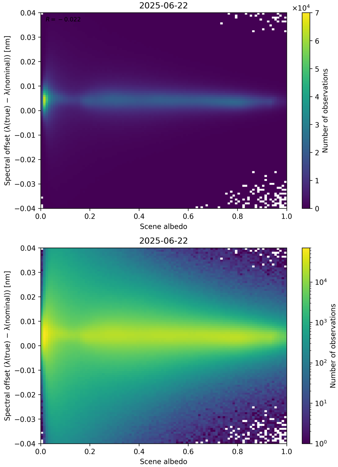
Figure 107: Scatter density plot of “Scene albedo” against “Spectral offset ( \lambda_{\text{true}} - \lambda_{\text{nominal}} )” for 2025-06-22 to 2025-06-23.
