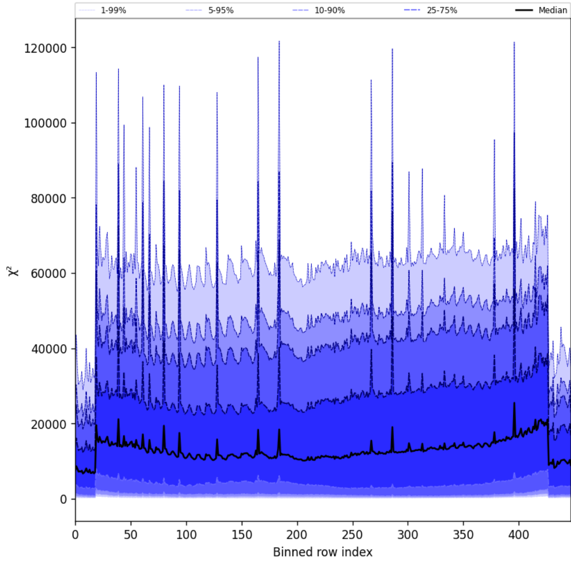
Figure 55: Along track statistics of “ \chi^2 ” for 2025-06-22 to 2025-06-23
