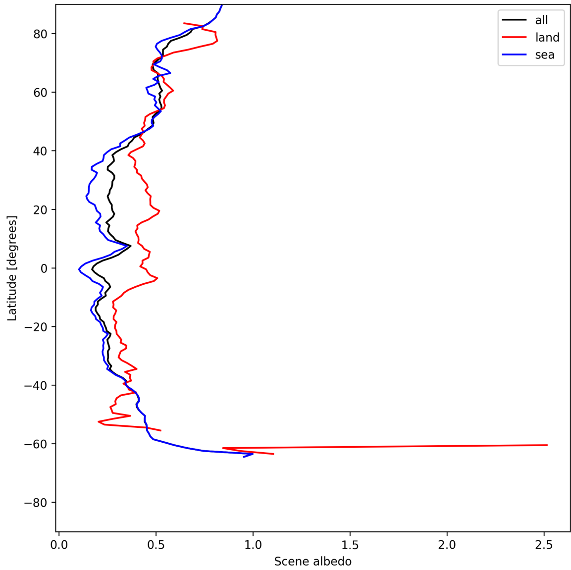
Figure 17: Zonal average of “Scene albedo” for 2025-06-22 to 2025-06-23.
