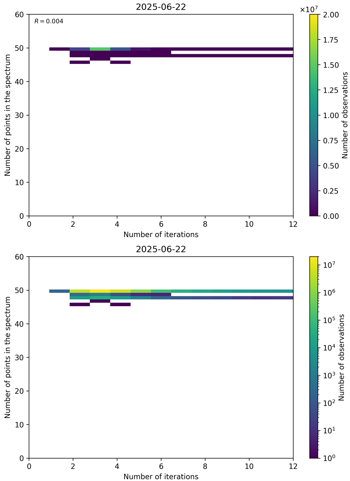
Figure 99: Scatter density plot of “Number of iterations” against “Number of points in the spectrum” for 2025-06-22 to 2025-06-23.
