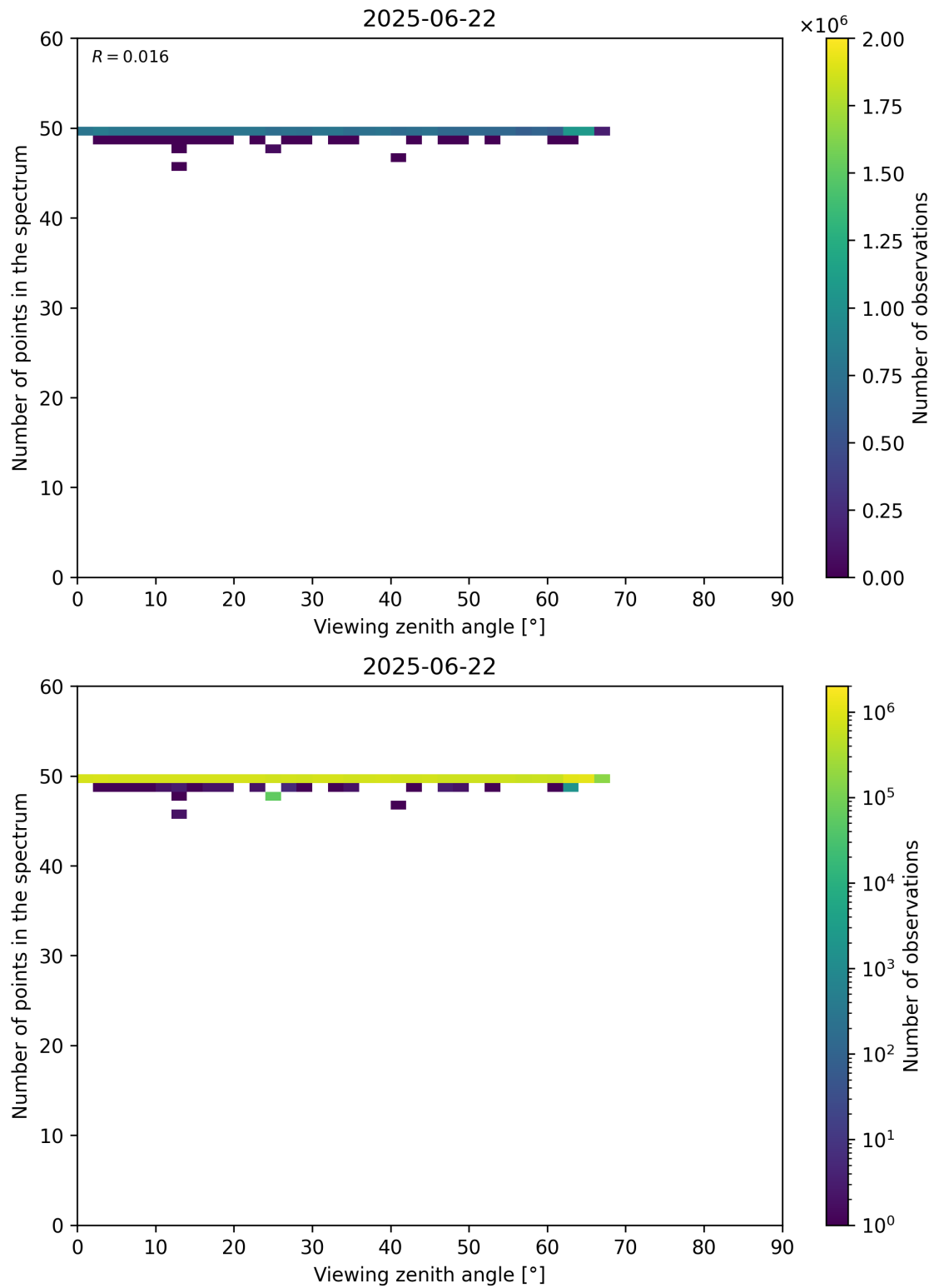
Figure 125: Scatter density plot of “Viewing zenith angle” against “Number of points in the spectrum” for 2025-06-22 to 2025-06-23.
