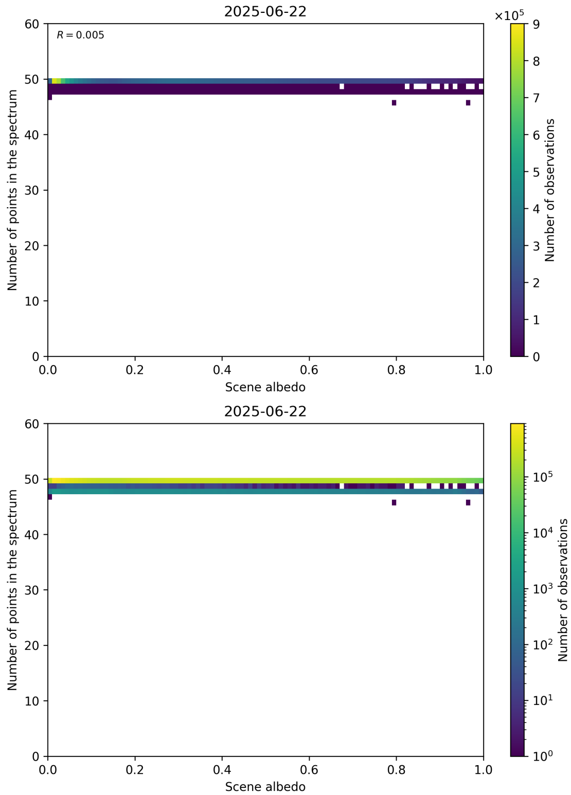
Figure 106: Scatter density plot of “Scene albedo” against “Number of points in the spectrum” for 2025-06-22 to 2025-06-23.
