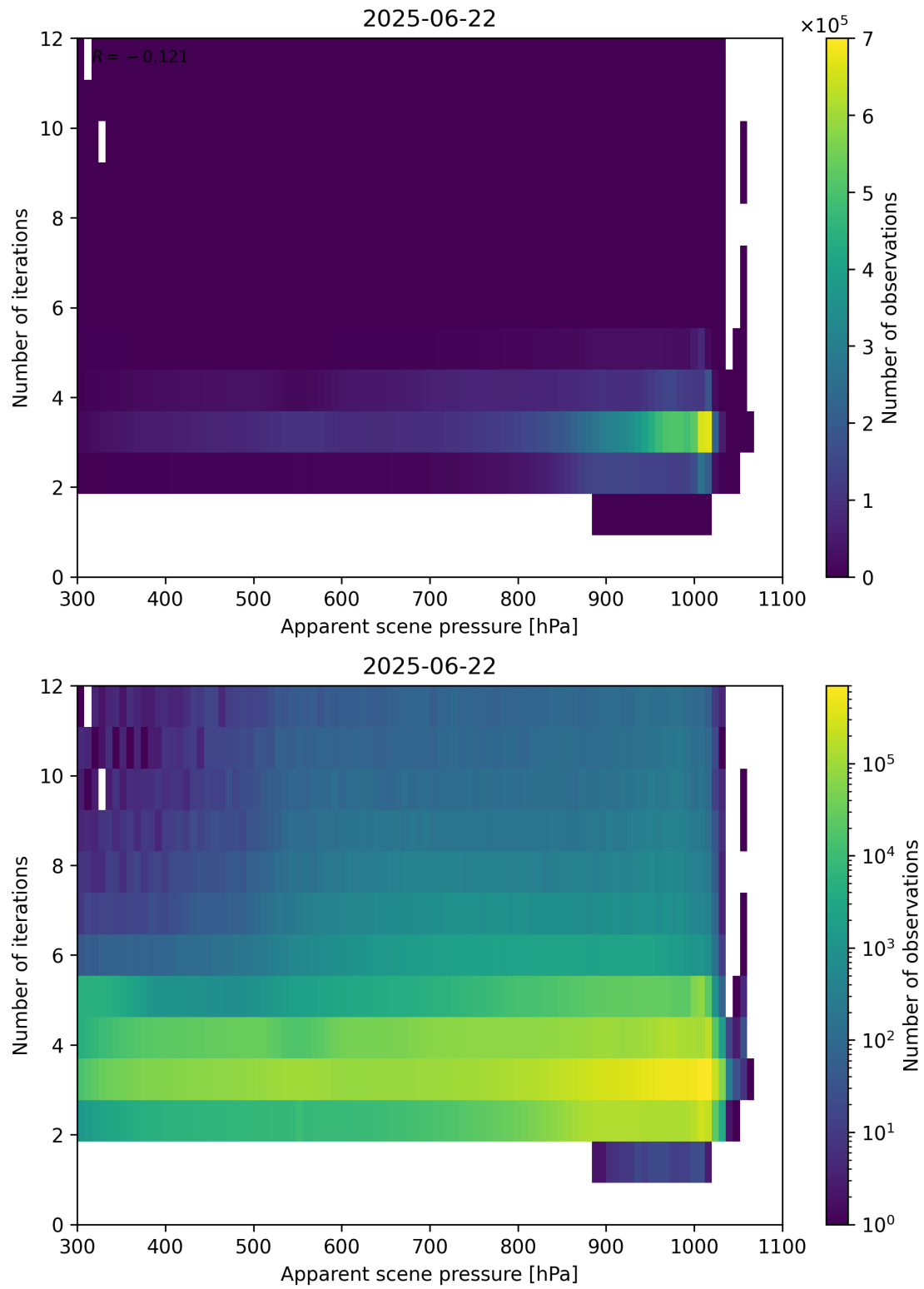
Figure 65: Scatter density plot of “Apparent scene pressure” against “Number of iterations” for 2025-06-22 to 2025-06-23.
