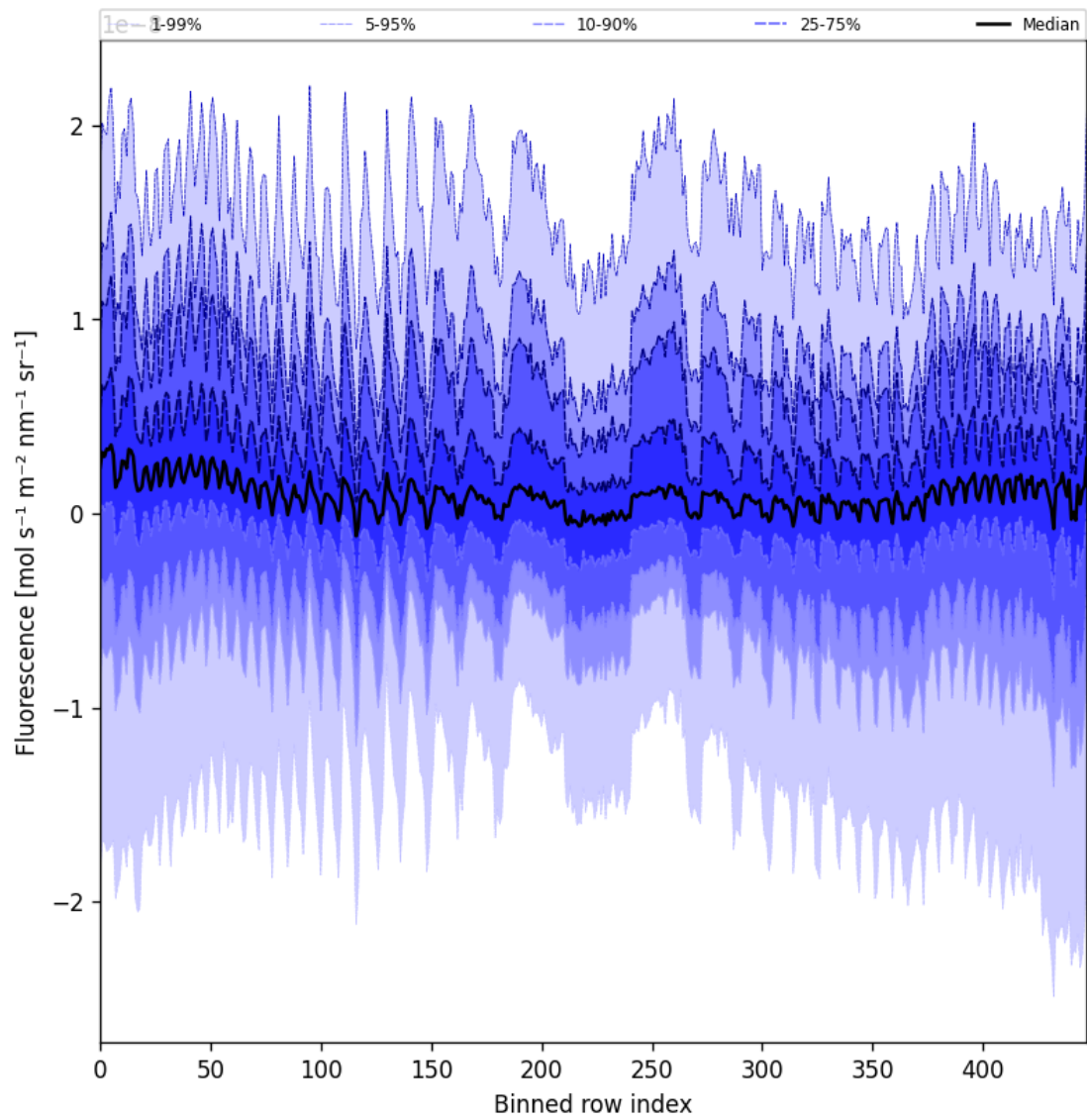
Figure 57: Along track statistics of “Fluorescence” for 2025-06-22 to 2025-06-23
