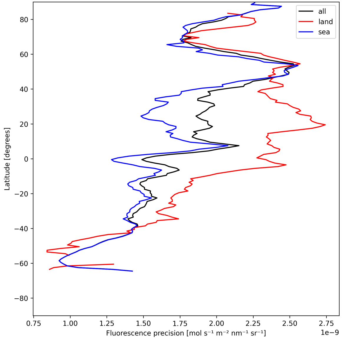
Figure 24: Zonal average of “Fluorescence precision” for 2025-06-22 to 2025-06-23.
