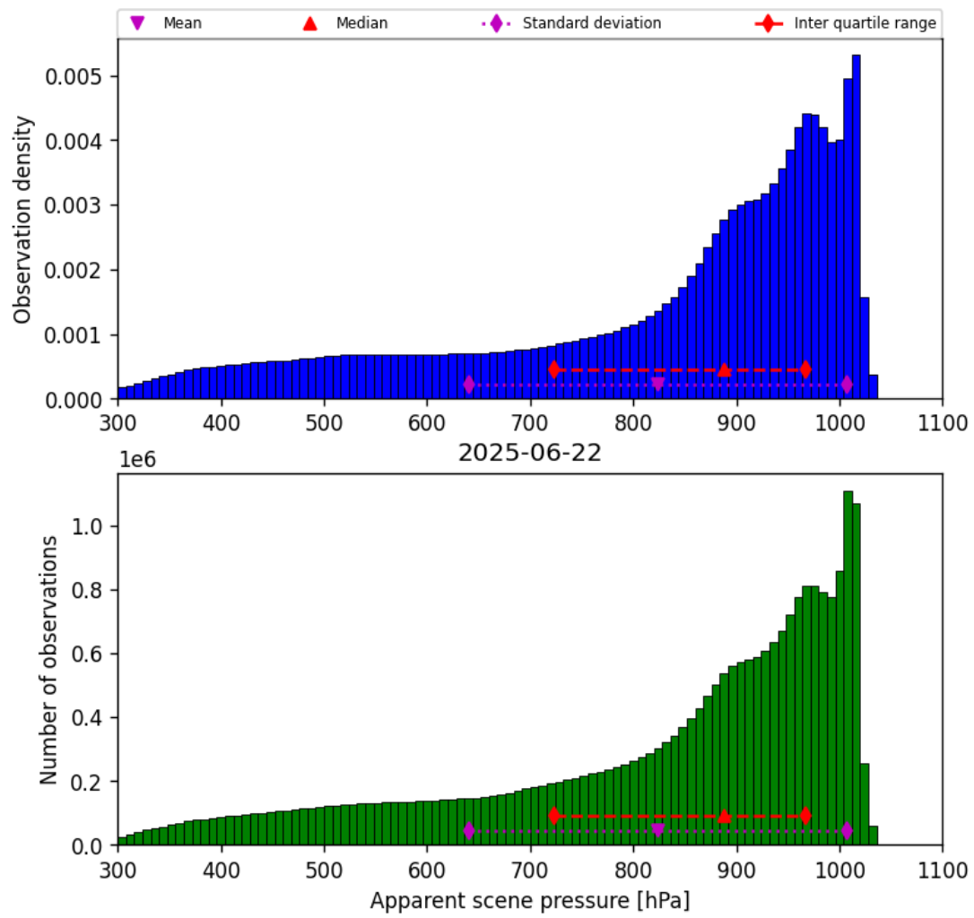
Figure 36: Histogram of “Apparent scene pressure” for 2025-06-22 to 2025-06-23
