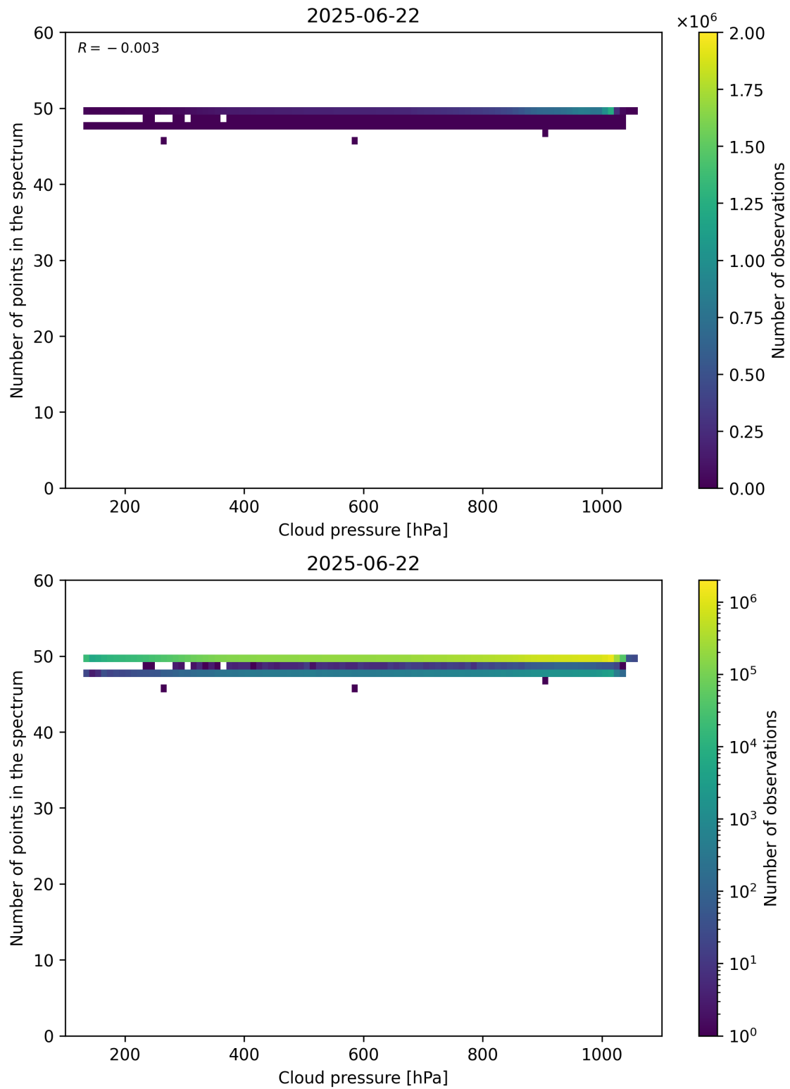
Figure 82: Scatter density plot of “Cloud pressure” against “Number of points in the spectrum” for 2025-06-22 to 2025-06-23.
