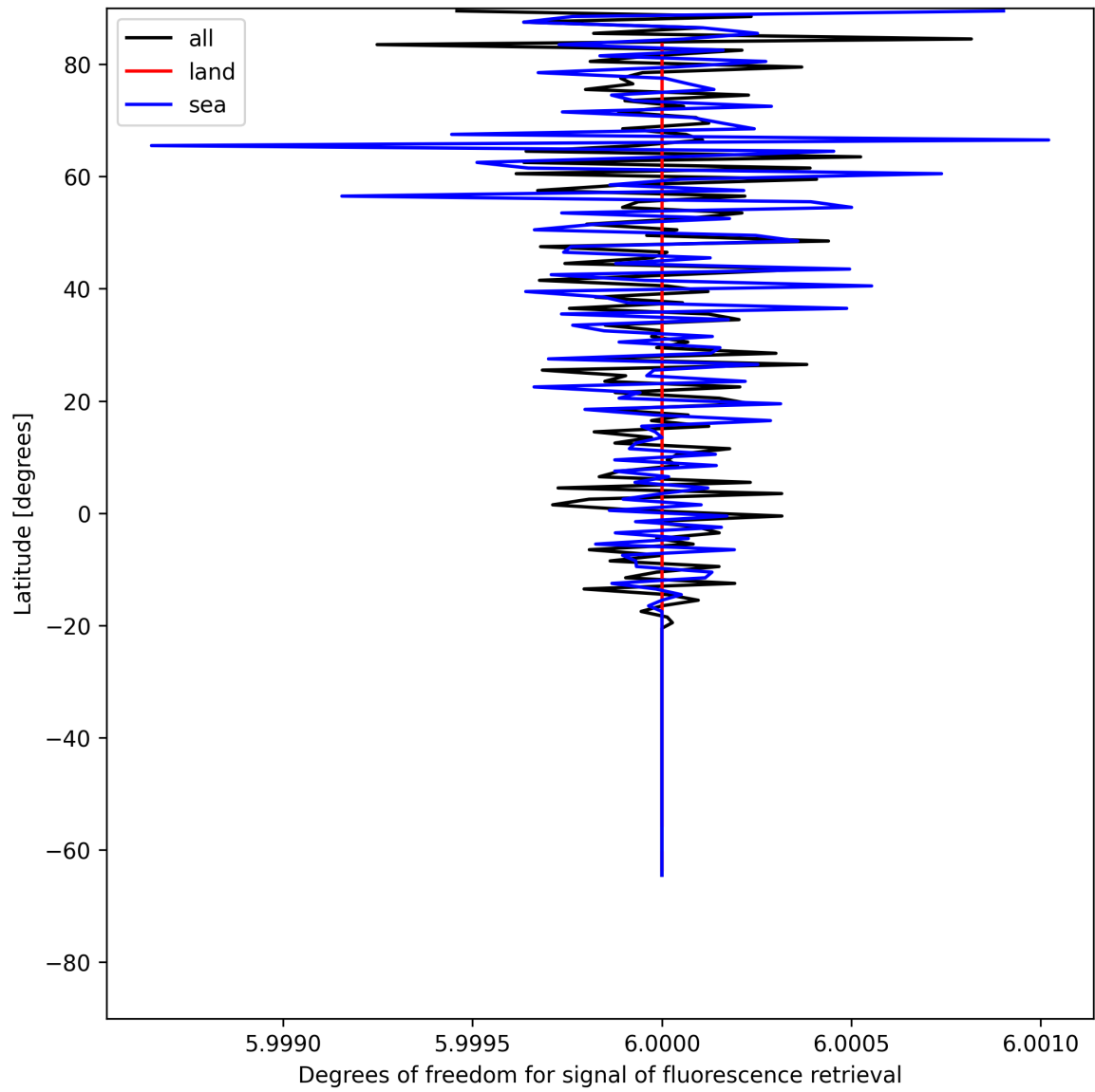
Figure 26: Zonal average of “Degrees of freedom for signal of fluorescence retrieval” for 2025-06-22 to 2025-06-23.
