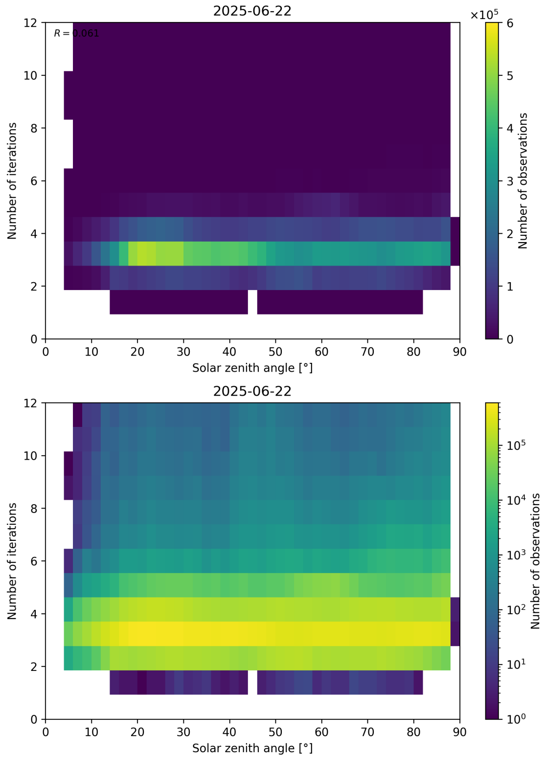
Figure 114: Scatter density plot of “Solar zenith angle” against “Number of iterations” for 2025-06-22 to 2025-06-23.
