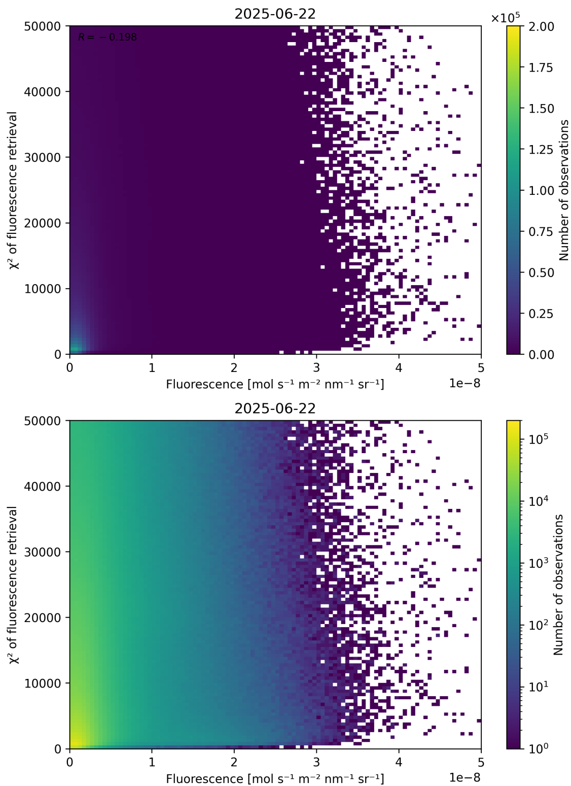
Figure 85: Scatter density plot of “Fluorescence” against “ \chi^2 of fluorescence retrieval” for 2025-06-22 to 2025-06-23.
