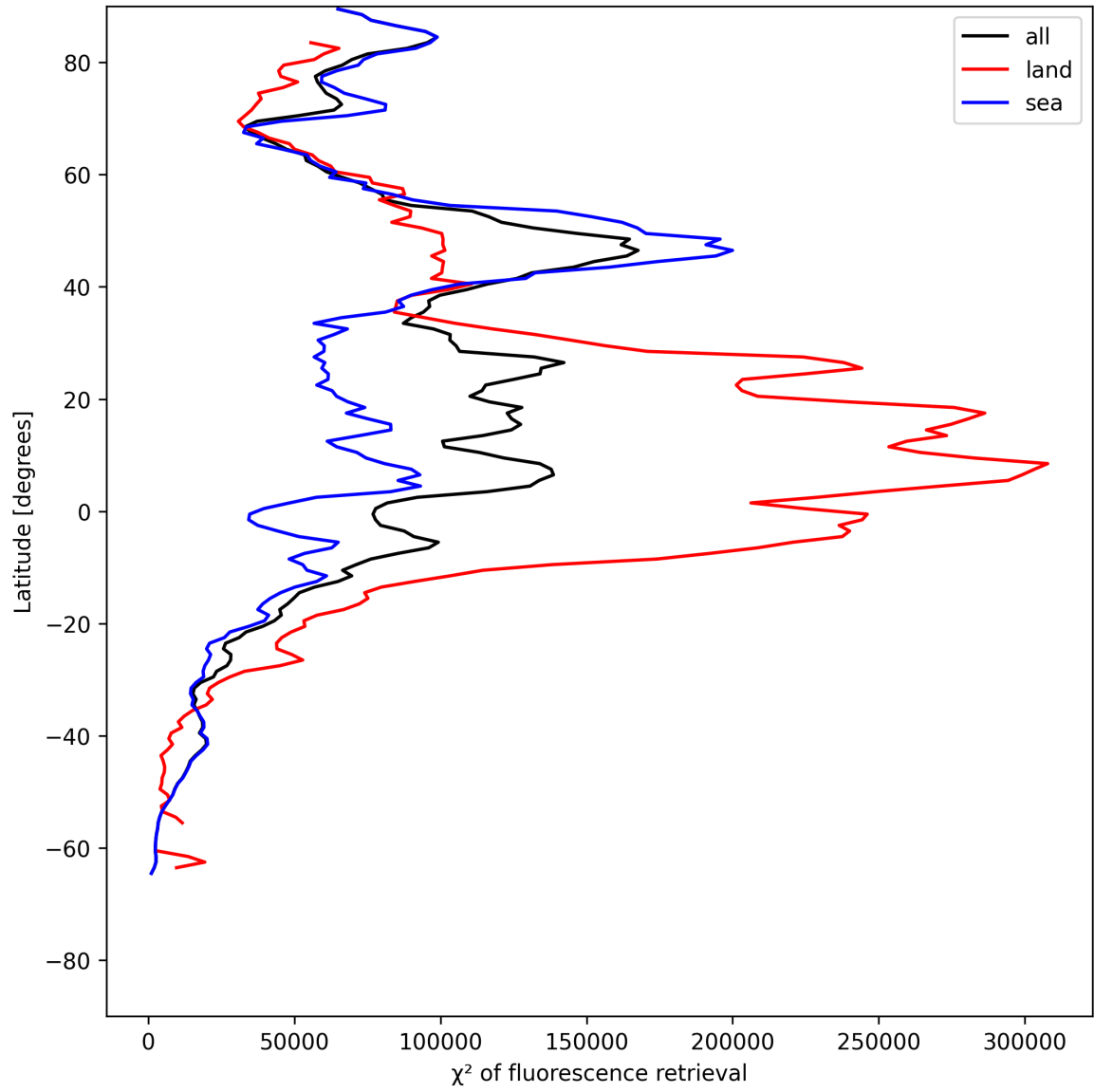
Figure 25: Zonal average of “ \chi^2 of fluorescence retrieval” for 2025-06-22 to 2025-06-23.
