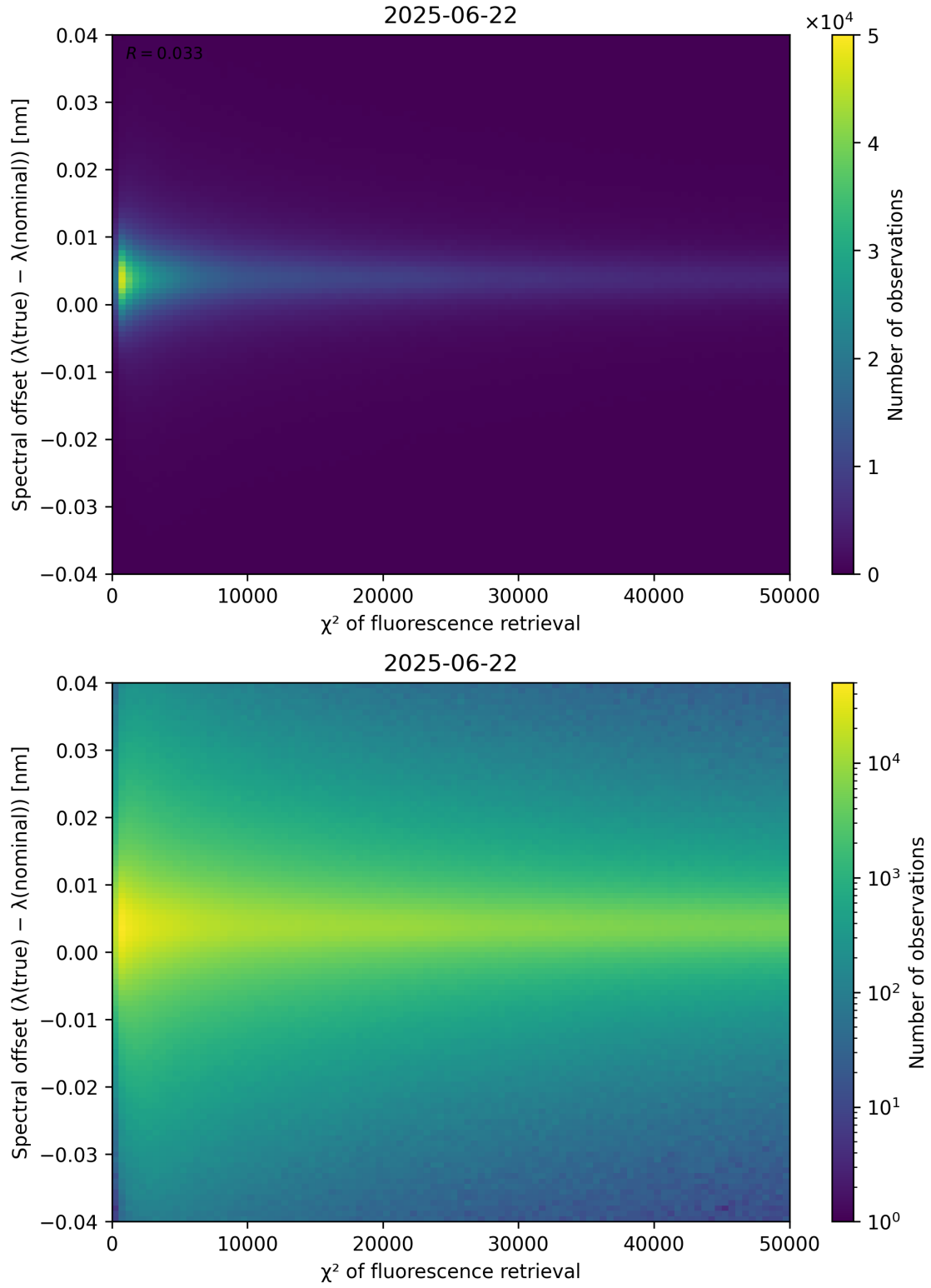
Figure 69: Scatter density plot of “ \chi^2 of fluorescence retrieval” against “Spectral offset ( \lambda_{\text{true}} - \lambda_{\text{nominal}} )” for 2025-06-22 to 2025-06-23.
