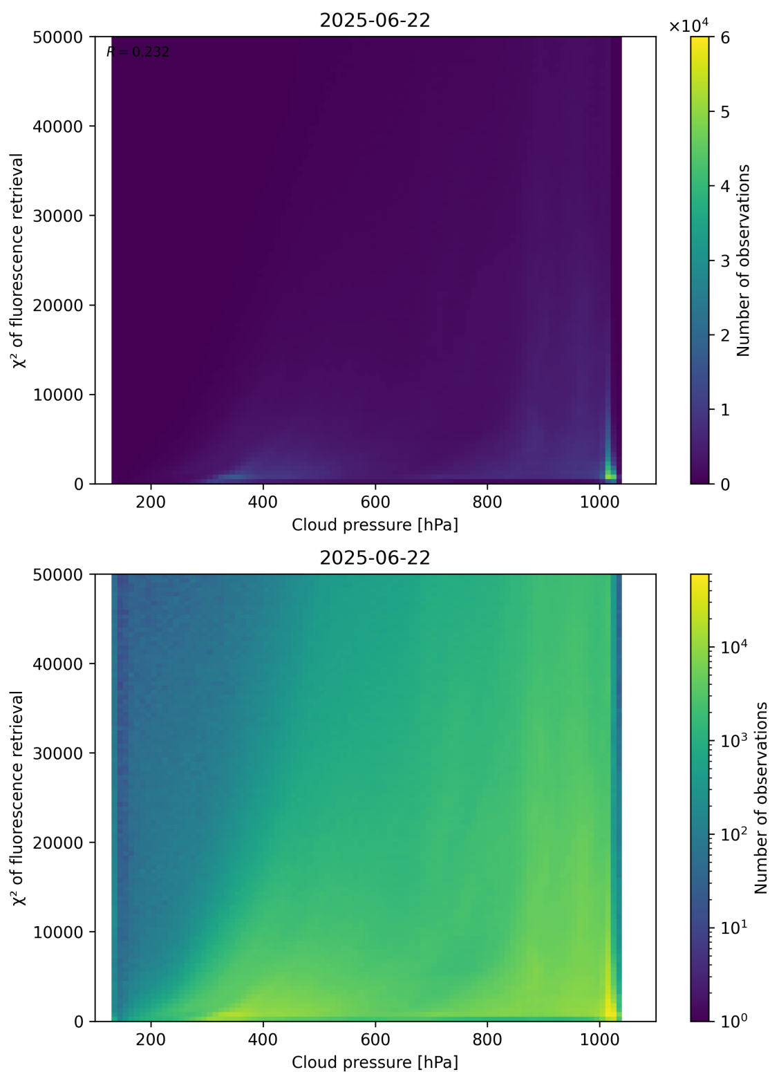
Figure 78: Scatter density plot of “Cloud pressure” against “ \chi^2 of fluorescence retrieval” for 2025-06-22 to 2025-06-23.
