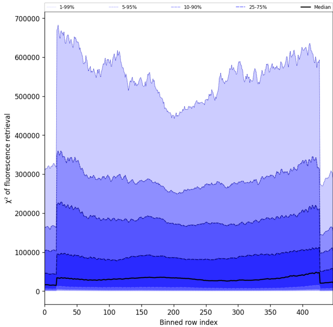
Figure 59: Along track statistics of “ \chi^2 of fluorescence retrieval” for 2025-06-22 to 2025-06-23
