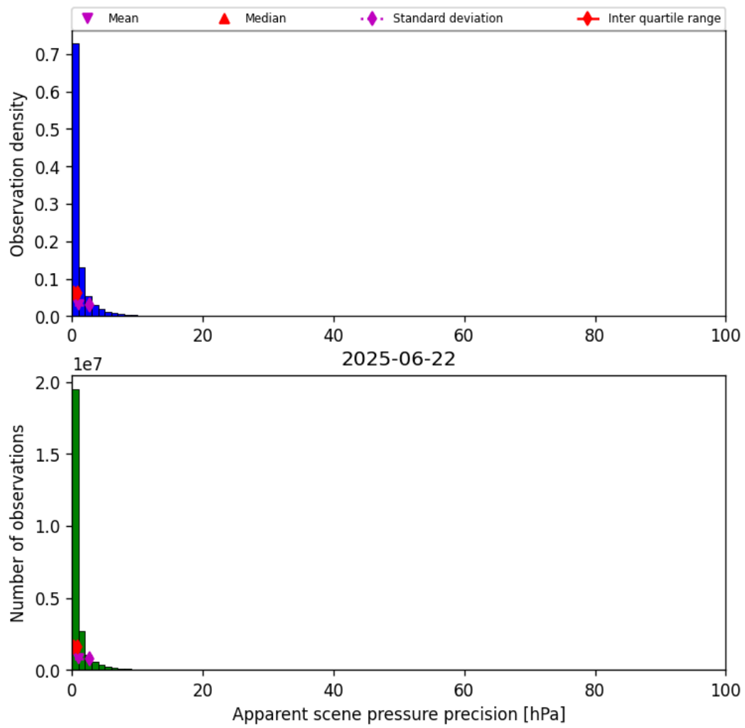
Figure 37: Histogram of “Apparent scene pressure precision” for 2025-06-22 to 2025-06-23
