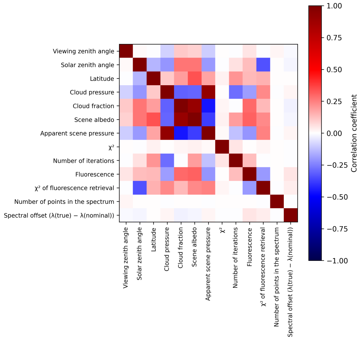
Figure 2: Map of correlation matrix for 2025-06-22 to 2025-06-23.
