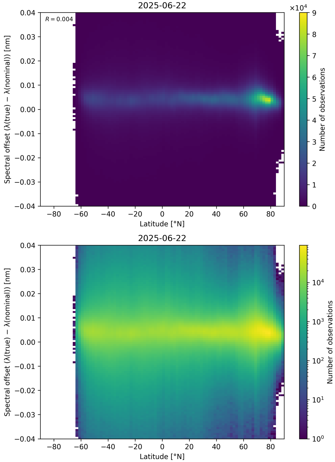
Figure 96: Scatter density plot of “Latitude” against “Spectral offset ( \lambda_{\text{true}} - \lambda_{\text{nominal}} )” for 2025-06-22 to 2025-06-23.
