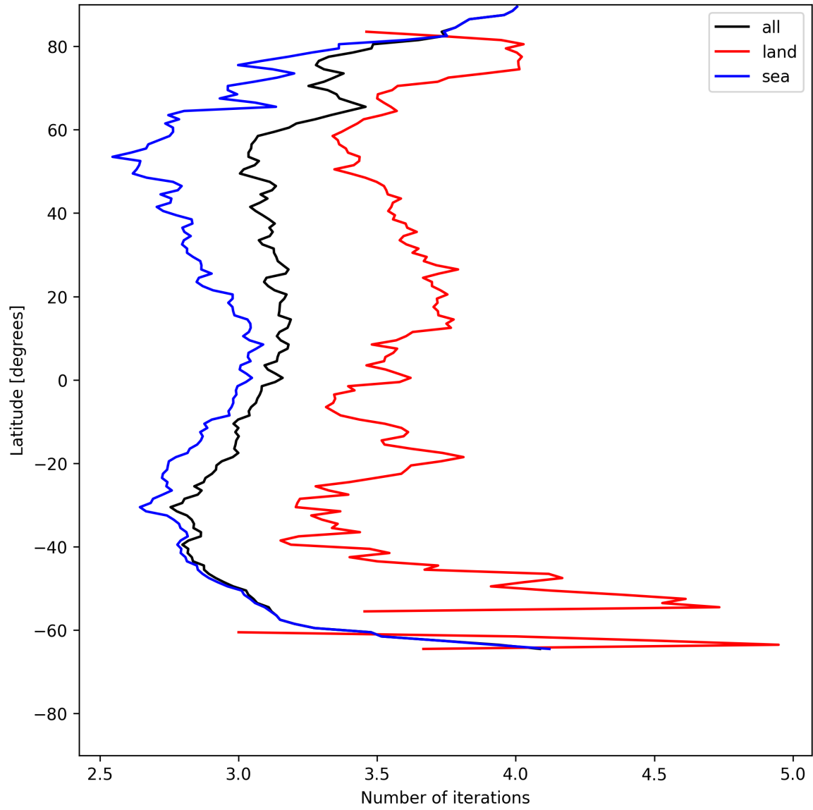
Figure 22: Zonal average of “Number of iterations” for 2025-06-22 to 2025-06-24.
