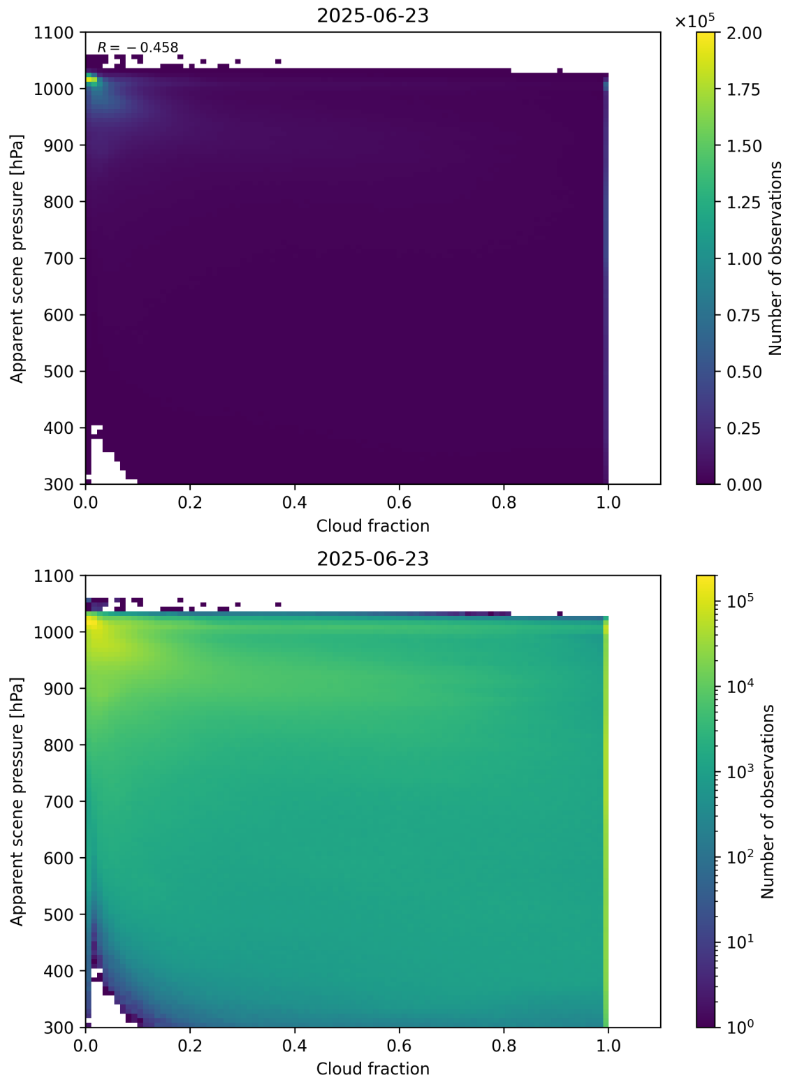
Figure 70: Scatter density plot of “Cloud fraction” against “Apparent scene pressure” for 2025-06-22 to 2025-06-24.
