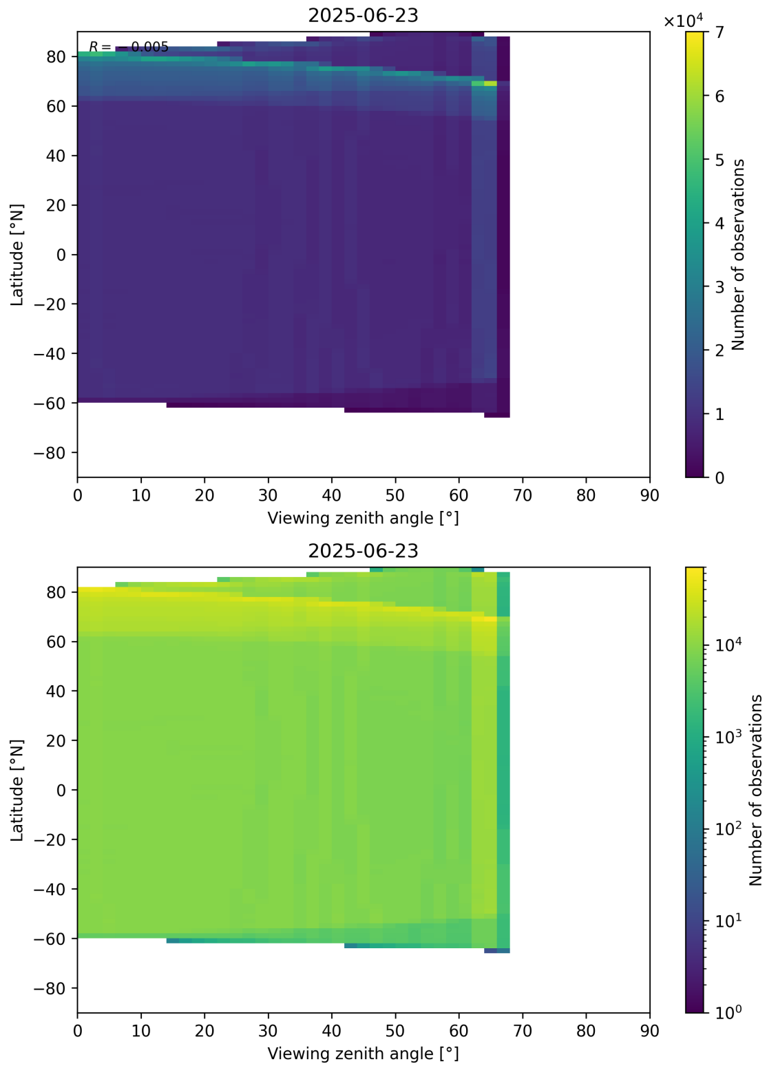
Figure 123: Scatter density plot of “Viewing zenith angle” against “Latitude” for 2025-06-22 to 2025-06-24.
