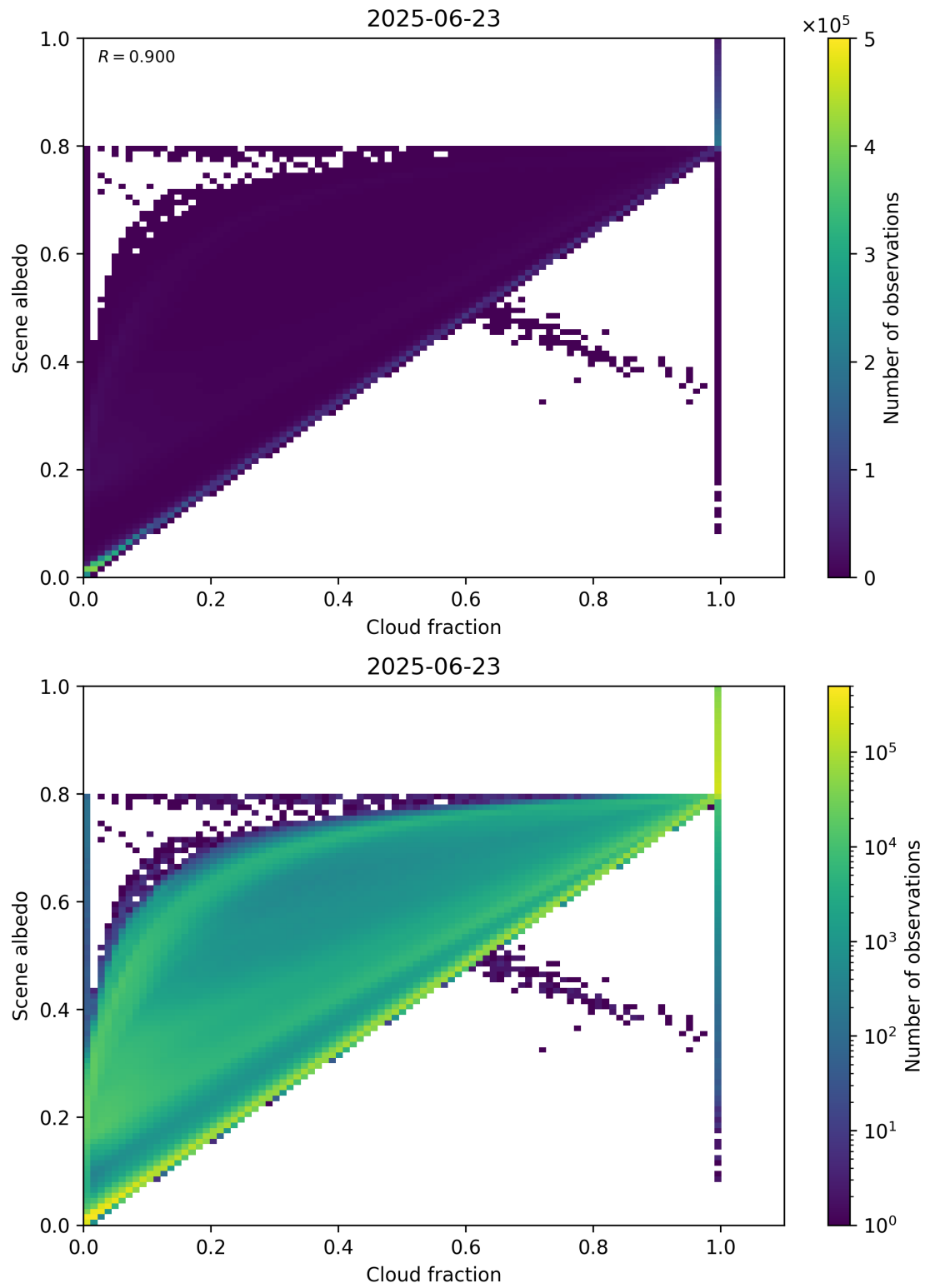
Figure 75: Scatter density plot of “Cloud fraction” against “Scene albedo” for 2025-06-22 to 2025-06-24.
