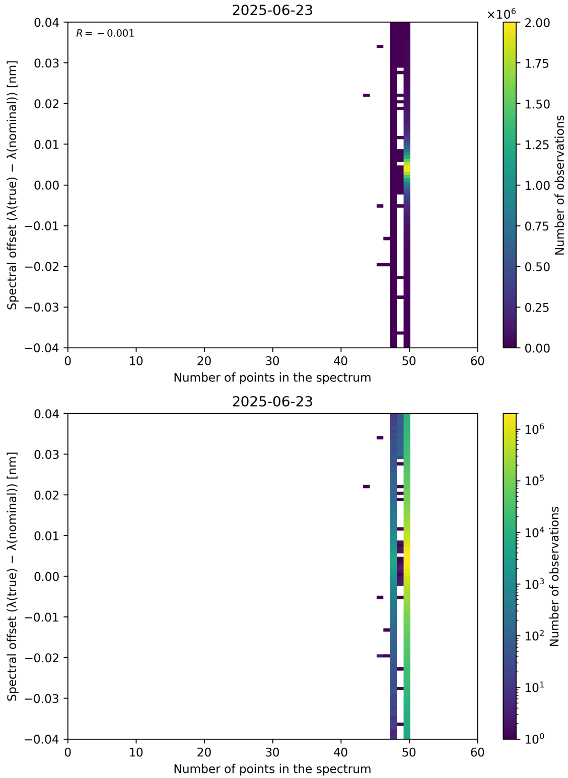
Figure 101: Scatter density plot of “Number of points in the spectrum” against “Spectral offset ( \lambda_{\text{true}} - \lambda_{\text{nominal}} )” for 2025-06-22 to 2025-06-24.
