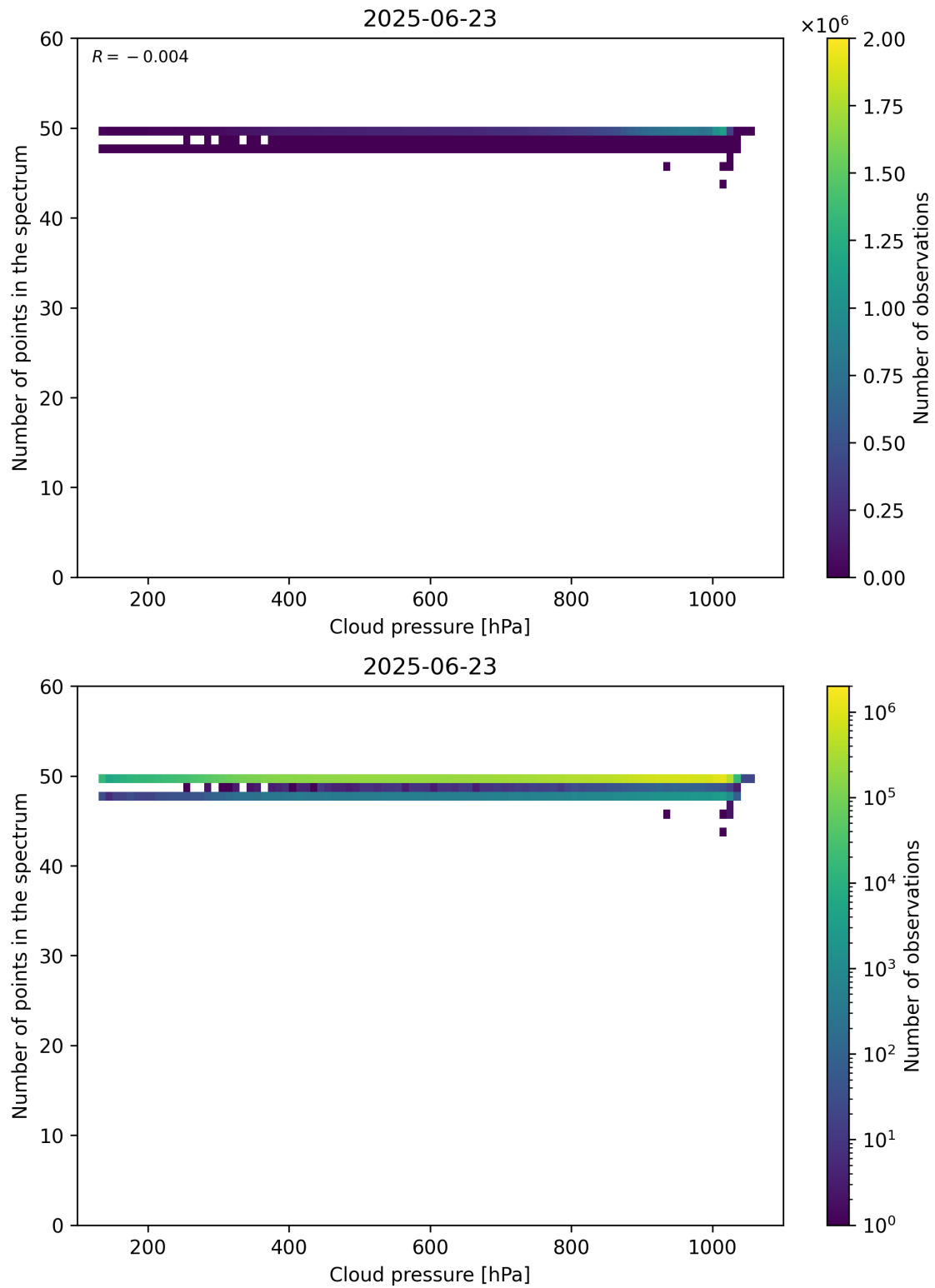
Figure 82: Scatter density plot of “Cloud pressure” against “Number of points in the spectrum” for 2025-06-22 to 2025-06-24.
