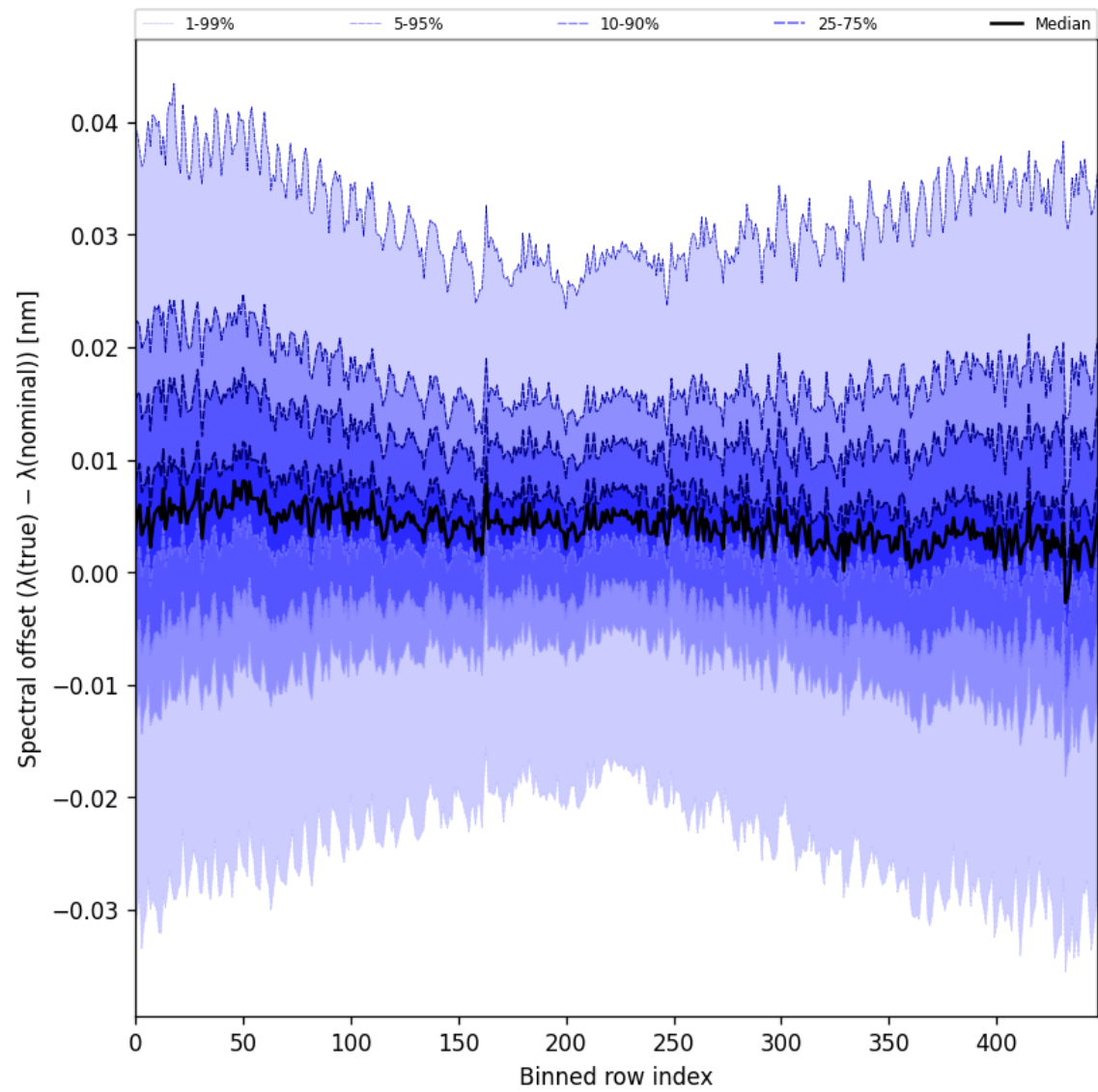
Figure 62: Along track statistics of “Spectral offset ( \lambda_{\text{true}} - \lambda_{\text{nominal}} )” for 2025-06-22 to 2025-06-24
