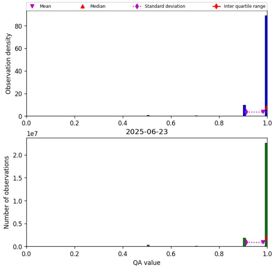
Figure 29: Histogram of “QA value” for 2025-06-22 to 2025-06-24
