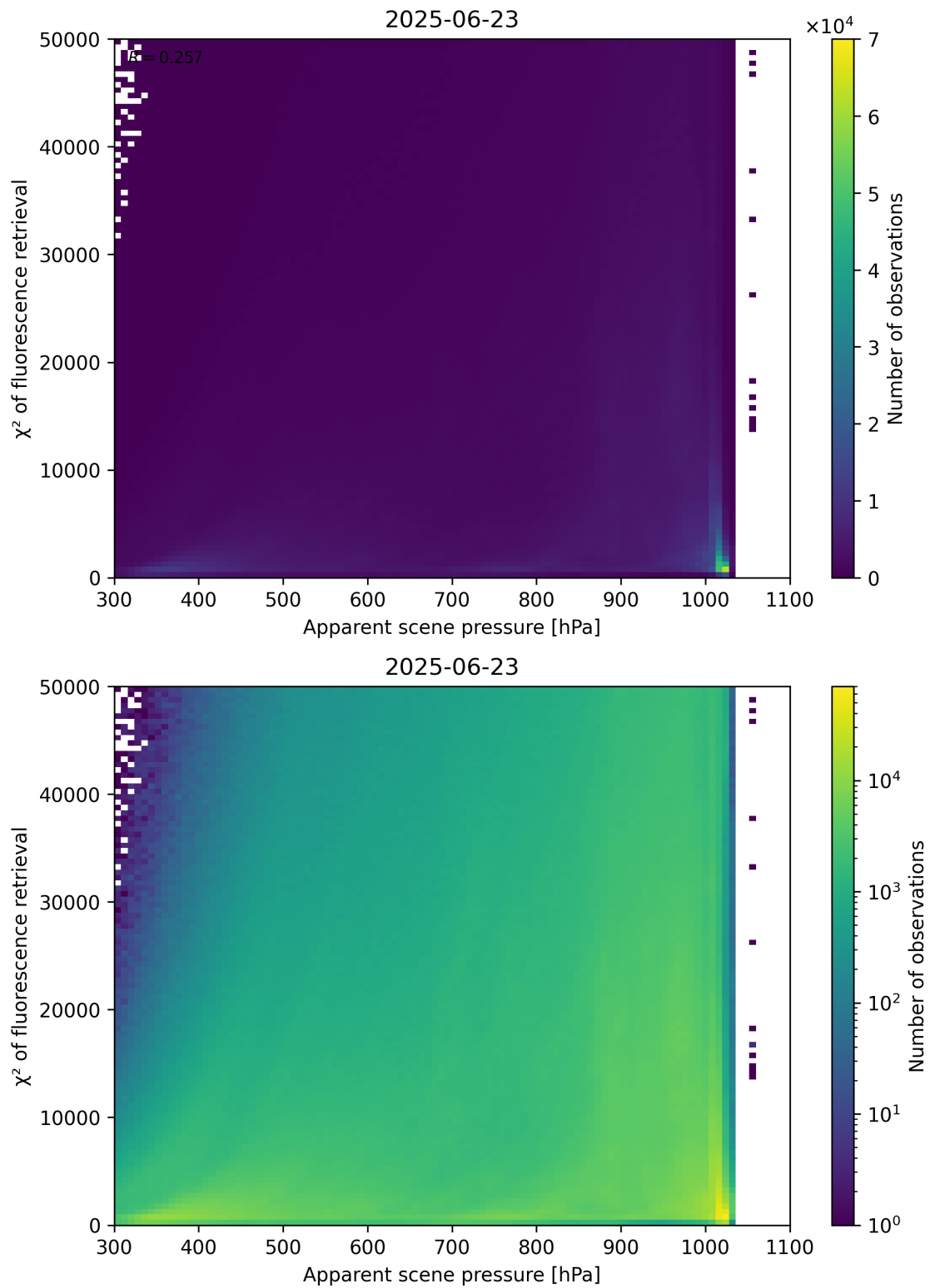
Figure 63: Scatter density plot of “Apparent scene pressure” against “ \chi^2 of fluorescence retrieval” for 2025-06-22 to 2025-06-24.
