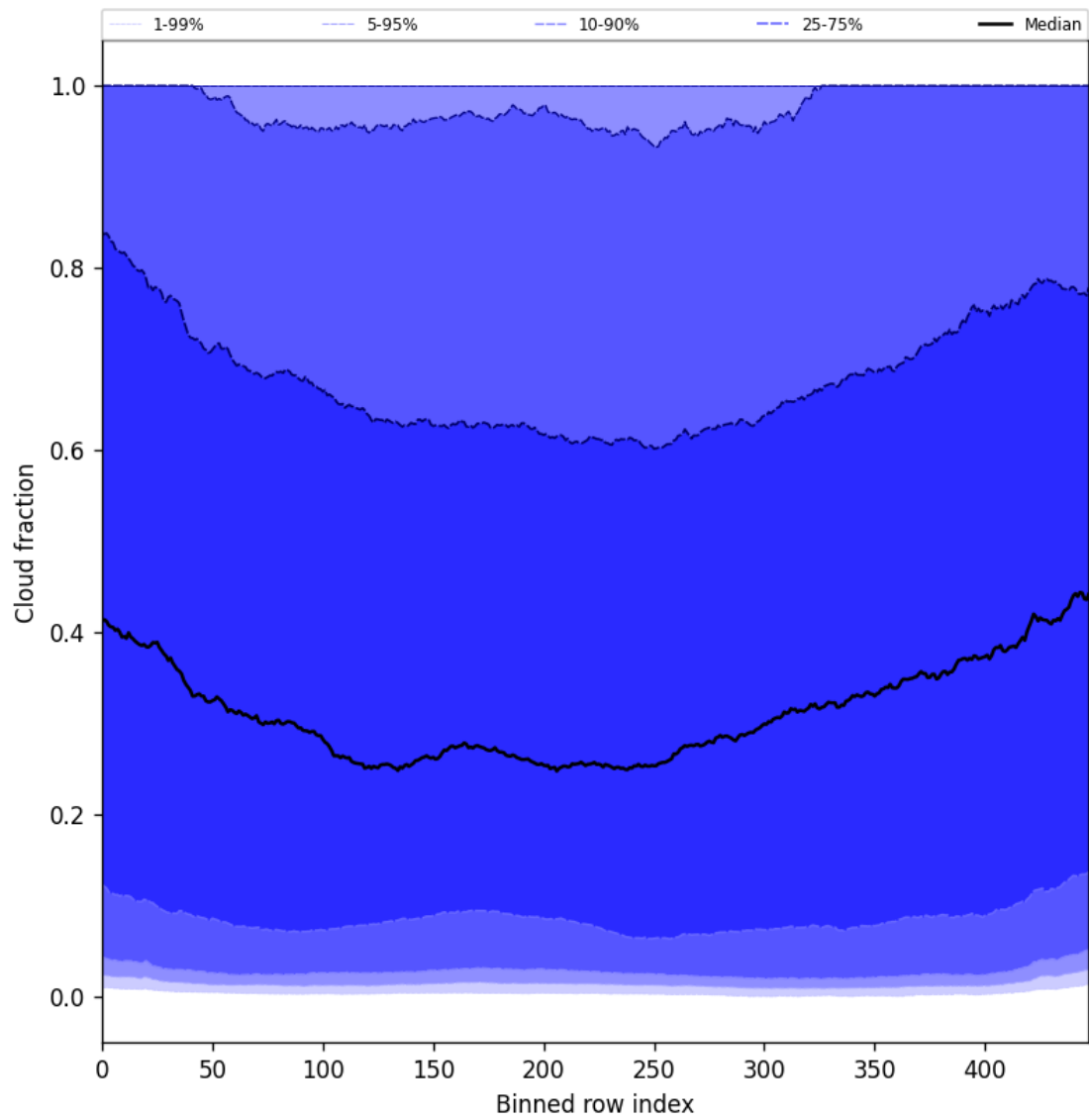
Figure 49: Along track statistics of “Cloud fraction” for 2025-06-22 to 2025-06-24
