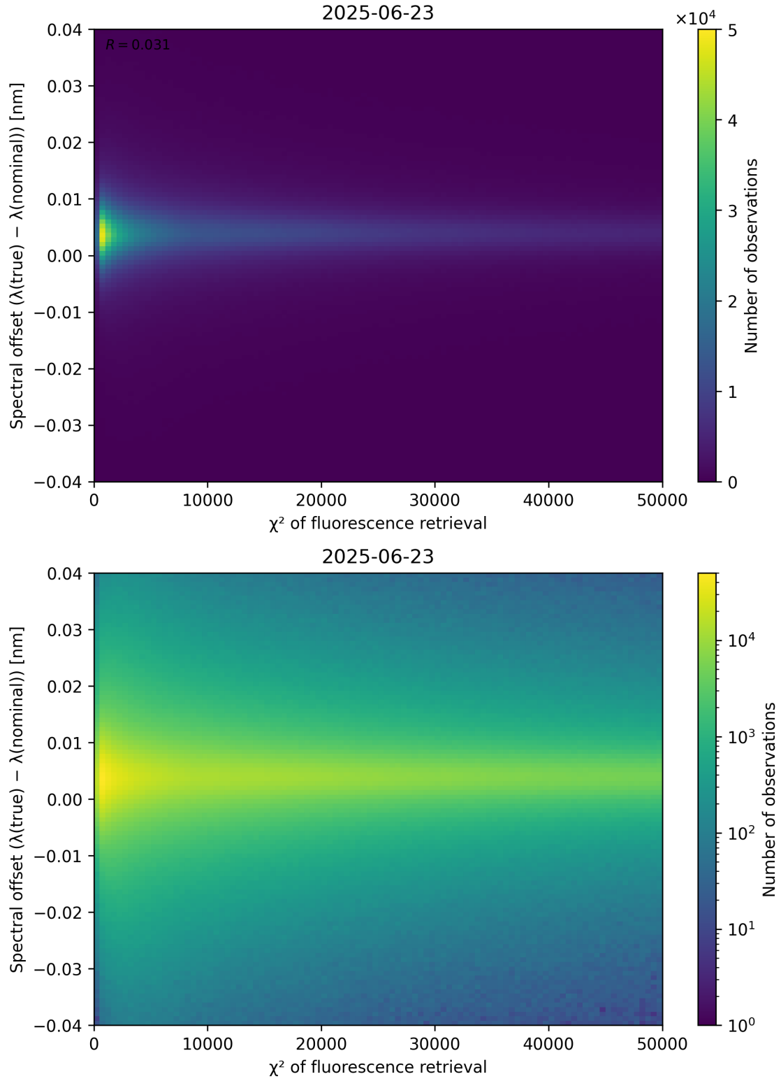
Figure 69: Scatter density plot of “ \chi^2 of fluorescence retrieval” against “Spectral offset ( \lambda_{\text{true}} - \lambda_{\text{nominal}} )” for 2025-06-22 to 2025-06-24.
