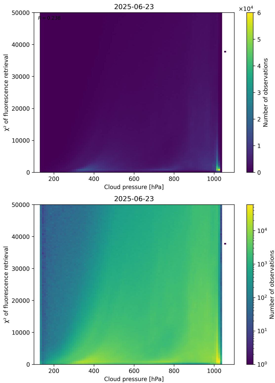
Figure 78: Scatter density plot of “Cloud pressure” against “ \chi^2 of fluorescence retrieval” for 2025-06-22 to 2025-06-24.
