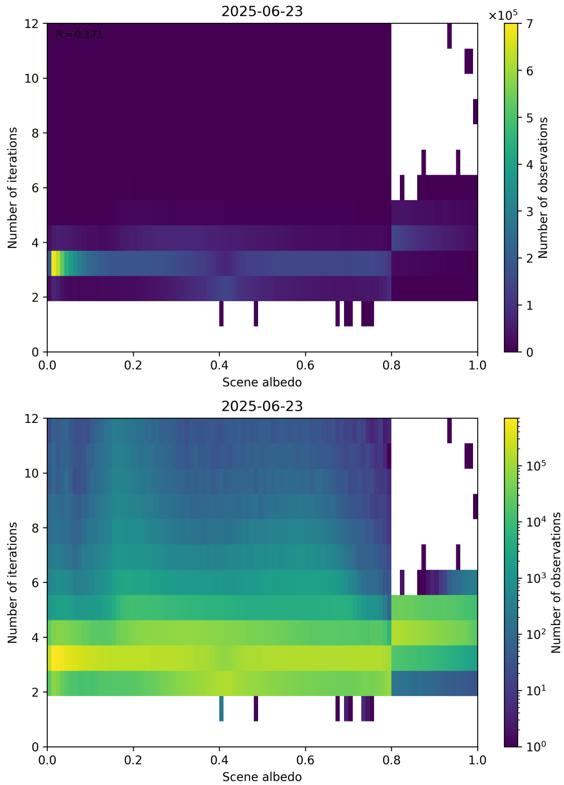
Figure 105: Scatter density plot of “Scene albedo” against “Number of iterations” for 2025-06-22 to 2025-06-24.
