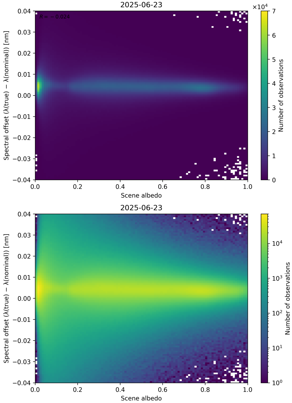
Figure 107: Scatter density plot of “Scene albedo” against “Spectral offset ( \lambda_{\text{true}} - \lambda_{\text{nominal}} )” for 2025-06-22 to 2025-06-24.
