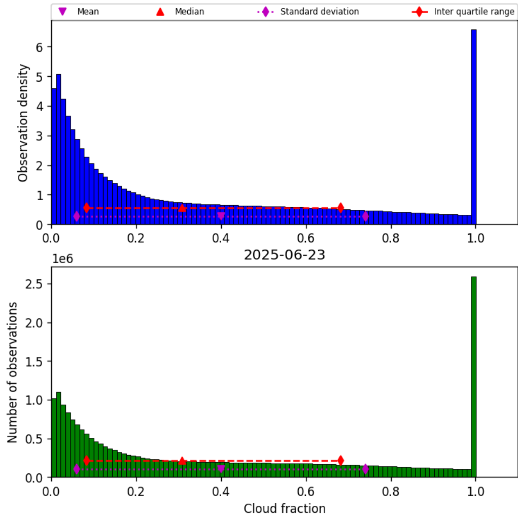
Figure 32: Histogram of “Cloud fraction” for 2025-06-22 to 2025-06-24
