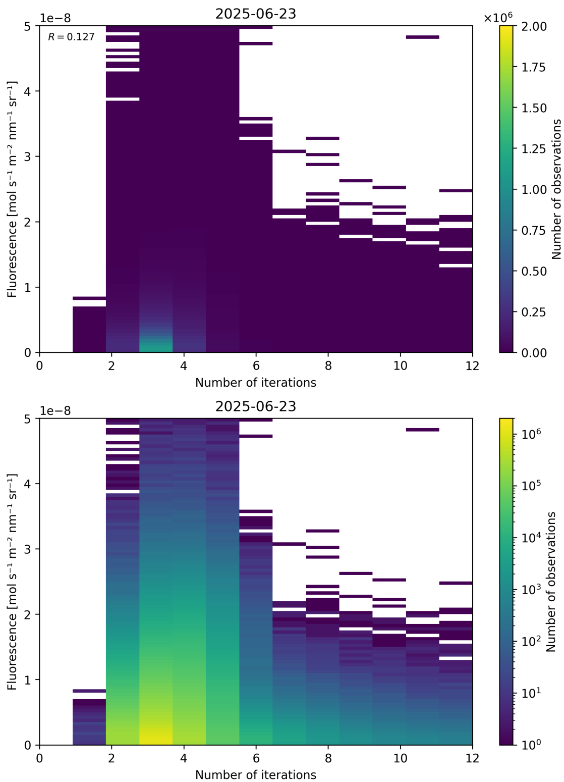
Figure 98: Scatter density plot of “Number of iterations” against “Fluorescence” for 2025-06-22 to 2025-06-24.
