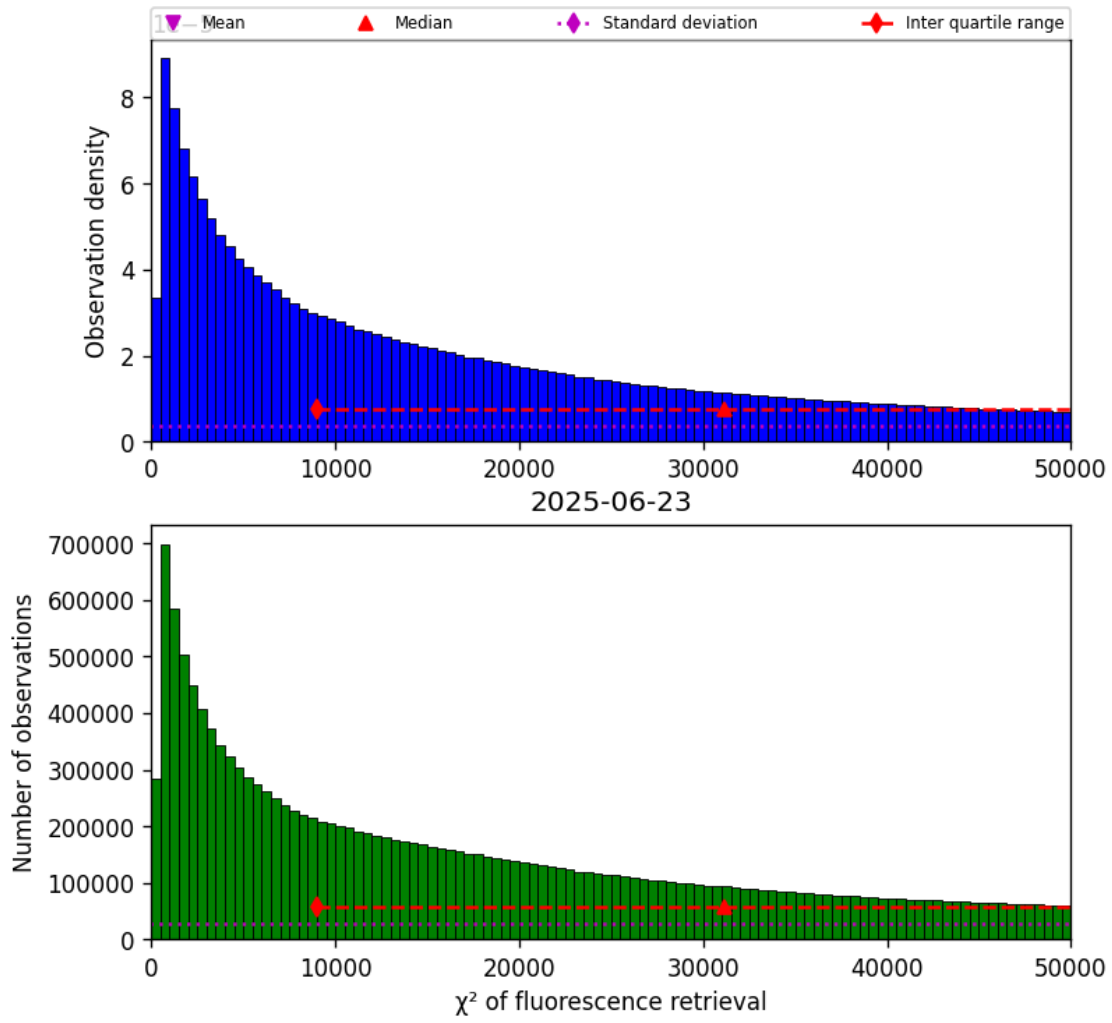
Figure 42: Histogram of “ \chi^2 of fluorescence retrieval” for 2025-06-22 to 2025-06-24
