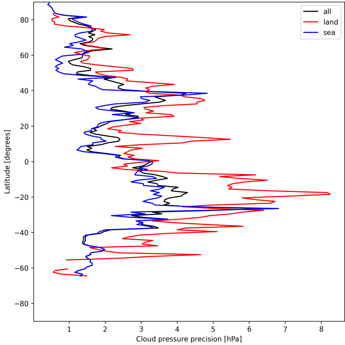
Figure 14: Zonal average of "Cloud pressure precision" for 2025-06-22 to 2025-06-24.
