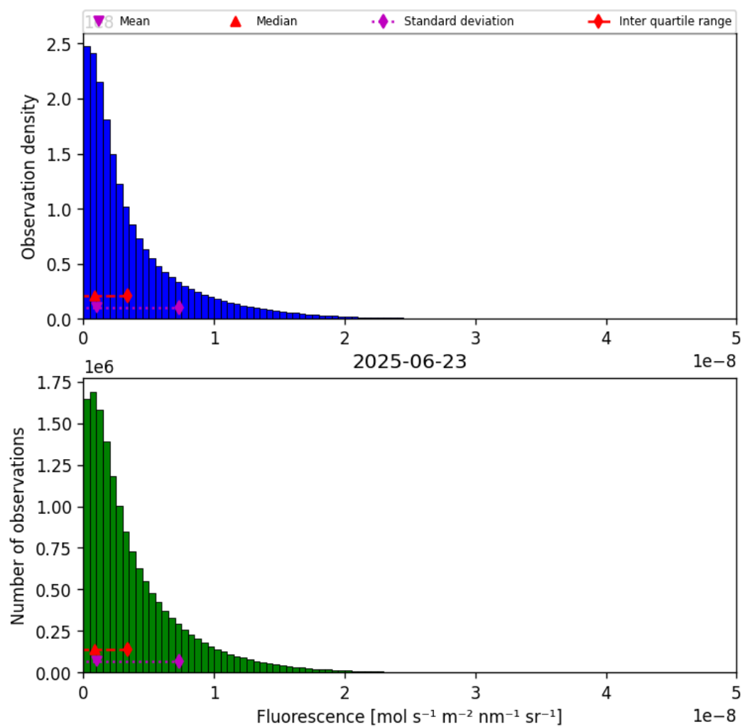
Figure 40: Histogram of “Fluorescence” for 2025-06-22 to 2025-06-24
