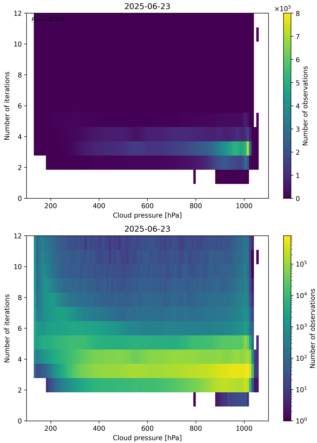
Figure 81: Scatter density plot of “Cloud pressure” against “Number of iterations” for 2025-06-22 to 2025-06-24.
