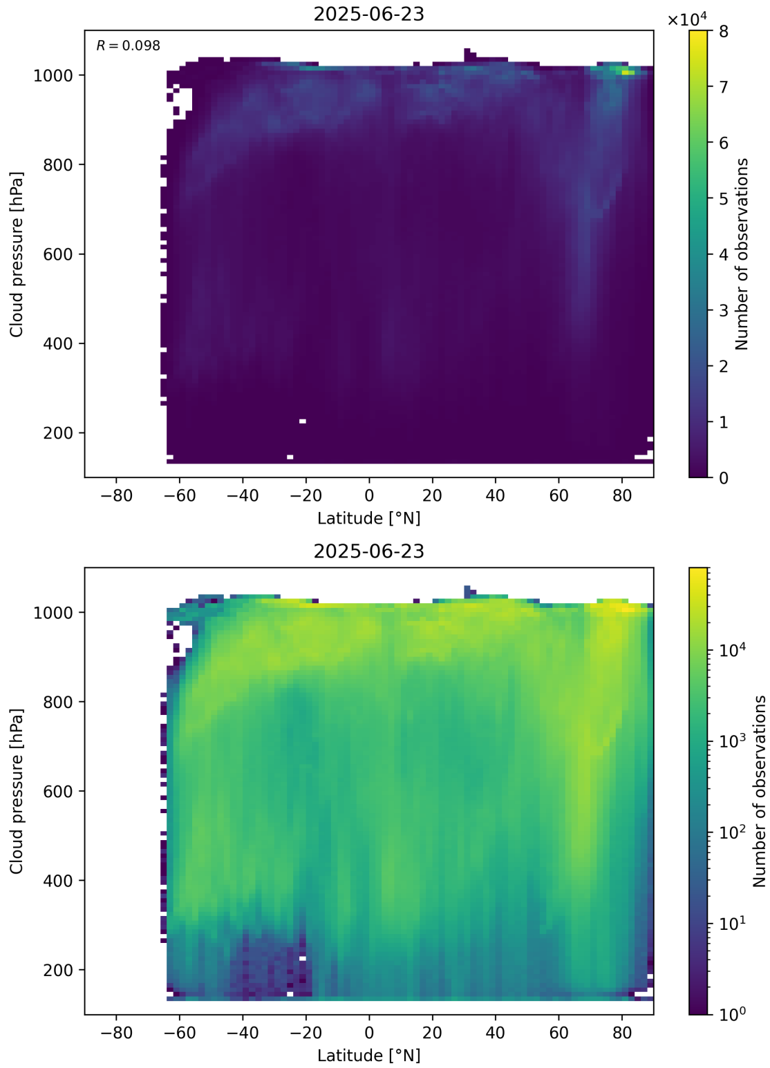
Figure 91: Scatter density plot of “Latitude” against “Cloud pressure” for 2025-06-22 to 2025-06-24.
