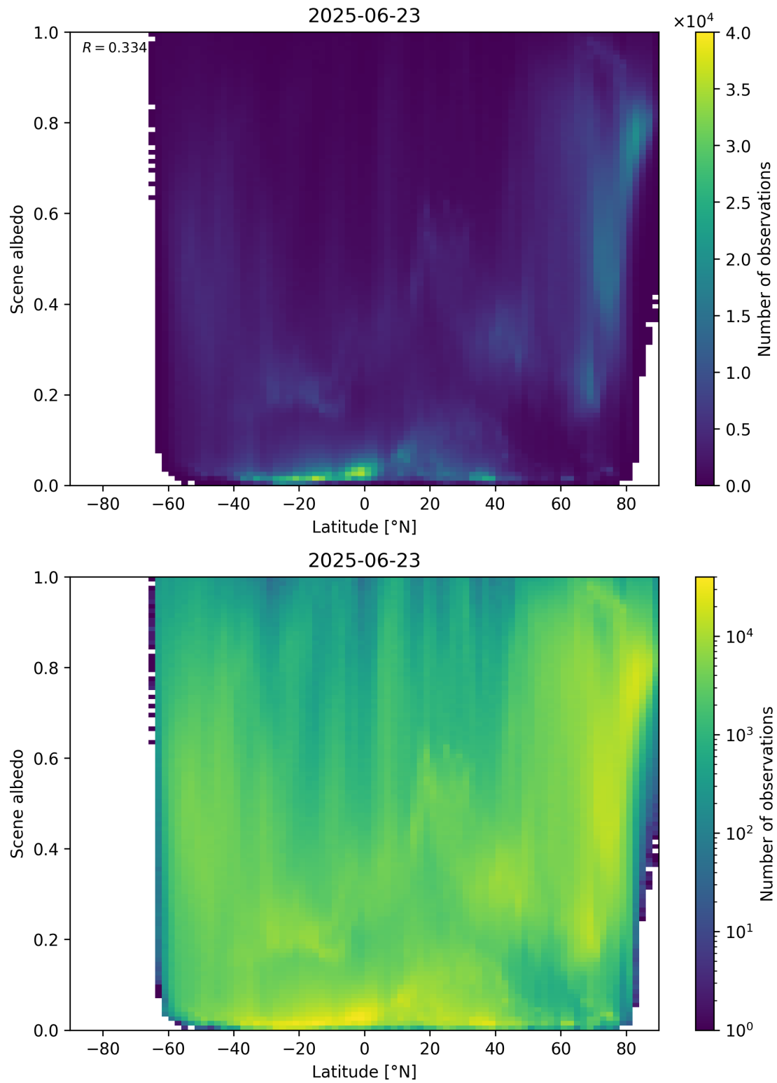
Figure 95: Scatter density plot of “Latitude” against “Scene albedo” for 2025-06-22 to 2025-06-24.
