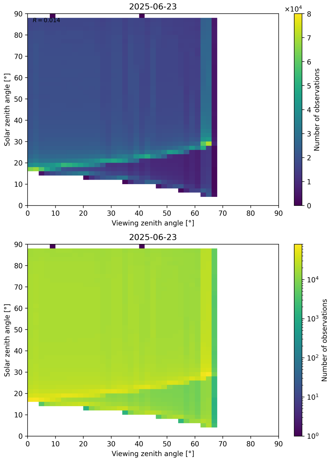
Figure 127: Scatter density plot of “Viewing zenith angle” against “Solar zenith angle” for 2025-06-22 to 2025-06-24.
