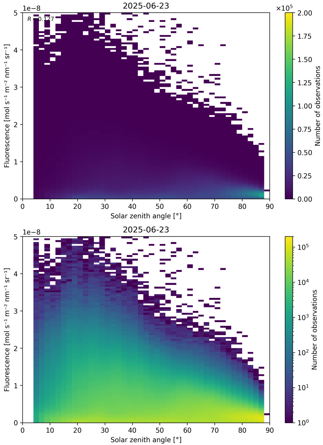
Figure 112: Scatter density plot of “Solar zenith angle” against “Fluorescence” for 2025-06-22 to 2025-06-24.
