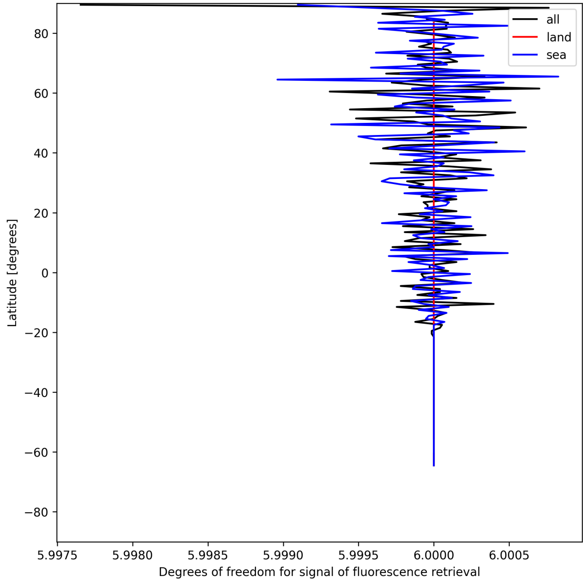
Figure 26: Zonal average of “Degrees of freedom for signal of fluorescence retrieval” for 2025-06-22 to 2025-06-24.
