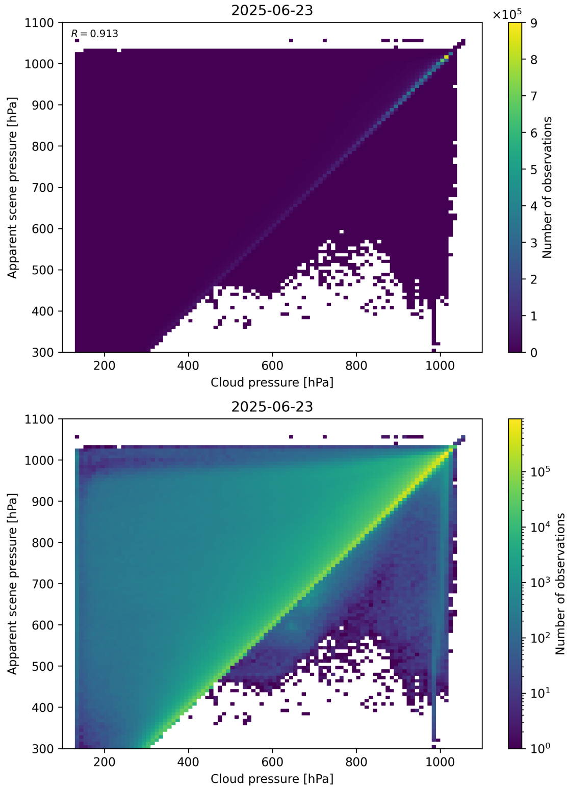
Figure 77: Scatter density plot of “Cloud pressure” against “Apparent scene pressure” for 2025-06-22 to 2025-06-24.
