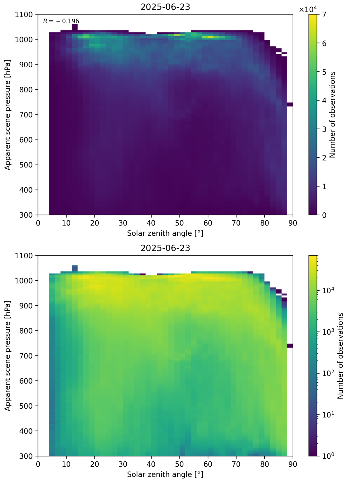
Figure 108: Scatter density plot of “Solar zenith angle” against “Apparent scene pressure” for 2025-06-22 to 2025-06-24.
