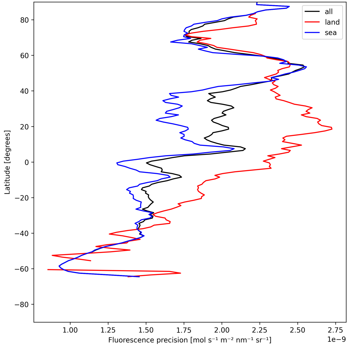
Figure 24: Zonal average of “Fluorescence precision” for 2025-06-22 to 2025-06-24.
