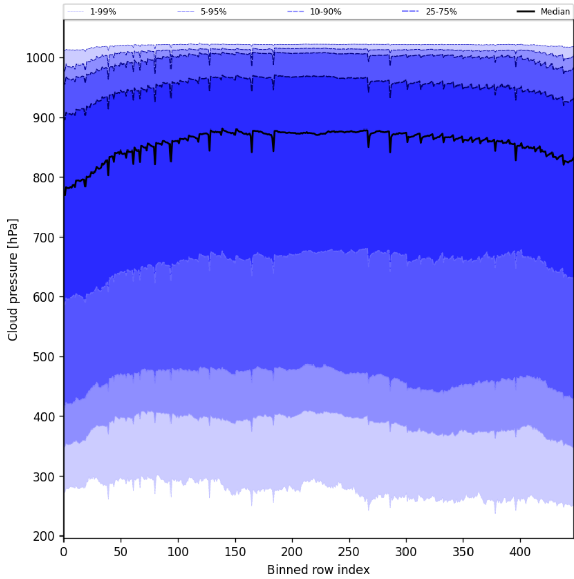
Figure 47: Along track statistics of “Cloud pressure” for 2025-06-22 to 2025-06-24
