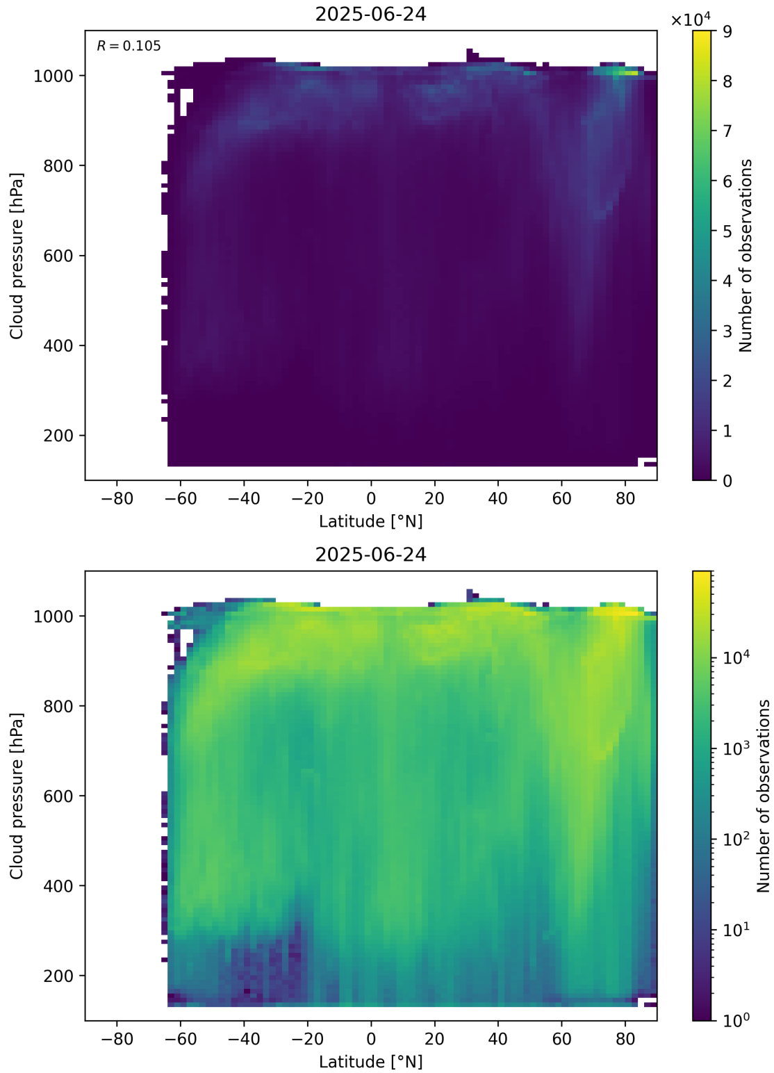
Figure 91: Scatter density plot of “Latitude” against “Cloud pressure” for 2025-06-23 to 2025-06-25.
