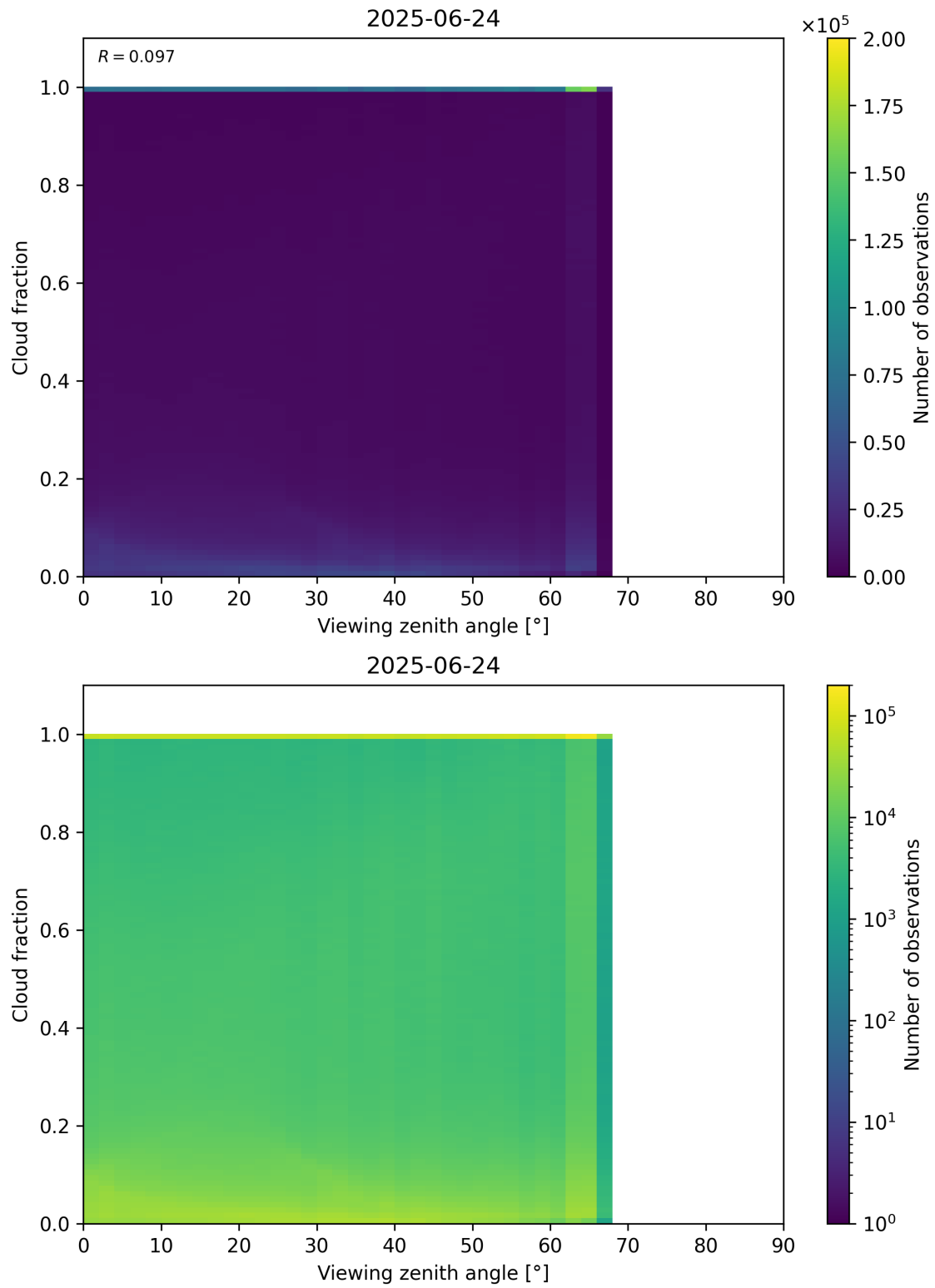
Figure 120: Scatter density plot of “Viewing zenith angle” against “Cloud fraction” for 2025-06-23 to 2025-06-25.
