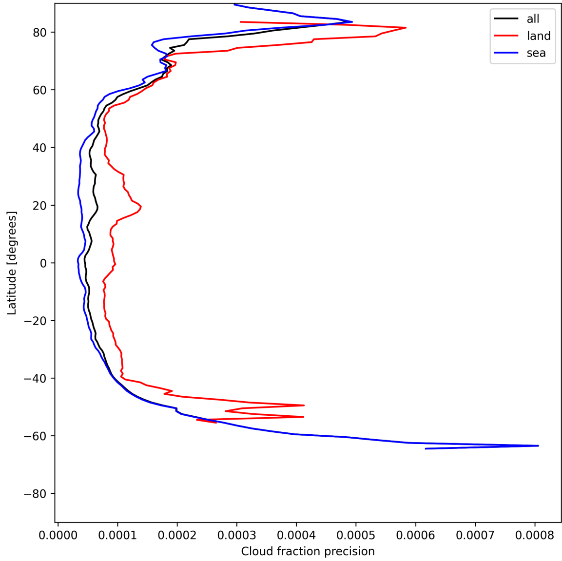
Figure 16: Zonal average of “Cloud fraction precision” for 2025-06-23 to 2025-06-25.
