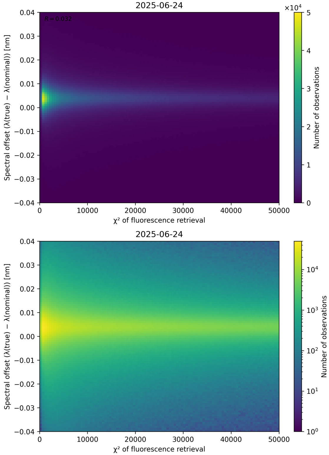
Figure 69: Scatter density plot of “ \chi^2 of fluorescence retrieval” against “Spectral offset ( \lambda_{\text{true}} - \lambda_{\text{nominal}} )” for 2025-06-23 to 2025-06-25.
