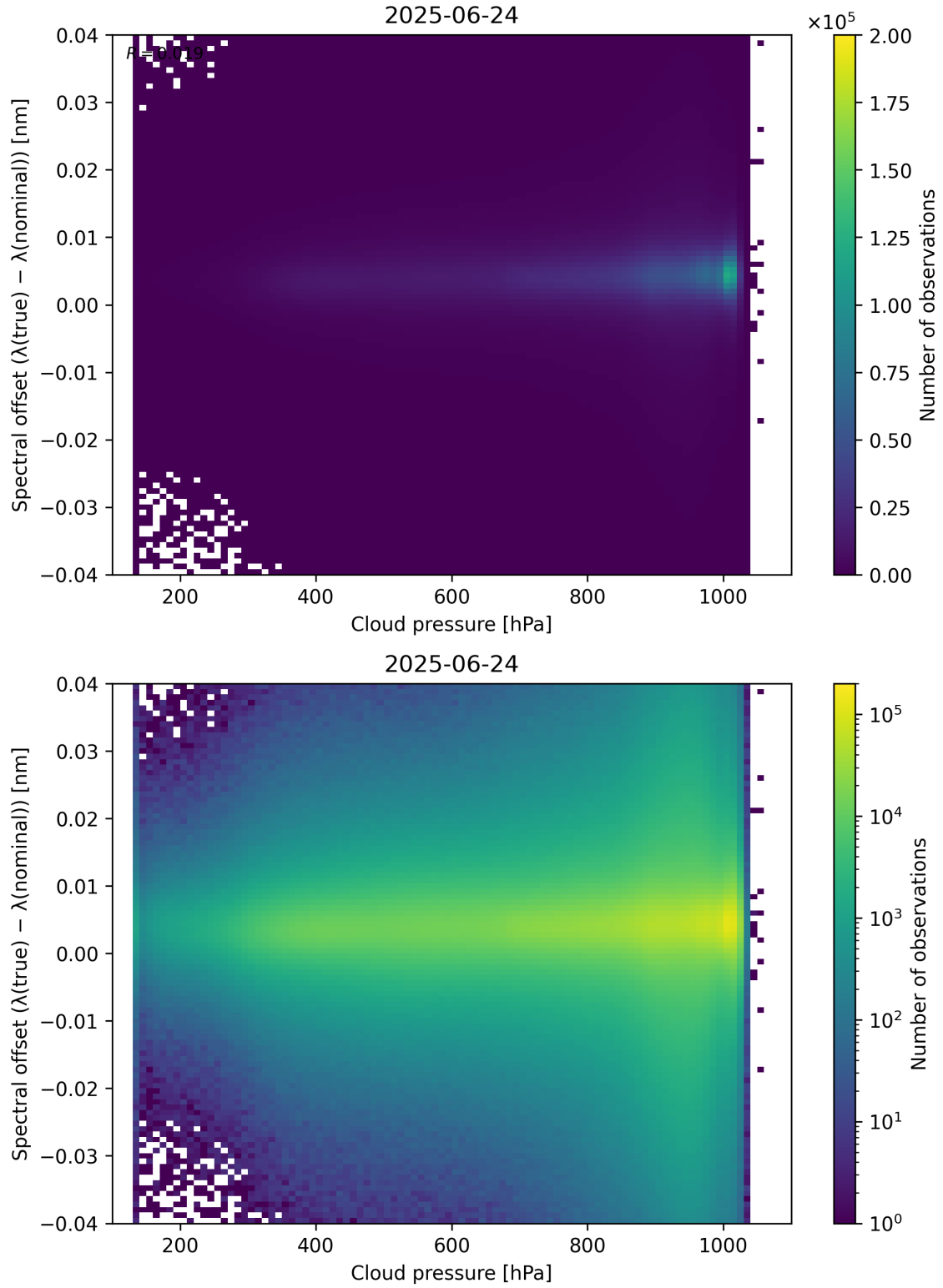
Figure 84: Scatter density plot of “Cloud pressure” against “Spectral offset ( \lambda_{\text{true}} - \lambda_{\text{nominal}} )” for 2025-06-23 to 2025-06-25.
