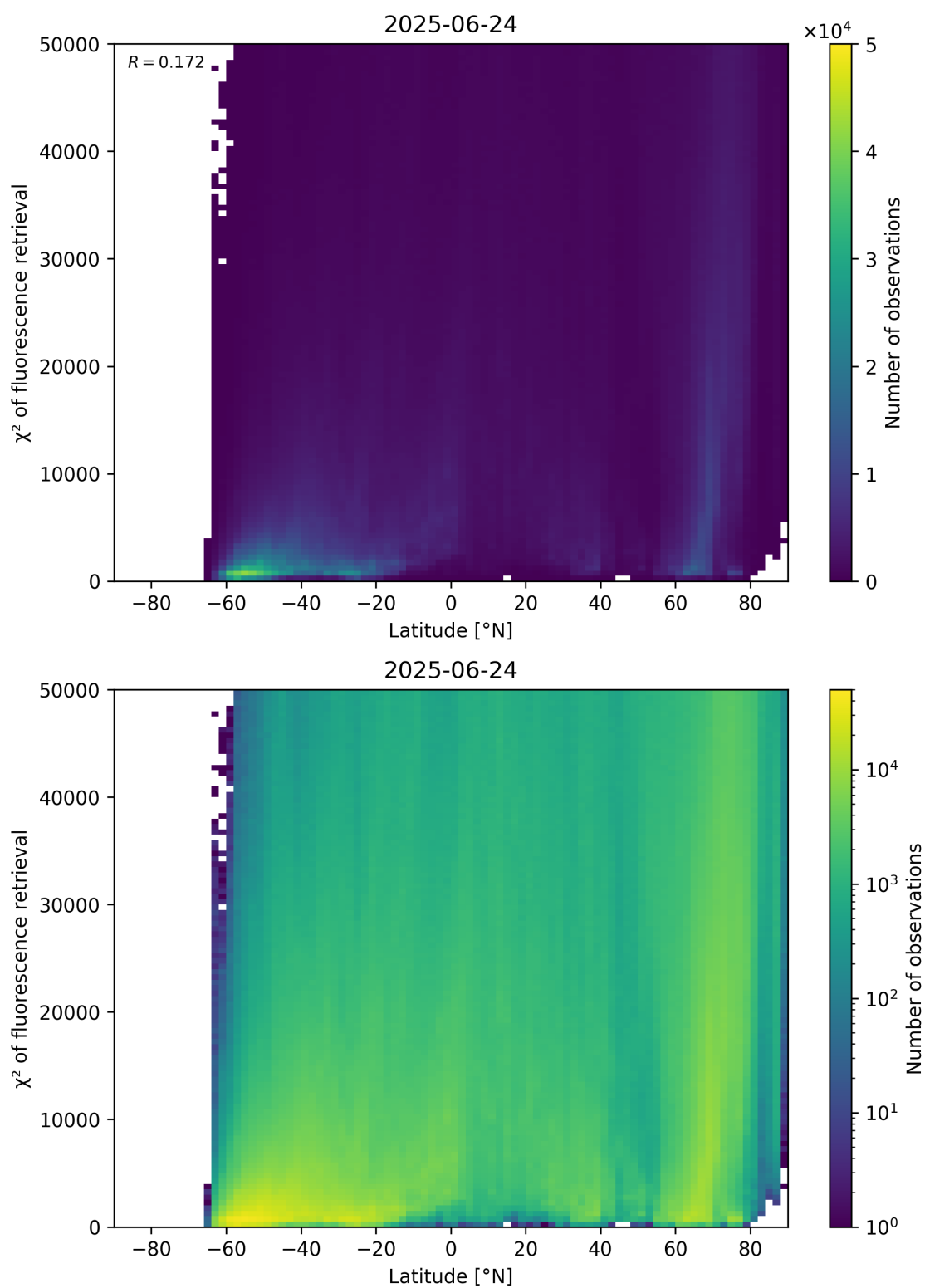
Figure 89: Scatter density plot of “Latitude” against “ \chi^2 of fluorescence retrieval” for 2025-06-23 to 2025-06-25.
