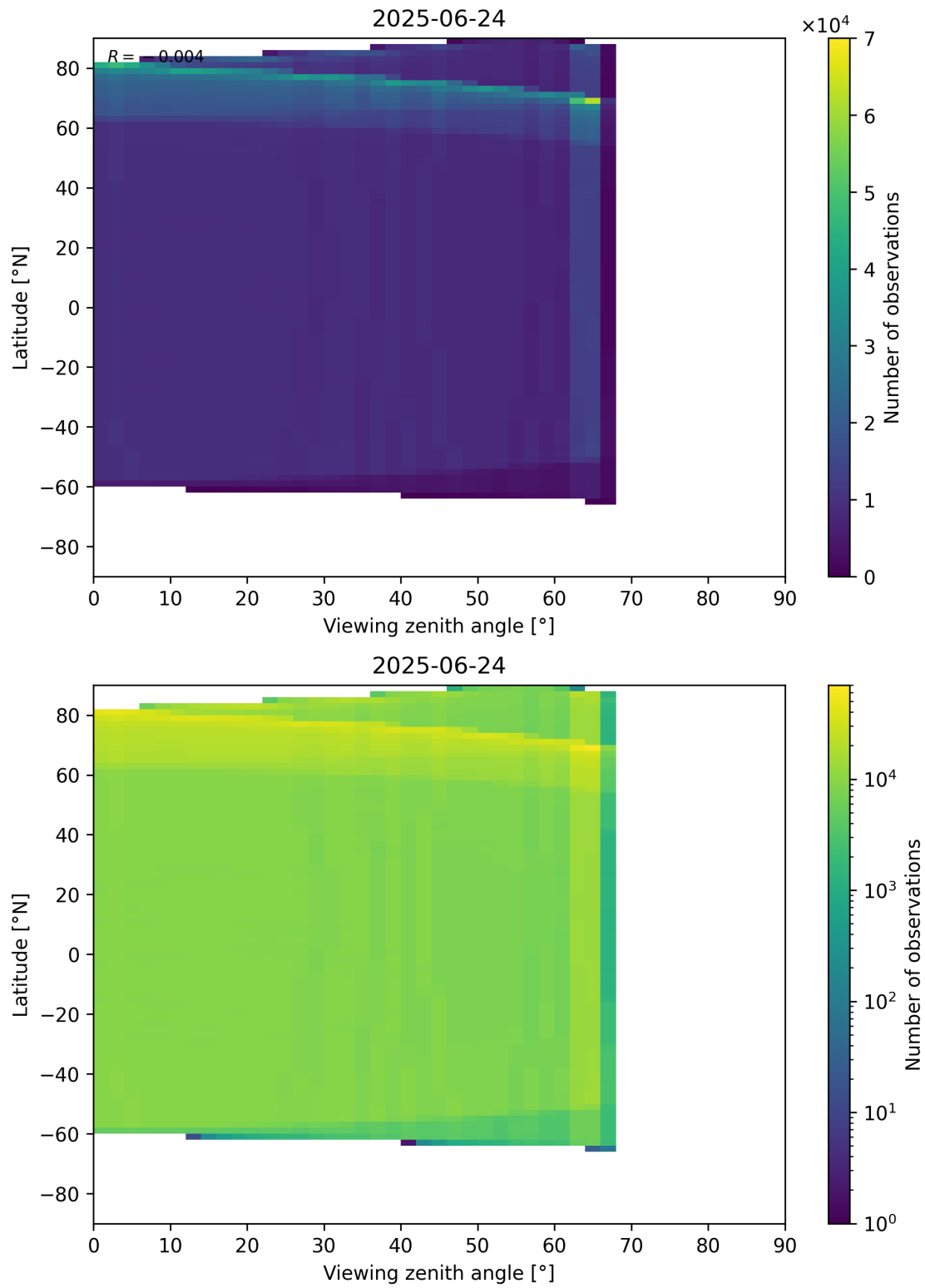
Figure 123: Scatter density plot of “Viewing zenith angle” against “Latitude” for 2025-06-23 to 2025-06-25.
