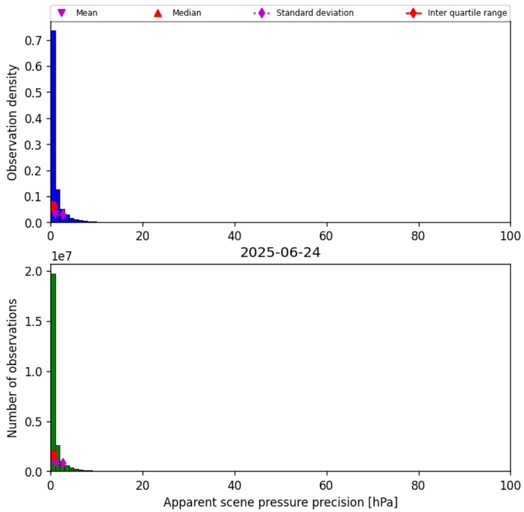
Figure 37: Histogram of “Apparent scene pressure precision” for 2025-06-23 to 2025-06-25
