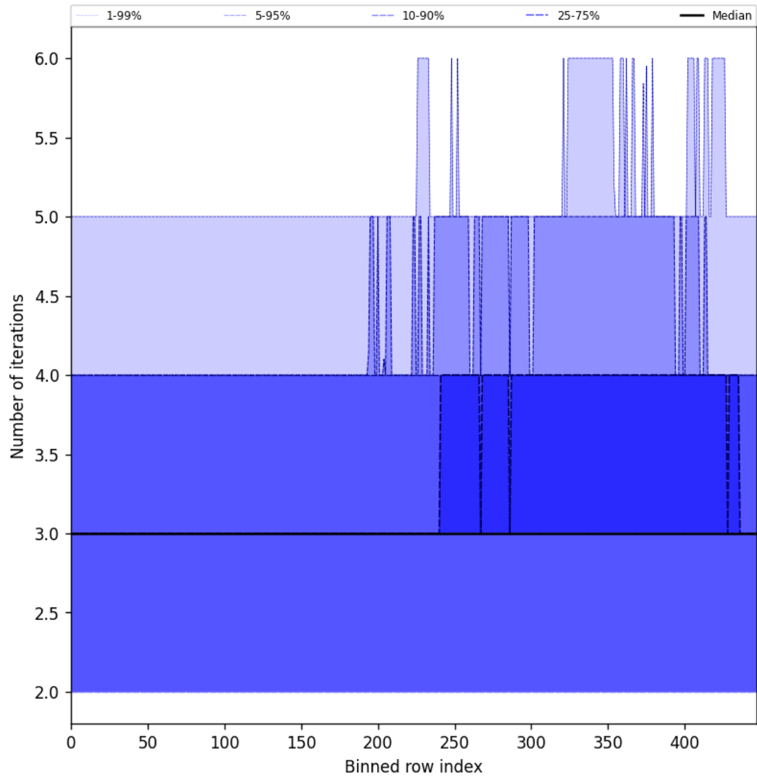
Figure 56: Along track statistics of “Number of iterations” for 2025-06-23 to 2025-06-25
