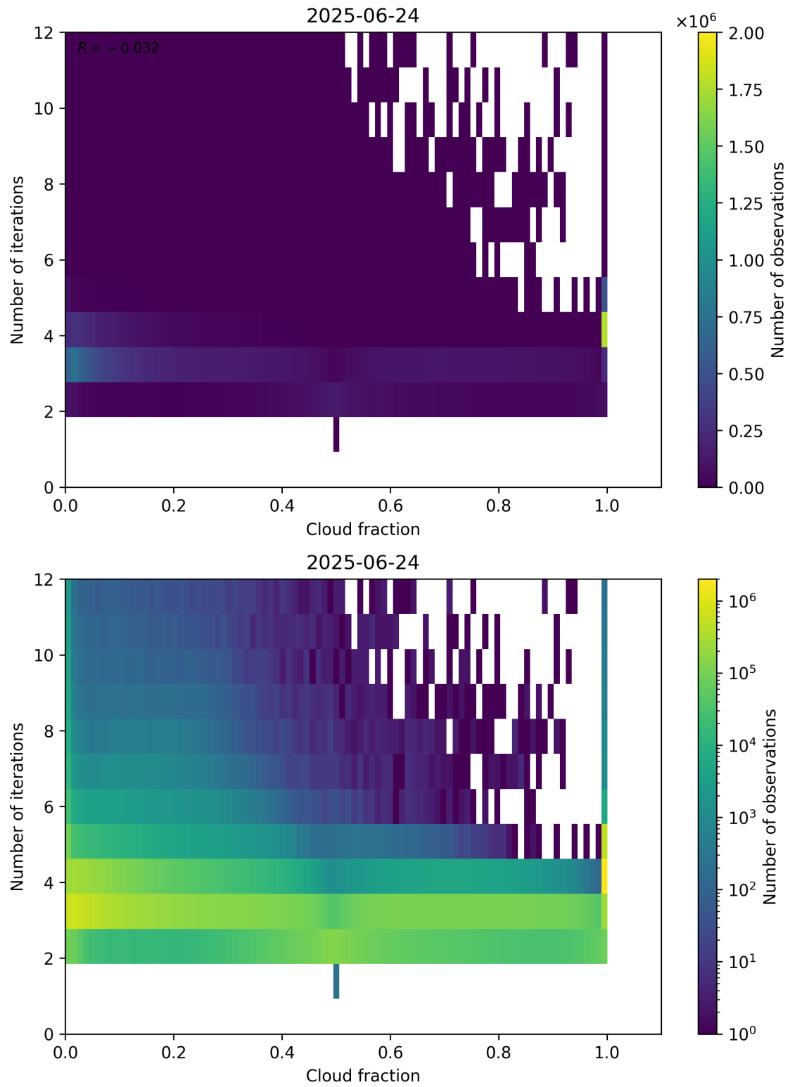
Figure 73: Scatter density plot of “Cloud fraction” against “Number of iterations” for 2025-06-23 to 2025-06-25.
