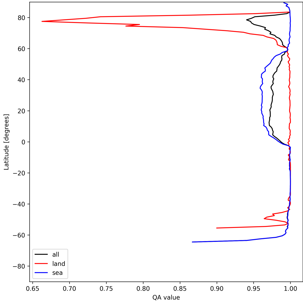
Figure 12: Zonal average of “QA value” for 2025-06-23 to 2025-06-25.
