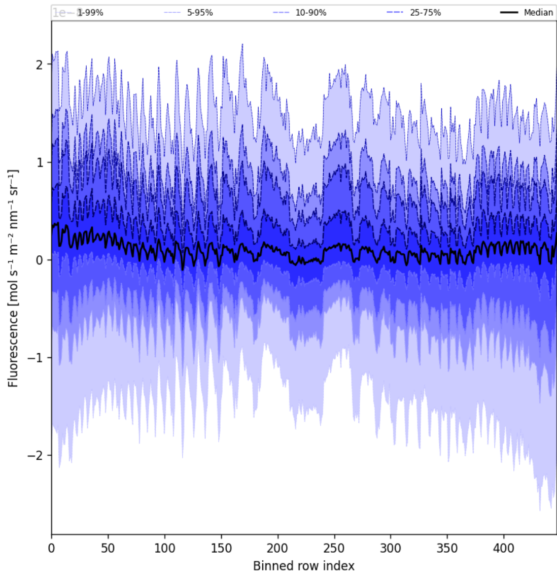
Figure 57: Along track statistics of “Fluorescence” for 2025-06-23 to 2025-06-25
