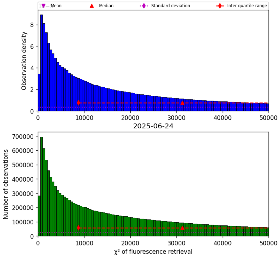
Figure 42: Histogram of “ \chi^2 of fluorescence retrieval” for 2025-06-23 to 2025-06-25
