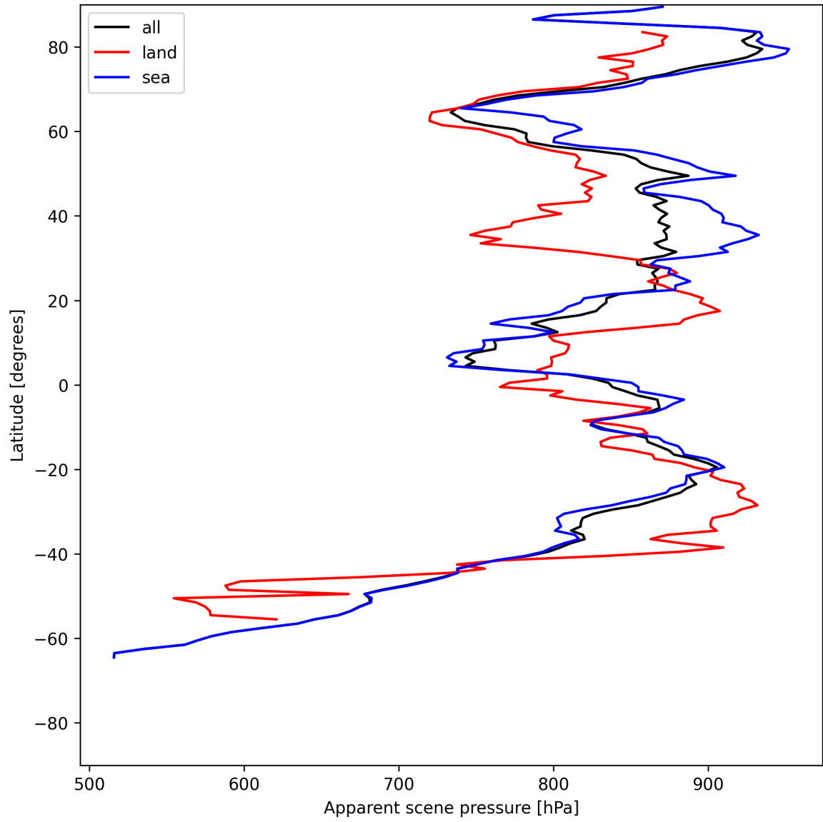
Figure 19: Zonal average of “Apparent scene pressure” for 2025-06-23 to 2025-06-25.
