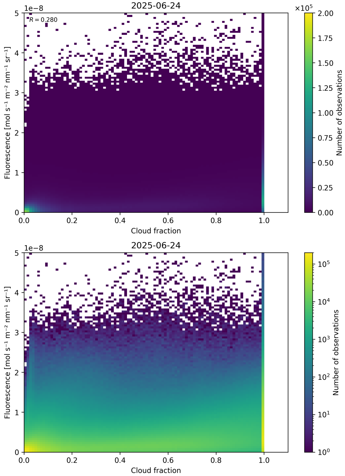
Figure 72: Scatter density plot of “Cloud fraction” against “Fluorescence” for 2025-06-23 to 2025-06-25.
