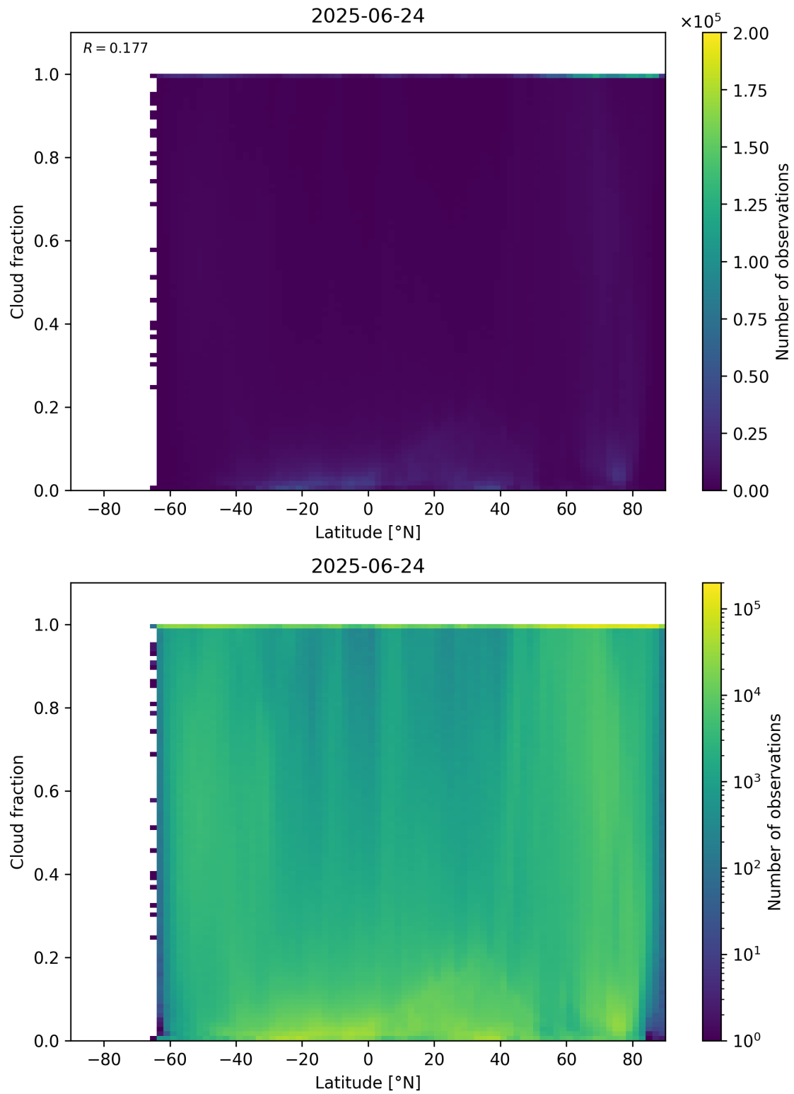
Figure 90: Scatter density plot of “Latitude” against “Cloud fraction” for 2025-06-23 to 2025-06-25.
