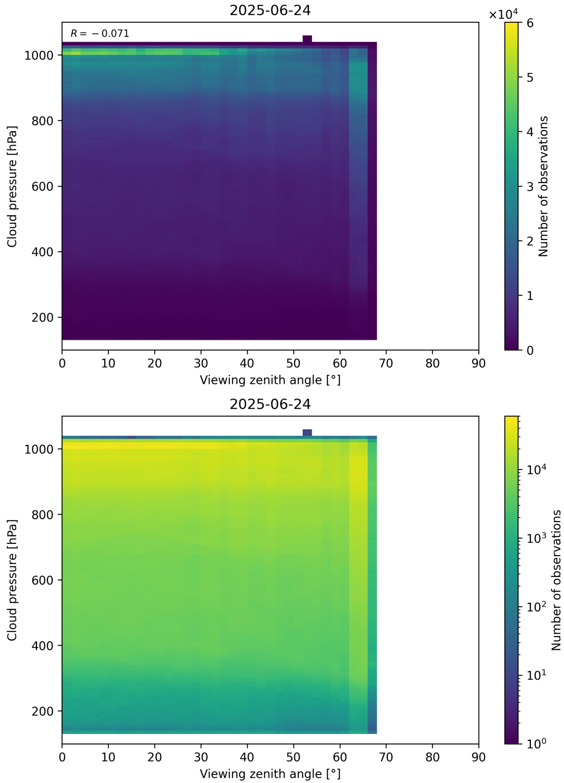
Figure 121: Scatter density plot of “Viewing zenith angle” against “Cloud pressure” for 2025-06-23 to 2025-06-25.
