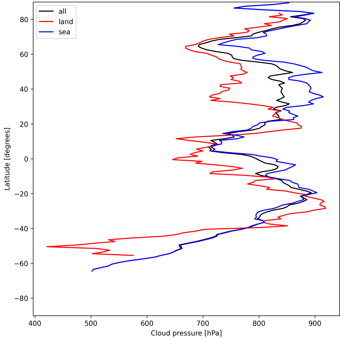
Figure 13: Zonal average of “Cloud pressure” for 2025-06-23 to 2025-06-25.
