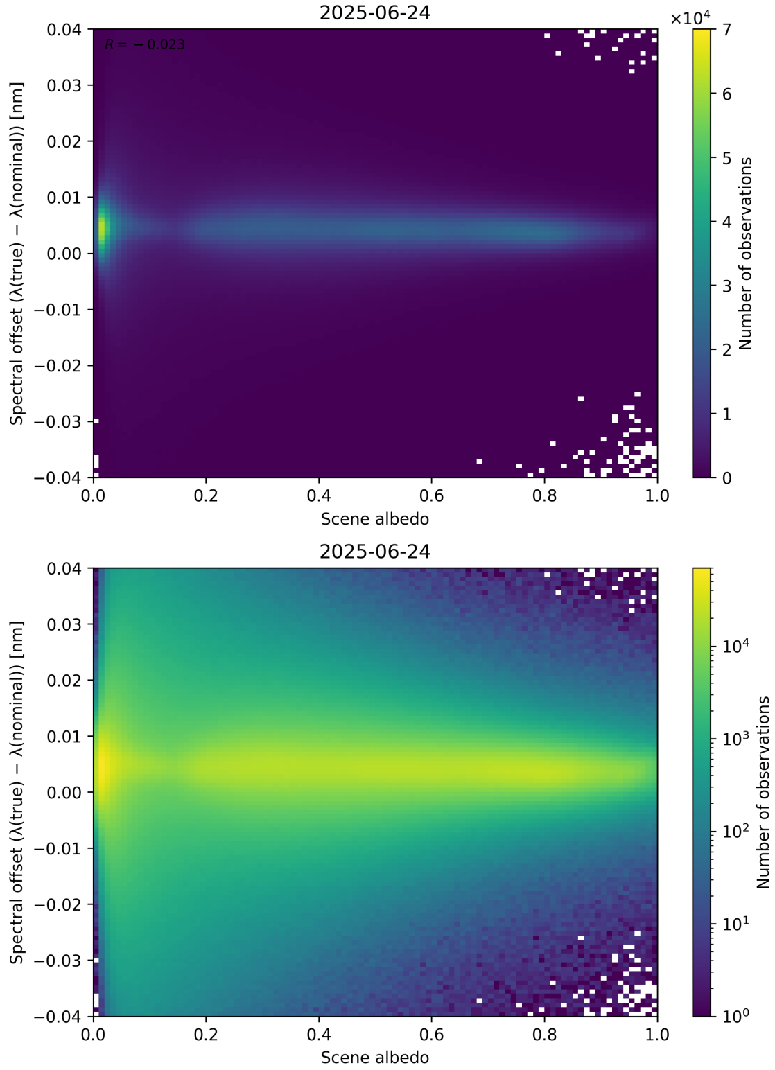
Figure 107: Scatter density plot of “Scene albedo” against “Spectral offset ( \lambda_{\text{true}} - \lambda_{\text{nominal}} )” for 2025-06-23 to 2025-06-25.
