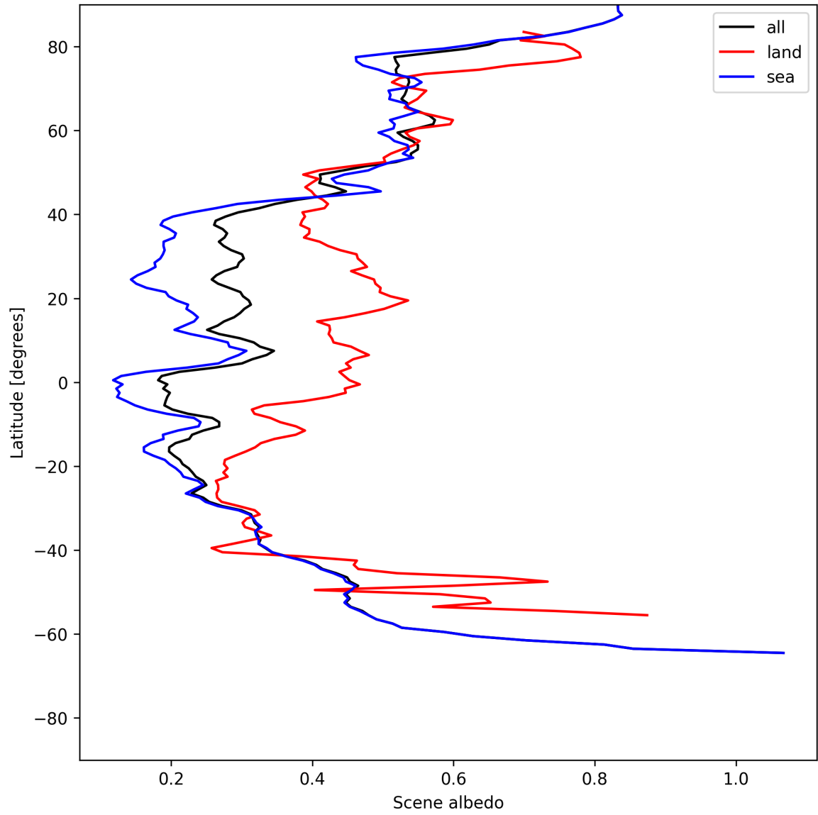
Figure 17: Zonal average of “Scene albedo” for 2025-06-23 to 2025-06-25.
