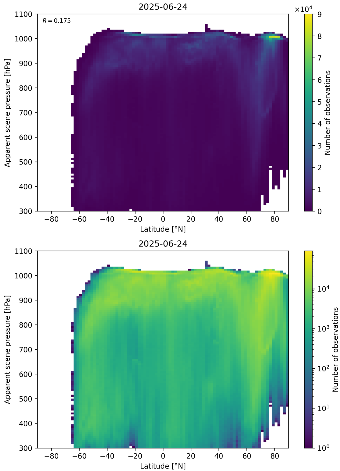
Figure 88: Scatter density plot of “Latitude” against “Apparent scene pressure” for 2025-06-23 to 2025-06-25.
