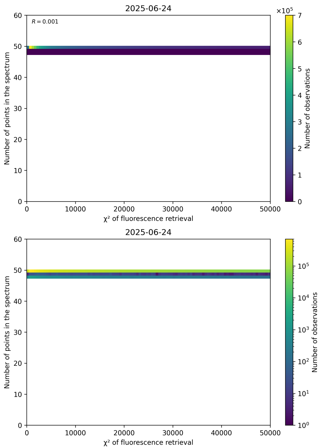
Figure 68: Scatter density plot of " \chi^2 of fluorescence retrieval" against "Number of points in the spectrum" for 2025-06-23 to 2025-06-25.
