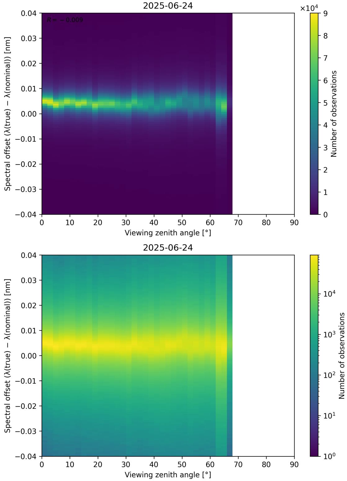
Figure 128: Scatter density plot of “Viewing zenith angle” against “Spectral offset ( \lambda_{\text{true}} - \lambda_{\text{nominal}} )” for 2025-06-23 to 2025-06-25.
