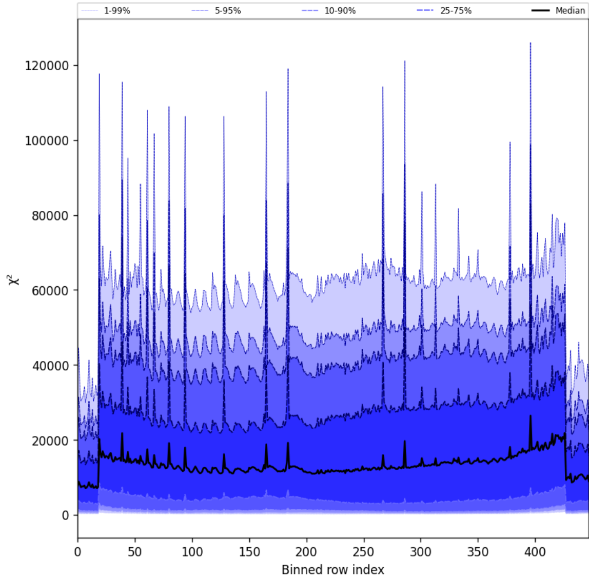
Figure 55: Along track statistics of “ \chi^2 ” for 2025-06-23 to 2025-06-25
