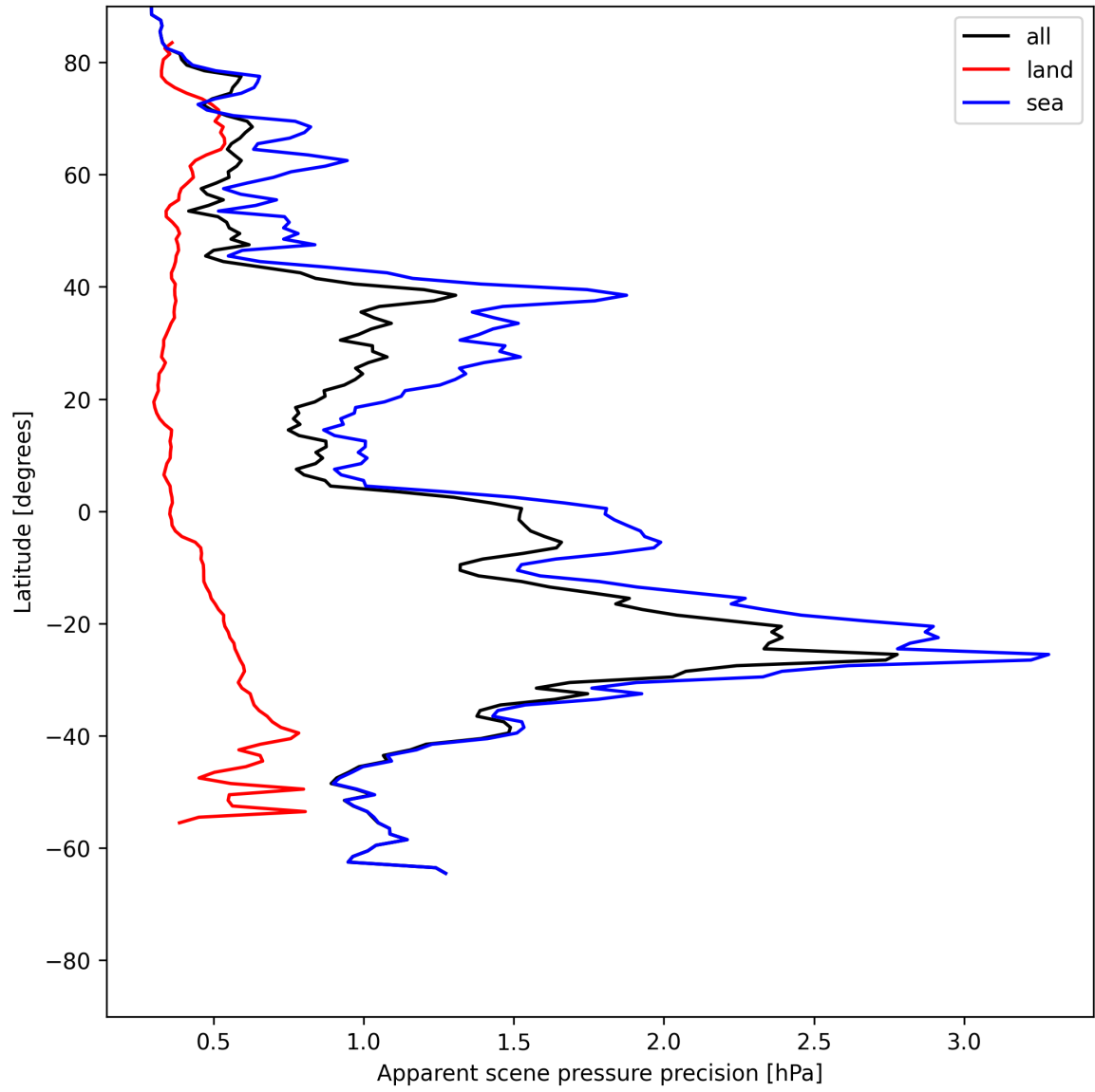
Figure 20: Zonal average of “Apparent scene pressure precision” for 2025-06-23 to 2025-06-25.
