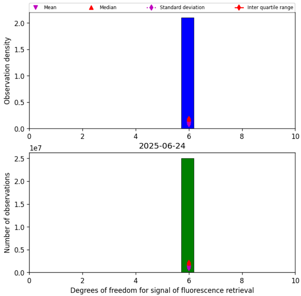
Figure 43: Histogram of “Degrees of freedom for signal of fluorescence retrieval” for 2025-06-23 to 2025-06-25
