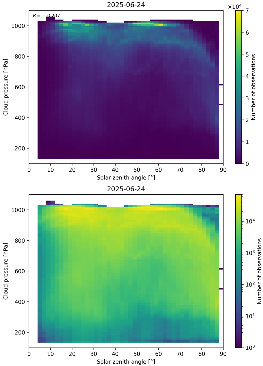
Figure 111: Scatter density plot of “Solar zenith angle” against “Cloud pressure” for 2025-06-23 to 2025-06-25.
