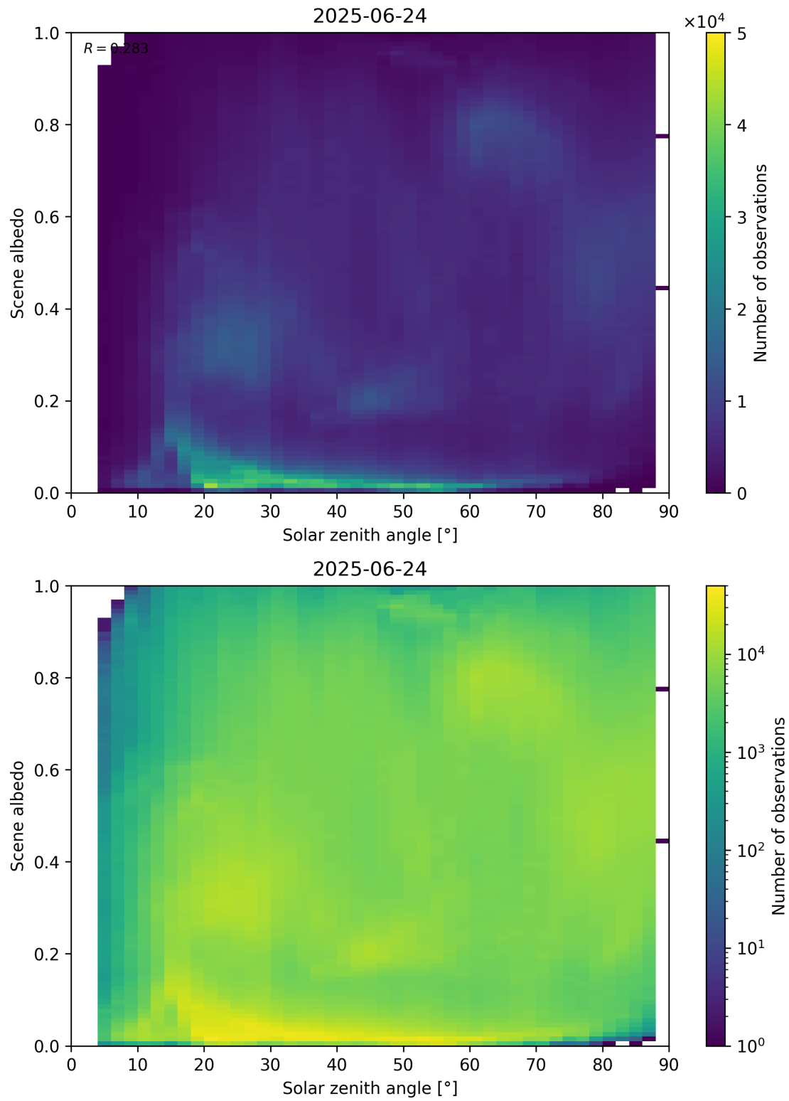
Figure 116: Scatter density plot of “Solar zenith angle” against “Scene albedo” for 2025-06-23 to 2025-06-25.
