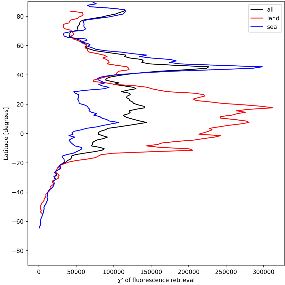
Figure 25: Zonal average of “ \chi^2 of fluorescence retrieval” for 2025-06-23 to 2025-06-25.
