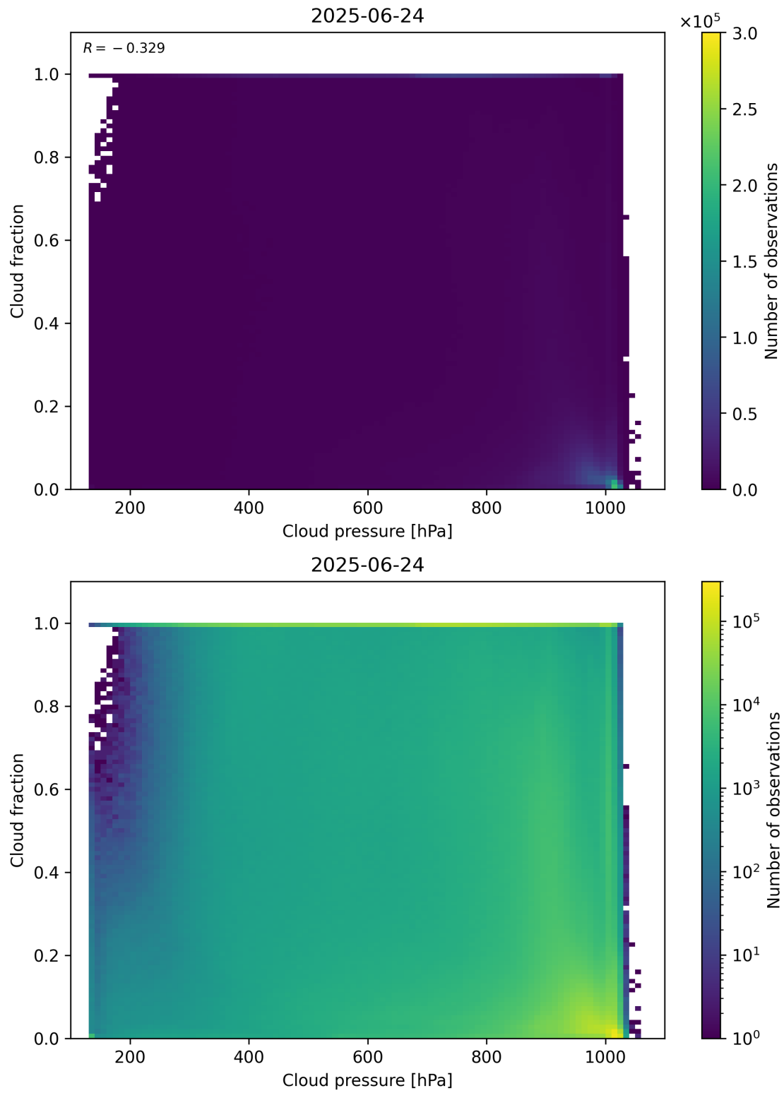
Figure 79: Scatter density plot of “Cloud pressure” against “Cloud fraction” for 2025-06-23 to 2025-06-25.
