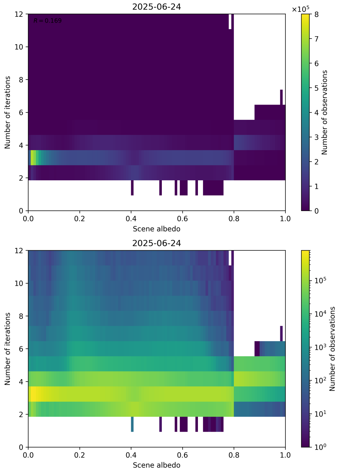
Figure 105: Scatter density plot of “Scene albedo” against “Number of iterations” for 2025-06-23 to 2025-06-25.
