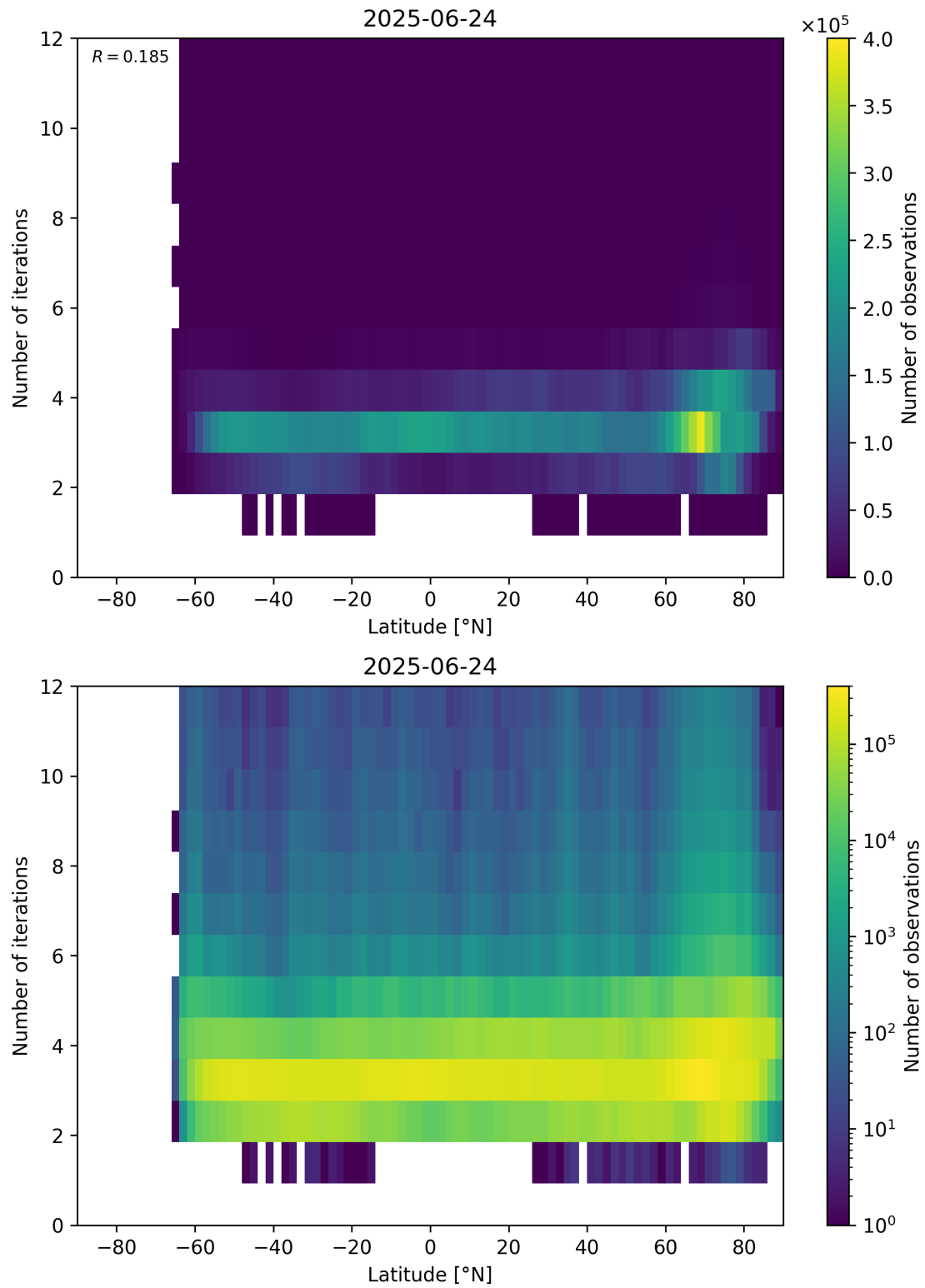
Figure 93: Scatter density plot of “Latitude” against “Number of iterations” for 2025-06-23 to 2025-06-25.
