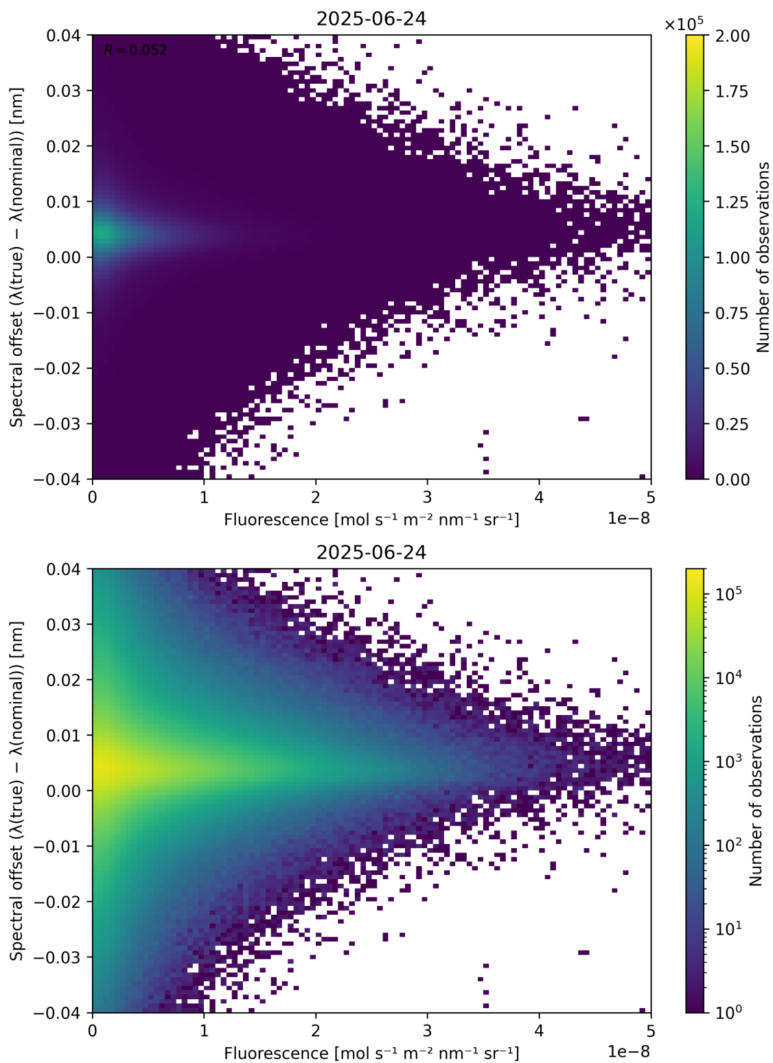
Figure 87: Scatter density plot of “Fluorescence” against “Spectral offset ( \lambda_{\text{true}} - \lambda_{\text{nominal}} )” for 2025-06-23 to 2025-06-25.
