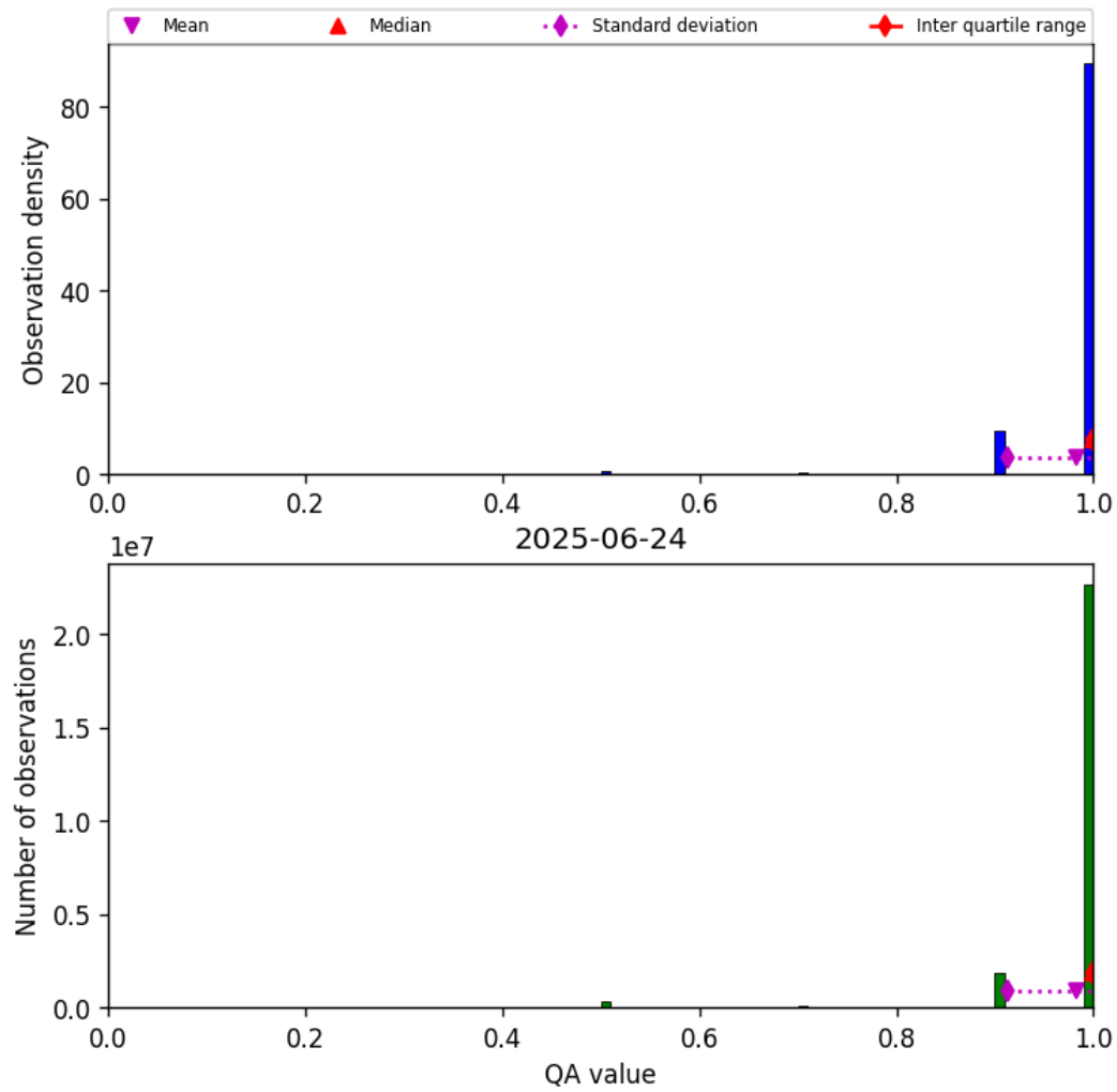
Figure 29: Histogram of “QA value” for 2025-06-23 to 2025-06-25
