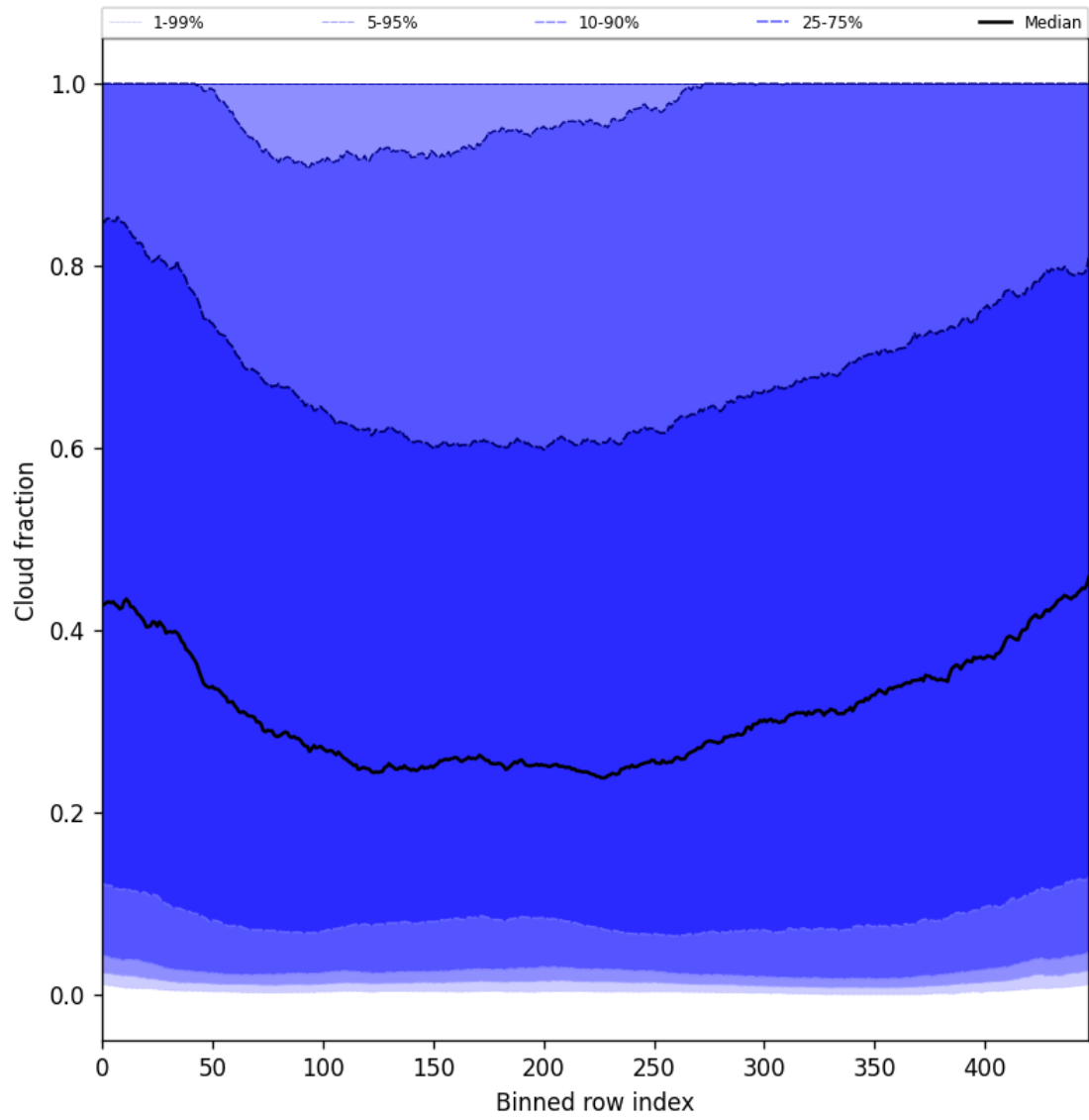
Figure 49: Along track statistics of “Cloud fraction” for 2025-06-23 to 2025-06-25
