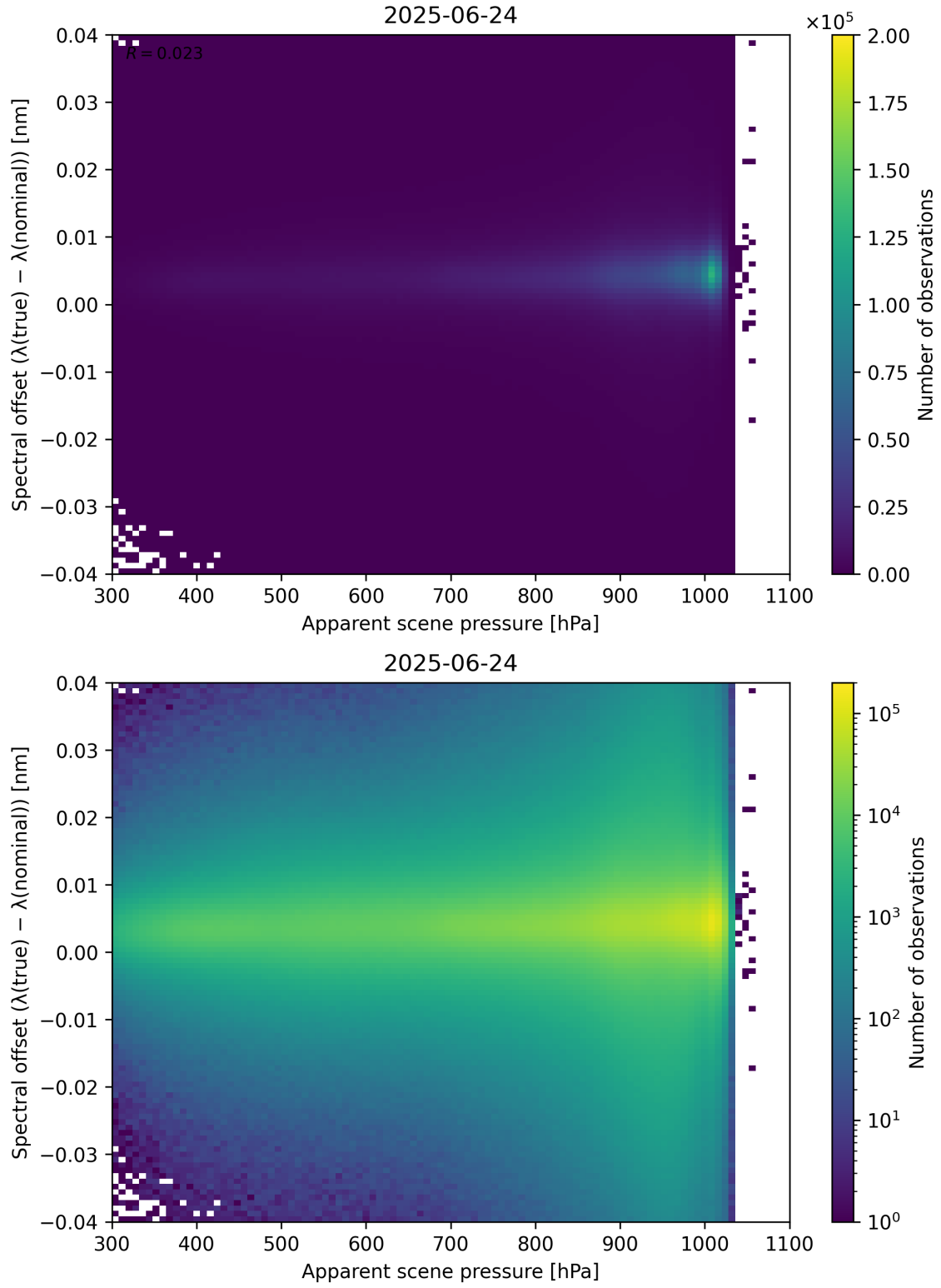
Figure 67: Scatter density plot of “Apparent scene pressure” against “Spectral offset ( \lambda_{\text{true}} - \lambda_{\text{nominal}} )” for 2025-06-23 to 2025-06-25.
