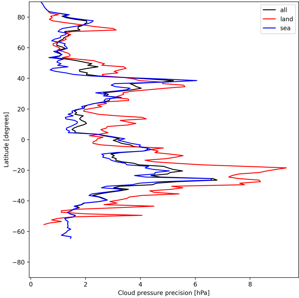
Figure 14: Zonal average of “Cloud pressure precision” for 2025-06-23 to 2025-06-25.
