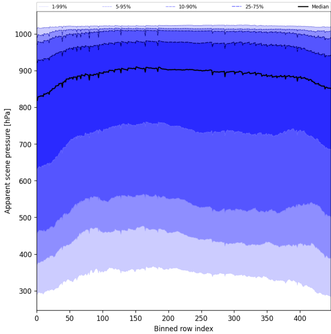
Figure 53: Along track statistics of “Apparent scene pressure” for 2025-06-23 to 2025-06-25
