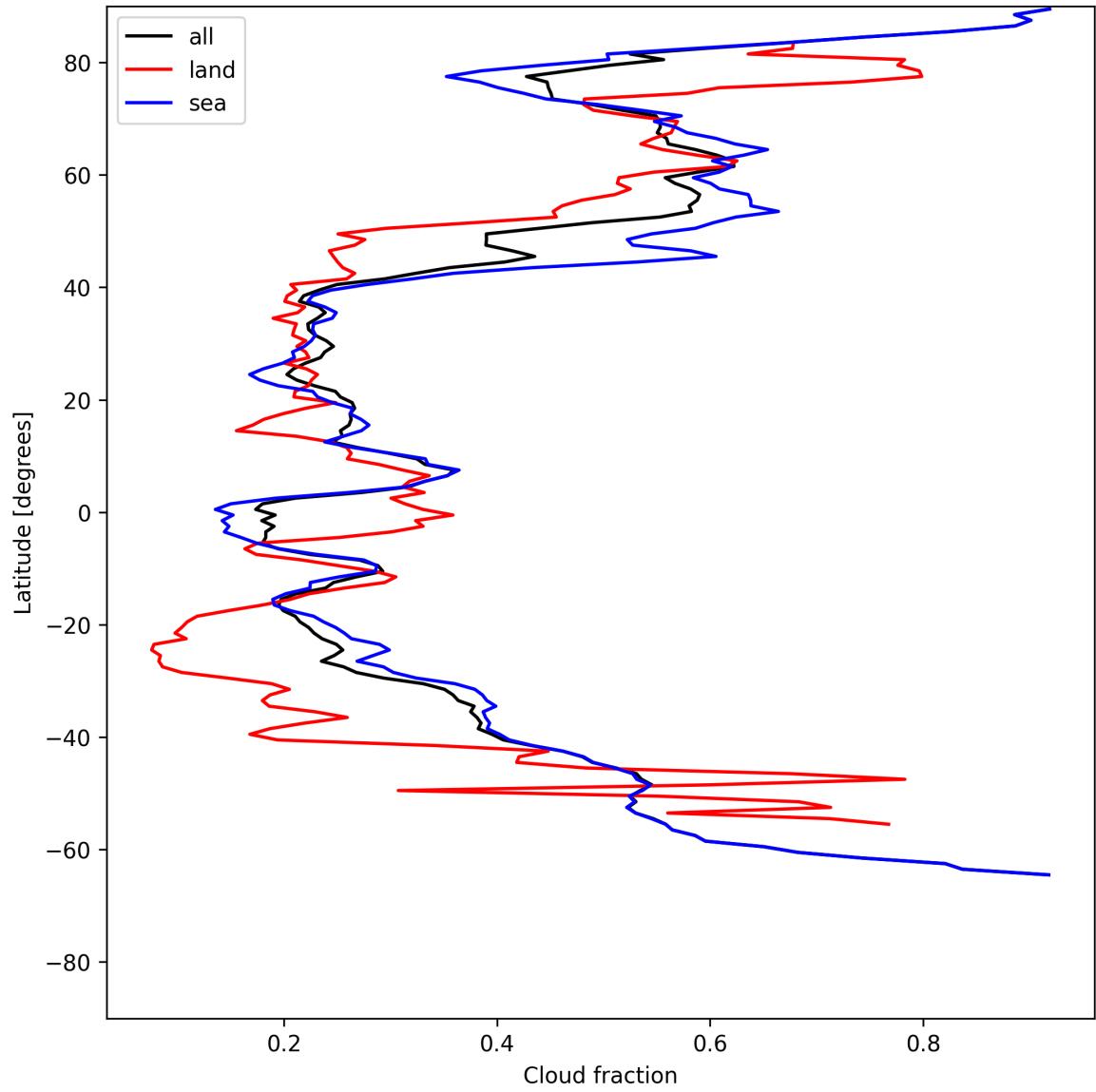
Figure 15: Zonal average of “Cloud fraction” for 2025-06-23 to 2025-06-25.
