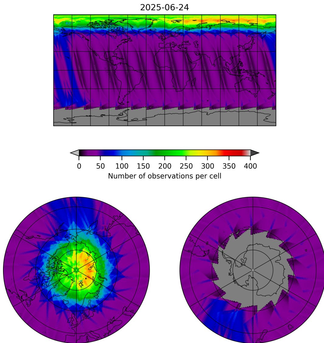
Figure 11: Map of the number of observations for 2025-06-23 to 2025-06-25
