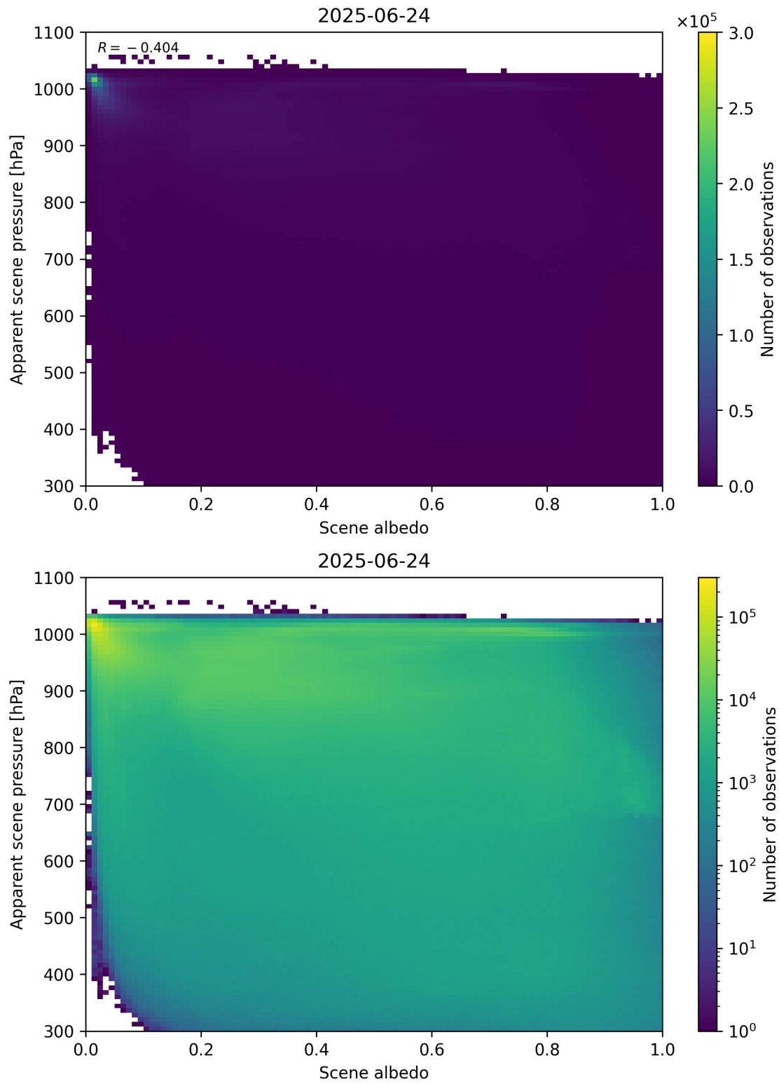
Figure 102: Scatter density plot of “Scene albedo” against “Apparent scene pressure” for 2025-06-23 to 2025-06-25.
