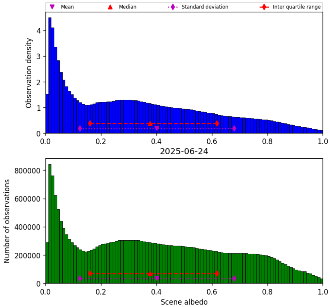
Figure 34: Histogram of “Scene albedo” for 2025-06-23 to 2025-06-25
