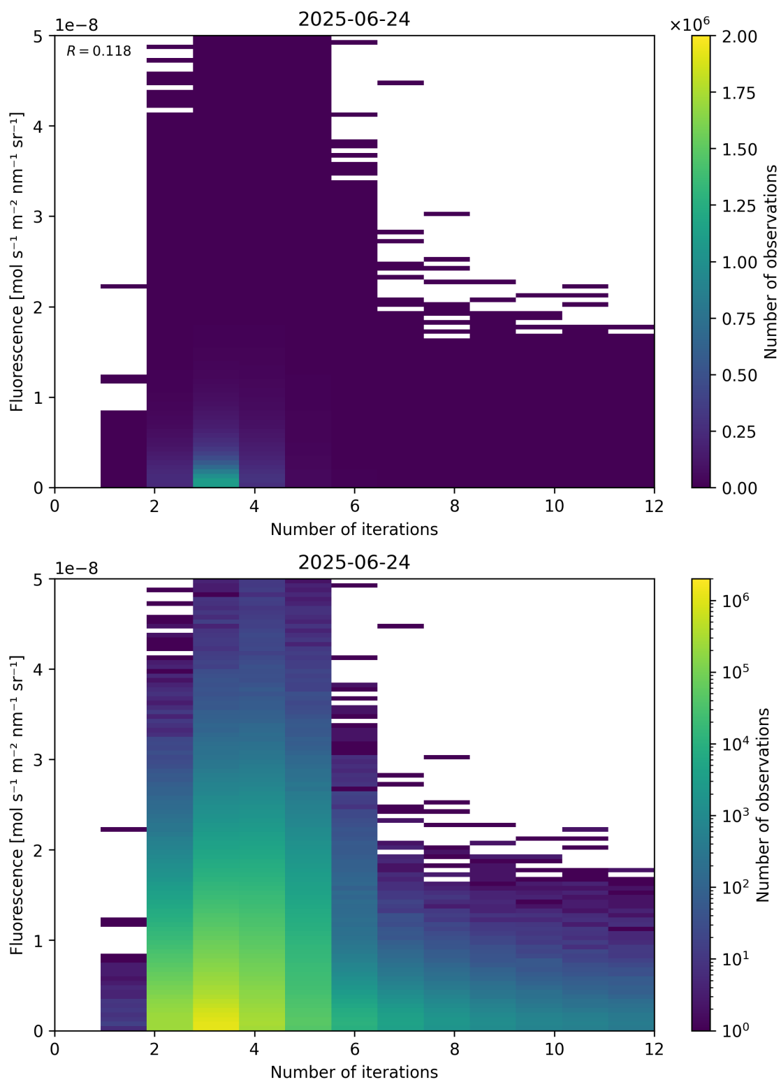
Figure 98: Scatter density plot of “Number of iterations” against “Fluorescence” for 2025-06-23 to 2025-06-25.
