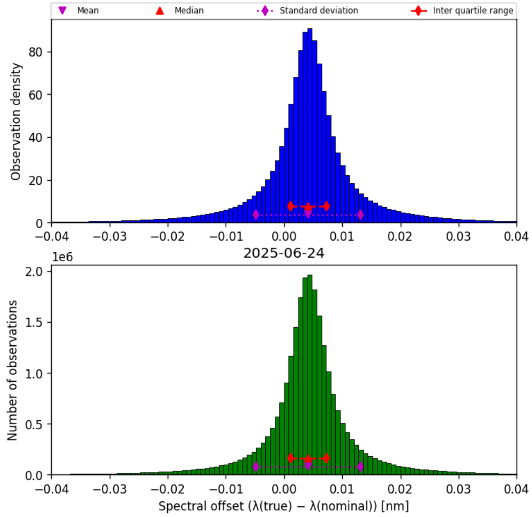
Figure 45: Histogram of “Spectral offset ( \lambda_{\text{true}} - \lambda_{\text{nominal}} )” for 2025-06-23 to 2025-06-25
