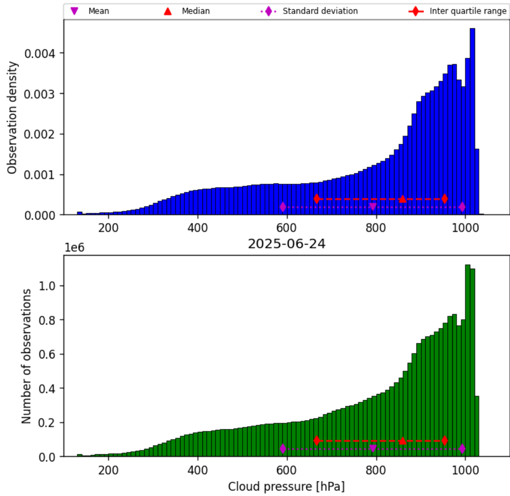
Figure 30: Histogram of “Cloud pressure” for 2025-06-23 to 2025-06-25
