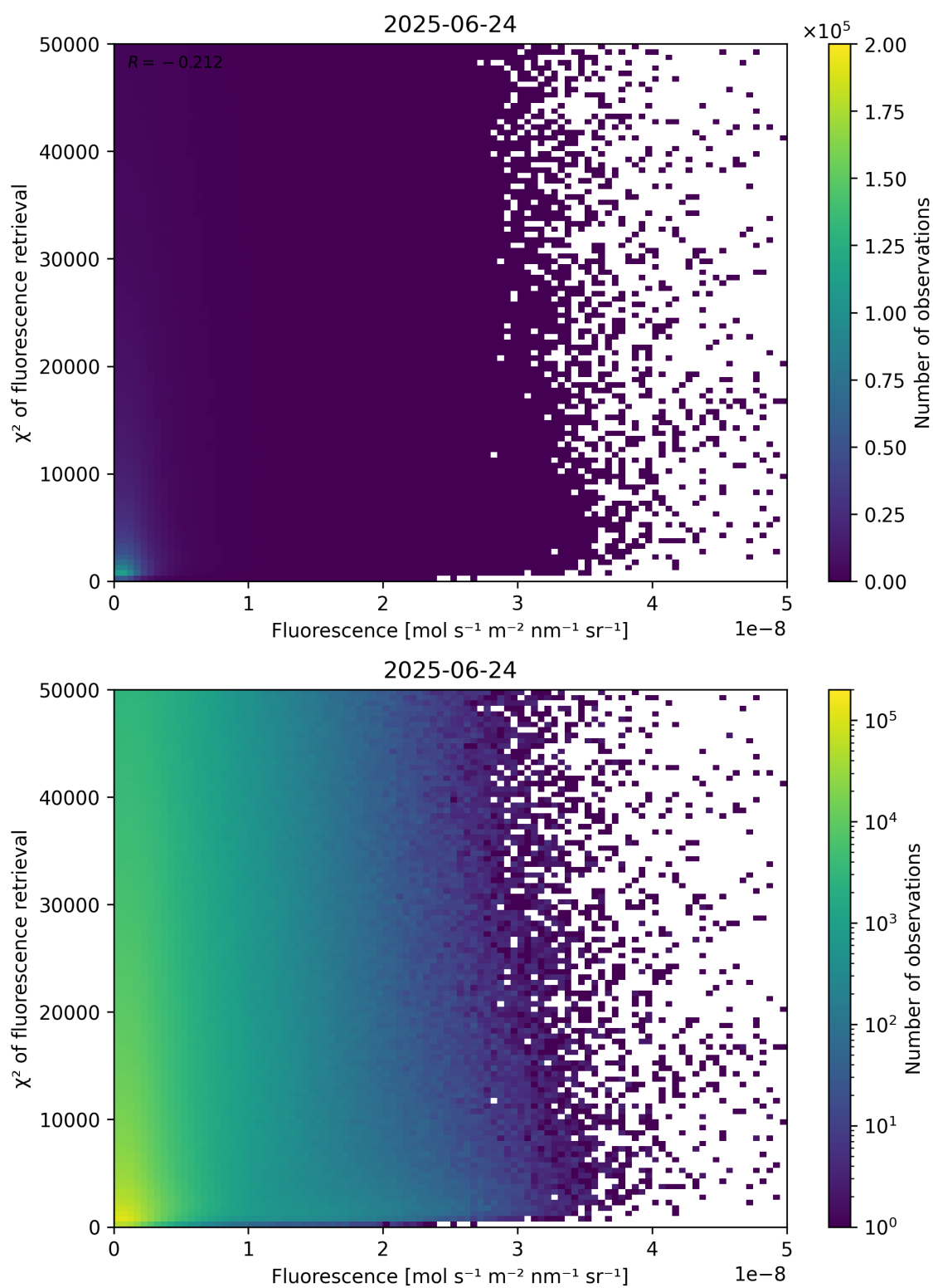
Figure 85: Scatter density plot of “Fluorescence” against “ \chi^2 of fluorescence retrieval” for 2025-06-23 to 2025-06-25.
