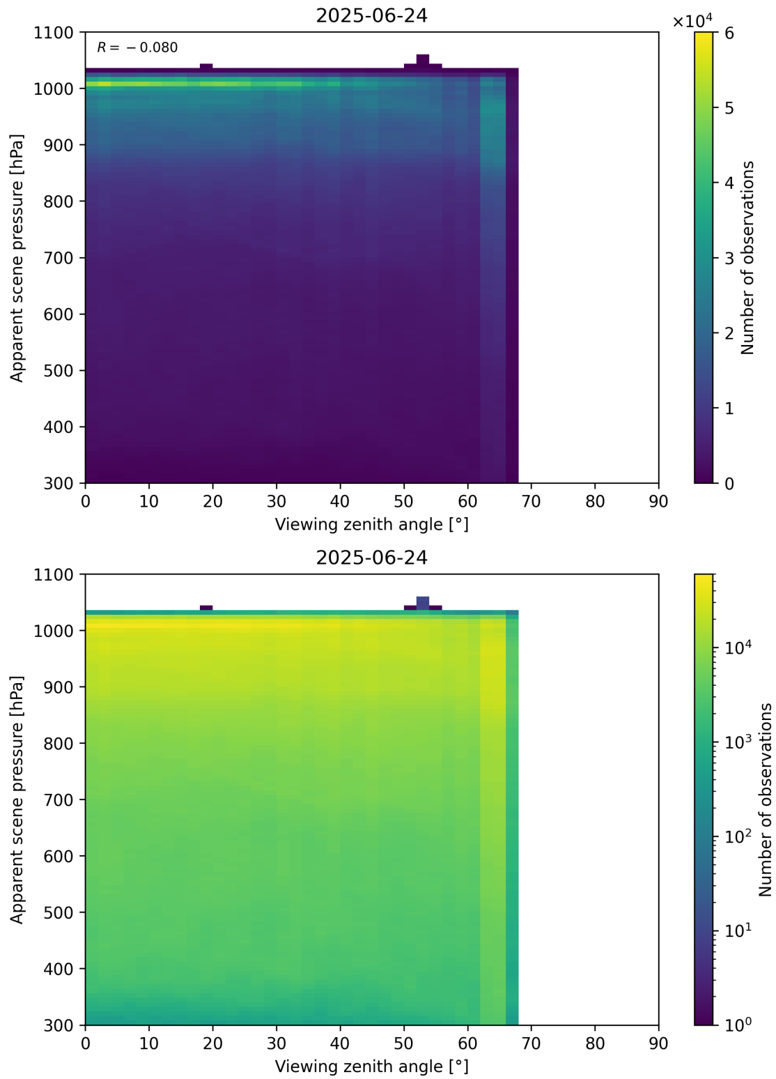
Figure 118: Scatter density plot of “Viewing zenith angle” against “Apparent scene pressure” for 2025-06-23 to 2025-06-25.
