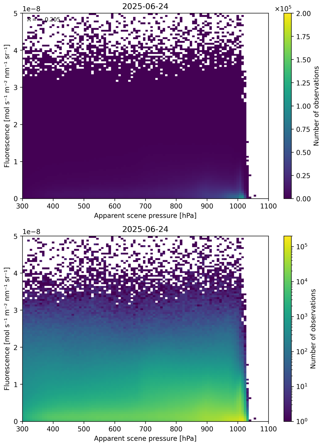
Figure 64: Scatter density plot of “Apparent scene pressure” against “Fluorescence” for 2025-06-23 to 2025-06-25.
