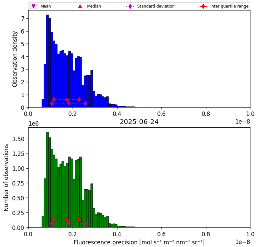
Figure 41: Histogram of “Fluorescence precision” for 2025-06-23 to 2025-06-25
