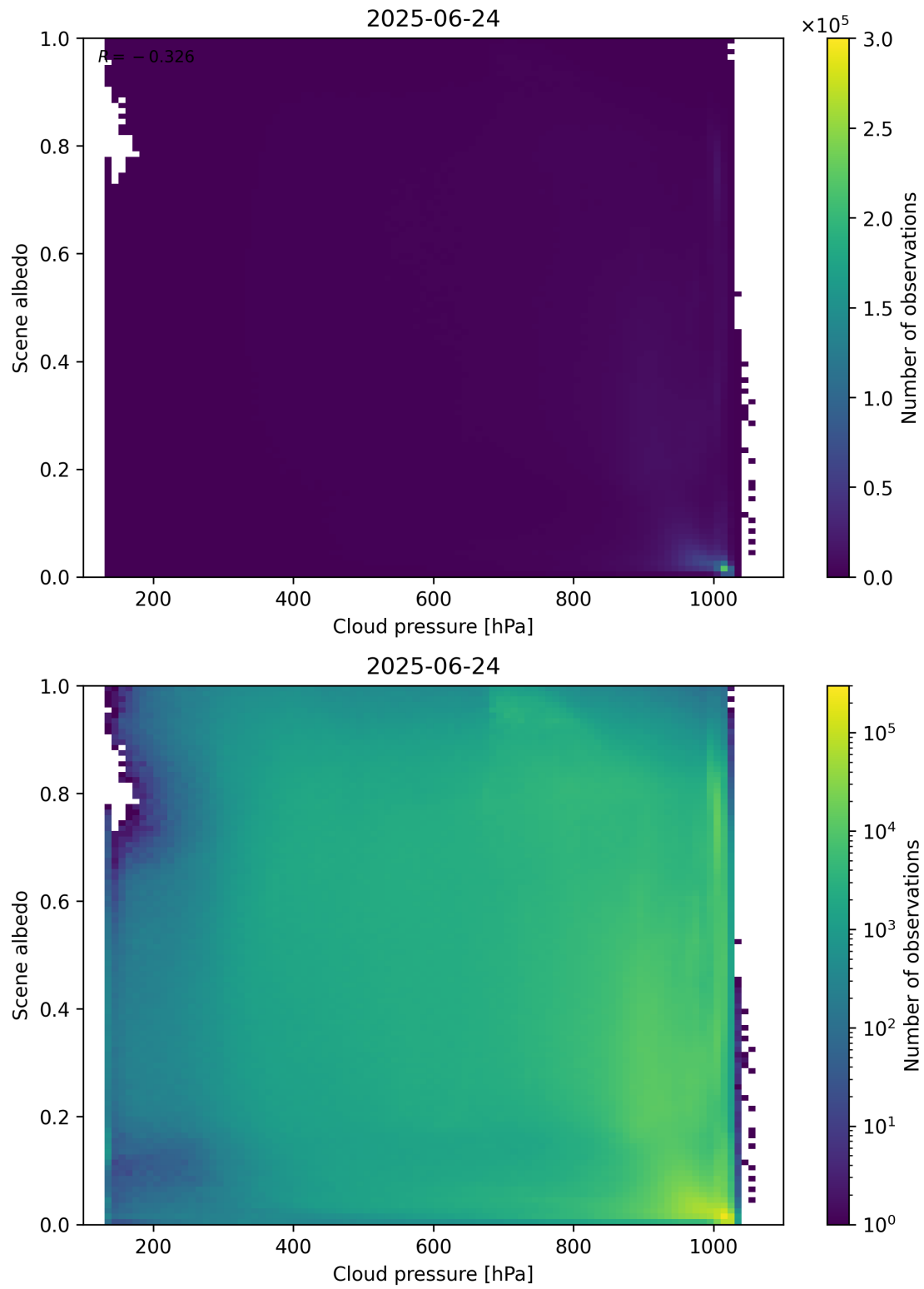
Figure 83: Scatter density plot of “Cloud pressure” against “Scene albedo” for 2025-06-23 to 2025-06-25.
