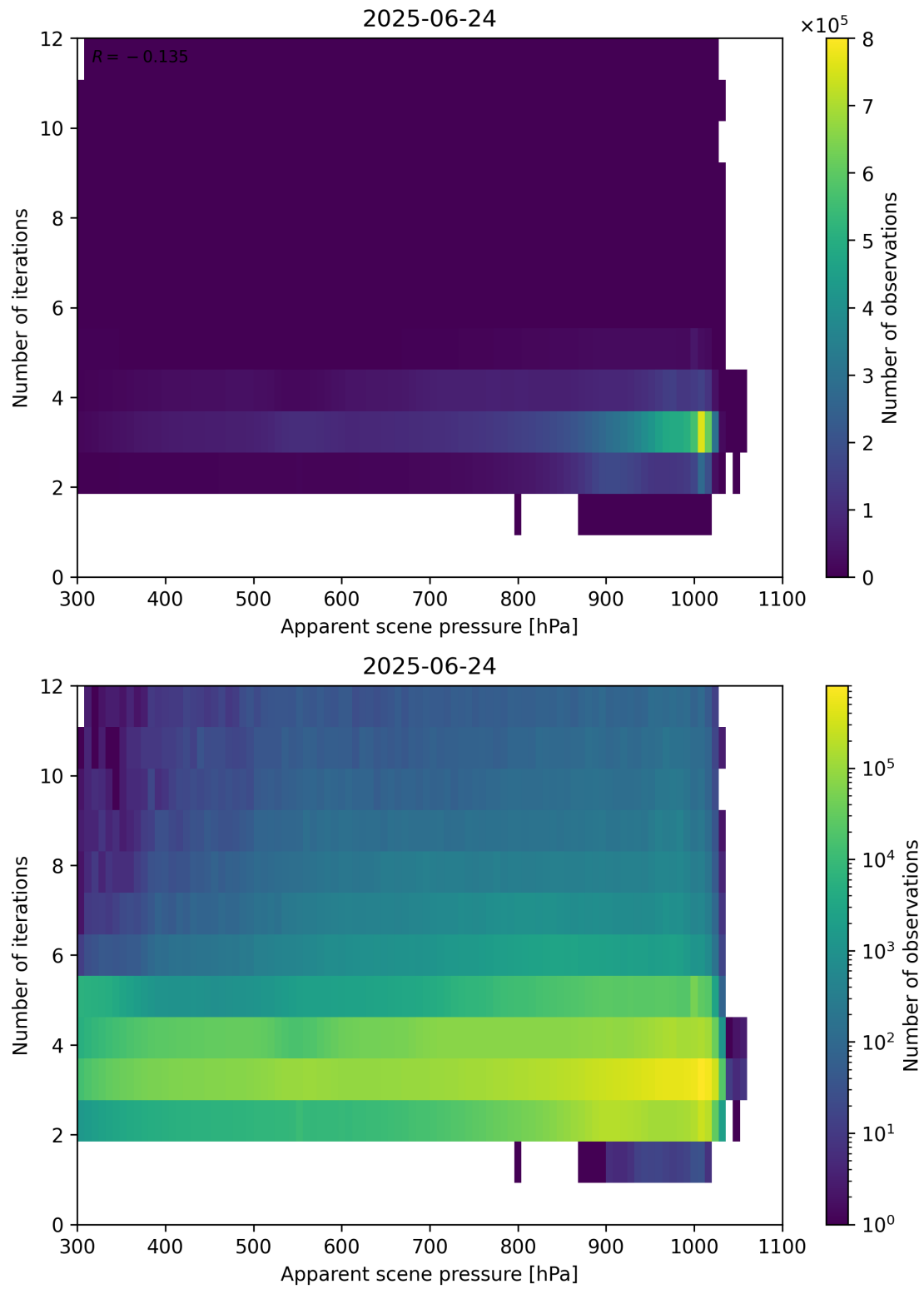
Figure 65: Scatter density plot of “Apparent scene pressure” against “Number of iterations” for 2025-06-23 to 2025-06-25.
