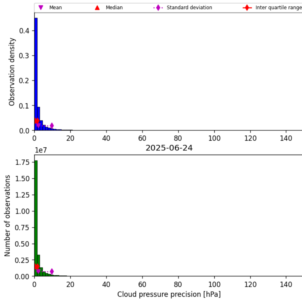
Figure 31: Histogram of “Cloud pressure precision” for 2025-06-23 to 2025-06-25
