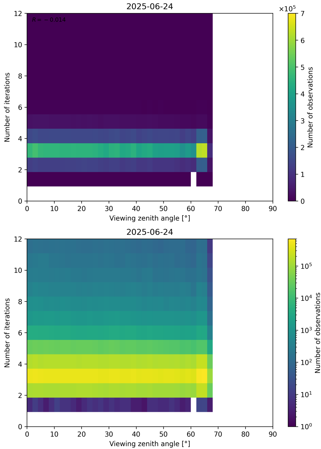
Figure 124: Scatter density plot of “Viewing zenith angle” against “Number of iterations” for 2025-06-23 to 2025-06-25.
