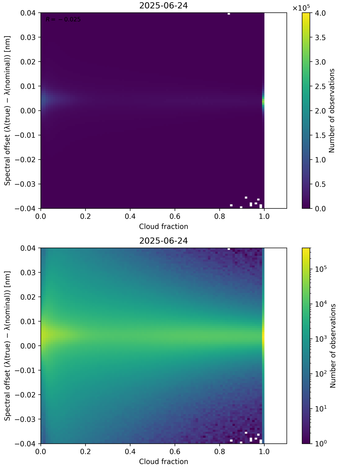
Figure 76: Scatter density plot of “Cloud fraction” against “Spectral offset ( \lambda_{\text{true}} - \lambda_{\text{nominal}} )” for 2025-06-23 to 2025-06-25.
