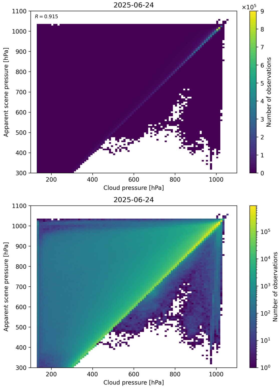
Figure 77: Scatter density plot of “Cloud pressure” against “Apparent scene pressure” for 2025-06-23 to 2025-06-25.
