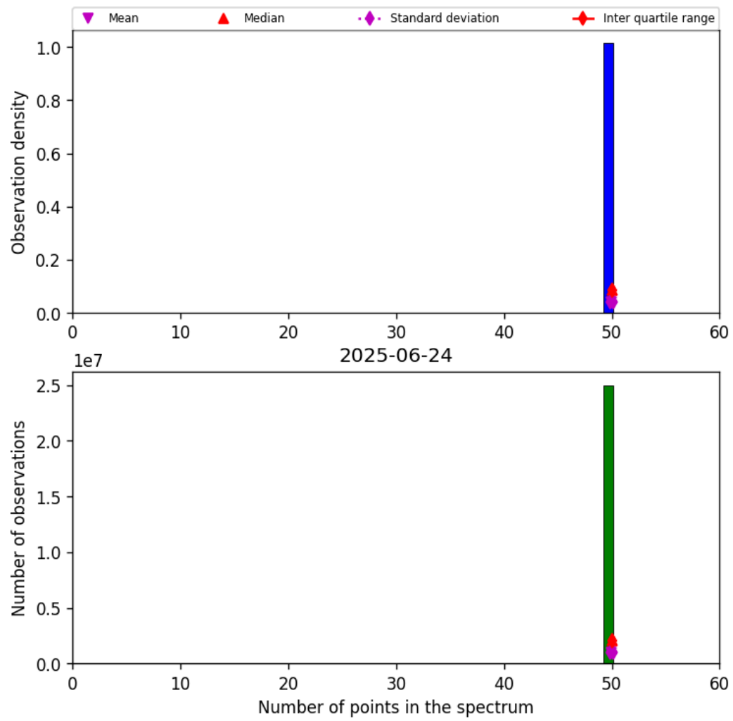
Figure 44: Histogram of “Number of points in the spectrum” for 2025-06-23 to 2025-06-25
