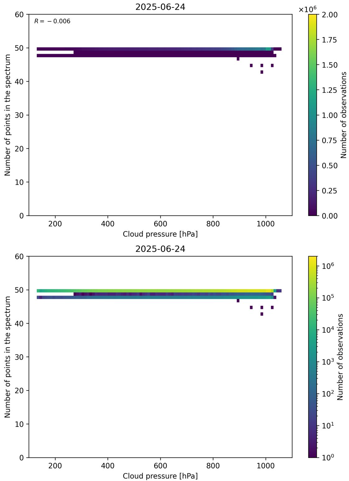
Figure 82: Scatter density plot of “Cloud pressure” against “Number of points in the spectrum” for 2025-06-23 to 2025-06-25.
