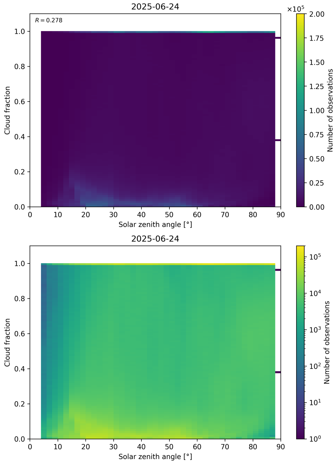
Figure 110: Scatter density plot of “Solar zenith angle” against “Cloud fraction” for 2025-06-23 to 2025-06-25.
