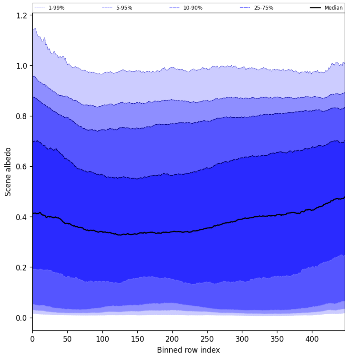
Figure 51: Along track statistics of “Scene albedo” for 2025-06-23 to 2025-06-25
