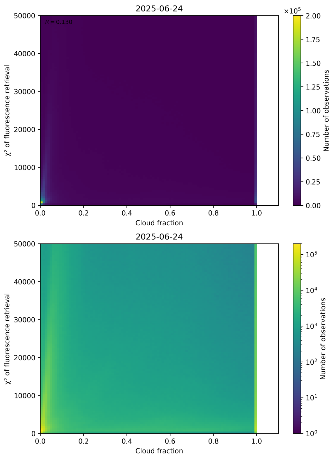
Figure 71: Scatter density plot of “Cloud fraction” against “ \chi^2 of fluorescence retrieval” for 2025-06-23 to 2025-06-25.
