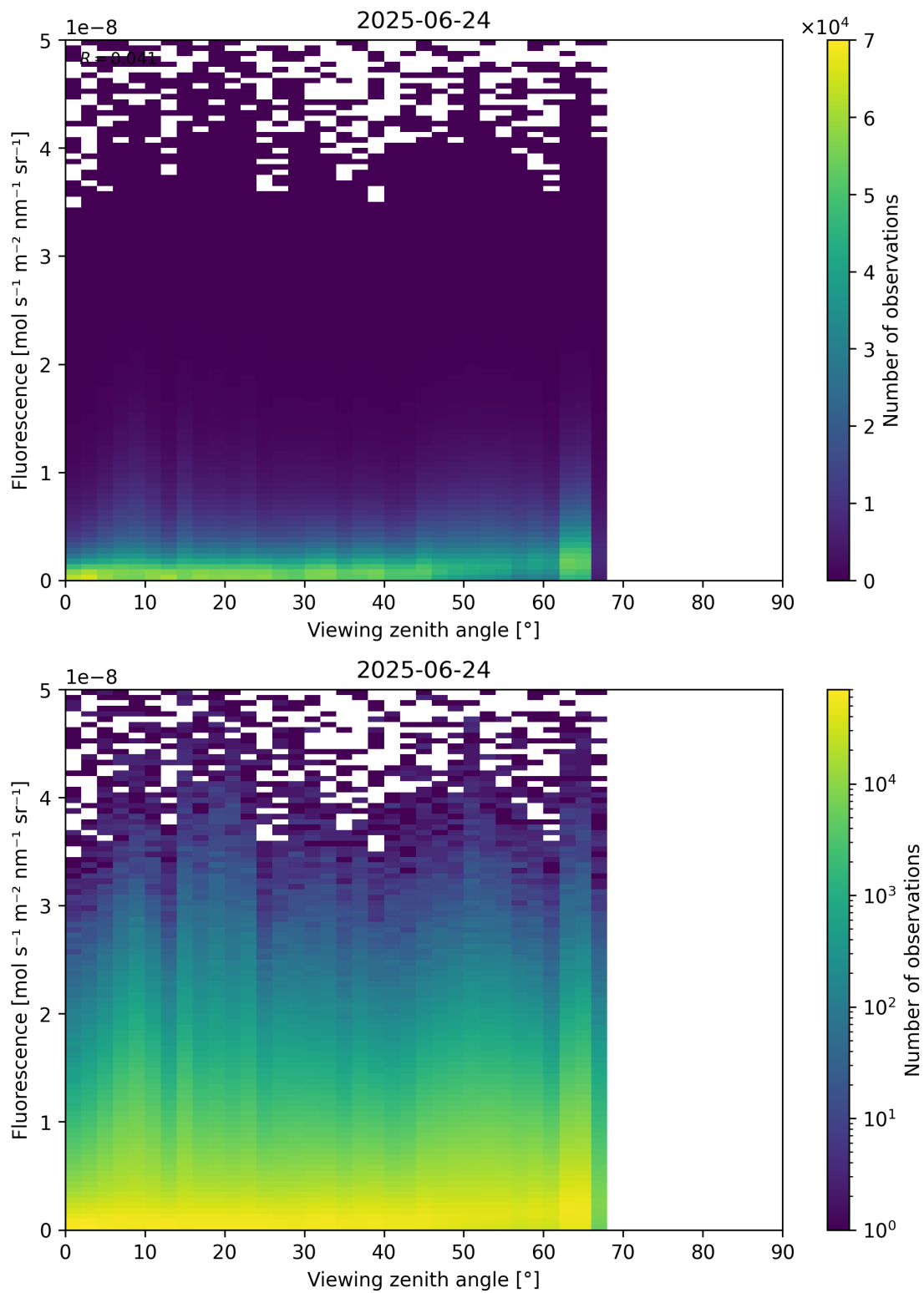
Figure 122: Scatter density plot of “Viewing zenith angle” against “Fluorescence” for 2025-06-23 to 2025-06-25.
