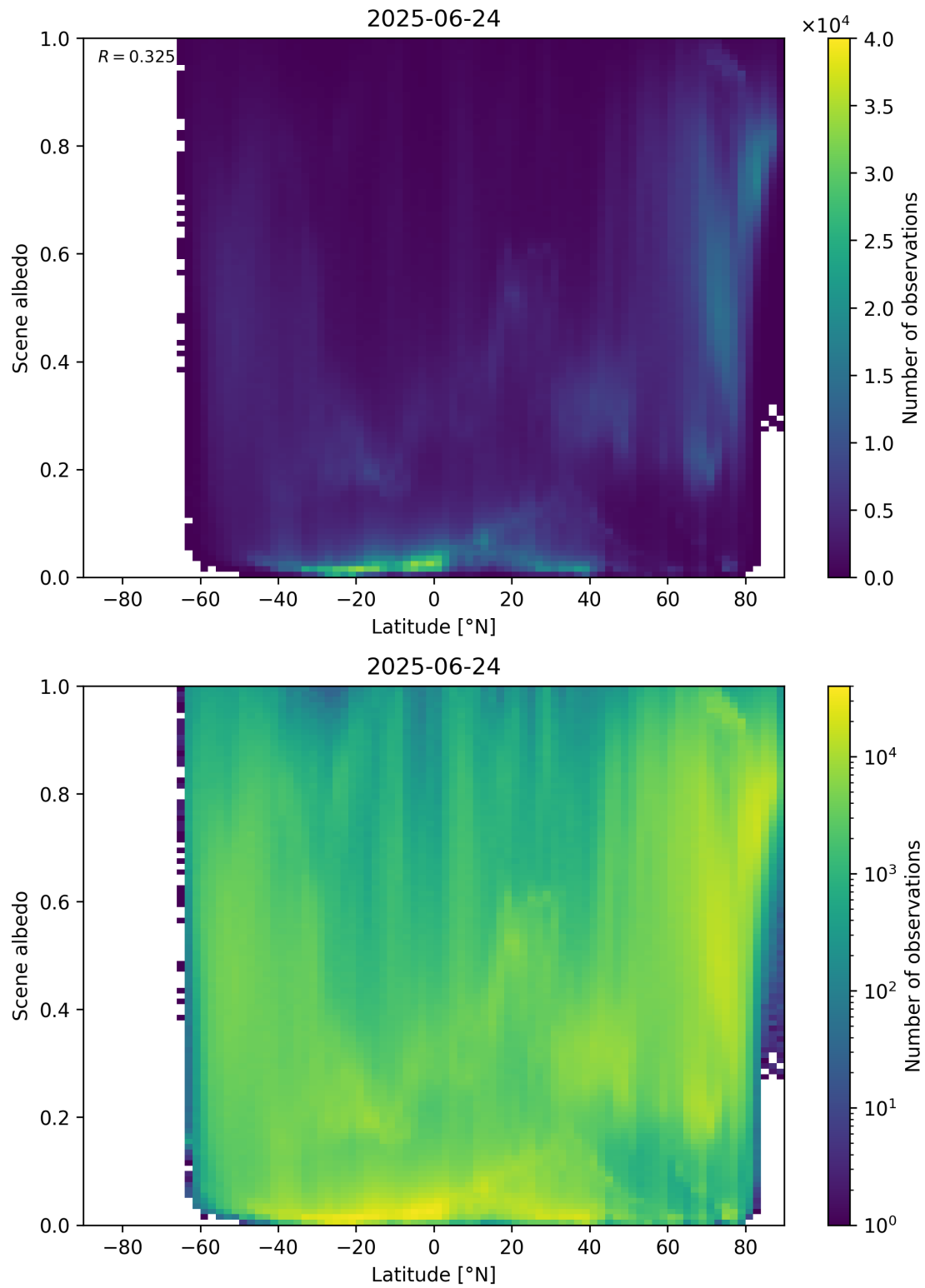
Figure 95: Scatter density plot of “Latitude” against “Scene albedo” for 2025-06-23 to 2025-06-25.
