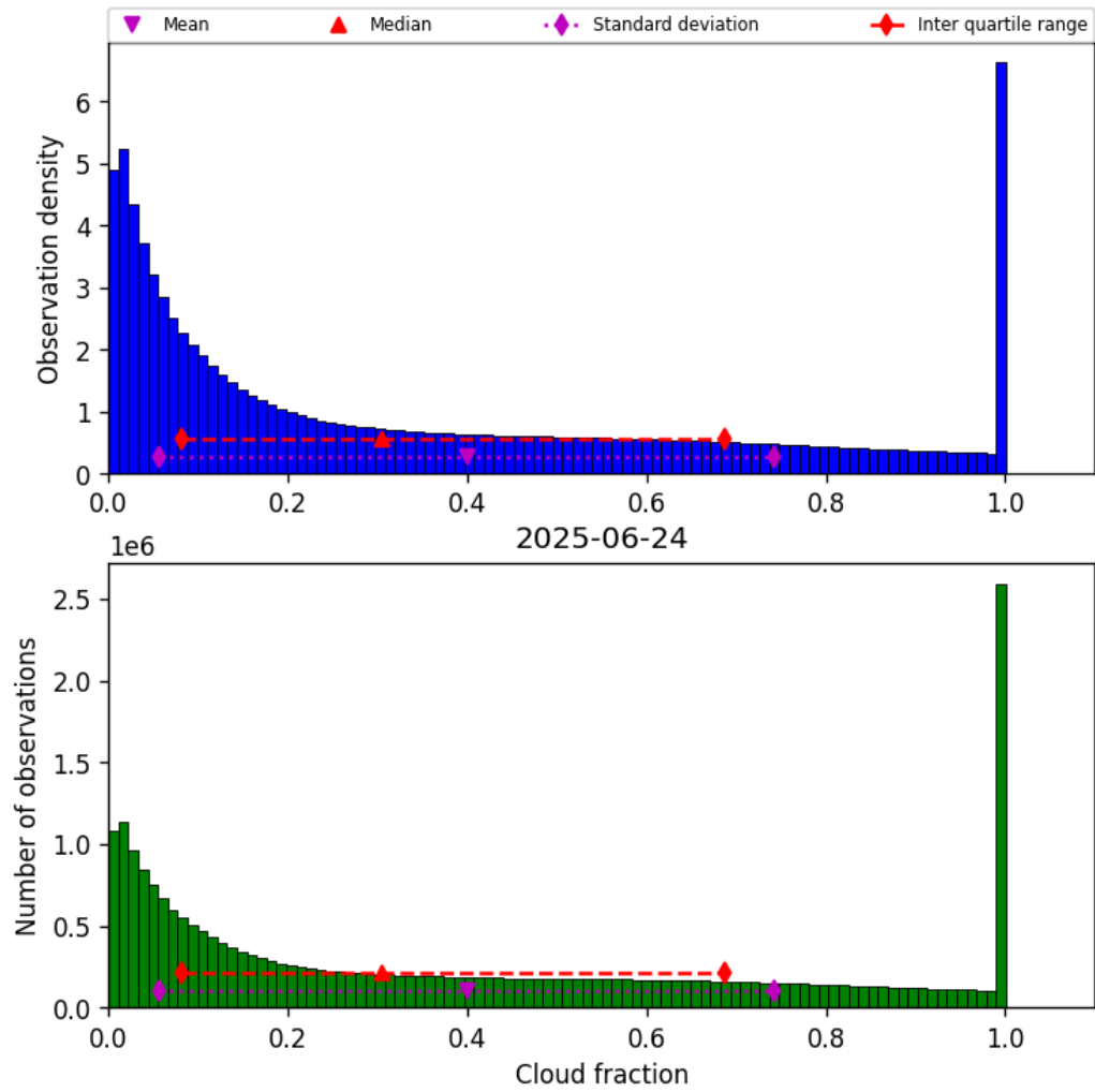
Figure 32: Histogram of “Cloud fraction” for 2025-06-23 to 2025-06-25
