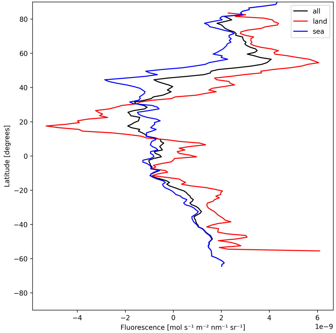
Figure 23: Zonal average of “Fluorescence” for 2025-06-23 to 2025-06-25.
