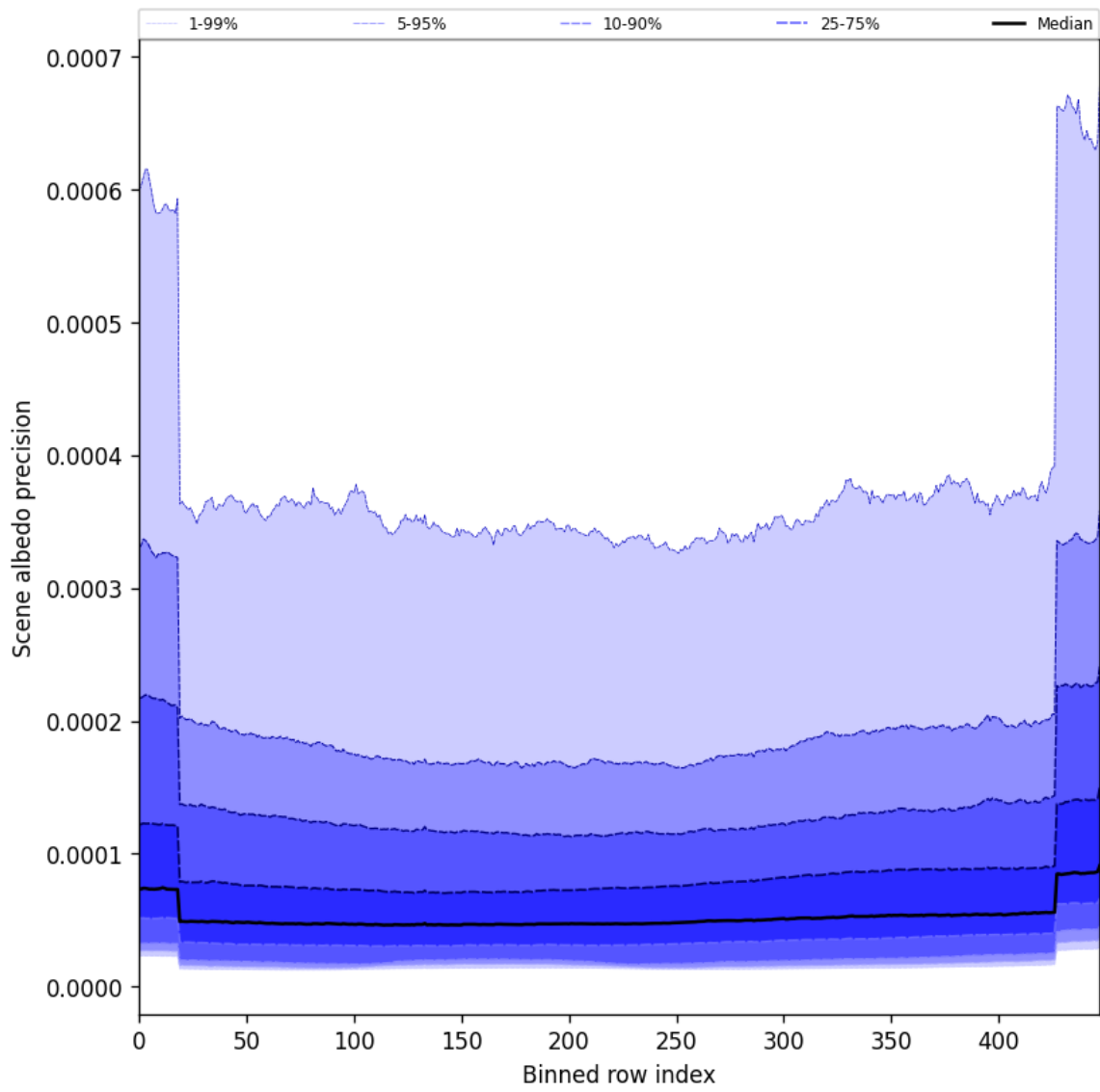
Figure 52: Along track statistics of “Scene albedo precision” for 2025-06-23 to 2025-06-25
