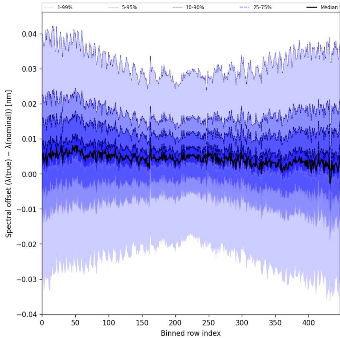
Figure 62: Along track statistics of “Spectral offset ( \lambda_{\text{true}} - \lambda_{\text{nominal}} )” for 2025-06-23 to 2025-06-25
