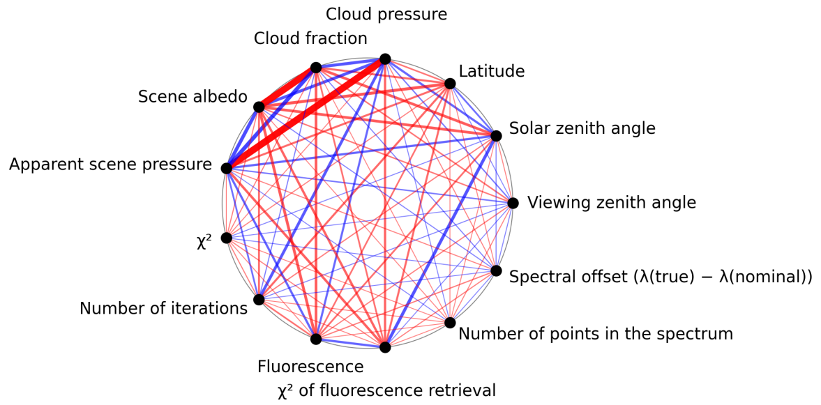
Figure 1: Map of correlation graph for 2025-06-23 to 2025-06-25.
