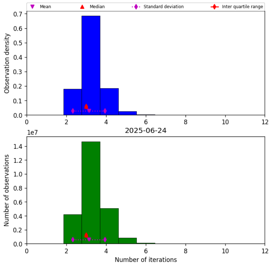
Figure 39: Histogram of “Number of iterations” for 2025-06-23 to 2025-06-25
