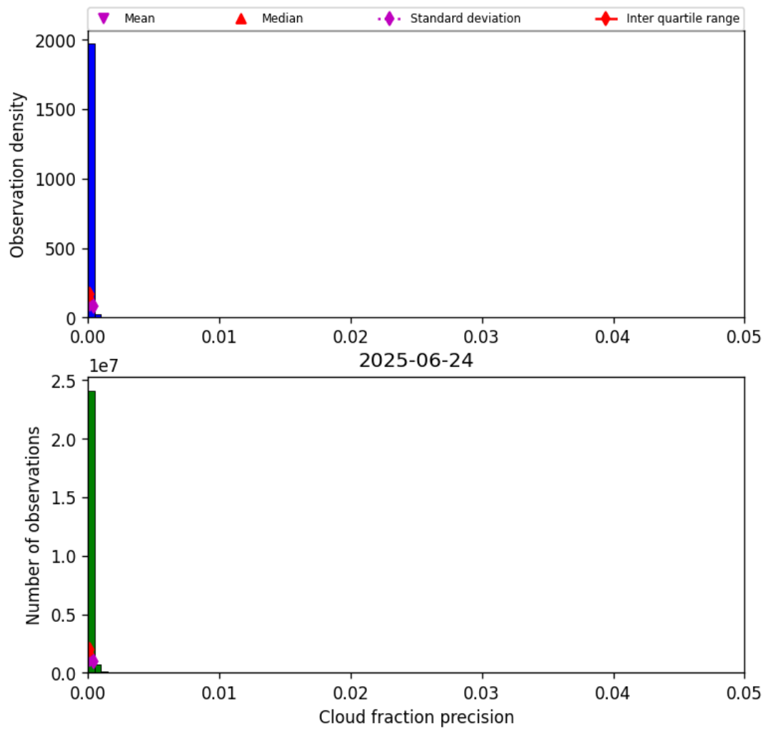
Figure 33: Histogram of “Cloud fraction precision” for 2025-06-23 to 2025-06-25
