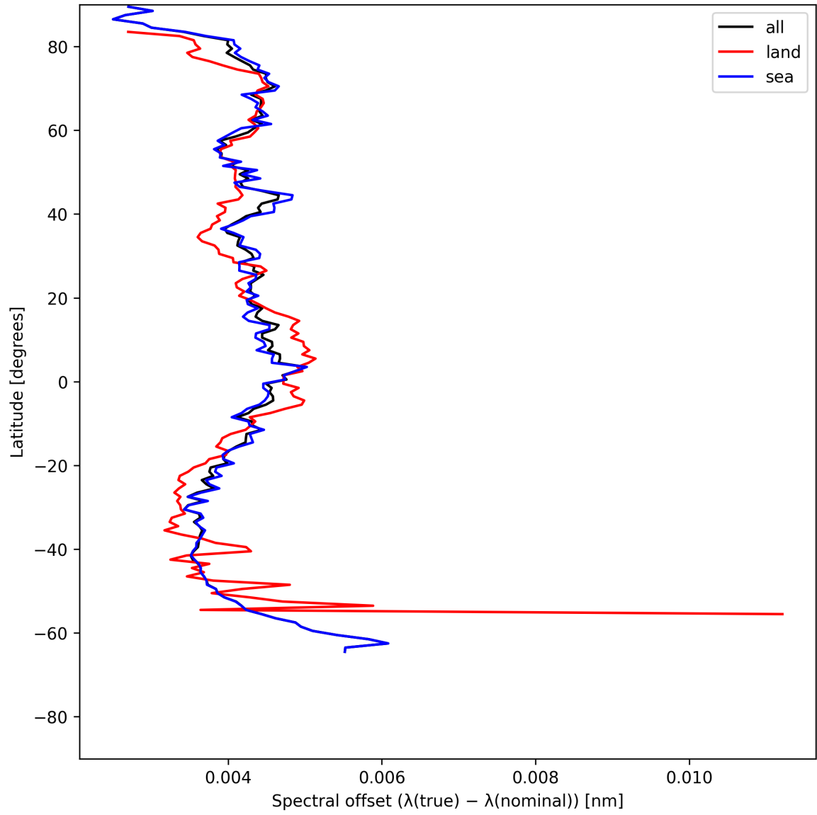
Figure 28: Zonal average of “Spectral offset ( \lambda_{\text{true}} - \lambda_{\text{nominal}} )” for 2025-06-23 to 2025-06-25.
