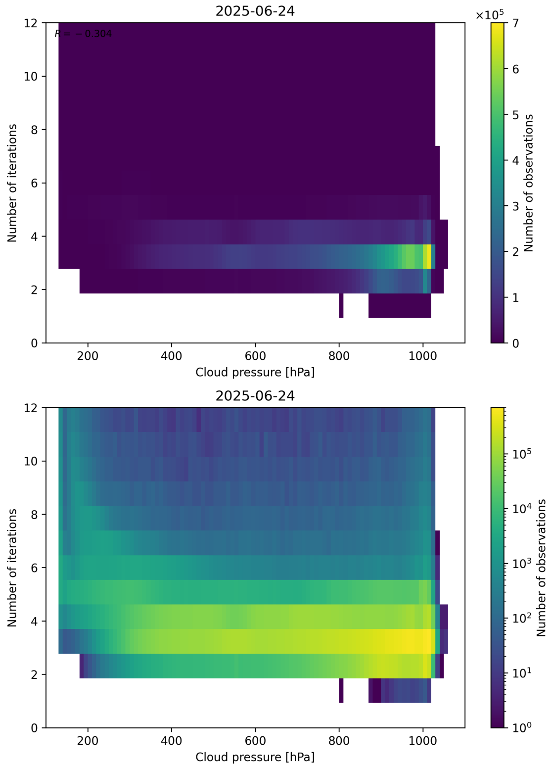
Figure 81: Scatter density plot of “Cloud pressure” against “Number of iterations” for 2025-06-23 to 2025-06-25.
