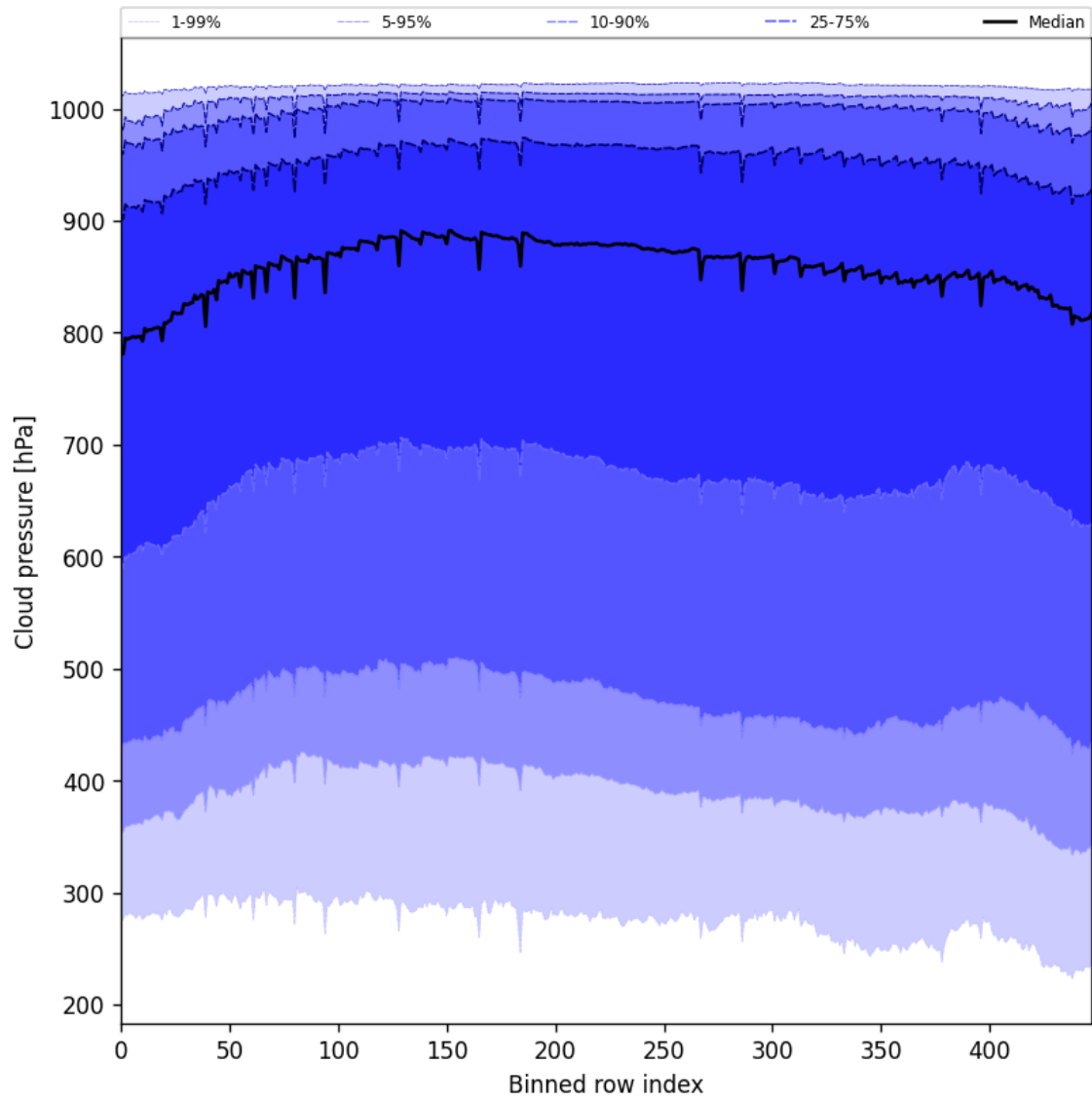
Figure 47: Along track statistics of “Cloud pressure” for 2025-06-23 to 2025-06-25
