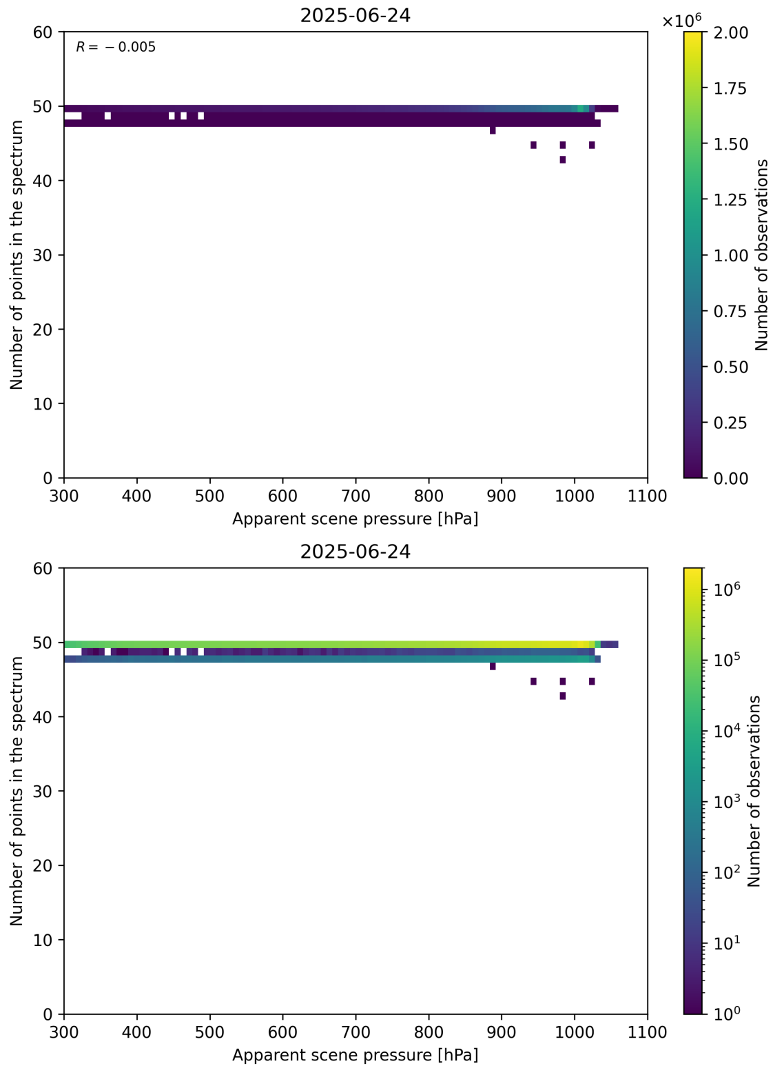
Figure 66: Scatter density plot of “Apparent scene pressure” against “Number of points in the spectrum” for 2025-06-23 to 2025-06-25.
