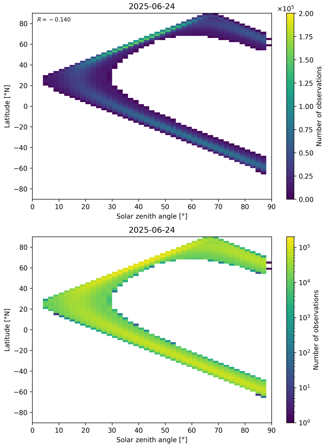
Figure 113: Scatter density plot of “Solar zenith angle” against “Latitude” for 2025-06-23 to 2025-06-25.
