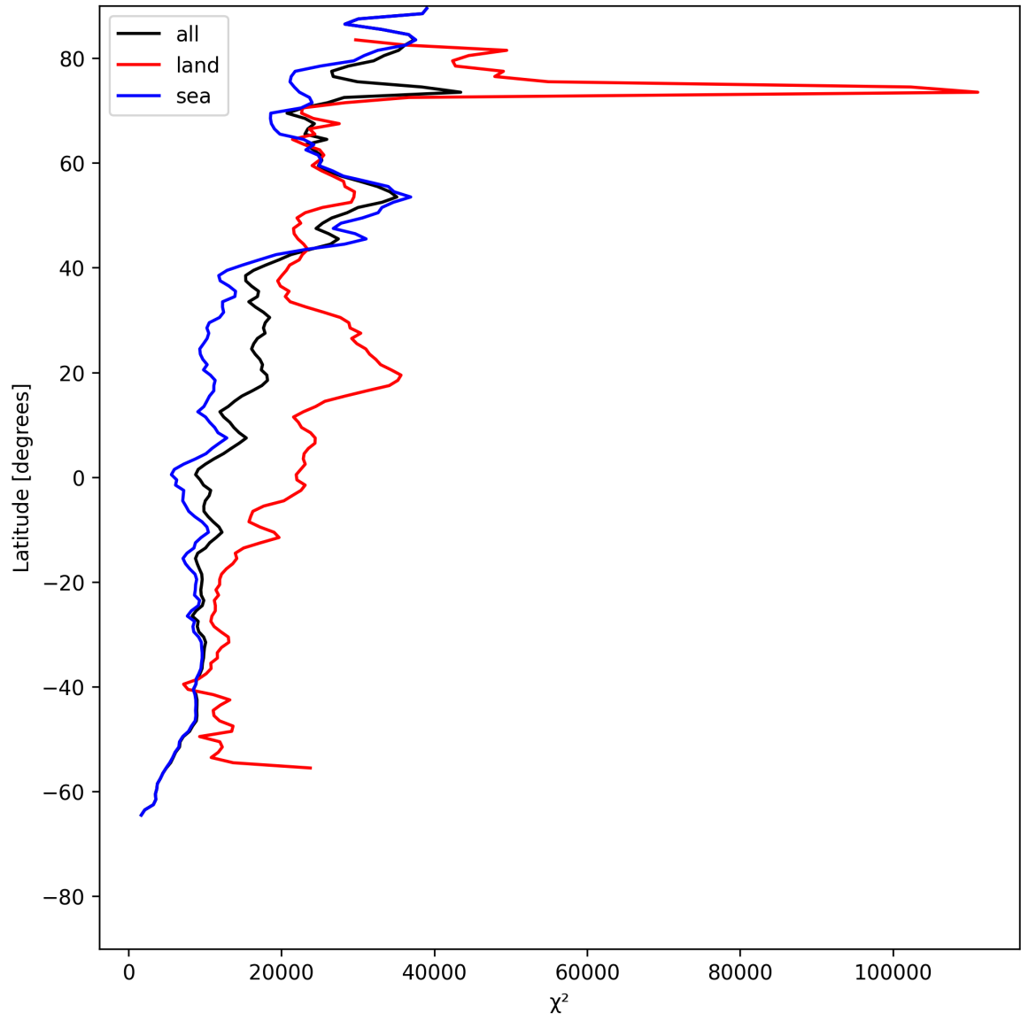
Figure 21: Zonal average of “ \chi^2 ” for 2025-06-23 to 2025-06-25.
