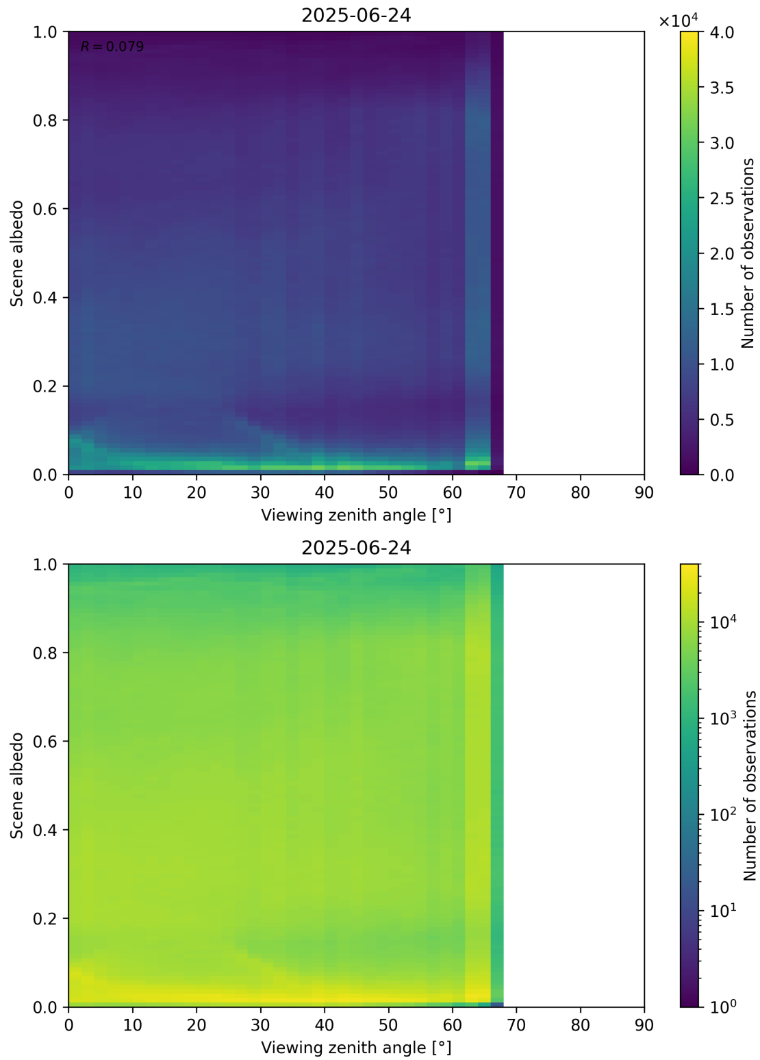
Figure 126: Scatter density plot of “Viewing zenith angle” against “Scene albedo” for 2025-06-23 to 2025-06-25.
