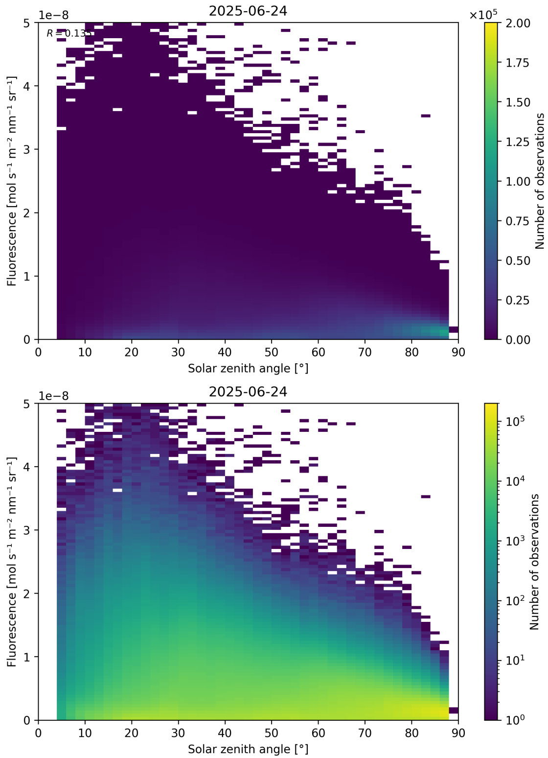
Figure 112: Scatter density plot of “Solar zenith angle” against “Fluorescence” for 2025-06-23 to 2025-06-25.
