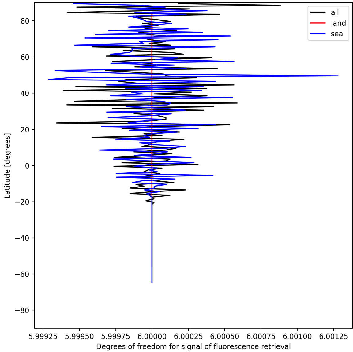
Figure 26: Zonal average of “Degrees of freedom for signal of fluorescence retrieval” for 2025-06-23 to 2025-06-25.
