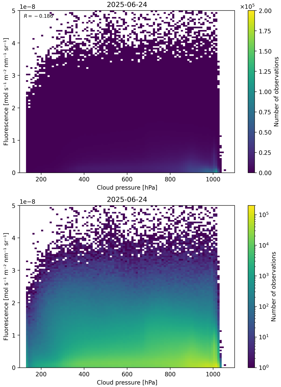
Figure 80: Scatter density plot of “Cloud pressure” against “Fluorescence” for 2025-06-23 to 2025-06-25.
