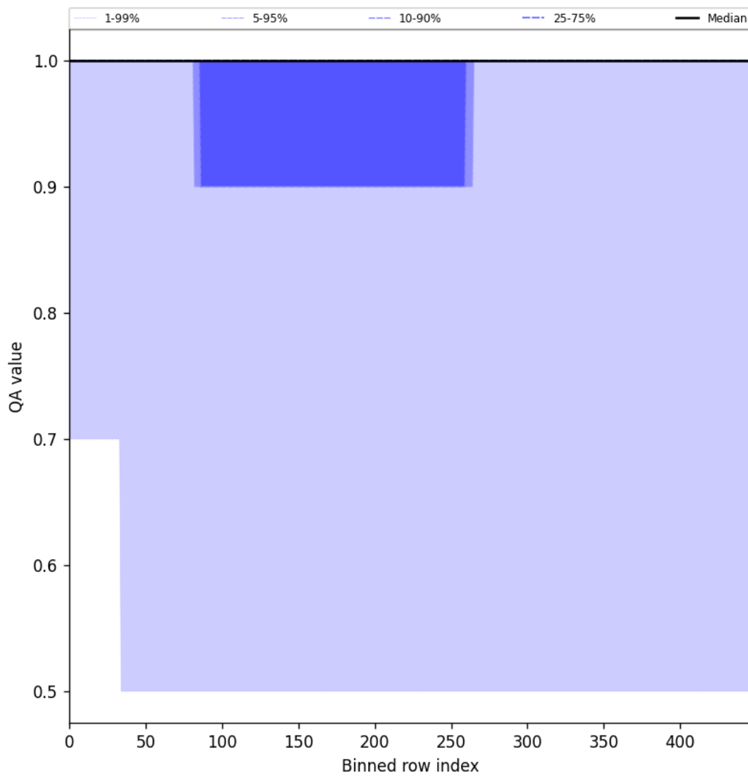
Figure 46: Along track statistics of “QA value” for 2025-06-23 to 2025-06-25
