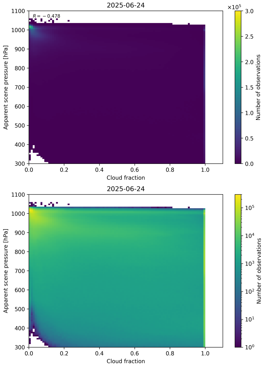
Figure 70: Scatter density plot of “Cloud fraction” against “Apparent scene pressure” for 2025-06-23 to 2025-06-25.
