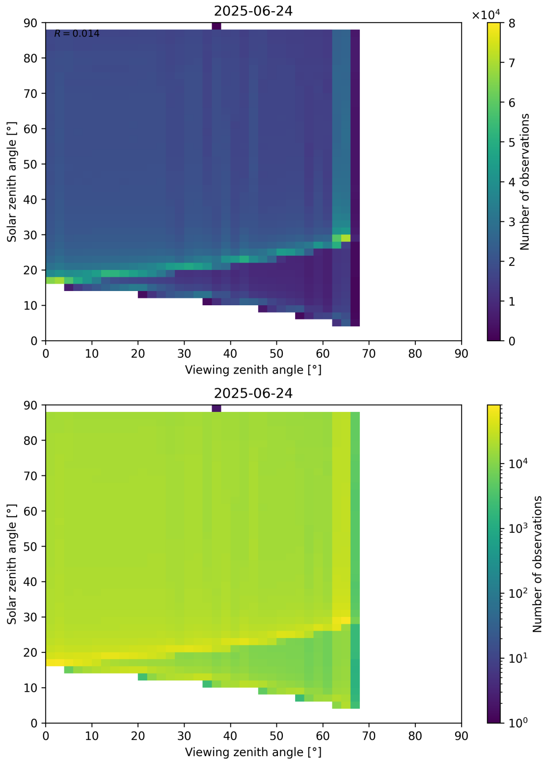
Figure 127: Scatter density plot of “Viewing zenith angle” against “Solar zenith angle” for 2025-06-23 to 2025-06-25.
