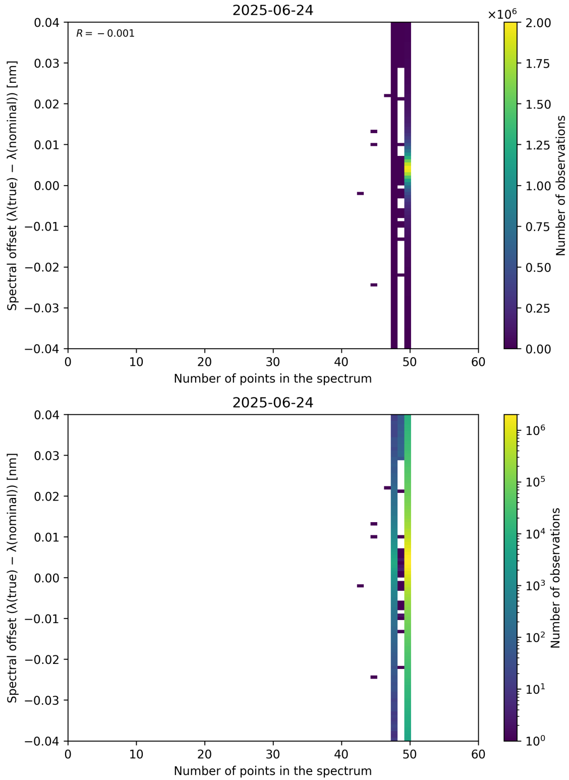
Figure 101: Scatter density plot of “Number of points in the spectrum” against “Spectral offset ( \lambda_{\text{true}} - \lambda_{\text{nominal}} )” for 2025-06-23 to 2025-06-25.
