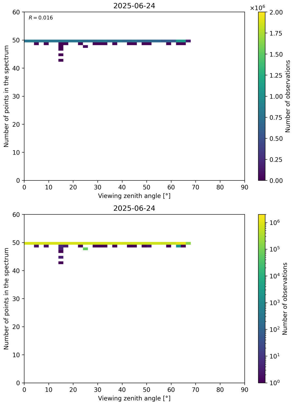
Figure 125: Scatter density plot of “Viewing zenith angle” against “Number of points in the spectrum” for 2025-06-23 to 2025-06-25.
