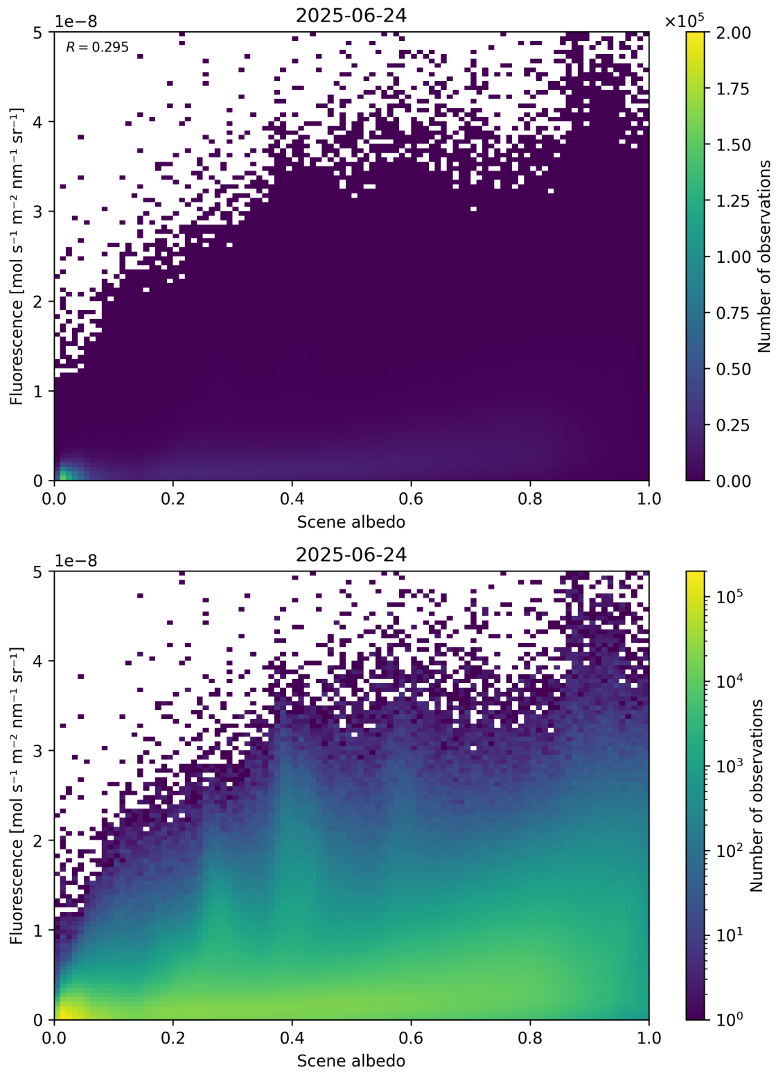
Figure 104: Scatter density plot of “Scene albedo” against “Fluorescence” for 2025-06-23 to 2025-06-25.
