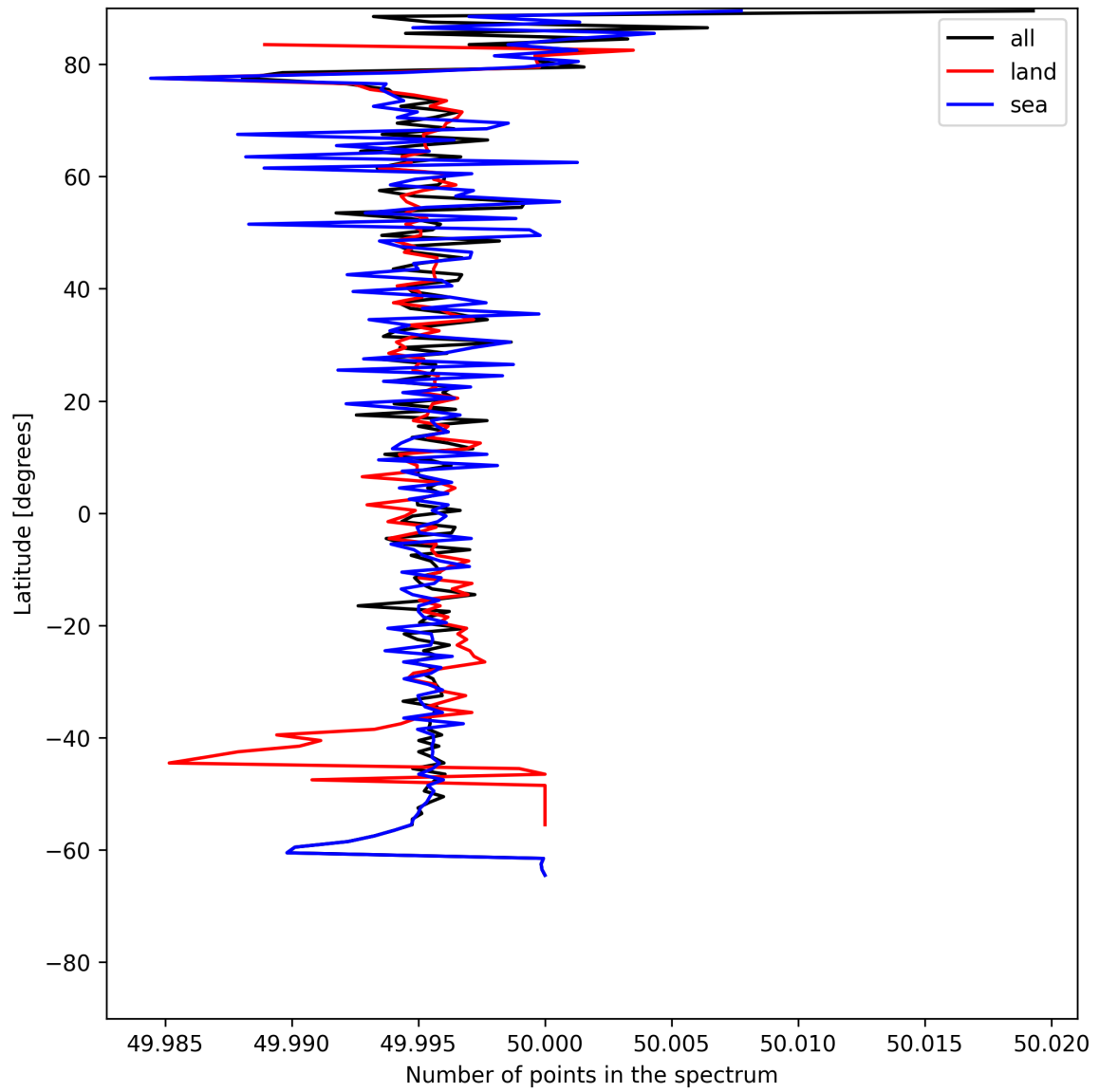
Figure 27: Zonal average of “Number of points in the spectrum” for 2025-06-23 to 2025-06-25.
