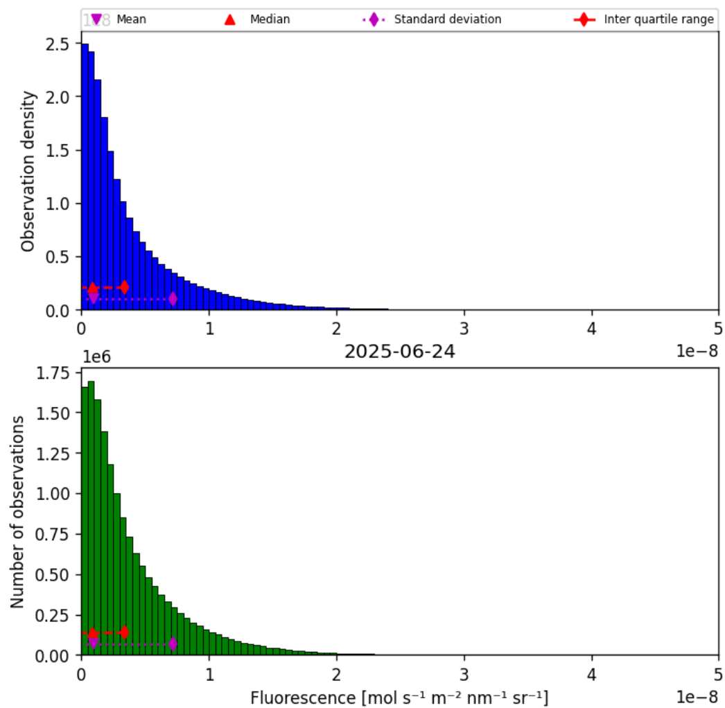
Figure 40: Histogram of “Fluorescence” for 2025-06-23 to 2025-06-25
