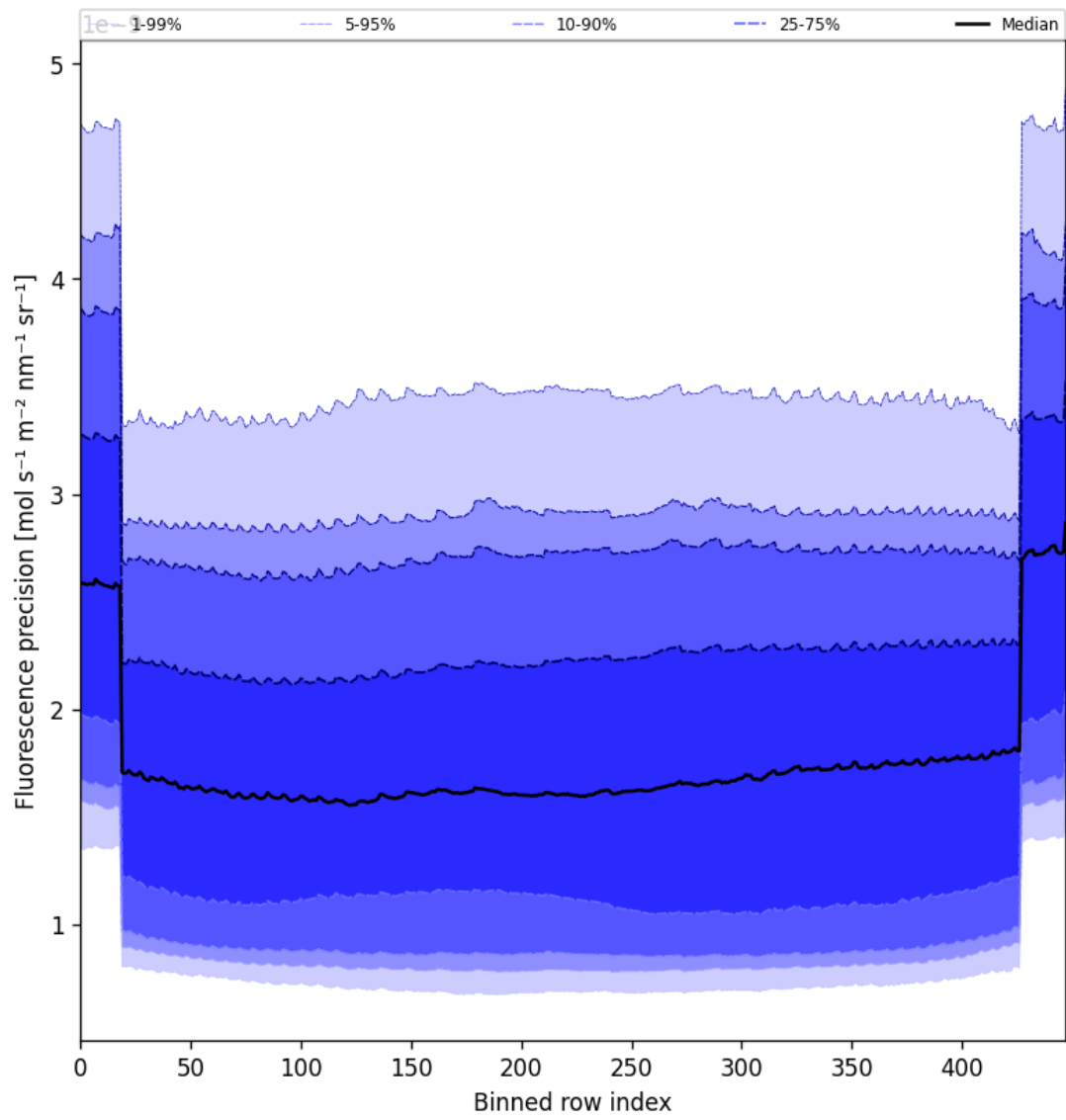
Figure 58: Along track statistics of “Fluorescence precision” for 2025-06-23 to 2025-06-25
