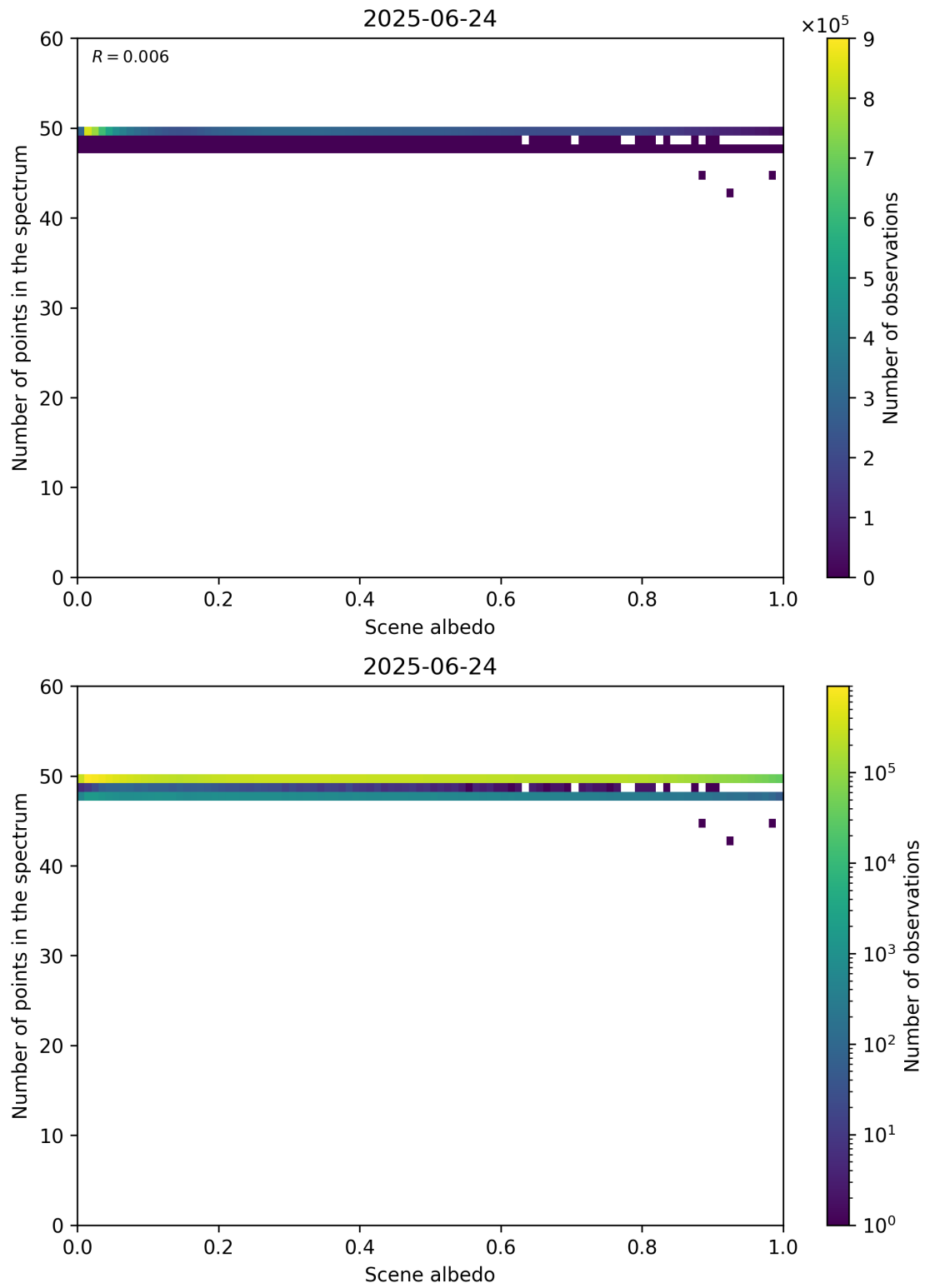
Figure 106: Scatter density plot of “Scene albedo” against “Number of points in the spectrum” for 2025-06-23 to 2025-06-25.
