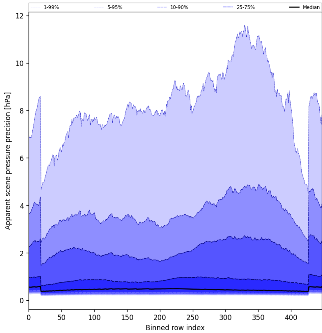
Figure 54: Along track statistics of “Apparent scene pressure precision” for 2025-06-23 to 2025-06-25
