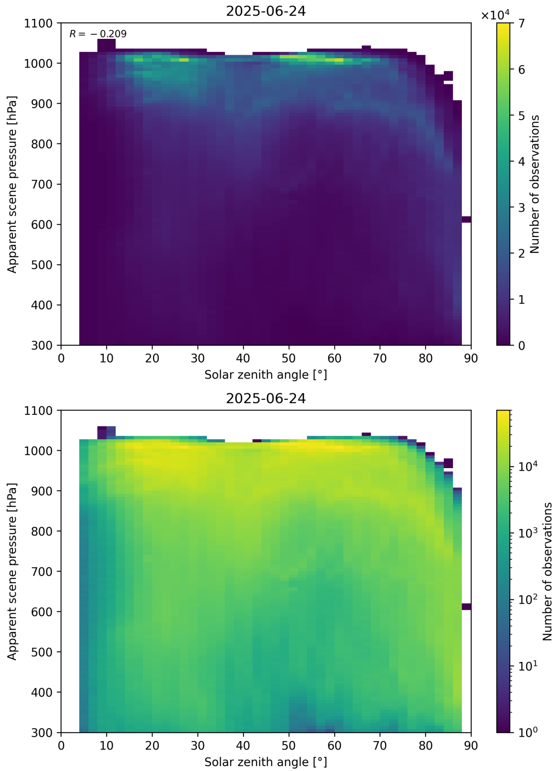
Figure 108: Scatter density plot of “Solar zenith angle” against “Apparent scene pressure” for 2025-06-23 to 2025-06-25.
