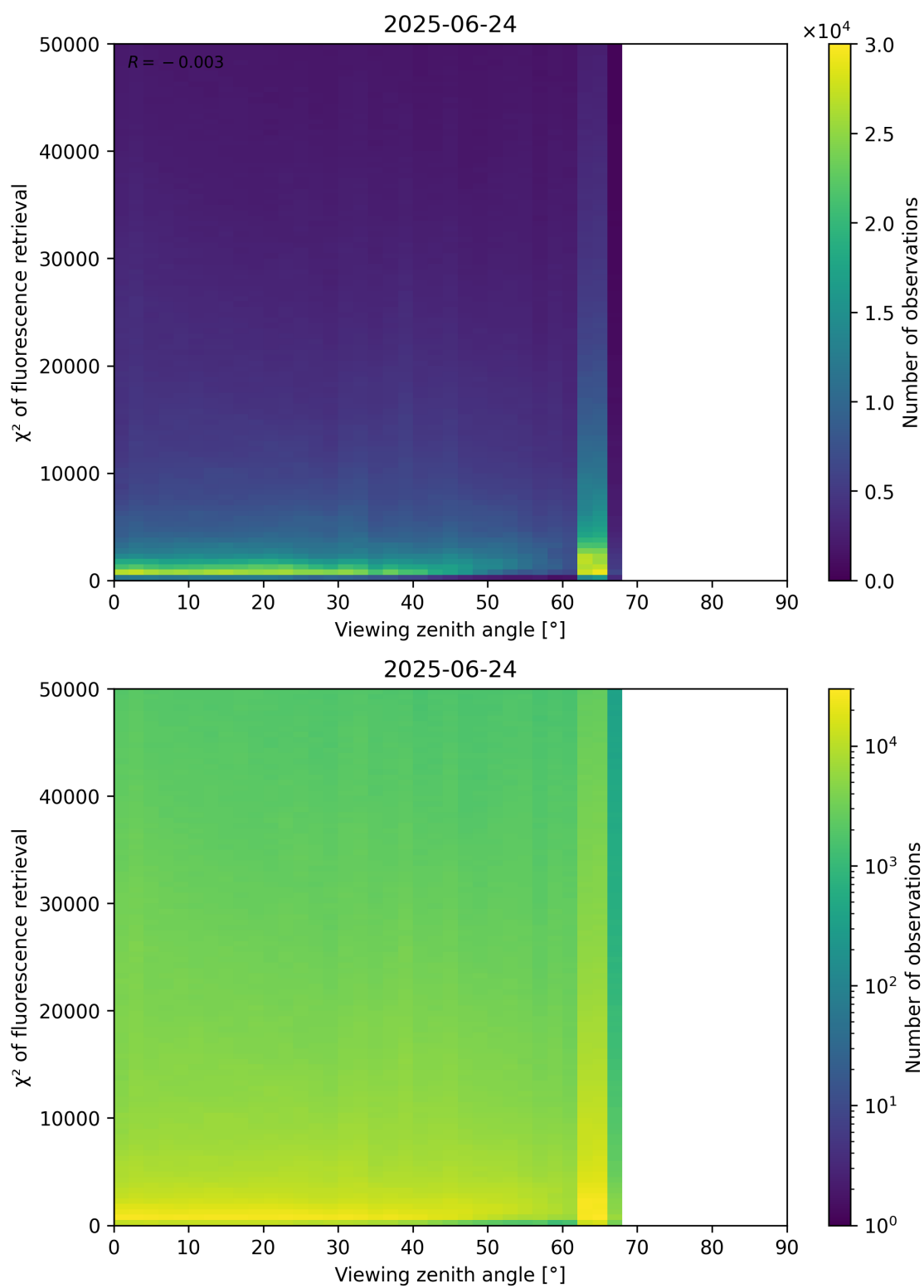
Figure 119: Scatter density plot of “Viewing zenith angle” against “ \chi^2 of fluorescence retrieval” for 2025-06-23 to 2025-06-25.
