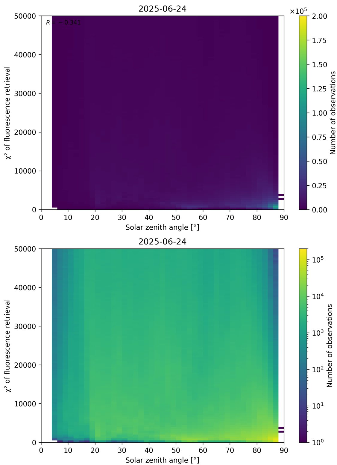
Figure 109: Scatter density plot of “Solar zenith angle” against “ \chi^2 of fluorescence retrieval” for 2025-06-23 to 2025-06-25.
