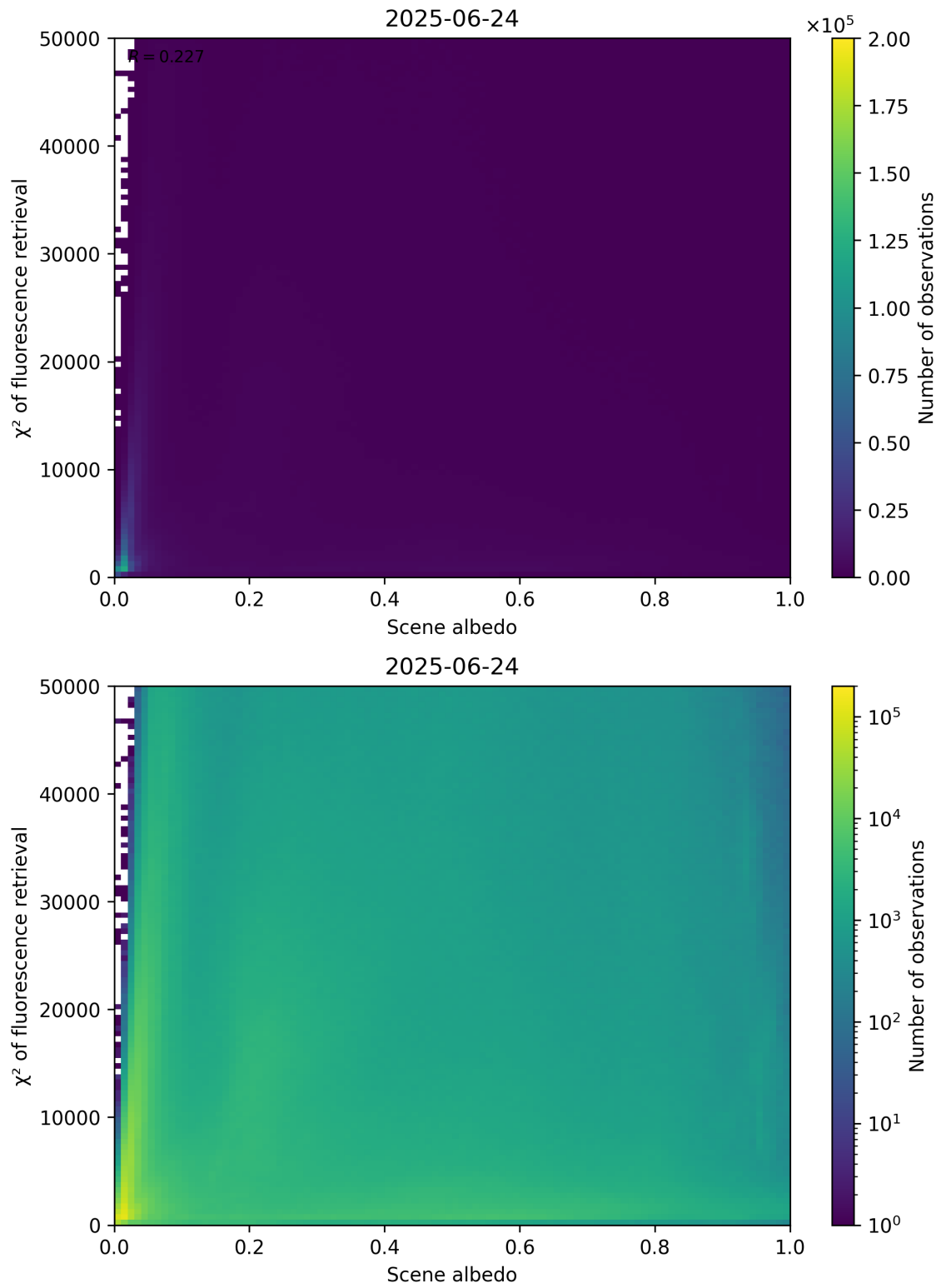
Figure 103: Scatter density plot of “Scene albedo” against “ \chi^2 of fluorescence retrieval” for 2025-06-23 to 2025-06-25.
