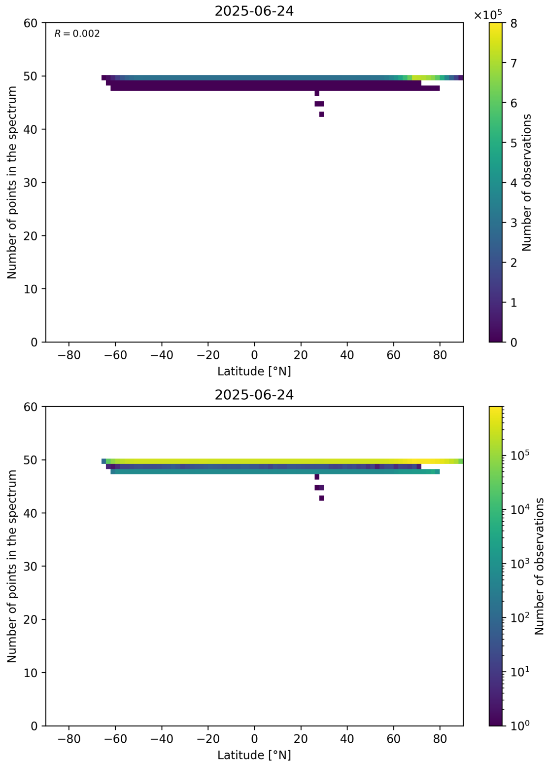
Figure 94: Scatter density plot of “Latitude” against “Number of points in the spectrum” for 2025-06-23 to 2025-06-25.
