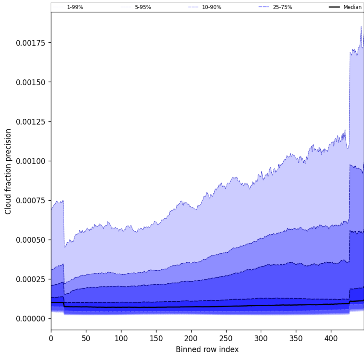
Figure 50: Along track statistics of “Cloud fraction precision” for 2025-06-23 to 2025-06-25
