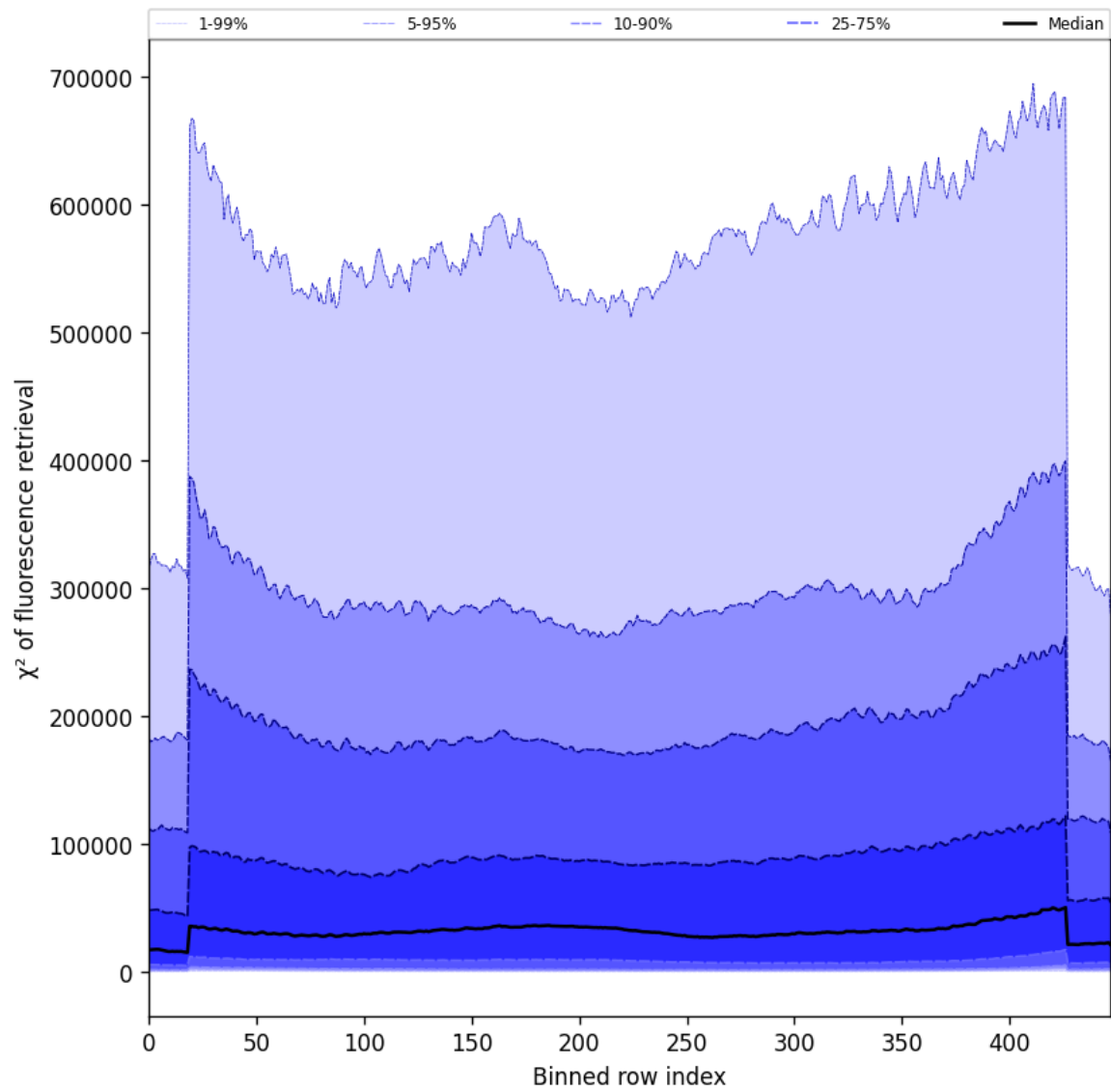
Figure 59: Along track statistics of “ \chi^2 of fluorescence retrieval” for 2025-06-23 to 2025-06-25
