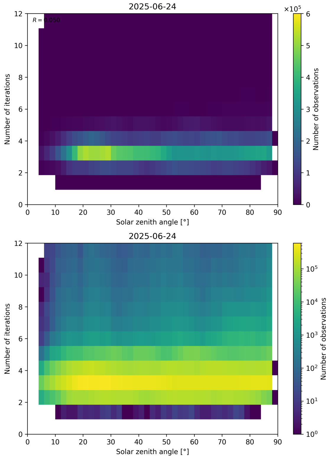
Figure 114: Scatter density plot of “Solar zenith angle” against “Number of iterations” for 2025-06-23 to 2025-06-25.
