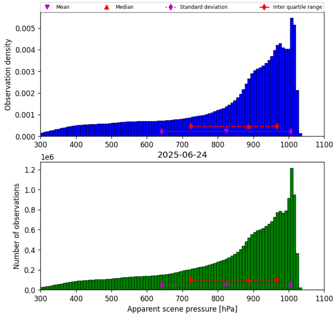
Figure 36: Histogram of “Apparent scene pressure” for 2025-06-23 to 2025-06-25
