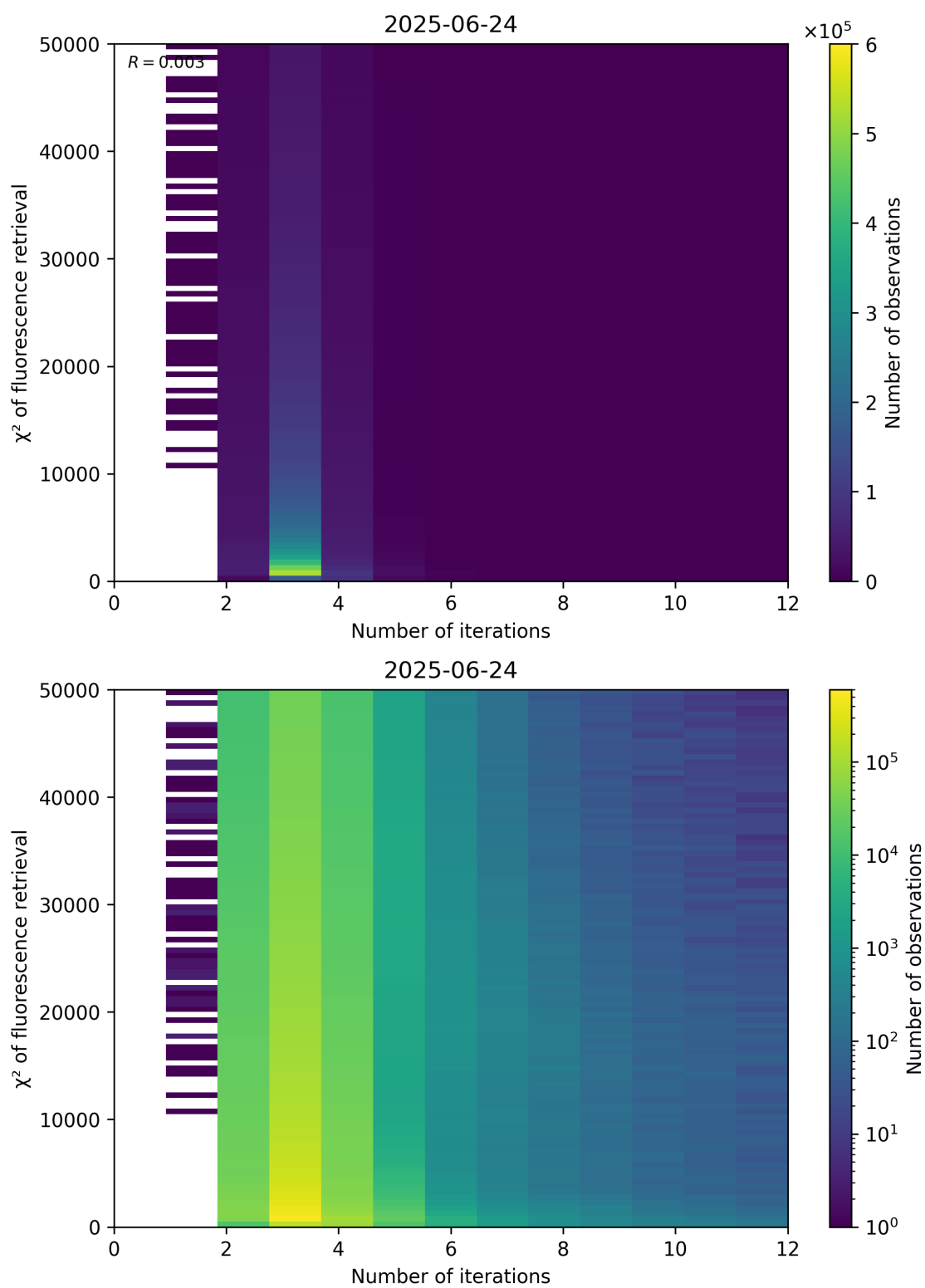
Figure 97: Scatter density plot of “Number of iterations” against “ \chi^2 of fluorescence retrieval” for 2025-06-23 to 2025-06-25.
