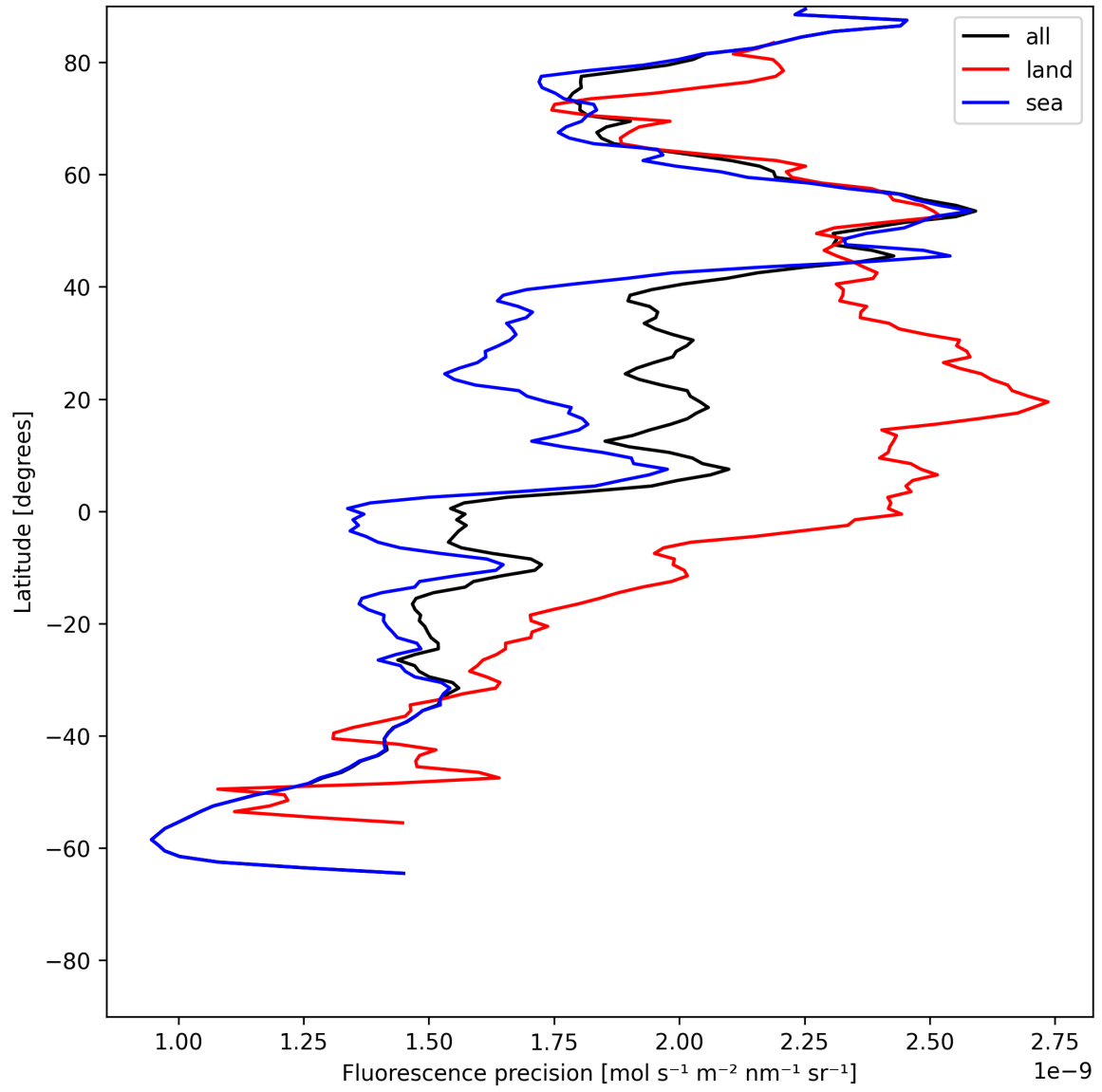
Figure 24: Zonal average of “Fluorescence precision” for 2025-06-23 to 2025-06-25.
