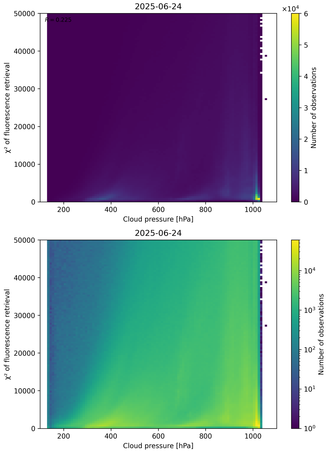
Figure 78: Scatter density plot of “Cloud pressure” against “ \chi^2 of fluorescence retrieval” for 2025-06-23 to 2025-06-25.
