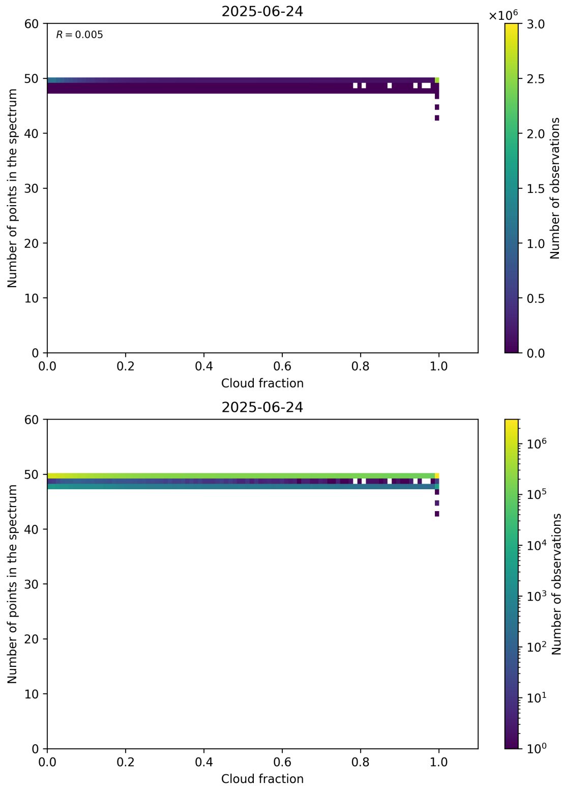
Figure 74: Scatter density plot of “Cloud fraction” against “Number of points in the spectrum” for 2025-06-23 to 2025-06-25.
