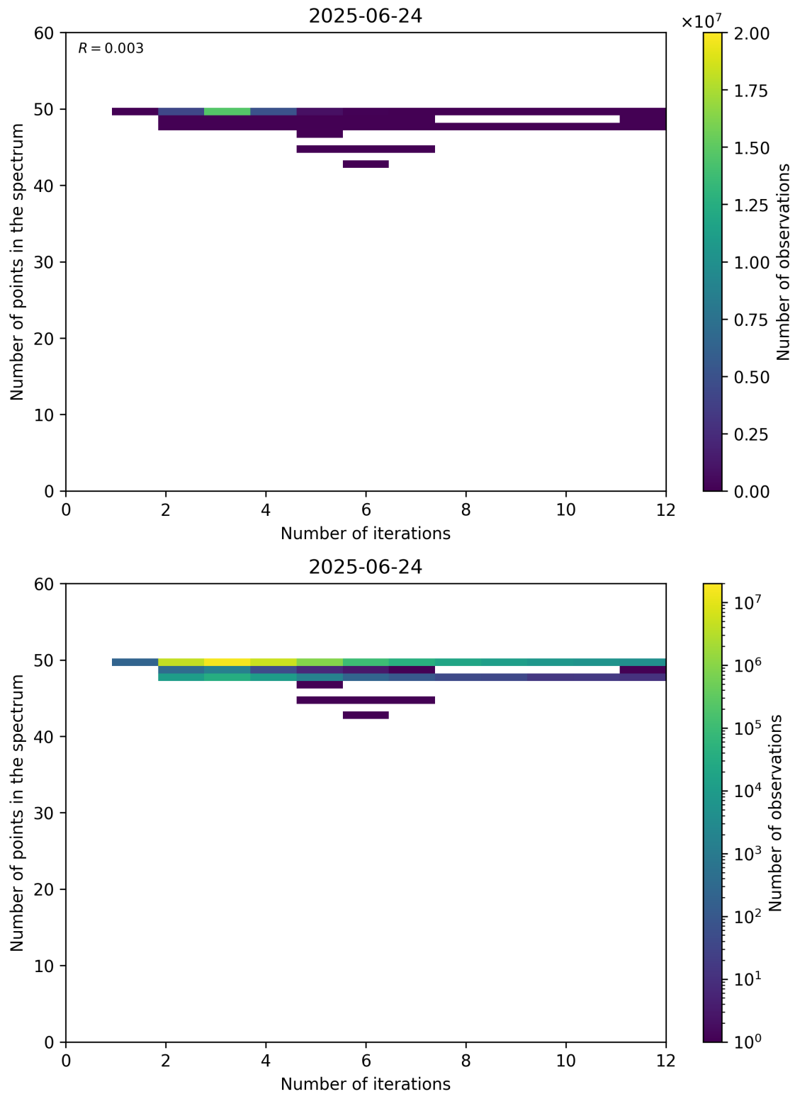
Figure 99: Scatter density plot of “Number of iterations” against “Number of points in the spectrum” for 2025-06-23 to 2025-06-25.
