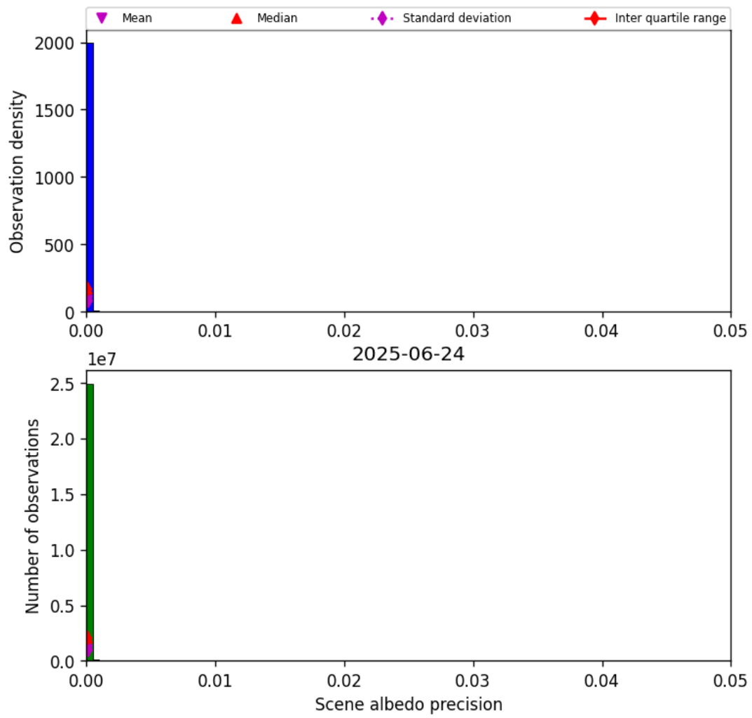
Figure 35: Histogram of “Scene albedo precision” for 2025-06-23 to 2025-06-25
