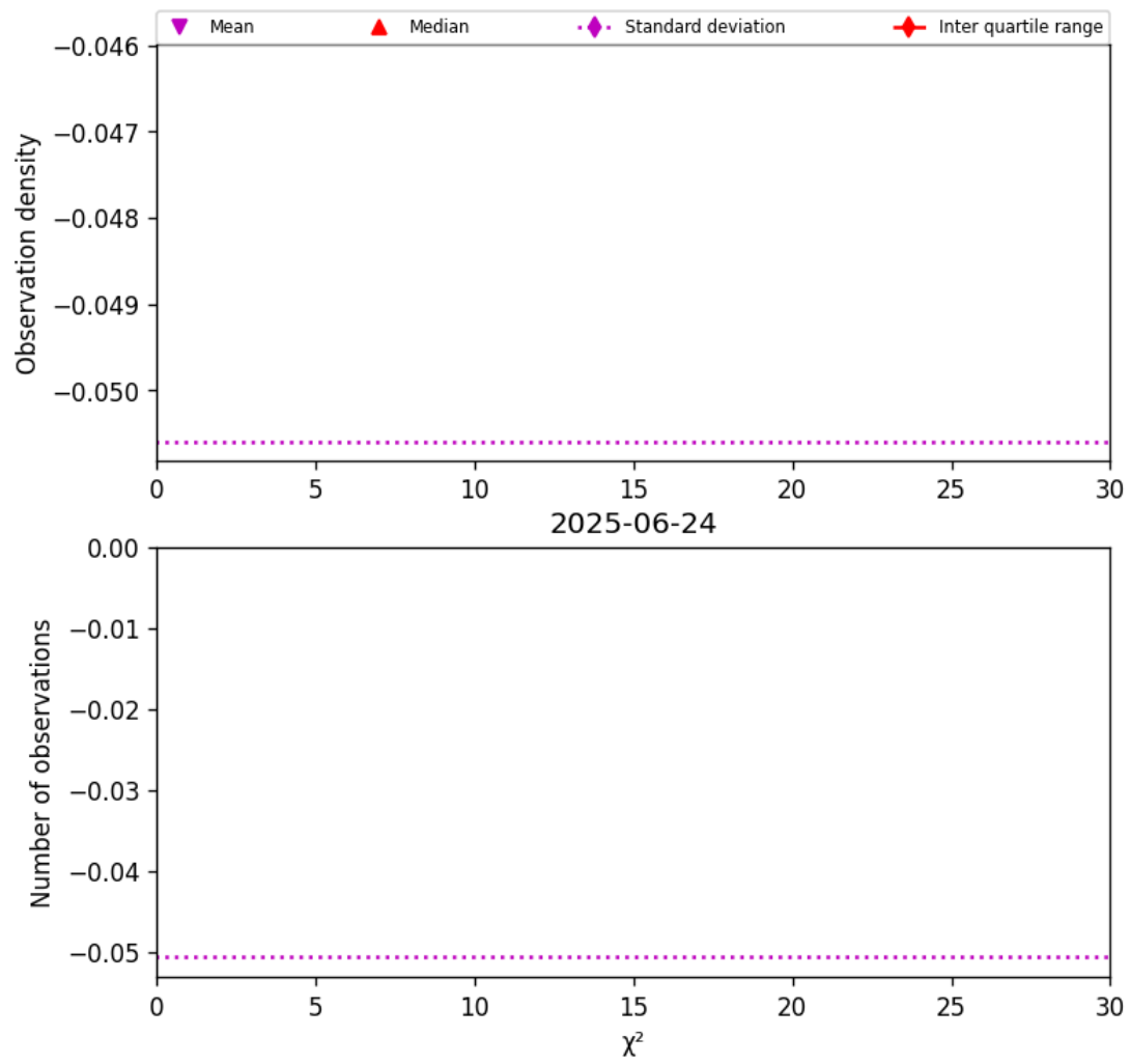
Figure 38: Histogram of “ \chi^2 ” for 2025-06-23 to 2025-06-25
