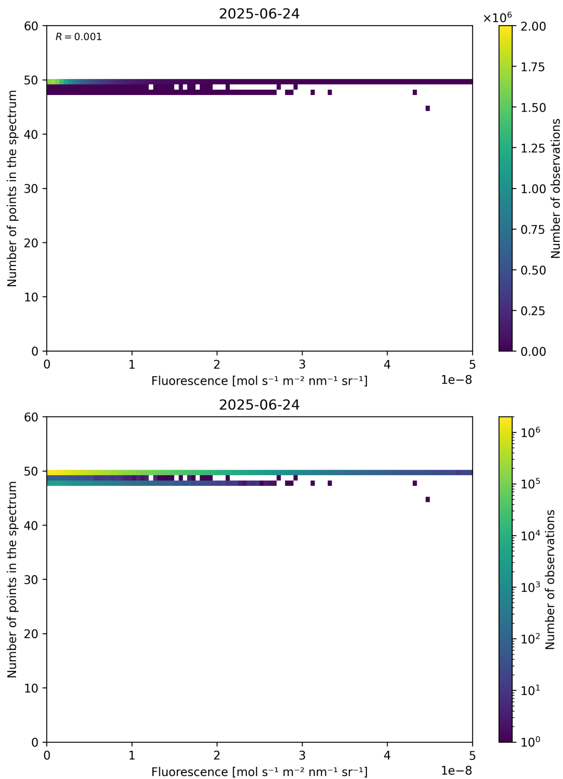
Figure 86: Scatter density plot of “Fluorescence” against “Number of points in the spectrum” for 2025-06-23 to 2025-06-25.
