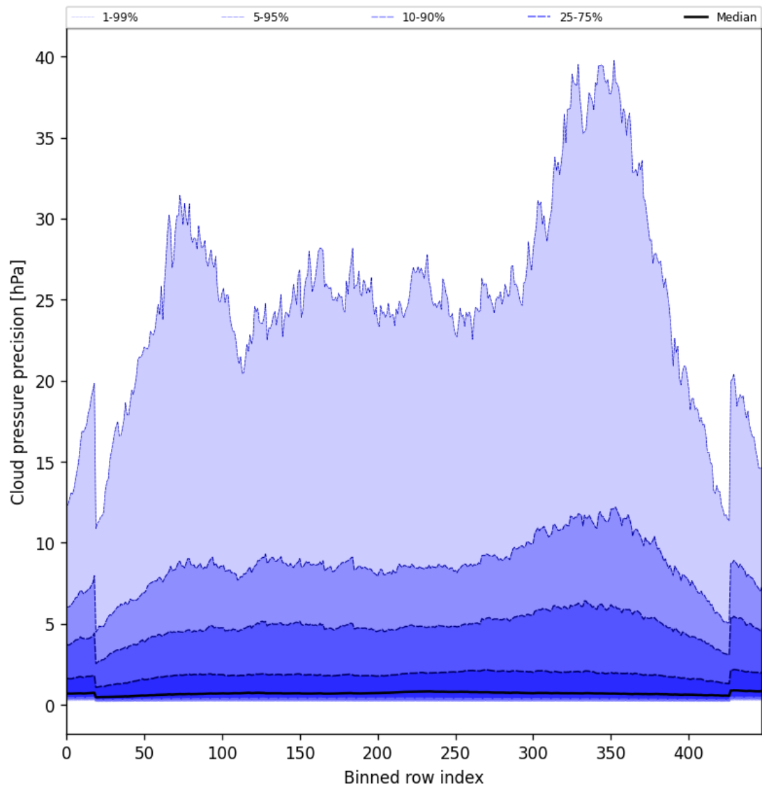
Figure 48: Along track statistics of “Cloud pressure precision” for 2025-06-23 to 2025-06-25
