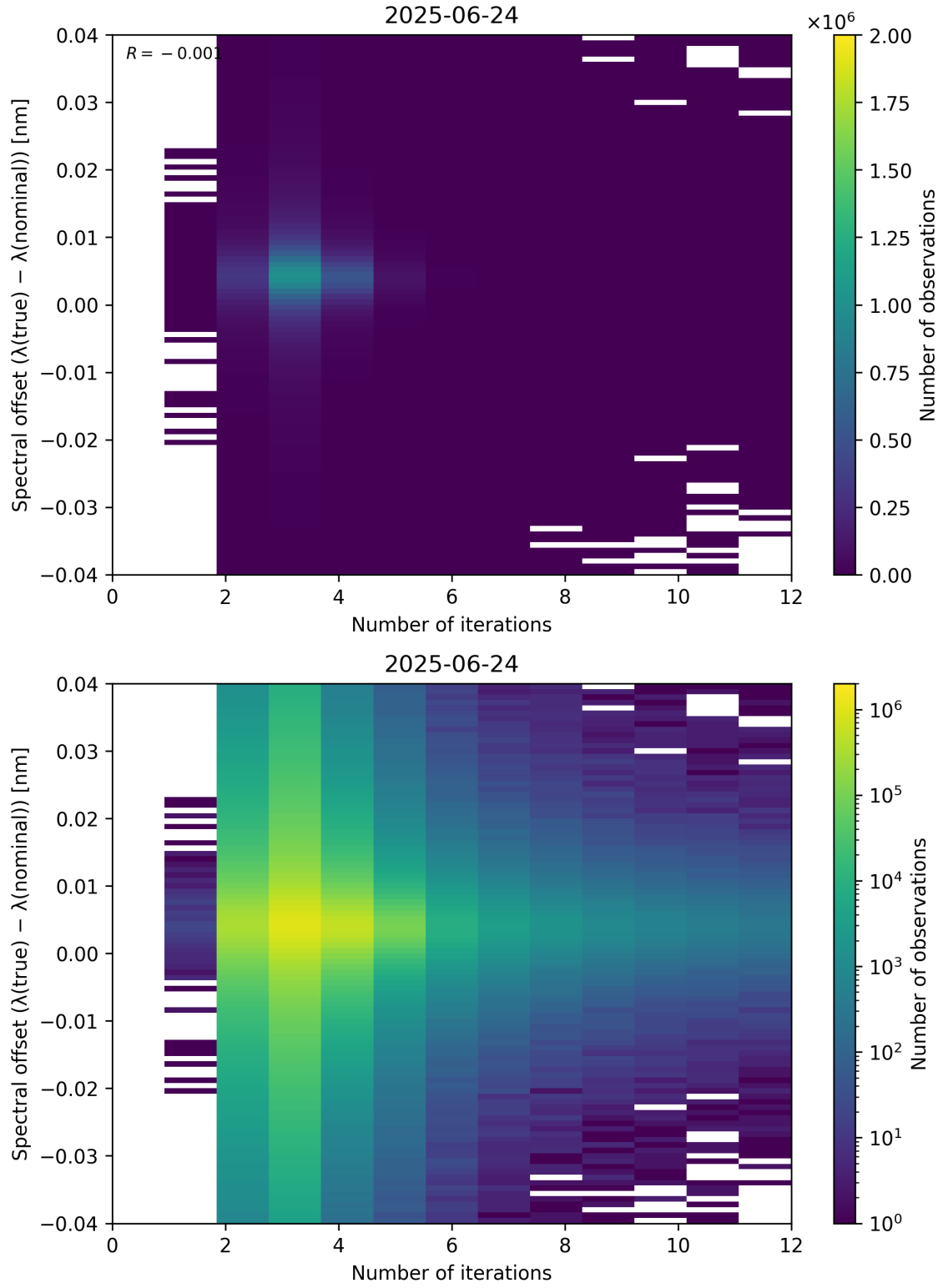
Figure 100: Scatter density plot of “Number of iterations” against “Spectral offset ( \lambda_{\text{true}} - \lambda_{\text{nominal}} )” for 2025-06-23 to 2025-06-25.
