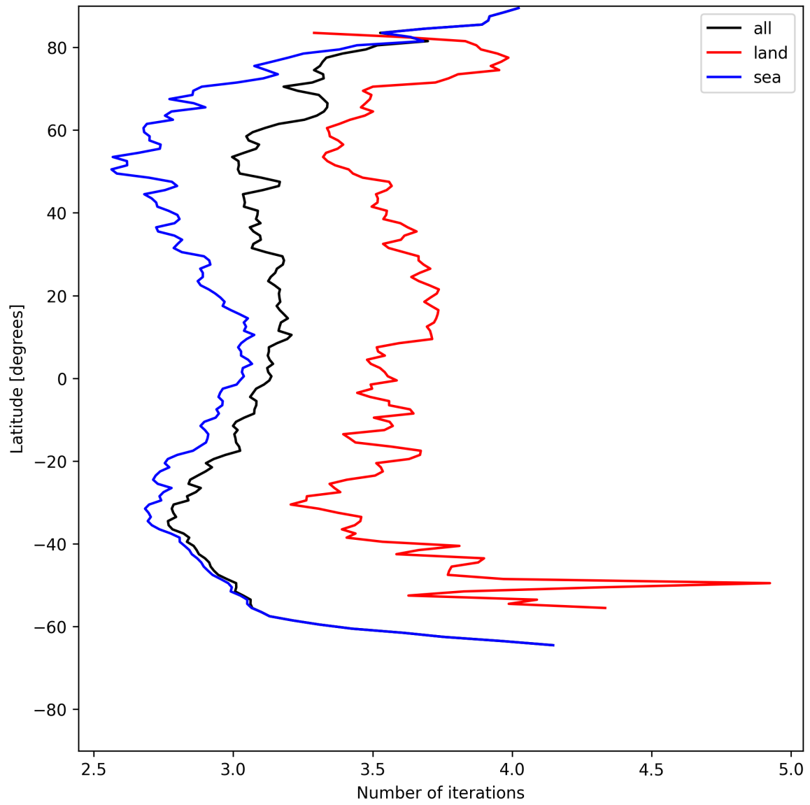
Figure 22: Zonal average of “Number of iterations” for 2025-06-23 to 2025-06-25.
