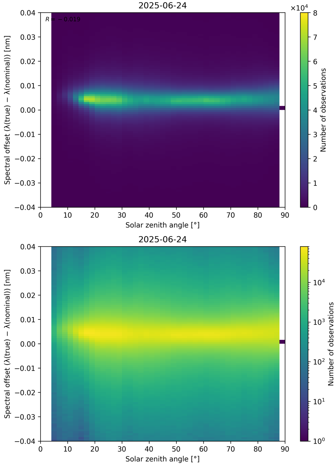
Figure 117: Scatter density plot of “Solar zenith angle” against “Spectral offset ( \lambda_{\text{true}} - \lambda_{\text{nominal}} )” for 2025-06-23 to 2025-06-25.
