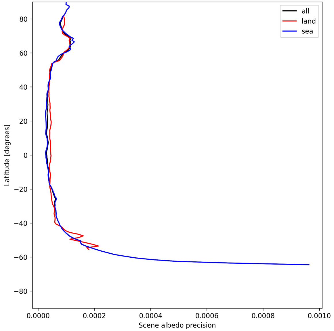
Figure 18: Zonal average of “Scene albedo precision” for 2025-06-23 to 2025-06-25.
