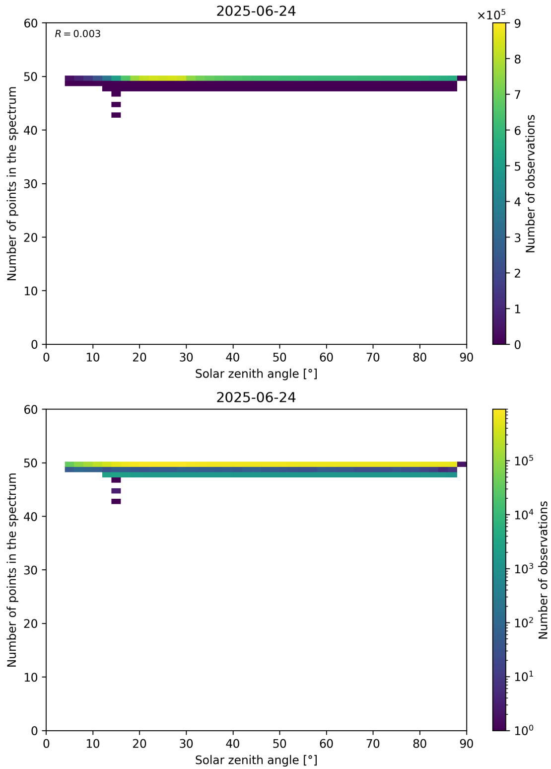
Figure 115: Scatter density plot of “Solar zenith angle” against “Number of points in the spectrum” for 2025-06-23 to 2025-06-25.
