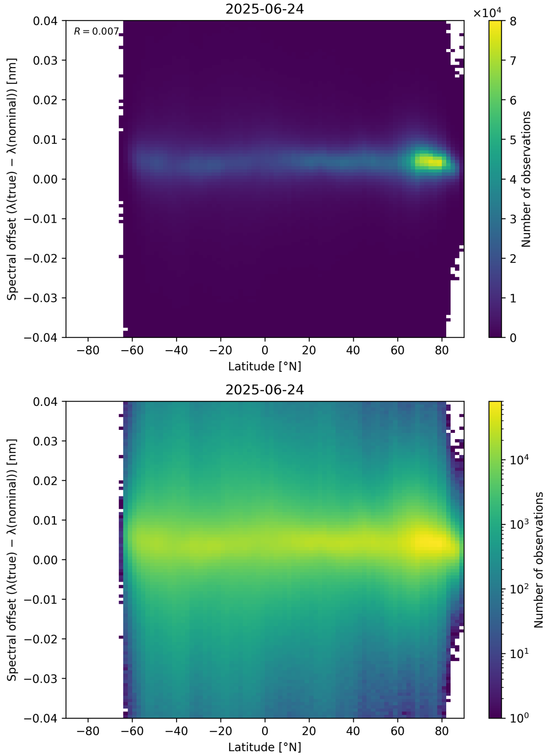
Figure 96: Scatter density plot of “Latitude” against “Spectral offset ( \lambda_{\text{true}} - \lambda_{\text{nominal}} )” for 2025-06-23 to 2025-06-25.
