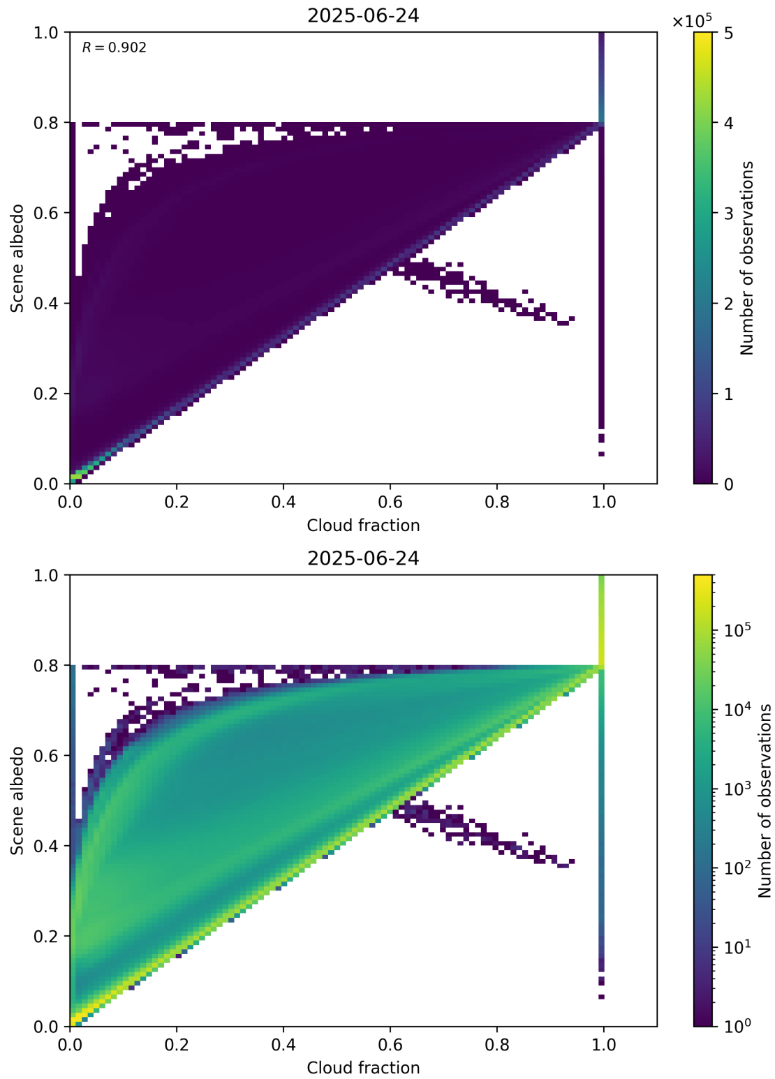
Figure 75: Scatter density plot of “Cloud fraction” against “Scene albedo” for 2025-06-23 to 2025-06-25.
