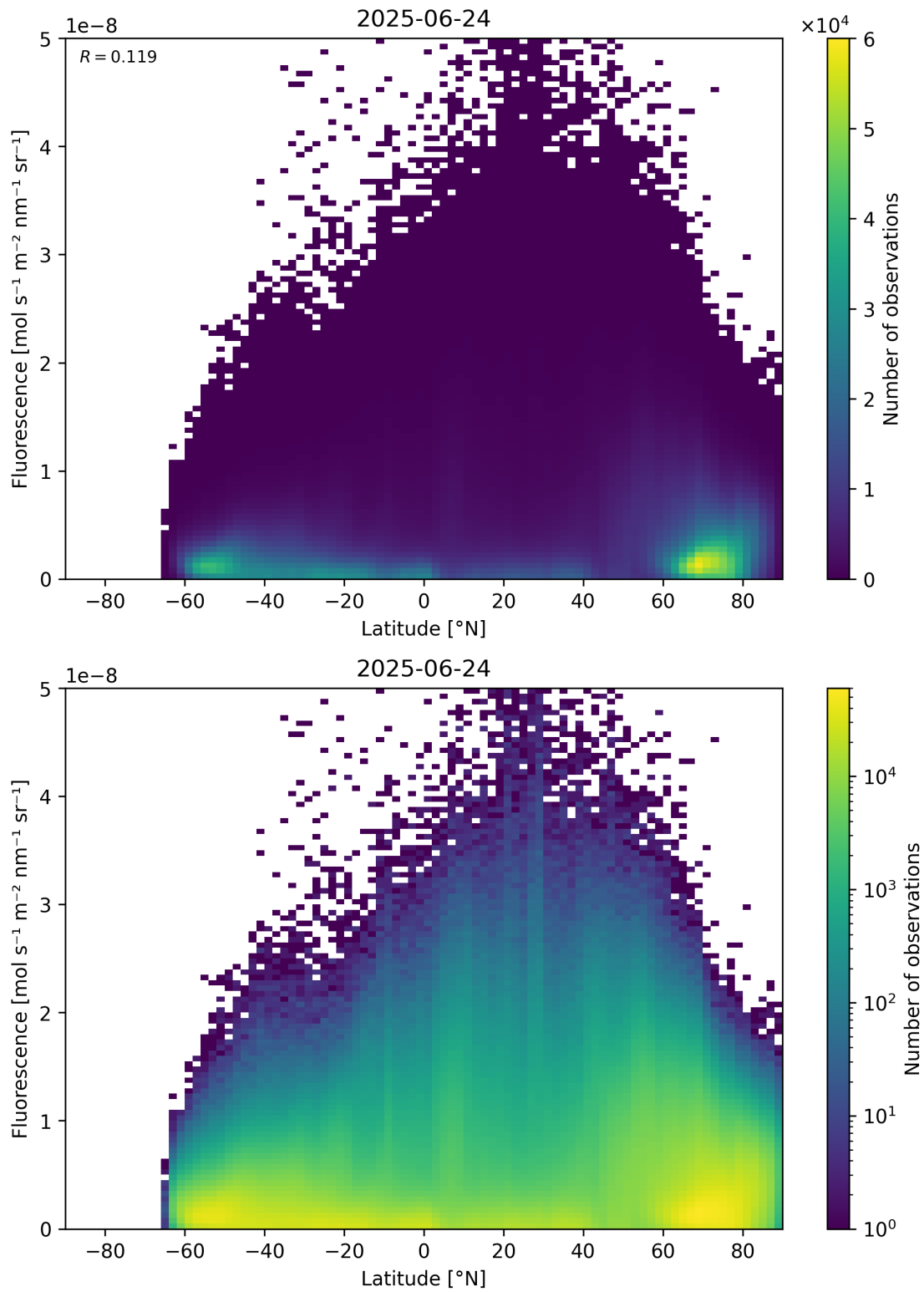
Figure 92: Scatter density plot of “Latitude” against “Fluorescence” for 2025-06-23 to 2025-06-25.
