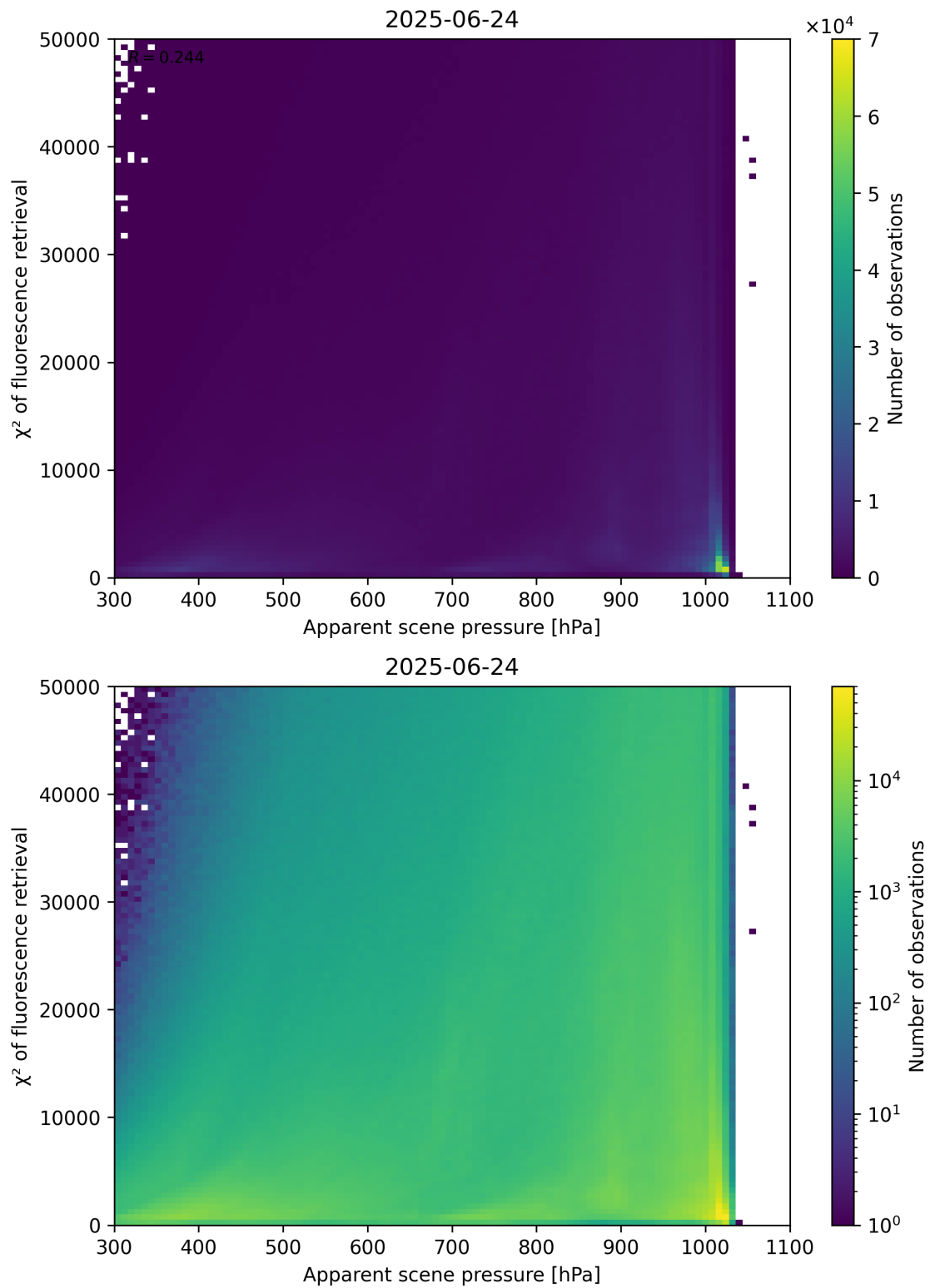
Figure 63: Scatter density plot of “Apparent scene pressure” against “ \chi^2 of fluorescence retrieval” for 2025-06-23 to 2025-06-25.
