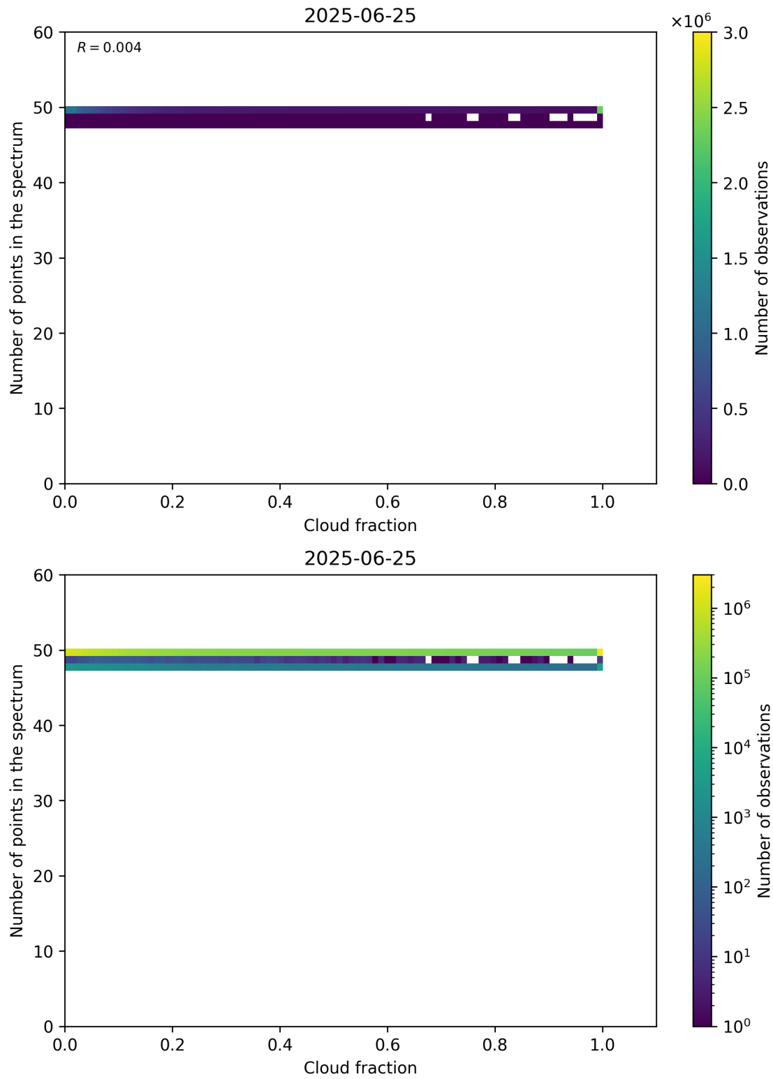
Figure 74: Scatter density plot of “Cloud fraction” against “Number of points in the spectrum” for 2025-06-24 to 2025-06-26.
