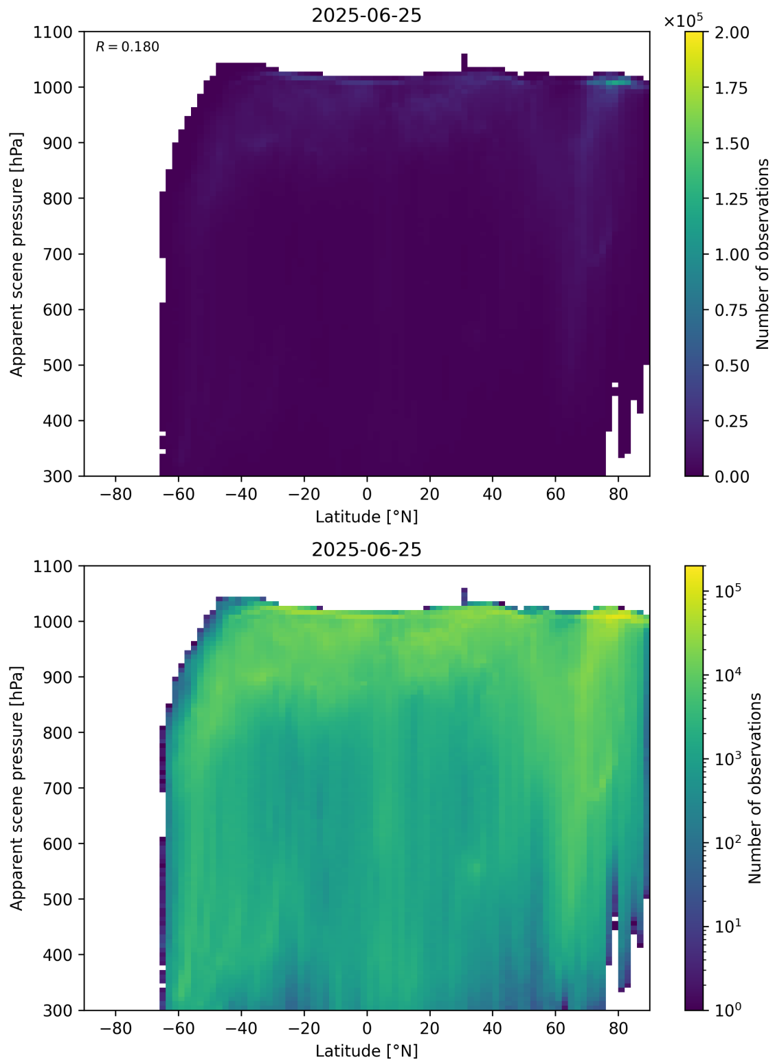
Figure 88: Scatter density plot of “Latitude” against “Apparent scene pressure” for 2025-06-24 to 2025-06-26.
