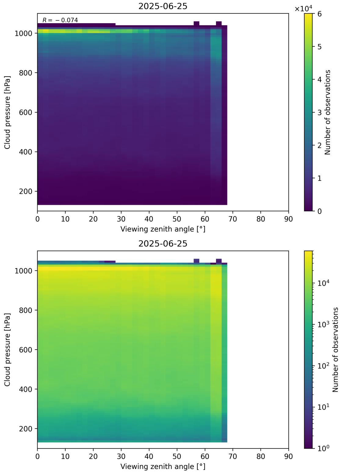
Figure 121: Scatter density plot of “Viewing zenith angle” against “Cloud pressure” for 2025-06-24 to 2025-06-26.
