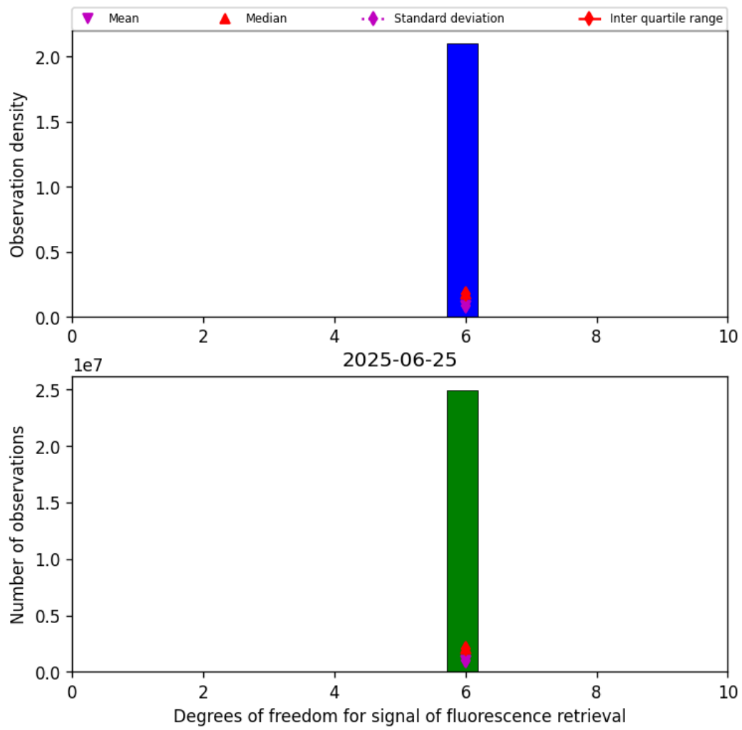
Figure 43: Histogram of "Degrees of freedom for signal of fluorescence retrieval" for 2025-06-24 to 2025-06-26
