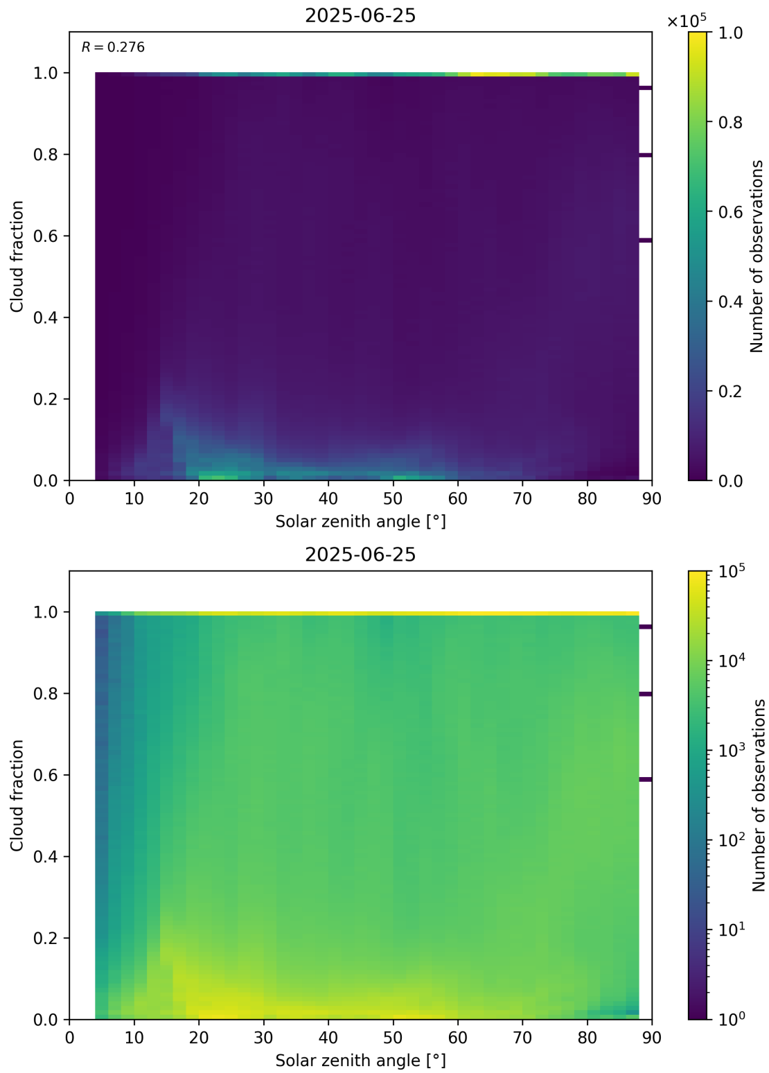
Figure 110: Scatter density plot of “Solar zenith angle” against “Cloud fraction” for 2025-06-24 to 2025-06-26.
