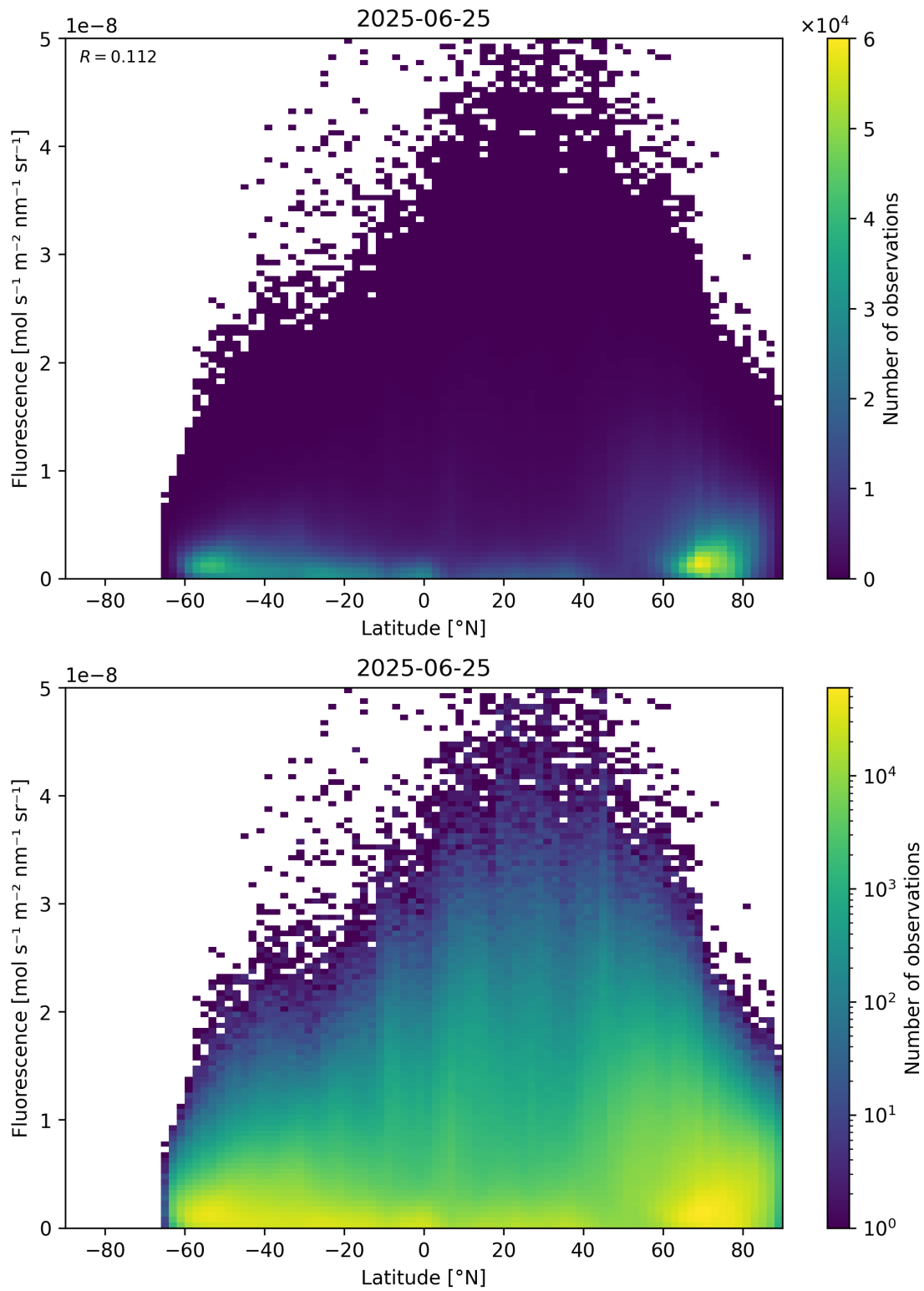
Figure 92: Scatter density plot of “Latitude” against “Fluorescence” for 2025-06-24 to 2025-06-26.
