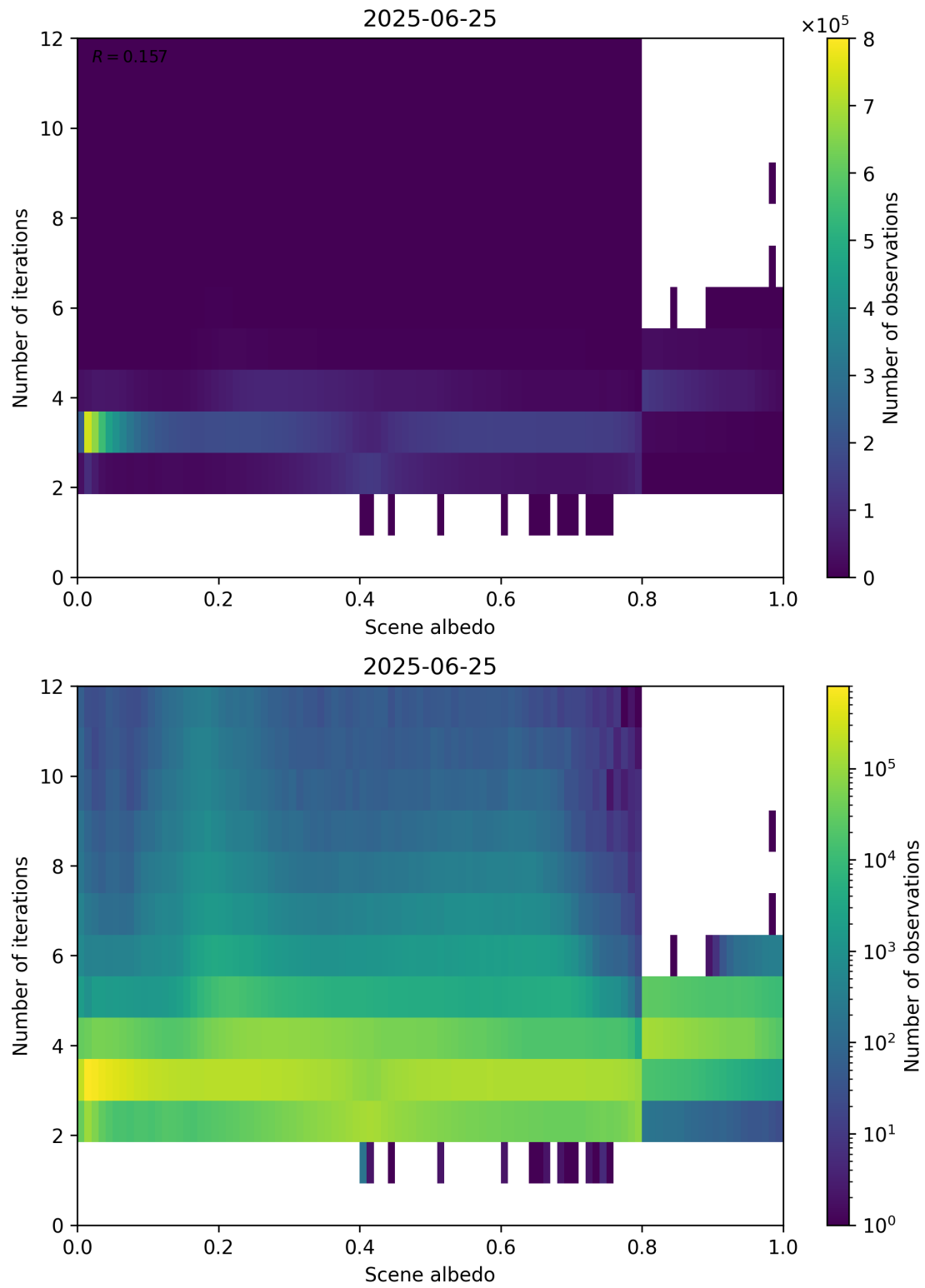
Figure 105: Scatter density plot of “Scene albedo” against “Number of iterations” for 2025-06-24 to 2025-06-26.
