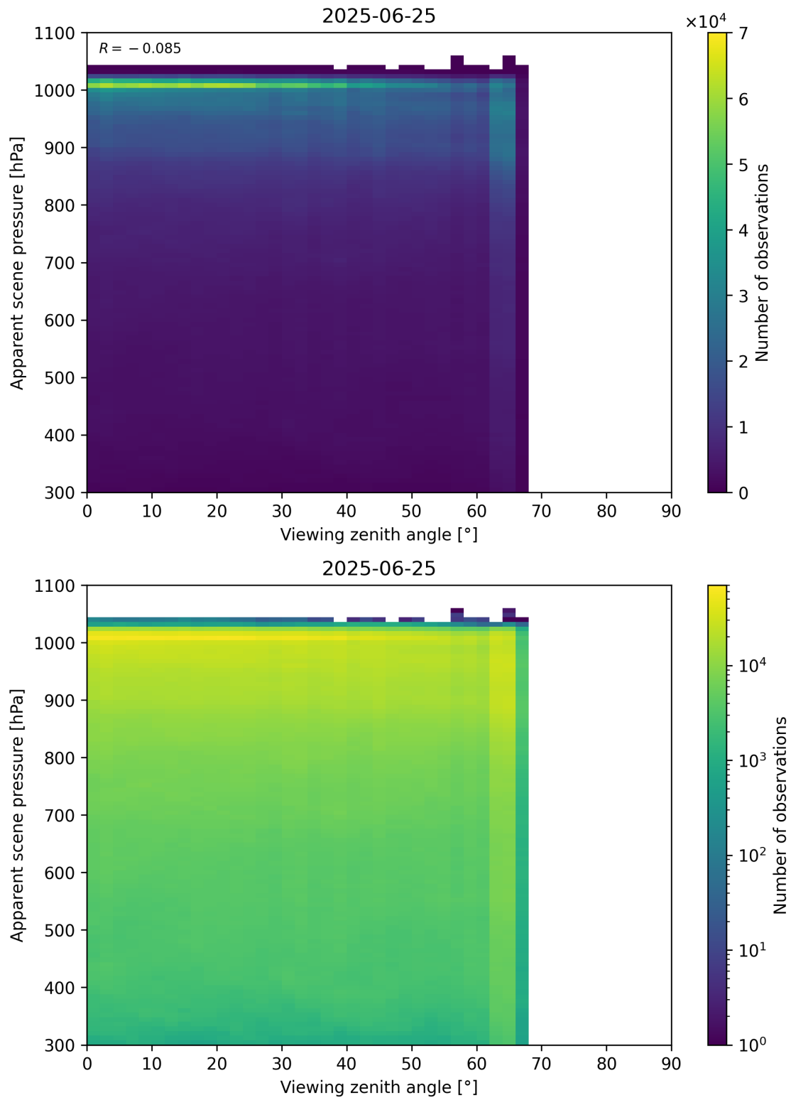
Figure 118: Scatter density plot of “Viewing zenith angle” against “Apparent scene pressure” for 2025-06-24 to 2025-06-26.
