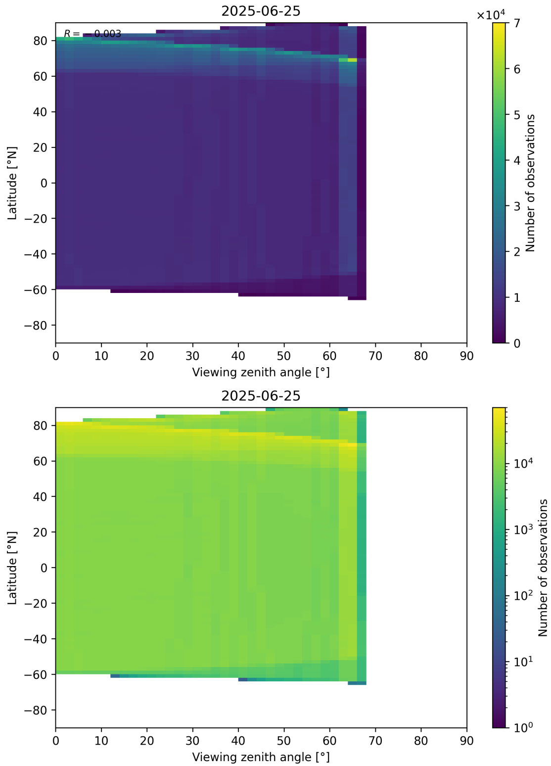
Figure 123: Scatter density plot of “Viewing zenith angle” against “Latitude” for 2025-06-24 to 2025-06-26.
