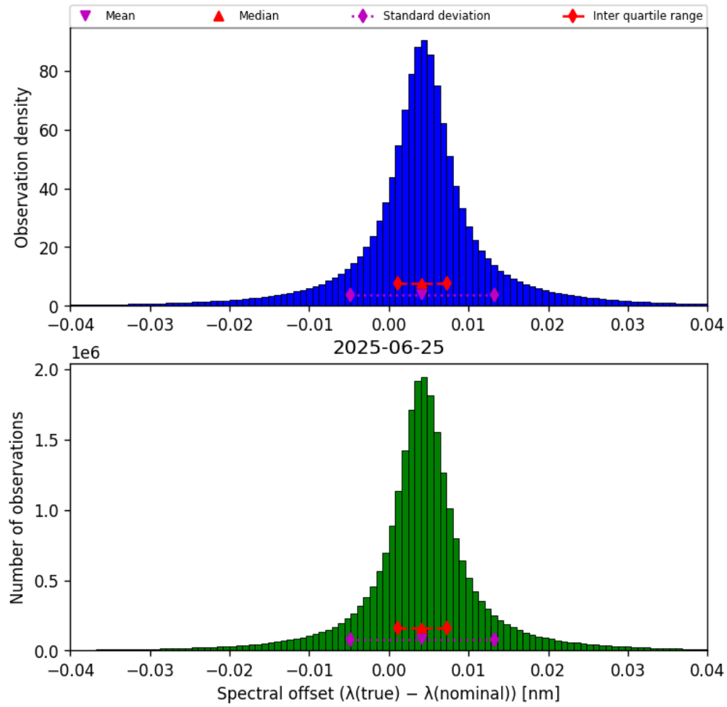
Figure 45: Histogram of “Spectral offset ( \lambda_{\text{true}} - \lambda_{\text{nominal}} )” for 2025-06-24 to 2025-06-26
