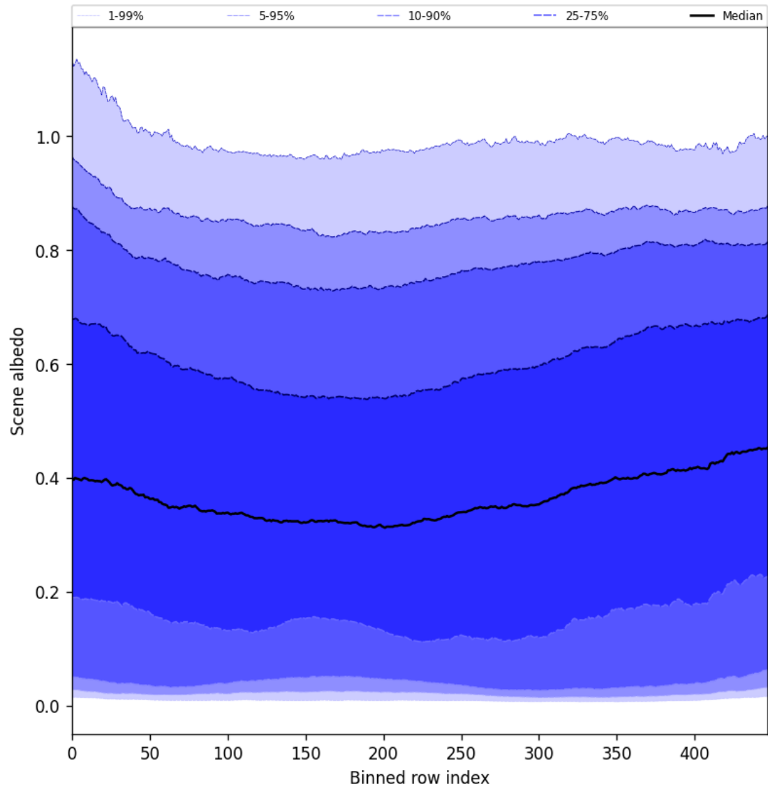
Figure 51: Along track statistics of “Scene albedo” for 2025-06-24 to 2025-06-26
