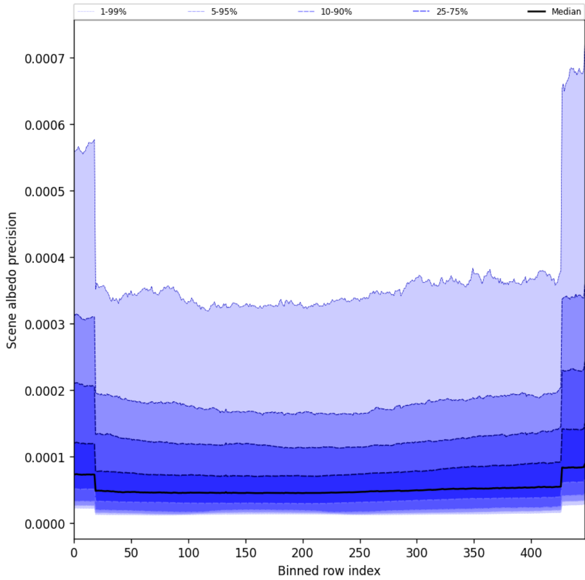
Figure 52: Along track statistics of “Scene albedo precision” for 2025-06-24 to 2025-06-26
