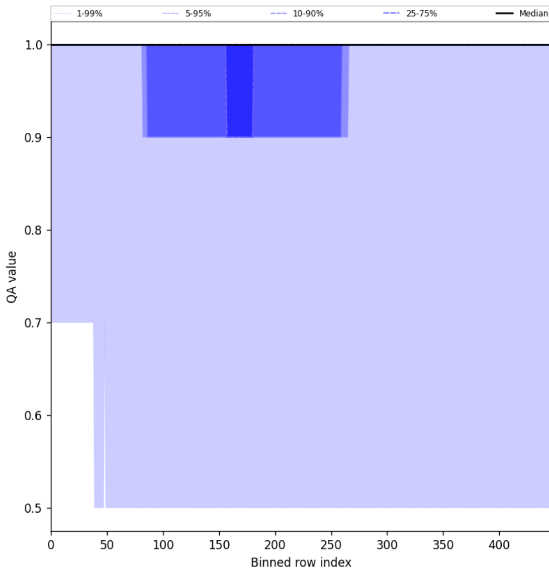
Figure 46: Along track statistics of “QA value” for 2025-06-24 to 2025-06-26
