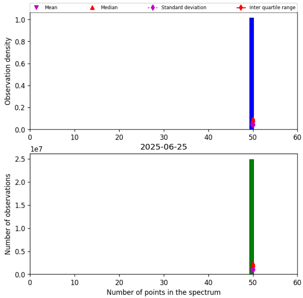
Figure 44: Histogram of “Number of points in the spectrum” for 2025-06-24 to 2025-06-26
