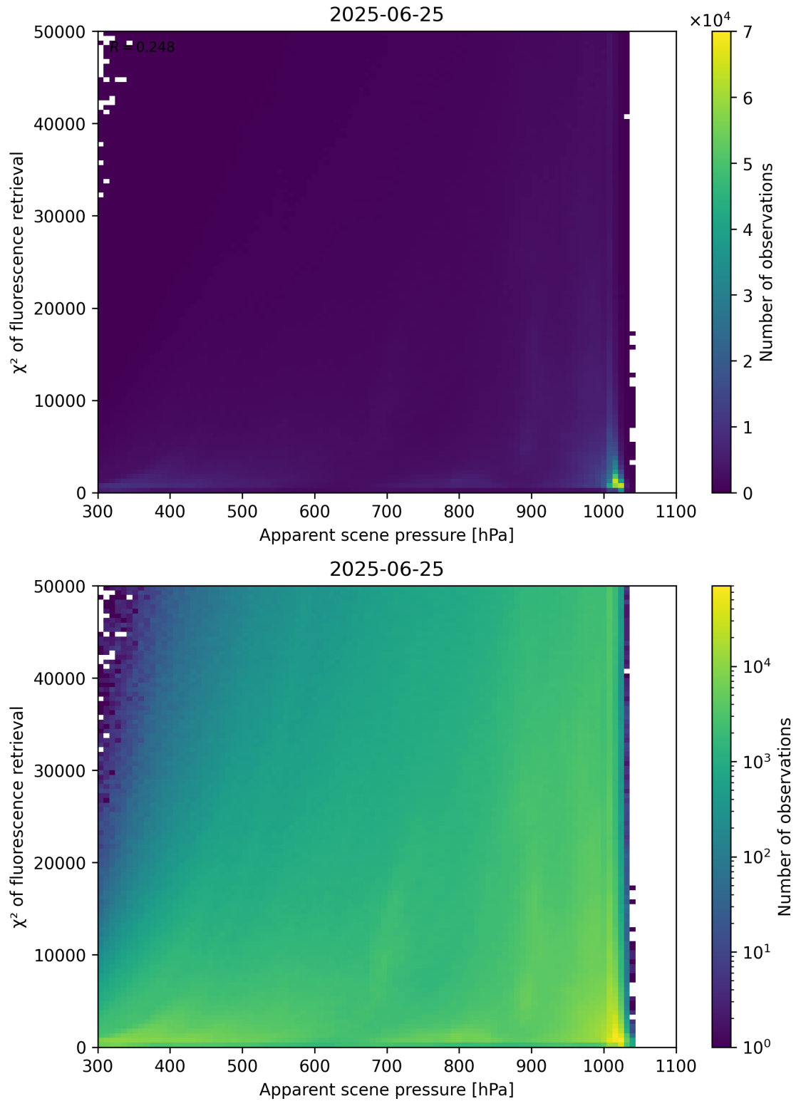
Figure 63: Scatter density plot of “Apparent scene pressure” against “ \chi^2 of fluorescence retrieval” for 2025-06-24 to 2025-06-26.
