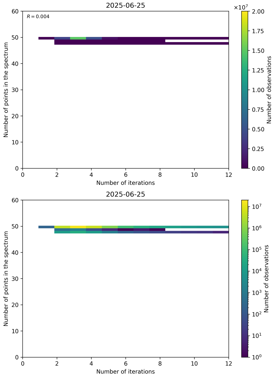
Figure 99: Scatter density plot of “Number of iterations” against “Number of points in the spectrum” for 2025-06-24 to 2025-06-26.
