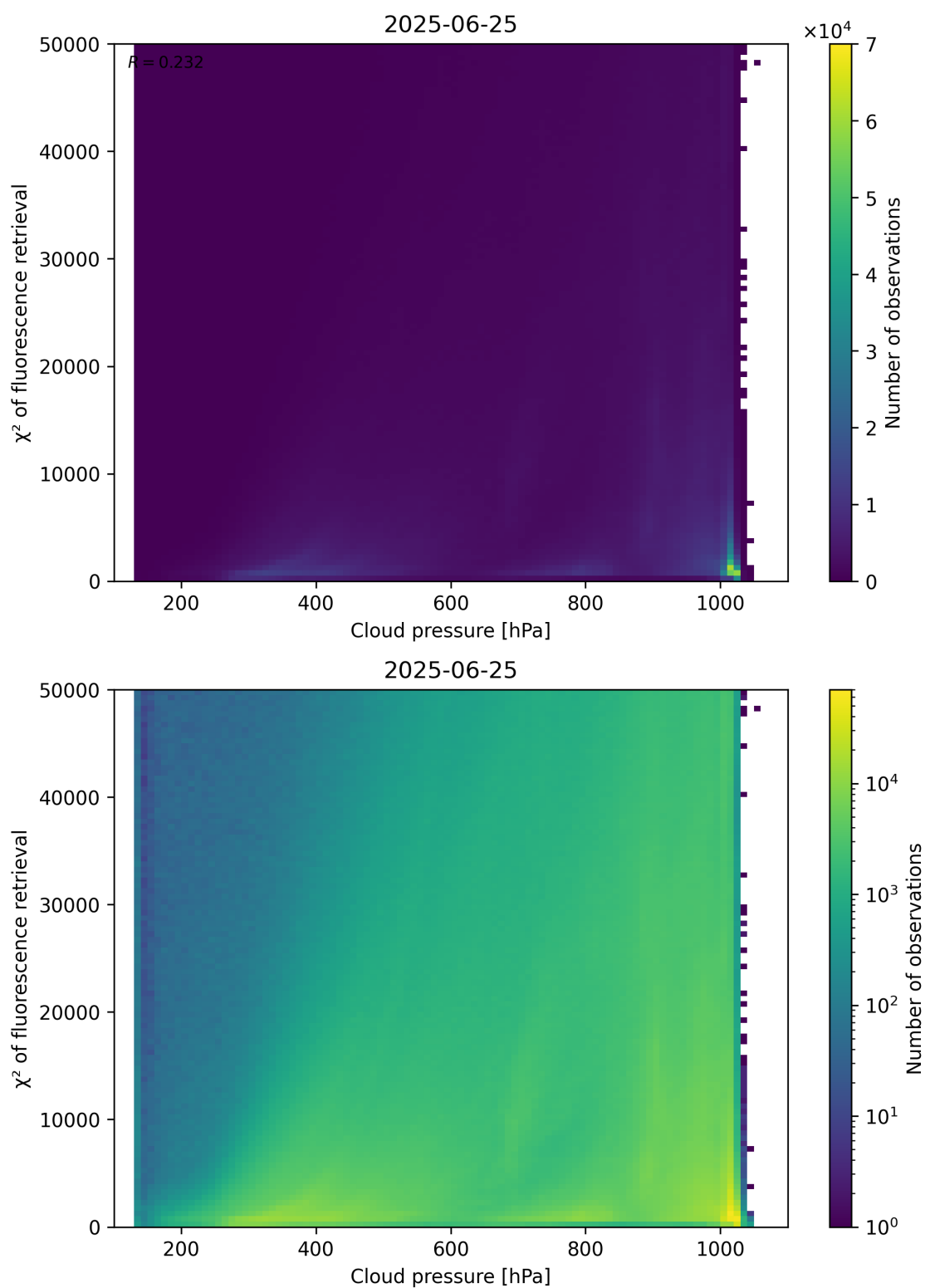
Figure 78: Scatter density plot of “Cloud pressure” against “ \chi^2 of fluorescence retrieval” for 2025-06-24 to 2025-06-26.
