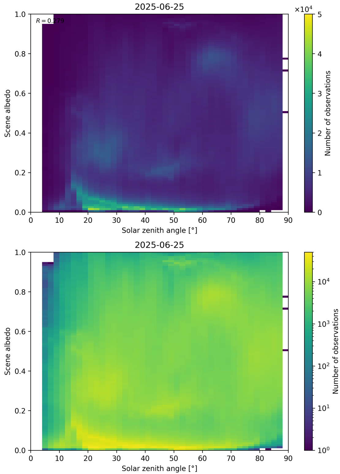
Figure 116: Scatter density plot of “Solar zenith angle” against “Scene albedo” for 2025-06-24 to 2025-06-26.
