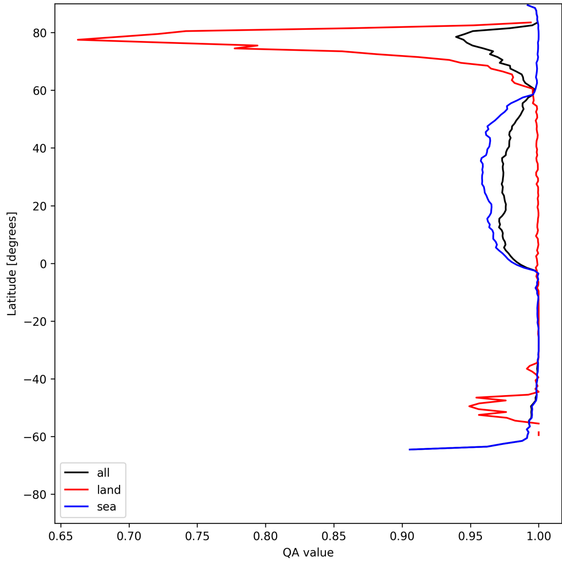
Figure 12: Zonal average of “QA value” for 2025-06-24 to 2025-06-26.
