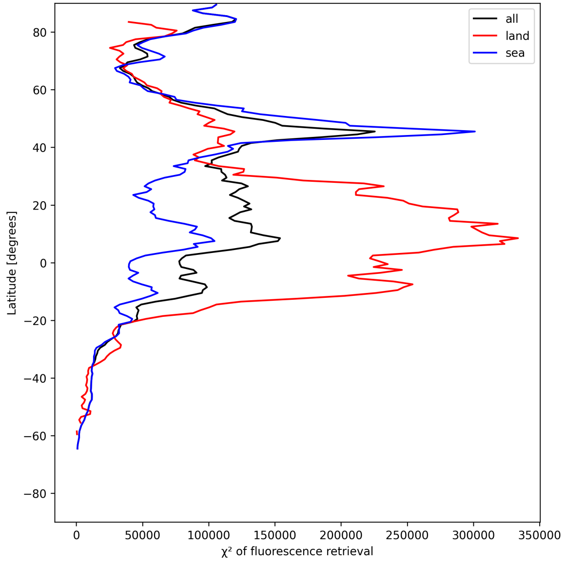
Figure 25: Zonal average of “ \chi^2 of fluorescence retrieval” for 2025-06-24 to 2025-06-26.
