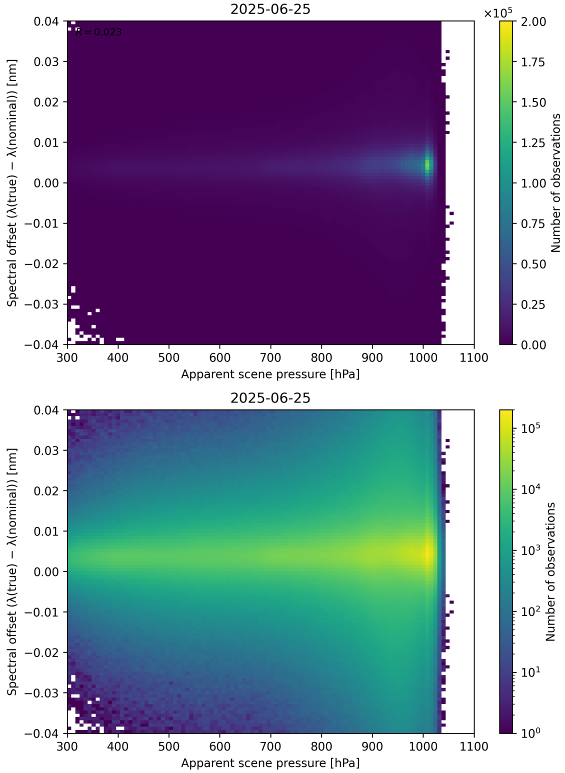
Figure 67: Scatter density plot of “Apparent scene pressure” against “Spectral offset ( \lambda_{\text{true}} - \lambda_{\text{nominal}} )” for 2025-06-24 to 2025-06-26.
