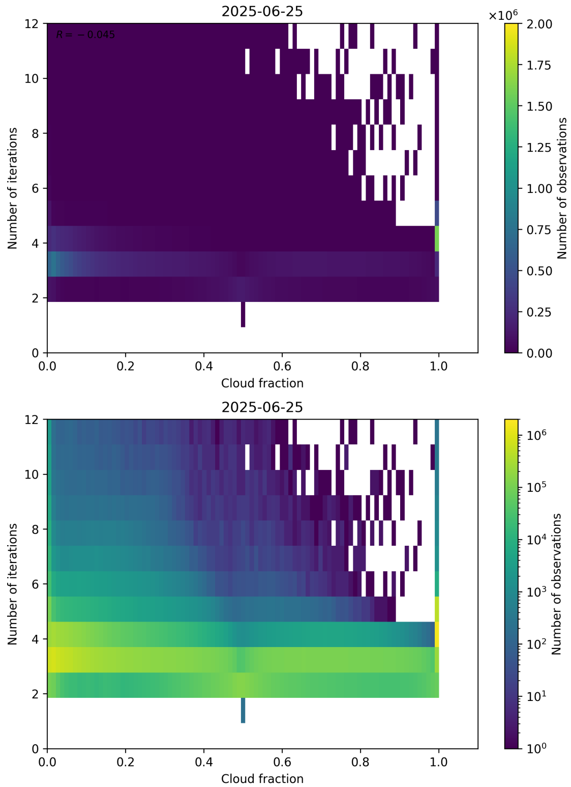
Figure 73: Scatter density plot of “Cloud fraction” against “Number of iterations” for 2025-06-24 to 2025-06-26.
