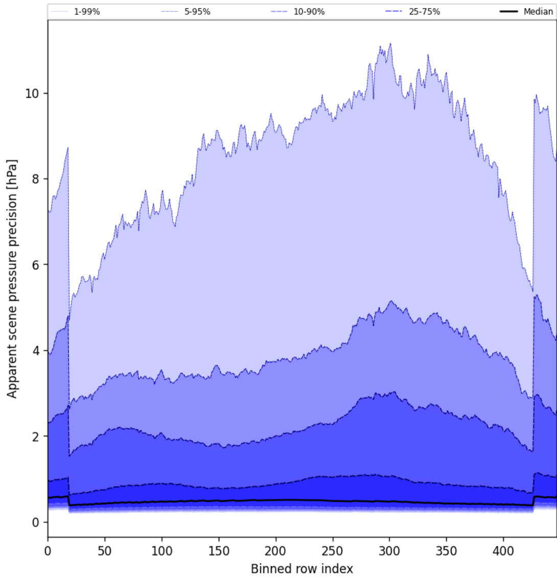
Figure 54: Along track statistics of “Apparent scene pressure precision” for 2025-06-24 to 2025-06-26
