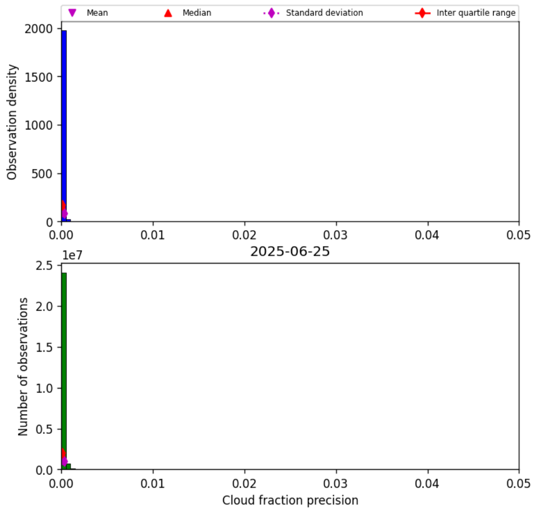
Figure 33: Histogram of “Cloud fraction precision” for 2025-06-24 to 2025-06-26
