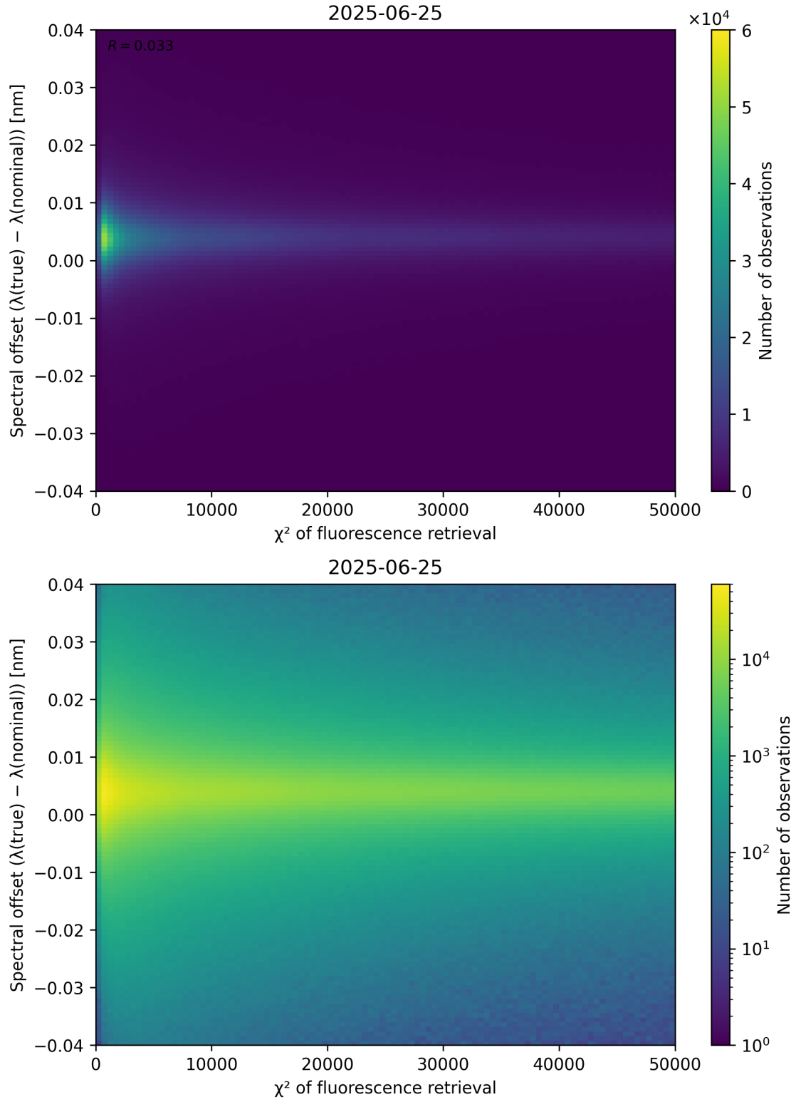
Figure 69: Scatter density plot of “ \chi^2 of fluorescence retrieval” against “Spectral offset ( \lambda_{\text{true}} - \lambda_{\text{nominal}} )” for 2025-06-24 to 2025-06-26.
