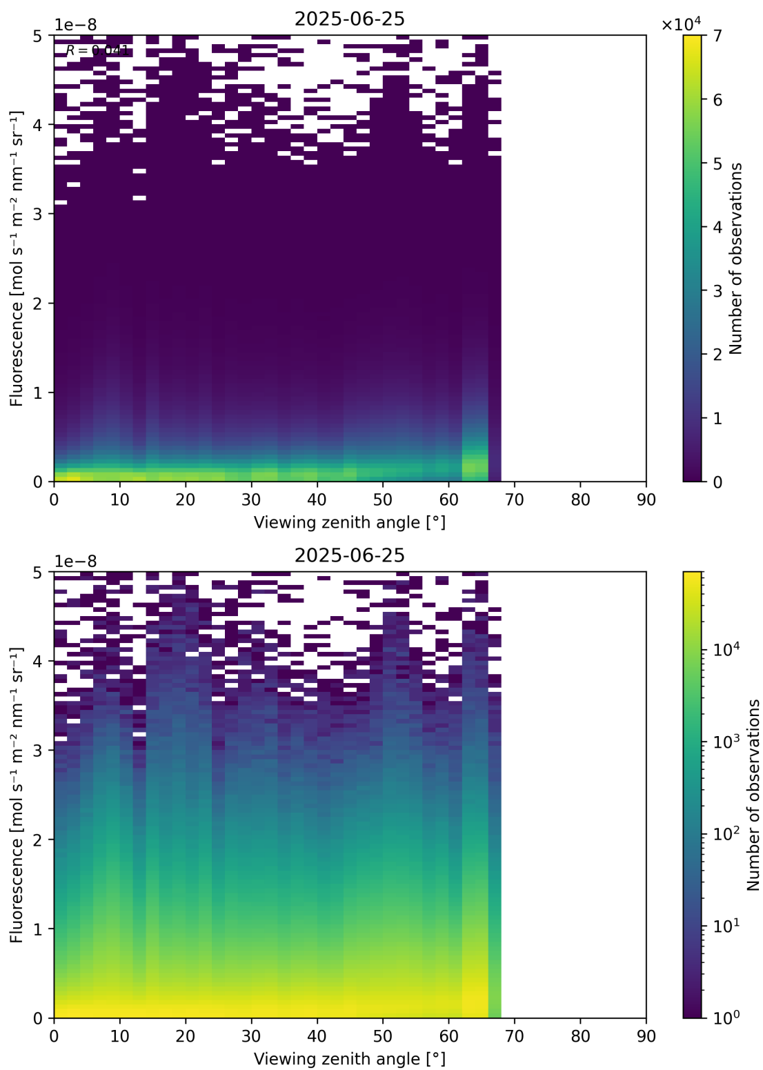
Figure 122: Scatter density plot of “Viewing zenith angle” against “Fluorescence” for 2025-06-24 to 2025-06-26.
