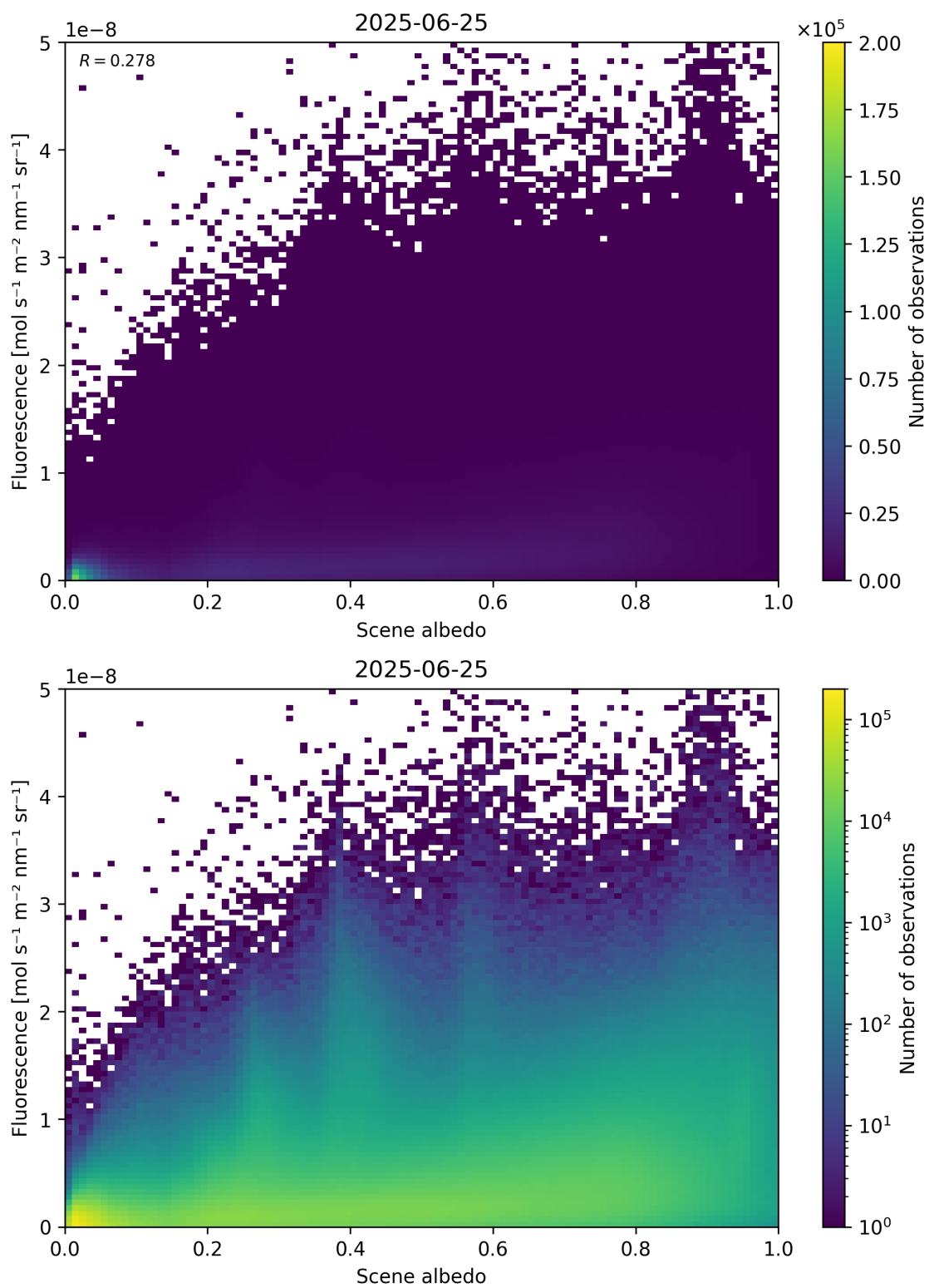
Figure 104: Scatter density plot of “Scene albedo” against “Fluorescence” for 2025-06-24 to 2025-06-26.
