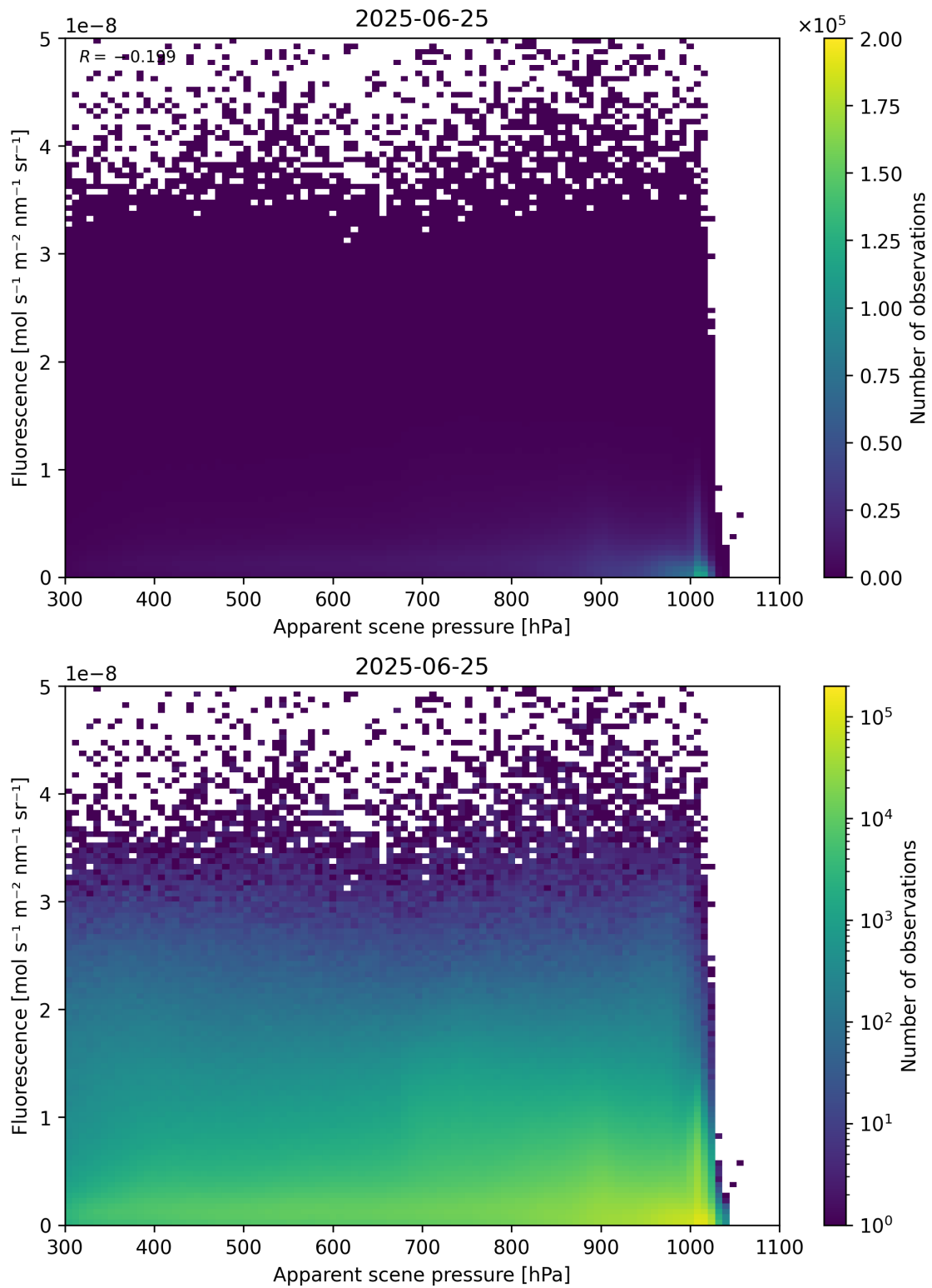
Figure 64: Scatter density plot of “Apparent scene pressure” against “Fluorescence” for 2025-06-24 to 2025-06-26.
