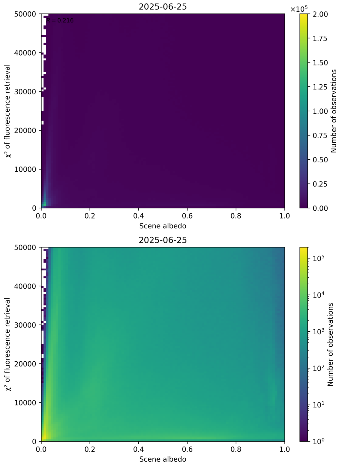
Figure 103: Scatter density plot of “Scene albedo” against “ \chi^2 of fluorescence retrieval” for 2025-06-24 to 2025-06-26.
