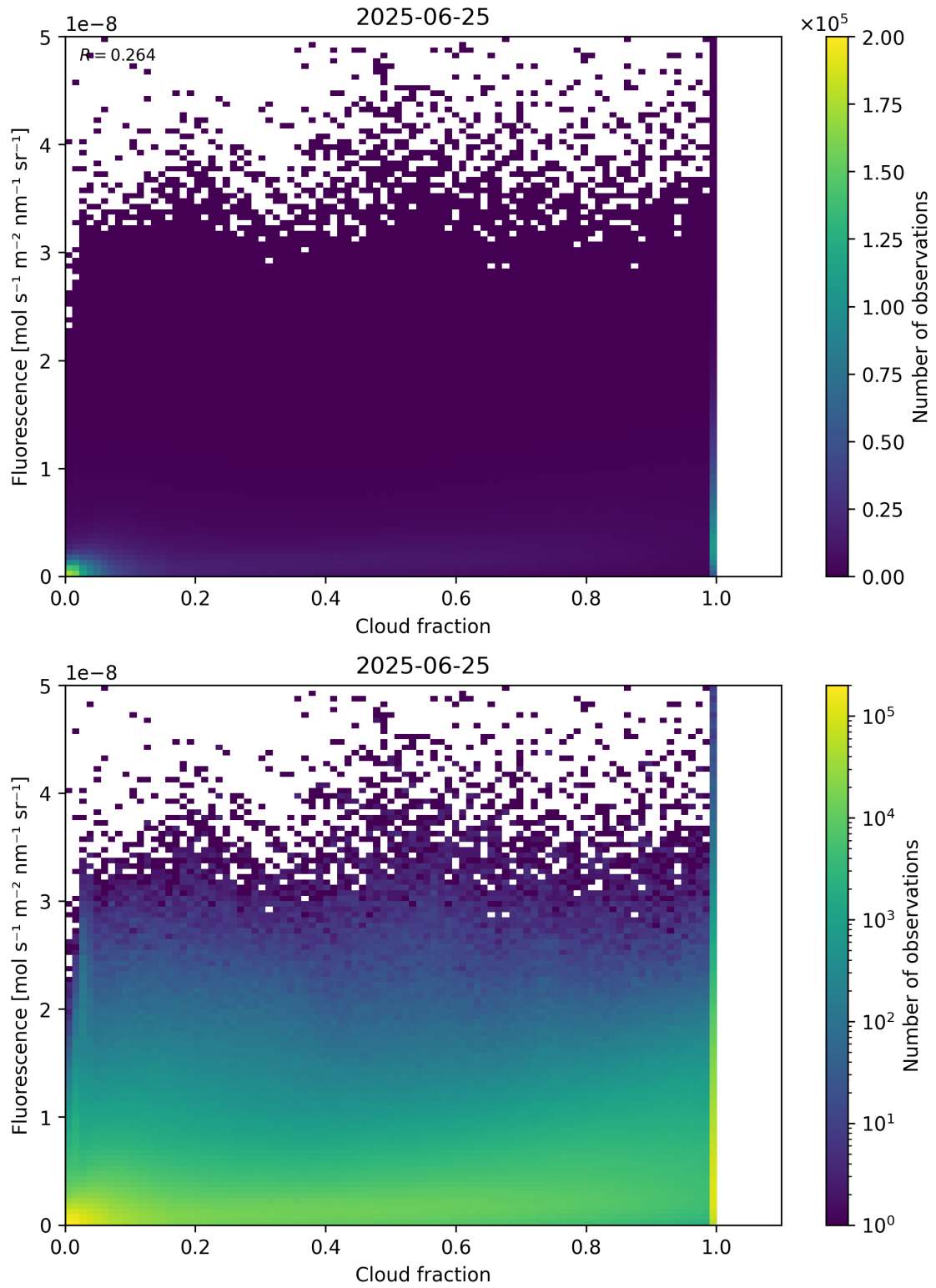
Figure 72: Scatter density plot of “Cloud fraction” against “Fluorescence” for 2025-06-24 to 2025-06-26.
