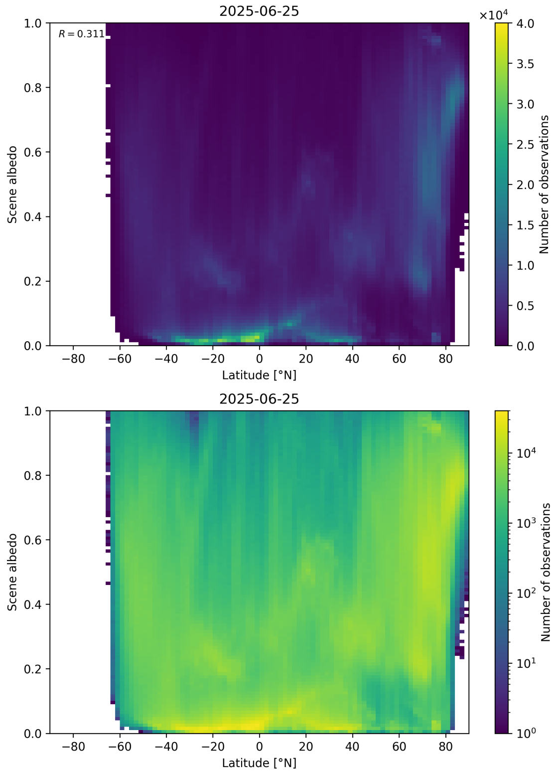
Figure 95: Scatter density plot of “Latitude” against “Scene albedo” for 2025-06-24 to 2025-06-26.
