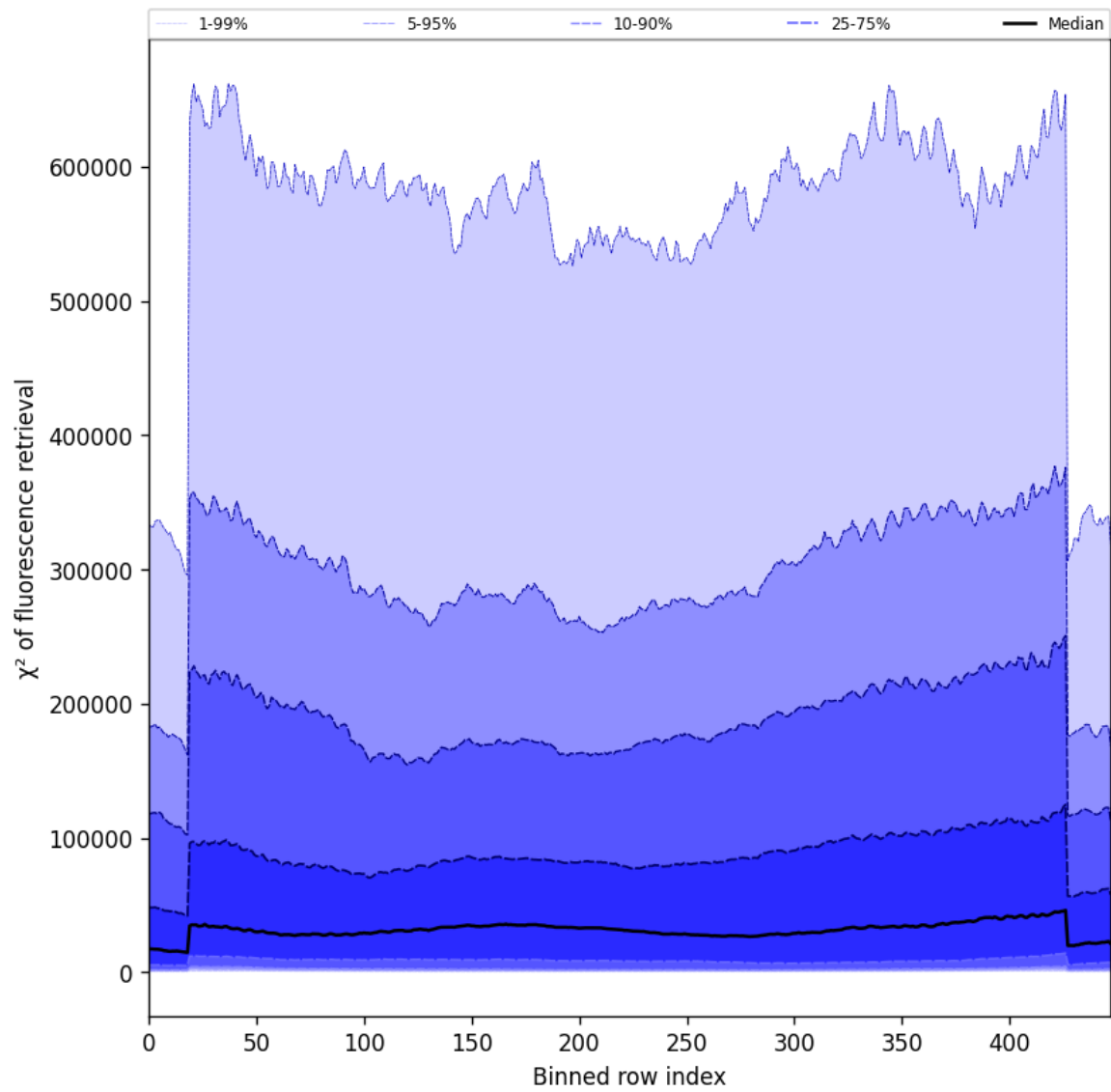
Figure 59: Along track statistics of “ \chi^2 of fluorescence retrieval” for 2025-06-24 to 2025-06-26
