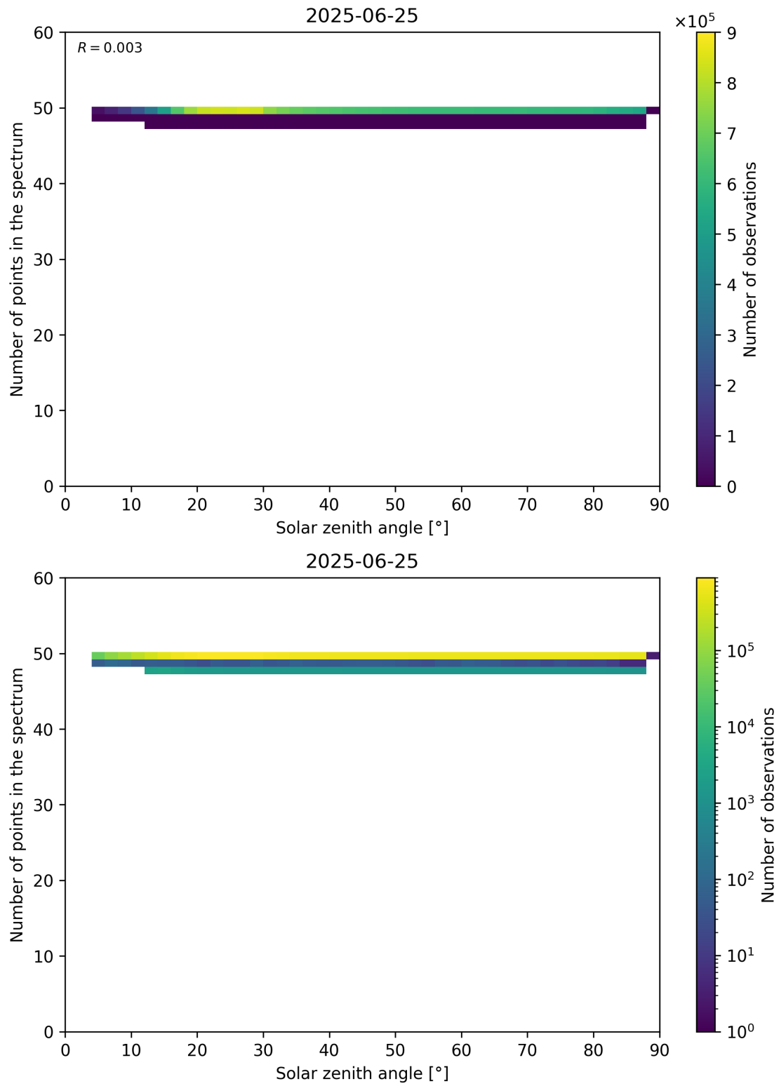
Figure 115: Scatter density plot of “Solar zenith angle” against “Number of points in the spectrum” for 2025-06-24 to 2025-06-26.
