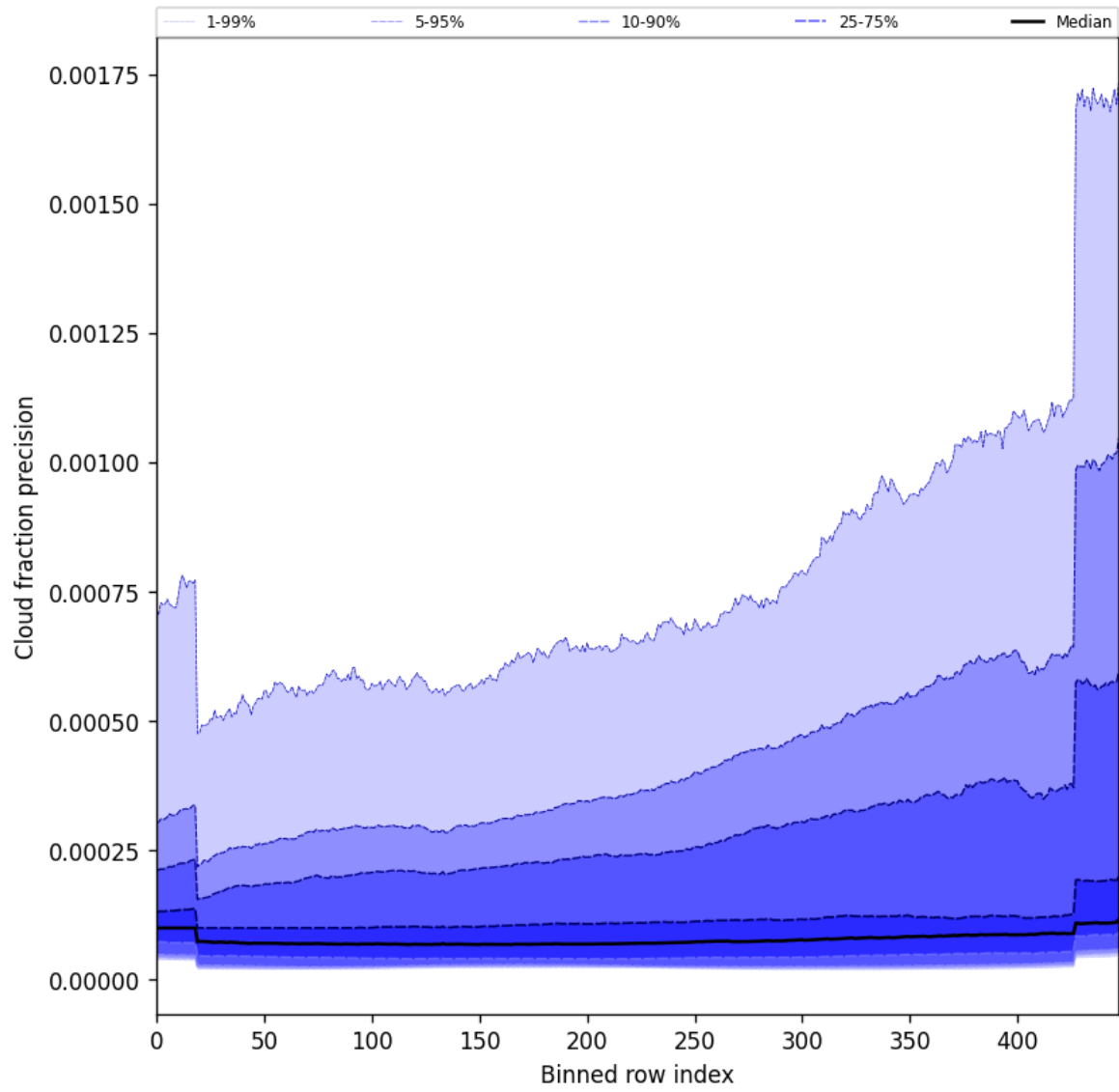
Figure 50: Along track statistics of “Cloud fraction precision” for 2025-06-24 to 2025-06-26
