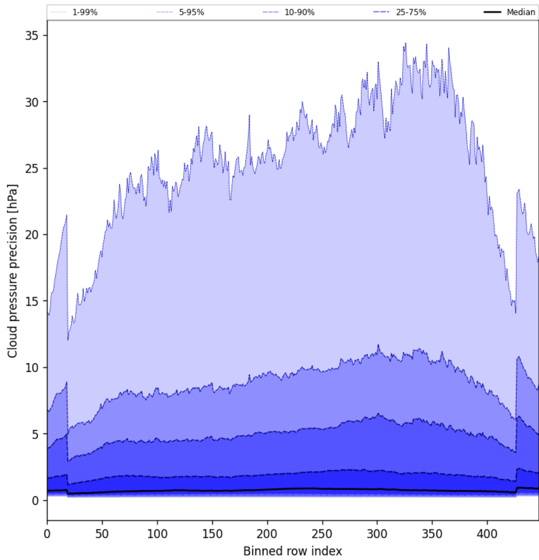
Figure 48: Along track statistics of “Cloud pressure precision” for 2025-06-24 to 2025-06-26
