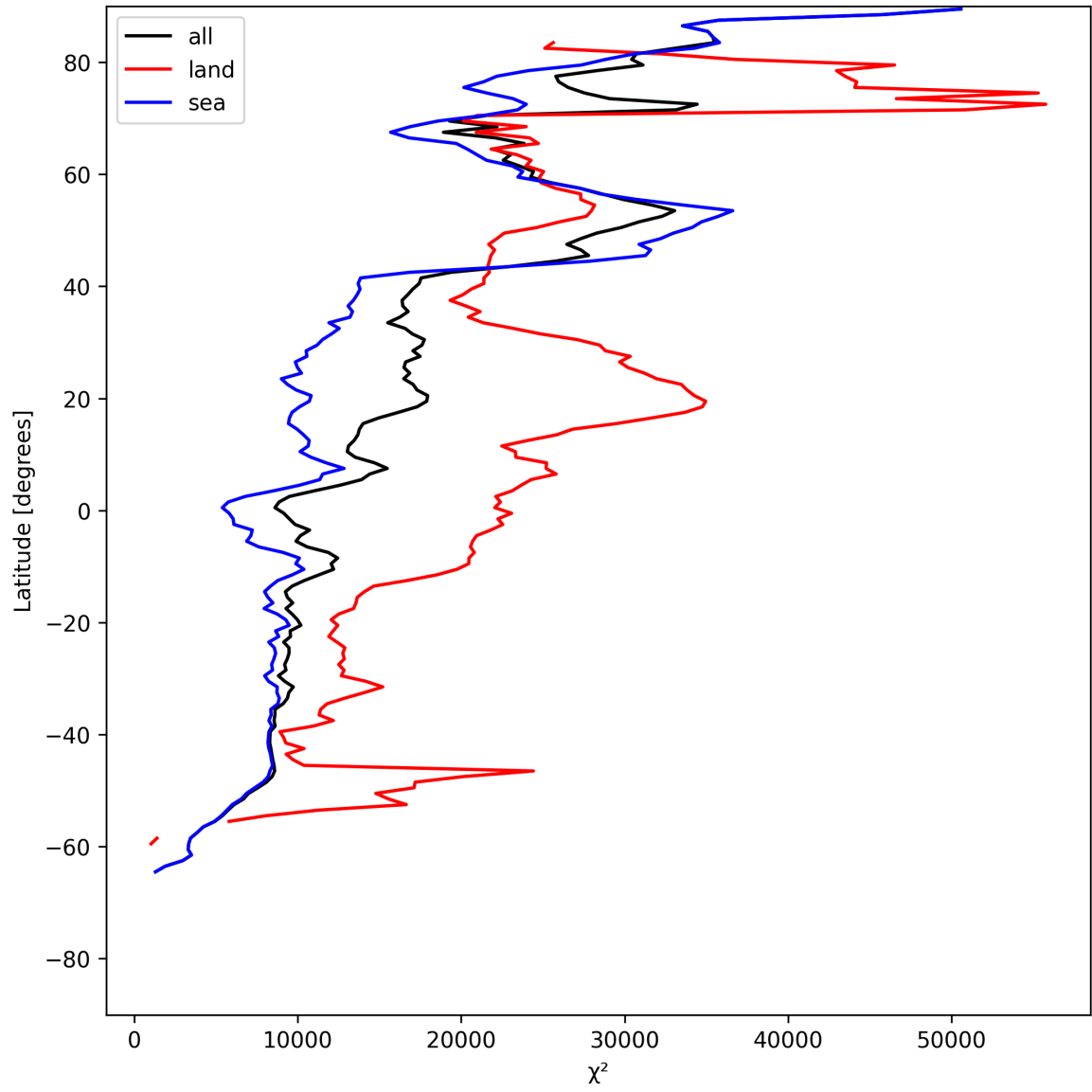
Figure 21: Zonal average of “ \chi^2 ” for 2025-06-24 to 2025-06-26.
