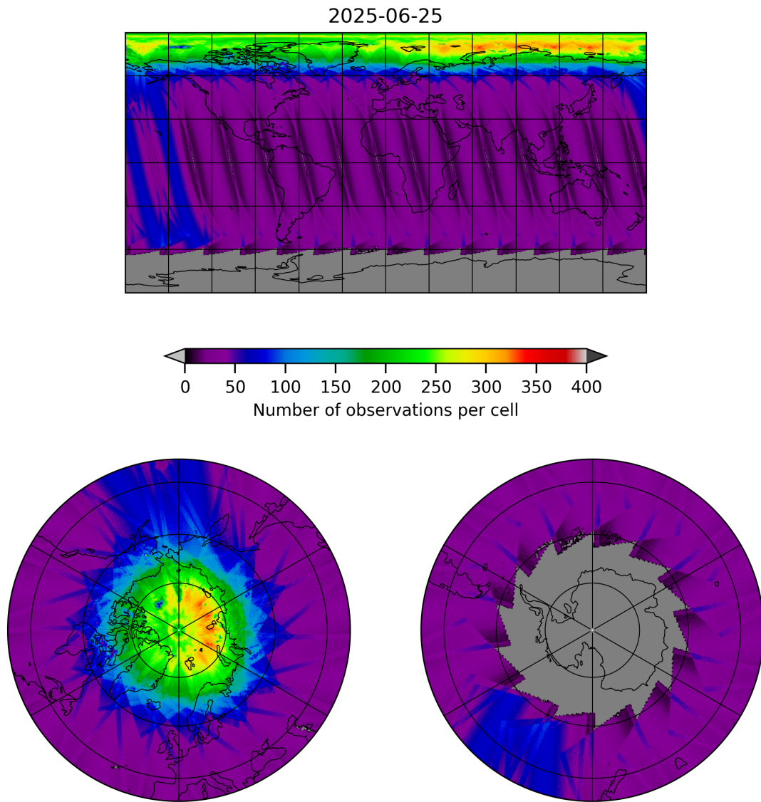
Figure 11: Map of the number of observations for 2025-06-24 to 2025-06-26
