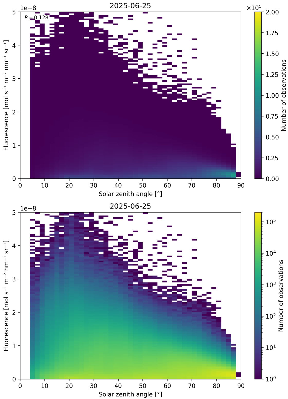
Figure 112: Scatter density plot of “Solar zenith angle” against “Fluorescence” for 2025-06-24 to 2025-06-26.
