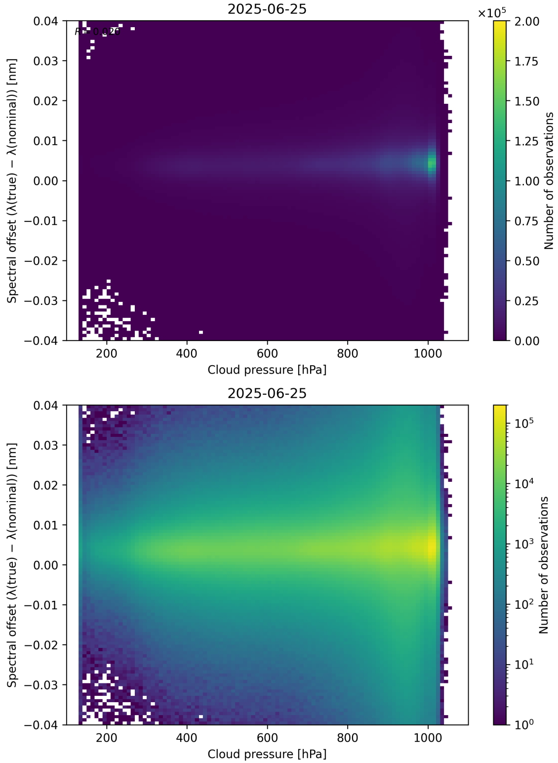
Figure 84: Scatter density plot of “Cloud pressure” against “Spectral offset ( \lambda_{\text{true}} - \lambda_{\text{nominal}} )” for 2025-06-24 to 2025-06-26.
