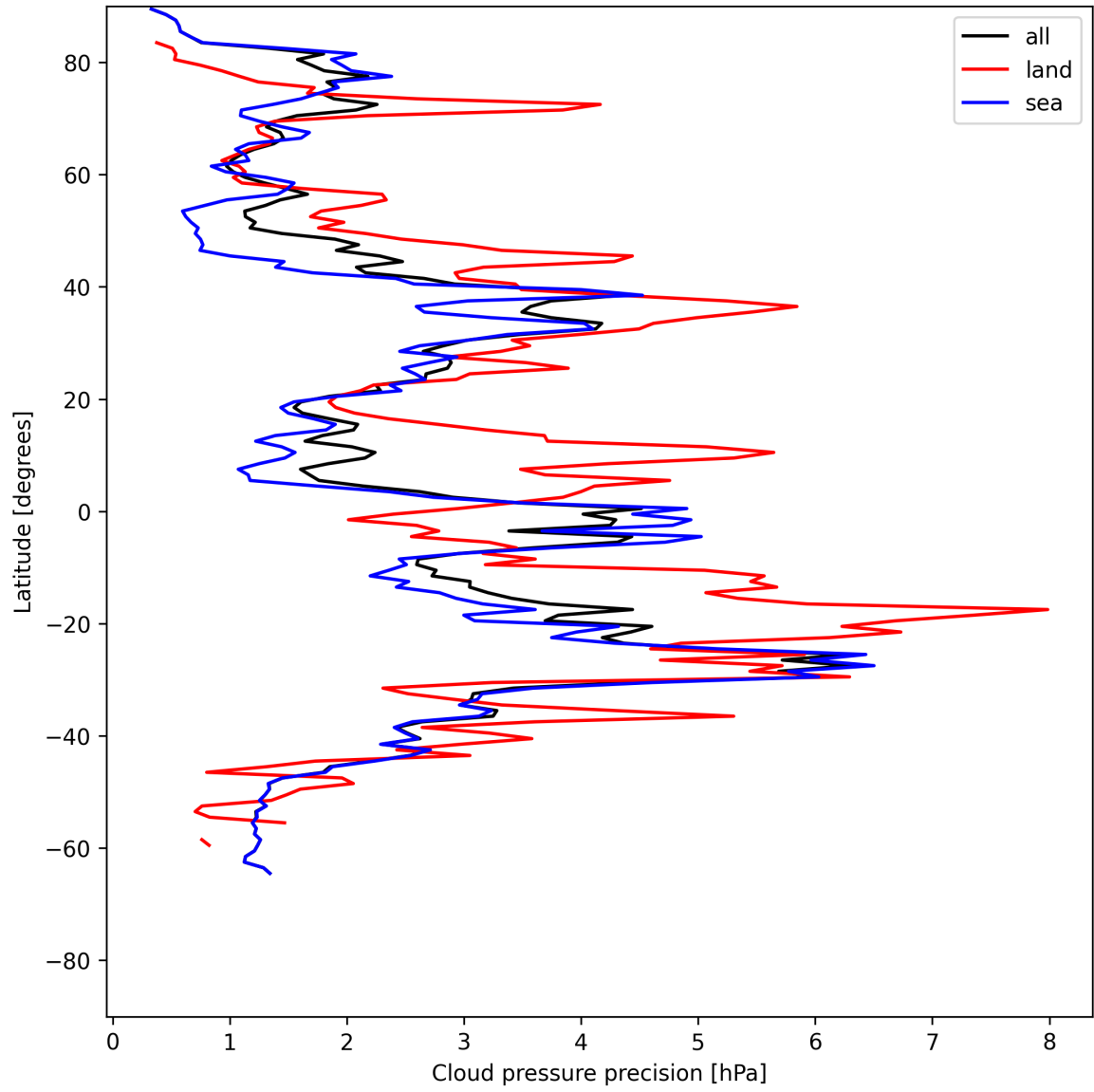
Figure 14: Zonal average of “Cloud pressure precision” for 2025-06-24 to 2025-06-26.
