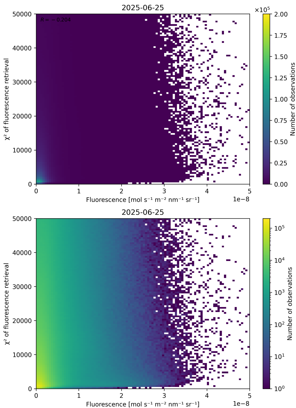
Figure 85: Scatter density plot of “Fluorescence” against “ \chi^2 of fluorescence retrieval” for 2025-06-24 to 2025-06-26.
