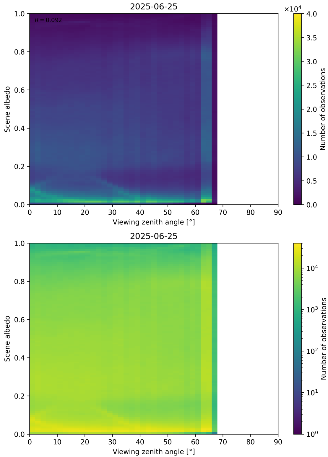
Figure 126: Scatter density plot of “Viewing zenith angle” against “Scene albedo” for 2025-06-24 to 2025-06-26.
