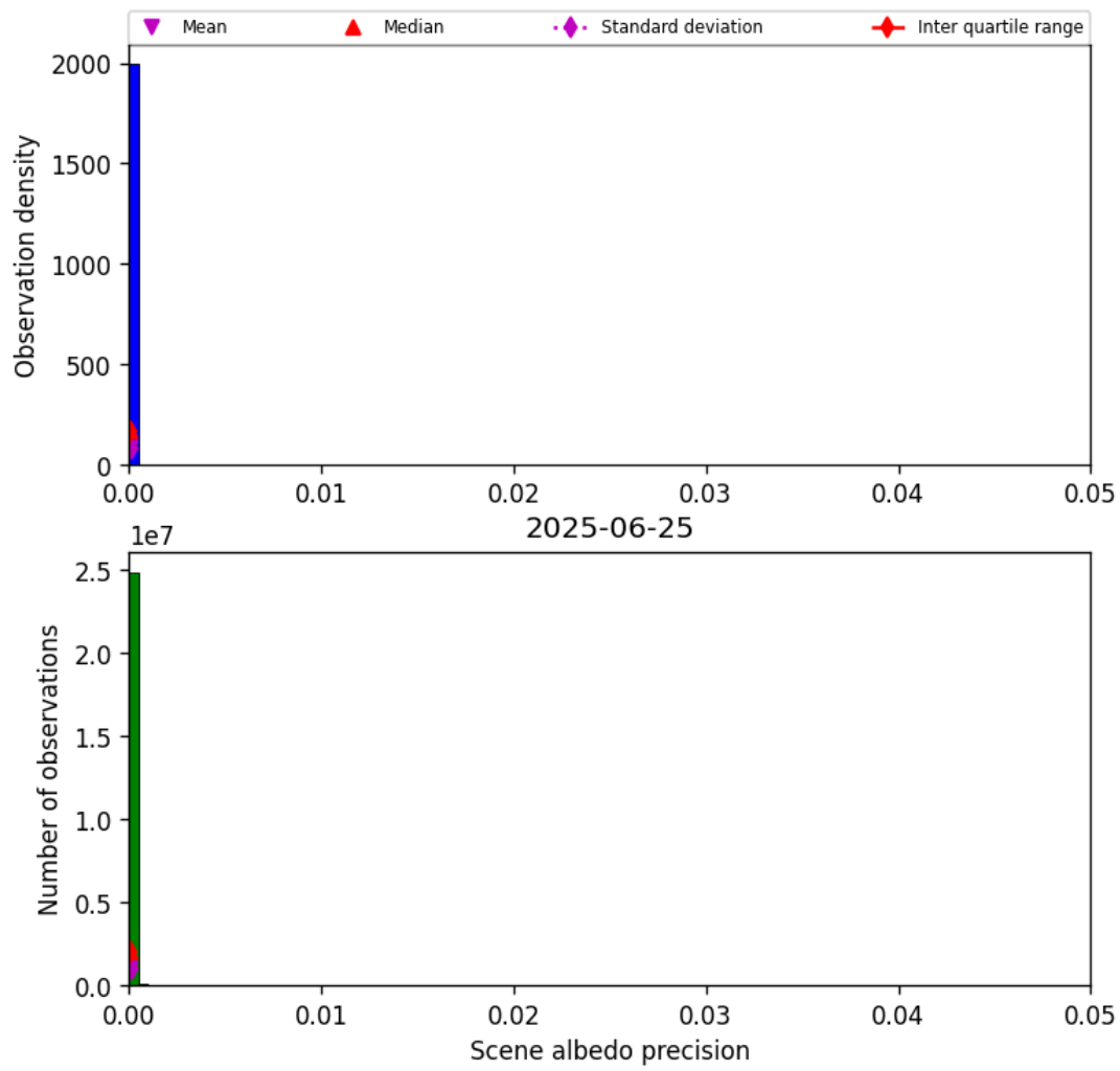
Figure 35: Histogram of “Scene albedo precision” for 2025-06-24 to 2025-06-26
