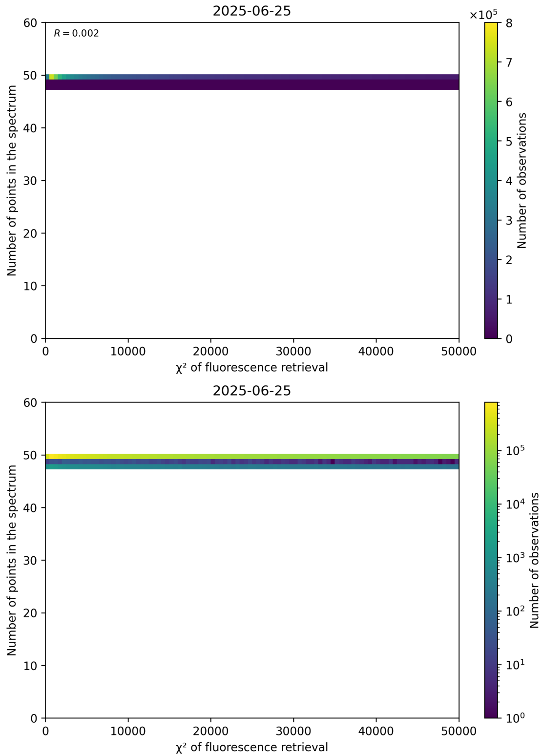
Figure 68: Scatter density plot of “ \chi^2 of fluorescence retrieval” against “Number of points in the spectrum” for 2025-06-24 to 2025-06-26.
