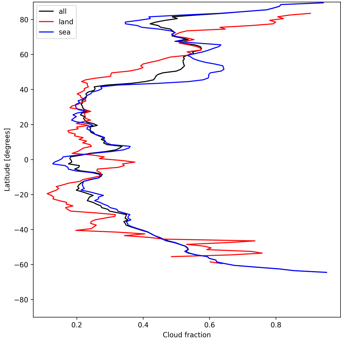
Figure 15: Zonal average of “Cloud fraction” for 2025-06-24 to 2025-06-26.
