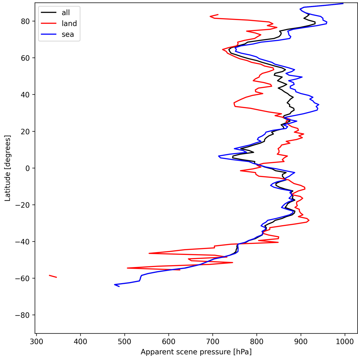
Figure 19: Zonal average of “Apparent scene pressure” for 2025-06-24 to 2025-06-26.
