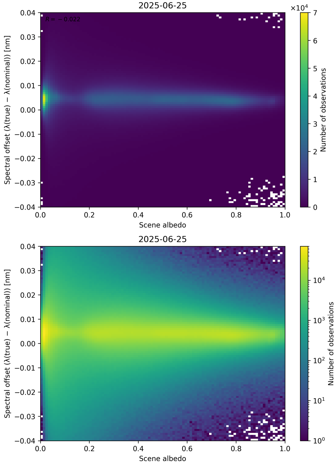
Figure 107: Scatter density plot of “Scene albedo” against “Spectral offset ( \lambda_{\text{true}} - \lambda_{\text{nominal}} )” for 2025-06-24 to 2025-06-26.
