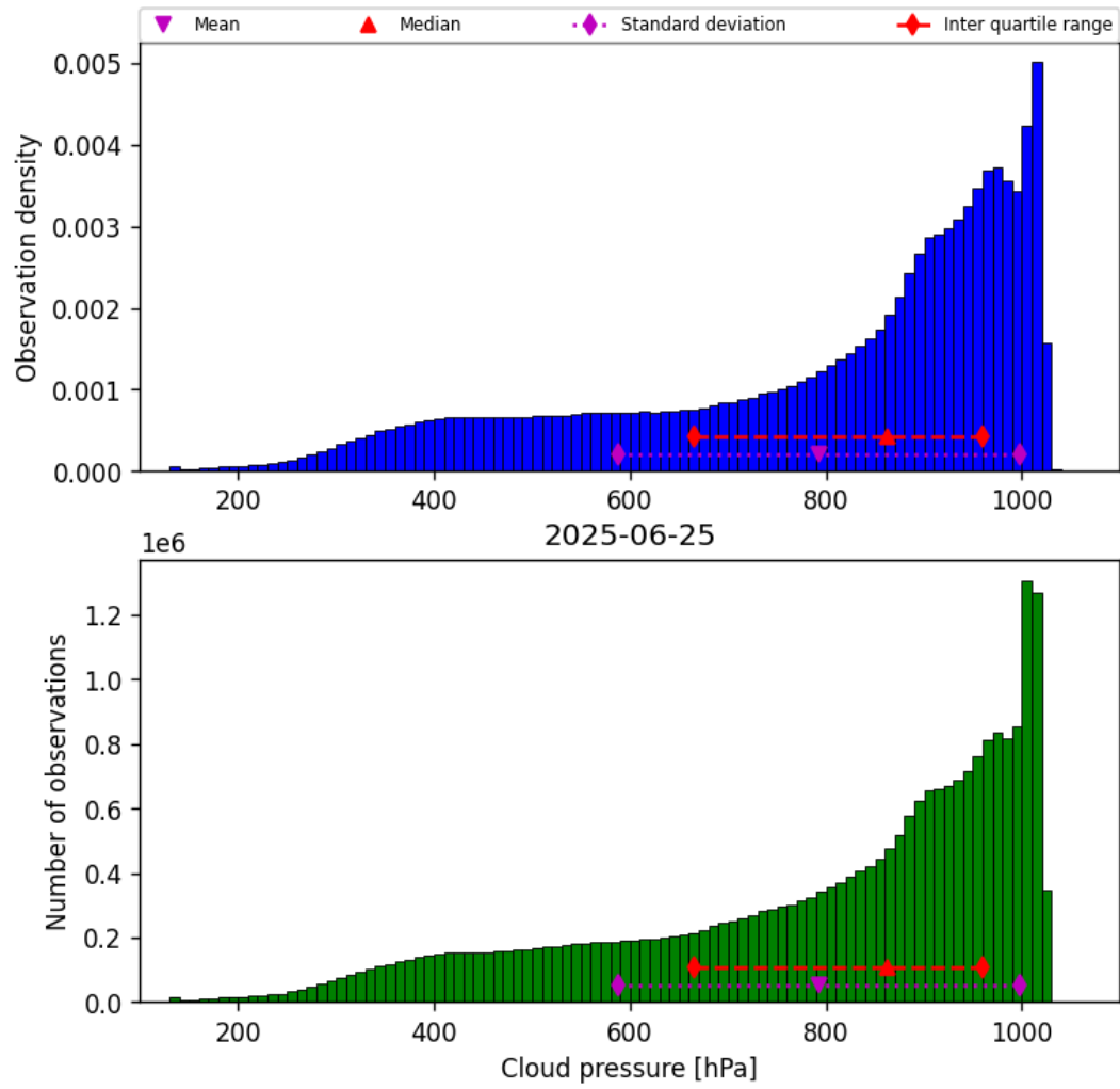
Figure 30: Histogram of “Cloud pressure” for 2025-06-24 to 2025-06-26
