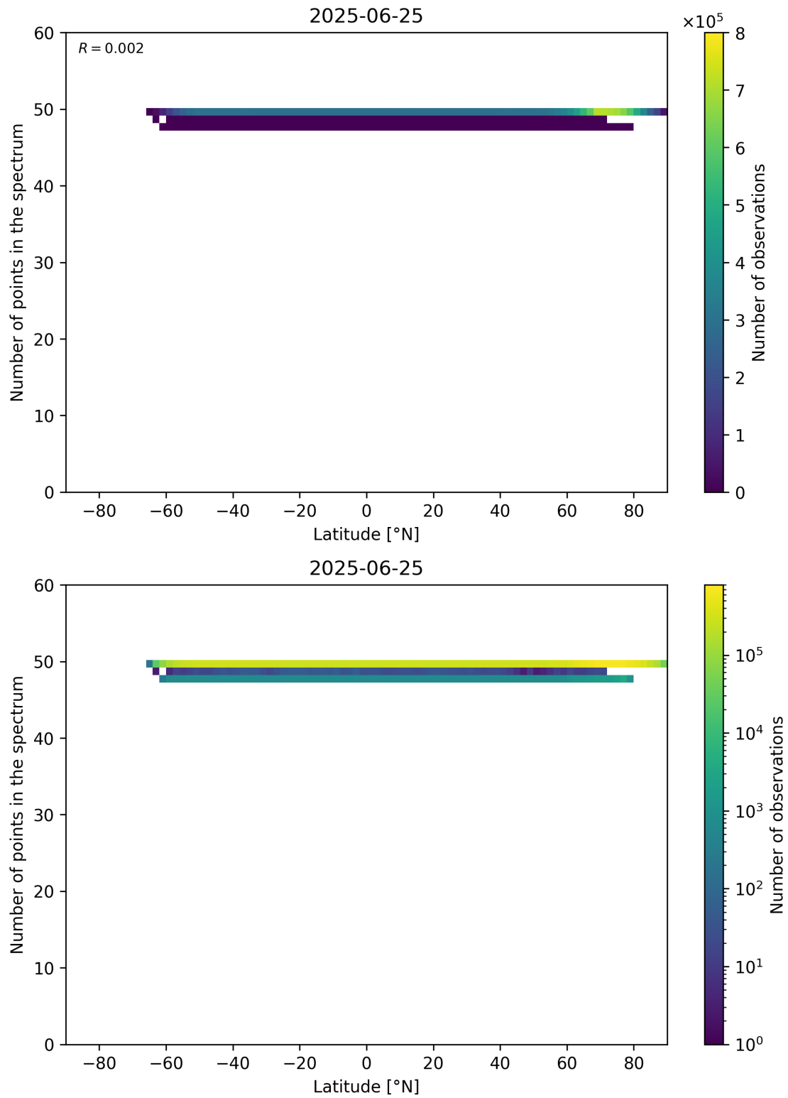
Figure 94: Scatter density plot of “Latitude” against “Number of points in the spectrum” for 2025-06-24 to 2025-06-26.
