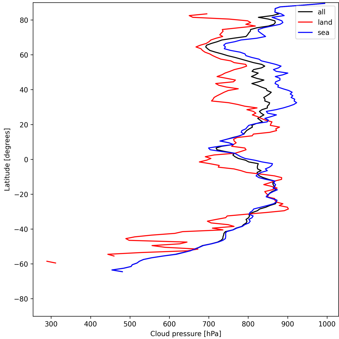
Figure 13: Zonal average of “Cloud pressure” for 2025-06-24 to 2025-06-26.
