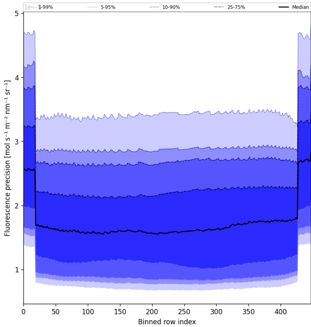
Figure 58: Along track statistics of “Fluorescence precision” for 2025-06-24 to 2025-06-26
