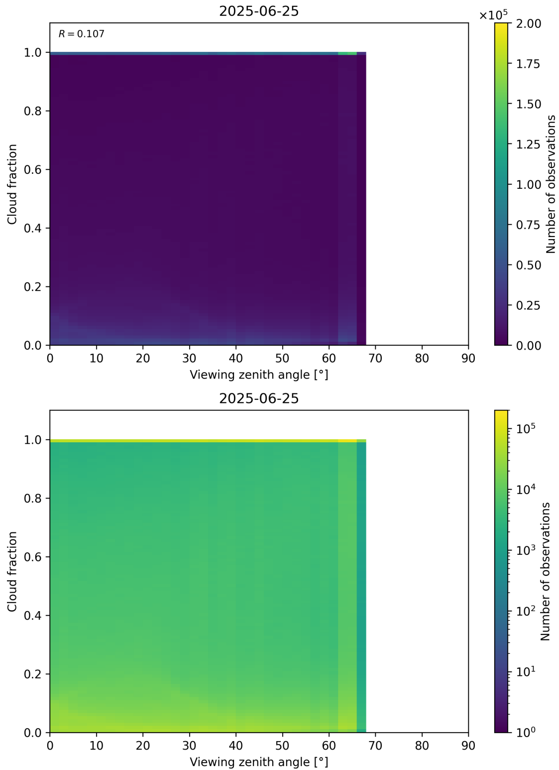
Figure 120: Scatter density plot of “Viewing zenith angle” against “Cloud fraction” for 2025-06-24 to 2025-06-26.
