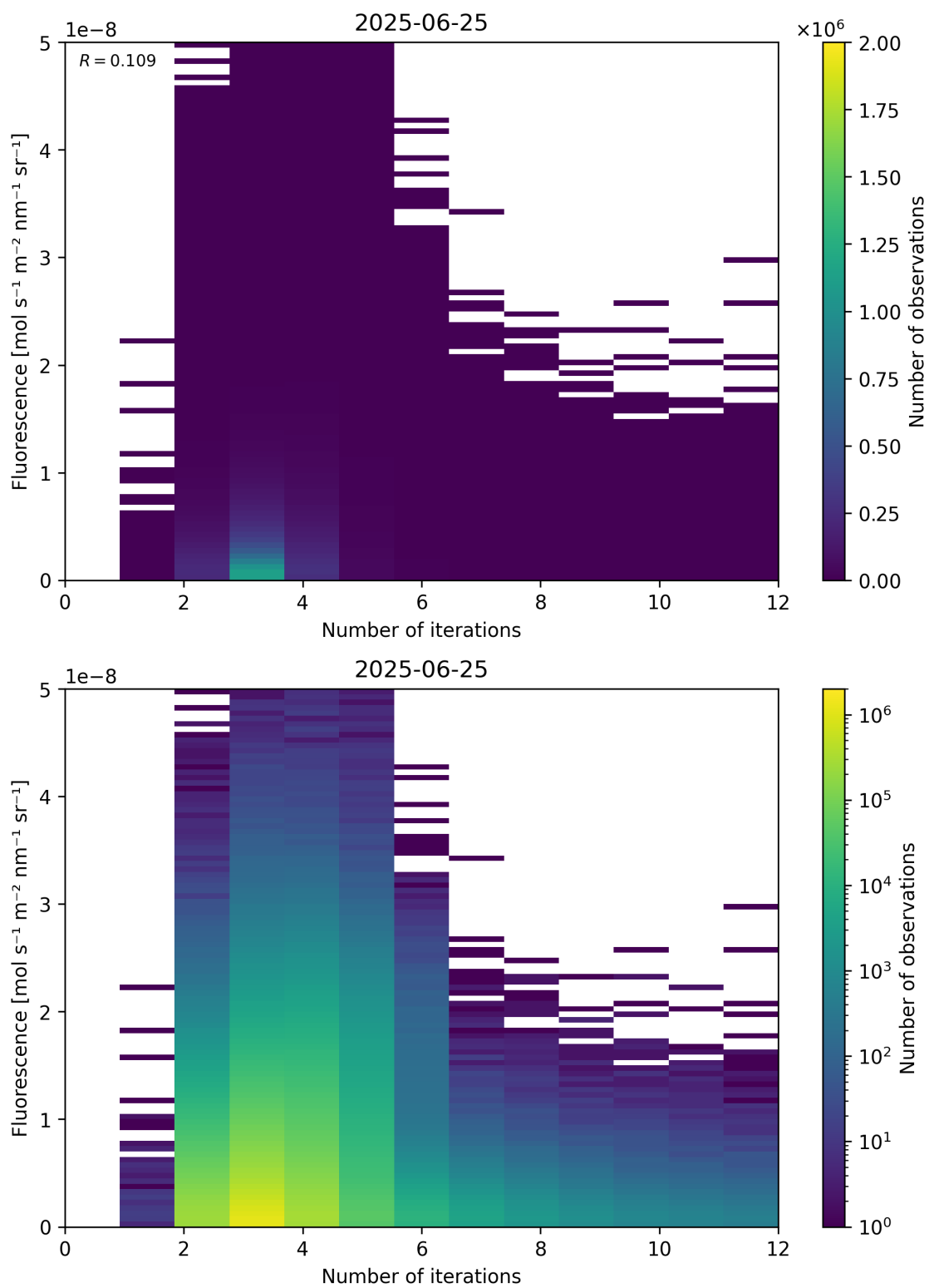
Figure 98: Scatter density plot of “Number of iterations” against “Fluorescence” for 2025-06-24 to 2025-06-26.
