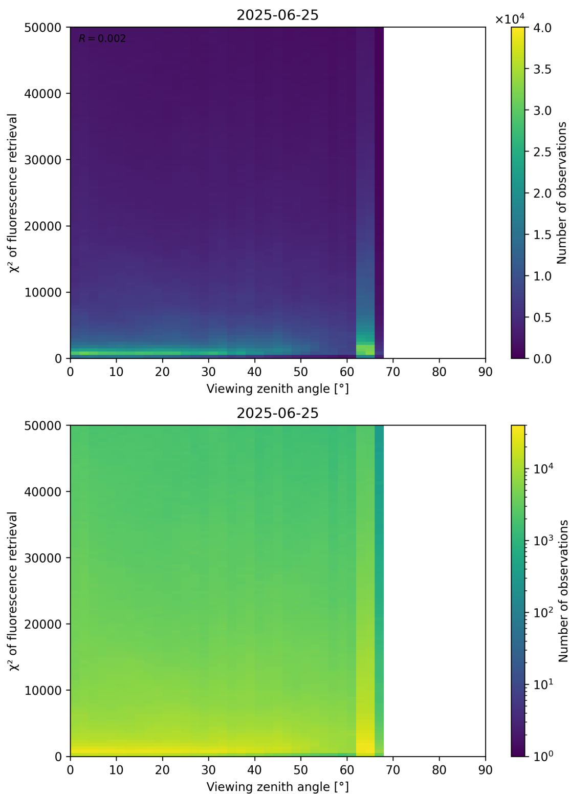
Figure 119: Scatter density plot of “Viewing zenith angle” against “ \chi^2 of fluorescence retrieval” for 2025-06-24 to 2025-06-26.
