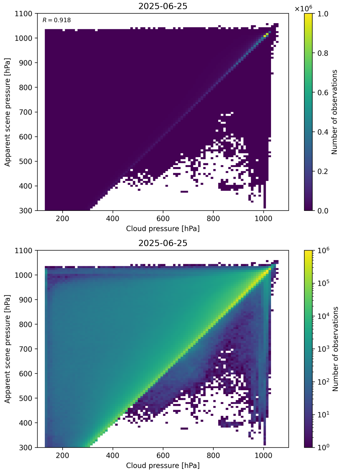
Figure 77: Scatter density plot of “Cloud pressure” against “Apparent scene pressure” for 2025-06-24 to 2025-06-26.
