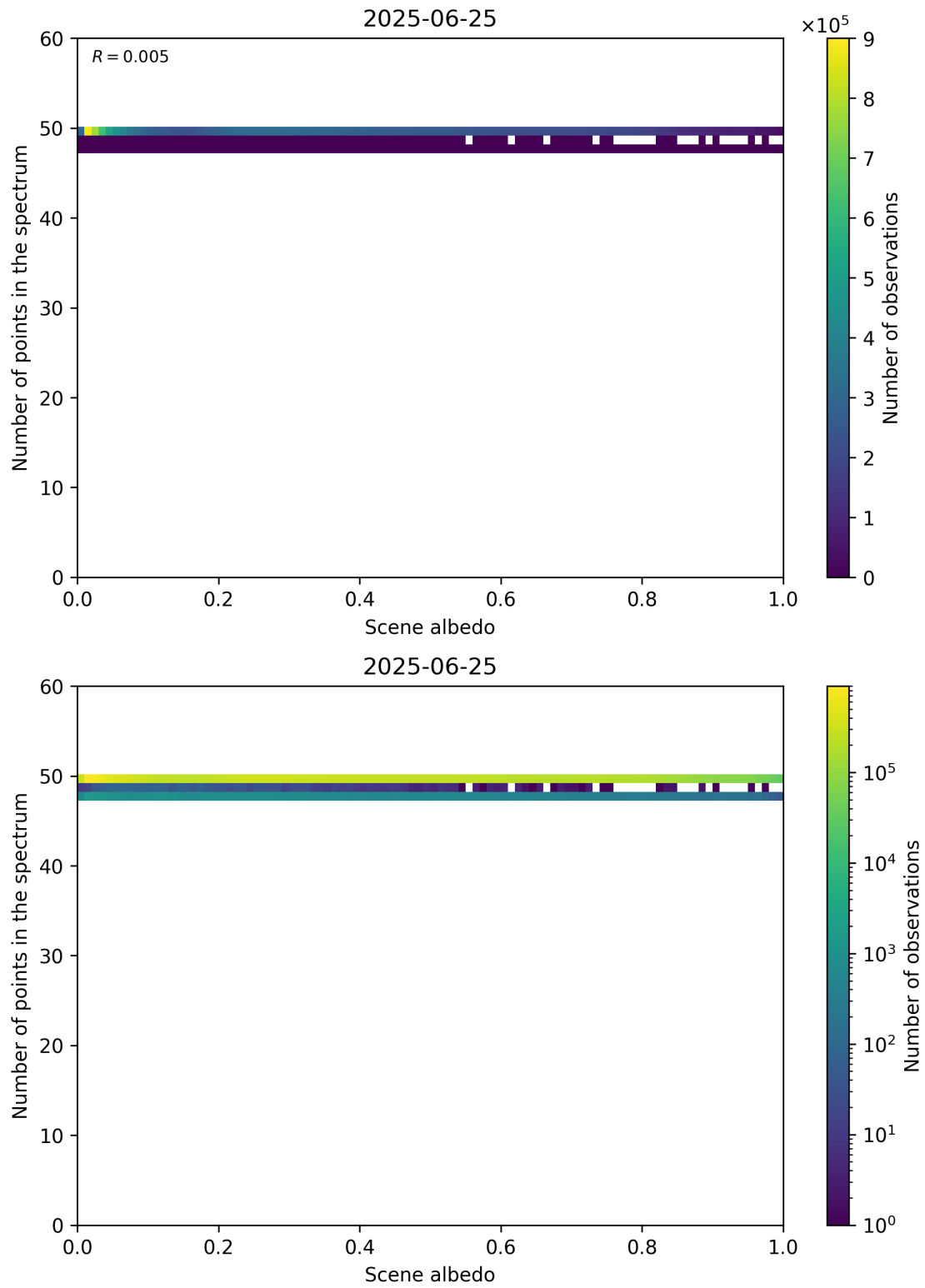
Figure 106: Scatter density plot of “Scene albedo” against “Number of points in the spectrum” for 2025-06-24 to 2025-06-26.
