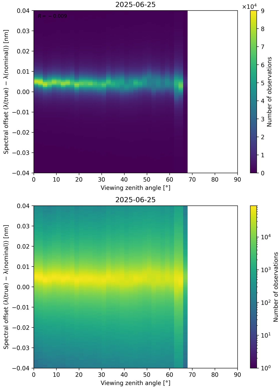
Figure 128: Scatter density plot of “Viewing zenith angle” against “Spectral offset ( \lambda_{\text{true}} - \lambda_{\text{nominal}} )” for 2025-06-24 to 2025-06-26.
