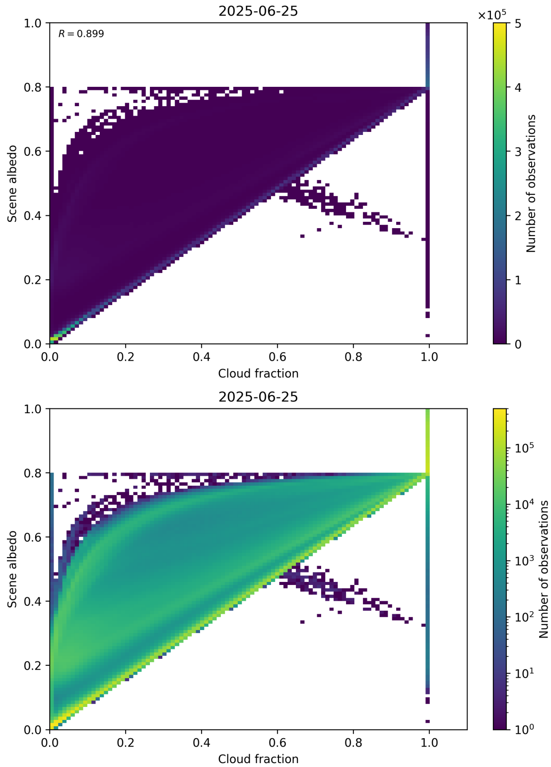
Figure 75: Scatter density plot of “Cloud fraction” against “Scene albedo” for 2025-06-24 to 2025-06-26.
