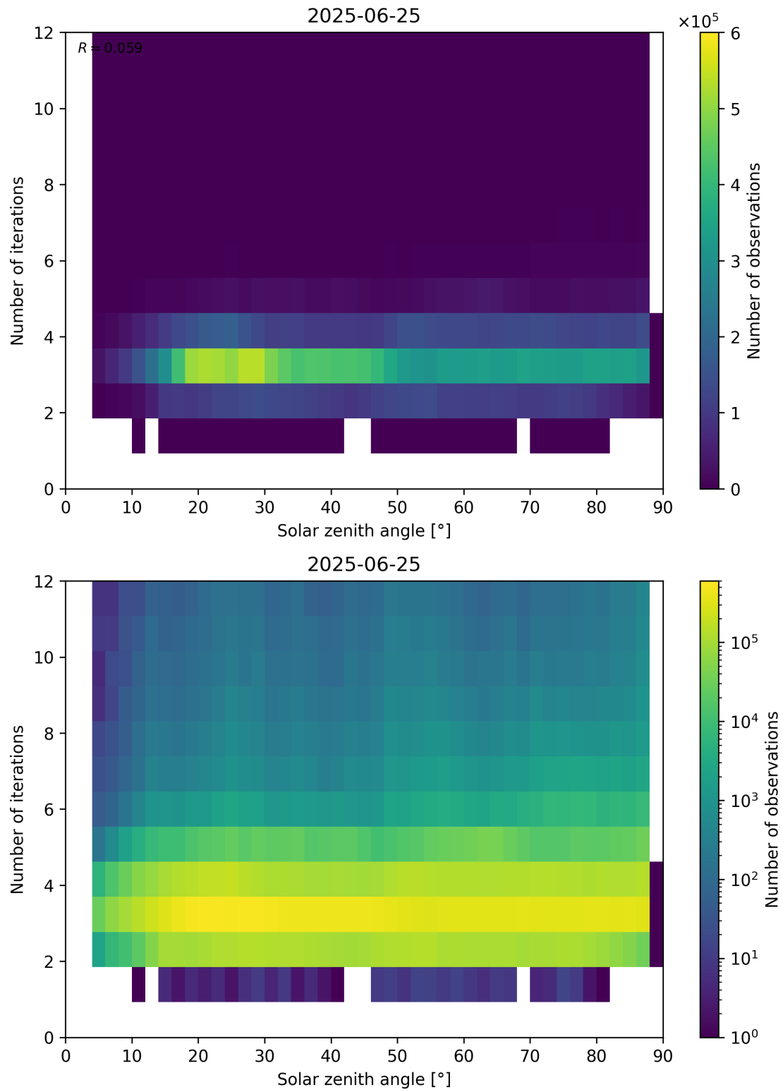
Figure 114: Scatter density plot of “Solar zenith angle” against “Number of iterations” for 2025-06-24 to 2025-06-26.
