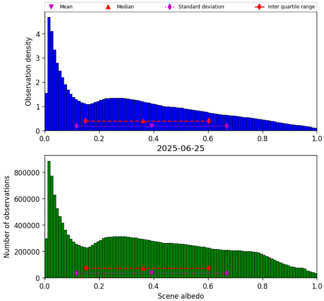
Figure 34: Histogram of “Scene albedo” for 2025-06-24 to 2025-06-26
