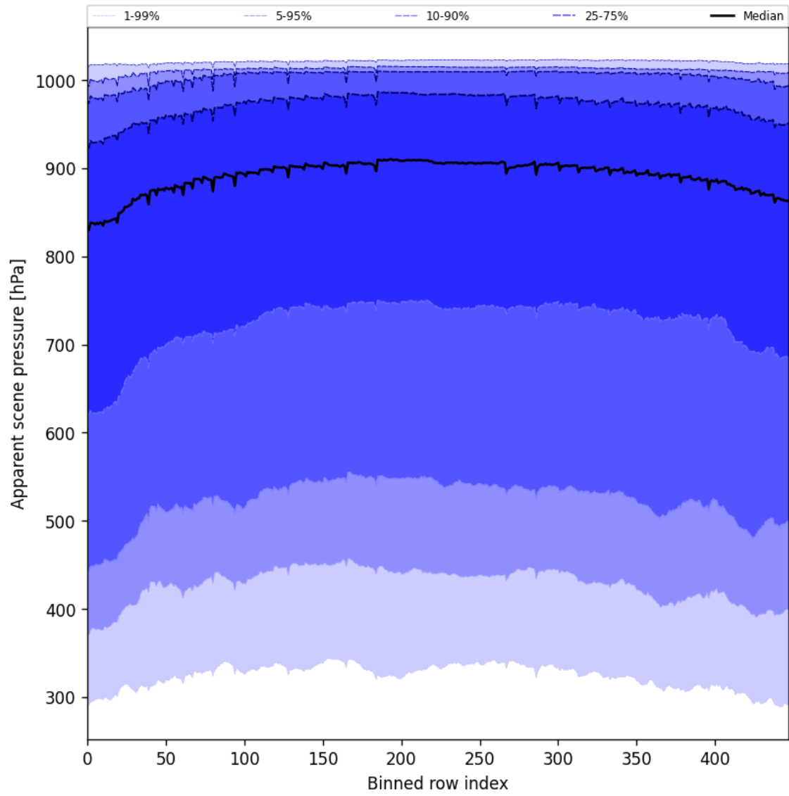
Figure 53: Along track statistics of “Apparent scene pressure” for 2025-06-24 to 2025-06-26
