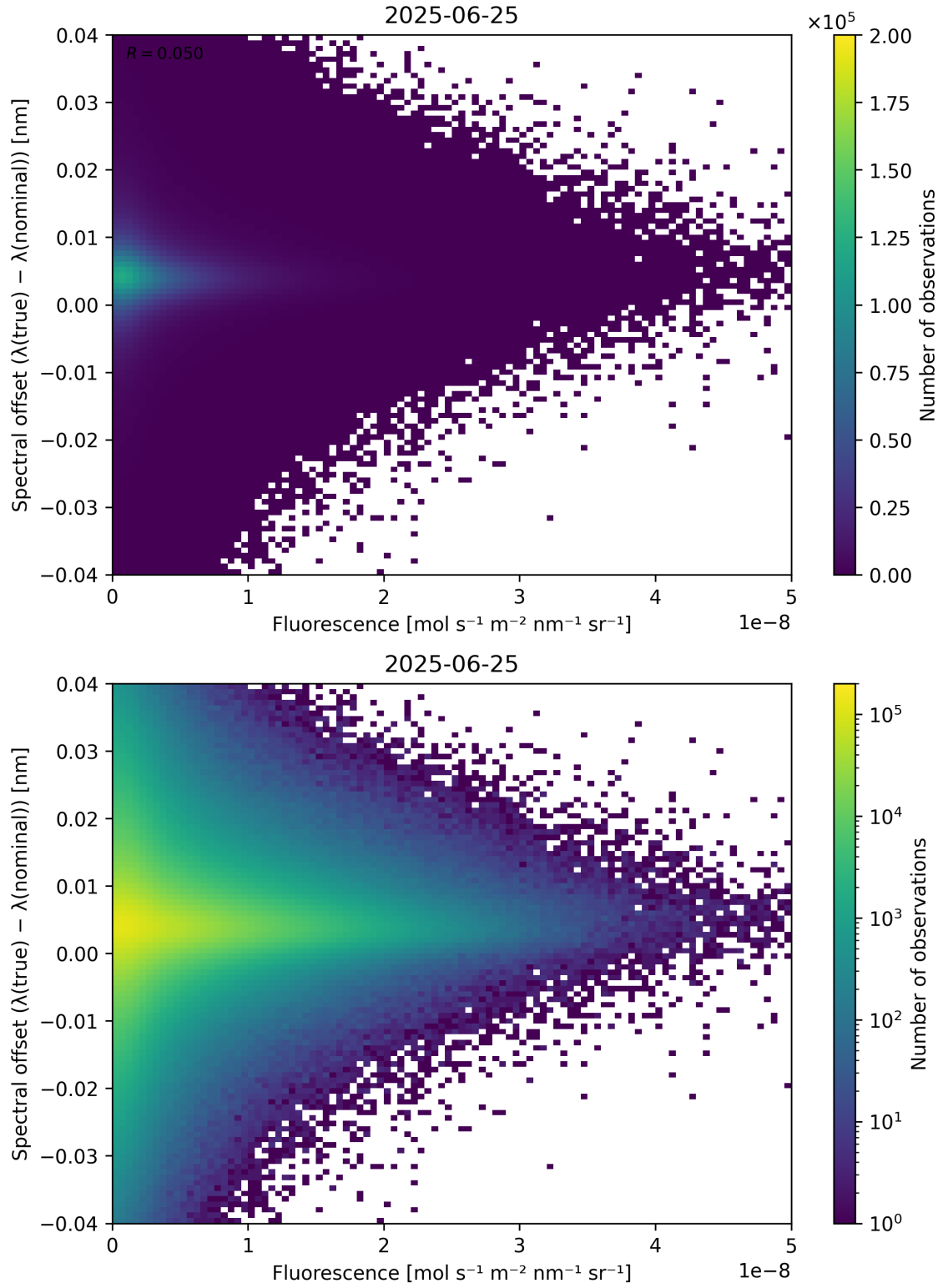
Figure 87: Scatter density plot of “Fluorescence” against “Spectral offset ( \lambda_{\text{true}} - \lambda_{\text{nominal}} )” for 2025-06-24 to 2025-06-26.
