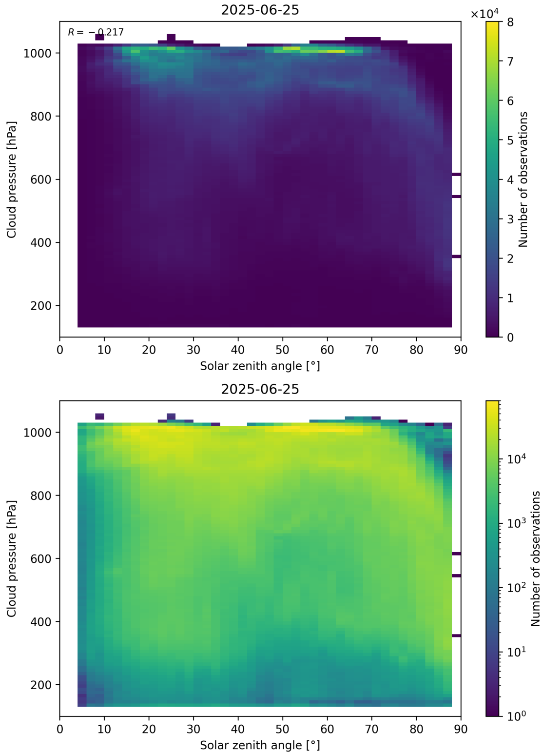
Figure 111: Scatter density plot of “Solar zenith angle” against “Cloud pressure” for 2025-06-24 to 2025-06-26.
