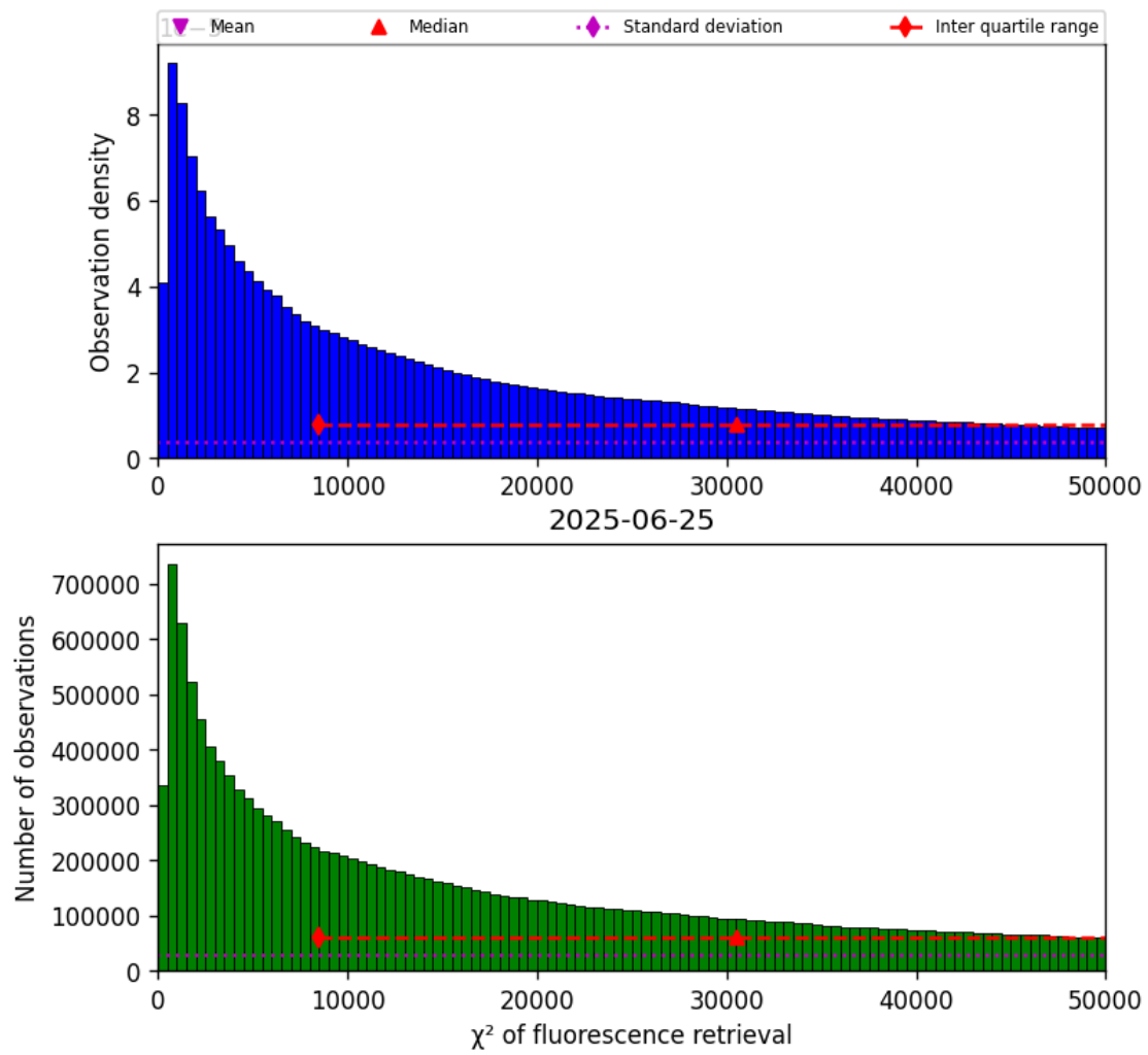
Figure 42: Histogram of “ \chi^2 of fluorescence retrieval” for 2025-06-24 to 2025-06-26
