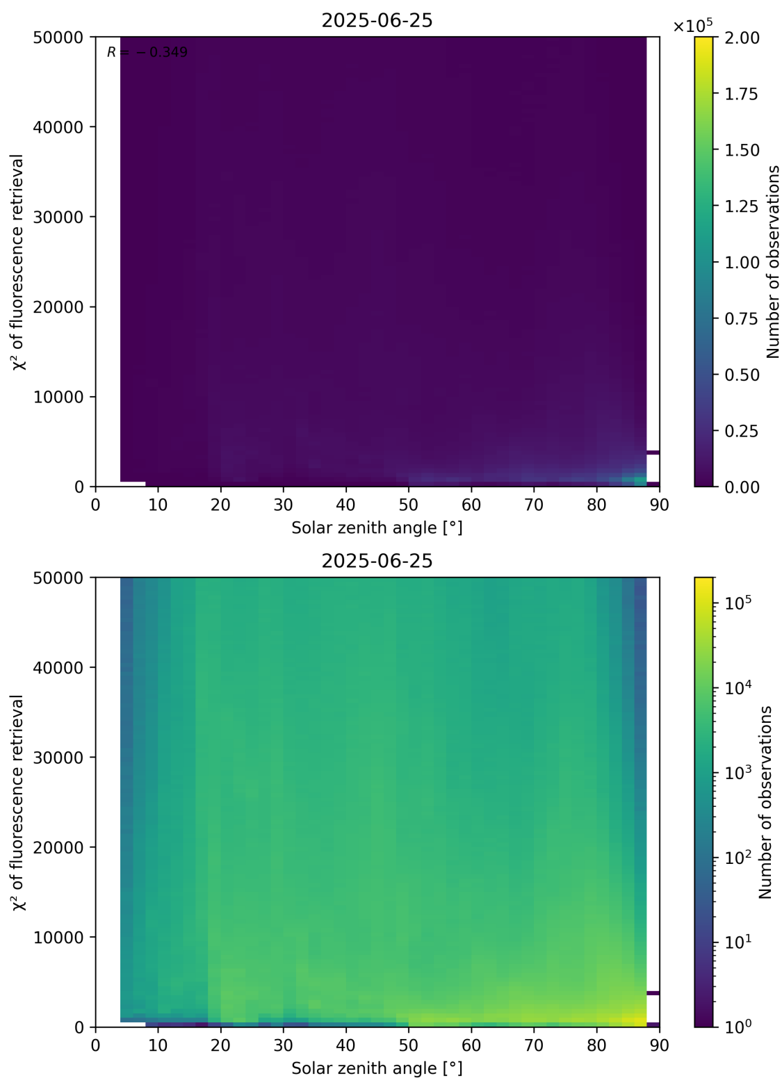
Figure 109: Scatter density plot of “Solar zenith angle” against “ \chi^2 of fluorescence retrieval” for 2025-06-24 to 2025-06-26.
