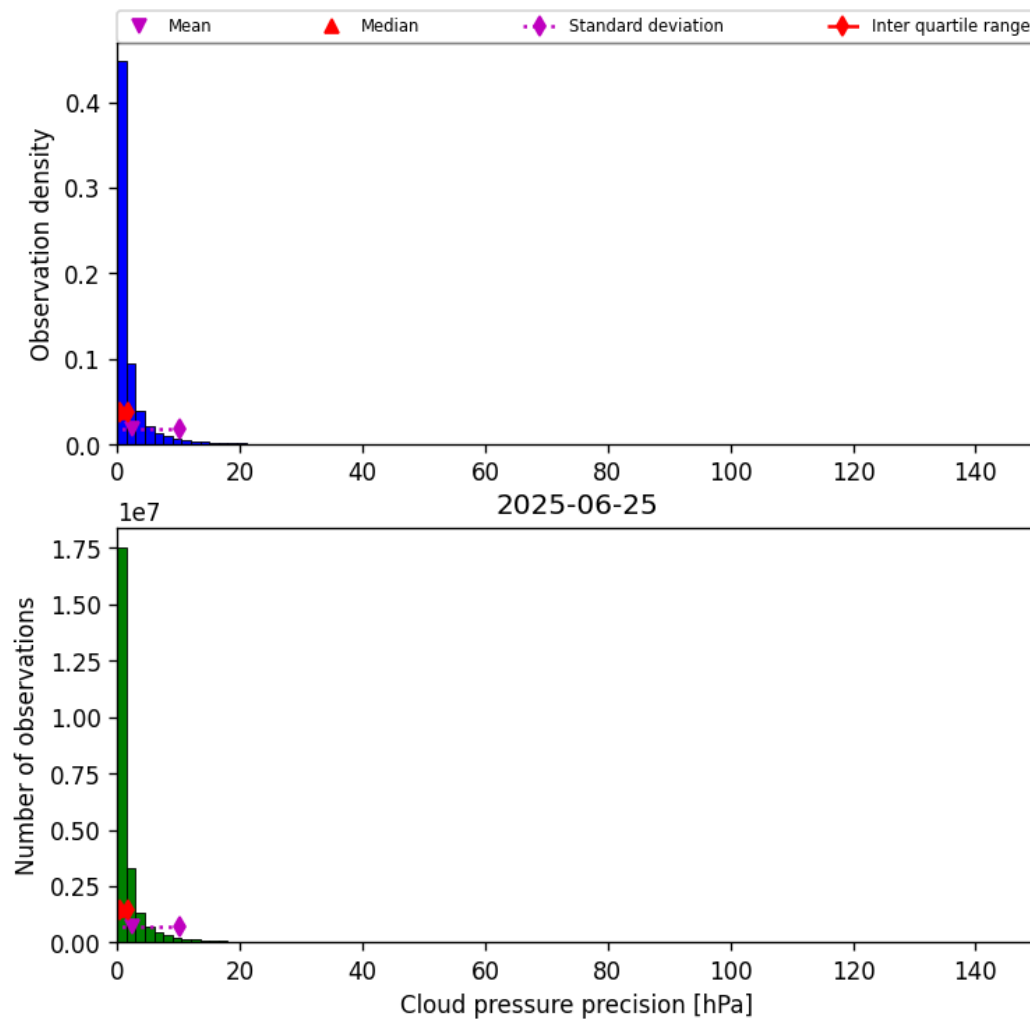
Figure 31: Histogram of “Cloud pressure precision” for 2025-06-24 to 2025-06-26
