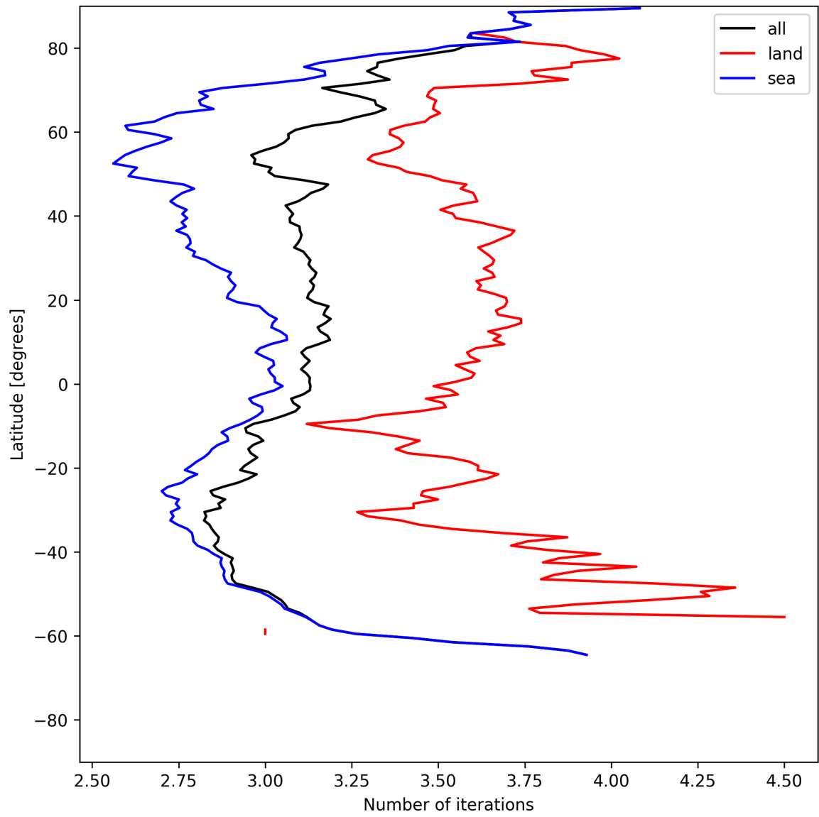
Figure 22: Zonal average of “Number of iterations” for 2025-06-24 to 2025-06-26.
