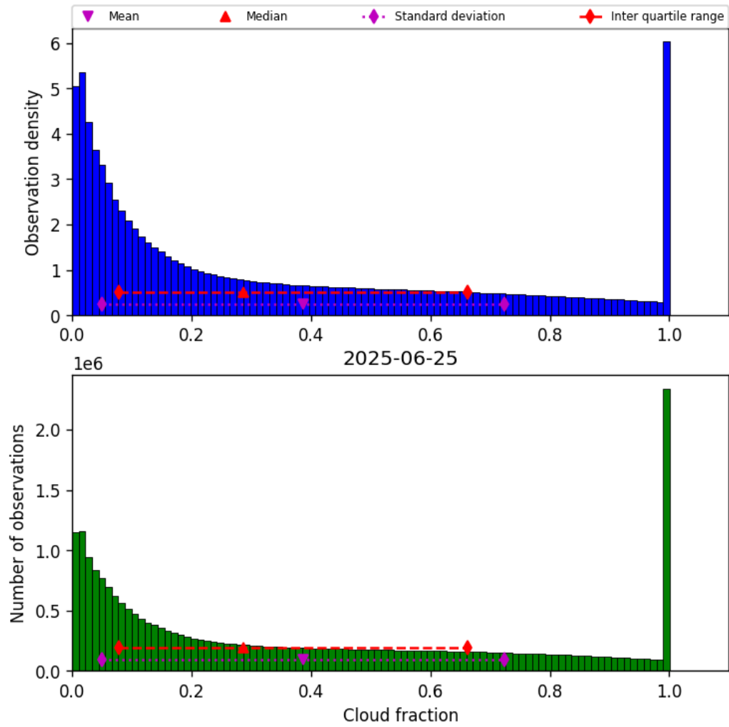
Figure 32: Histogram of “Cloud fraction” for 2025-06-24 to 2025-06-26
