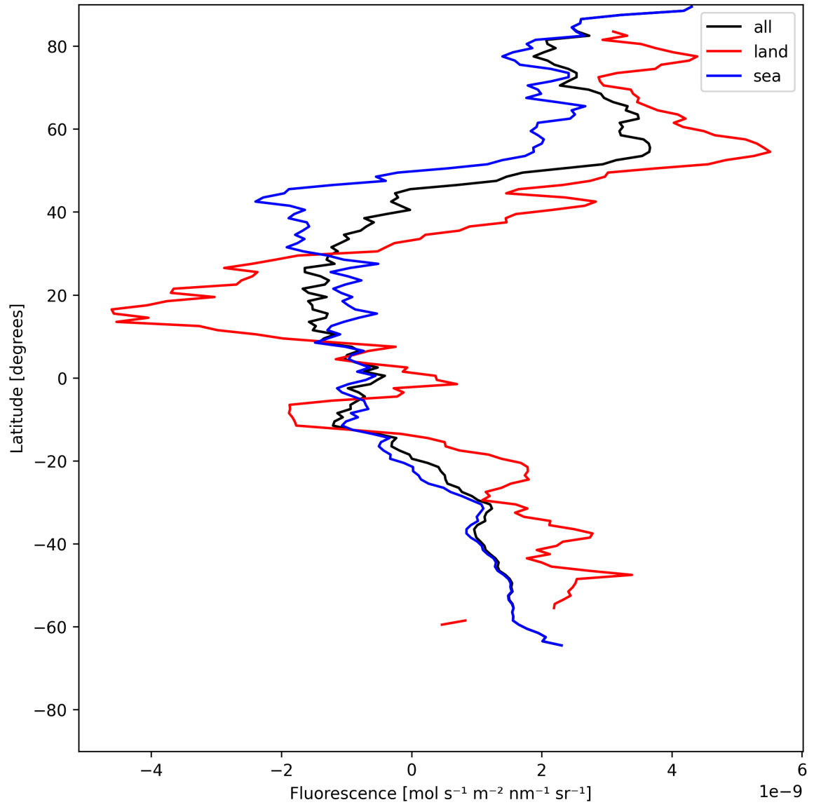
Figure 23: Zonal average of “Fluorescence” for 2025-06-24 to 2025-06-26.
