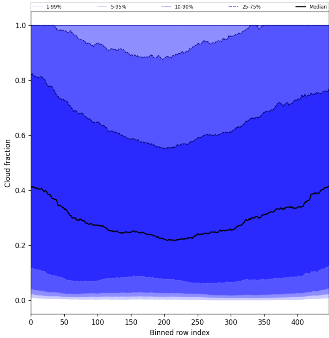
Figure 49: Along track statistics of “Cloud fraction” for 2025-06-24 to 2025-06-26
