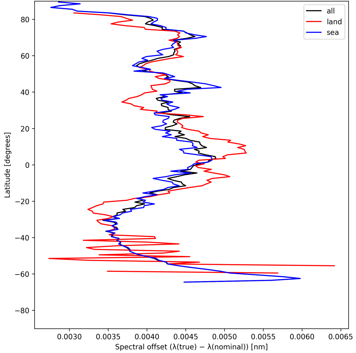
Figure 28: Zonal average of “Spectral offset ( \lambda_{\text{true}} - \lambda_{\text{nominal}} )” for 2025-06-24 to 2025-06-26.
