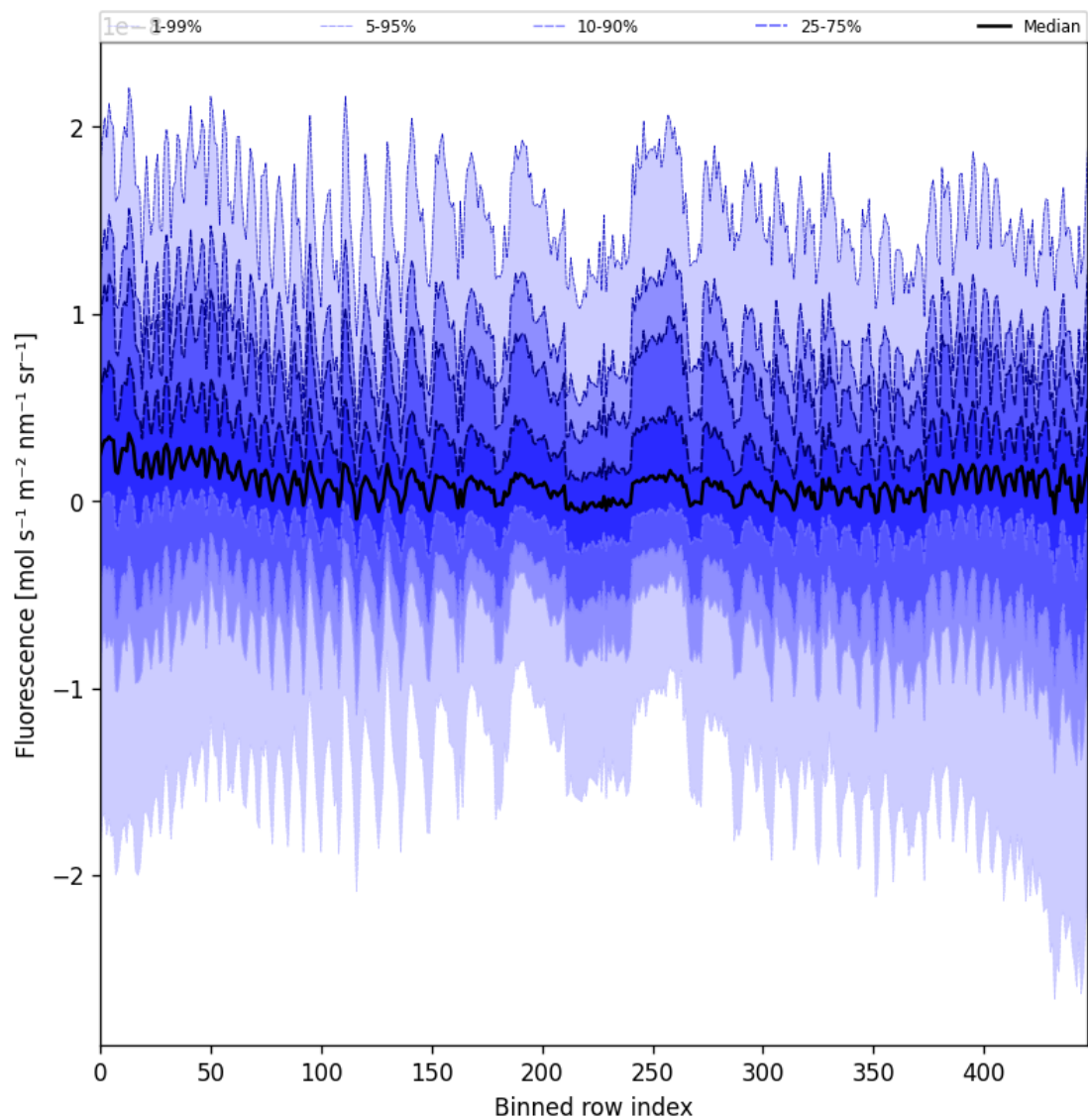
Figure 57: Along track statistics of “Fluorescence” for 2025-06-24 to 2025-06-26
