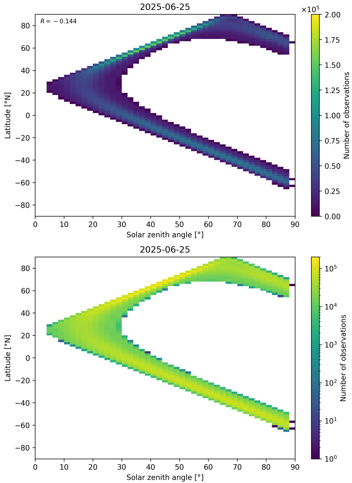
Figure 113: Scatter density plot of “Solar zenith angle” against “Latitude” for 2025-06-24 to 2025-06-26.
