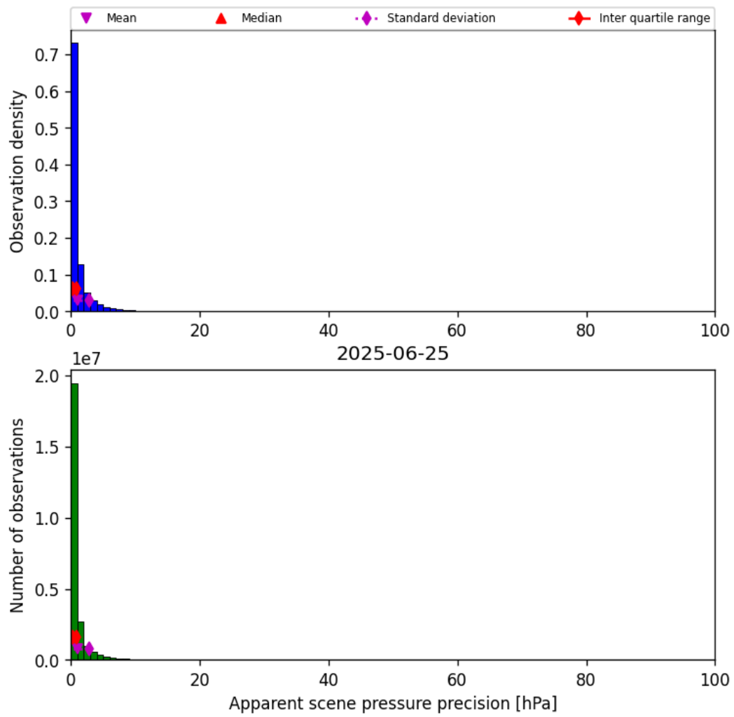
Figure 37: Histogram of “Apparent scene pressure precision” for 2025-06-24 to 2025-06-26
