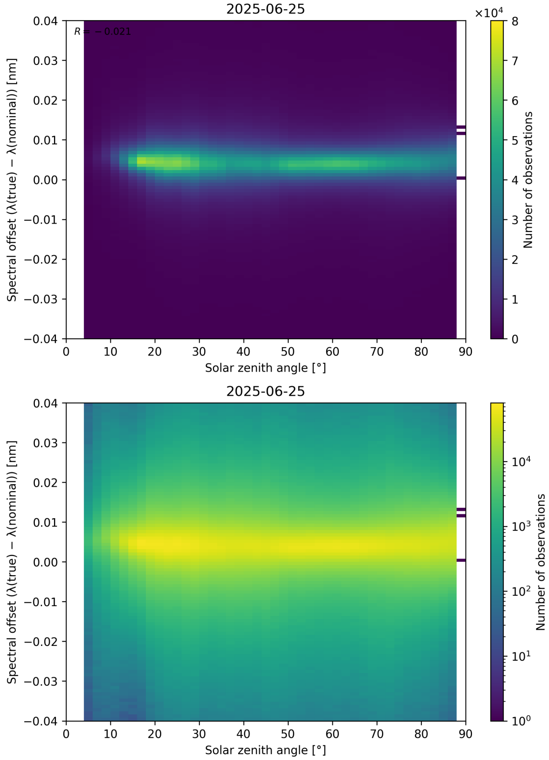
Figure 117: Scatter density plot of “Solar zenith angle” against “Spectral offset ( \lambda_{\text{true}} - \lambda_{\text{nominal}} )” for 2025-06-24 to 2025-06-26.
