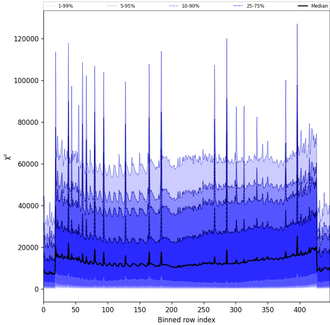
Figure 55: Along track statistics of “ \chi^2 ” for 2025-06-24 to 2025-06-26
