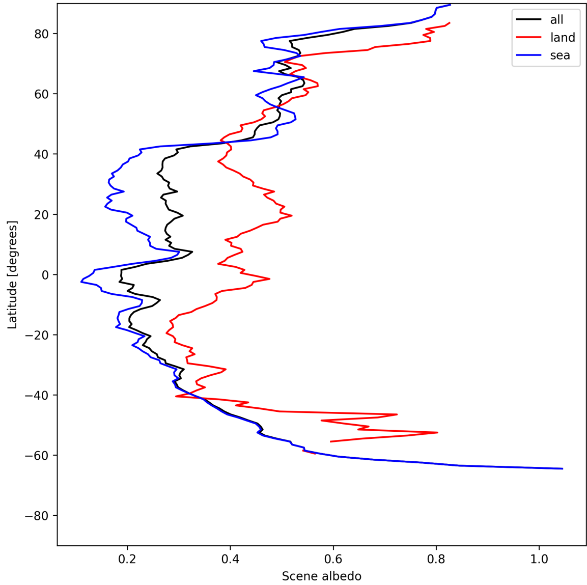
Figure 17: Zonal average of “Scene albedo” for 2025-06-24 to 2025-06-26.
