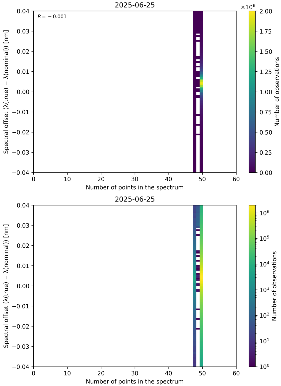
Figure 101: Scatter density plot of “Number of points in the spectrum” against “Spectral offset ( \lambda_{\text{true}} - \lambda_{\text{nominal}} )” for 2025-06-24 to 2025-06-26.
