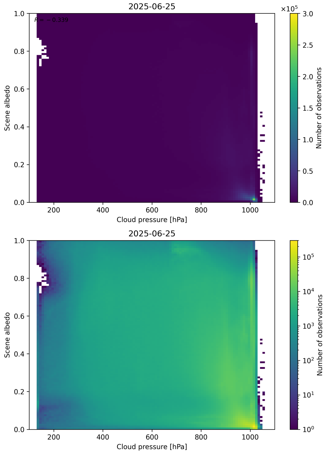
Figure 83: Scatter density plot of “Cloud pressure” against “Scene albedo” for 2025-06-24 to 2025-06-26.
