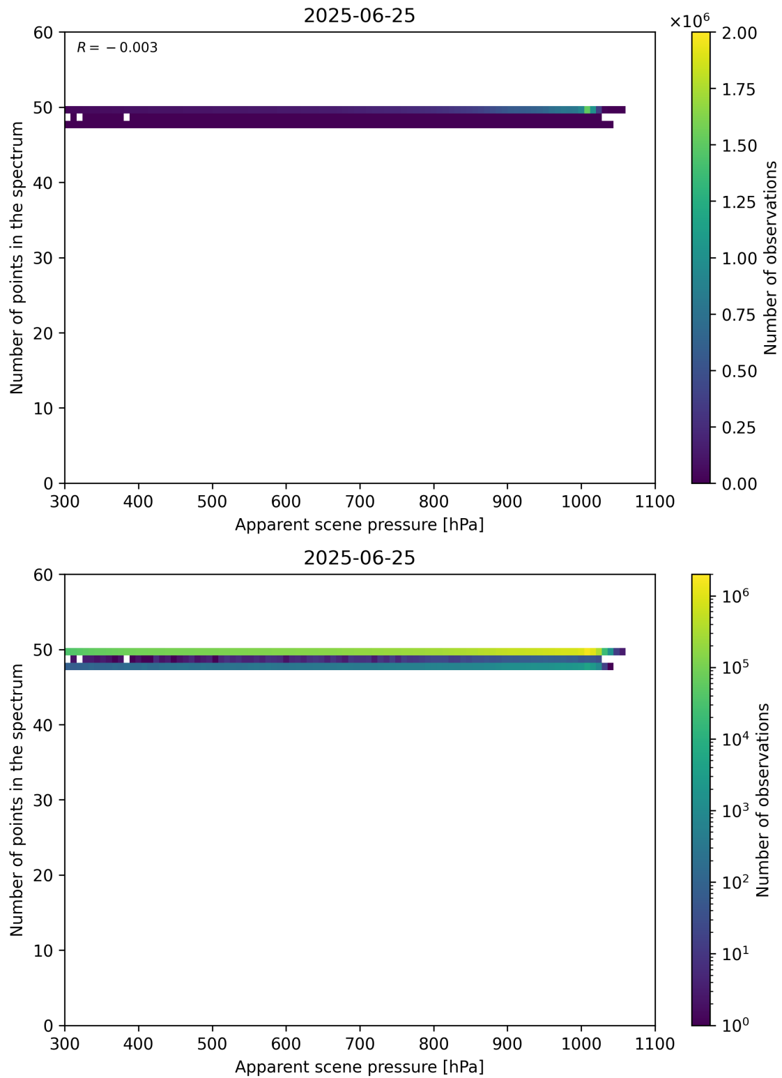
Figure 66: Scatter density plot of “Apparent scene pressure” against “Number of points in the spectrum” for 2025-06-24 to 2025-06-26.
