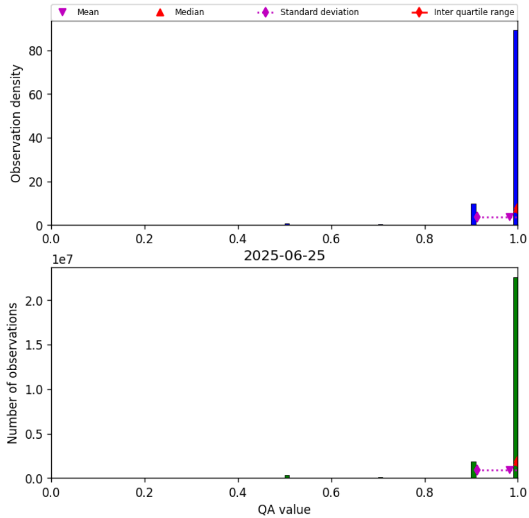
Figure 29: Histogram of “QA value” for 2025-06-24 to 2025-06-26
