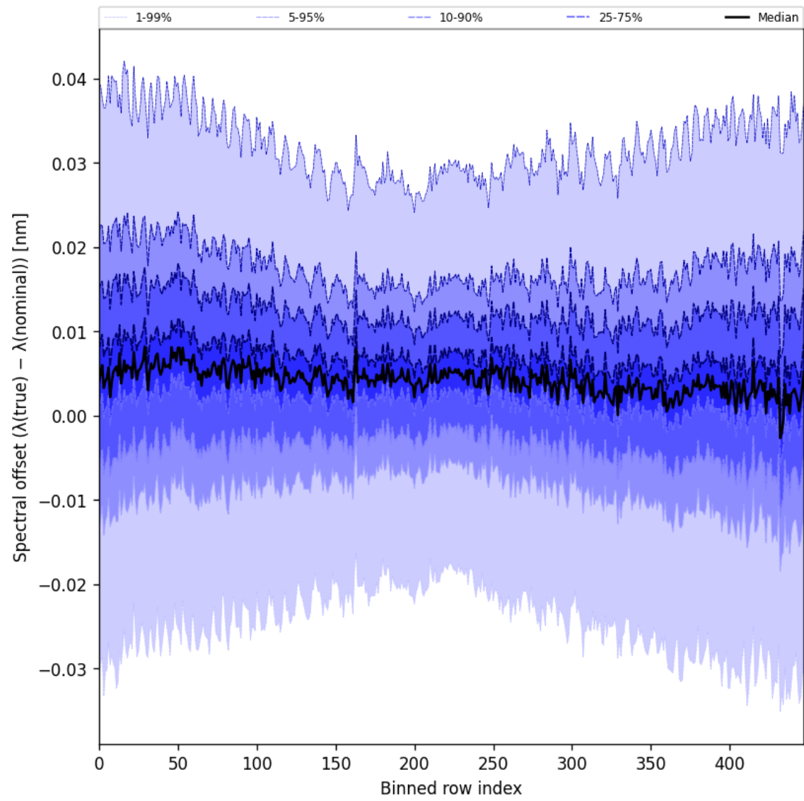
Figure 62: Along track statistics of “Spectral offset ( \lambda_{\text{true}} - \lambda_{\text{nominal}} )” for 2025-06-24 to 2025-06-26
