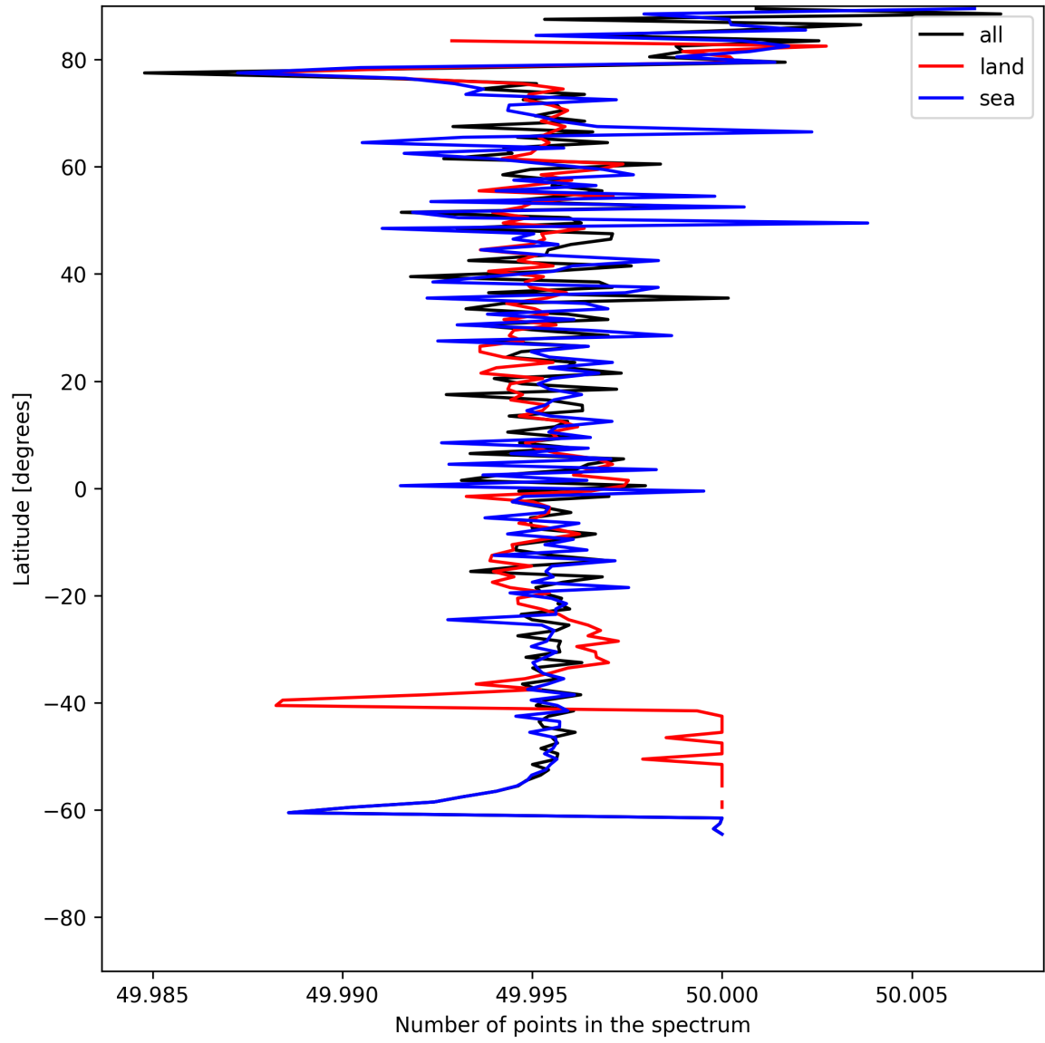
Figure 27: Zonal average of “Number of points in the spectrum” for 2025-06-24 to 2025-06-26.
