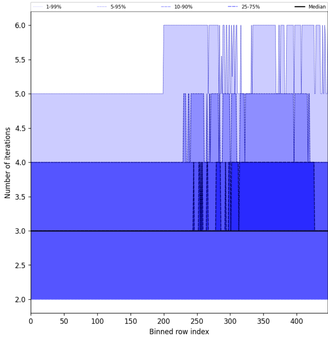
Figure 56: Along track statistics of "Number of iterations" for 2025-06-24 to 2025-06-26
