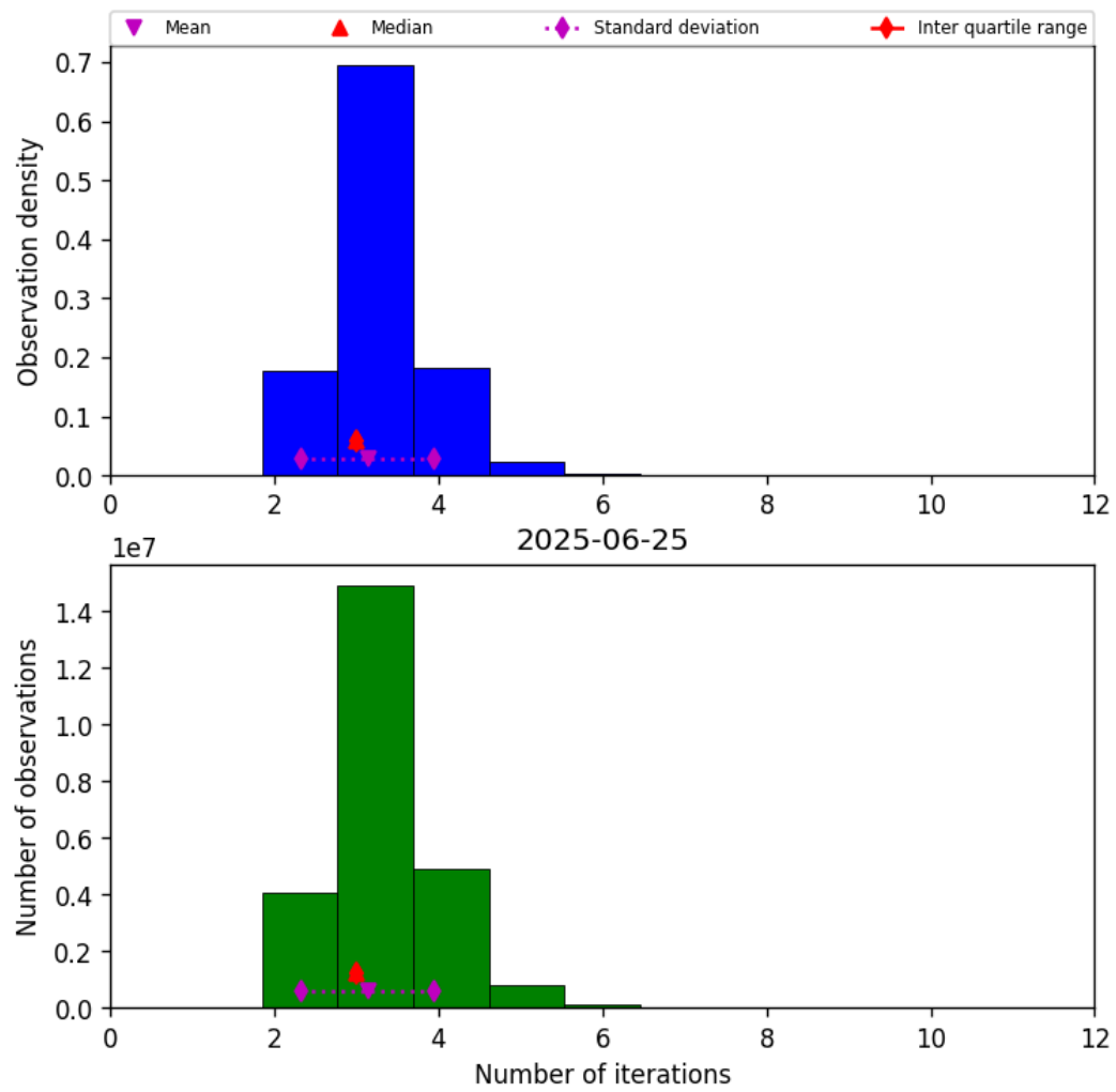
Figure 39: Histogram of “Number of iterations” for 2025-06-24 to 2025-06-26
