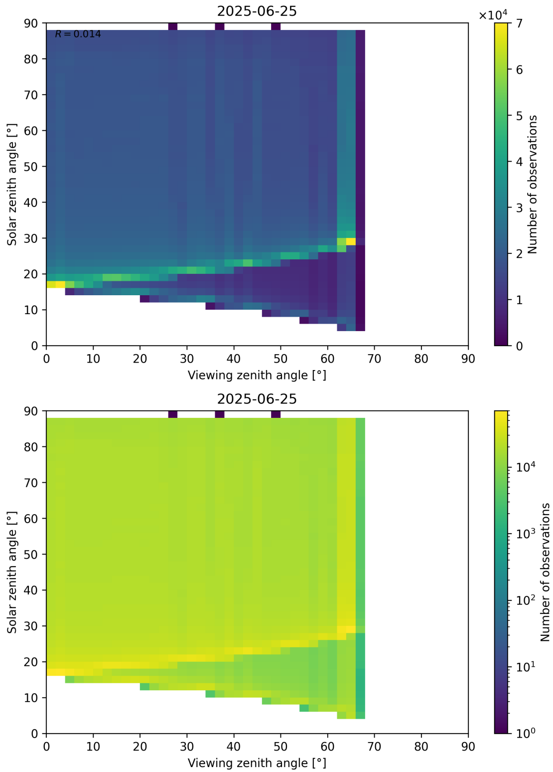
Figure 127: Scatter density plot of “Viewing zenith angle” against “Solar zenith angle” for 2025-06-24 to 2025-06-26.
