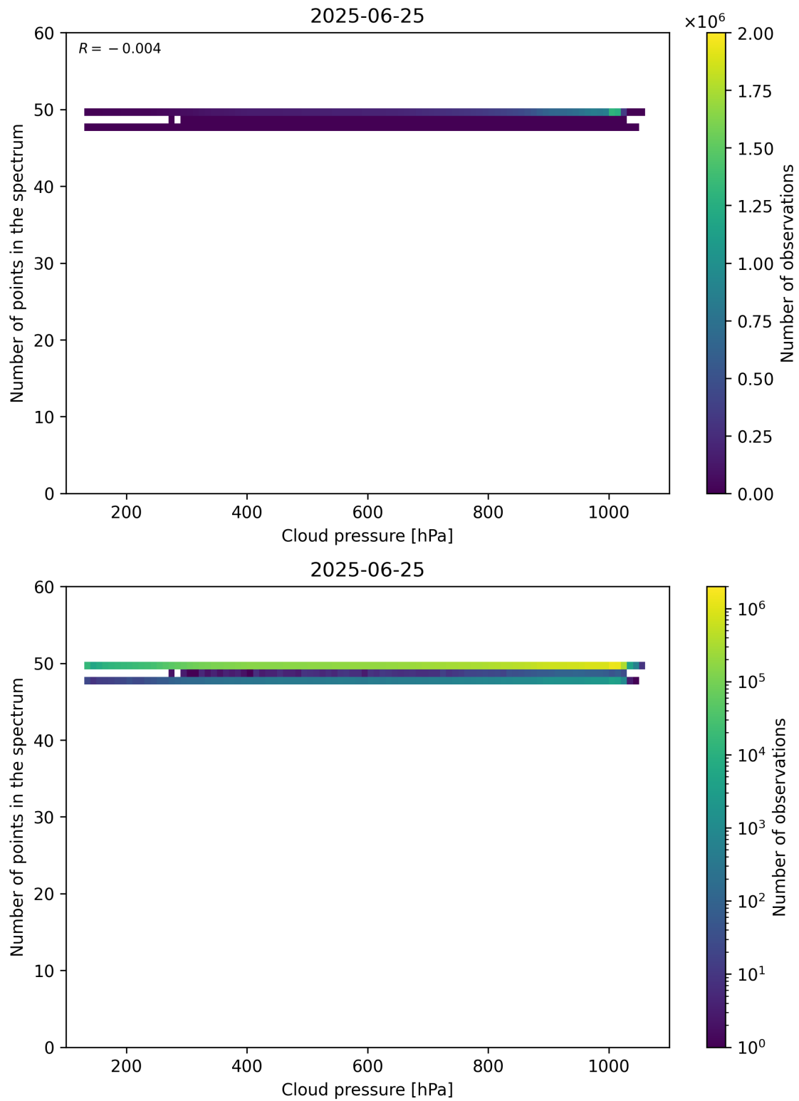
Figure 82: Scatter density plot of “Cloud pressure” against “Number of points in the spectrum” for 2025-06-24 to 2025-06-26.
