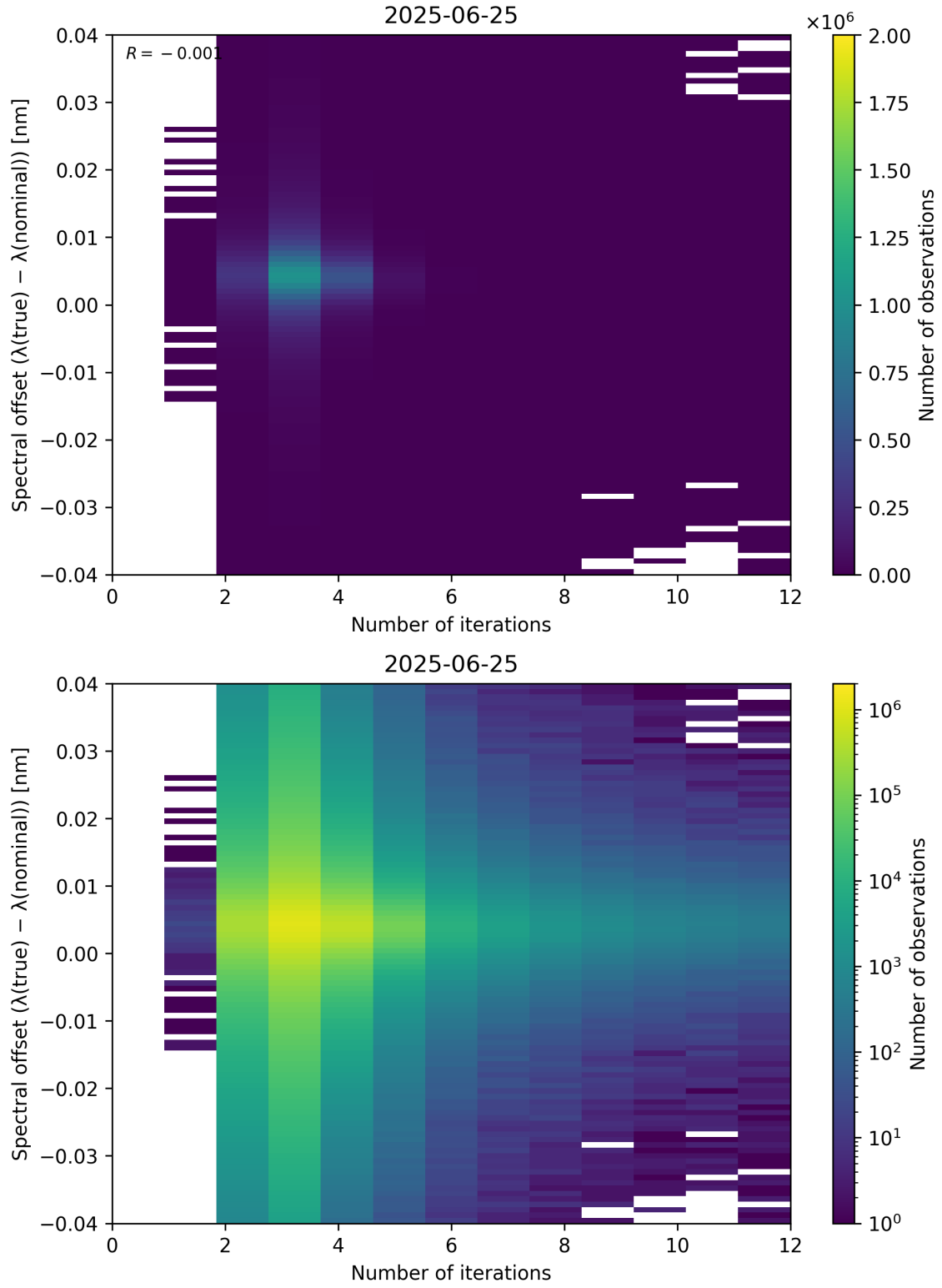
Figure 100: Scatter density plot of “Number of iterations” against “Spectral offset ( \lambda_{\text{true}} - \lambda_{\text{nominal}} )” for 2025-06-24 to 2025-06-26.
