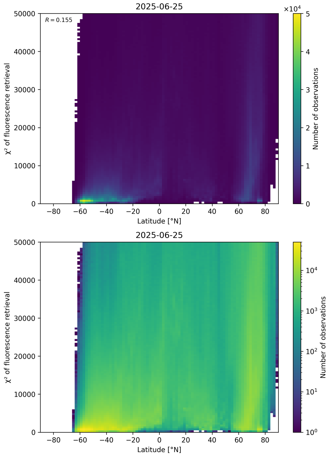
Figure 89: Scatter density plot of “Latitude” against “ \chi^2 of fluorescence retrieval” for 2025-06-24 to 2025-06-26.
