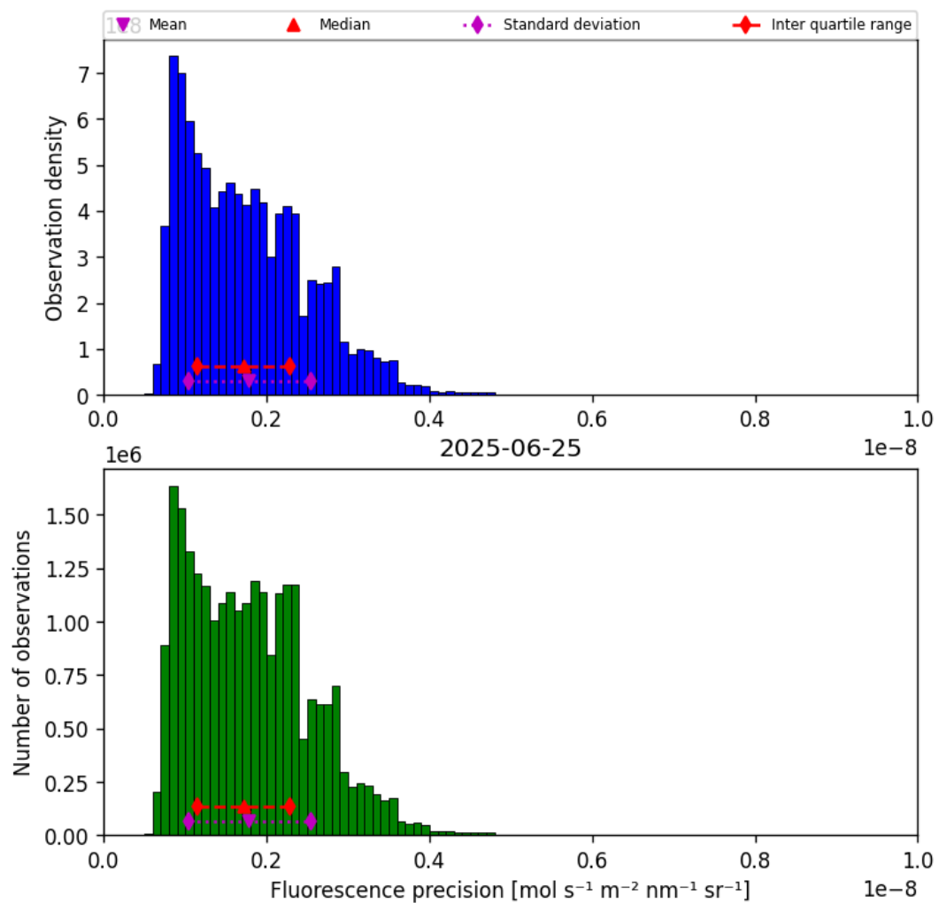
Figure 41: Histogram of “Fluorescence precision” for 2025-06-24 to 2025-06-26
