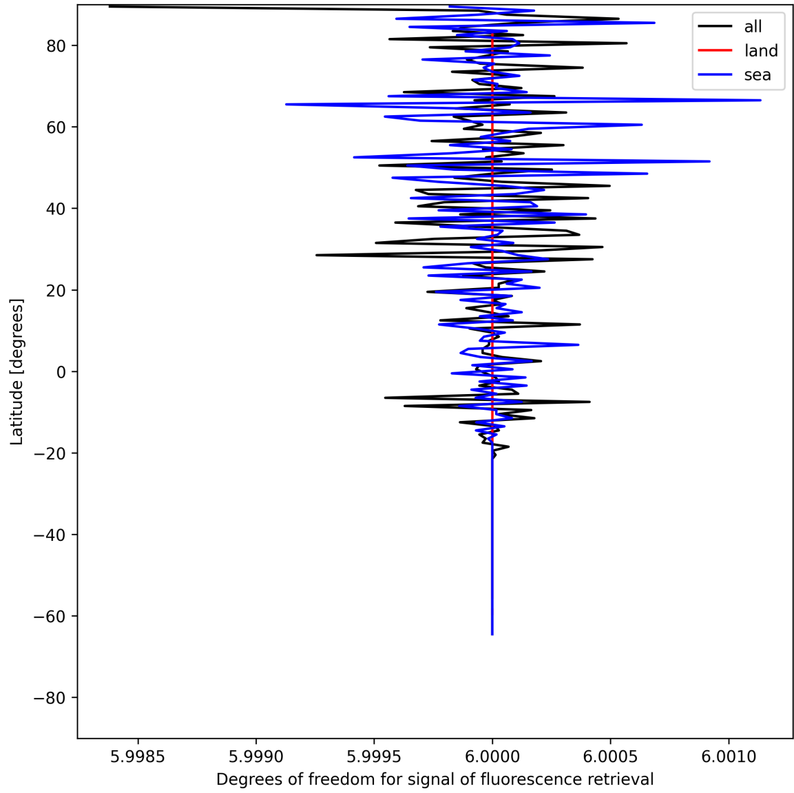
Figure 26: Zonal average of “Degrees of freedom for signal of fluorescence retrieval” for 2025-06-24 to 2025-06-26.
