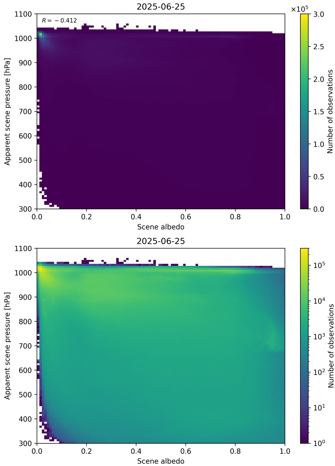
Figure 102: Scatter density plot of “Scene albedo” against “Apparent scene pressure” for 2025-06-24 to 2025-06-26.
