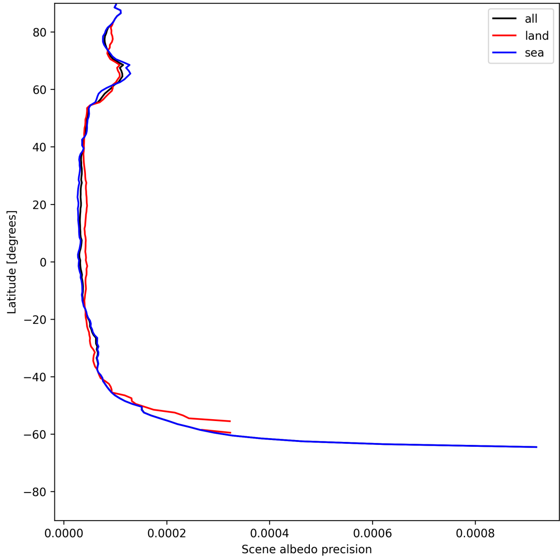
Figure 18: Zonal average of “Scene albedo precision” for 2025-06-24 to 2025-06-26.
