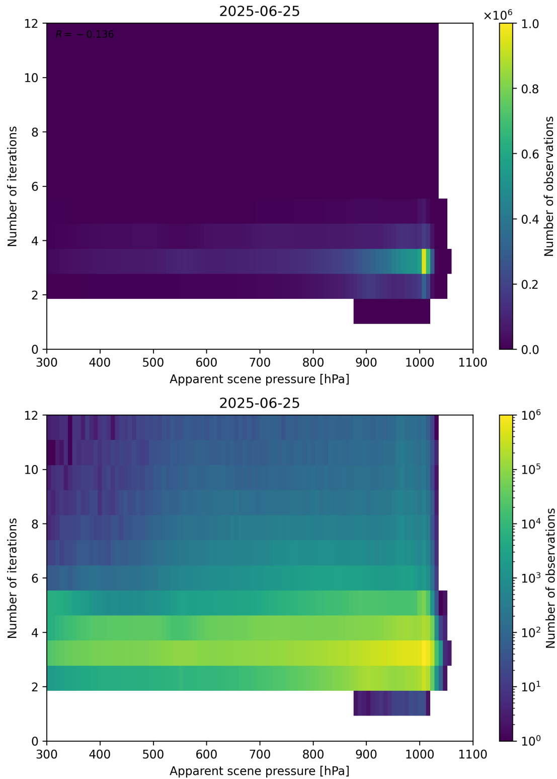
Figure 65: Scatter density plot of “Apparent scene pressure” against “Number of iterations” for 2025-06-24 to 2025-06-26.
