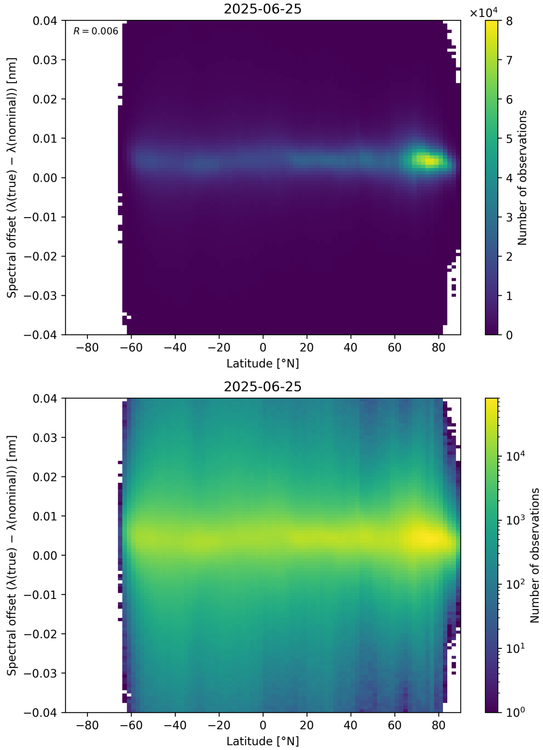
Figure 96: Scatter density plot of “Latitude” against “Spectral offset ( \lambda_{\text{true}} - \lambda_{\text{nominal}} )” for 2025-06-24 to 2025-06-26.
