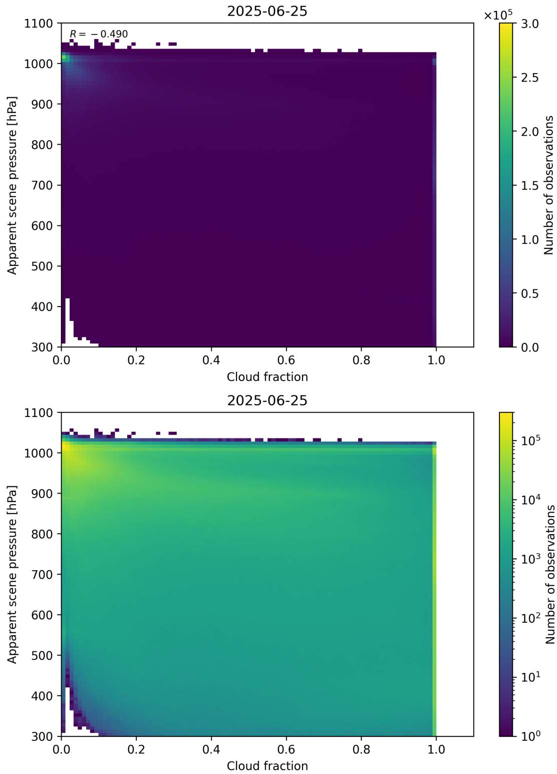
Figure 70: Scatter density plot of “Cloud fraction” against “Apparent scene pressure” for 2025-06-24 to 2025-06-26.
