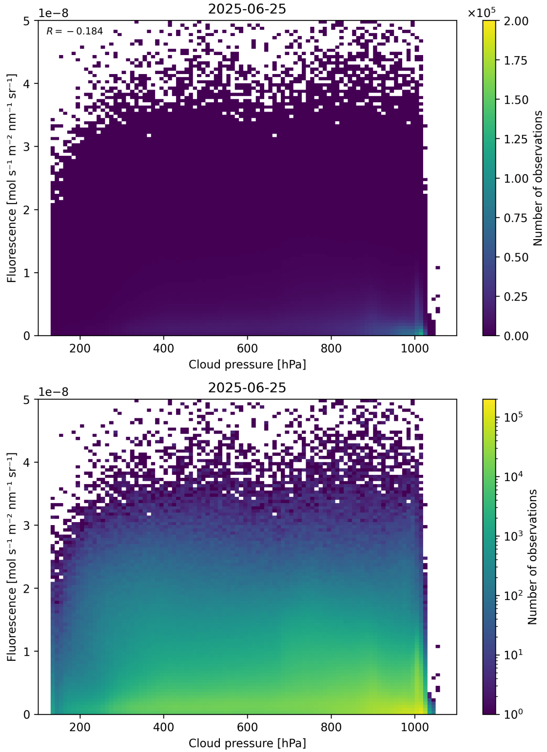
Figure 80: Scatter density plot of “Cloud pressure” against “Fluorescence” for 2025-06-24 to 2025-06-26.
