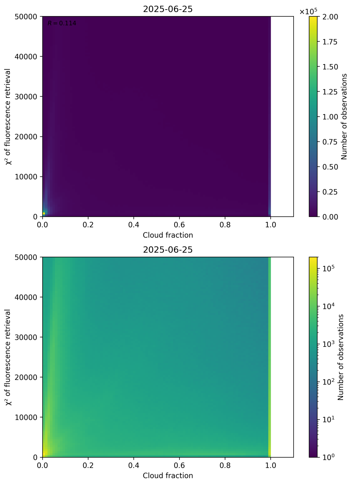
Figure 71: Scatter density plot of “Cloud fraction” against “ \chi^2 of fluorescence retrieval” for 2025-06-24 to 2025-06-26.
