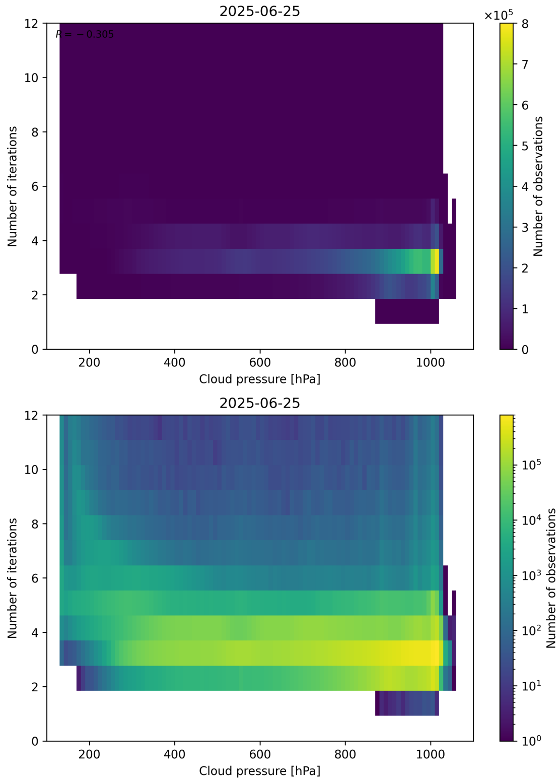
Figure 81: Scatter density plot of “Cloud pressure” against “Number of iterations” for 2025-06-24 to 2025-06-26.
