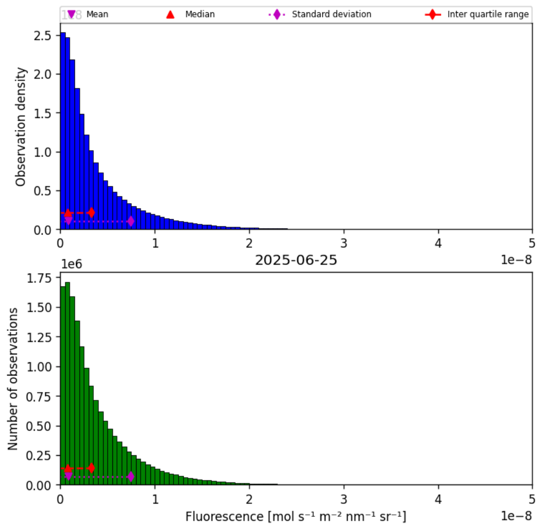
Figure 40: Histogram of “Fluorescence” for 2025-06-24 to 2025-06-26
