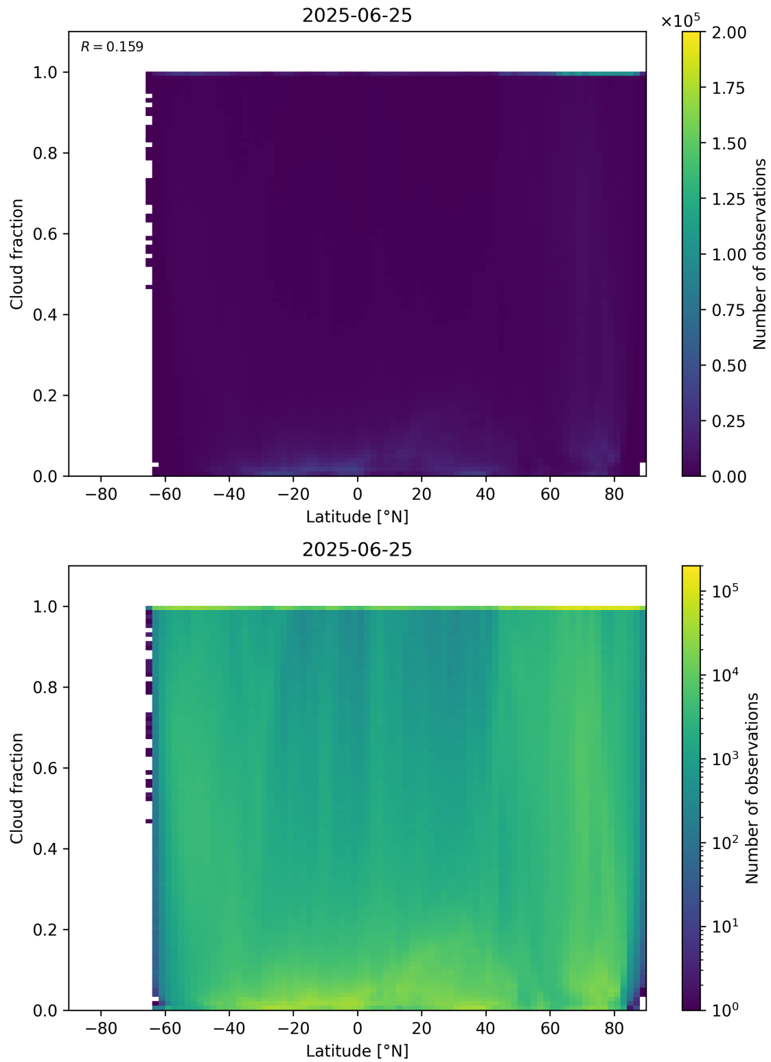
Figure 90: Scatter density plot of “Latitude” against “Cloud fraction” for 2025-06-24 to 2025-06-26.
