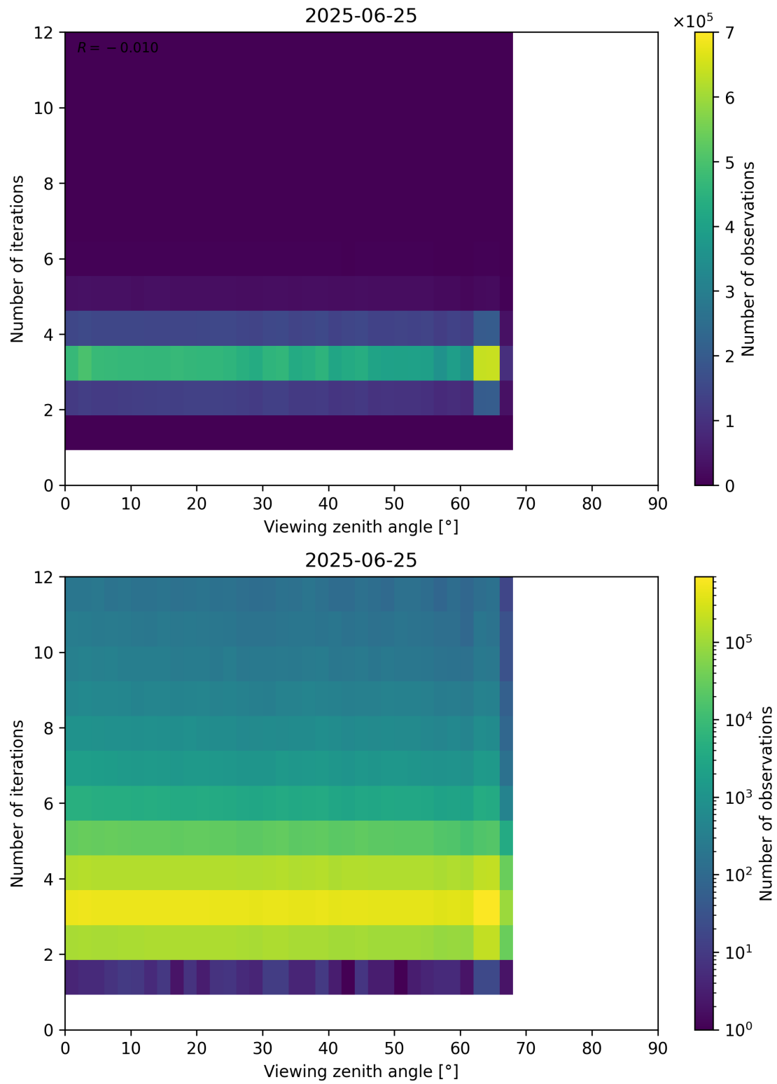
Figure 124: Scatter density plot of “Viewing zenith angle” against “Number of iterations” for 2025-06-24 to 2025-06-26.
