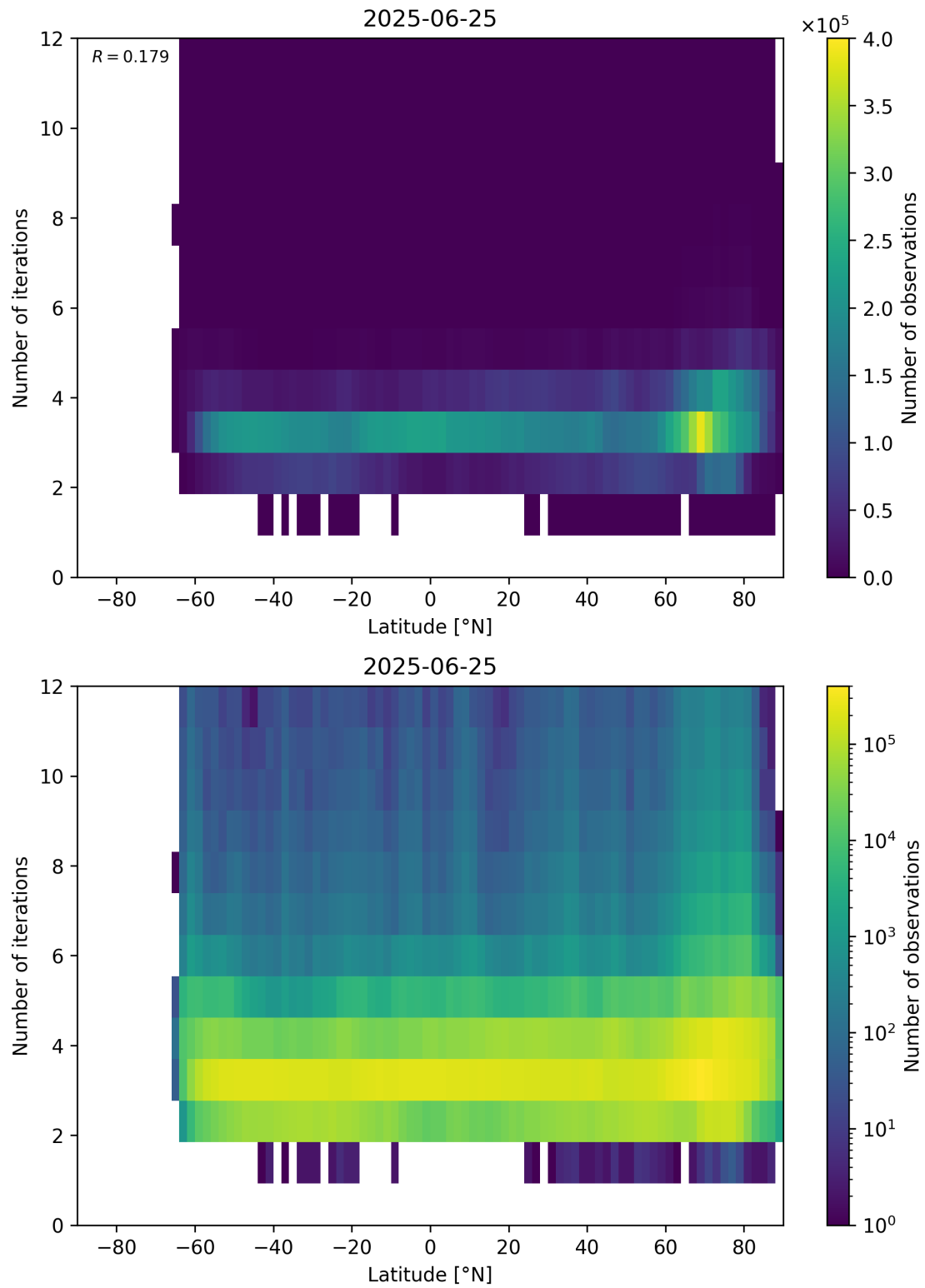
Figure 93: Scatter density plot of “Latitude” against “Number of iterations” for 2025-06-24 to 2025-06-26.
