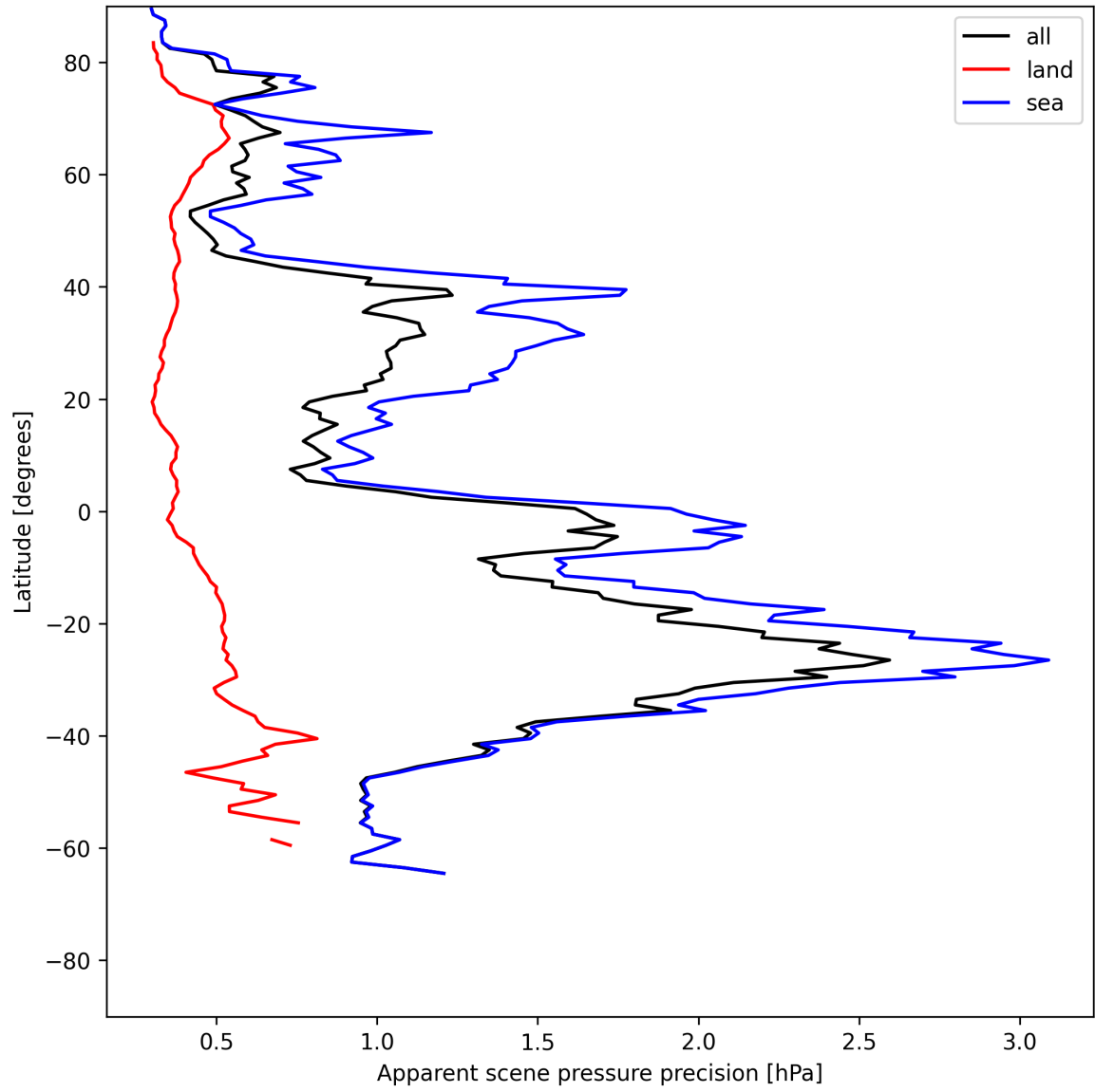
Figure 20: Zonal average of “Apparent scene pressure precision” for 2025-06-24 to 2025-06-26.
