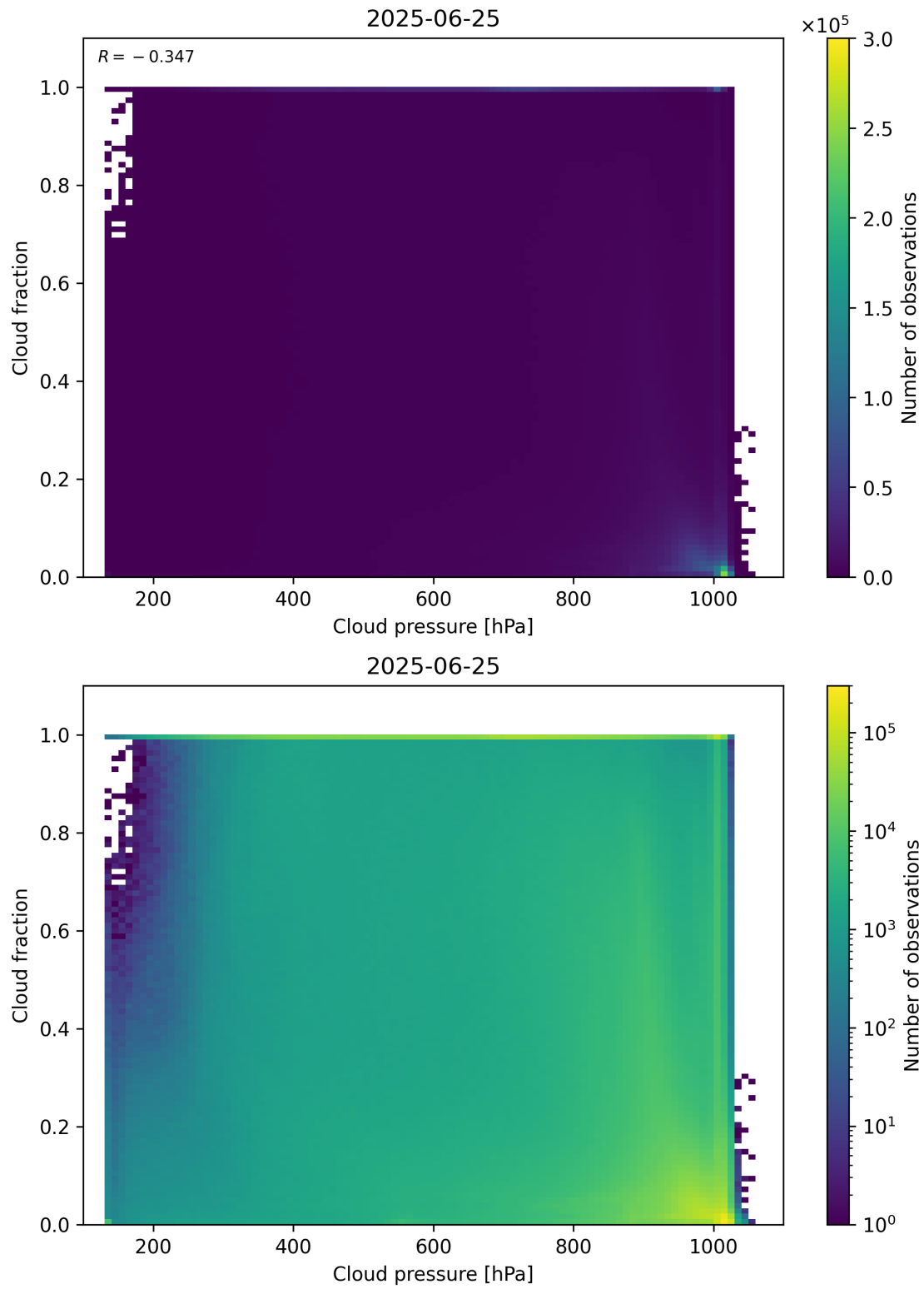
Figure 79: Scatter density plot of “Cloud pressure” against “Cloud fraction” for 2025-06-24 to 2025-06-26.
