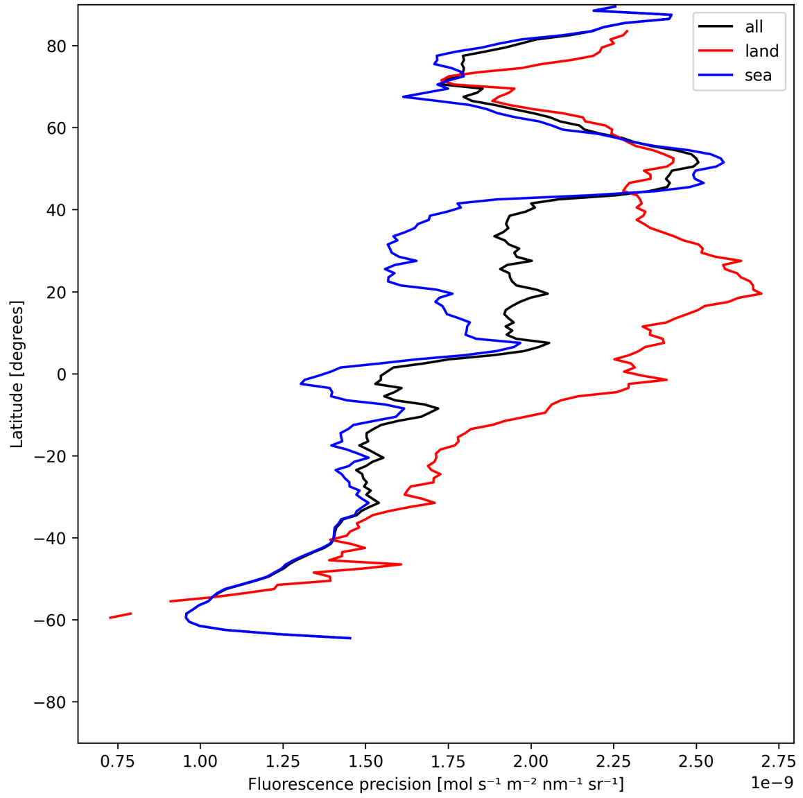
Figure 24: Zonal average of “Fluorescence precision” for 2025-06-24 to 2025-06-26.
