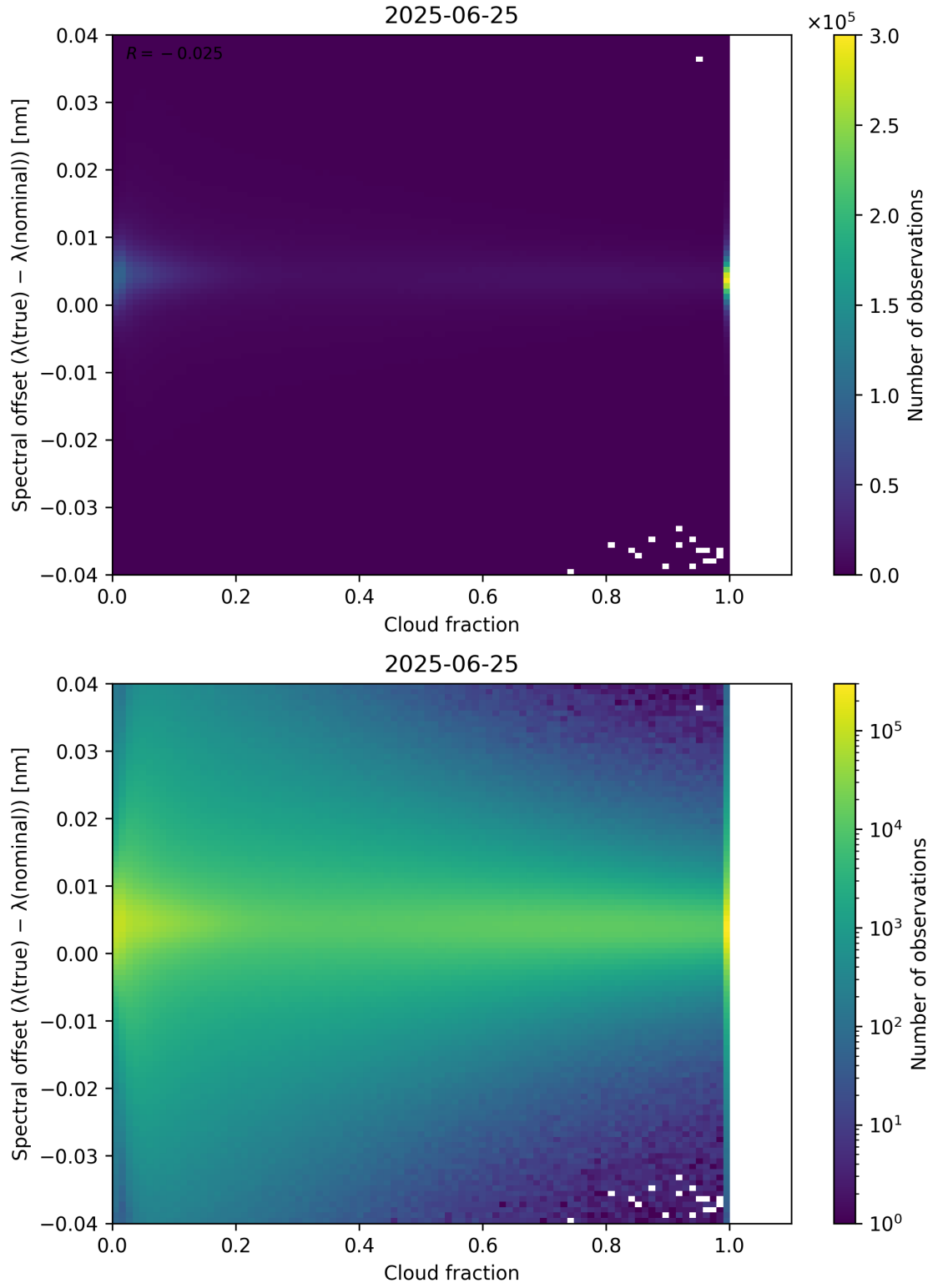
Figure 76: Scatter density plot of “Cloud fraction” against “Spectral offset ( \lambda_{\text{true}} - \lambda_{\text{nominal}} )” for 2025-06-24 to 2025-06-26.
