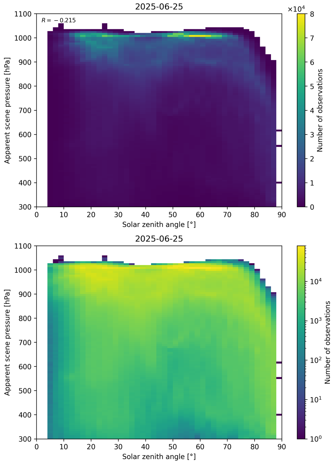
Figure 108: Scatter density plot of “Solar zenith angle” against “Apparent scene pressure” for 2025-06-24 to 2025-06-26.
