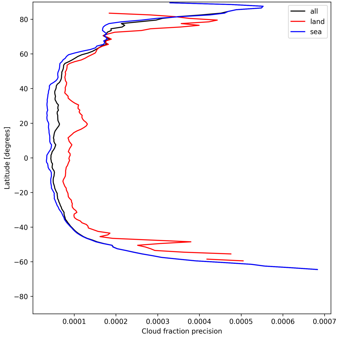
Figure 16: Zonal average of “Cloud fraction precision” for 2025-06-24 to 2025-06-26.
