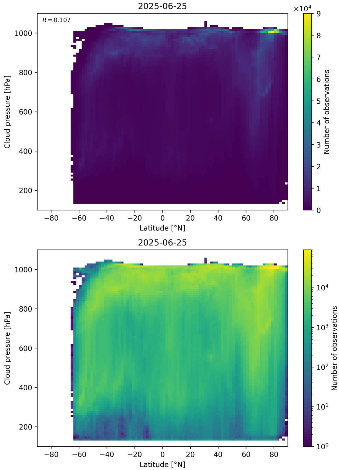
Figure 91: Scatter density plot of “Latitude” against “Cloud pressure” for 2025-06-24 to 2025-06-26.
