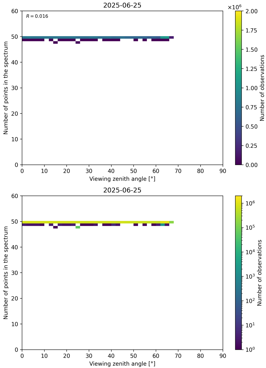
Figure 125: Scatter density plot of “Viewing zenith angle” against “Number of points in the spectrum” for 2025-06-24 to 2025-06-26.
