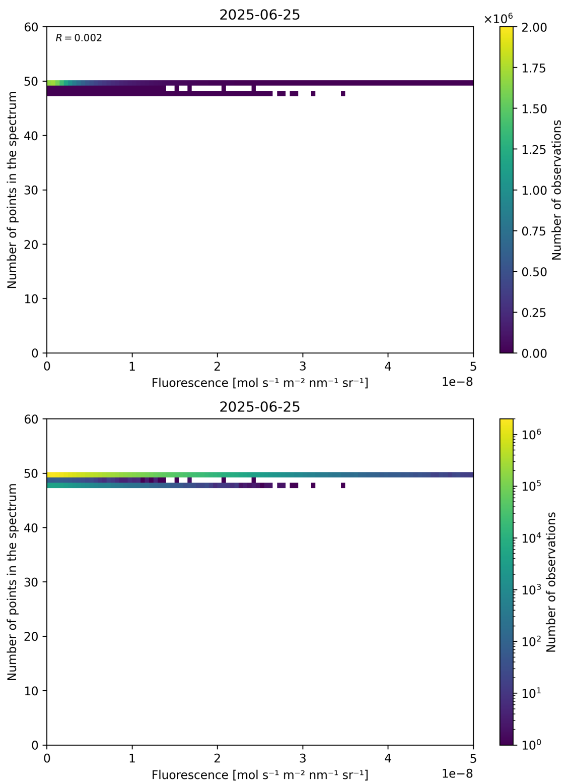
Figure 86: Scatter density plot of “Fluorescence” against “Number of points in the spectrum” for 2025-06-24 to 2025-06-26.
