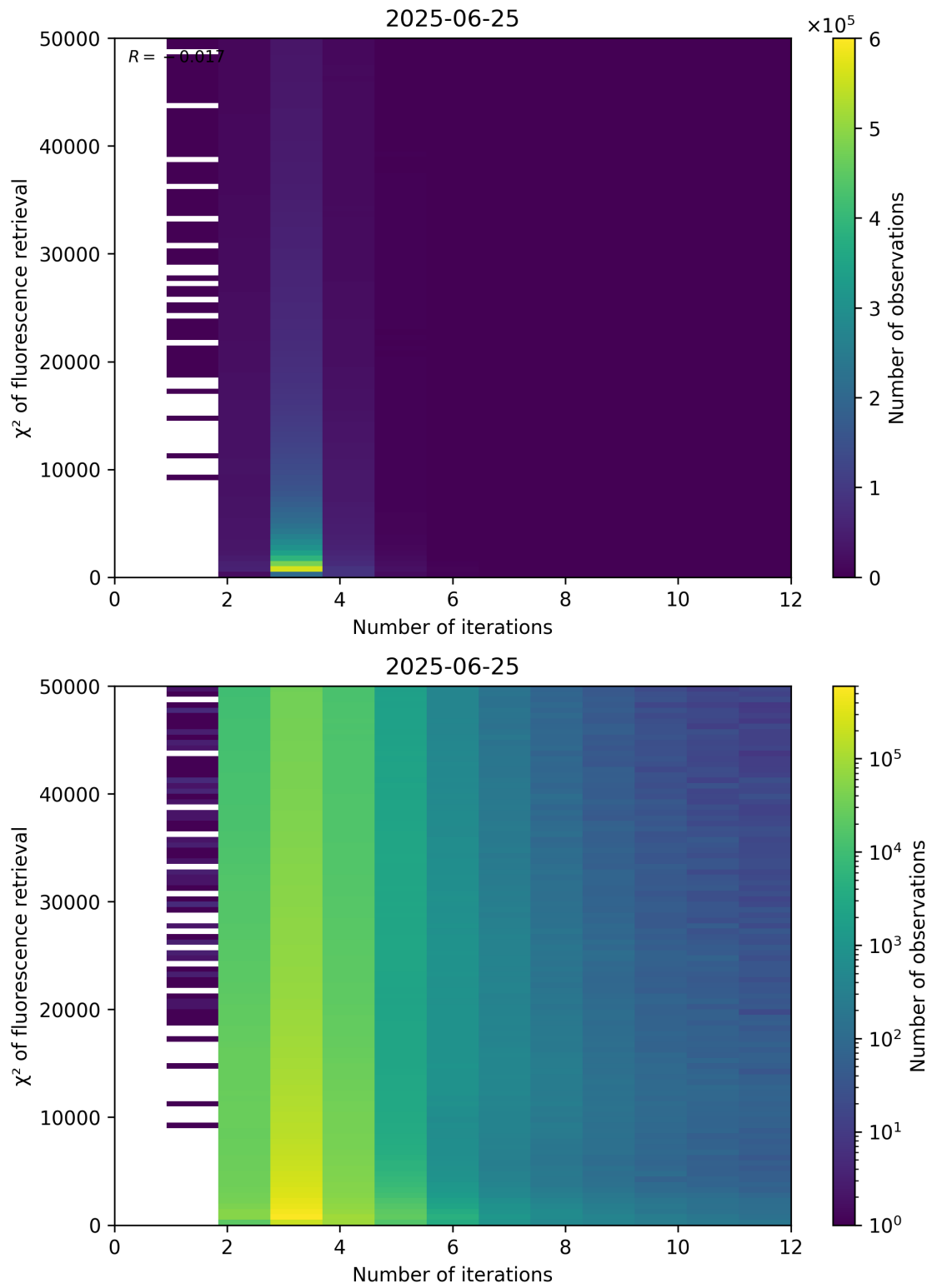
Figure 97: Scatter density plot of “Number of iterations” against “ \chi^2 of fluorescence retrieval” for 2025-06-24 to 2025-06-26.
