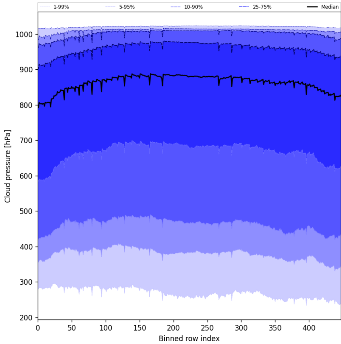
Figure 47: Along track statistics of “Cloud pressure” for 2025-06-24 to 2025-06-26
