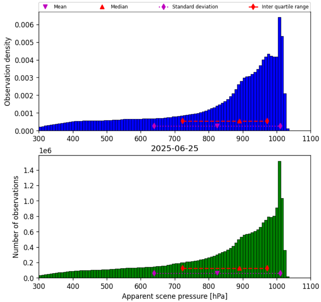
Figure 36: Histogram of “Apparent scene pressure” for 2025-06-24 to 2025-06-26
