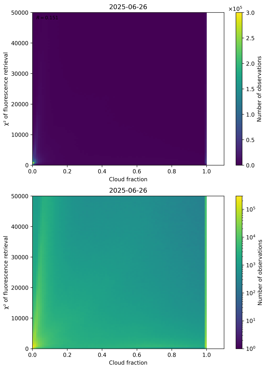
Figure 71: Scatter density plot of “Cloud fraction” against “ \chi^2 of fluorescence retrieval” for 2025-06-25 to 2025-06-27.
