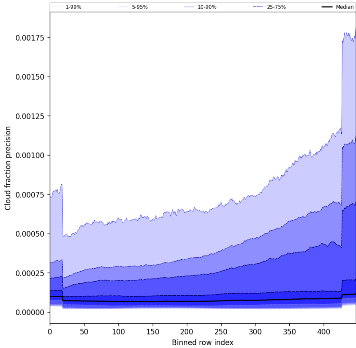
Figure 50: Along track statistics of “Cloud fraction precision” for 2025-06-25 to 2025-06-27
