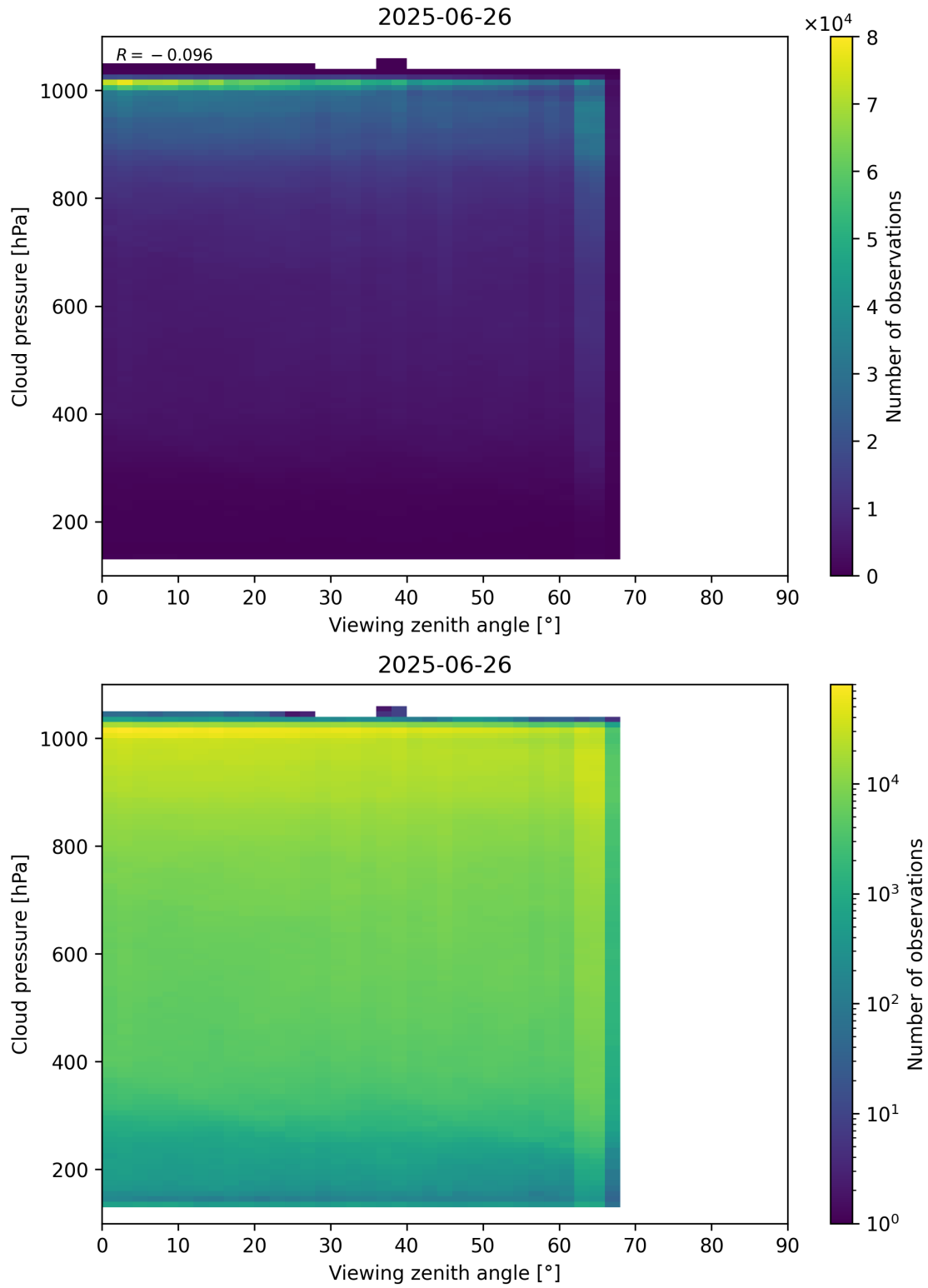
Figure 121: Scatter density plot of “Viewing zenith angle” against “Cloud pressure” for 2025-06-25 to 2025-06-27.
