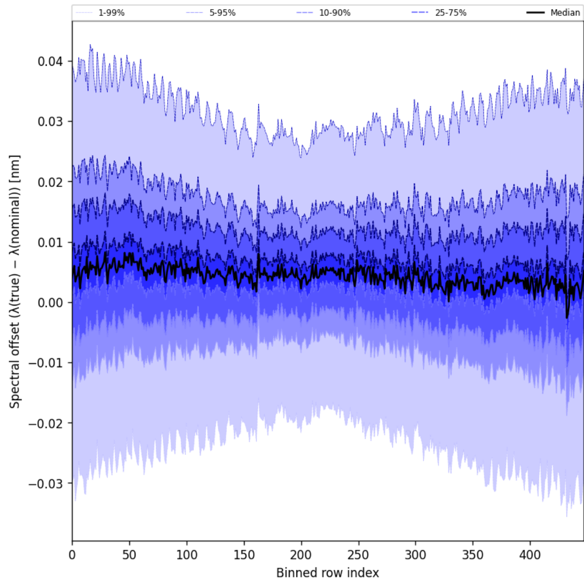
Figure 62: Along track statistics of “Spectral offset ( \lambda_{\text{true}} - \lambda_{\text{nominal}} )” for 2025-06-25 to 2025-06-27
