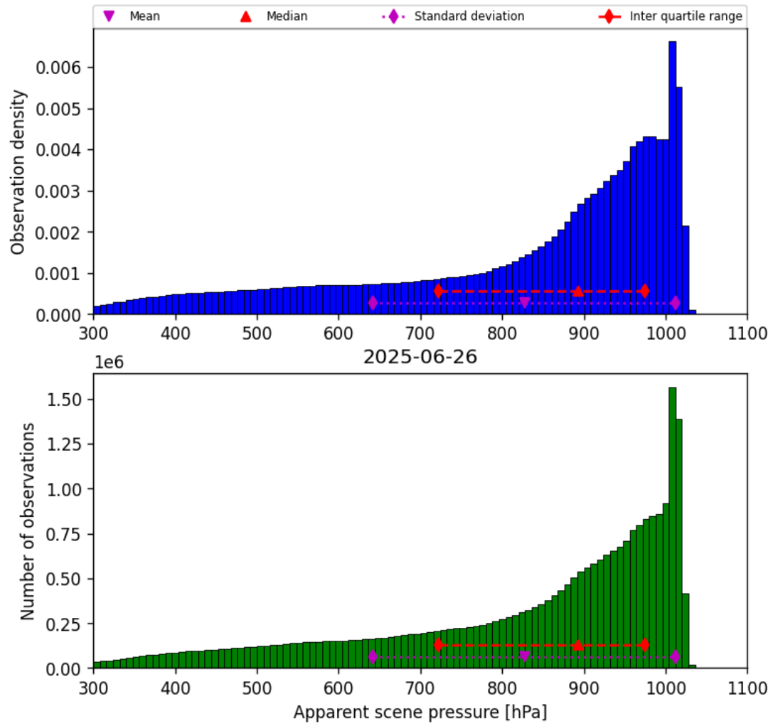
Figure 36: Histogram of “Apparent scene pressure” for 2025-06-25 to 2025-06-27
