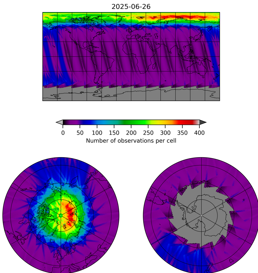
Figure 11: Map of the number of observations for 2025-06-25 to 2025-06-27
