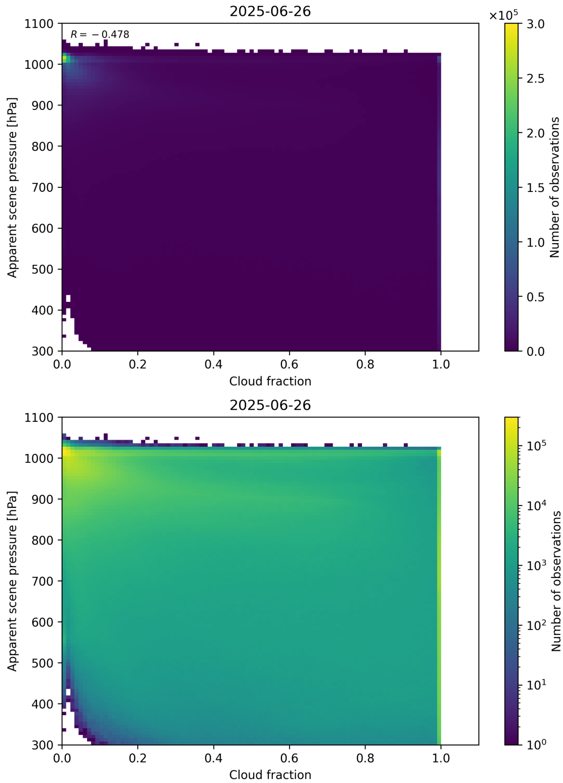
Figure 70: Scatter density plot of “Cloud fraction” against “Apparent scene pressure” for 2025-06-25 to 2025-06-27.
