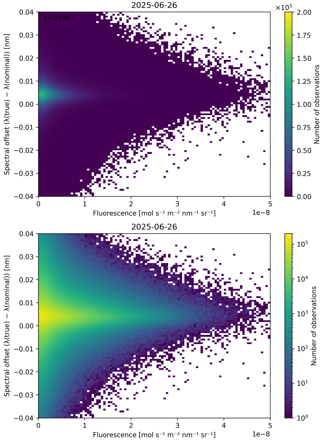
Figure 87: Scatter density plot of “Fluorescence” against “Spectral offset ( \lambda_{\text{true}} - \lambda_{\text{nominal}} )” for 2025-06-25 to 2025-06-27.
