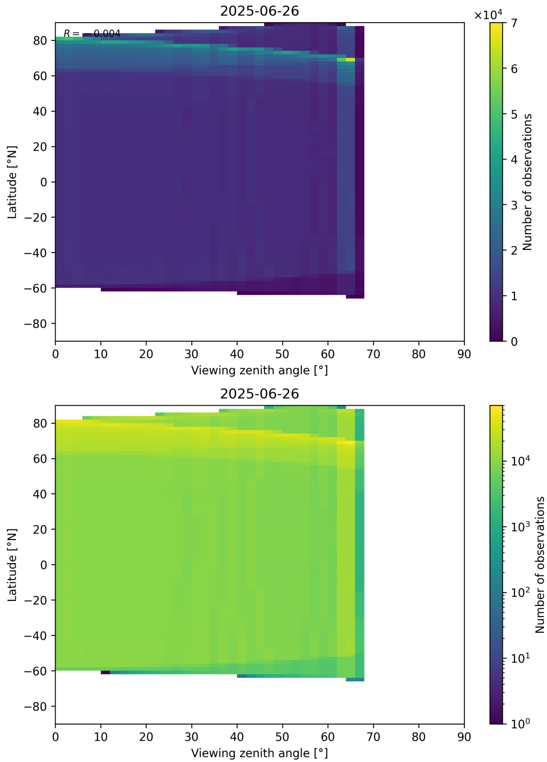
Figure 123: Scatter density plot of “Viewing zenith angle” against “Latitude” for 2025-06-25 to 2025-06-27.
