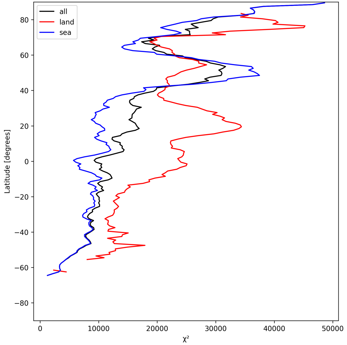
Figure 21: Zonal average of “ \chi^2 ” for 2025-06-25 to 2025-06-27.
