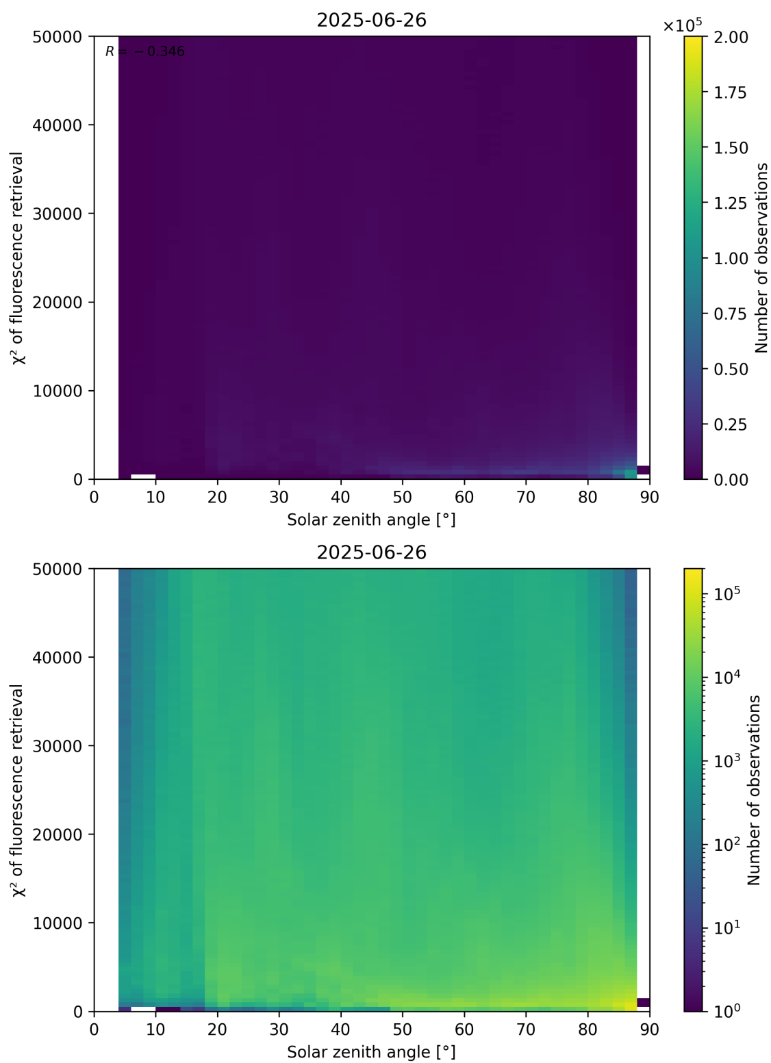
Figure 109: Scatter density plot of “Solar zenith angle” against “ \chi^2 of fluorescence retrieval” for 2025-06-25 to 2025-06-27.
