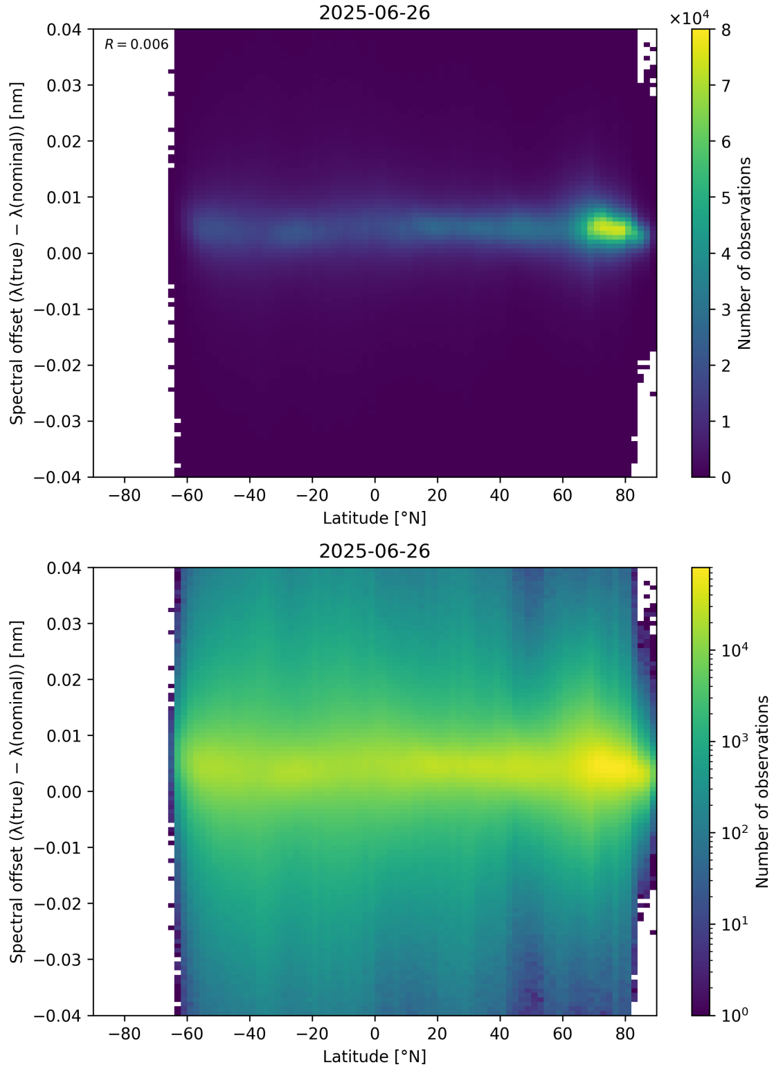
Figure 96: Scatter density plot of “Latitude” against “Spectral offset ( \lambda_{\text{true}} - \lambda_{\text{nominal}} )” for 2025-06-25 to 2025-06-27.
