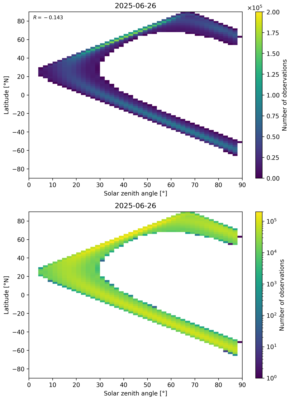
Figure 113: Scatter density plot of “Solar zenith angle” against “Latitude” for 2025-06-25 to 2025-06-27.
