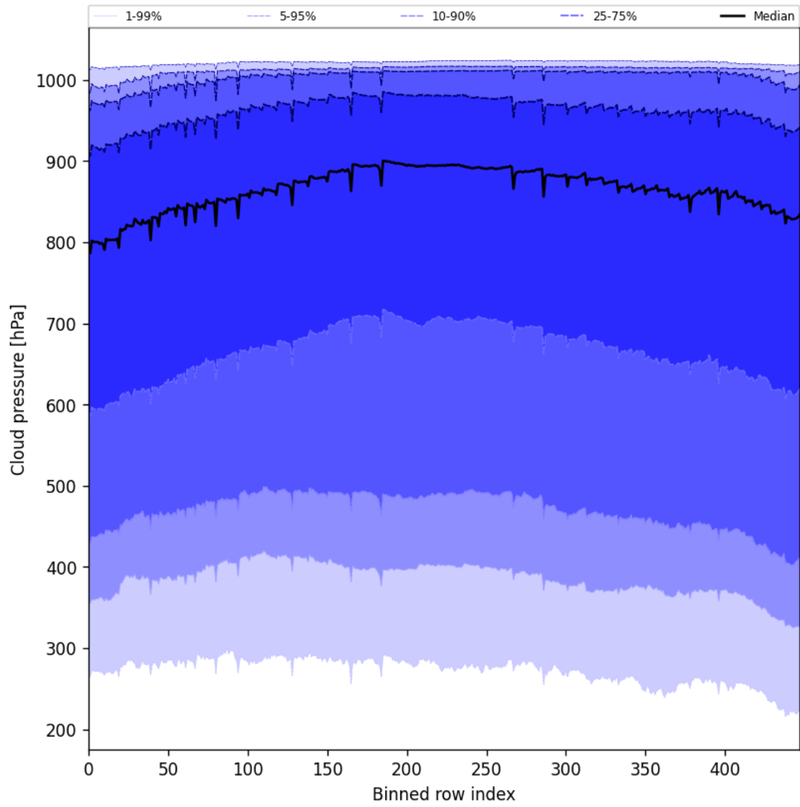
Figure 47: Along track statistics of “Cloud pressure” for 2025-06-25 to 2025-06-27
