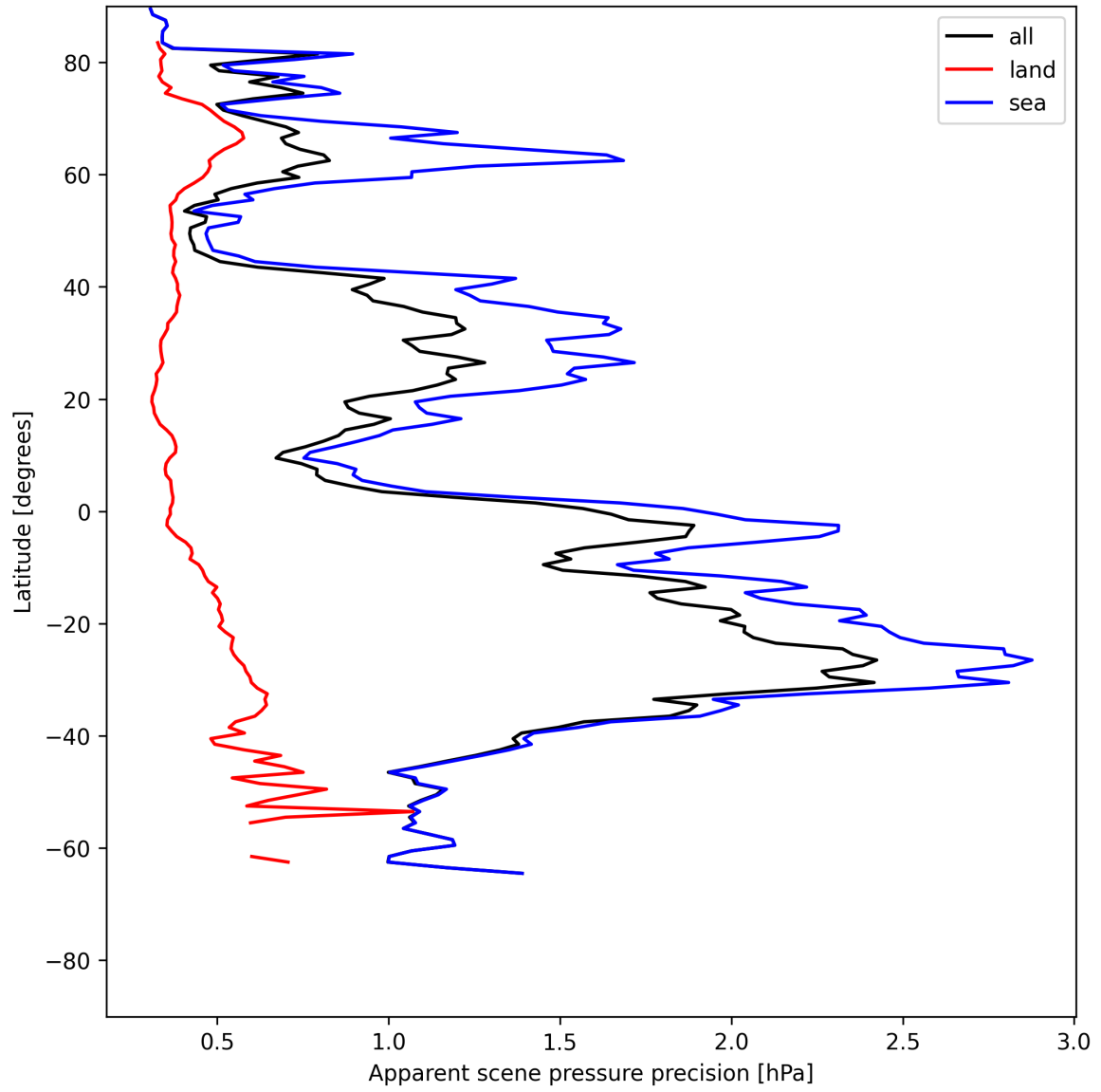
Figure 20: Zonal average of “Apparent scene pressure precision” for 2025-06-25 to 2025-06-27.
