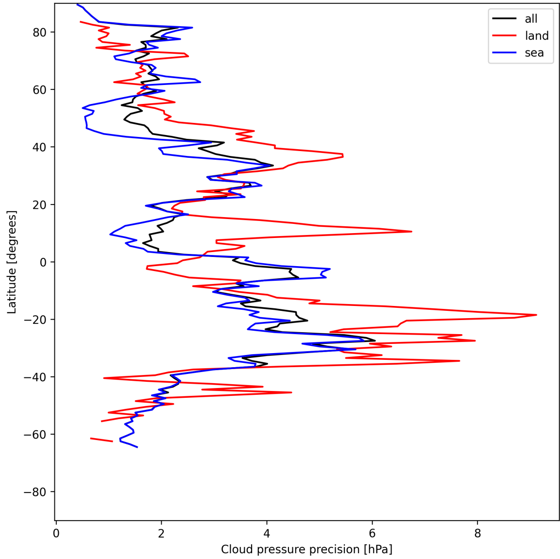
Figure 14: Zonal average of “Cloud pressure precision” for 2025-06-25 to 2025-06-27.
