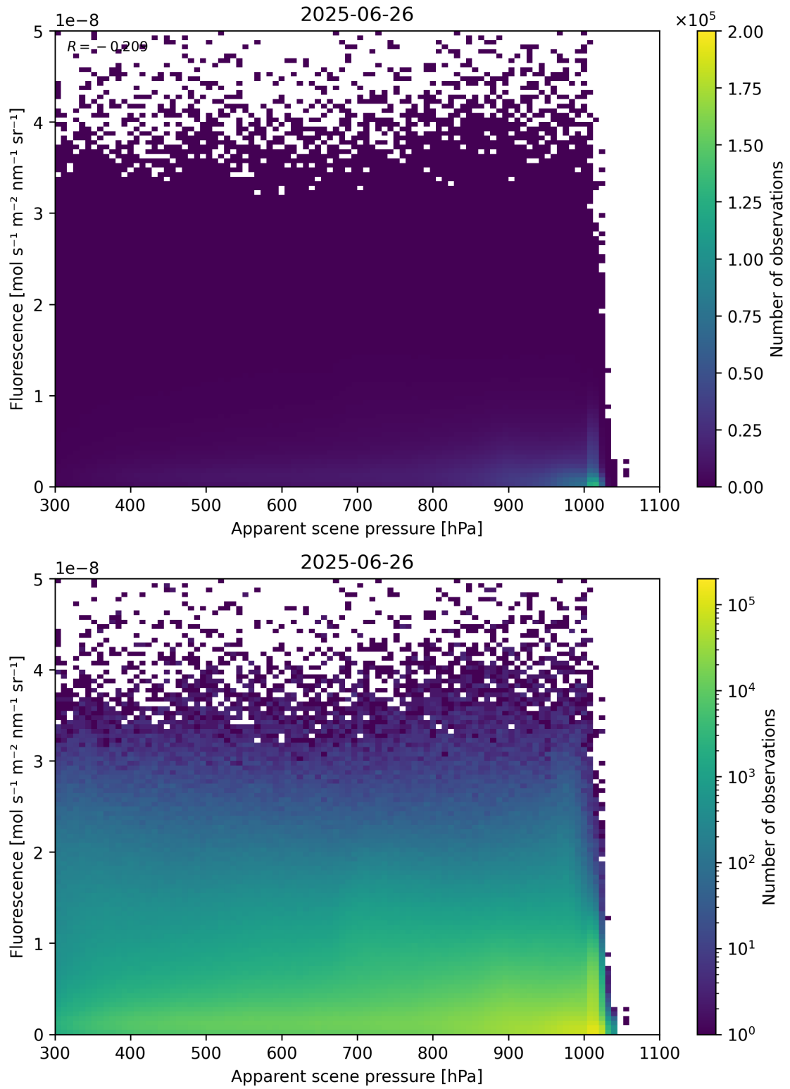
Figure 64: Scatter density plot of “Apparent scene pressure” against “Fluorescence” for 2025-06-25 to 2025-06-27.
