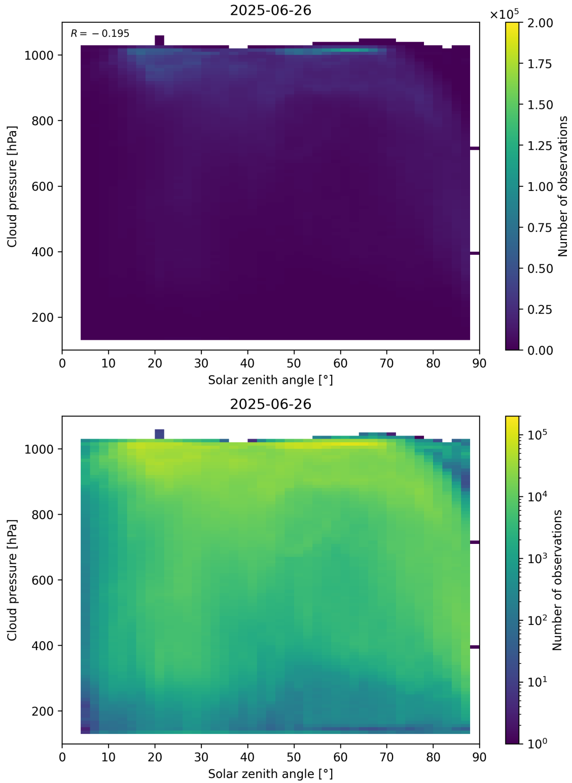
Figure 111: Scatter density plot of “Solar zenith angle” against “Cloud pressure” for 2025-06-25 to 2025-06-27.
