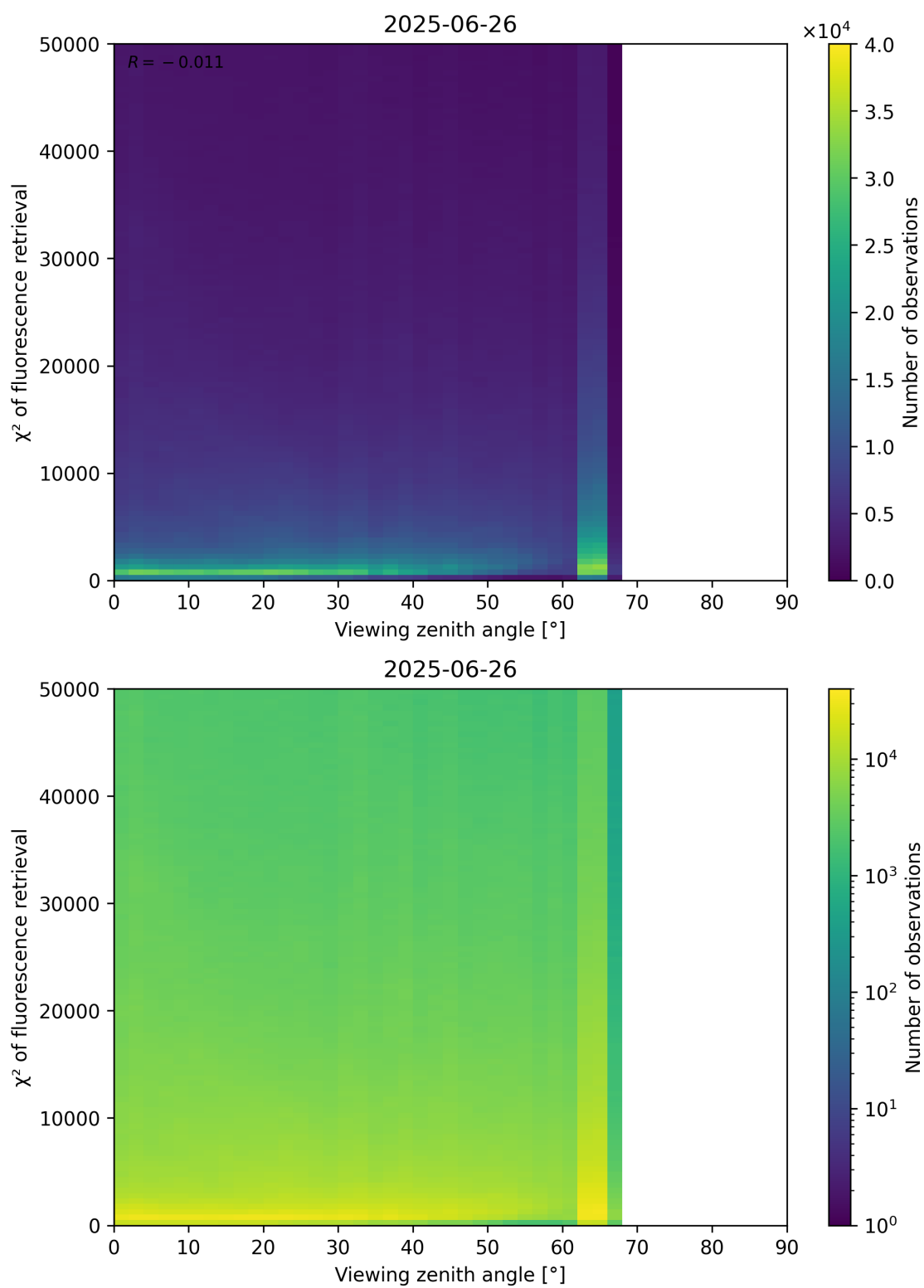
Figure 119: Scatter density plot of “Viewing zenith angle” against “ \chi^2 of fluorescence retrieval” for 2025-06-25 to 2025-06-27.
