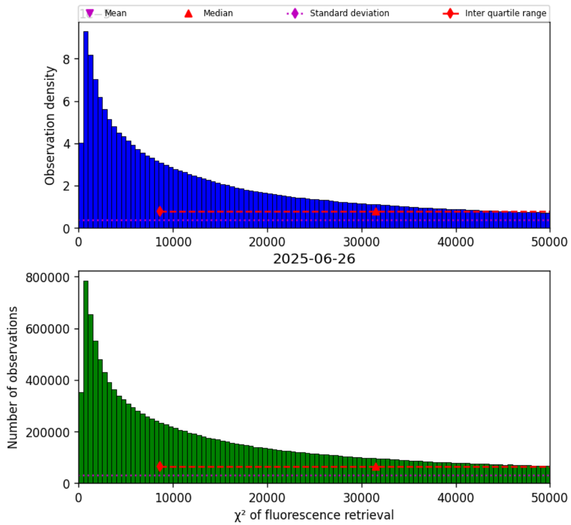
Figure 42: Histogram of “ \chi^2 of fluorescence retrieval” for 2025-06-25 to 2025-06-27
