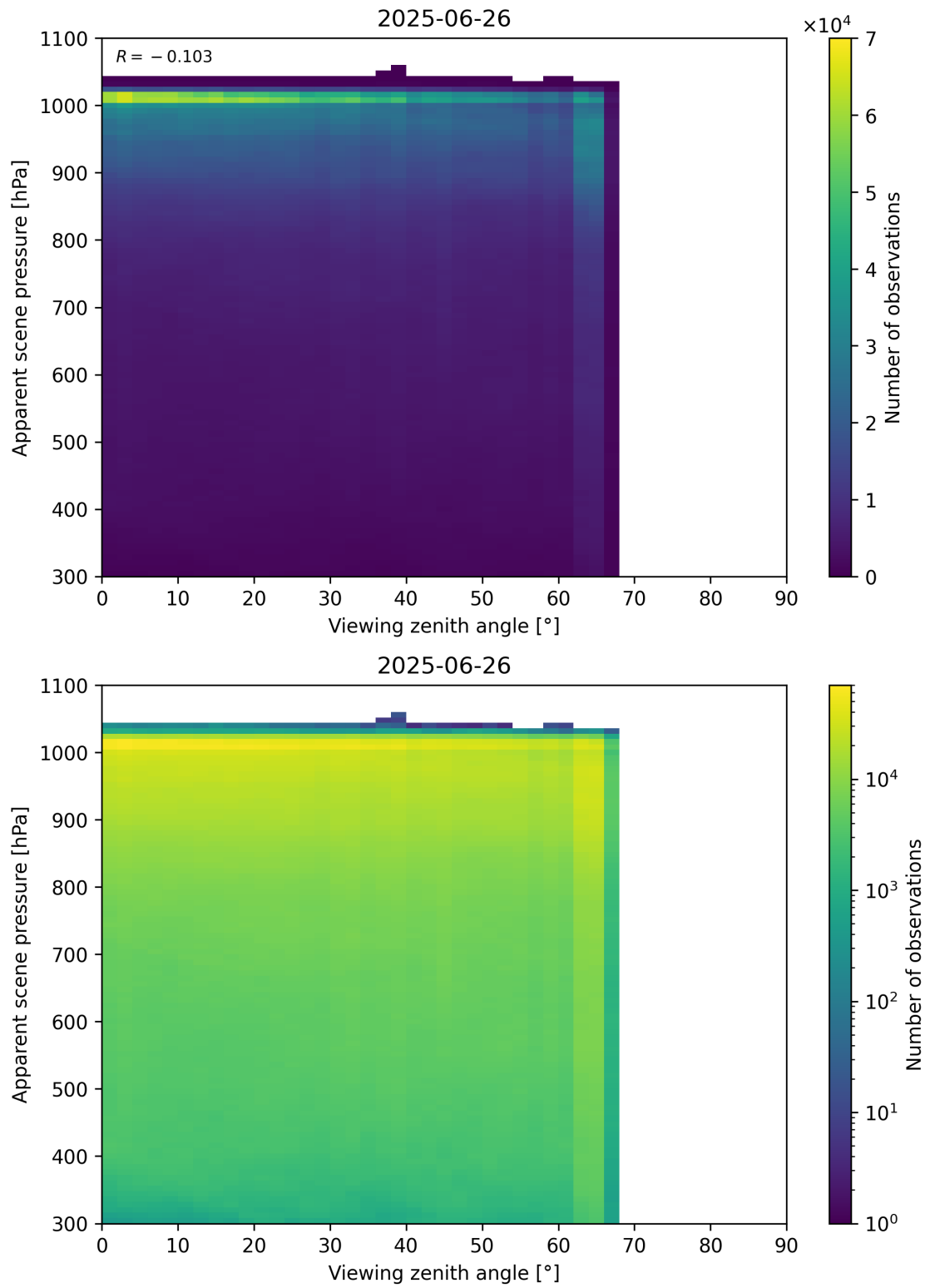
Figure 118: Scatter density plot of “Viewing zenith angle” against “Apparent scene pressure” for 2025-06-25 to 2025-06-27.
