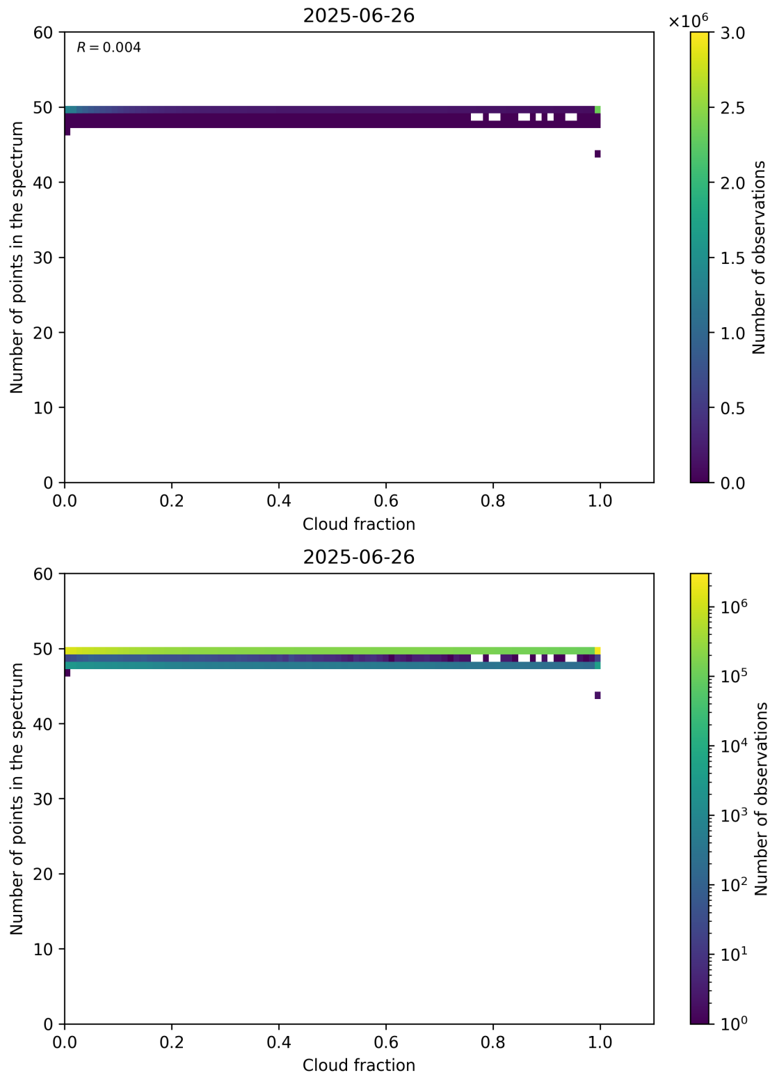
Figure 74: Scatter density plot of “Cloud fraction” against “Number of points in the spectrum” for 2025-06-25 to 2025-06-27.
