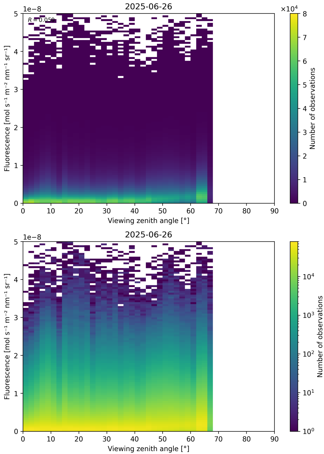
Figure 122: Scatter density plot of “Viewing zenith angle” against “Fluorescence” for 2025-06-25 to 2025-06-27.
