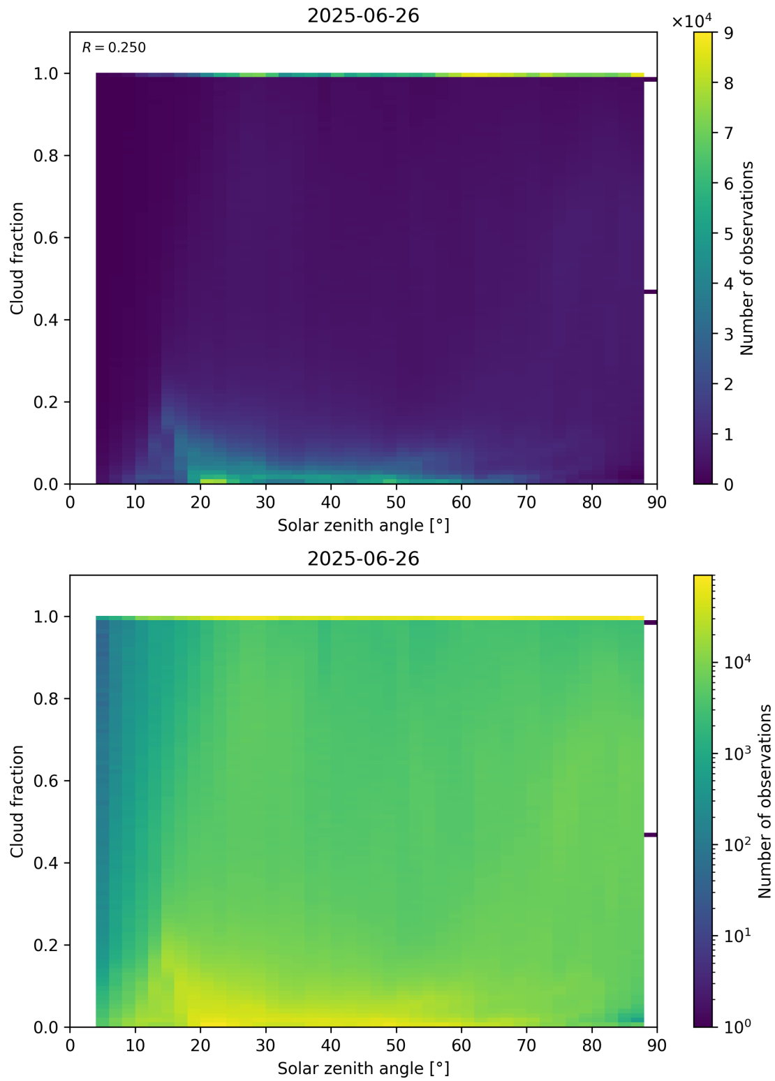
Figure 110: Scatter density plot of “Solar zenith angle” against “Cloud fraction” for 2025-06-25 to 2025-06-27.
