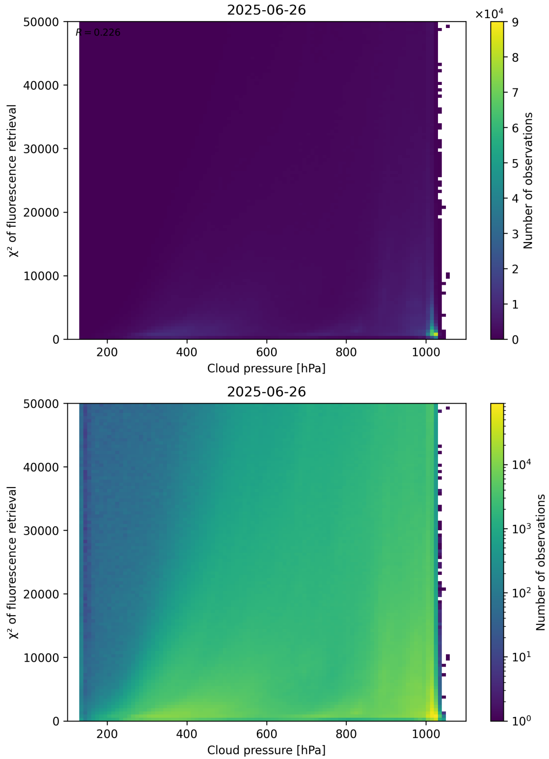
Figure 78: Scatter density plot of “Cloud pressure” against “ \chi^2 of fluorescence retrieval” for 2025-06-25 to 2025-06-27.
