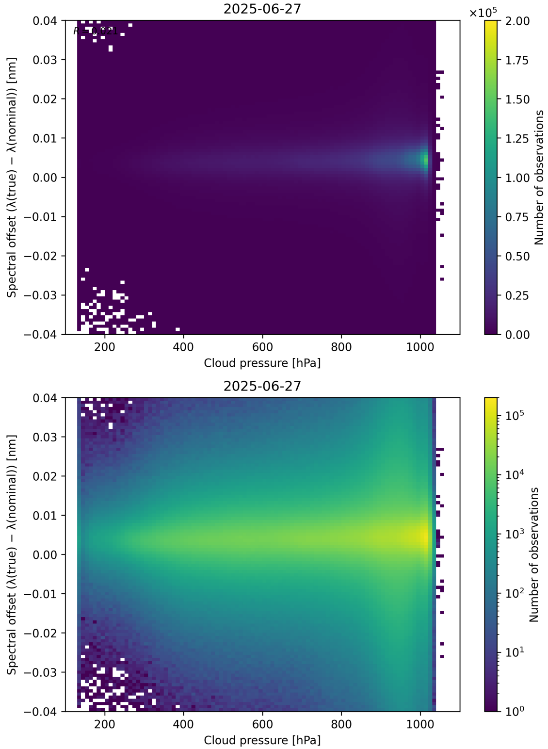
Figure 84: Scatter density plot of “Cloud pressure” against “Spectral offset ( \lambda_{\text{true}} - \lambda_{\text{nominal}} )” for 2025-06-27 to 2025-06-28.
