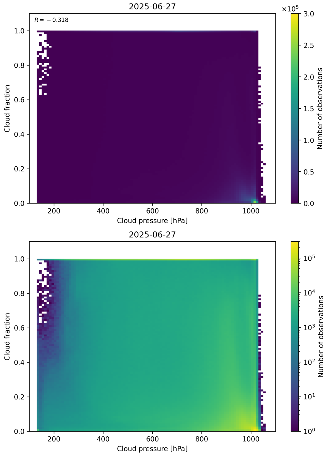
Figure 79: Scatter density plot of “Cloud pressure” against “Cloud fraction” for 2025-06-27 to 2025-06-28.
