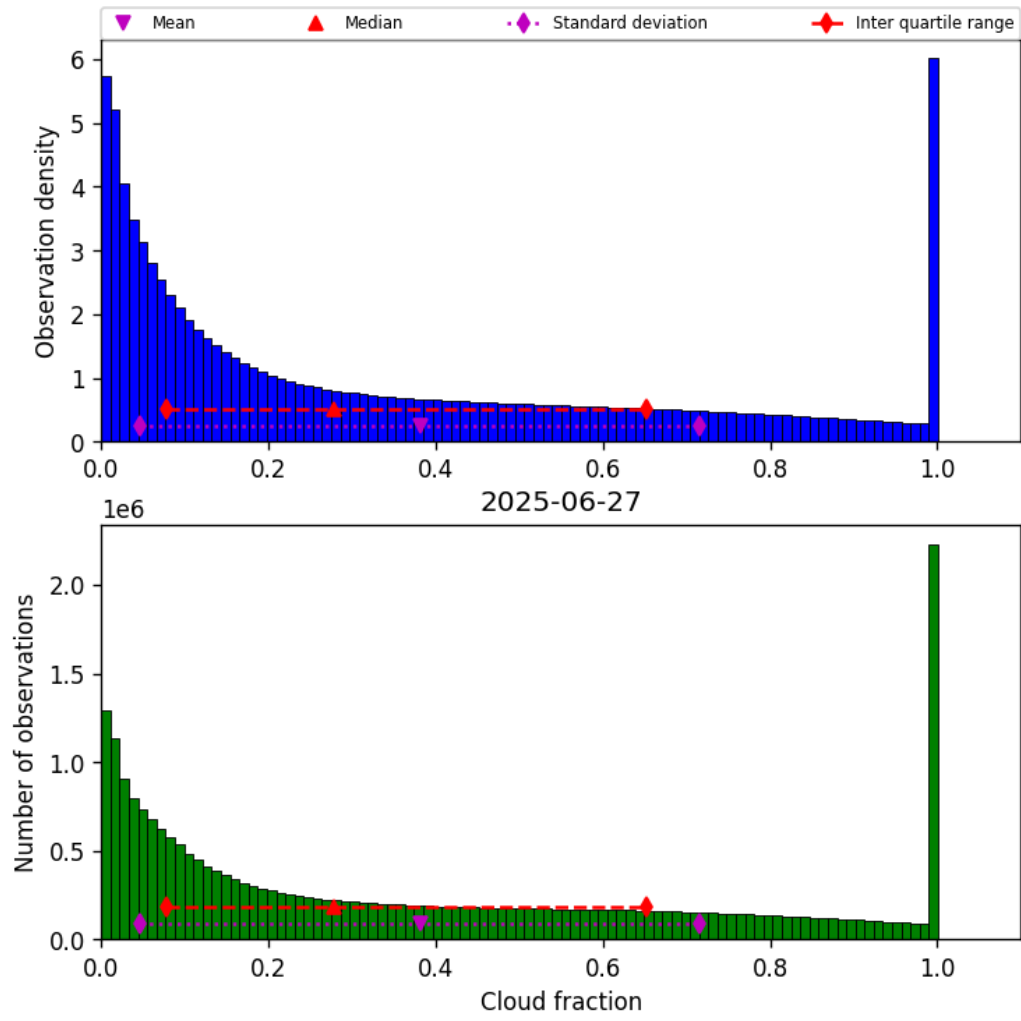
Figure 32: Histogram of “Cloud fraction” for 2025-06-27 to 2025-06-28
