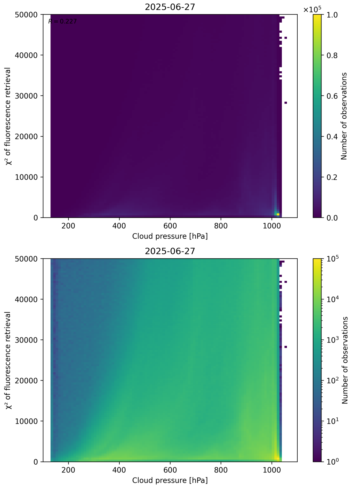
Figure 78: Scatter density plot of “Cloud pressure” against “ \chi^2 of fluorescence retrieval” for 2025-06-27 to 2025-06-28.
