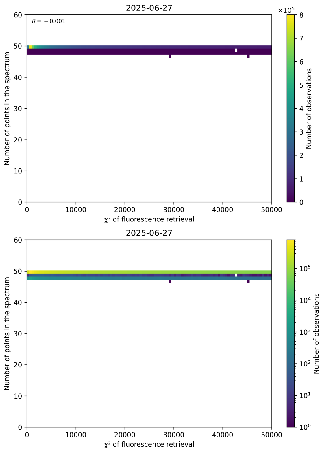
Figure 68: Scatter density plot of “ \chi^2 of fluorescence retrieval” against “Number of points in the spectrum” for 2025-06-27 to 2025-06-28.
