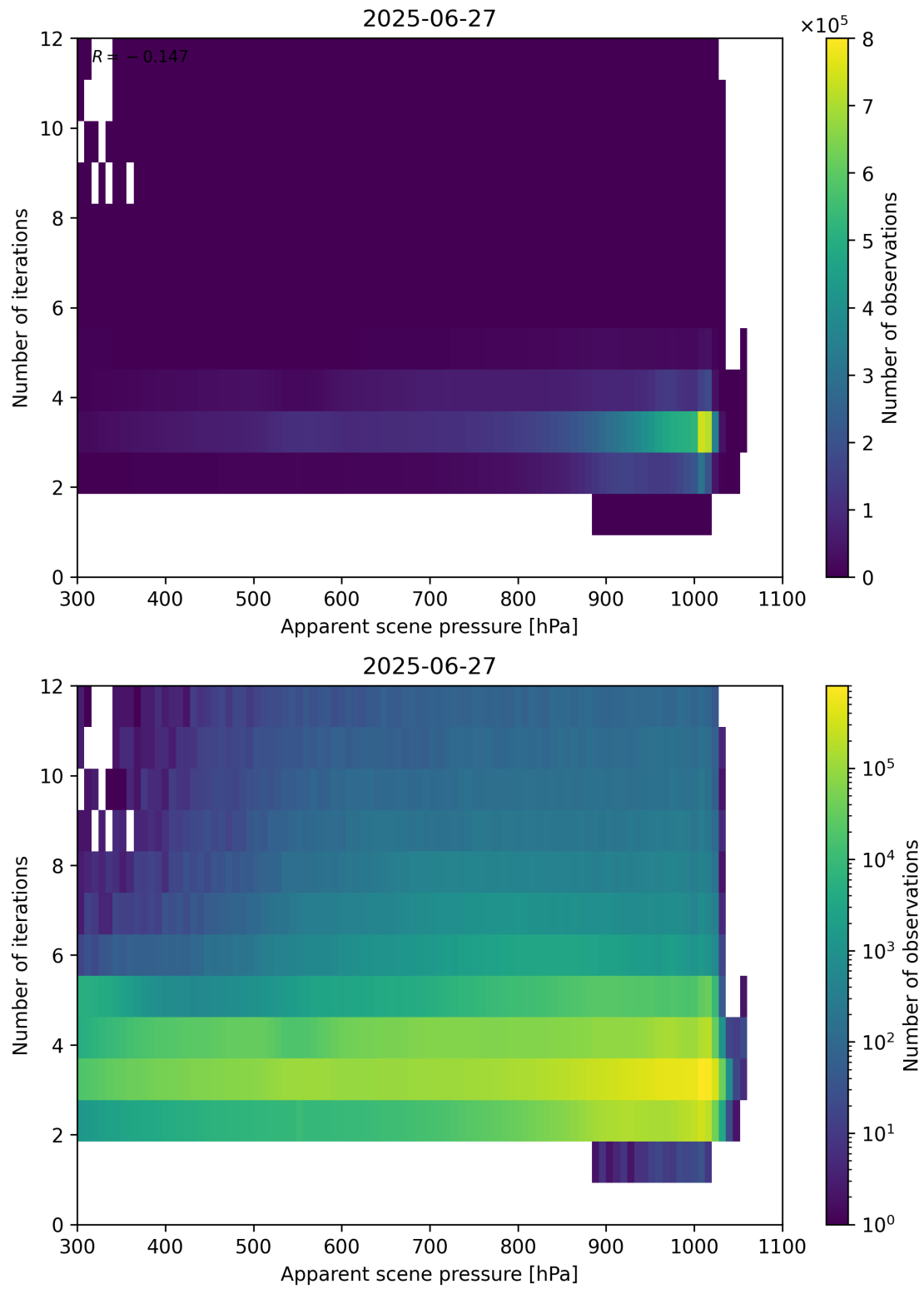
Figure 65: Scatter density plot of “Apparent scene pressure” against “Number of iterations” for 2025-06-27 to 2025-06-28.
