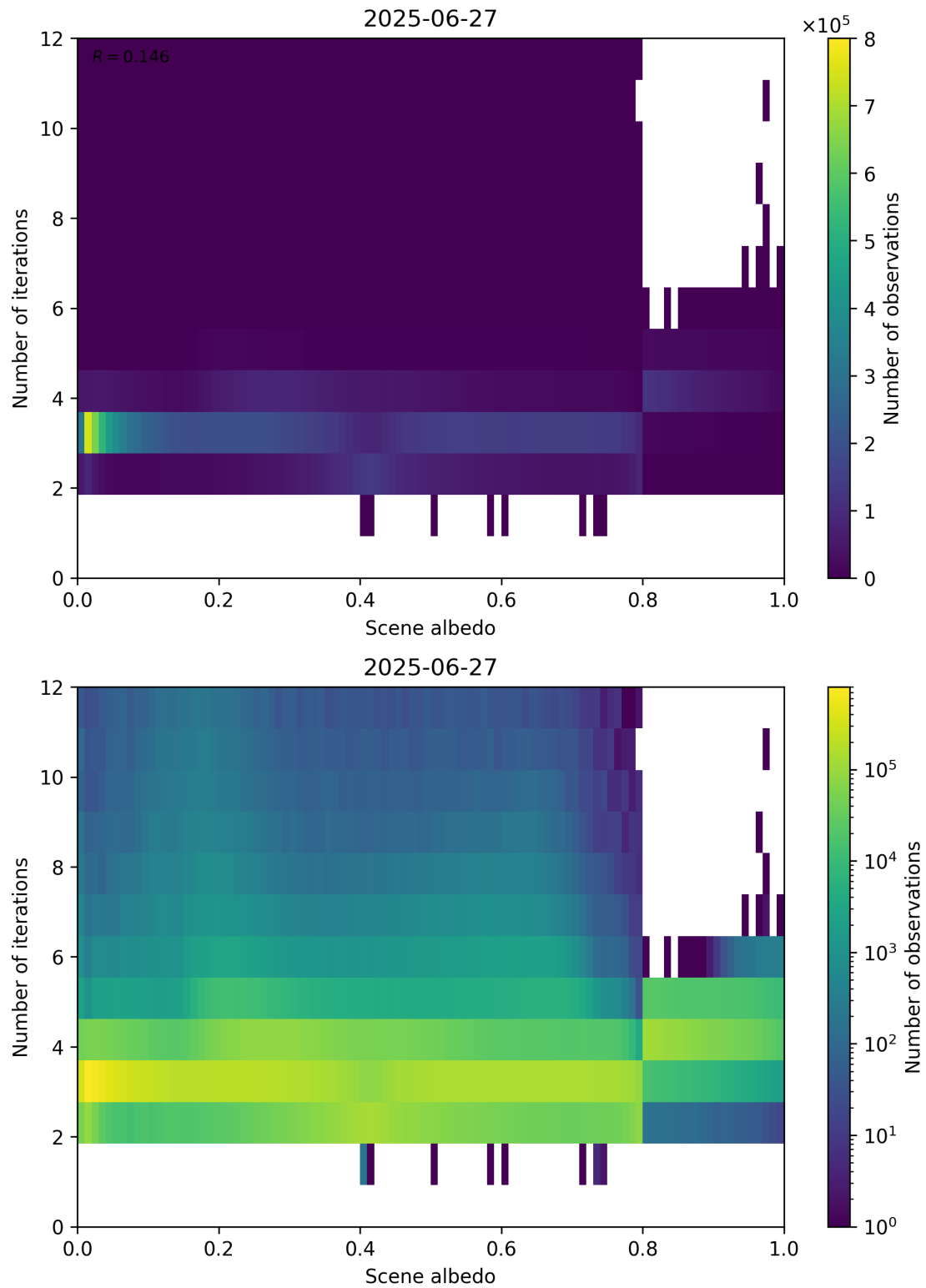
Figure 105: Scatter density plot of “Scene albedo” against “Number of iterations” for 2025-06-27 to 2025-06-28.
