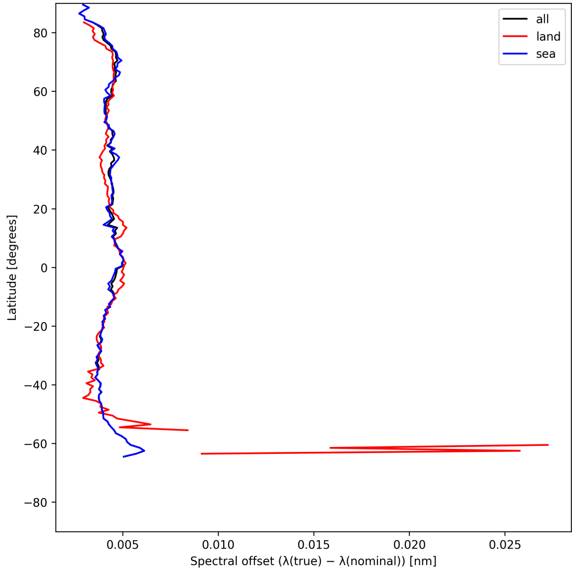
Figure 28: Zonal average of “Spectral offset ( \lambda_{\text{true}} - \lambda_{\text{nominal}} )” for 2025-06-27 to 2025-06-28.
