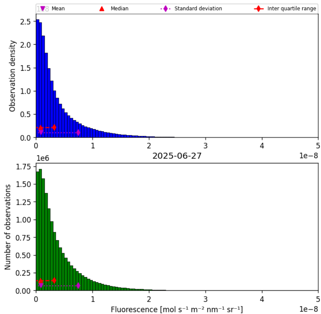
Figure 40: Histogram of “Fluorescence” for 2025-06-27 to 2025-06-28
