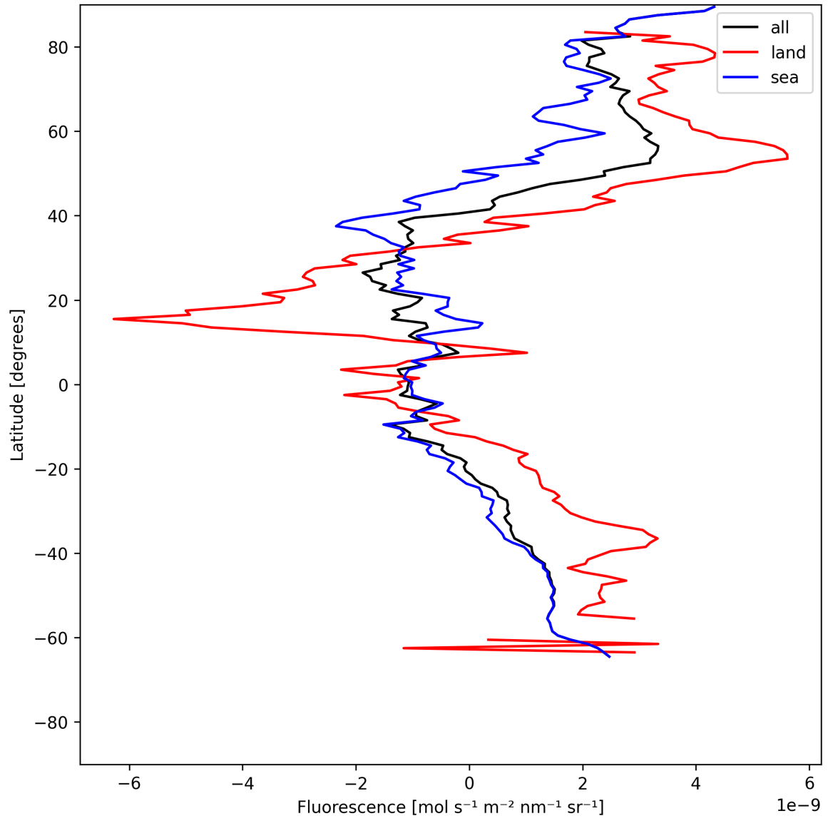
Figure 23: Zonal average of “Fluorescence” for 2025-06-27 to 2025-06-28.
