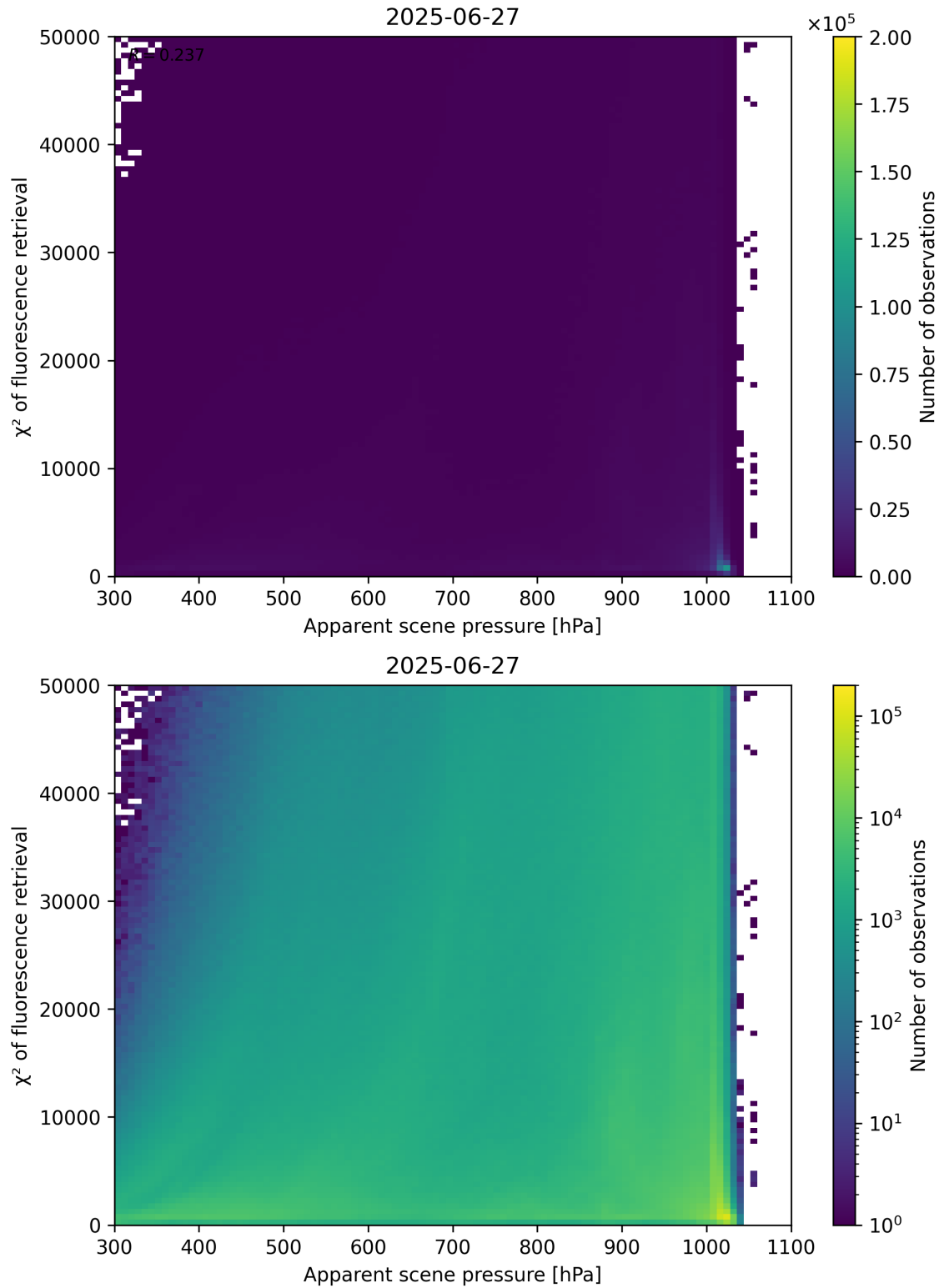
Figure 63: Scatter density plot of “Apparent scene pressure” against “ \chi^2 of fluorescence retrieval” for 2025-06-27 to 2025-06-28.
