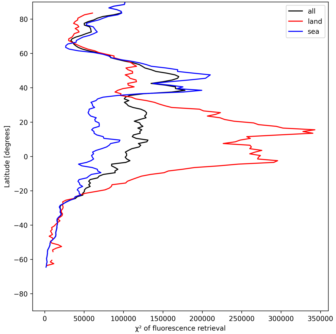
Figure 25: Zonal average of “ \chi^2 of fluorescence retrieval” for 2025-06-27 to 2025-06-28.
