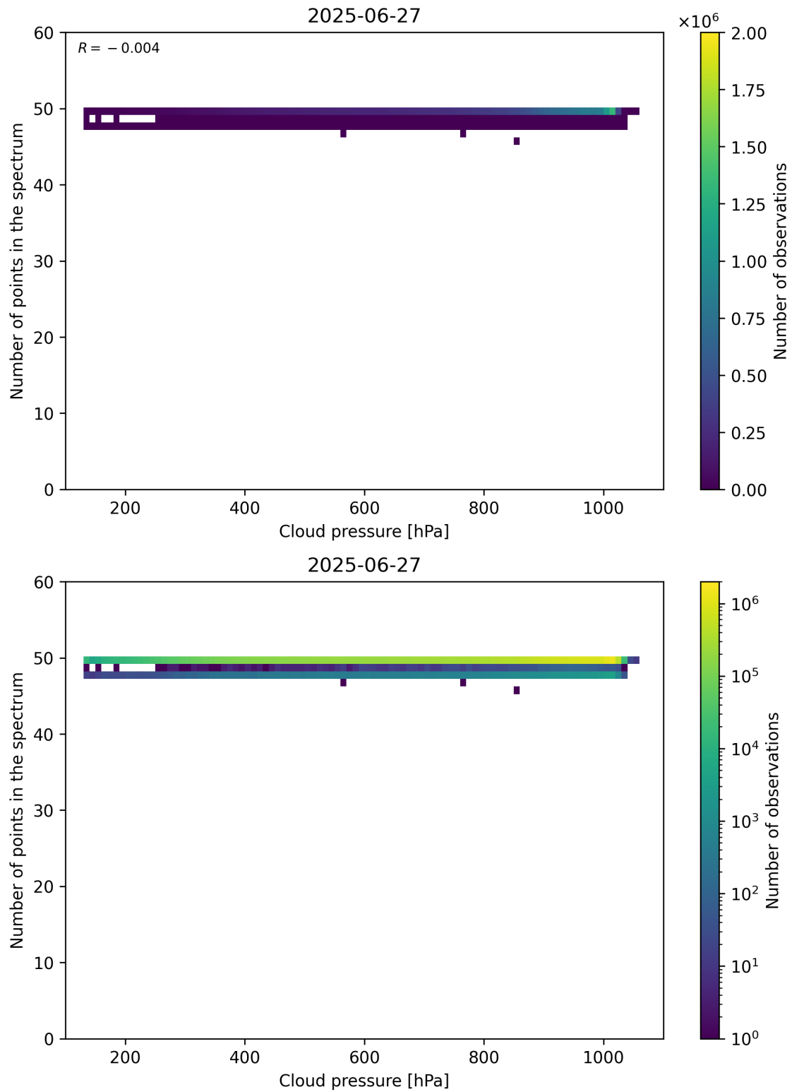
Figure 82: Scatter density plot of “Cloud pressure” against “Number of points in the spectrum” for 2025-06-27 to 2025-06-28.
