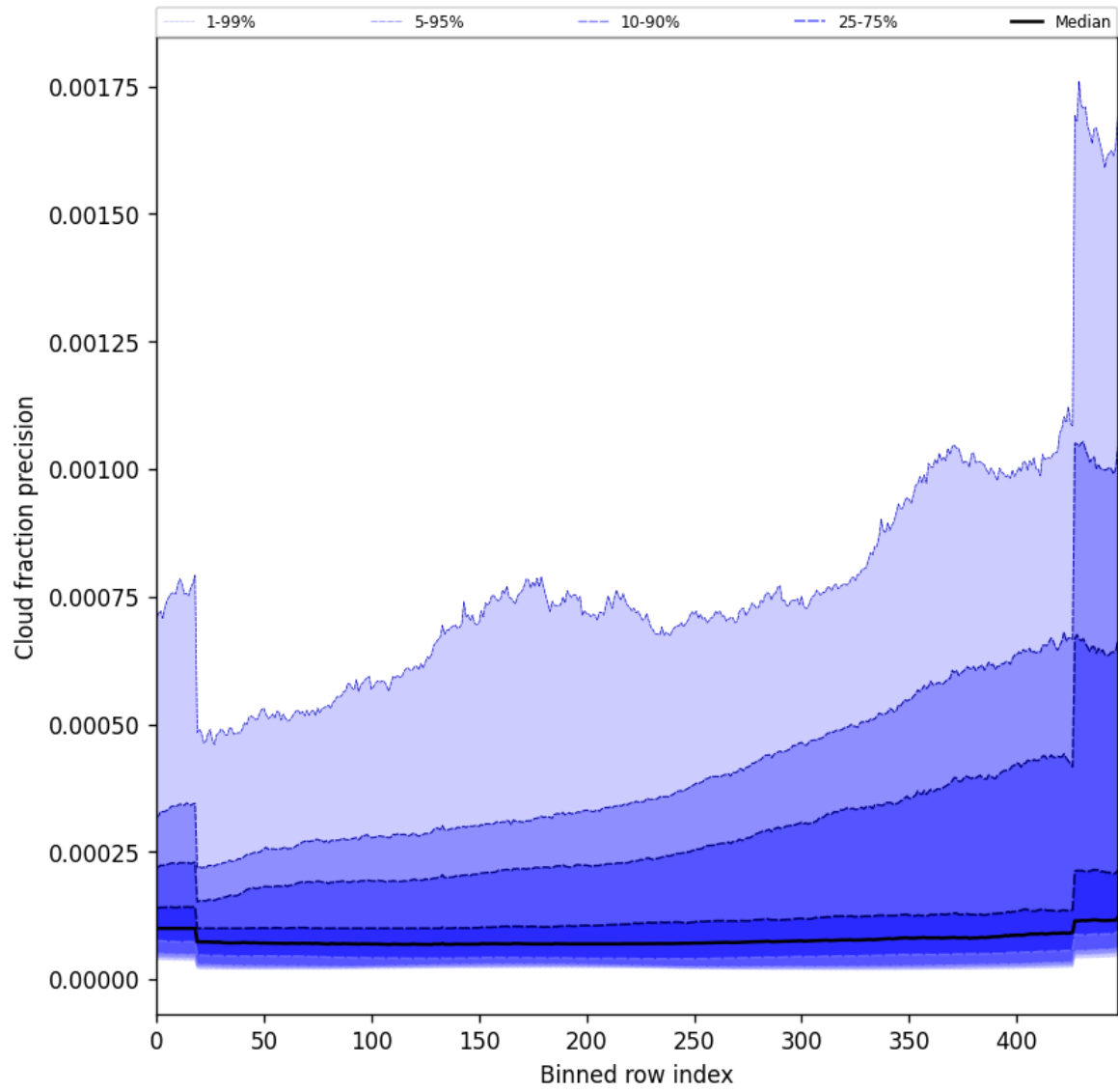
Figure 50: Along track statistics of “Cloud fraction precision” for 2025-06-27 to 2025-06-28
