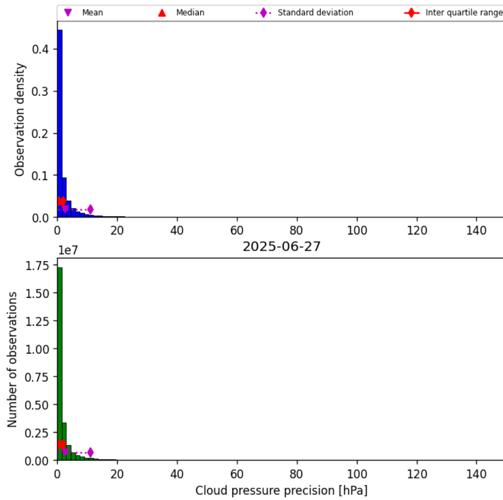
Figure 31: Histogram of “Cloud pressure precision” for 2025-06-27 to 2025-06-28
