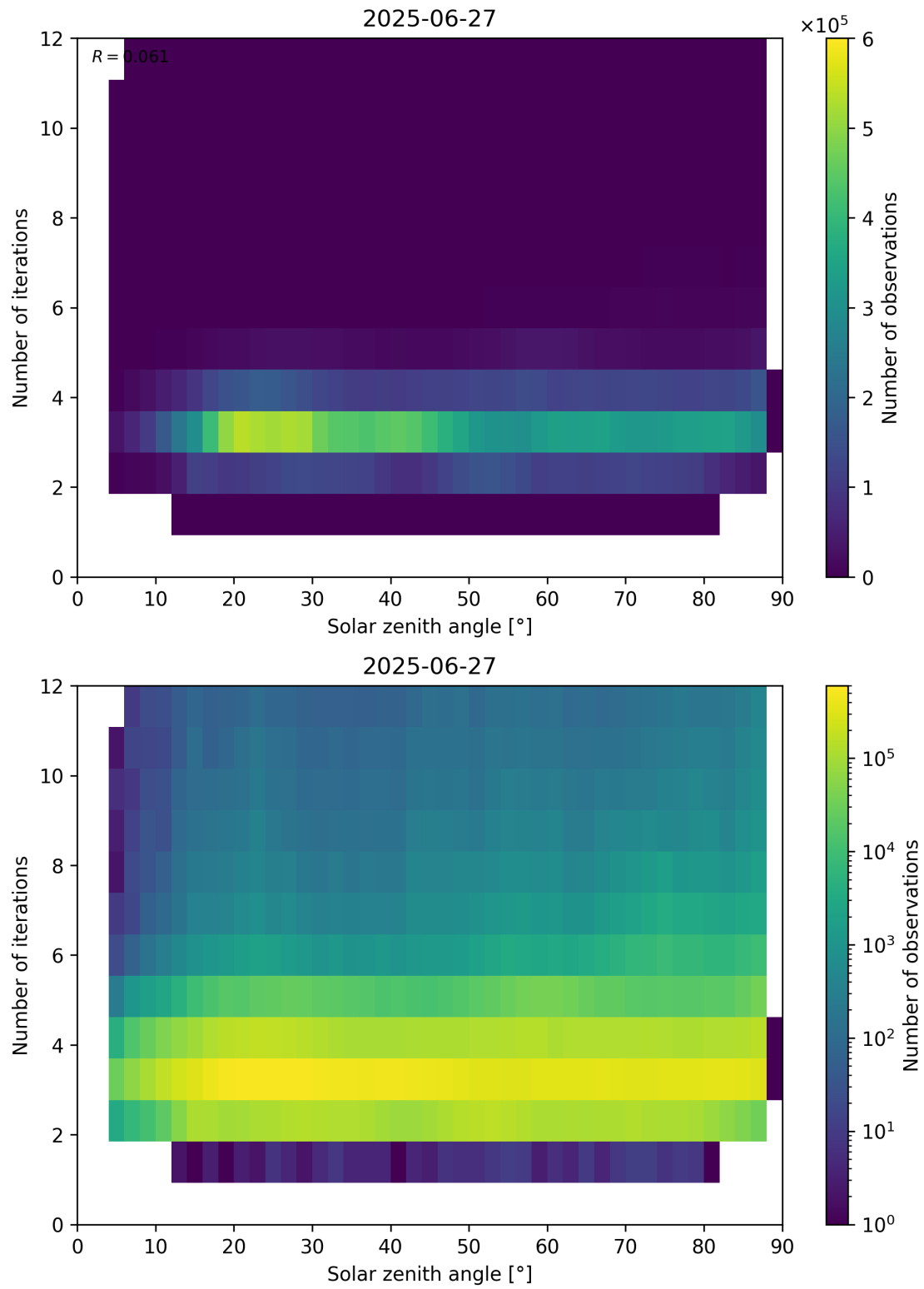
Figure 114: Scatter density plot of “Solar zenith angle” against “Number of iterations” for 2025-06-27 to 2025-06-28.
