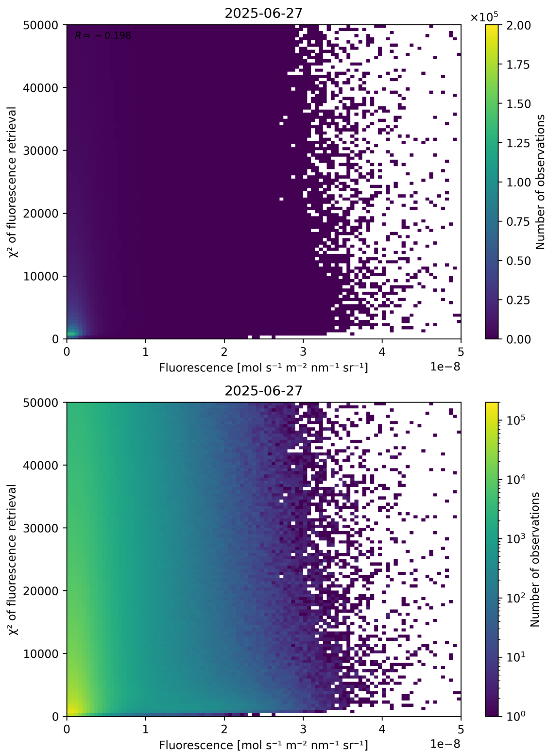
Figure 85: Scatter density plot of “Fluorescence” against “ \chi^2 of fluorescence retrieval” for 2025-06-27 to 2025-06-28.
