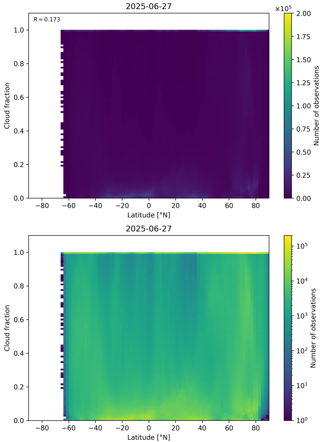
Figure 90: Scatter density plot of “Latitude” against “Cloud fraction” for 2025-06-27 to 2025-06-28.
