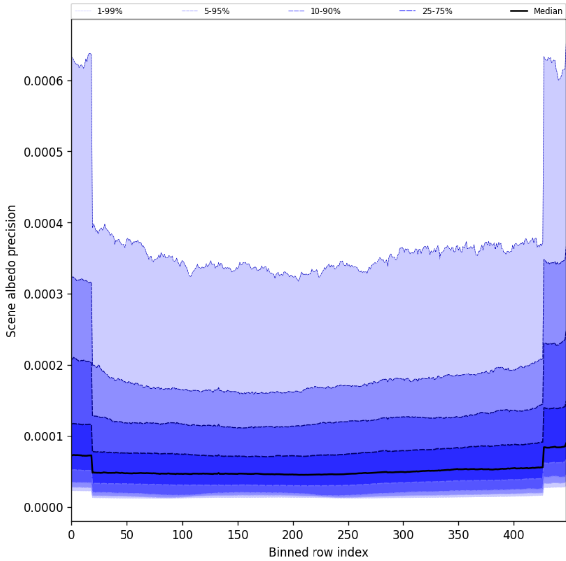
Figure 52: Along track statistics of “Scene albedo precision” for 2025-06-27 to 2025-06-28
