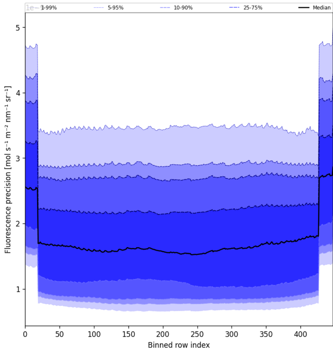
Figure 58: Along track statistics of “Fluorescence precision” for 2025-06-27 to 2025-06-28
