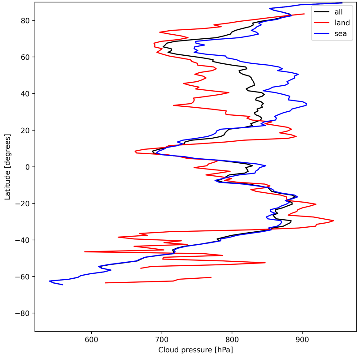
Figure 13: Zonal average of “Cloud pressure” for 2025-06-27 to 2025-06-28.
