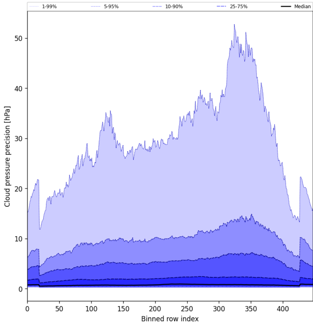
Figure 48: Along track statistics of “Cloud pressure precision” for 2025-06-27 to 2025-06-28
