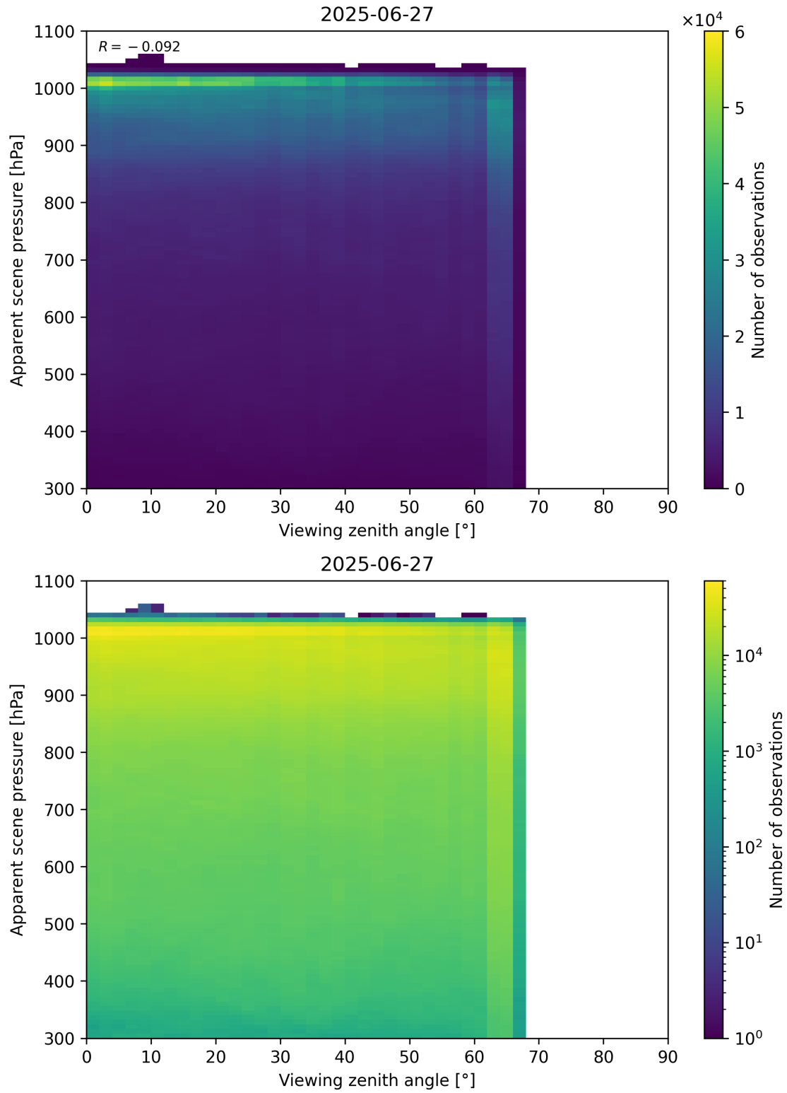
Figure 118: Scatter density plot of “Viewing zenith angle” against “Apparent scene pressure” for 2025-06-27 to 2025-06-28.
