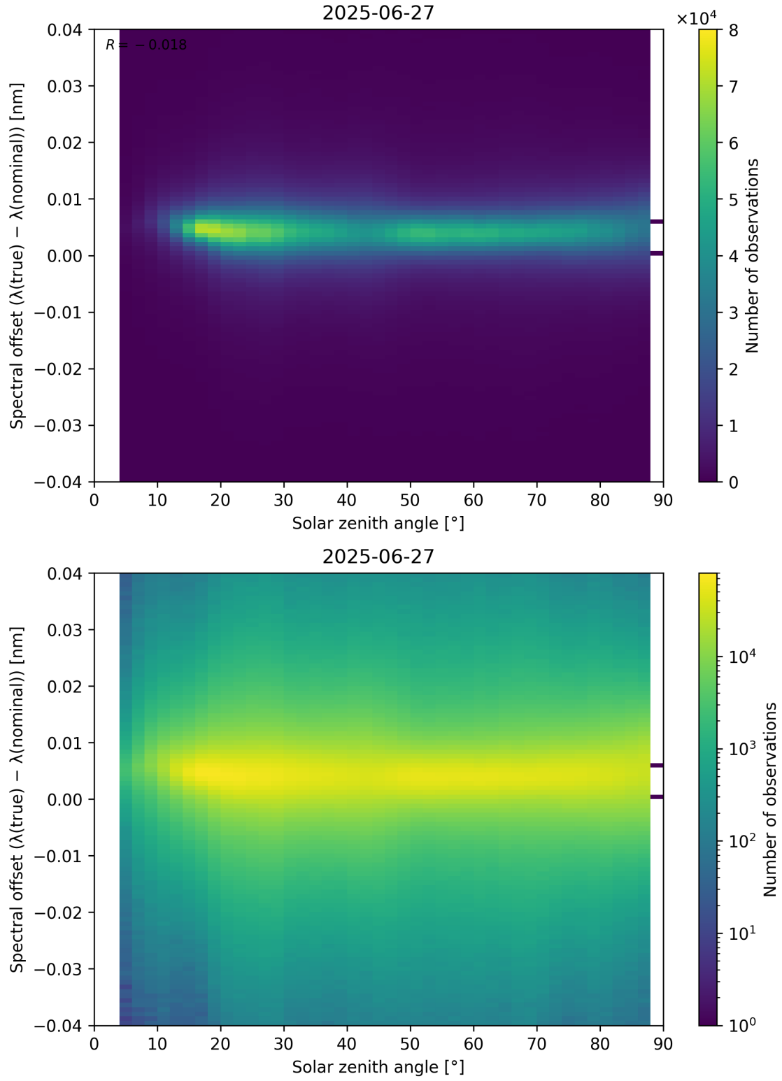
Figure 117: Scatter density plot of “Solar zenith angle” against “Spectral offset ( \lambda_{\text{true}} - \lambda_{\text{nominal}} )” for 2025-06-27 to 2025-06-28.
