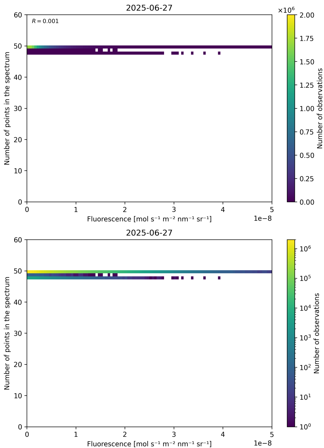
Figure 86: Scatter density plot of “Fluorescence” against “Number of points in the spectrum” for 2025-06-27 to 2025-06-28.
