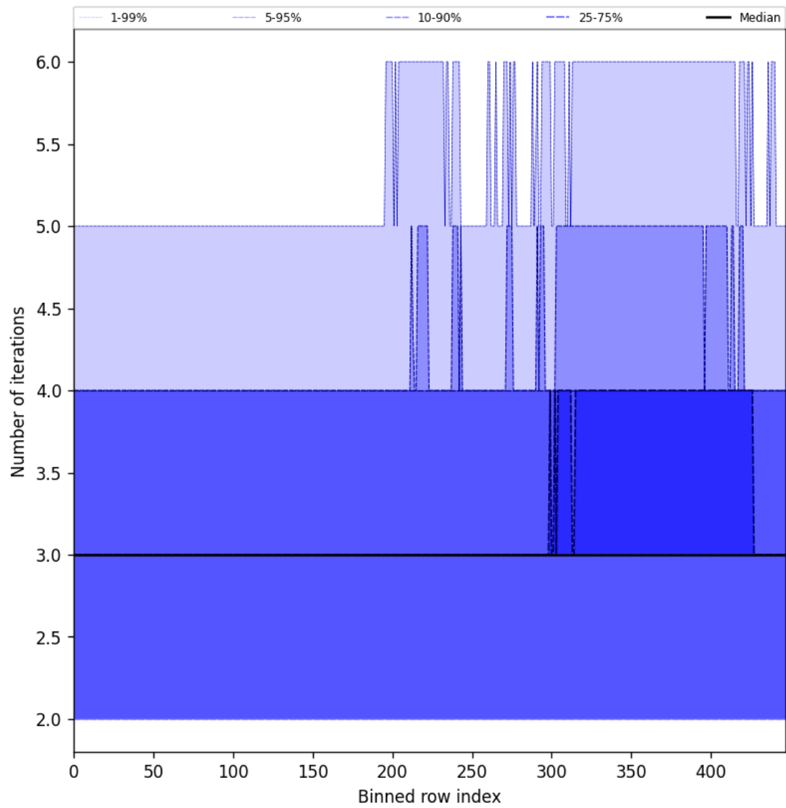
Figure 56: Along track statistics of “Number of iterations” for 2025-06-27 to 2025-06-28
