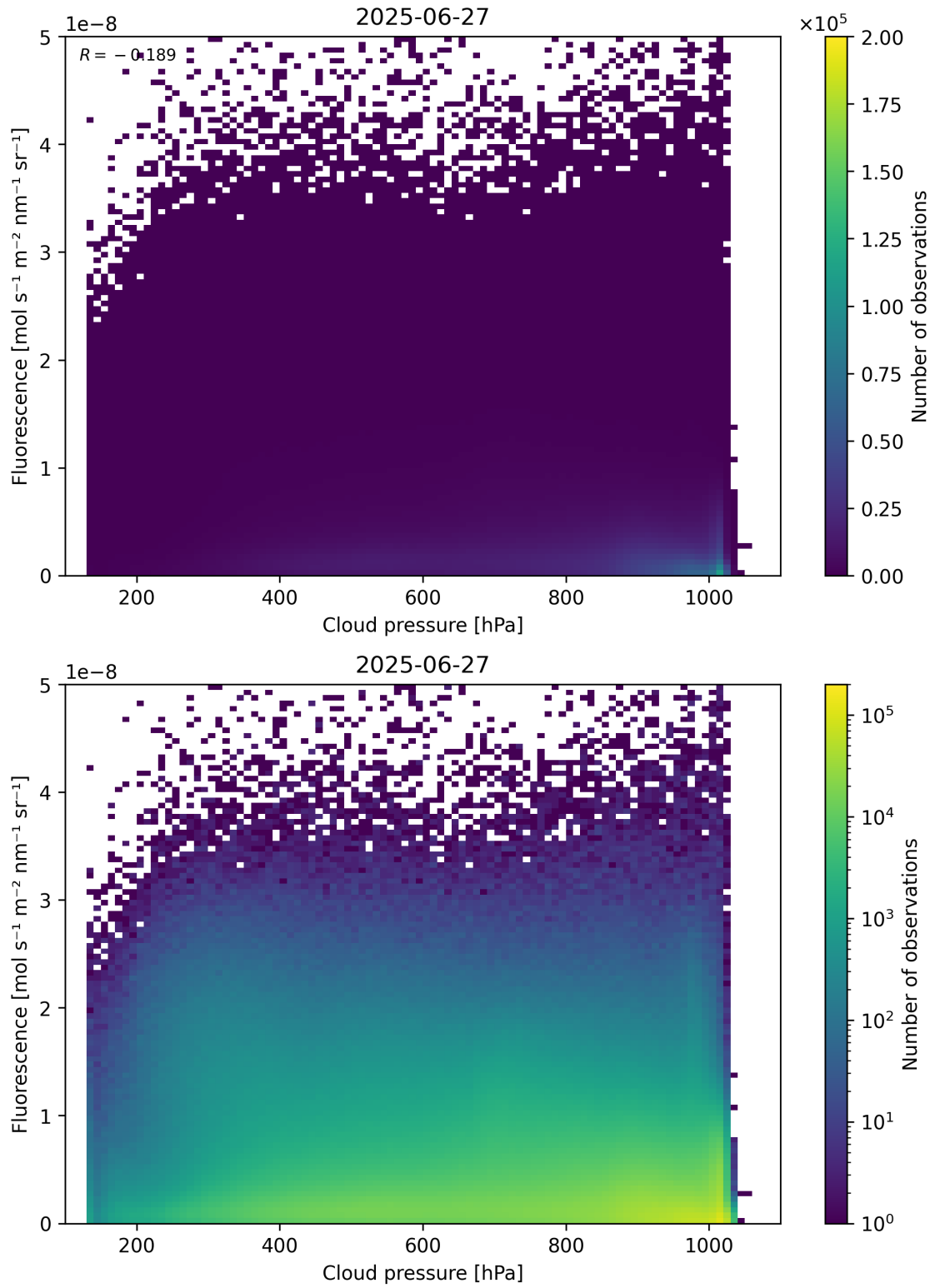
Figure 80: Scatter density plot of “Cloud pressure” against “Fluorescence” for 2025-06-27 to 2025-06-28.
