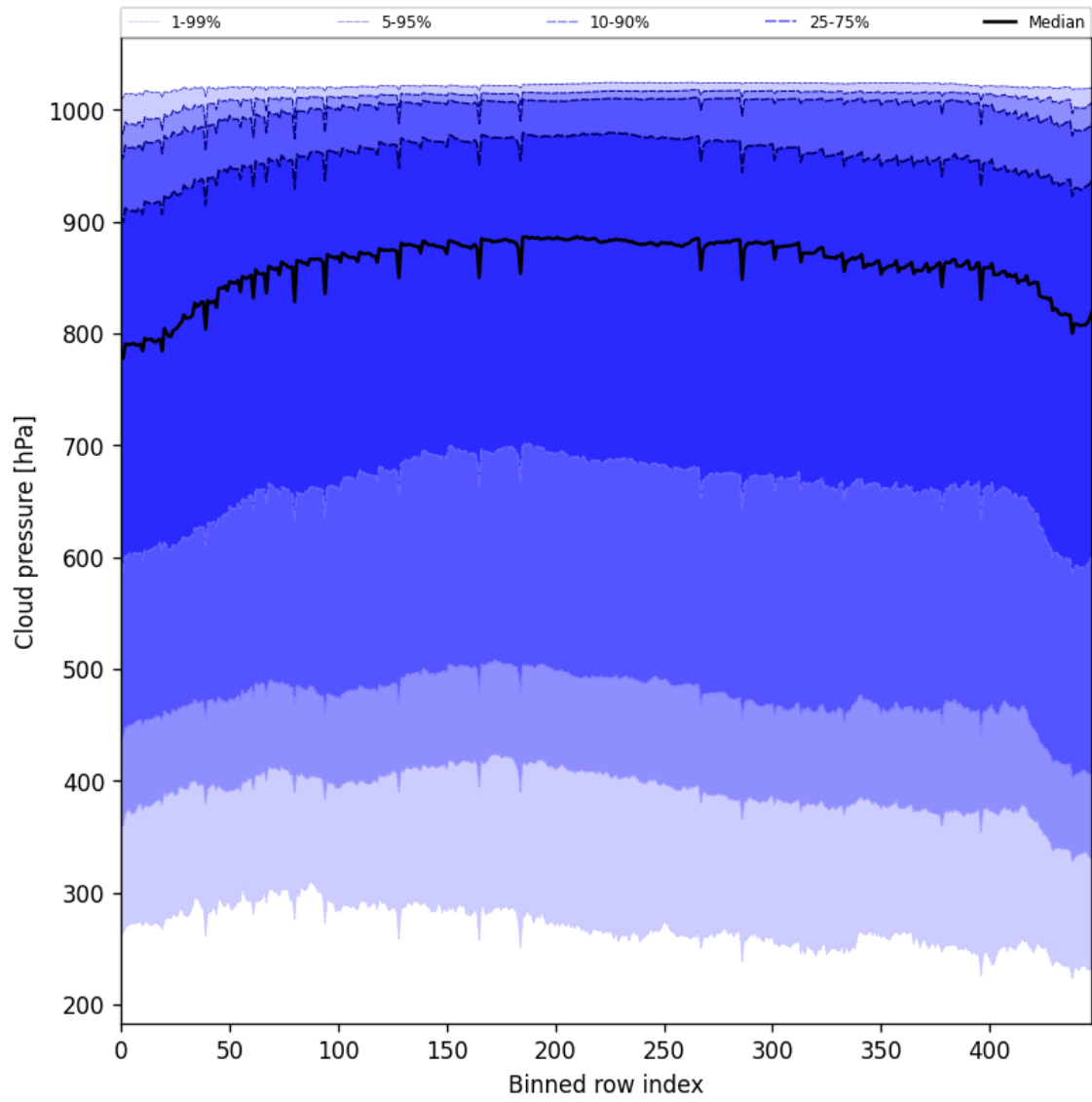
Figure 47: Along track statistics of “Cloud pressure” for 2025-06-27 to 2025-06-28
