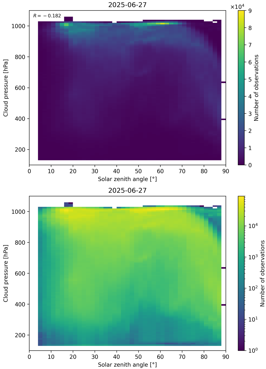
Figure 111: Scatter density plot of “Solar zenith angle” against “Cloud pressure” for 2025-06-27 to 2025-06-28.
