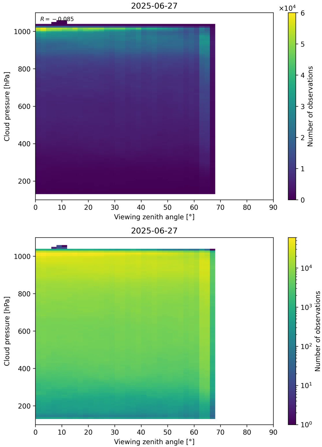
Figure 121: Scatter density plot of “Viewing zenith angle” against “Cloud pressure” for 2025-06-27 to 2025-06-28.
