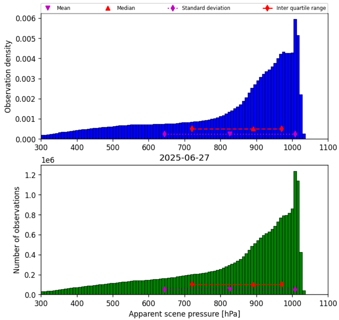
Figure 36: Histogram of “Apparent scene pressure” for 2025-06-27 to 2025-06-28
