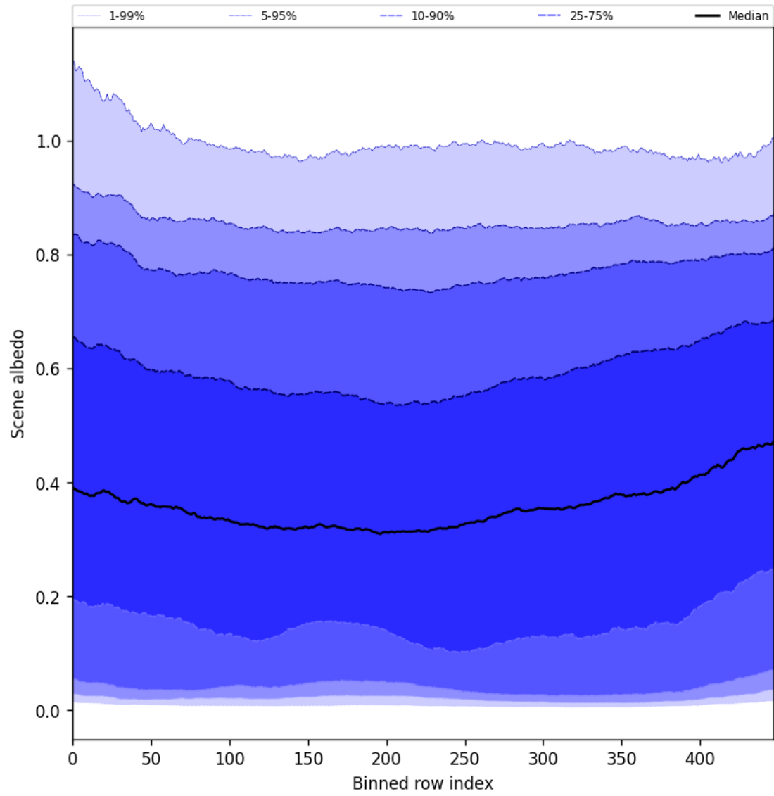
Figure 51: Along track statistics of “Scene albedo” for 2025-06-27 to 2025-06-28
