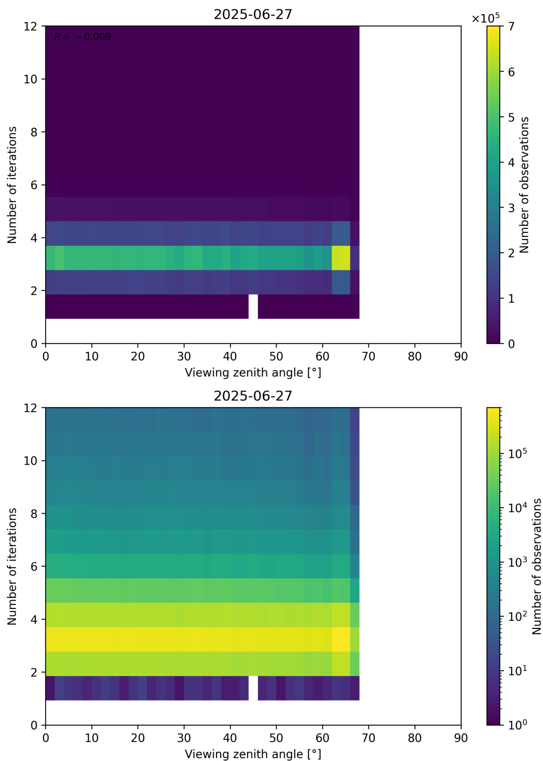
Figure 124: Scatter density plot of “Viewing zenith angle” against “Number of iterations” for 2025-06-27 to 2025-06-28.
