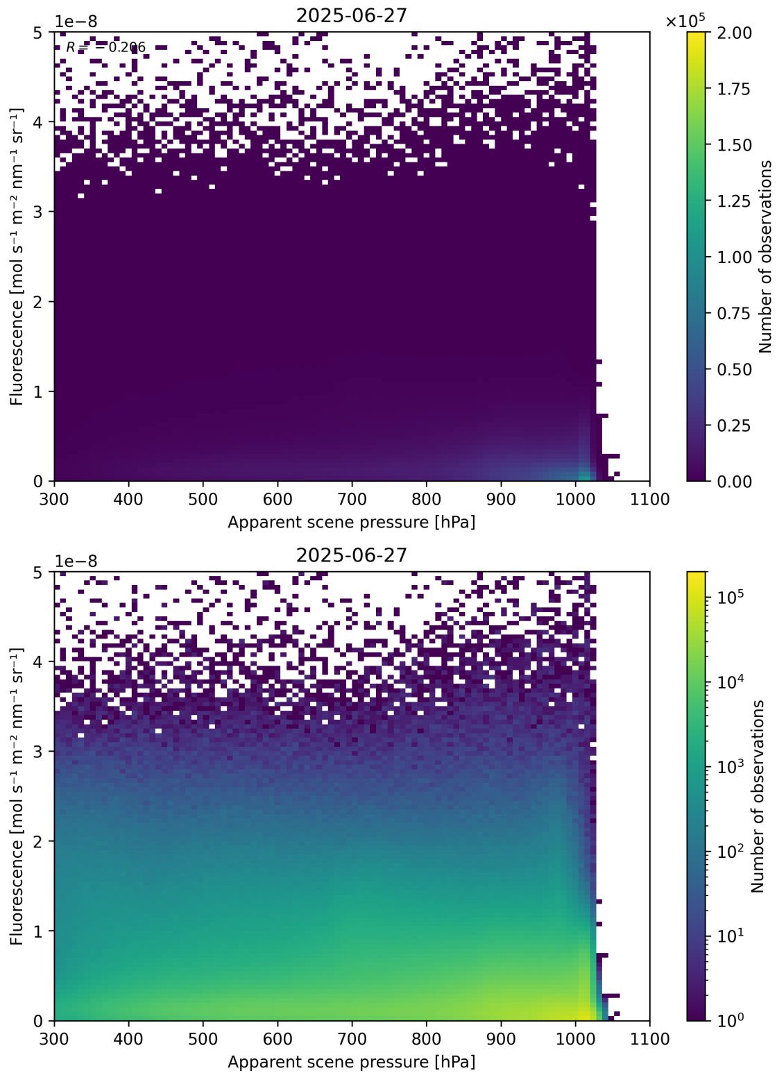
Figure 64: Scatter density plot of “Apparent scene pressure” against “Fluorescence” for 2025-06-27 to 2025-06-28.
