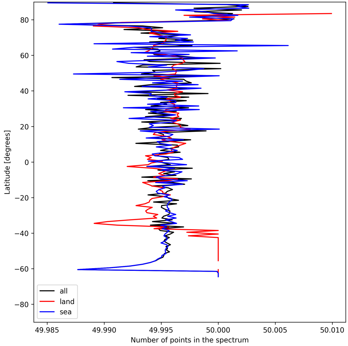
Figure 27: Zonal average of “Number of points in the spectrum” for 2025-06-27 to 2025-06-28.
