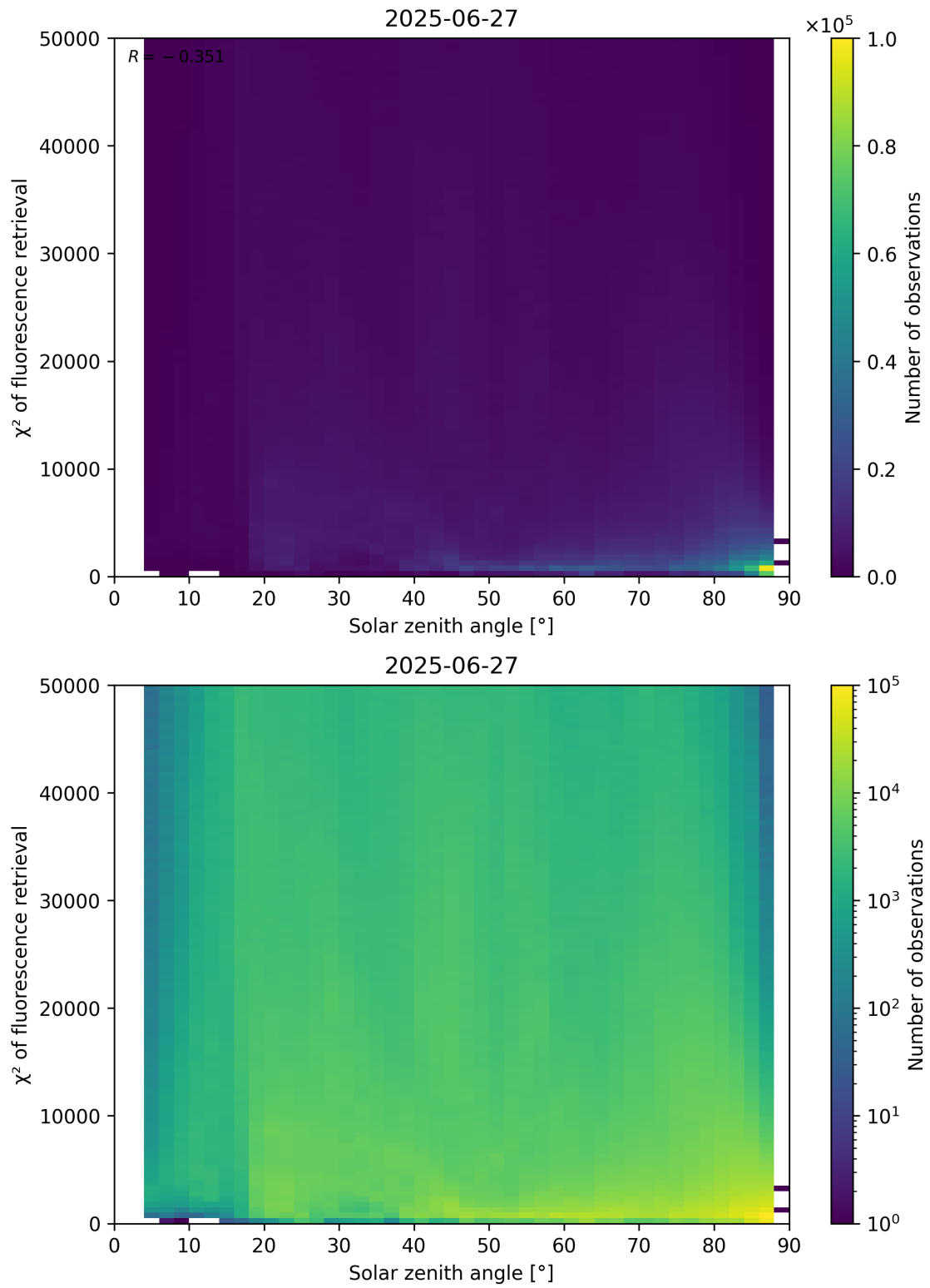
Figure 109: Scatter density plot of “Solar zenith angle” against “ \chi^2 of fluorescence retrieval” for 2025-06-27 to 2025-06-28.
