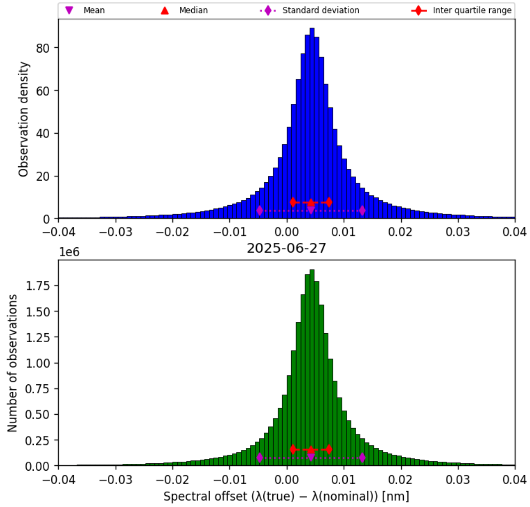
Figure 45: Histogram of “Spectral offset ( \lambda_{\text{true}} - \lambda_{\text{nominal}} )” for 2025-06-27 to 2025-06-28
