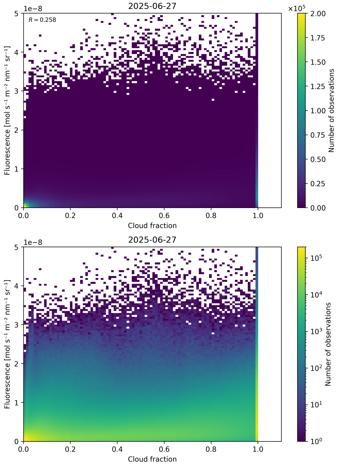
Figure 72: Scatter density plot of “Cloud fraction” against “Fluorescence” for 2025-06-27 to 2025-06-28.
