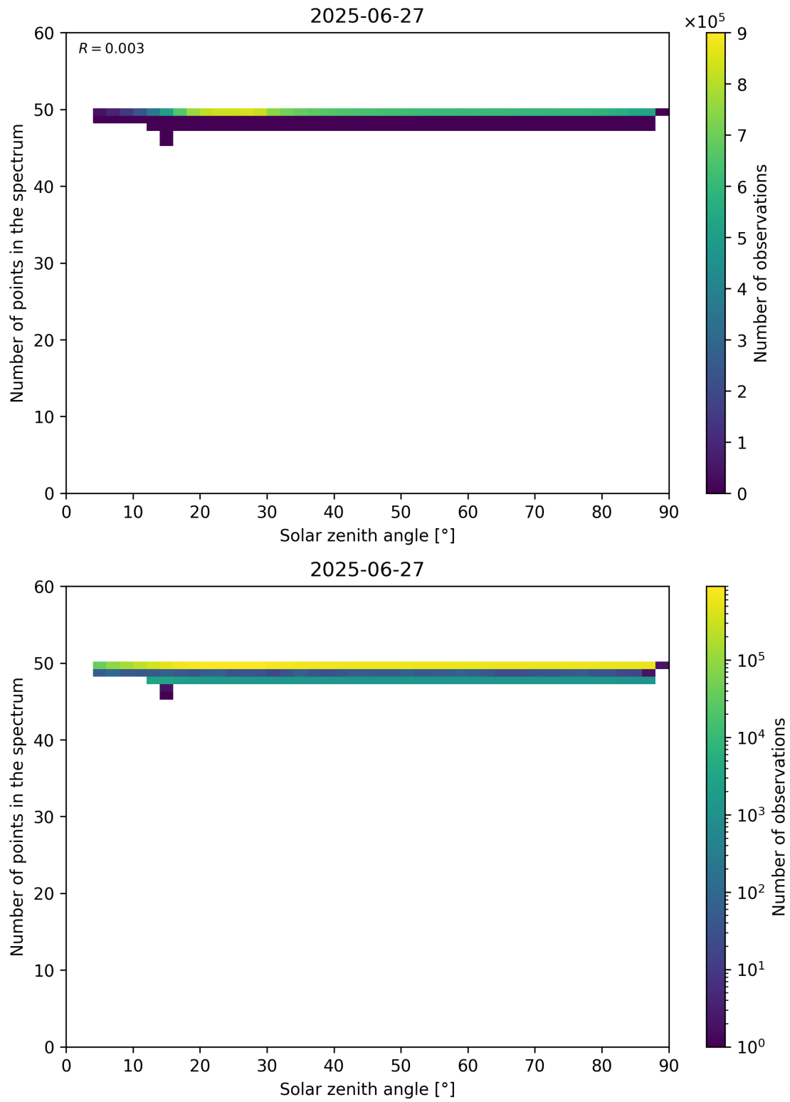
Figure 115: Scatter density plot of “Solar zenith angle” against “Number of points in the spectrum” for 2025-06-27 to 2025-06-28.
