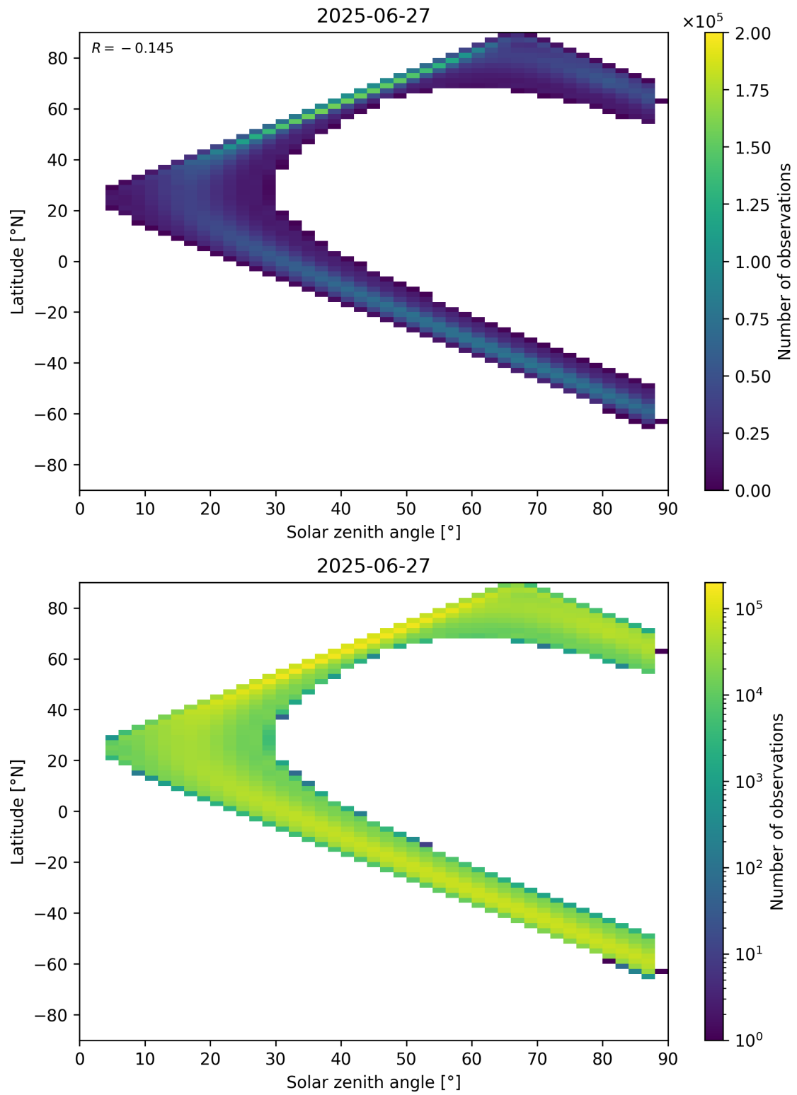
Figure 113: Scatter density plot of “Solar zenith angle” against “Latitude” for 2025-06-27 to 2025-06-28.
