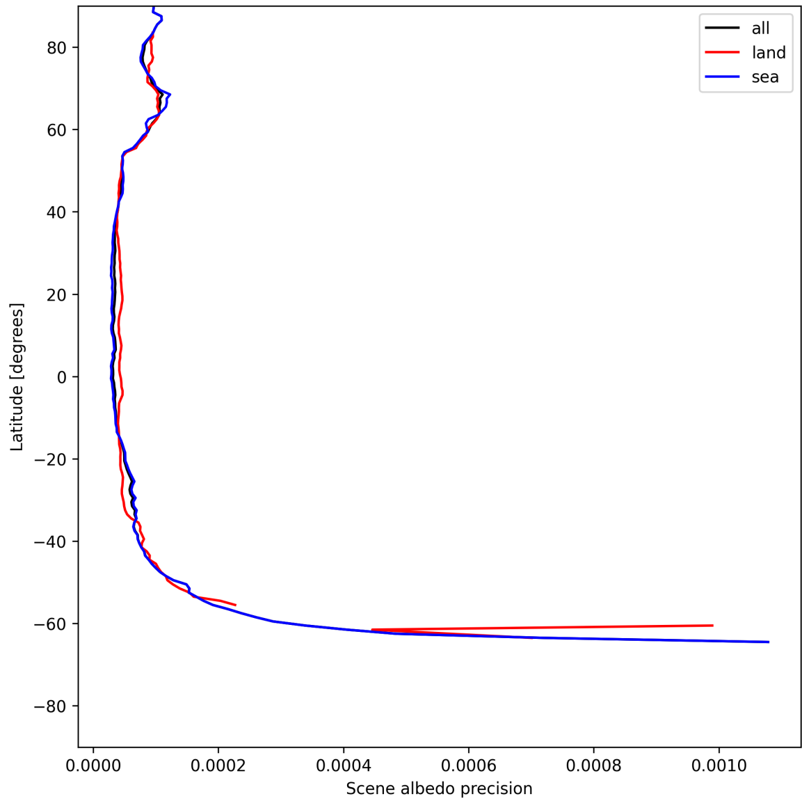
Figure 18: Zonal average of “Scene albedo precision” for 2025-06-27 to 2025-06-28.
