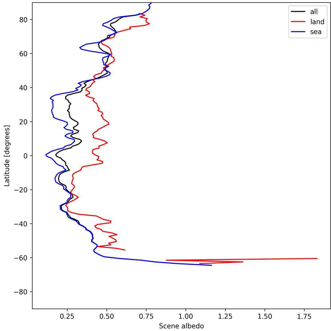
Figure 17: Zonal average of “Scene albedo” for 2025-06-27 to 2025-06-28.
