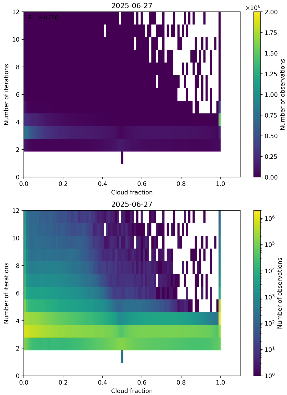
Figure 73: Scatter density plot of “Cloud fraction” against “Number of iterations” for 2025-06-27 to 2025-06-28.
