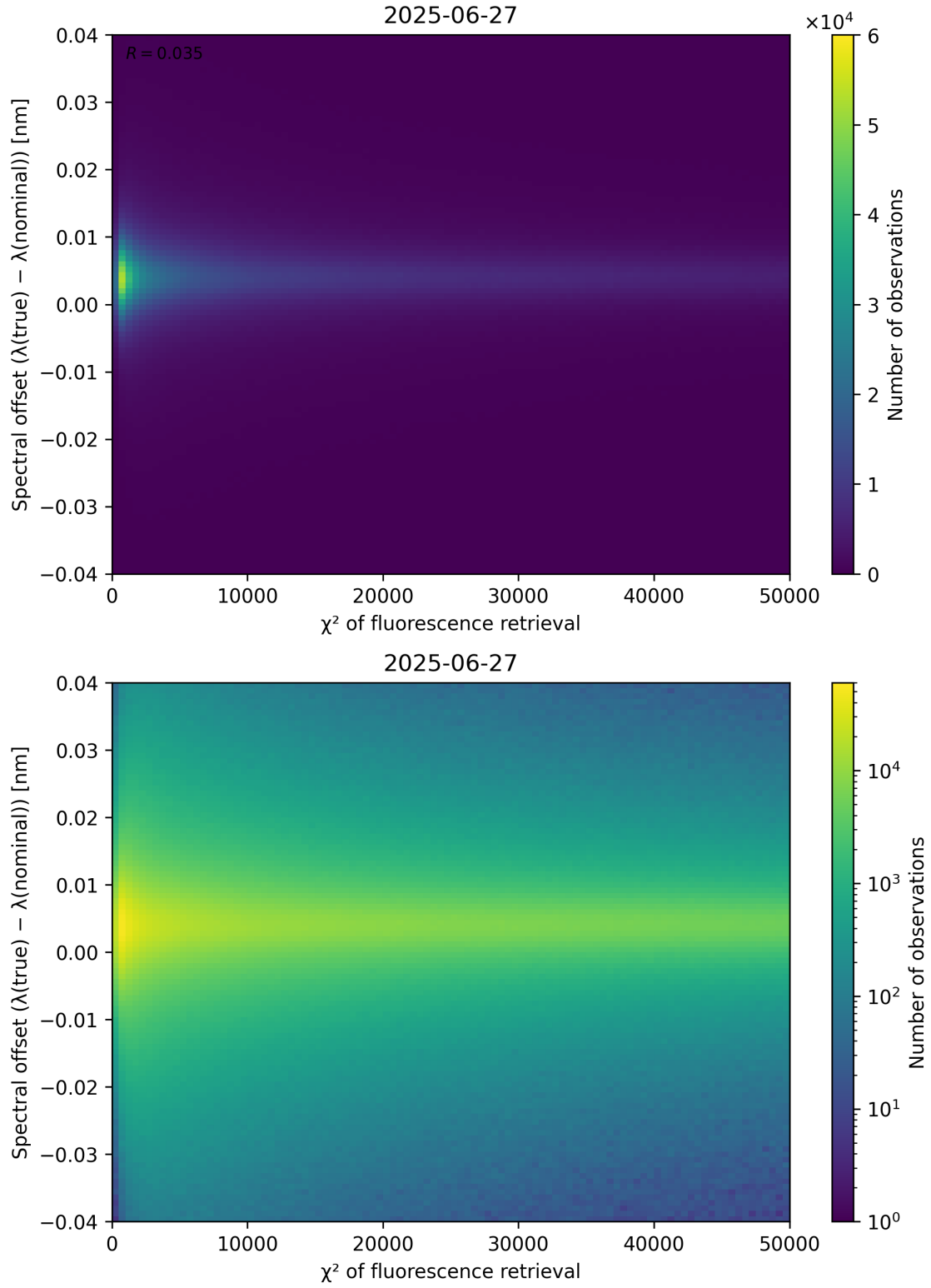
Figure 69: Scatter density plot of “ \chi^2 of fluorescence retrieval” against “Spectral offset ( \lambda_{\text{true}} - \lambda_{\text{nominal}} )” for 2025-06-27 to 2025-06-28.
