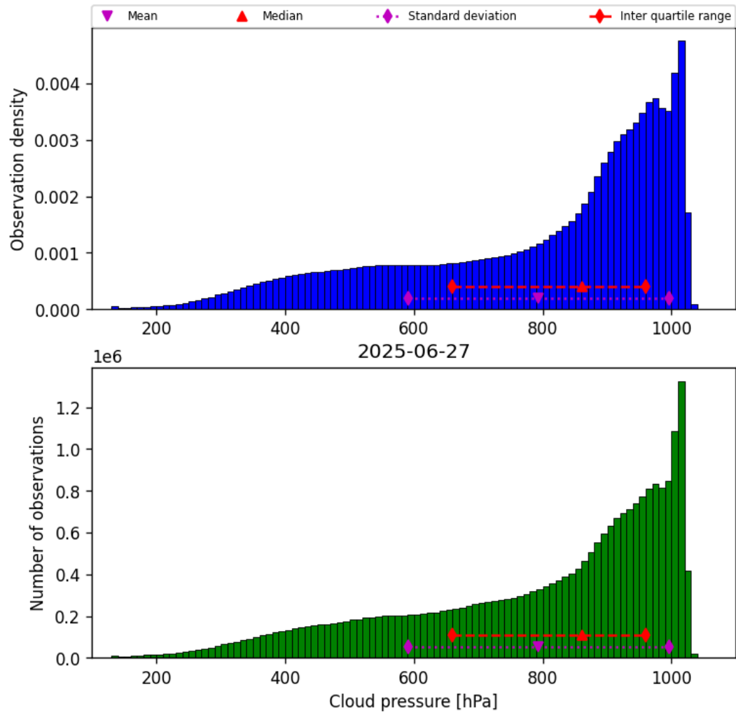
Figure 30: Histogram of “Cloud pressure” for 2025-06-27 to 2025-06-28
