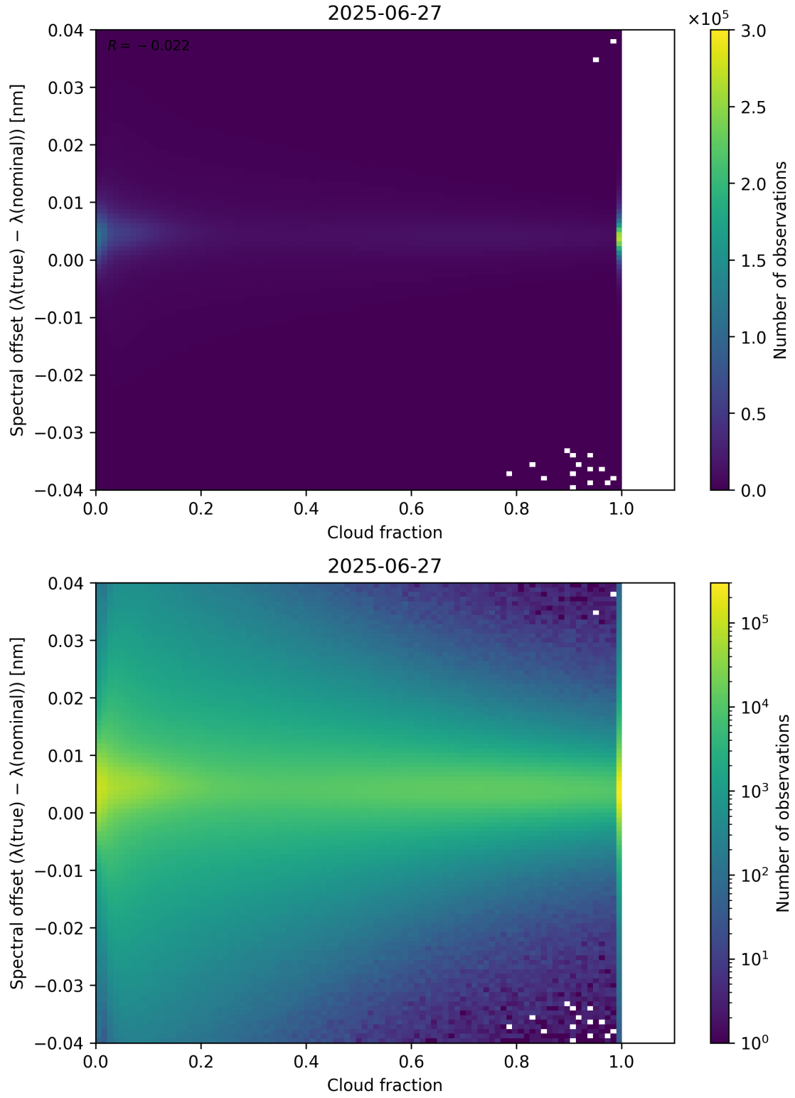
Figure 76: Scatter density plot of “Cloud fraction” against “Spectral offset ( \lambda_{\text{true}} - \lambda_{\text{nominal}} )” for 2025-06-27 to 2025-06-28.
