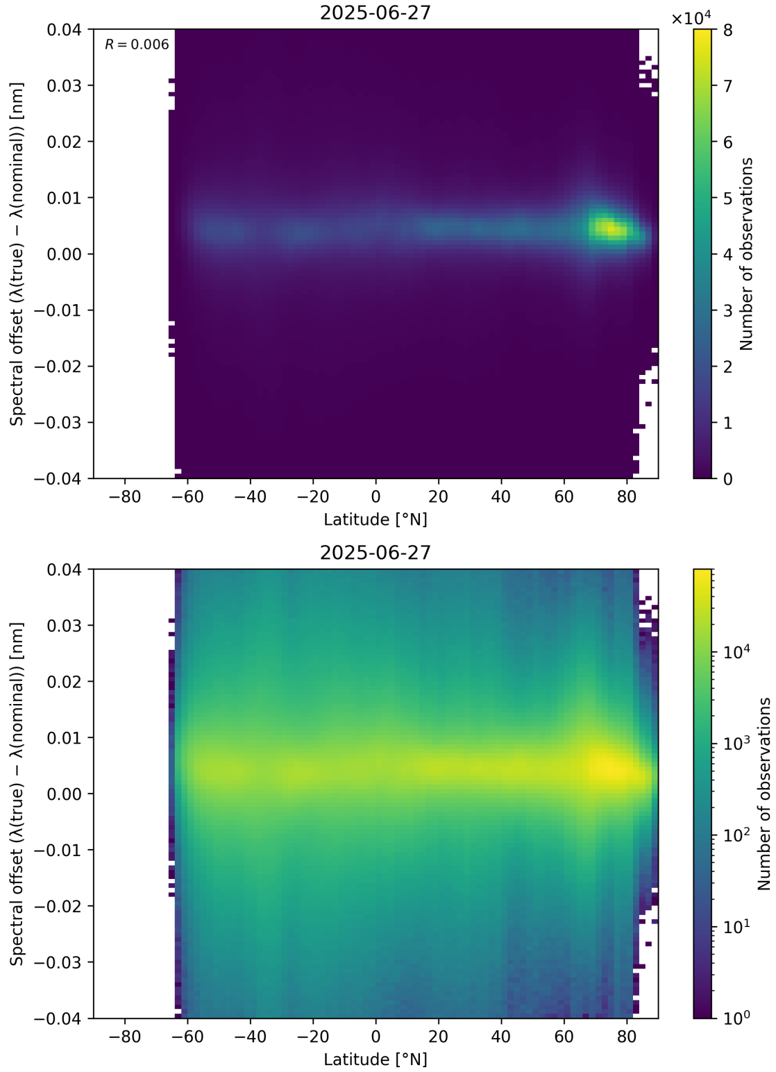
Figure 96: Scatter density plot of “Latitude” against “Spectral offset ( \lambda_{\text{true}} - \lambda_{\text{nominal}} )” for 2025-06-27 to 2025-06-28.
