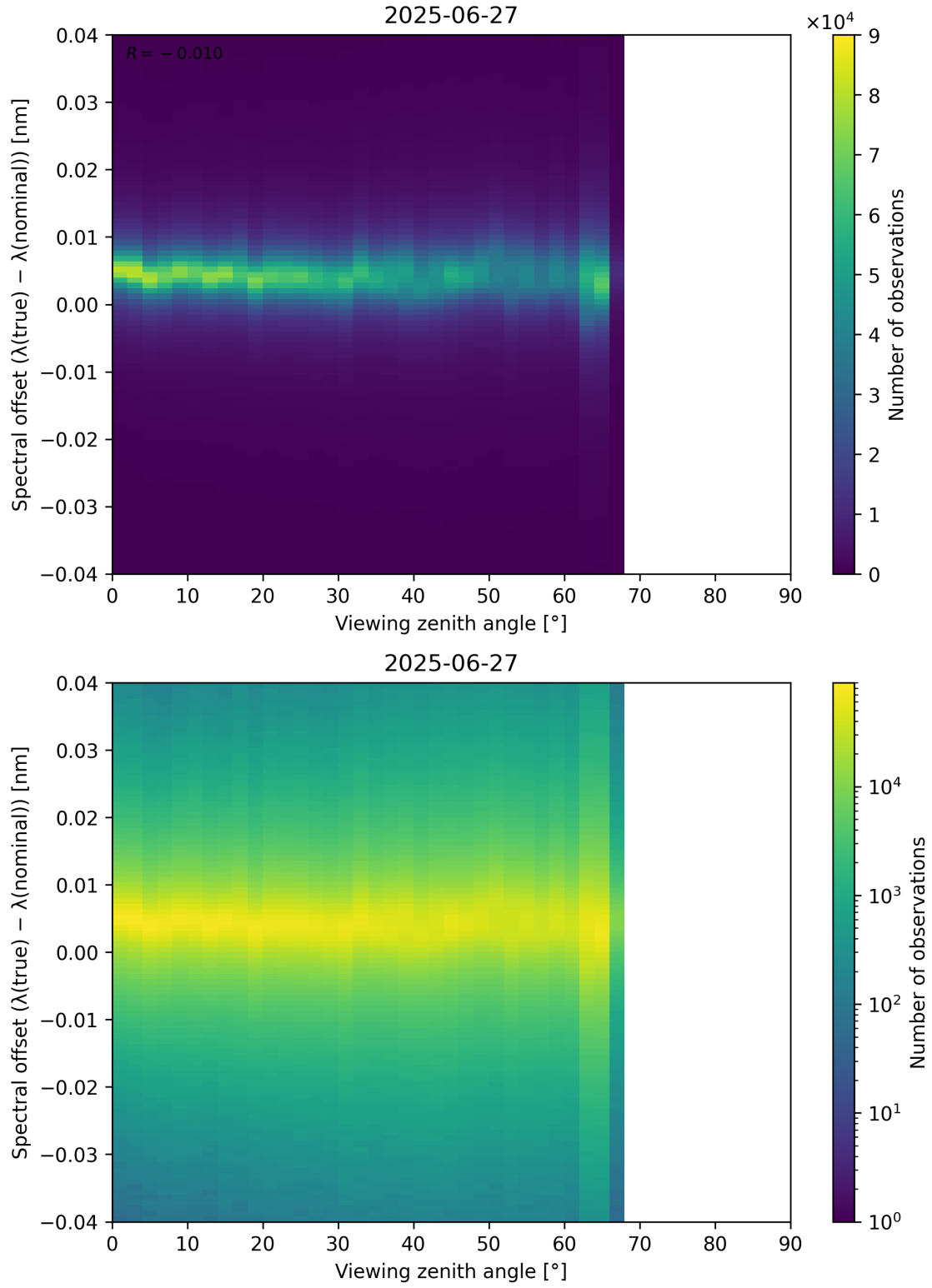
Figure 128: Scatter density plot of “Viewing zenith angle” against “Spectral offset ( \lambda_{\text{true}} - \lambda_{\text{nominal}} )” for 2025-06-27 to 2025-06-28.
