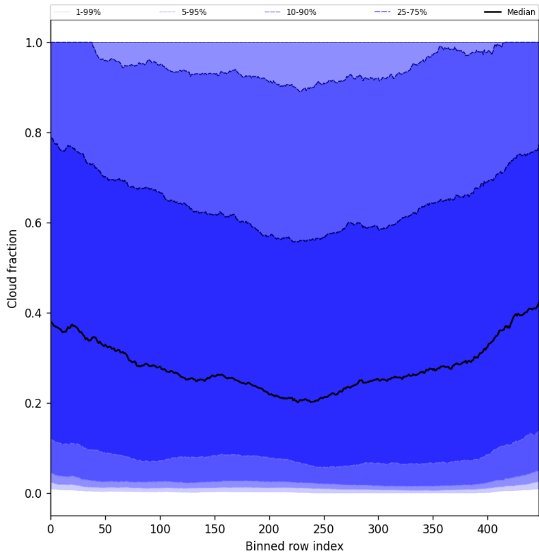
Figure 49: Along track statistics of “Cloud fraction” for 2025-06-27 to 2025-06-28
