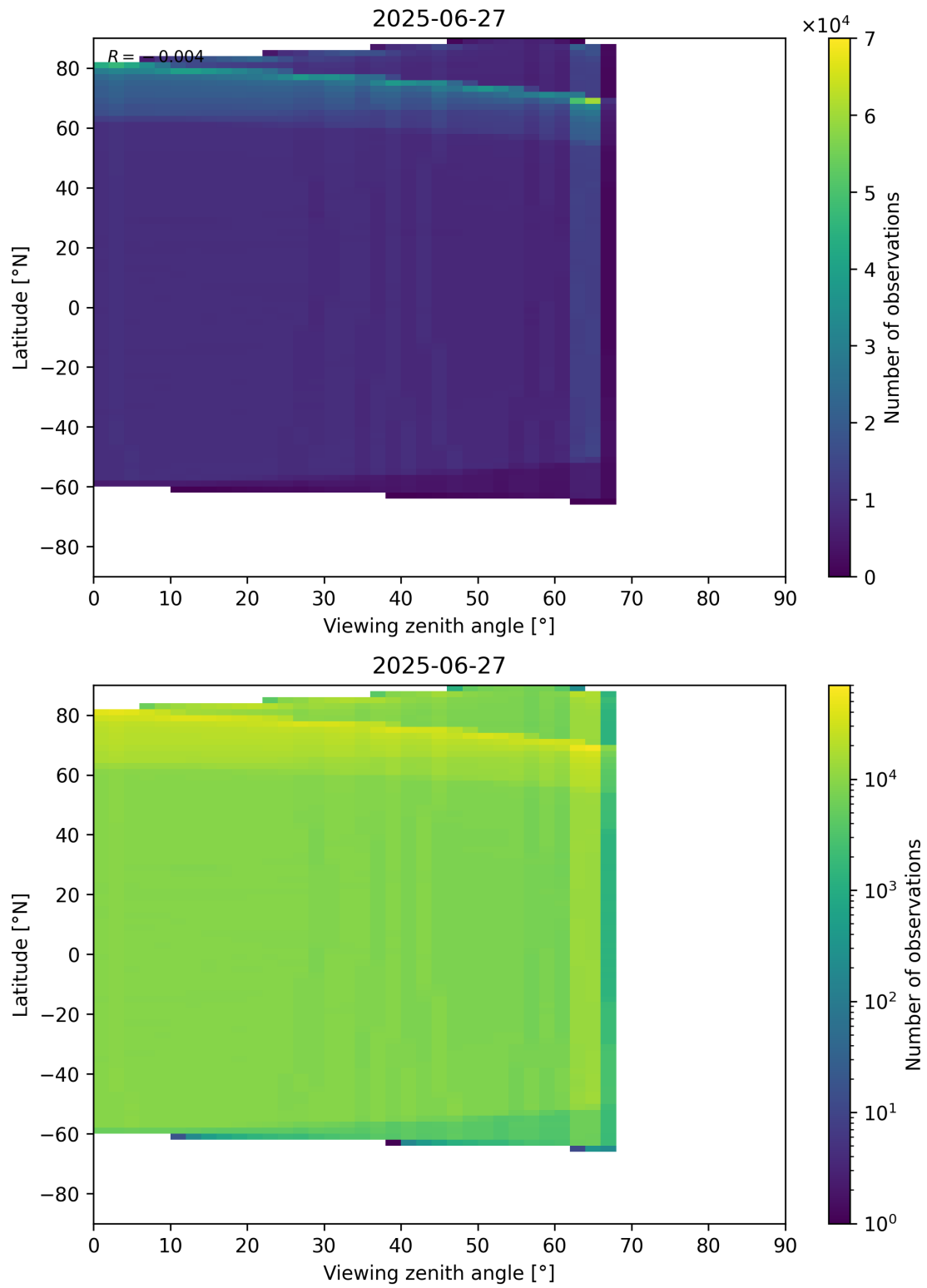
Figure 123: Scatter density plot of “Viewing zenith angle” against “Latitude” for 2025-06-27 to 2025-06-28.
