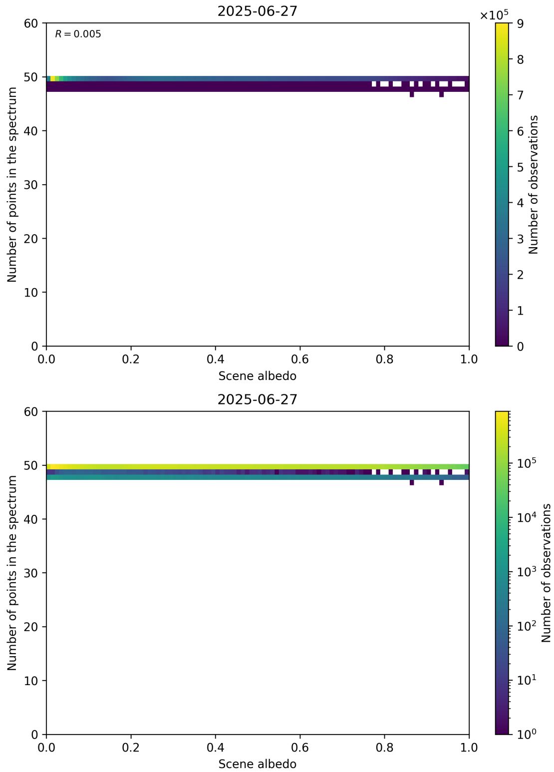
Figure 106: Scatter density plot of “Scene albedo” against “Number of points in the spectrum” for 2025-06-27 to 2025-06-28.
