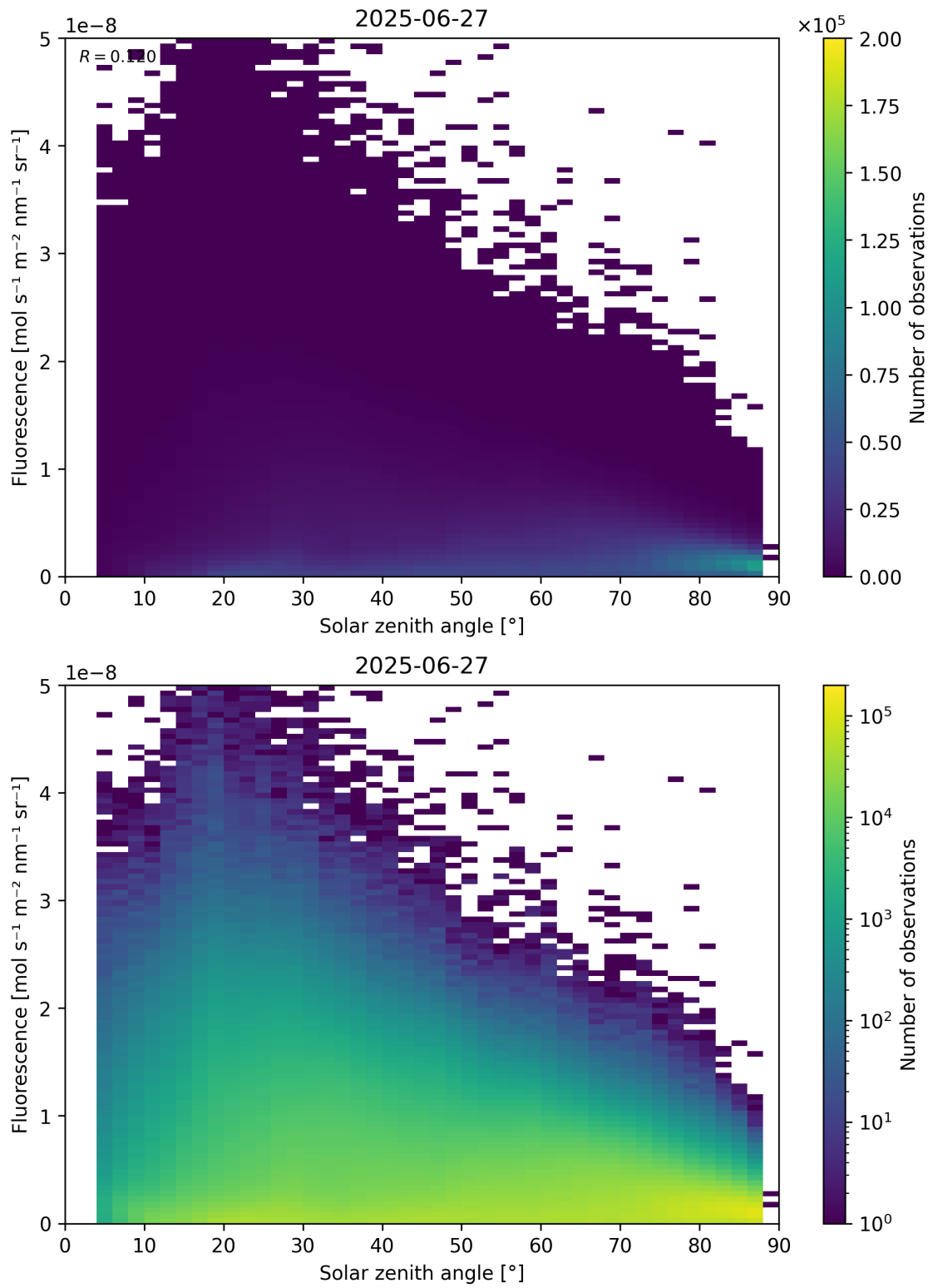
Figure 112: Scatter density plot of “Solar zenith angle” against “Fluorescence” for 2025-06-27 to 2025-06-28.
