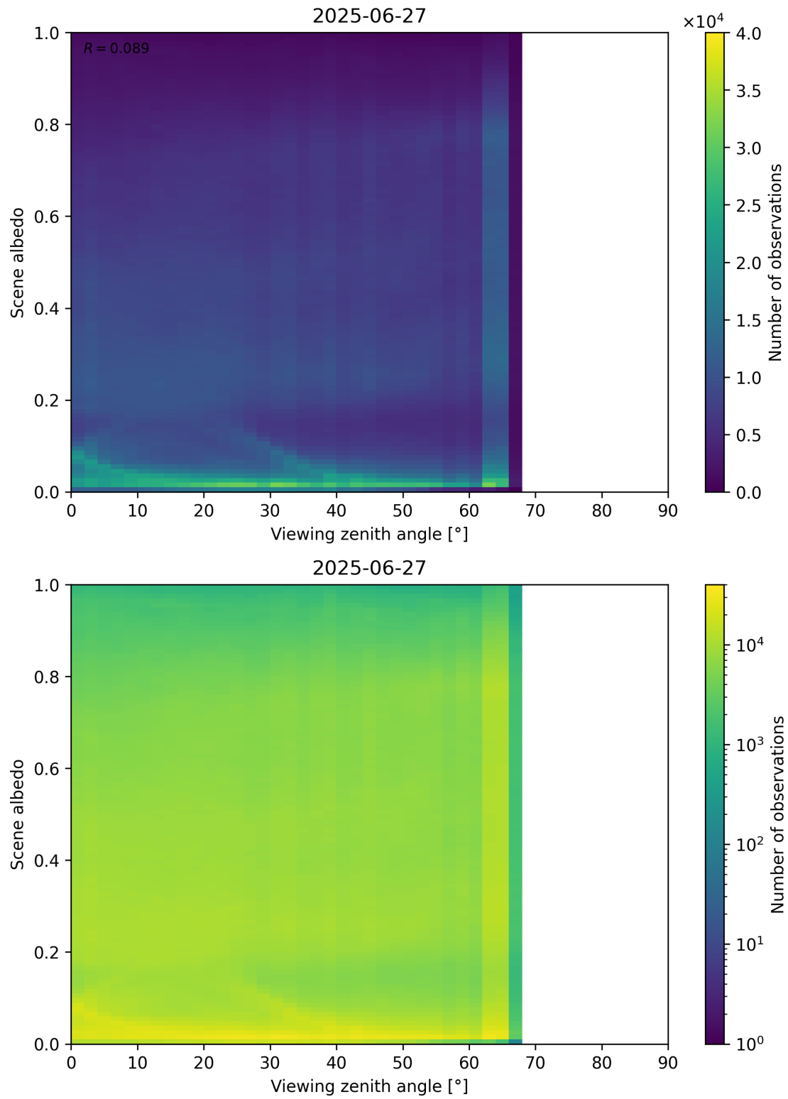
Figure 126: Scatter density plot of “Viewing zenith angle” against “Scene albedo” for 2025-06-27 to 2025-06-28.
