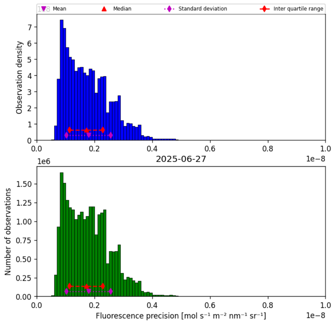
Figure 41: Histogram of “Fluorescence precision” for 2025-06-27 to 2025-06-28
