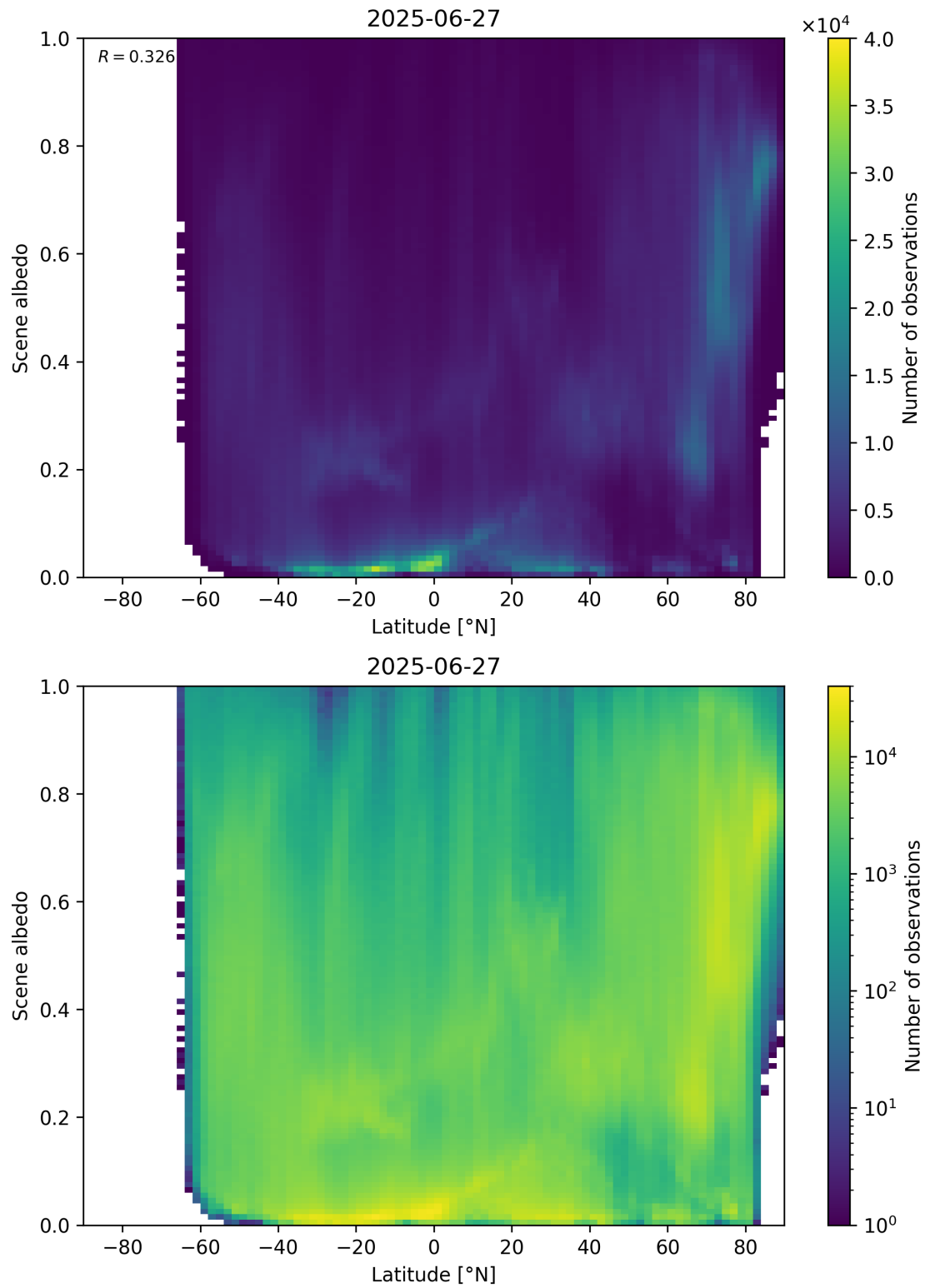
Figure 95: Scatter density plot of “Latitude” against “Scene albedo” for 2025-06-27 to 2025-06-28.
