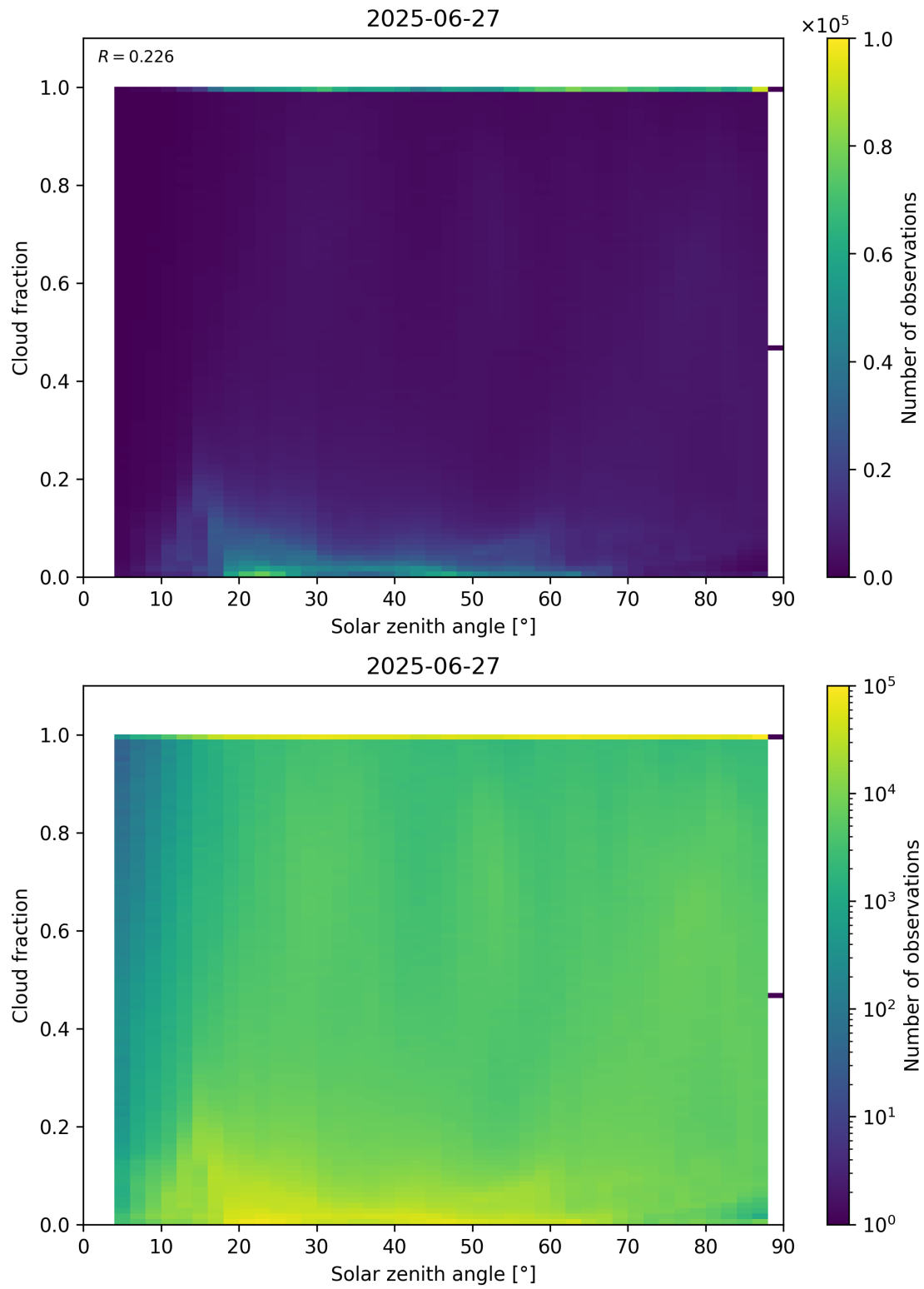
Figure 110: Scatter density plot of “Solar zenith angle” against “Cloud fraction” for 2025-06-27 to 2025-06-28.
