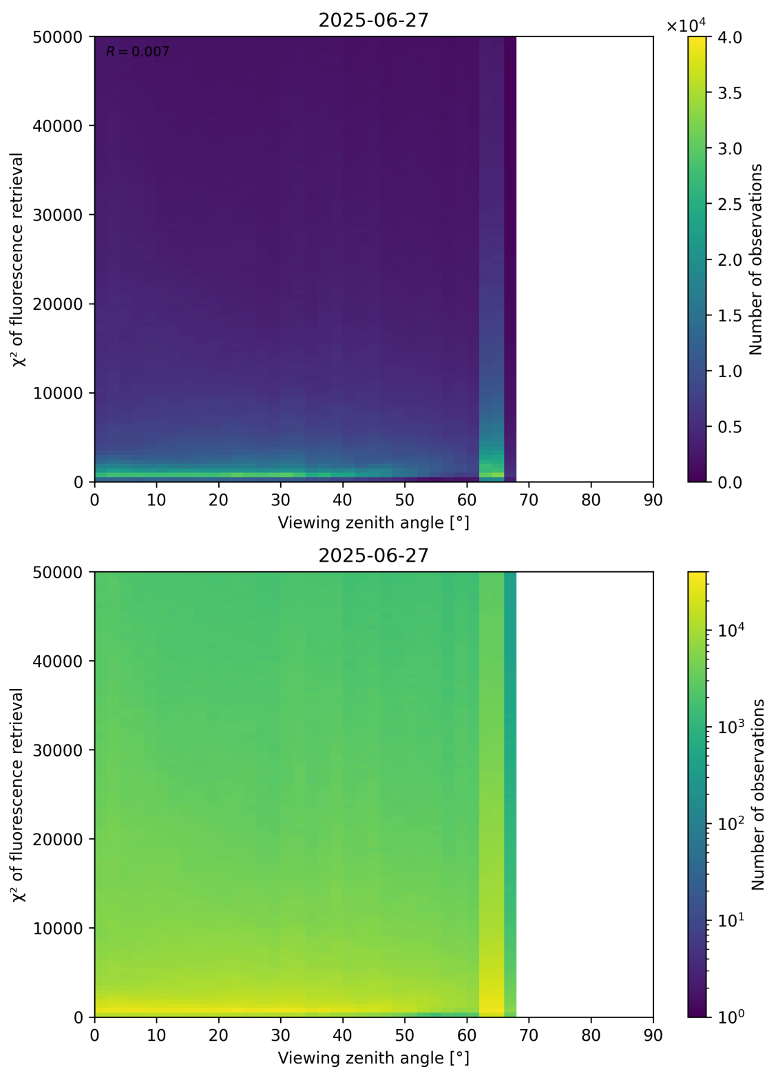
Figure 119: Scatter density plot of “Viewing zenith angle” against “ \chi^2 of fluorescence retrieval” for 2025-06-27 to 2025-06-28.
