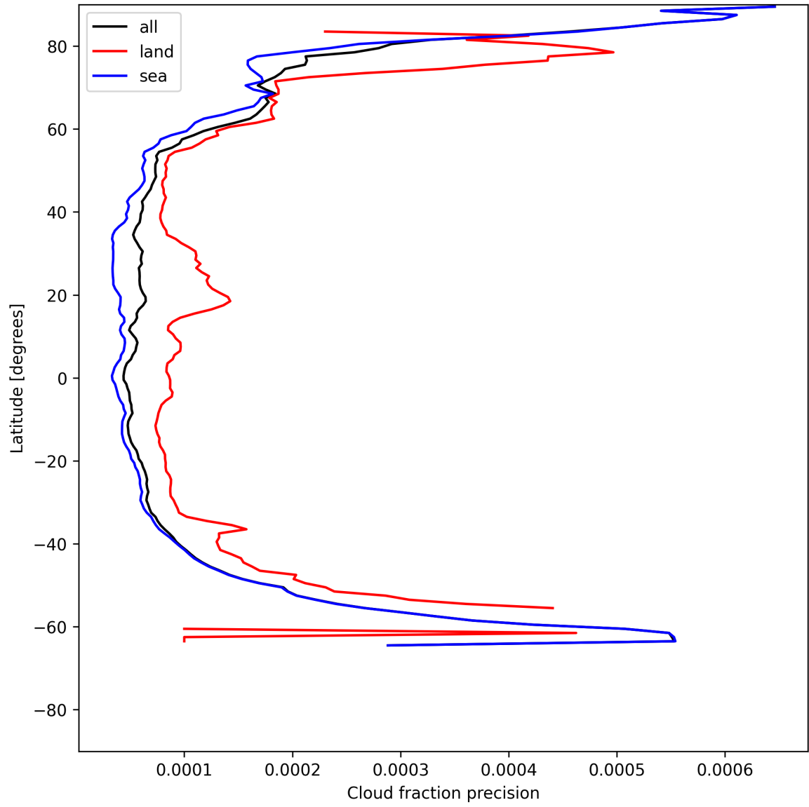
Figure 16: Zonal average of “Cloud fraction precision” for 2025-06-27 to 2025-06-28.
