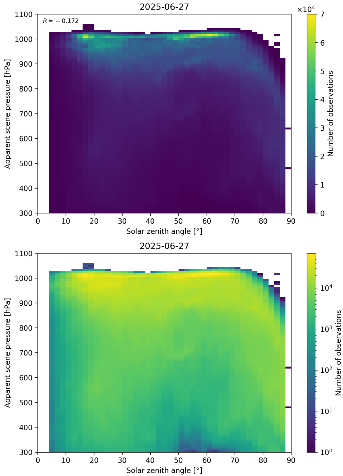
Figure 108: Scatter density plot of “Solar zenith angle” against “Apparent scene pressure” for 2025-06-27 to 2025-06-28.
