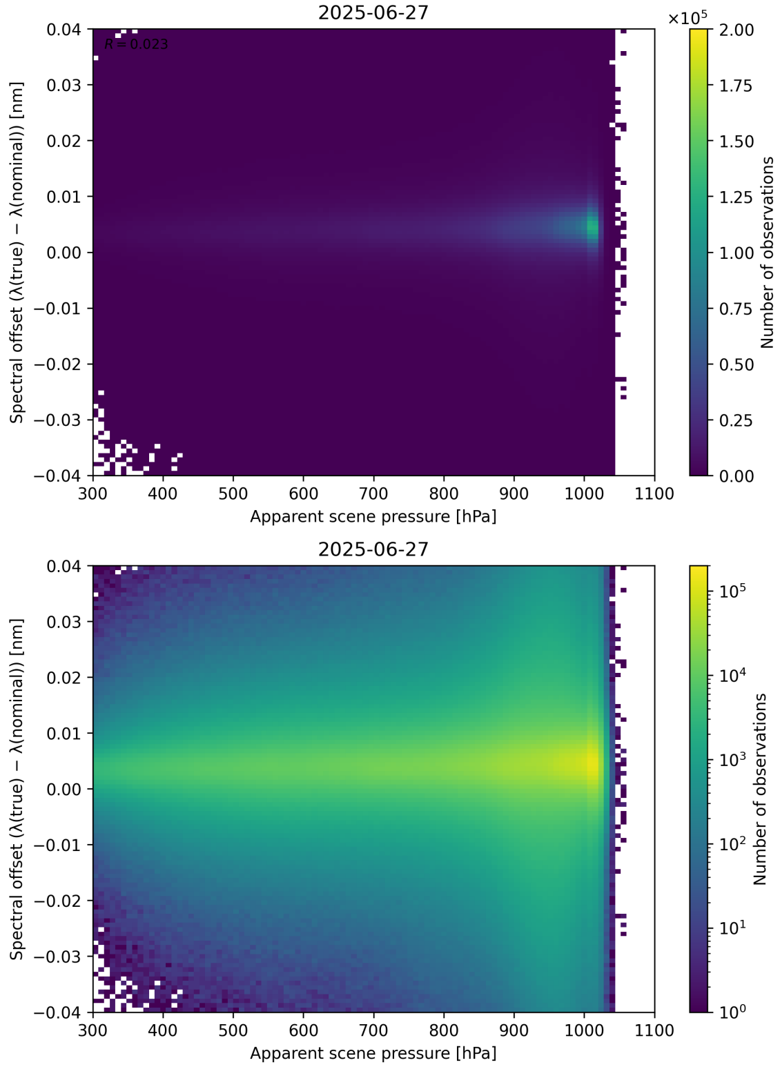
Figure 67: Scatter density plot of “Apparent scene pressure” against “Spectral offset ( \lambda_{\text{true}} - \lambda_{\text{nominal}} )” for 2025-06-27 to 2025-06-28.
