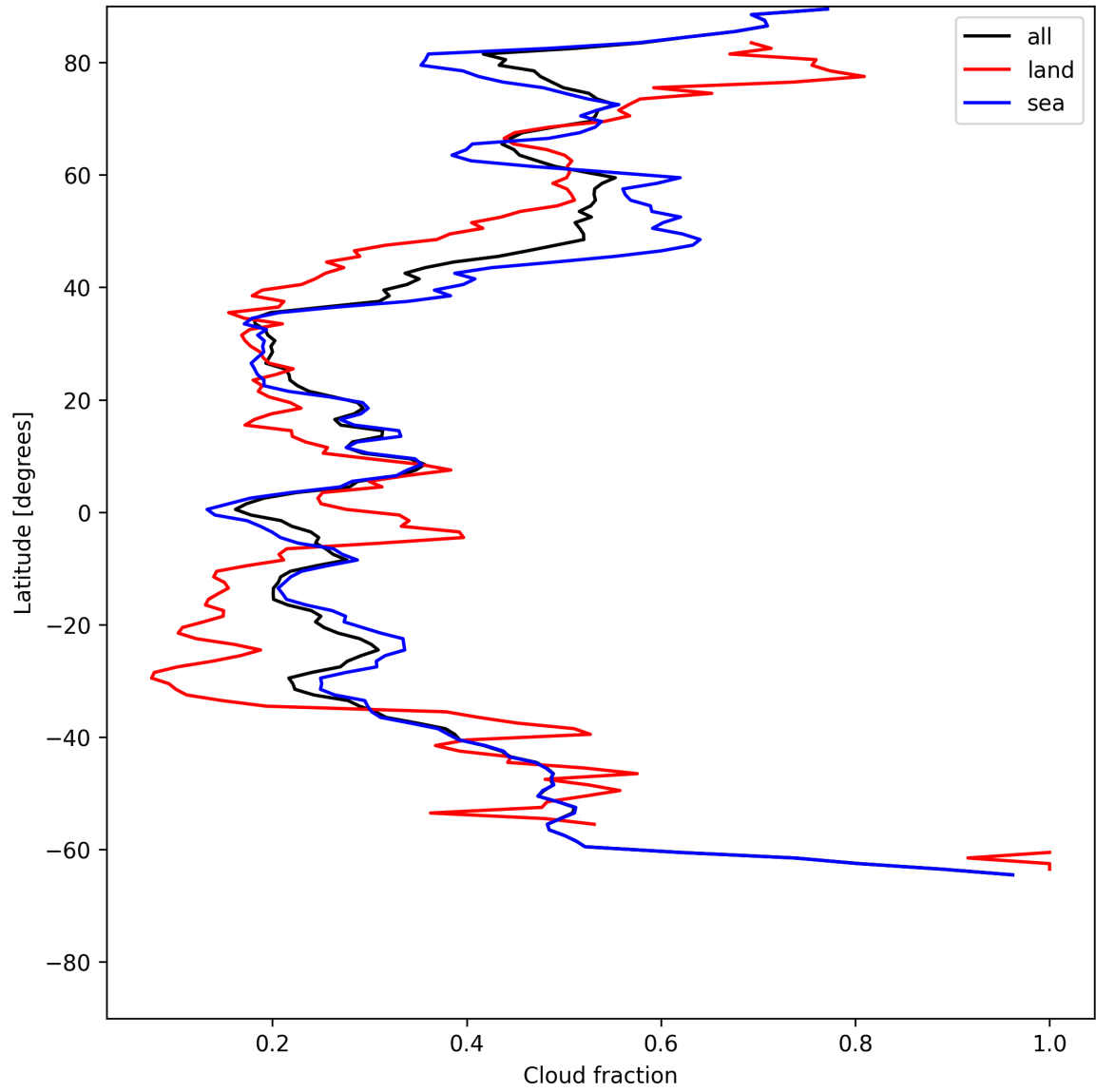
Figure 15: Zonal average of “Cloud fraction” for 2025-06-27 to 2025-06-28.
