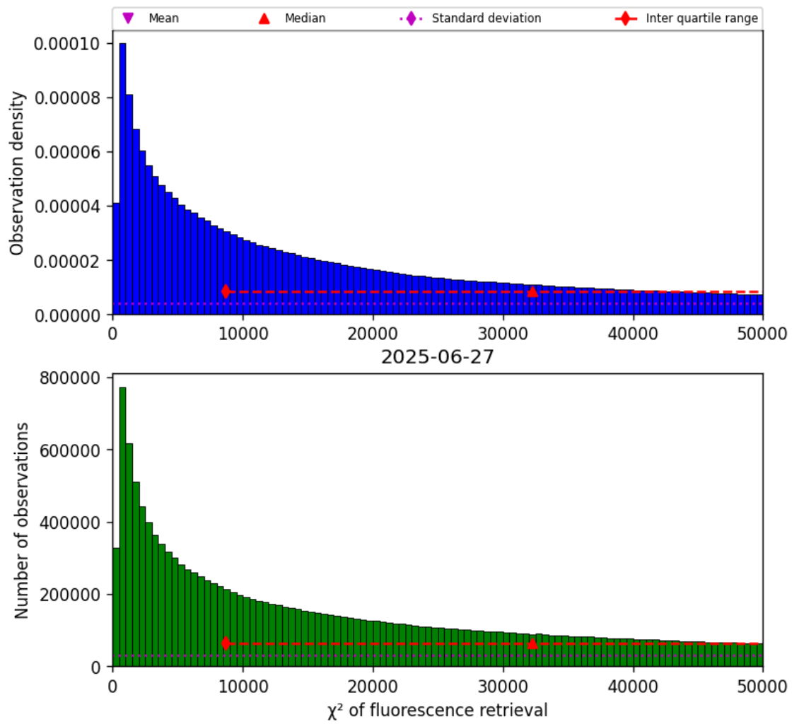
Figure 42: Histogram of “ \chi^2 of fluorescence retrieval” for 2025-06-27 to 2025-06-28
