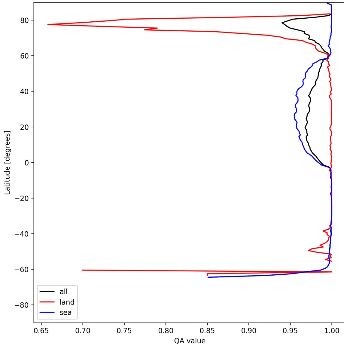
Figure 12: Zonal average of “QA value” for 2025-06-27 to 2025-06-28.
