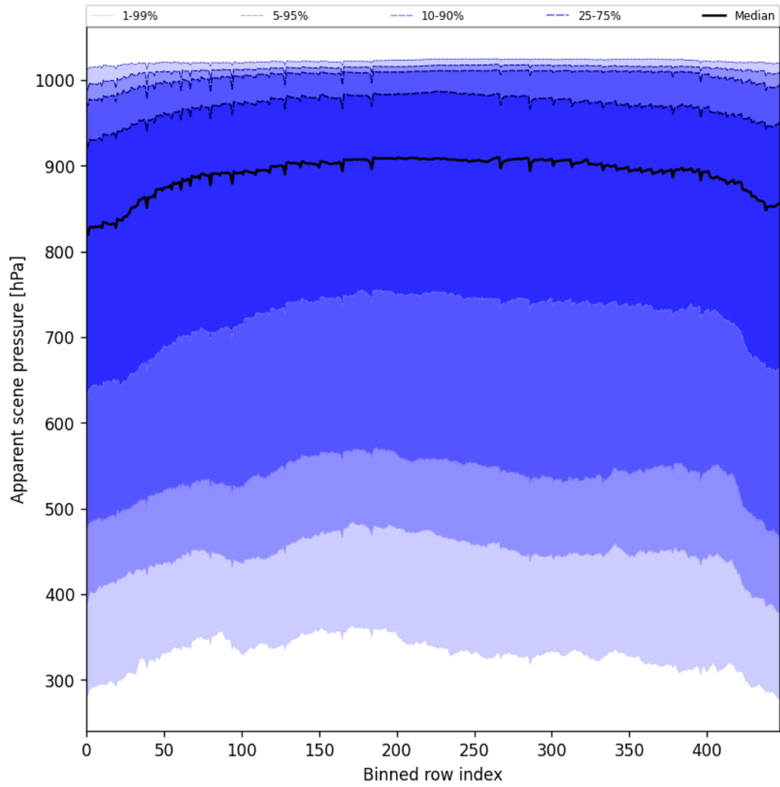
Figure 53: Along track statistics of “Apparent scene pressure” for 2025-06-27 to 2025-06-28
