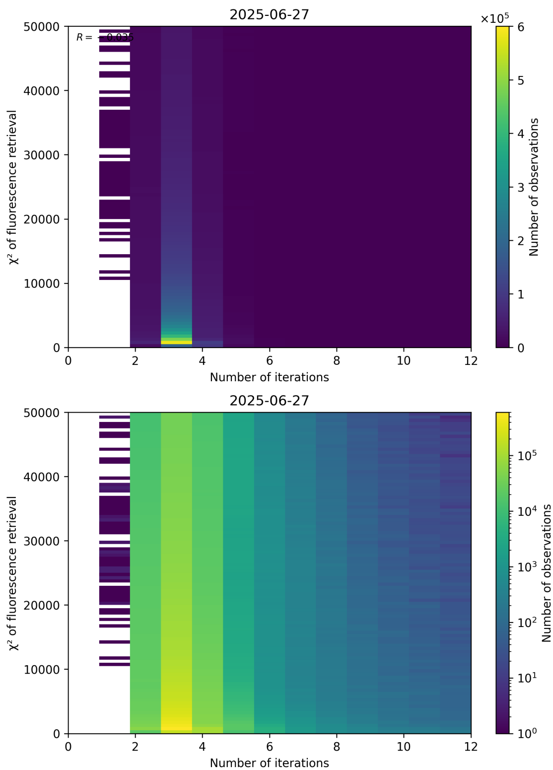
Figure 97: Scatter density plot of “Number of iterations” against “ \chi^2 of fluorescence retrieval” for 2025-06-27 to 2025-06-28.
