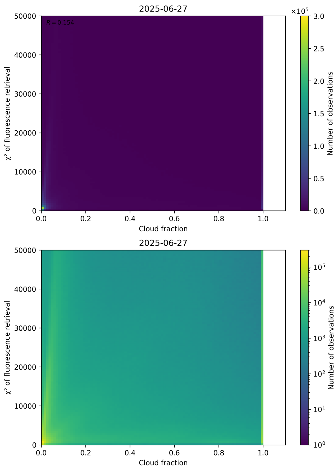
Figure 71: Scatter density plot of “Cloud fraction” against “ \chi^2 of fluorescence retrieval” for 2025-06-27 to 2025-06-28.
