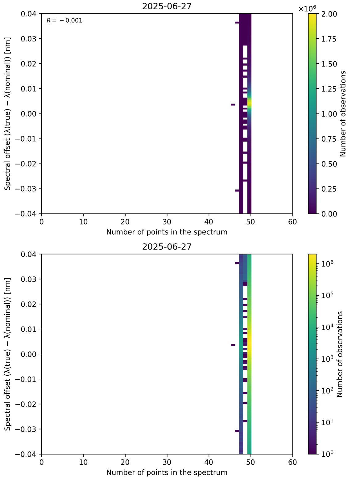
Figure 101: Scatter density plot of “Number of points in the spectrum” against “Spectral offset ( \lambda_{\text{true}} - \lambda_{\text{nominal}} )” for 2025-06-27 to 2025-06-28.
