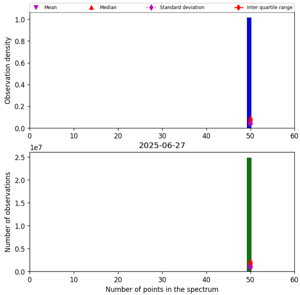
Figure 44: Histogram of “Number of points in the spectrum” for 2025-06-27 to 2025-06-28
