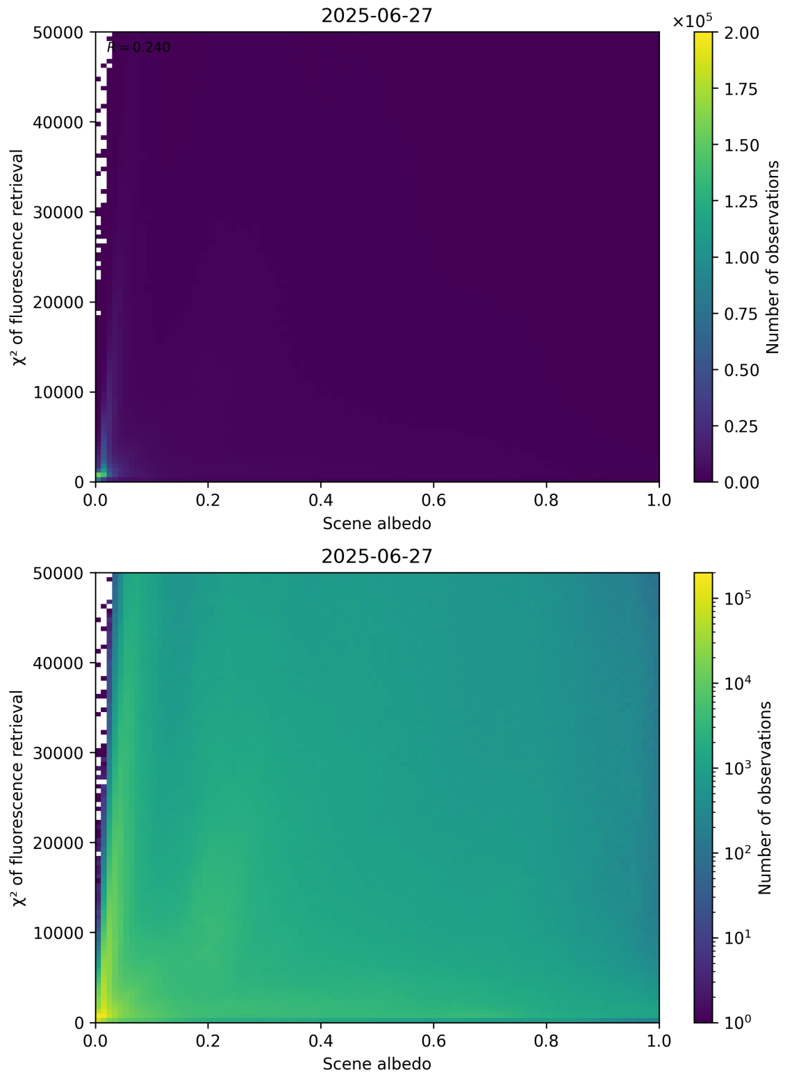
Figure 103: Scatter density plot of “Scene albedo” against “ \chi^2 of fluorescence retrieval” for 2025-06-27 to 2025-06-28.
