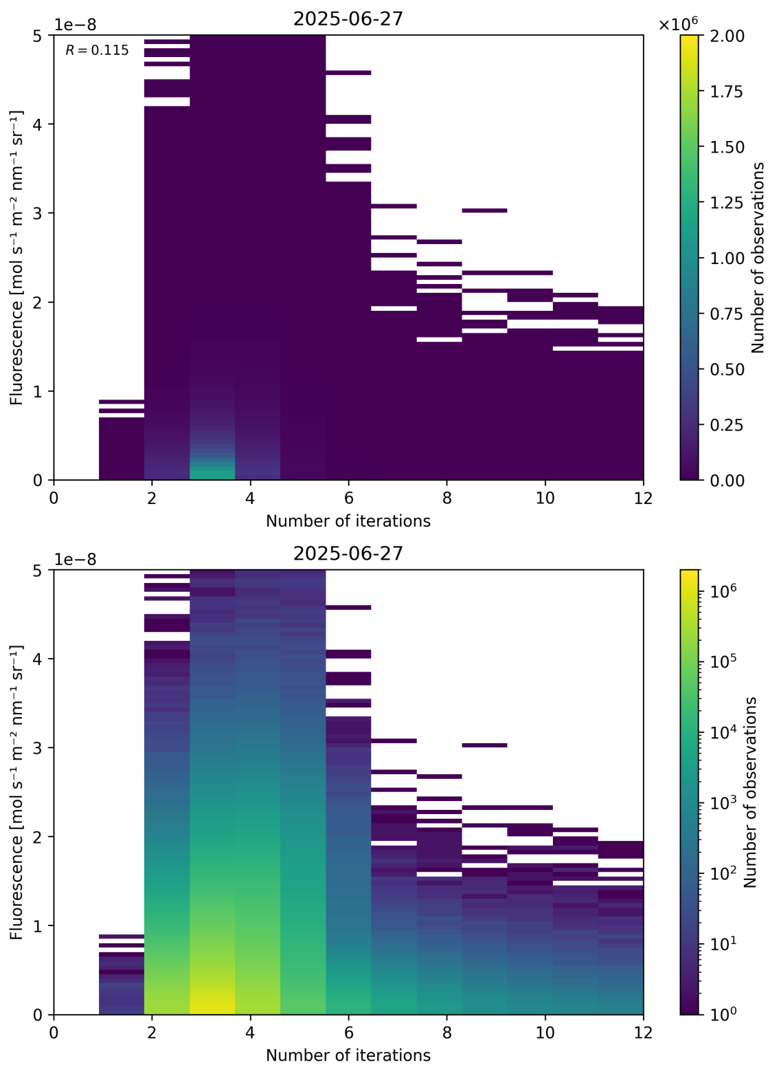
Figure 98: Scatter density plot of “Number of iterations” against “Fluorescence” for 2025-06-27 to 2025-06-28.
