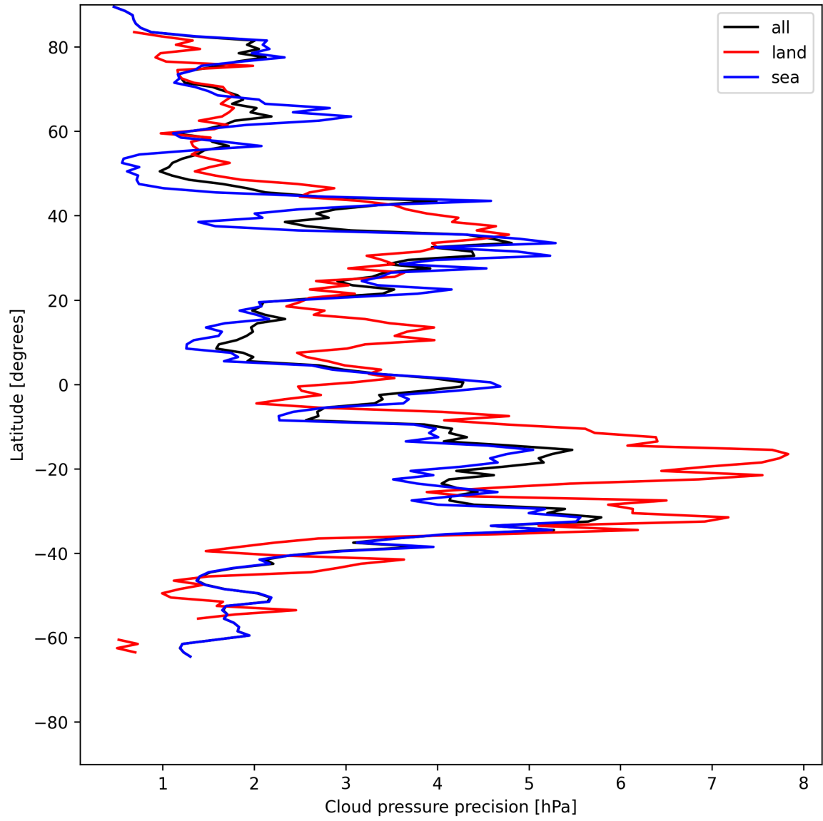
Figure 14: Zonal average of “Cloud pressure precision” for 2025-06-27 to 2025-06-28.
