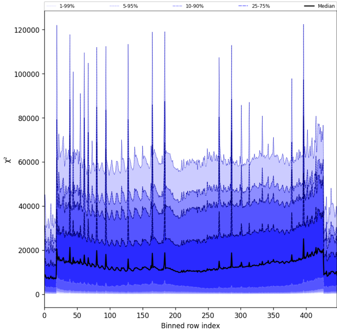
Figure 55: Along track statistics of “ \chi^2 ” for 2025-06-27 to 2025-06-28
