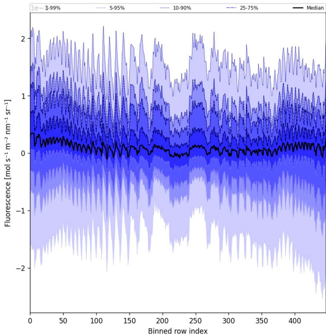
Figure 57: Along track statistics of “Fluorescence” for 2025-06-27 to 2025-06-28
