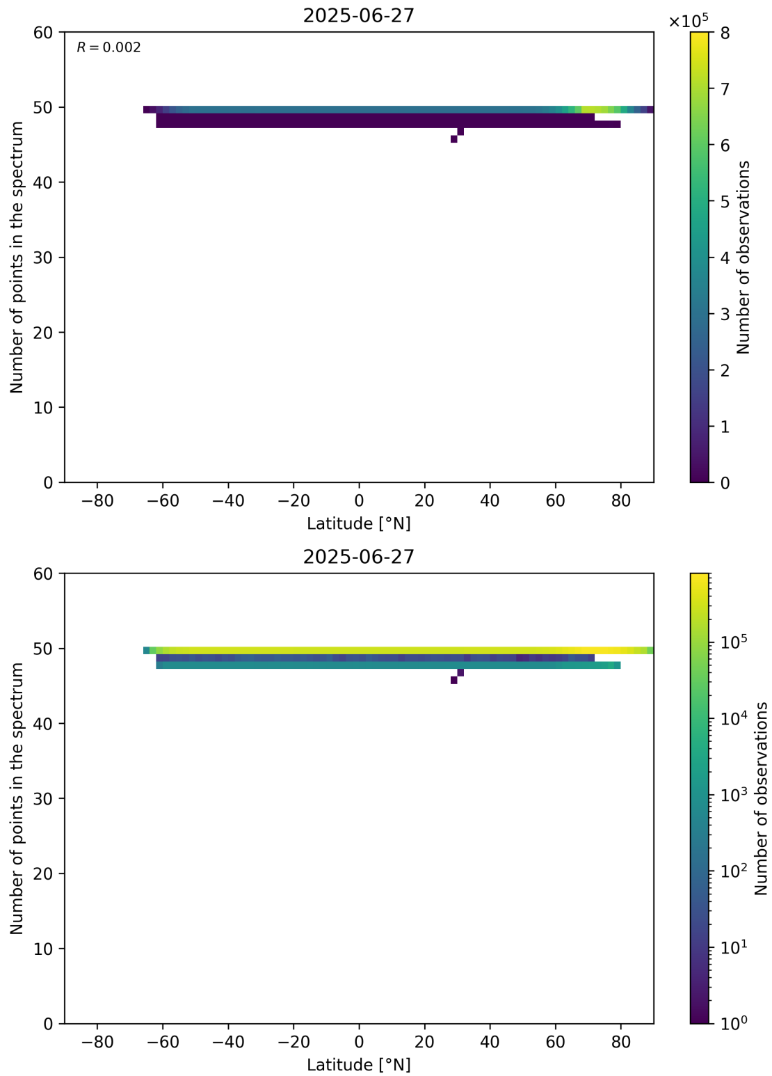
Figure 94: Scatter density plot of “Latitude” against “Number of points in the spectrum” for 2025-06-27 to 2025-06-28.
