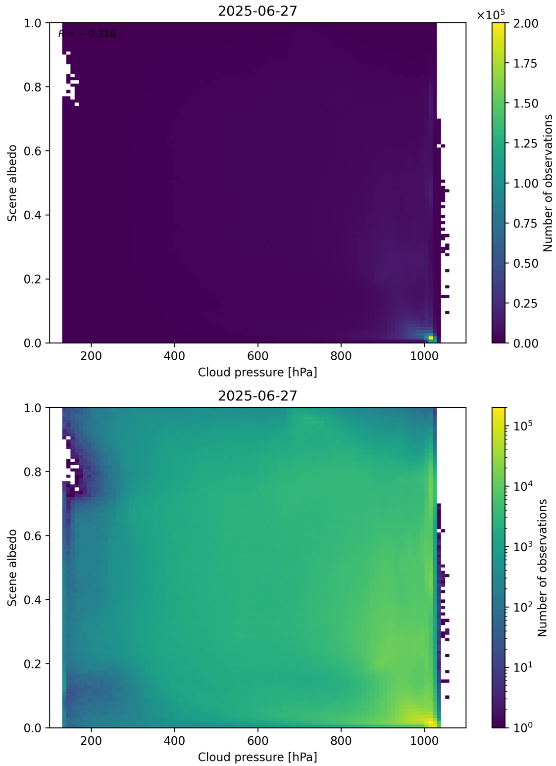
Figure 83: Scatter density plot of “Cloud pressure” against “Scene albedo” for 2025-06-27 to 2025-06-28.
