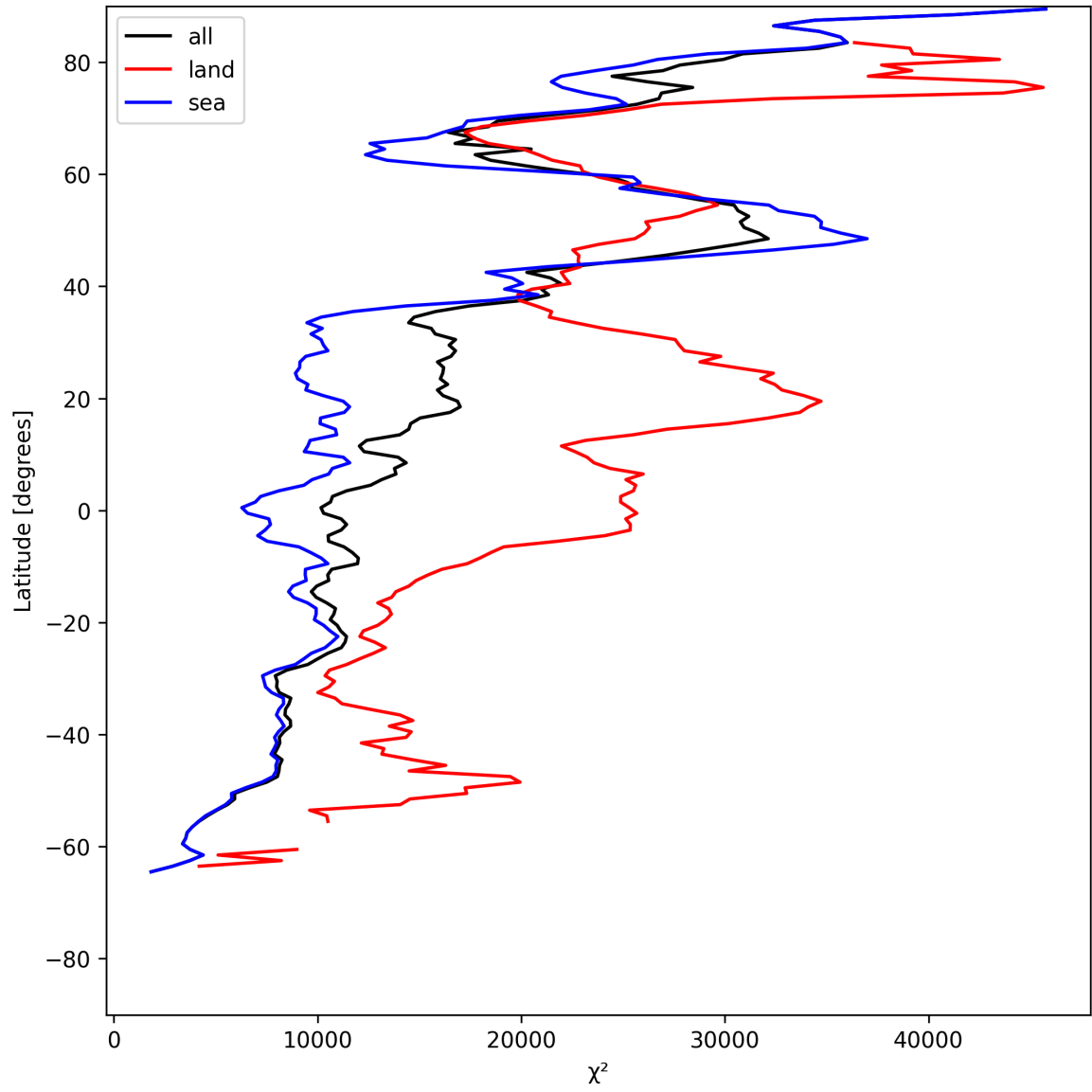
Figure 21: Zonal average of “ \chi^2 ” for 2025-06-27 to 2025-06-28.
