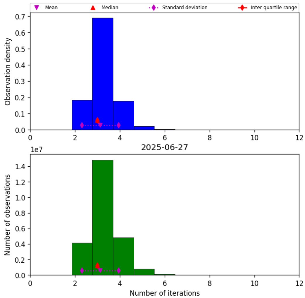
Figure 39: Histogram of “Number of iterations” for 2025-06-27 to 2025-06-28
