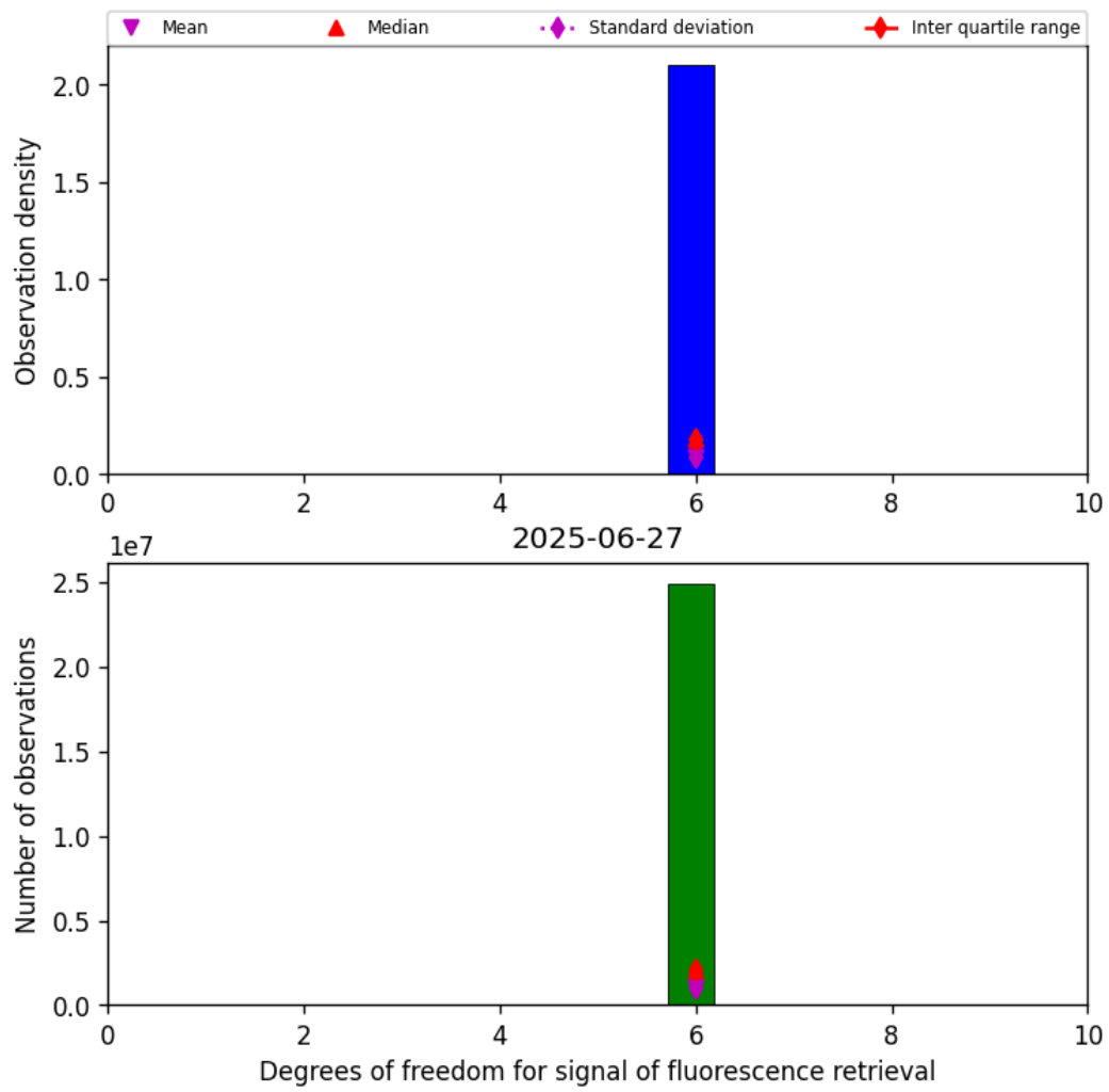
Figure 43: Histogram of “Degrees of freedom for signal of fluorescence retrieval” for 2025-06-27 to 2025-06-28
