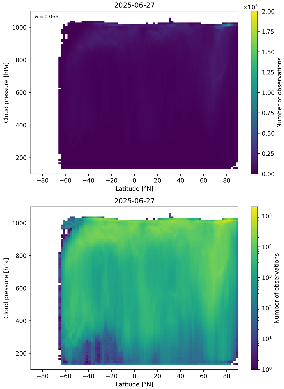
Figure 91: Scatter density plot of “Latitude” against “Cloud pressure” for 2025-06-27 to 2025-06-28.
