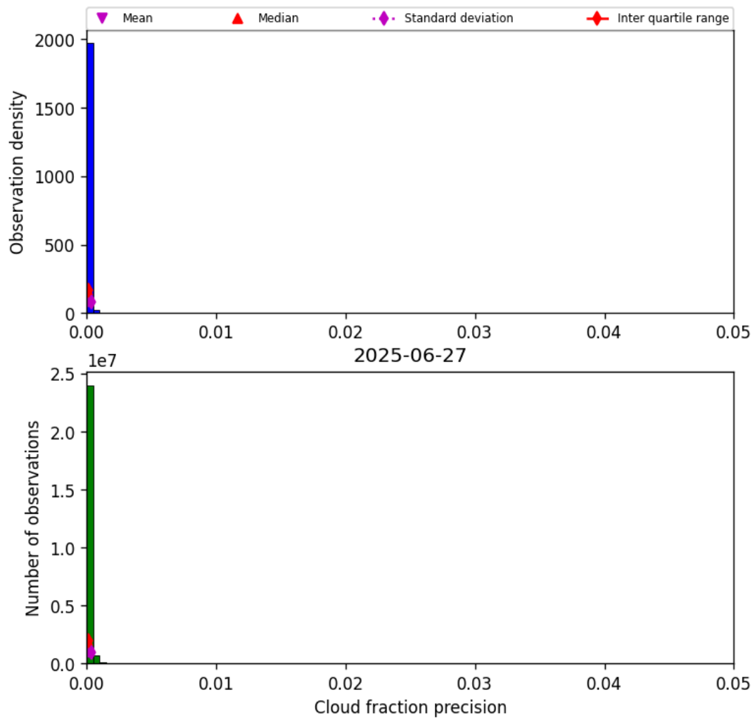
Figure 33: Histogram of “Cloud fraction precision” for 2025-06-27 to 2025-06-28
