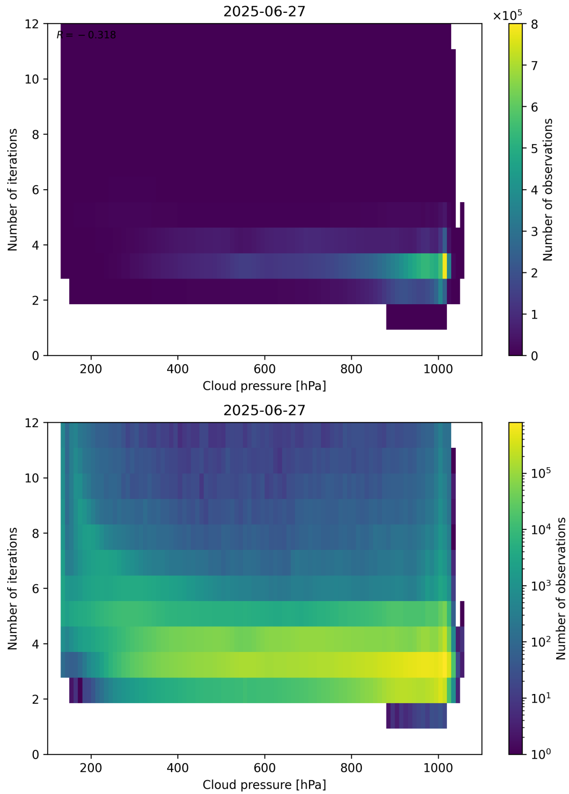
Figure 81: Scatter density plot of “Cloud pressure” against “Number of iterations” for 2025-06-27 to 2025-06-28.
