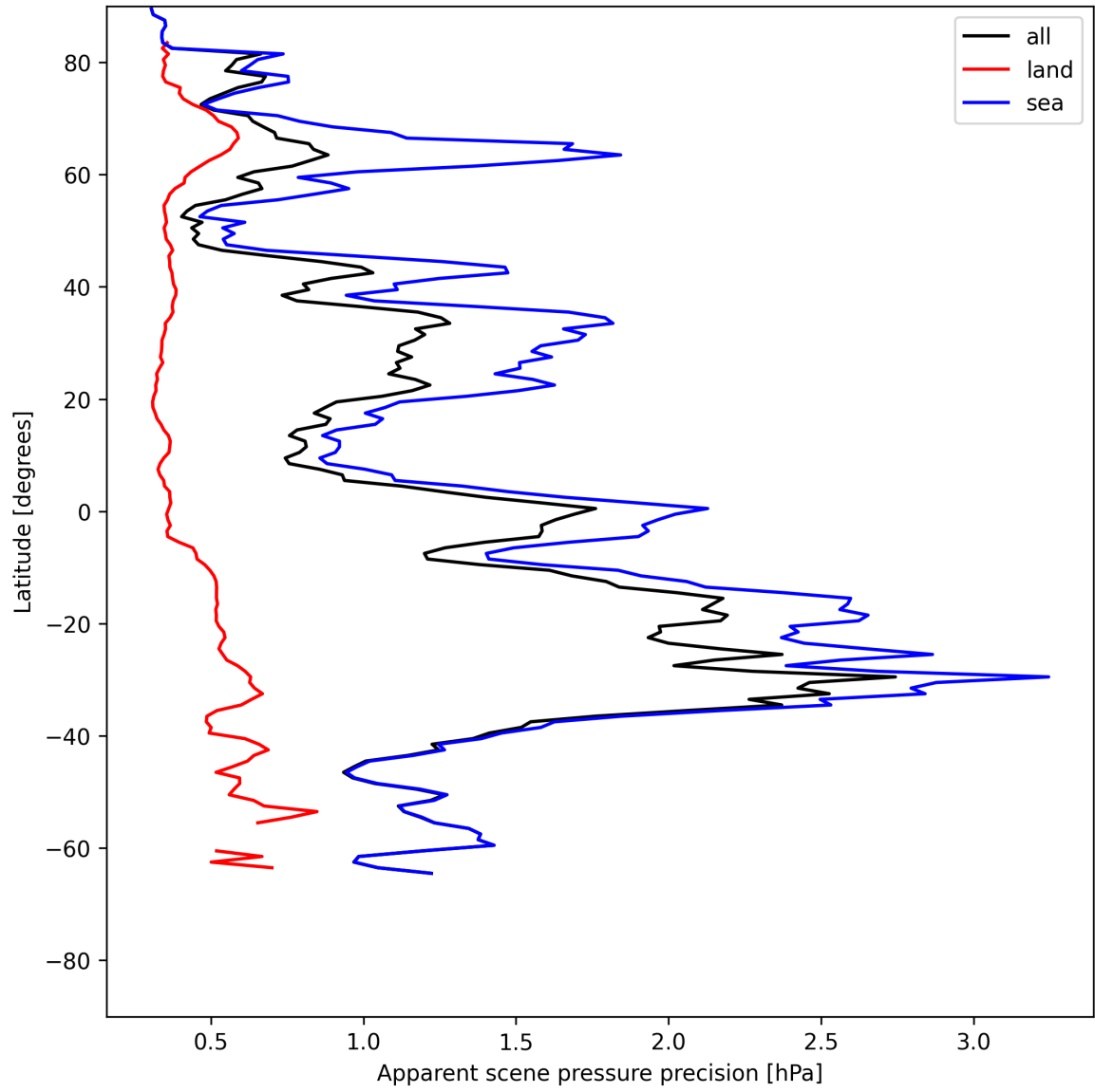
Figure 20: Zonal average of “Apparent scene pressure precision” for 2025-06-27 to 2025-06-28.
