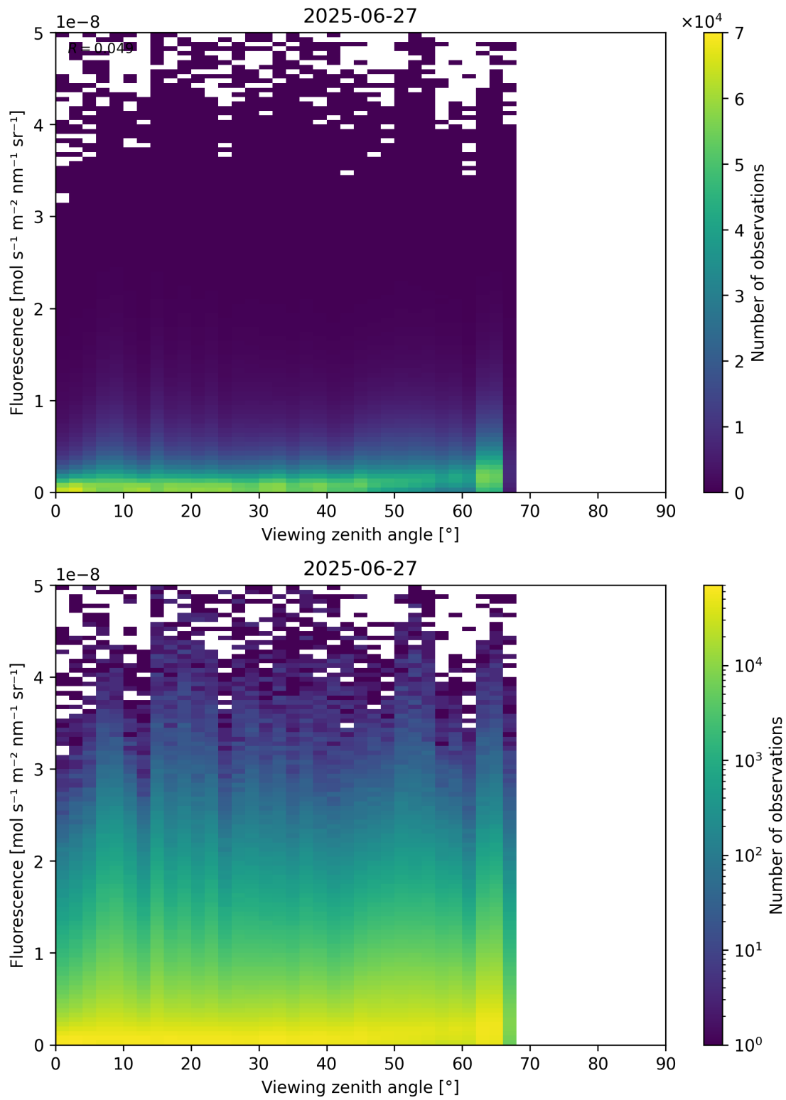
Figure 122: Scatter density plot of “Viewing zenith angle” against “Fluorescence” for 2025-06-27 to 2025-06-28.
