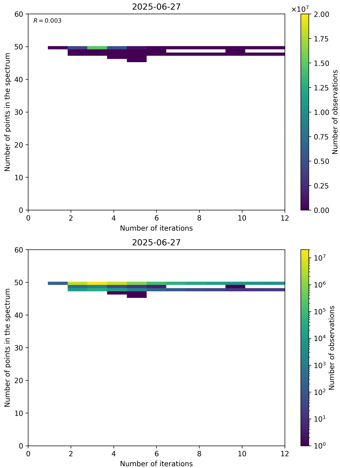
Figure 99: Scatter density plot of “Number of iterations” against “Number of points in the spectrum” for 2025-06-27 to 2025-06-28.
