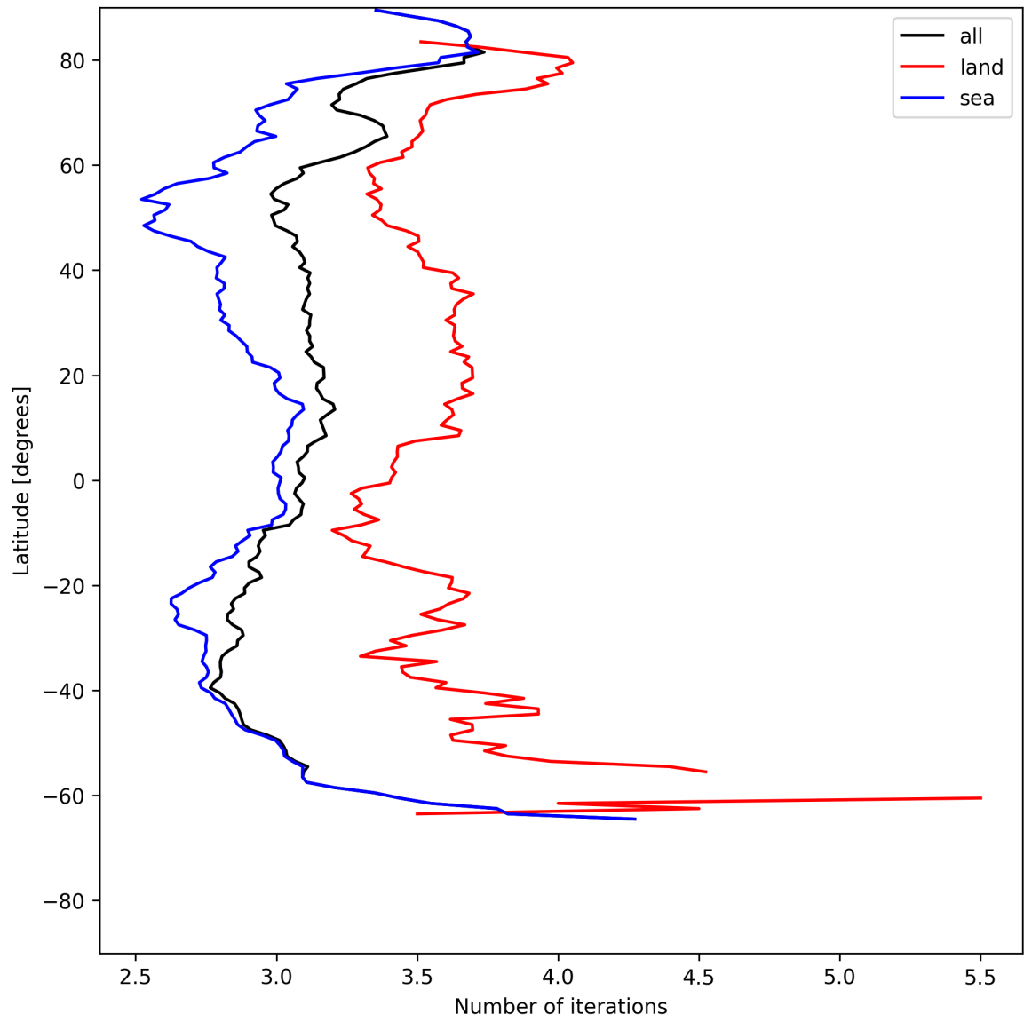
Figure 22: Zonal average of “Number of iterations” for 2025-06-27 to 2025-06-28.
