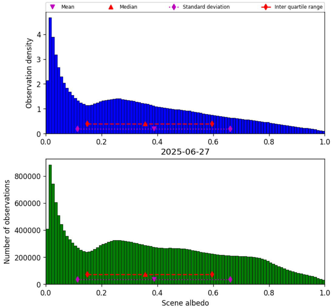
Figure 34: Histogram of “Scene albedo” for 2025-06-27 to 2025-06-28
