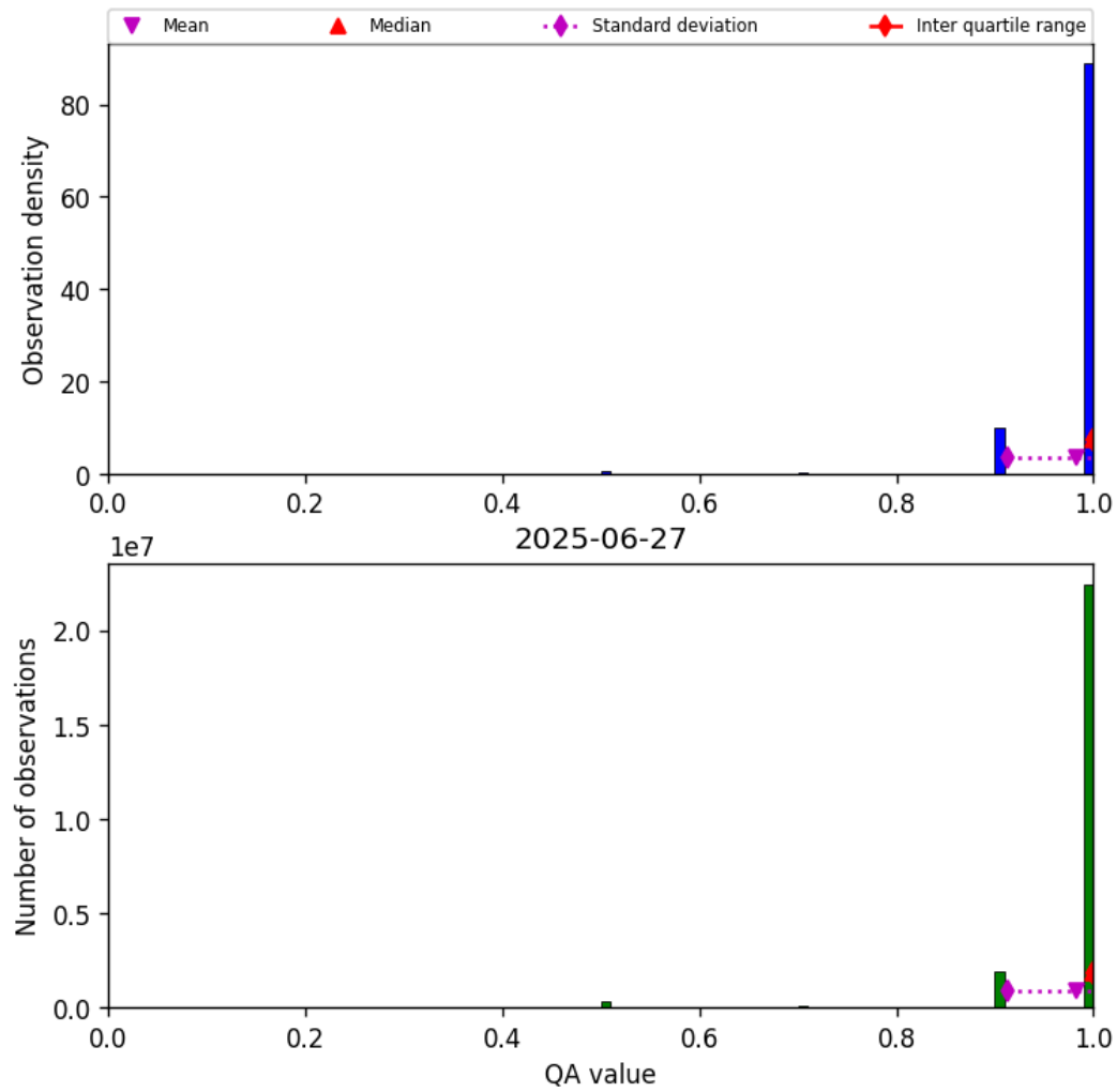
Figure 29: Histogram of “QA value” for 2025-06-27 to 2025-06-28
