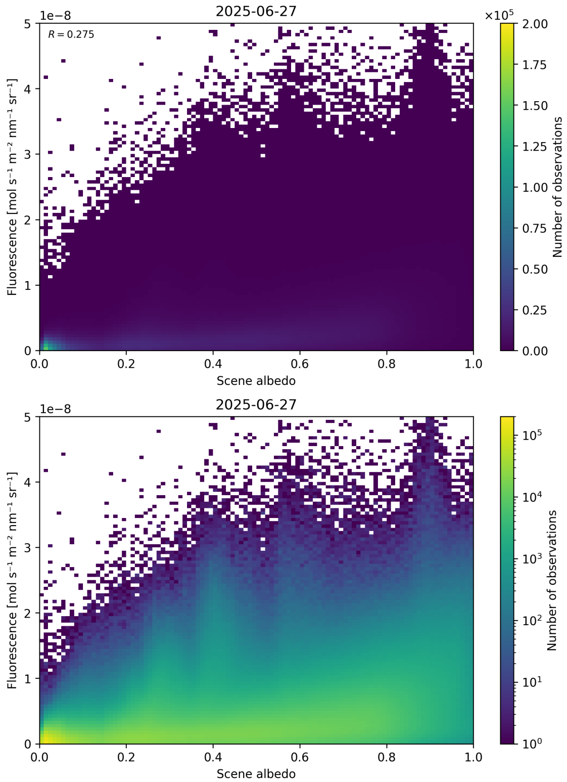
Figure 104: Scatter density plot of “Scene albedo” against “Fluorescence” for 2025-06-27 to 2025-06-28.
