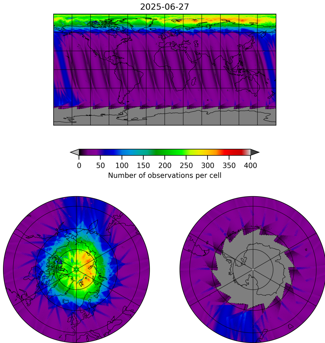
Figure 11: Map of the number of observations for 2025-06-27 to 2025-06-28
