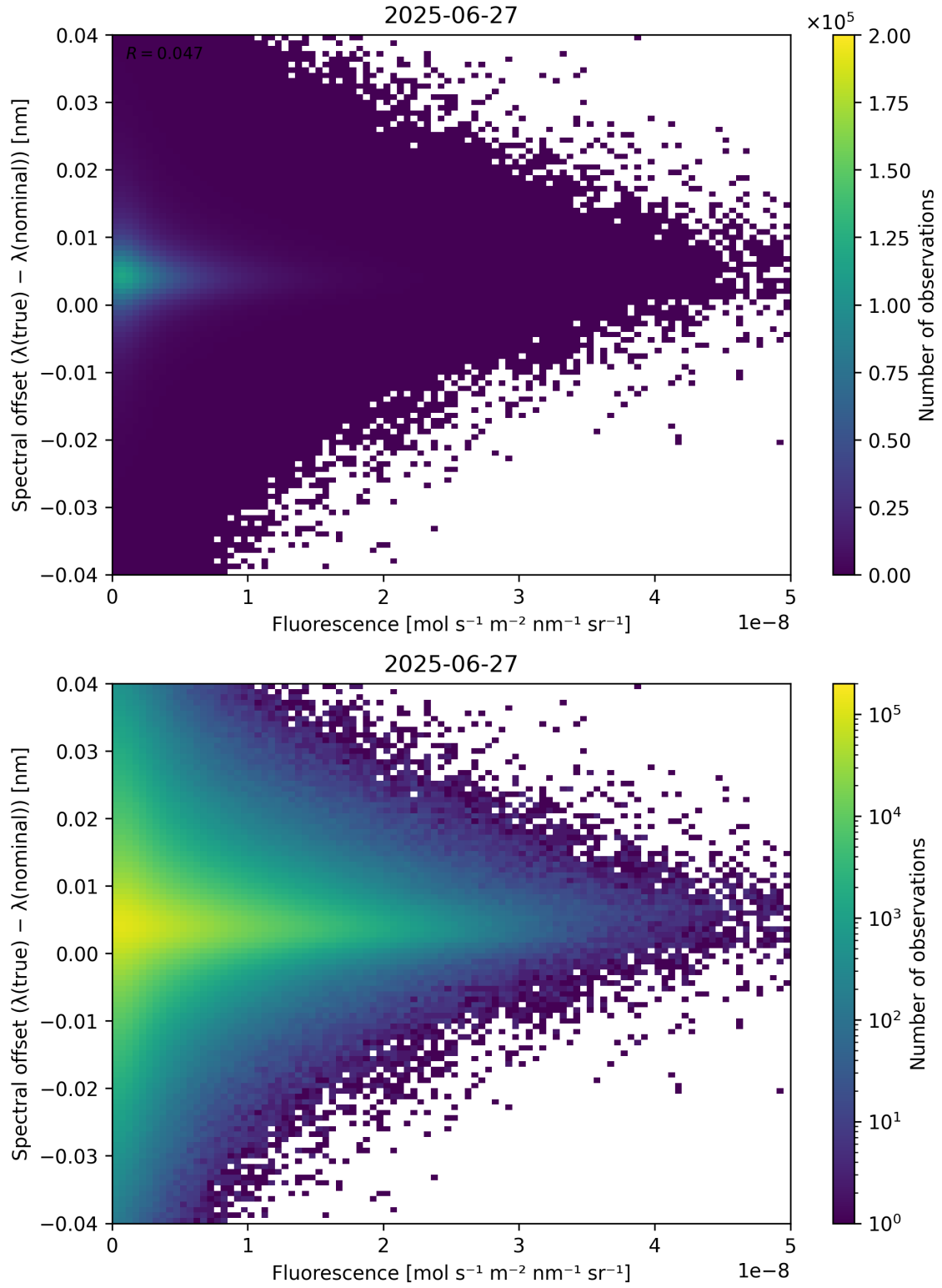
Figure 87: Scatter density plot of “Fluorescence” against “Spectral offset ( \lambda_{\text{true}} - \lambda_{\text{nominal}} )” for 2025-06-27 to 2025-06-28.
