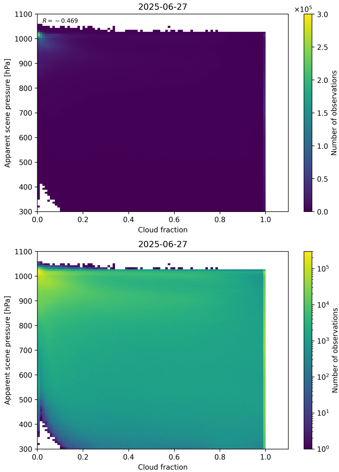
Figure 70: Scatter density plot of “Cloud fraction” against “Apparent scene pressure” for 2025-06-27 to 2025-06-28.
