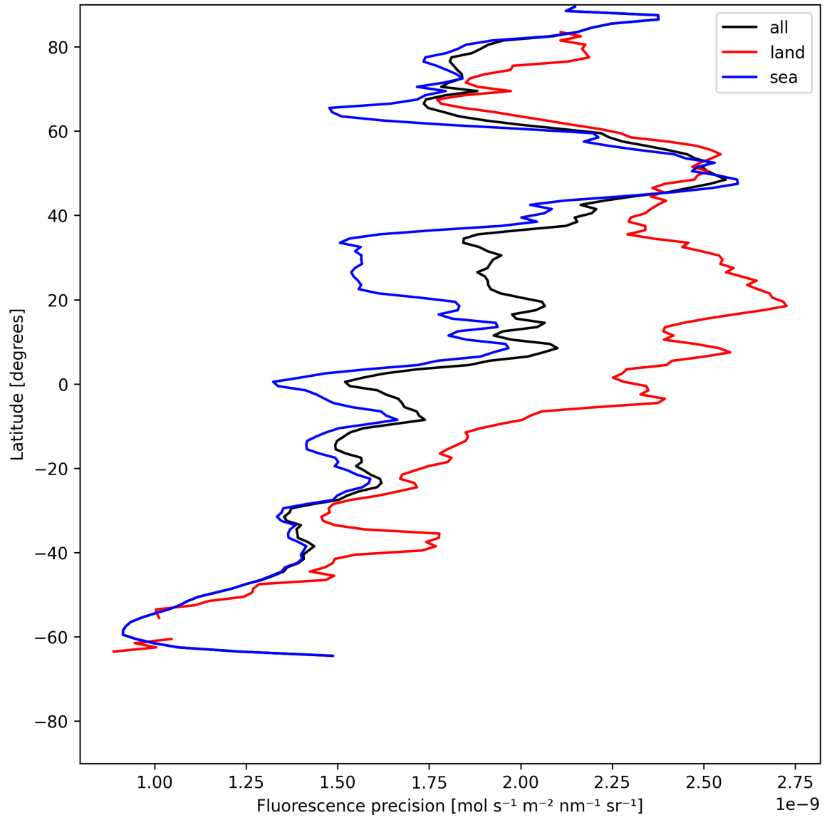
Figure 24: Zonal average of “Fluorescence precision” for 2025-06-27 to 2025-06-28.
