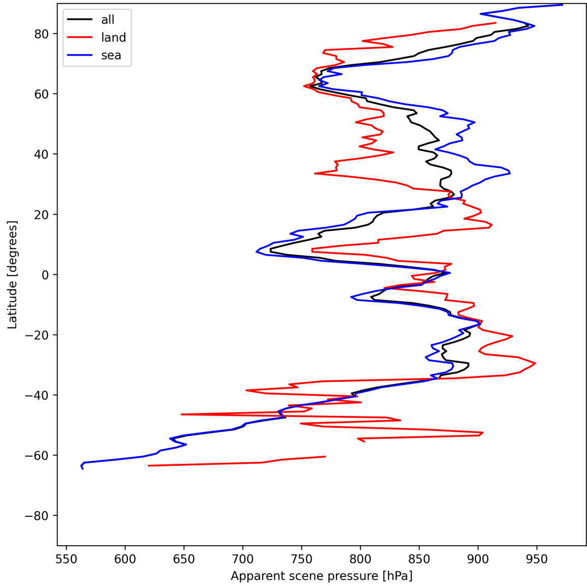
Figure 19: Zonal average of “Apparent scene pressure” for 2025-06-27 to 2025-06-28.
