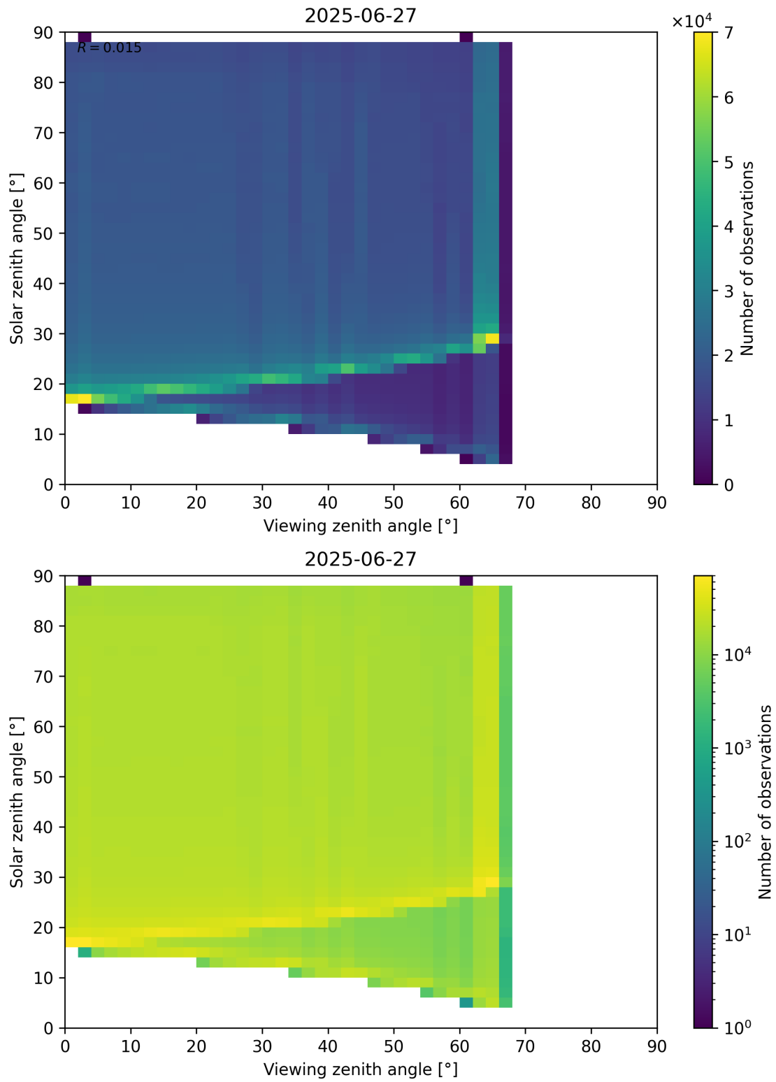
Figure 127: Scatter density plot of “Viewing zenith angle” against “Solar zenith angle” for 2025-06-27 to 2025-06-28.
