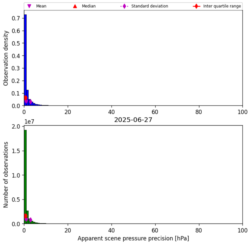
Figure 37: Histogram of “Apparent scene pressure precision” for 2025-06-27 to 2025-06-28
