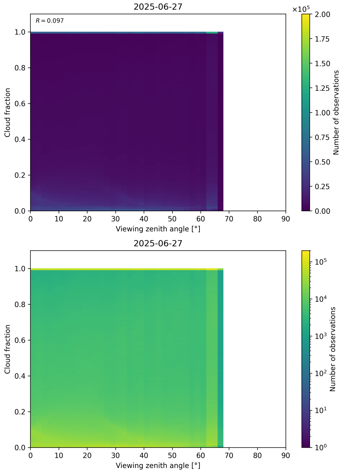
Figure 120: Scatter density plot of “Viewing zenith angle” against “Cloud fraction” for 2025-06-27 to 2025-06-28.
