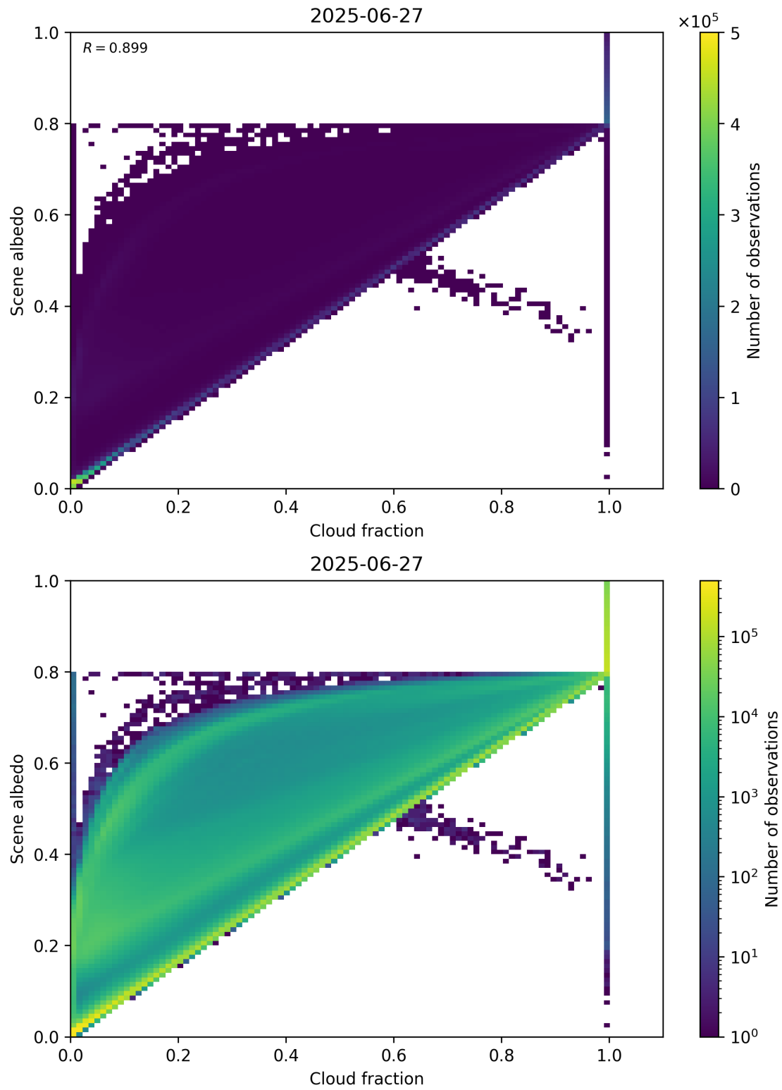
Figure 75: Scatter density plot of “Cloud fraction” against “Scene albedo” for 2025-06-27 to 2025-06-28.
