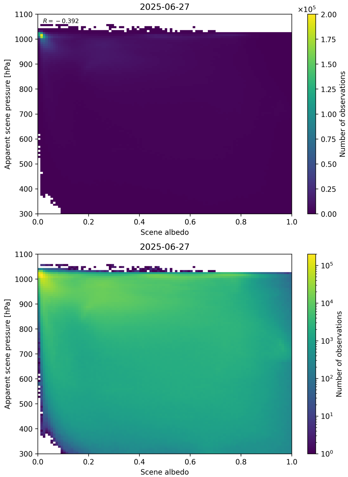
Figure 102: Scatter density plot of “Scene albedo” against “Apparent scene pressure” for 2025-06-27 to 2025-06-28.
