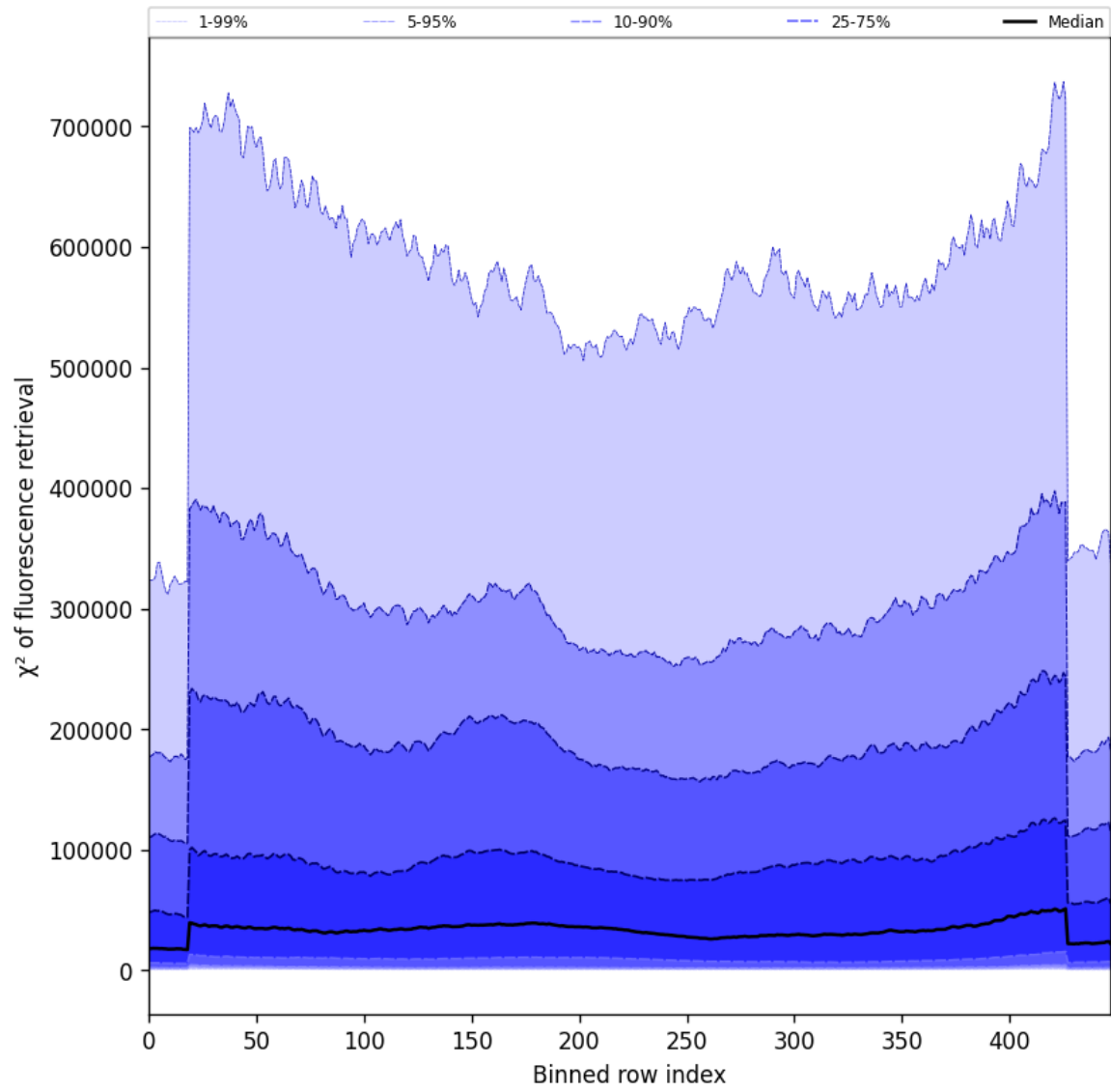
Figure 59: Along track statistics of “ \chi^2 of fluorescence retrieval” for 2025-06-27 to 2025-06-28
