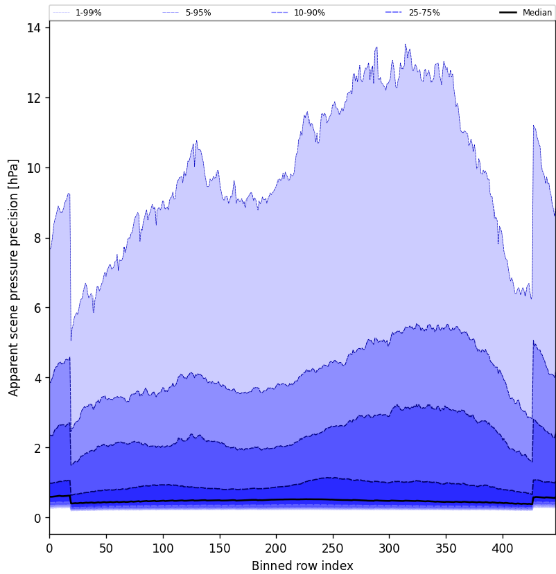
Figure 54: Along track statistics of “Apparent scene pressure precision” for 2025-06-27 to 2025-06-28
