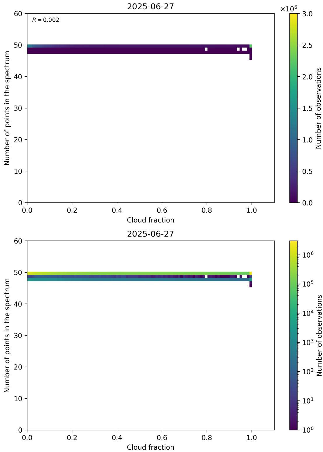
Figure 74: Scatter density plot of “Cloud fraction” against “Number of points in the spectrum” for 2025-06-27 to 2025-06-28.
