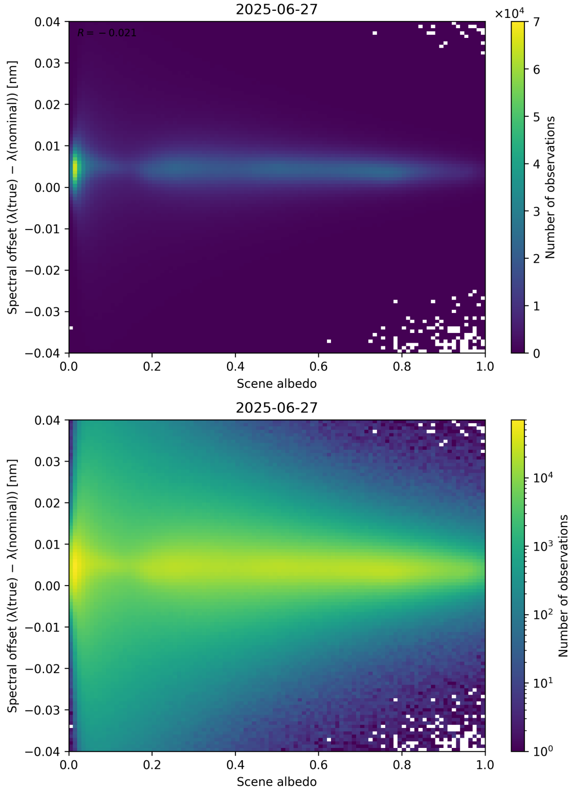
Figure 107: Scatter density plot of “Scene albedo” against “Spectral offset ( \lambda_{\text{true}} - \lambda_{\text{nominal}} )” for 2025-06-27 to 2025-06-28.
