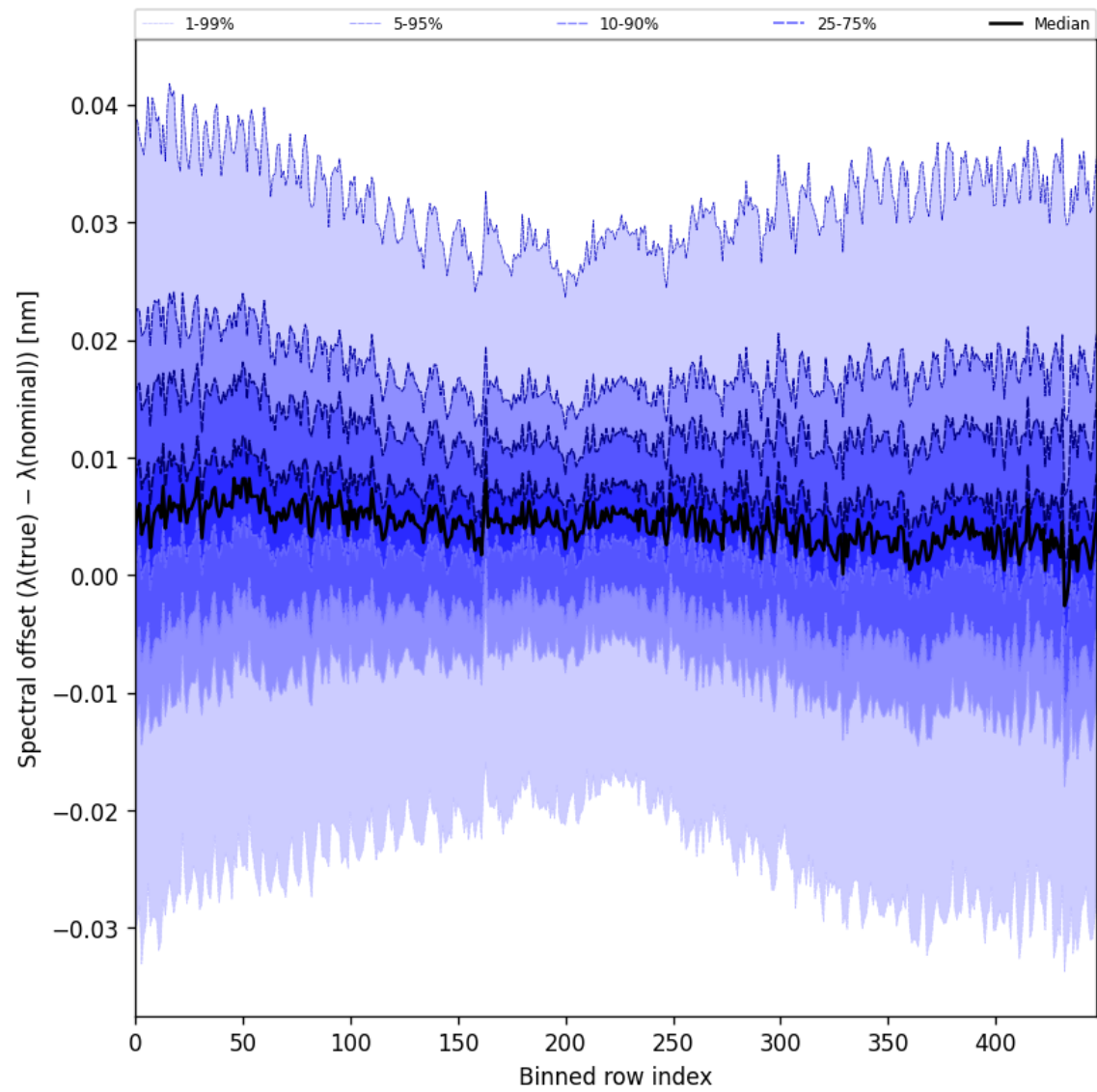
Figure 62: Along track statistics of “Spectral offset ( \lambda_{\text{true}} - \lambda_{\text{nominal}} )” for 2025-06-27 to 2025-06-28
