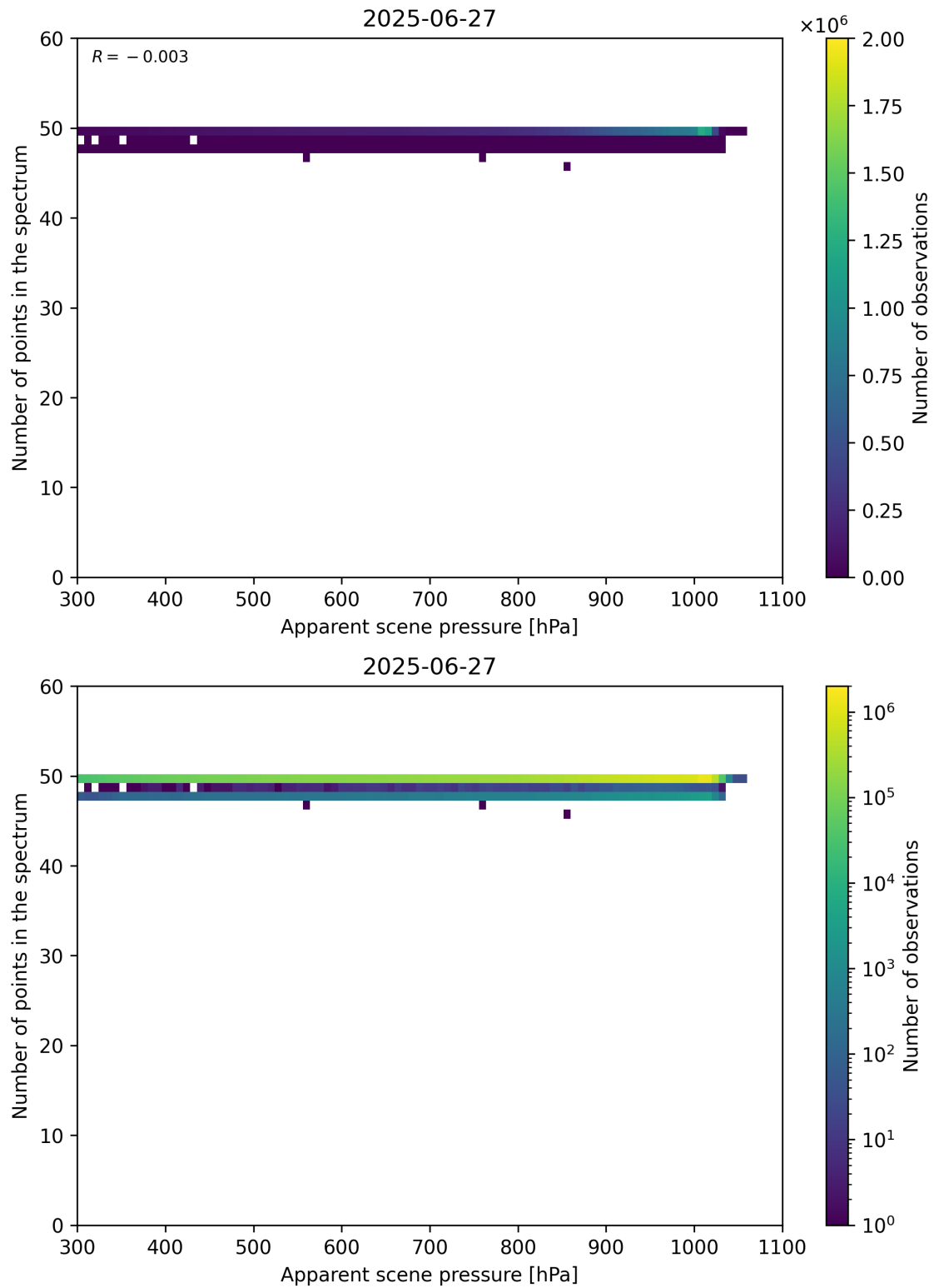
Figure 66: Scatter density plot of “Apparent scene pressure” against “Number of points in the spectrum” for 2025-06-27 to 2025-06-28.
