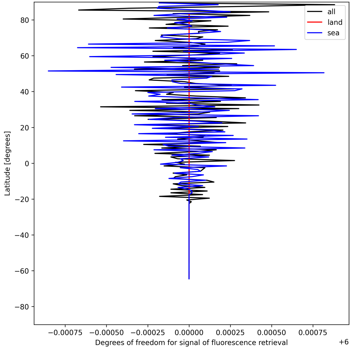
Figure 26: Zonal average of “Degrees of freedom for signal of fluorescence retrieval” for 2025-06-27 to 2025-06-28.
