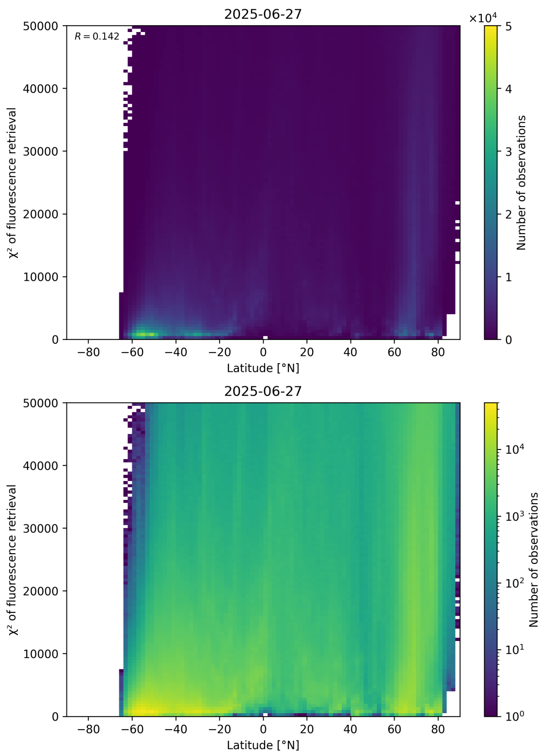
Figure 89: Scatter density plot of “Latitude” against “ \chi^2 of fluorescence retrieval” for 2025-06-27 to 2025-06-28.
