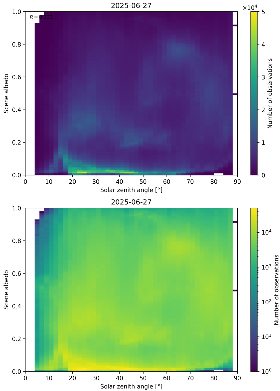
Figure 116: Scatter density plot of “Solar zenith angle” against “Scene albedo” for 2025-06-27 to 2025-06-28.
