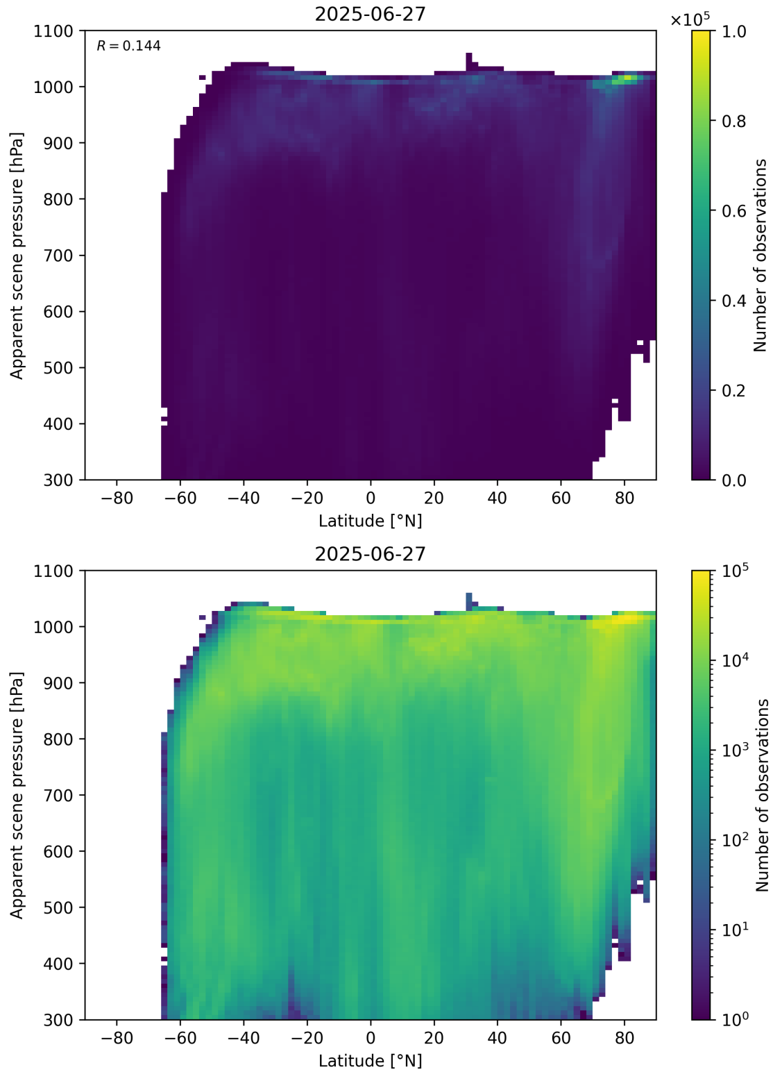
Figure 88: Scatter density plot of “Latitude” against “Apparent scene pressure” for 2025-06-27 to 2025-06-28.
