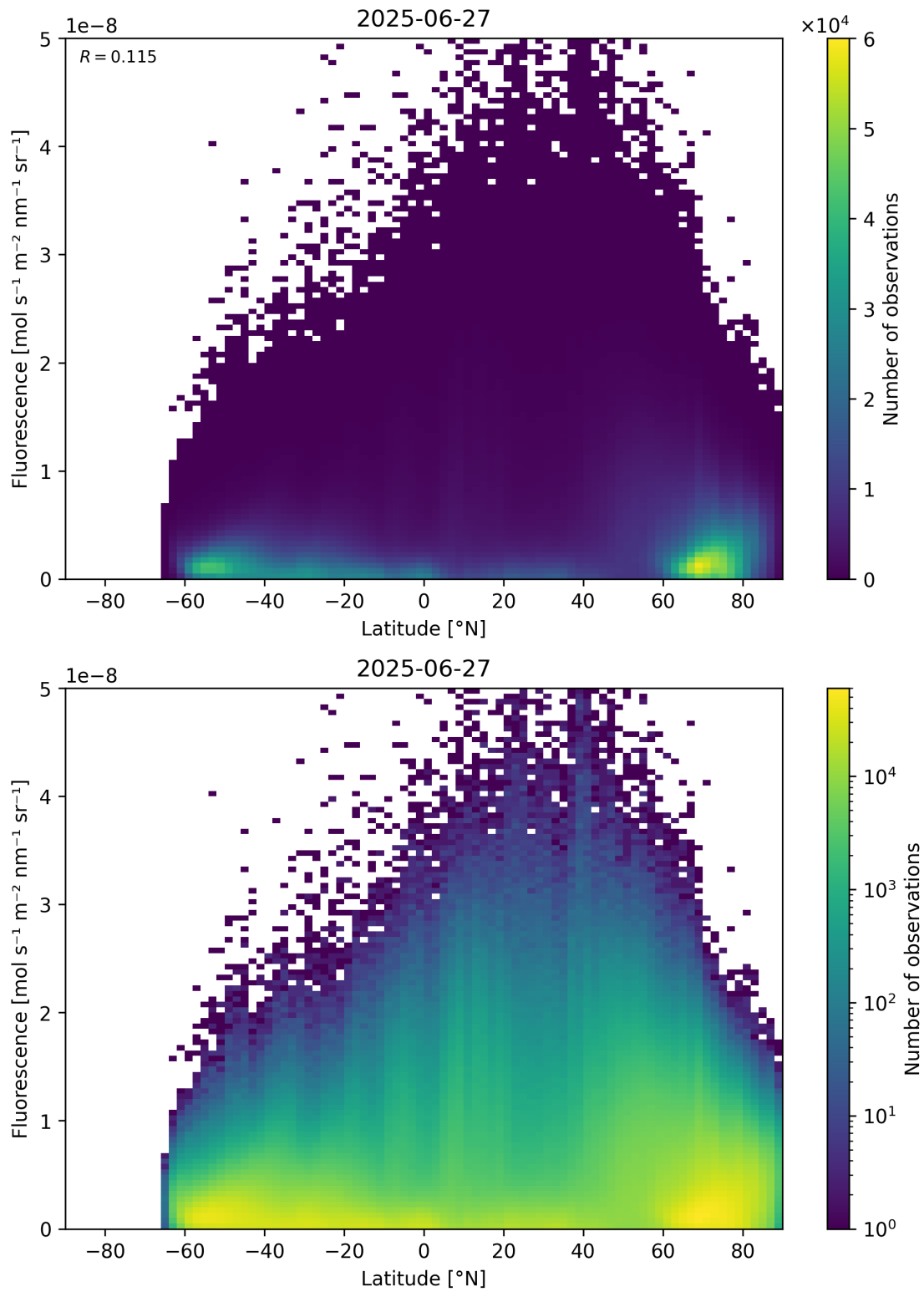
Figure 92: Scatter density plot of “Latitude” against “Fluorescence” for 2025-06-27 to 2025-06-28.
