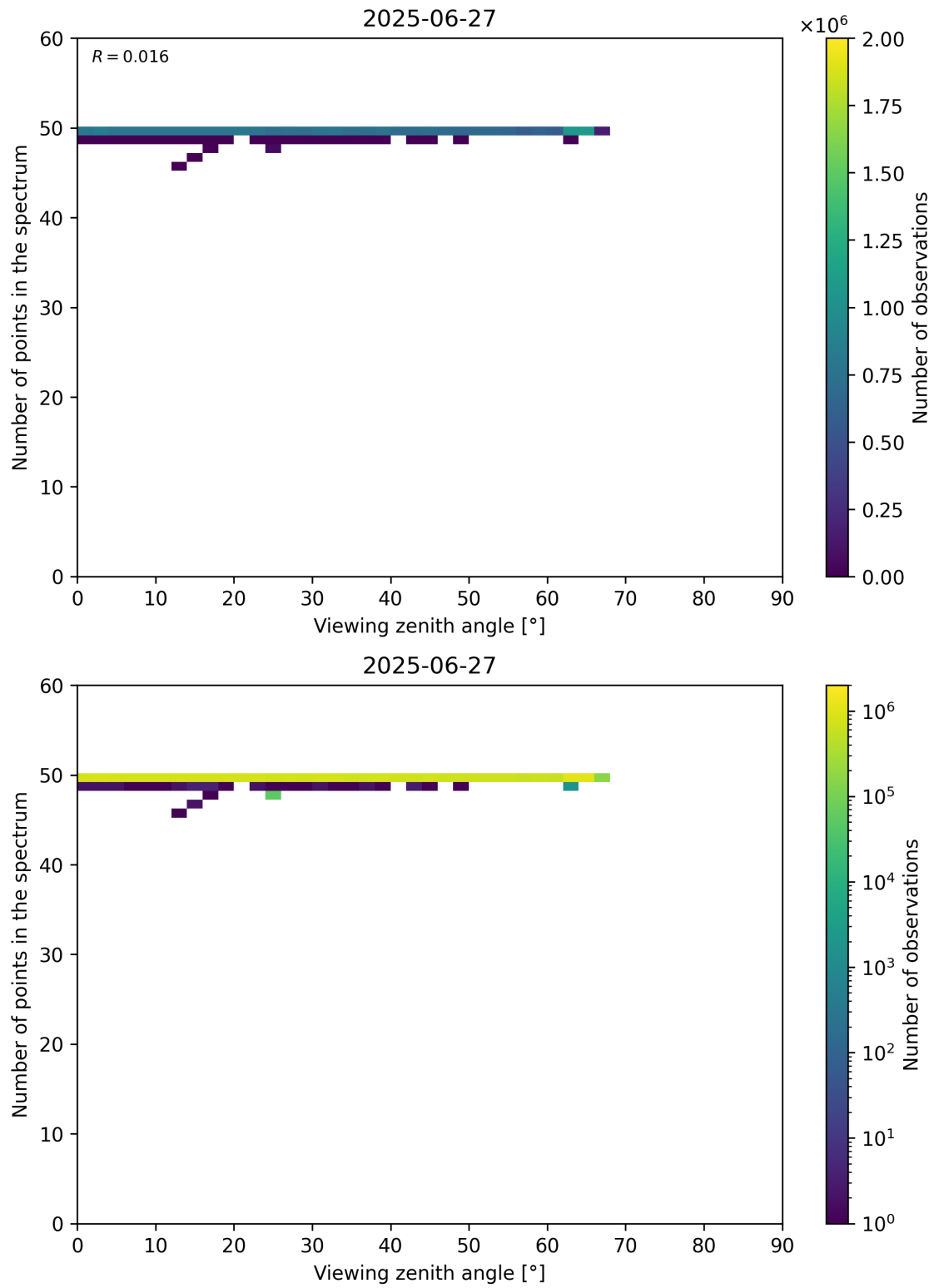
Figure 125: Scatter density plot of “Viewing zenith angle” against “Number of points in the spectrum” for 2025-06-27 to 2025-06-28.
