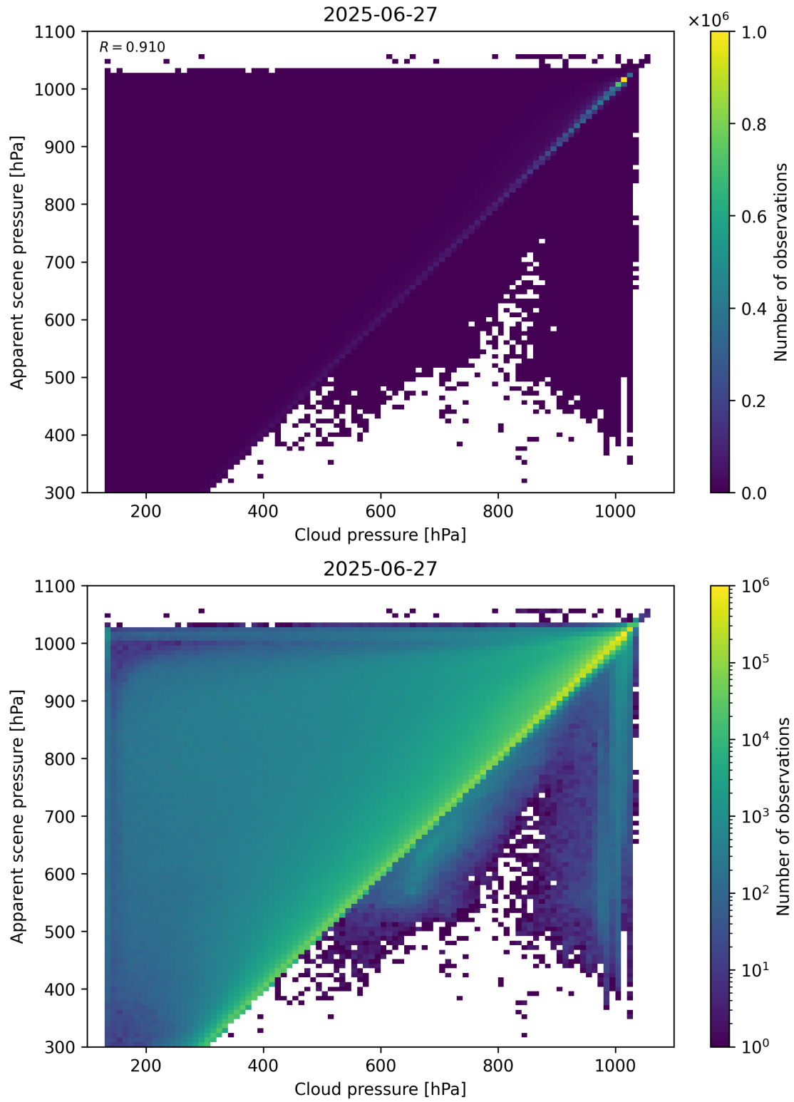
Figure 77: Scatter density plot of “Cloud pressure” against “Apparent scene pressure” for 2025-06-27 to 2025-06-28.
