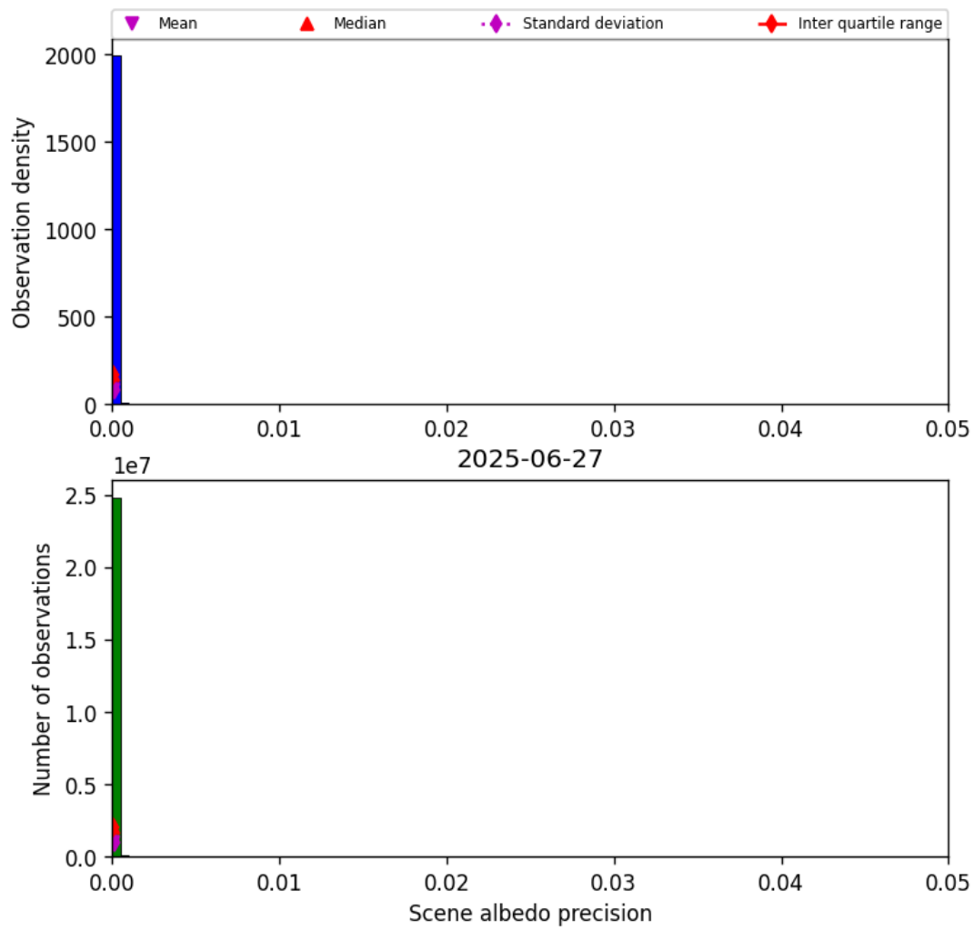
Figure 35: Histogram of “Scene albedo precision” for 2025-06-27 to 2025-06-28
