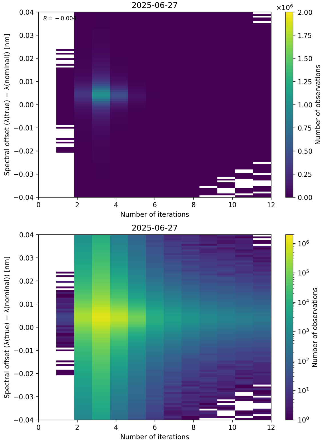
Figure 100: Scatter density plot of “Number of iterations” against “Spectral offset ( \lambda_{\text{true}} - \lambda_{\text{nominal}} )” for 2025-06-27 to 2025-06-28.
