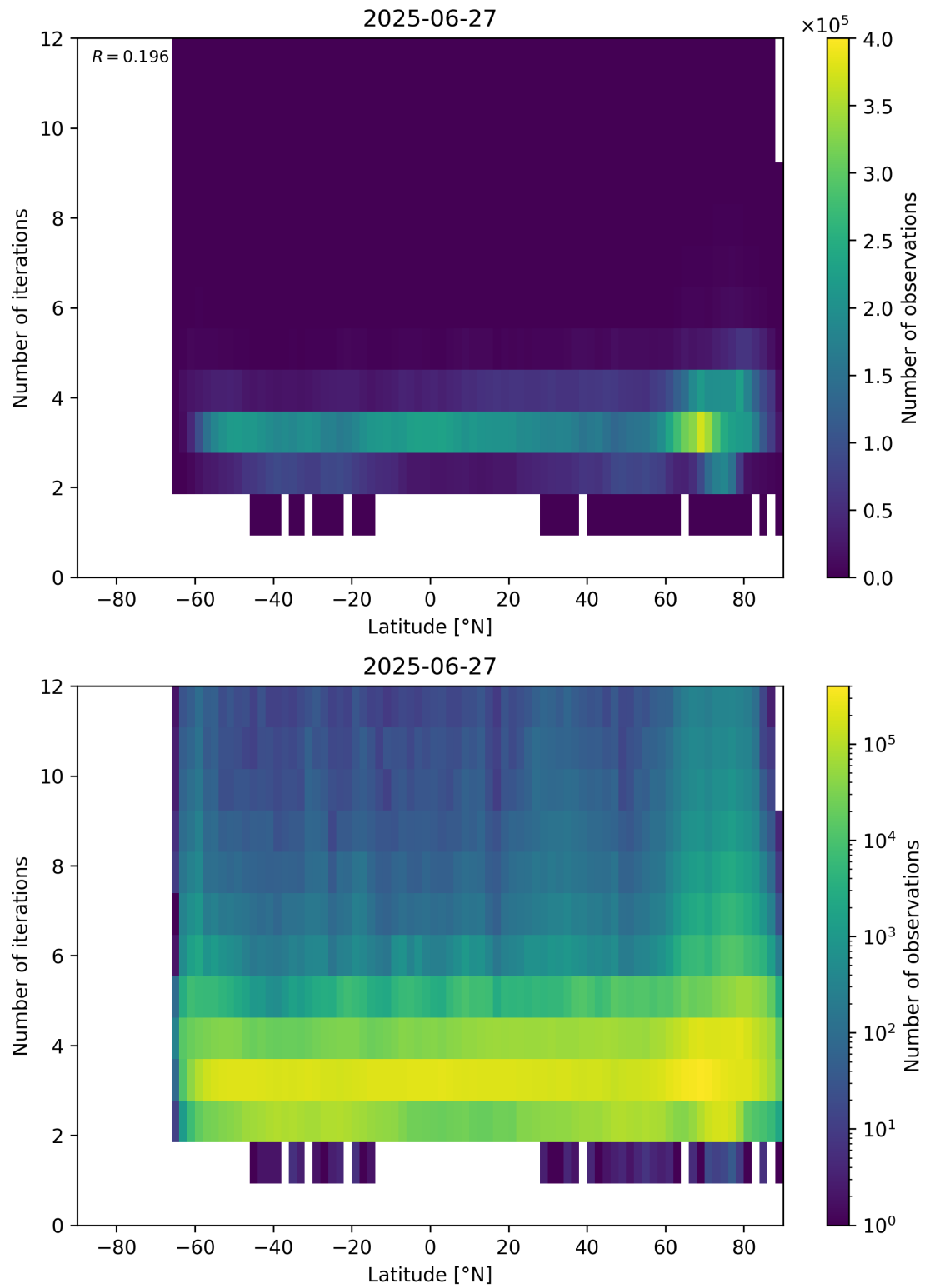
Figure 93: Scatter density plot of “Latitude” against “Number of iterations” for 2025-06-27 to 2025-06-28.
