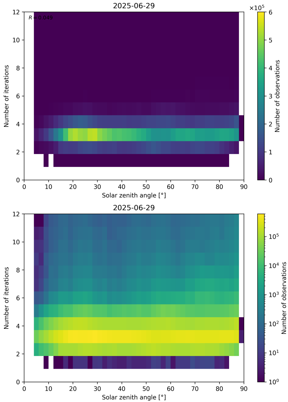
Figure 114: Scatter density plot of “Solar zenith angle” against “Number of iterations” for 2025-06-28 to 2025-06-30.
