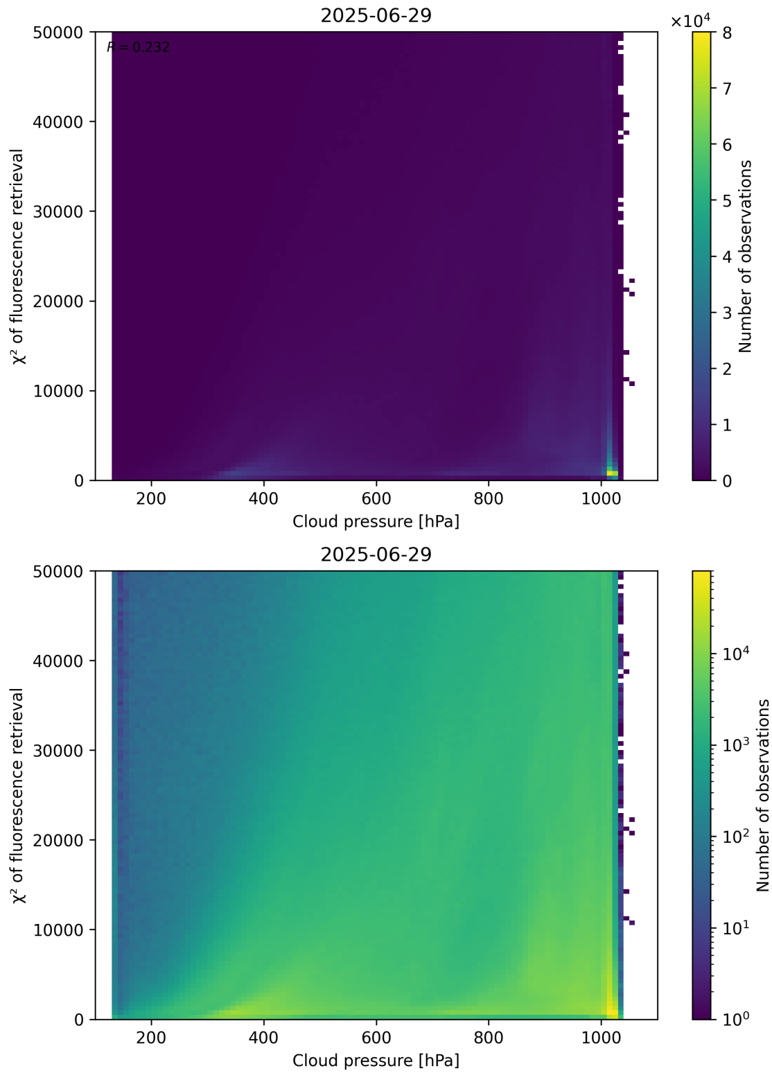
Figure 78: Scatter density plot of “Cloud pressure” against “ \chi^2 of fluorescence retrieval” for 2025-06-28 to 2025-06-30.
