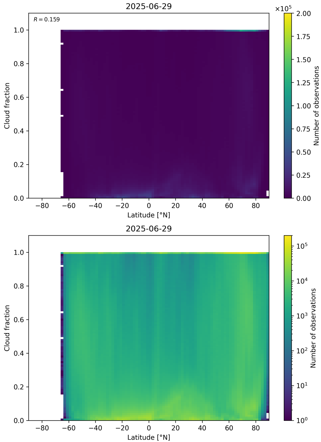
Figure 90: Scatter density plot of “Latitude” against “Cloud fraction” for 2025-06-28 to 2025-06-30.
