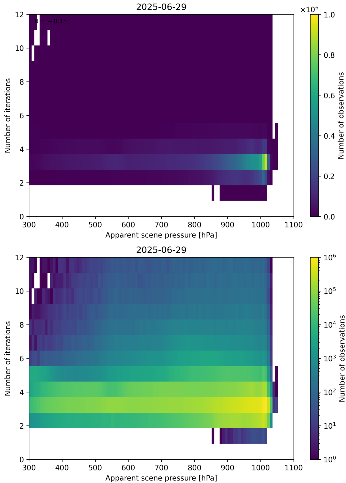
Figure 65: Scatter density plot of “Apparent scene pressure” against “Number of iterations” for 2025-06-28 to 2025-06-30.
