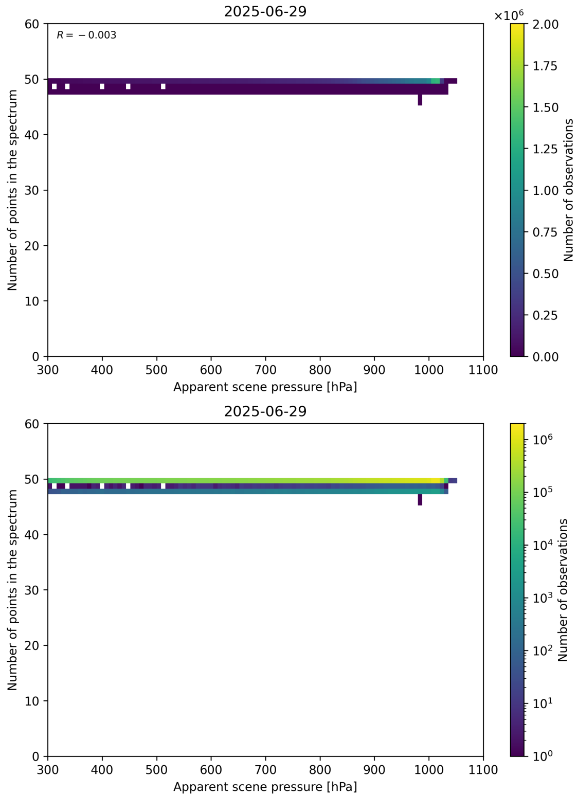
Figure 66: Scatter density plot of “Apparent scene pressure” against “Number of points in the spectrum” for 2025-06-28 to 2025-06-30.
