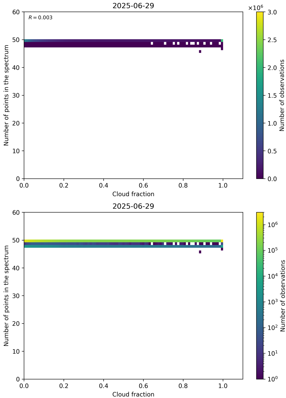
Figure 74: Scatter density plot of “Cloud fraction” against “Number of points in the spectrum” for 2025-06-28 to 2025-06-30.
