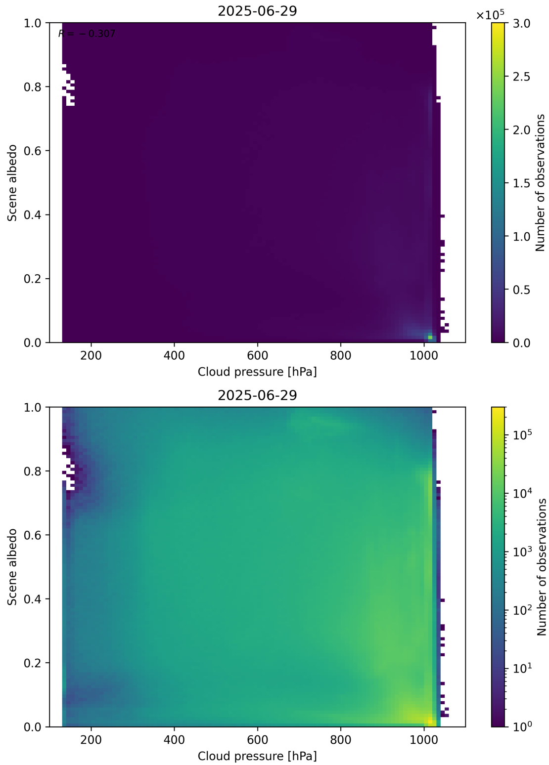
Figure 83: Scatter density plot of “Cloud pressure” against “Scene albedo” for 2025-06-28 to 2025-06-30.
