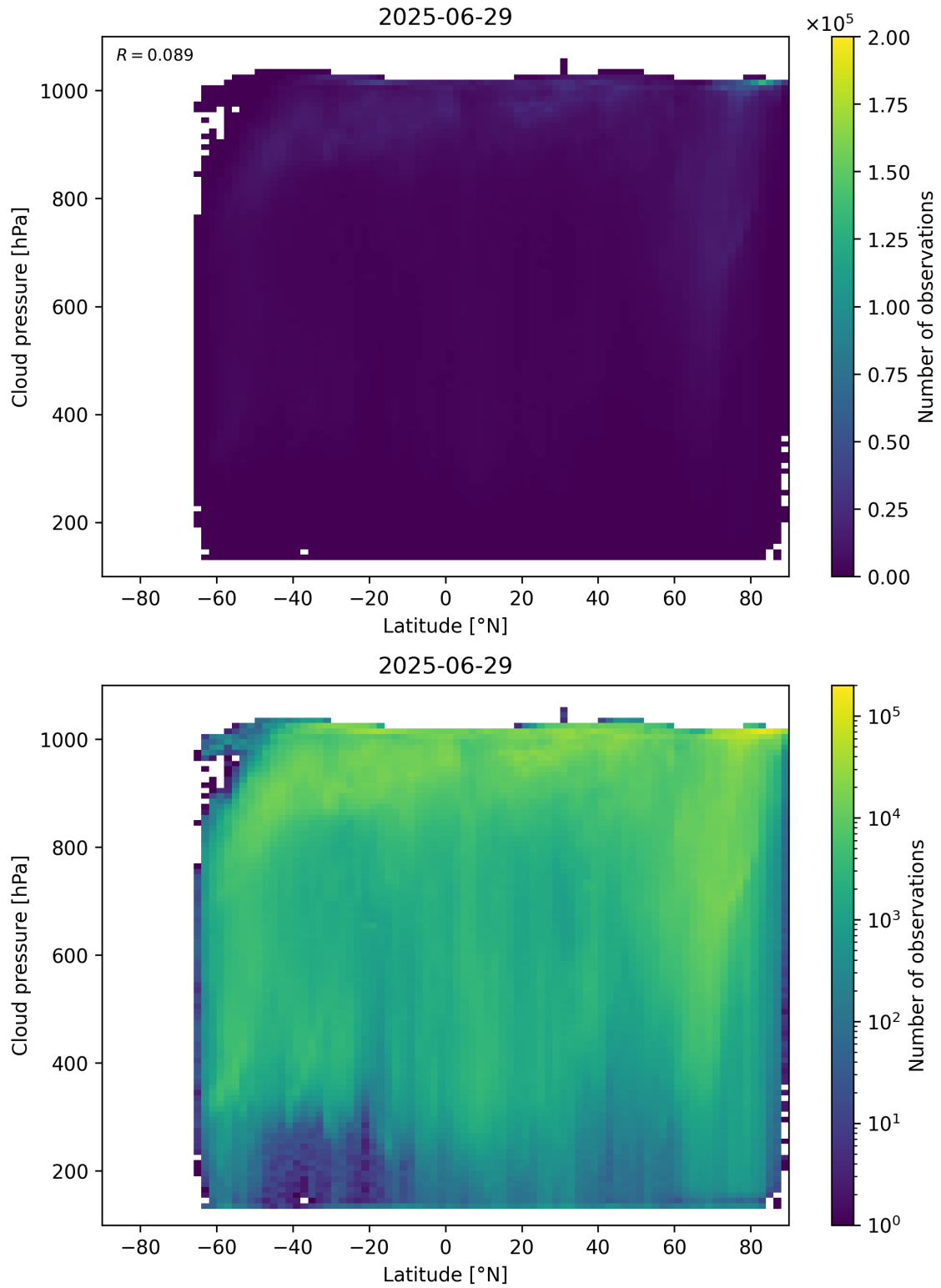
Figure 91: Scatter density plot of “Latitude” against “Cloud pressure” for 2025-06-28 to 2025-06-30.
