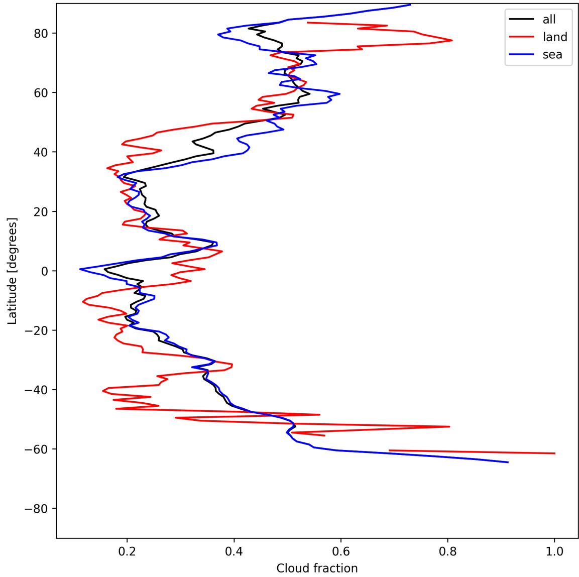
Figure 15: Zonal average of “Cloud fraction” for 2025-06-28 to 2025-06-30.
