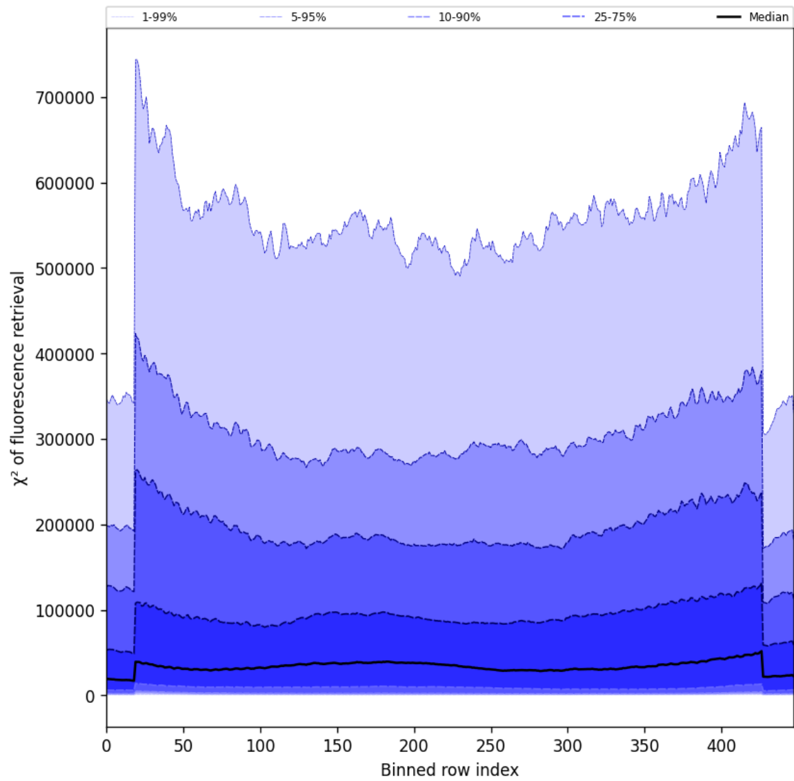
Figure 59: Along track statistics of “ \chi^2 of fluorescence retrieval” for 2025-06-28 to 2025-06-30
