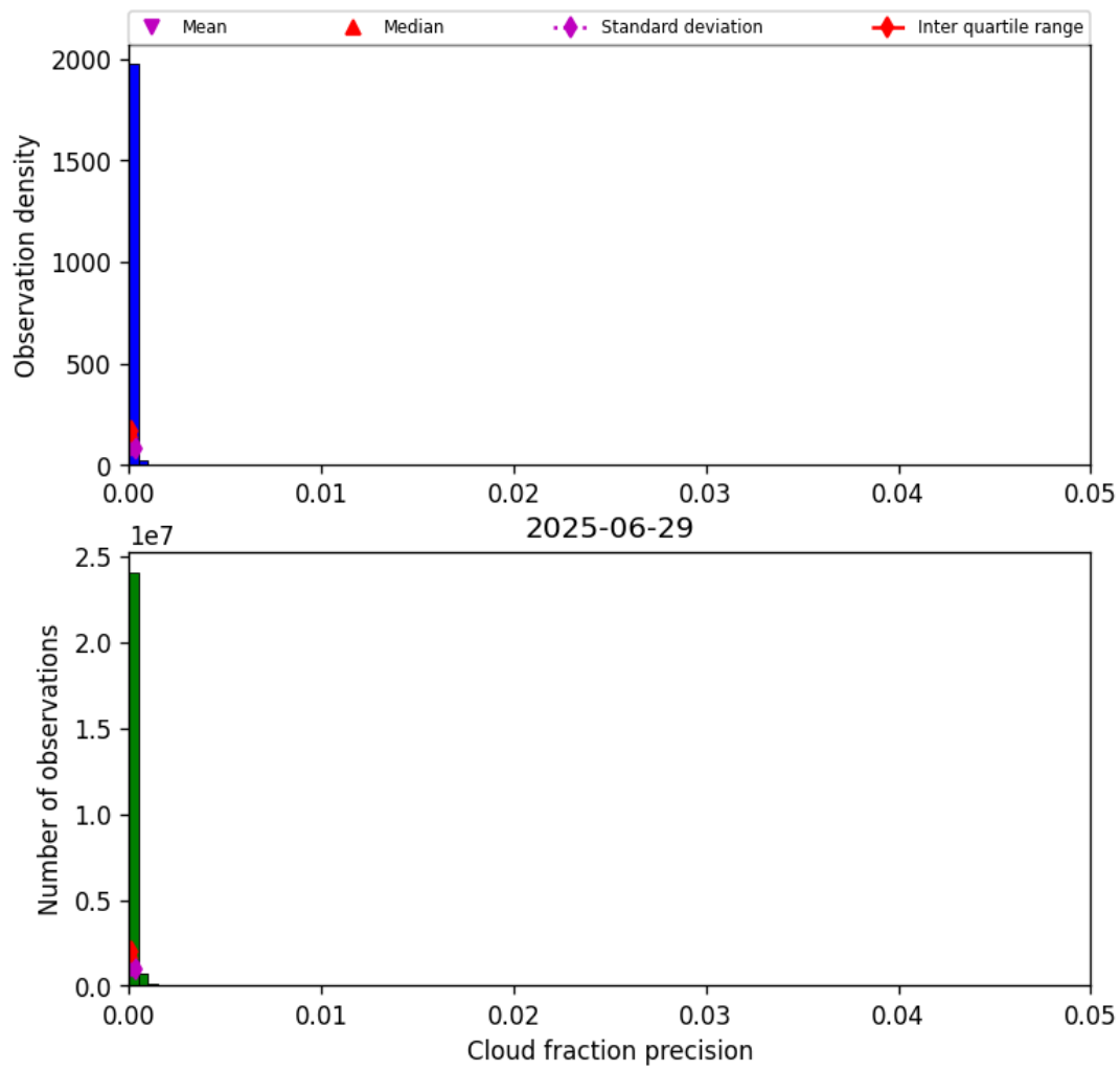
Figure 33: Histogram of “Cloud fraction precision” for 2025-06-28 to 2025-06-30
