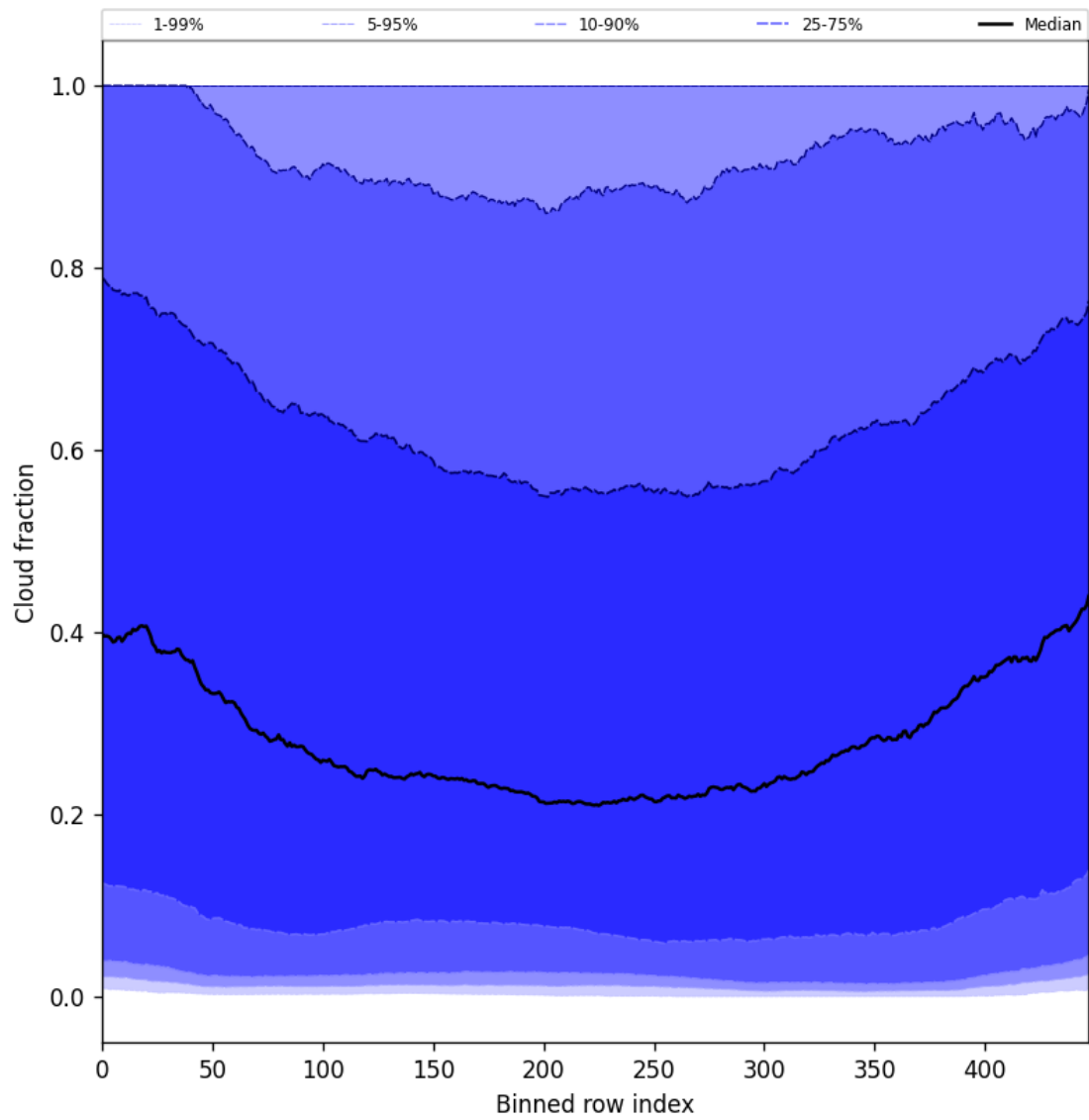
Figure 49: Along track statistics of “Cloud fraction” for 2025-06-28 to 2025-06-30
