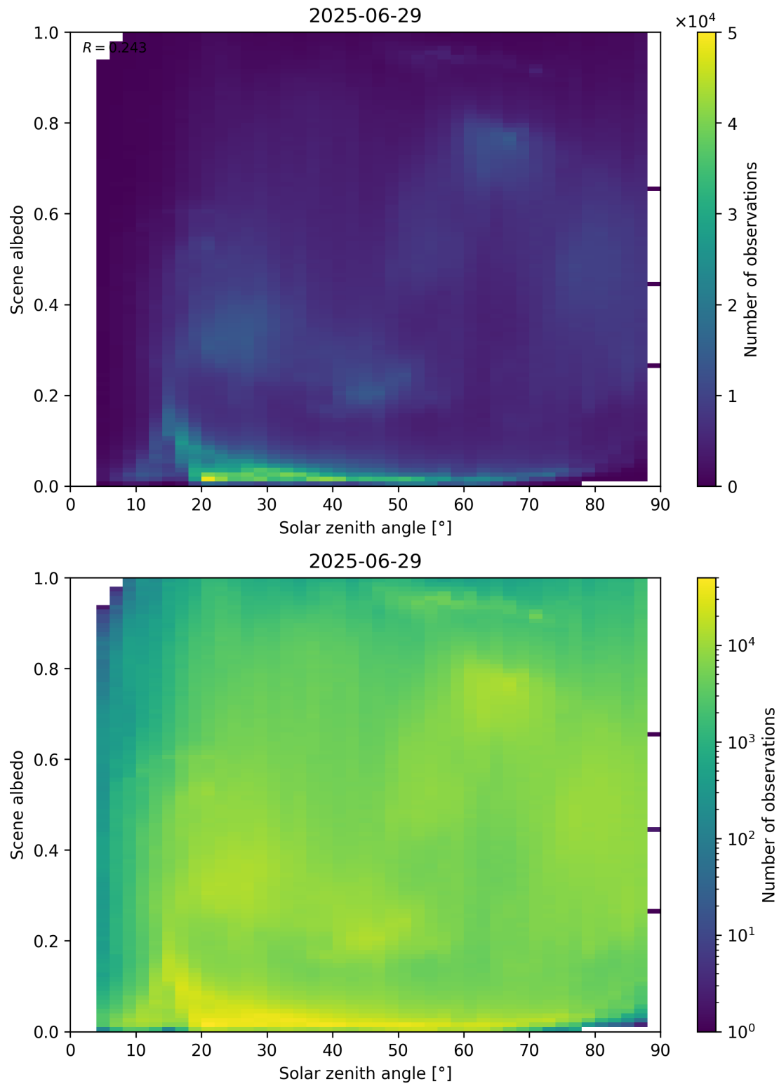
Figure 116: Scatter density plot of “Solar zenith angle” against “Scene albedo” for 2025-06-28 to 2025-06-30.
