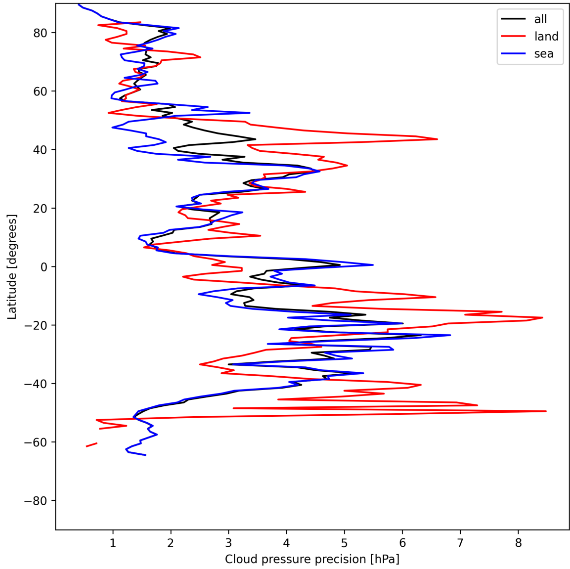
Figure 14: Zonal average of “Cloud pressure precision” for 2025-06-28 to 2025-06-30.
