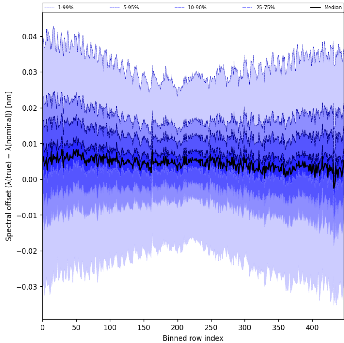
Figure 62: Along track statistics of “Spectral offset ( \lambda_{\text{true}} - \lambda_{\text{nominal}} )” for 2025-06-28 to 2025-06-30
