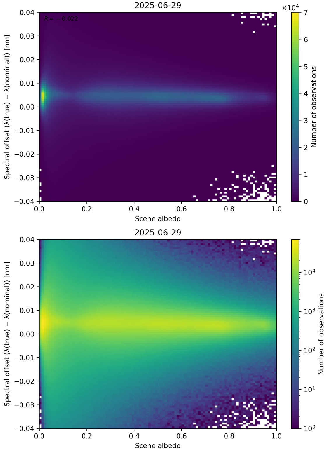
Figure 107: Scatter density plot of “Scene albedo” against “Spectral offset ( \lambda_{\text{true}} - \lambda_{\text{nominal}} )” for 2025-06-28 to 2025-06-30.
