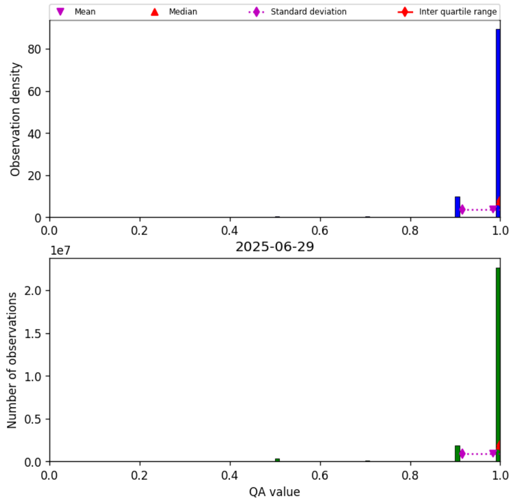
Figure 29: Histogram of “QA value” for 2025-06-28 to 2025-06-30
