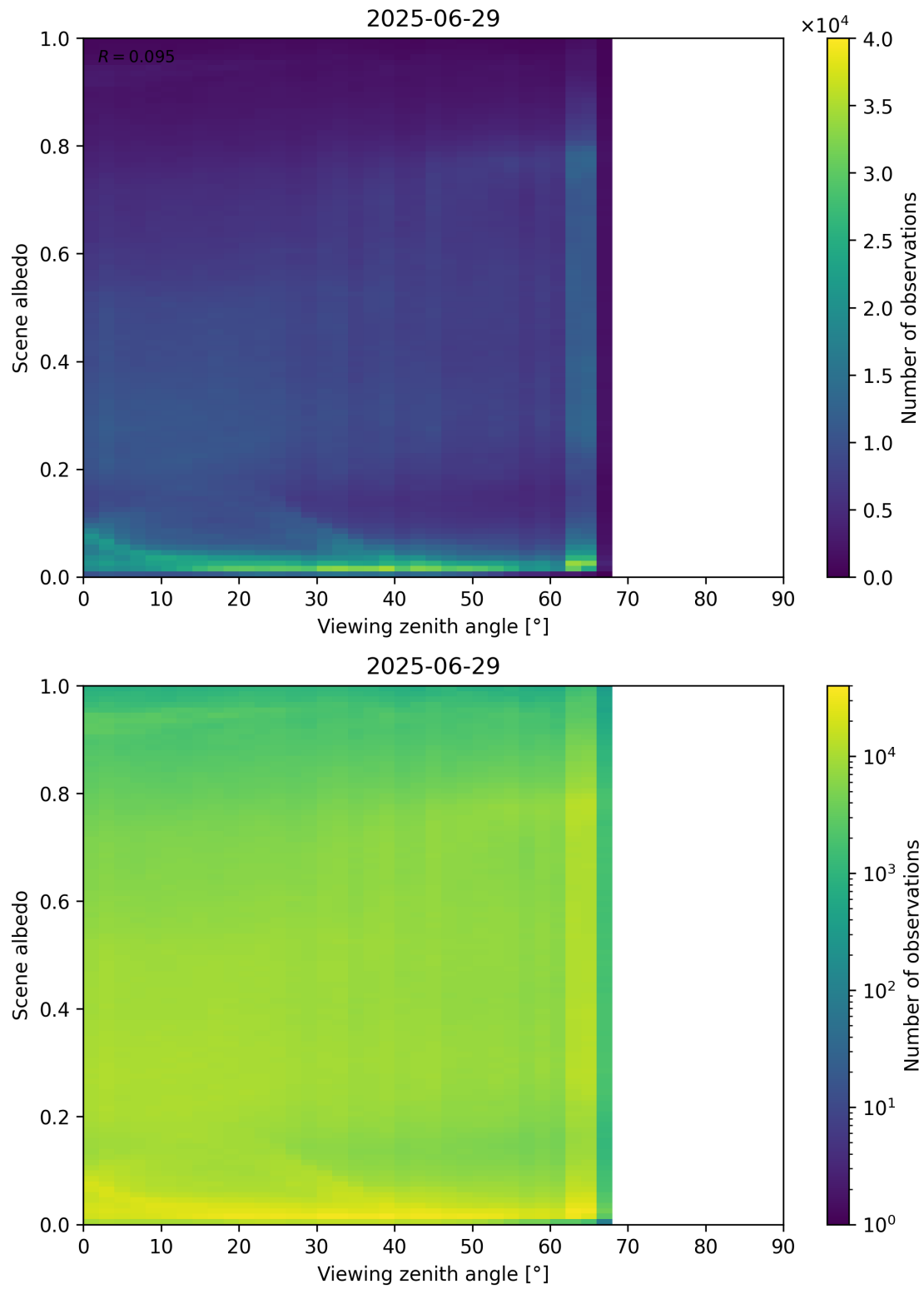
Figure 126: Scatter density plot of “Viewing zenith angle” against “Scene albedo” for 2025-06-28 to 2025-06-30.
