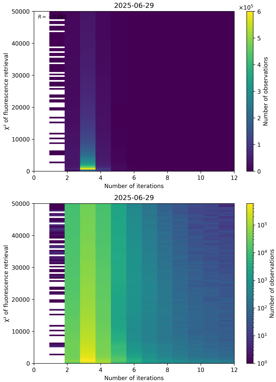
Figure 97: Scatter density plot of “Number of iterations” against “ \chi^2 of fluorescence retrieval” for 2025-06-28 to 2025-06-30.
