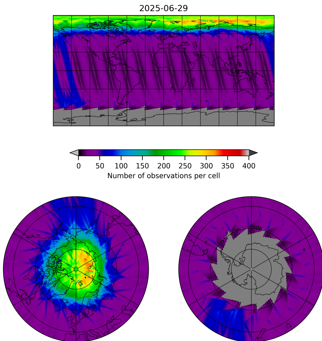
Figure 11: Map of the number of observations for 2025-06-28 to 2025-06-30
