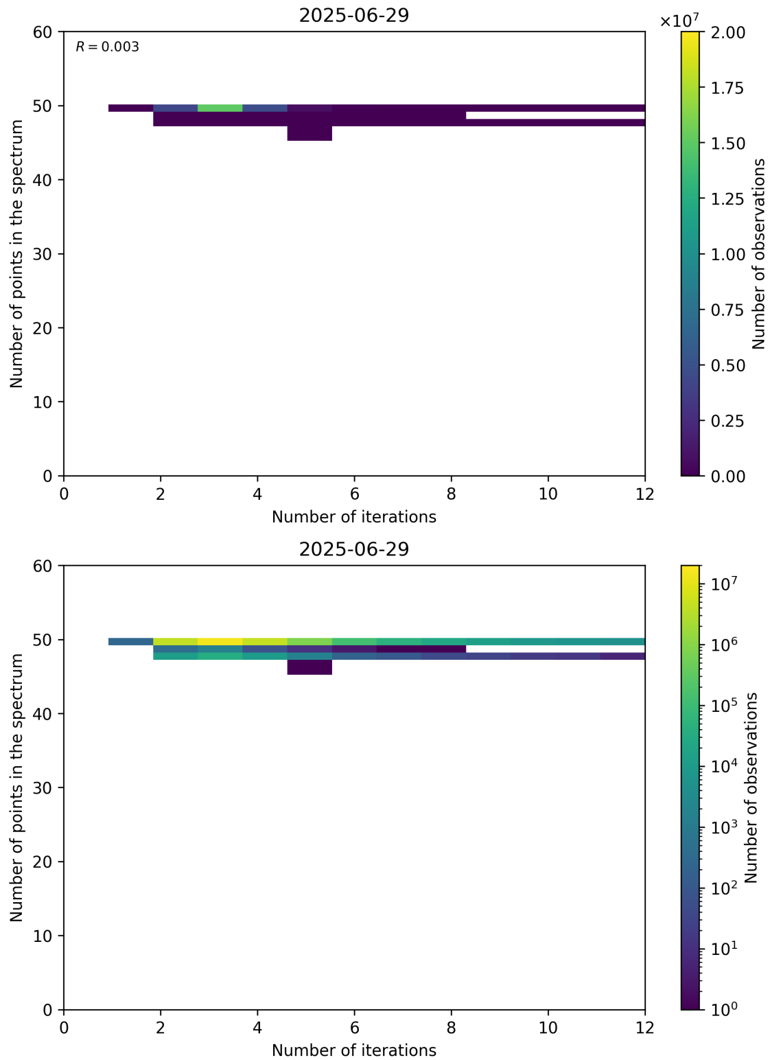
Figure 99: Scatter density plot of “Number of iterations” against “Number of points in the spectrum” for 2025-06-28 to 2025-06-30.
