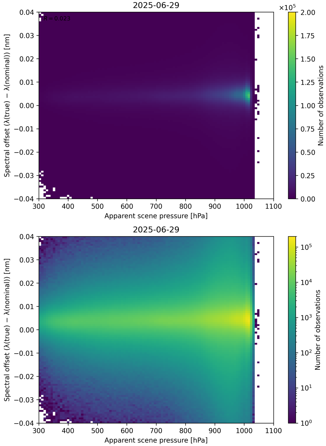
Figure 67: Scatter density plot of “Apparent scene pressure” against “Spectral offset ( \lambda_{\text{true}} - \lambda_{\text{nominal}} )” for 2025-06-28 to 2025-06-30.
