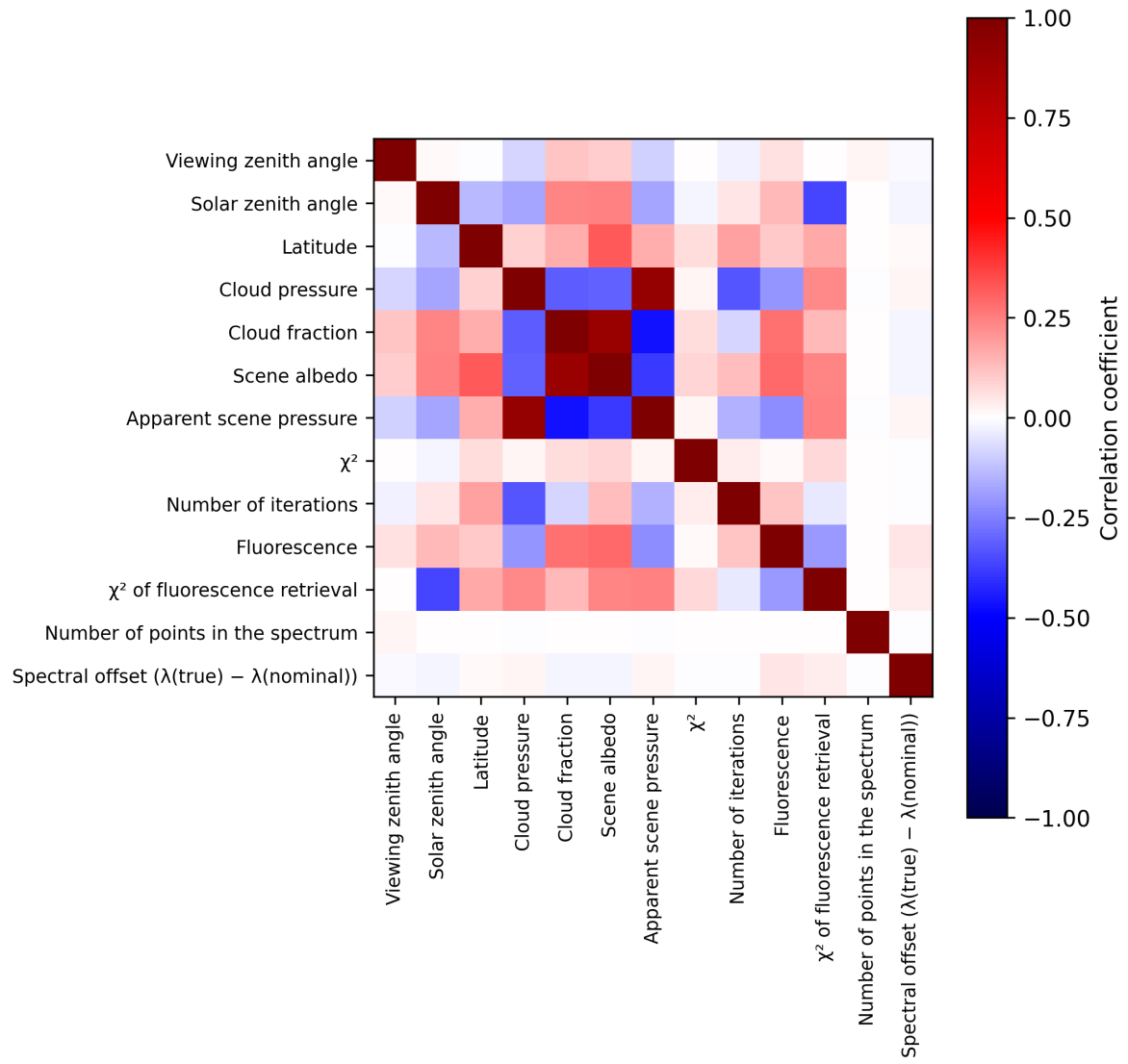
Figure 2: Map of correlation matrix for 2025-06-28 to 2025-06-30.
