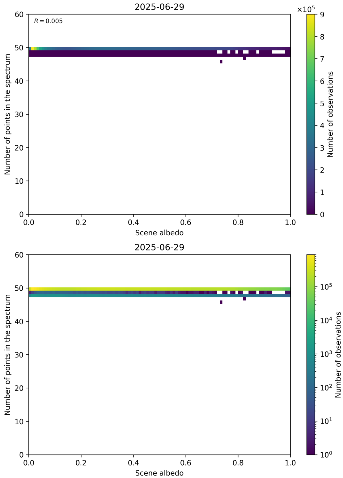
Figure 106: Scatter density plot of “Scene albedo” against “Number of points in the spectrum” for 2025-06-28 to 2025-06-30.
