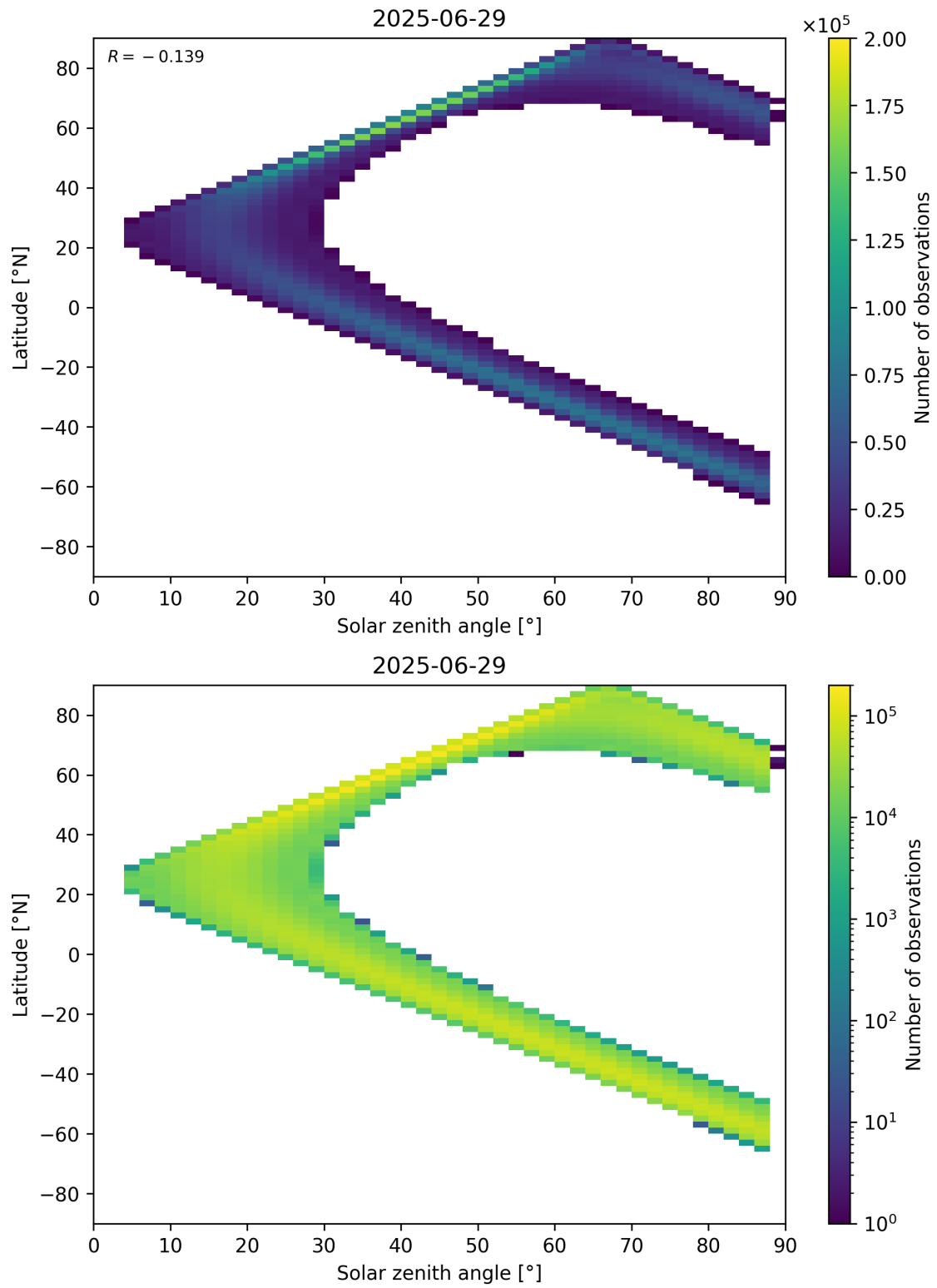
Figure 113: Scatter density plot of “Solar zenith angle” against “Latitude” for 2025-06-28 to 2025-06-30.
