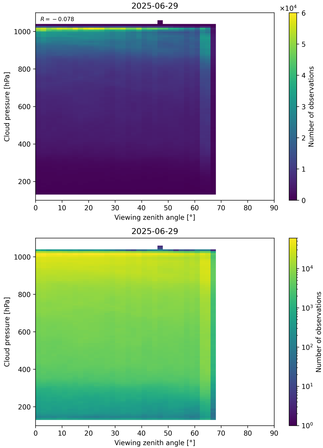
Figure 121: Scatter density plot of “Viewing zenith angle” against “Cloud pressure” for 2025-06-28 to 2025-06-30.
