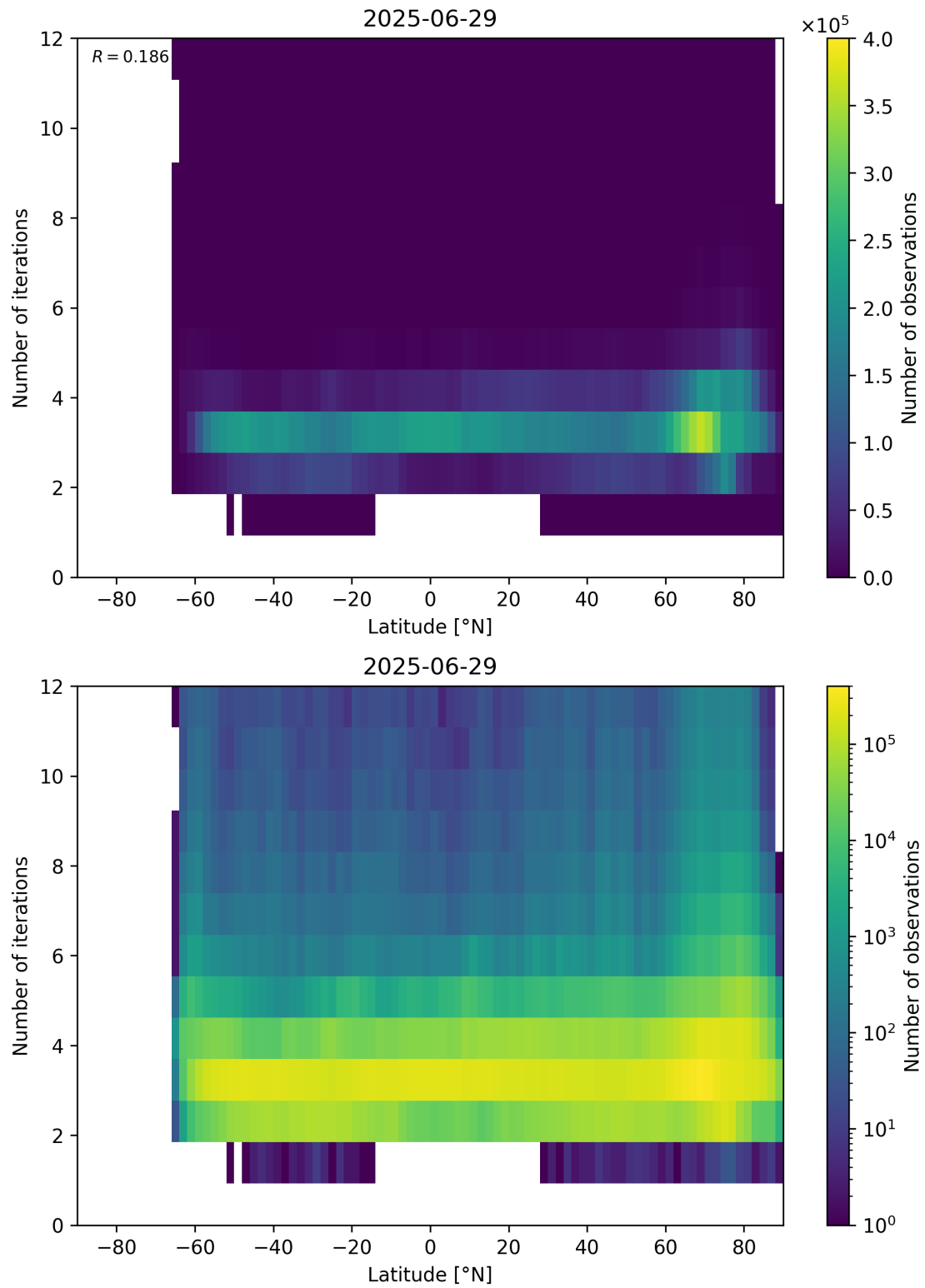
Figure 93: Scatter density plot of “Latitude” against “Number of iterations” for 2025-06-28 to 2025-06-30.
