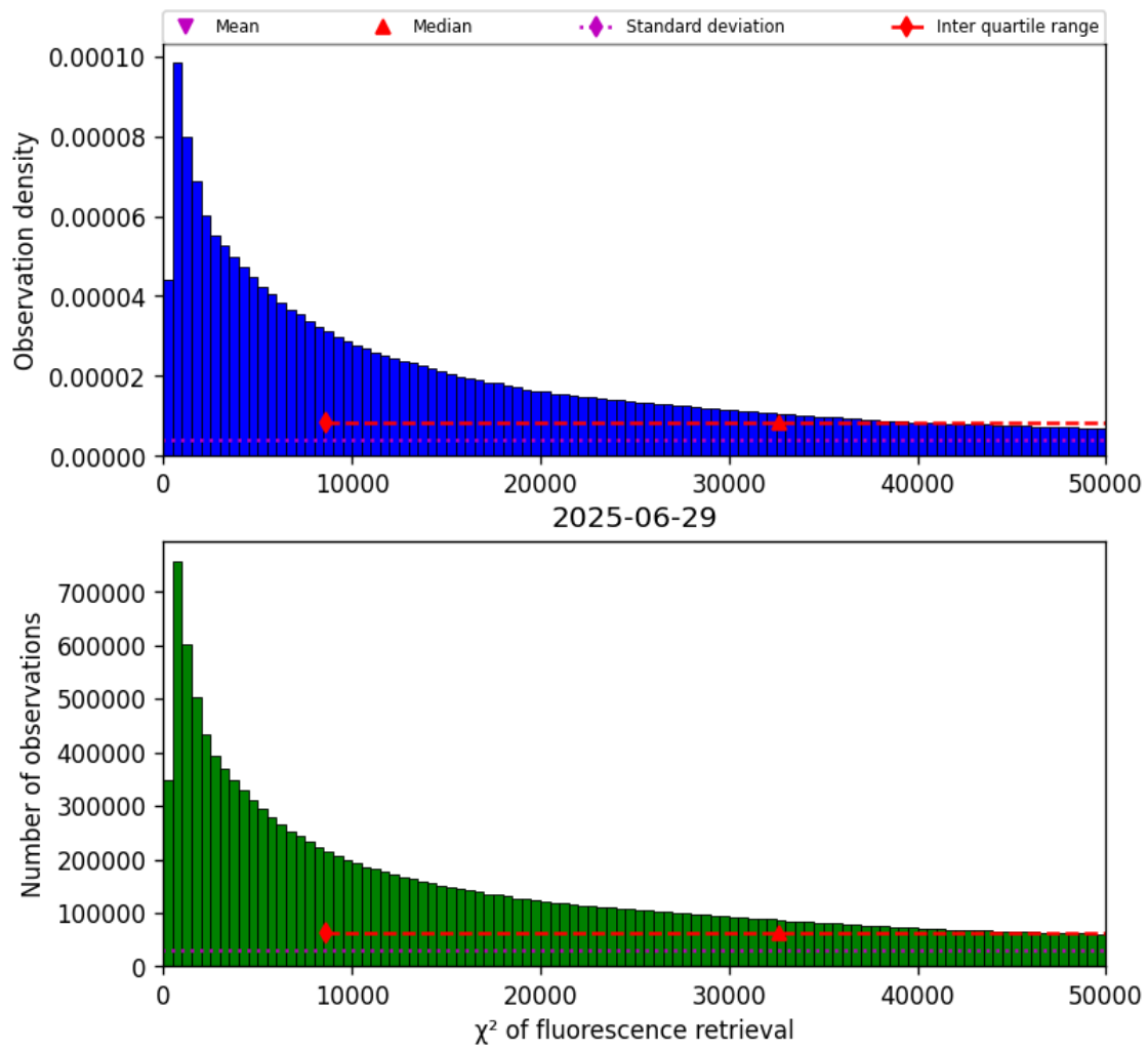
Figure 42: Histogram of “ \chi^2 of fluorescence retrieval” for 2025-06-28 to 2025-06-30
