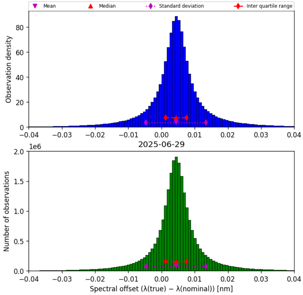
Figure 45: Histogram of “Spectral offset ( \lambda_{\text{true}} - \lambda_{\text{nominal}} )” for 2025-06-28 to 2025-06-30
