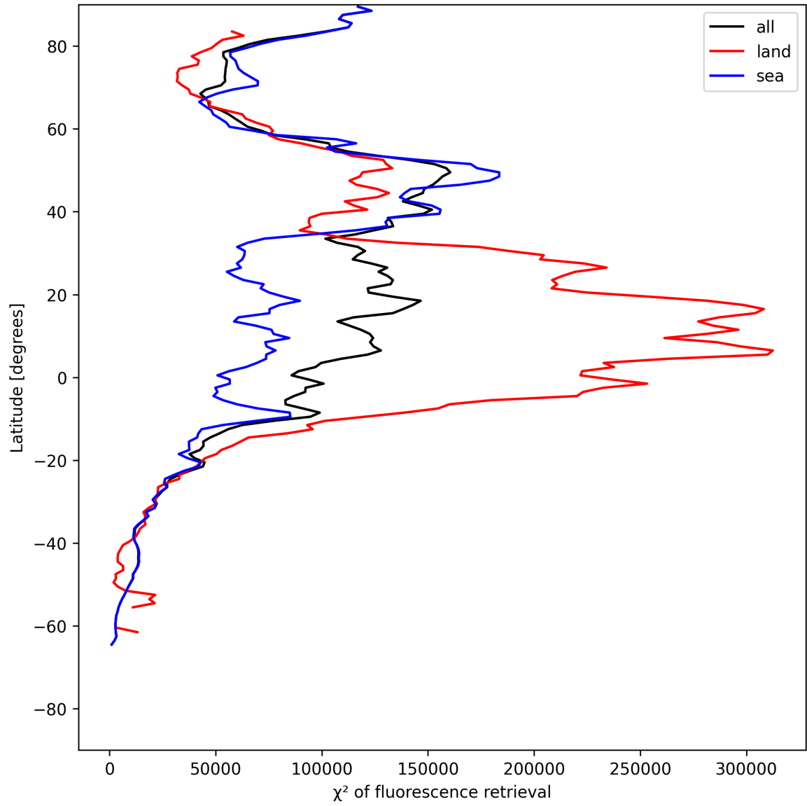
Figure 25: Zonal average of “ \chi^2 of fluorescence retrieval” for 2025-06-28 to 2025-06-30.
