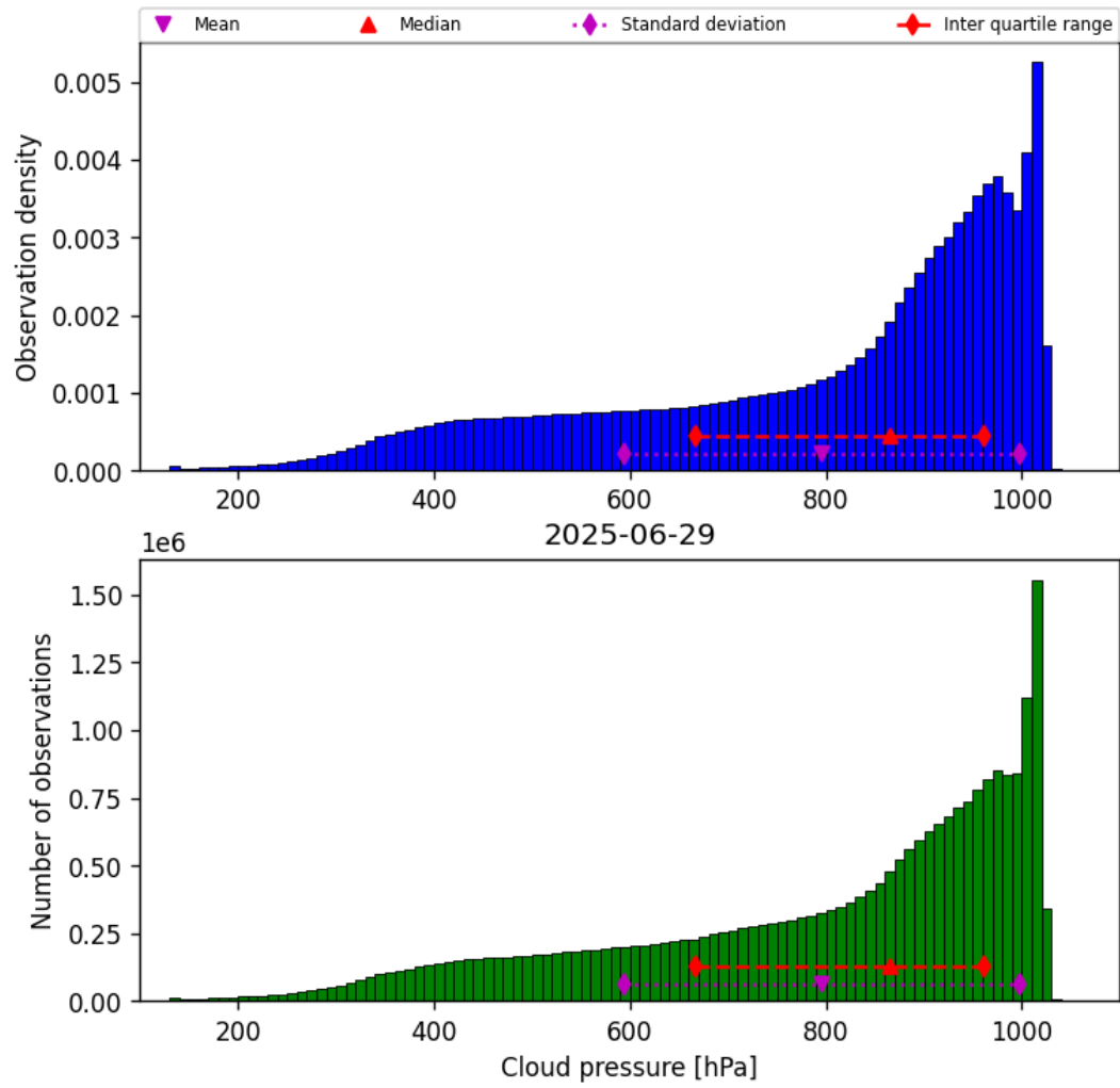
Figure 30: Histogram of “Cloud pressure” for 2025-06-28 to 2025-06-30
