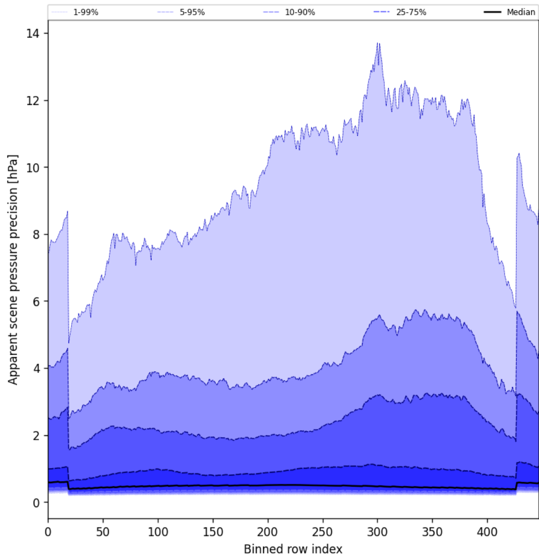
Figure 54: Along track statistics of “Apparent scene pressure precision” for 2025-06-28 to 2025-06-30
