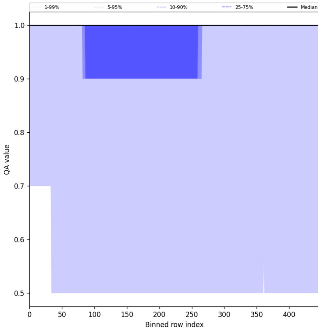
Figure 46: Along track statistics of “QA value” for 2025-06-28 to 2025-06-30
