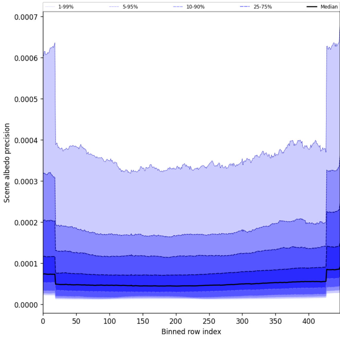
Figure 52: Along track statistics of “Scene albedo precision” for 2025-06-28 to 2025-06-30
