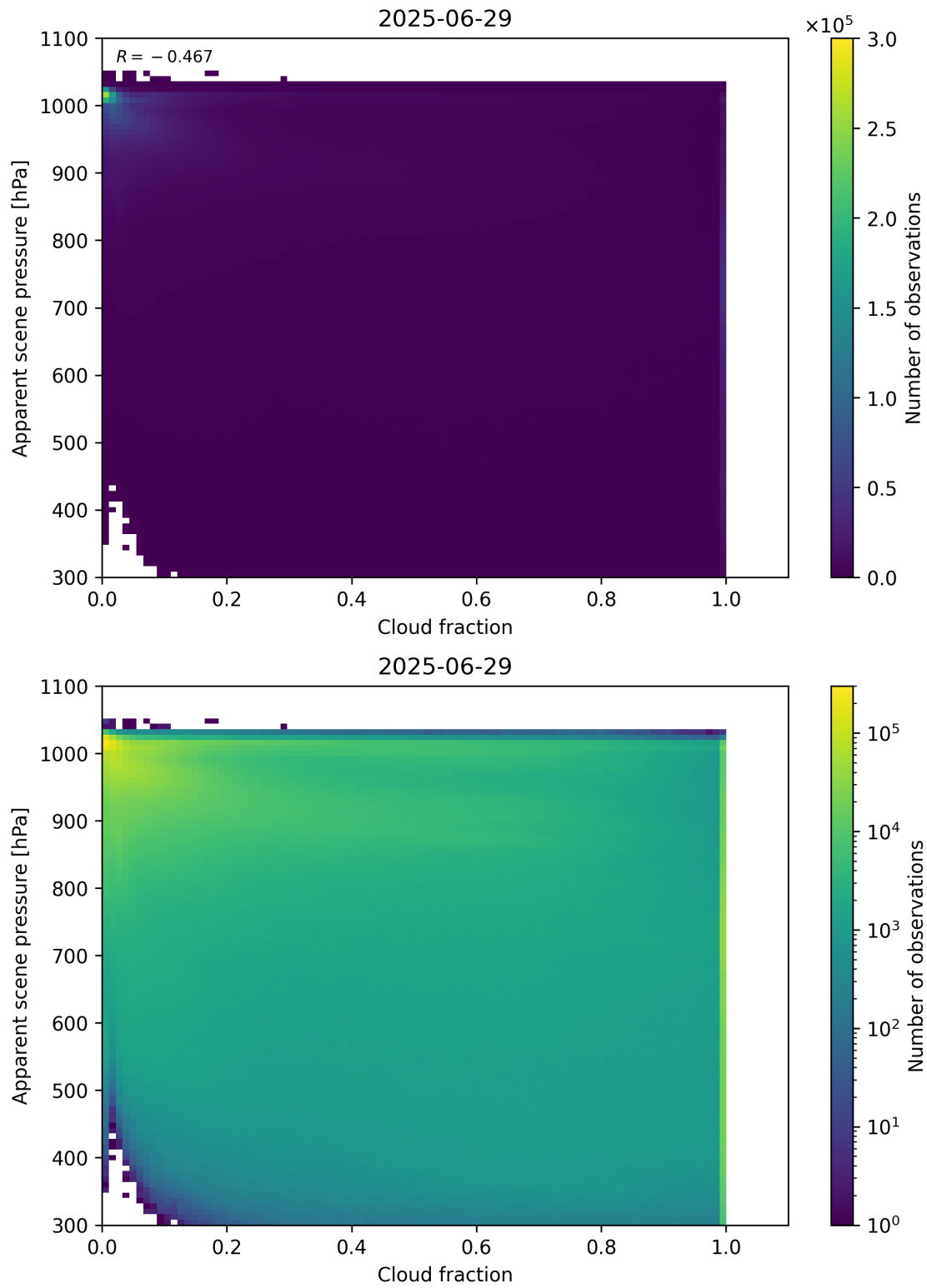
Figure 70: Scatter density plot of “Cloud fraction” against “Apparent scene pressure” for 2025-06-28 to 2025-06-30.
