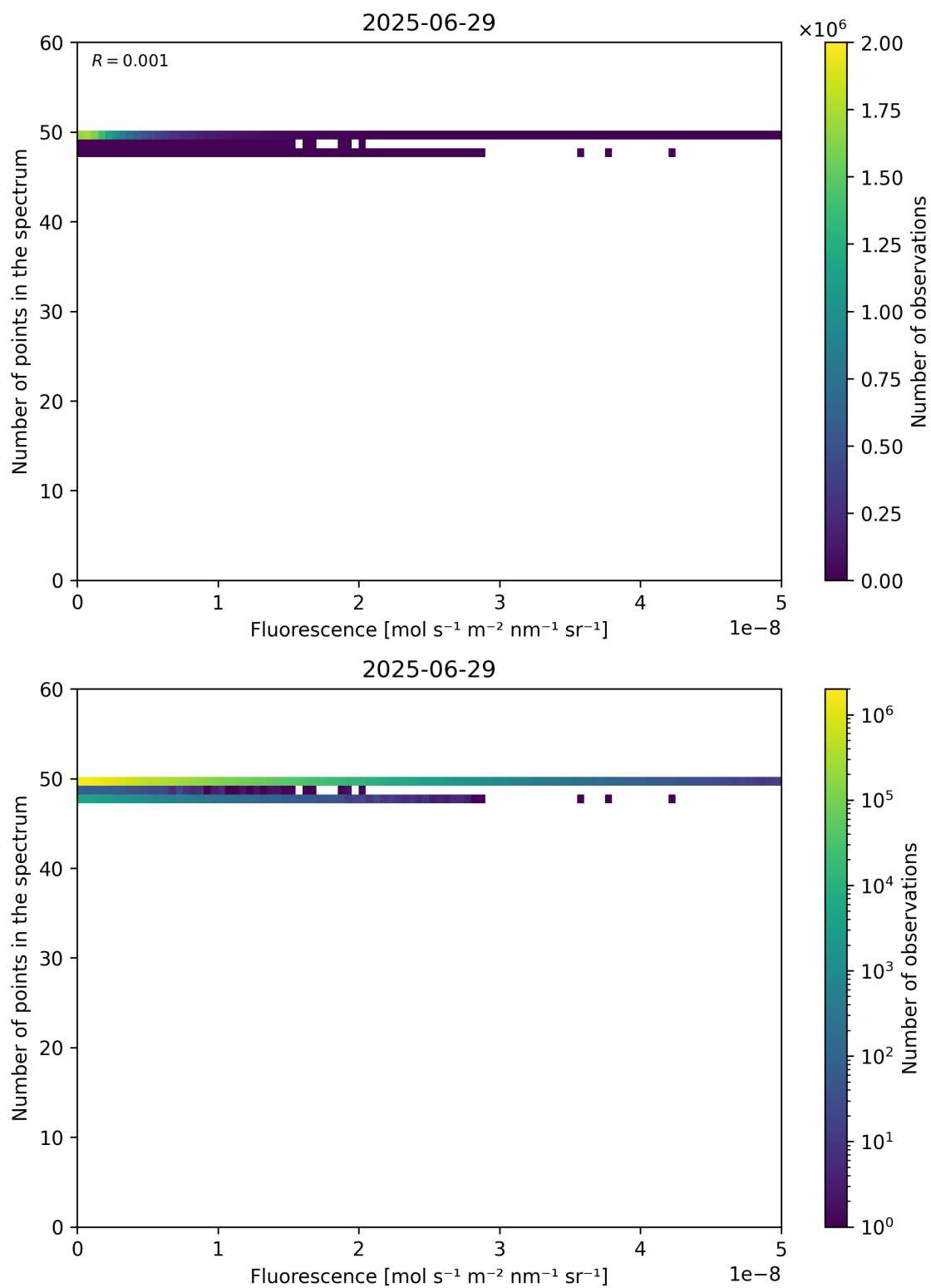
Figure 86: Scatter density plot of “Fluorescence” against “Number of points in the spectrum” for 2025-06-28 to 2025-06-30.
