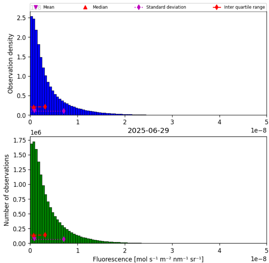
Figure 40: Histogram of “Fluorescence” for 2025-06-28 to 2025-06-30
