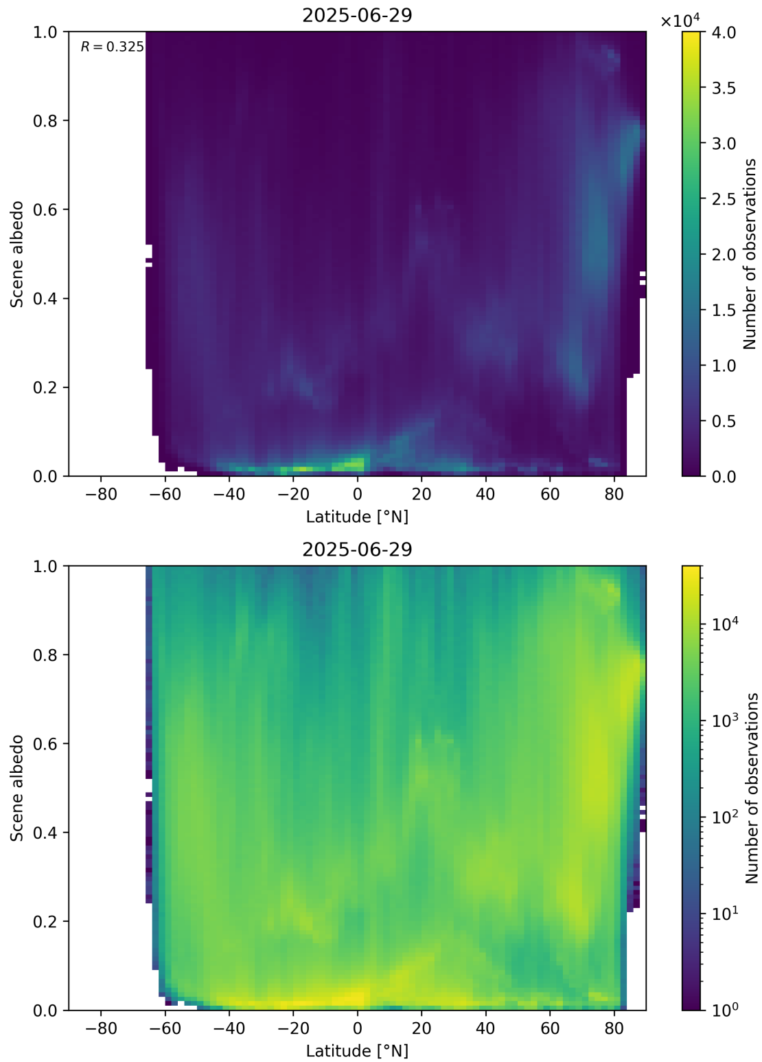
Figure 95: Scatter density plot of “Latitude” against “Scene albedo” for 2025-06-28 to 2025-06-30.
