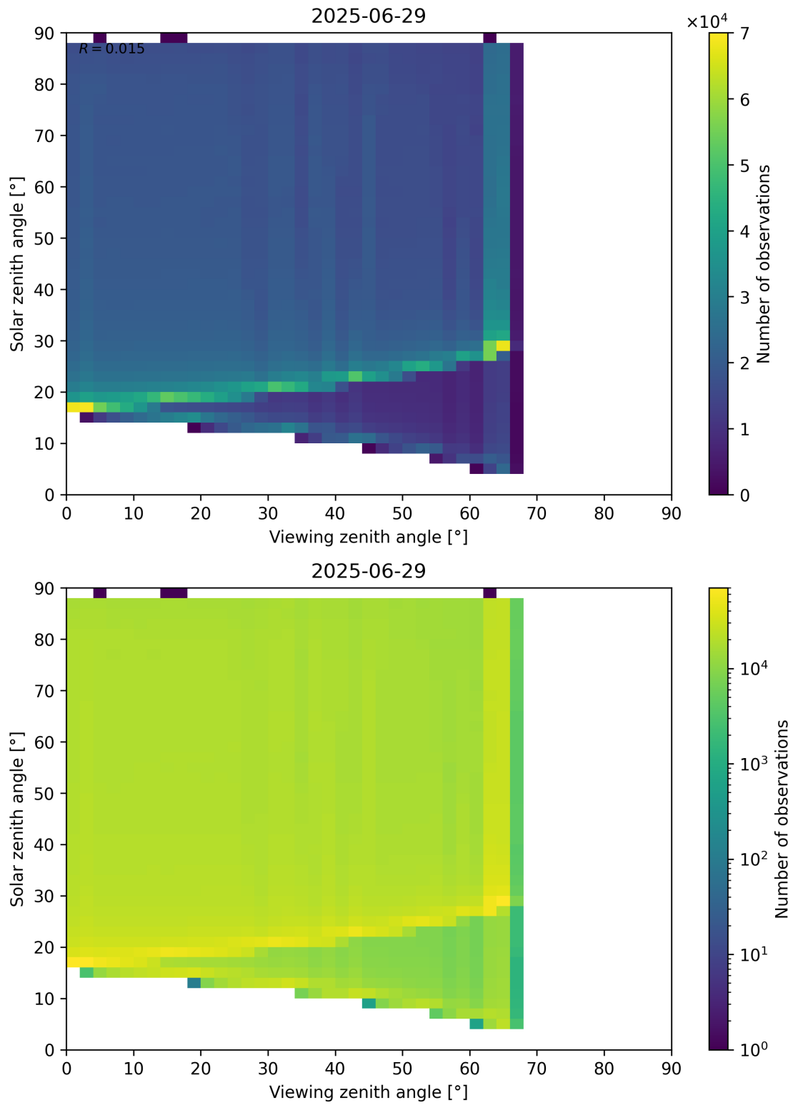
Figure 127: Scatter density plot of “Viewing zenith angle” against “Solar zenith angle” for 2025-06-28 to 2025-06-30.
