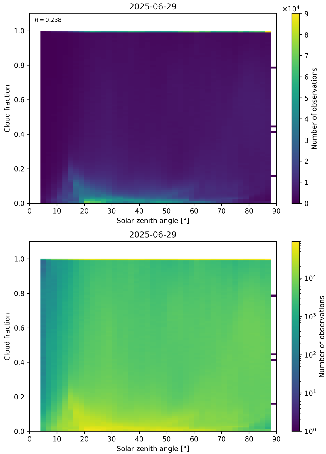
Figure 110: Scatter density plot of “Solar zenith angle” against “Cloud fraction” for 2025-06-28 to 2025-06-30.
