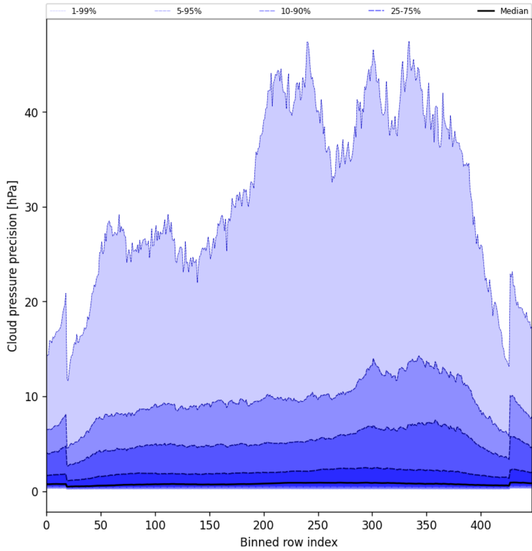
Figure 48: Along track statistics of “Cloud pressure precision” for 2025-06-28 to 2025-06-30
