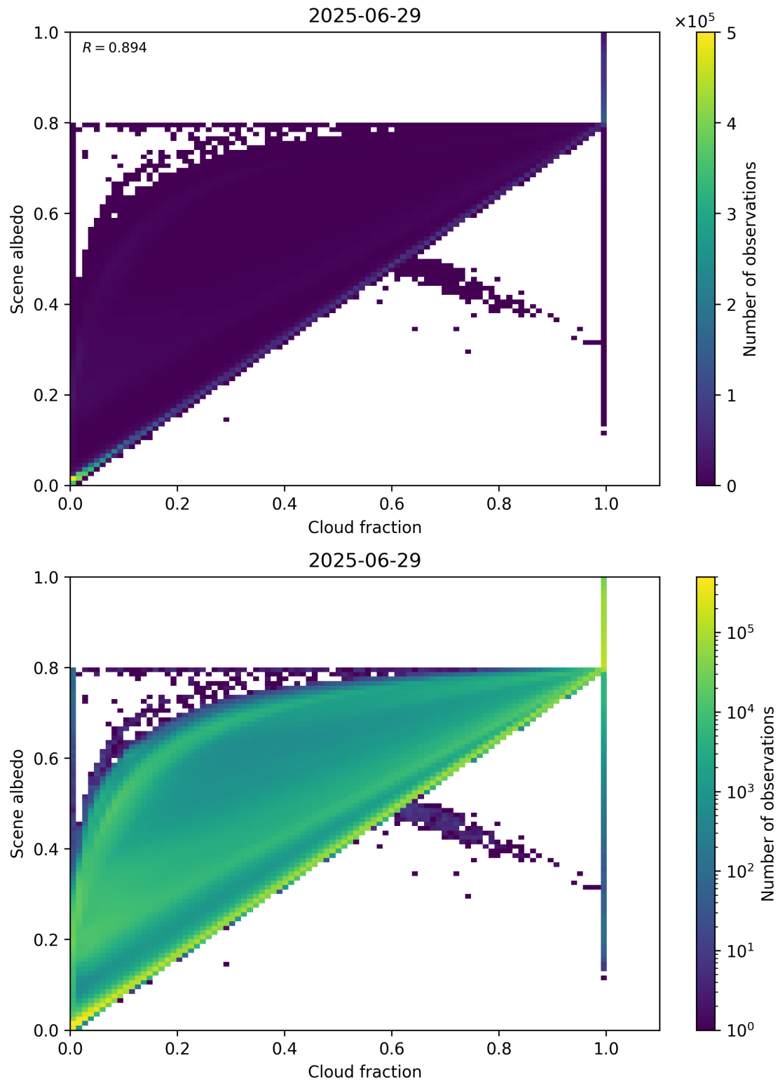
Figure 75: Scatter density plot of “Cloud fraction” against “Scene albedo” for 2025-06-28 to 2025-06-30.
