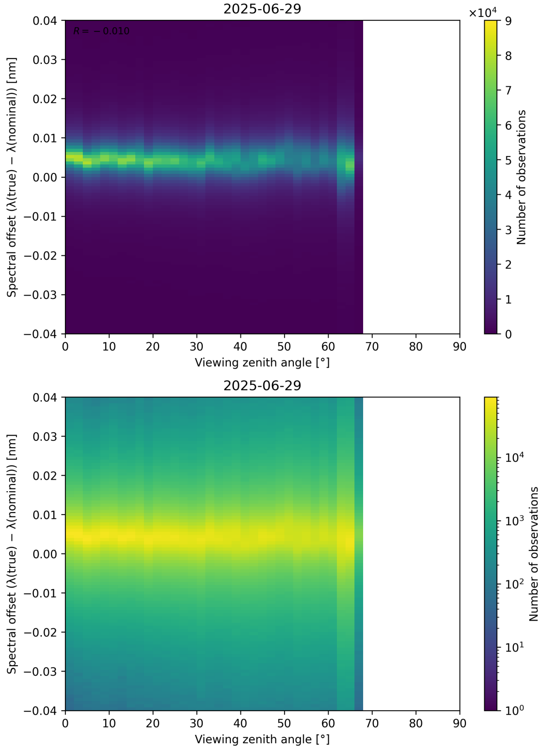
Figure 128: Scatter density plot of “Viewing zenith angle” against “Spectral offset ( \lambda_{\text{true}} - \lambda_{\text{nominal}} )” for 2025-06-28 to 2025-06-30.
