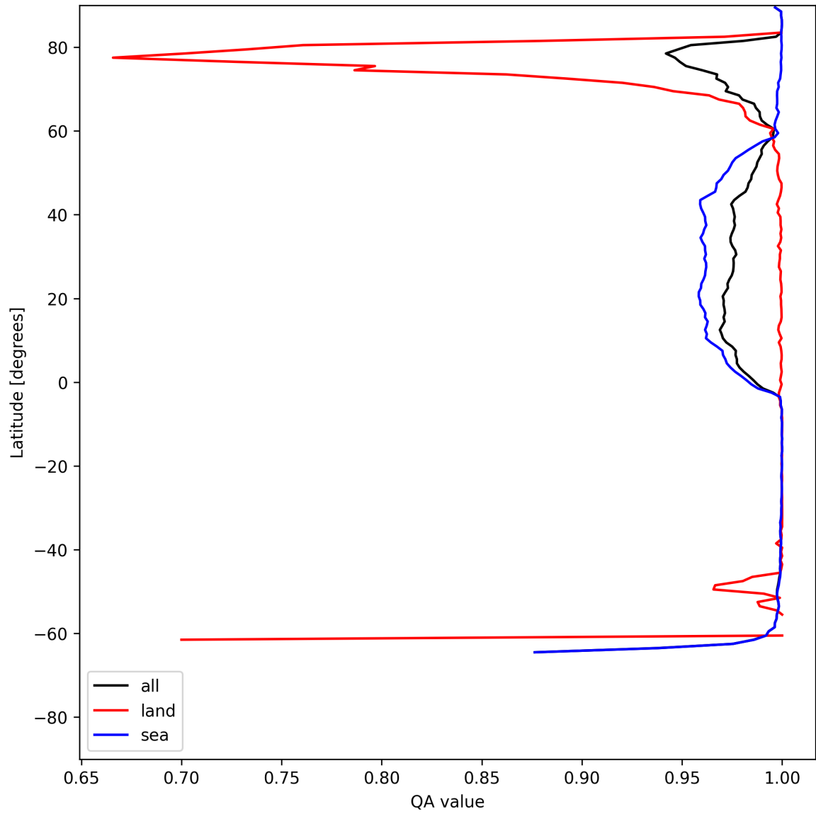
Figure 12: Zonal average of “QA value” for 2025-06-28 to 2025-06-30.
