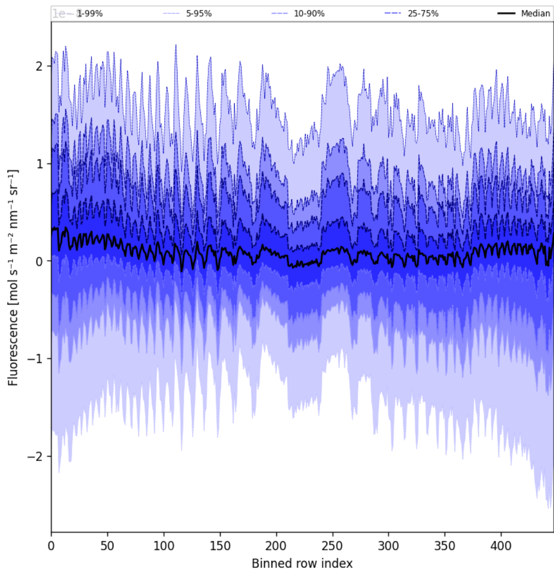
Figure 57: Along track statistics of “Fluorescence” for 2025-06-28 to 2025-06-30
