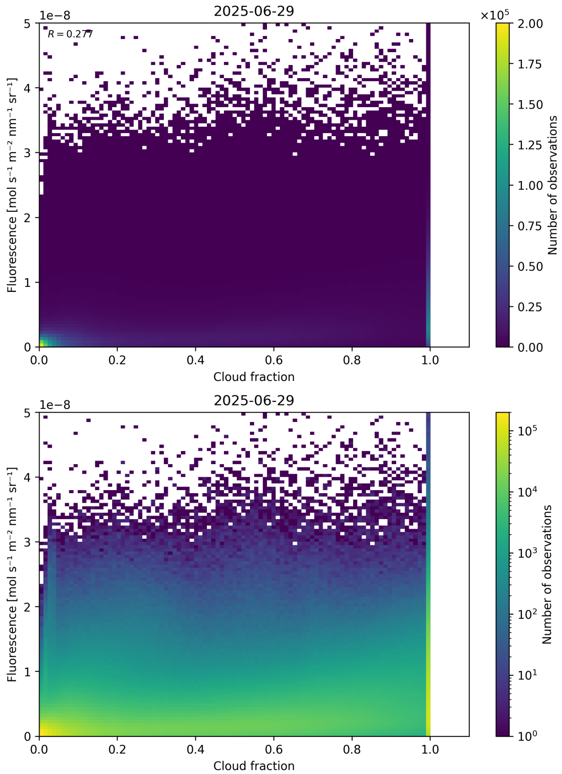
Figure 72: Scatter density plot of “Cloud fraction” against “Fluorescence” for 2025-06-28 to 2025-06-30.
