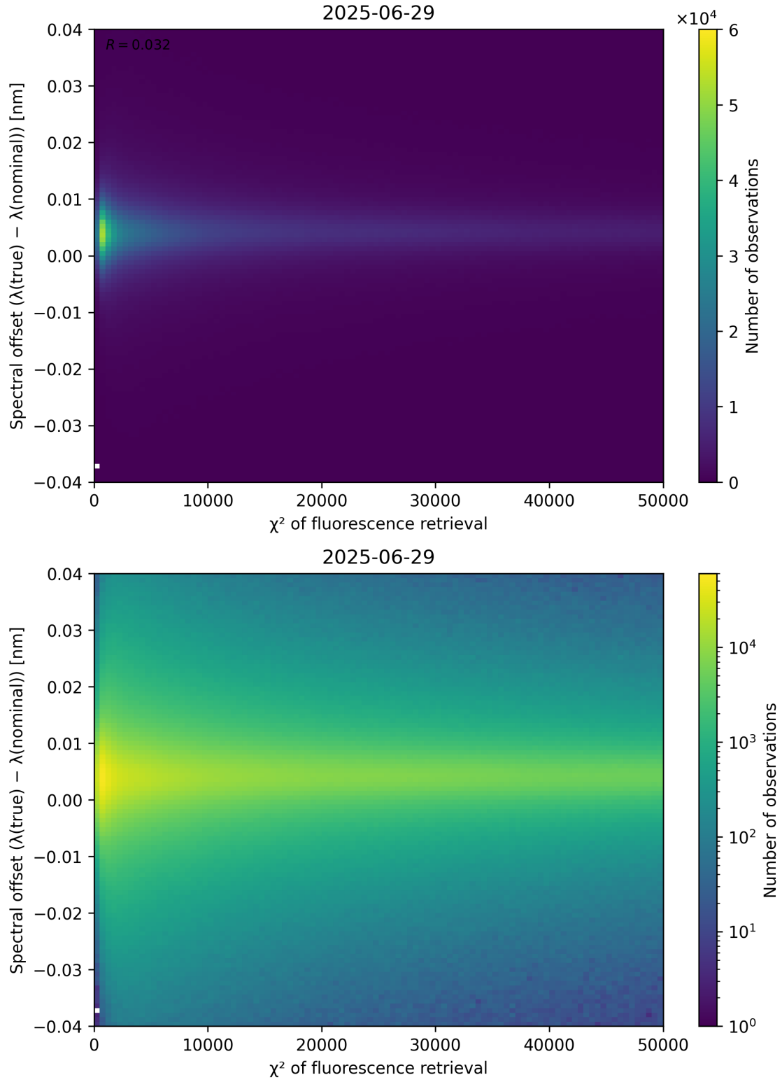
Figure 69: Scatter density plot of “ \chi^2 of fluorescence retrieval” against “Spectral offset ( \lambda_{\text{true}} - \lambda_{\text{nominal}} )” for 2025-06-28 to 2025-06-30.
