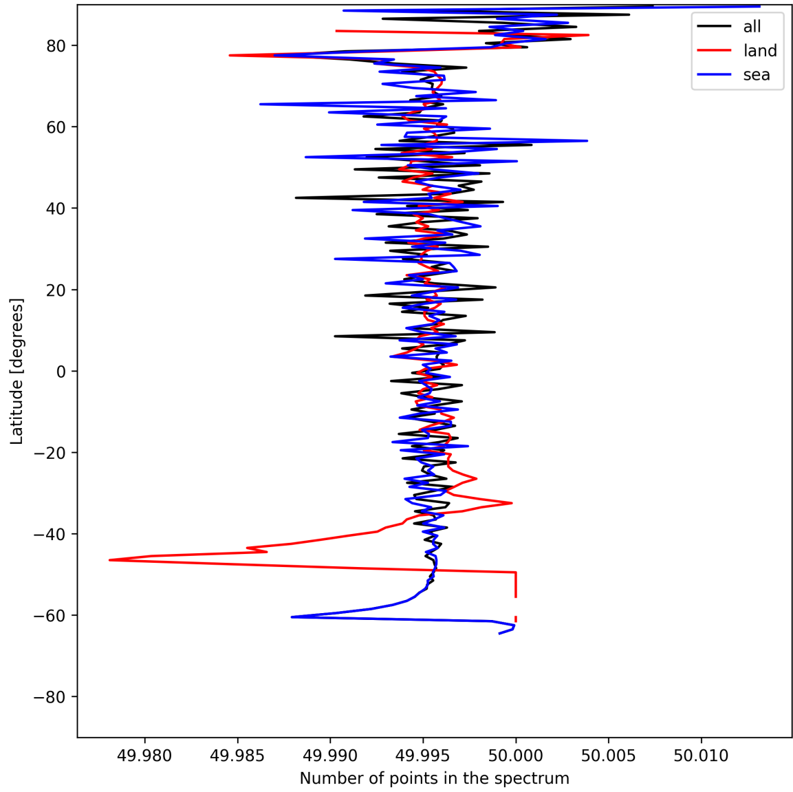
Figure 27: Zonal average of “Number of points in the spectrum” for 2025-06-28 to 2025-06-30.
