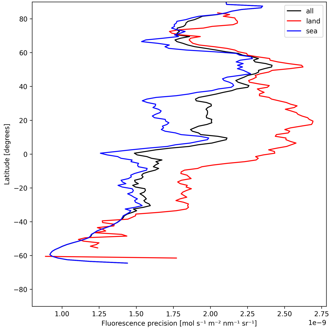
Figure 24: Zonal average of “Fluorescence precision” for 2025-06-28 to 2025-06-30.
