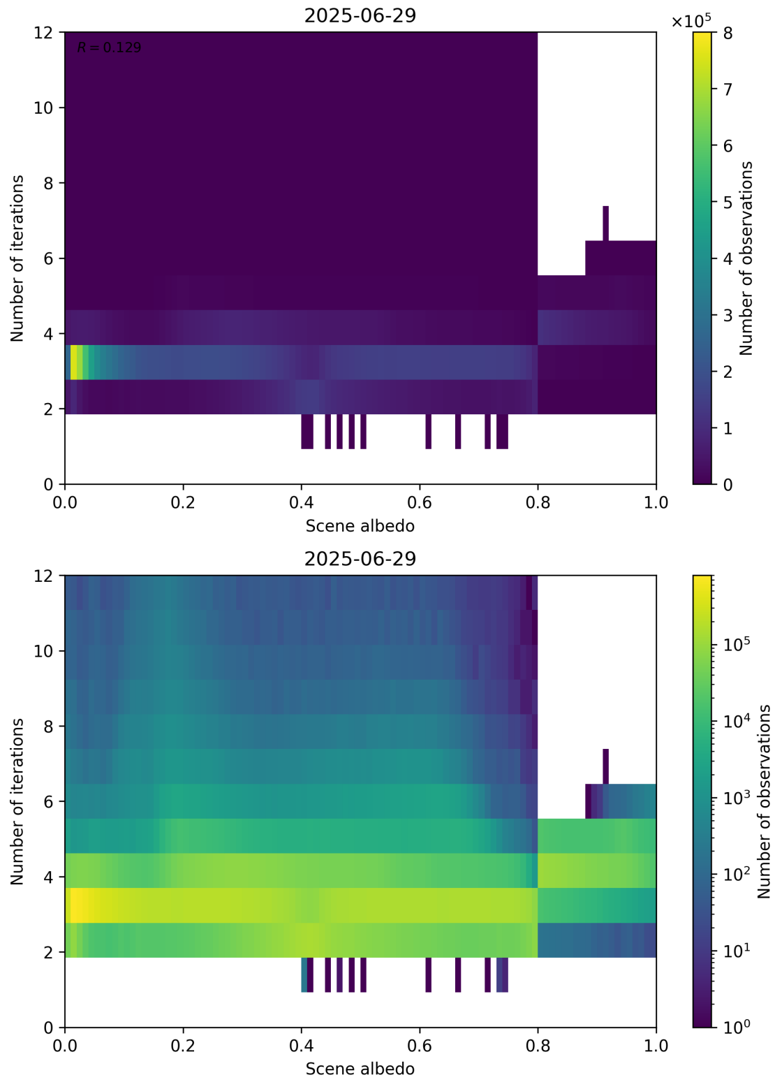
Figure 105: Scatter density plot of “Scene albedo” against “Number of iterations” for 2025-06-28 to 2025-06-30.
