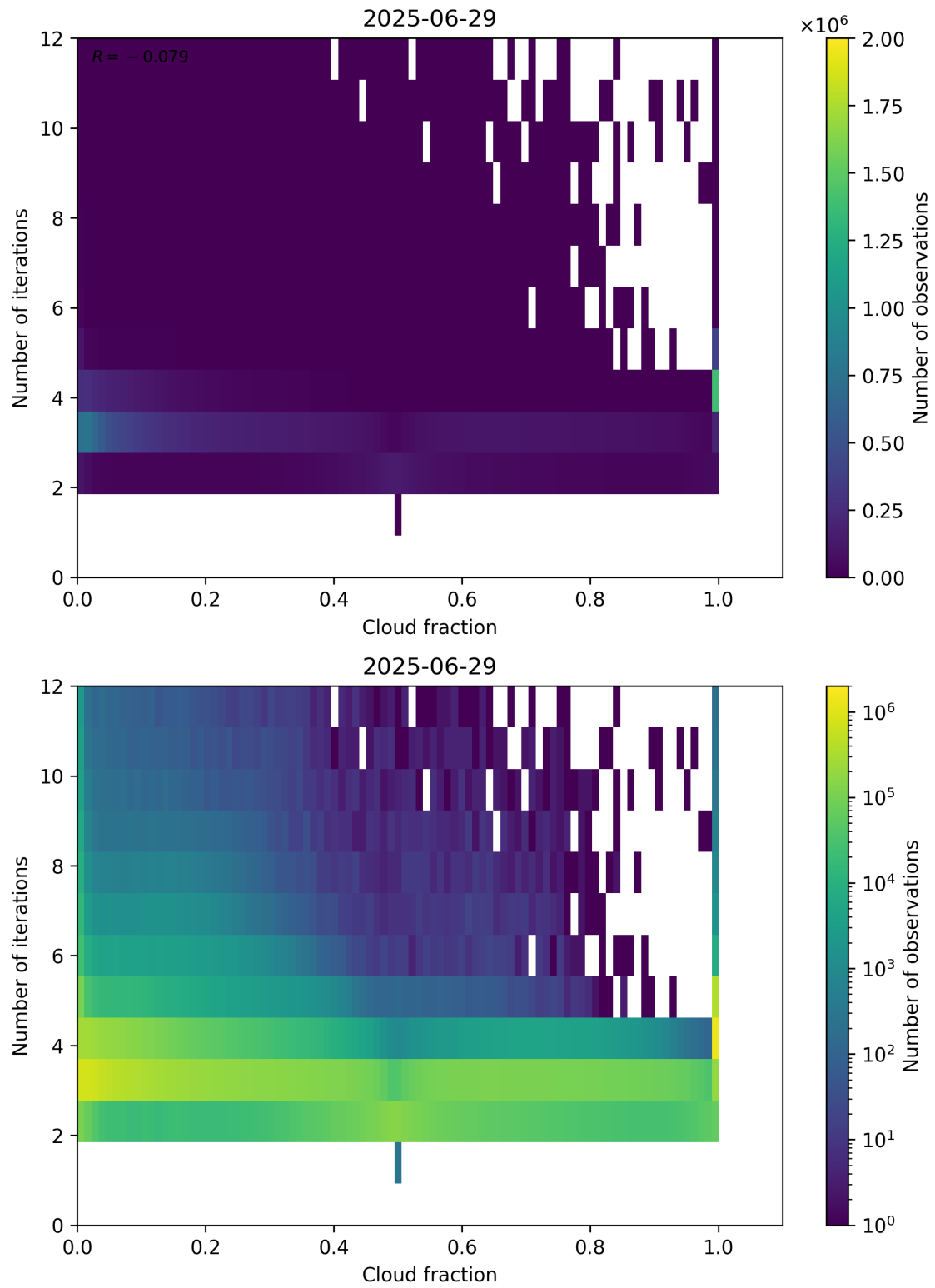
Figure 73: Scatter density plot of “Cloud fraction” against “Number of iterations” for 2025-06-28 to 2025-06-30.
