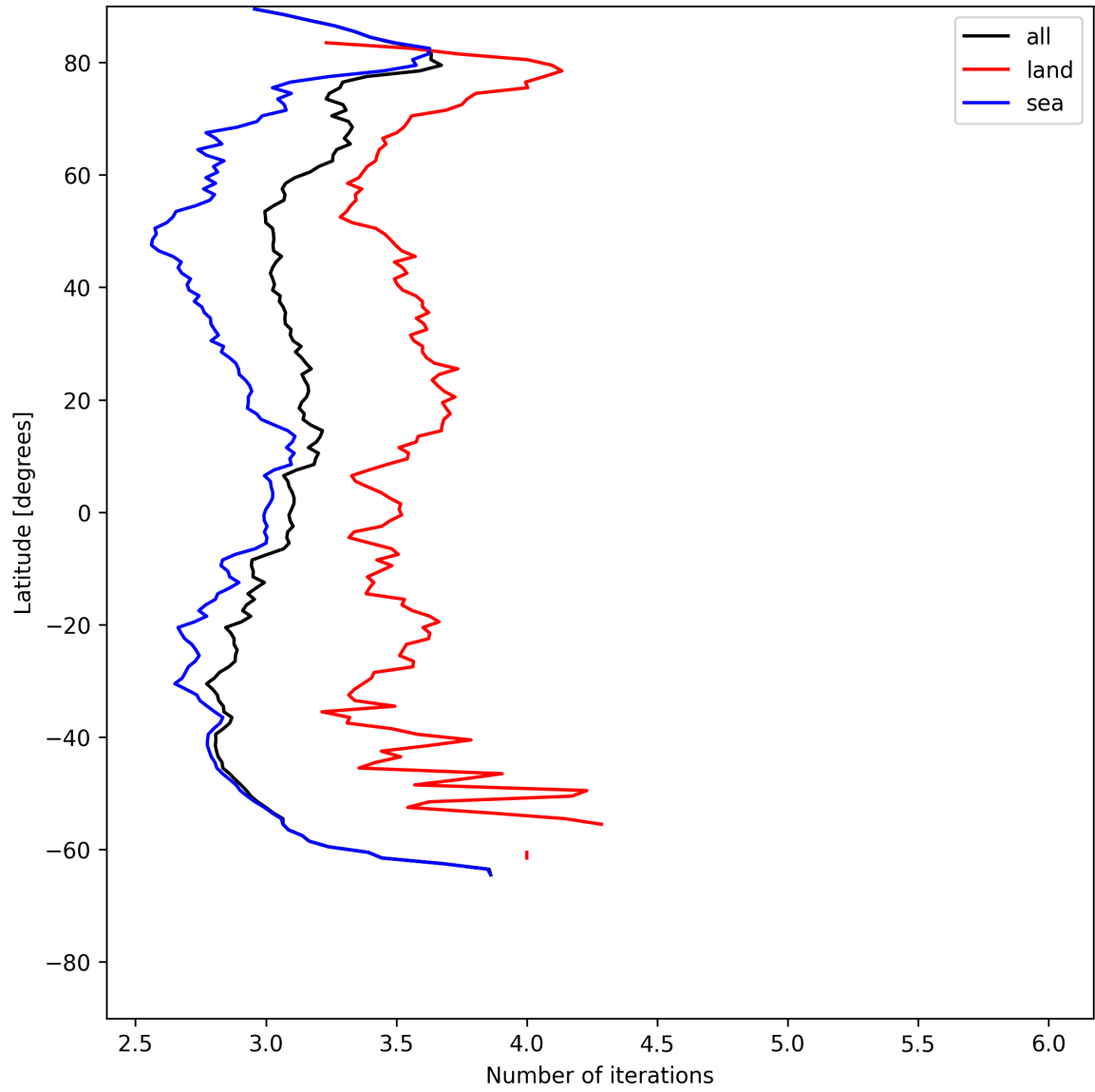
Figure 22: Zonal average of “Number of iterations” for 2025-06-28 to 2025-06-30.
