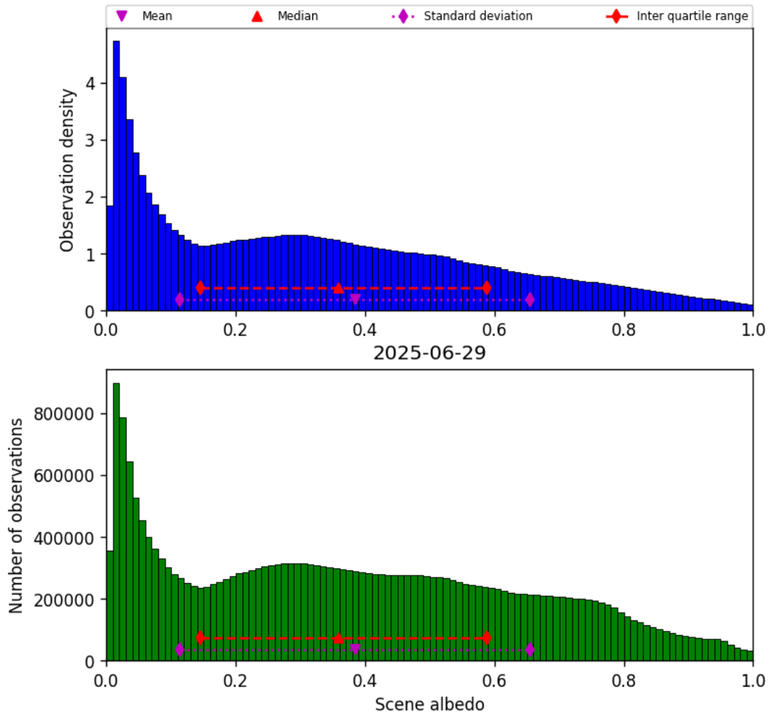
Figure 34: Histogram of “Scene albedo” for 2025-06-28 to 2025-06-30
