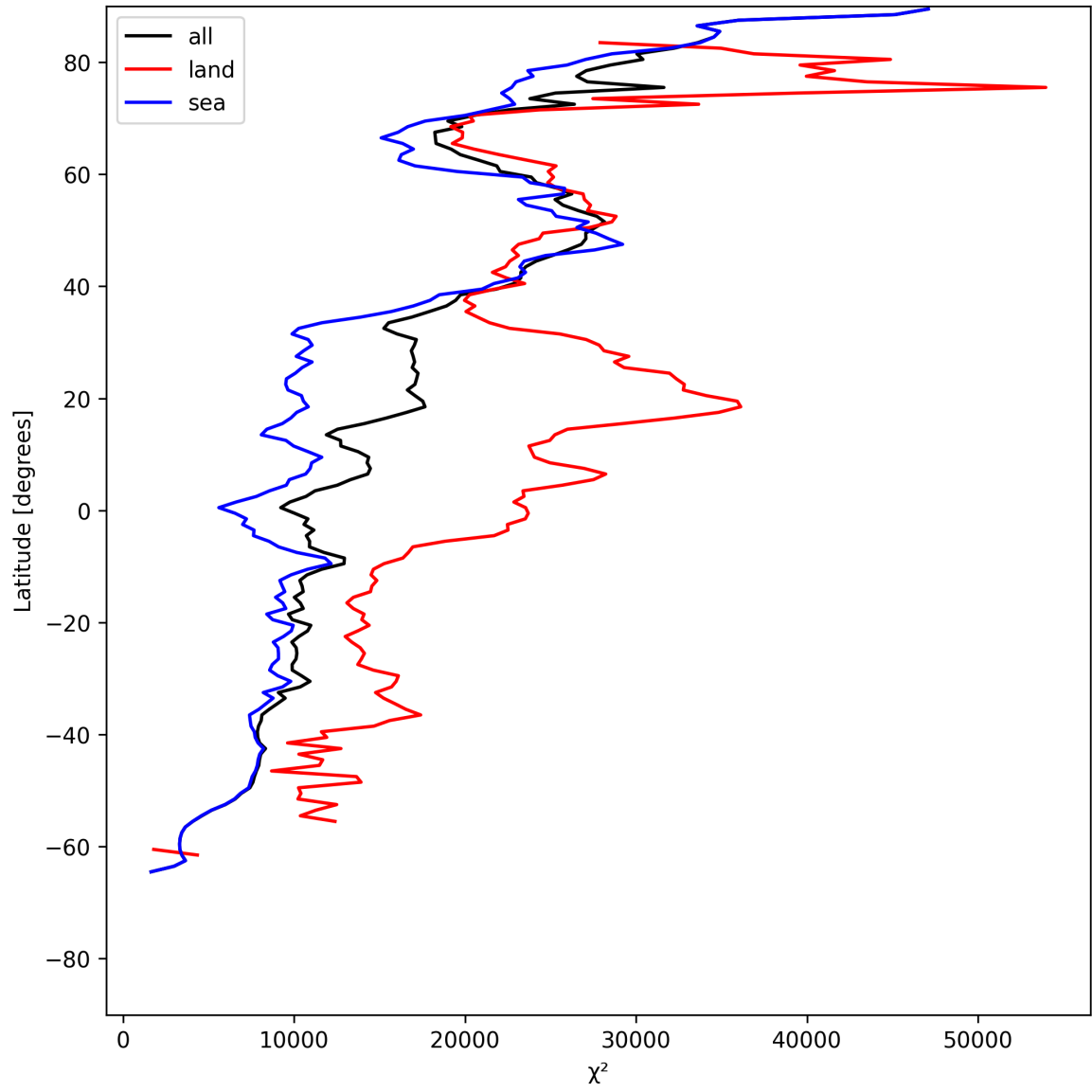
Figure 21: Zonal average of “ \chi^2 ” for 2025-06-28 to 2025-06-30.
