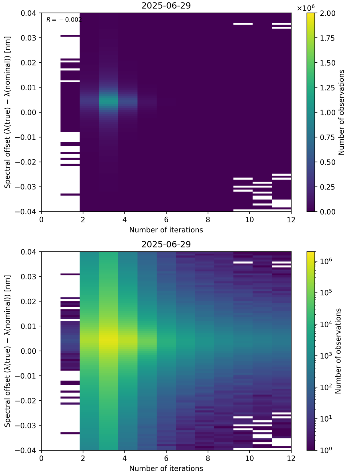
Figure 100: Scatter density plot of “Number of iterations” against “Spectral offset ( \lambda_{\text{true}} - \lambda_{\text{nominal}} )” for 2025-06-28 to 2025-06-30.
