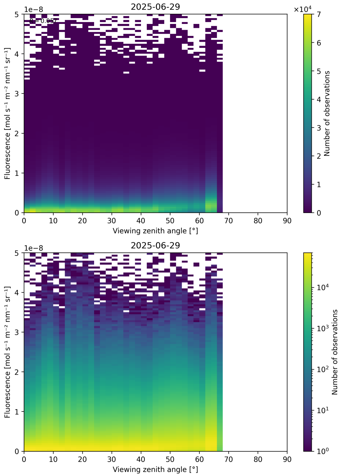
Figure 122: Scatter density plot of “Viewing zenith angle” against “Fluorescence” for 2025-06-28 to 2025-06-30.
