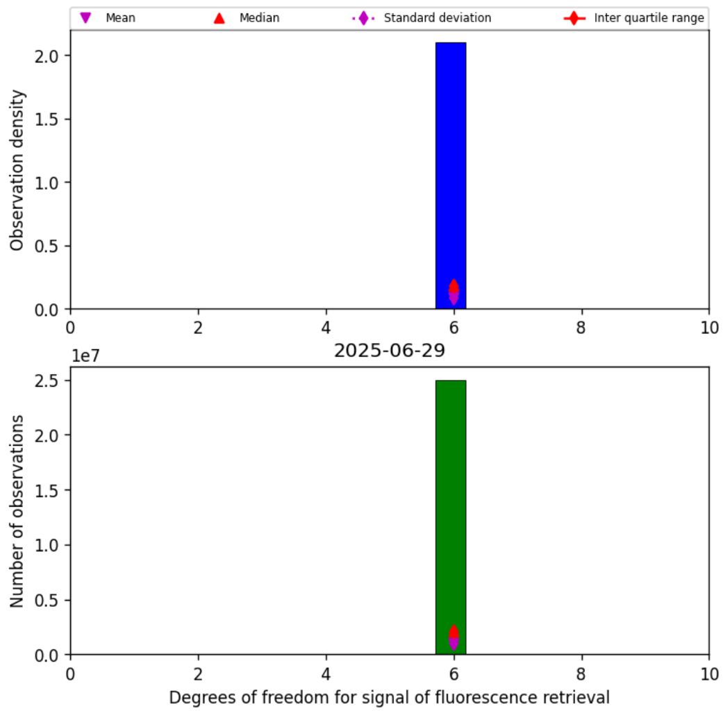
Figure 43: Histogram of "Degrees of freedom for signal of fluorescence retrieval" for 2025-06-28 to 2025-06-30
