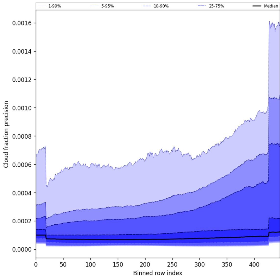
Figure 50: Along track statistics of “Cloud fraction precision” for 2025-06-28 to 2025-06-30
