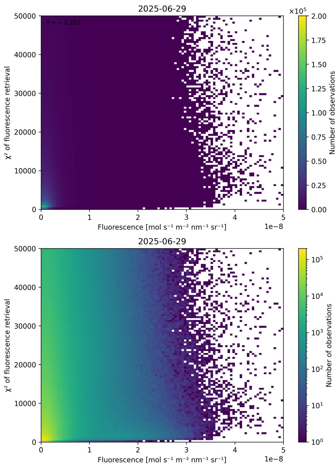
Figure 85: Scatter density plot of “Fluorescence” against “ \chi^2 of fluorescence retrieval” for 2025-06-28 to 2025-06-30.
