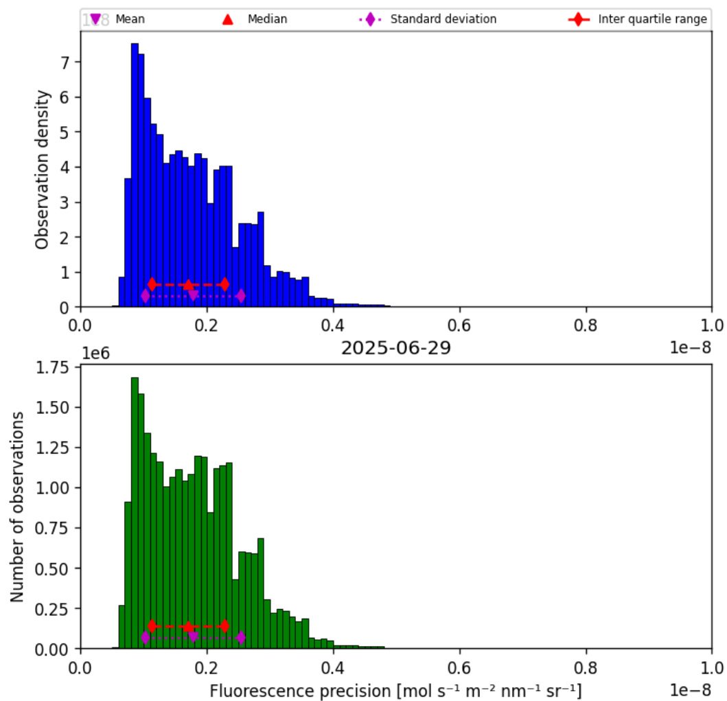
Figure 41: Histogram of “Fluorescence precision” for 2025-06-28 to 2025-06-30
