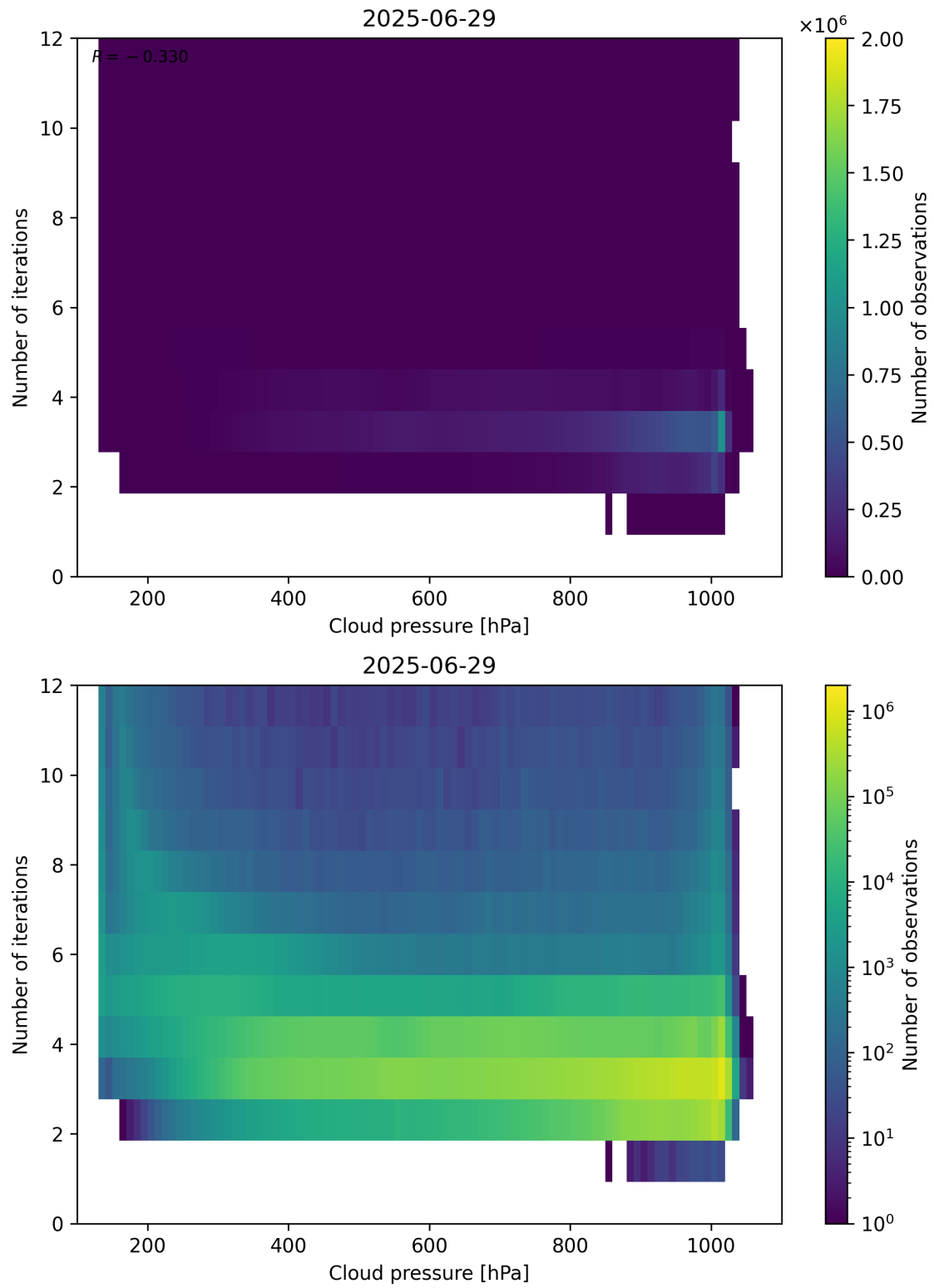
Figure 81: Scatter density plot of “Cloud pressure” against “Number of iterations” for 2025-06-28 to 2025-06-30.
