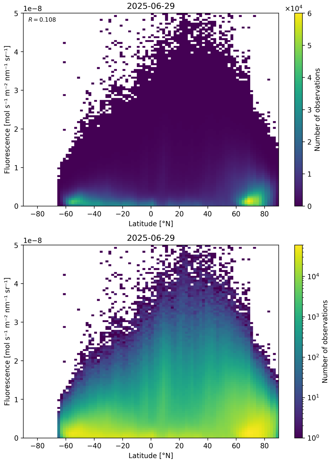
Figure 92: Scatter density plot of “Latitude” against “Fluorescence” for 2025-06-28 to 2025-06-30.
