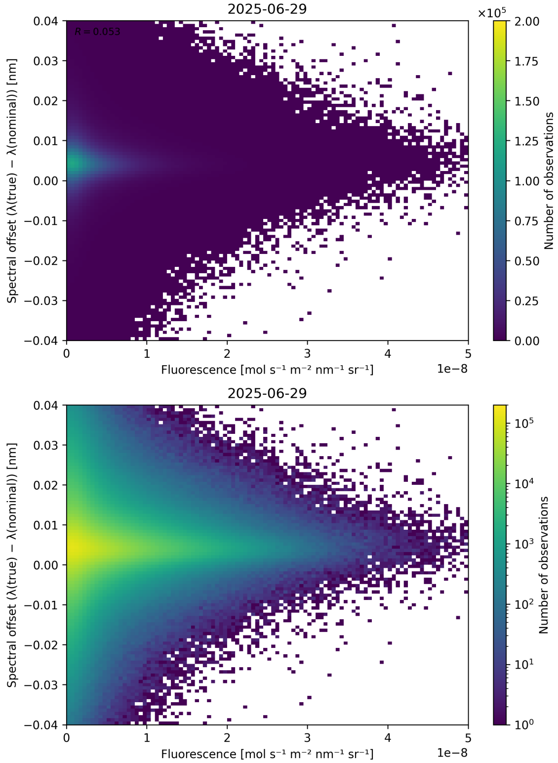
Figure 87: Scatter density plot of “Fluorescence” against “Spectral offset ( \lambda_{\text{true}} - \lambda_{\text{nominal}} )” for 2025-06-28 to 2025-06-30.
