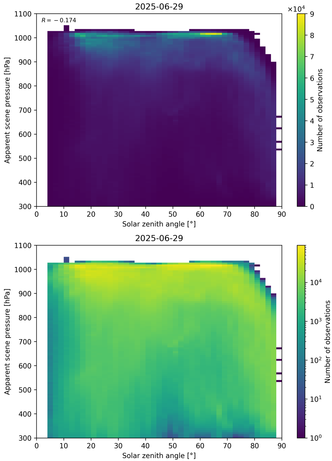
Figure 108: Scatter density plot of “Solar zenith angle” against “Apparent scene pressure” for 2025-06-28 to 2025-06-30.
