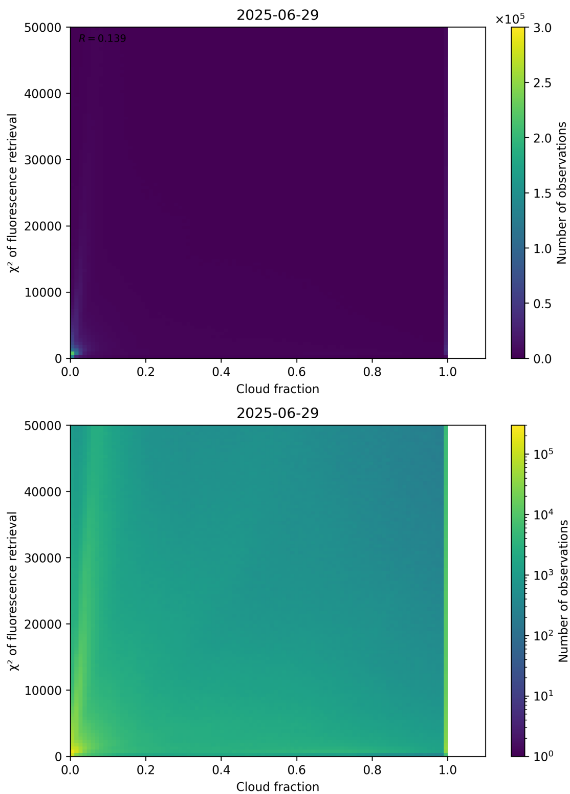
Figure 71: Scatter density plot of “Cloud fraction” against “ \chi^2 of fluorescence retrieval” for 2025-06-28 to 2025-06-30.
