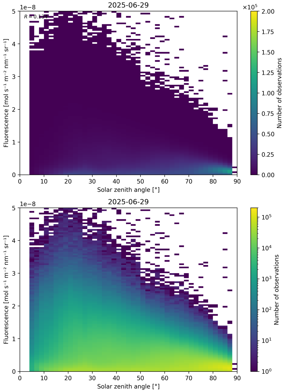
Figure 112: Scatter density plot of “Solar zenith angle” against “Fluorescence” for 2025-06-28 to 2025-06-30.
