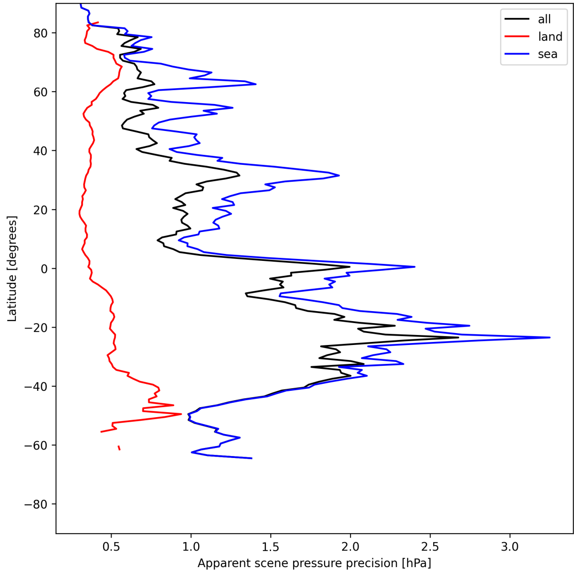
Figure 20: Zonal average of “Apparent scene pressure precision” for 2025-06-28 to 2025-06-30.
