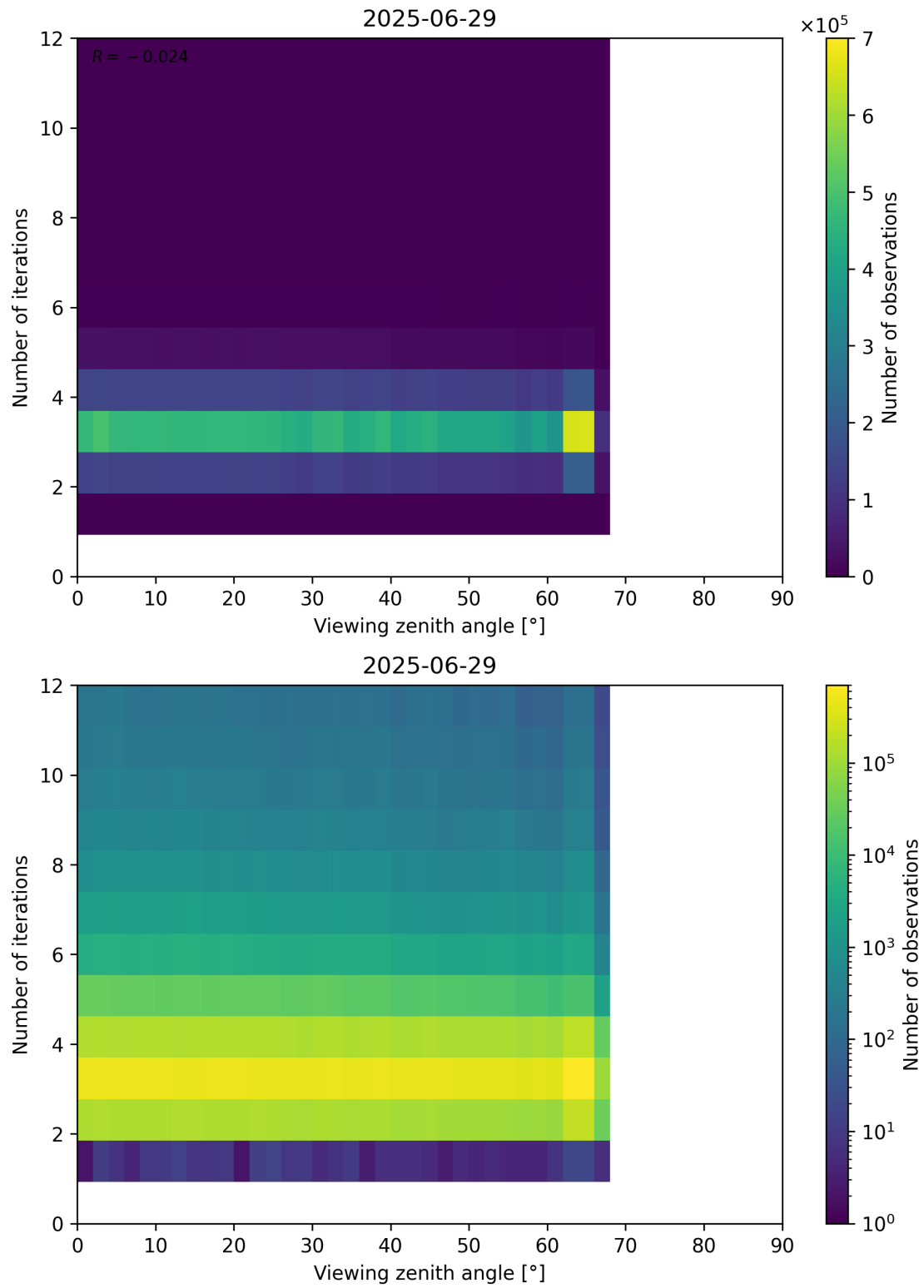
Figure 124: Scatter density plot of “Viewing zenith angle” against “Number of iterations” for 2025-06-28 to 2025-06-30.
