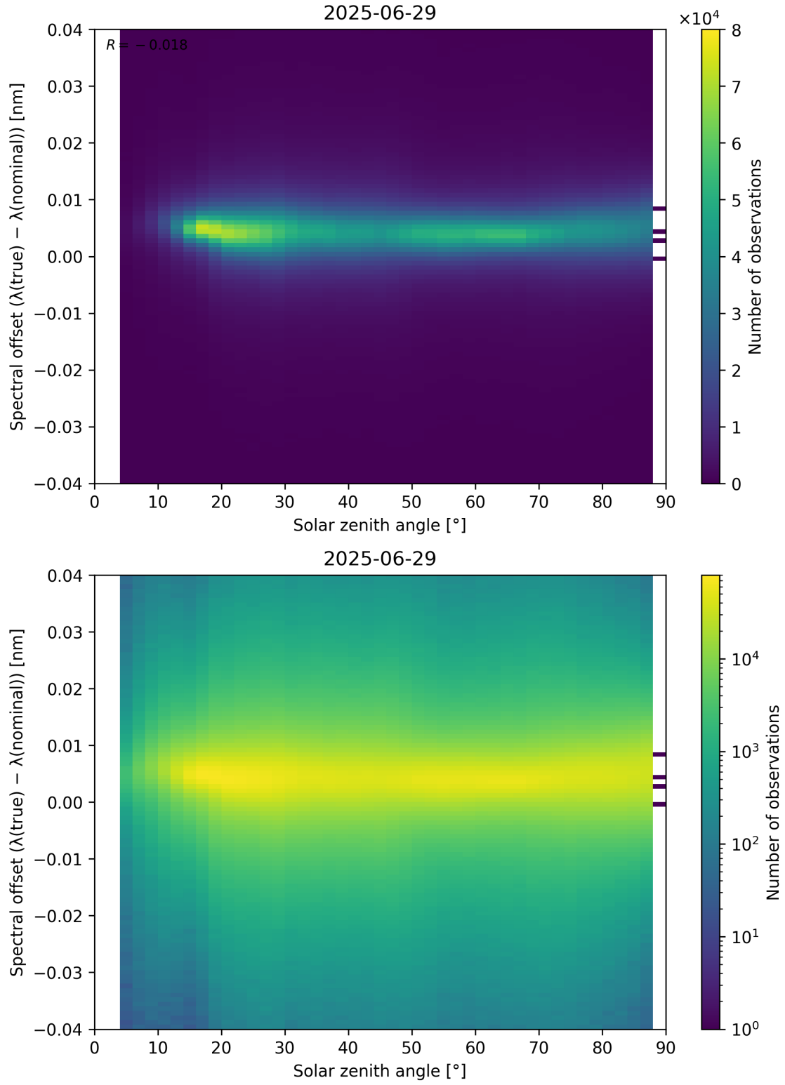
Figure 117: Scatter density plot of “Solar zenith angle” against “Spectral offset ( \lambda_{\text{true}} - \lambda_{\text{nominal}} )” for 2025-06-28 to 2025-06-30.
