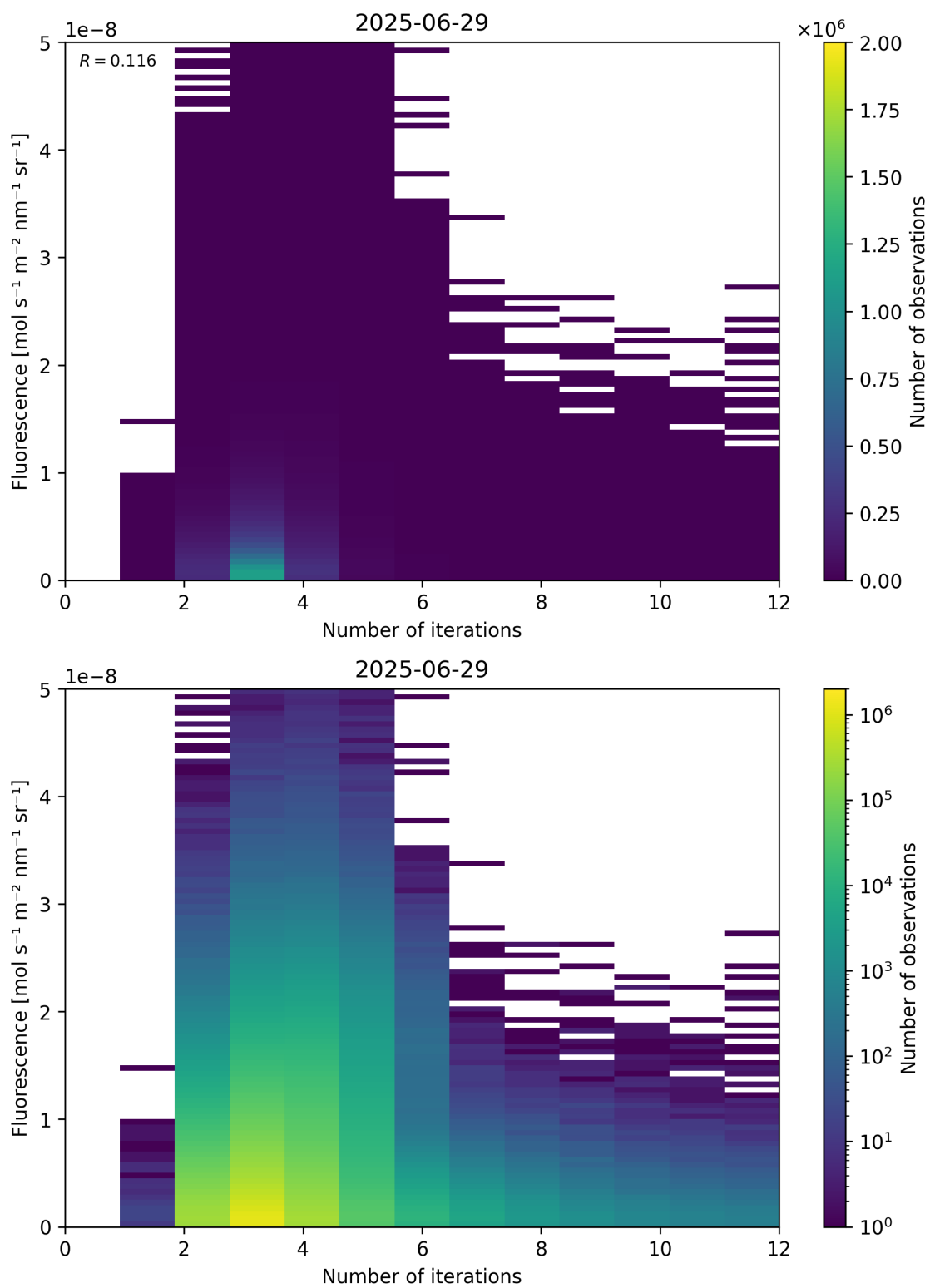
Figure 98: Scatter density plot of “Number of iterations” against “Fluorescence” for 2025-06-28 to 2025-06-30.
