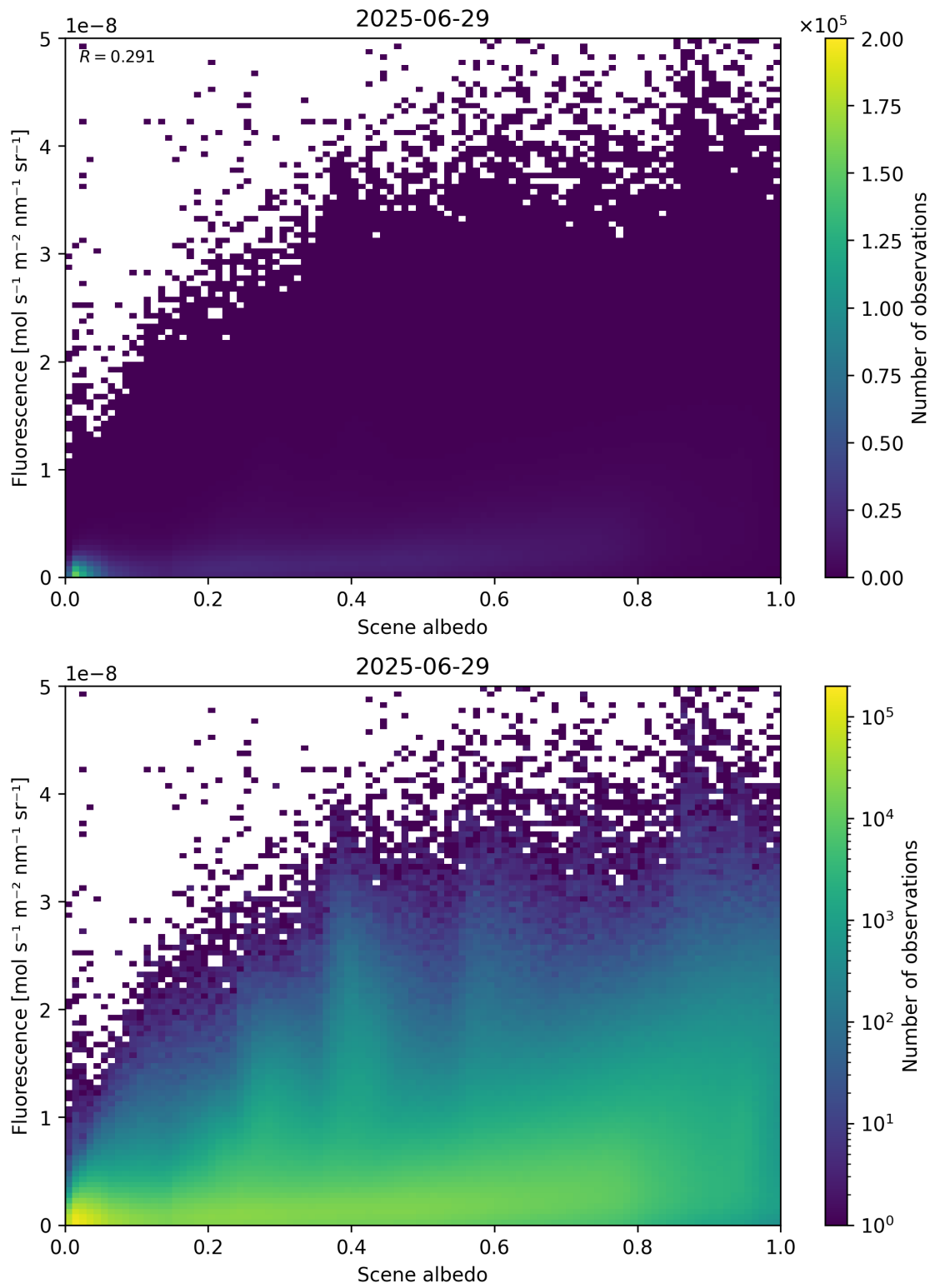
Figure 104: Scatter density plot of “Scene albedo” against “Fluorescence” for 2025-06-28 to 2025-06-30.
