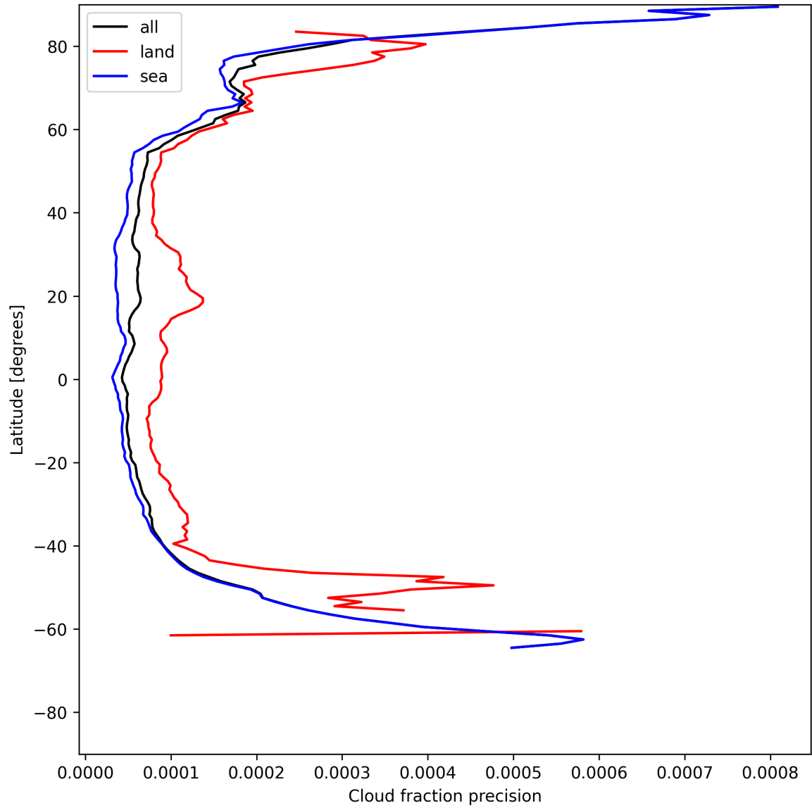
Figure 16: Zonal average of “Cloud fraction precision” for 2025-06-28 to 2025-06-30.
