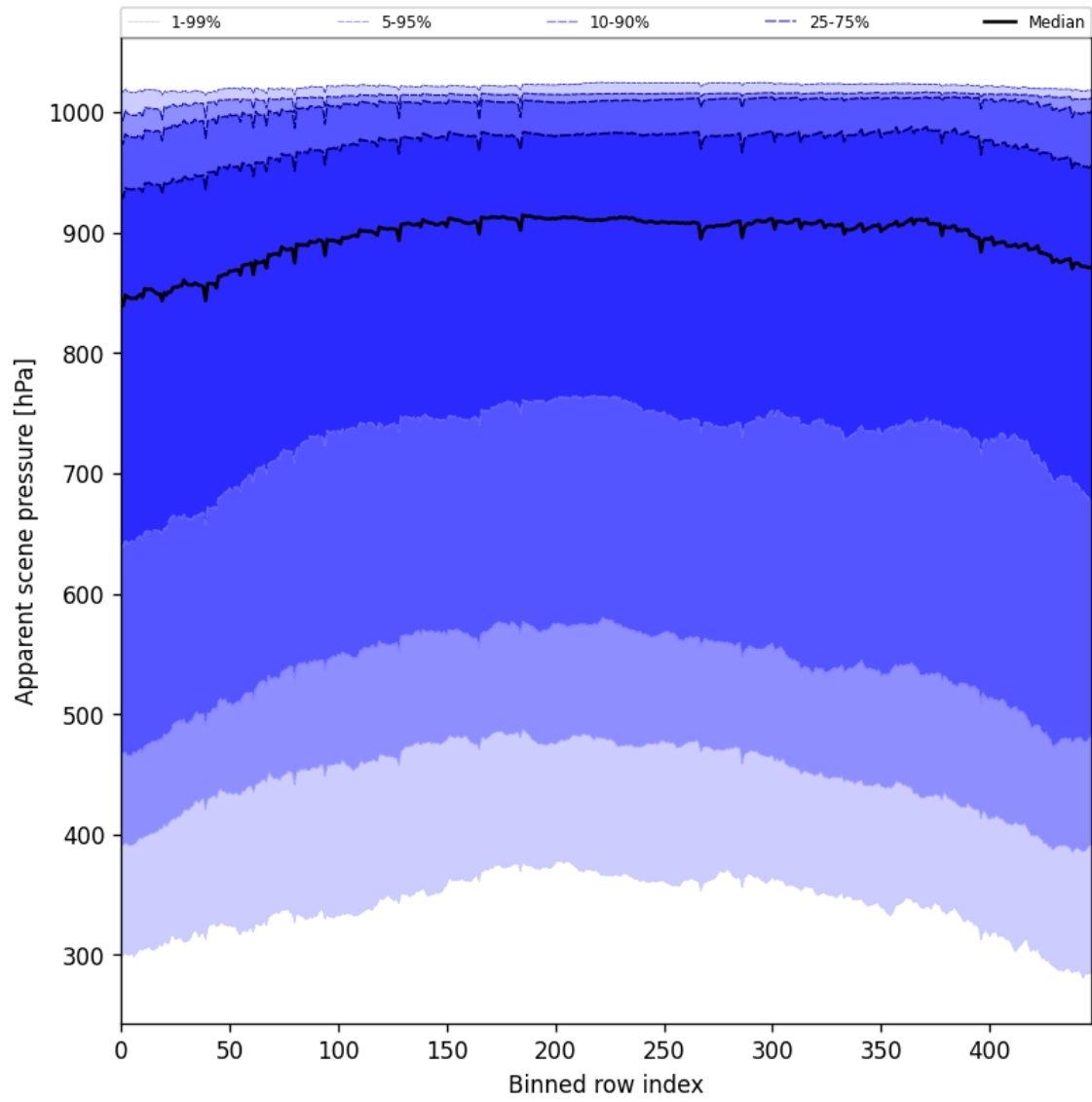
Figure 53: Along track statistics of “Apparent scene pressure” for 2025-06-28 to 2025-06-30
