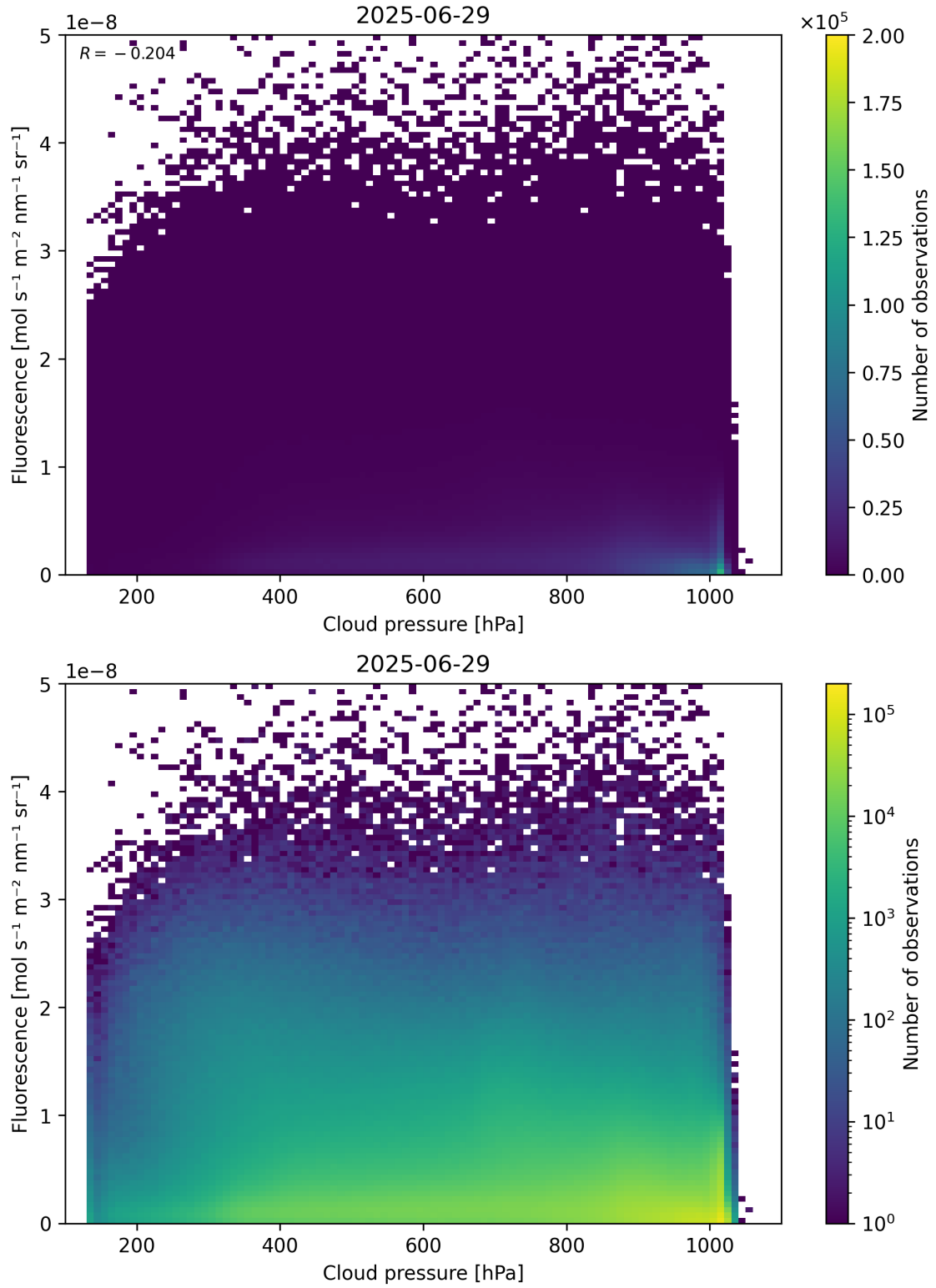
Figure 80: Scatter density plot of “Cloud pressure” against “Fluorescence” for 2025-06-28 to 2025-06-30.
