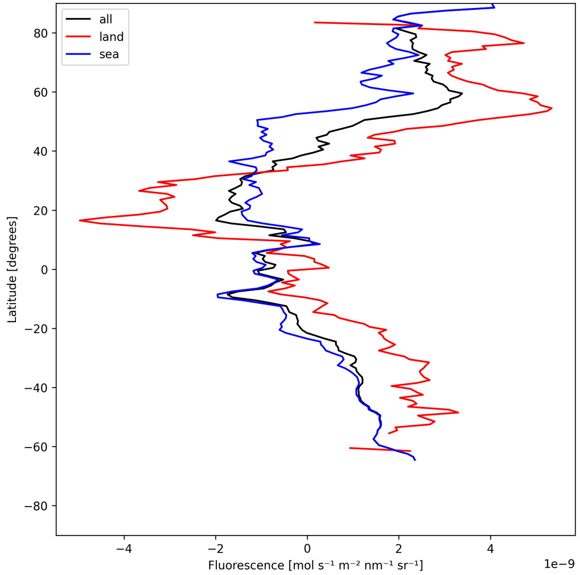
Figure 23: Zonal average of “Fluorescence” for 2025-06-28 to 2025-06-30.
