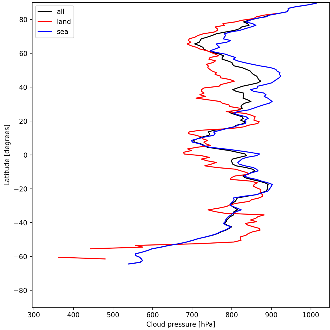
Figure 13: Zonal average of “Cloud pressure” for 2025-06-28 to 2025-06-30.
