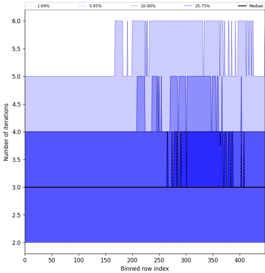
Figure 56: Along track statistics of “Number of iterations” for 2025-06-28 to 2025-06-30
