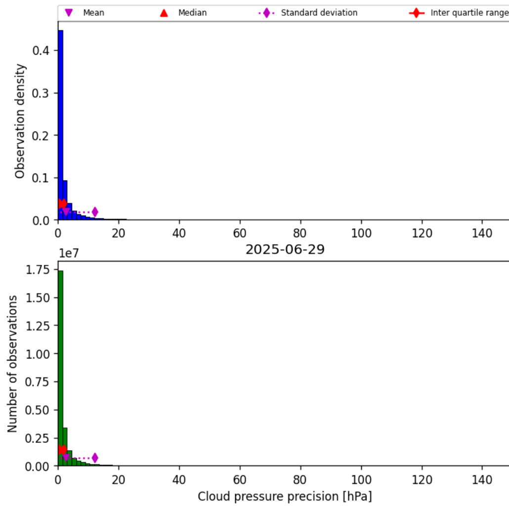
Figure 31: Histogram of “Cloud pressure precision” for 2025-06-28 to 2025-06-30
