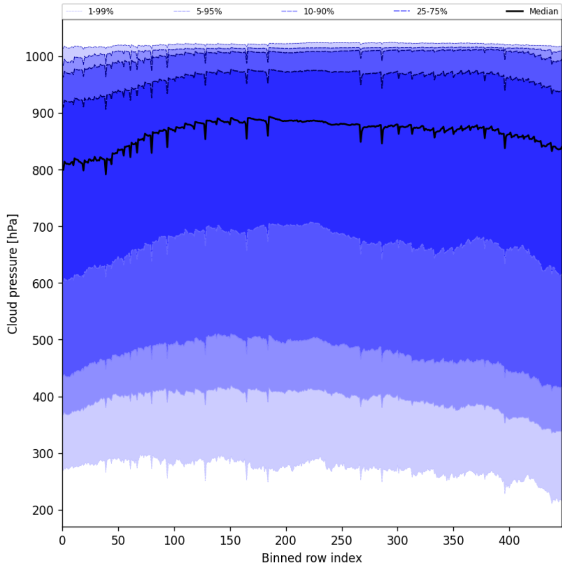
Figure 47: Along track statistics of “Cloud pressure” for 2025-06-28 to 2025-06-30
