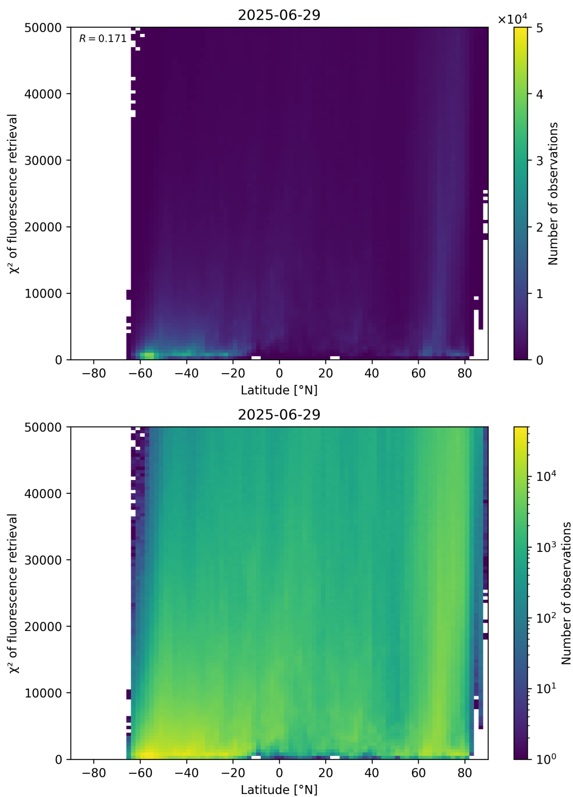
Figure 89: Scatter density plot of “Latitude” against “ \chi^2 of fluorescence retrieval” for 2025-06-28 to 2025-06-30.
