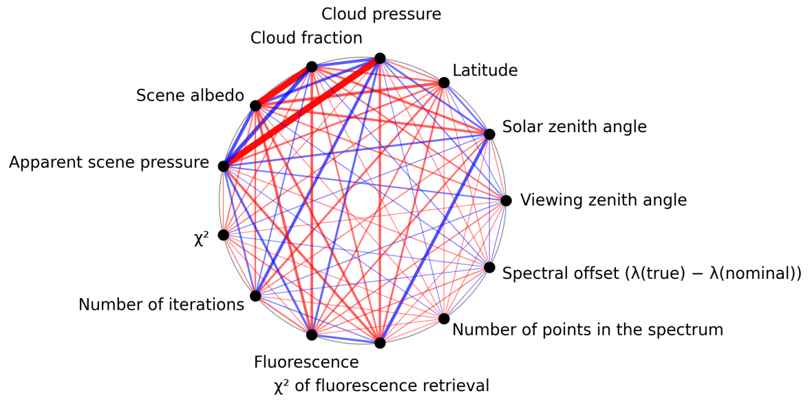
Figure 1: Map of correlation graph for 2025-06-28 to 2025-06-30.
