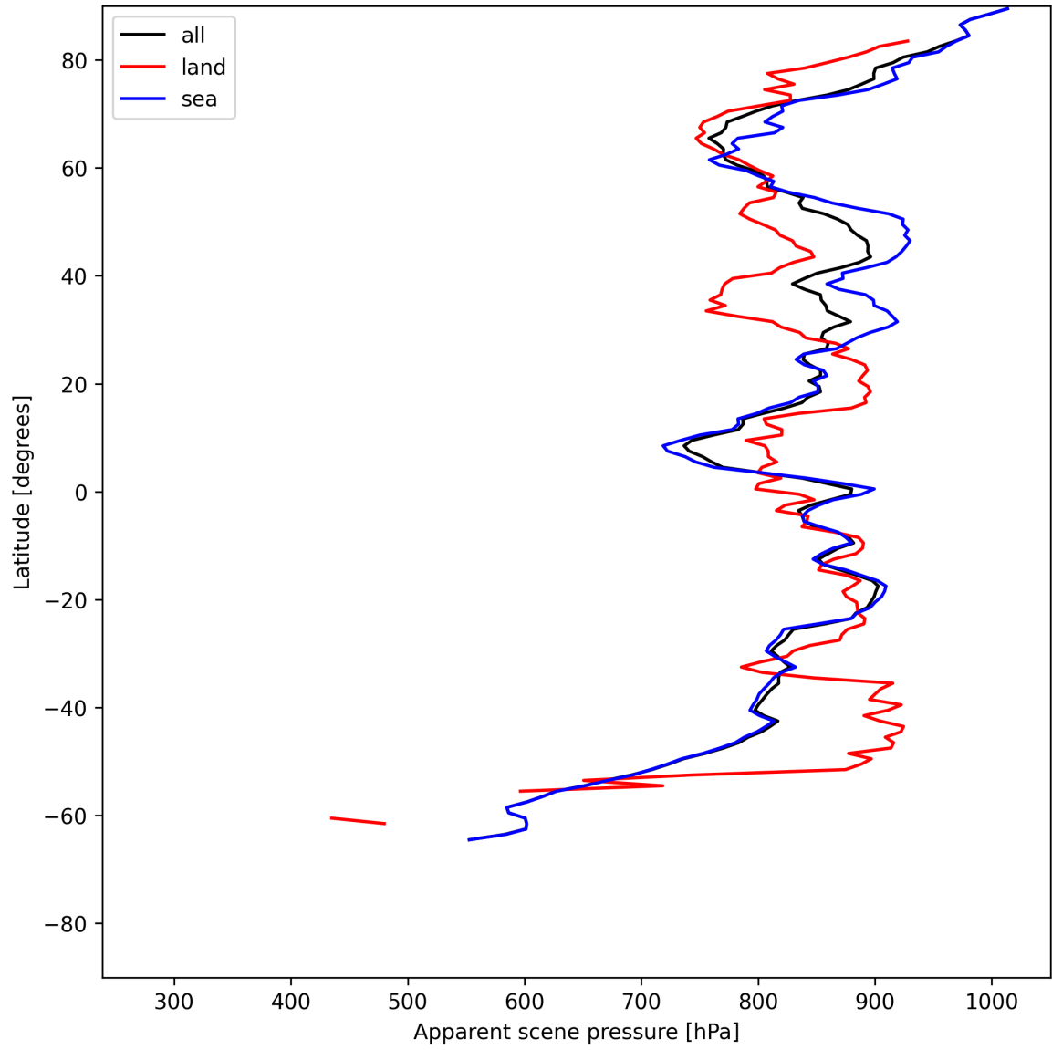
Figure 19: Zonal average of “Apparent scene pressure” for 2025-06-28 to 2025-06-30.
