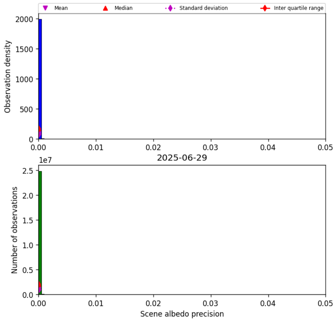
Figure 35: Histogram of “Scene albedo precision” for 2025-06-28 to 2025-06-30
