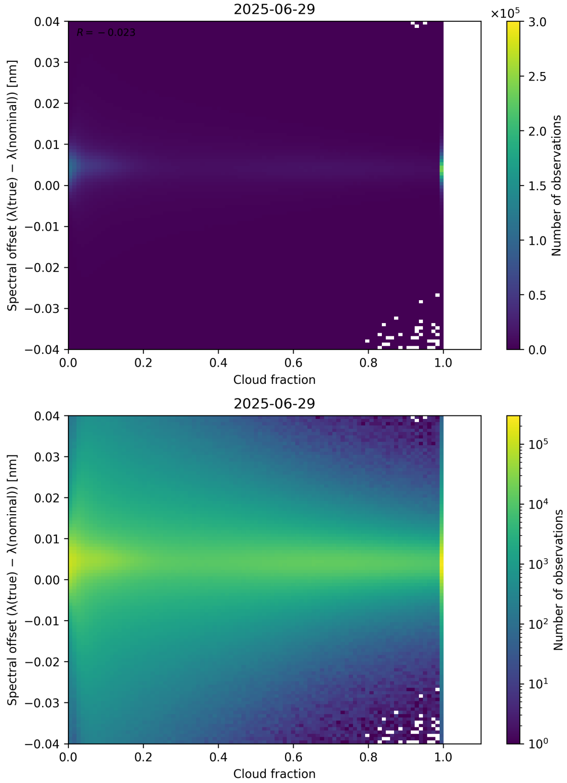
Figure 76: Scatter density plot of “Cloud fraction” against “Spectral offset ( \lambda_{\text{true}} - \lambda_{\text{nominal}} )” for 2025-06-28 to 2025-06-30.
