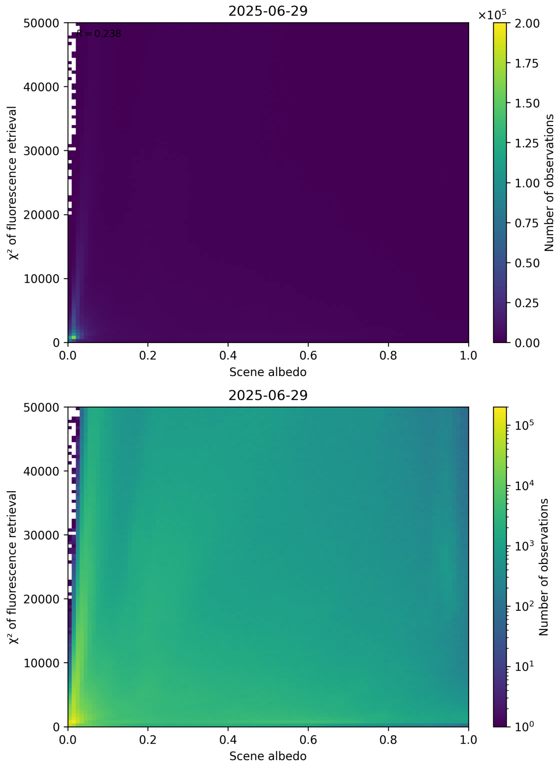
Figure 103: Scatter density plot of “Scene albedo” against “ \chi^2 of fluorescence retrieval” for 2025-06-28 to 2025-06-30.
