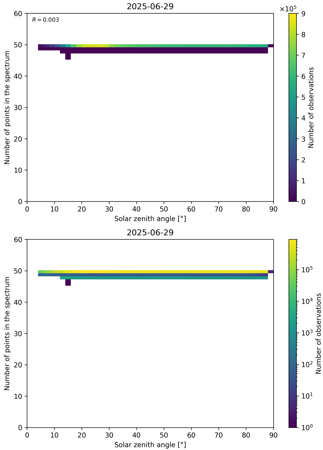
Figure 115: Scatter density plot of “Solar zenith angle” against “Number of points in the spectrum” for 2025-06-28 to 2025-06-30.
