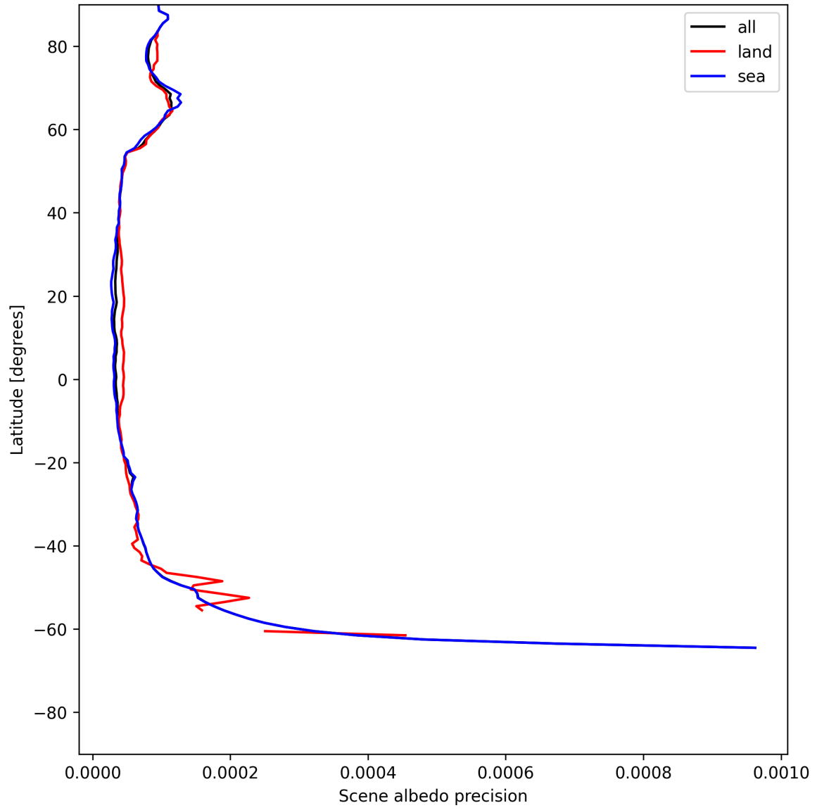
Figure 18: Zonal average of “Scene albedo precision” for 2025-06-28 to 2025-06-30.
