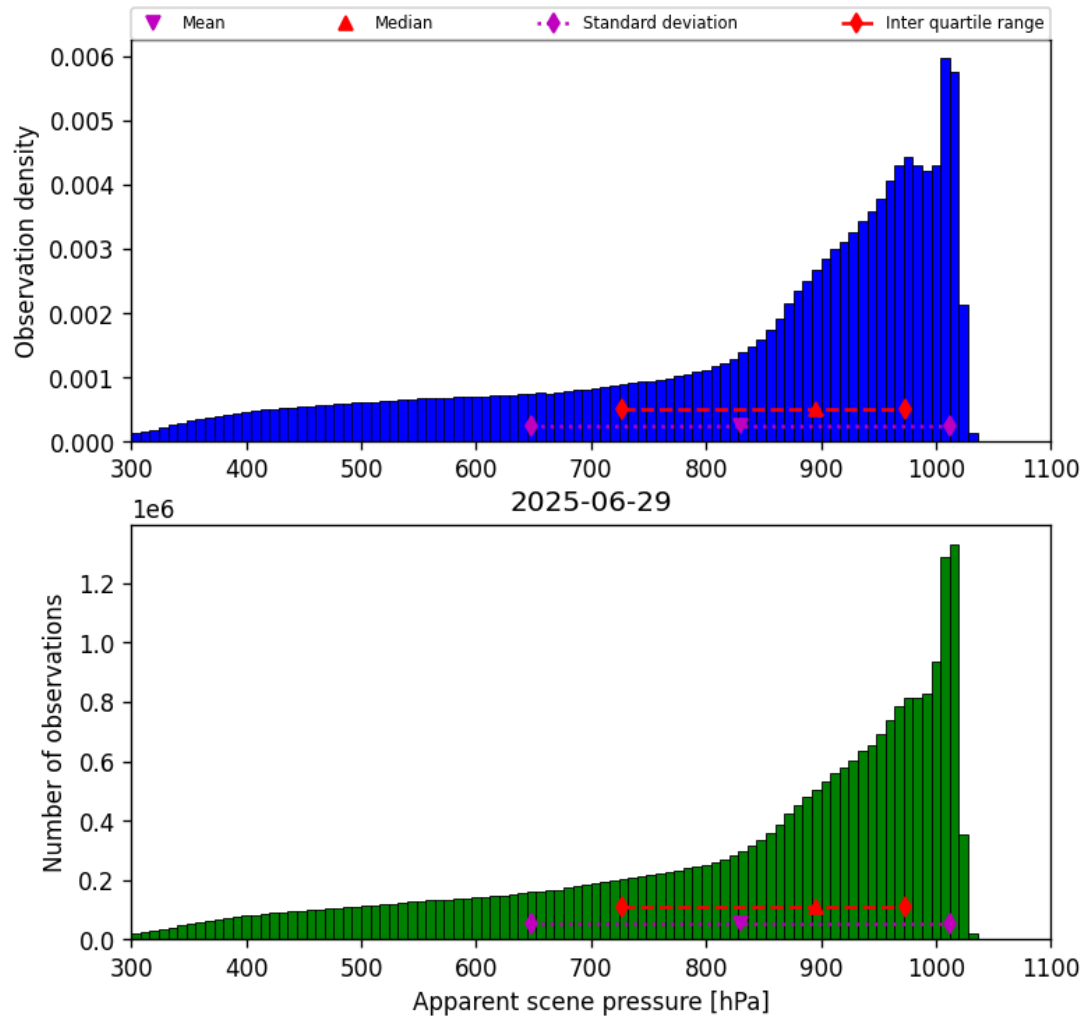
Figure 36: Histogram of “Apparent scene pressure” for 2025-06-28 to 2025-06-30
