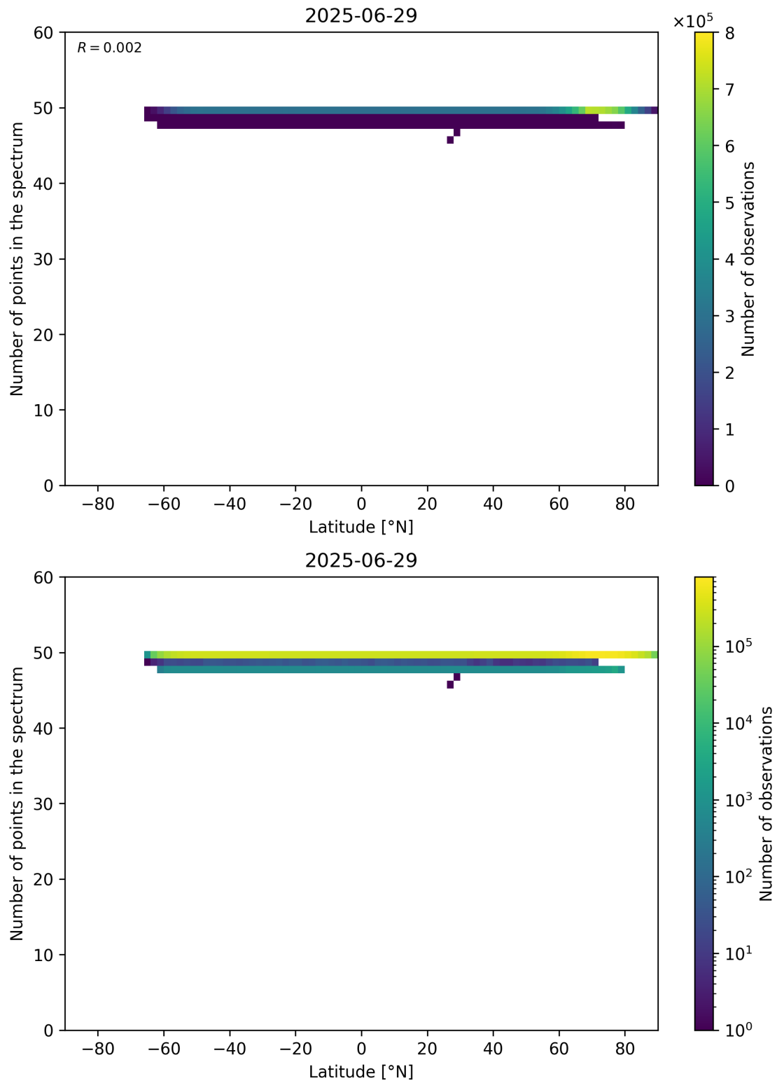
Figure 94: Scatter density plot of “Latitude” against “Number of points in the spectrum” for 2025-06-28 to 2025-06-30.
