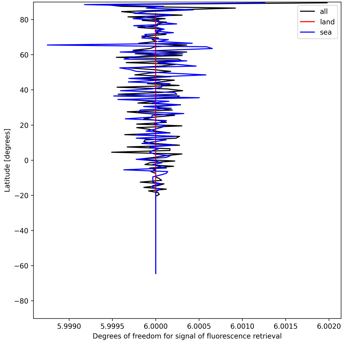
Figure 26: Zonal average of “Degrees of freedom for signal of fluorescence retrieval” for 2025-06-28 to 2025-06-30.
