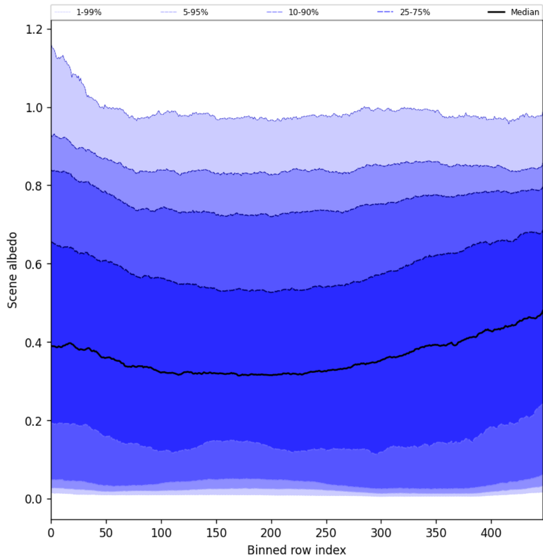
Figure 51: Along track statistics of “Scene albedo” for 2025-06-28 to 2025-06-30
