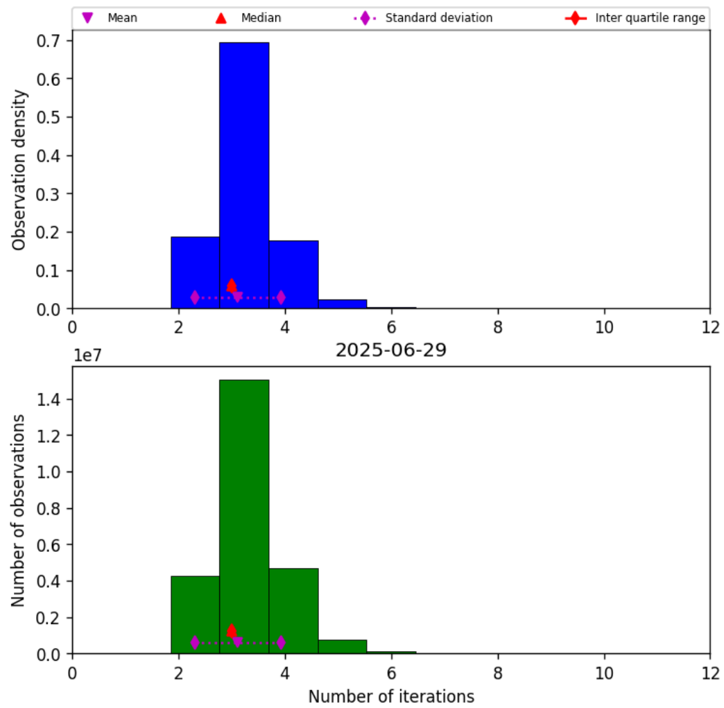
Figure 39: Histogram of “Number of iterations” for 2025-06-28 to 2025-06-30
