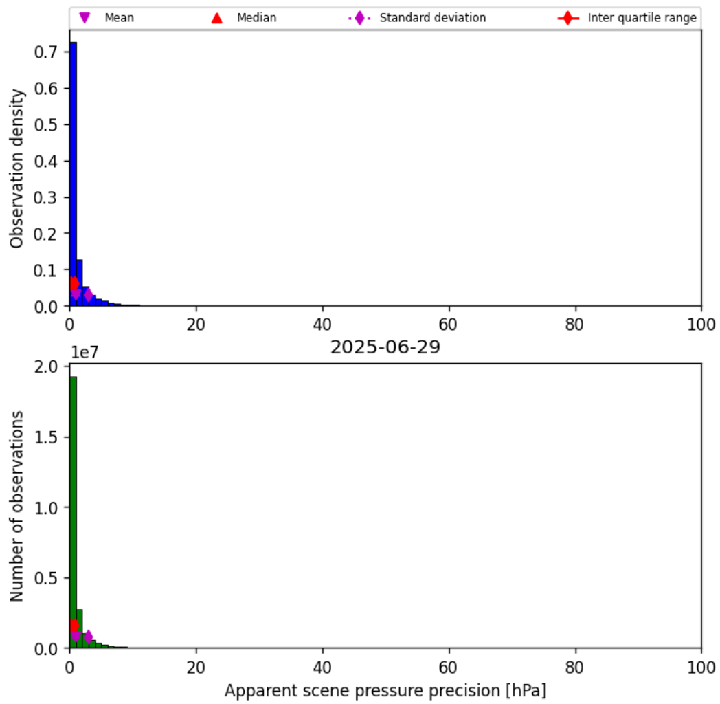
Figure 37: Histogram of “Apparent scene pressure precision” for 2025-06-28 to 2025-06-30
