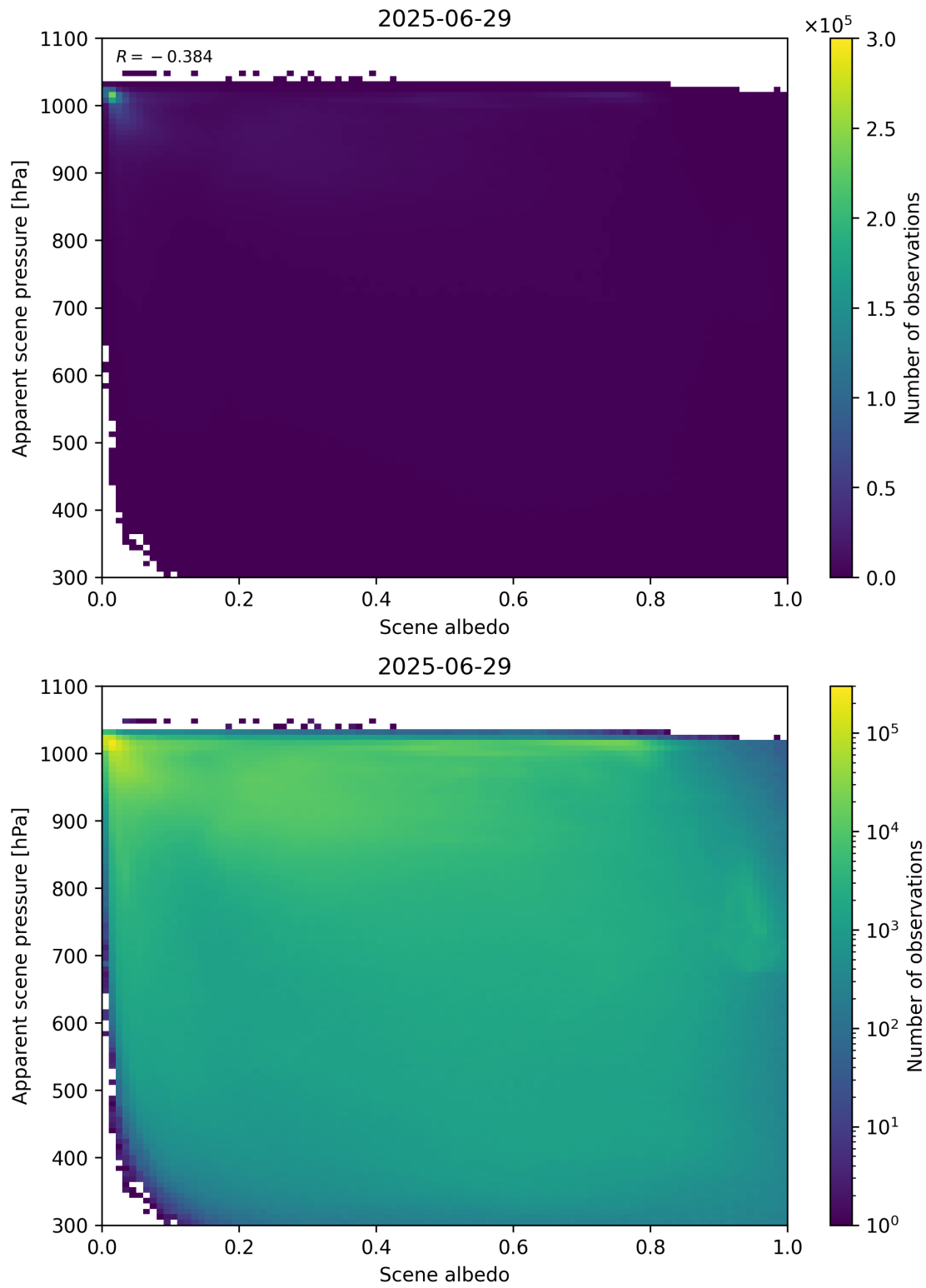
Figure 102: Scatter density plot of “Scene albedo” against “Apparent scene pressure” for 2025-06-28 to 2025-06-30.
