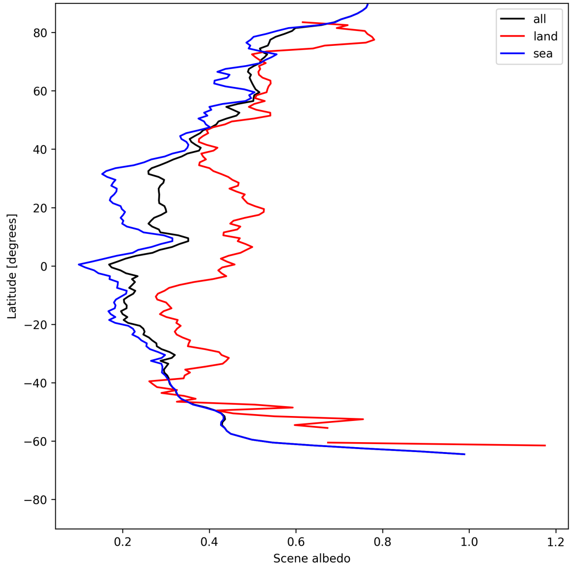
Figure 17: Zonal average of “Scene albedo” for 2025-06-28 to 2025-06-30.
