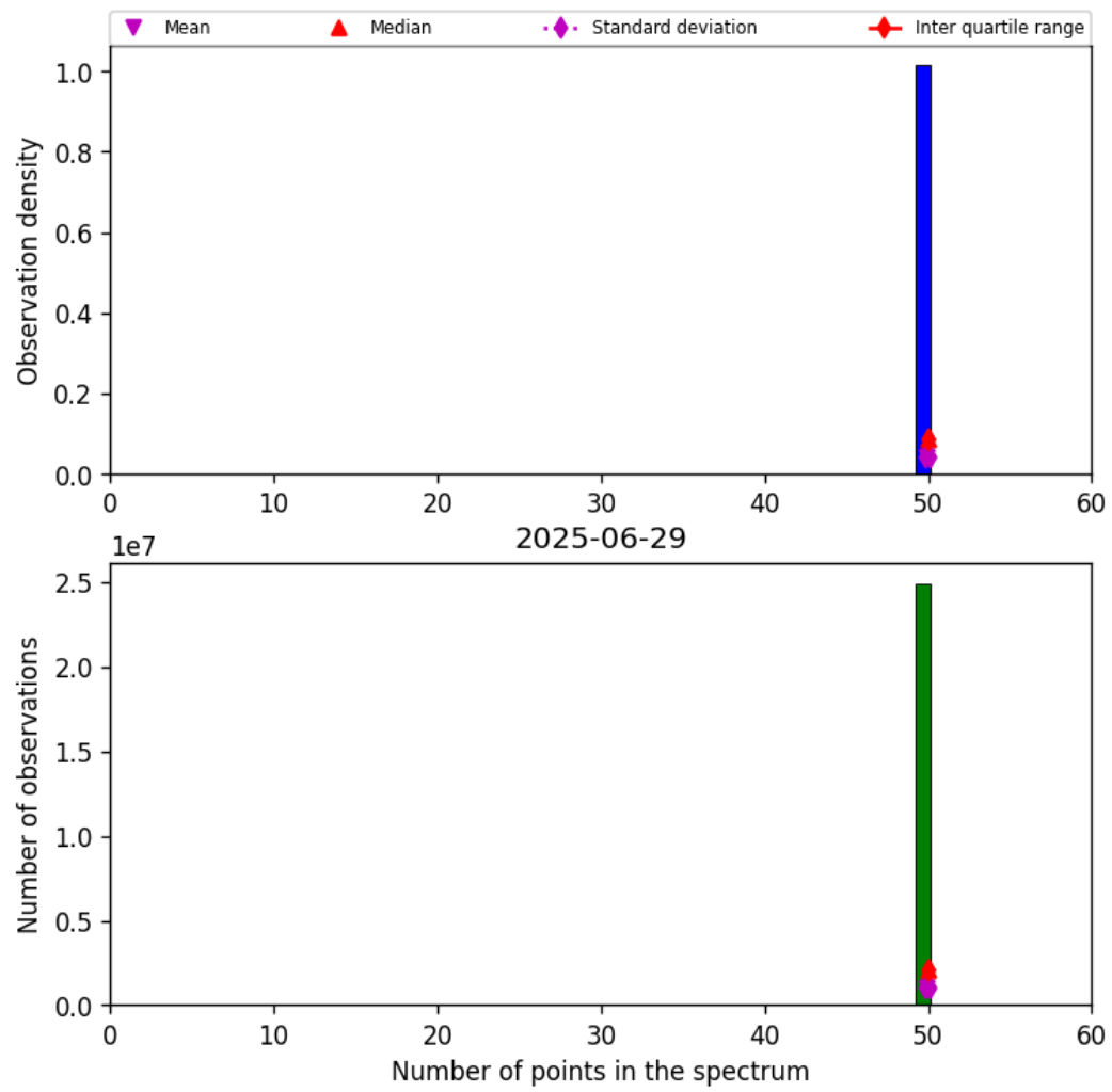
Figure 44: Histogram of “Number of points in the spectrum” for 2025-06-28 to 2025-06-30
