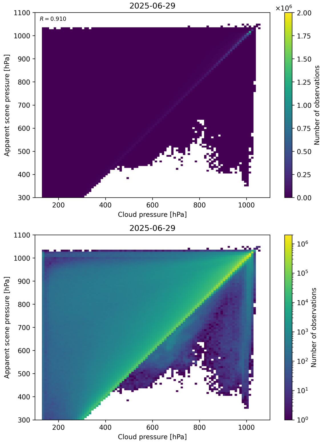
Figure 77: Scatter density plot of “Cloud pressure” against “Apparent scene pressure” for 2025-06-28 to 2025-06-30.
