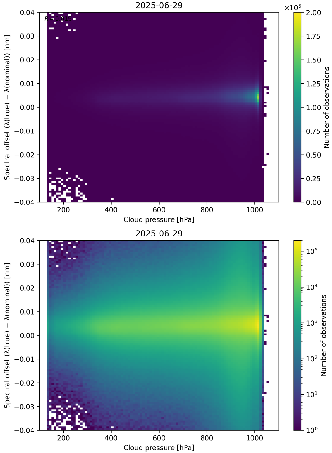
Figure 84: Scatter density plot of “Cloud pressure” against “Spectral offset ( \lambda_{\text{true}} - \lambda_{\text{nominal}} )” for 2025-06-28 to 2025-06-30.
