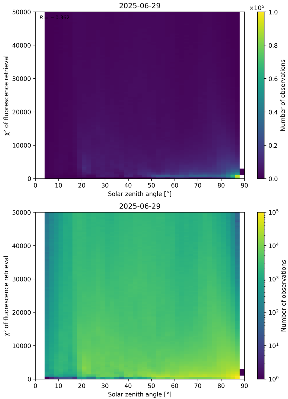
Figure 109: Scatter density plot of “Solar zenith angle” against “ \chi^2 of fluorescence retrieval” for 2025-06-28 to 2025-06-30.
