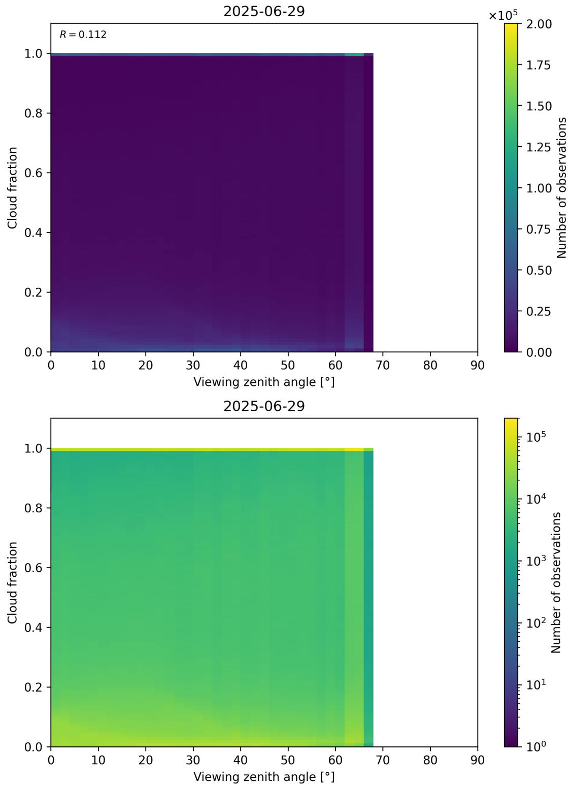
Figure 120: Scatter density plot of “Viewing zenith angle” against “Cloud fraction” for 2025-06-28 to 2025-06-30.
