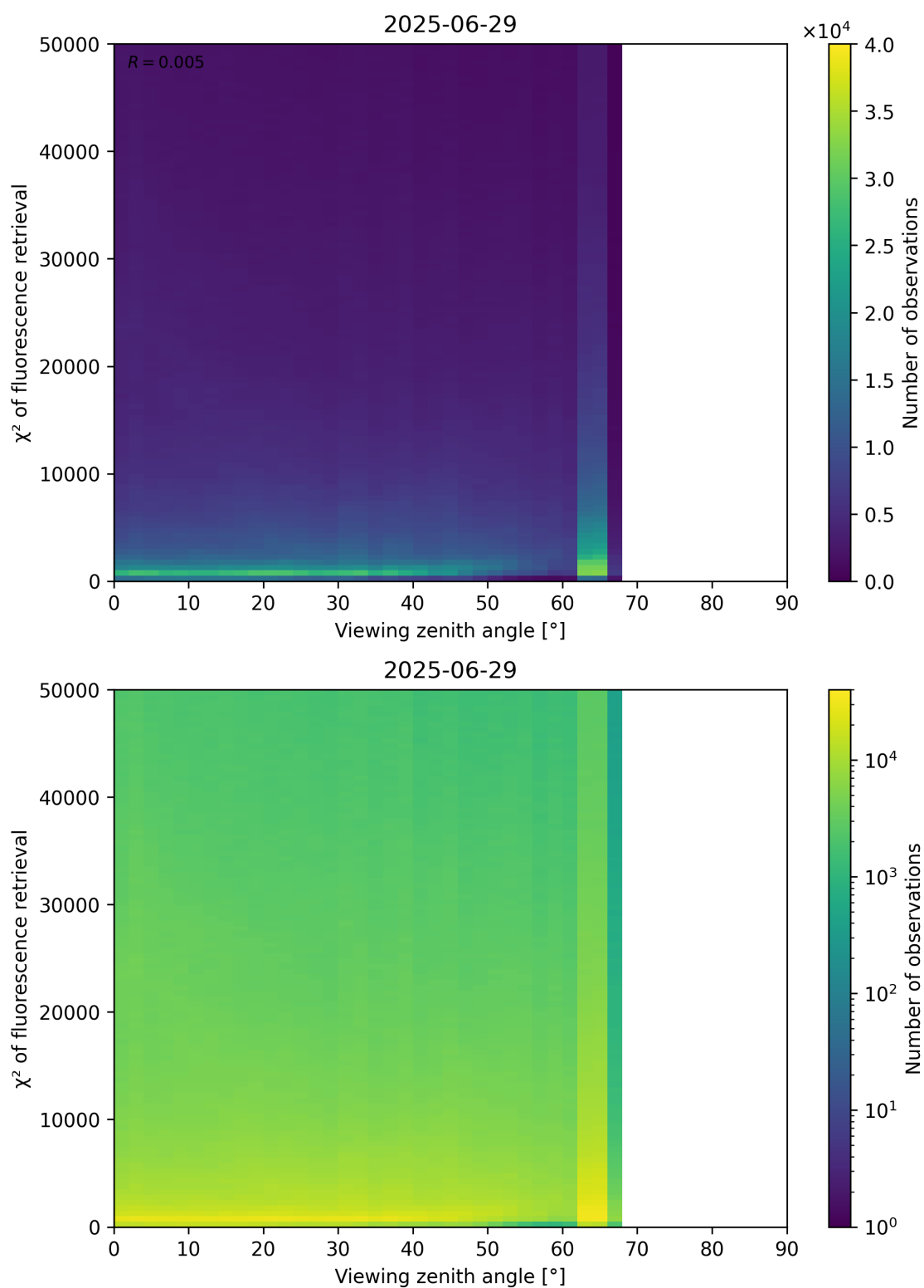
Figure 119: Scatter density plot of “Viewing zenith angle” against “ \chi^2 of fluorescence retrieval” for 2025-06-28 to 2025-06-30.
