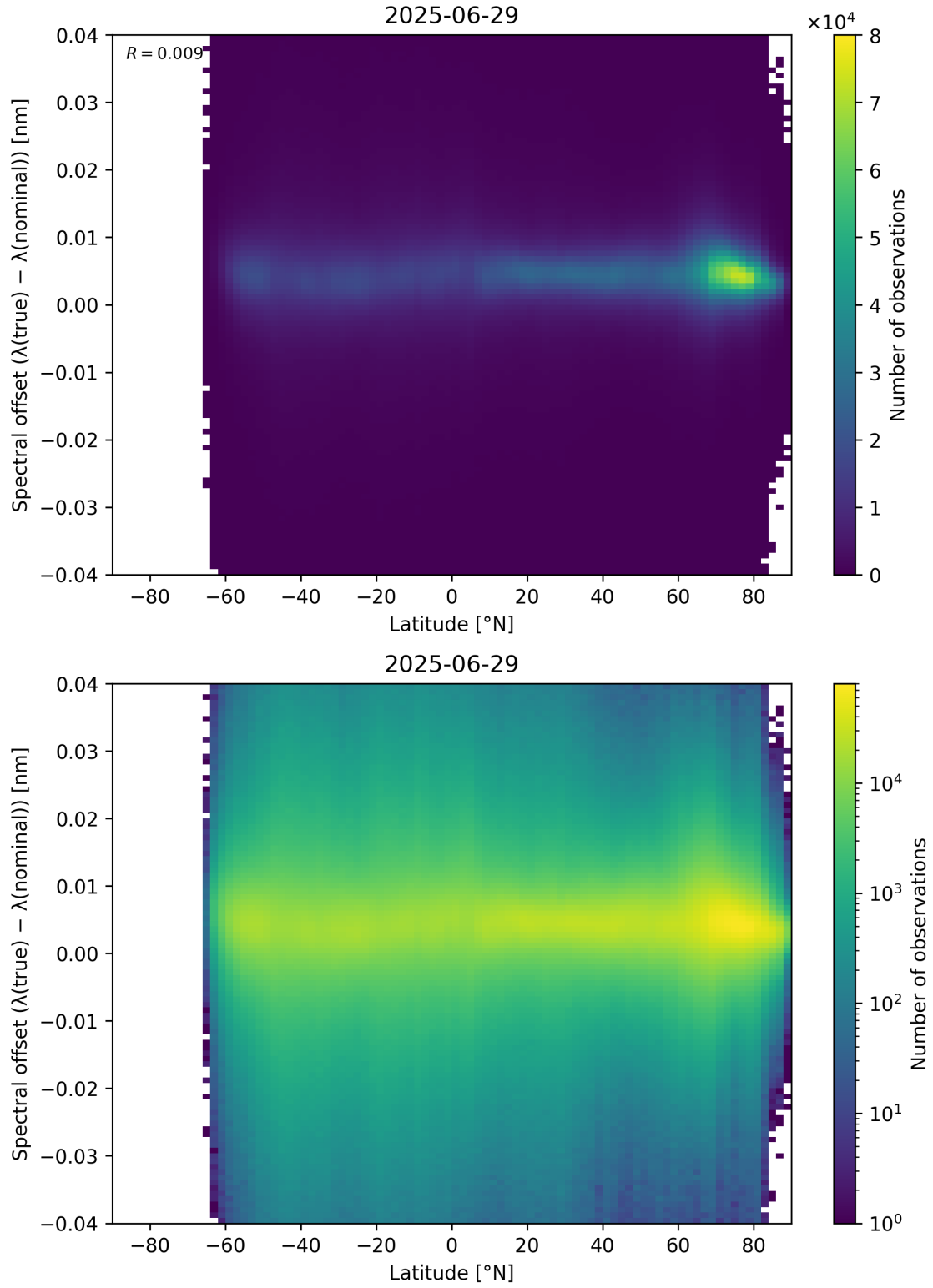
Figure 96: Scatter density plot of “Latitude” against “Spectral offset ( \lambda_{\text{true}} - \lambda_{\text{nominal}} )” for 2025-06-28 to 2025-06-30.
