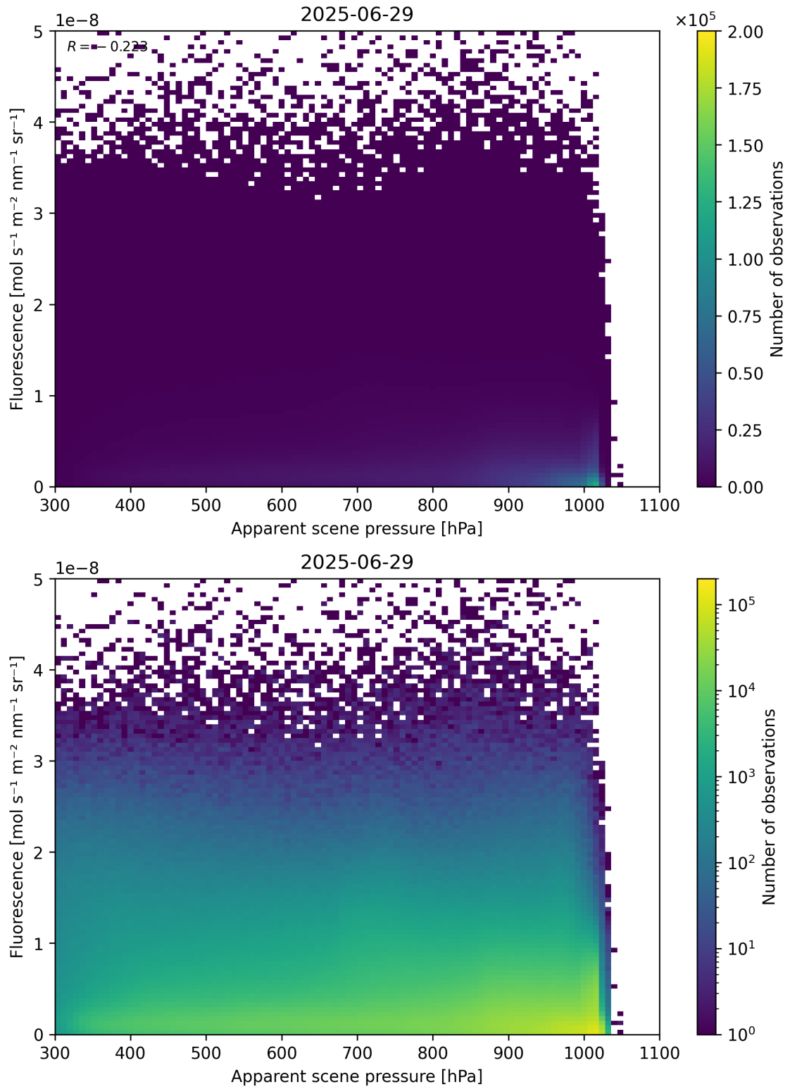
Figure 64: Scatter density plot of “Apparent scene pressure” against “Fluorescence” for 2025-06-28 to 2025-06-30.
