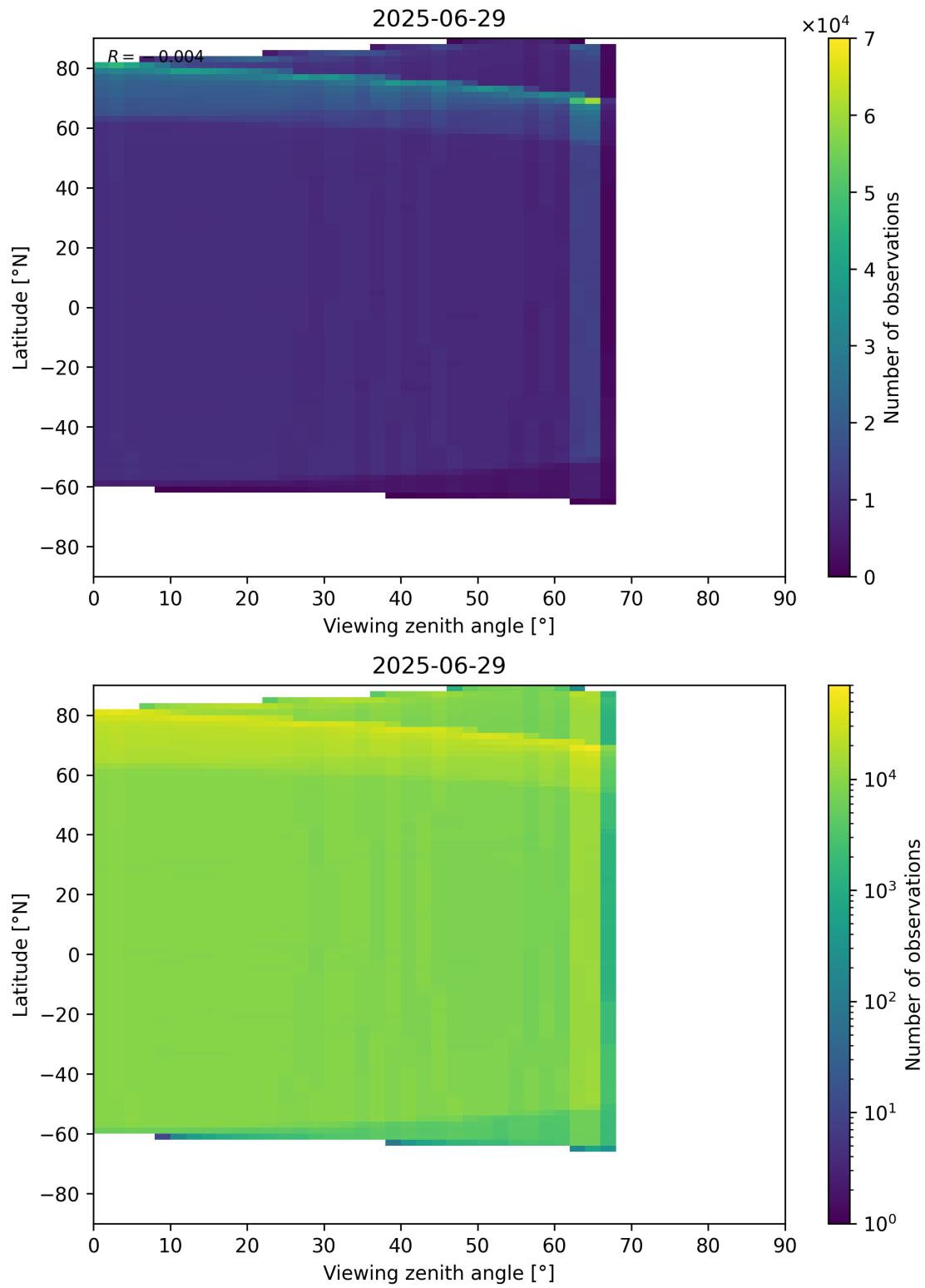
Figure 123: Scatter density plot of “Viewing zenith angle” against “Latitude” for 2025-06-28 to 2025-06-30.
