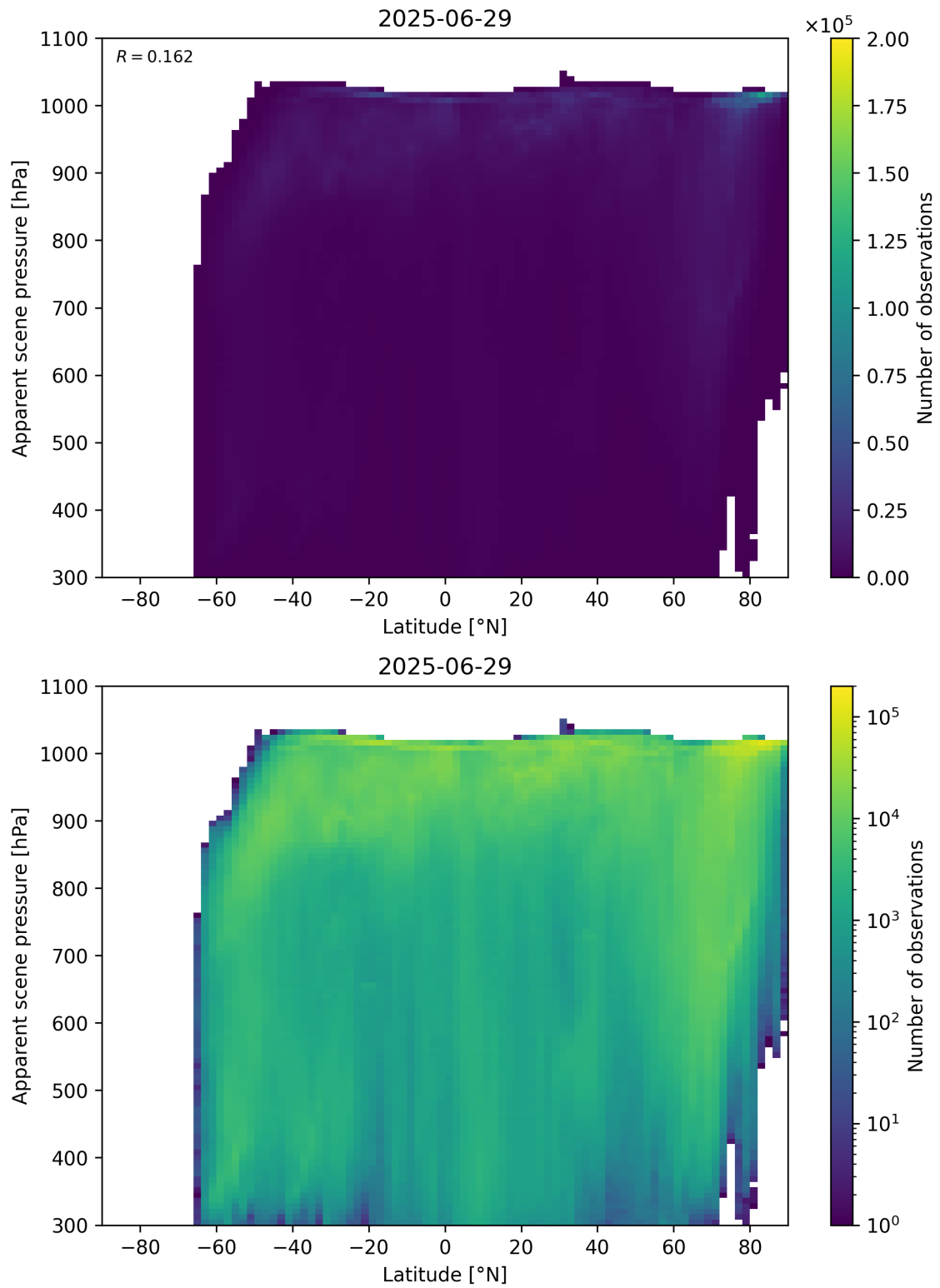
Figure 88: Scatter density plot of “Latitude” against “Apparent scene pressure” for 2025-06-28 to 2025-06-30.
