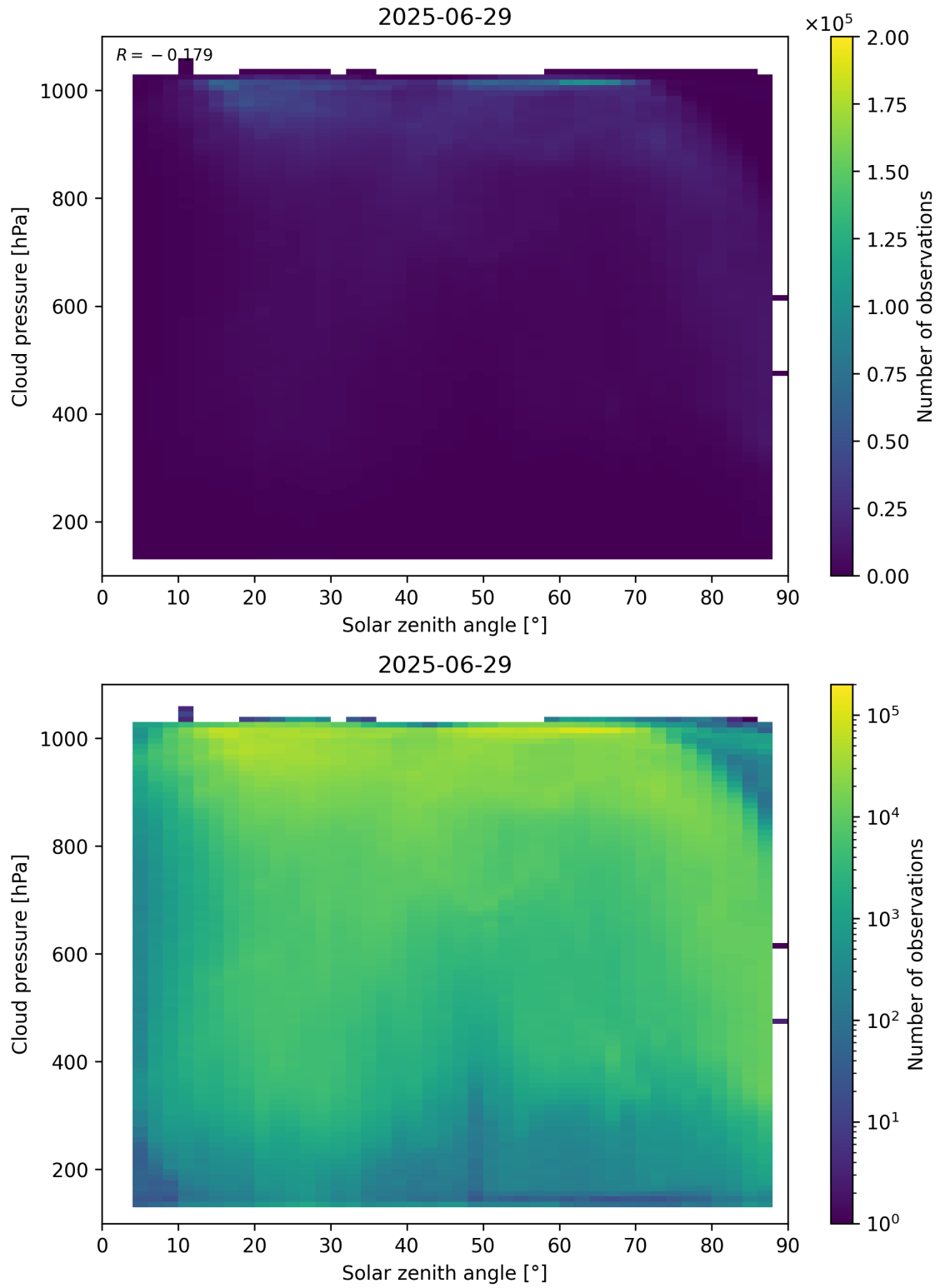
Figure 111: Scatter density plot of “Solar zenith angle” against “Cloud pressure” for 2025-06-28 to 2025-06-30.
