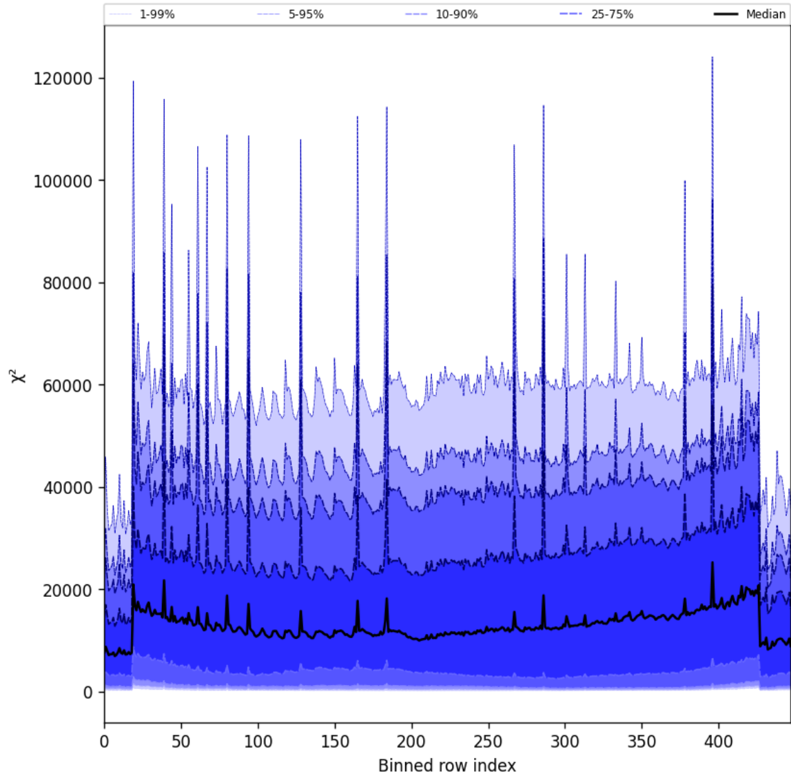
Figure 55: Along track statistics of “ \chi^2 ” for 2025-06-28 to 2025-06-30
