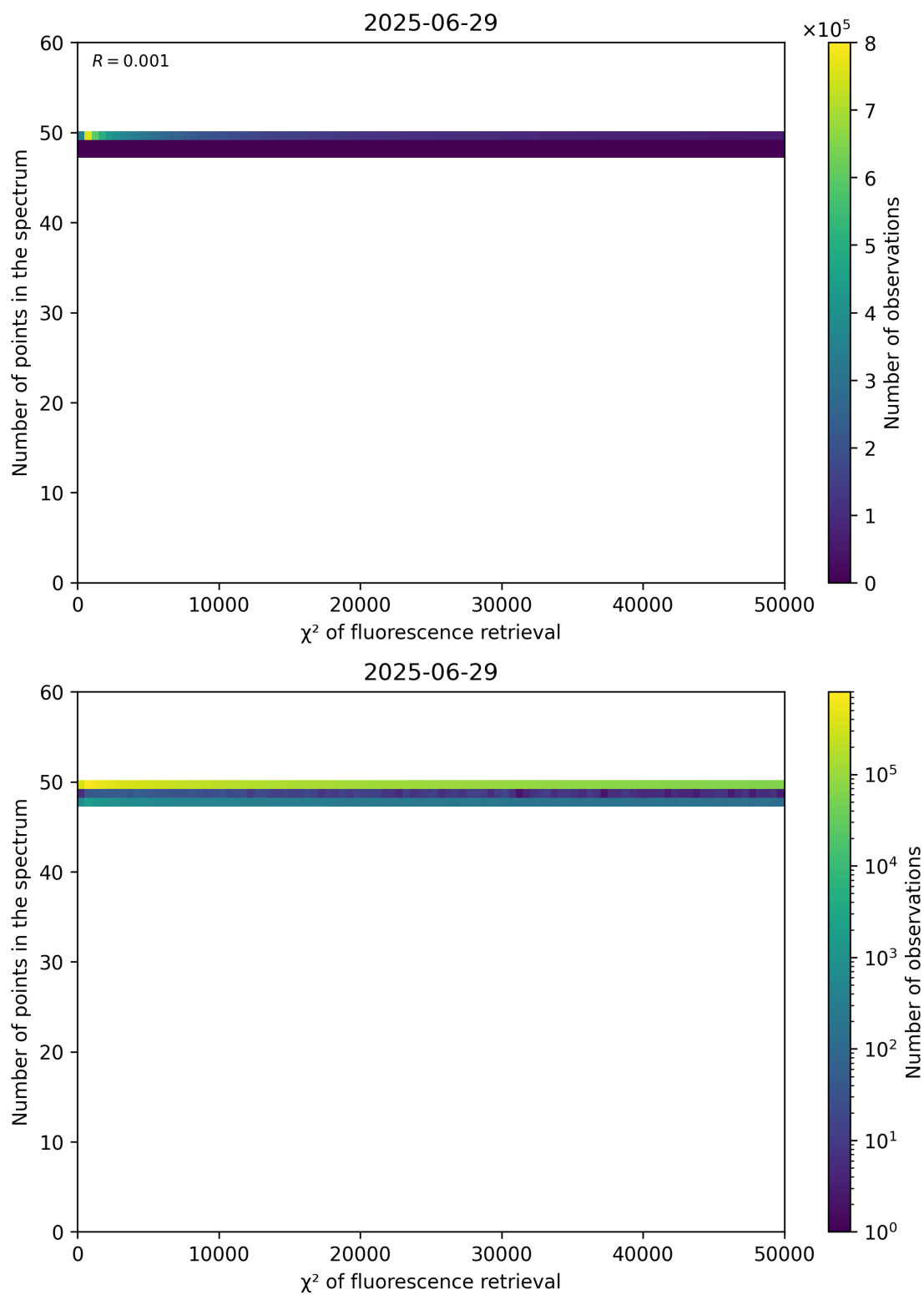
Figure 68: Scatter density plot of “ \chi^2 of fluorescence retrieval” against “Number of points in the spectrum” for 2025-06-28 to 2025-06-30.
