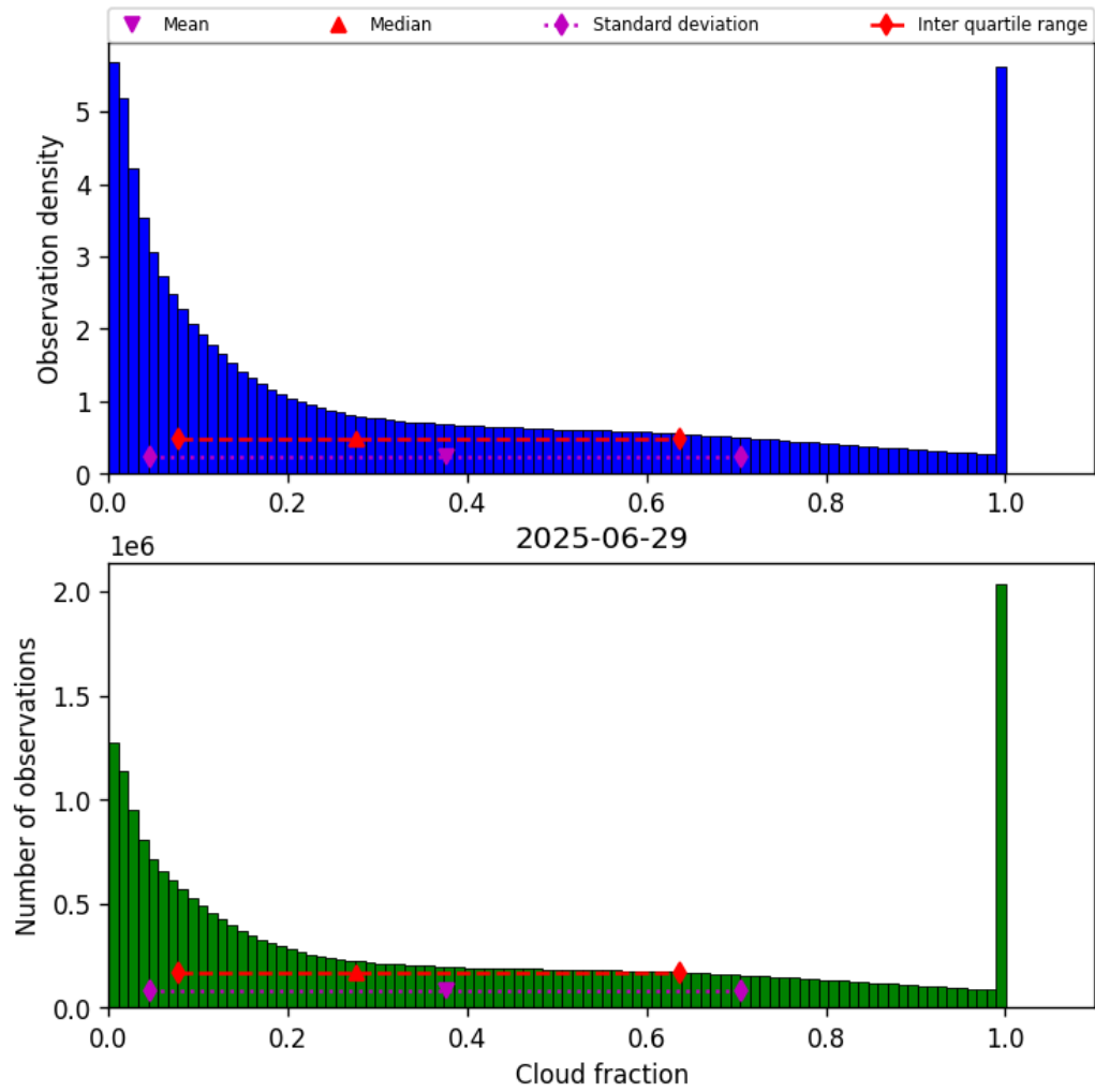
Figure 32: Histogram of “Cloud fraction” for 2025-06-28 to 2025-06-30
