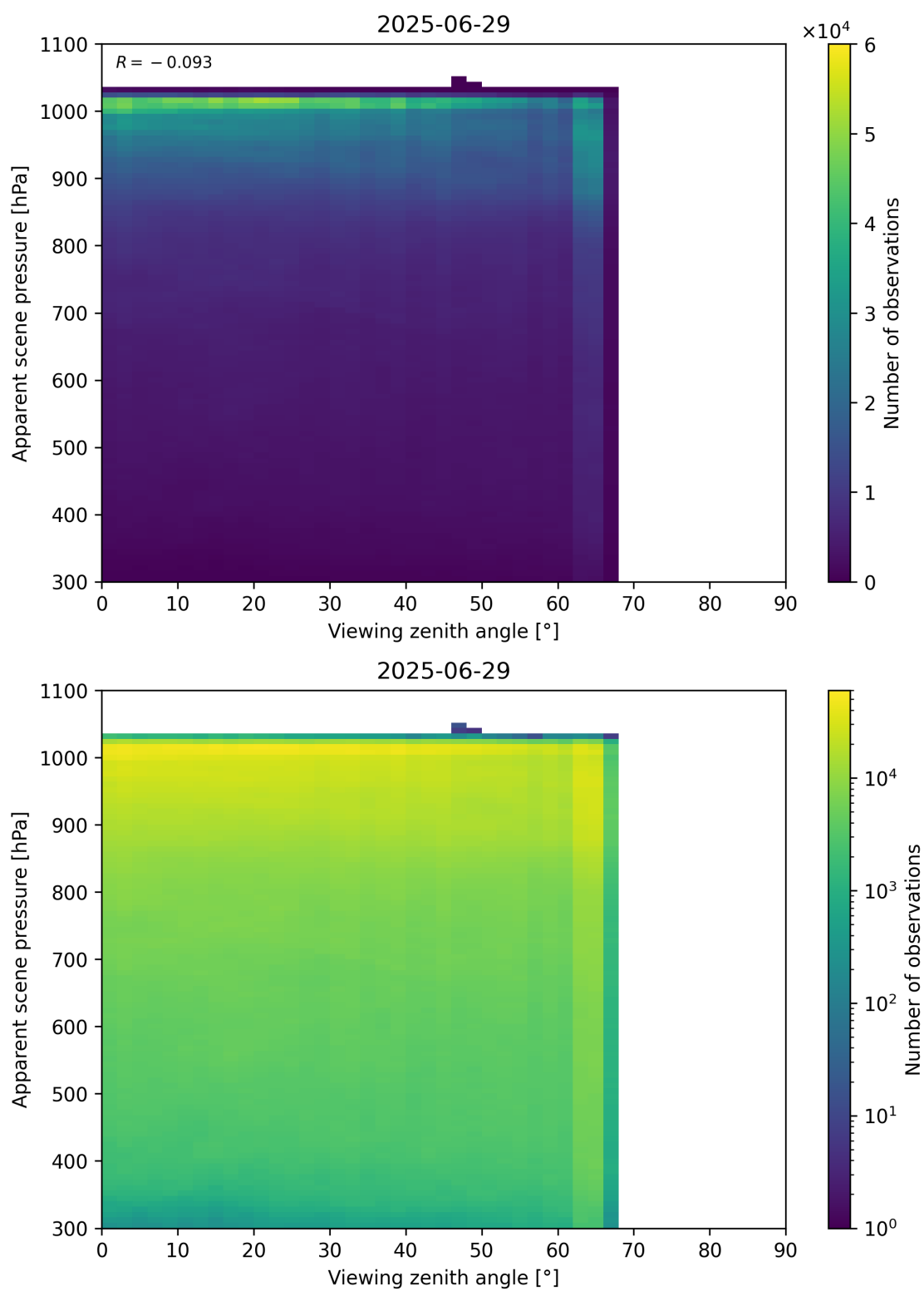
Figure 118: Scatter density plot of “Viewing zenith angle” against “Apparent scene pressure” for 2025-06-28 to 2025-06-30.
