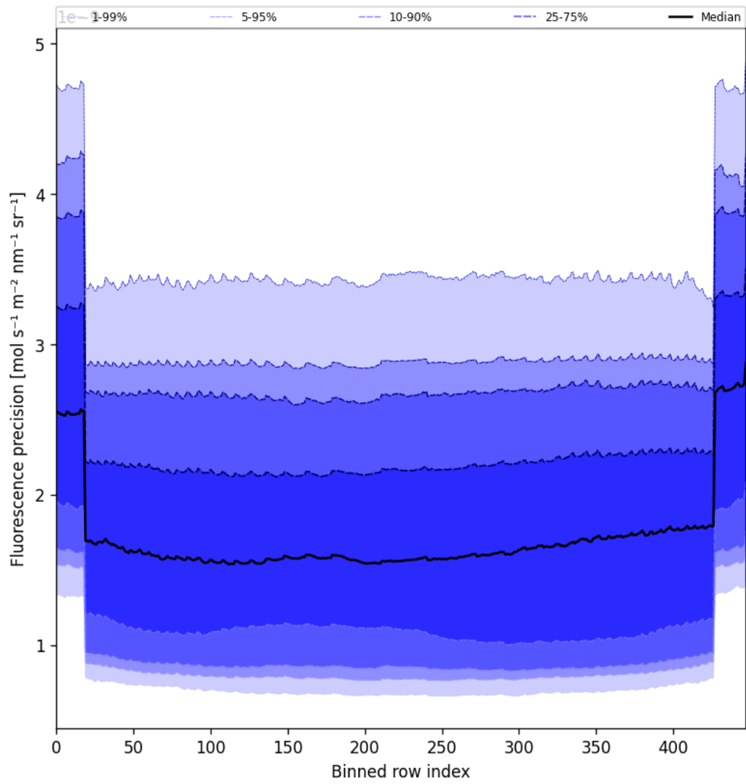
Figure 58: Along track statistics of “Fluorescence precision” for 2025-06-28 to 2025-06-30
