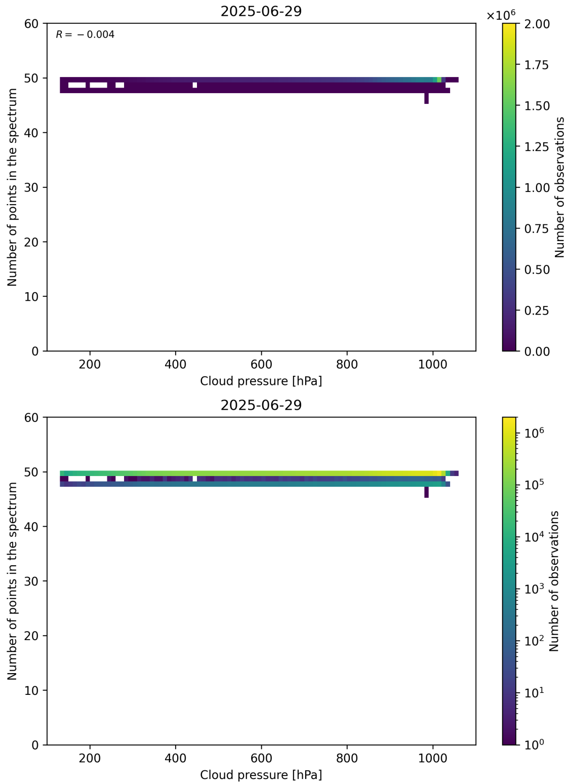
Figure 82: Scatter density plot of “Cloud pressure” against “Number of points in the spectrum” for 2025-06-28 to 2025-06-30.
