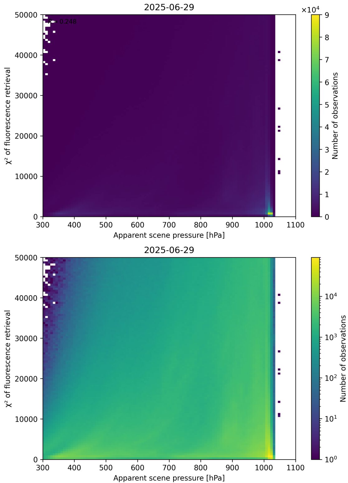
Figure 63: Scatter density plot of “Apparent scene pressure” against “ \chi^2 of fluorescence retrieval” for 2025-06-28 to 2025-06-30.
