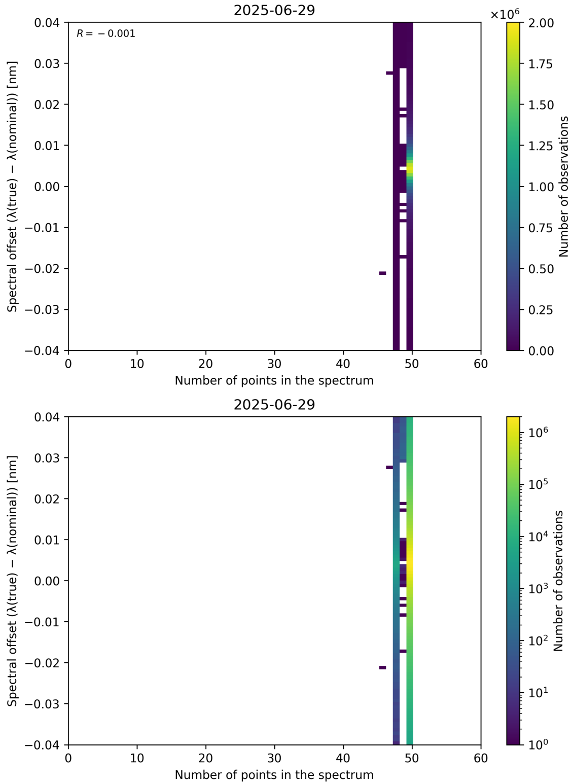
Figure 101: Scatter density plot of “Number of points in the spectrum” against “Spectral offset ( \lambda_{\text{true}} - \lambda_{\text{nominal}} )” for 2025-06-28 to 2025-06-30.
