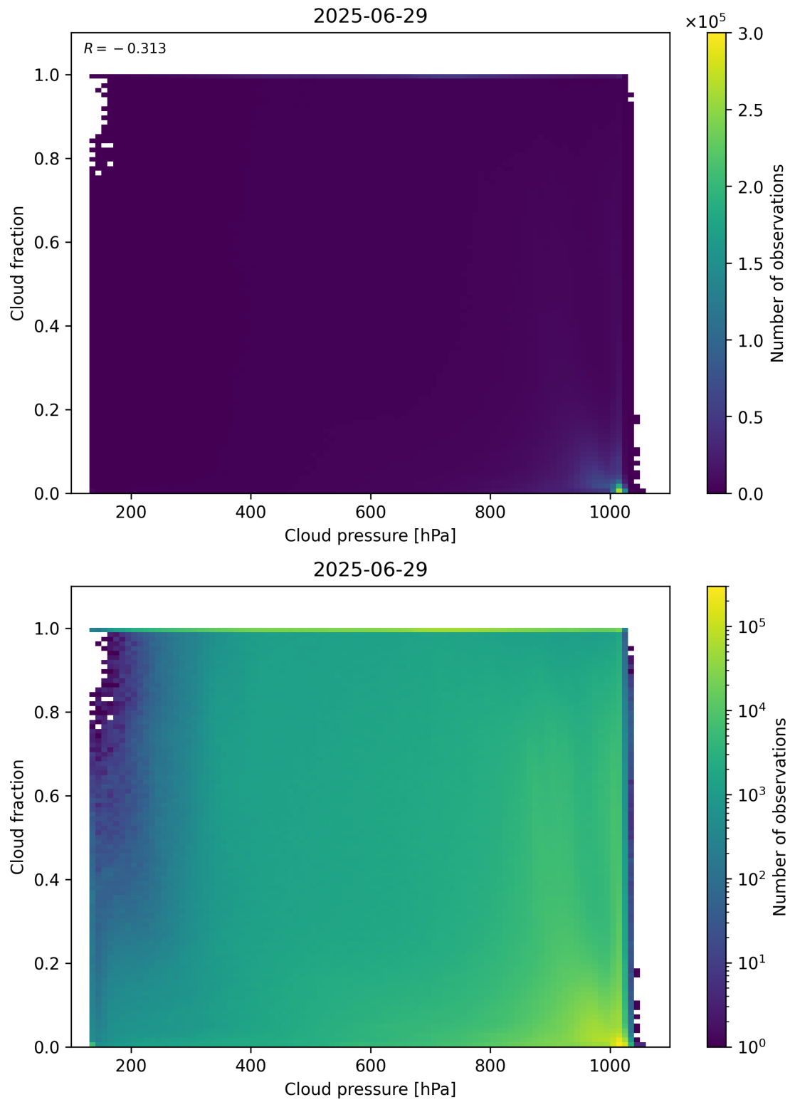
Figure 79: Scatter density plot of “Cloud pressure” against “Cloud fraction” for 2025-06-28 to 2025-06-30.
