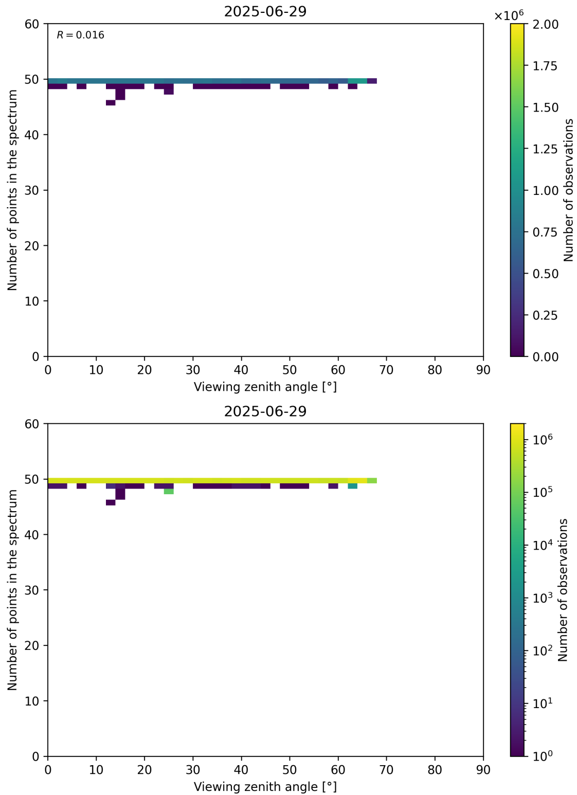
Figure 125: Scatter density plot of “Viewing zenith angle” against “Number of points in the spectrum” for 2025-06-28 to 2025-06-30.
