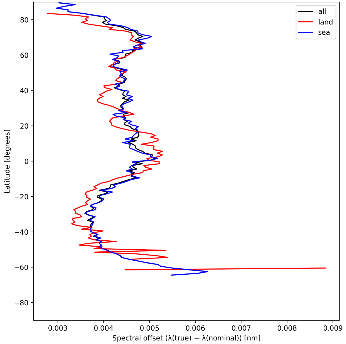
Figure 28: Zonal average of “Spectral offset ( \lambda_{\text{true}} - \lambda_{\text{nominal}} )” for 2025-06-28 to 2025-06-30.
