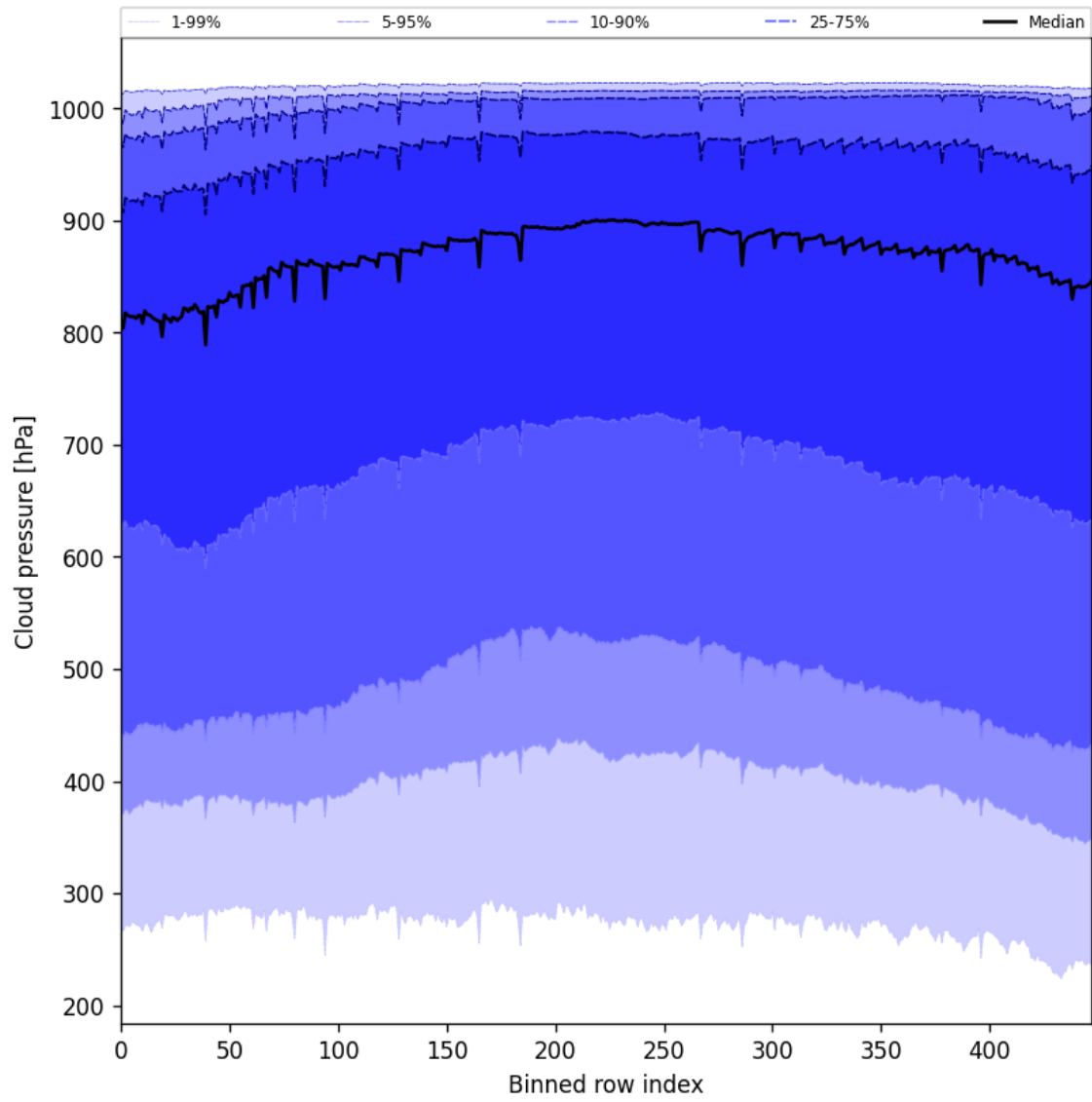
Figure 47: Along track statistics of “Cloud pressure” for 2025-06-29 to 2025-07-01
