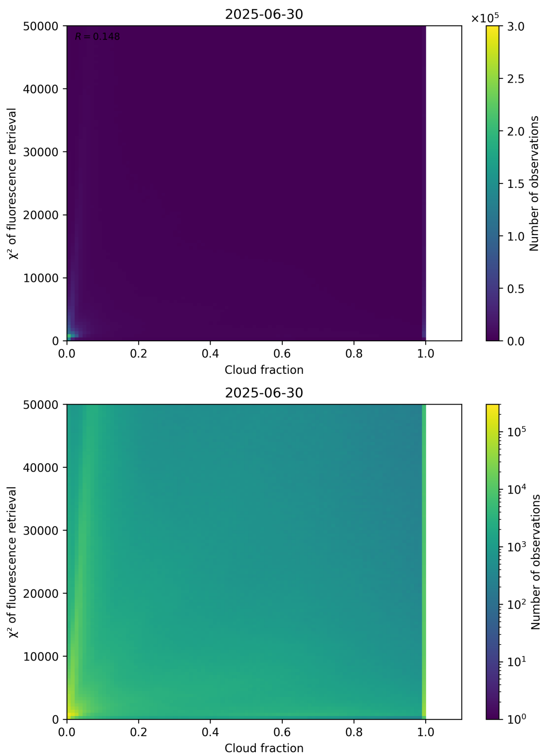
Figure 71: Scatter density plot of “Cloud fraction” against “ \chi^2 of fluorescence retrieval” for 2025-06-29 to 2025-07-01.
