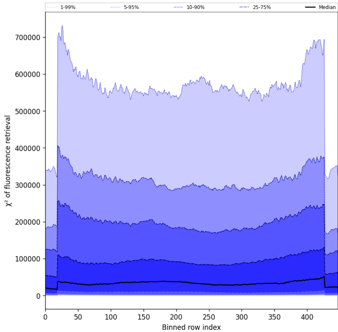
Figure 59: Along track statistics of “ \chi^2 of fluorescence retrieval” for 2025-06-29 to 2025-07-01
