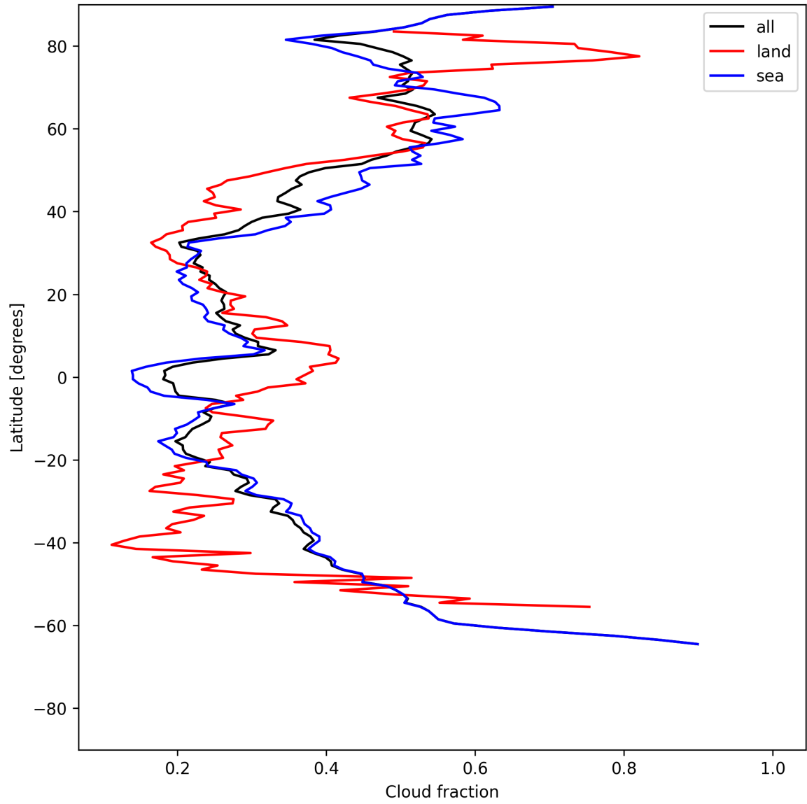
Figure 15: Zonal average of “Cloud fraction” for 2025-06-29 to 2025-07-01.
