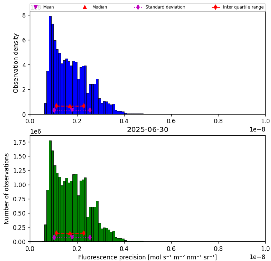
Figure 41: Histogram of “Fluorescence precision” for 2025-06-29 to 2025-07-01
