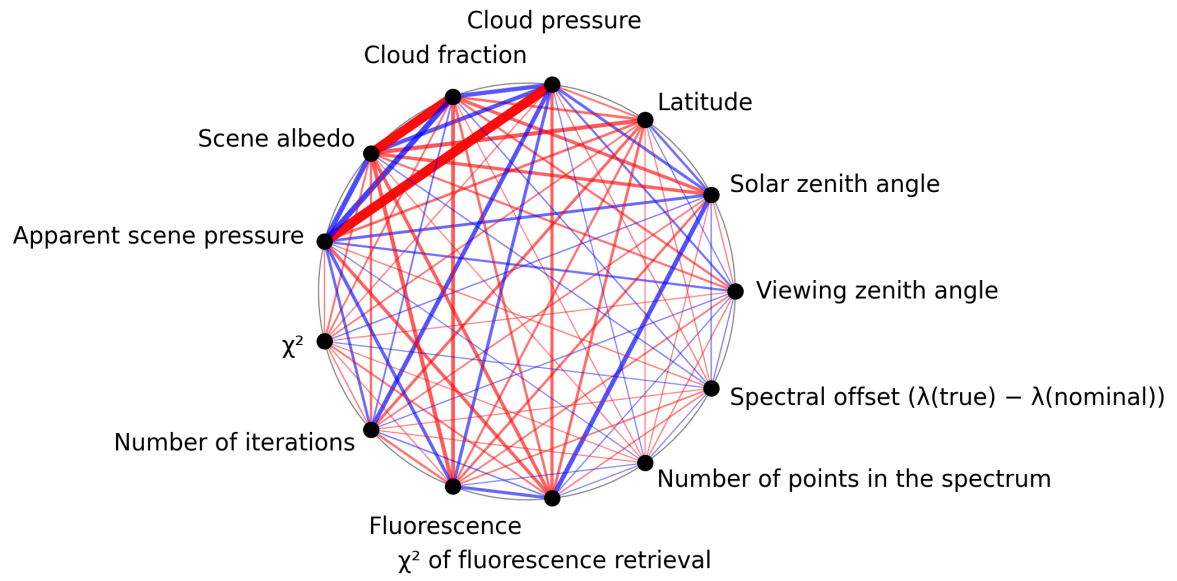
Figure 1: Map of correlation graph for 2025-06-29 to 2025-07-01.
