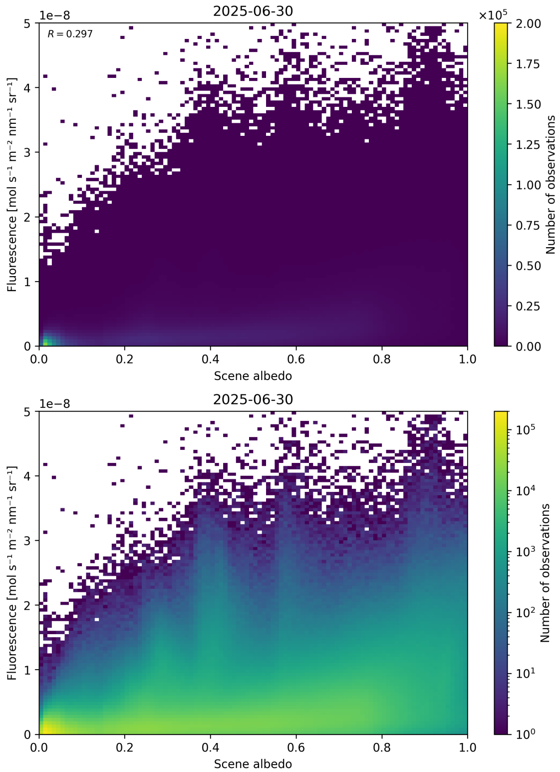
Figure 104: Scatter density plot of “Scene albedo” against “Fluorescence” for 2025-06-29 to 2025-07-01.
