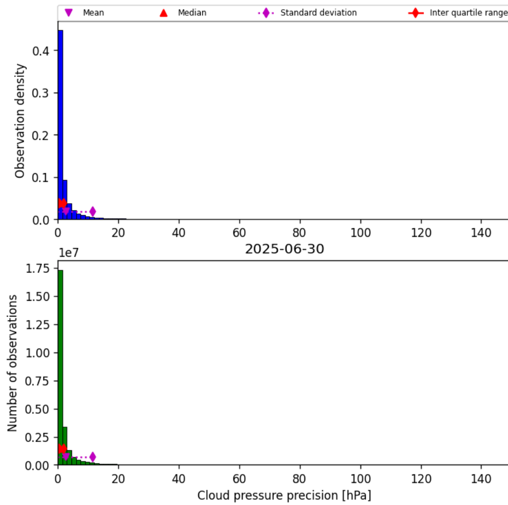
Figure 31: Histogram of “Cloud pressure precision” for 2025-06-29 to 2025-07-01
