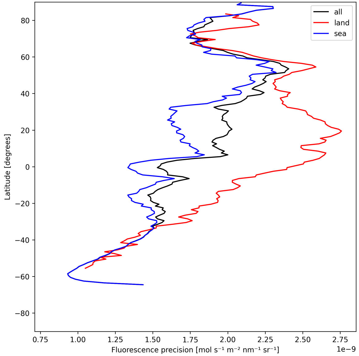
Figure 24: Zonal average of “Fluorescence precision” for 2025-06-29 to 2025-07-01.
