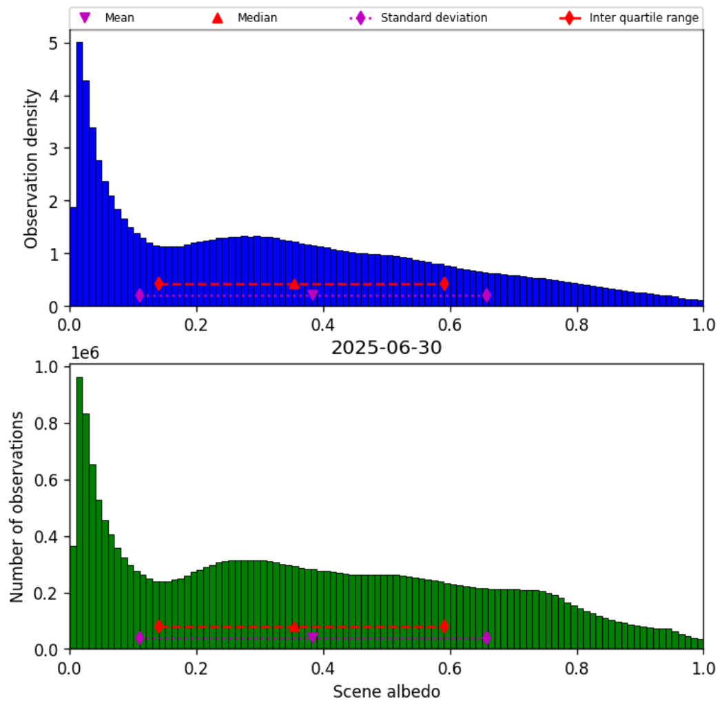
Figure 34: Histogram of “Scene albedo” for 2025-06-29 to 2025-07-01
