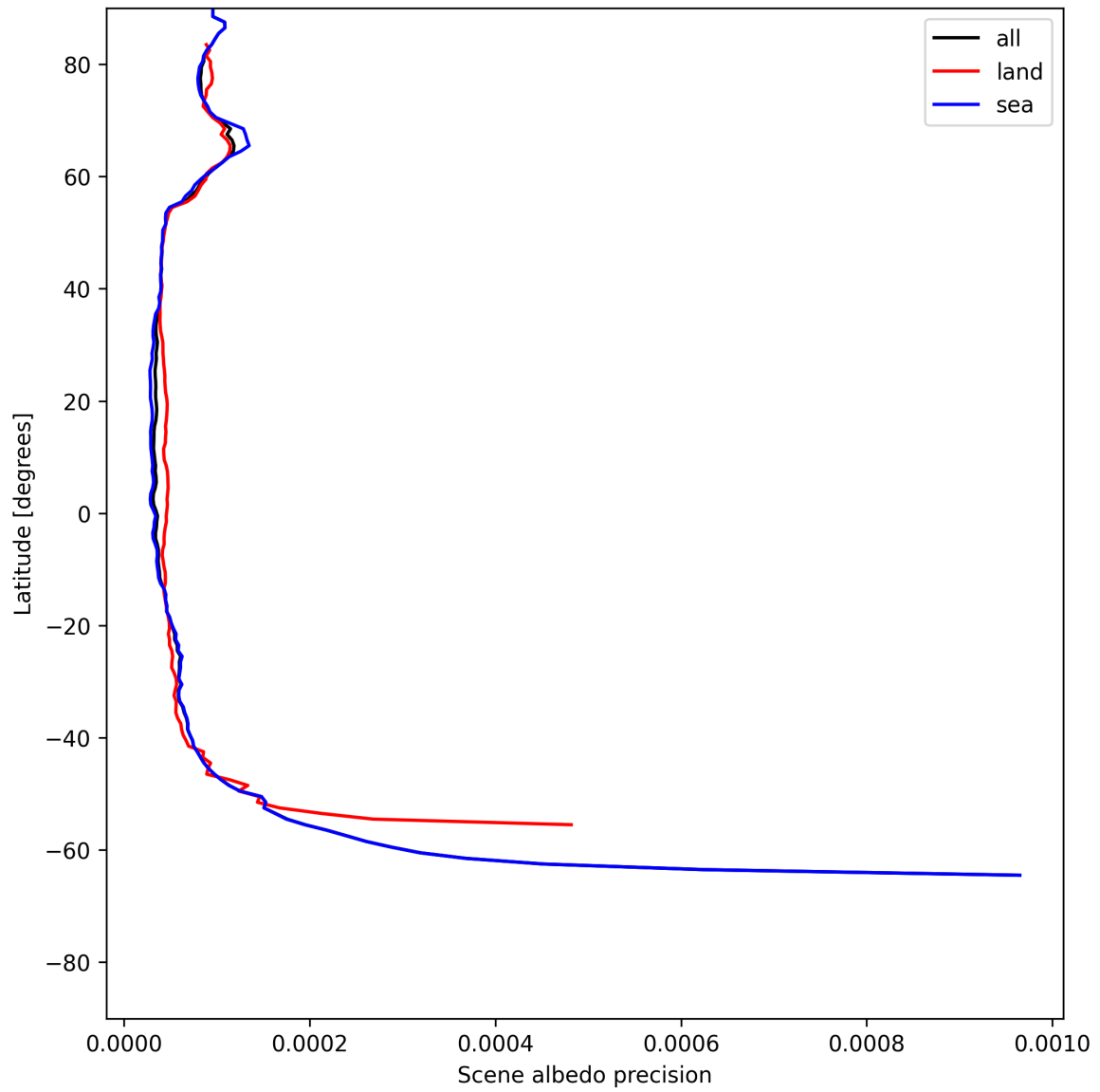
Figure 18: Zonal average of “Scene albedo precision” for 2025-06-29 to 2025-07-01.
