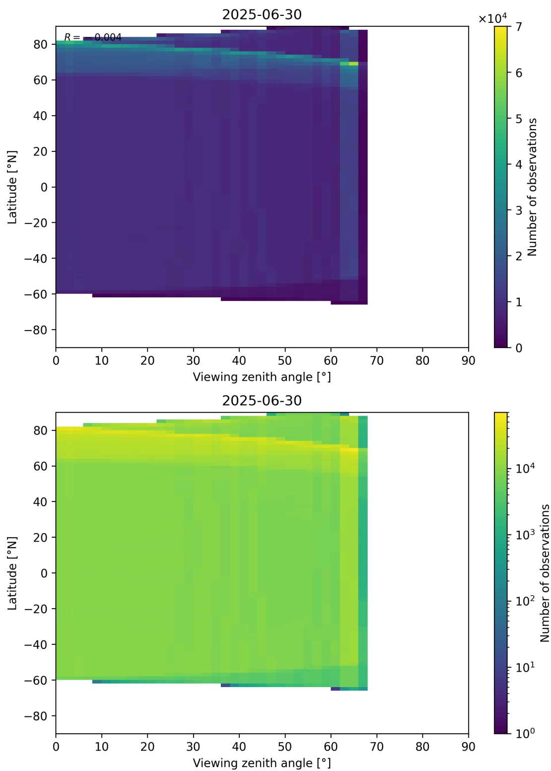
Figure 123: Scatter density plot of “Viewing zenith angle” against “Latitude” for 2025-06-29 to 2025-07-01.
