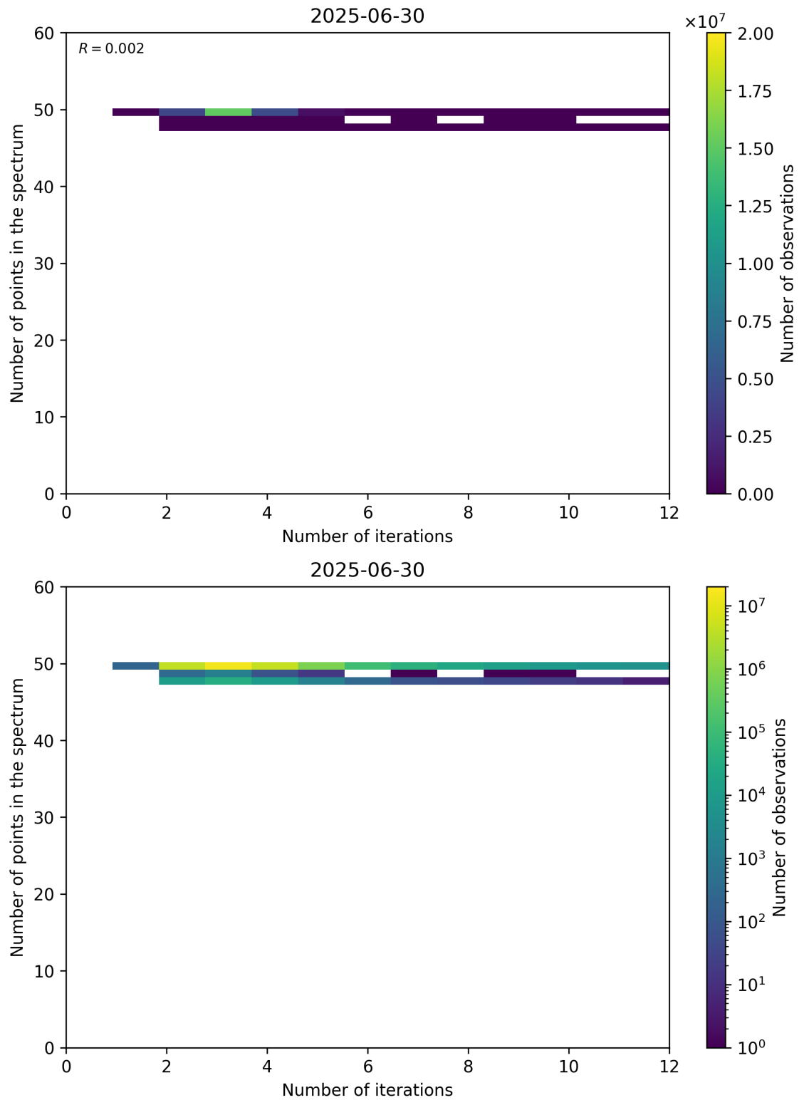
Figure 99: Scatter density plot of “Number of iterations” against “Number of points in the spectrum” for 2025-06-29 to 2025-07-01.
