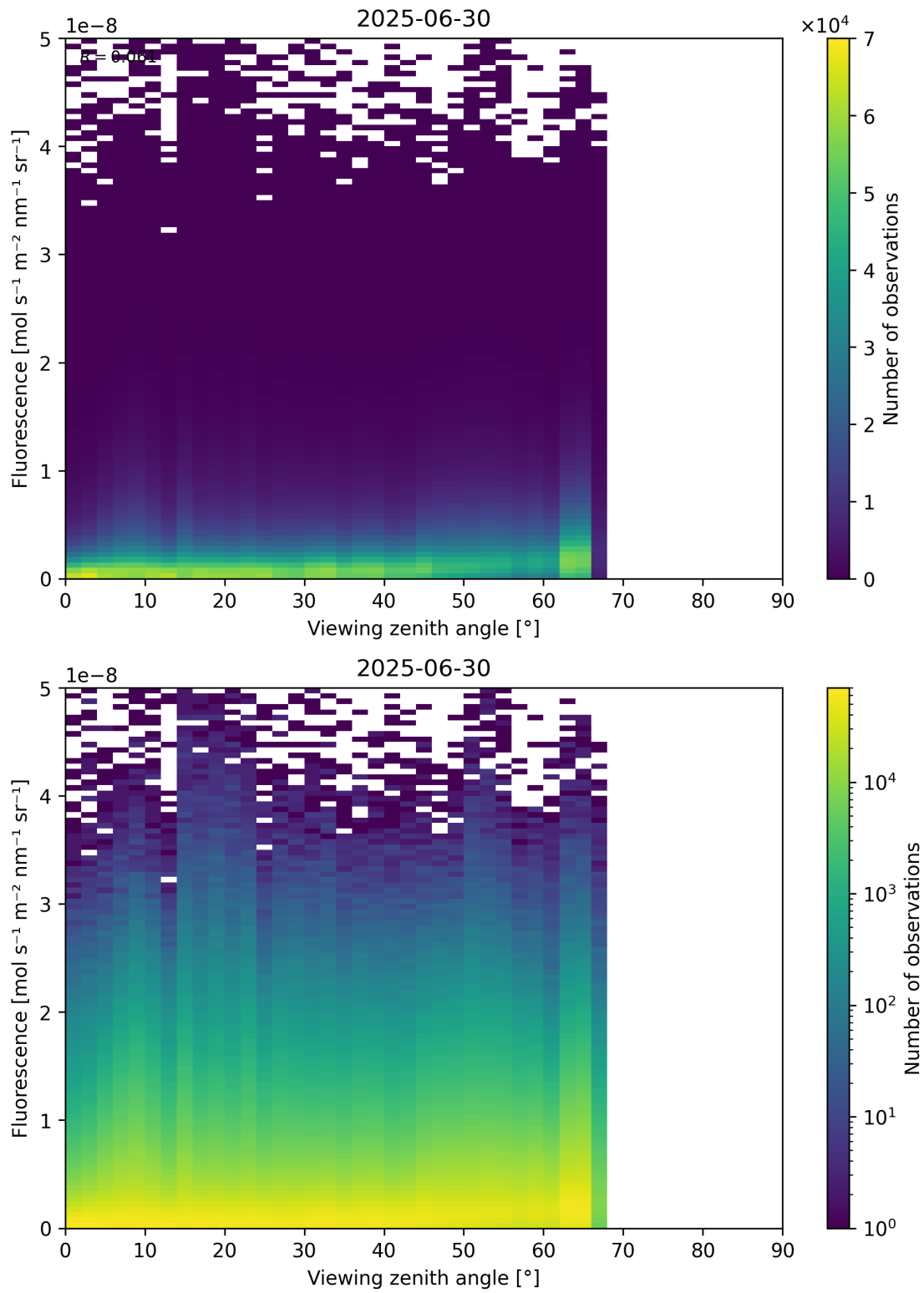
Figure 122: Scatter density plot of “Viewing zenith angle” against “Fluorescence” for 2025-06-29 to 2025-07-01.
