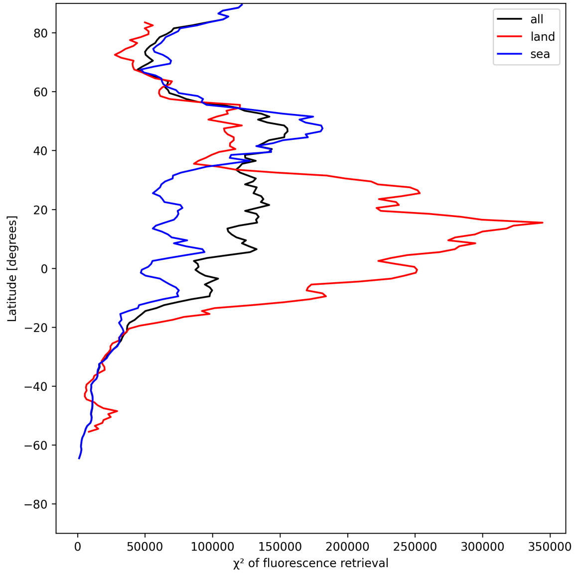
Figure 25: Zonal average of “ \chi^2 of fluorescence retrieval” for 2025-06-29 to 2025-07-01.
