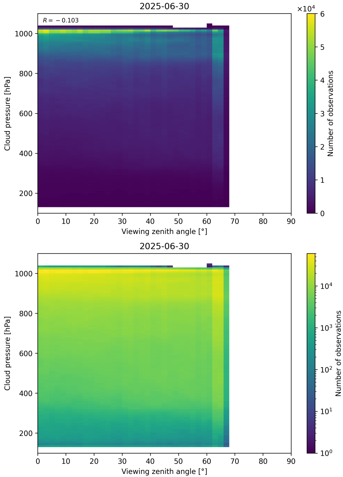
Figure 121: Scatter density plot of “Viewing zenith angle” against “Cloud pressure” for 2025-06-29 to 2025-07-01.
