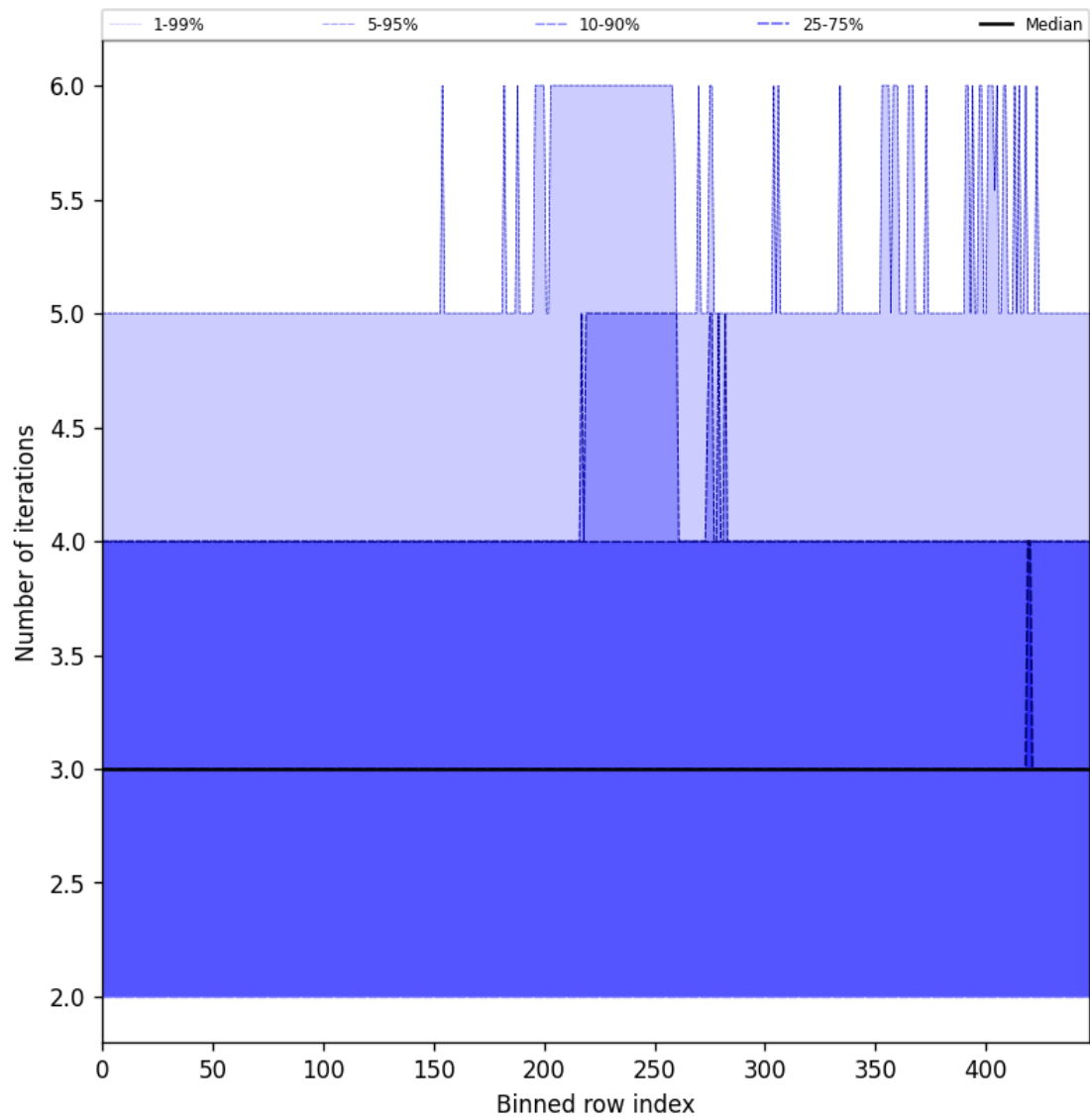
Figure 56: Along track statistics of “Number of iterations” for 2025-06-29 to 2025-07-01
