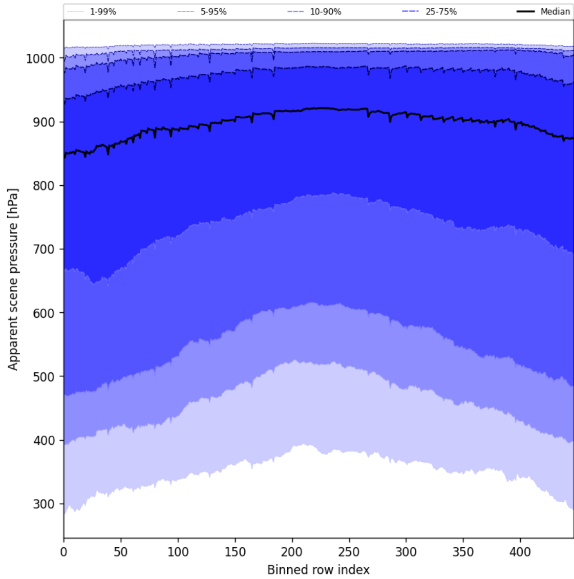
Figure 53: Along track statistics of “Apparent scene pressure” for 2025-06-29 to 2025-07-01
