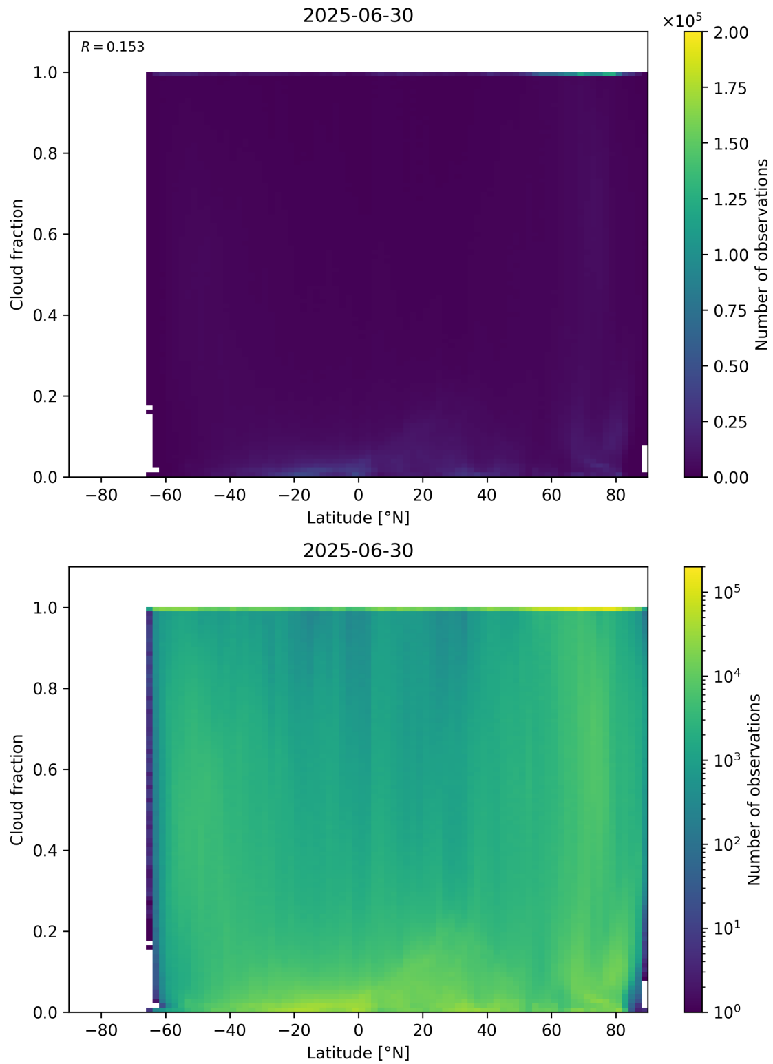
Figure 90: Scatter density plot of “Latitude” against “Cloud fraction” for 2025-06-29 to 2025-07-01.
