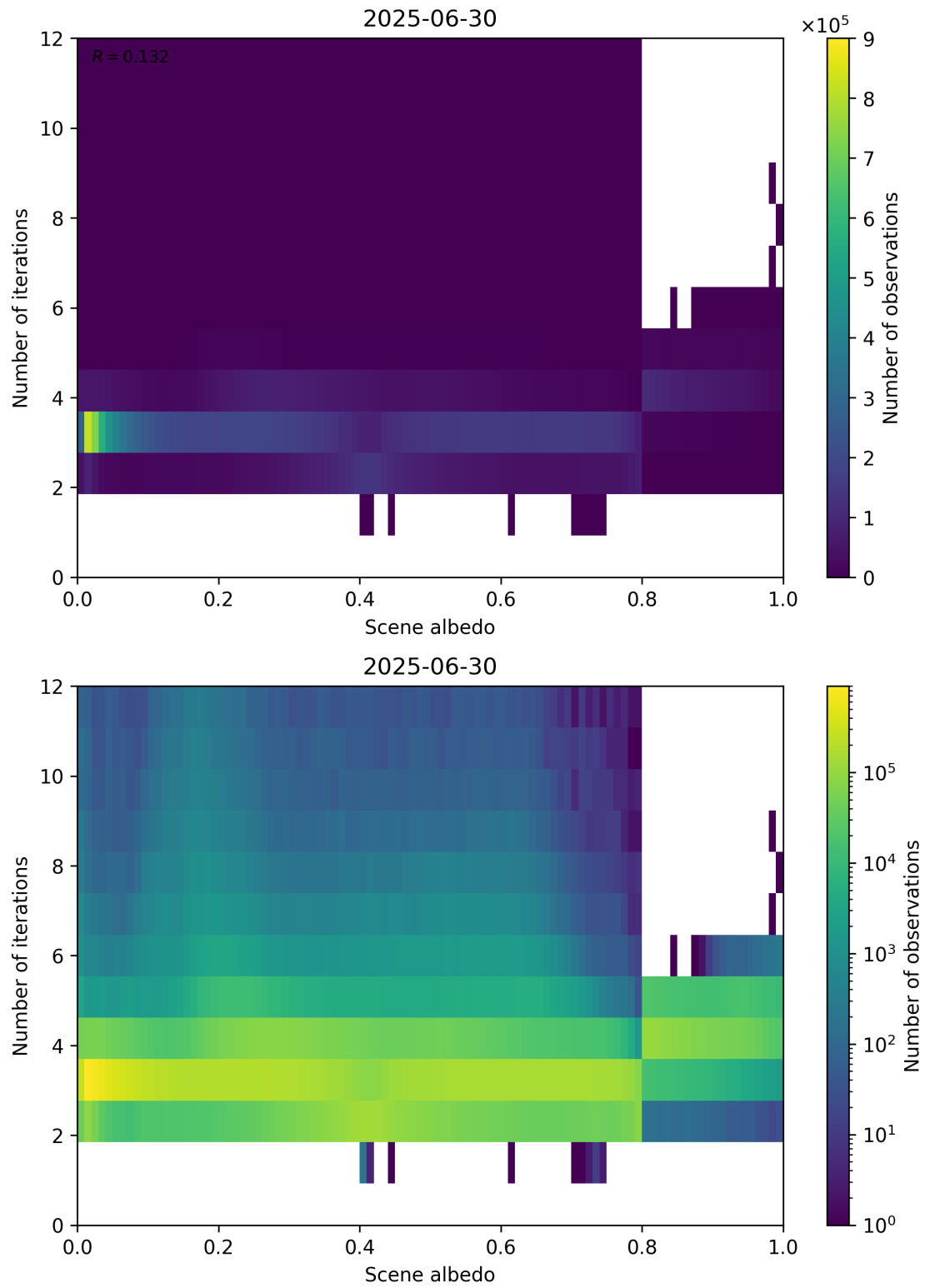
Figure 105: Scatter density plot of “Scene albedo” against “Number of iterations” for 2025-06-29 to 2025-07-01.
