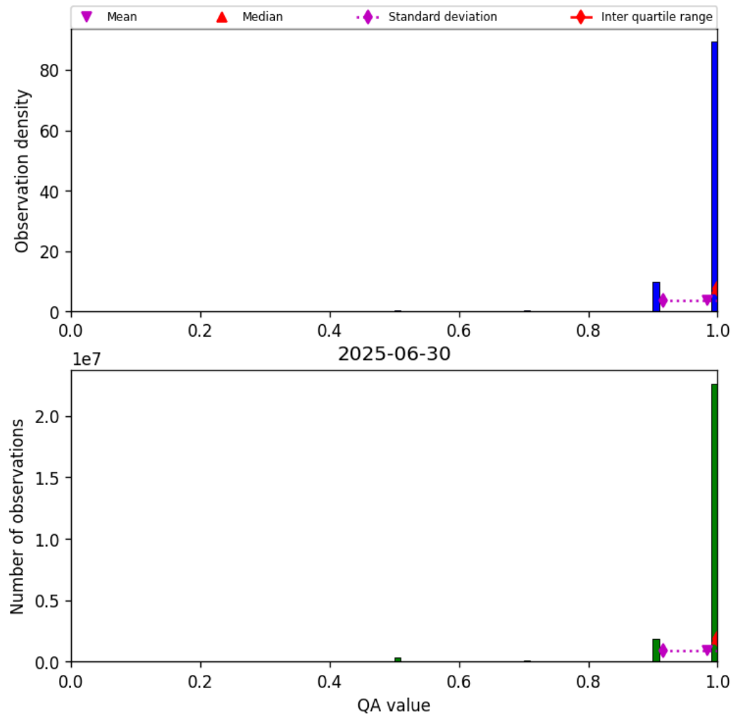
Figure 29: Histogram of “QA value” for 2025-06-29 to 2025-07-01
