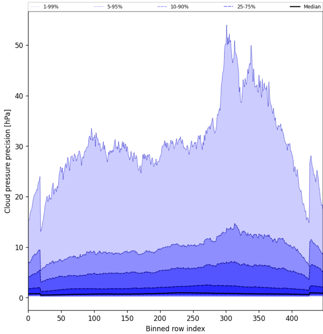
Figure 48: Along track statistics of “Cloud pressure precision” for 2025-06-29 to 2025-07-01
