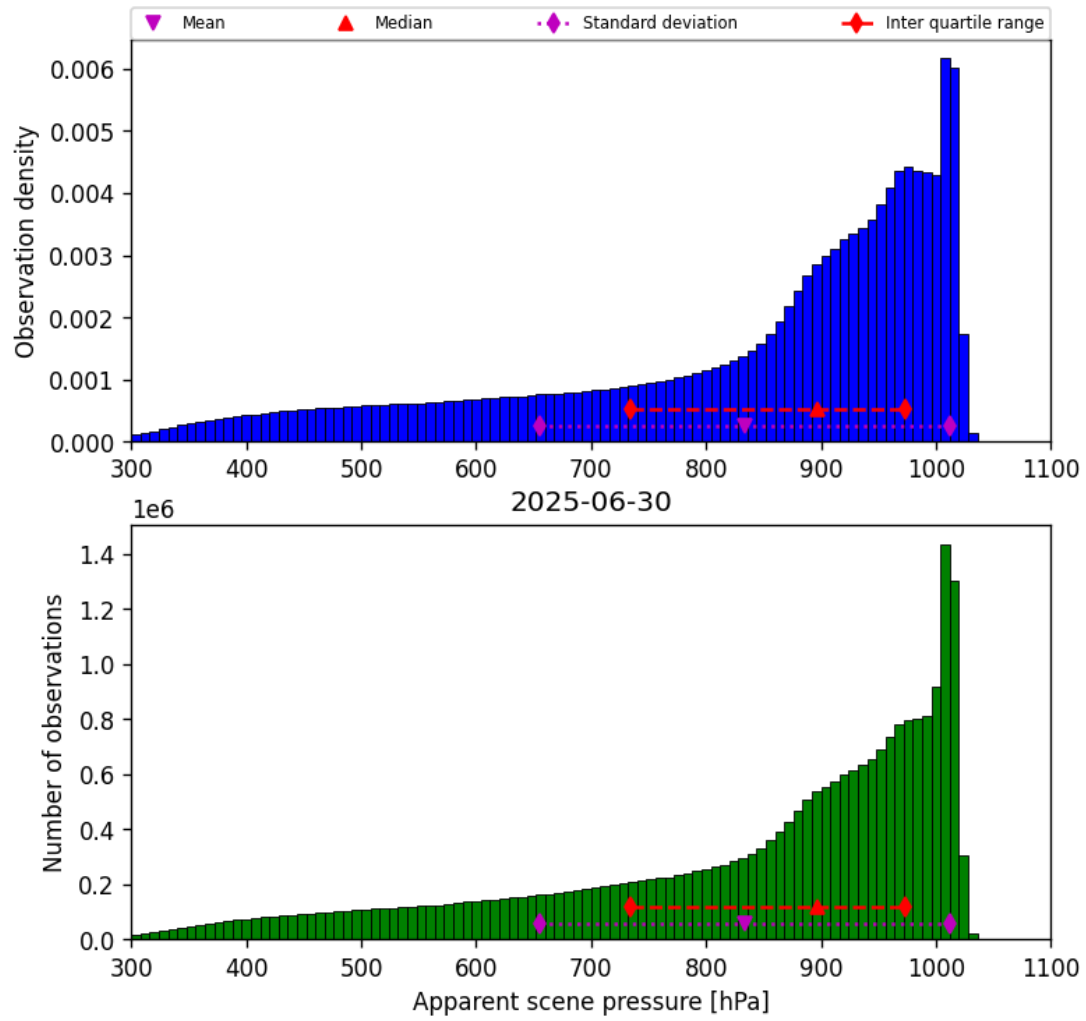
Figure 36: Histogram of “Apparent scene pressure” for 2025-06-29 to 2025-07-01
