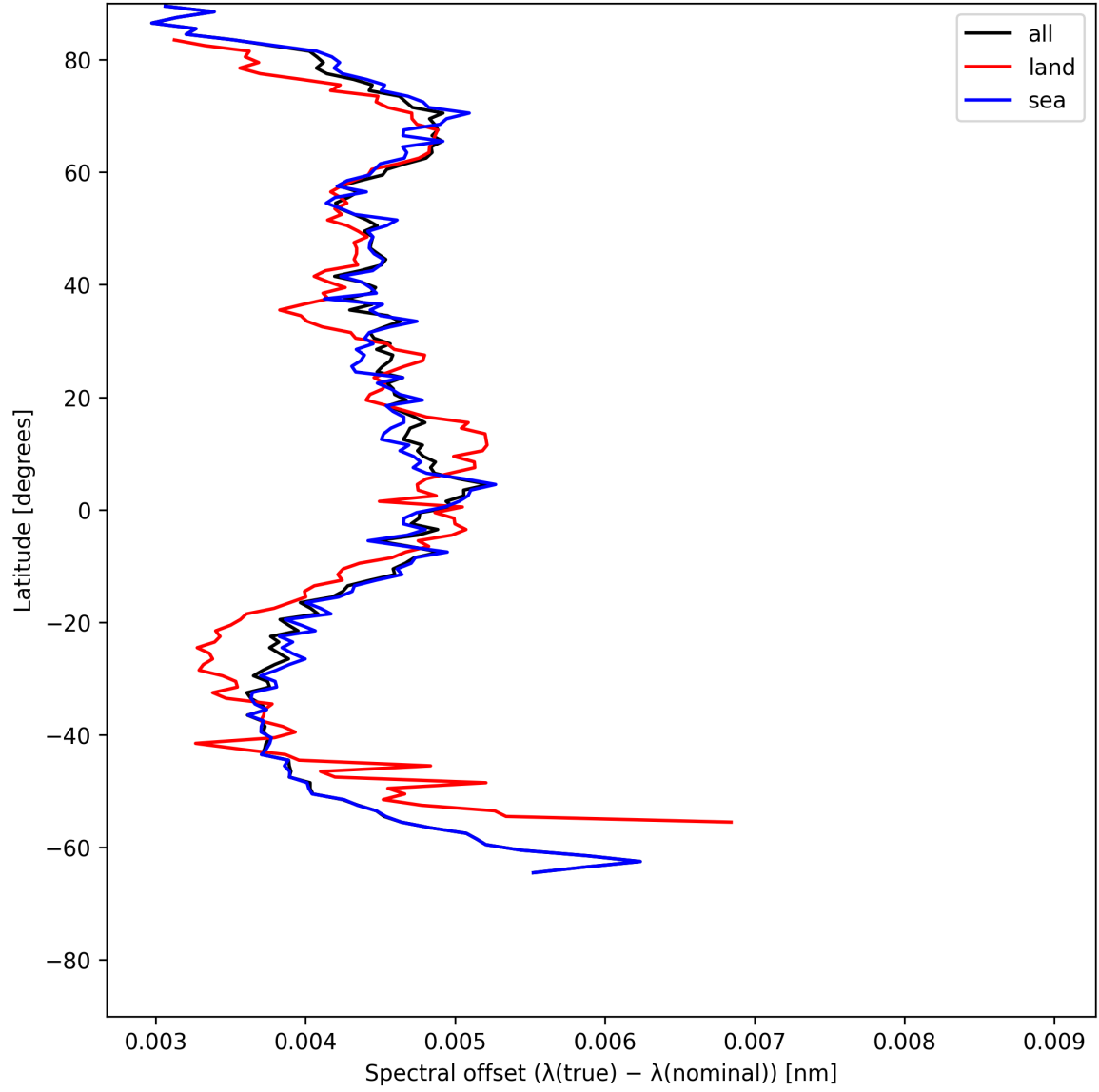
Figure 28: Zonal average of “Spectral offset ( \lambda_{\text{true}} - \lambda_{\text{nominal}} )” for 2025-06-29 to 2025-07-01.
