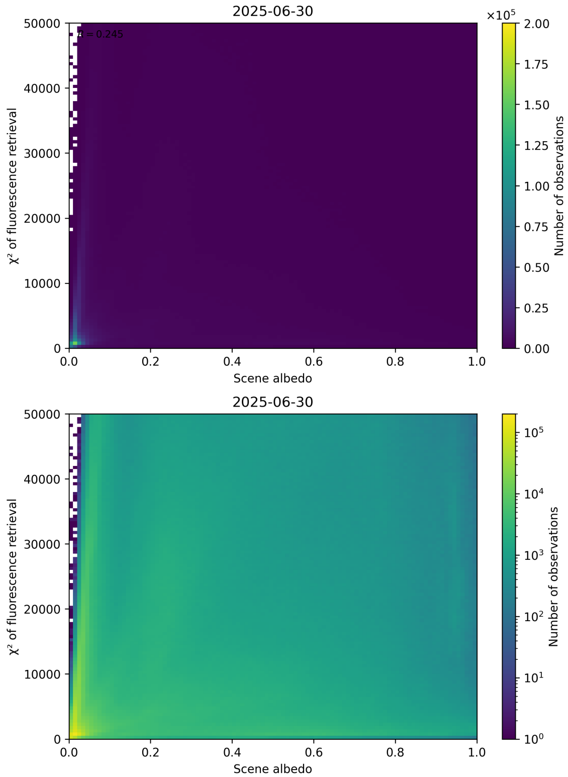
Figure 103: Scatter density plot of “Scene albedo” against “ \chi^2 of fluorescence retrieval” for 2025-06-29 to 2025-07-01.
