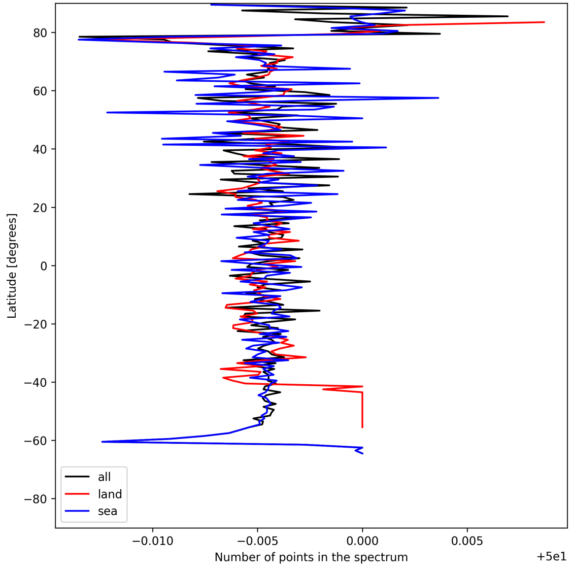
Figure 27: Zonal average of “Number of points in the spectrum” for 2025-06-29 to 2025-07-01.
