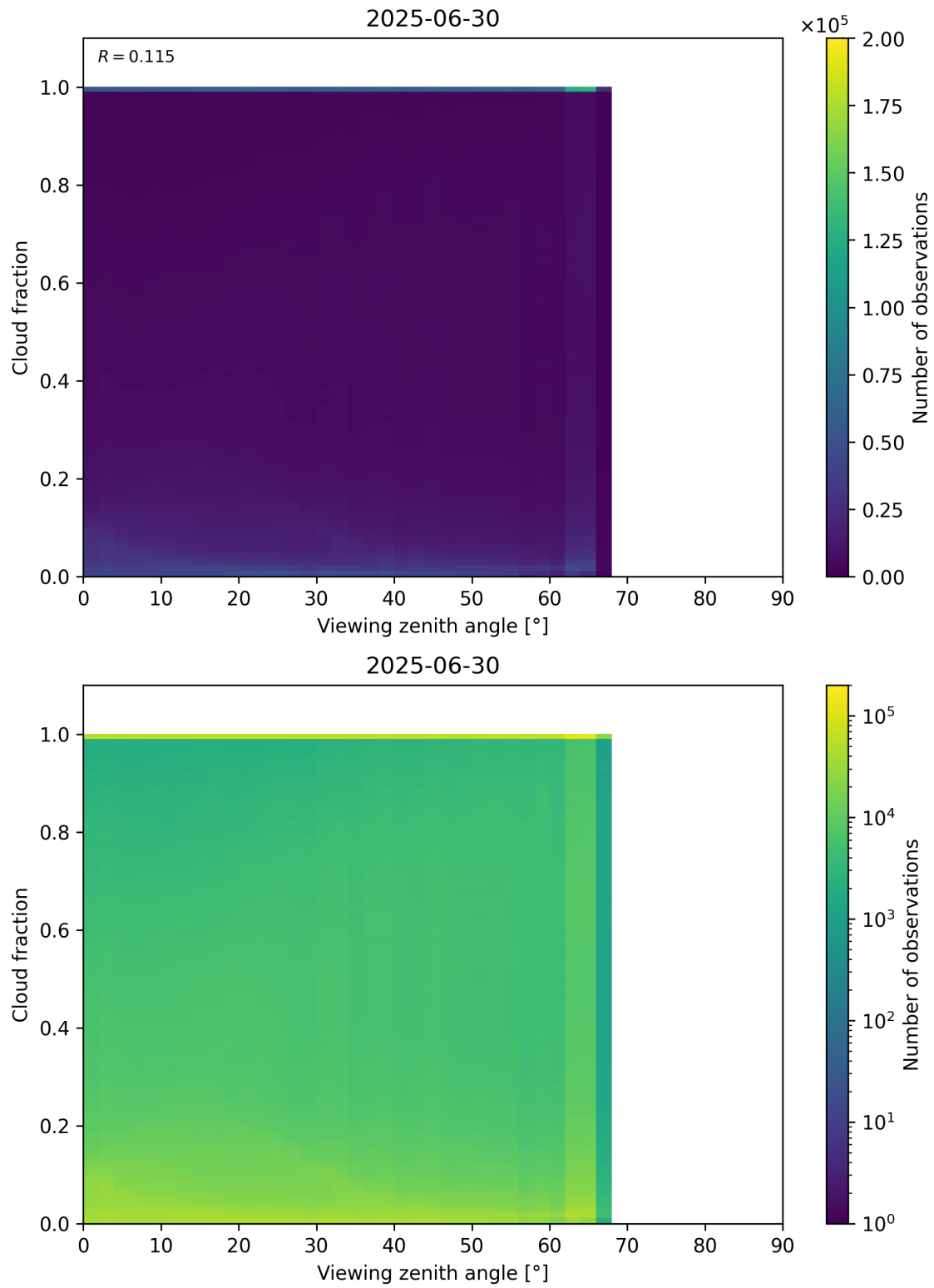
Figure 120: Scatter density plot of “Viewing zenith angle” against “Cloud fraction” for 2025-06-29 to 2025-07-01.
