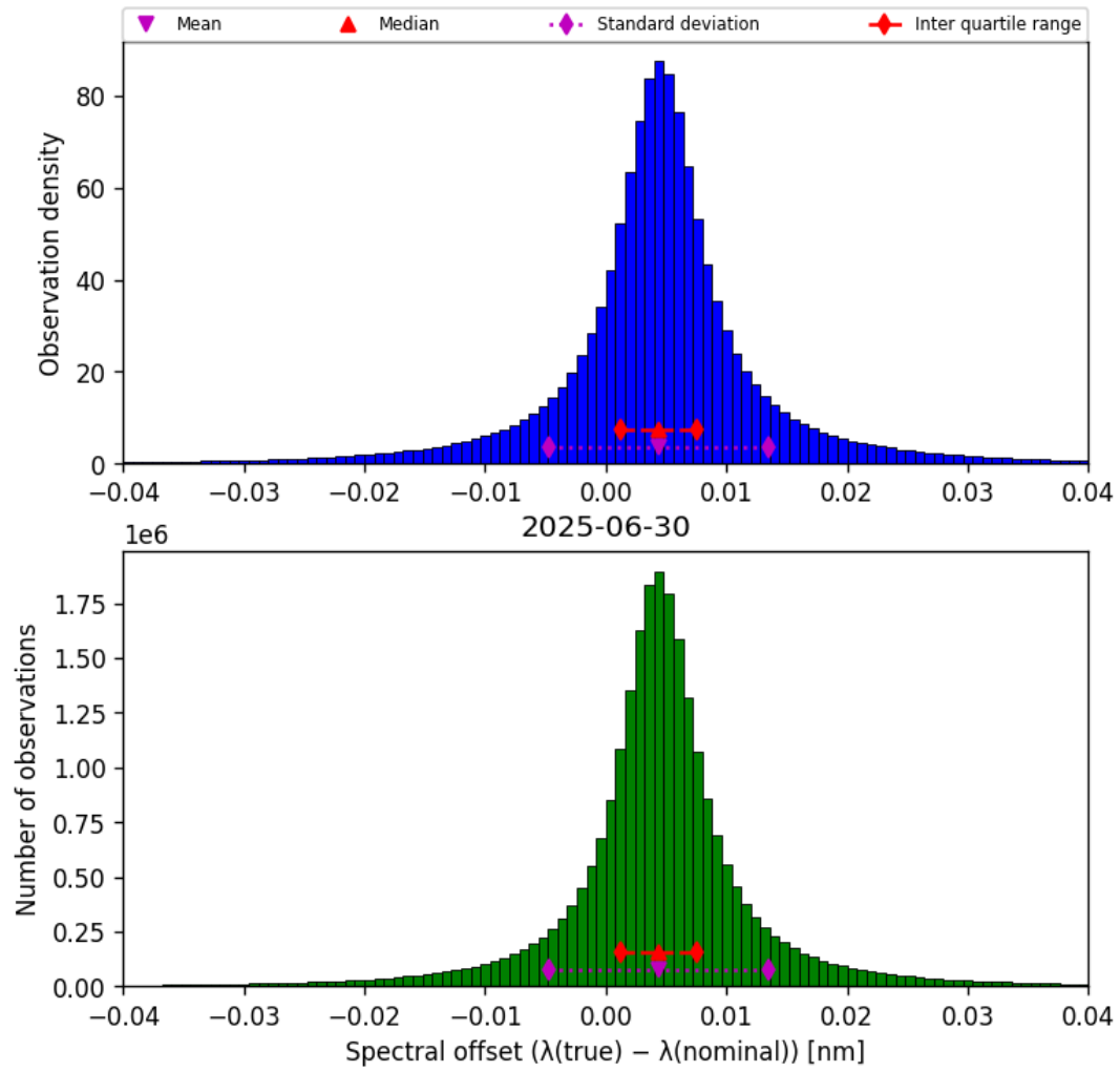
Figure 45: Histogram of “Spectral offset ( \lambda_{\text{true}} - \lambda_{\text{nominal}} )” for 2025-06-29 to 2025-07-01
