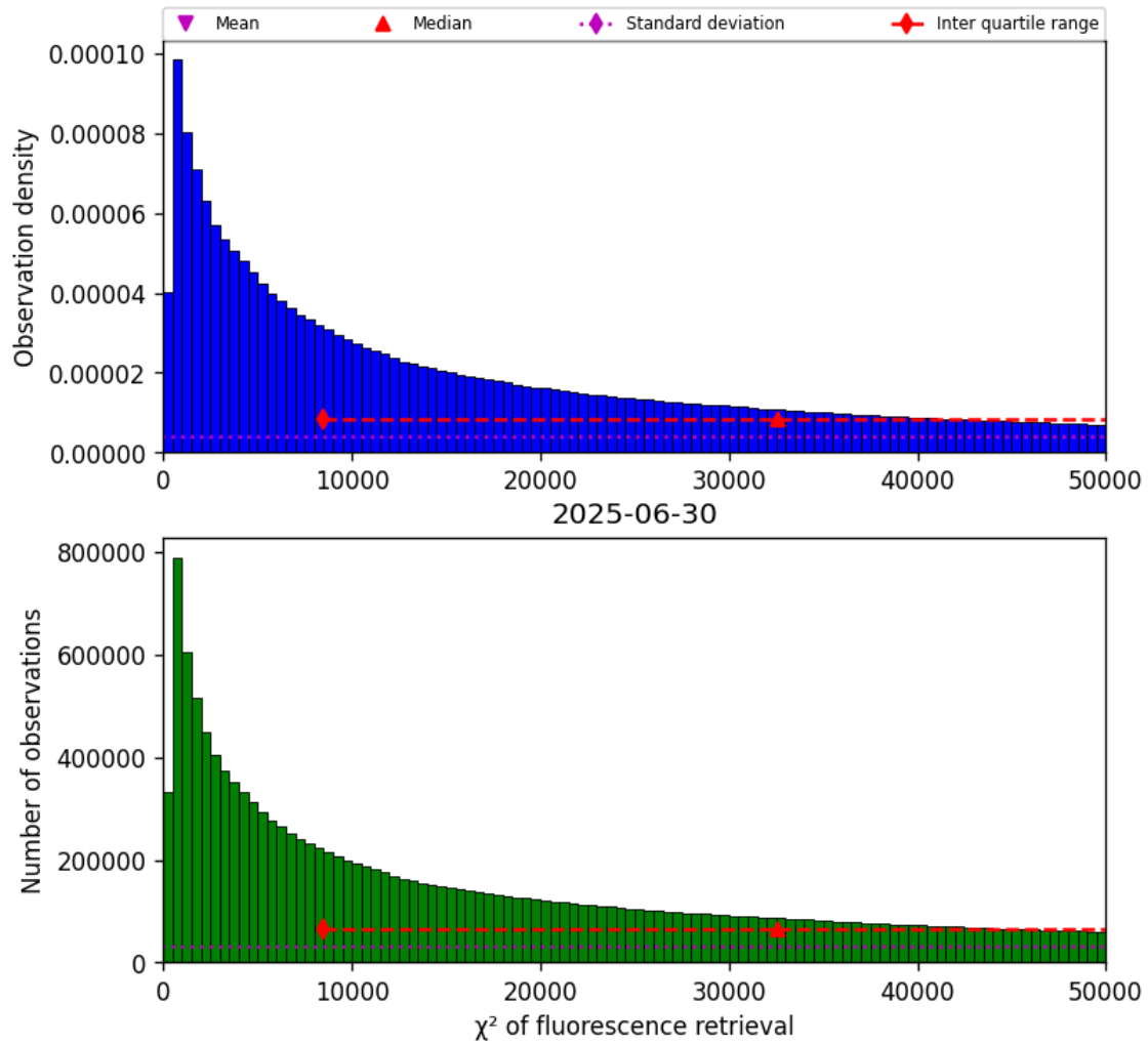
Figure 42: Histogram of “ \chi^2 of fluorescence retrieval” for 2025-06-29 to 2025-07-01
