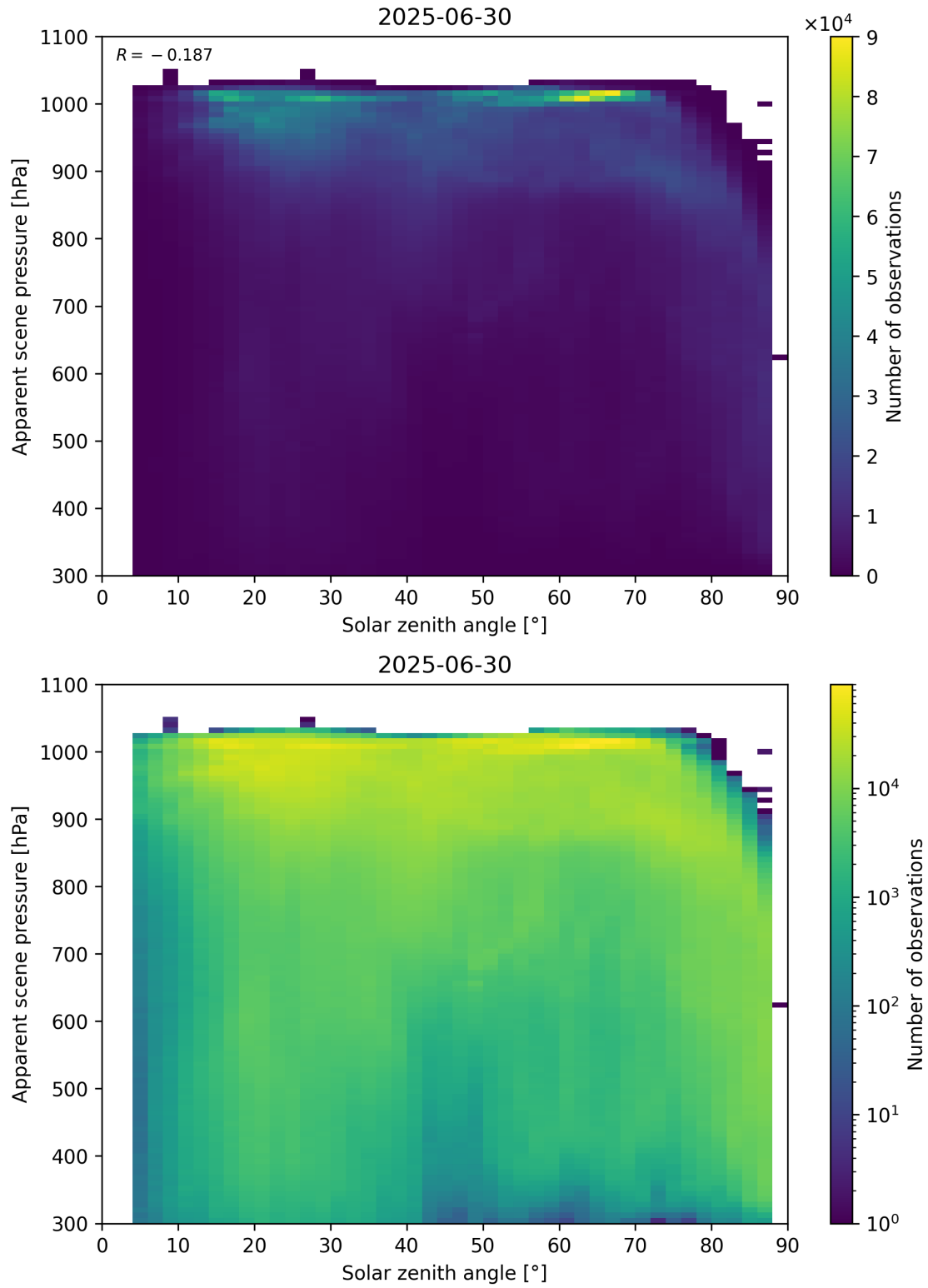
Figure 108: Scatter density plot of “Solar zenith angle” against “Apparent scene pressure” for 2025-06-29 to 2025-07-01.
