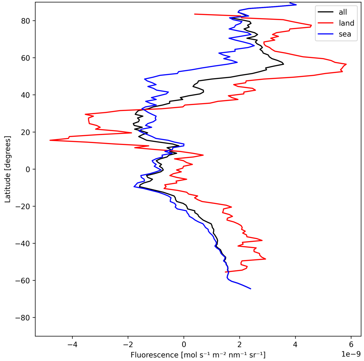
Figure 23: Zonal average of “Fluorescence” for 2025-06-29 to 2025-07-01.
