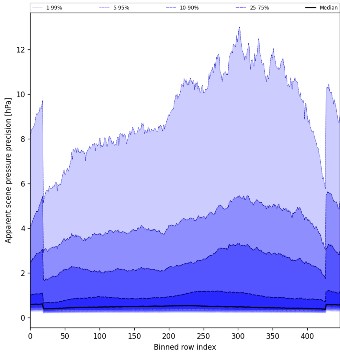
Figure 54: Along track statistics of “Apparent scene pressure precision” for 2025-06-29 to 2025-07-01
