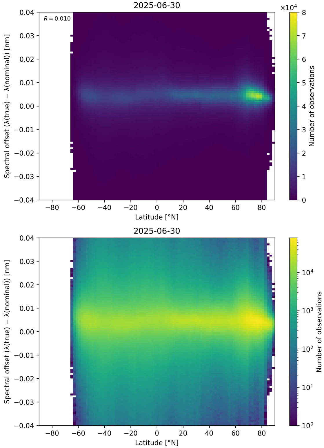
Figure 96: Scatter density plot of “Latitude” against “Spectral offset ( \lambda_{\text{true}} - \lambda_{\text{nominal}} )” for 2025-06-29 to 2025-07-01.
