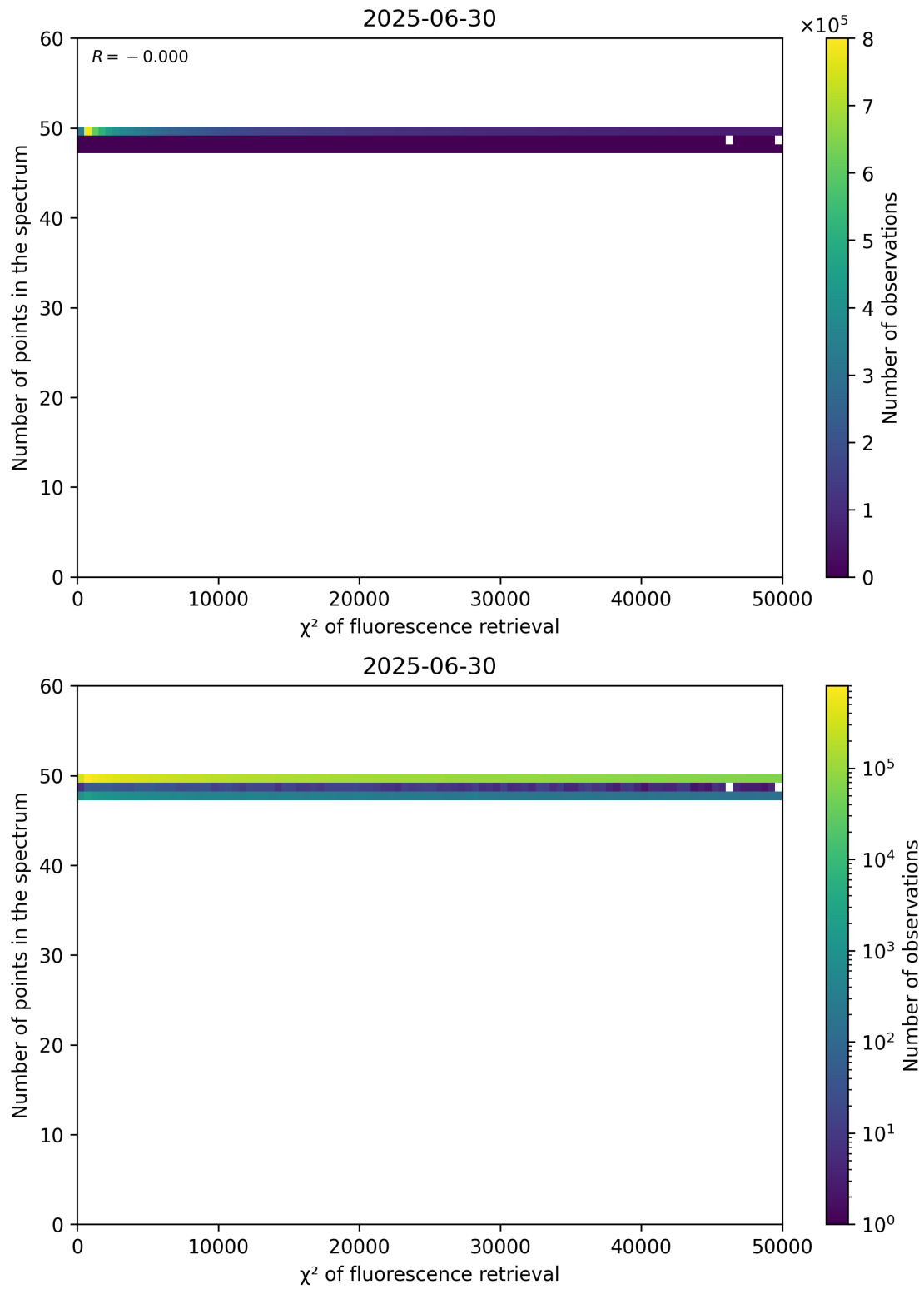
Figure 68: Scatter density plot of " \chi^2 of fluorescence retrieval" against "Number of points in the spectrum" for 2025-06-29 to 2025-07-01.
