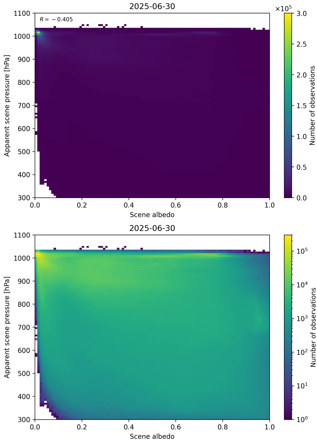
Figure 102: Scatter density plot of “Scene albedo” against “Apparent scene pressure” for 2025-06-29 to 2025-07-01.
