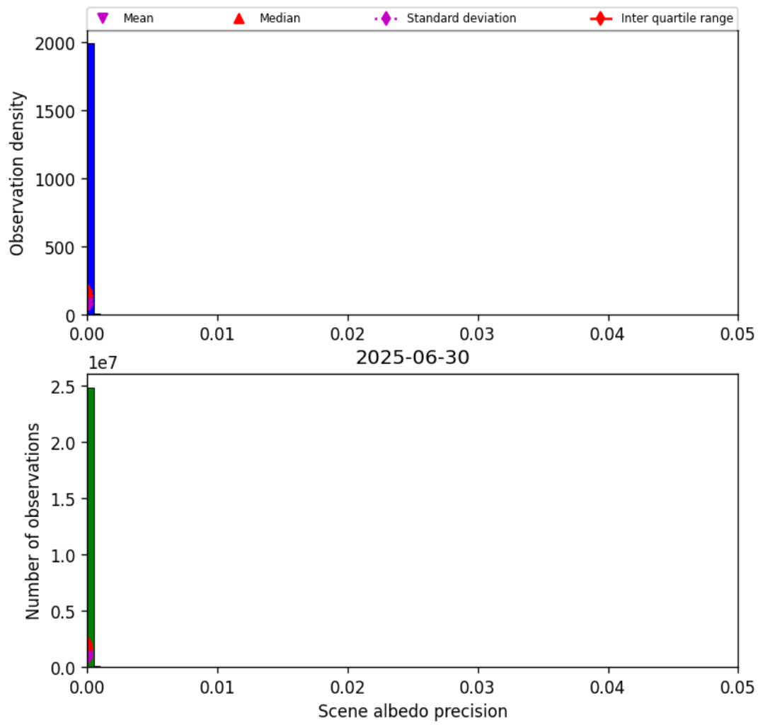
Figure 35: Histogram of “Scene albedo precision” for 2025-06-29 to 2025-07-01
