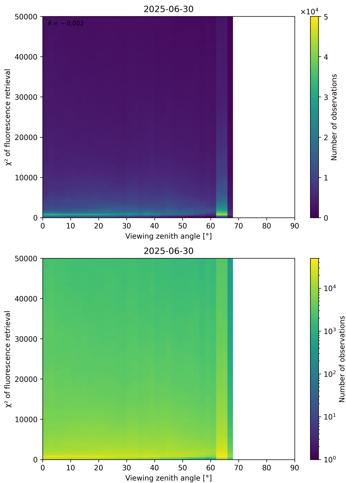
Figure 119: Scatter density plot of “Viewing zenith angle” against “ \chi^2 of fluorescence retrieval” for 2025-06-29 to 2025-07-01.
