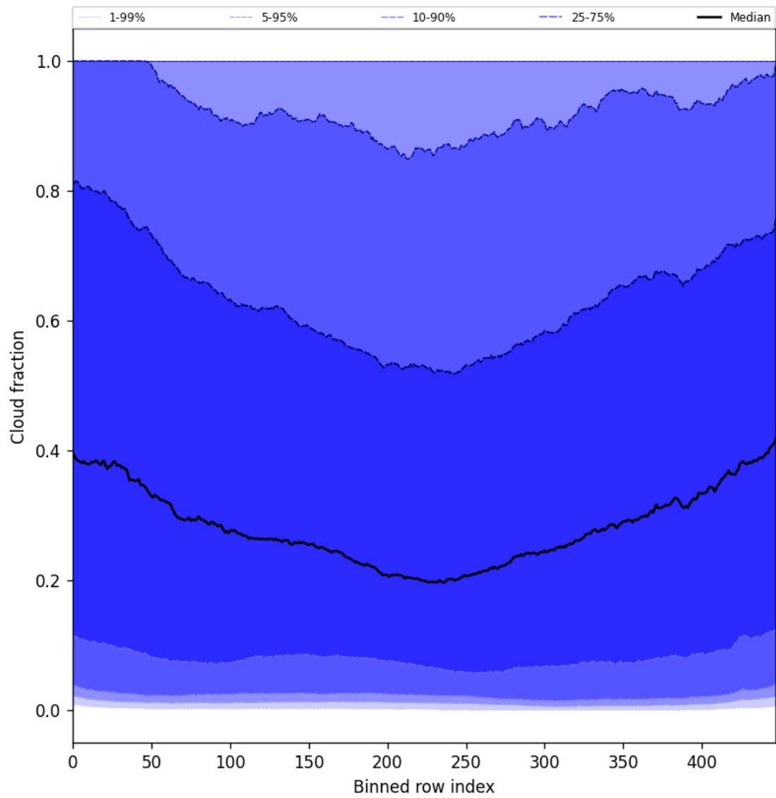
Figure 49: Along track statistics of “Cloud fraction” for 2025-06-29 to 2025-07-01
