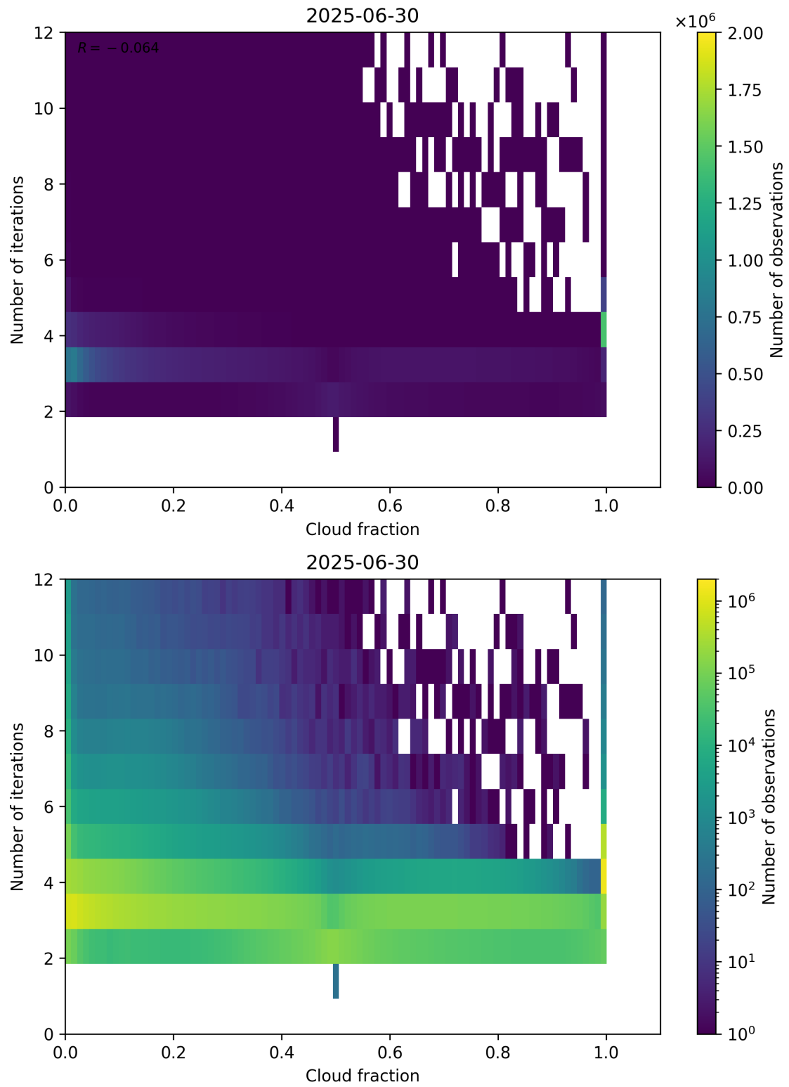
Figure 73: Scatter density plot of “Cloud fraction” against “Number of iterations” for 2025-06-29 to 2025-07-01.
