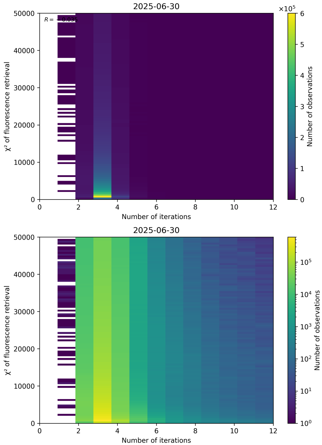
Figure 97: Scatter density plot of “Number of iterations” against “ \chi^2 of fluorescence retrieval” for 2025-06-29 to 2025-07-01.
