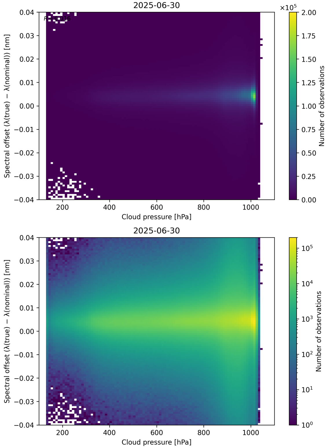
Figure 84: Scatter density plot of “Cloud pressure” against “Spectral offset ( \lambda_{\text{true}} - \lambda_{\text{nominal}} )” for 2025-06-29 to 2025-07-01.
