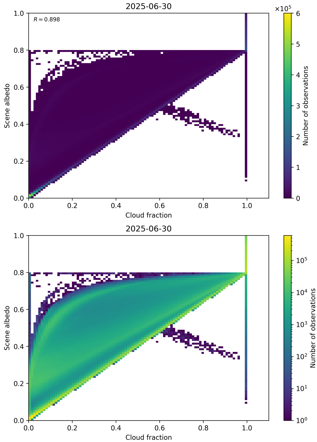
Figure 75: Scatter density plot of “Cloud fraction” against “Scene albedo” for 2025-06-29 to 2025-07-01.
