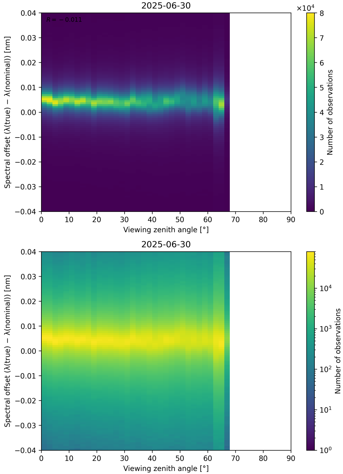
Figure 128: Scatter density plot of “Viewing zenith angle” against “Spectral offset ( \lambda_{\text{true}} - \lambda_{\text{nominal}} )” for 2025-06-29 to 2025-07-01.
