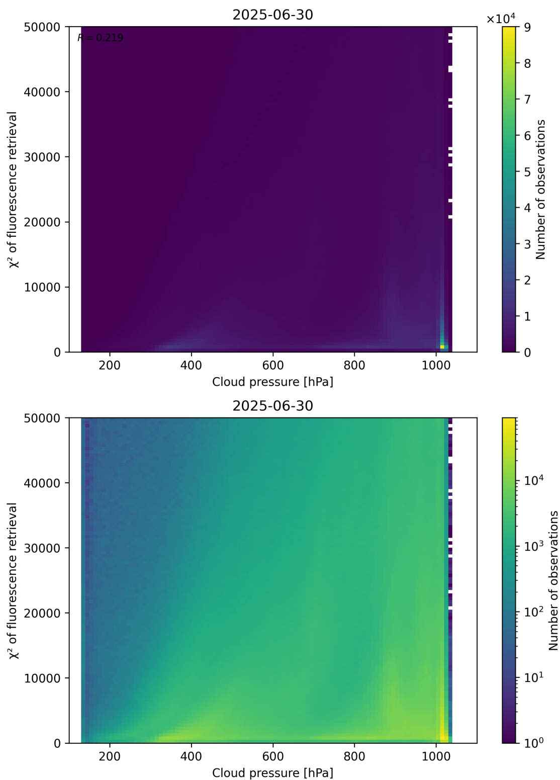
Figure 78: Scatter density plot of “Cloud pressure” against “ \chi^2 of fluorescence retrieval” for 2025-06-29 to 2025-07-01.
