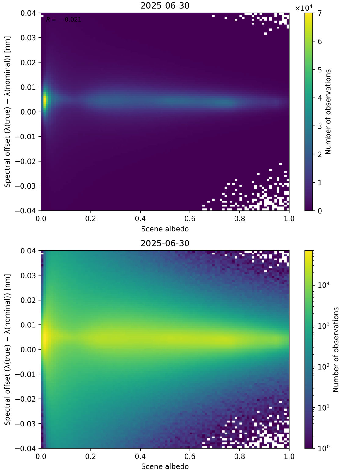
Figure 107: Scatter density plot of “Scene albedo” against “Spectral offset ( \lambda_{\text{true}} - \lambda_{\text{nominal}} )” for 2025-06-29 to 2025-07-01.
