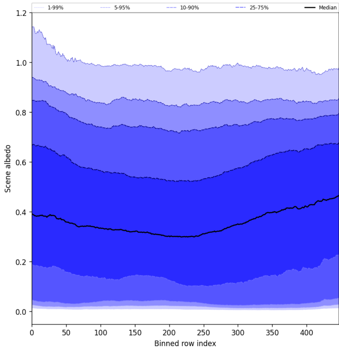
Figure 51: Along track statistics of “Scene albedo” for 2025-06-29 to 2025-07-01
