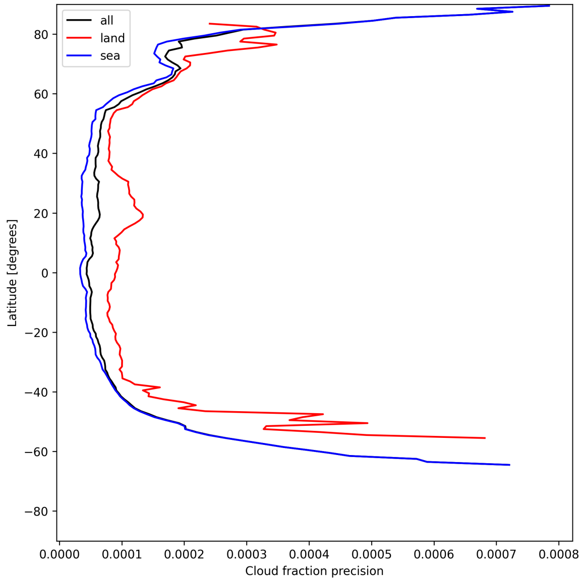
Figure 16: Zonal average of “Cloud fraction precision” for 2025-06-29 to 2025-07-01.
