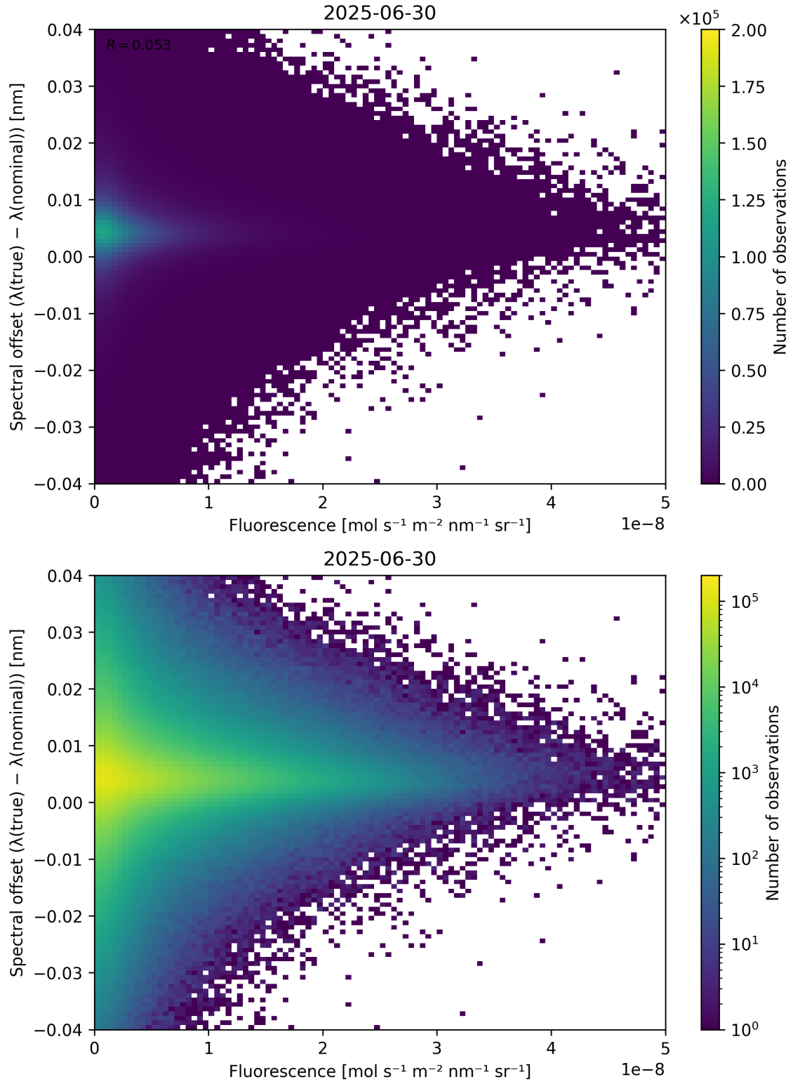
Figure 87: Scatter density plot of “Fluorescence” against “Spectral offset ( \lambda_{\text{true}} - \lambda_{\text{nominal}} )” for 2025-06-29 to 2025-07-01.
