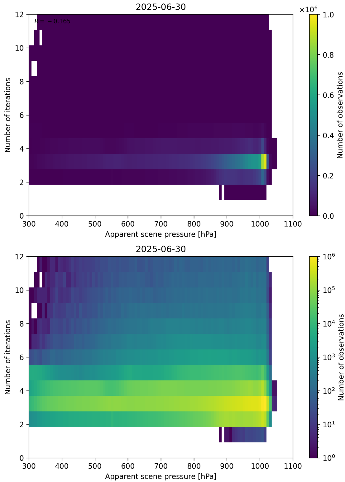
Figure 65: Scatter density plot of “Apparent scene pressure” against “Number of iterations” for 2025-06-29 to 2025-07-01.
