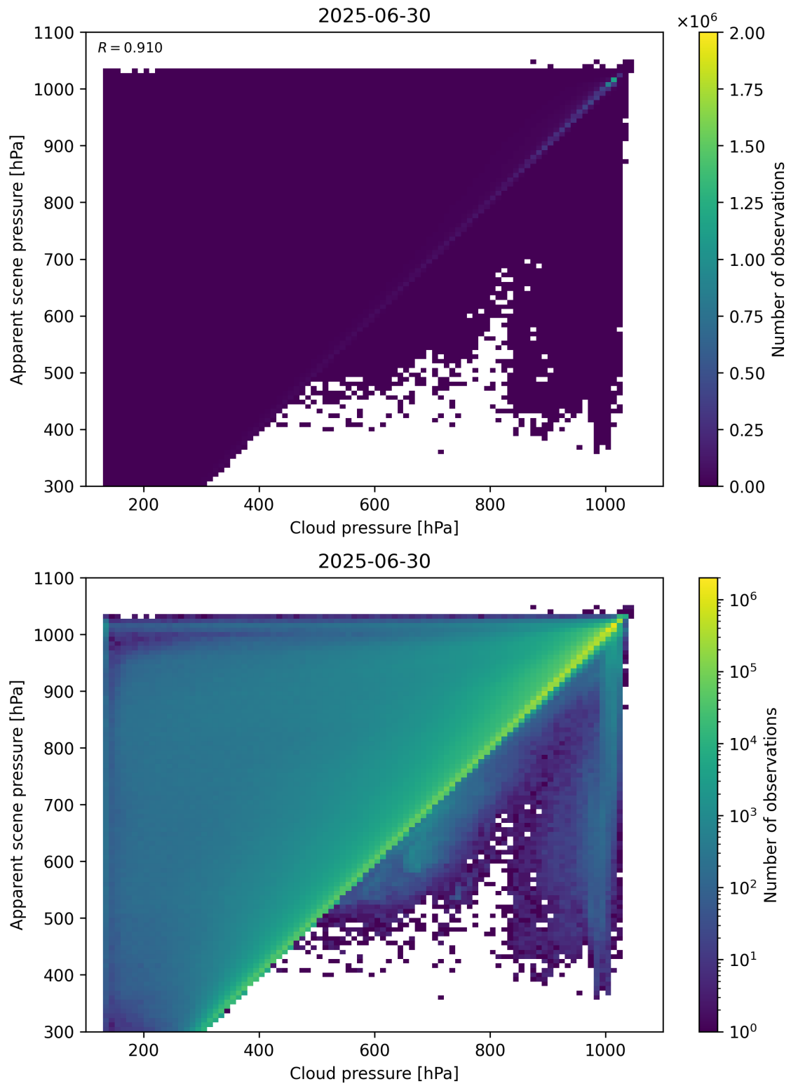
Figure 77: Scatter density plot of “Cloud pressure” against “Apparent scene pressure” for 2025-06-29 to 2025-07-01.
