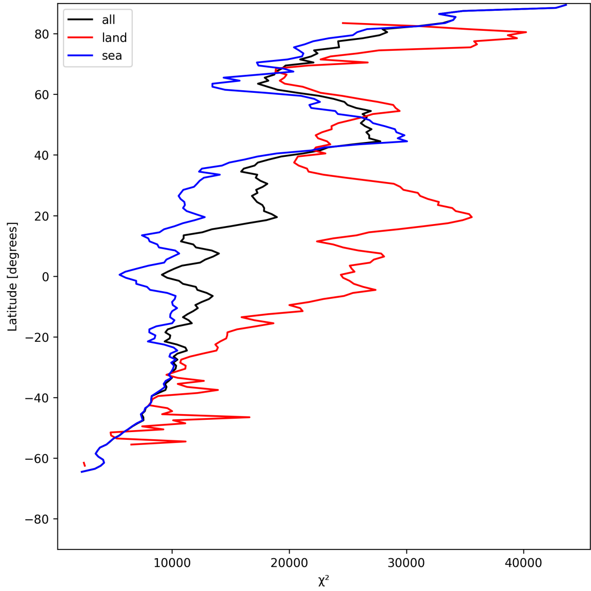
Figure 21: Zonal average of “ \chi^2 ” for 2025-06-30 to 2025-07-02.
