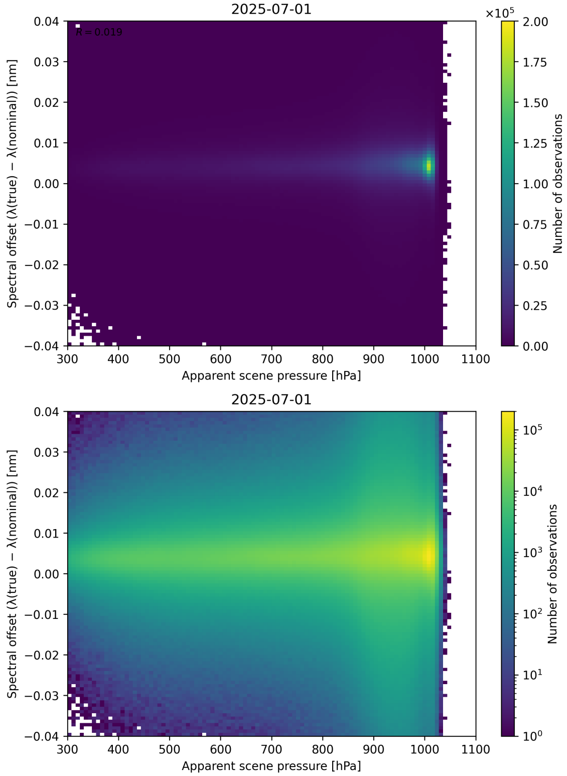
Figure 67: Scatter density plot of “Apparent scene pressure” against “Spectral offset ( \lambda_{\text{true}} - \lambda_{\text{nominal}} )” for 2025-06-30 to 2025-07-02.
