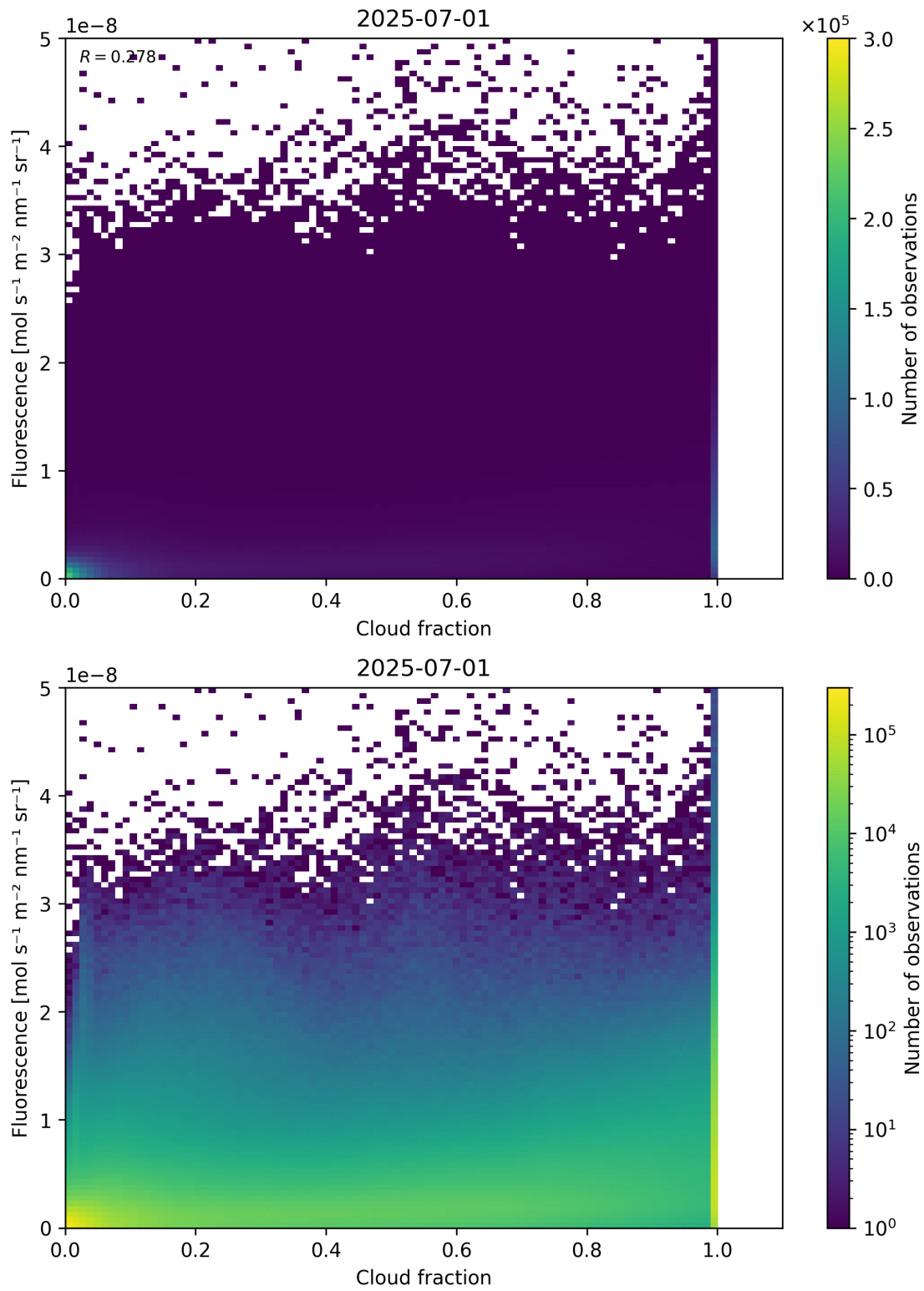
Figure 72: Scatter density plot of “Cloud fraction” against “Fluorescence” for 2025-06-30 to 2025-07-02.
