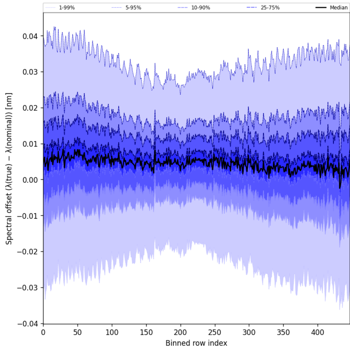
Figure 62: Along track statistics of “Spectral offset ( \lambda_{\text{true}} - \lambda_{\text{nominal}} )” for 2025-06-30 to 2025-07-02
