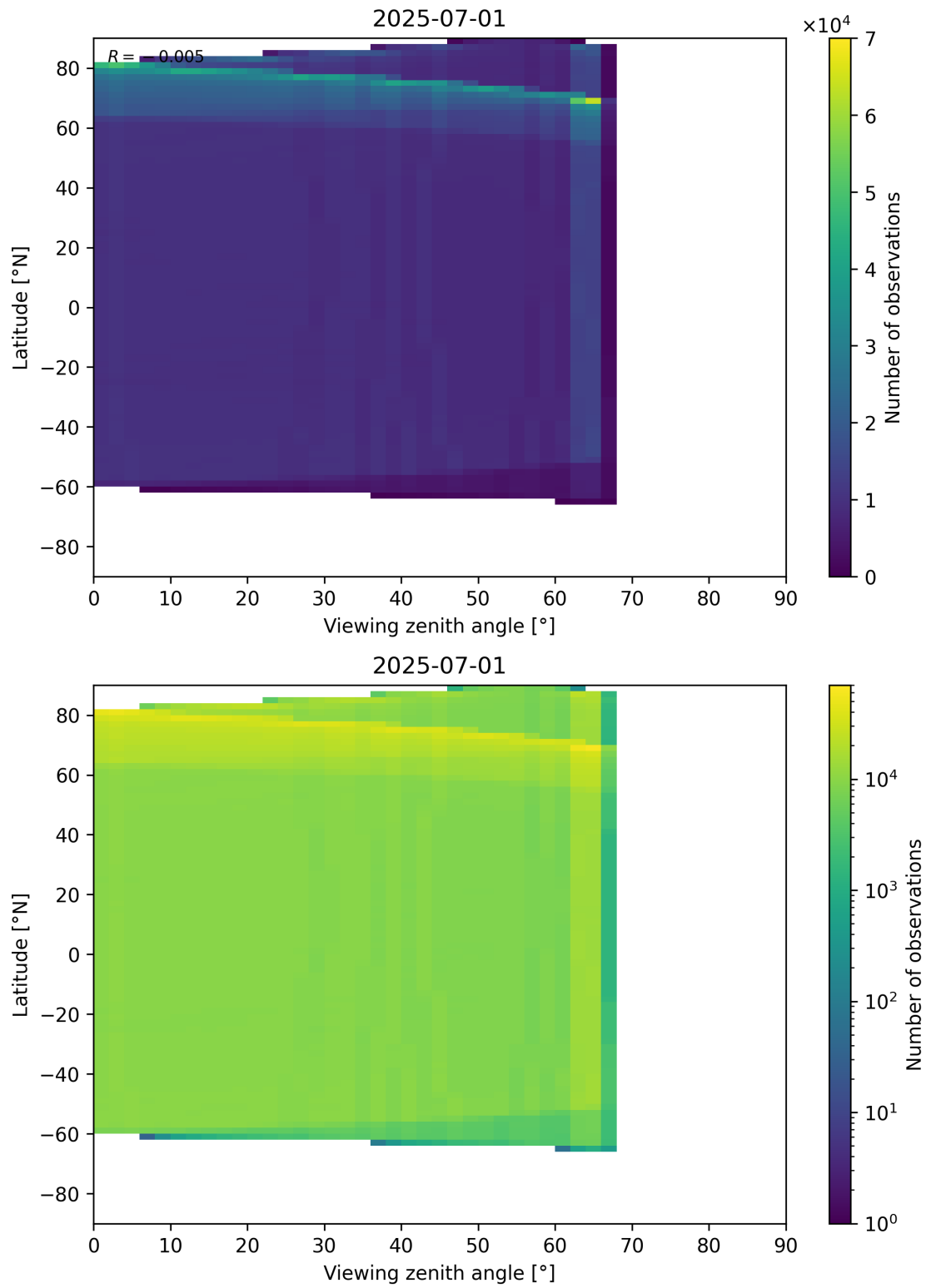
Figure 123: Scatter density plot of “Viewing zenith angle” against “Latitude” for 2025-06-30 to 2025-07-02.
