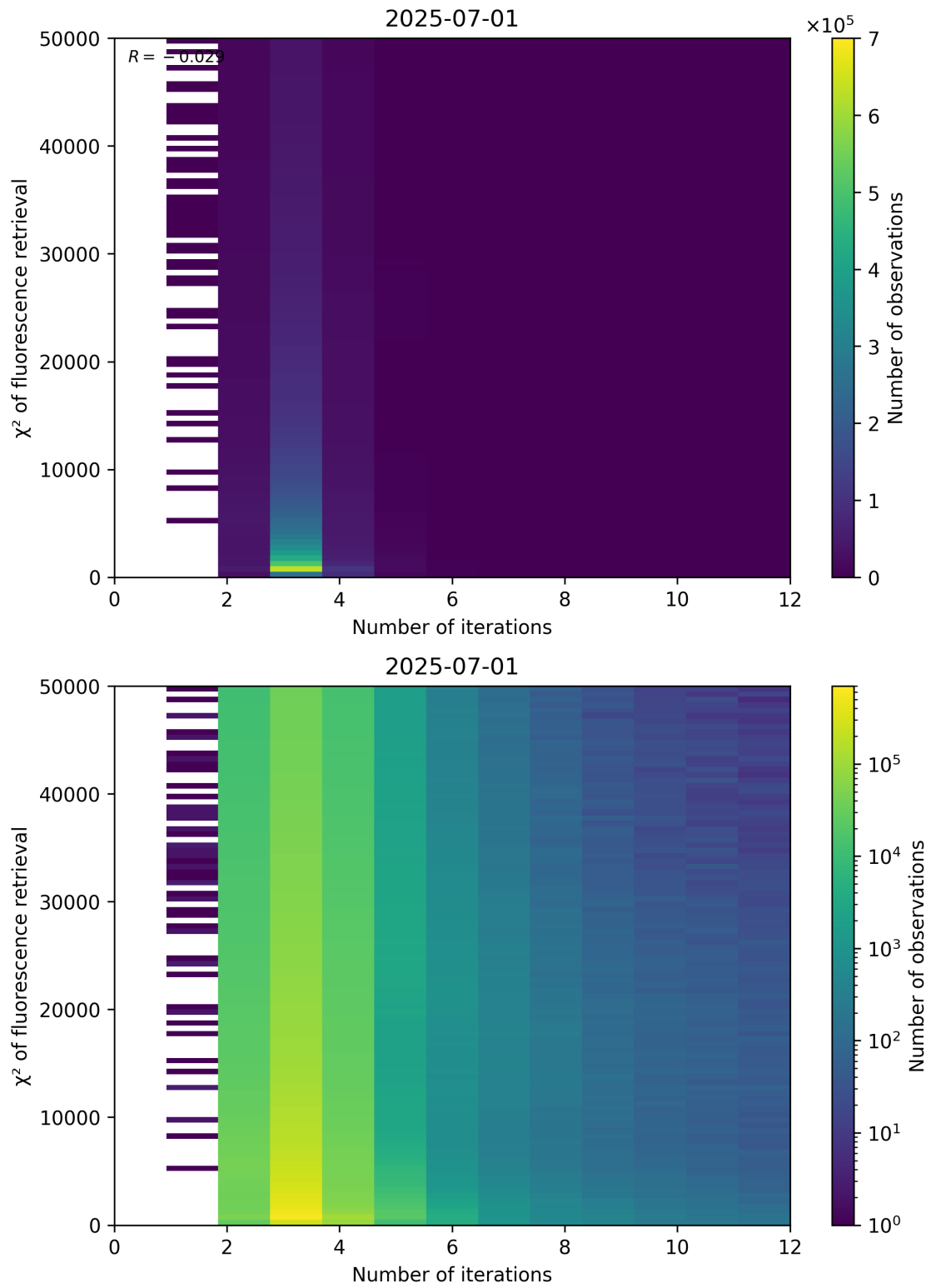
Figure 97: Scatter density plot of “Number of iterations” against “ \chi^2 of fluorescence retrieval” for 2025-06-30 to 2025-07-02.
