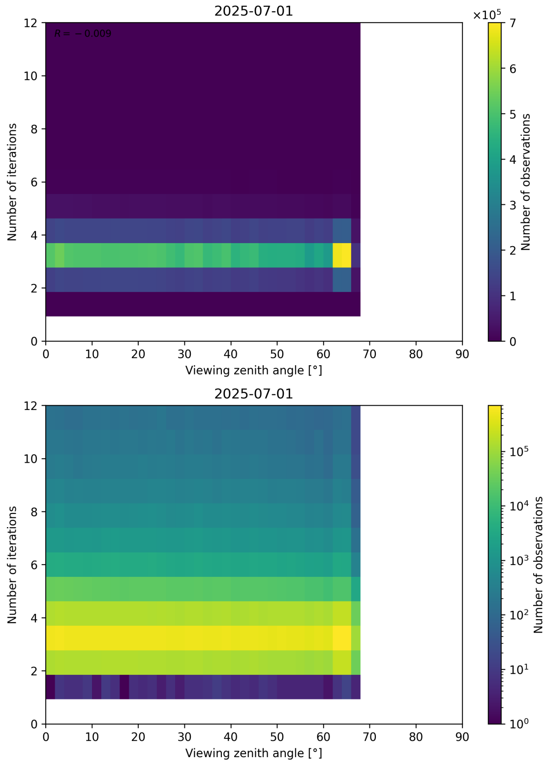
Figure 124: Scatter density plot of “Viewing zenith angle” against “Number of iterations” for 2025-06-30 to 2025-07-02.
