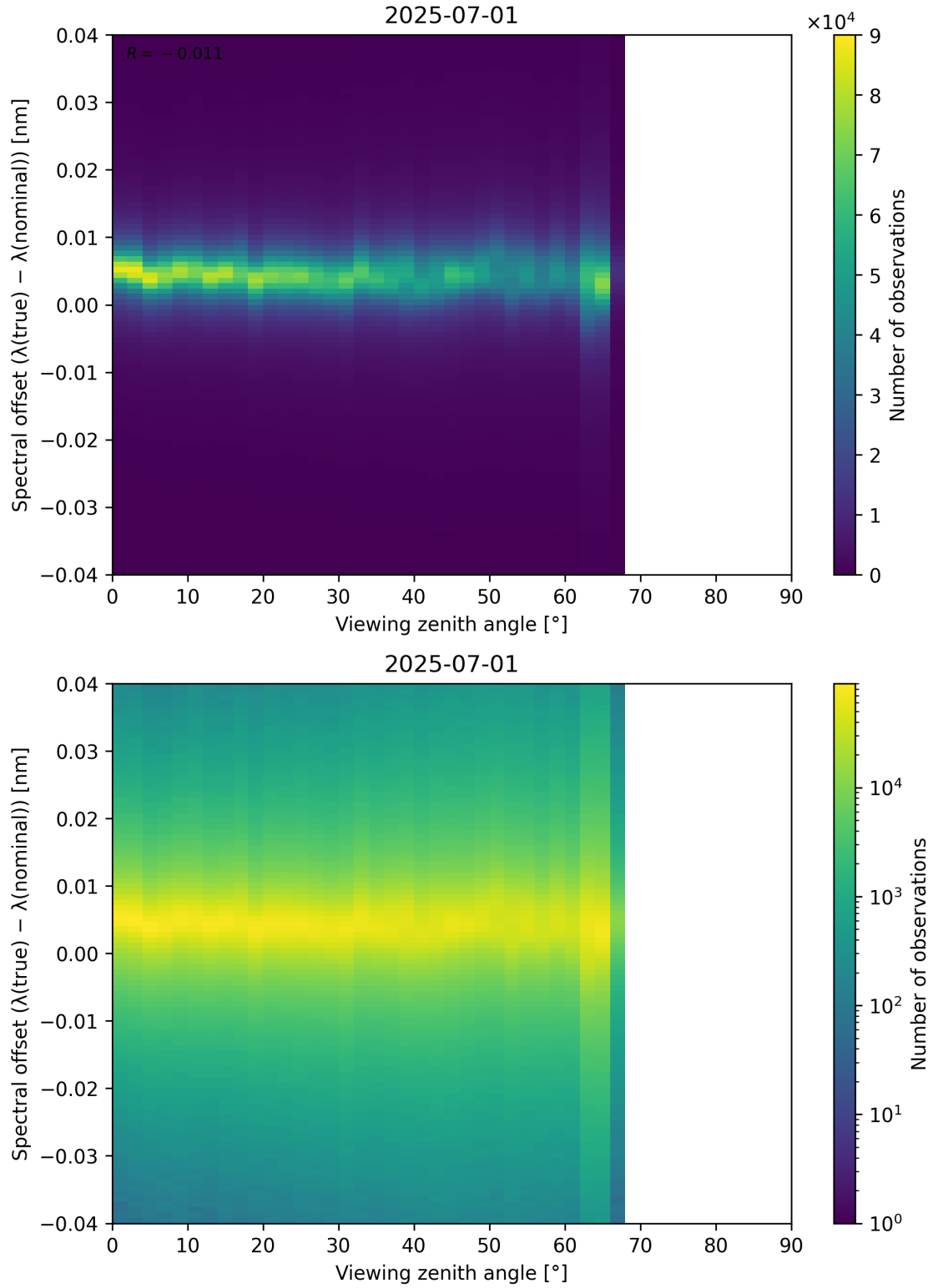
Figure 128: Scatter density plot of “Viewing zenith angle” against “Spectral offset ( \lambda_{\text{true}} - \lambda_{\text{nominal}} )” for 2025-06-30 to 2025-07-02.
