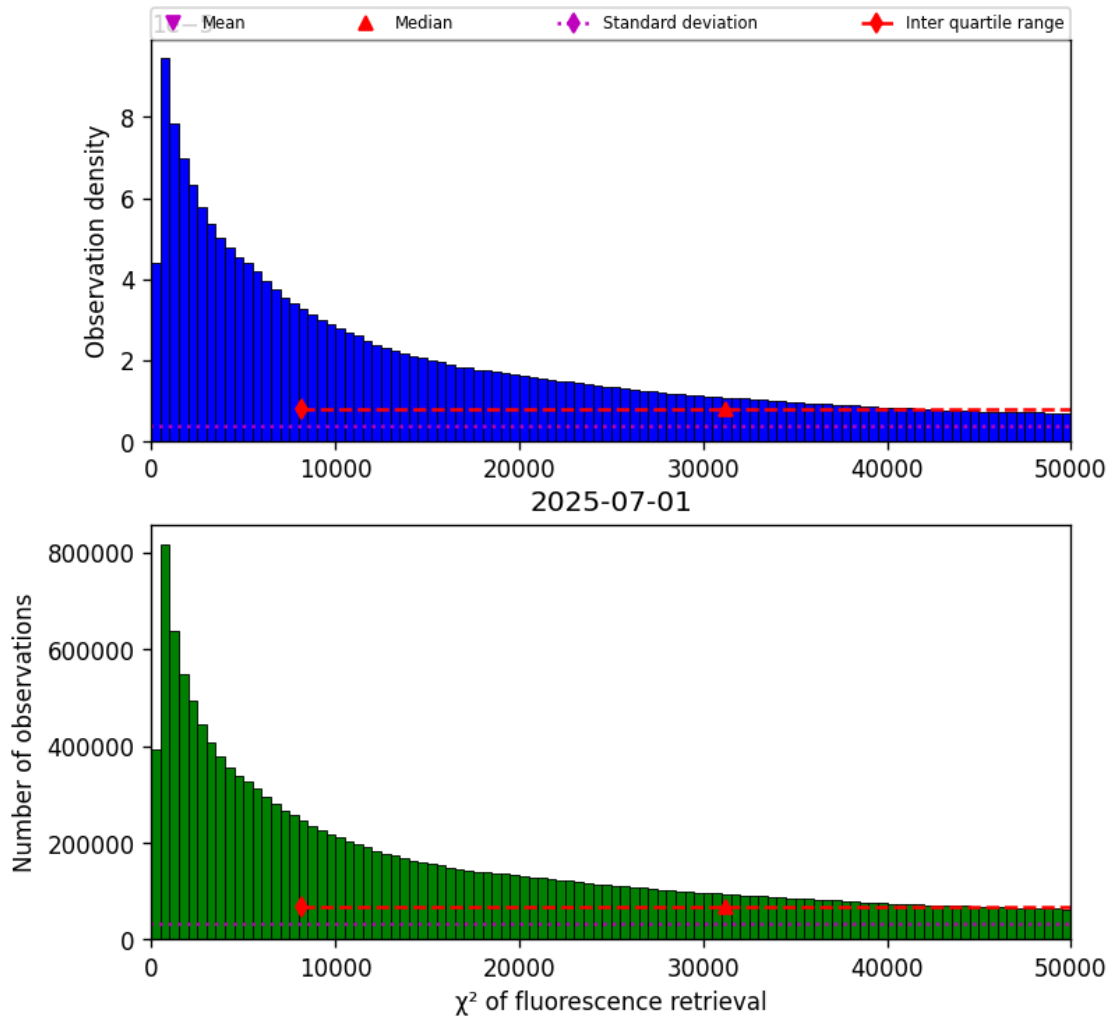
Figure 42: Histogram of “ \chi^2 of fluorescence retrieval” for 2025-06-30 to 2025-07-02
