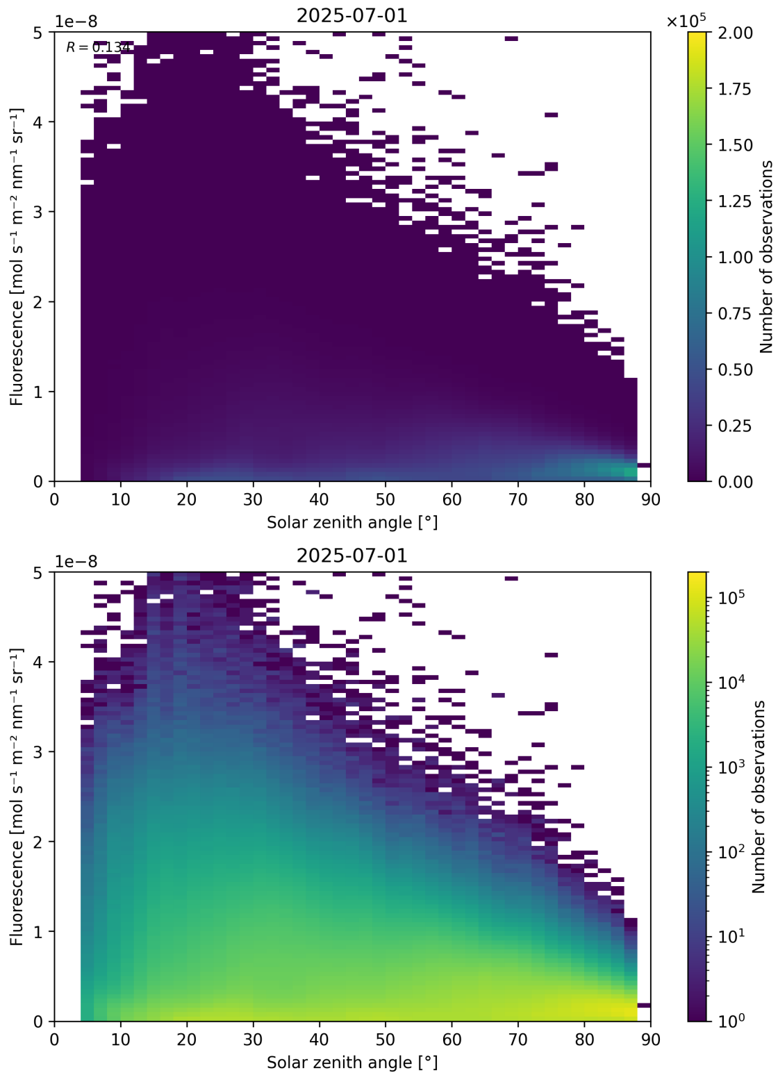
Figure 112: Scatter density plot of “Solar zenith angle” against “Fluorescence” for 2025-06-30 to 2025-07-02.
