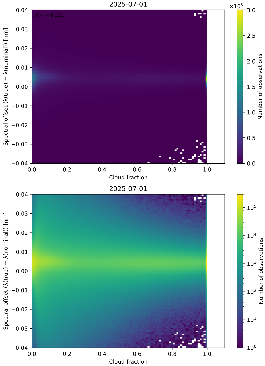
Figure 76: Scatter density plot of “Cloud fraction” against “Spectral offset ( \lambda_{\text{true}} - \lambda_{\text{nominal}} )” for 2025-06-30 to 2025-07-02.
