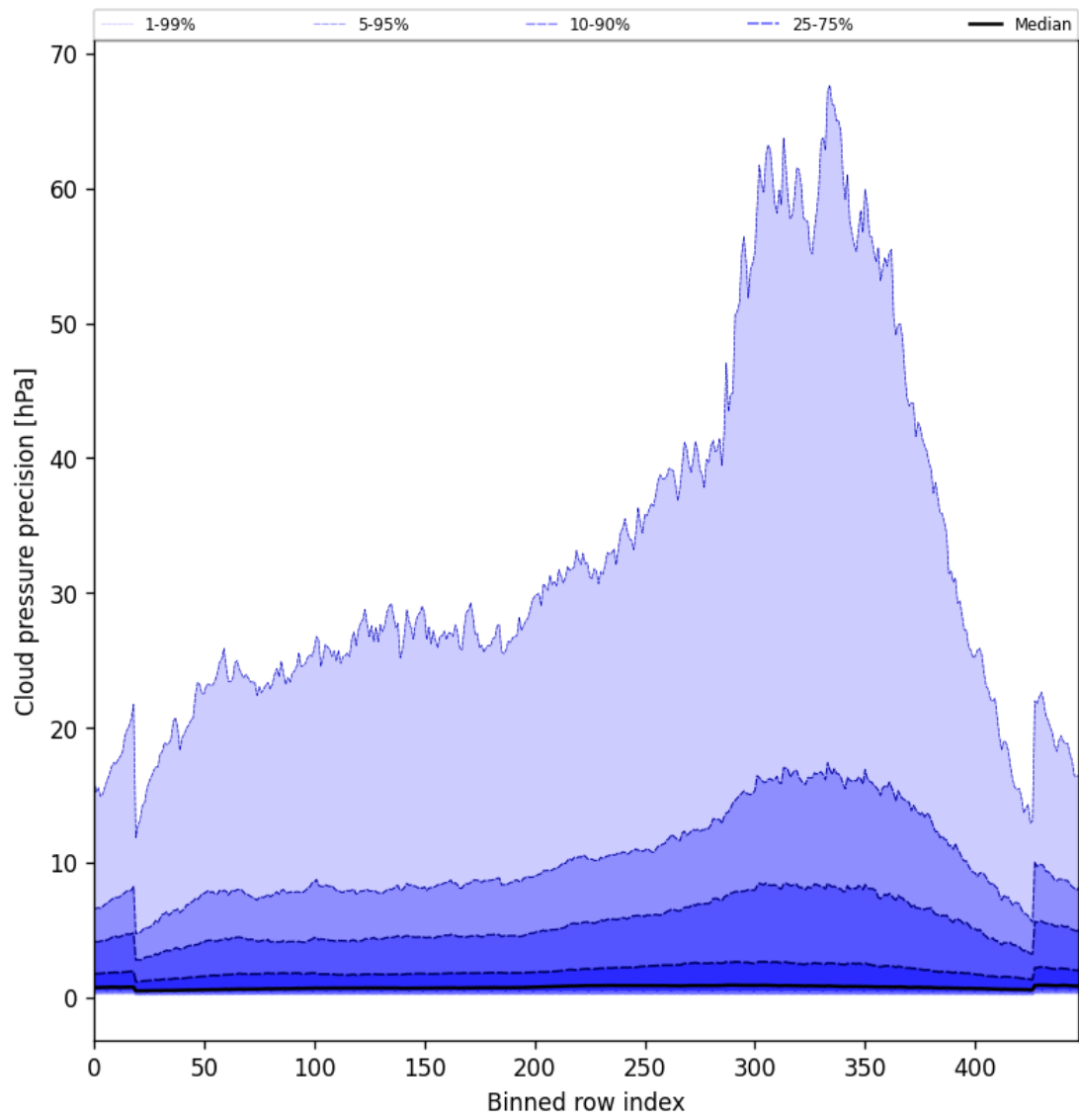
Figure 48: Along track statistics of “Cloud pressure precision” for 2025-06-30 to 2025-07-02
