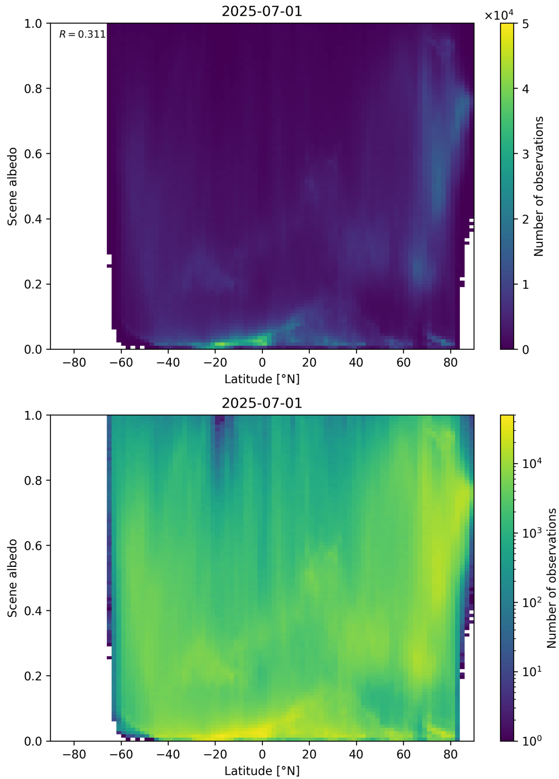
Figure 95: Scatter density plot of “Latitude” against “Scene albedo” for 2025-06-30 to 2025-07-02.
