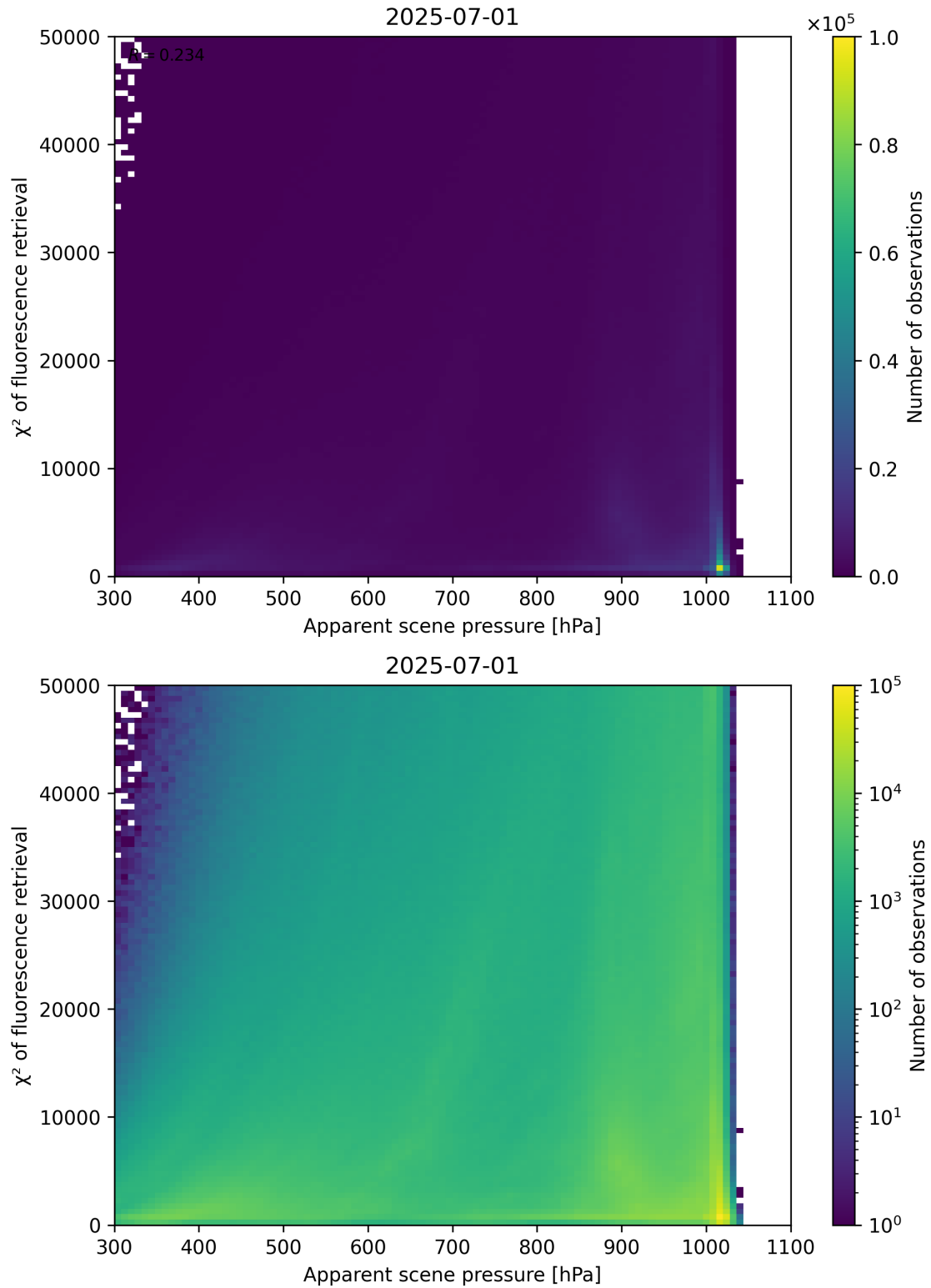
Figure 63: Scatter density plot of “Apparent scene pressure” against “ \chi^2 of fluorescence retrieval” for 2025-06-30 to 2025-07-02.
