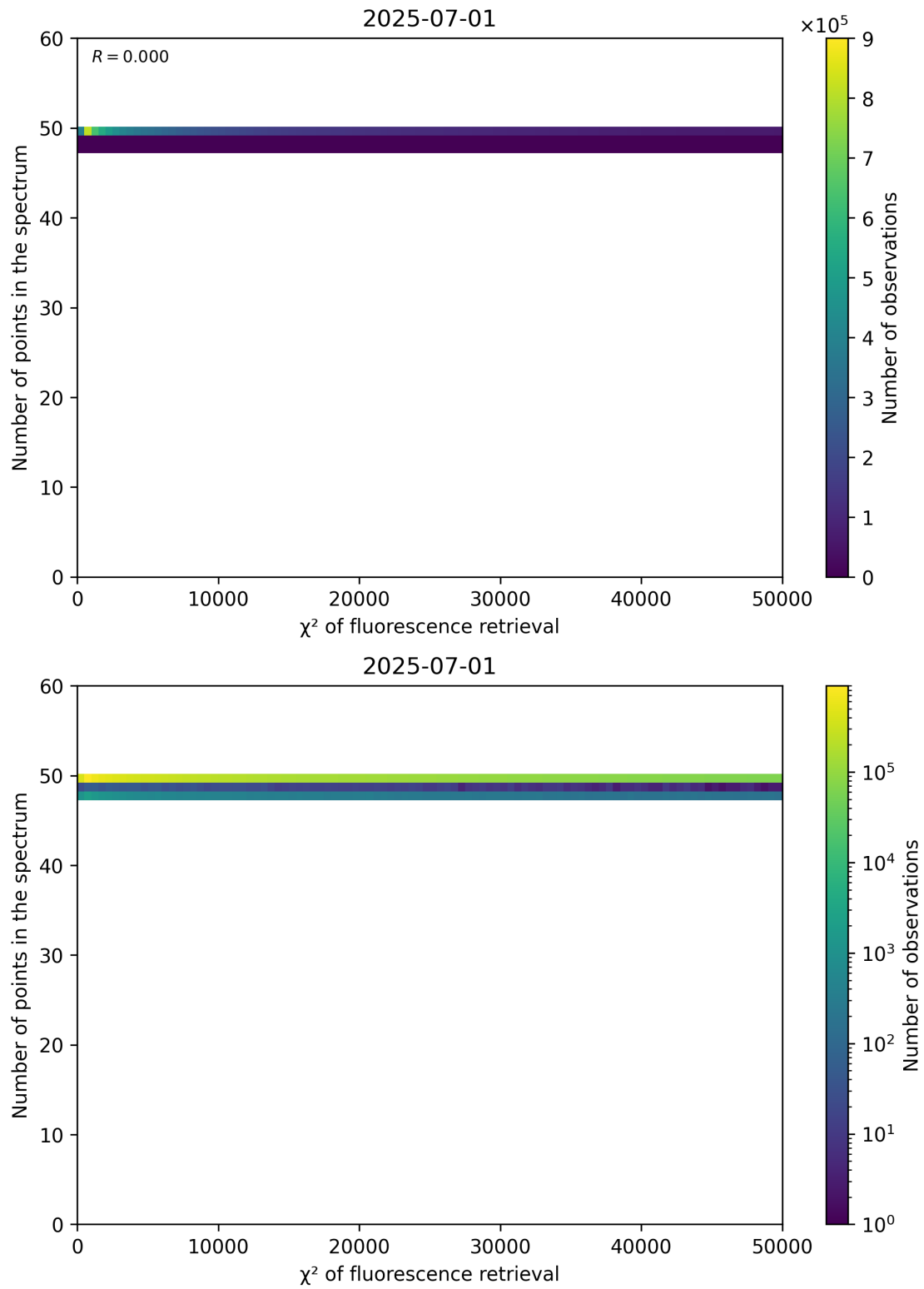
Figure 68: Scatter density plot of “ \chi^2 of fluorescence retrieval” against “Number of points in the spectrum” for 2025-06-30 to 2025-07-02.
