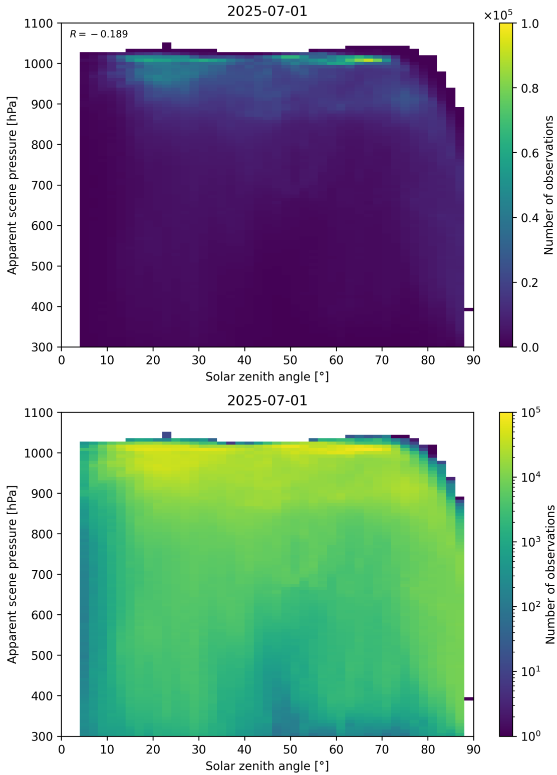
Figure 108: Scatter density plot of “Solar zenith angle” against “Apparent scene pressure” for 2025-06-30 to 2025-07-02.
