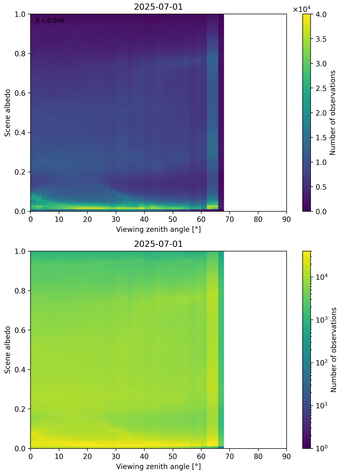
Figure 126: Scatter density plot of “Viewing zenith angle” against “Scene albedo” for 2025-06-30 to 2025-07-02.
