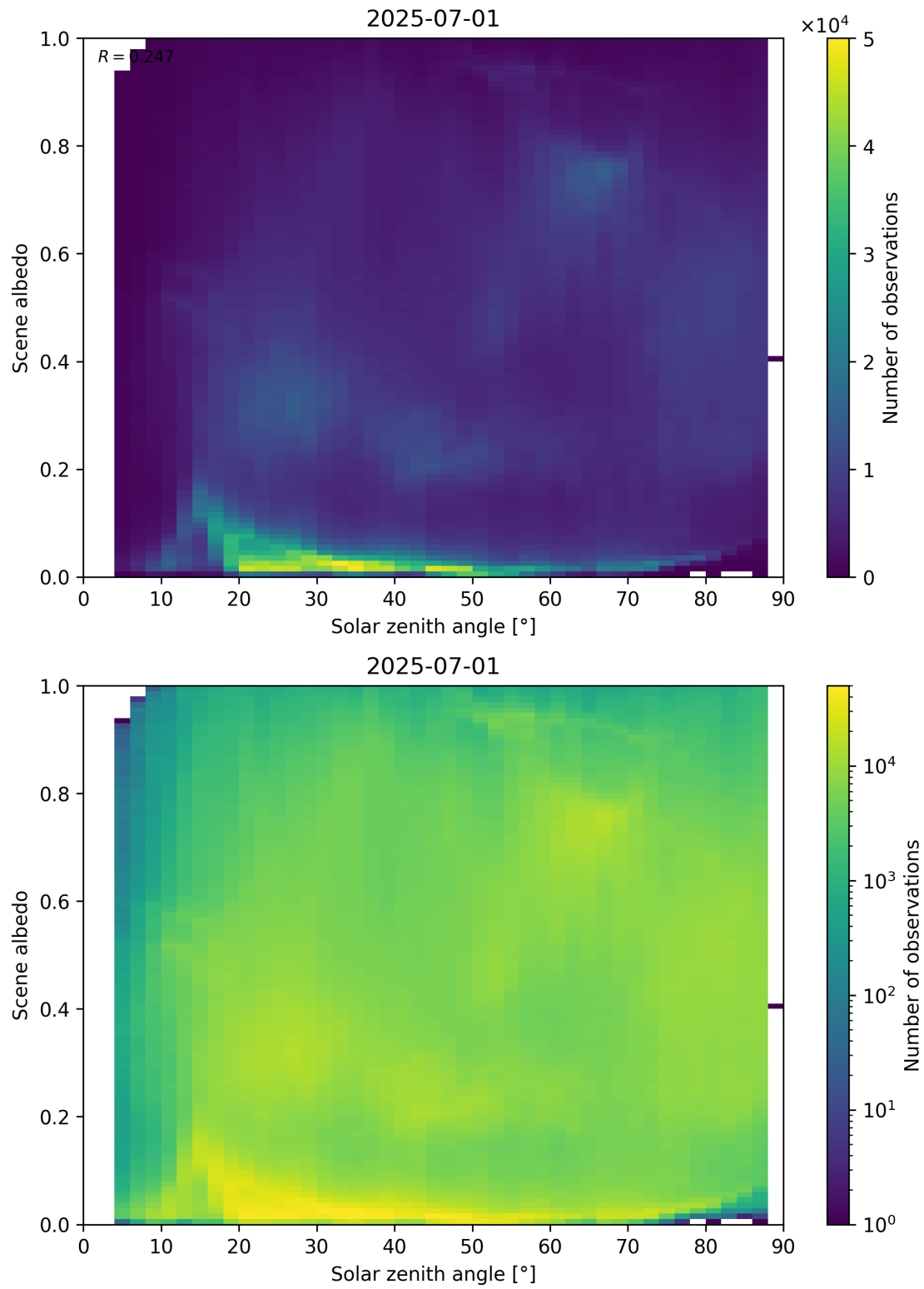
Figure 116: Scatter density plot of “Solar zenith angle” against “Scene albedo” for 2025-06-30 to 2025-07-02.
