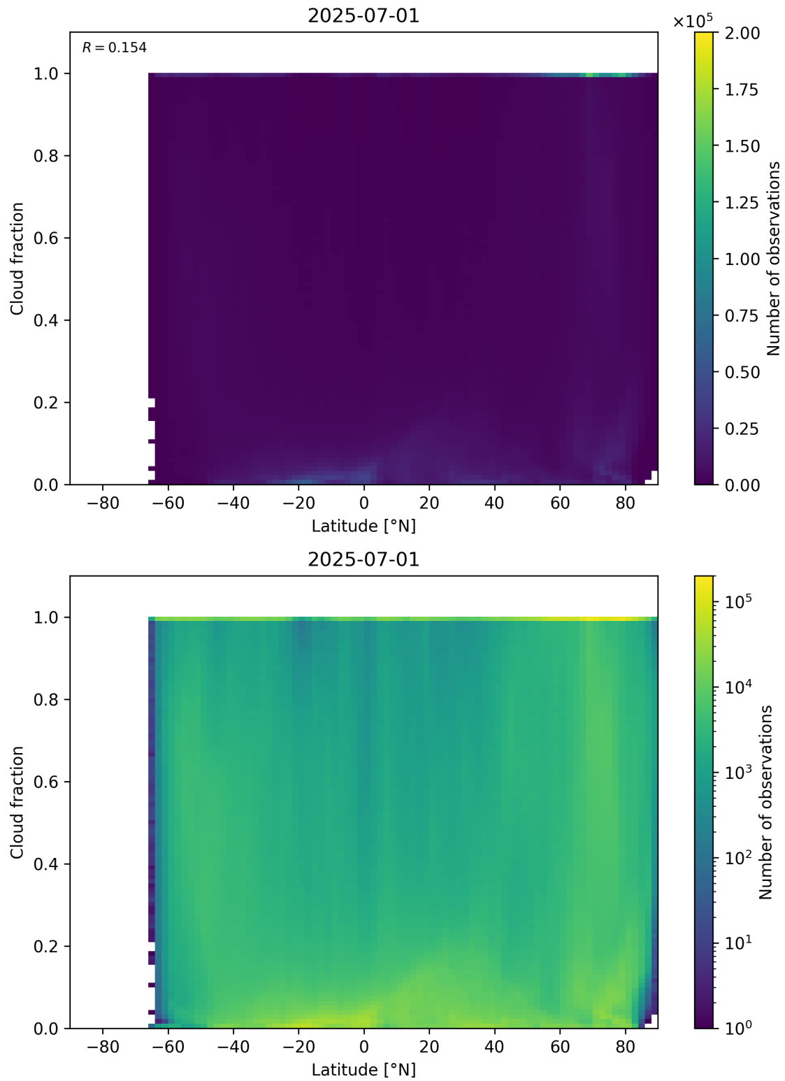
Figure 90: Scatter density plot of “Latitude” against “Cloud fraction” for 2025-06-30 to 2025-07-02.
