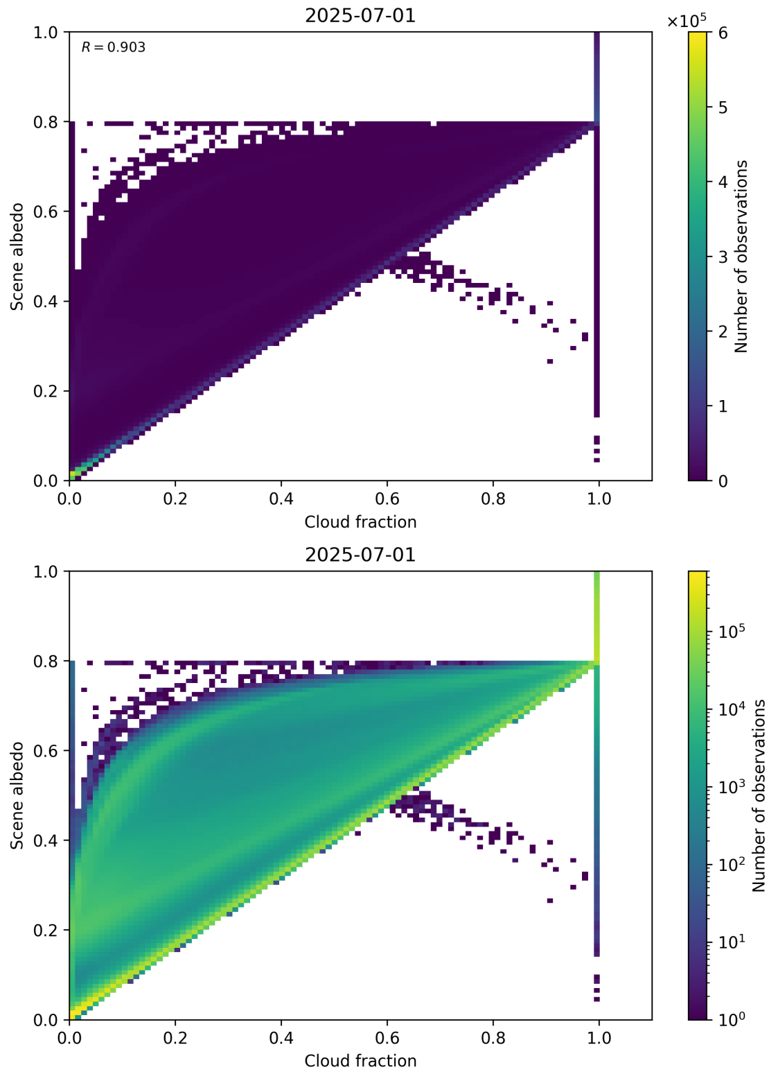
Figure 75: Scatter density plot of “Cloud fraction” against “Scene albedo” for 2025-06-30 to 2025-07-02.
