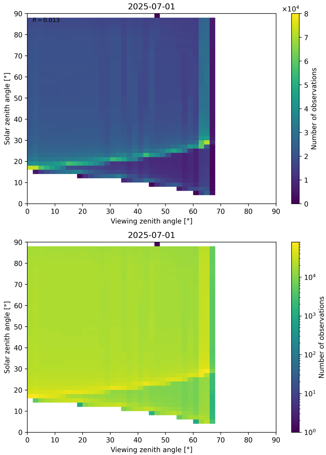
Figure 127: Scatter density plot of “Viewing zenith angle” against “Solar zenith angle” for 2025-06-30 to 2025-07-02.
