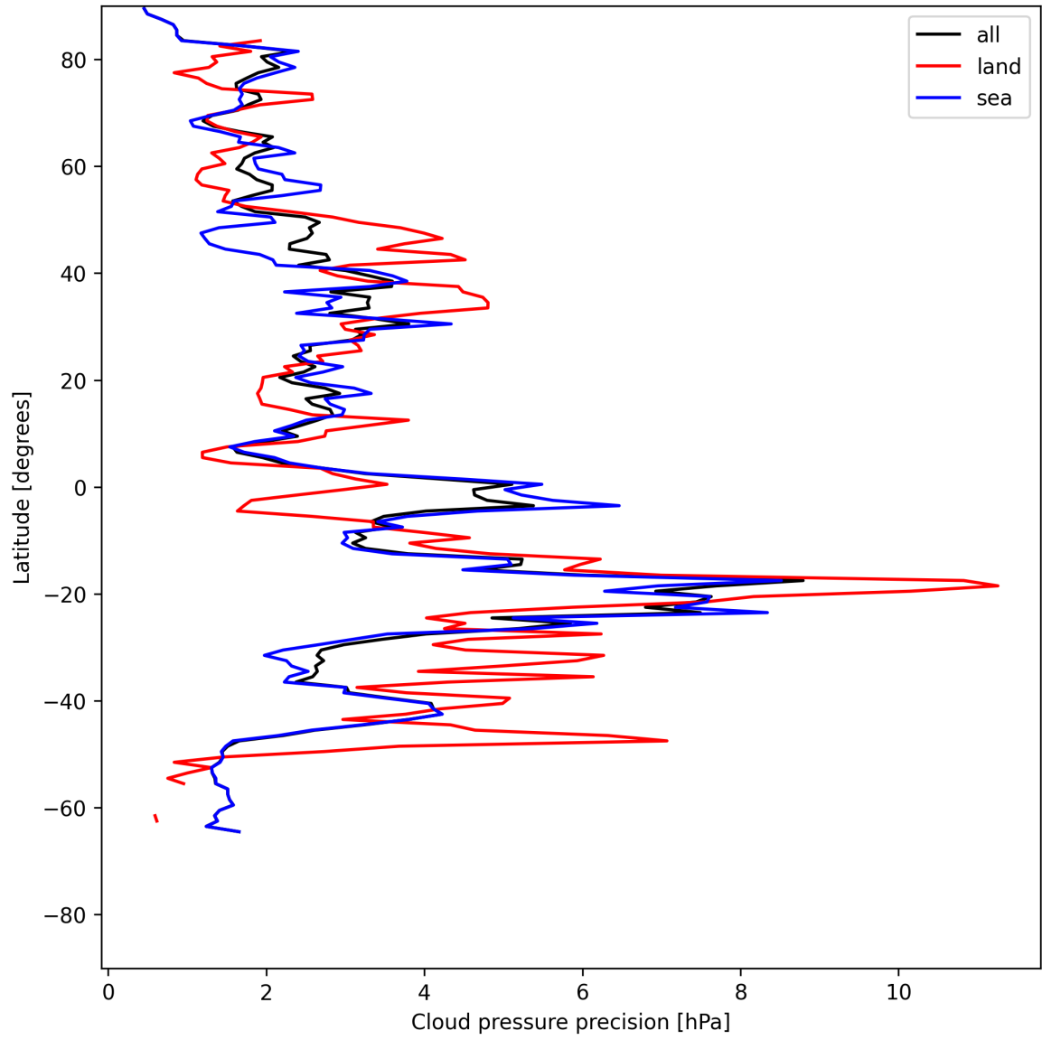
Figure 14: Zonal average of "Cloud pressure precision" for 2025-06-30 to 2025-07-02.
