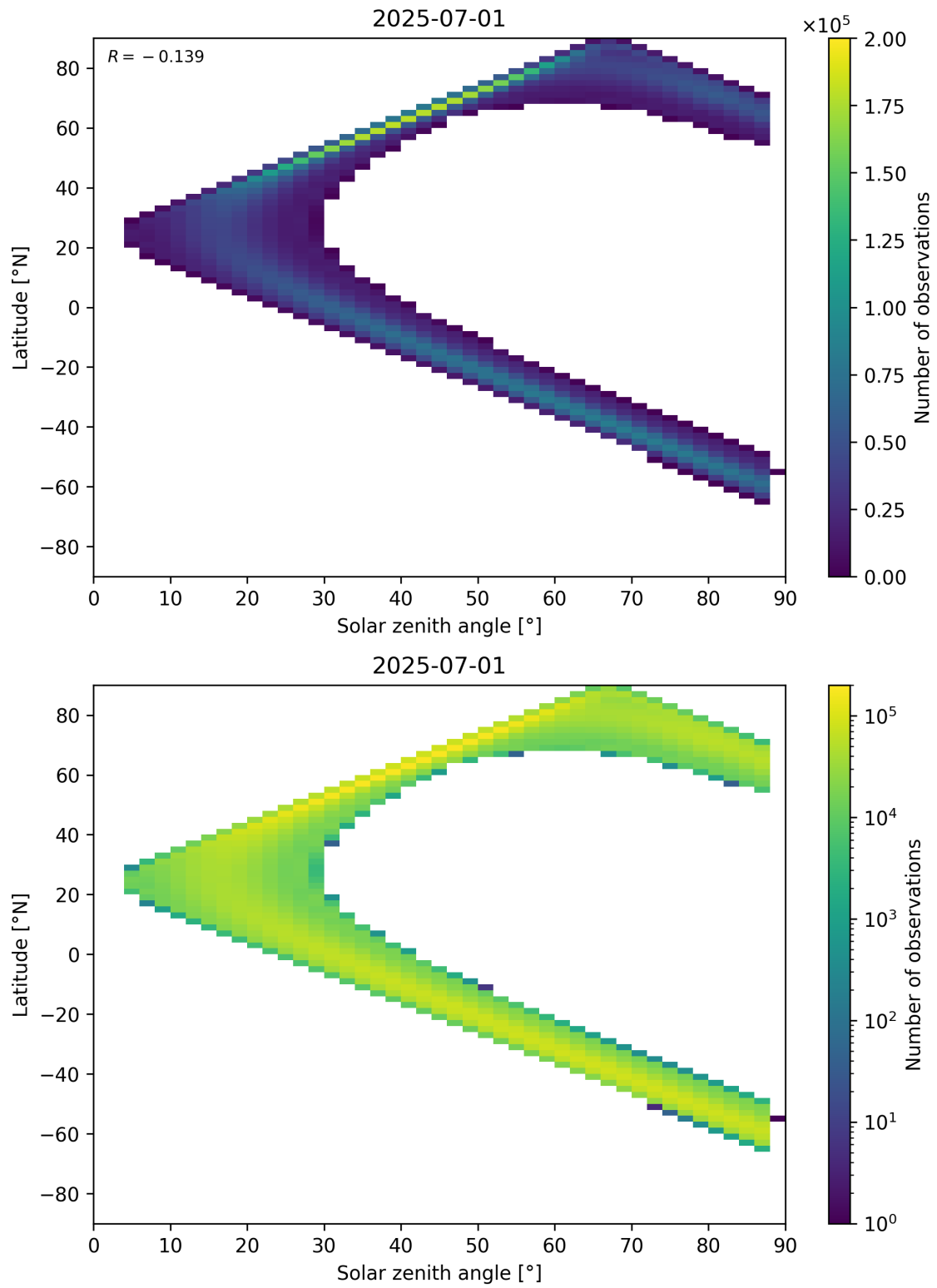
Figure 113: Scatter density plot of “Solar zenith angle” against “Latitude” for 2025-06-30 to 2025-07-02.
