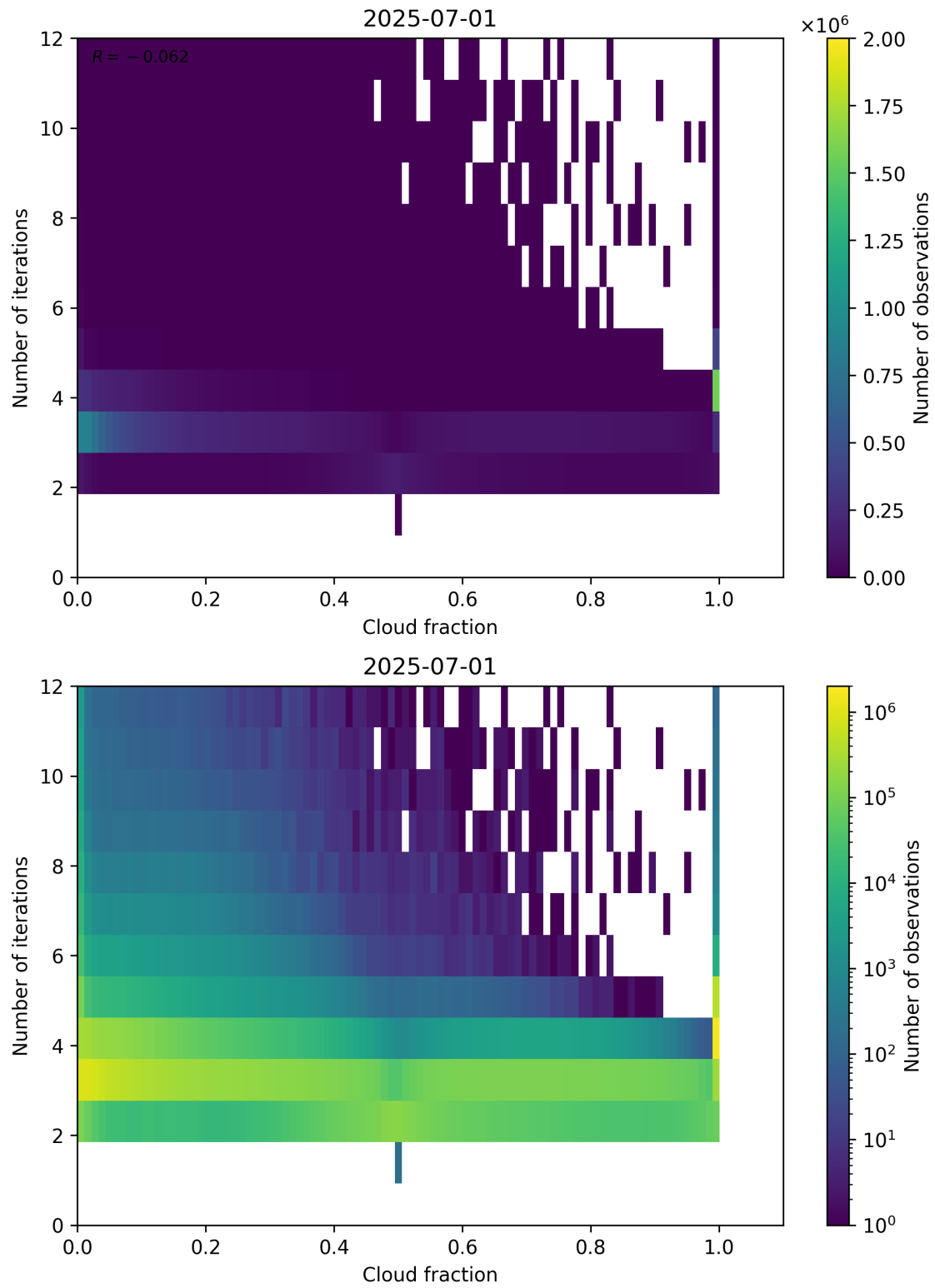
Figure 73: Scatter density plot of “Cloud fraction” against “Number of iterations” for 2025-06-30 to 2025-07-02.
