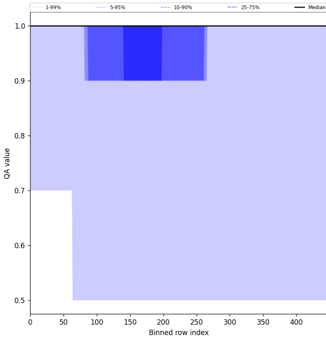
Figure 46: Along track statistics of “QA value” for 2025-06-30 to 2025-07-02
