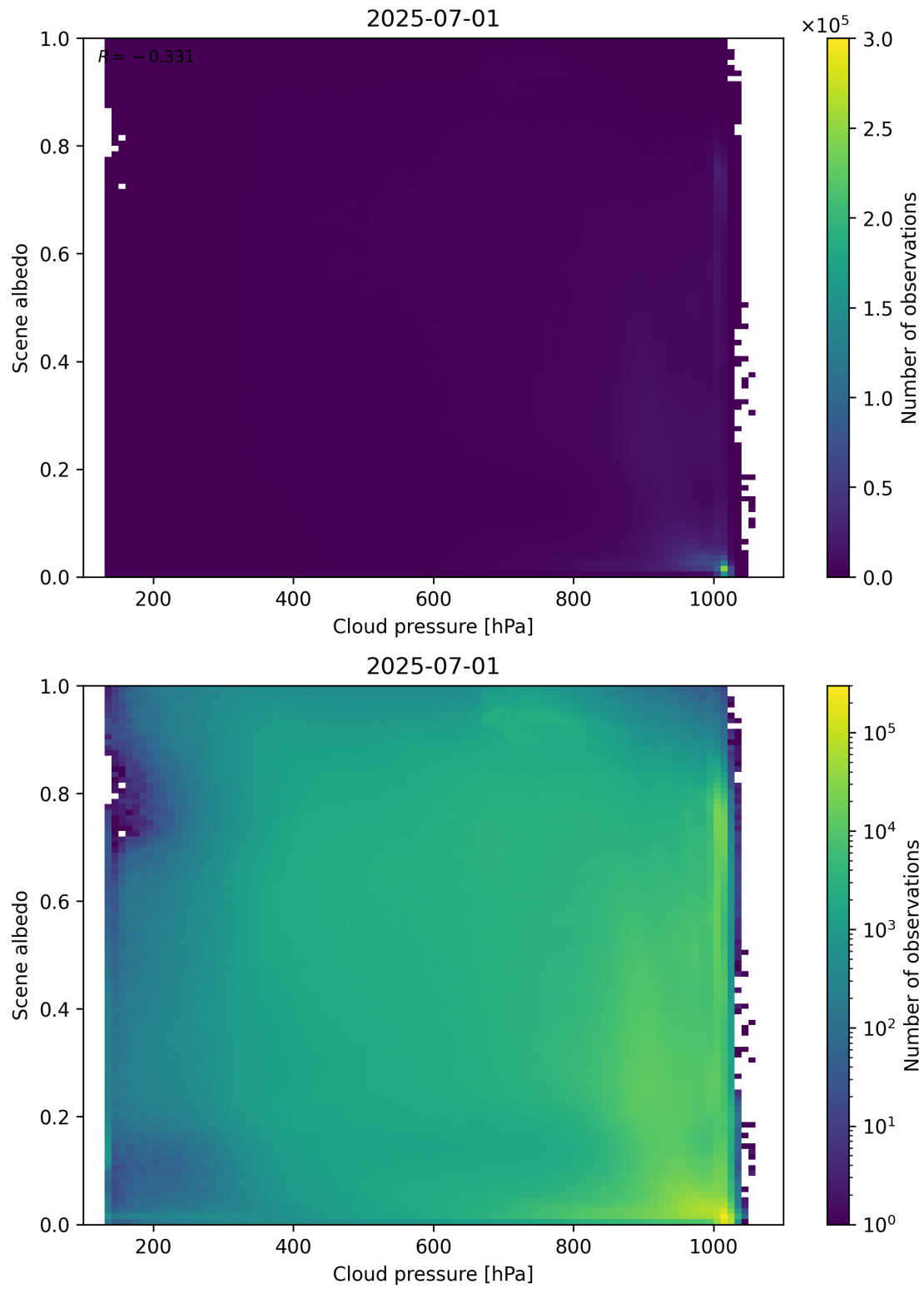
Figure 83: Scatter density plot of “Cloud pressure” against “Scene albedo” for 2025-06-30 to 2025-07-02.
