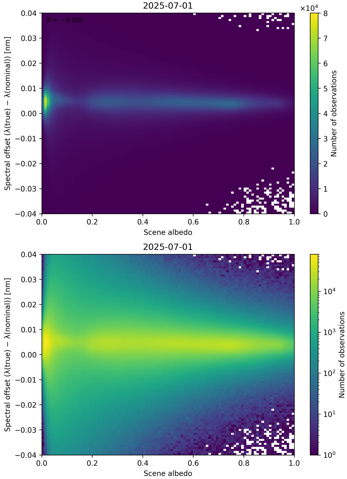
Figure 107: Scatter density plot of “Scene albedo” against “Spectral offset ( \lambda_{\text{true}} - \lambda_{\text{nominal}} )” for 2025-06-30 to 2025-07-02.
