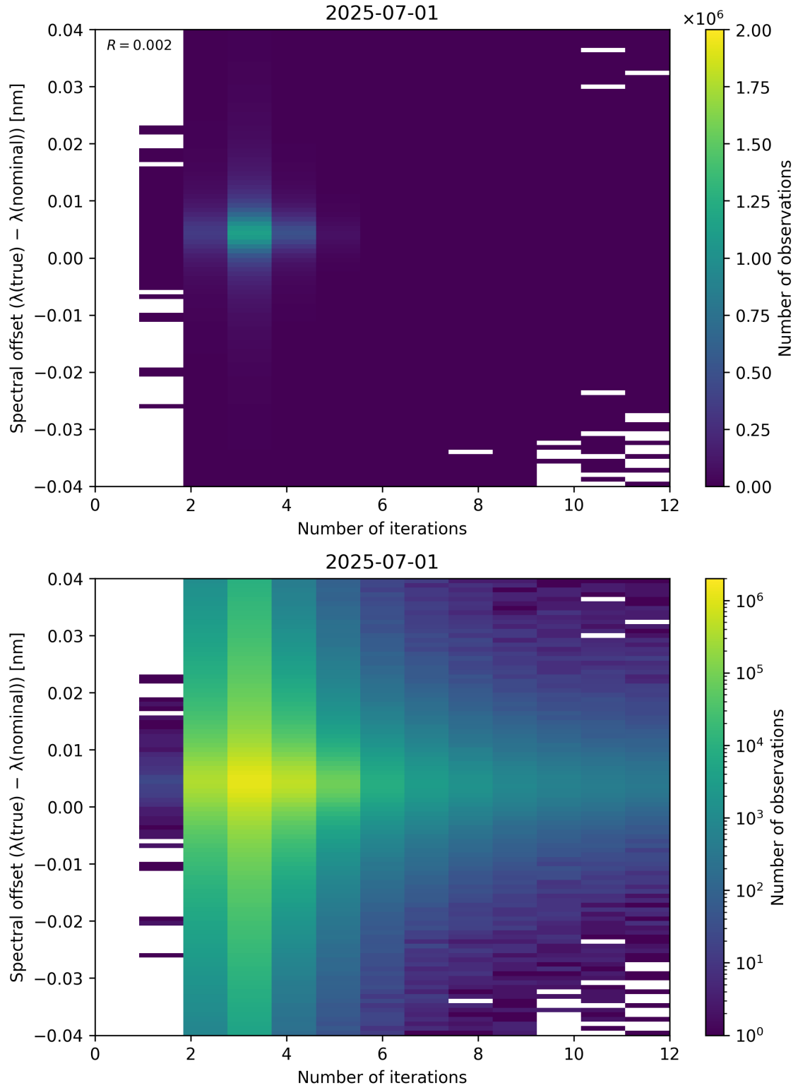
Figure 100: Scatter density plot of “Number of iterations” against “Spectral offset ( \lambda_{\text{true}} - \lambda_{\text{nominal}} )” for 2025-06-30 to 2025-07-02.
