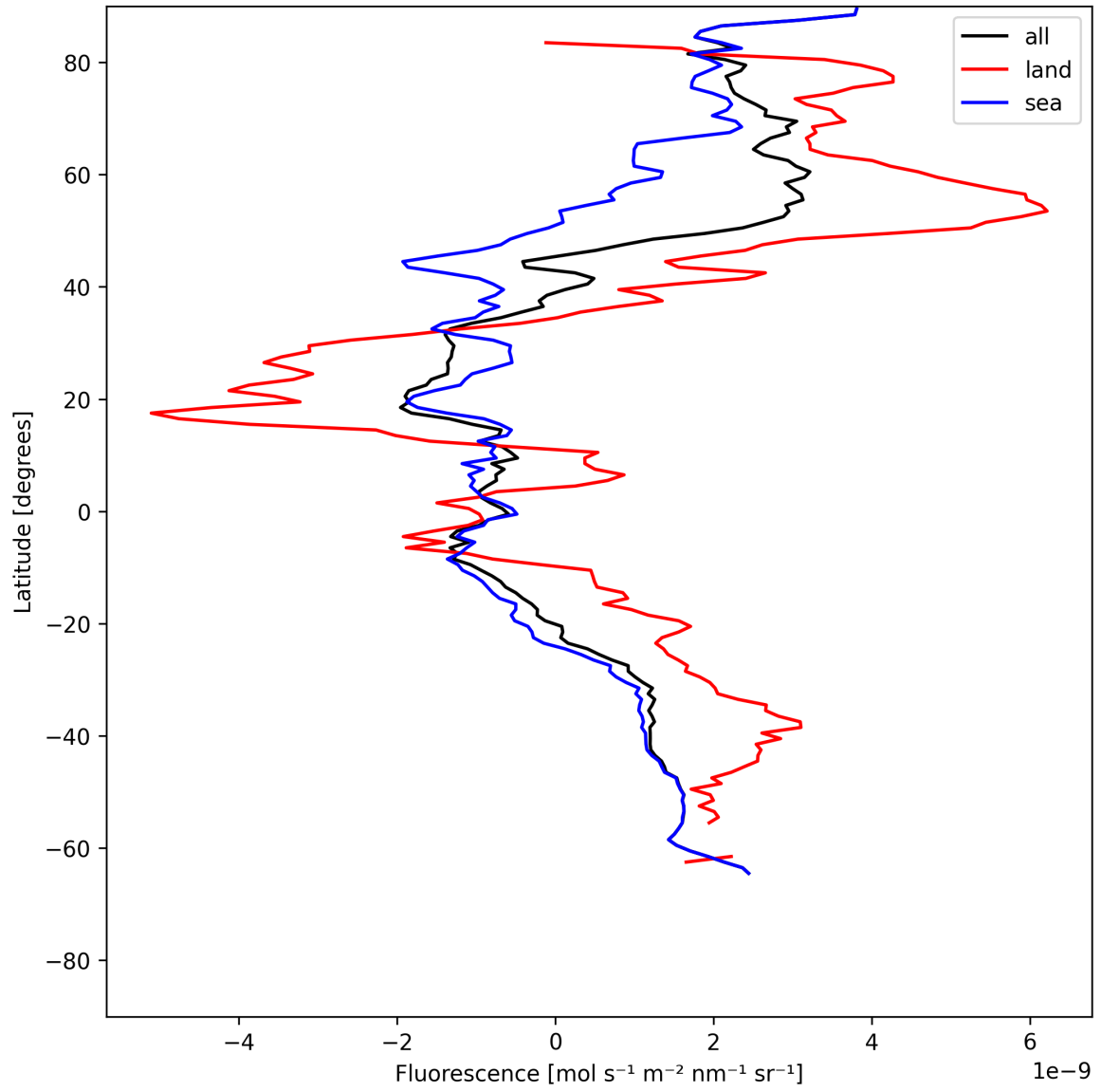
Figure 23: Zonal average of “Fluorescence” for 2025-06-30 to 2025-07-02.
