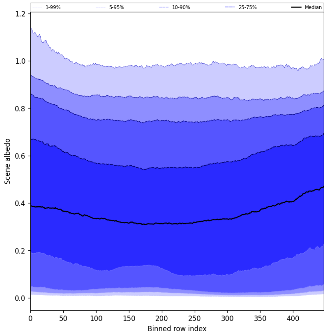
Figure 51: Along track statistics of “Scene albedo” for 2025-06-30 to 2025-07-02
