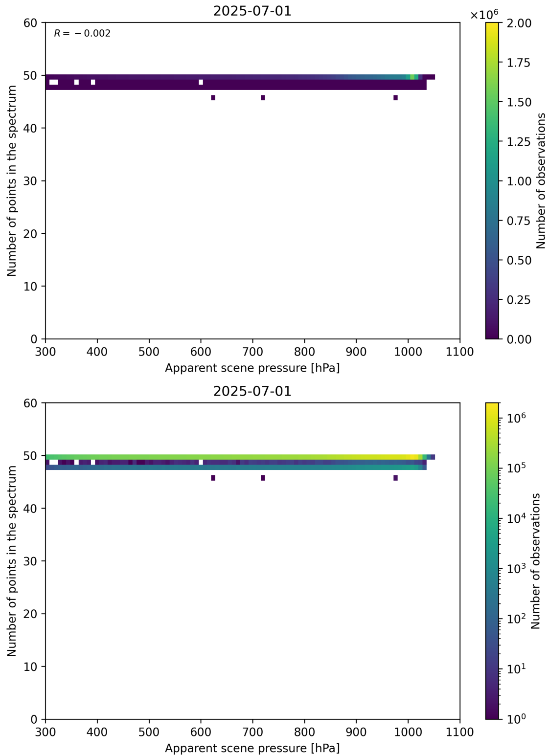
Figure 66: Scatter density plot of “Apparent scene pressure” against “Number of points in the spectrum” for 2025-06-30 to 2025-07-02.
