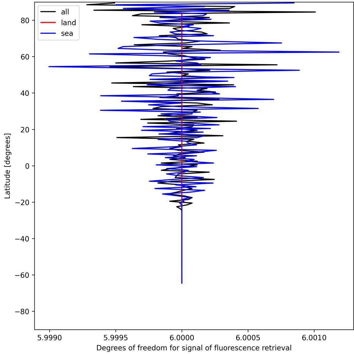
Figure 26: Zonal average of “Degrees of freedom for signal of fluorescence retrieval” for 2025-06-30 to 2025-07-02.
