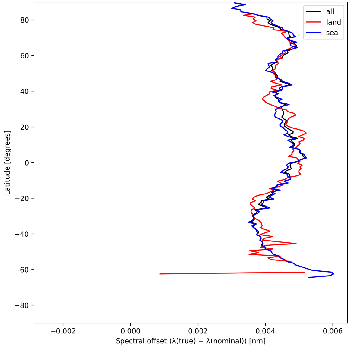
Figure 28: Zonal average of “Spectral offset ( \lambda_{\text{true}} - \lambda_{\text{nominal}} )” for 2025-06-30 to 2025-07-02.
