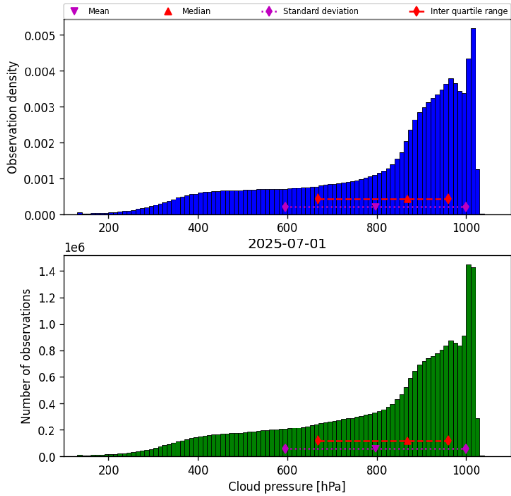
Figure 30: Histogram of “Cloud pressure” for 2025-06-30 to 2025-07-02
