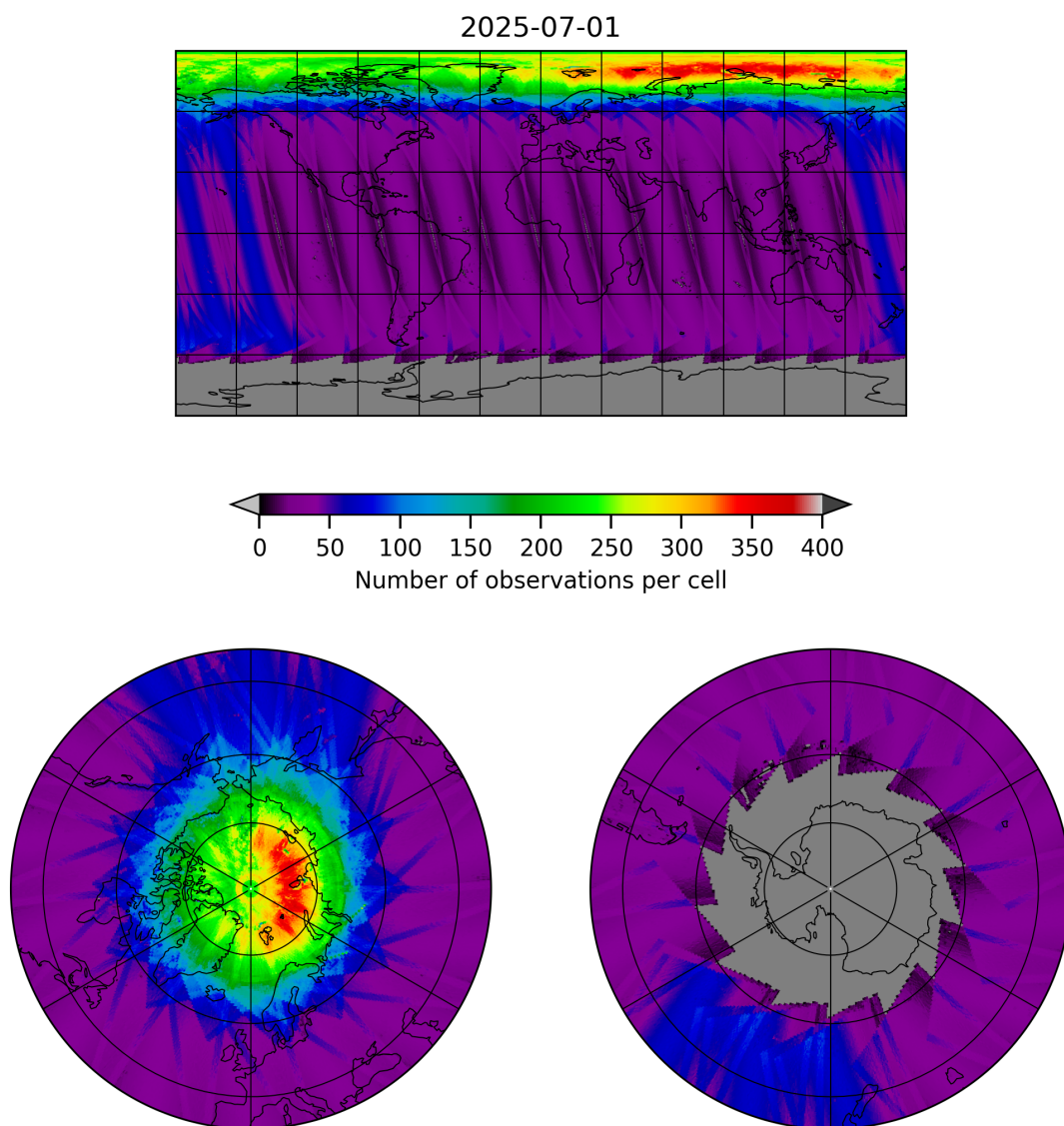
Figure 11: Map of the number of observations for 2025-06-30 to 2025-07-02
