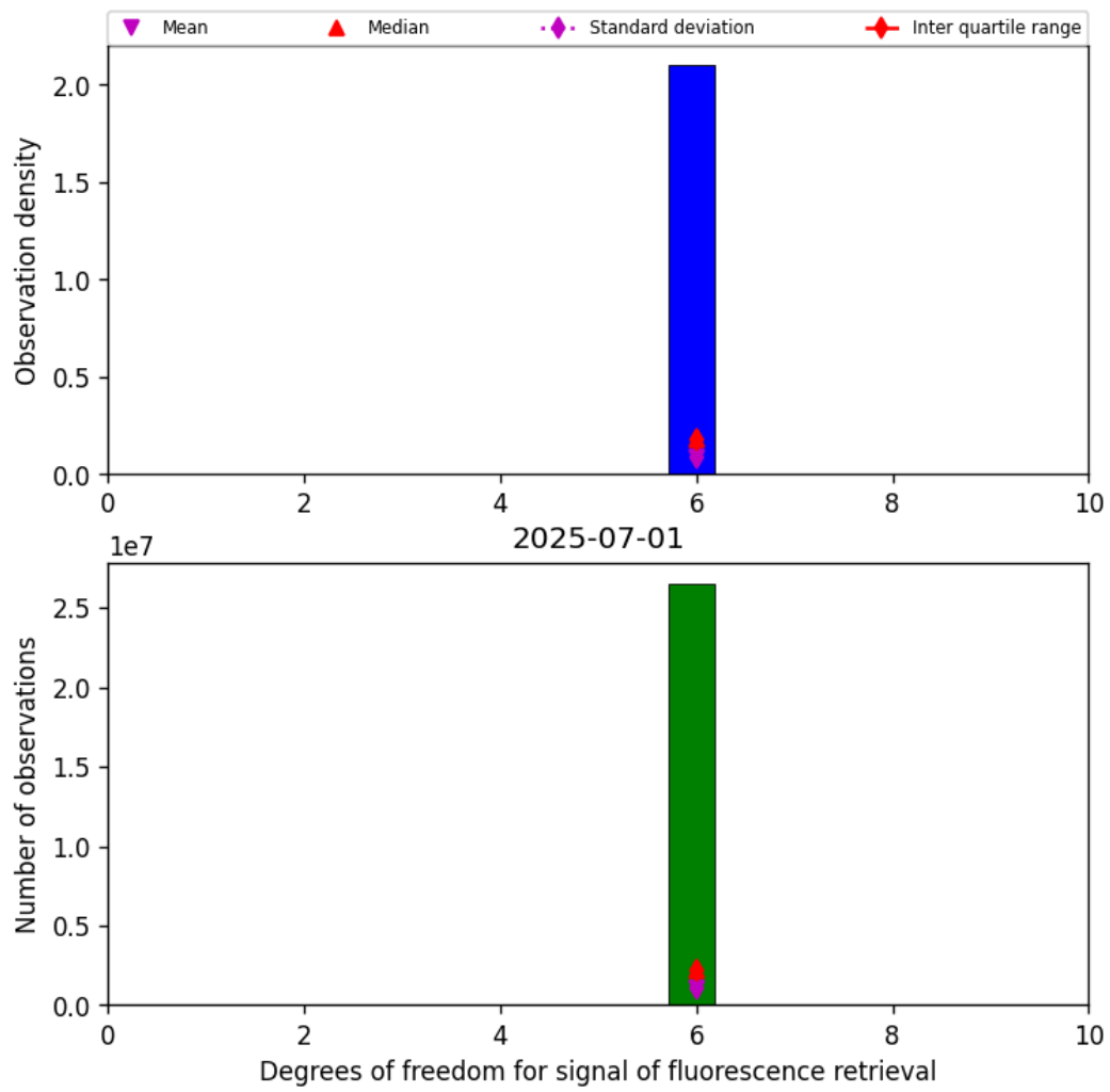
Figure 43: Histogram of "Degrees of freedom for signal of fluorescence retrieval" for 2025-06-30 to 2025-07-02
