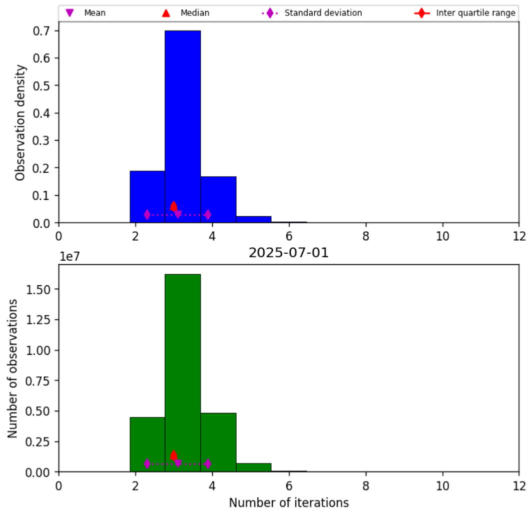
Figure 39: Histogram of “Number of iterations” for 2025-06-30 to 2025-07-02
