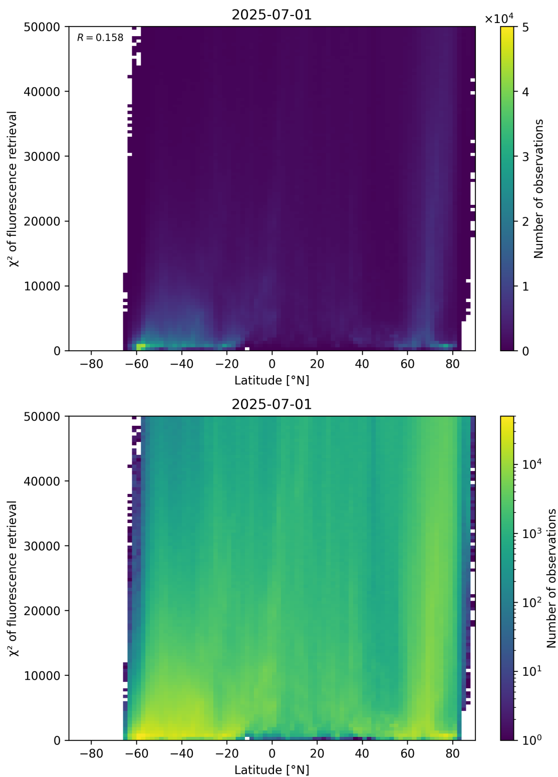
Figure 89: Scatter density plot of “Latitude” against “ \chi^2 of fluorescence retrieval” for 2025-06-30 to 2025-07-02.
