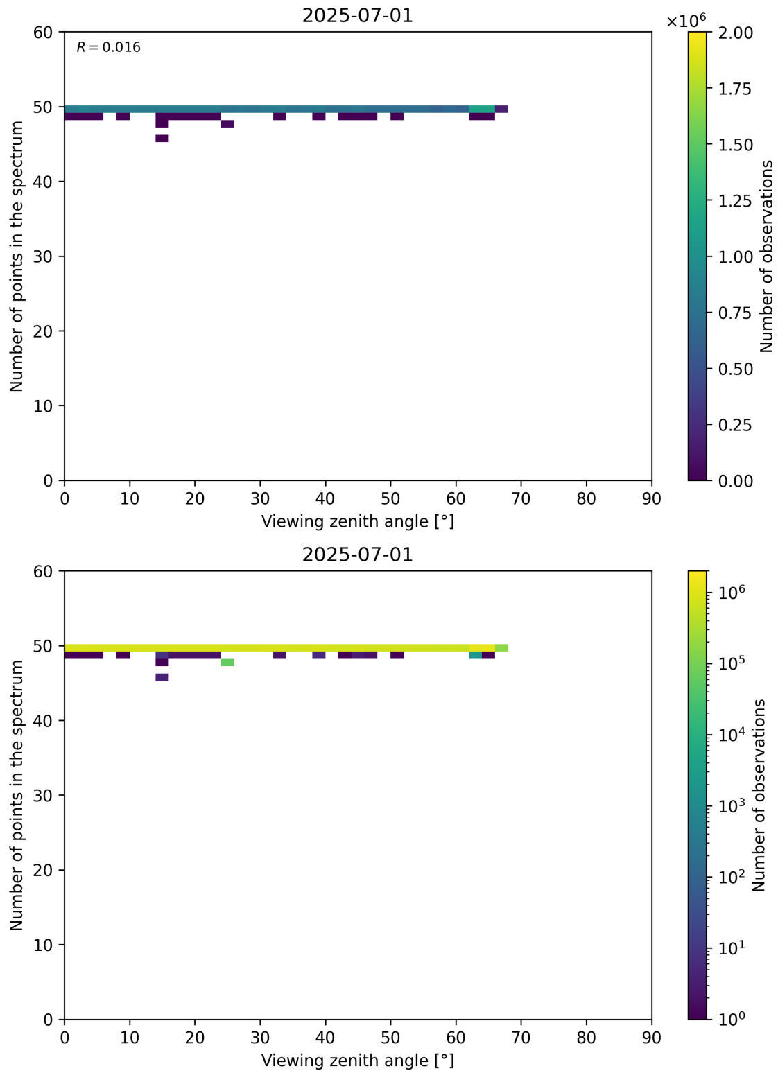
Figure 125: Scatter density plot of “Viewing zenith angle” against “Number of points in the spectrum” for 2025-06-30 to 2025-07-02.
