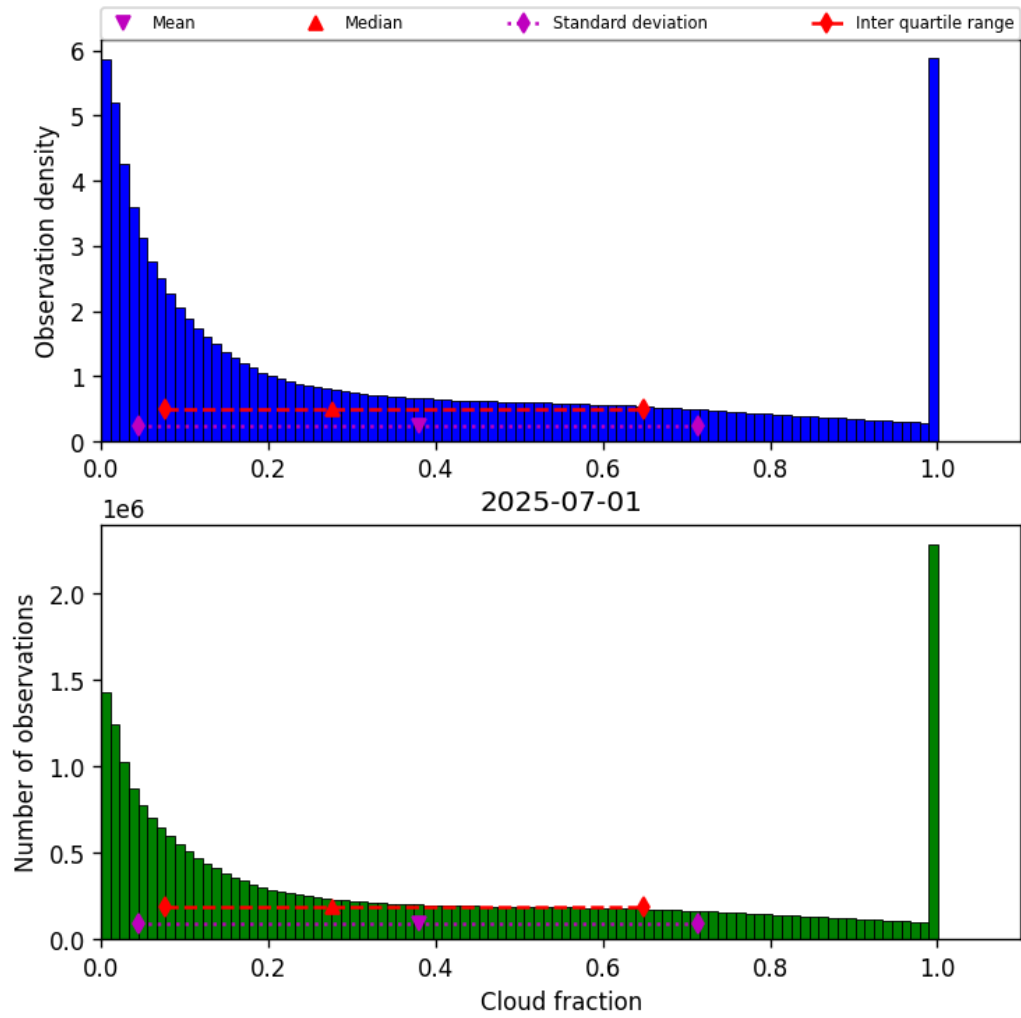
Figure 32: Histogram of “Cloud fraction” for 2025-06-30 to 2025-07-02
