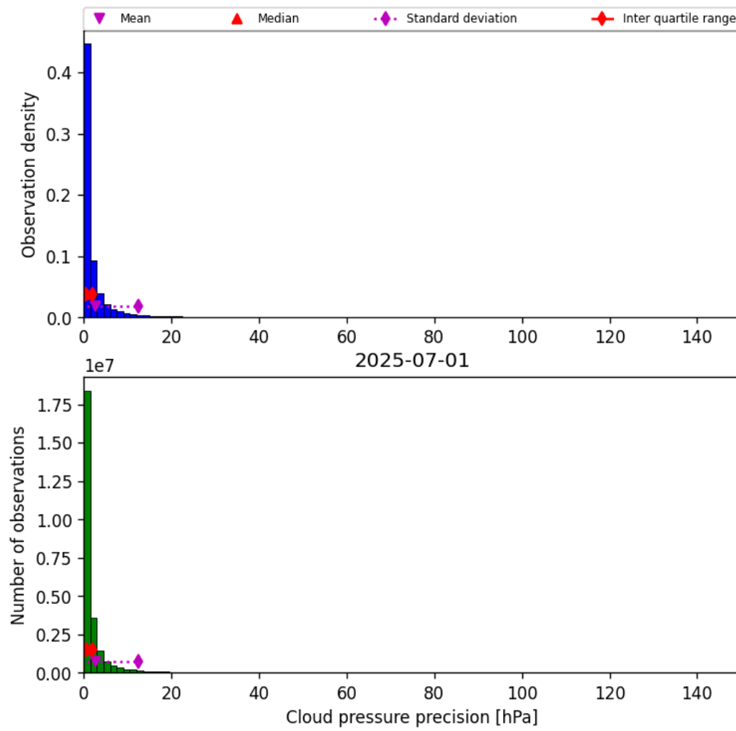
Figure 31: Histogram of “Cloud pressure precision” for 2025-06-30 to 2025-07-02
