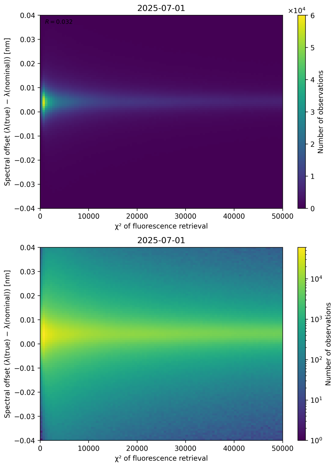
Figure 69: Scatter density plot of “ \chi^2 of fluorescence retrieval” against “Spectral offset ( \lambda_{\text{true}} - \lambda_{\text{nominal}} )” for 2025-06-30 to 2025-07-02.
