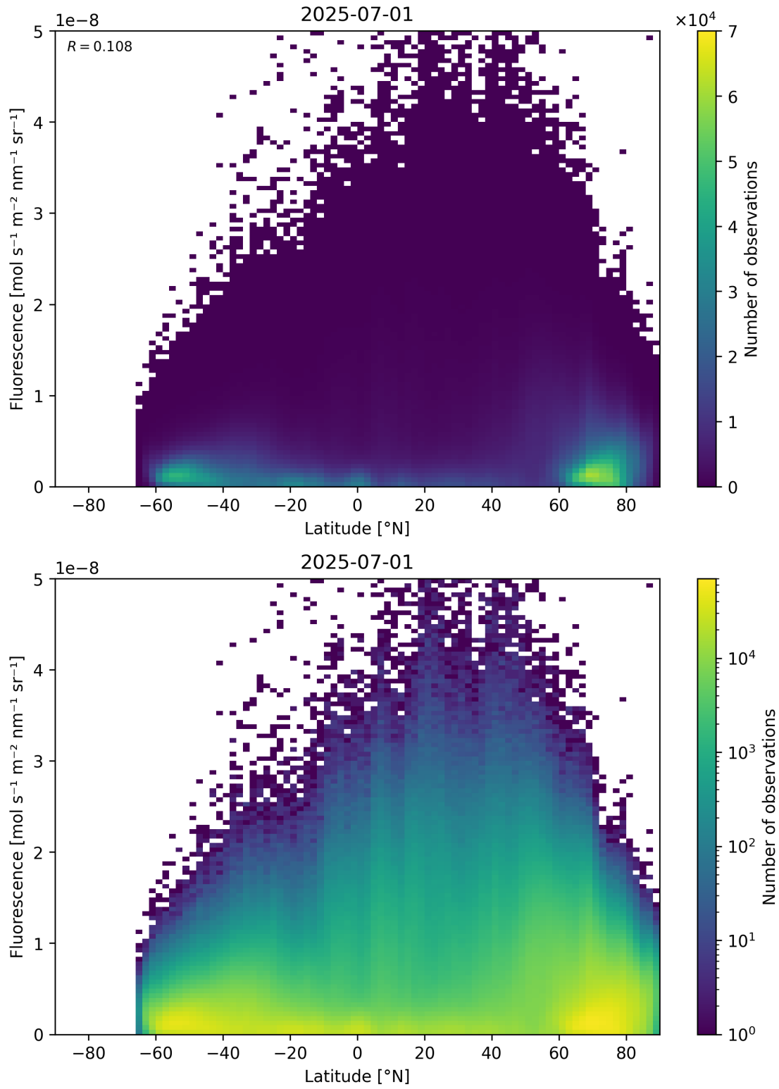
Figure 92: Scatter density plot of “Latitude” against “Fluorescence” for 2025-06-30 to 2025-07-02.
