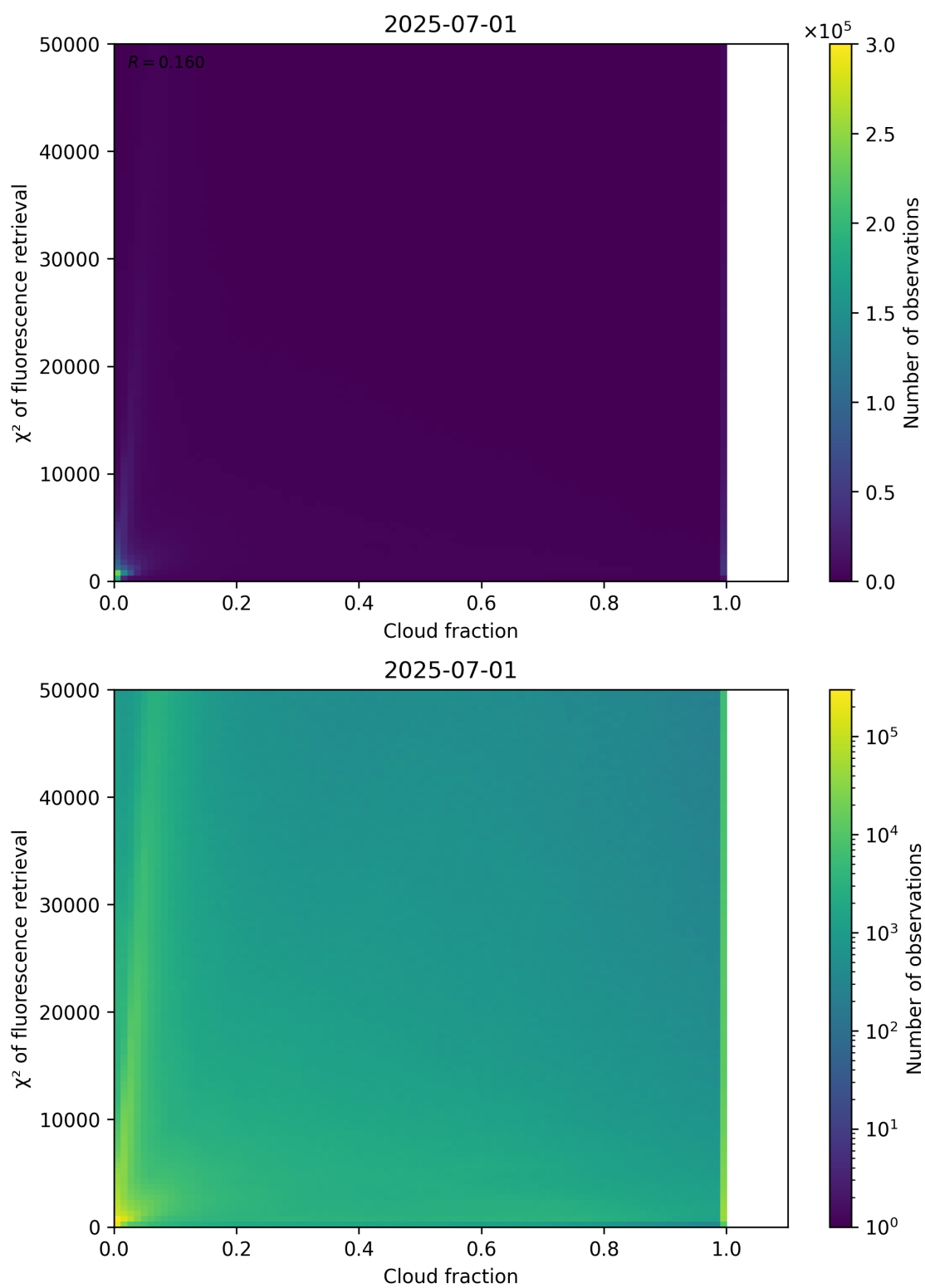
Figure 71: Scatter density plot of “Cloud fraction” against “ \chi^2 of fluorescence retrieval” for 2025-06-30 to 2025-07-02.
