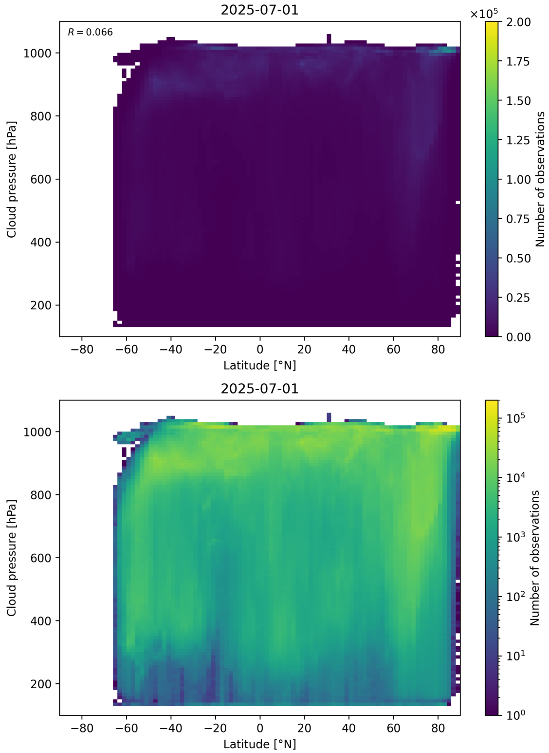
Figure 91: Scatter density plot of “Latitude” against “Cloud pressure” for 2025-06-30 to 2025-07-02.
