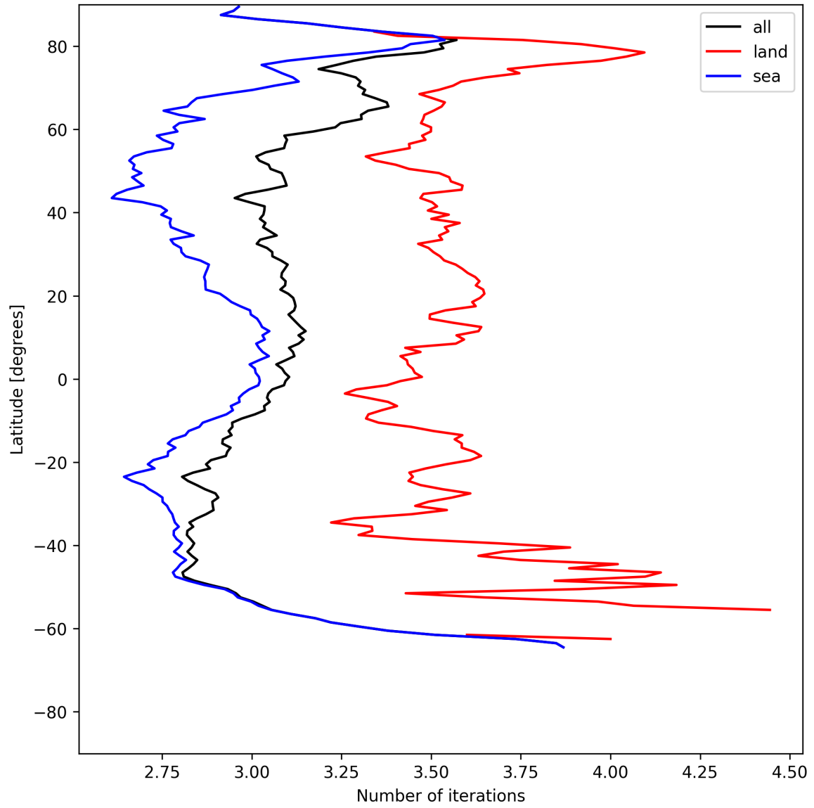
Figure 22: Zonal average of “Number of iterations” for 2025-06-30 to 2025-07-02.
