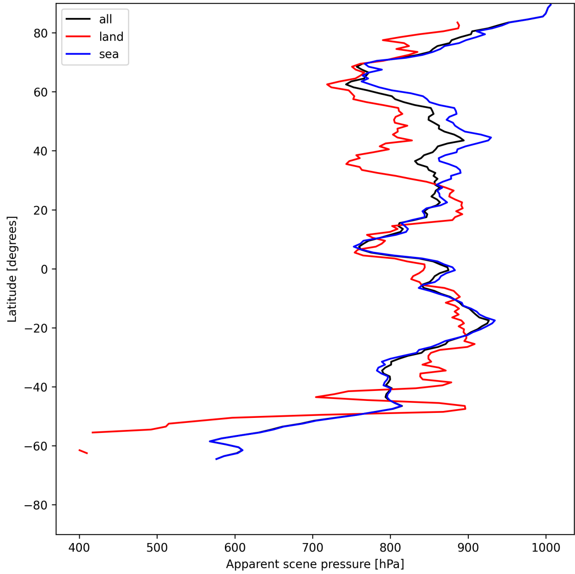
Figure 19: Zonal average of “Apparent scene pressure” for 2025-06-30 to 2025-07-02.
