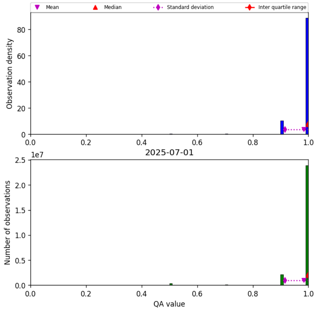
Figure 29: Histogram of “QA value” for 2025-06-30 to 2025-07-02
