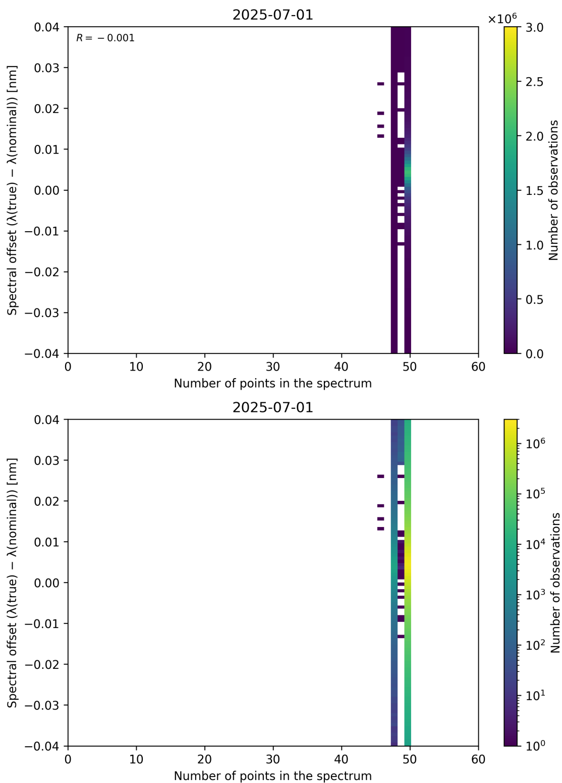
Figure 101: Scatter density plot of “Number of points in the spectrum” against “Spectral offset ( \lambda_{\text{true}} - \lambda_{\text{nominal}} )” for 2025-06-30 to 2025-07-02.
