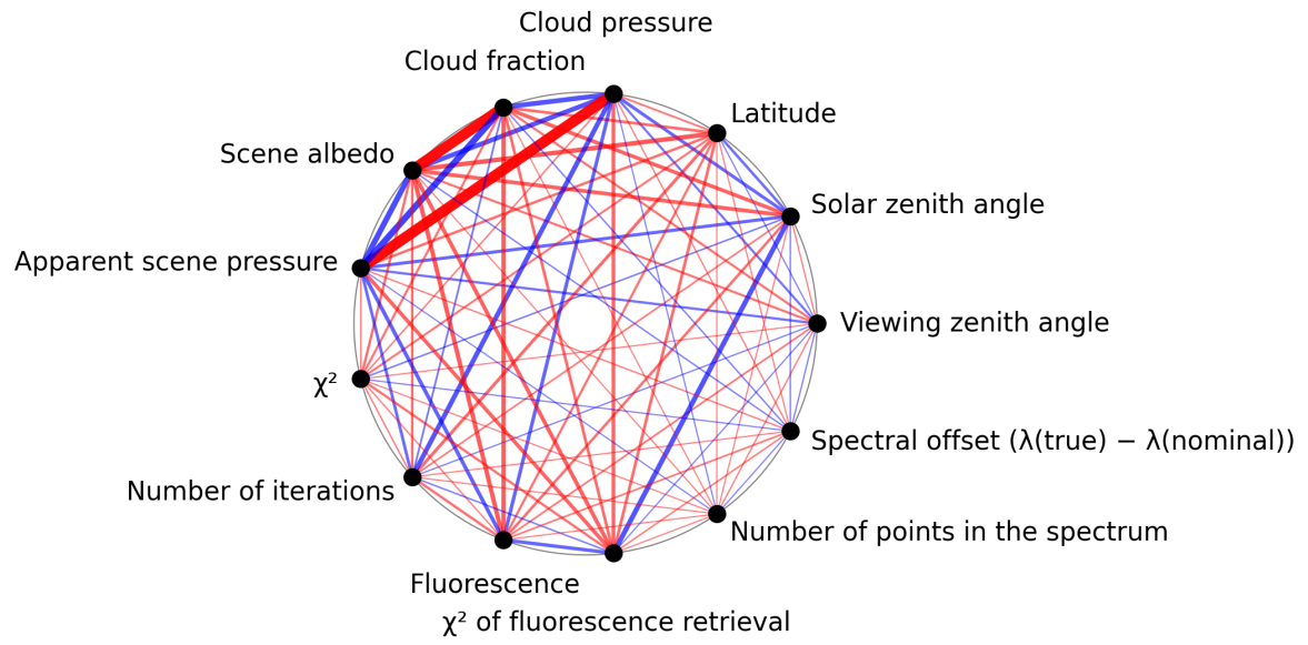
Figure 1: Map of correlation graph for 2025-06-30 to 2025-07-02.
