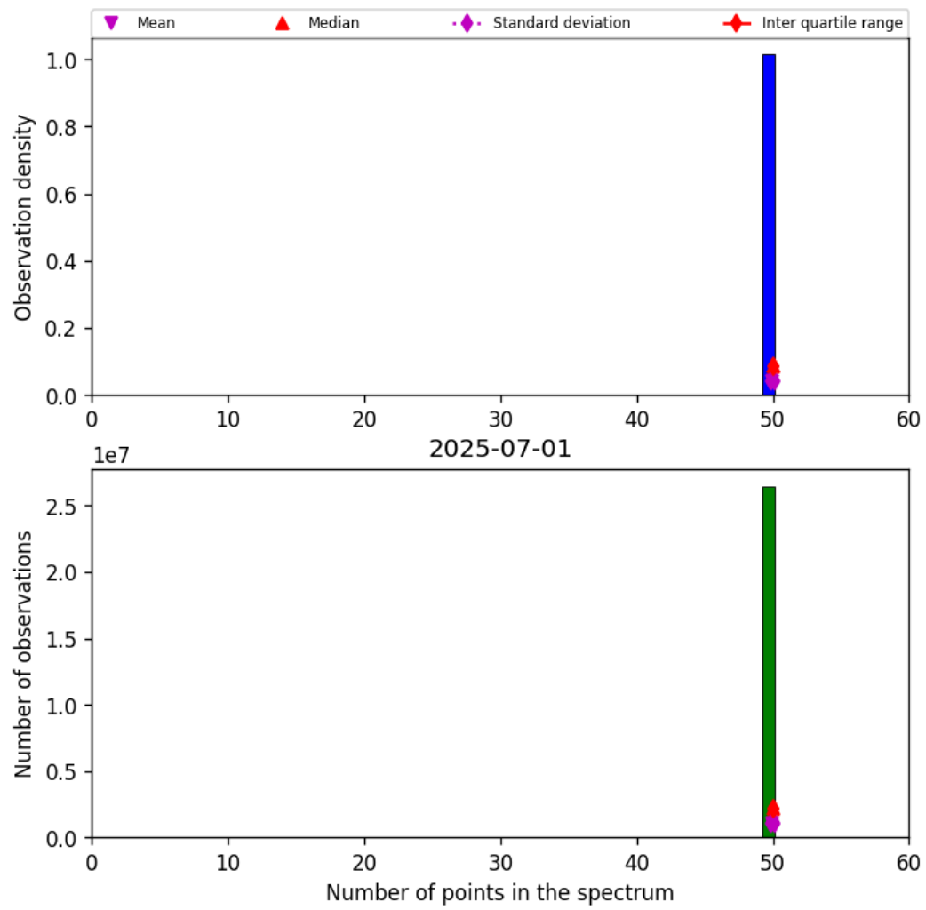
Figure 44: Histogram of "Number of points in the spectrum" for 2025-06-30 to 2025-07-02
