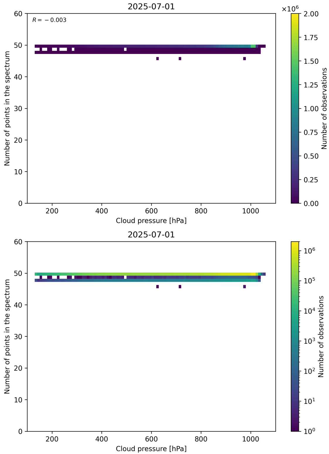
Figure 82: Scatter density plot of “Cloud pressure” against “Number of points in the spectrum” for 2025-06-30 to 2025-07-02.
