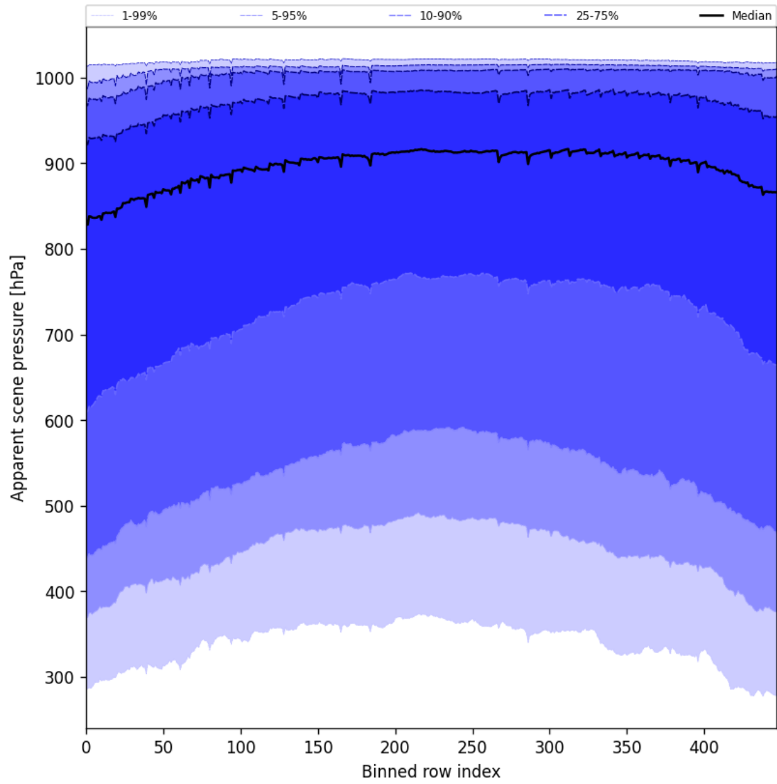
Figure 53: Along track statistics of “Apparent scene pressure” for 2025-06-30 to 2025-07-02
