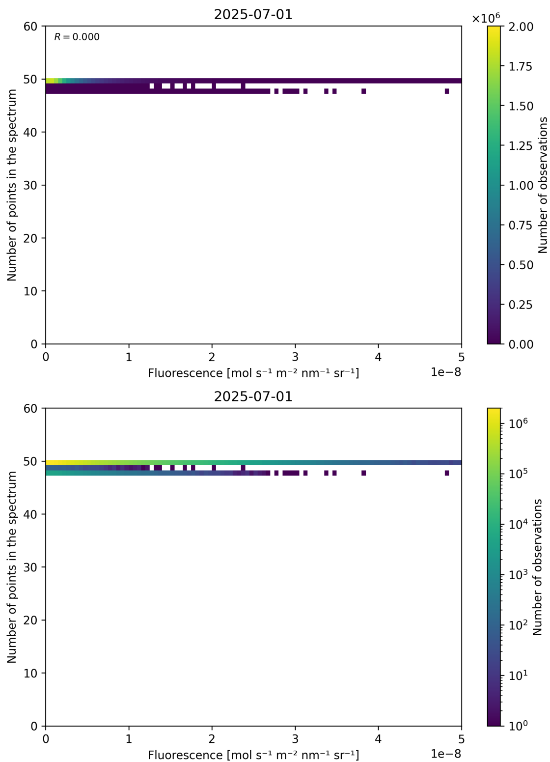
Figure 86: Scatter density plot of “Fluorescence” against “Number of points in the spectrum” for 2025-06-30 to 2025-07-02.
