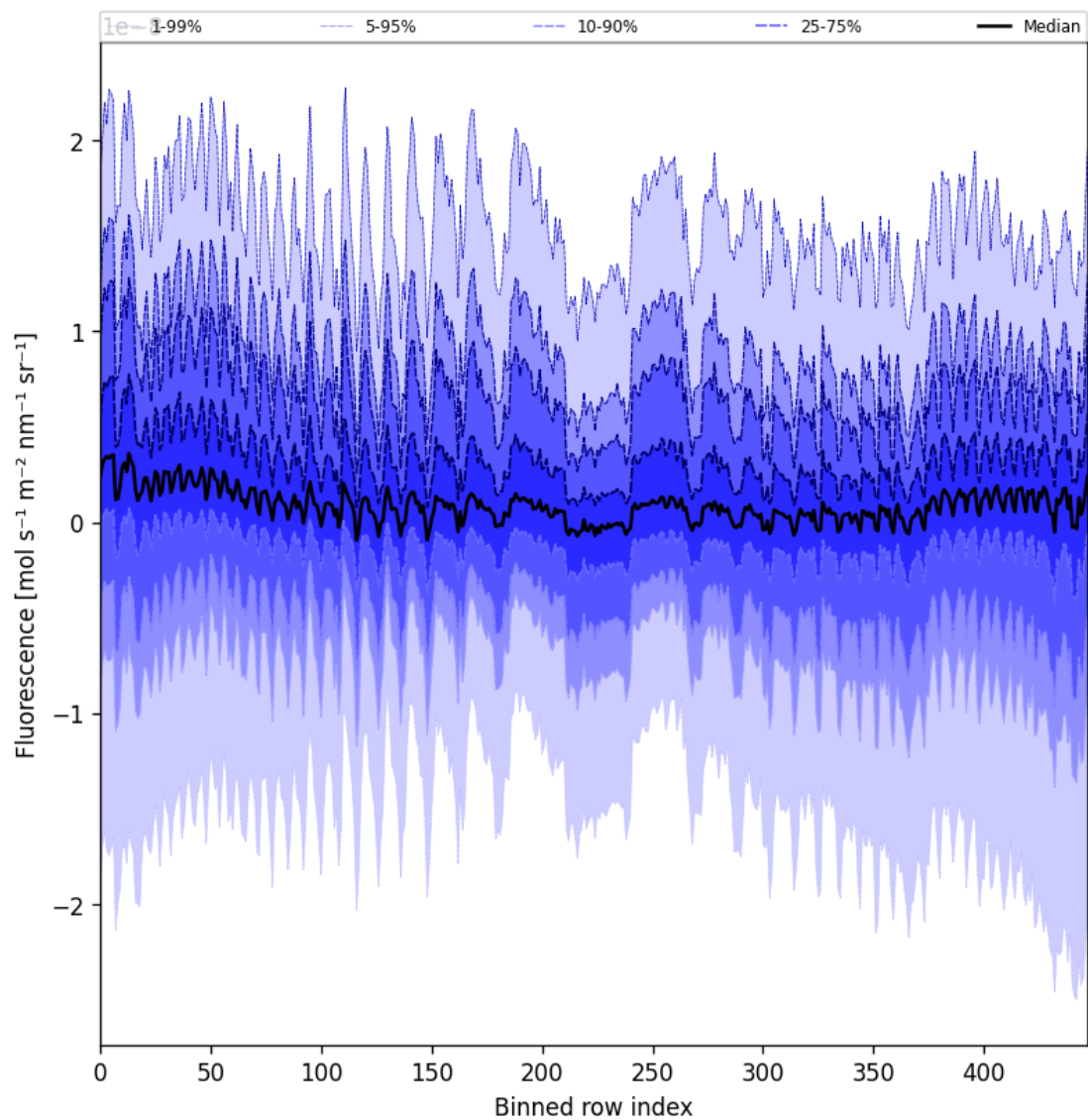
Figure 57: Along track statistics of “Fluorescence” for 2025-06-30 to 2025-07-02
