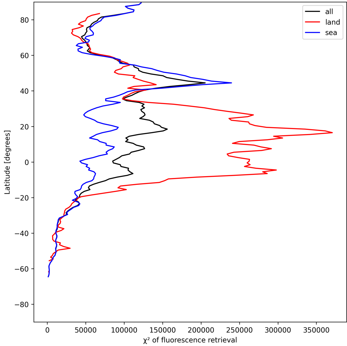
Figure 25: Zonal average of “ \chi^2 of fluorescence retrieval” for 2025-06-30 to 2025-07-02.
