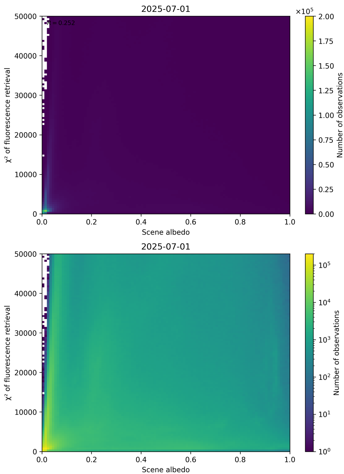
Figure 103: Scatter density plot of “Scene albedo” against “ \chi^2 of fluorescence retrieval” for 2025-06-30 to 2025-07-02.
