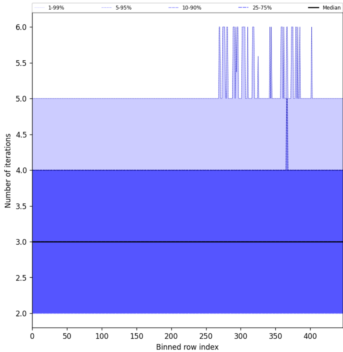
Figure 56: Along track statistics of "Number of iterations" for 2025-06-30 to 2025-07-02
