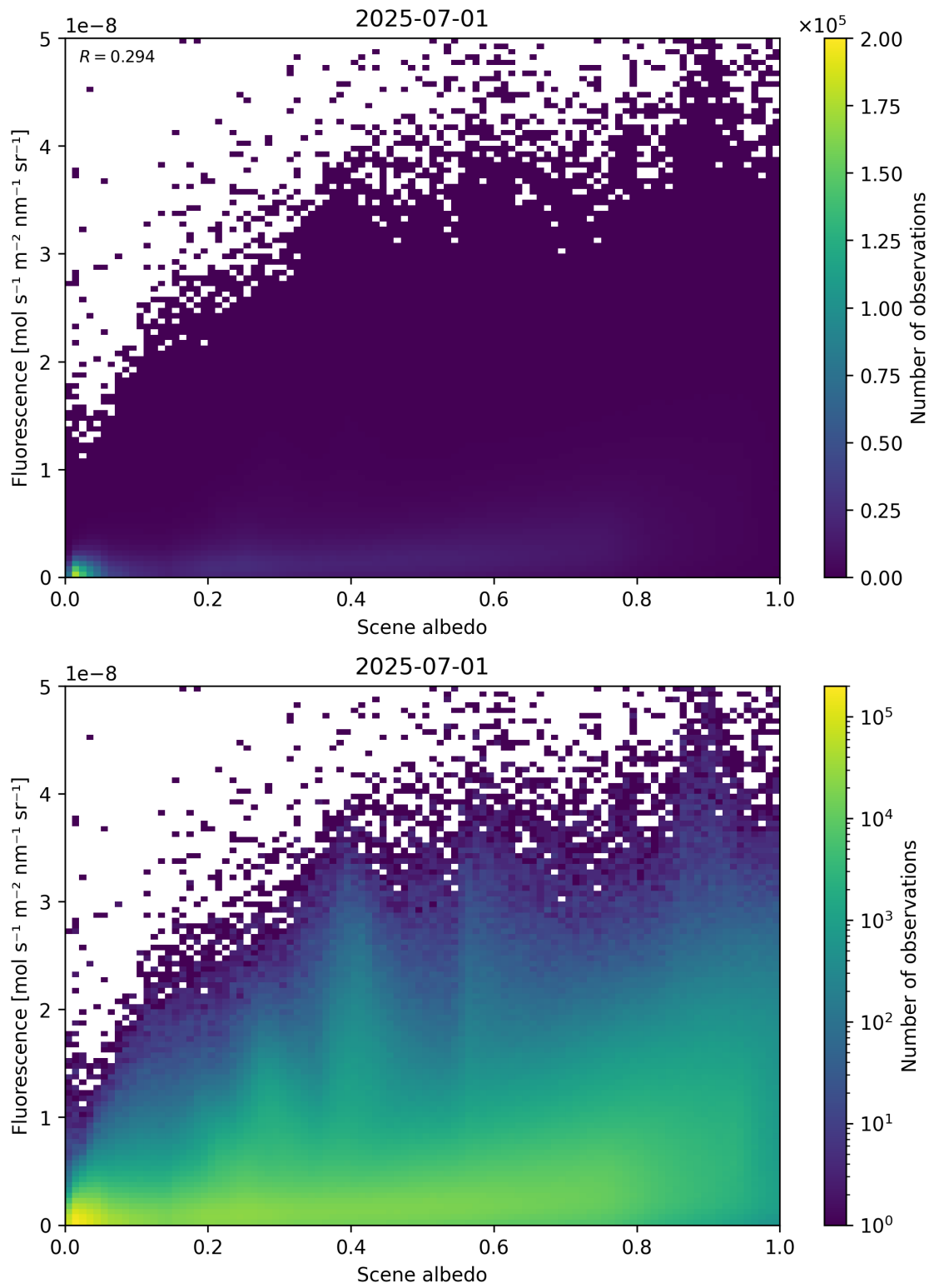
Figure 104: Scatter density plot of “Scene albedo” against “Fluorescence” for 2025-06-30 to 2025-07-02.
