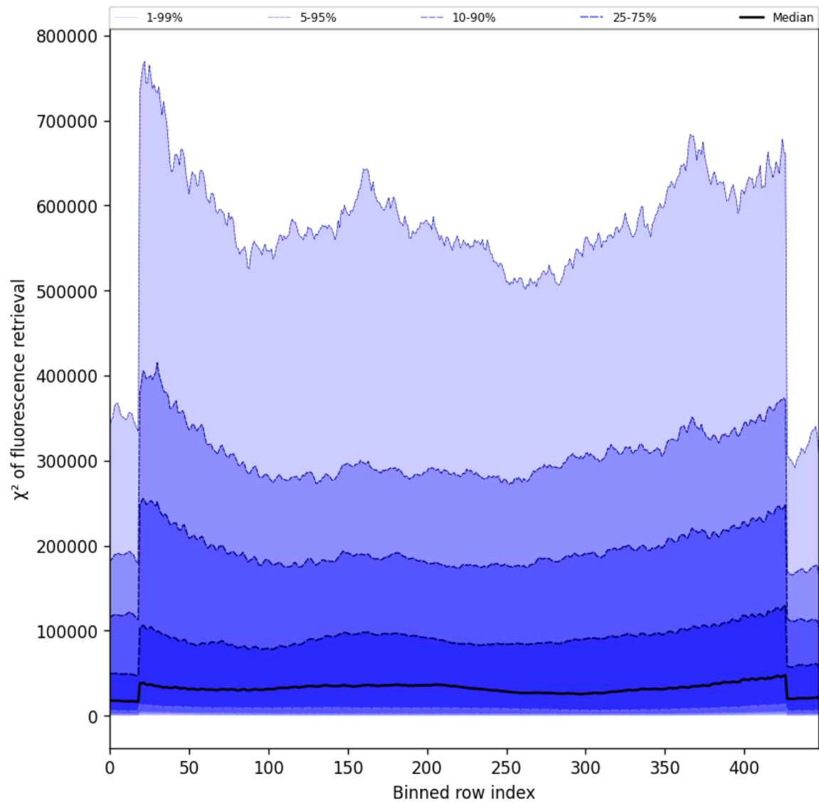
Figure 59: Along track statistics of “ \chi^2 of fluorescence retrieval” for 2025-06-30 to 2025-07-02
