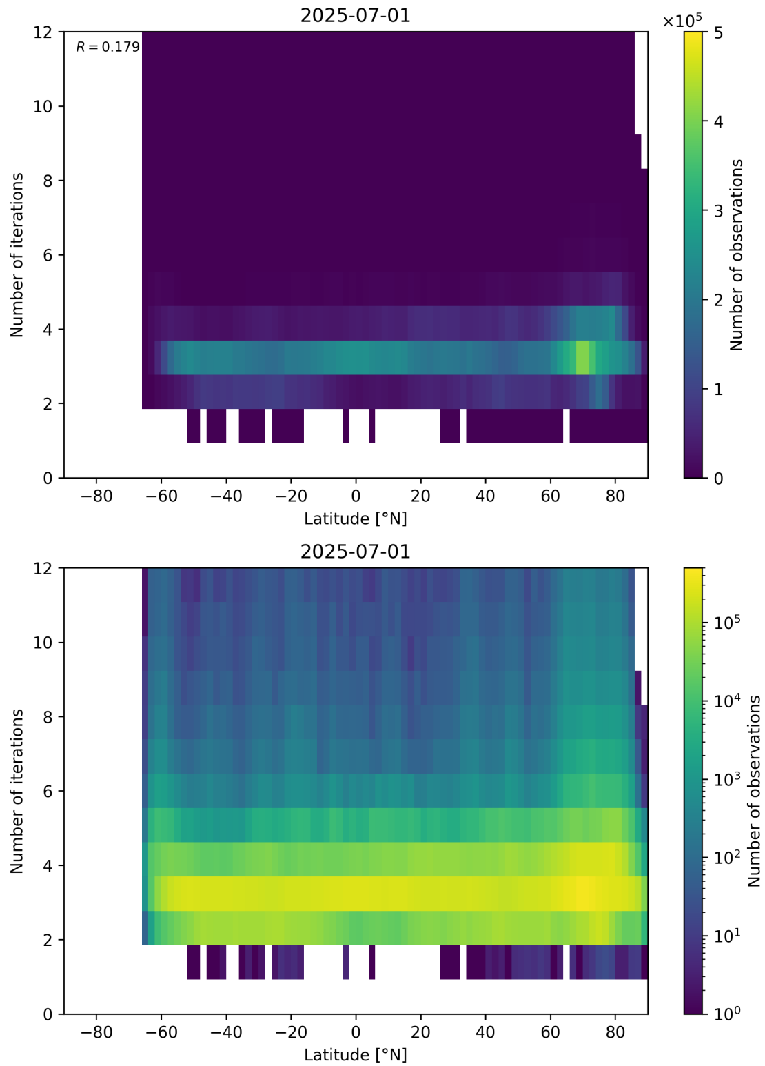
Figure 93: Scatter density plot of “Latitude” against “Number of iterations” for 2025-06-30 to 2025-07-02.
