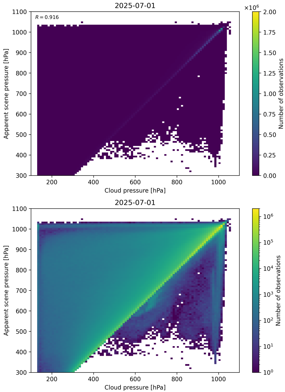
Figure 77: Scatter density plot of “Cloud pressure” against “Apparent scene pressure” for 2025-06-30 to 2025-07-02.
