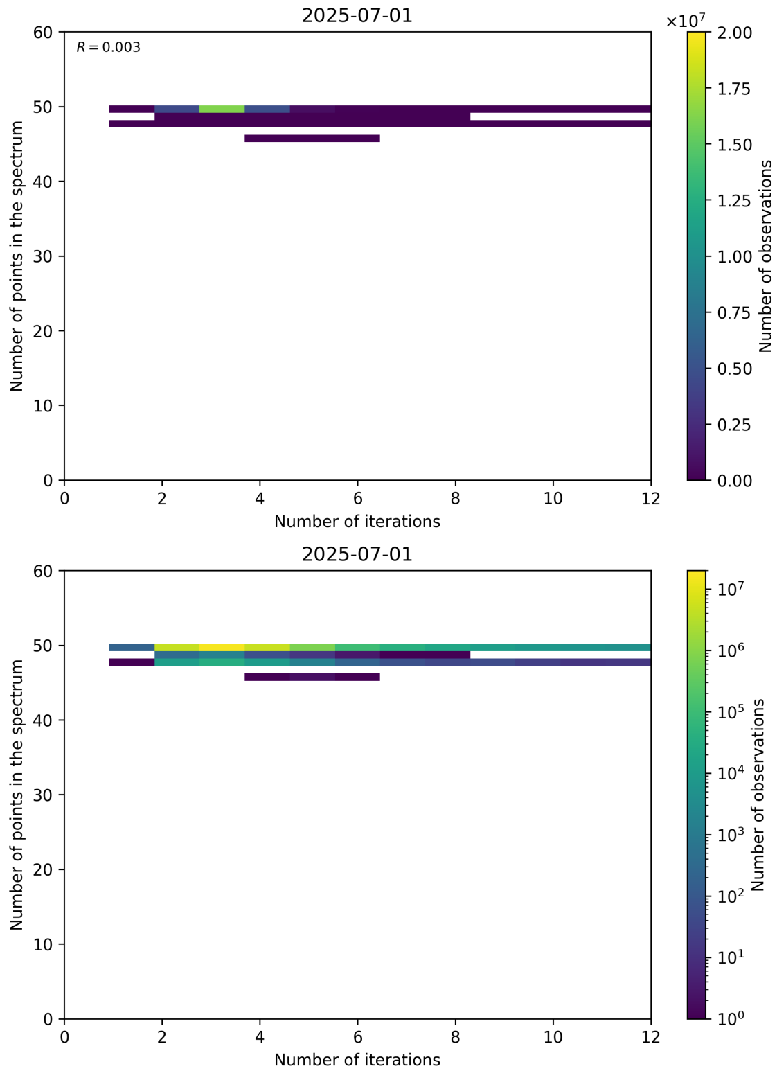
Figure 99: Scatter density plot of “Number of iterations” against “Number of points in the spectrum” for 2025-06-30 to 2025-07-02.
