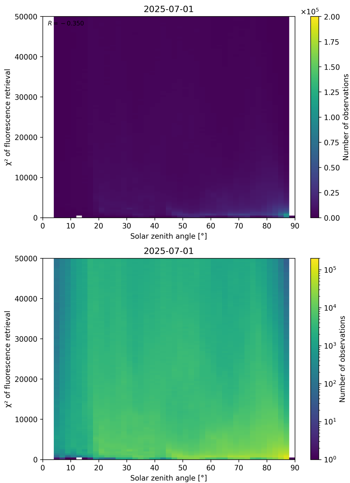
Figure 109: Scatter density plot of “Solar zenith angle” against “ \chi^2 of fluorescence retrieval” for 2025-06-30 to 2025-07-02.
