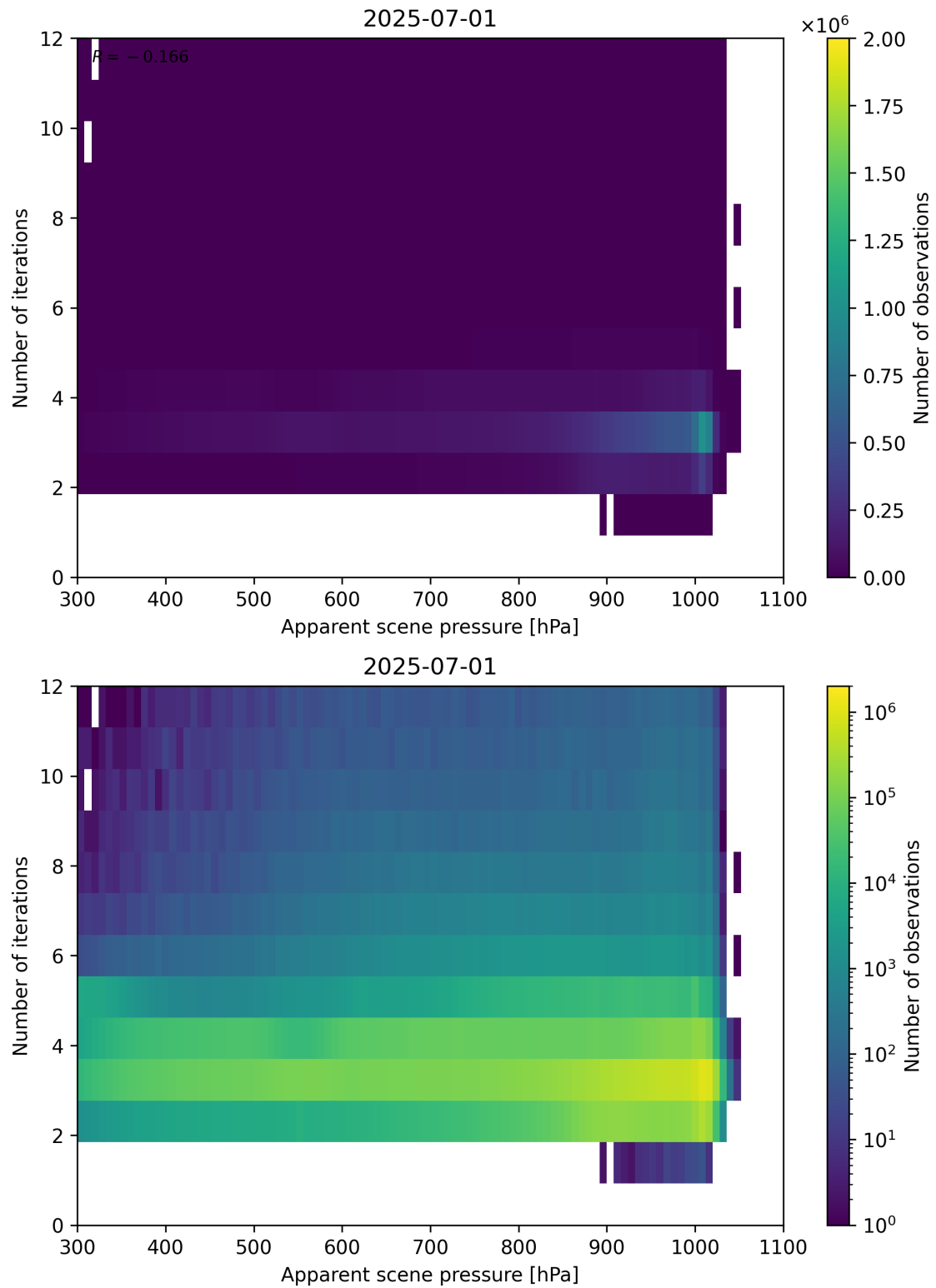
Figure 65: Scatter density plot of “Apparent scene pressure” against “Number of iterations” for 2025-06-30 to 2025-07-02.
