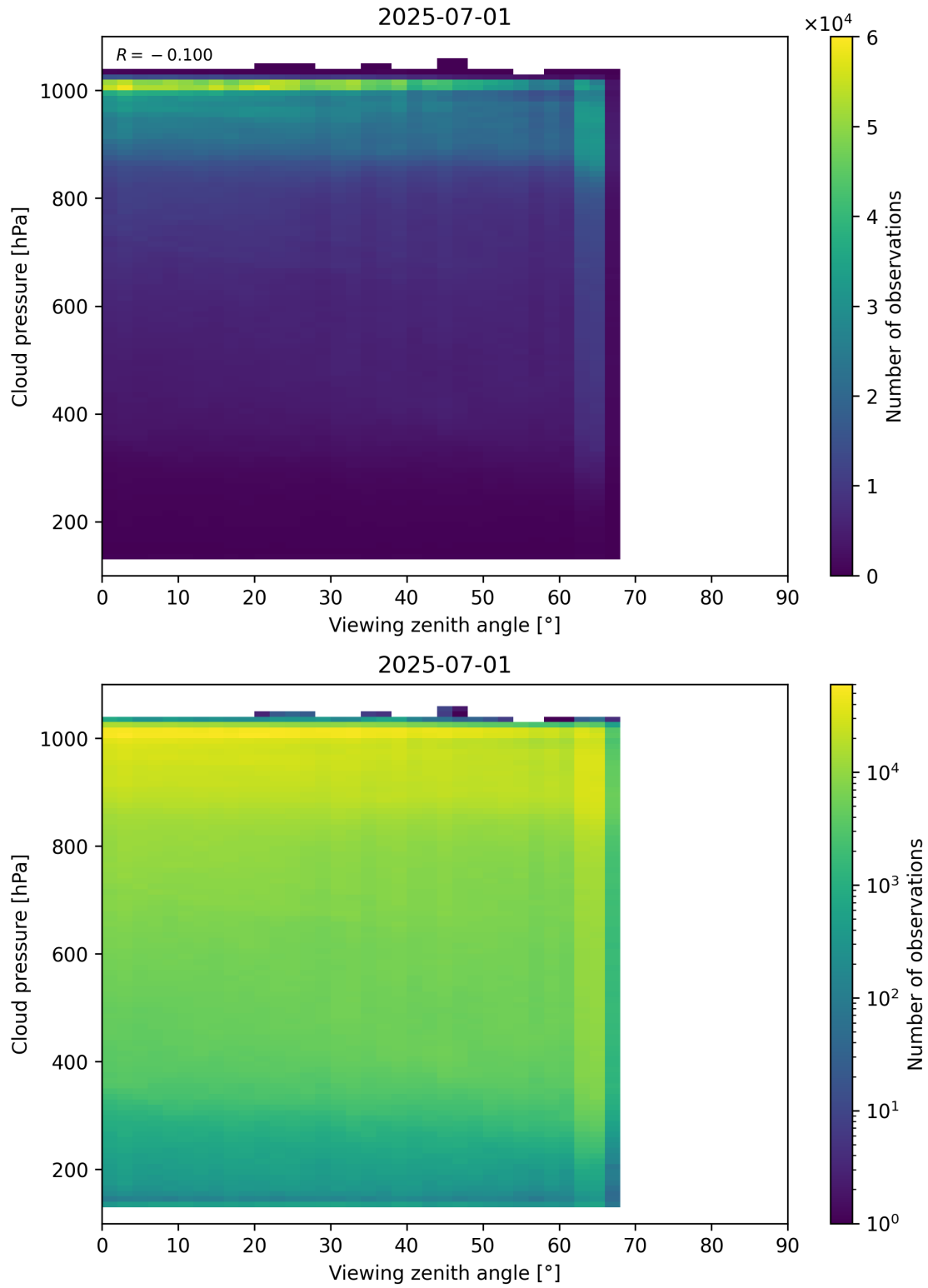
Figure 121: Scatter density plot of “Viewing zenith angle” against “Cloud pressure” for 2025-06-30 to 2025-07-02.
