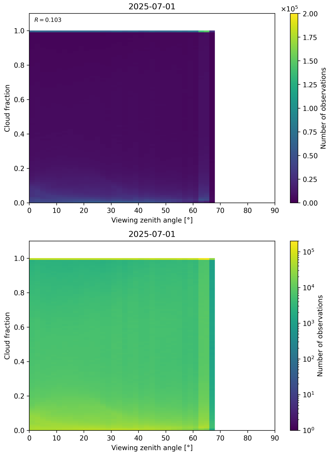
Figure 120: Scatter density plot of “Viewing zenith angle” against “Cloud fraction” for 2025-06-30 to 2025-07-02.
