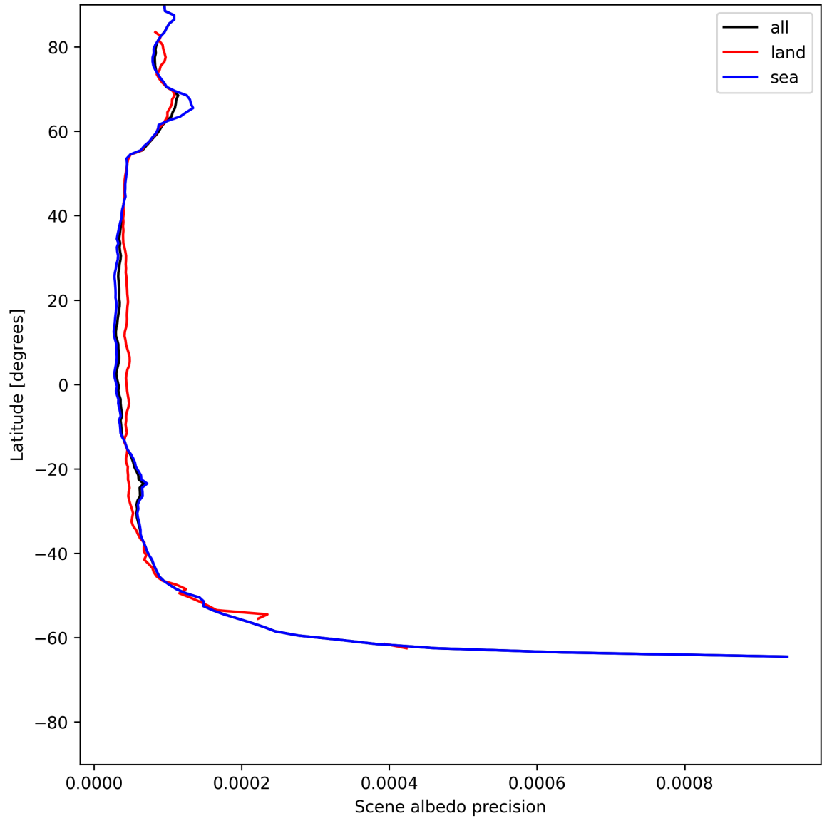
Figure 18: Zonal average of “Scene albedo precision” for 2025-06-30 to 2025-07-02.
