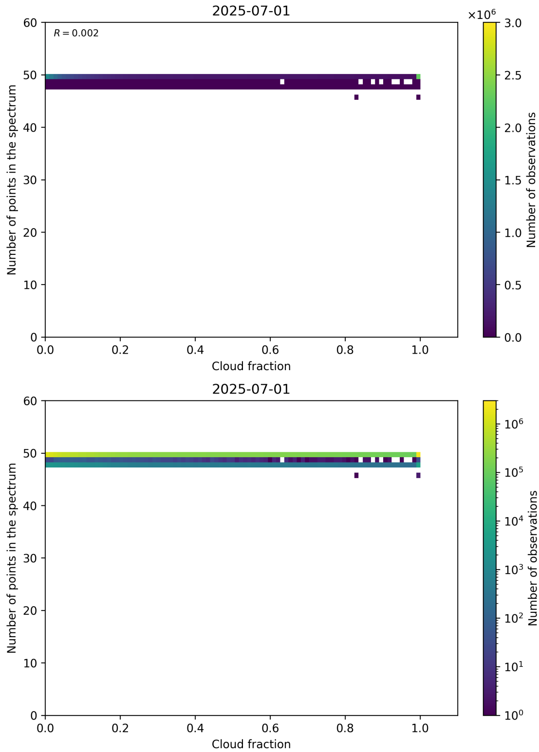
Figure 74: Scatter density plot of “Cloud fraction” against “Number of points in the spectrum” for 2025-06-30 to 2025-07-02.
