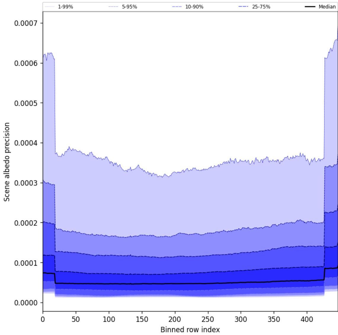
Figure 52: Along track statistics of “Scene albedo precision” for 2025-06-30 to 2025-07-02
