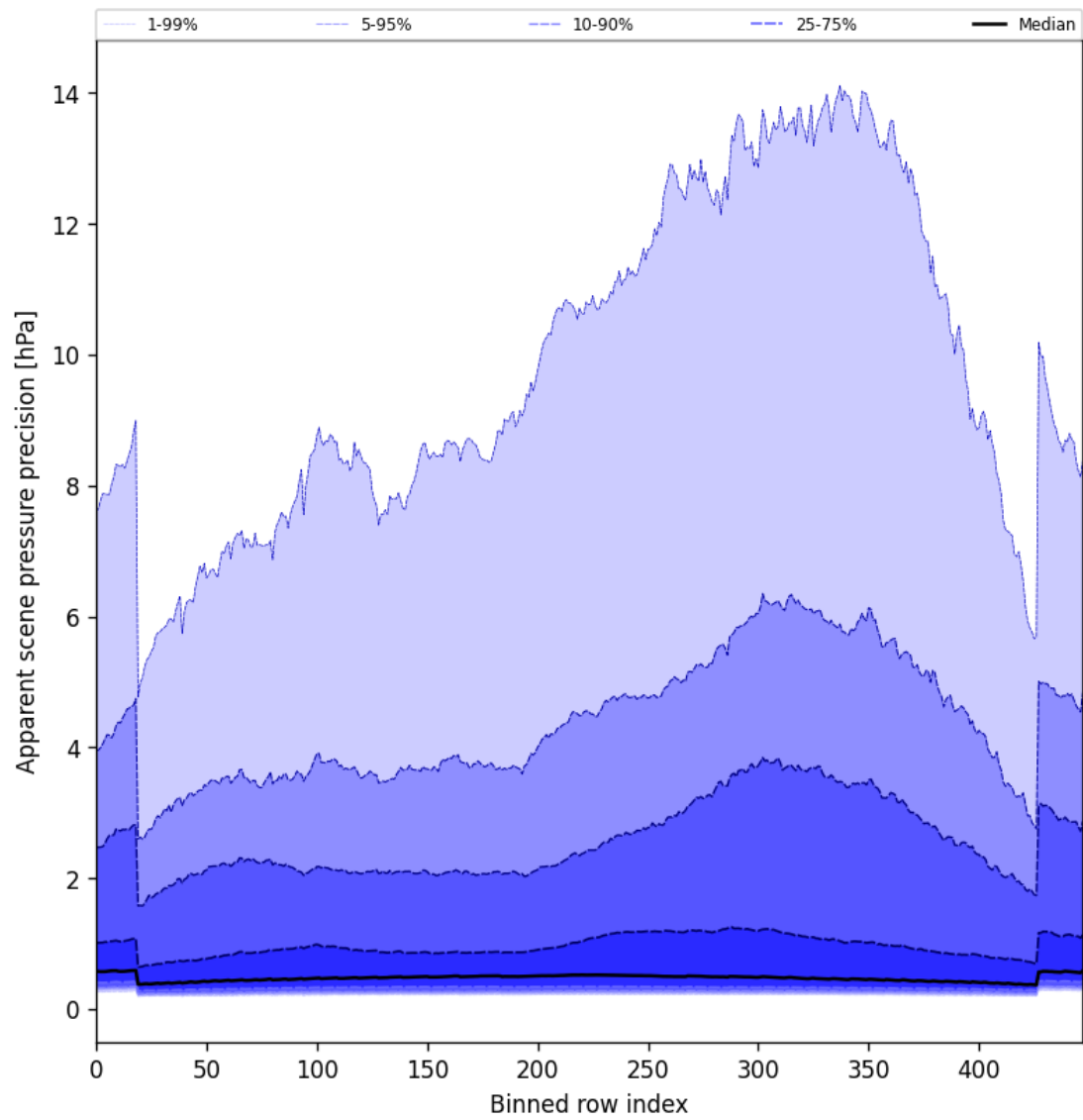
Figure 54: Along track statistics of “Apparent scene pressure precision” for 2025-06-30 to 2025-07-02
