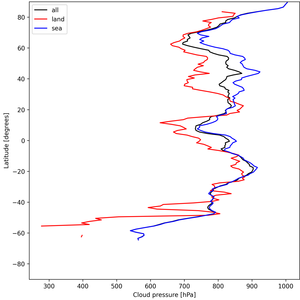
Figure 13: Zonal average of “Cloud pressure” for 2025-06-30 to 2025-07-02.
