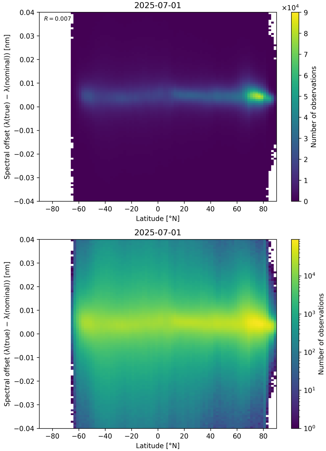
Figure 96: Scatter density plot of “Latitude” against “Spectral offset ( \lambda_{\text{true}} - \lambda_{\text{nominal}} )” for 2025-06-30 to 2025-07-02.
