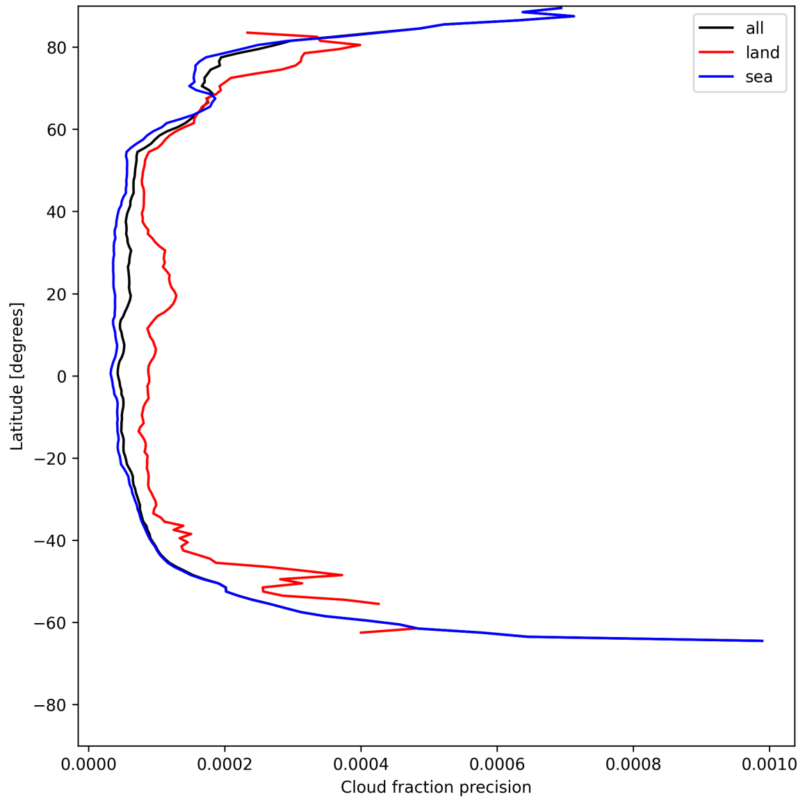
Figure 16: Zonal average of “Cloud fraction precision” for 2025-06-30 to 2025-07-02.
