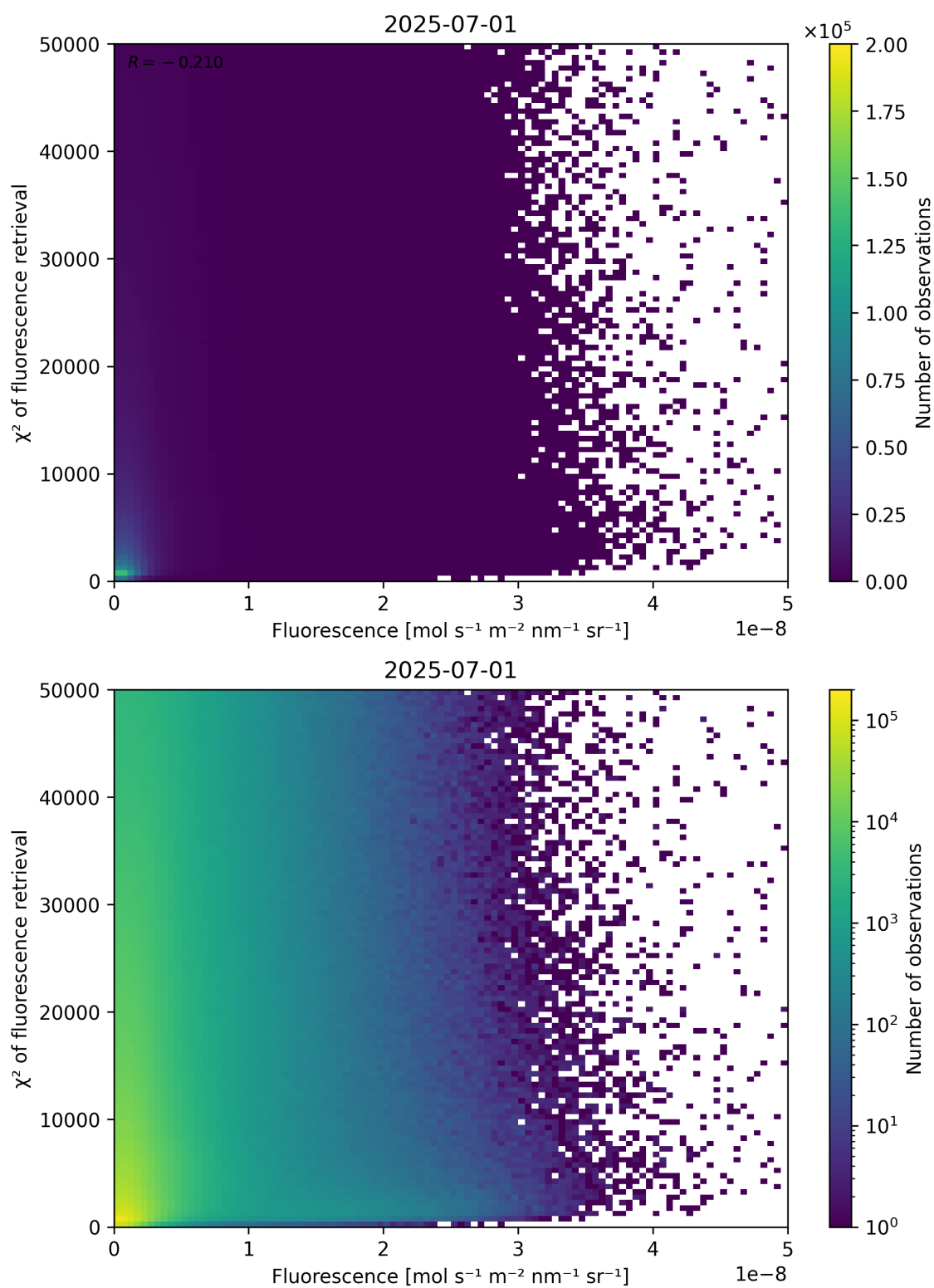
Figure 85: Scatter density plot of “Fluorescence” against “ \chi^2 of fluorescence retrieval” for 2025-06-30 to 2025-07-02.
