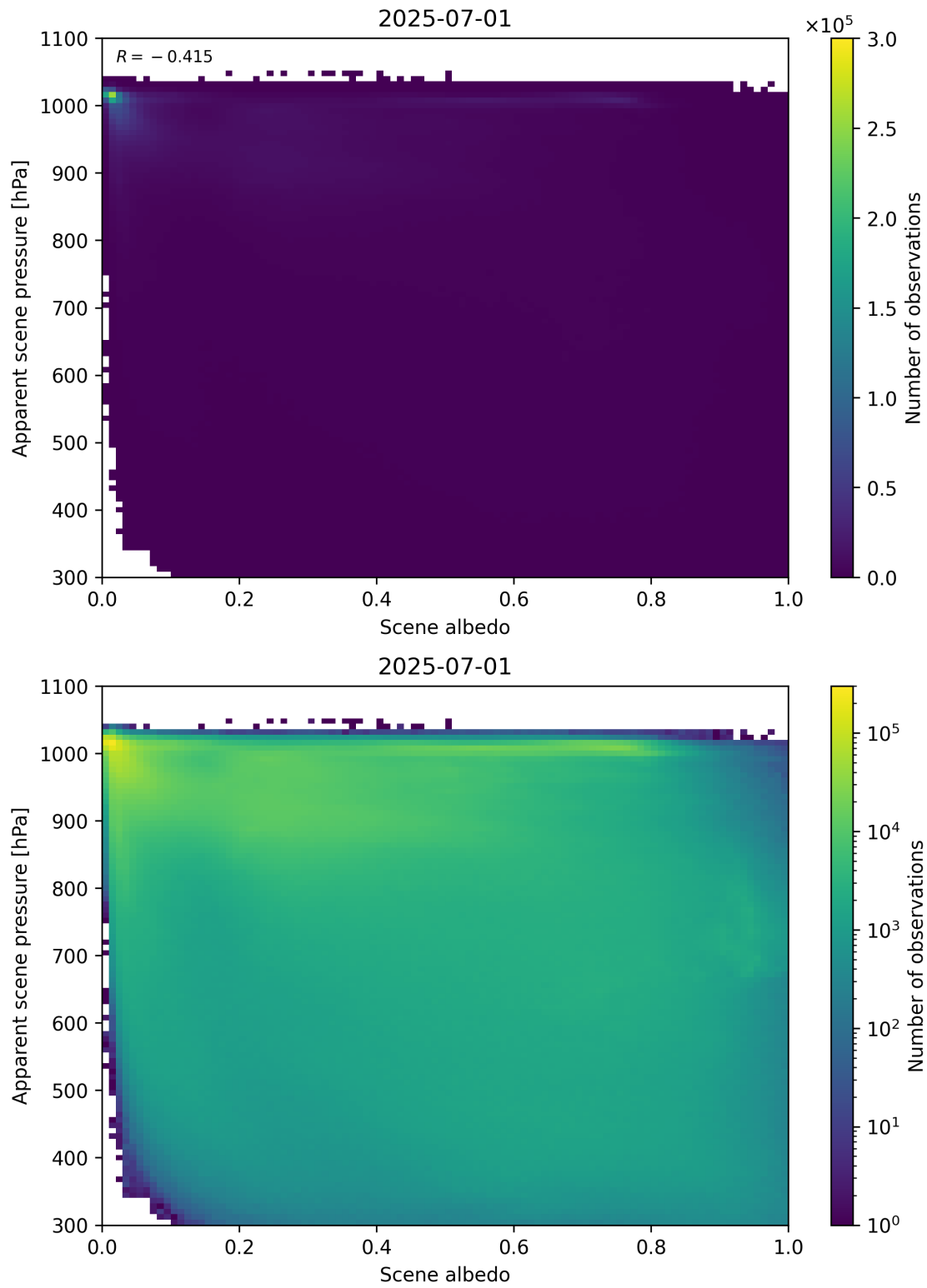
Figure 102: Scatter density plot of “Scene albedo” against “Apparent scene pressure” for 2025-06-30 to 2025-07-02.
