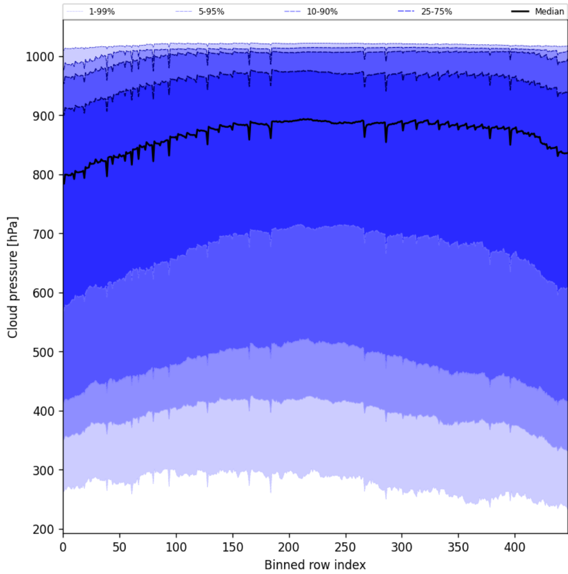
Figure 47: Along track statistics of “Cloud pressure” for 2025-06-30 to 2025-07-02
