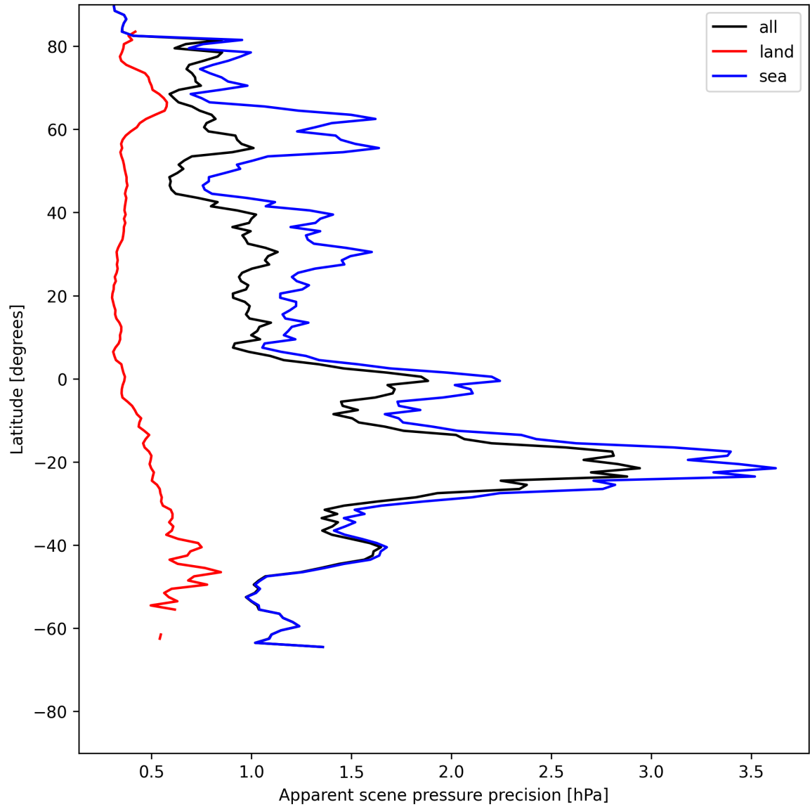
Figure 20: Zonal average of “Apparent scene pressure precision” for 2025-06-30 to 2025-07-02.
