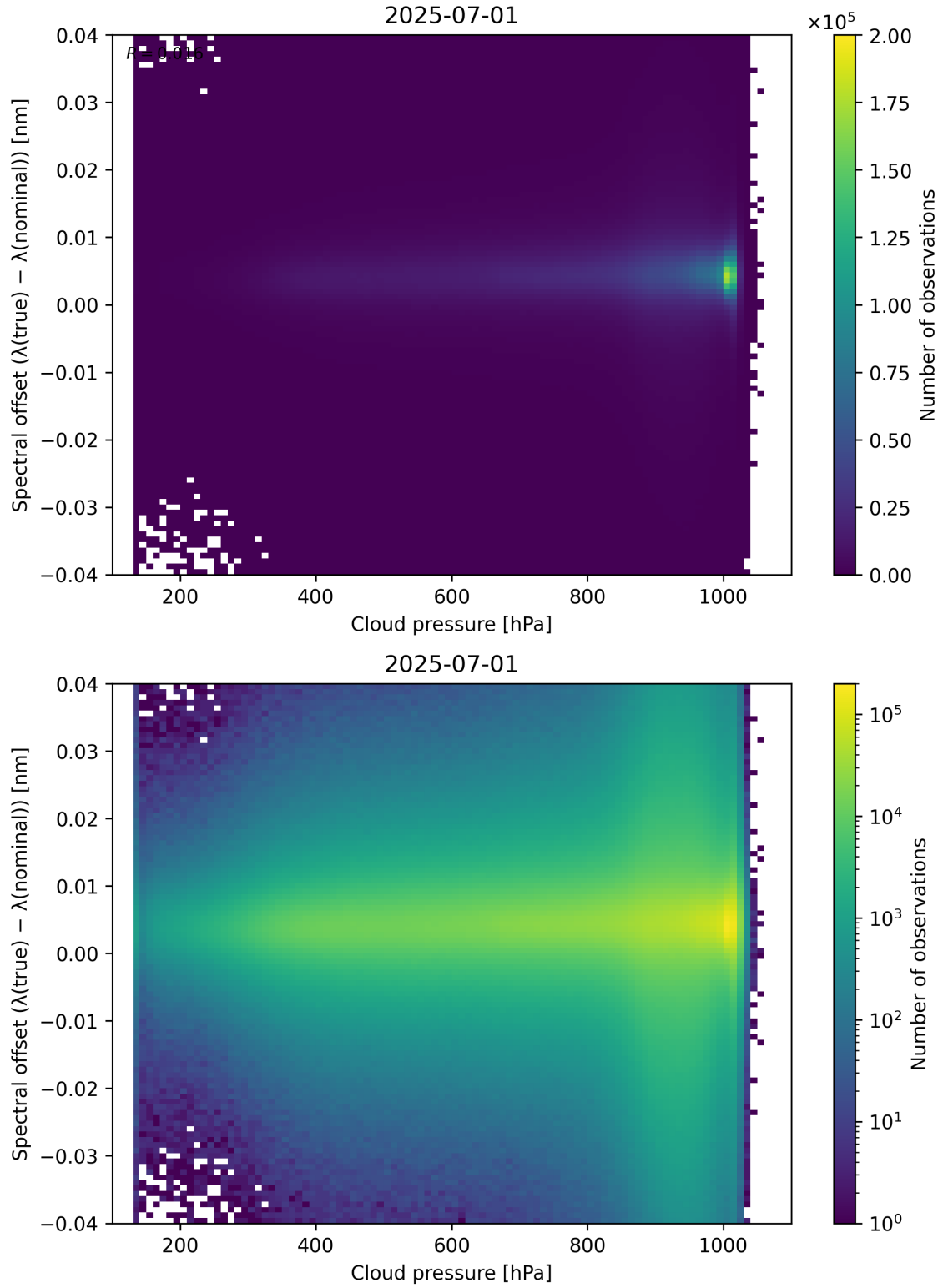
Figure 84: Scatter density plot of “Cloud pressure” against “Spectral offset ( \lambda_{\text{true}} - \lambda_{\text{nominal}} )” for 2025-06-30 to 2025-07-02.
