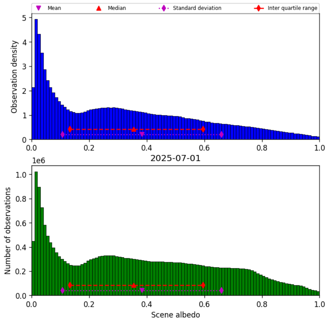
Figure 34: Histogram of “Scene albedo” for 2025-06-30 to 2025-07-02
