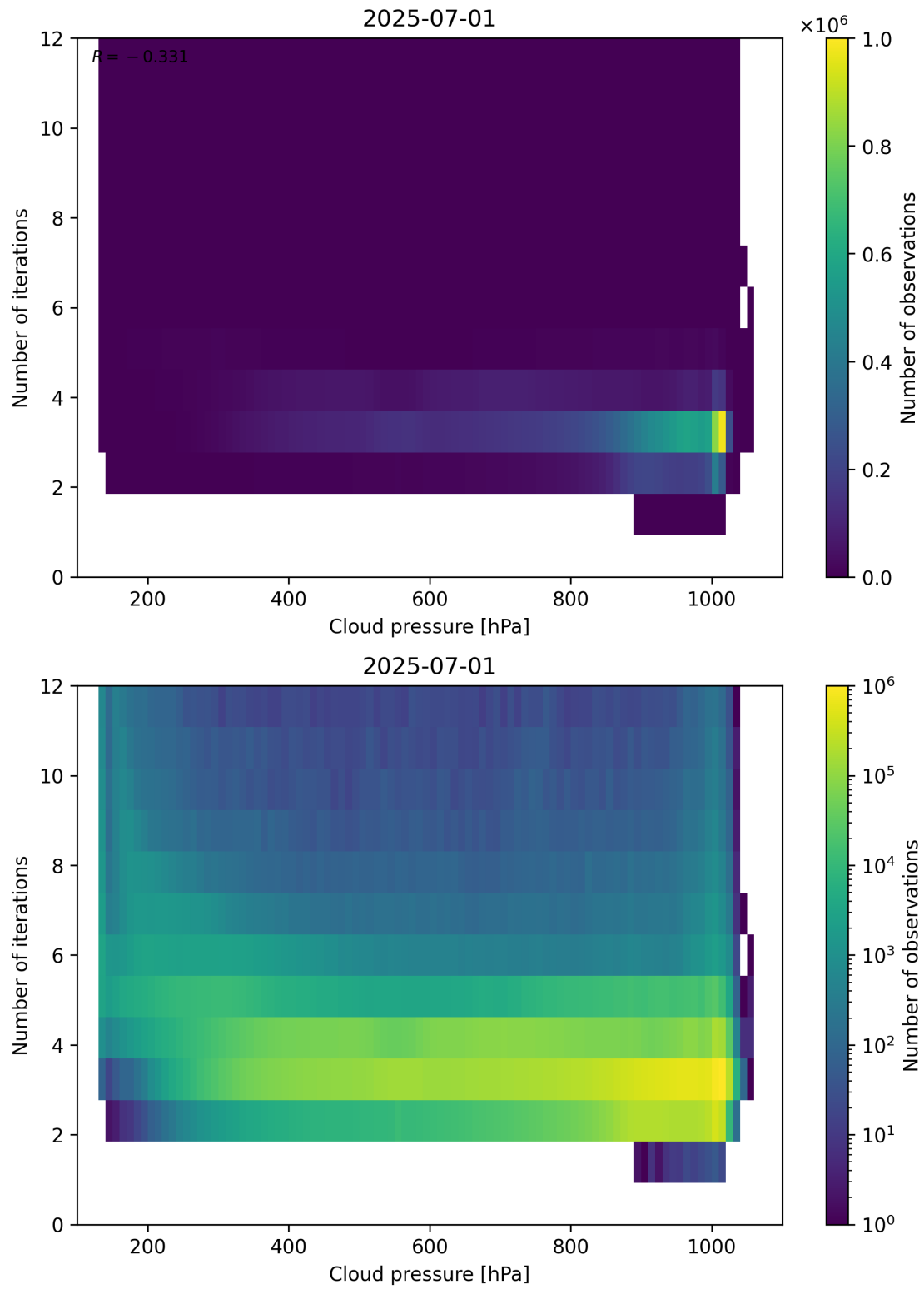
Figure 81: Scatter density plot of “Cloud pressure” against “Number of iterations” for 2025-06-30 to 2025-07-02.
