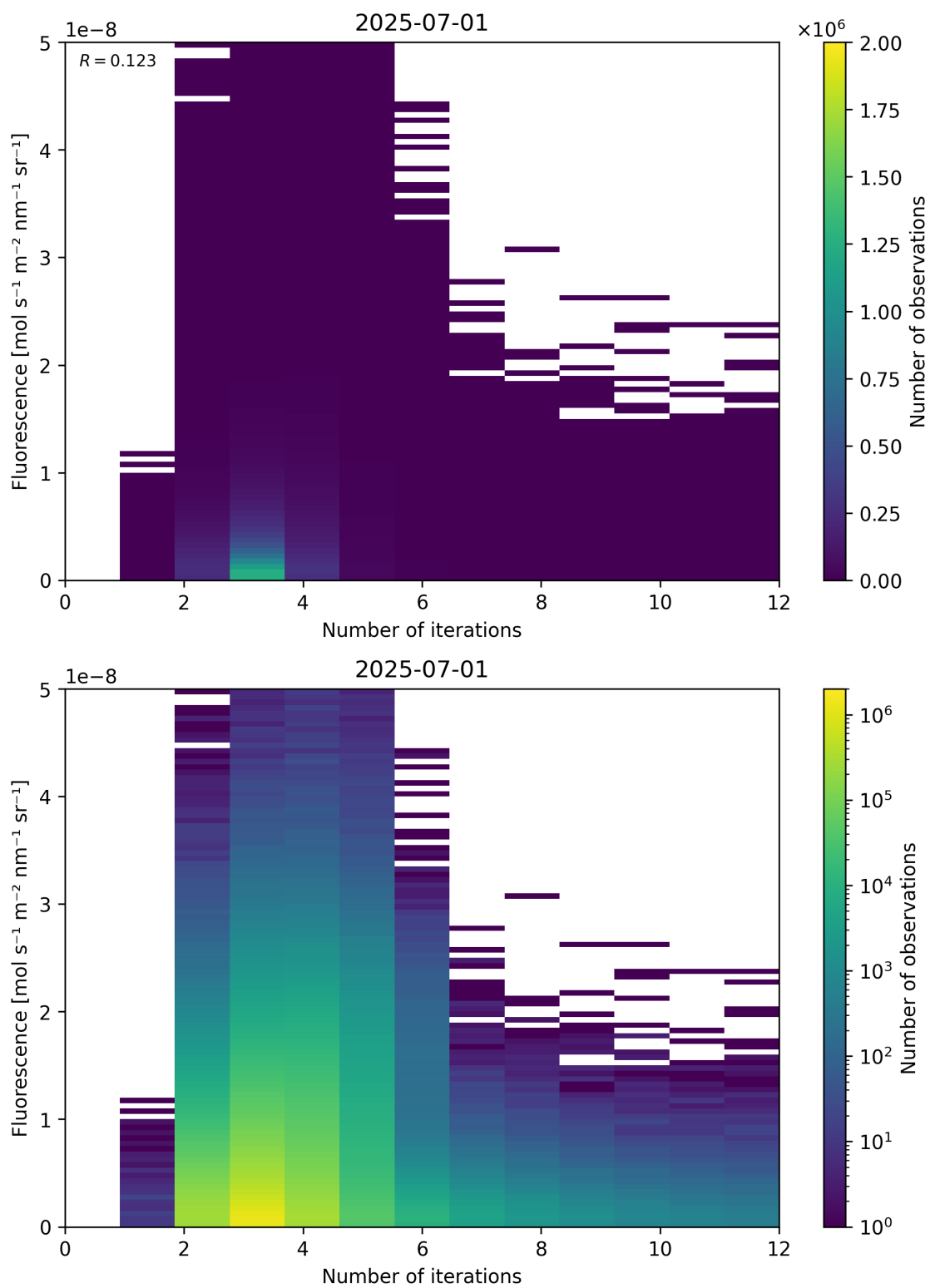
Figure 98: Scatter density plot of “Number of iterations” against “Fluorescence” for 2025-06-30 to 2025-07-02.
