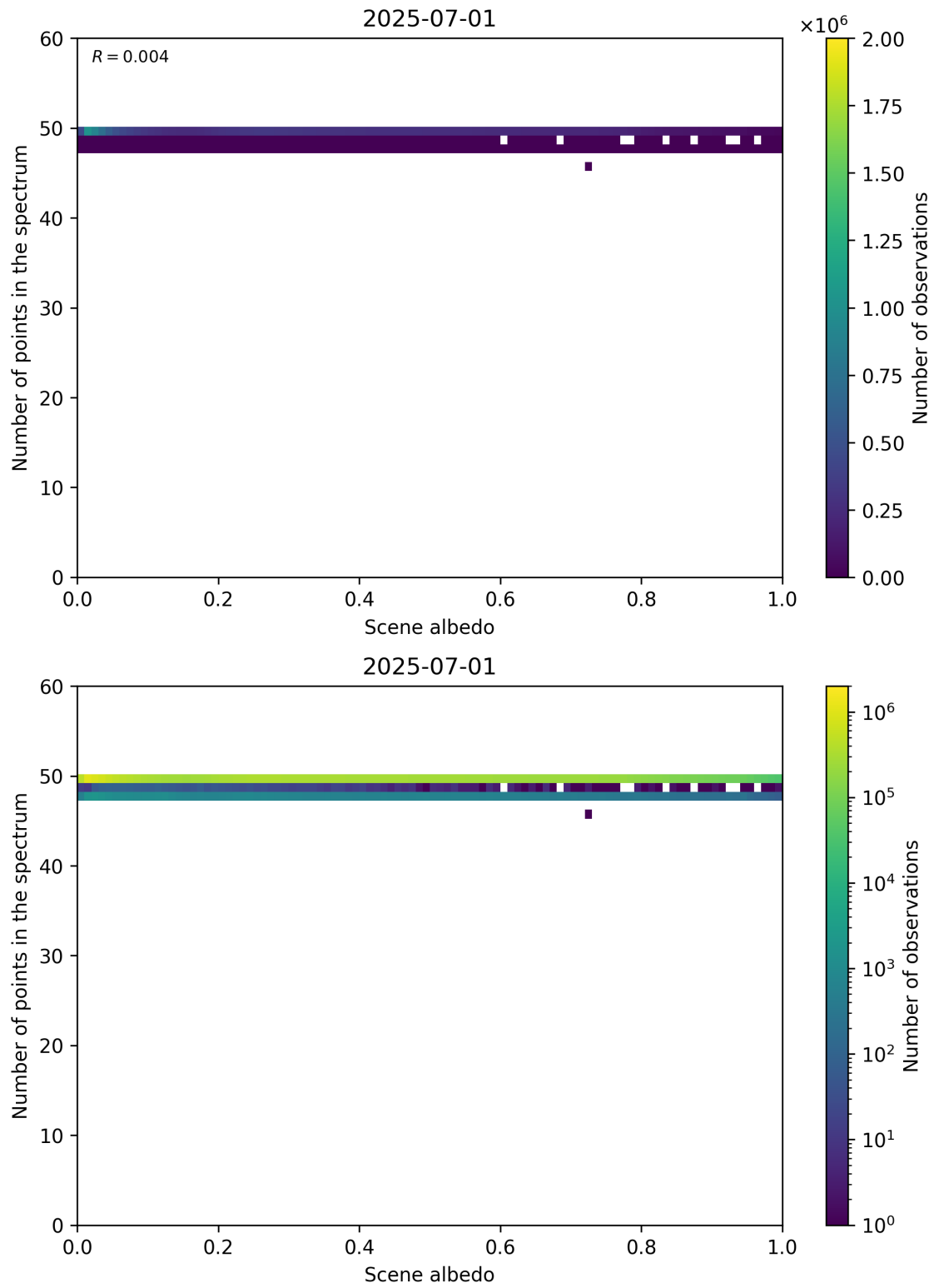
Figure 106: Scatter density plot of “Scene albedo” against “Number of points in the spectrum” for 2025-06-30 to 2025-07-02.
