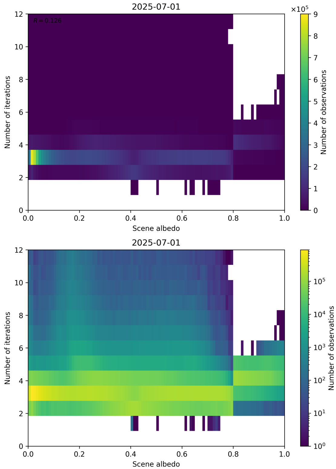
Figure 105: Scatter density plot of “Scene albedo” against “Number of iterations” for 2025-06-30 to 2025-07-02.
