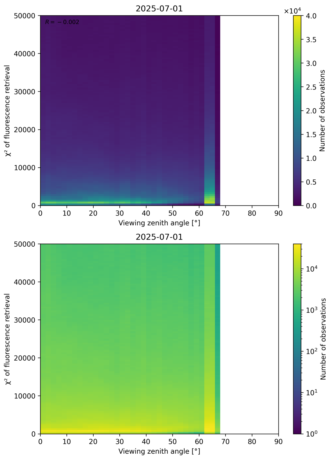
Figure 119: Scatter density plot of “Viewing zenith angle” against “ \chi^2 of fluorescence retrieval” for 2025-06-30 to 2025-07-02.
