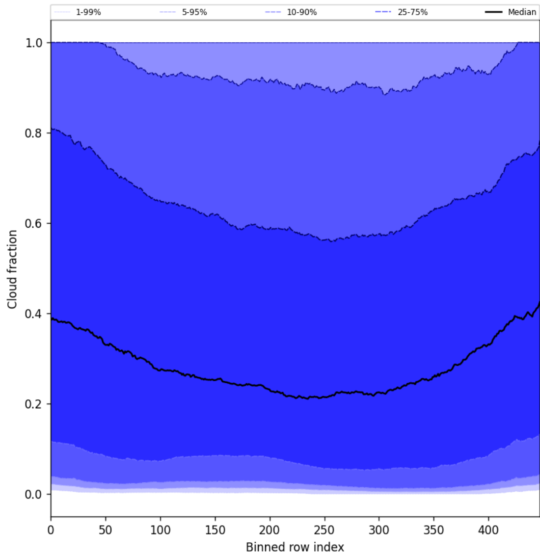
Figure 49: Along track statistics of “Cloud fraction” for 2025-06-30 to 2025-07-02
