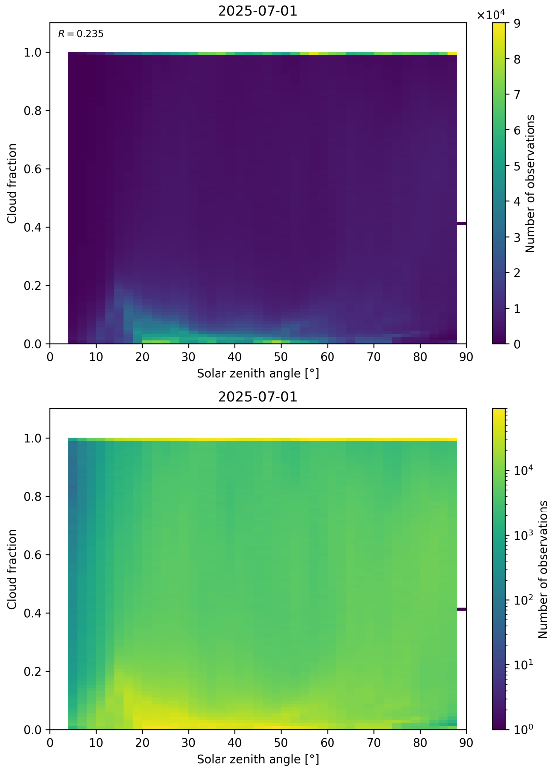
Figure 110: Scatter density plot of “Solar zenith angle” against “Cloud fraction” for 2025-06-30 to 2025-07-02.
