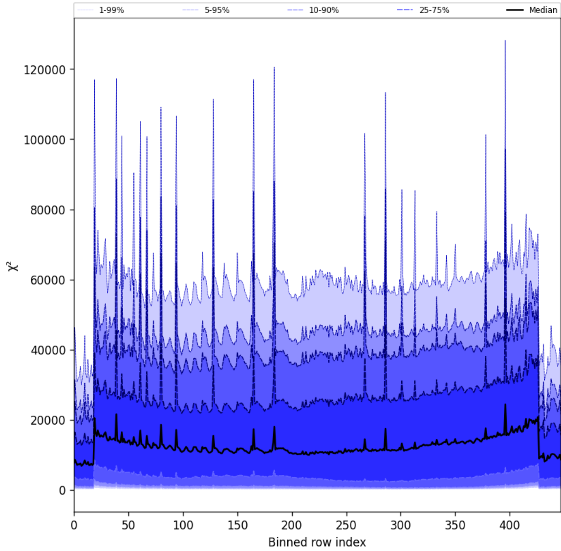
Figure 55: Along track statistics of “ \chi^2 ” for 2025-06-30 to 2025-07-02
