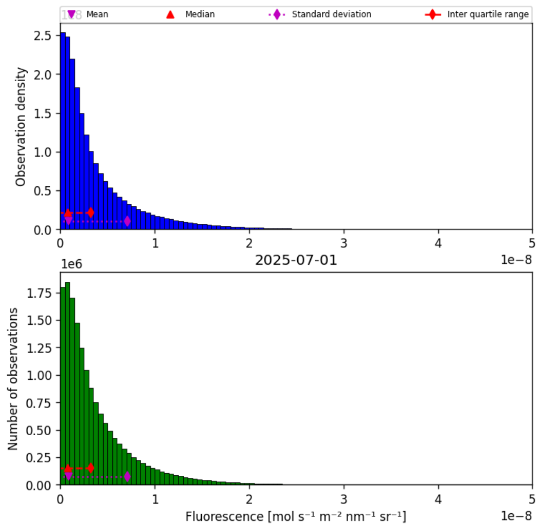
Figure 40: Histogram of “Fluorescence” for 2025-06-30 to 2025-07-02
