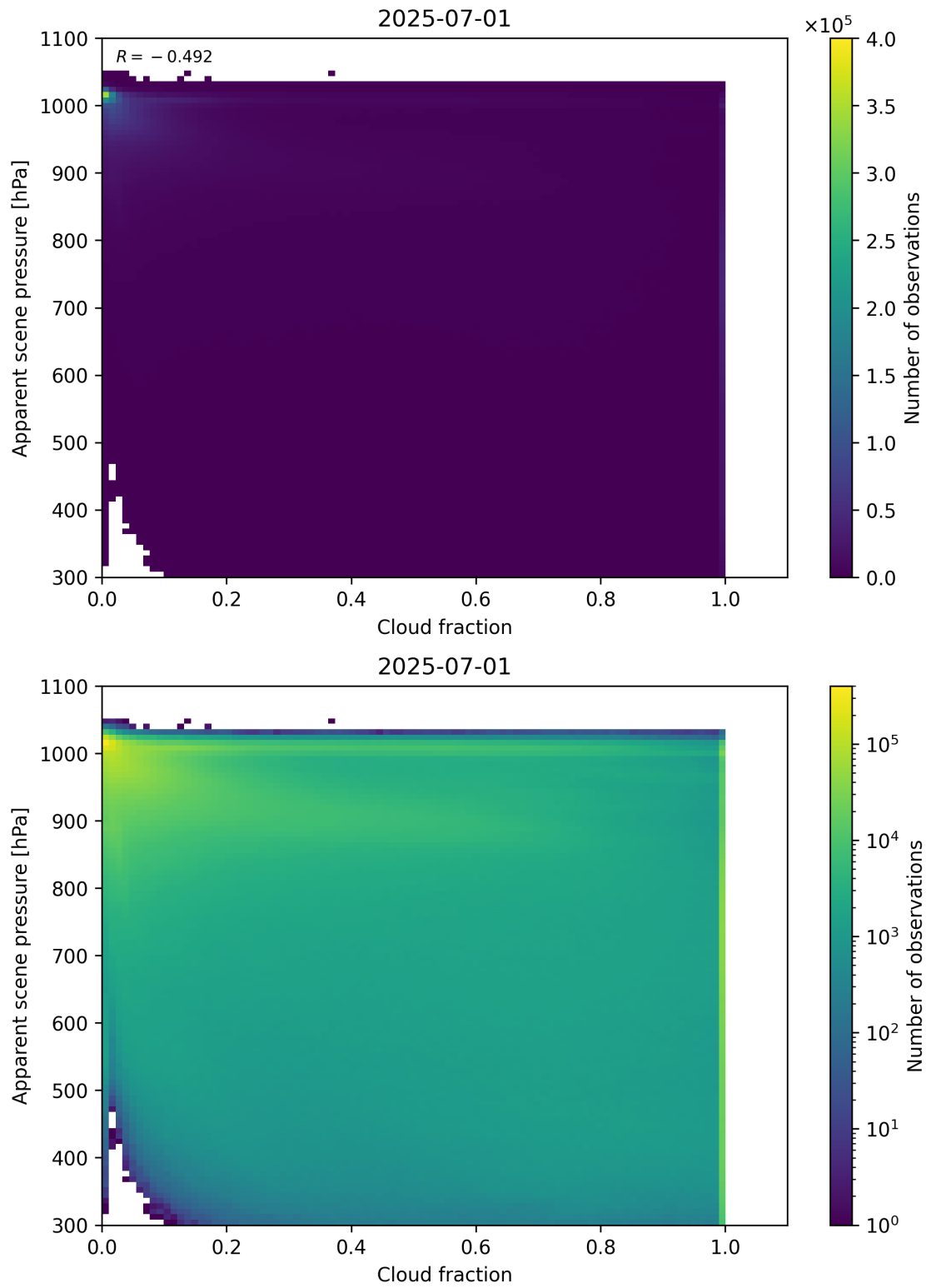
Figure 70: Scatter density plot of “Cloud fraction” against “Apparent scene pressure” for 2025-06-30 to 2025-07-02.
