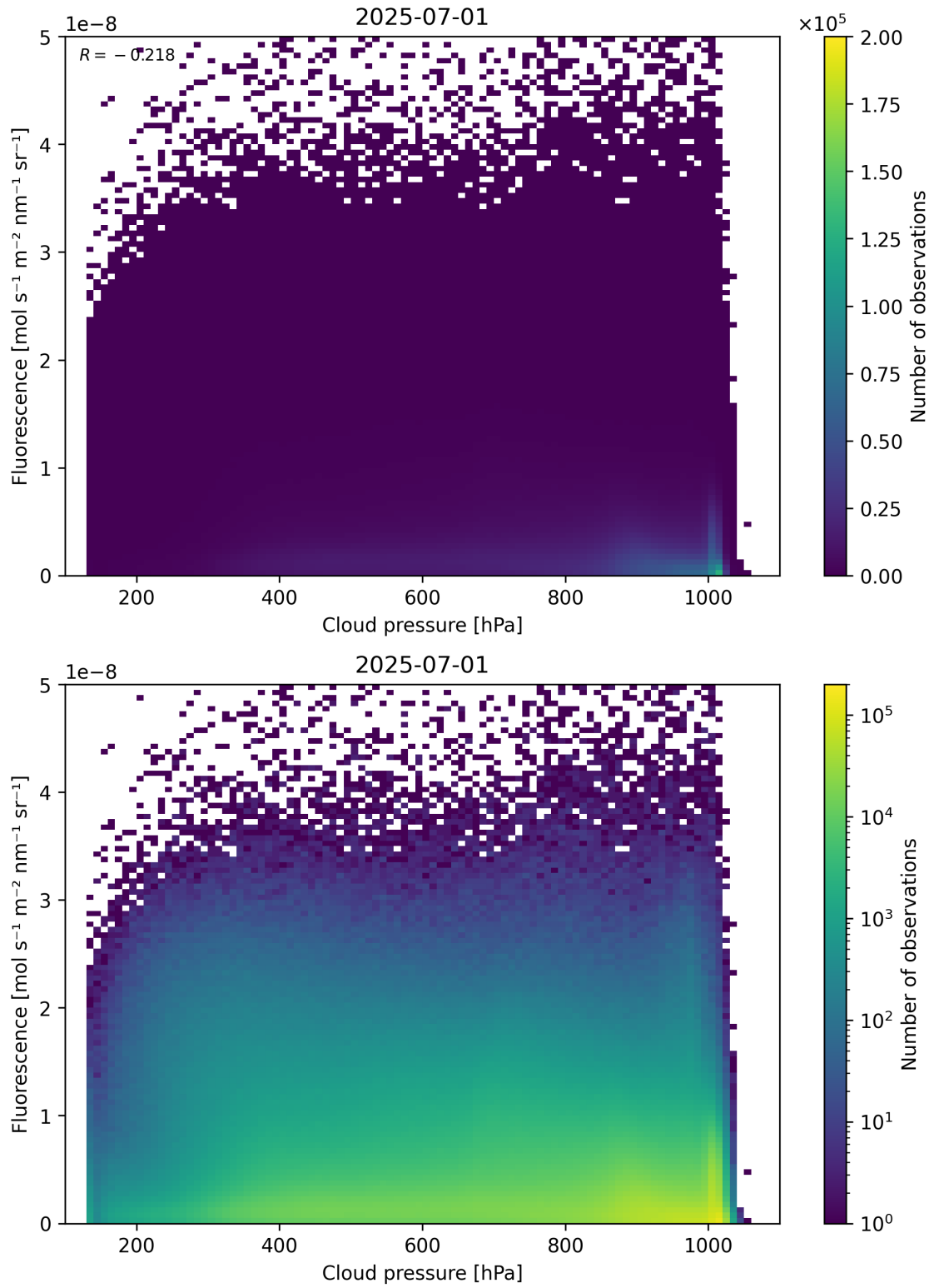
Figure 80: Scatter density plot of “Cloud pressure” against “Fluorescence” for 2025-06-30 to 2025-07-02.
