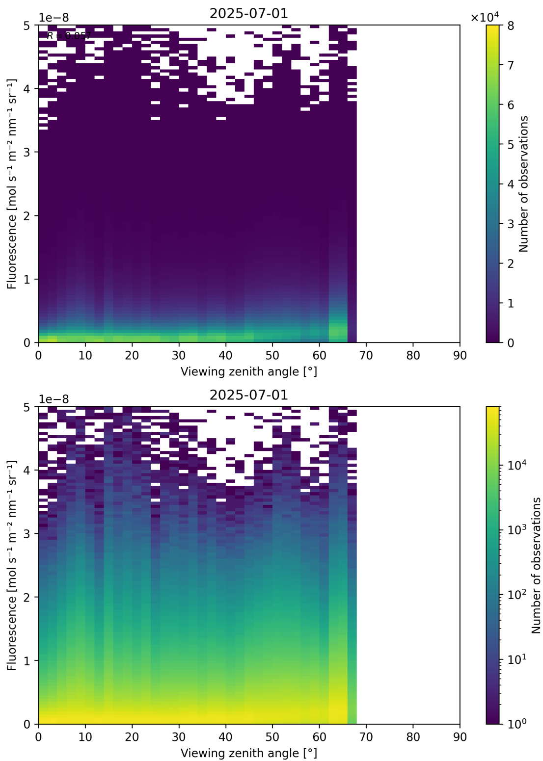
Figure 122: Scatter density plot of “Viewing zenith angle” against “Fluorescence” for 2025-06-30 to 2025-07-02.
