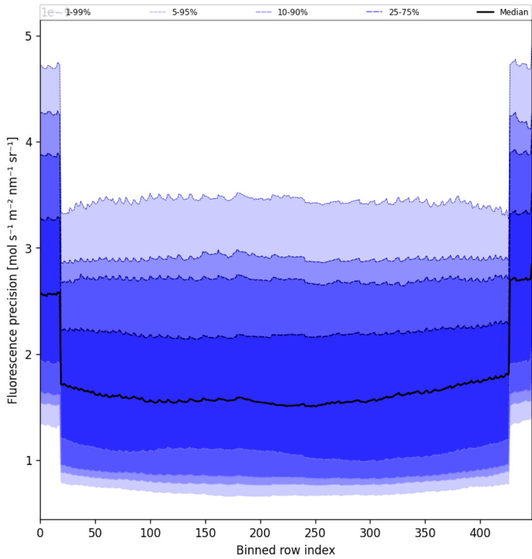
Figure 58: Along track statistics of “Fluorescence precision” for 2025-06-30 to 2025-07-02
