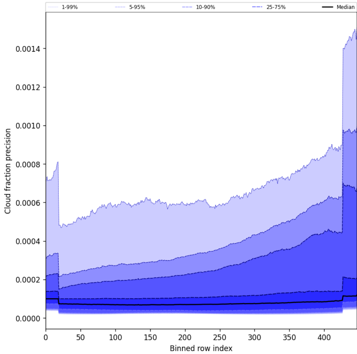
Figure 50: Along track statistics of “Cloud fraction precision” for 2025-06-30 to 2025-07-02
