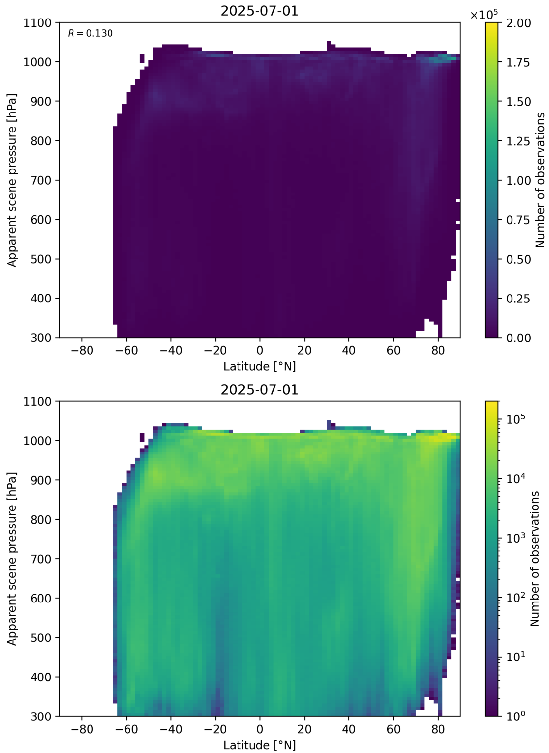
Figure 88: Scatter density plot of “Latitude” against “Apparent scene pressure” for 2025-06-30 to 2025-07-02.
