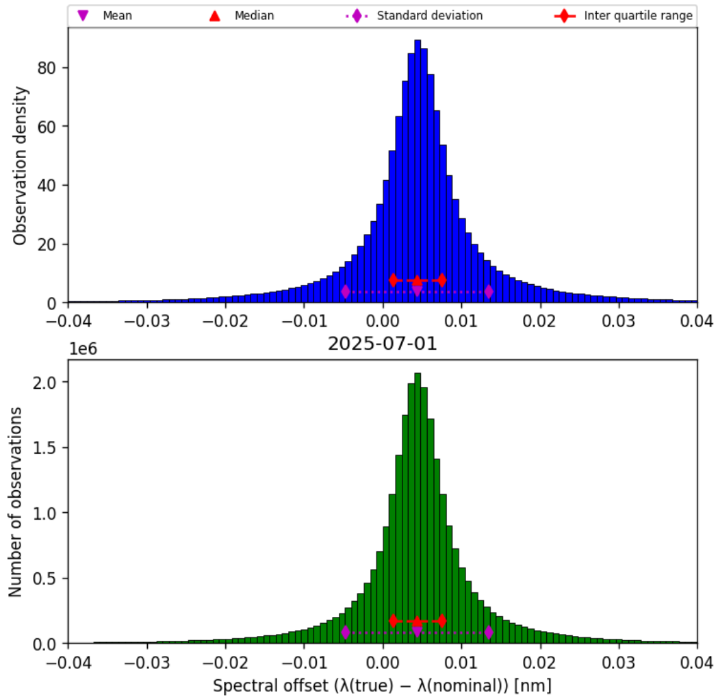
Figure 45: Histogram of “Spectral offset ( \lambda_{\text{true}} - \lambda_{\text{nominal}} )” for 2025-06-30 to 2025-07-02
