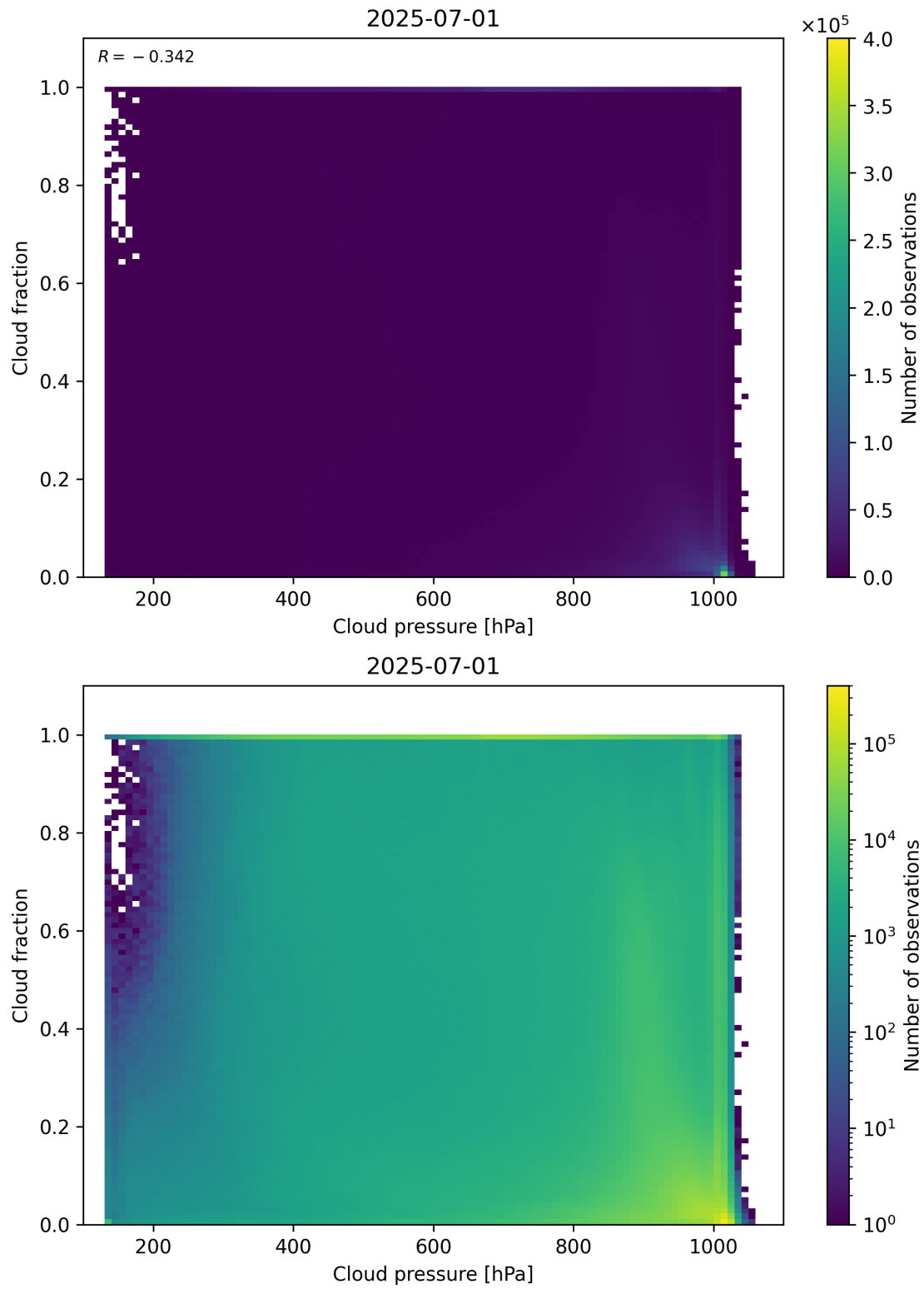
Figure 79: Scatter density plot of “Cloud pressure” against “Cloud fraction” for 2025-06-30 to 2025-07-02.
