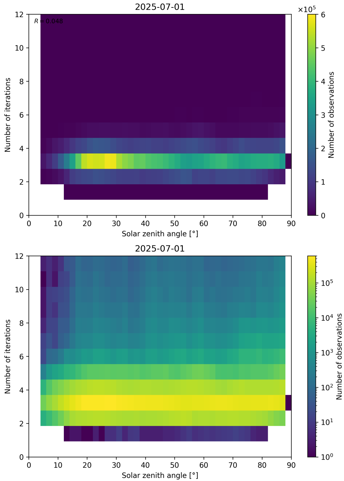
Figure 114: Scatter density plot of “Solar zenith angle” against “Number of iterations” for 2025-06-30 to 2025-07-02.
