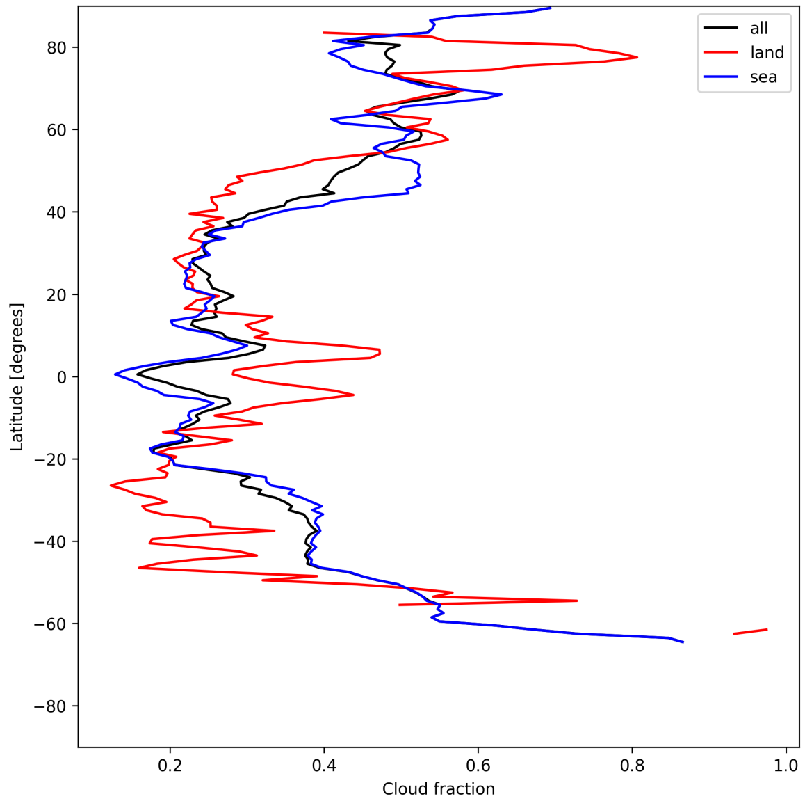
Figure 15: Zonal average of “Cloud fraction” for 2025-06-30 to 2025-07-02.
