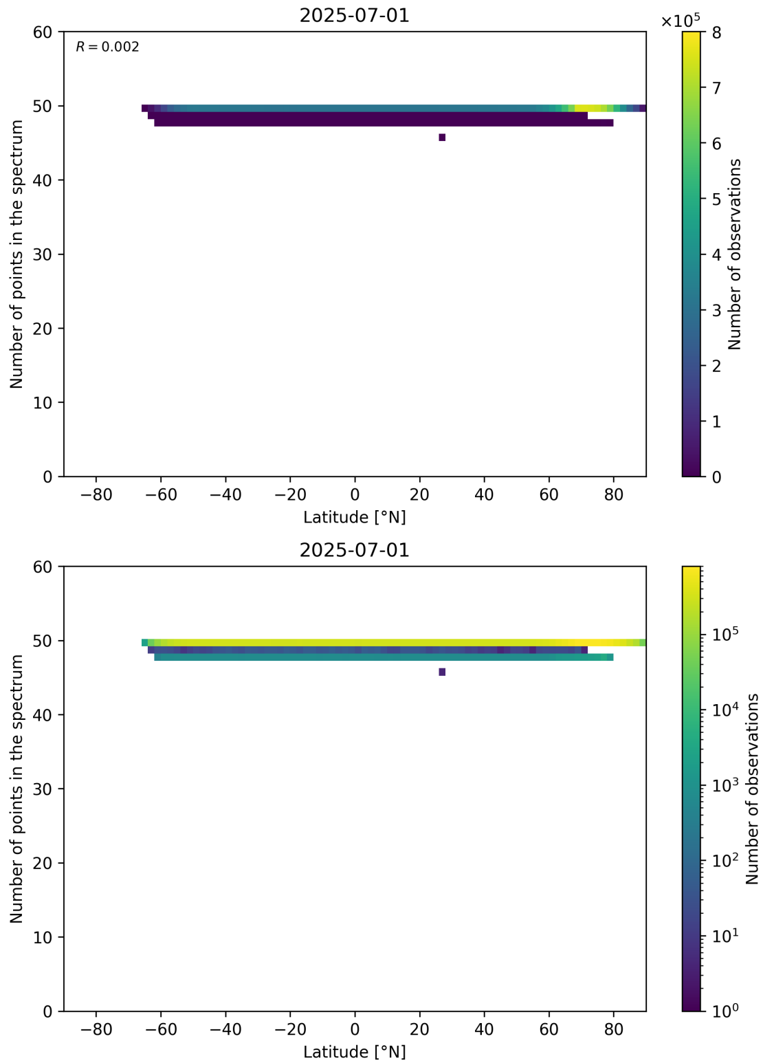
Figure 94: Scatter density plot of “Latitude” against “Number of points in the spectrum” for 2025-06-30 to 2025-07-02.
