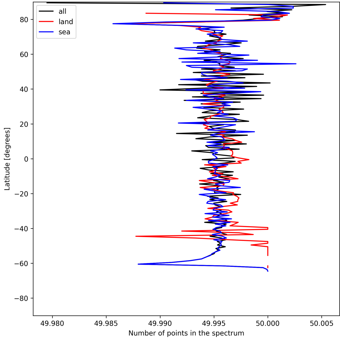
Figure 27: Zonal average of “Number of points in the spectrum” for 2025-06-30 to 2025-07-02.
