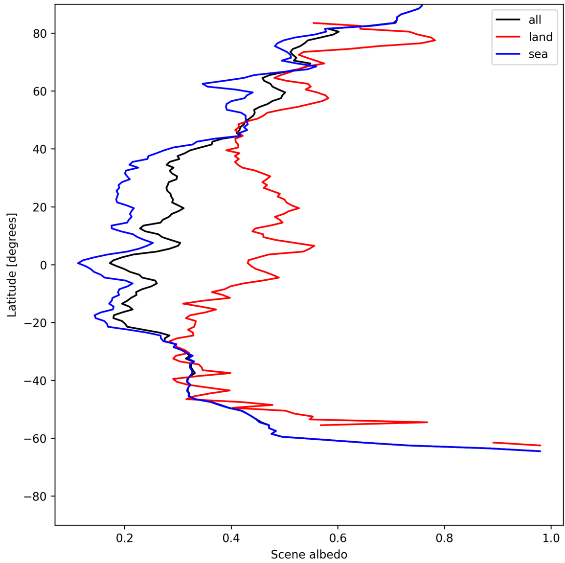
Figure 17: Zonal average of “Scene albedo” for 2025-06-30 to 2025-07-02.
