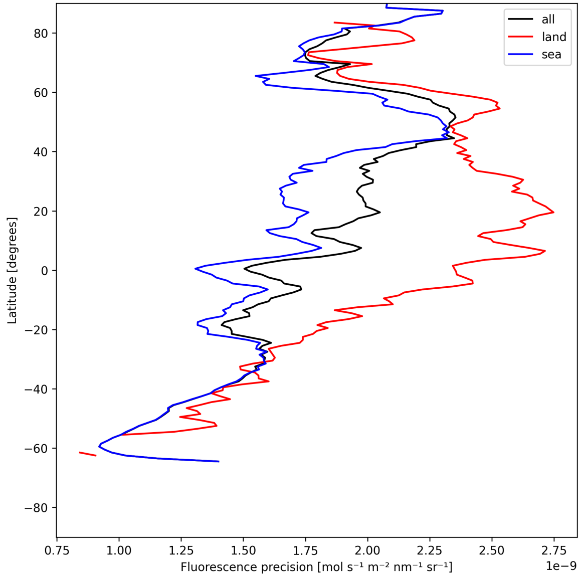
Figure 24: Zonal average of “Fluorescence precision” for 2025-06-30 to 2025-07-02.
