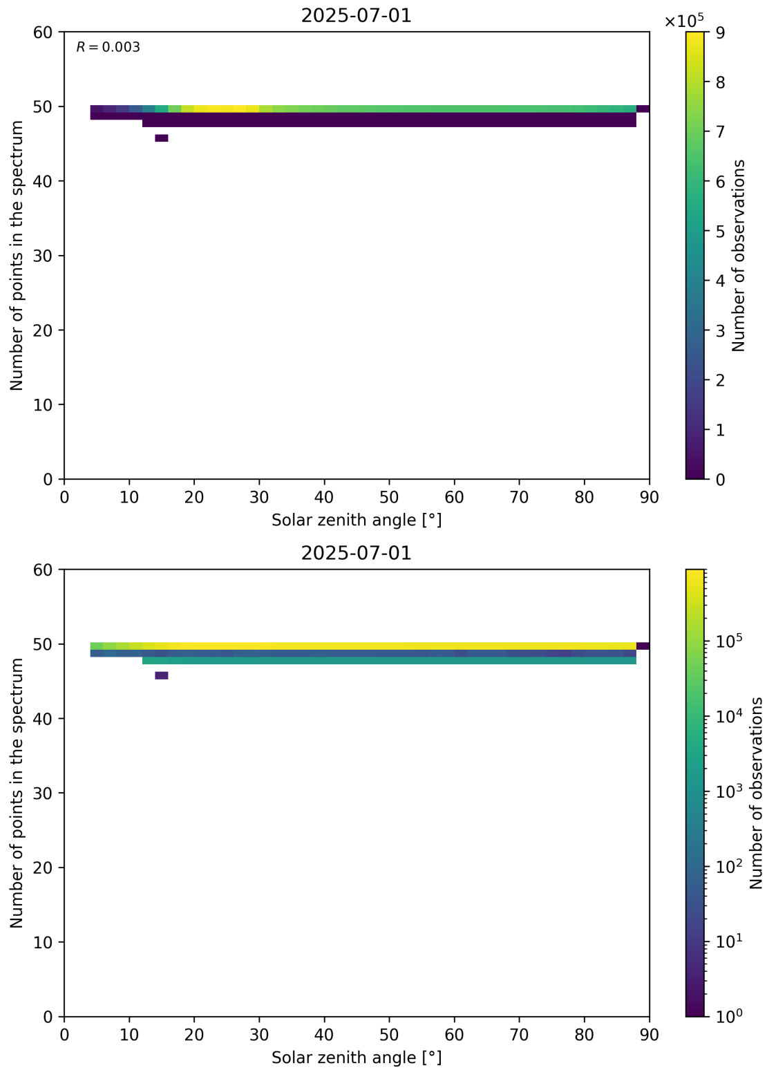
Figure 115: Scatter density plot of “Solar zenith angle” against “Number of points in the spectrum” for 2025-06-30 to 2025-07-02.
