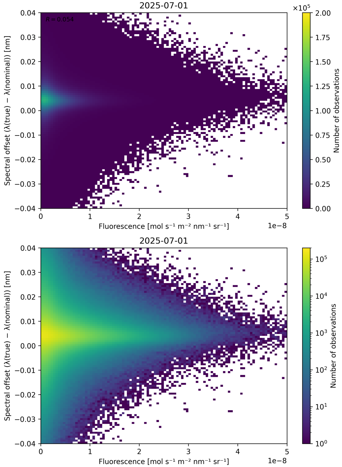
Figure 87: Scatter density plot of “Fluorescence” against “Spectral offset ( \lambda_{\text{true}} - \lambda_{\text{nominal}} )” for 2025-06-30 to 2025-07-02.
