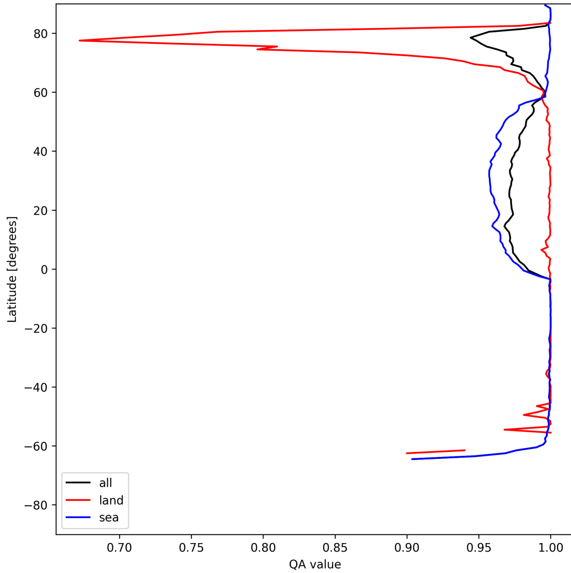
Figure 12: Zonal average of “QA value” for 2025-06-30 to 2025-07-02.
