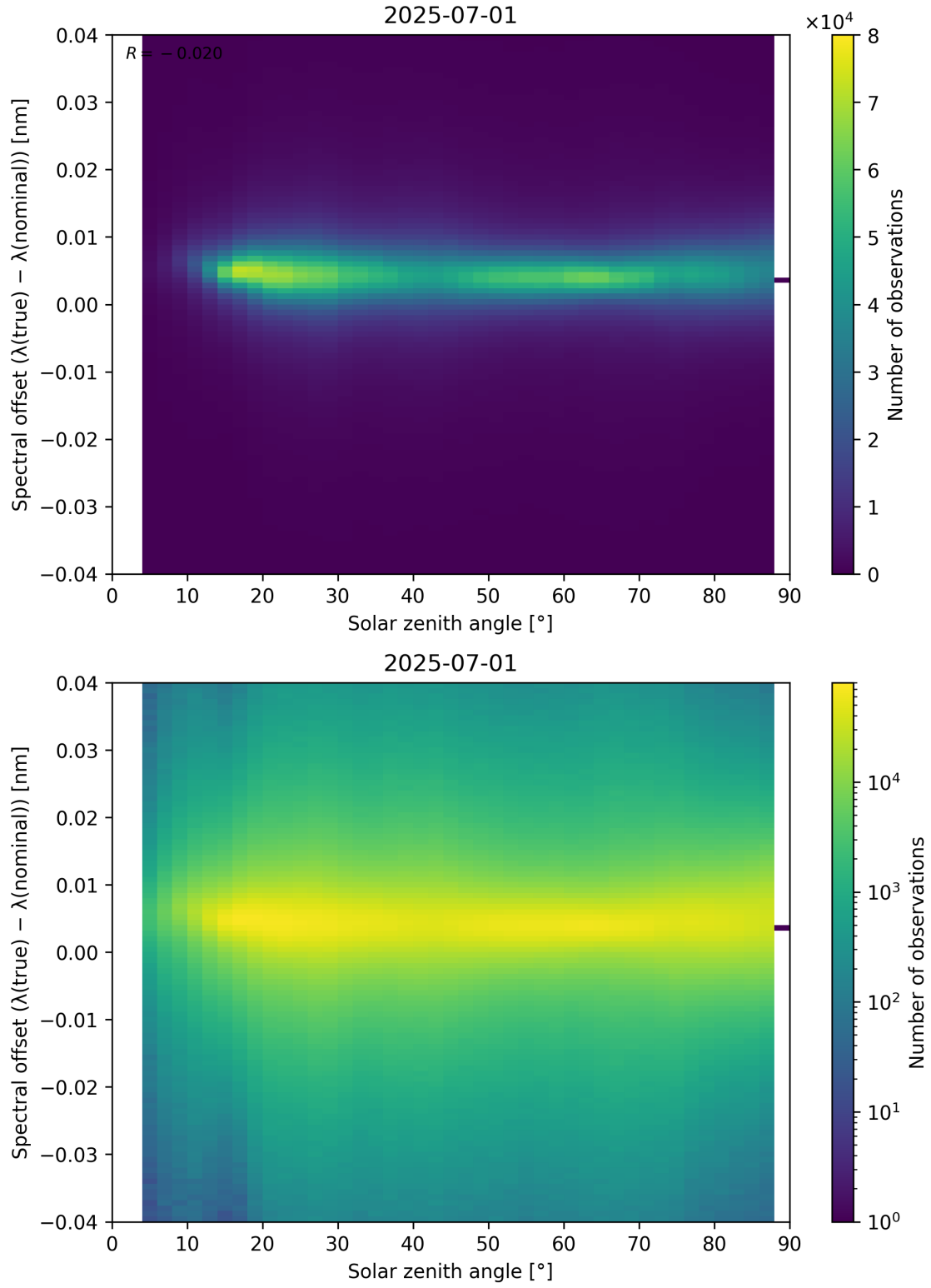
Figure 117: Scatter density plot of “Solar zenith angle” against “Spectral offset ( \lambda_{\text{true}} - \lambda_{\text{nominal}} )” for 2025-06-30 to 2025-07-02.
