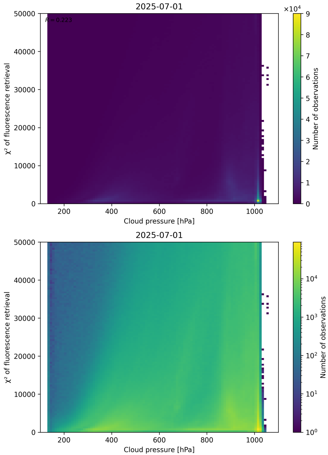
Figure 78: Scatter density plot of “Cloud pressure” against “ \chi^2 of fluorescence retrieval” for 2025-06-30 to 2025-07-02.
