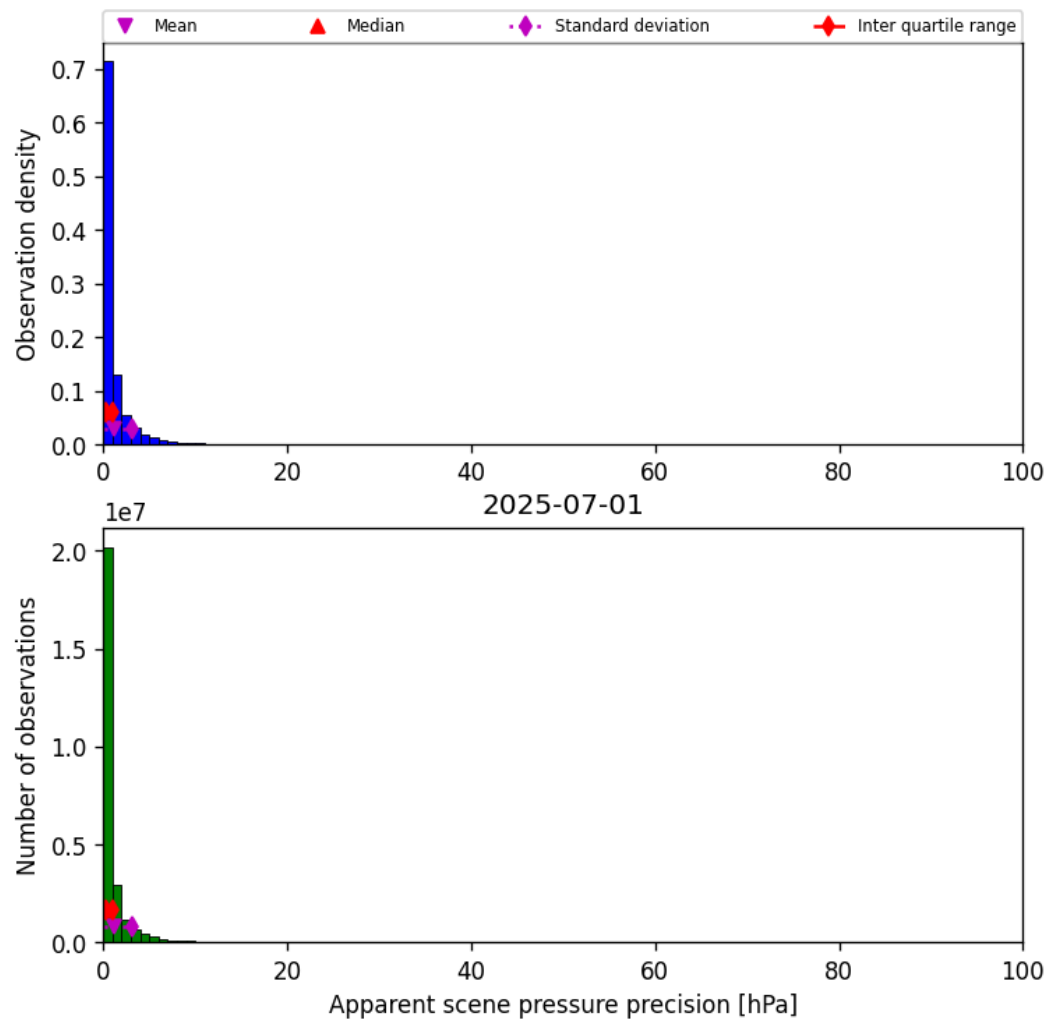
Figure 37: Histogram of “Apparent scene pressure precision” for 2025-06-30 to 2025-07-02
