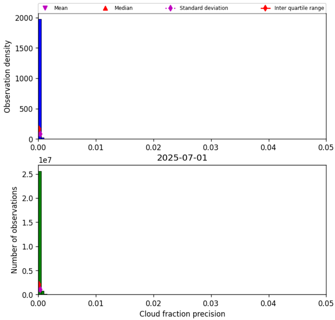
Figure 33: Histogram of “Cloud fraction precision” for 2025-06-30 to 2025-07-02
