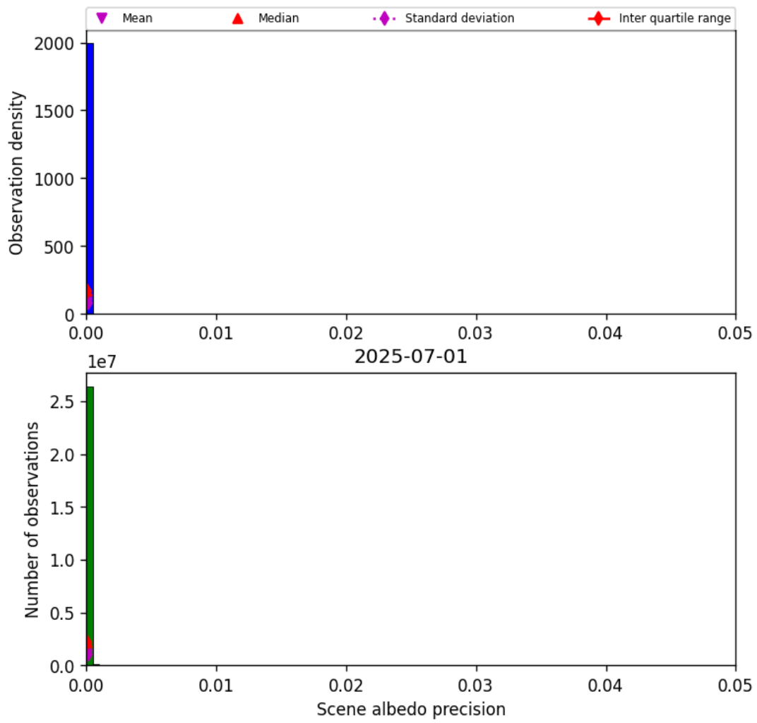
Figure 35: Histogram of “Scene albedo precision” for 2025-06-30 to 2025-07-02
