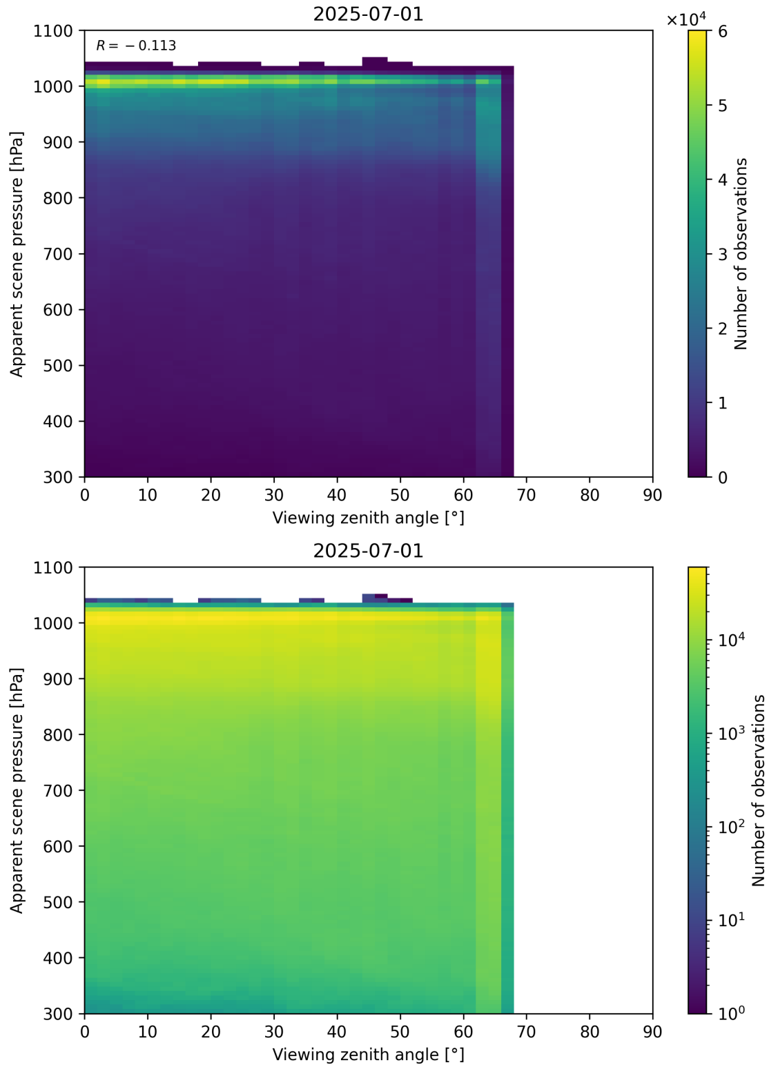
Figure 118: Scatter density plot of “Viewing zenith angle” against “Apparent scene pressure” for 2025-06-30 to 2025-07-02.
