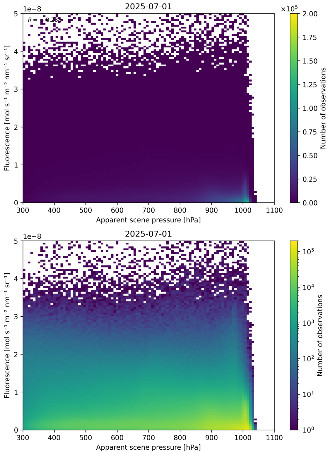
Figure 64: Scatter density plot of “Apparent scene pressure” against “Fluorescence” for 2025-06-30 to 2025-07-02.
