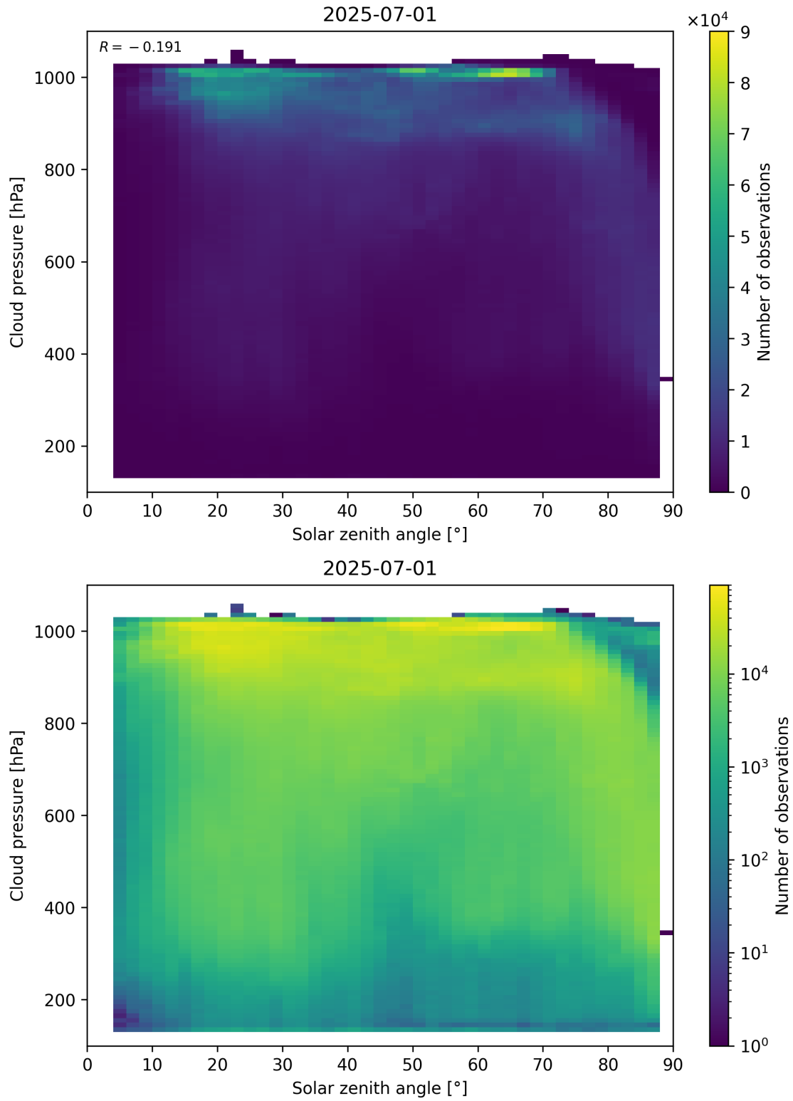
Figure 111: Scatter density plot of “Solar zenith angle” against “Cloud pressure” for 2025-06-30 to 2025-07-02.
