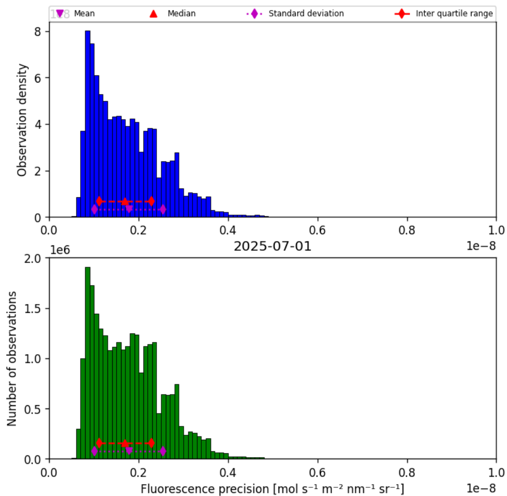
Figure 41: Histogram of “Fluorescence precision” for 2025-06-30 to 2025-07-02
