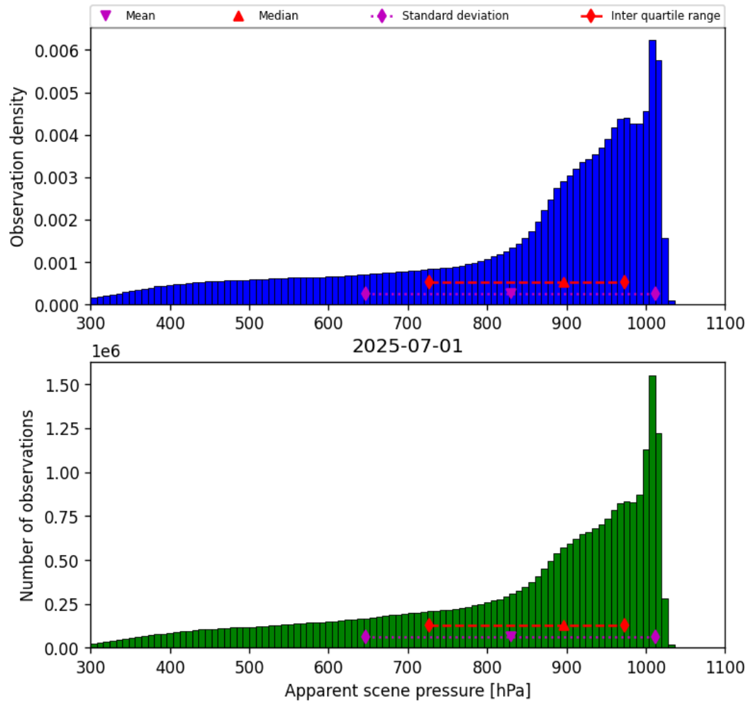
Figure 36: Histogram of “Apparent scene pressure” for 2025-06-30 to 2025-07-02
