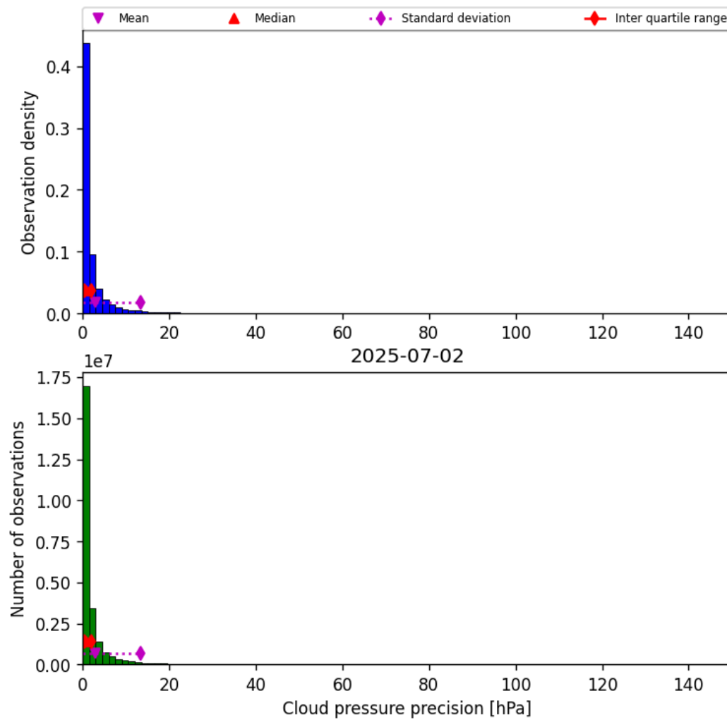
Figure 31: Histogram of “Cloud pressure precision” for 2025-07-02 to 2025-07-03
