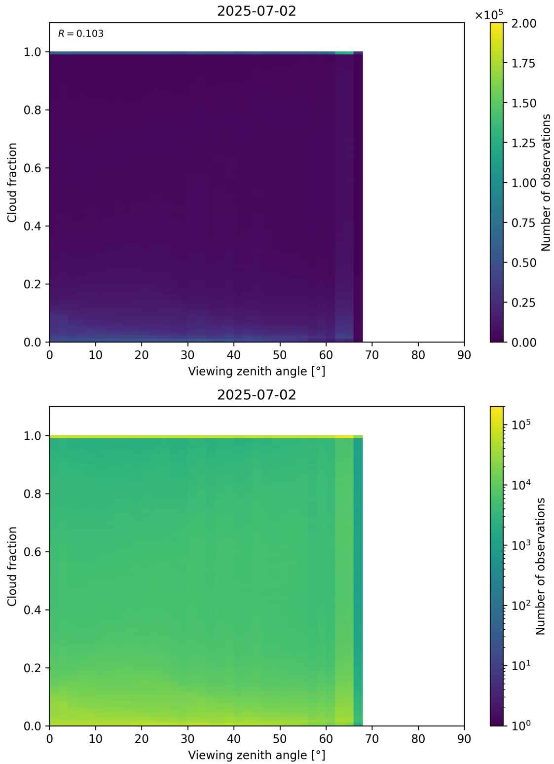
Figure 120: Scatter density plot of “Viewing zenith angle” against “Cloud fraction” for 2025-07-02 to 2025-07-03.
