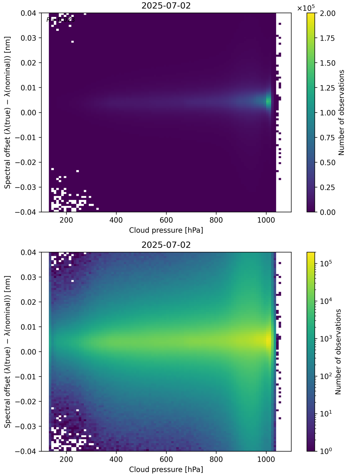
Figure 84: Scatter density plot of “Cloud pressure” against “Spectral offset ( \lambda_{\text{true}} - \lambda_{\text{nominal}} )” for 2025-07-02 to 2025-07-03.
