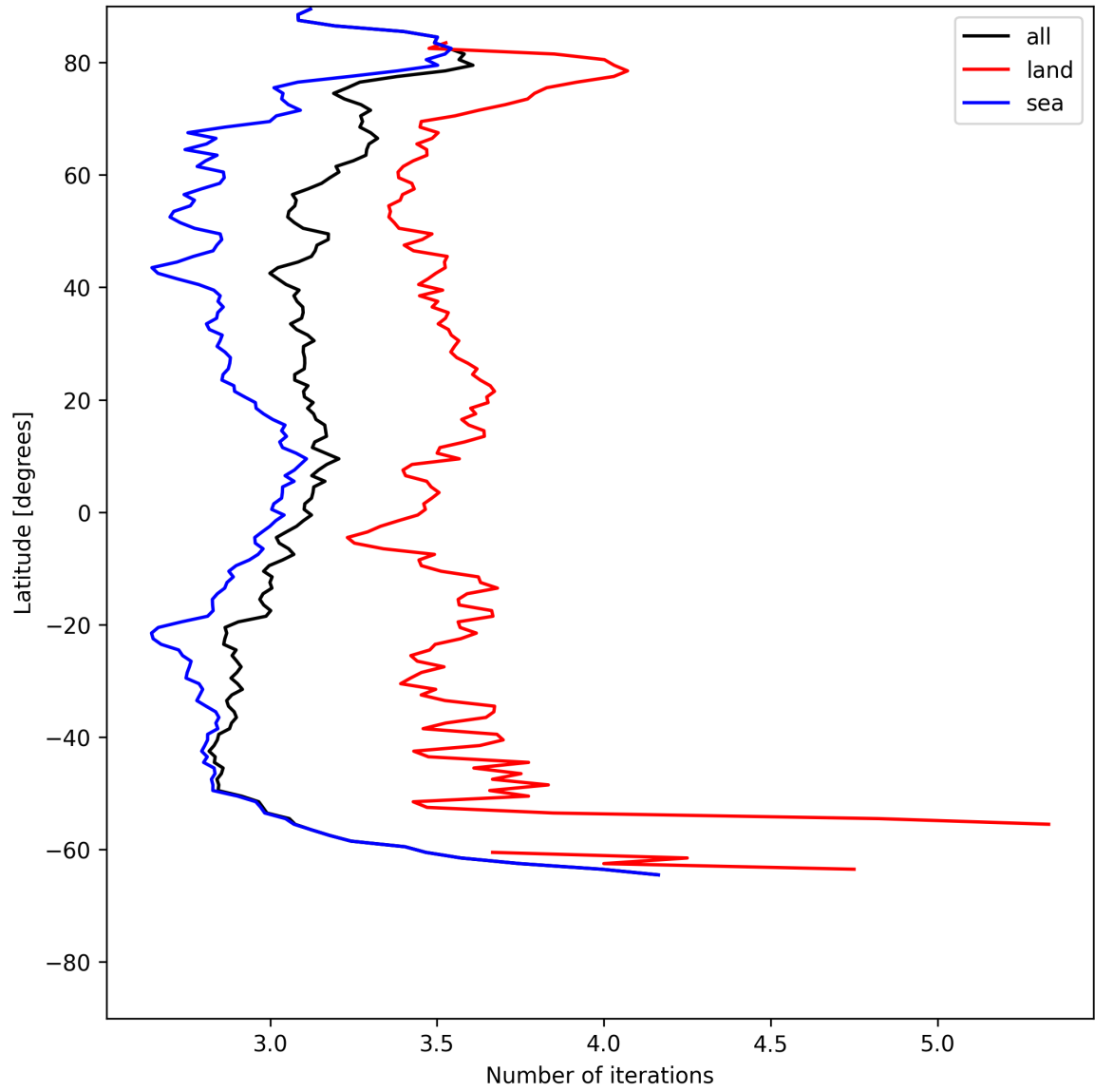
Figure 22: Zonal average of “Number of iterations” for 2025-07-02 to 2025-07-03.
