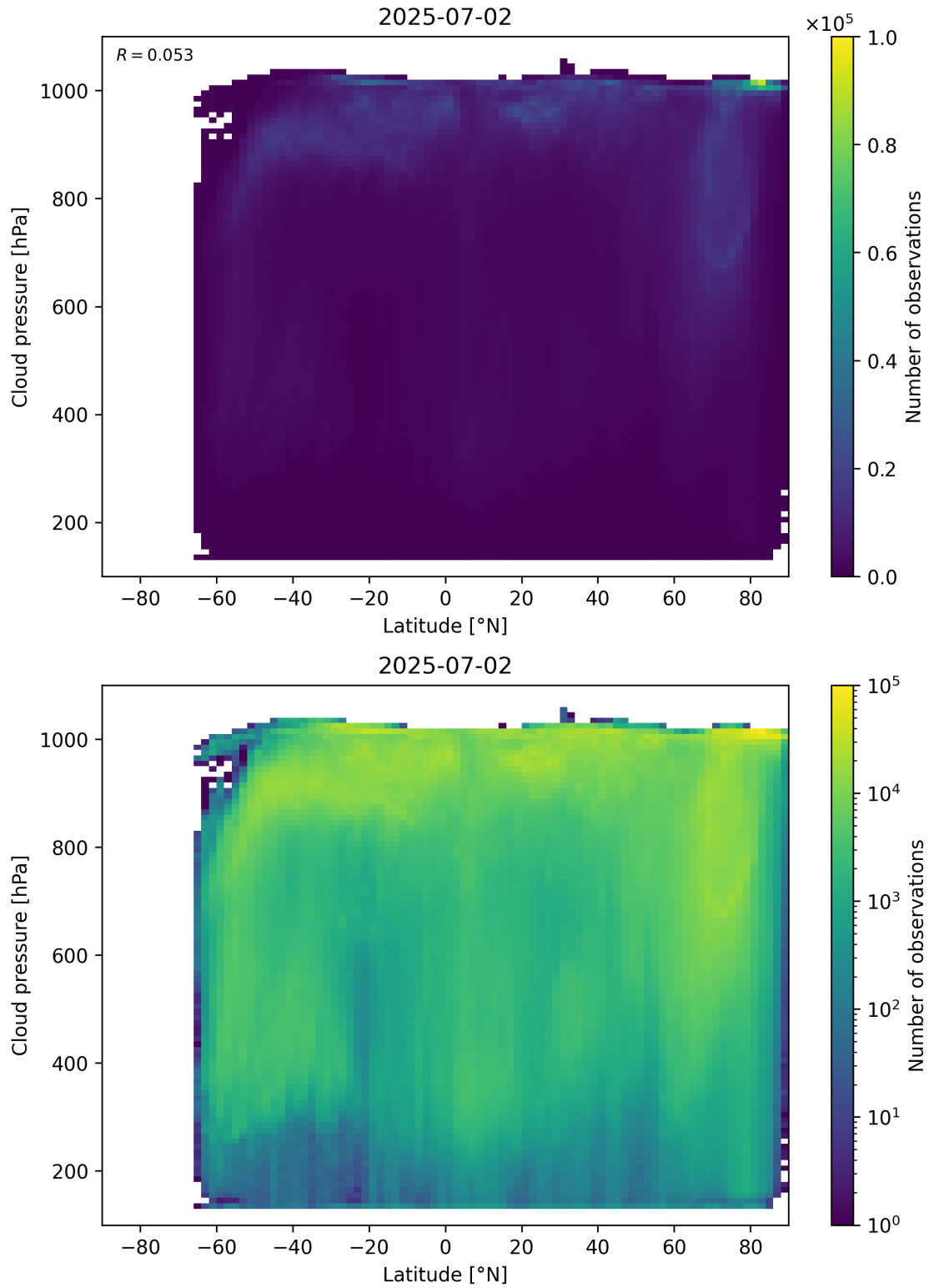
Figure 91: Scatter density plot of “Latitude” against “Cloud pressure” for 2025-07-02 to 2025-07-03.
