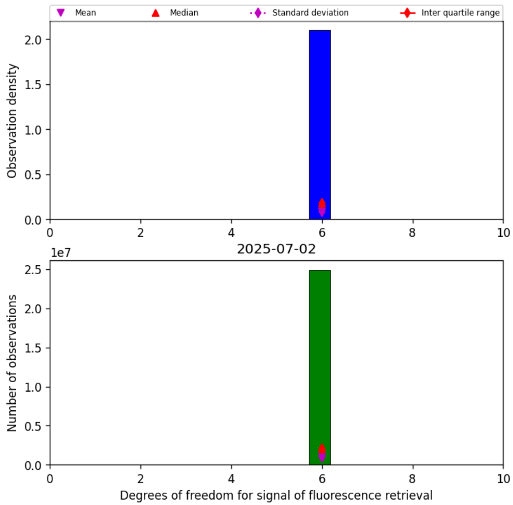
Figure 43: Histogram of “Degrees of freedom for signal of fluorescence retrieval” for 2025-07-02 to 2025-07-03
