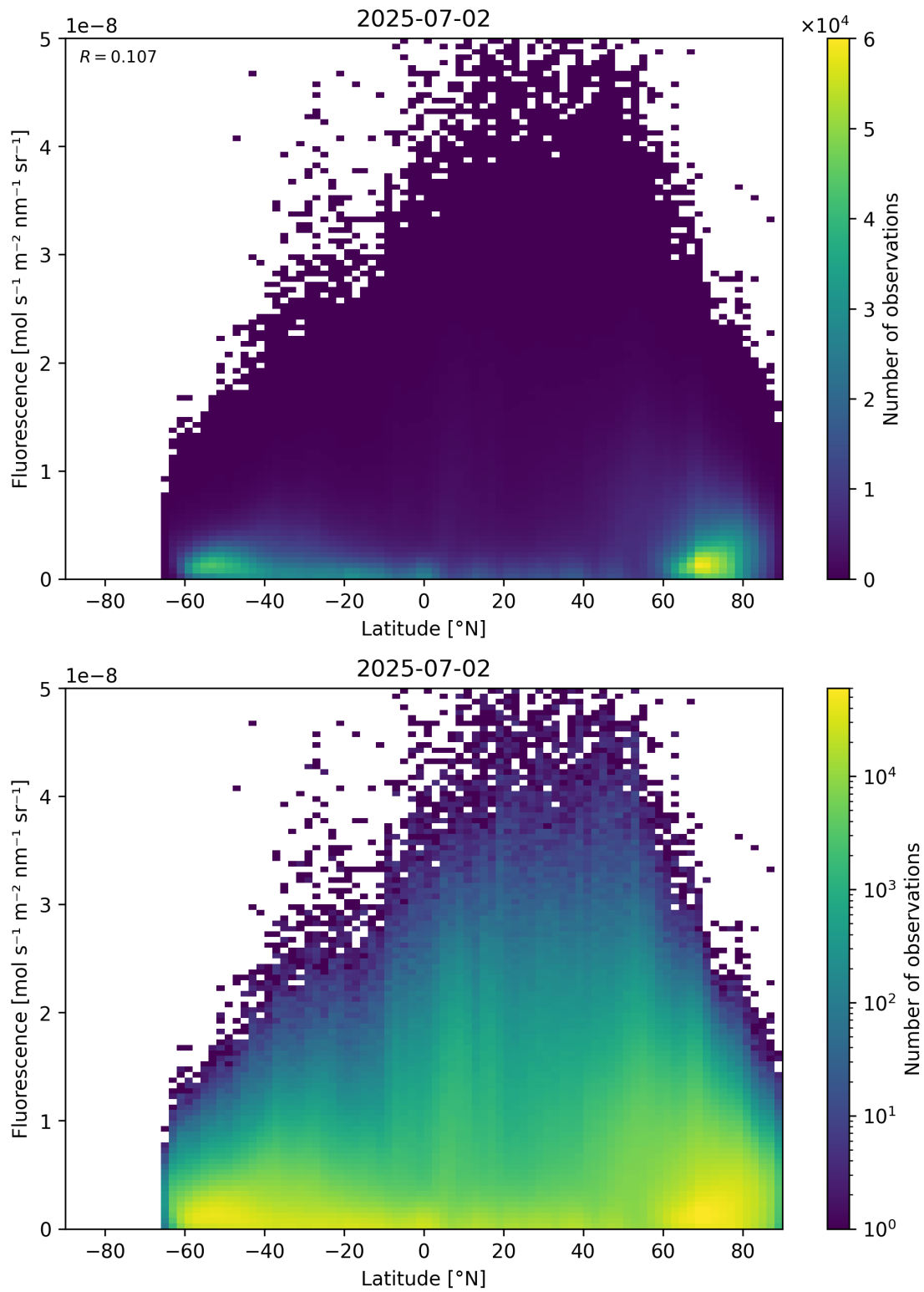
Figure 92: Scatter density plot of “Latitude” against “Fluorescence” for 2025-07-02 to 2025-07-03.
