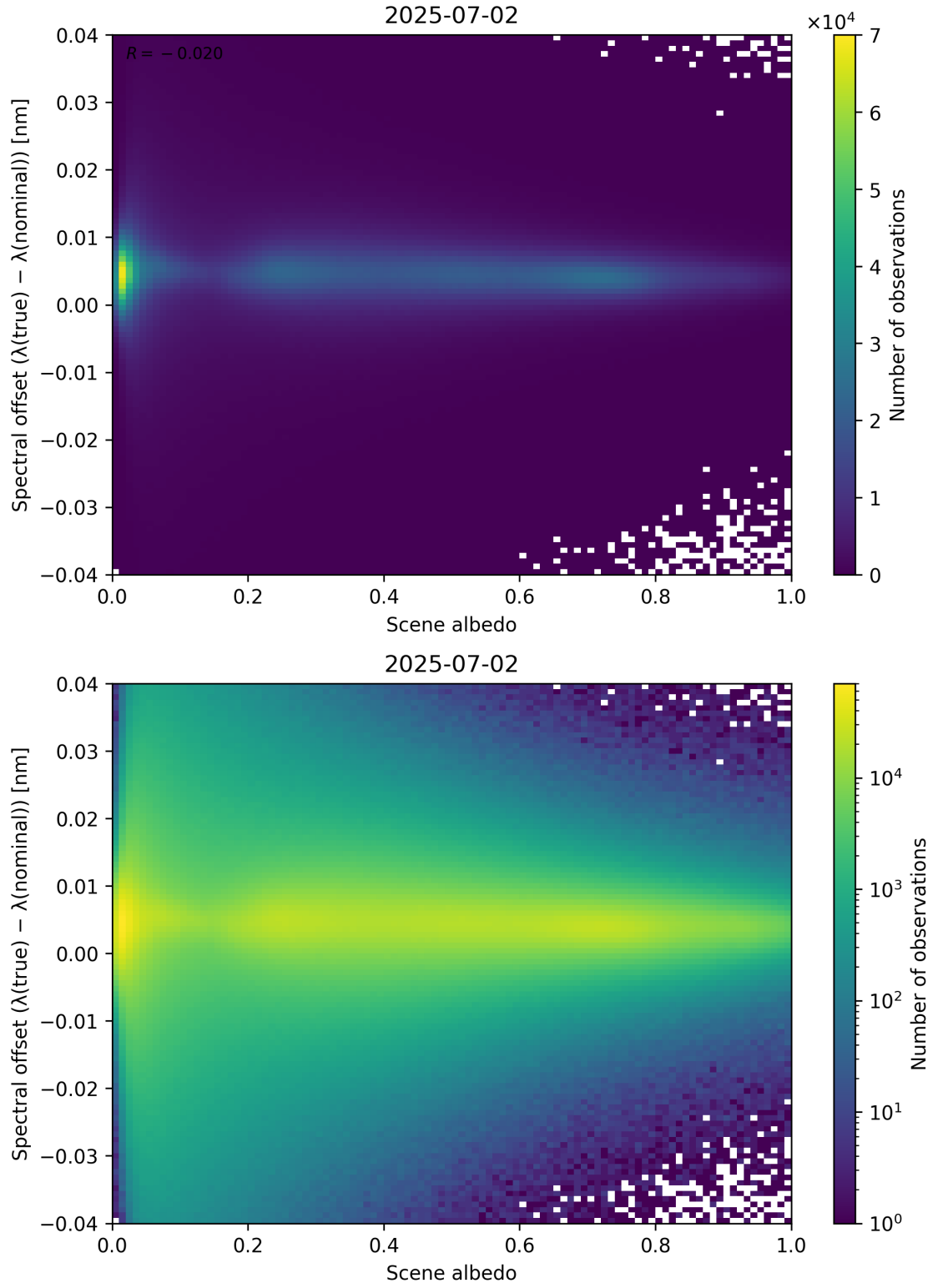
Figure 107: Scatter density plot of “Scene albedo” against “Spectral offset ( \lambda_{\text{true}} - \lambda_{\text{nominal}} )” for 2025-07-02 to 2025-07-03.
