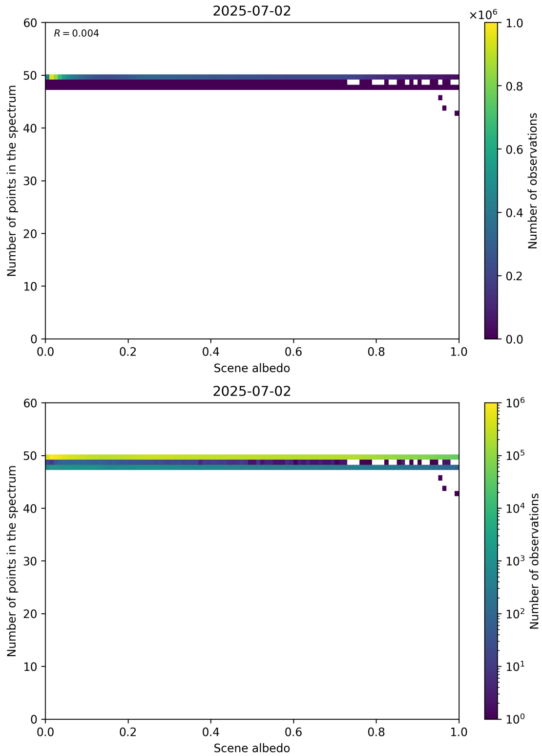
Figure 106: Scatter density plot of “Scene albedo” against “Number of points in the spectrum” for 2025-07-02 to 2025-07-03.
