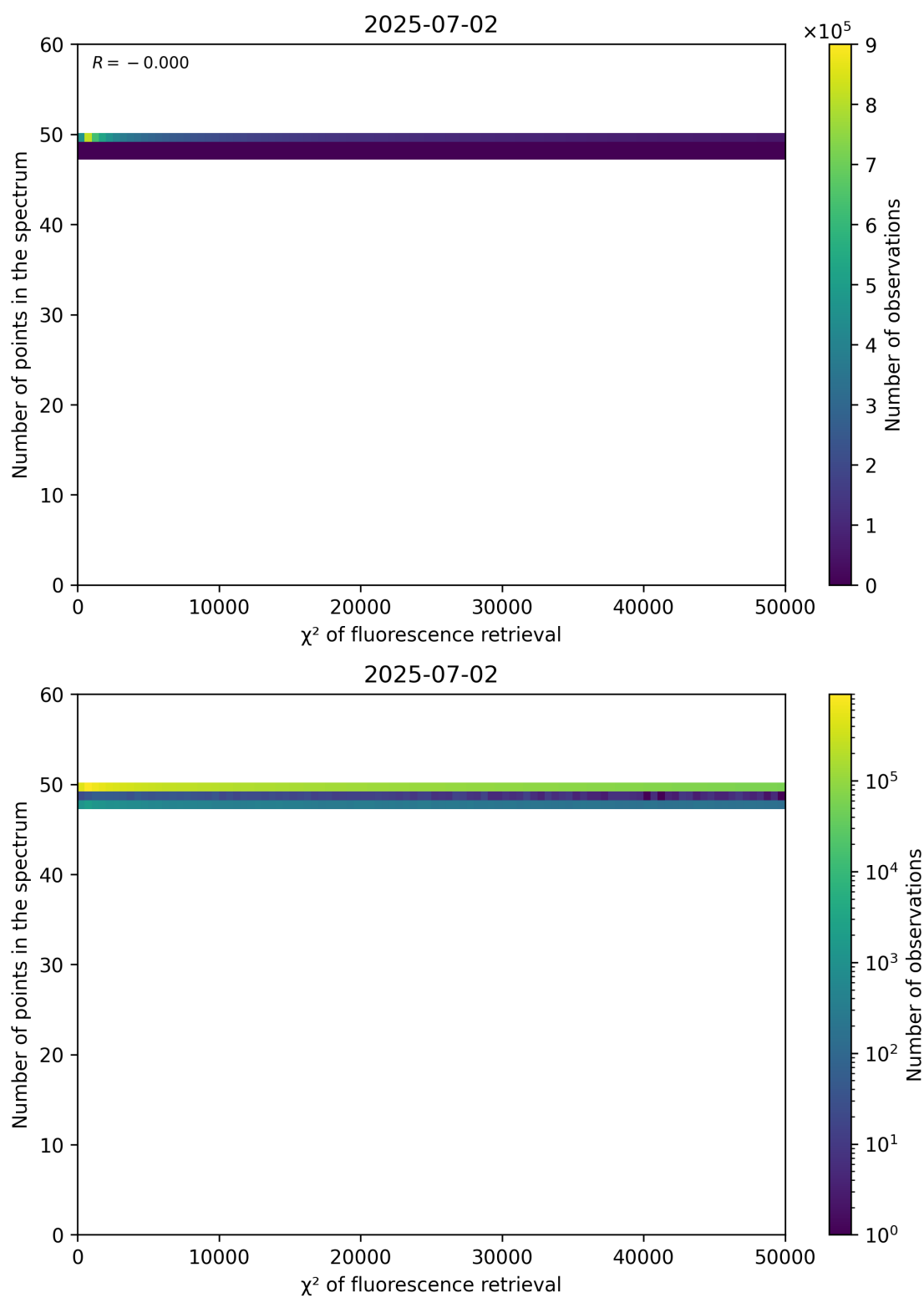
Figure 68: Scatter density plot of “ \chi^2 of fluorescence retrieval” against “Number of points in the spectrum” for 2025-07-02 to 2025-07-03.
