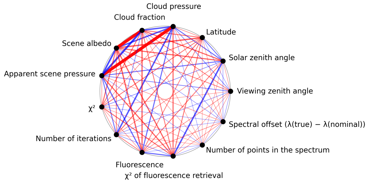
Figure 1: Map of correlation graph for 2025-07-02 to 2025-07-03.
