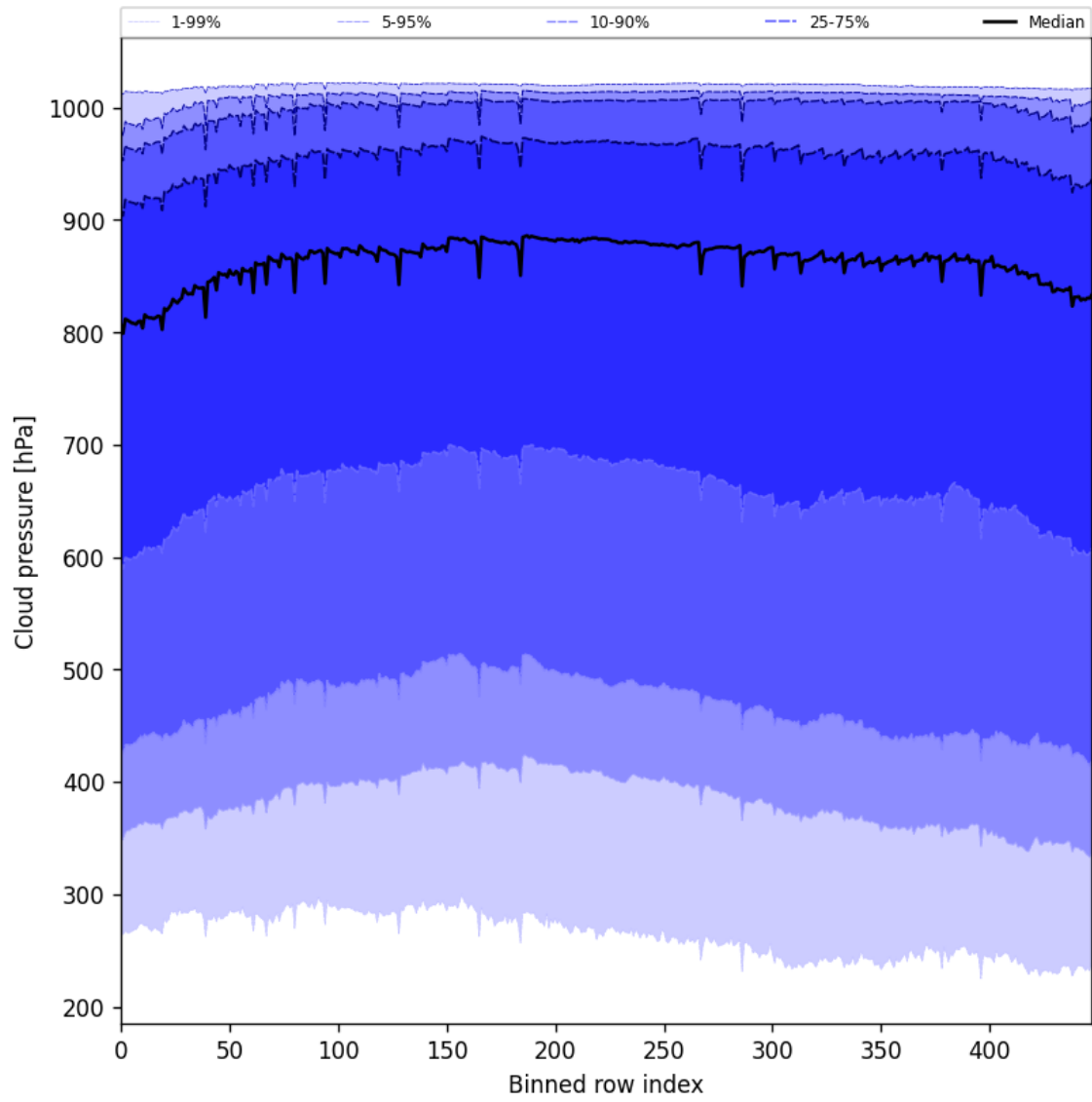
Figure 47: Along track statistics of “Cloud pressure” for 2025-07-02 to 2025-07-03
