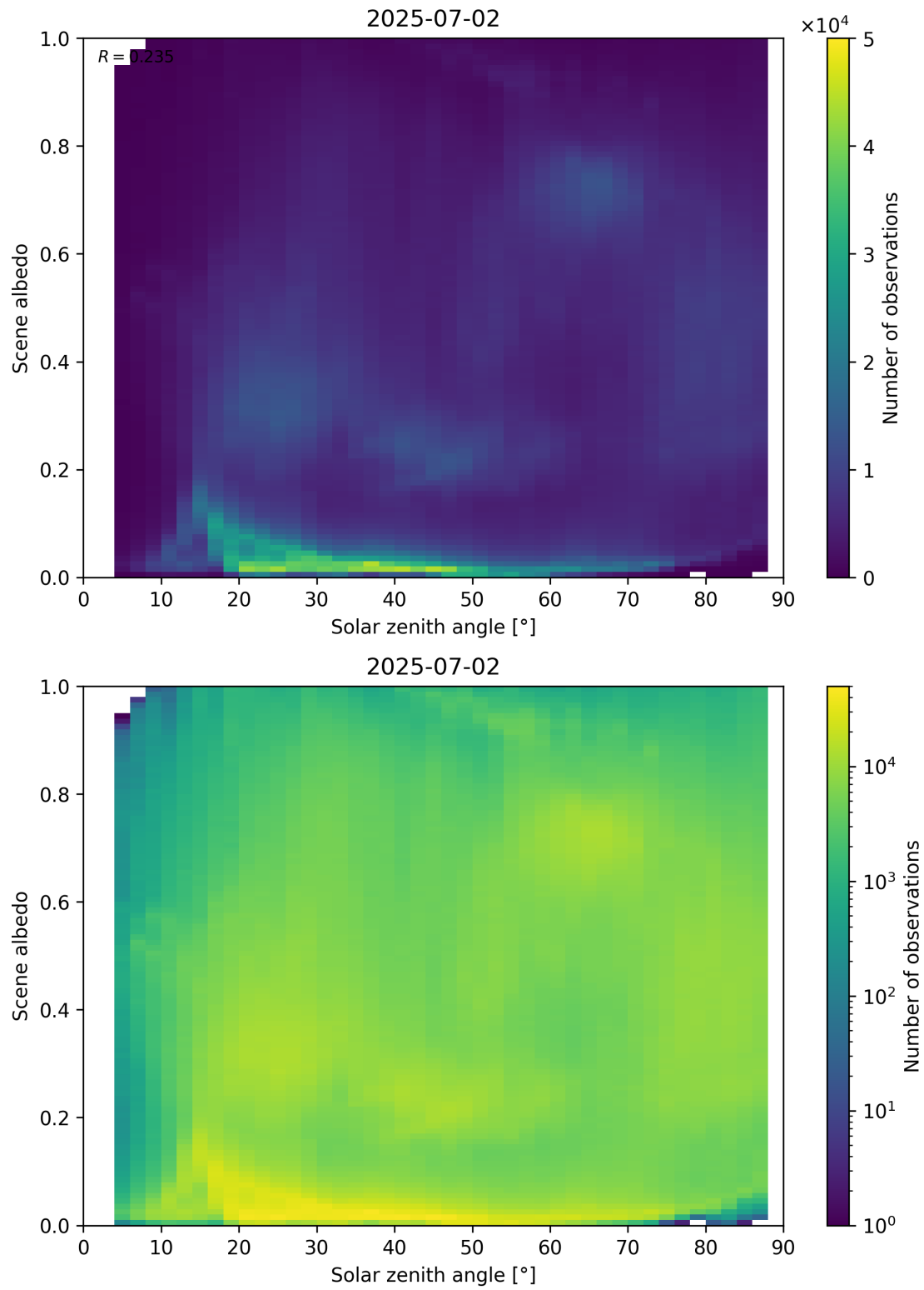
Figure 116: Scatter density plot of “Solar zenith angle” against “Scene albedo” for 2025-07-02 to 2025-07-03.
