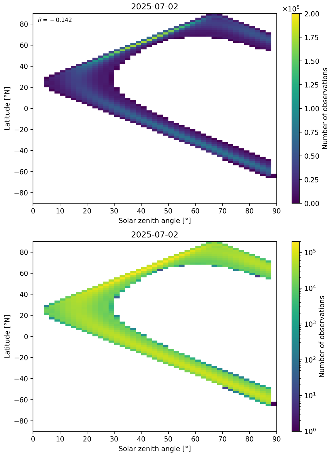
Figure 113: Scatter density plot of “Solar zenith angle” against “Latitude” for 2025-07-02 to 2025-07-03.
