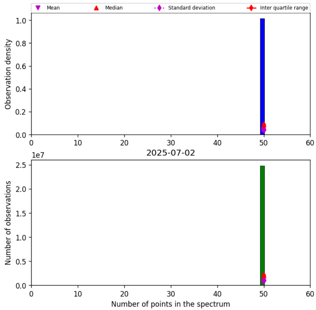
Figure 44: Histogram of “Number of points in the spectrum” for 2025-07-02 to 2025-07-03
