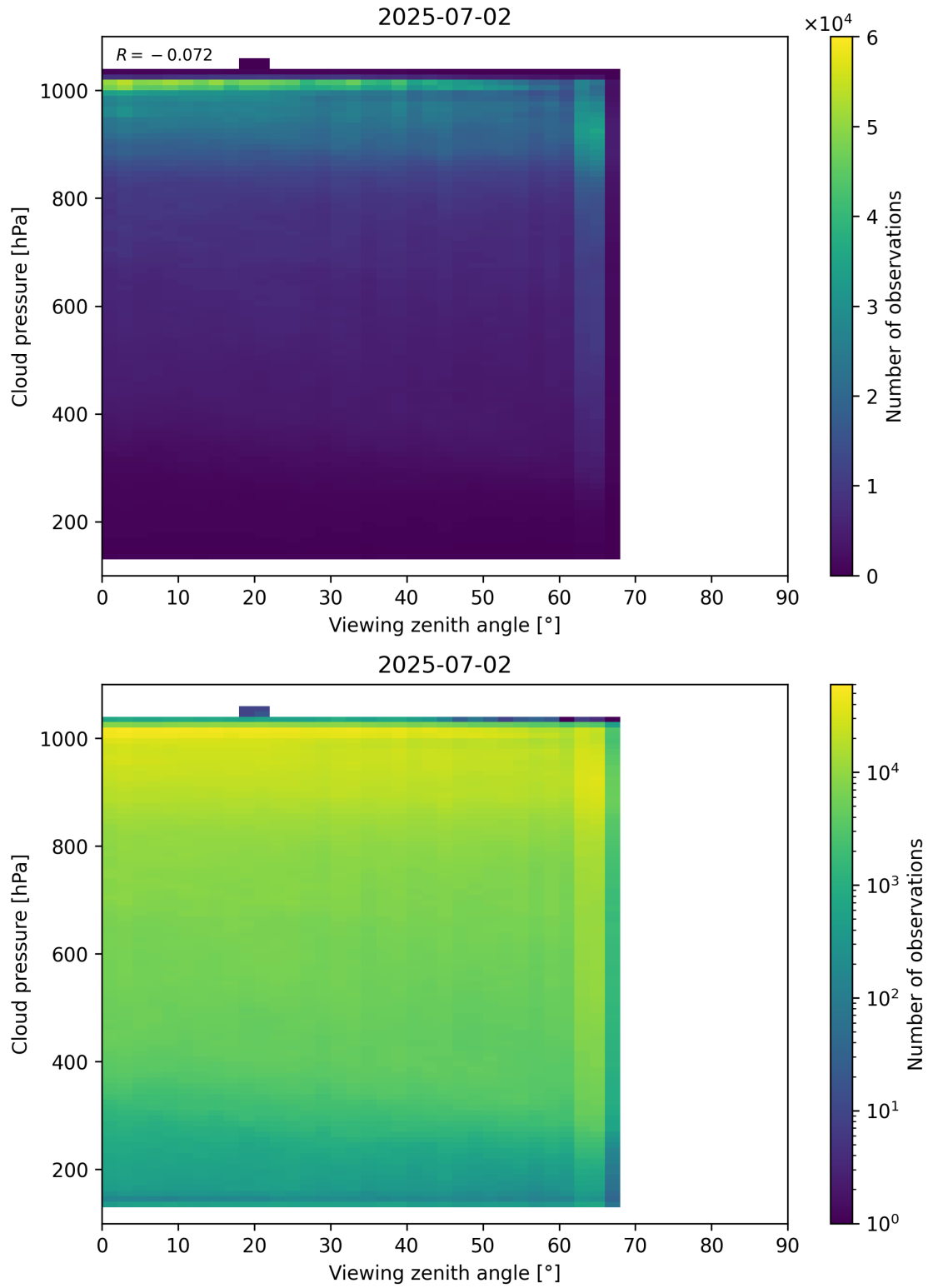
Figure 121: Scatter density plot of “Viewing zenith angle” against “Cloud pressure” for 2025-07-02 to 2025-07-03.
