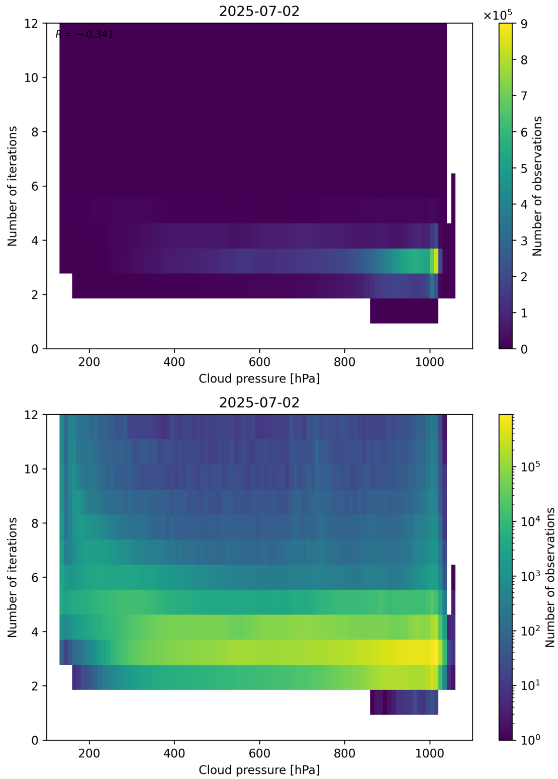
Figure 81: Scatter density plot of “Cloud pressure” against “Number of iterations” for 2025-07-02 to 2025-07-03.
