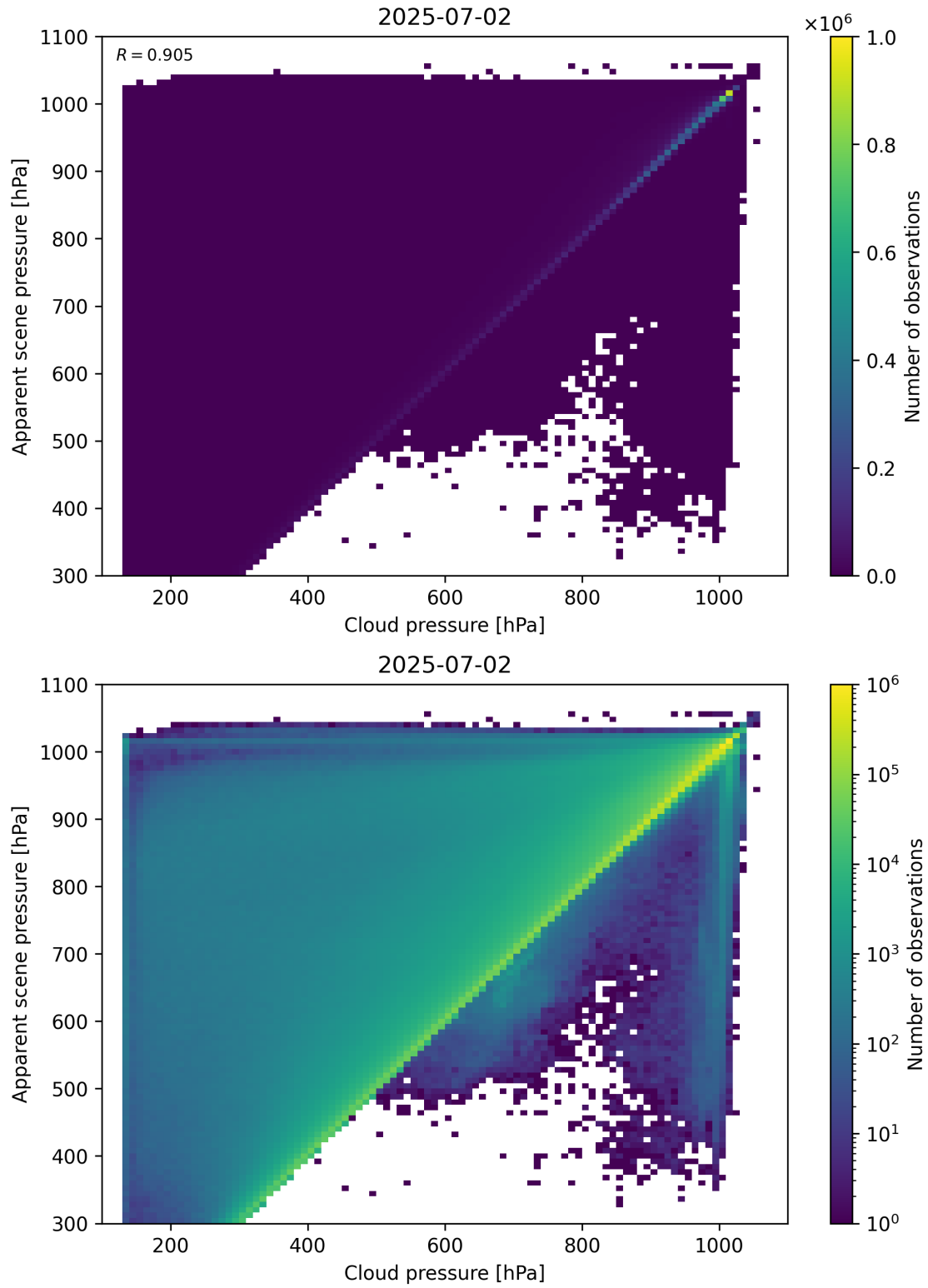
Figure 77: Scatter density plot of “Cloud pressure” against “Apparent scene pressure” for 2025-07-02 to 2025-07-03.
