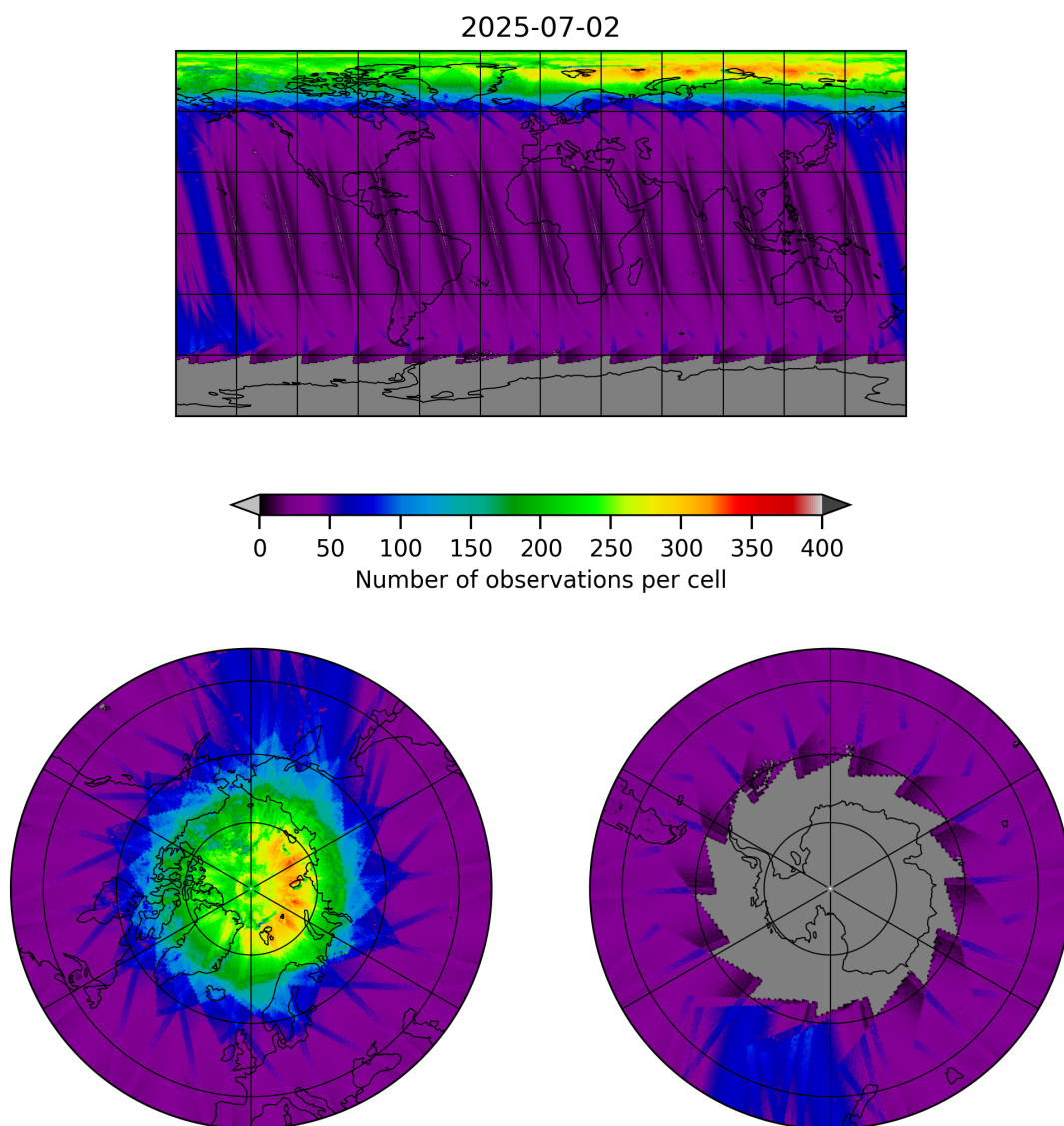
Figure 11: Map of the number of observations for 2025-07-02 to 2025-07-03
