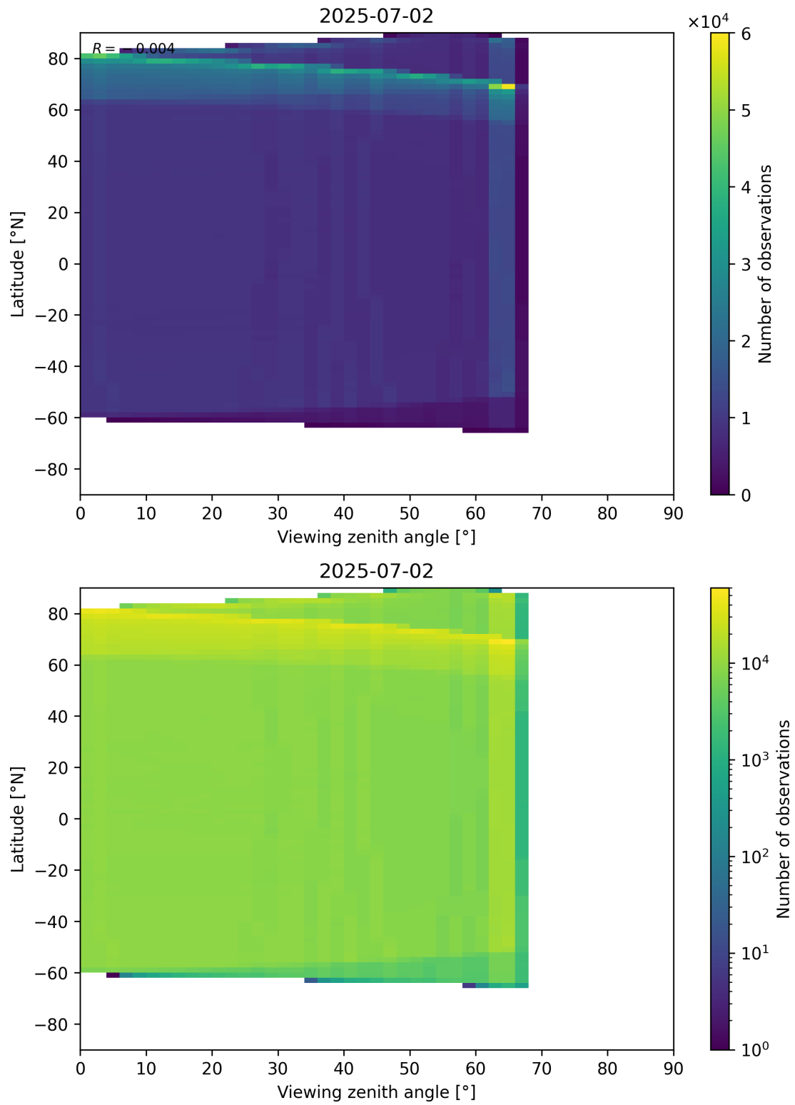
Figure 123: Scatter density plot of “Viewing zenith angle” against “Latitude” for 2025-07-02 to 2025-07-03.
