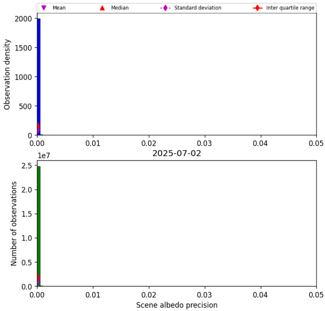
Figure 35: Histogram of “Scene albedo precision” for 2025-07-02 to 2025-07-03
