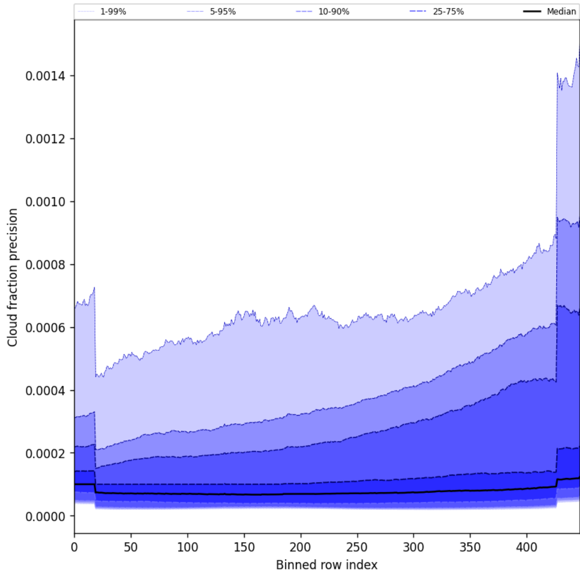
Figure 50: Along track statistics of “Cloud fraction precision” for 2025-07-02 to 2025-07-03
