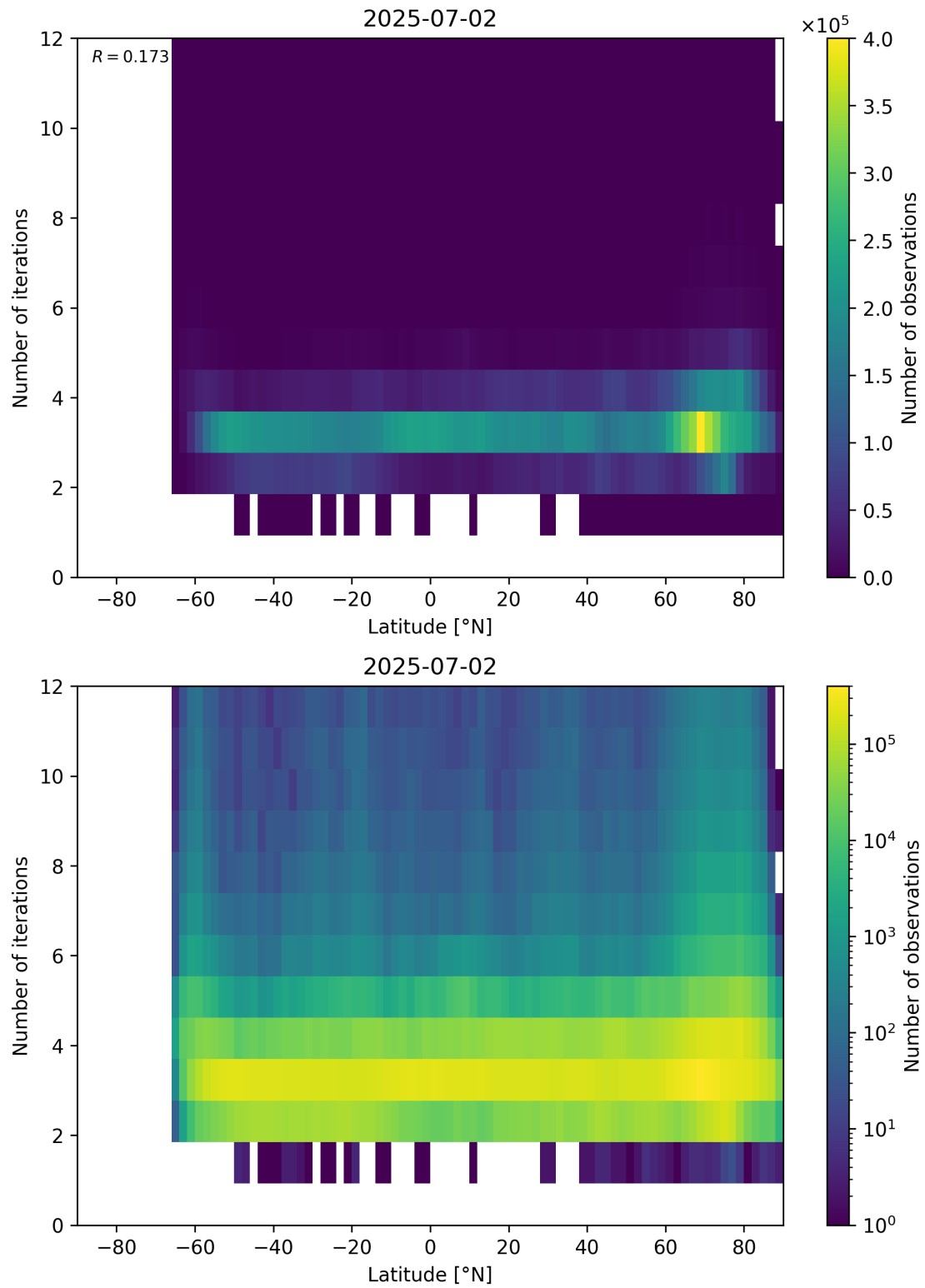
Figure 93: Scatter density plot of “Latitude” against “Number of iterations” for 2025-07-02 to 2025-07-03.
