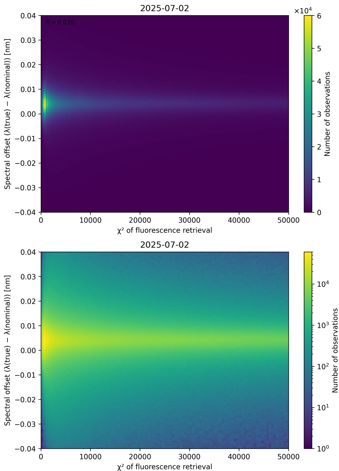
Figure 69: Scatter density plot of “ \chi^2 of fluorescence retrieval” against “Spectral offset ( \lambda_{\text{true}} - \lambda_{\text{nominal}} )” for 2025-07-02 to 2025-07-03.
