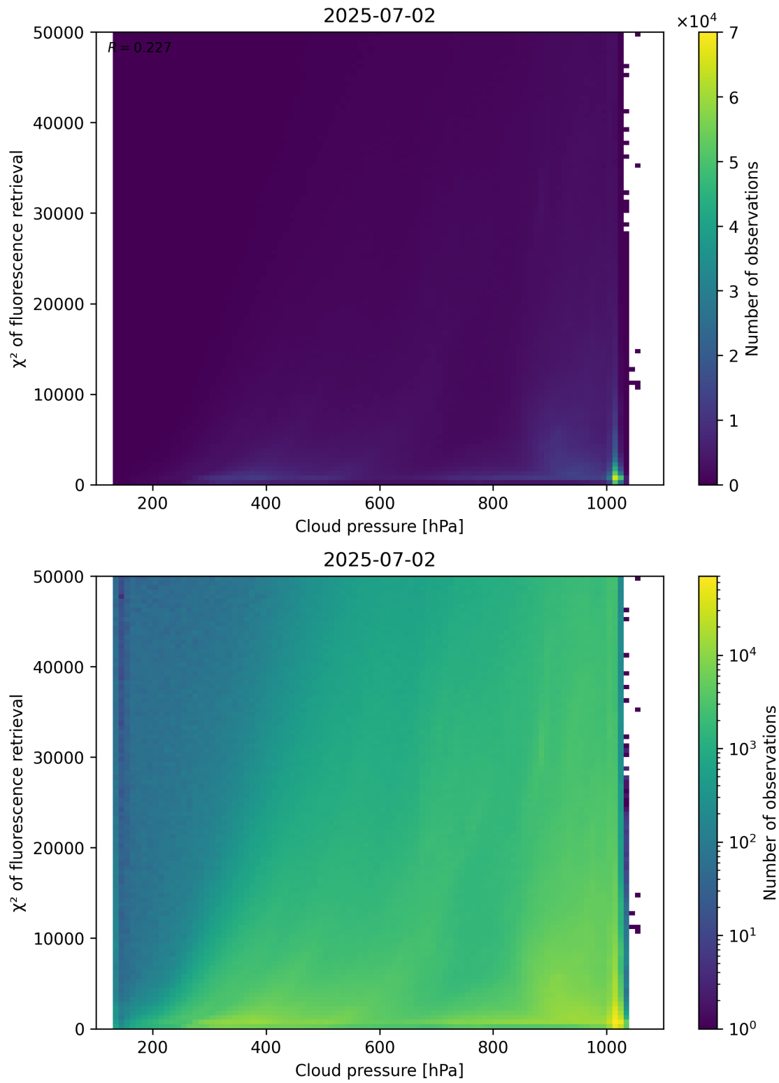
Figure 78: Scatter density plot of “Cloud pressure” against “ \chi^2 of fluorescence retrieval” for 2025-07-02 to 2025-07-03.
