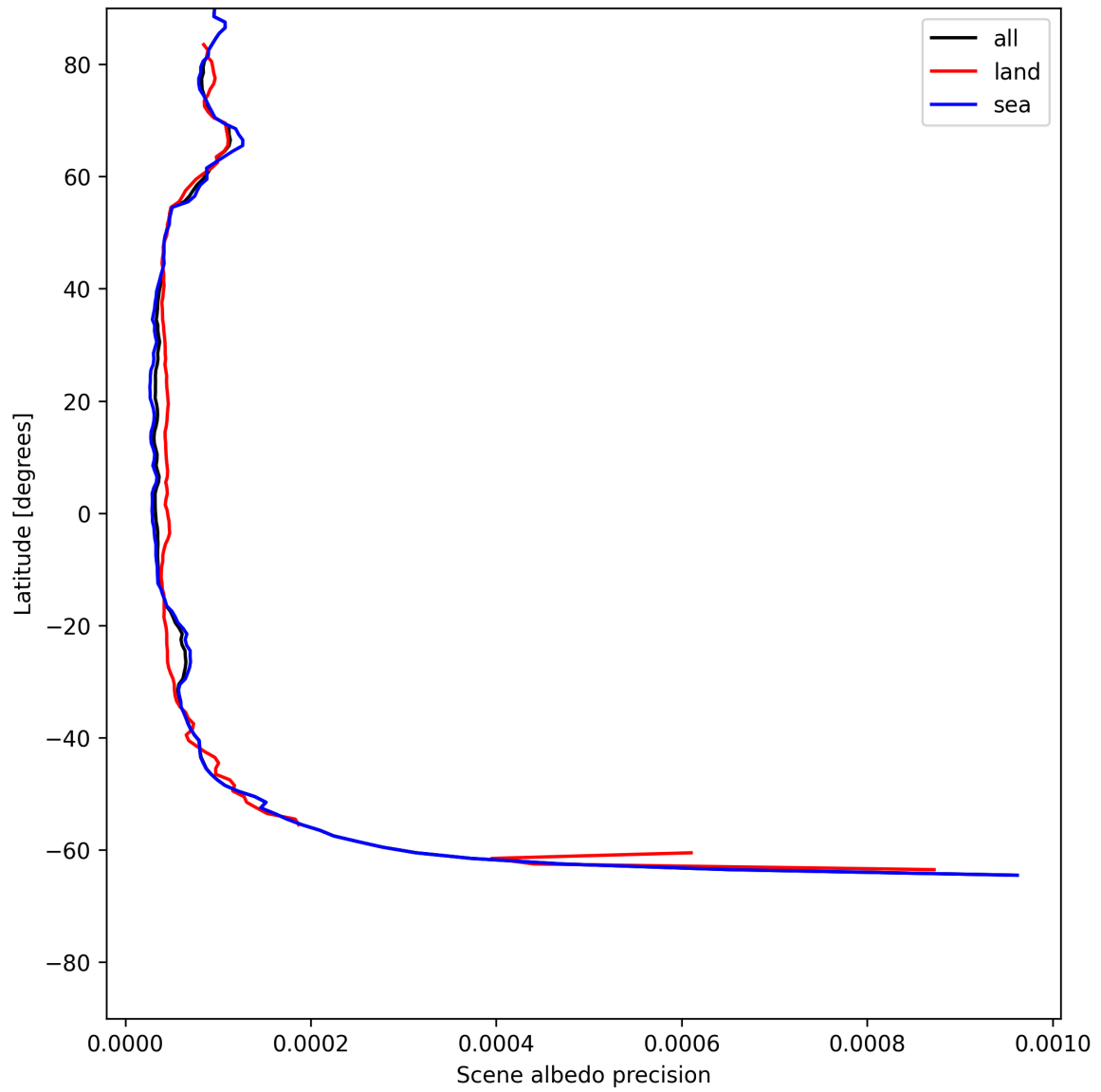
Figure 18: Zonal average of “Scene albedo precision” for 2025-07-02 to 2025-07-03.
