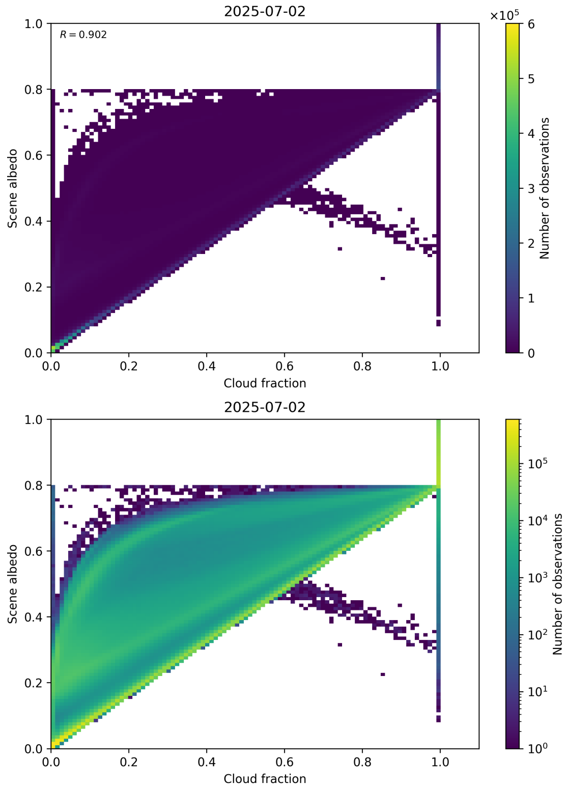
Figure 75: Scatter density plot of “Cloud fraction” against “Scene albedo” for 2025-07-02 to 2025-07-03.
