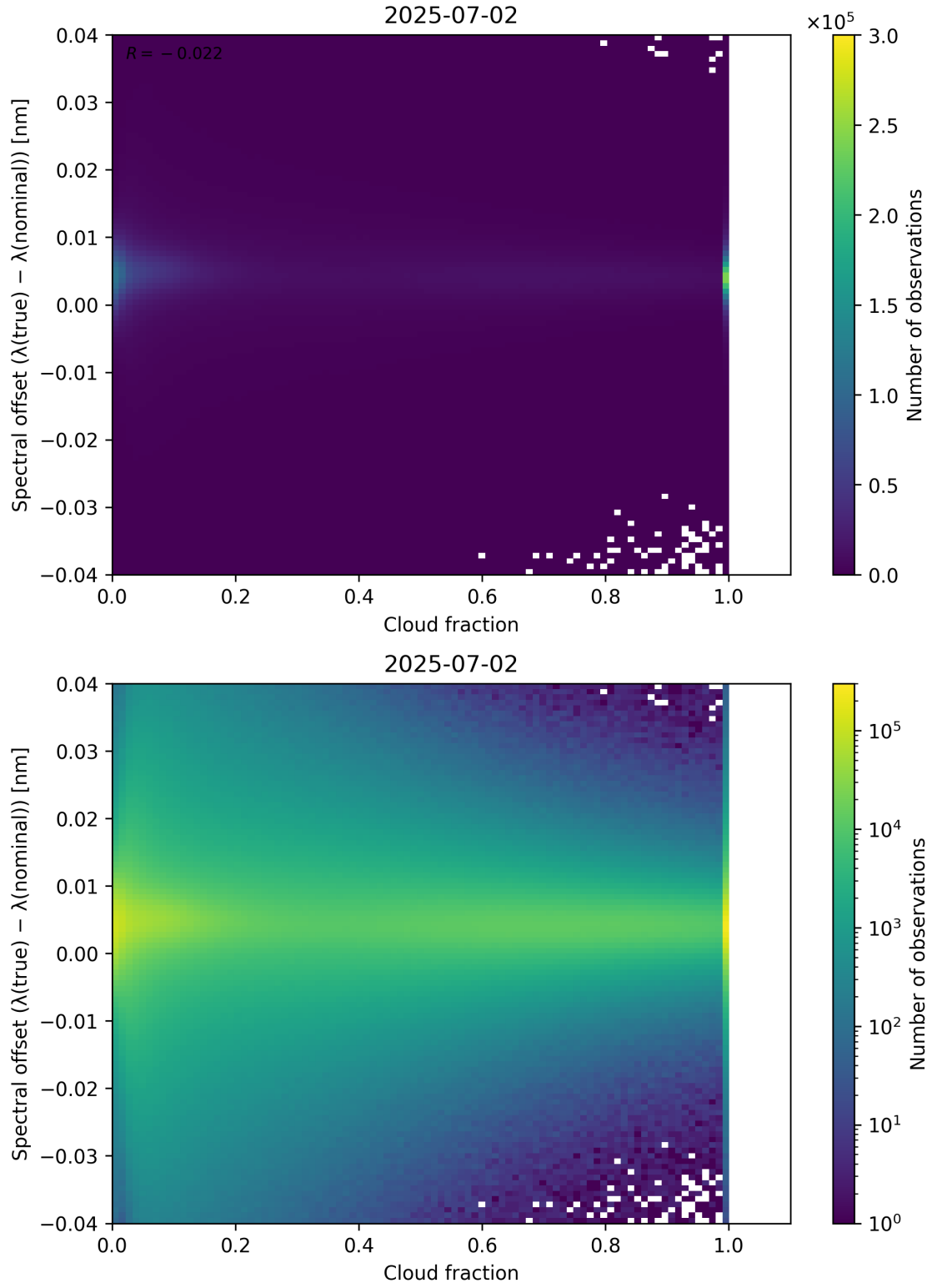
Figure 76: Scatter density plot of “Cloud fraction” against “Spectral offset ( \lambda_{\text{true}} - \lambda_{\text{nominal}} )” for 2025-07-02 to 2025-07-03.
