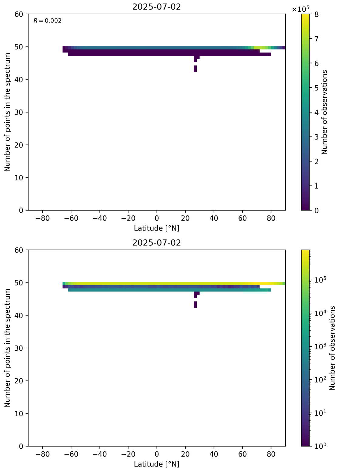
Figure 94: Scatter density plot of “Latitude” against “Number of points in the spectrum” for 2025-07-02 to 2025-07-03.
