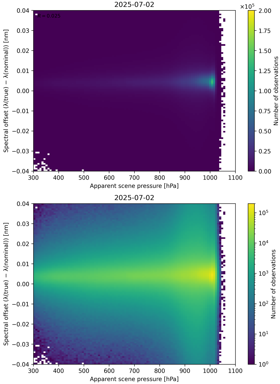
Figure 67: Scatter density plot of “Apparent scene pressure” against “Spectral offset ( \lambda_{\text{true}} - \lambda_{\text{nominal}} )” for 2025-07-02 to 2025-07-03.
