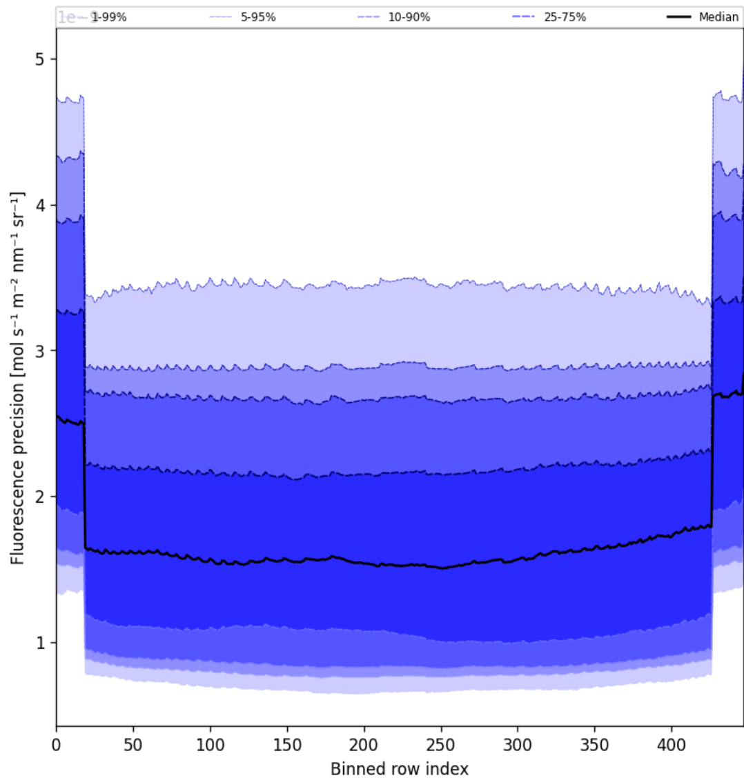
Figure 58: Along track statistics of “Fluorescence precision” for 2025-07-02 to 2025-07-03
