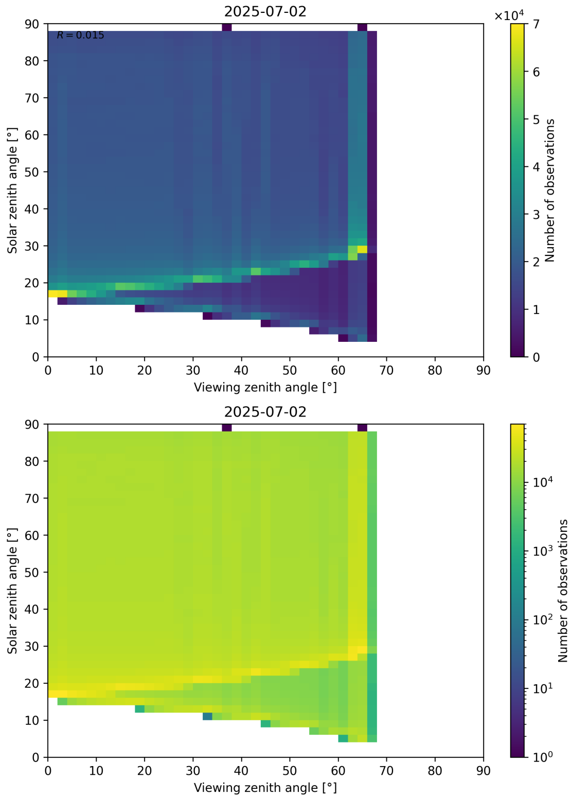
Figure 127: Scatter density plot of “Viewing zenith angle” against “Solar zenith angle” for 2025-07-02 to 2025-07-03.
