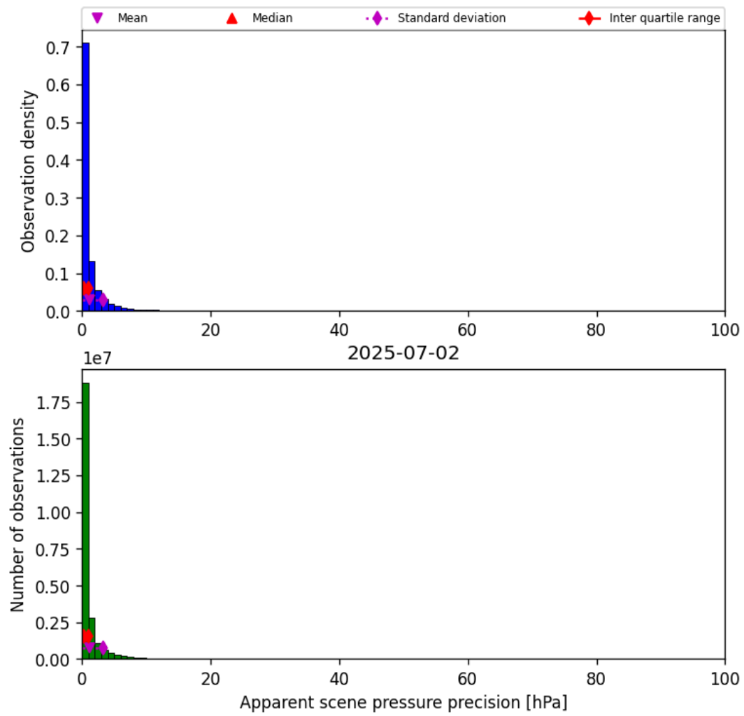
Figure 37: Histogram of "Apparent scene pressure precision" for 2025-07-02 to 2025-07-03
