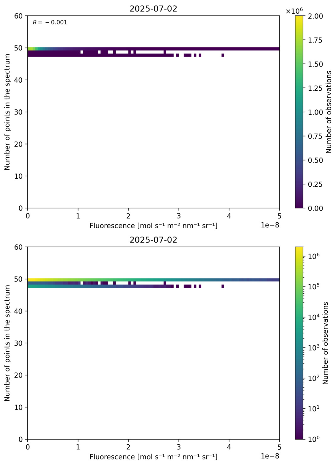
Figure 86: Scatter density plot of “Fluorescence” against “Number of points in the spectrum” for 2025-07-02 to 2025-07-03.
