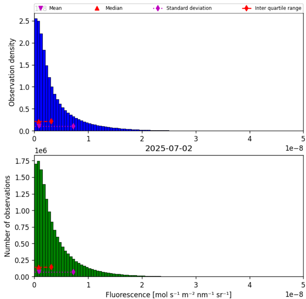
Figure 40: Histogram of “Fluorescence” for 2025-07-02 to 2025-07-03
