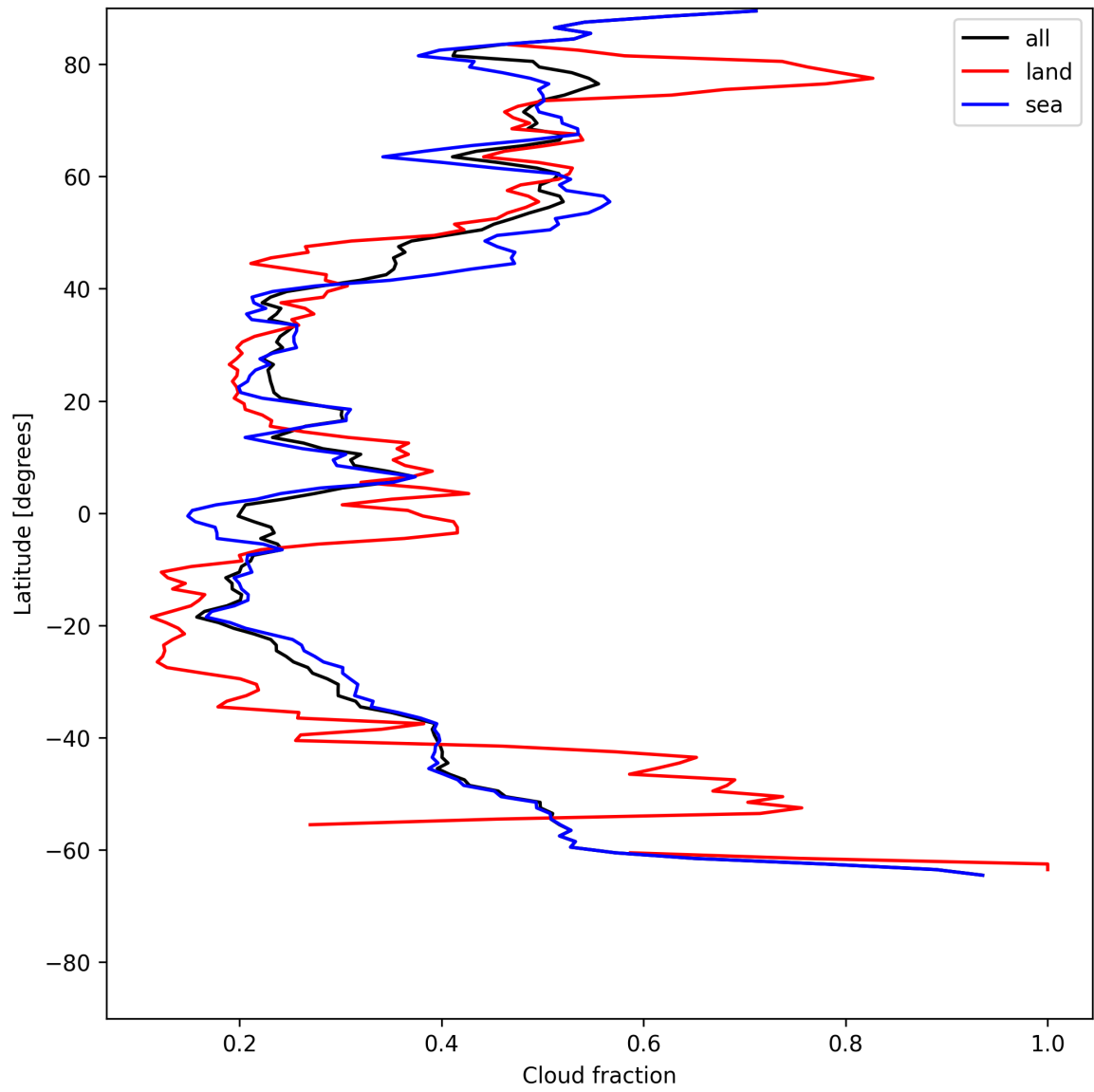
Figure 15: Zonal average of “Cloud fraction” for 2025-07-02 to 2025-07-03.
