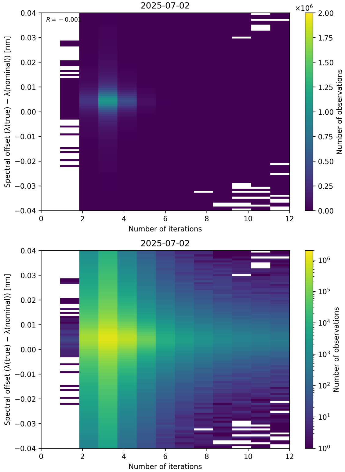
Figure 100: Scatter density plot of “Number of iterations” against “Spectral offset ( \lambda_{\text{true}} - \lambda_{\text{nominal}} )” for 2025-07-02 to 2025-07-03.
