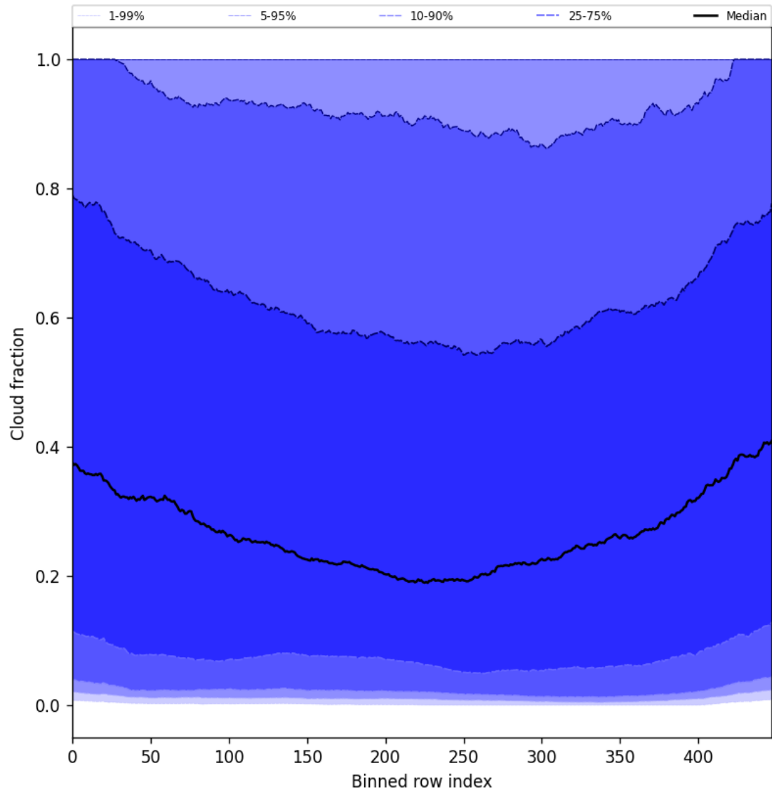
Figure 49: Along track statistics of “Cloud fraction” for 2025-07-02 to 2025-07-03
