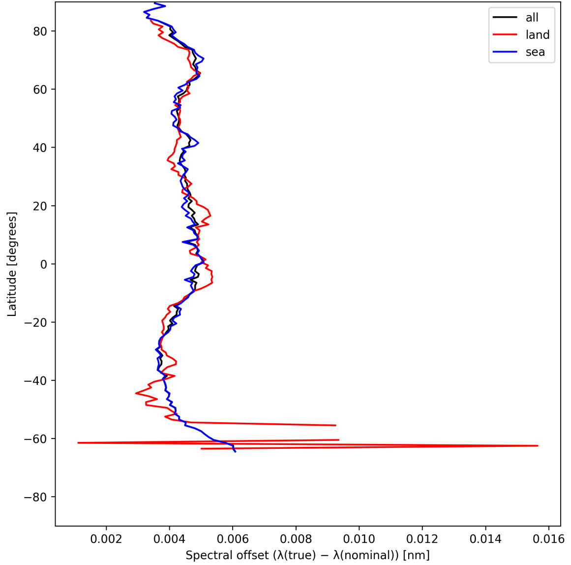
Figure 28: Zonal average of “Spectral offset ( \lambda_{\text{true}} - \lambda_{\text{nominal}} )” for 2025-07-02 to 2025-07-03.
