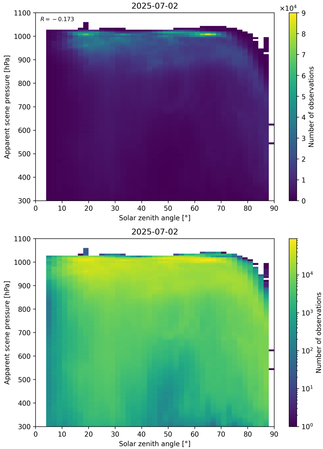
Figure 108: Scatter density plot of “Solar zenith angle” against “Apparent scene pressure” for 2025-07-02 to 2025-07-03.
