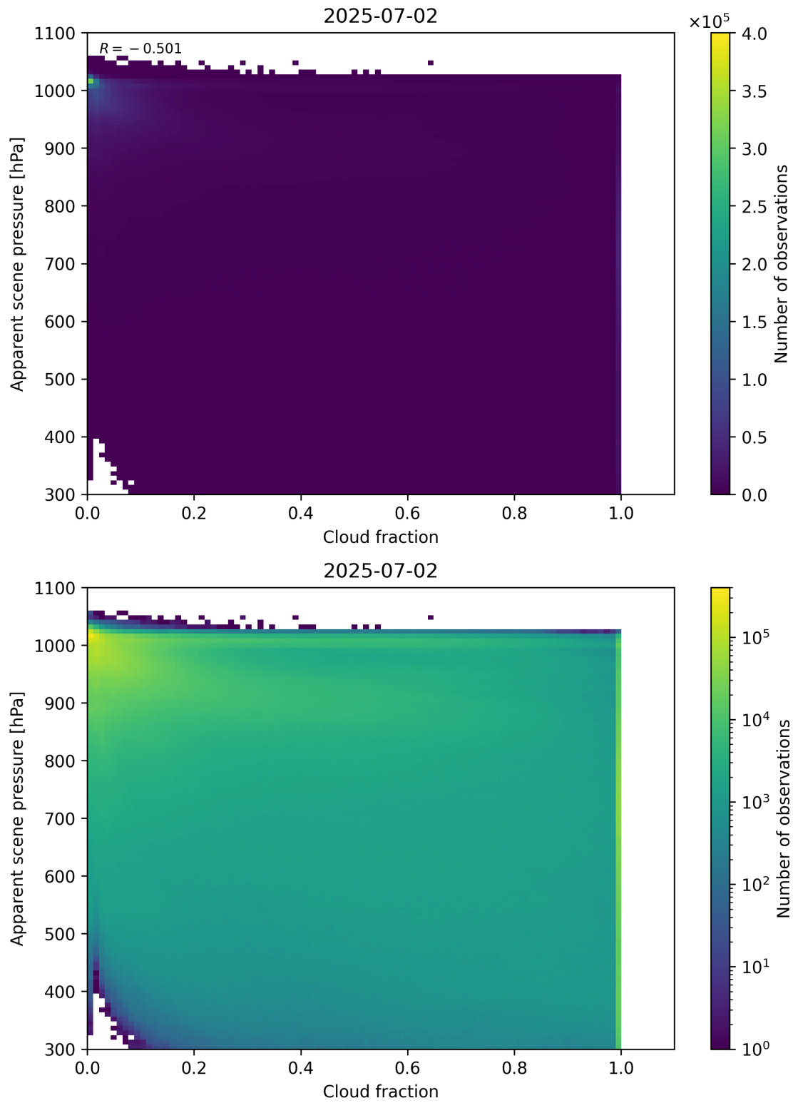
Figure 70: Scatter density plot of “Cloud fraction” against “Apparent scene pressure” for 2025-07-02 to 2025-07-03.
