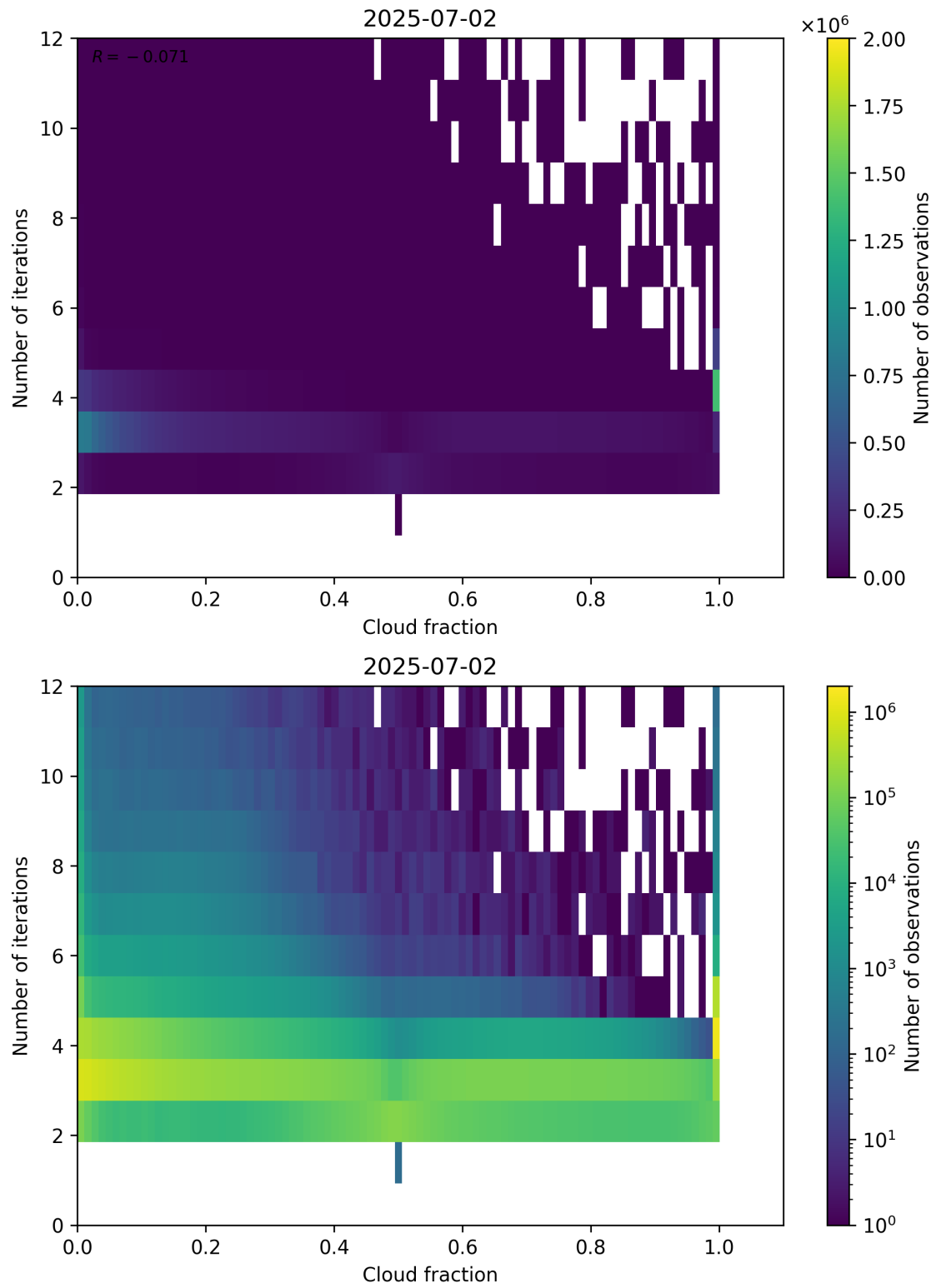
Figure 73: Scatter density plot of “Cloud fraction” against “Number of iterations” for 2025-07-02 to 2025-07-03.
