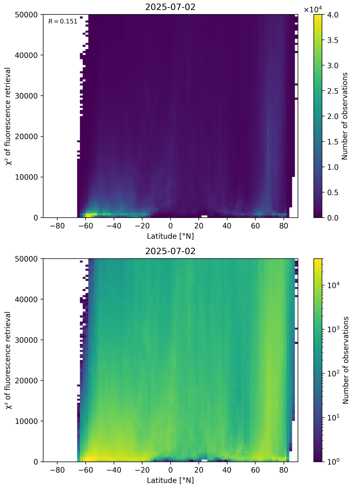
Figure 89: Scatter density plot of “Latitude” against “ \chi^2 of fluorescence retrieval” for 2025-07-02 to 2025-07-03.
