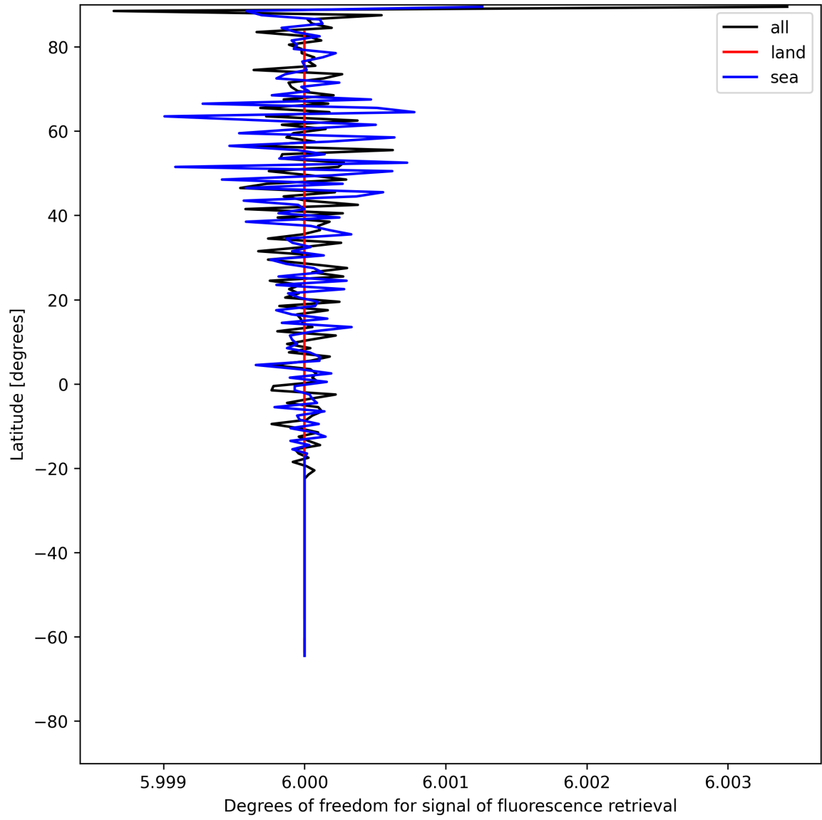
Figure 26: Zonal average of “Degrees of freedom for signal of fluorescence retrieval” for 2025-07-02 to 2025-07-03.
