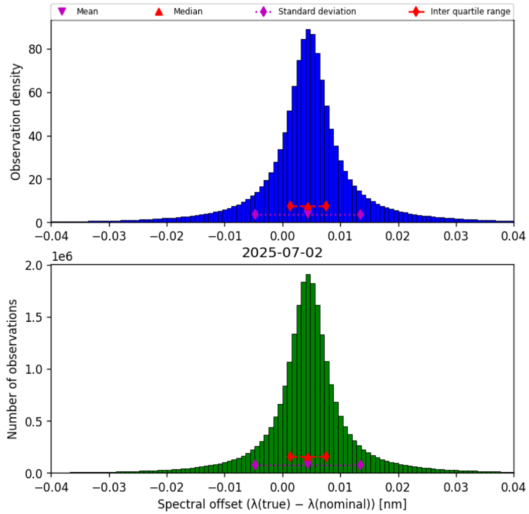
Figure 45: Histogram of “Spectral offset ( \lambda_{\text{true}} - \lambda_{\text{nominal}} )” for 2025-07-02 to 2025-07-03
