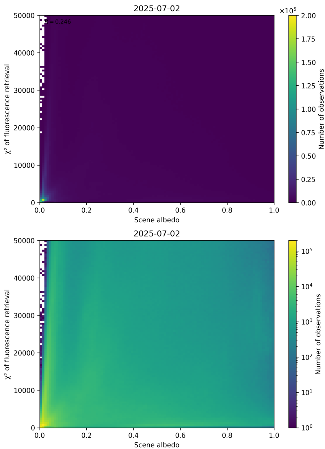
Figure 103: Scatter density plot of “Scene albedo” against “ \chi^2 of fluorescence retrieval” for 2025-07-02 to 2025-07-03.
