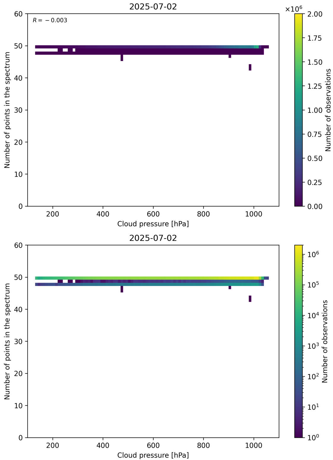
Figure 82: Scatter density plot of “Cloud pressure” against “Number of points in the spectrum” for 2025-07-02 to 2025-07-03.
