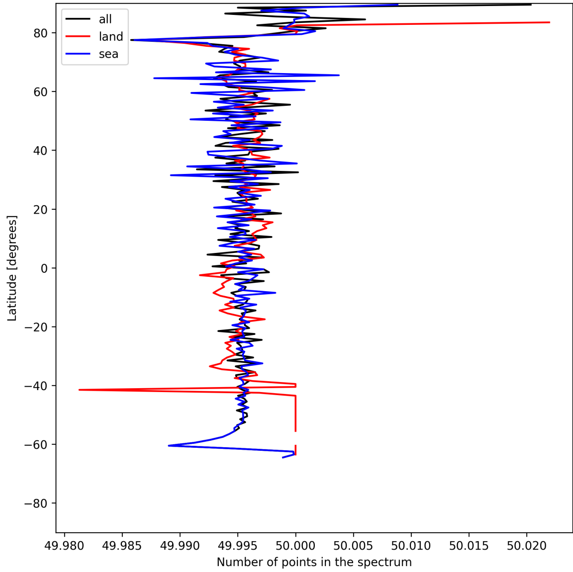
Figure 27: Zonal average of “Number of points in the spectrum” for 2025-07-02 to 2025-07-03.
