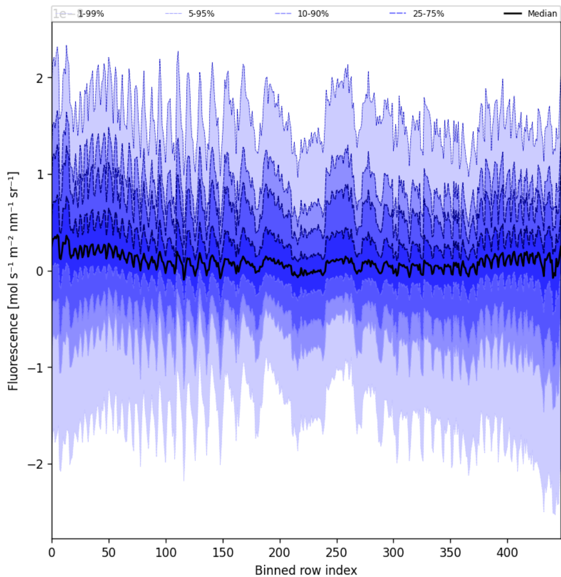
Figure 57: Along track statistics of “Fluorescence” for 2025-07-02 to 2025-07-03
