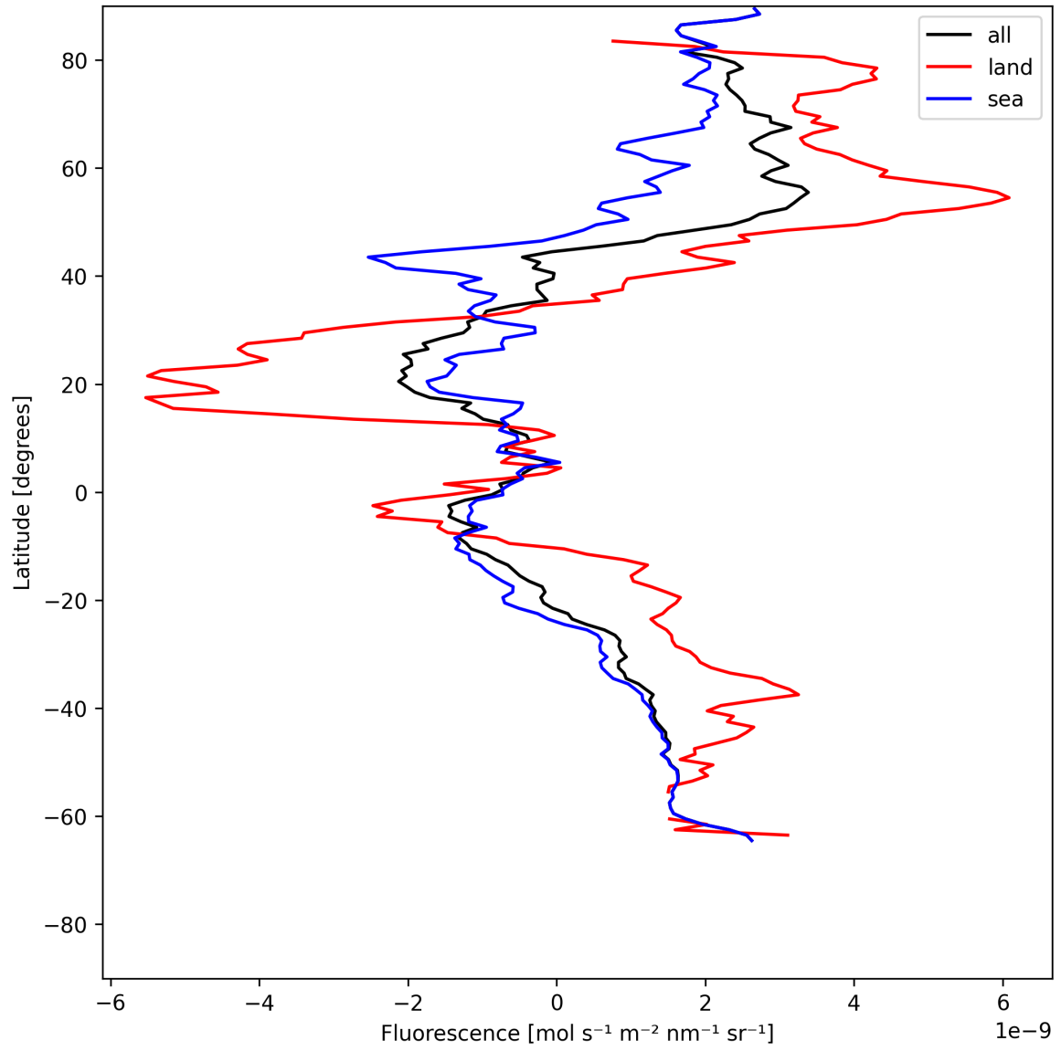
Figure 23: Zonal average of “Fluorescence” for 2025-07-02 to 2025-07-03.
