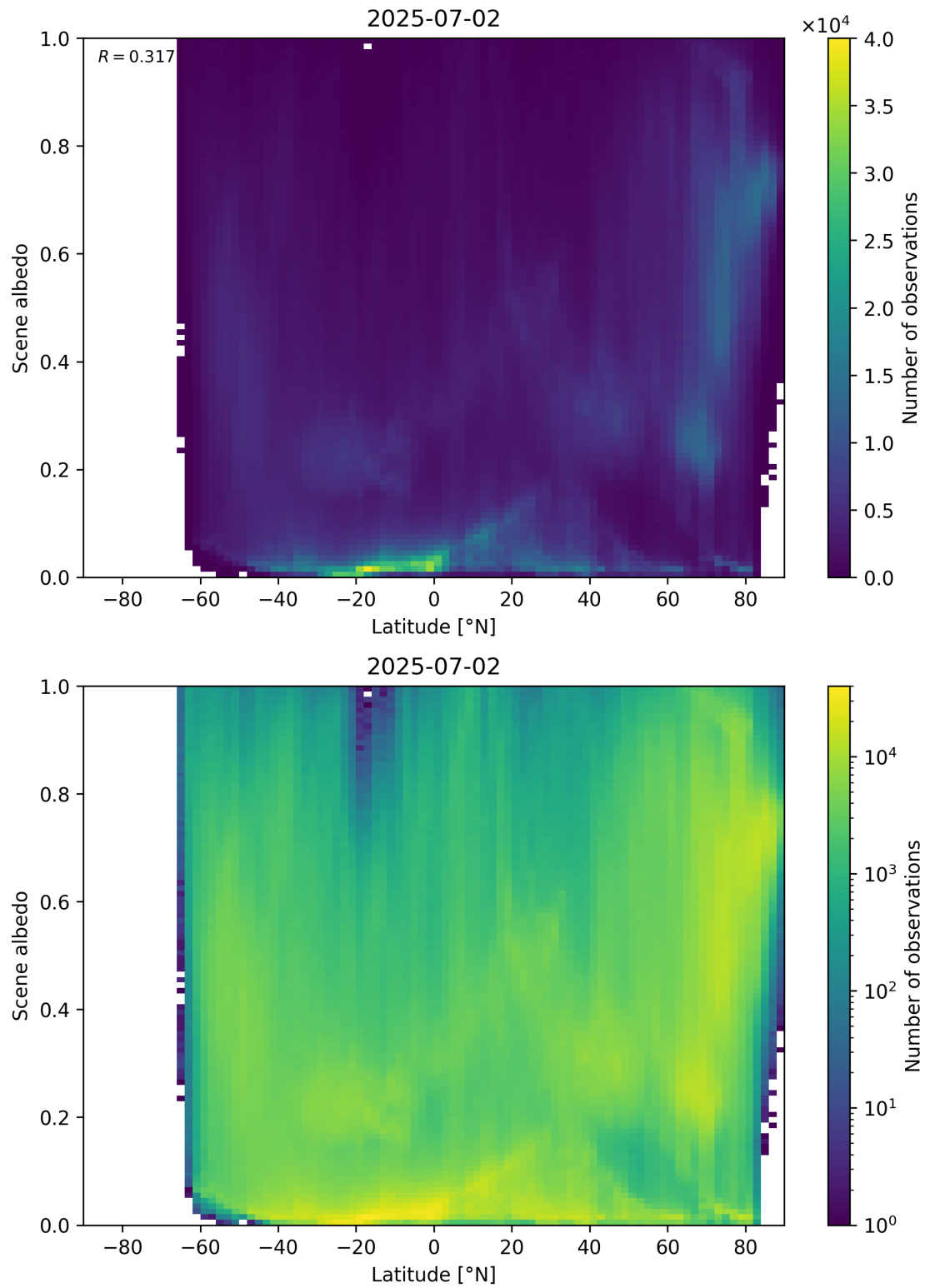
Figure 95: Scatter density plot of “Latitude” against “Scene albedo” for 2025-07-02 to 2025-07-03.
