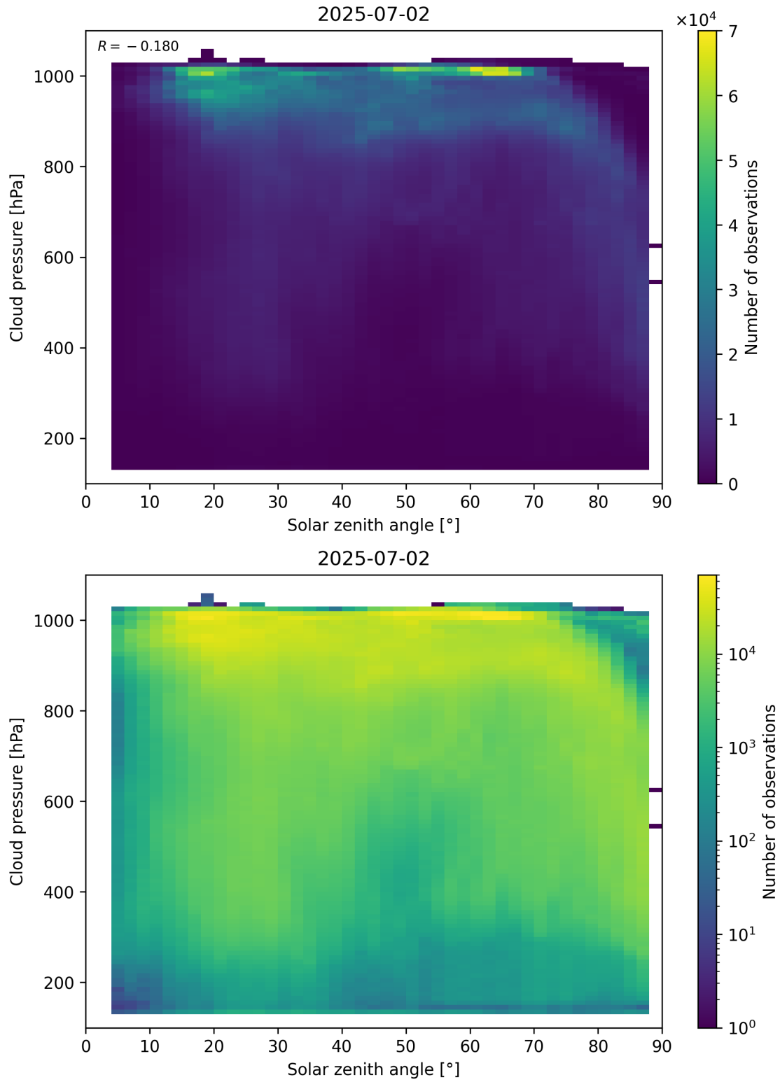
Figure 111: Scatter density plot of “Solar zenith angle” against “Cloud pressure” for 2025-07-02 to 2025-07-03.
