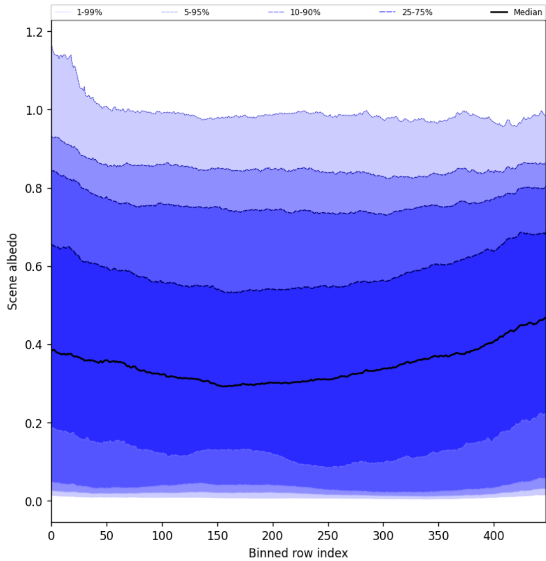
Figure 51: Along track statistics of “Scene albedo” for 2025-07-02 to 2025-07-03
