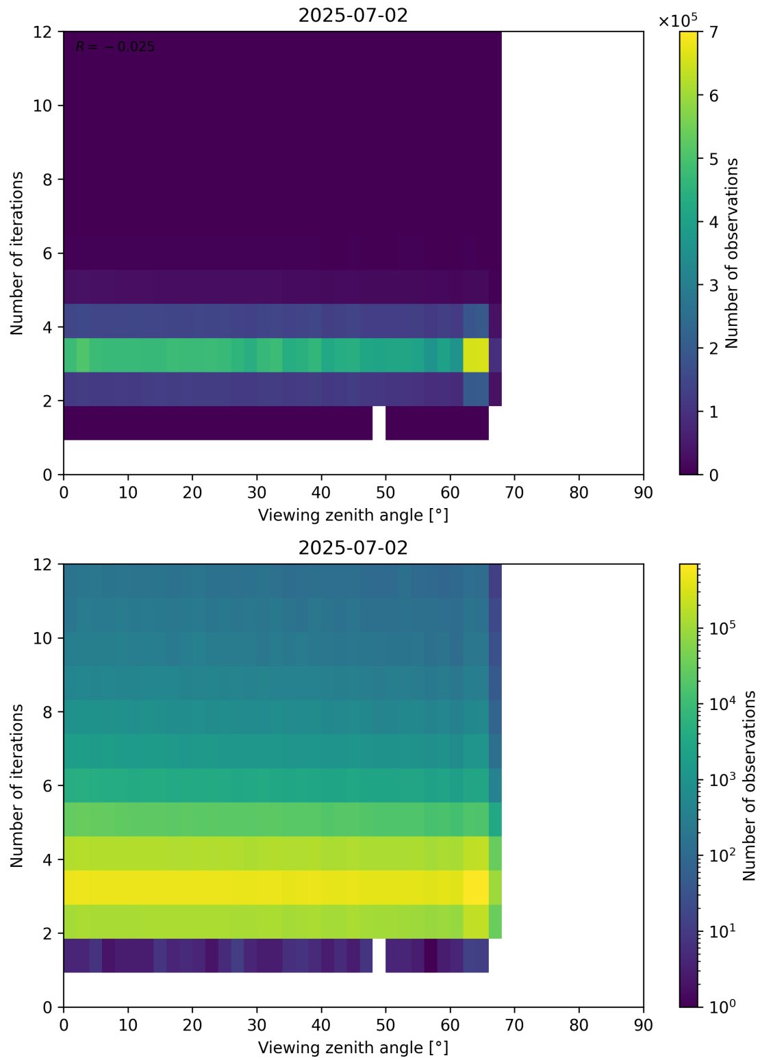
Figure 124: Scatter density plot of “Viewing zenith angle” against “Number of iterations” for 2025-07-02 to 2025-07-03.
