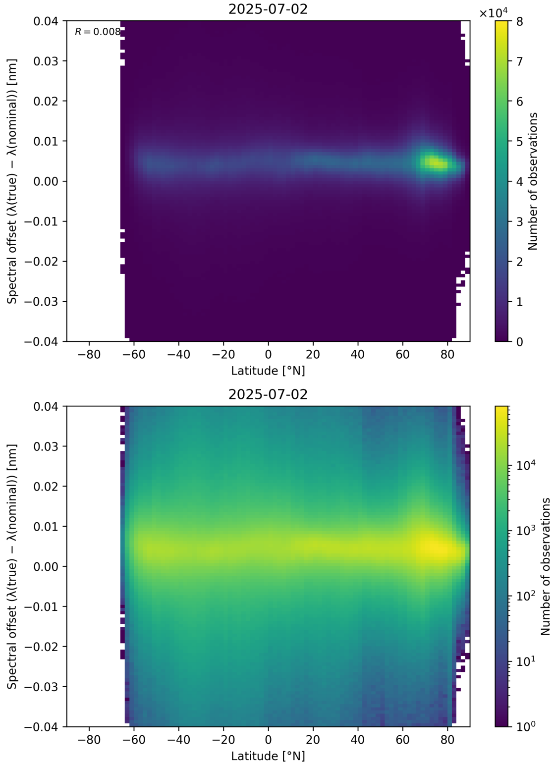
Figure 96: Scatter density plot of “Latitude” against “Spectral offset ( \lambda_{\text{true}} - \lambda_{\text{nominal}} )” for 2025-07-02 to 2025-07-03.
