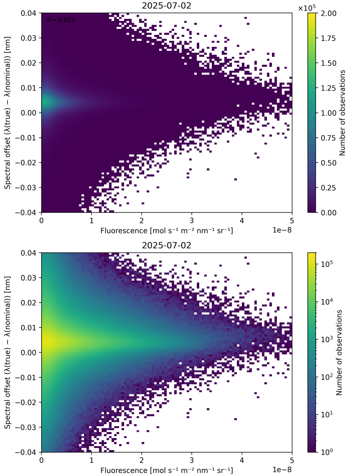
Figure 87: Scatter density plot of “Fluorescence” against “Spectral offset ( \lambda_{\text{true}} - \lambda_{\text{nominal}} )” for 2025-07-02 to 2025-07-03.
