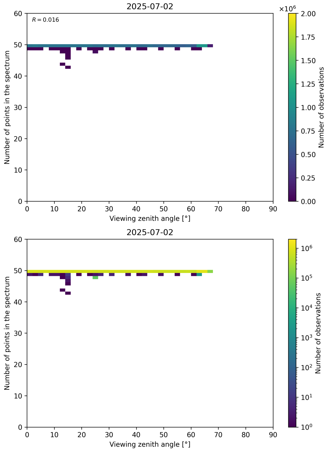
Figure 125: Scatter density plot of “Viewing zenith angle” against “Number of points in the spectrum” for 2025-07-02 to 2025-07-03.
