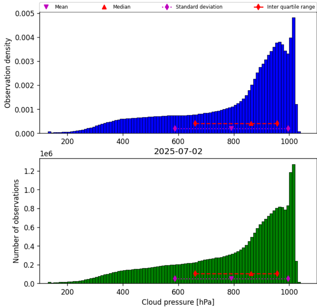
Figure 30: Histogram of “Cloud pressure” for 2025-07-02 to 2025-07-03
