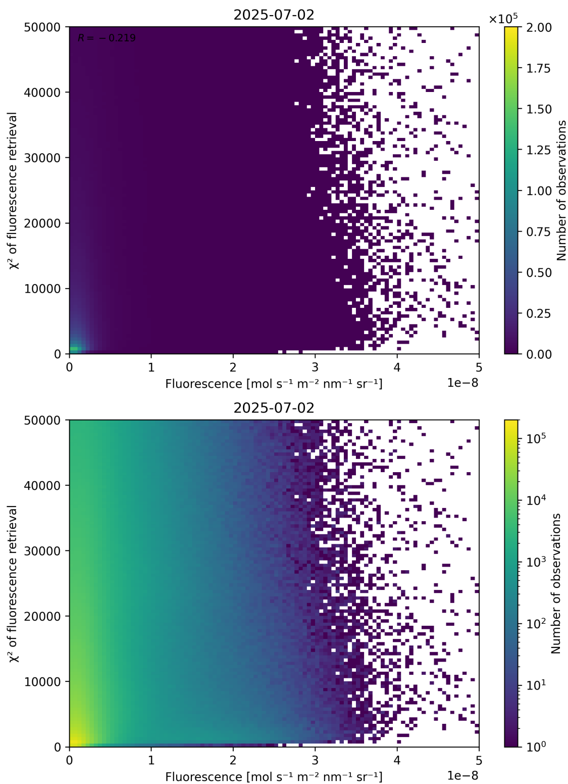
Figure 85: Scatter density plot of “Fluorescence” against “ \chi^2 of fluorescence retrieval” for 2025-07-02 to 2025-07-03.
