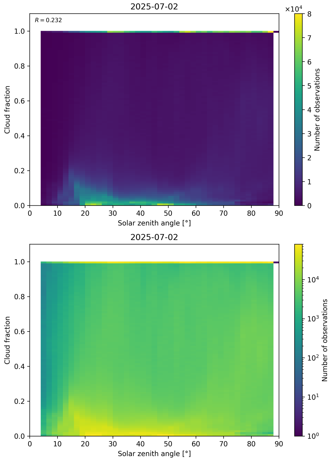
Figure 110: Scatter density plot of “Solar zenith angle” against “Cloud fraction” for 2025-07-02 to 2025-07-03.
