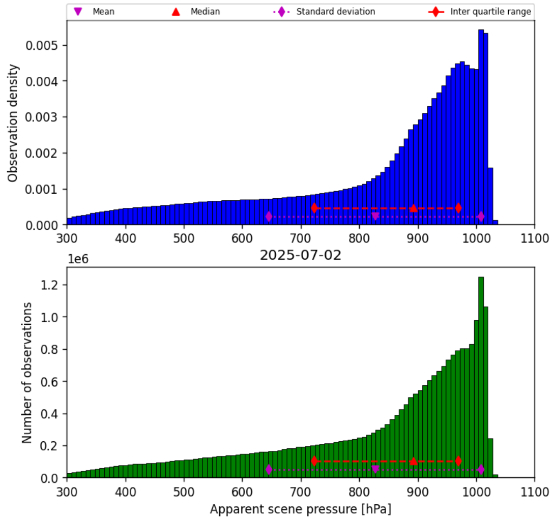
Figure 36: Histogram of “Apparent scene pressure” for 2025-07-02 to 2025-07-03
