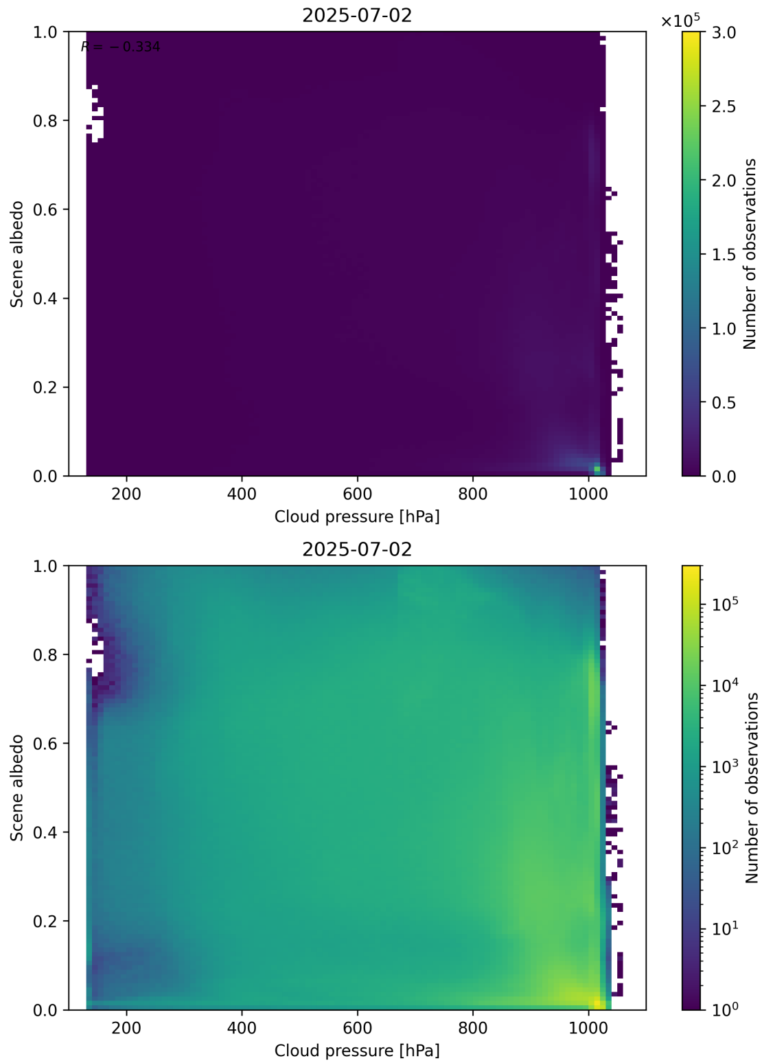
Figure 83: Scatter density plot of “Cloud pressure” against “Scene albedo” for 2025-07-02 to 2025-07-03.
