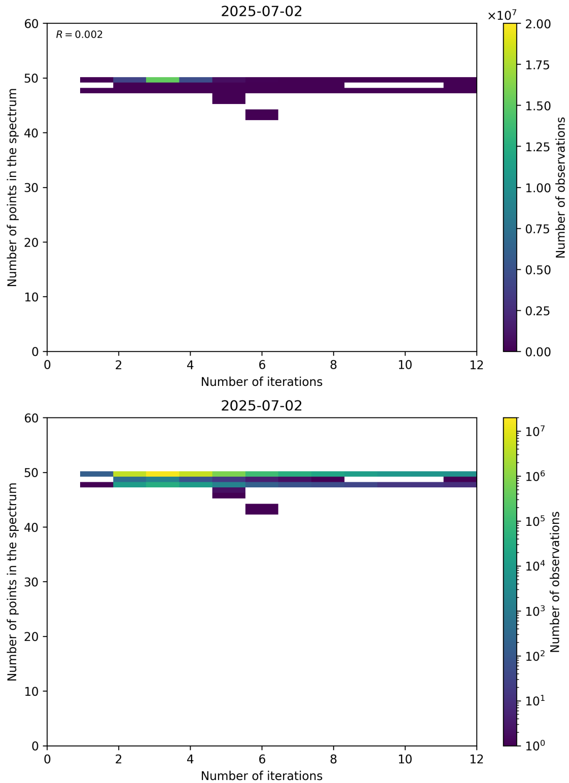
Figure 99: Scatter density plot of “Number of iterations” against “Number of points in the spectrum” for 2025-07-02 to 2025-07-03.
