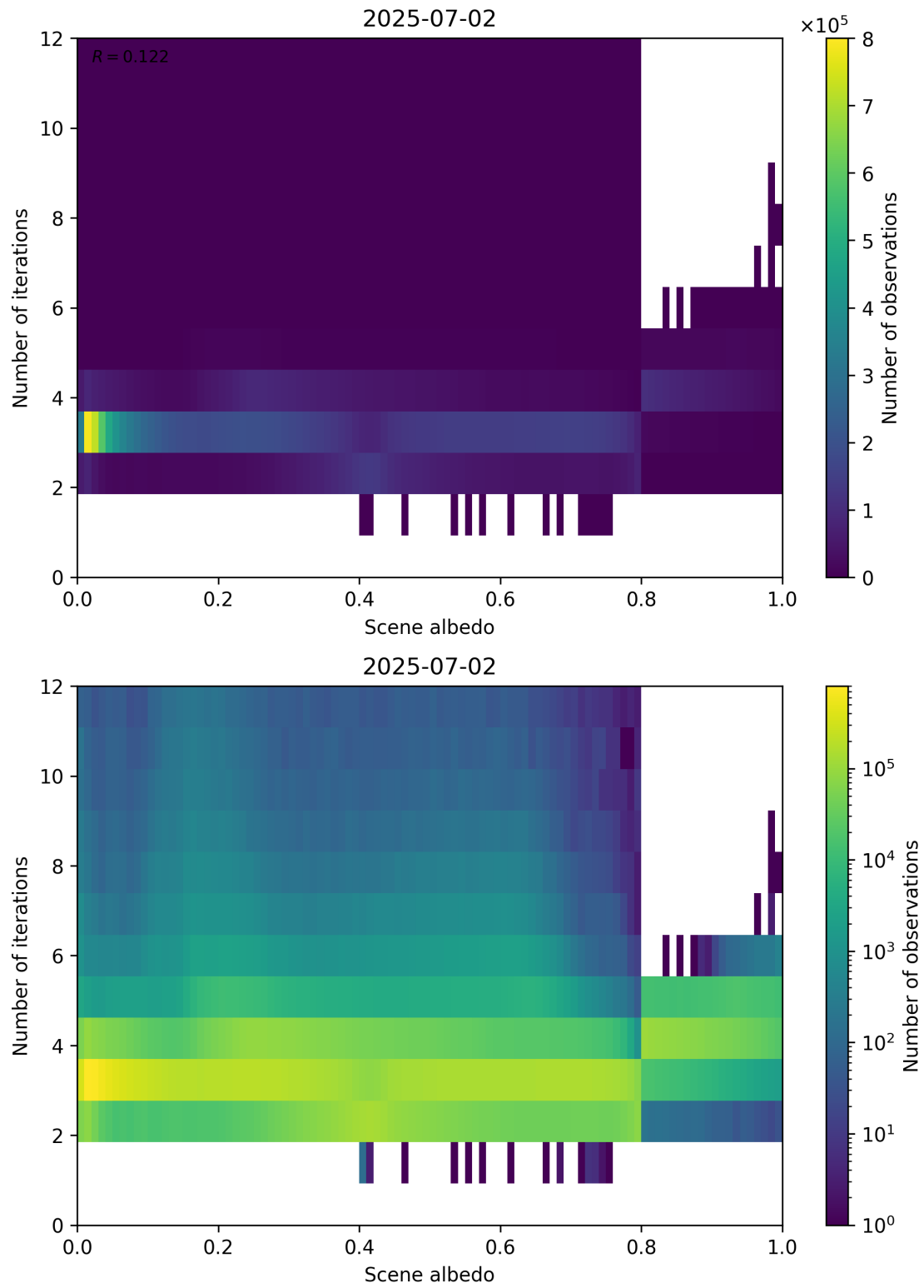
Figure 105: Scatter density plot of “Scene albedo” against “Number of iterations” for 2025-07-02 to 2025-07-03.
