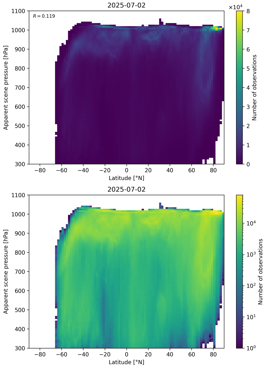
Figure 88: Scatter density plot of “Latitude” against “Apparent scene pressure” for 2025-07-02 to 2025-07-03.
