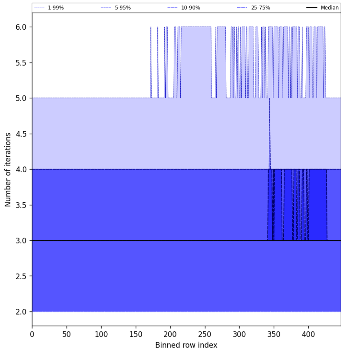
Figure 56: Along track statistics of “Number of iterations” for 2025-07-02 to 2025-07-03
