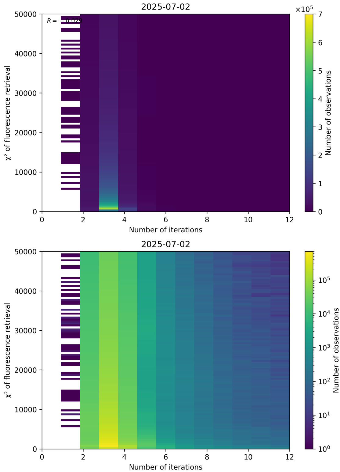
Figure 97: Scatter density plot of “Number of iterations” against “ \chi^2 of fluorescence retrieval” for 2025-07-02 to 2025-07-03.
