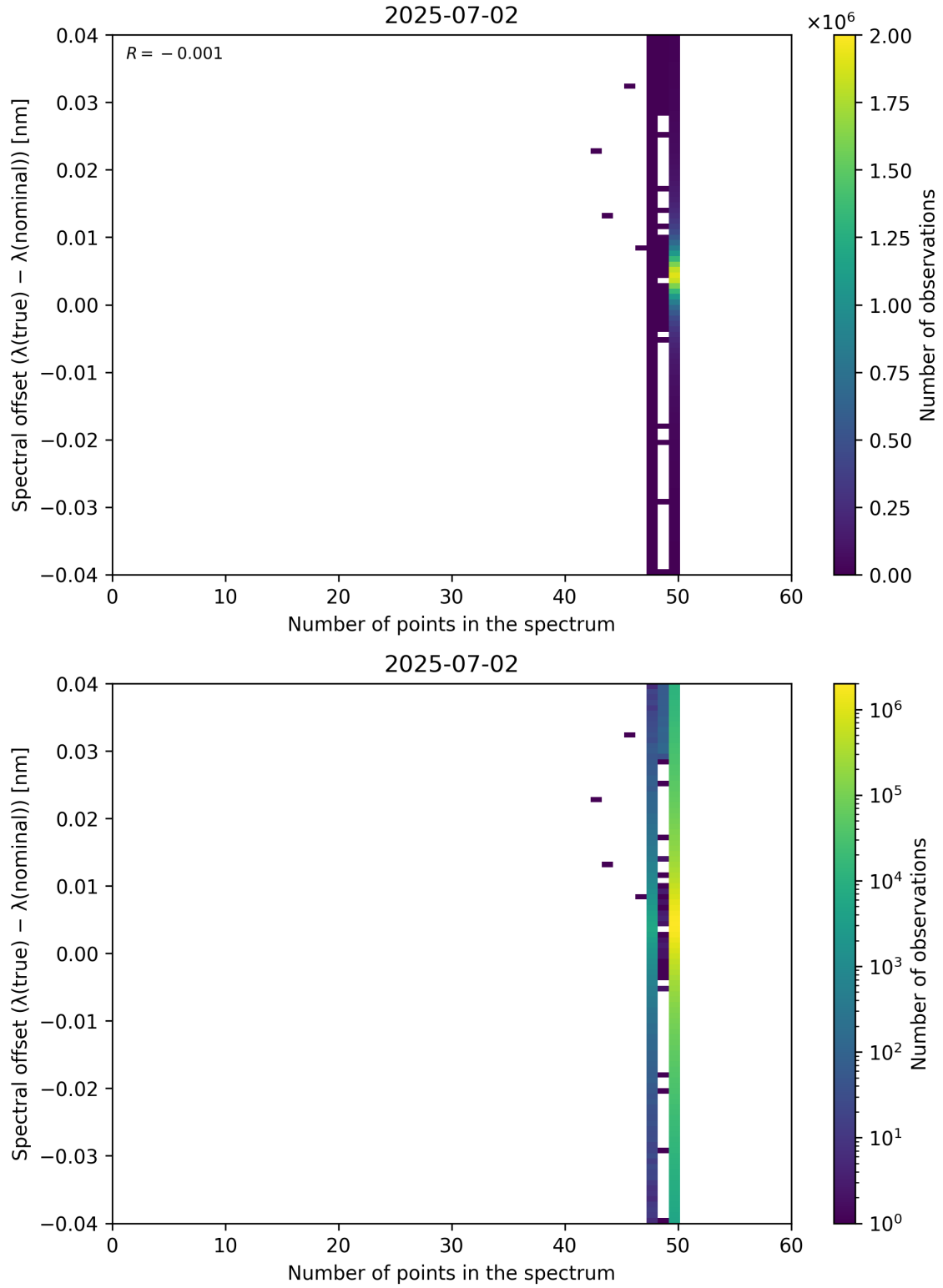
Figure 101: Scatter density plot of “Number of points in the spectrum” against “Spectral offset ( \lambda_{\text{true}} - \lambda_{\text{nominal}} )” for 2025-07-02 to 2025-07-03.
