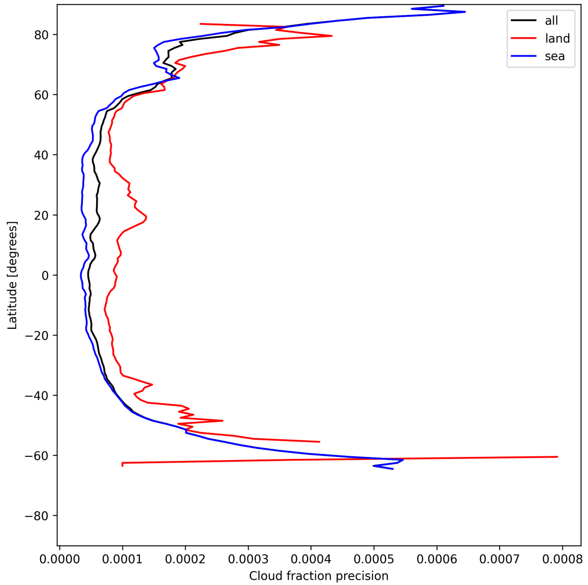
Figure 16: Zonal average of “Cloud fraction precision” for 2025-07-02 to 2025-07-03.
