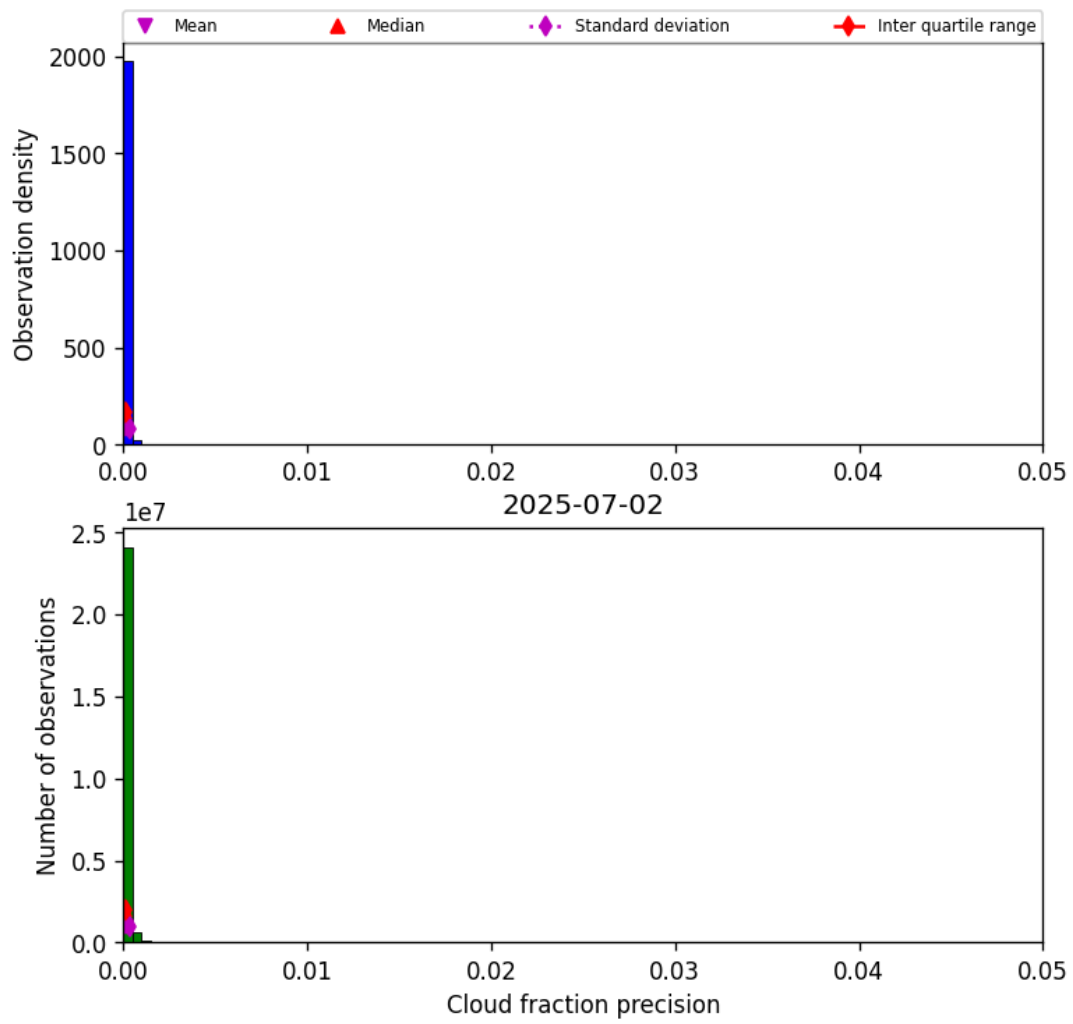
Figure 33: Histogram of “Cloud fraction precision” for 2025-07-02 to 2025-07-03
