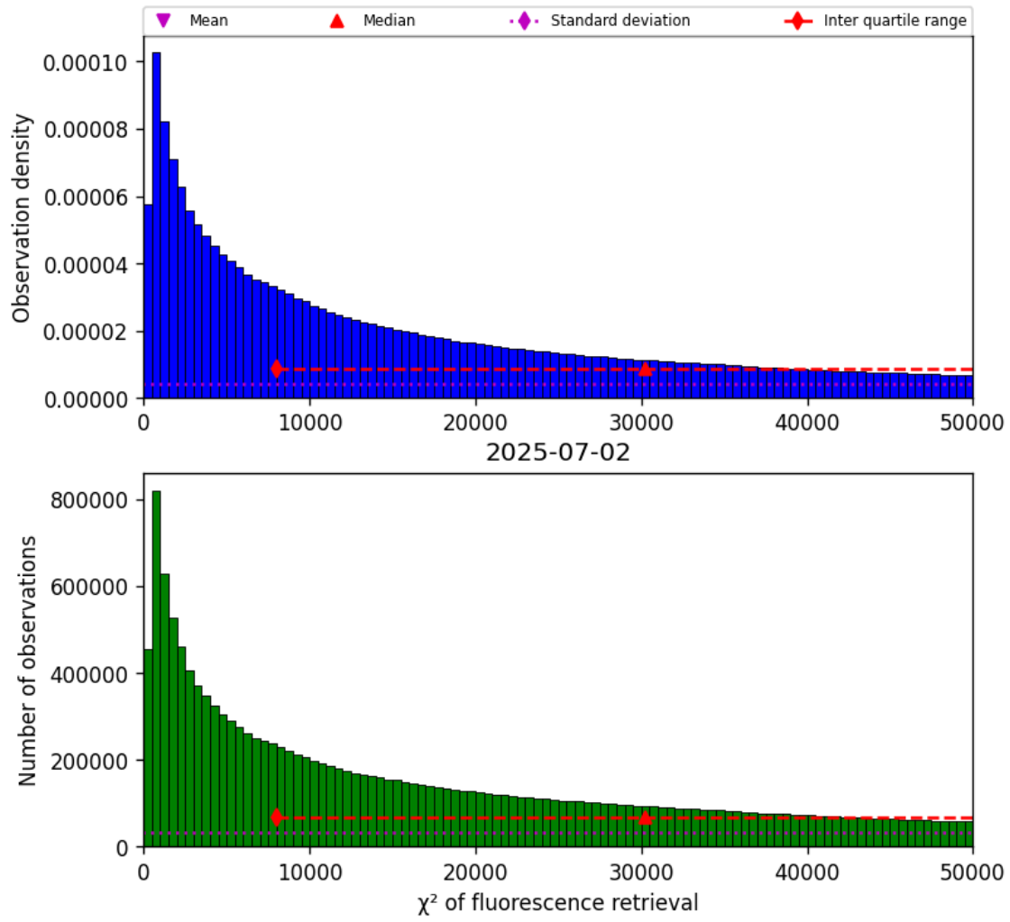
Figure 42: Histogram of “ \chi^2 of fluorescence retrieval” for 2025-07-02 to 2025-07-03
