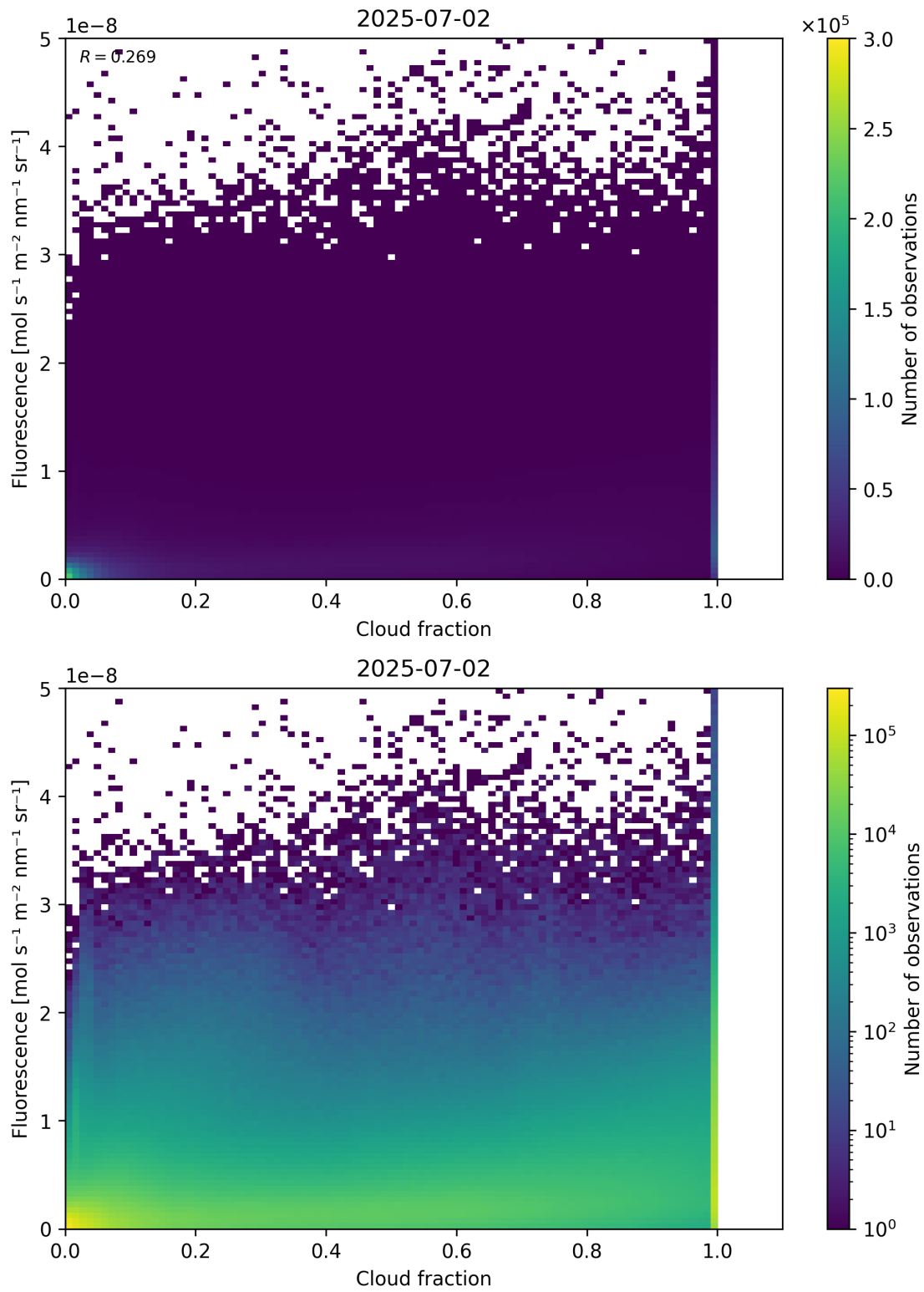
Figure 72: Scatter density plot of “Cloud fraction” against “Fluorescence” for 2025-07-02 to 2025-07-03.
