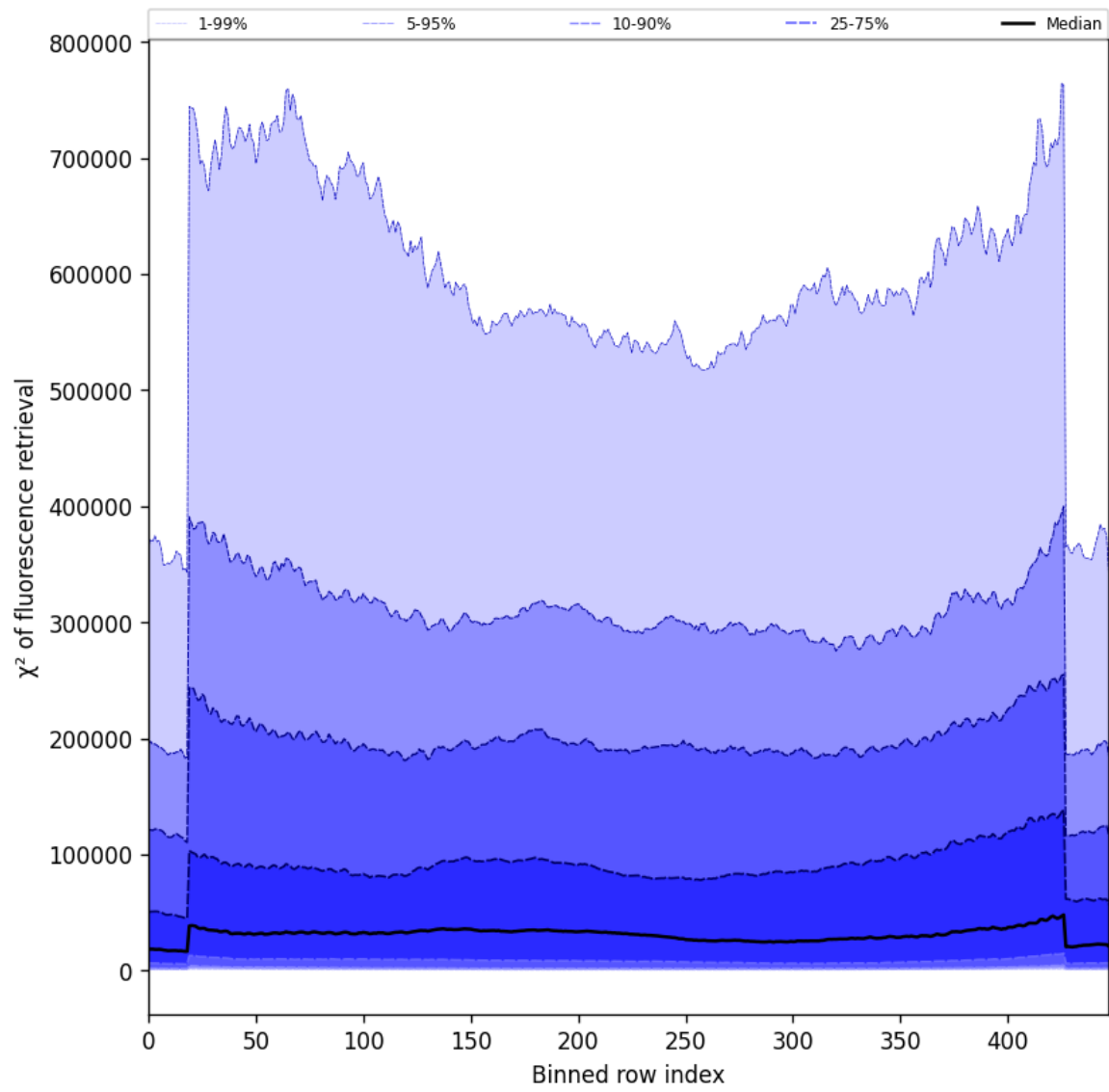
Figure 59: Along track statistics of “ \chi^2 of fluorescence retrieval” for 2025-07-02 to 2025-07-03
