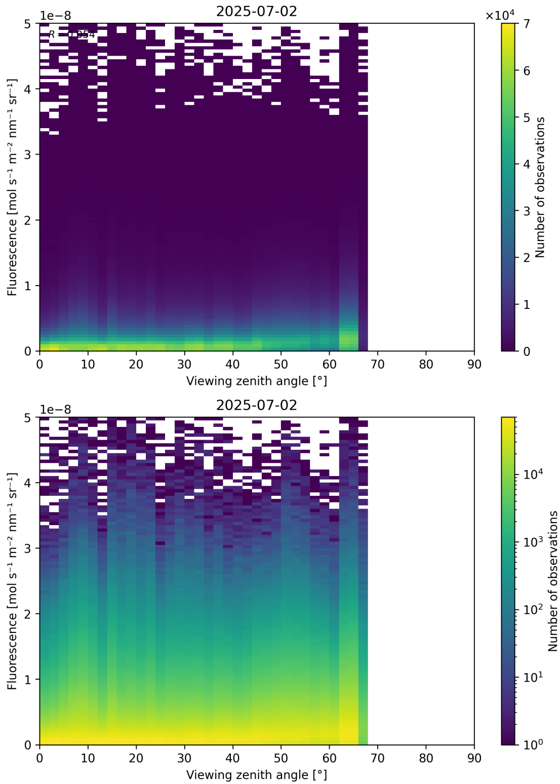
Figure 122: Scatter density plot of “Viewing zenith angle” against “Fluorescence” for 2025-07-02 to 2025-07-03.
