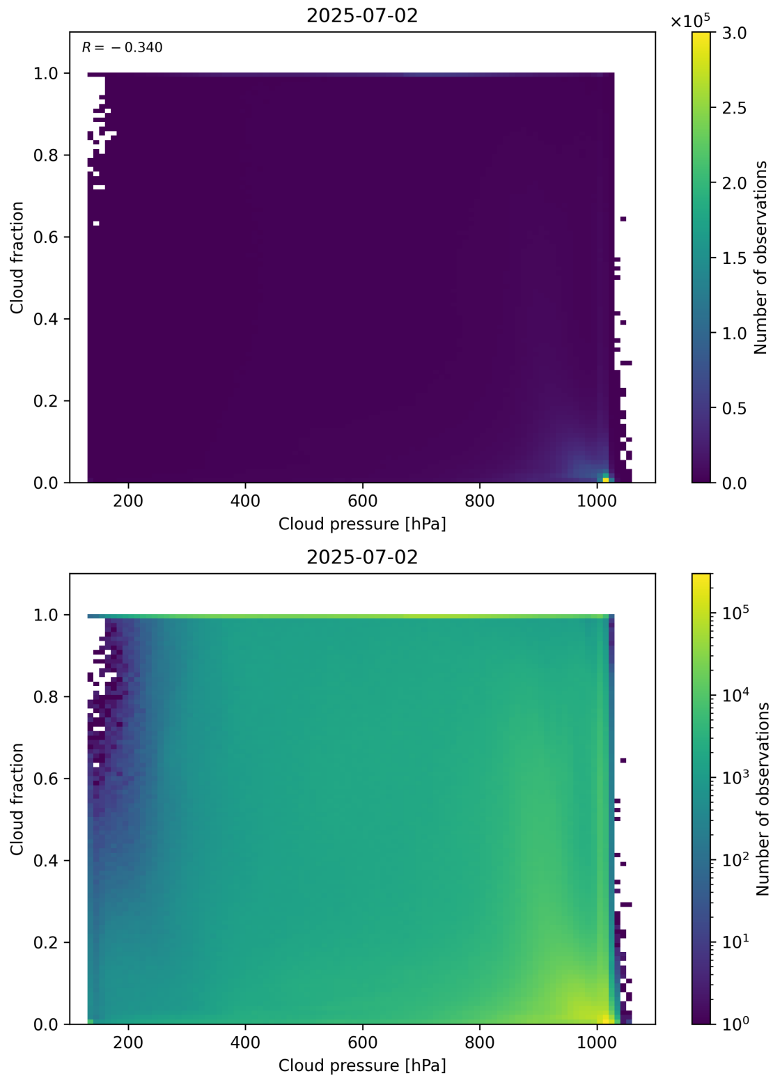
Figure 79: Scatter density plot of “Cloud pressure” against “Cloud fraction” for 2025-07-02 to 2025-07-03.
