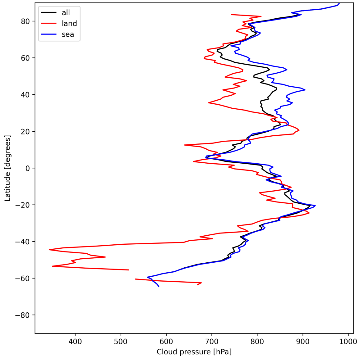
Figure 13: Zonal average of “Cloud pressure” for 2025-07-02 to 2025-07-03.
