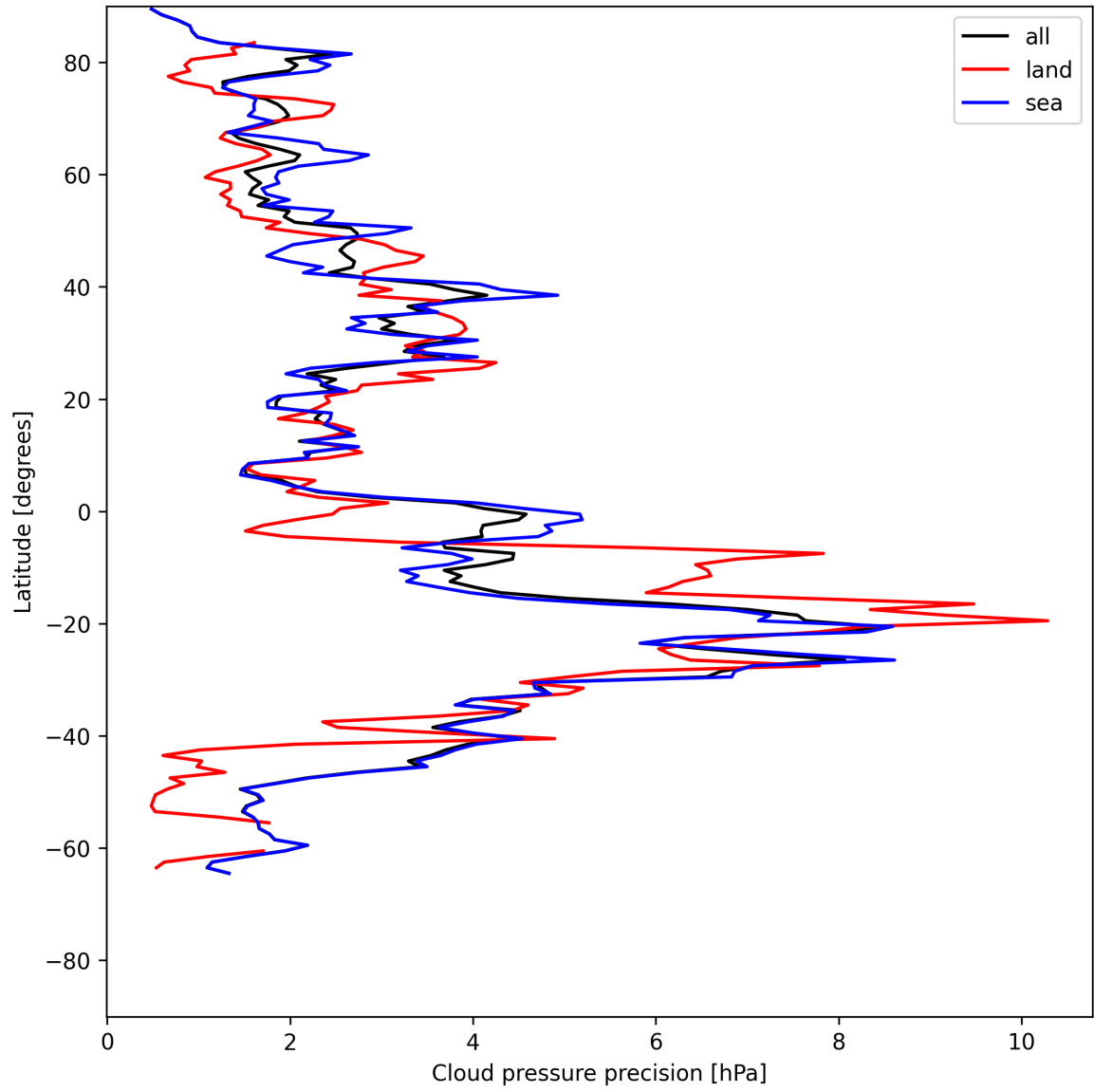
Figure 14: Zonal average of “Cloud pressure precision” for 2025-07-02 to 2025-07-03.
