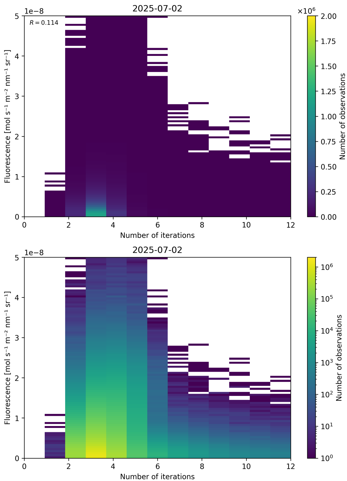
Figure 98: Scatter density plot of “Number of iterations” against “Fluorescence” for 2025-07-02 to 2025-07-03.
