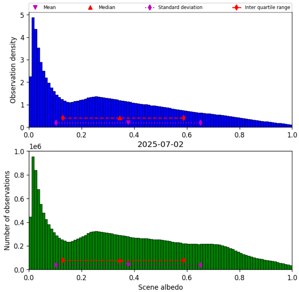
Figure 34: Histogram of “Scene albedo” for 2025-07-02 to 2025-07-03
