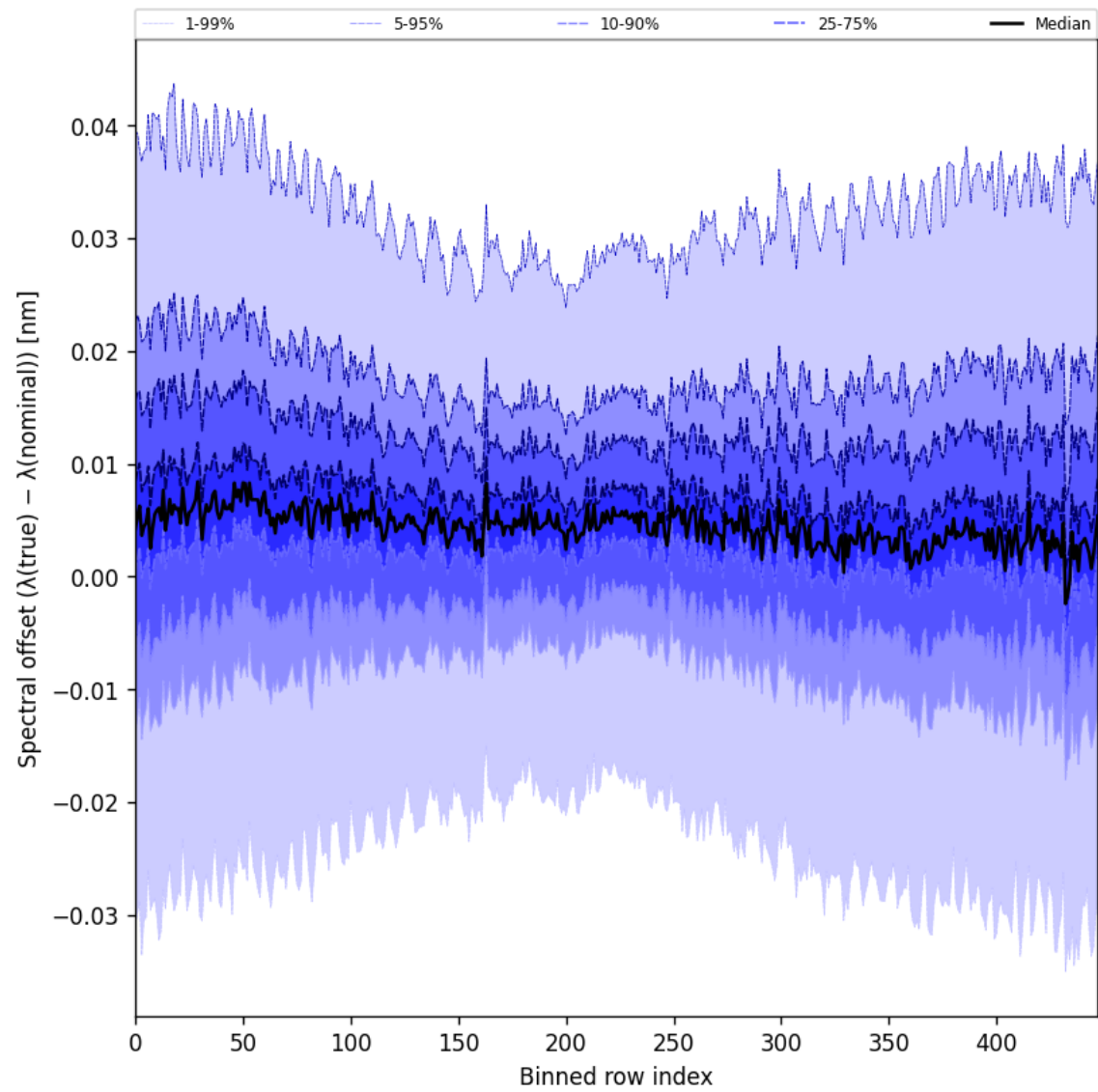
Figure 62: Along track statistics of “Spectral offset ( \lambda_{\text{true}} - \lambda_{\text{nominal}} )” for 2025-07-02 to 2025-07-03
