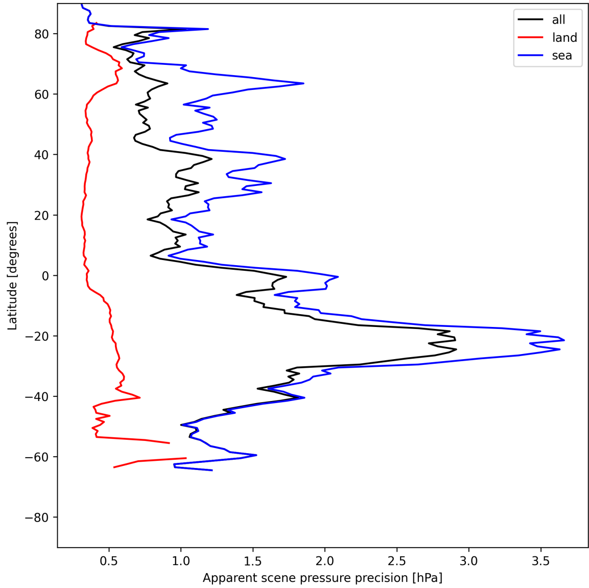
Figure 20: Zonal average of “Apparent scene pressure precision” for 2025-07-02 to 2025-07-03.
