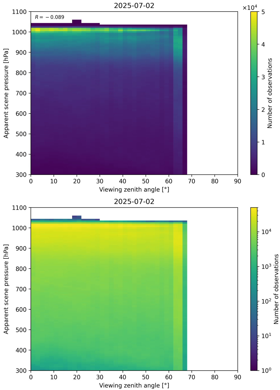
Figure 118: Scatter density plot of “Viewing zenith angle” against “Apparent scene pressure” for 2025-07-02 to 2025-07-03.
