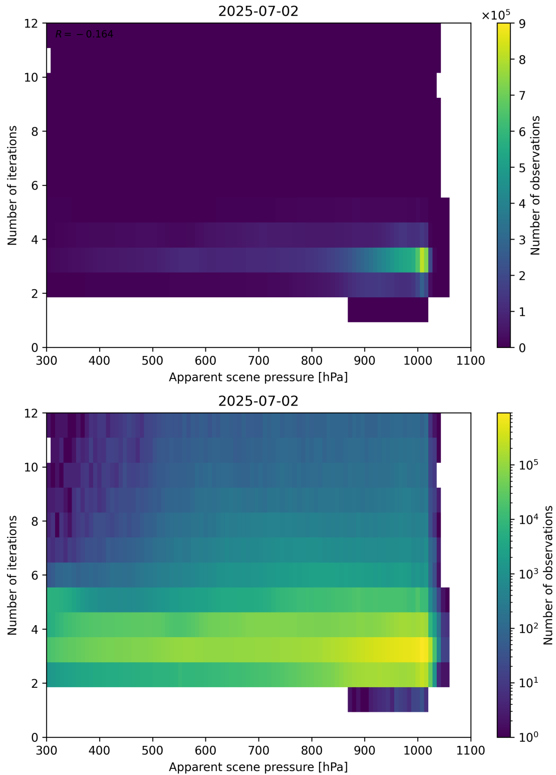
Figure 65: Scatter density plot of “Apparent scene pressure” against “Number of iterations” for 2025-07-02 to 2025-07-03.
