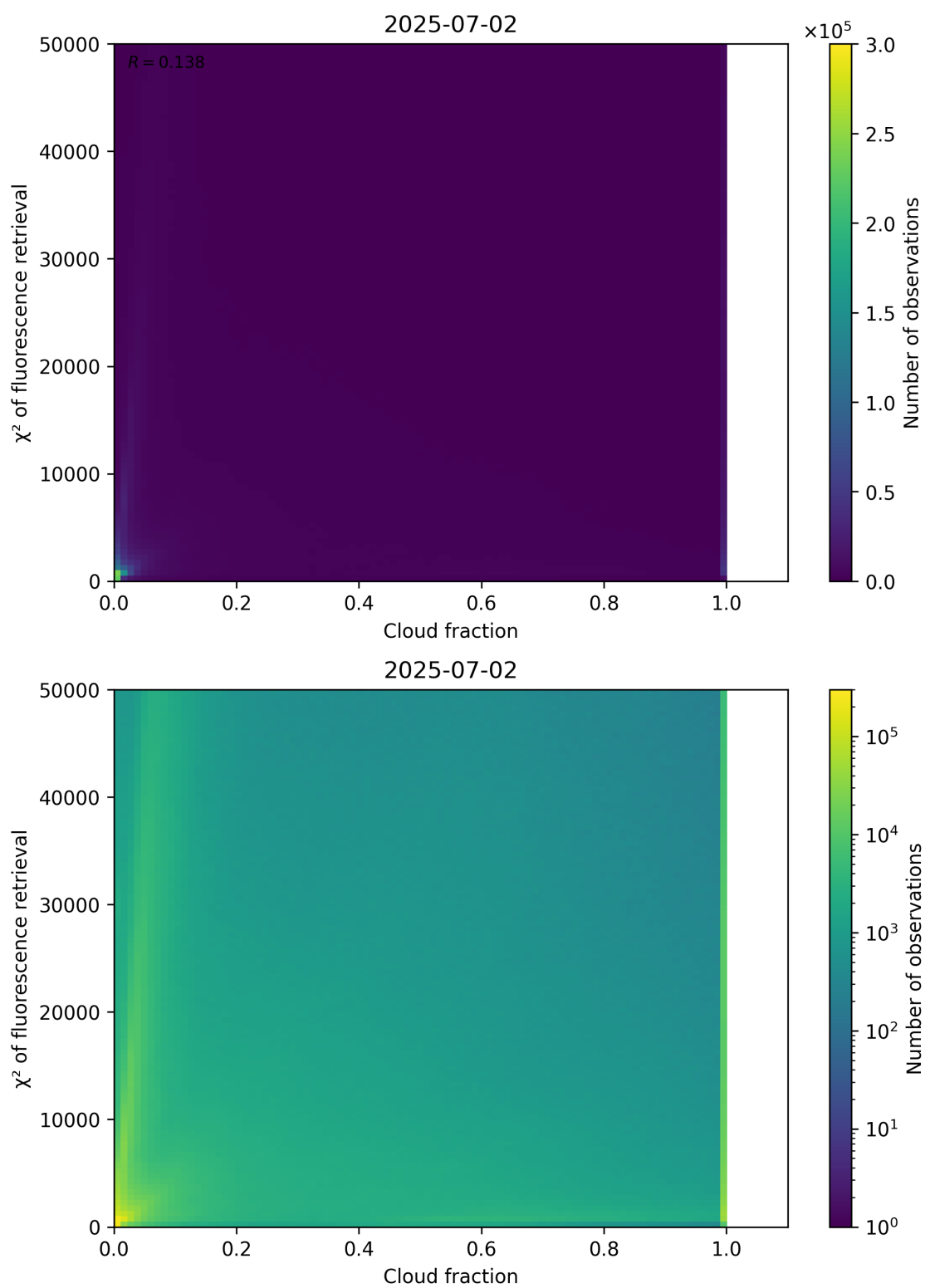
Figure 71: Scatter density plot of “Cloud fraction” against “ \chi^2 of fluorescence retrieval” for 2025-07-02 to 2025-07-03.
