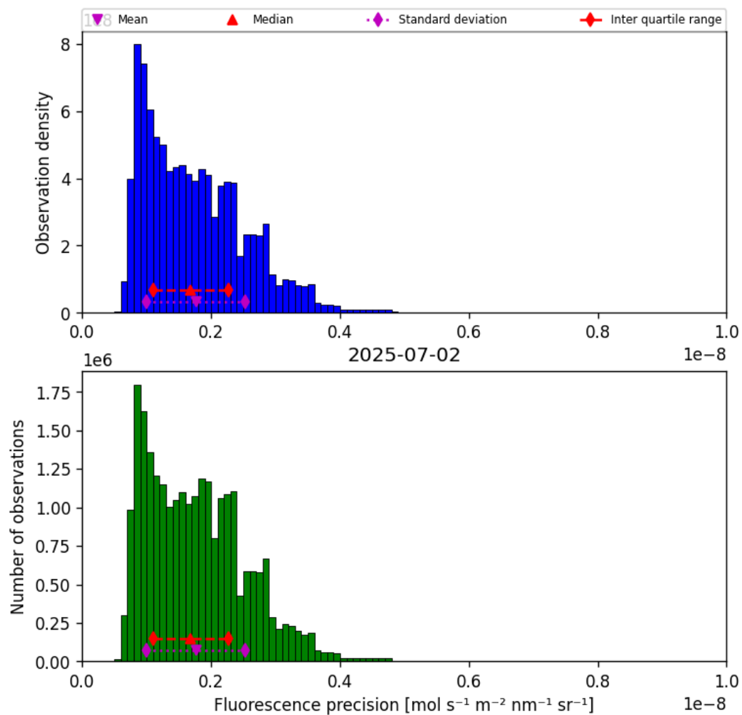
Figure 41: Histogram of “Fluorescence precision” for 2025-07-02 to 2025-07-03
