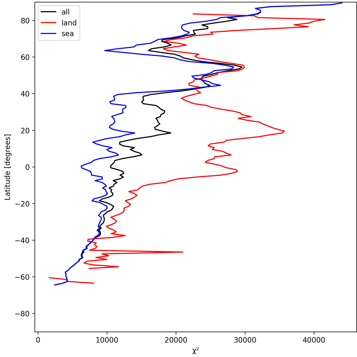
Figure 21: Zonal average of “ \chi^2 ” for 2025-07-02 to 2025-07-03.
