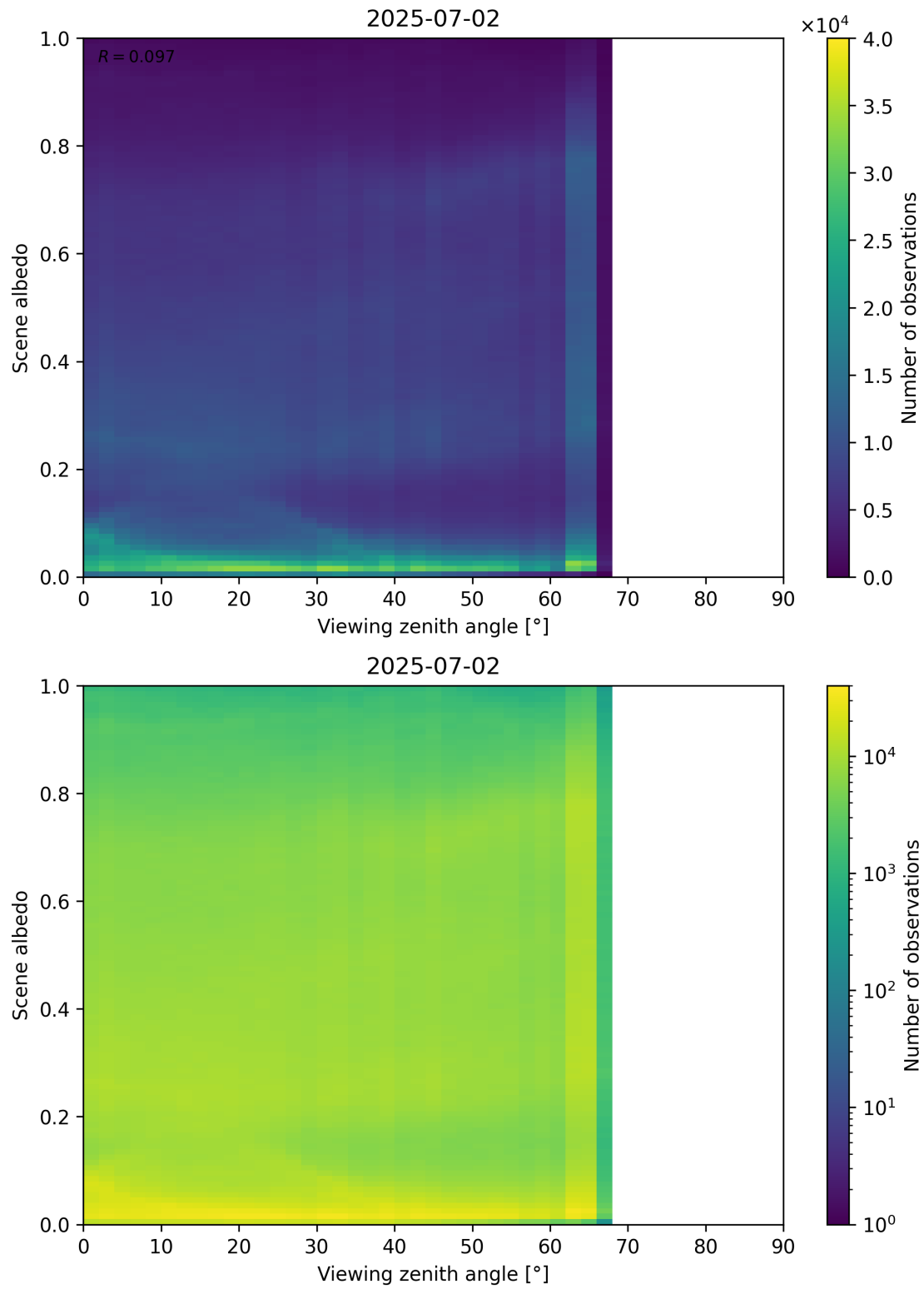
Figure 126: Scatter density plot of “Viewing zenith angle” against “Scene albedo” for 2025-07-02 to 2025-07-03.
