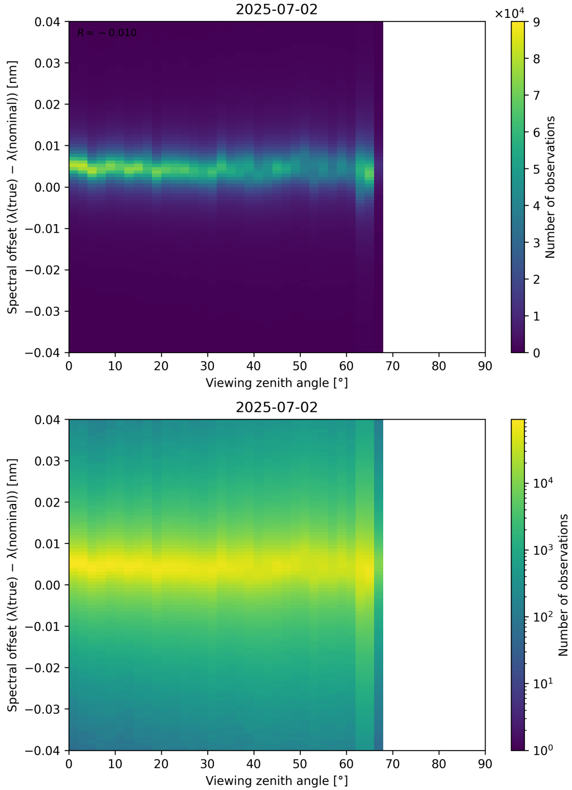
Figure 128: Scatter density plot of “Viewing zenith angle” against “Spectral offset ( \lambda_{\text{true}} - \lambda_{\text{nominal}} )” for 2025-07-02 to 2025-07-03.
