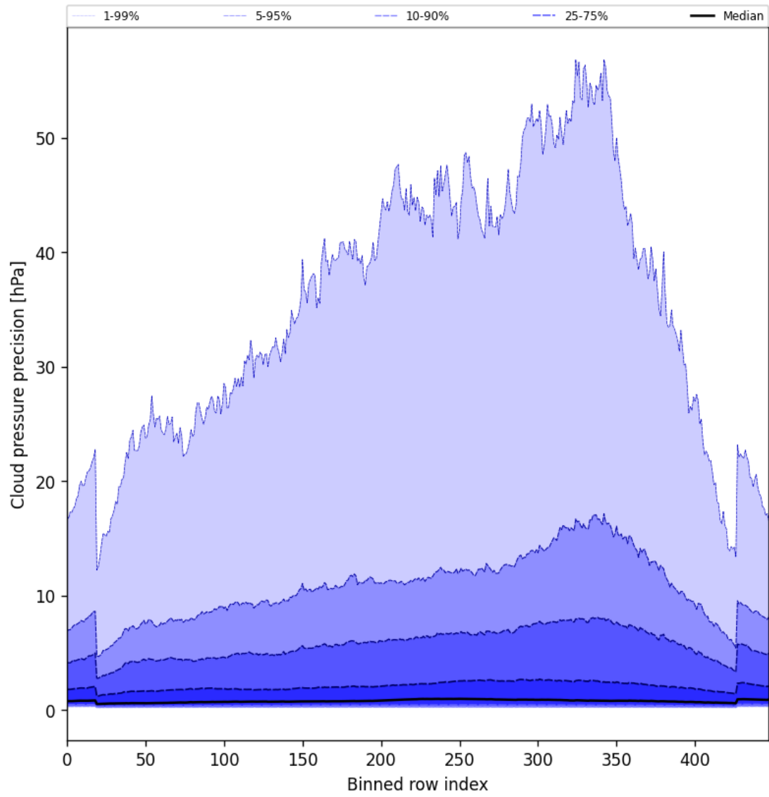
Figure 48: Along track statistics of “Cloud pressure precision” for 2025-07-02 to 2025-07-03
