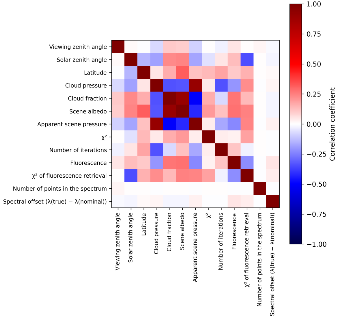
Figure 2: Map of correlation matrix for 2025-07-02 to 2025-07-03.
