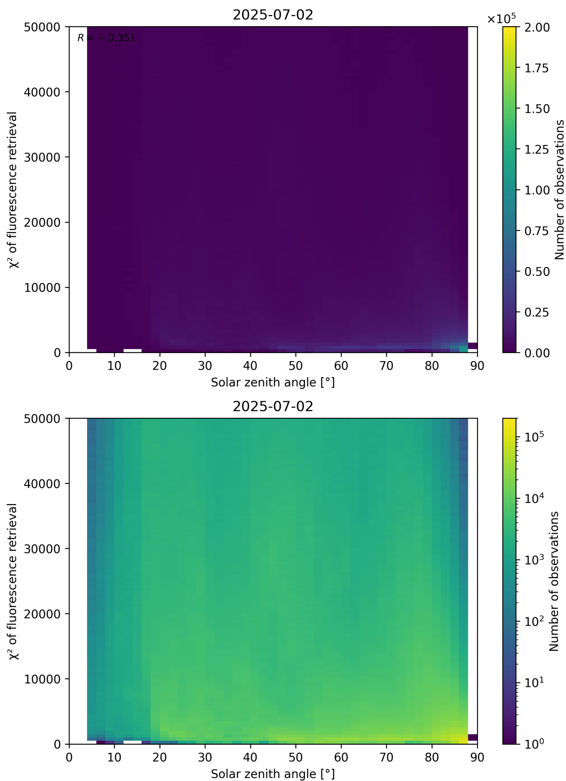
Figure 109: Scatter density plot of “Solar zenith angle” against “ \chi^2 of fluorescence retrieval” for 2025-07-02 to 2025-07-03.
