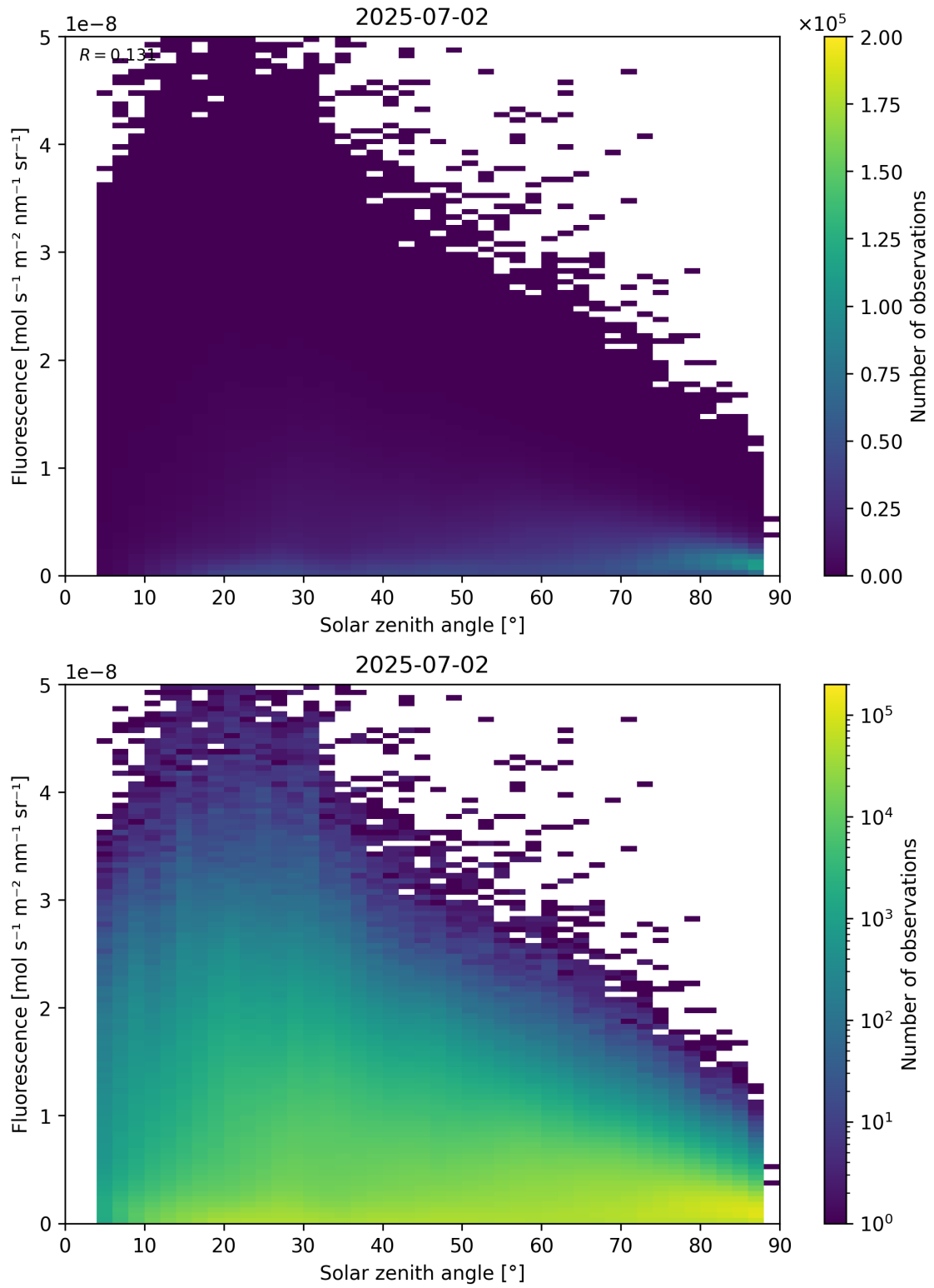
Figure 112: Scatter density plot of “Solar zenith angle” against “Fluorescence” for 2025-07-02 to 2025-07-03.
