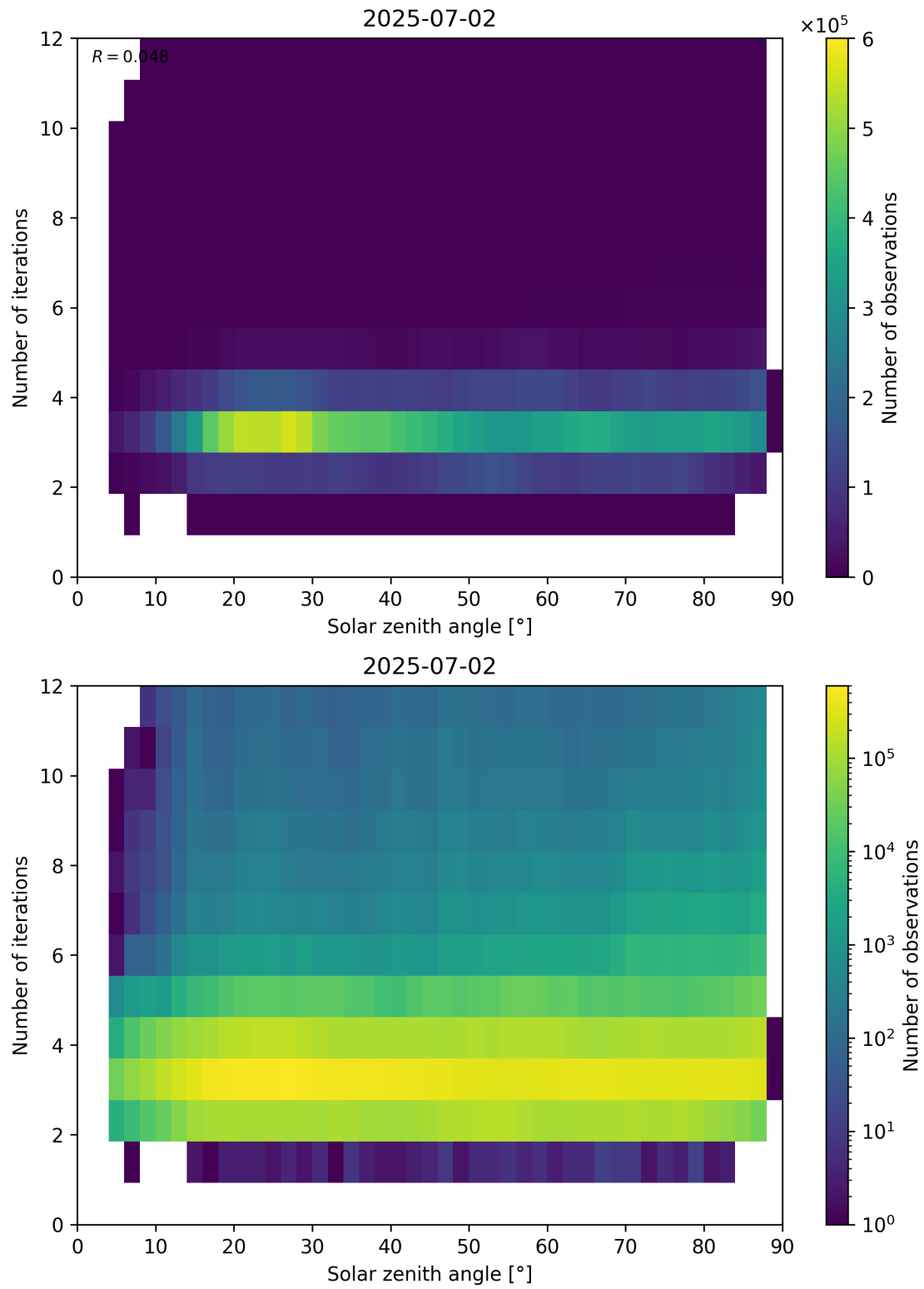
Figure 114: Scatter density plot of “Solar zenith angle” against “Number of iterations” for 2025-07-02 to 2025-07-03.
