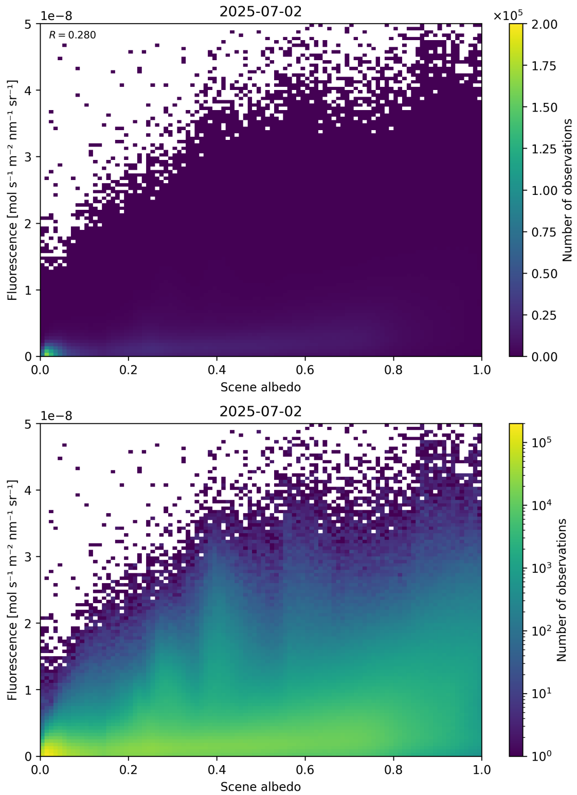
Figure 104: Scatter density plot of “Scene albedo” against “Fluorescence” for 2025-07-02 to 2025-07-03.
