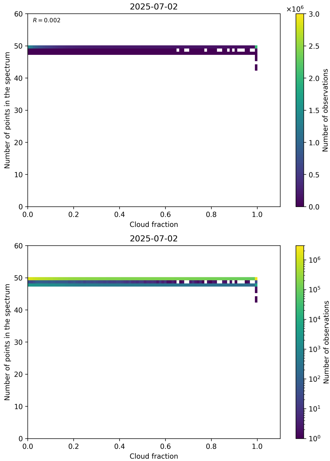
Figure 74: Scatter density plot of “Cloud fraction” against “Number of points in the spectrum” for 2025-07-02 to 2025-07-03.
