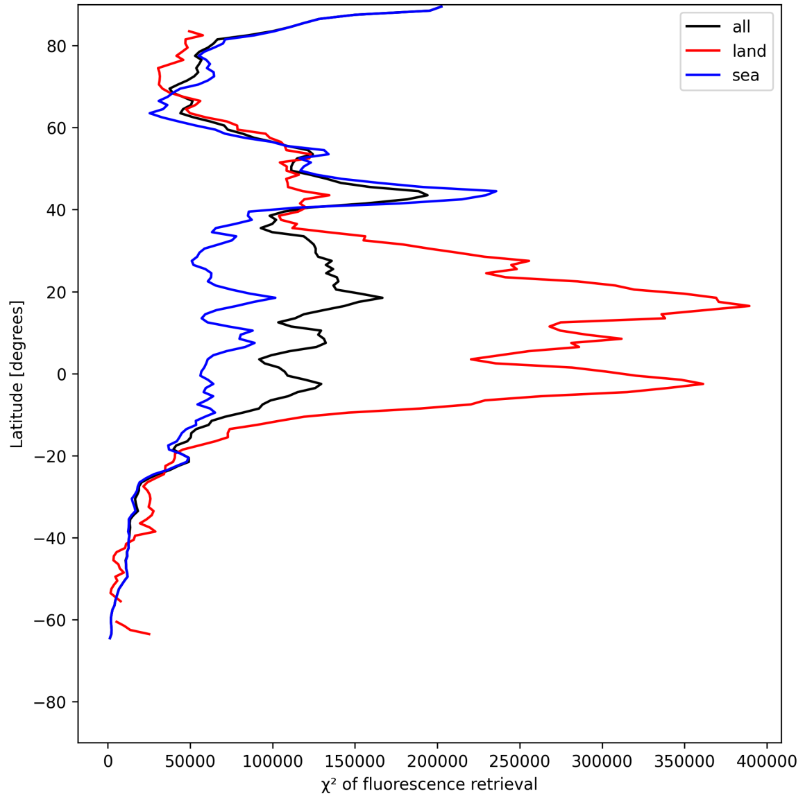
Figure 25: Zonal average of “ \chi^2 of fluorescence retrieval” for 2025-07-02 to 2025-07-03.
