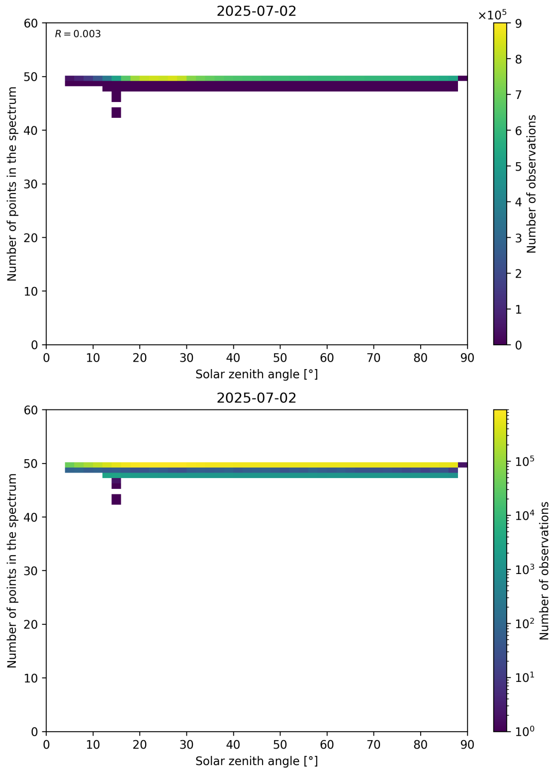
Figure 115: Scatter density plot of “Solar zenith angle” against “Number of points in the spectrum” for 2025-07-02 to 2025-07-03.
