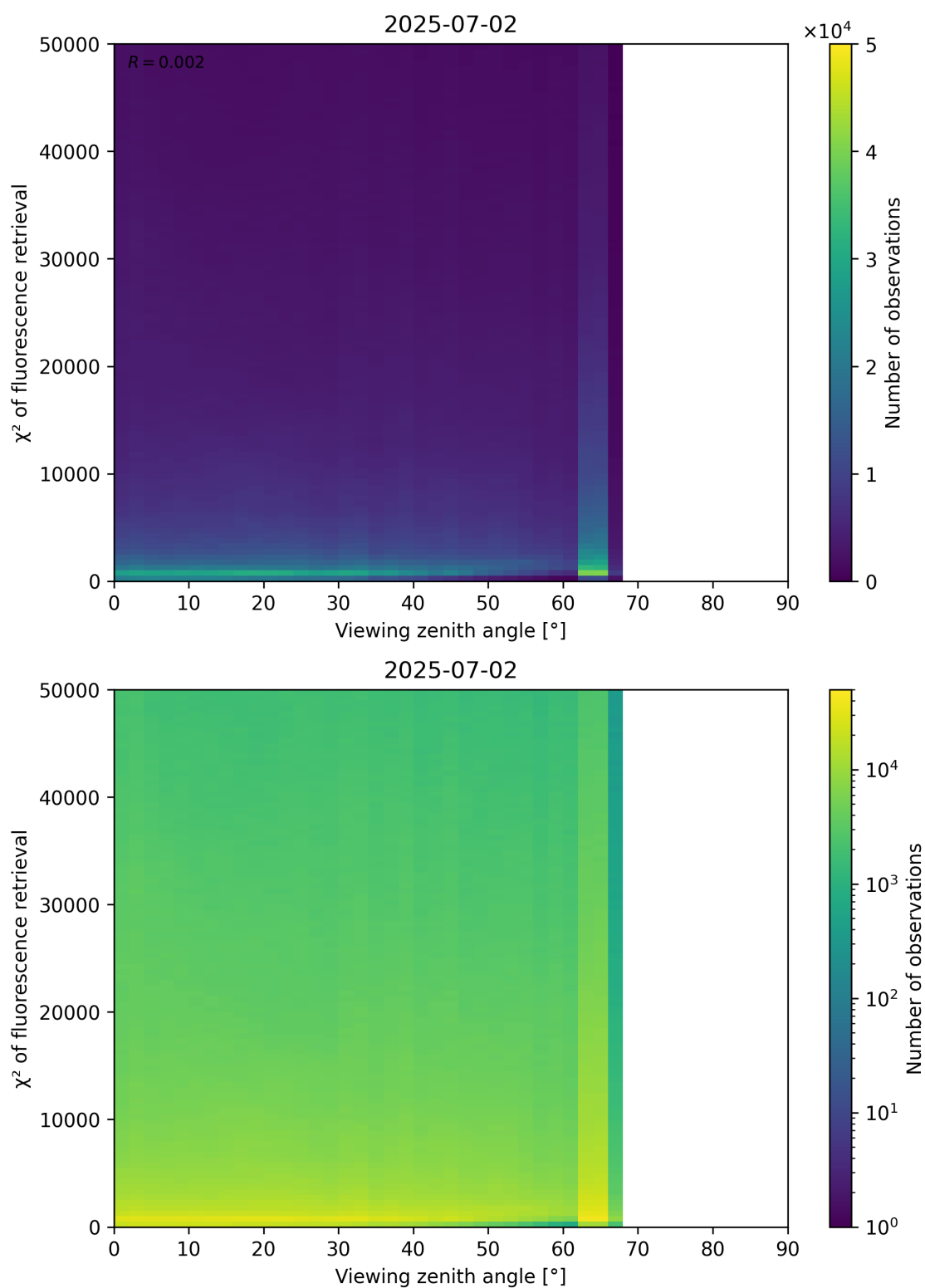
Figure 119: Scatter density plot of “Viewing zenith angle” against “ \chi^2 of fluorescence retrieval” for 2025-07-02 to 2025-07-03.
