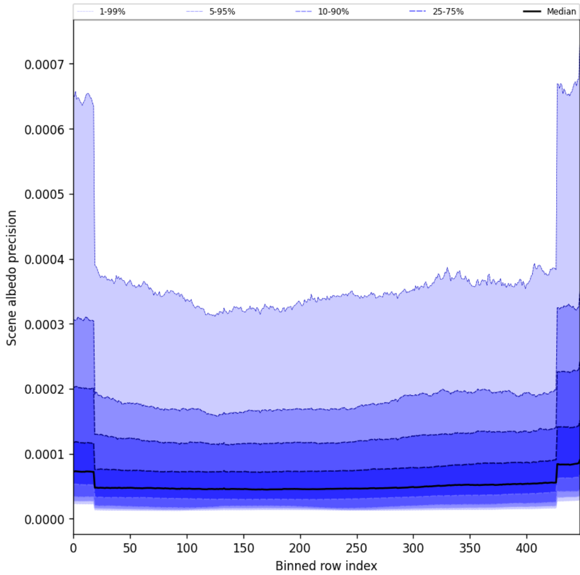
Figure 52: Along track statistics of “Scene albedo precision” for 2025-07-02 to 2025-07-03
