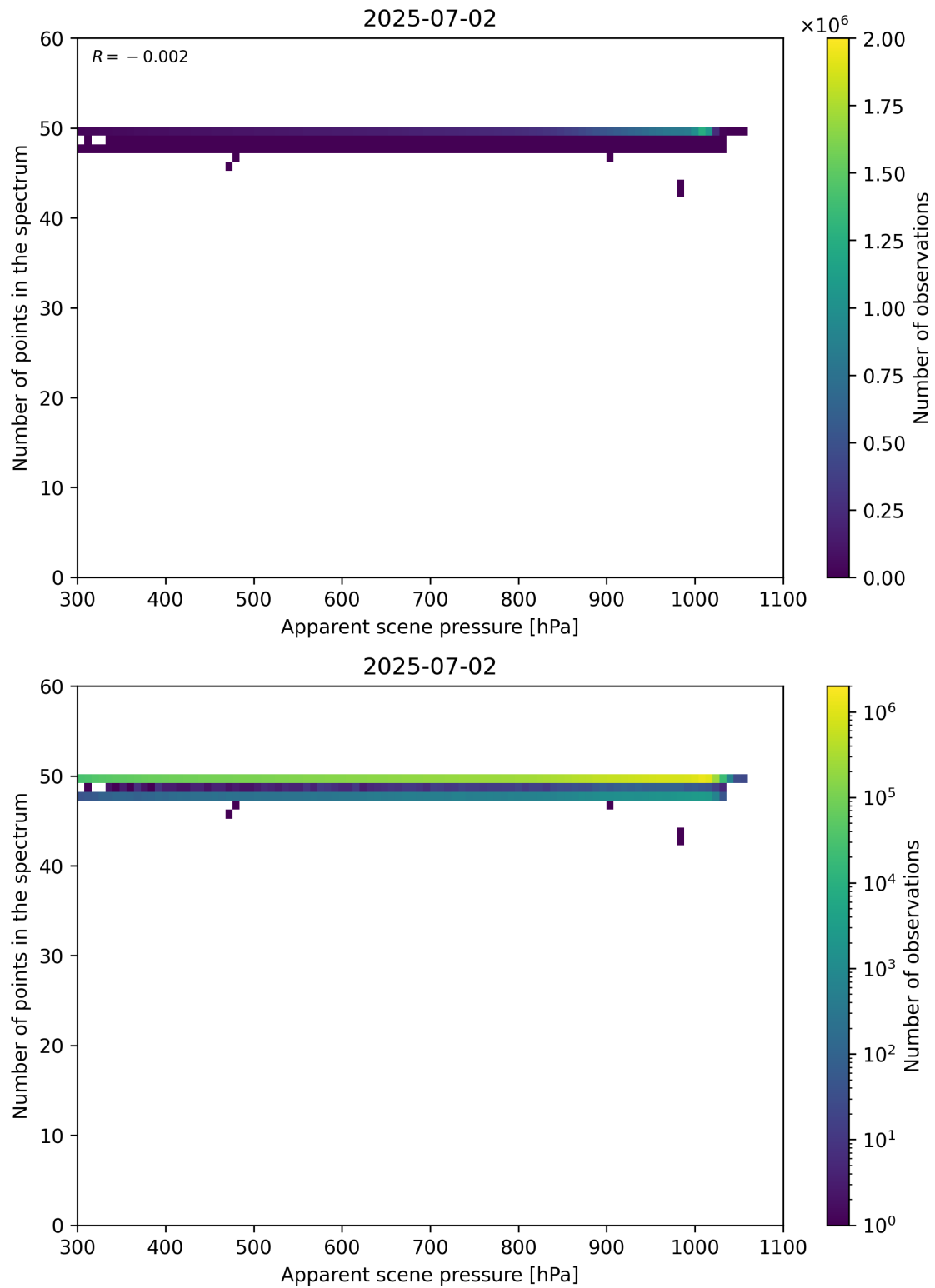
Figure 66: Scatter density plot of “Apparent scene pressure” against “Number of points in the spectrum” for 2025-07-02 to 2025-07-03.
