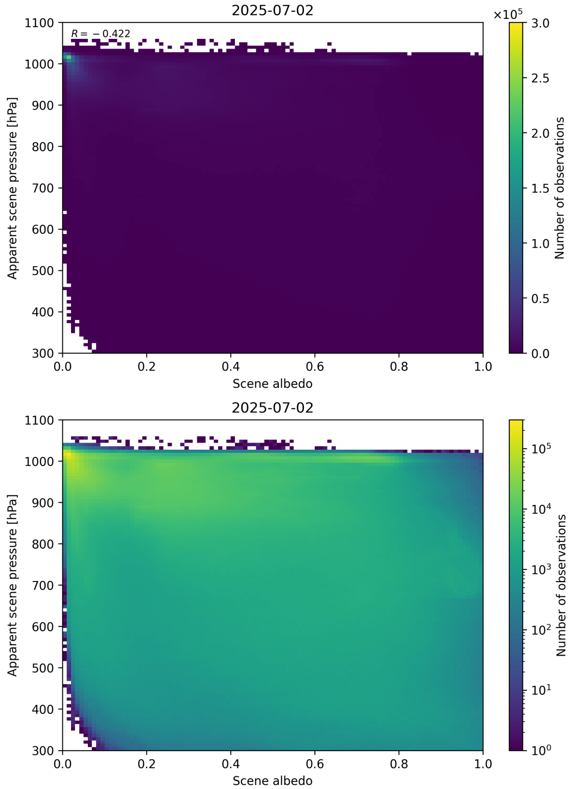
Figure 102: Scatter density plot of “Scene albedo” against “Apparent scene pressure” for 2025-07-02 to 2025-07-03.
