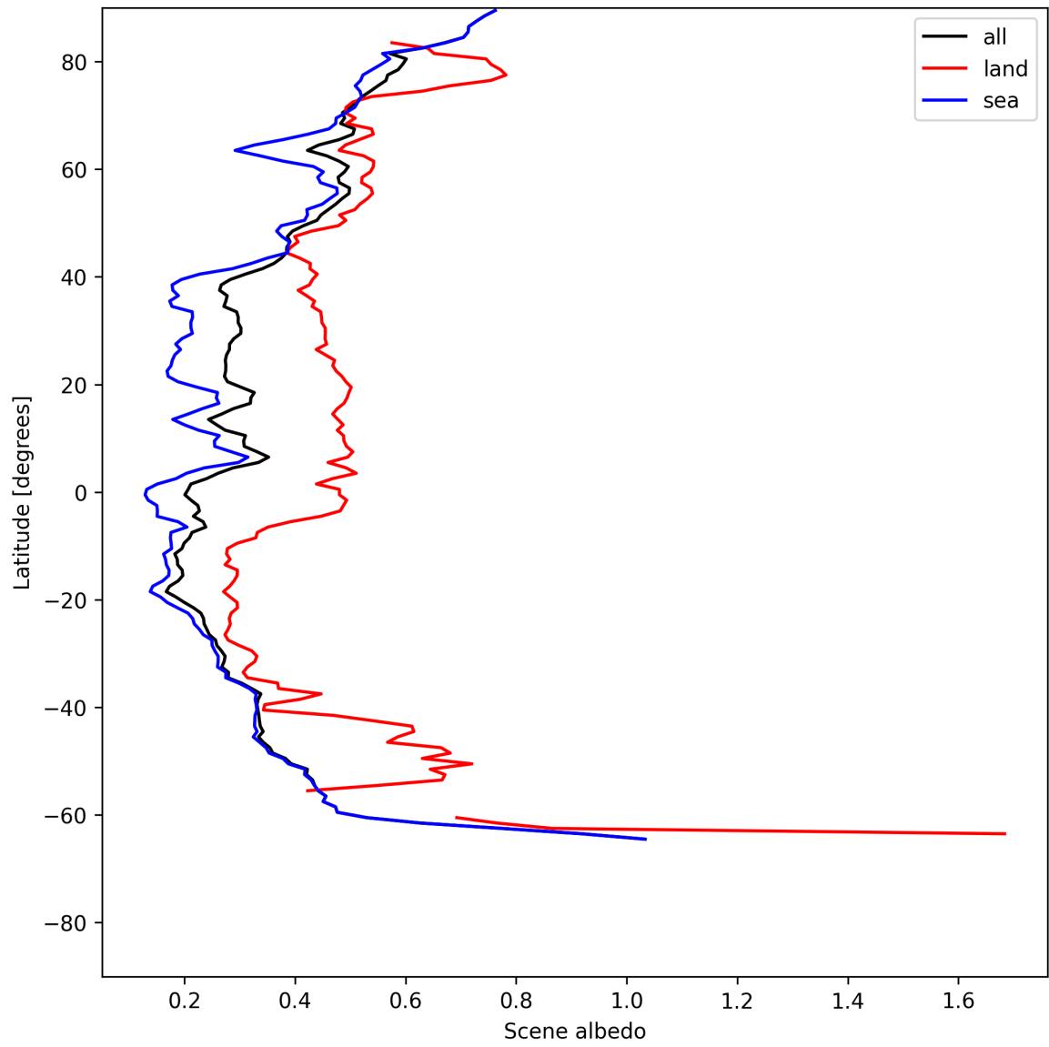
Figure 17: Zonal average of “Scene albedo” for 2025-07-02 to 2025-07-03.
