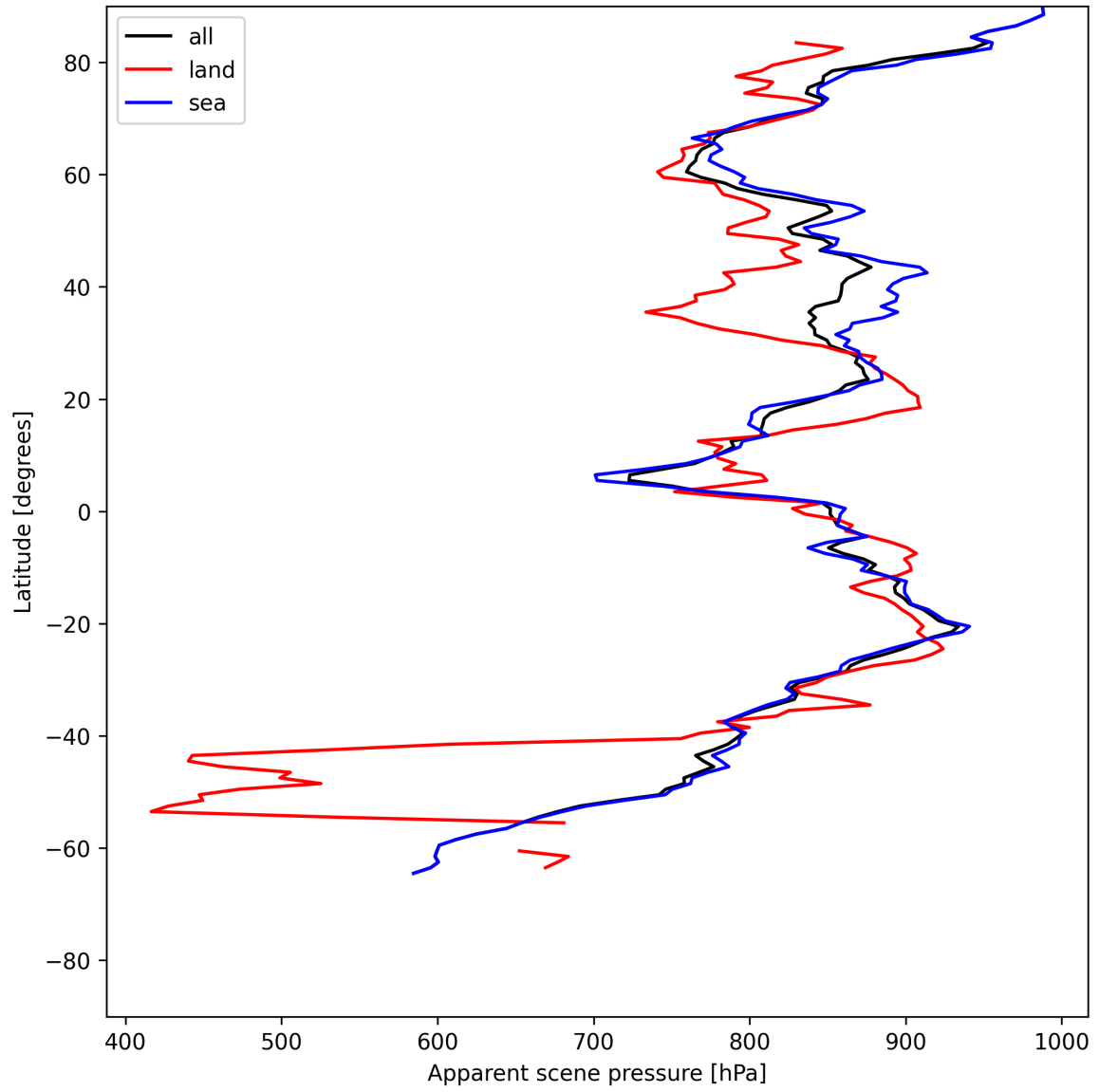
Figure 19: Zonal average of “Apparent scene pressure” for 2025-07-02 to 2025-07-03.
