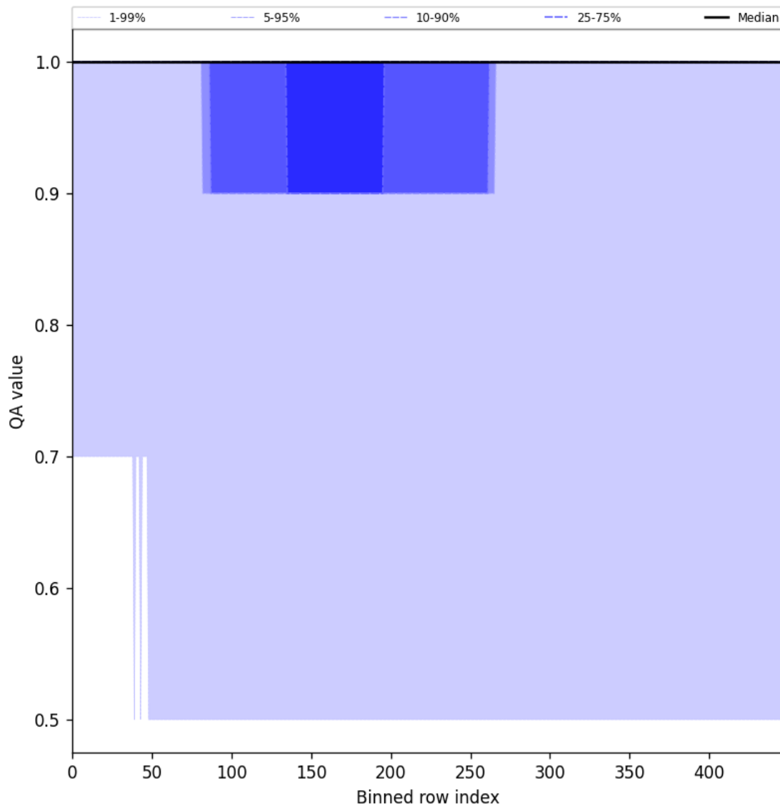
Figure 46: Along track statistics of “QA value” for 2025-07-02 to 2025-07-03
