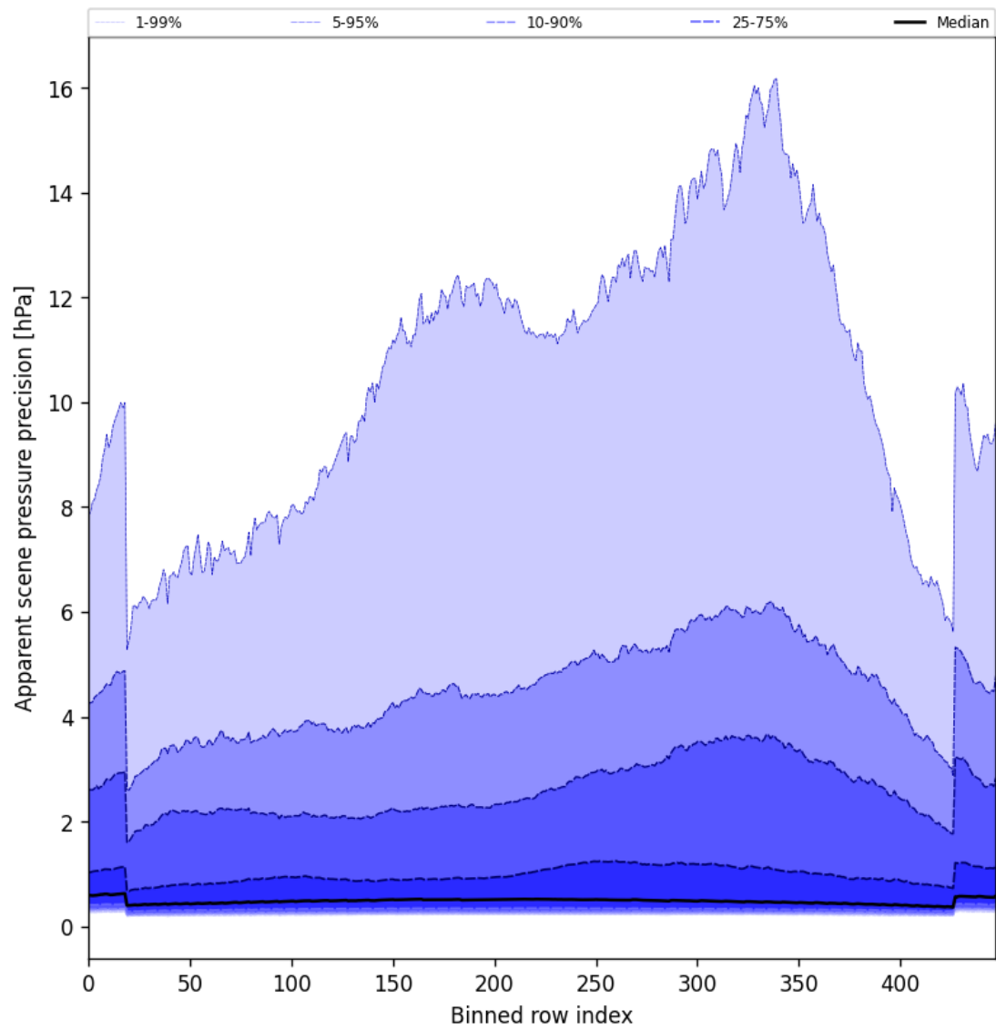
Figure 54: Along track statistics of “Apparent scene pressure precision” for 2025-07-02 to 2025-07-03
