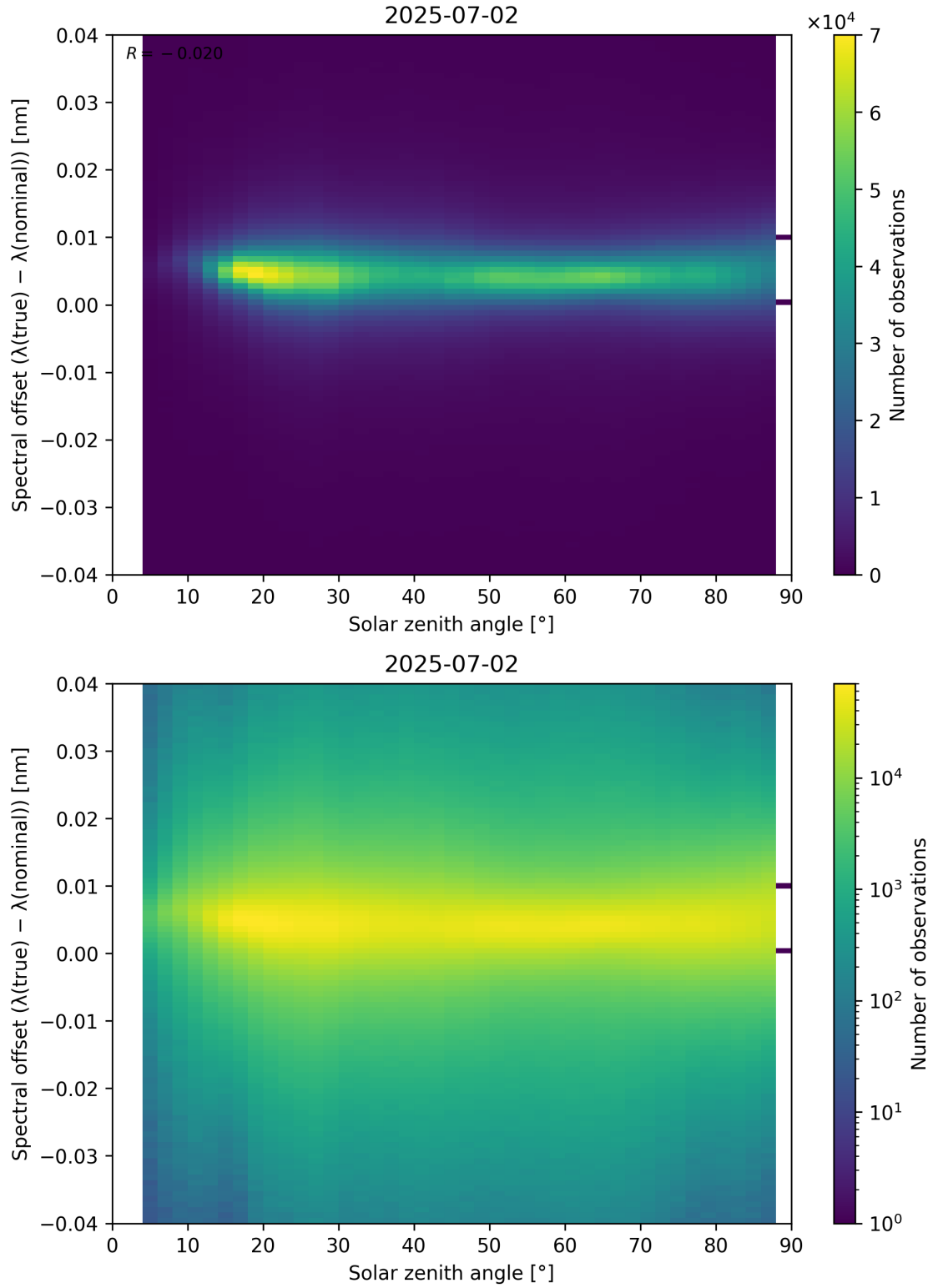
Figure 117: Scatter density plot of “Solar zenith angle” against “Spectral offset ( \lambda_{\text{true}} - \lambda_{\text{nominal}} )” for 2025-07-02 to 2025-07-03.
