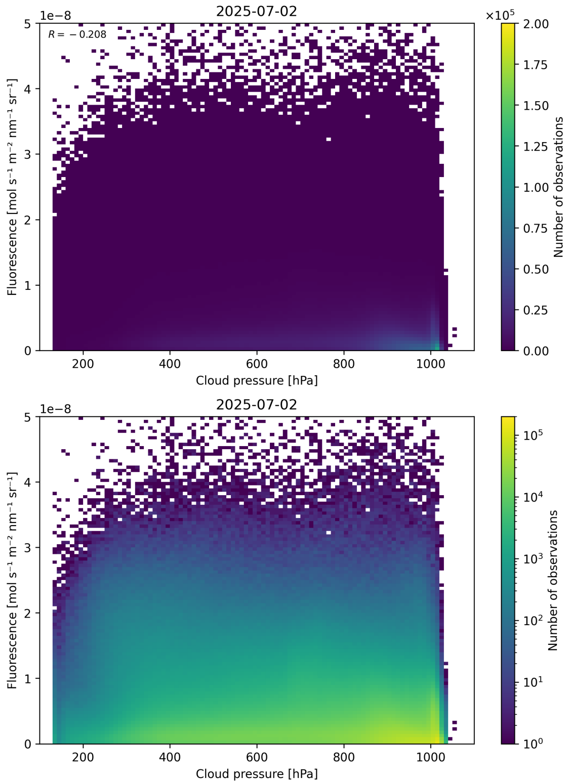
Figure 80: Scatter density plot of “Cloud pressure” against “Fluorescence” for 2025-07-02 to 2025-07-03.
