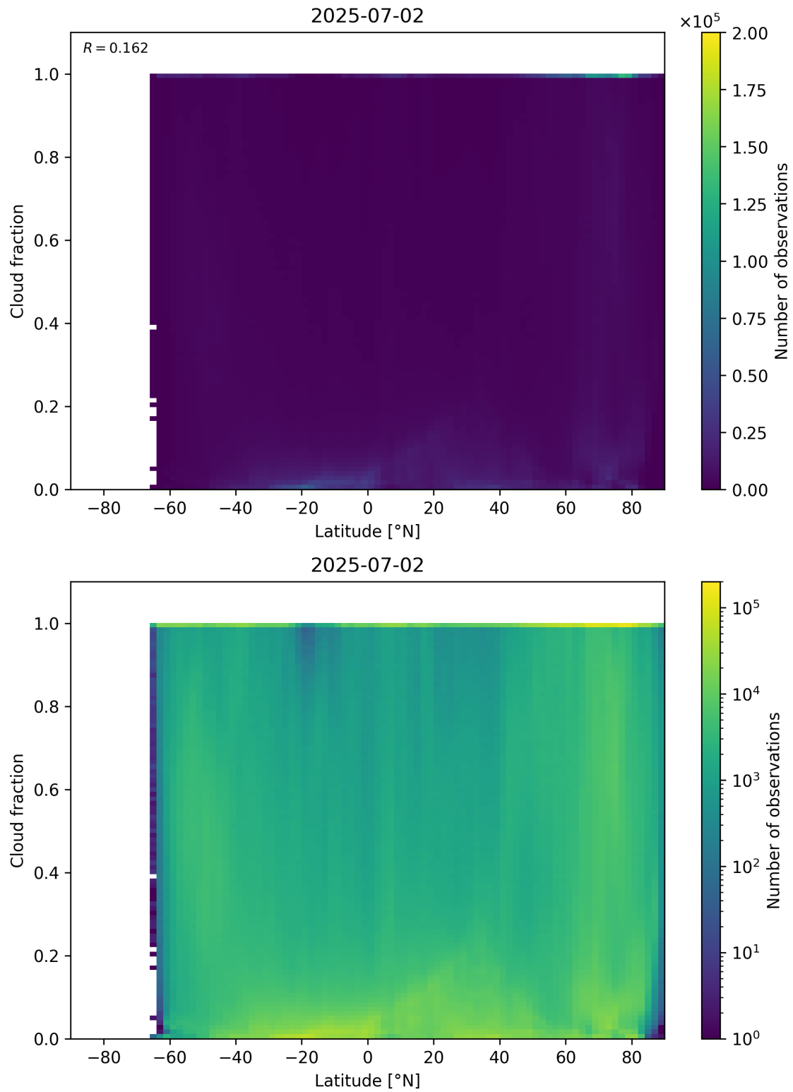
Figure 90: Scatter density plot of “Latitude” against “Cloud fraction” for 2025-07-02 to 2025-07-03.
