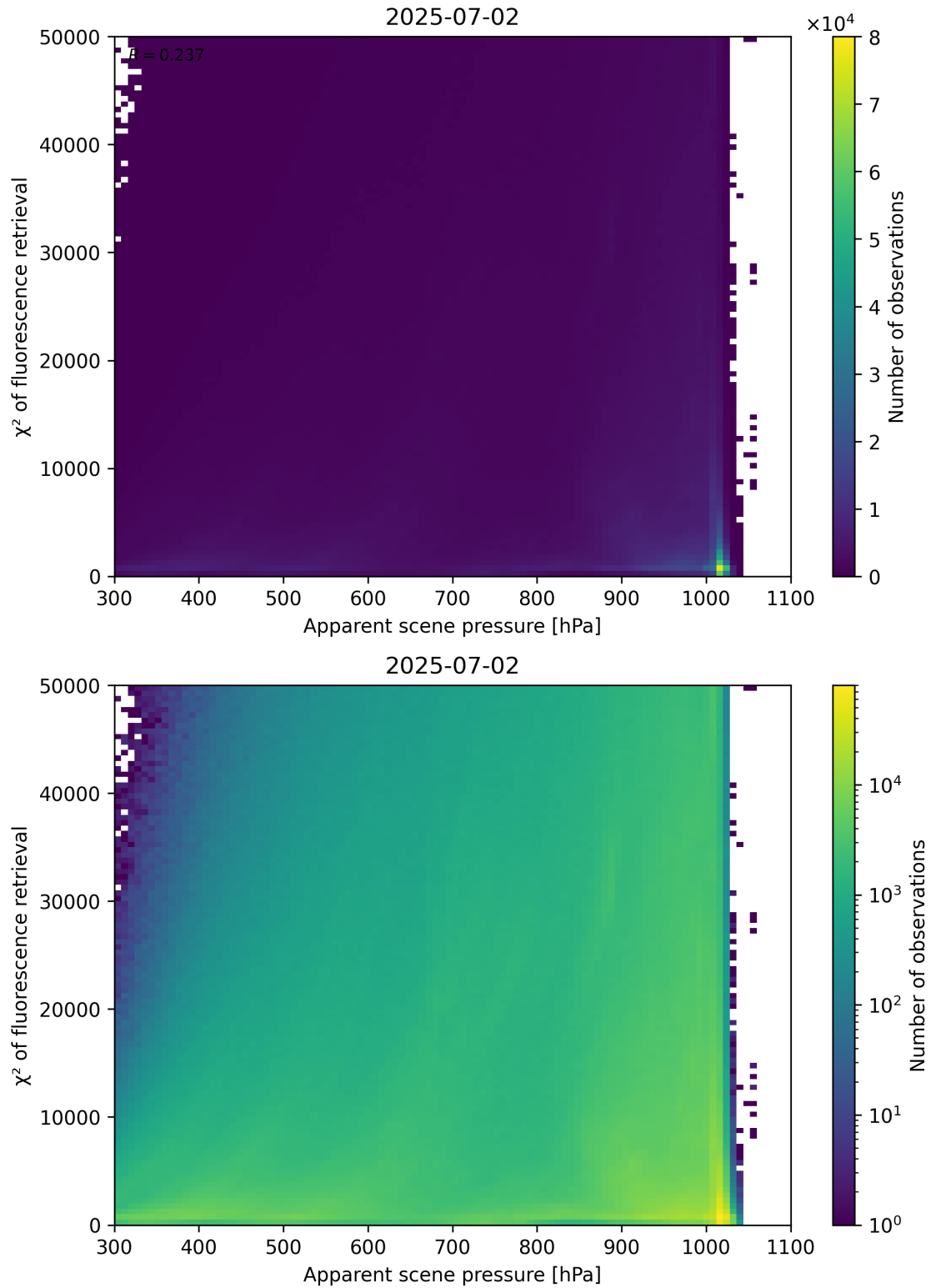
Figure 63: Scatter density plot of “Apparent scene pressure” against “ \chi^2 of fluorescence retrieval” for 2025-07-02 to 2025-07-03.
