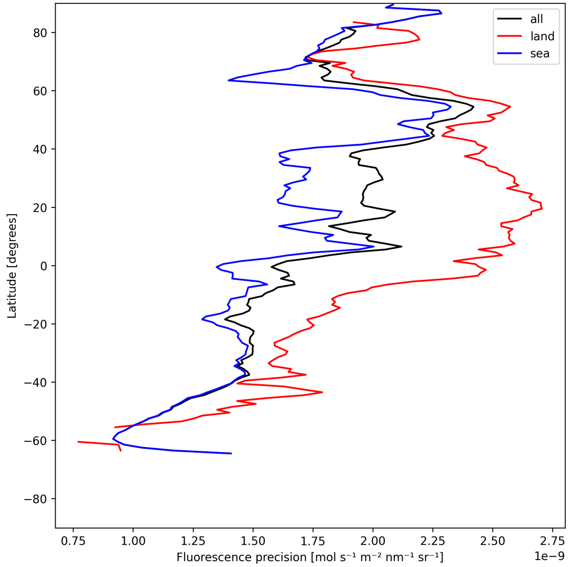
Figure 24: Zonal average of “Fluorescence precision” for 2025-07-02 to 2025-07-03.
