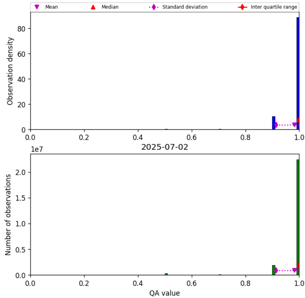
Figure 29: Histogram of “QA value” for 2025-07-02 to 2025-07-03
