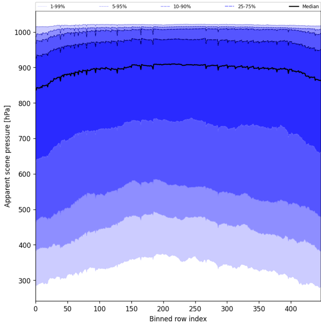
Figure 53: Along track statistics of “Apparent scene pressure” for 2025-07-02 to 2025-07-03
