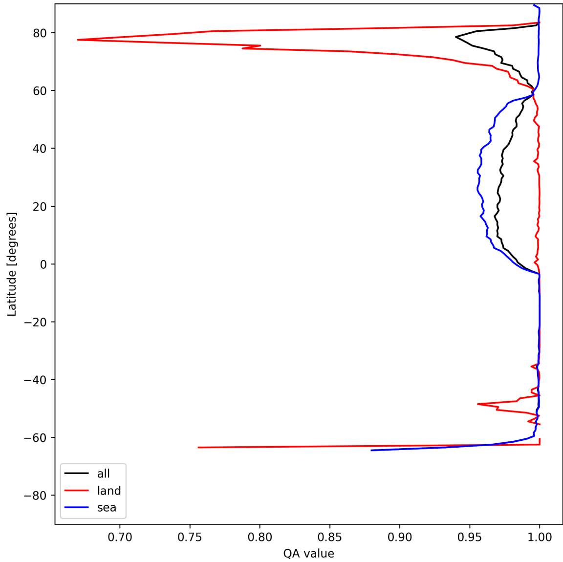
Figure 12: Zonal average of “QA value” for 2025-07-02 to 2025-07-03.
