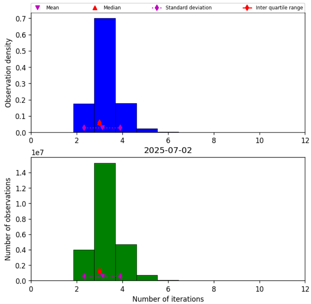
Figure 39: Histogram of “Number of iterations” for 2025-07-02 to 2025-07-03
