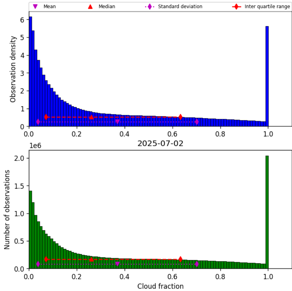
Figure 32: Histogram of “Cloud fraction” for 2025-07-02 to 2025-07-03
