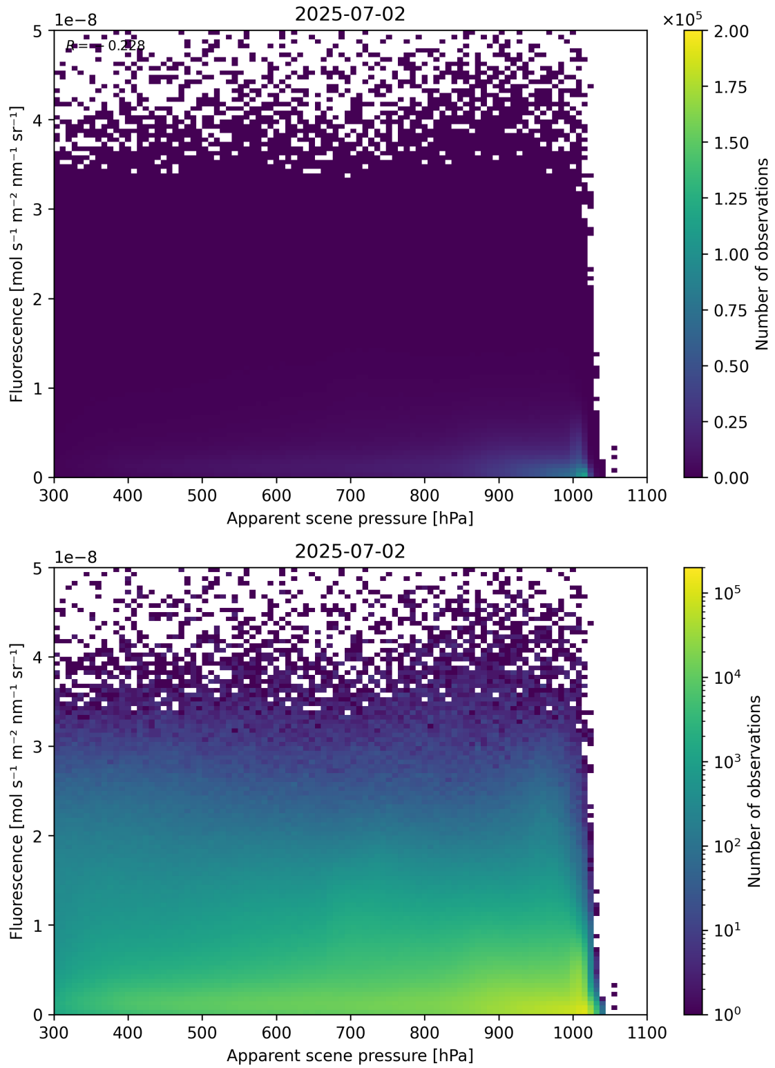
Figure 64: Scatter density plot of “Apparent scene pressure” against “Fluorescence” for 2025-07-02 to 2025-07-03.
