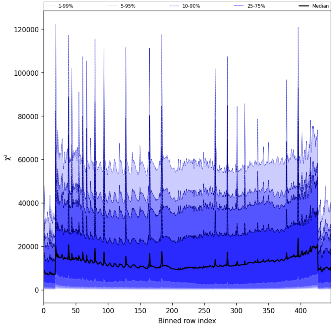
Figure 55: Along track statistics of “ \chi^2 ” for 2025-07-02 to 2025-07-03
