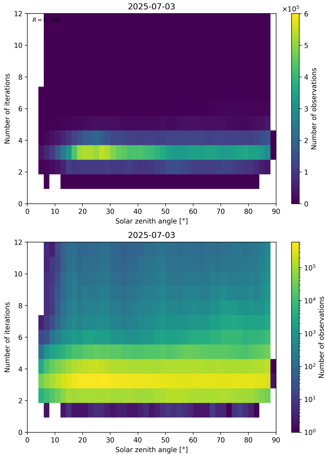
Figure 114: Scatter density plot of “Solar zenith angle” against “Number of iterations” for 2025-07-03 to 2025-07-04.
