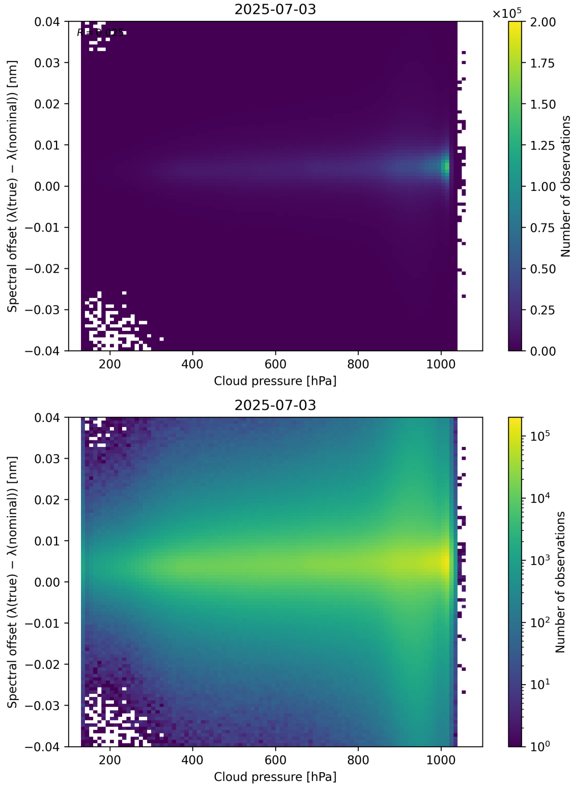
Figure 84: Scatter density plot of “Cloud pressure” against “Spectral offset ( \lambda_{\text{true}} - \lambda_{\text{nominal}} )” for 2025-07-03 to 2025-07-04.
