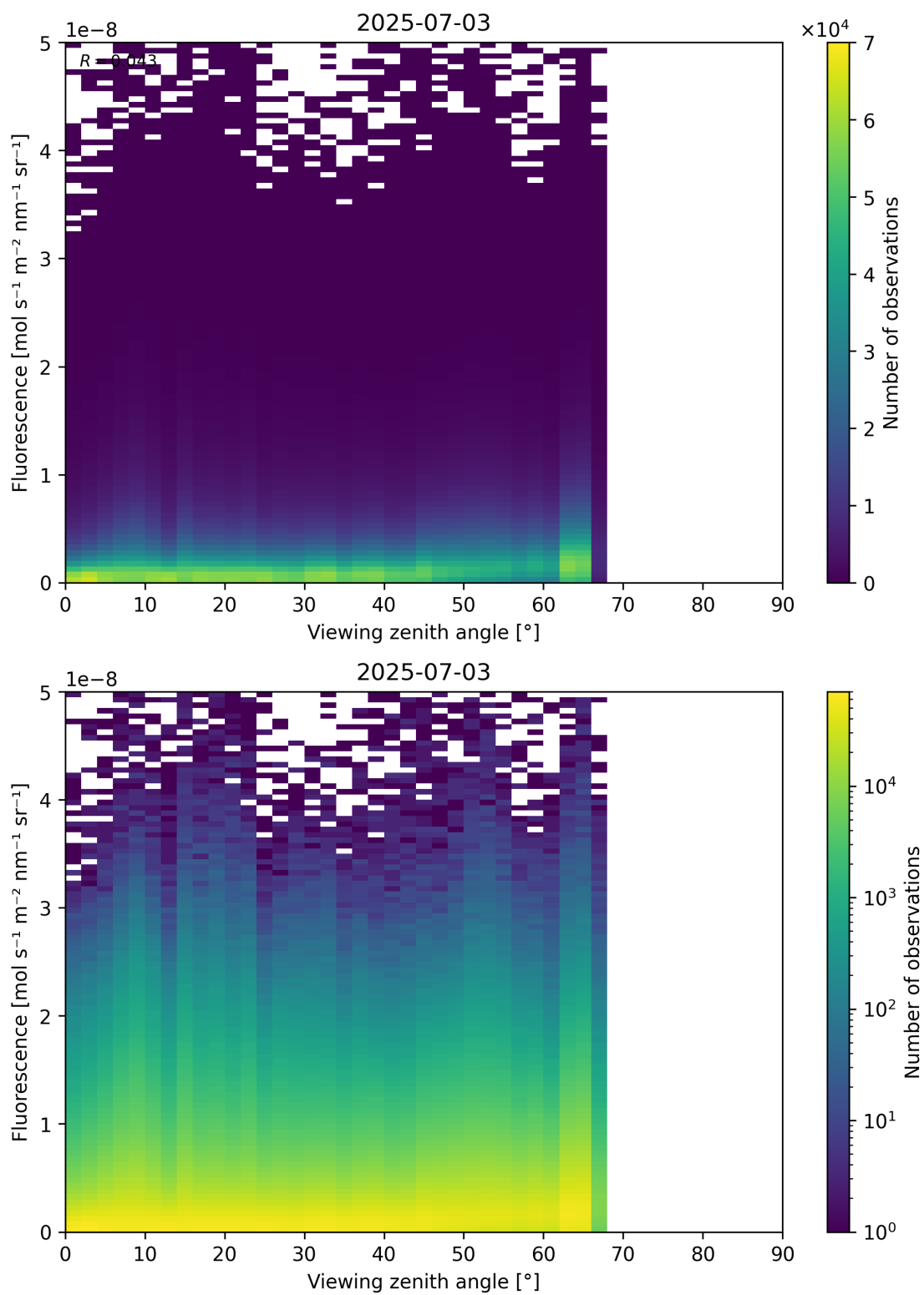
Figure 122: Scatter density plot of “Viewing zenith angle” against “Fluorescence” for 2025-07-03 to 2025-07-04.
