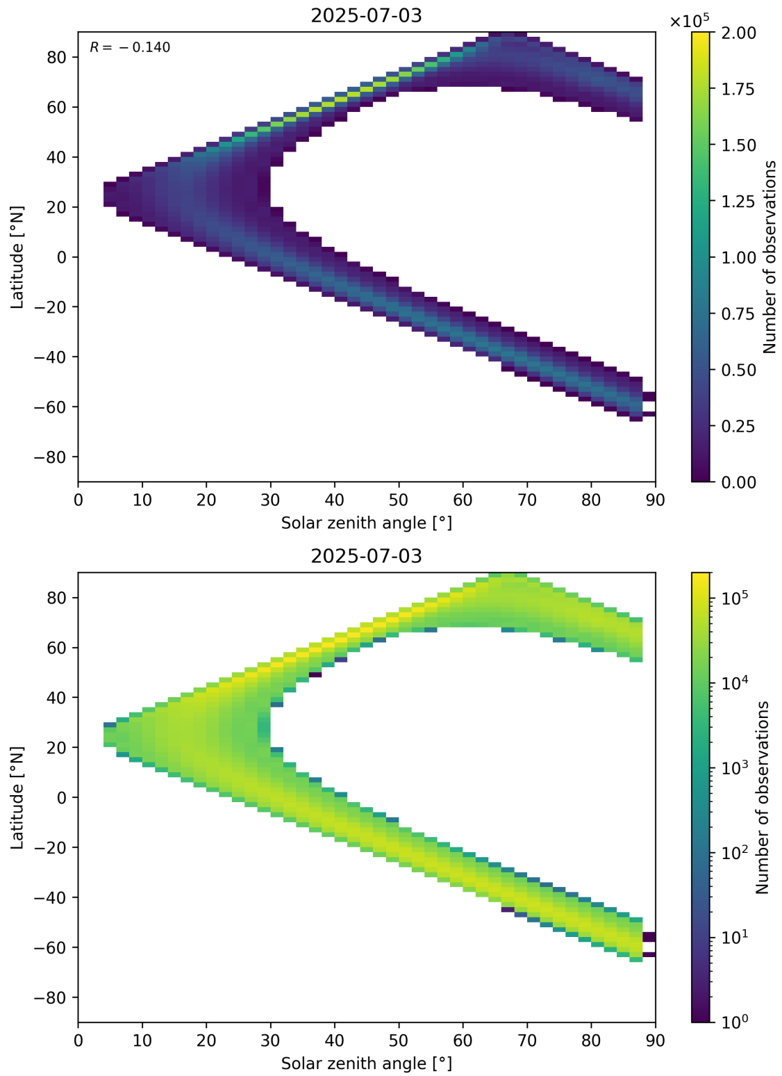
Figure 113: Scatter density plot of “Solar zenith angle” against “Latitude” for 2025-07-03 to 2025-07-04.
