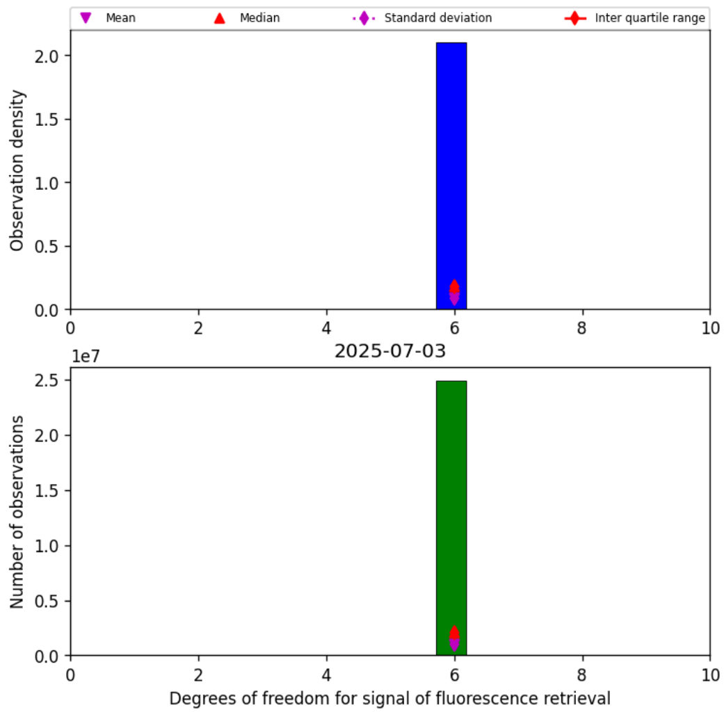
Figure 43: Histogram of “Degrees of freedom for signal of fluorescence retrieval” for 2025-07-03 to 2025-07-04
