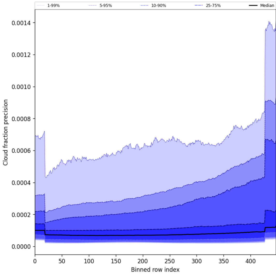
Figure 50: Along track statistics of “Cloud fraction precision” for 2025-07-03 to 2025-07-04
