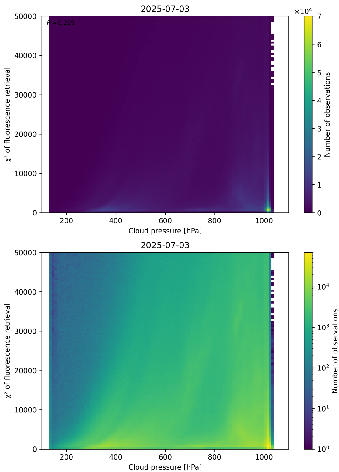
Figure 78: Scatter density plot of “Cloud pressure” against “ \chi^2 of fluorescence retrieval” for 2025-07-03 to 2025-07-04.
