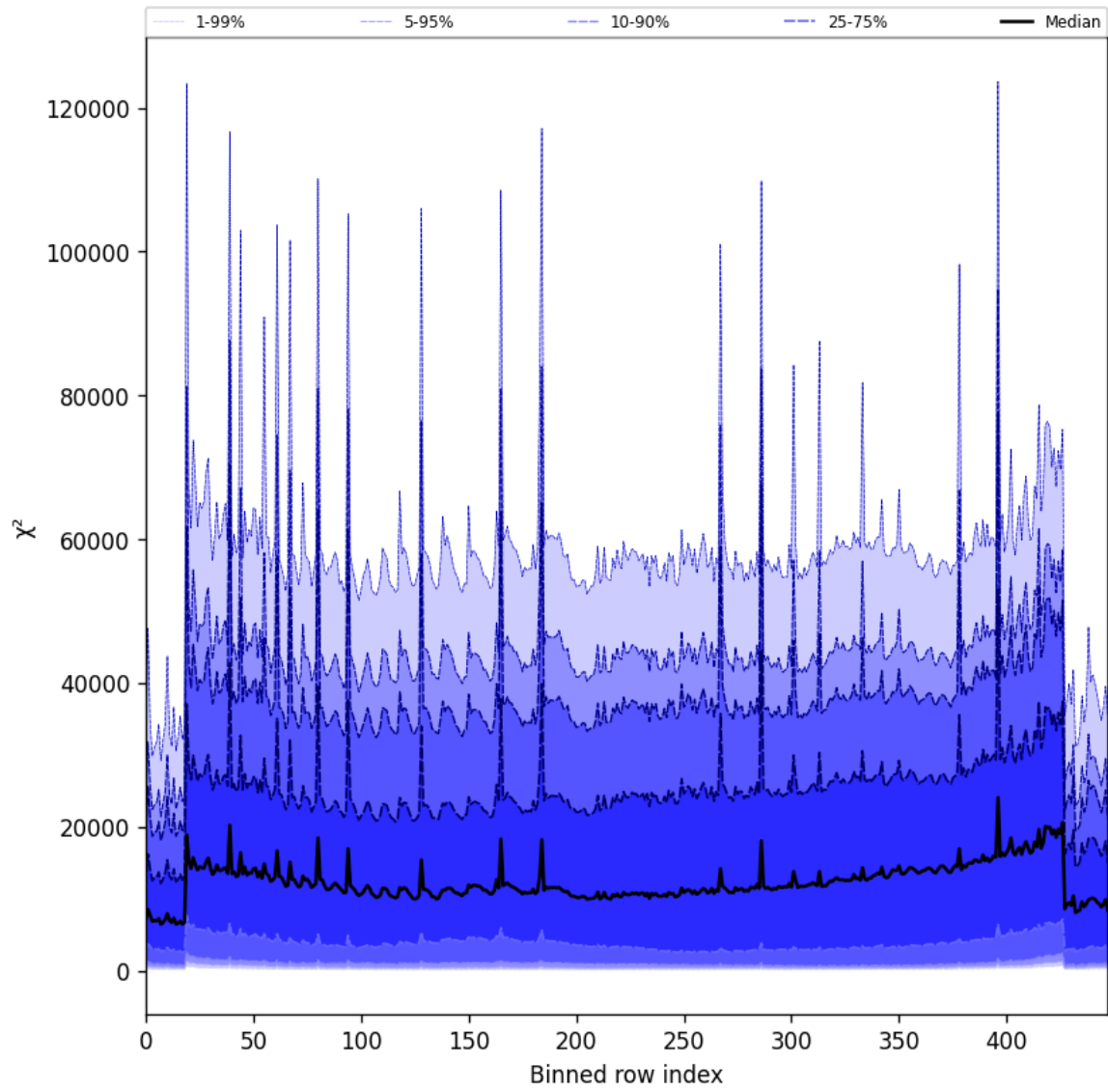
Figure 55: Along track statistics of “ \chi^2 ” for 2025-07-03 to 2025-07-04
