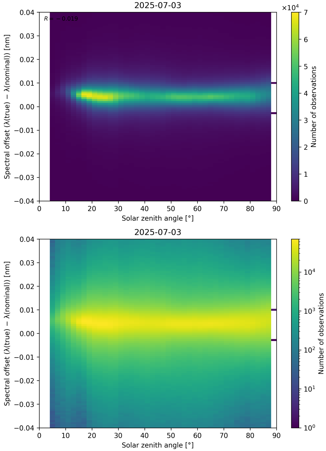
Figure 117: Scatter density plot of “Solar zenith angle” against “Spectral offset ( \lambda_{\text{true}} - \lambda_{\text{nominal}} )” for 2025-07-03 to 2025-07-04.
