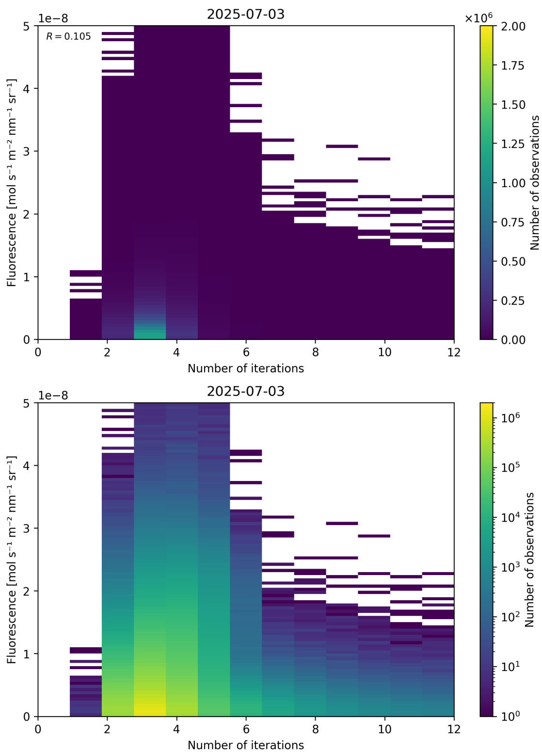
Figure 98: Scatter density plot of “Number of iterations” against “Fluorescence” for 2025-07-03 to 2025-07-04.
