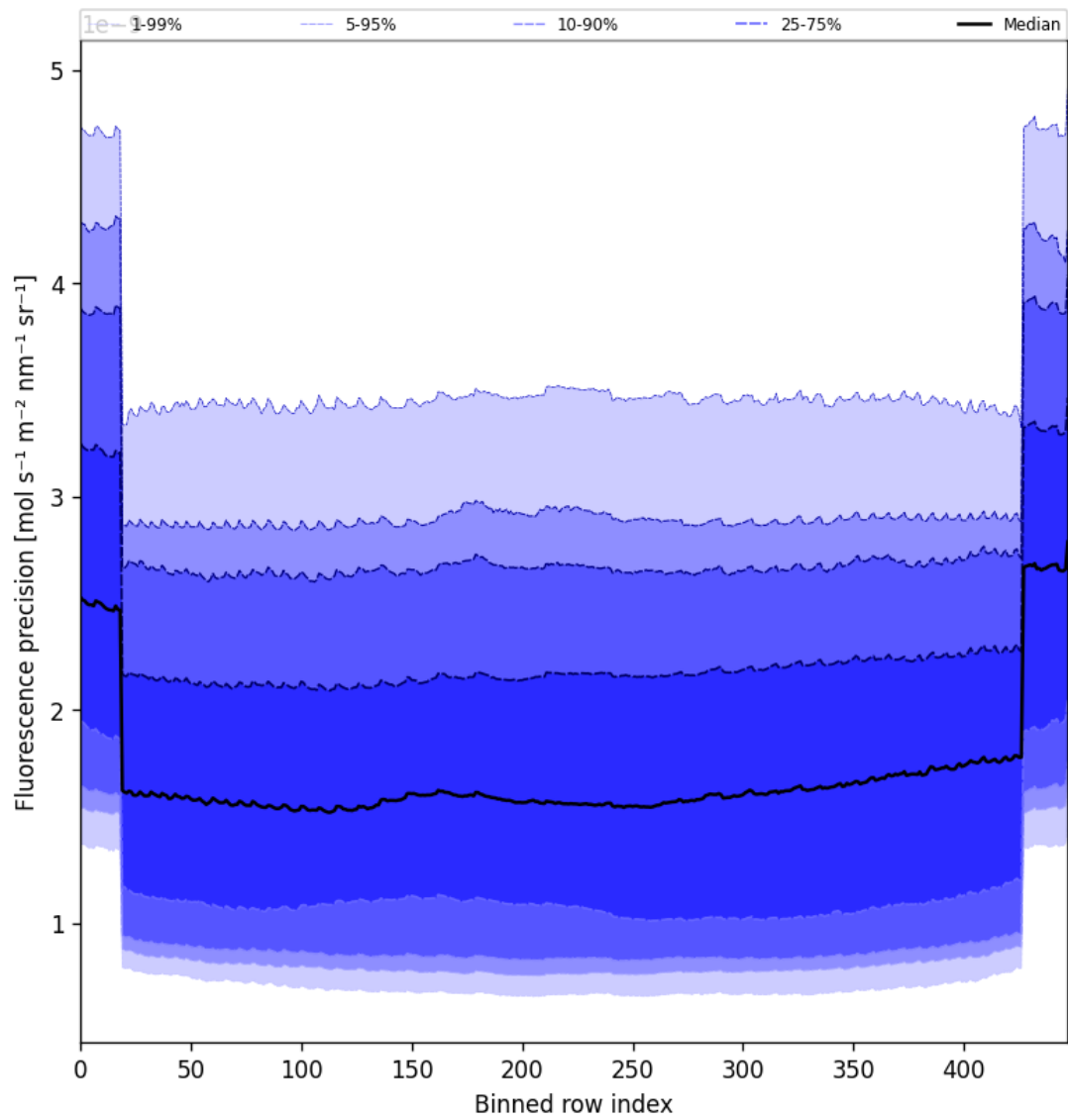
Figure 58: Along track statistics of "Fluorescence precision" for 2025-07-03 to 2025-07-04
