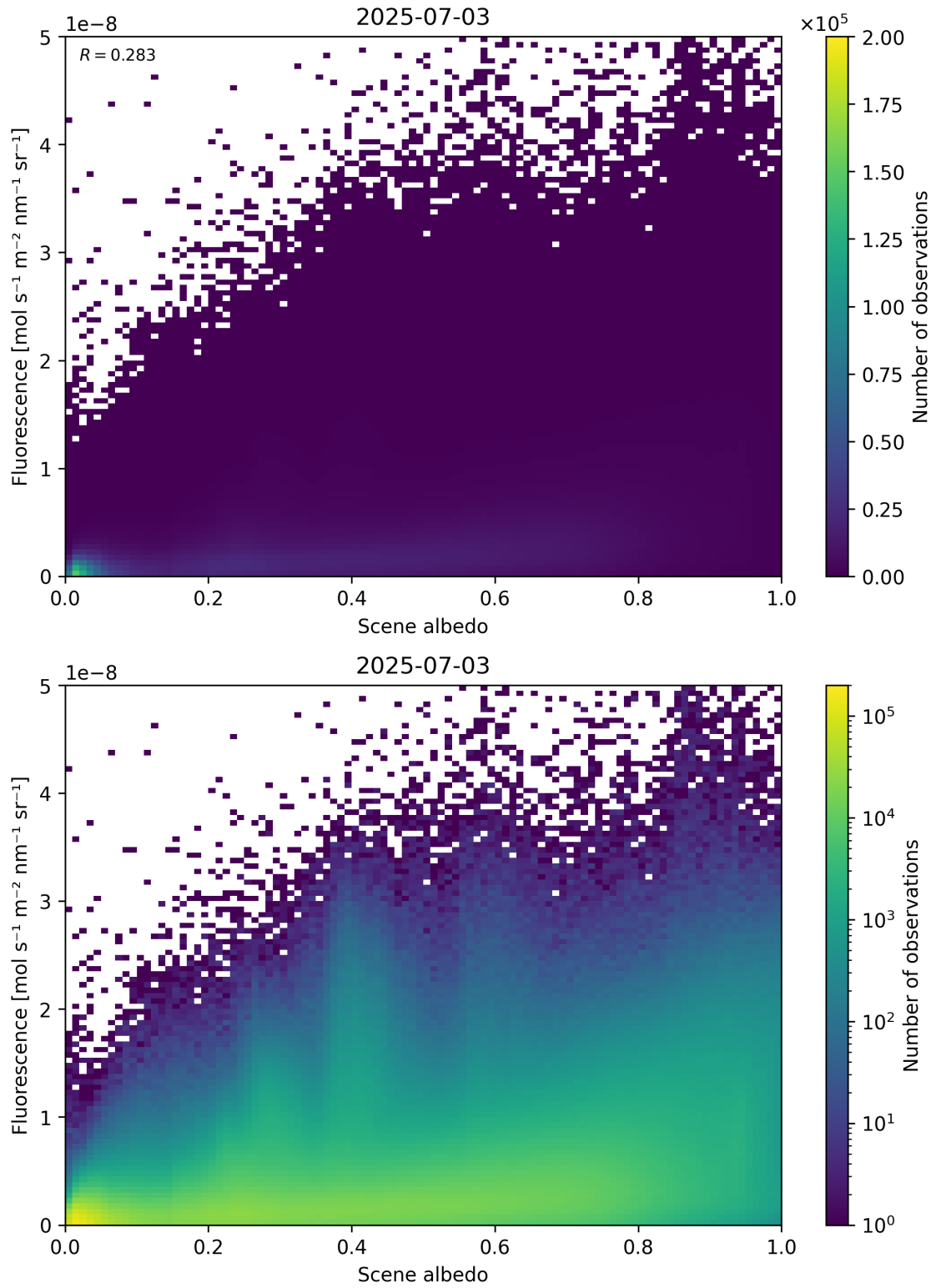
Figure 104: Scatter density plot of “Scene albedo” against “Fluorescence” for 2025-07-03 to 2025-07-04.
