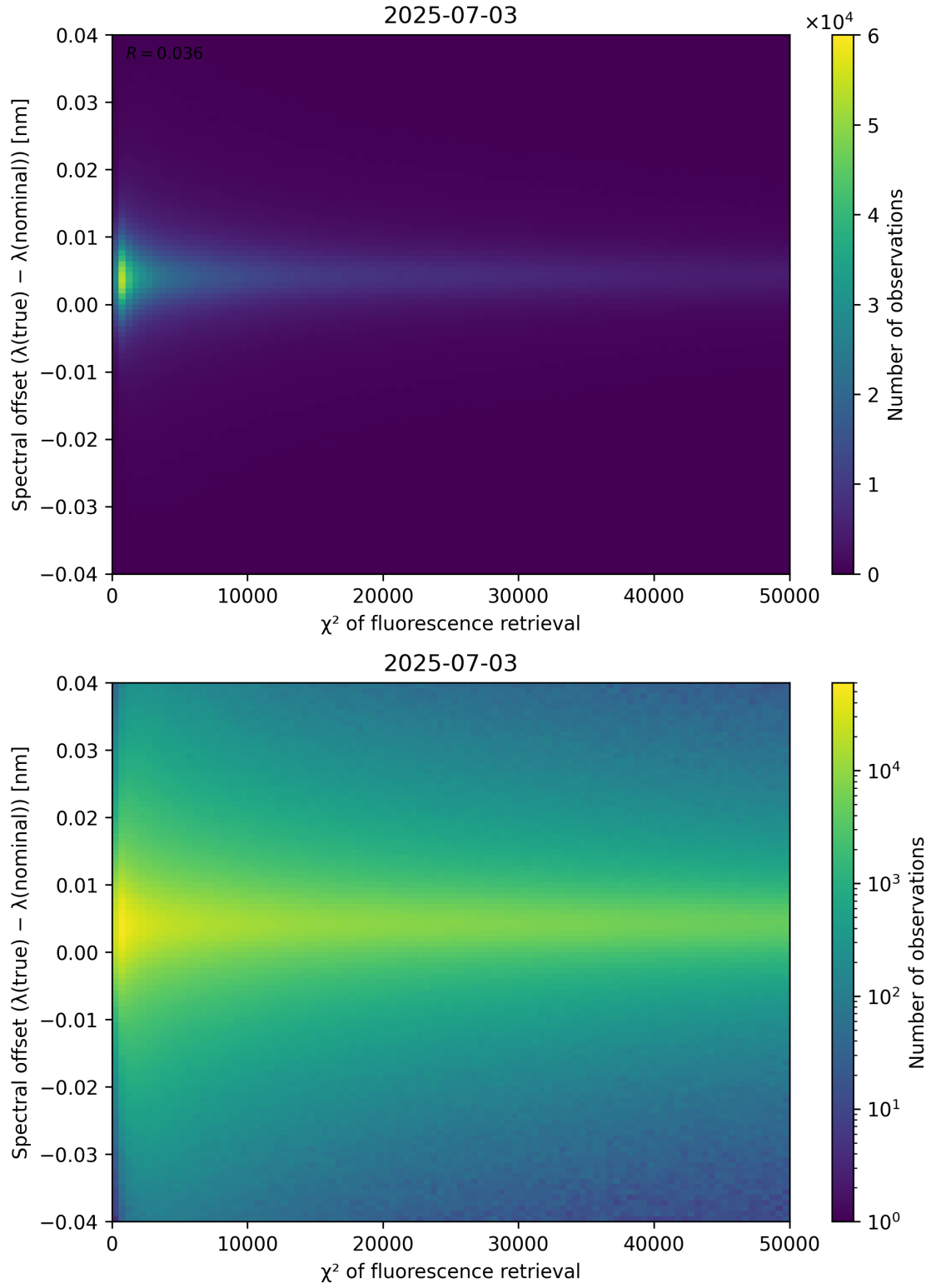
Figure 69: Scatter density plot of “ \chi^2 of fluorescence retrieval” against “Spectral offset ( \lambda_{\text{true}} - \lambda_{\text{nominal}} )” for 2025-07-03 to 2025-07-04.
