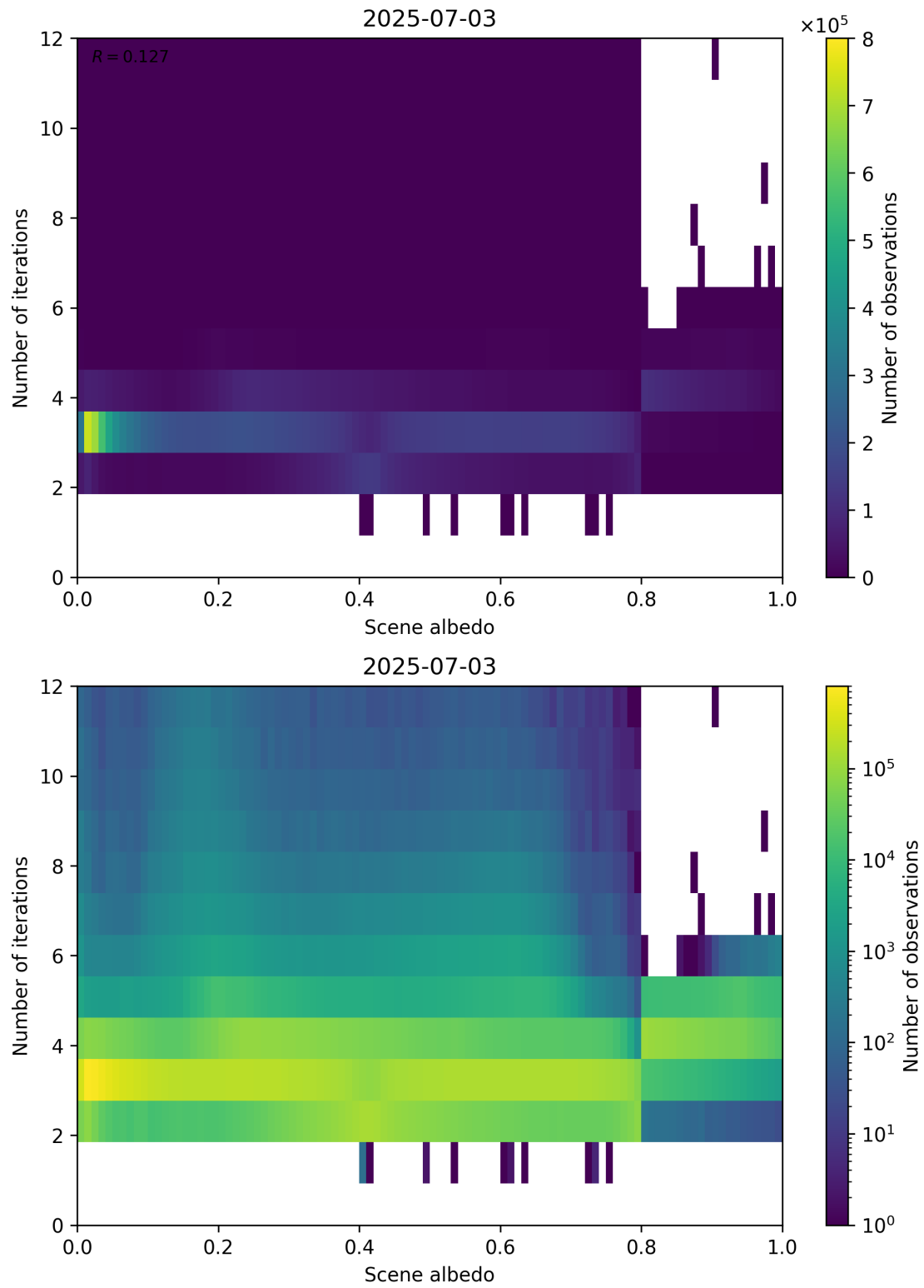
Figure 105: Scatter density plot of “Scene albedo” against “Number of iterations” for 2025-07-03 to 2025-07-04.
