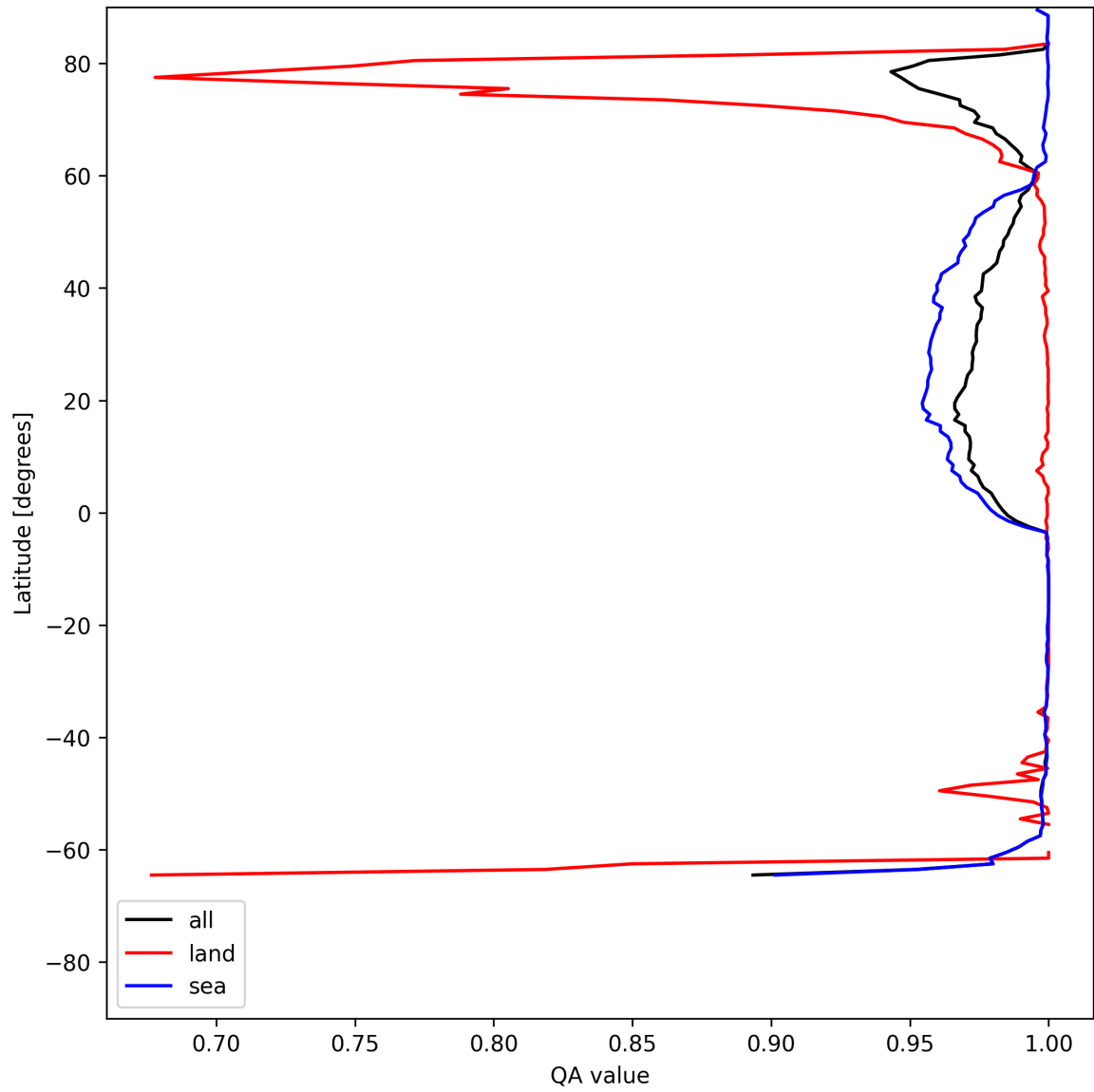
Figure 12: Zonal average of “QA value” for 2025-07-03 to 2025-07-04.
