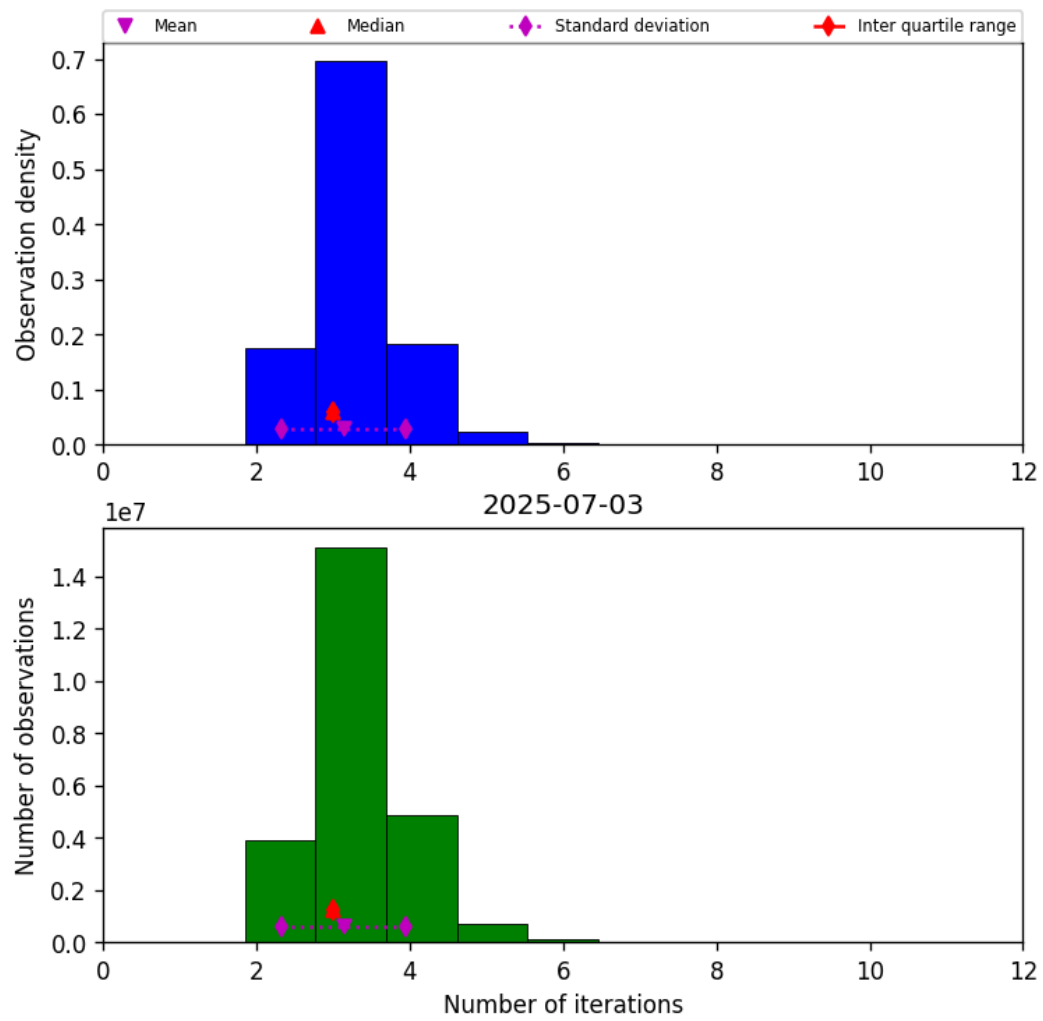
Figure 39: Histogram of “Number of iterations” for 2025-07-03 to 2025-07-04
