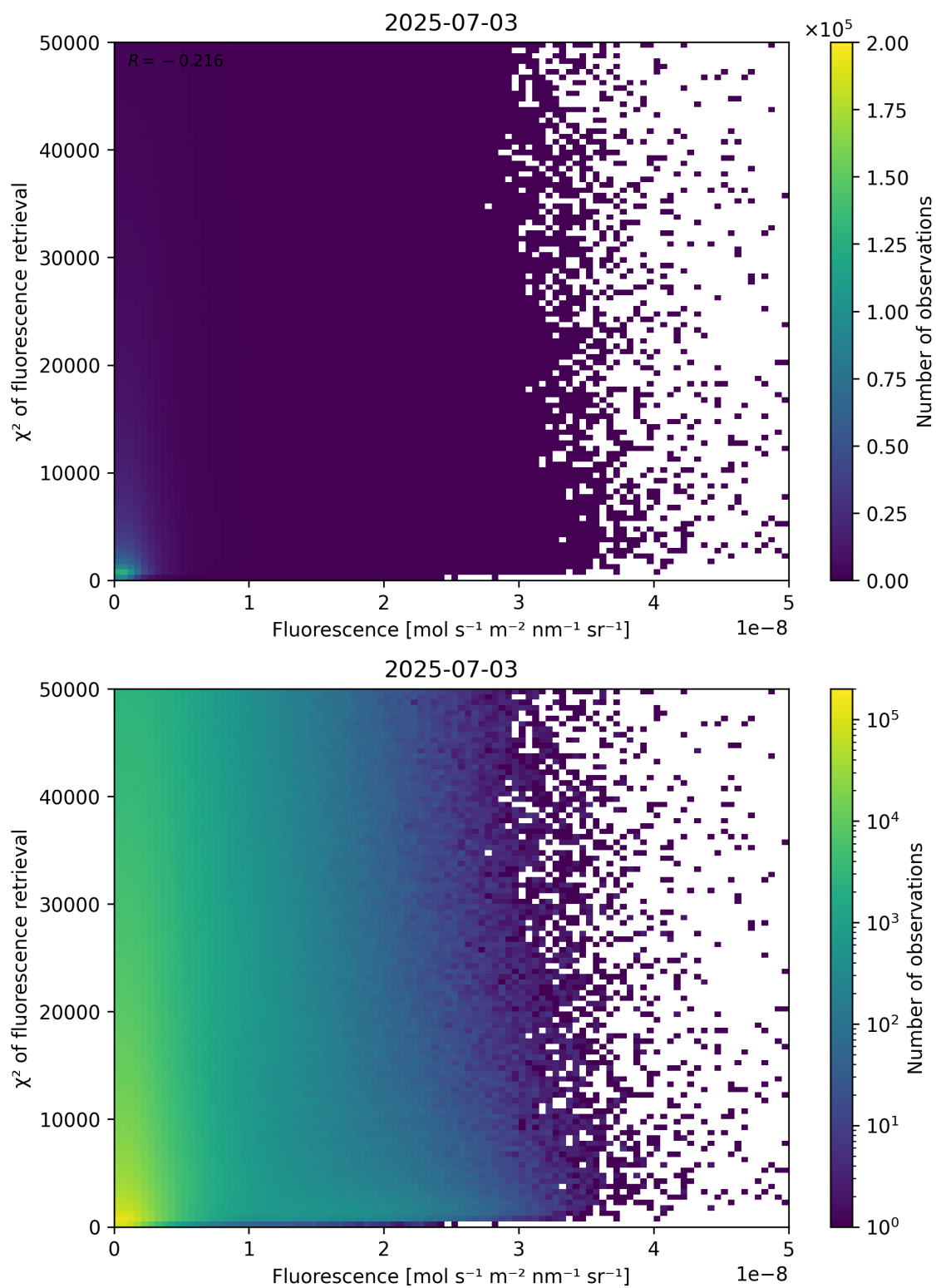
Figure 85: Scatter density plot of “Fluorescence” against “ \chi^2 of fluorescence retrieval” for 2025-07-03 to 2025-07-04.
