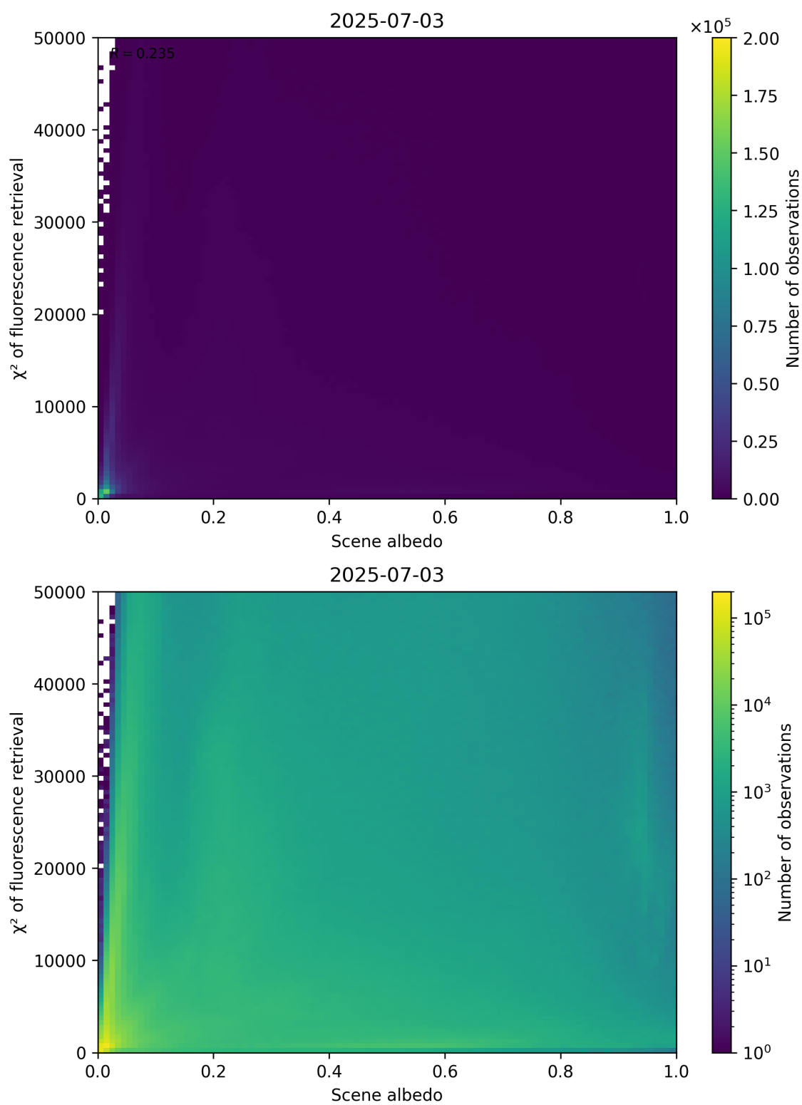
Figure 103: Scatter density plot of “Scene albedo” against “ \chi^2 of fluorescence retrieval” for 2025-07-03 to 2025-07-04.
