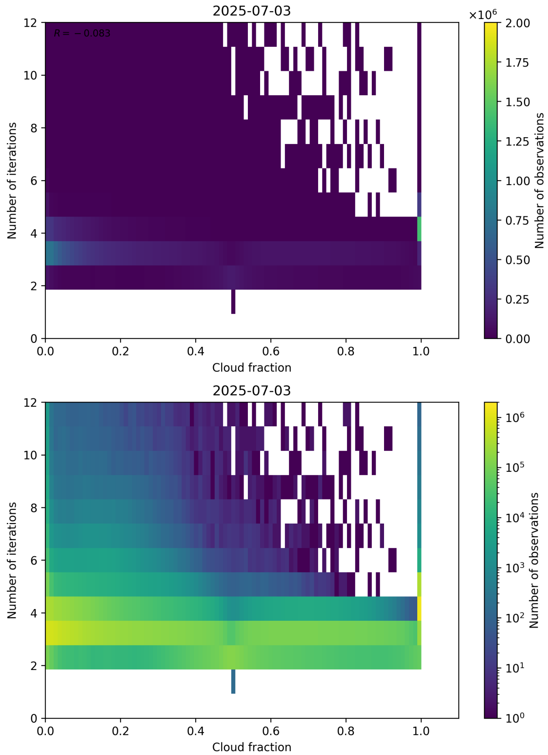
Figure 73: Scatter density plot of “Cloud fraction” against “Number of iterations” for 2025-07-03 to 2025-07-04.
