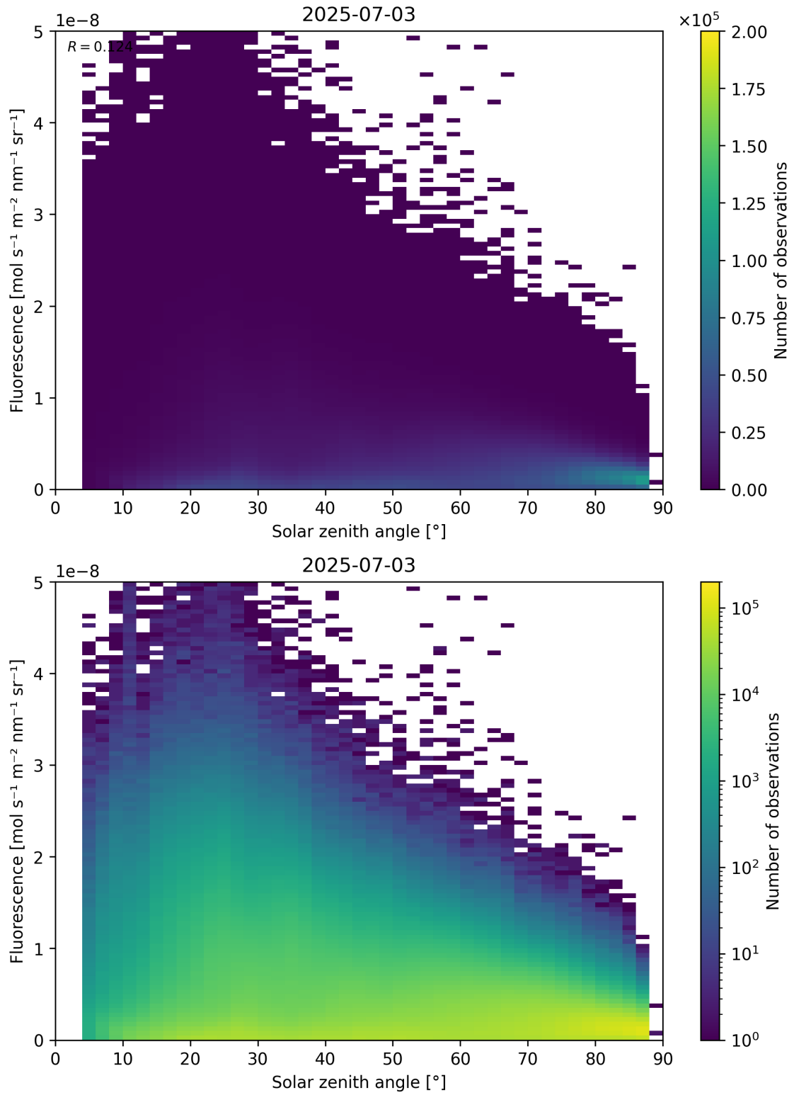
Figure 112: Scatter density plot of “Solar zenith angle” against “Fluorescence” for 2025-07-03 to 2025-07-04.
