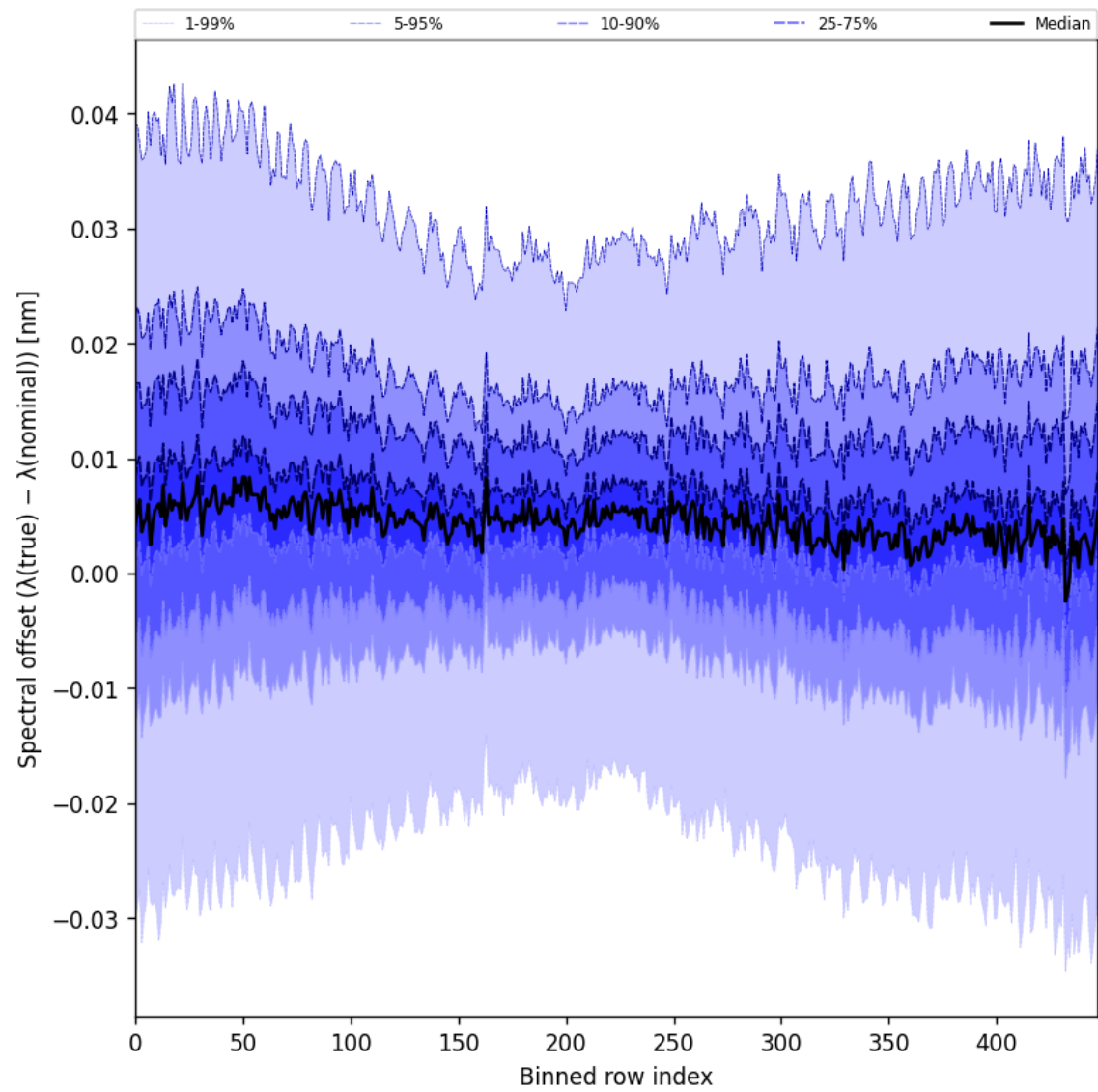
Figure 62: Along track statistics of “Spectral offset ( \lambda_{\text{true}} - \lambda_{\text{nominal}} )” for 2025-07-03 to 2025-07-04
