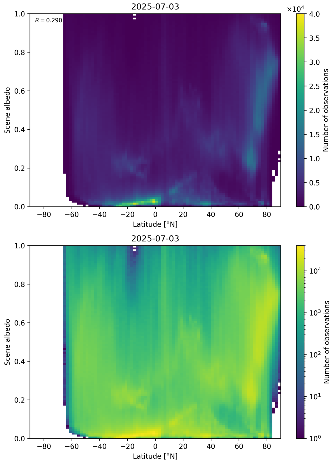
Figure 95: Scatter density plot of “Latitude” against “Scene albedo” for 2025-07-03 to 2025-07-04.
