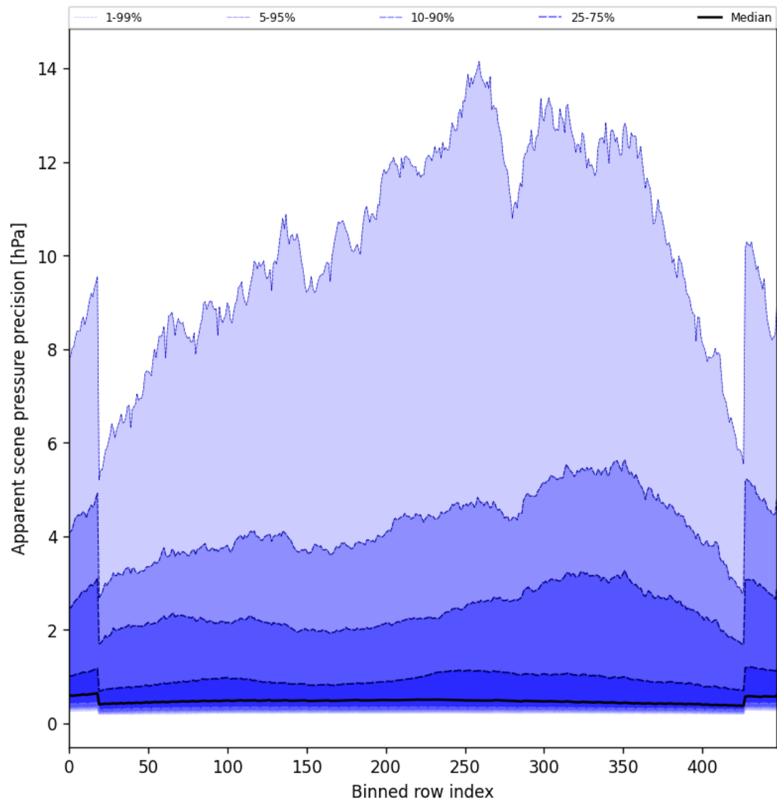
Figure 54: Along track statistics of “Apparent scene pressure precision” for 2025-07-03 to 2025-07-04
