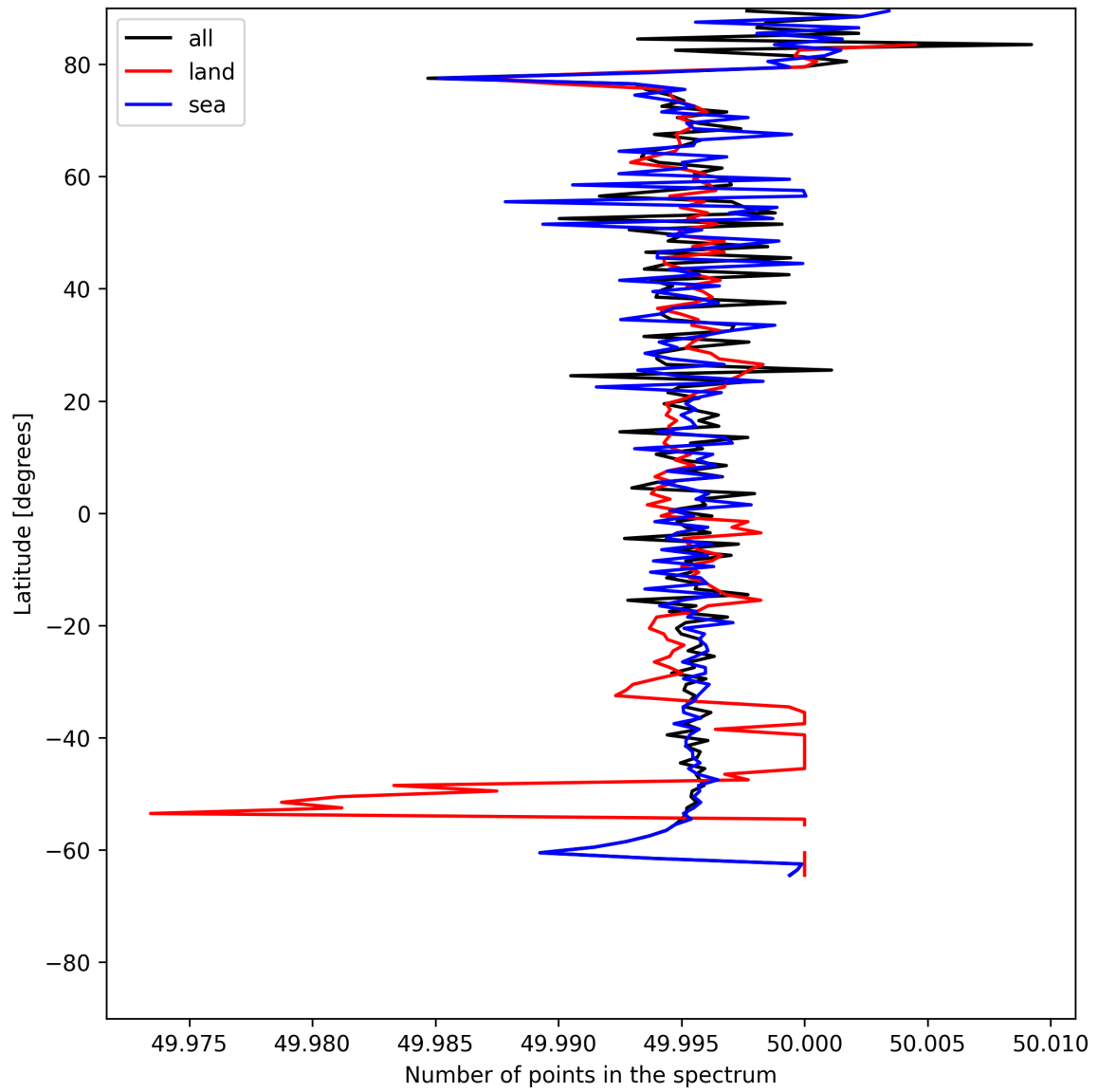
Figure 27: Zonal average of “Number of points in the spectrum” for 2025-07-03 to 2025-07-04.
