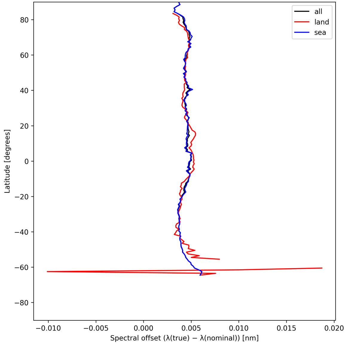
Figure 28: Zonal average of “Spectral offset ( \lambda_{\text{true}} - \lambda_{\text{nominal}} )” for 2025-07-03 to 2025-07-04.
