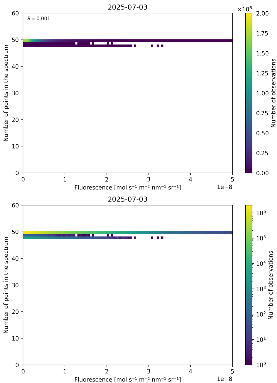
Figure 86: Scatter density plot of “Fluorescence” against “Number of points in the spectrum” for 2025-07-03 to 2025-07-04.
