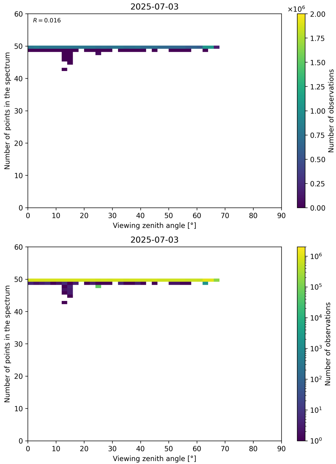
Figure 125: Scatter density plot of “Viewing zenith angle” against “Number of points in the spectrum” for 2025-07-03 to 2025-07-04.
