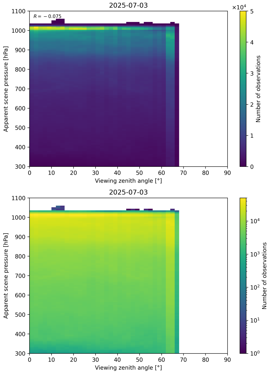
Figure 118: Scatter density plot of “Viewing zenith angle” against “Apparent scene pressure” for 2025-07-03 to 2025-07-04.
