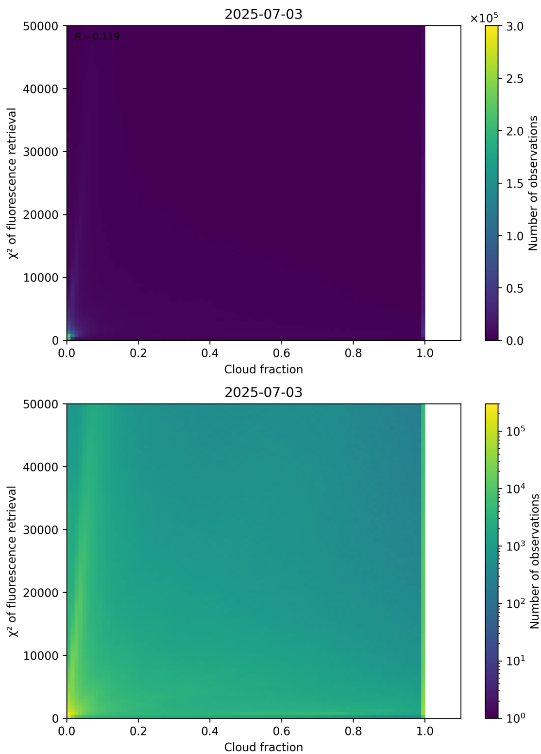
Figure 71: Scatter density plot of “Cloud fraction” against “ \chi^2 of fluorescence retrieval” for 2025-07-03 to 2025-07-04.
