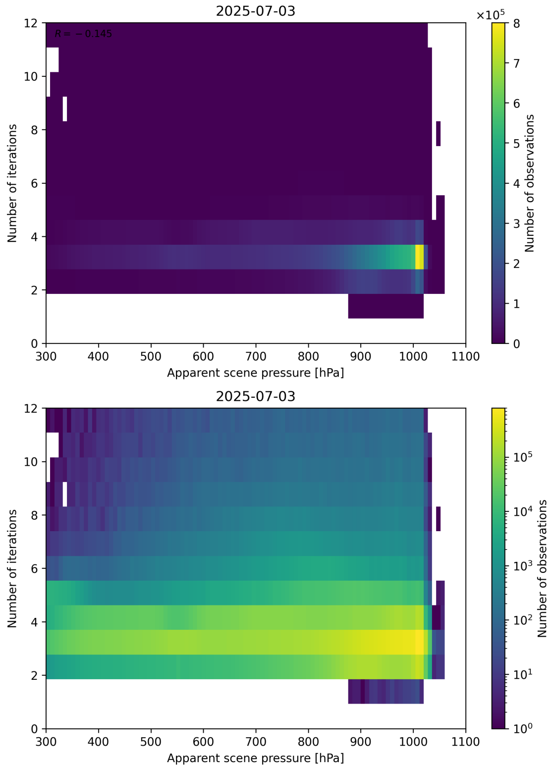
Figure 65: Scatter density plot of “Apparent scene pressure” against “Number of iterations” for 2025-07-03 to 2025-07-04.
