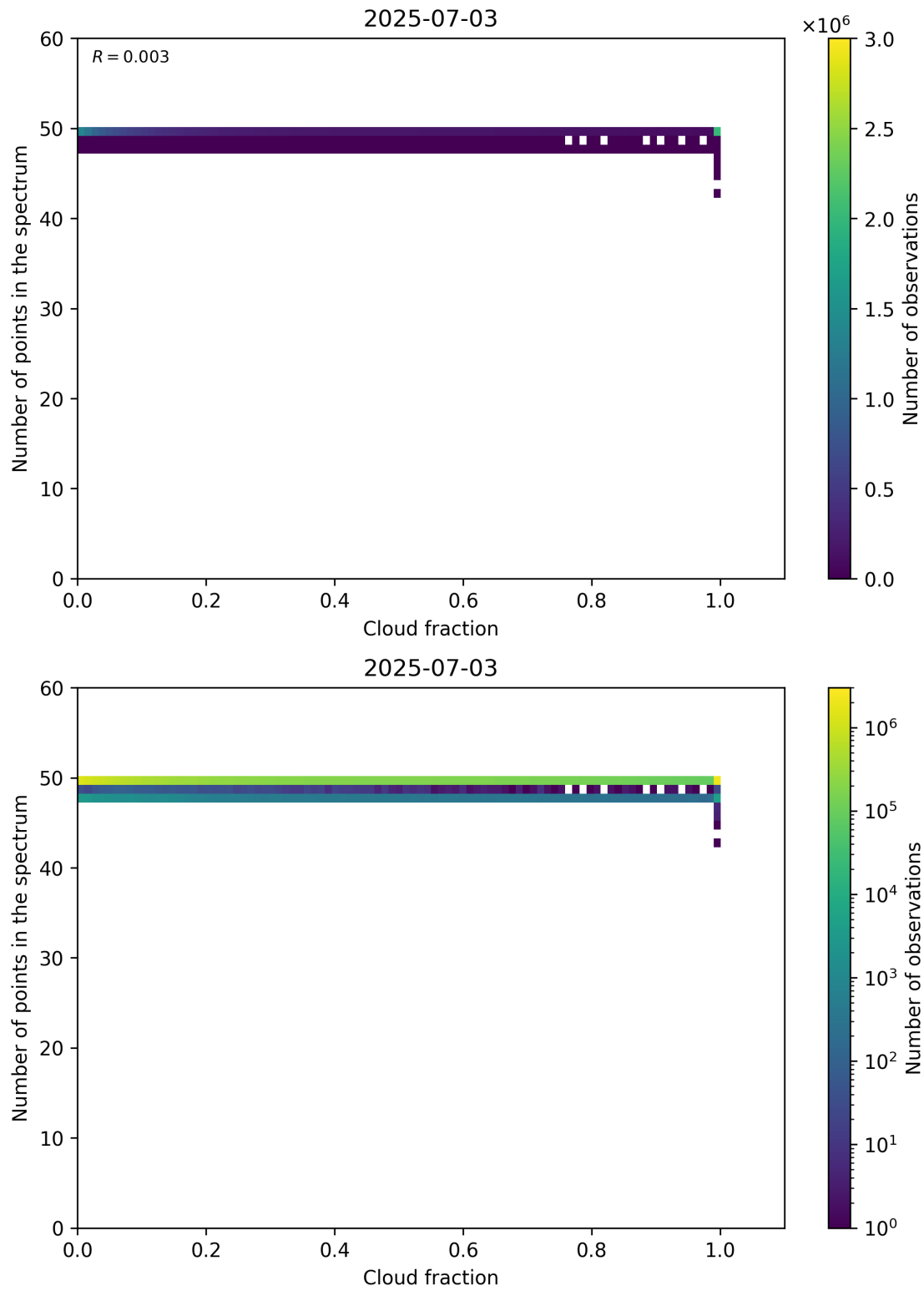
Figure 74: Scatter density plot of “Cloud fraction” against “Number of points in the spectrum” for 2025-07-03 to 2025-07-04.
