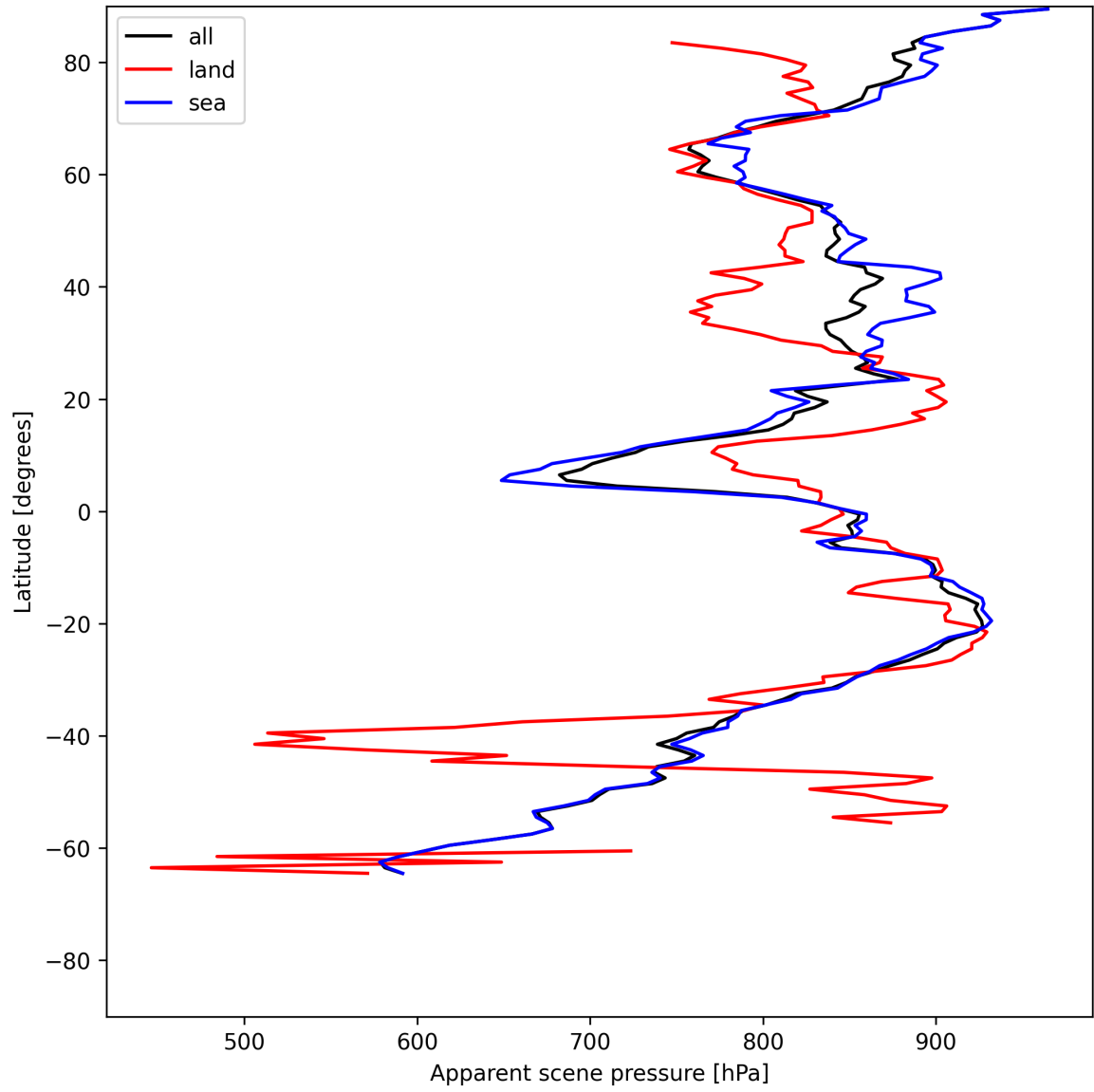
Figure 19: Zonal average of “Apparent scene pressure” for 2025-07-03 to 2025-07-04.
