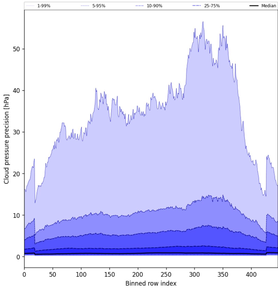
Figure 48: Along track statistics of “Cloud pressure precision” for 2025-07-03 to 2025-07-04
