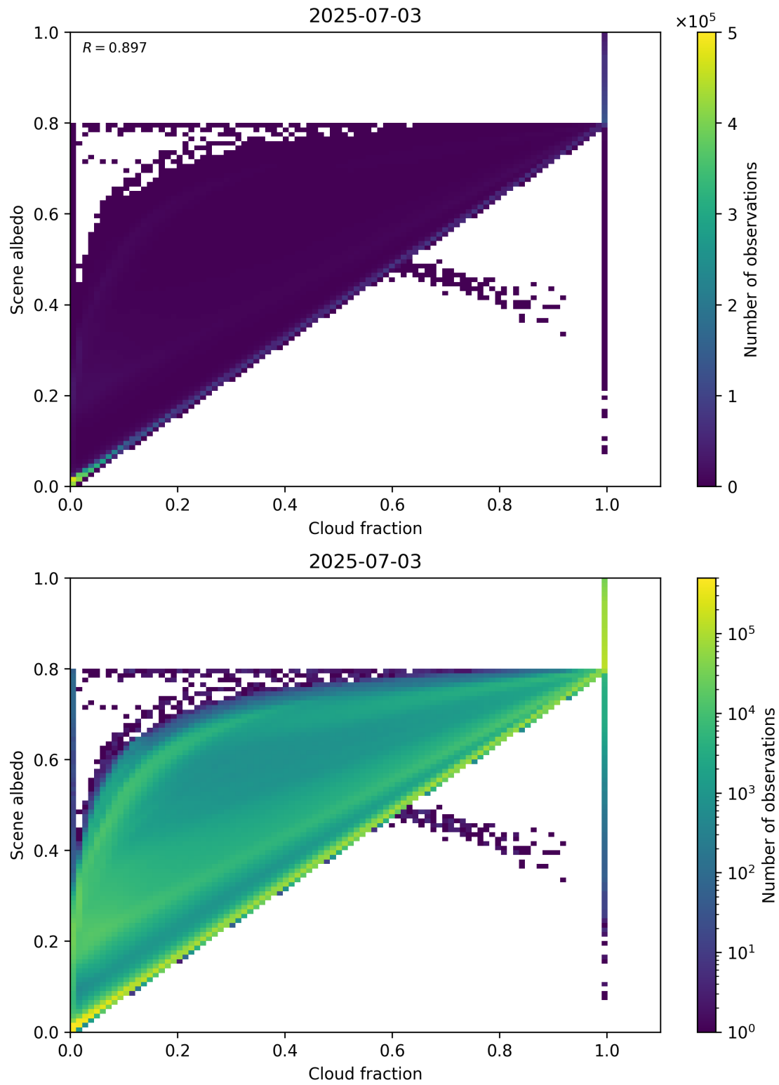
Figure 75: Scatter density plot of “Cloud fraction” against “Scene albedo” for 2025-07-03 to 2025-07-04.
