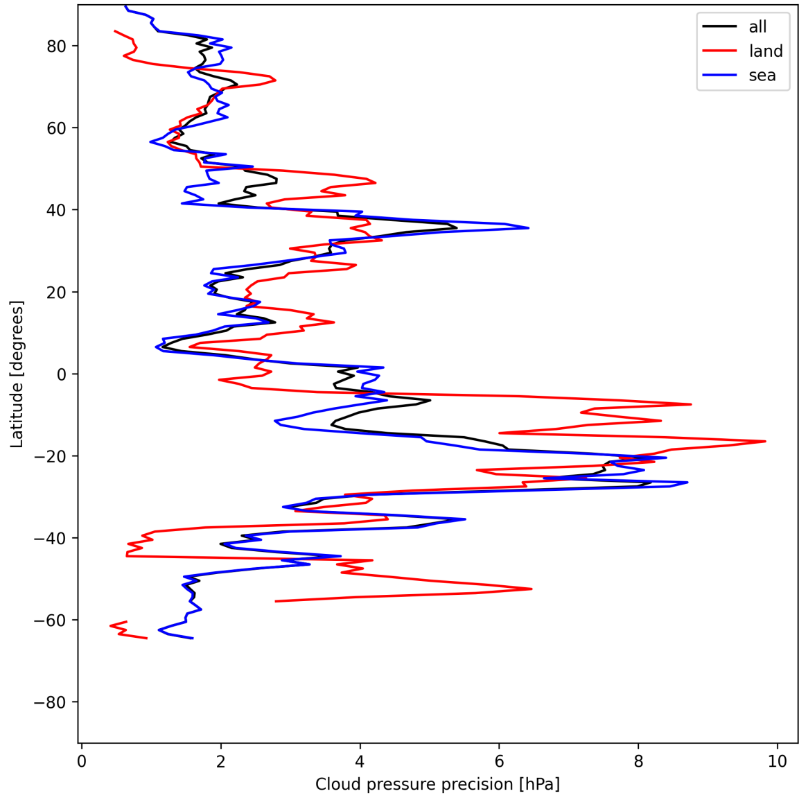
Figure 14: Zonal average of “Cloud pressure precision” for 2025-07-03 to 2025-07-04.
