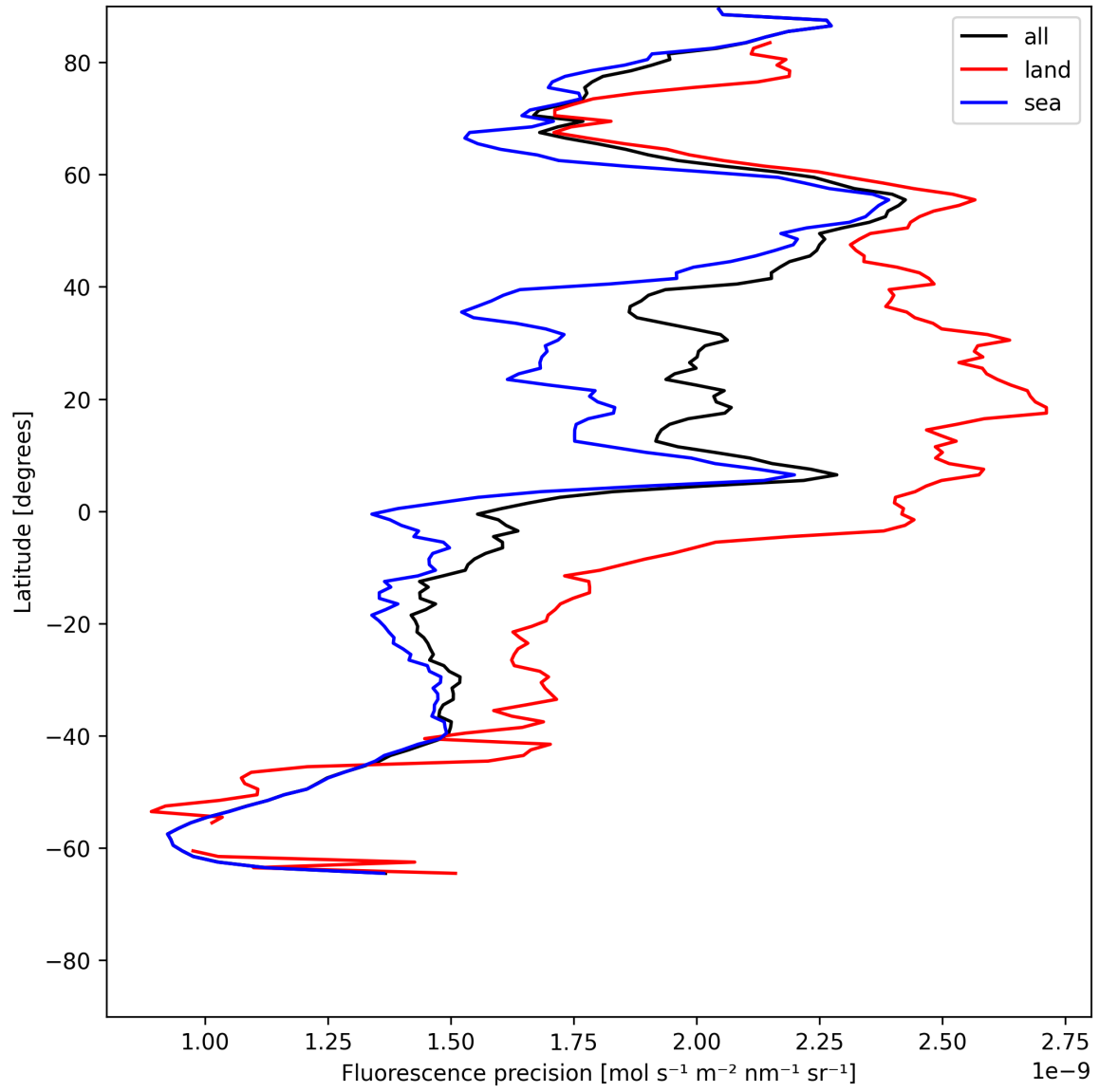
Figure 24: Zonal average of “Fluorescence precision” for 2025-07-03 to 2025-07-04.
