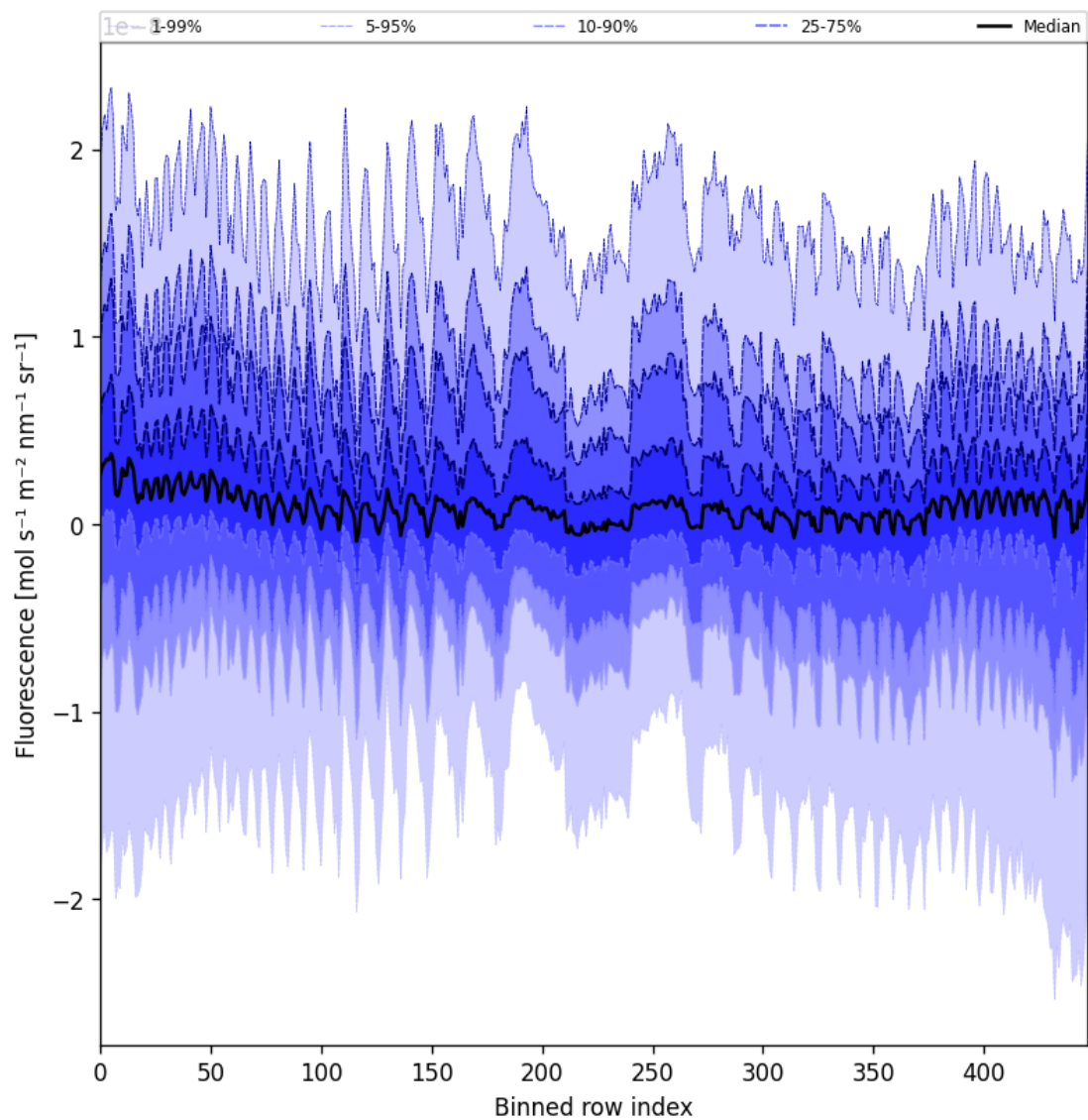
Figure 57: Along track statistics of “Fluorescence” for 2025-07-03 to 2025-07-04
