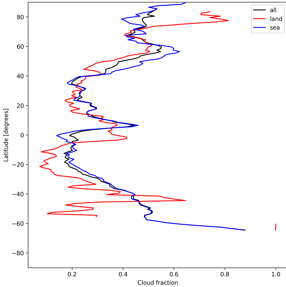
Figure 15: Zonal average of “Cloud fraction” for 2025-07-03 to 2025-07-04.
