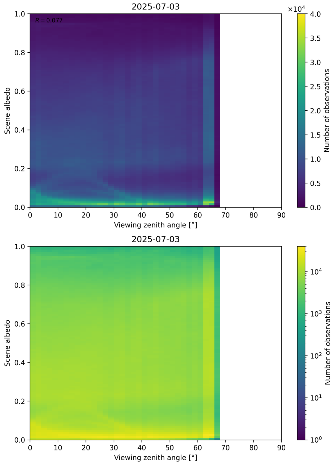
Figure 126: Scatter density plot of “Viewing zenith angle” against “Scene albedo” for 2025-07-03 to 2025-07-04.
