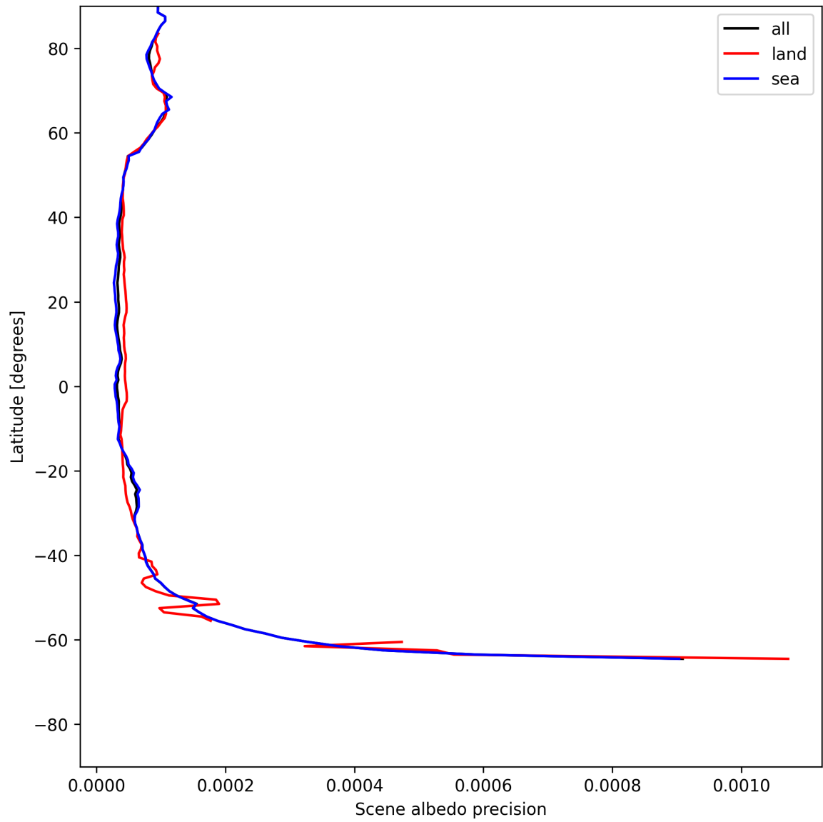
Figure 18: Zonal average of “Scene albedo precision” for 2025-07-03 to 2025-07-04.
