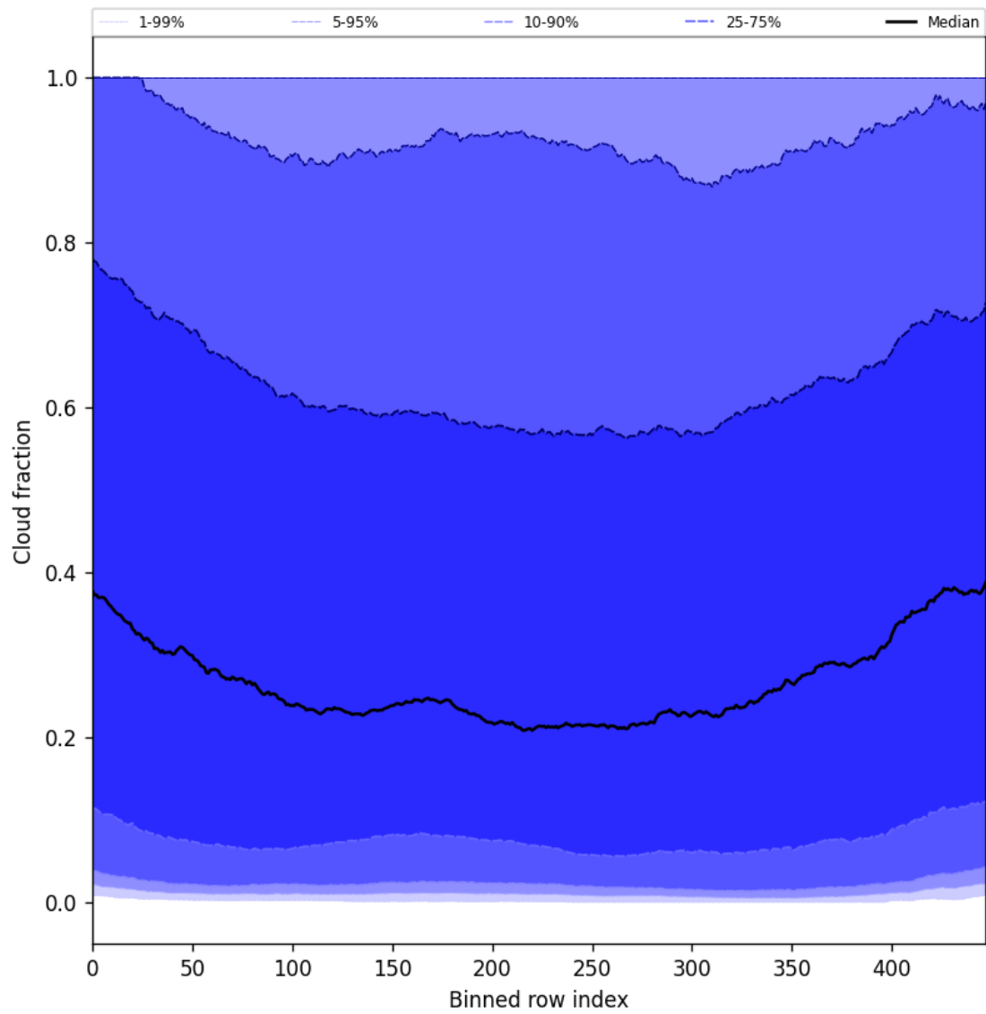
Figure 49: Along track statistics of “Cloud fraction” for 2025-07-03 to 2025-07-04
