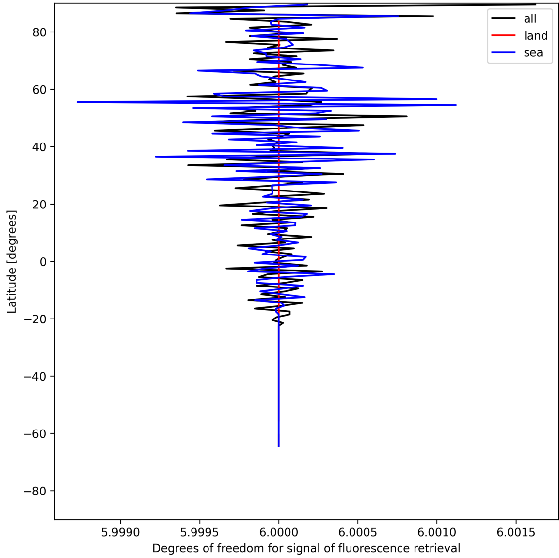
Figure 26: Zonal average of “Degrees of freedom for signal of fluorescence retrieval” for 2025-07-03 to 2025-07-04.
