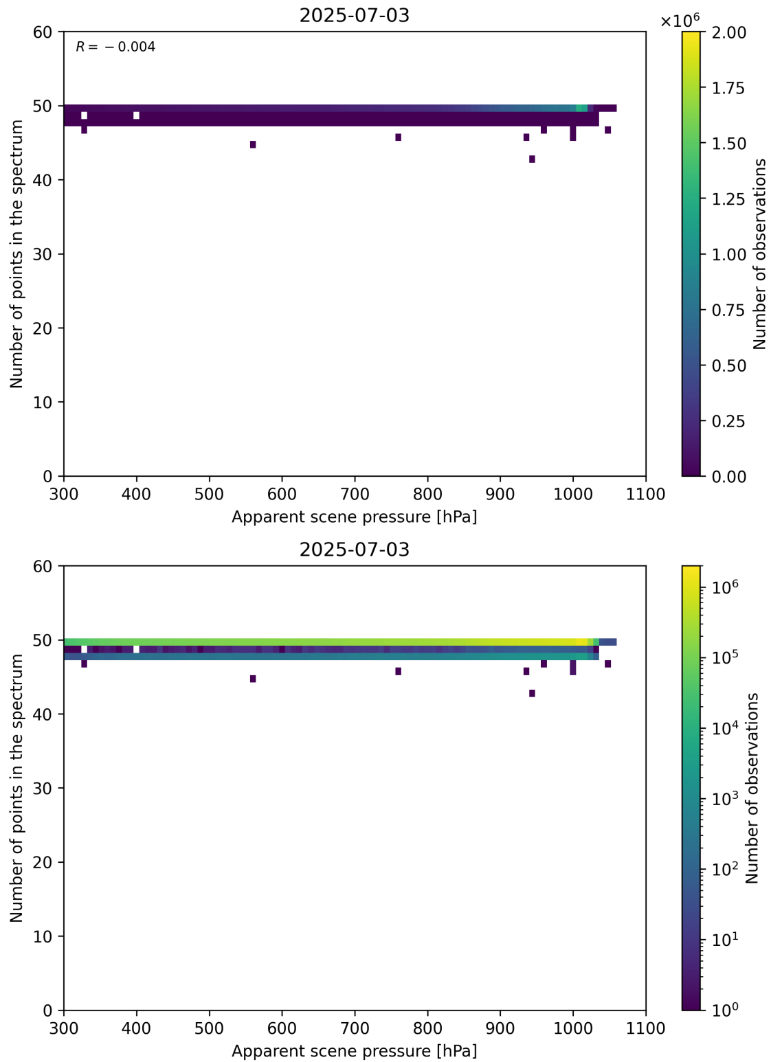
Figure 66: Scatter density plot of “Apparent scene pressure” against “Number of points in the spectrum” for 2025-07-03 to 2025-07-04.
