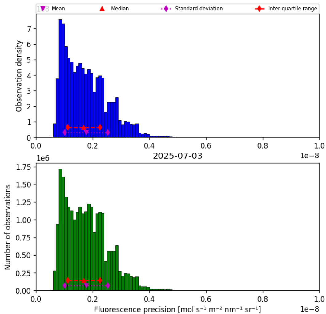
Figure 41: Histogram of “Fluorescence precision” for 2025-07-03 to 2025-07-04
