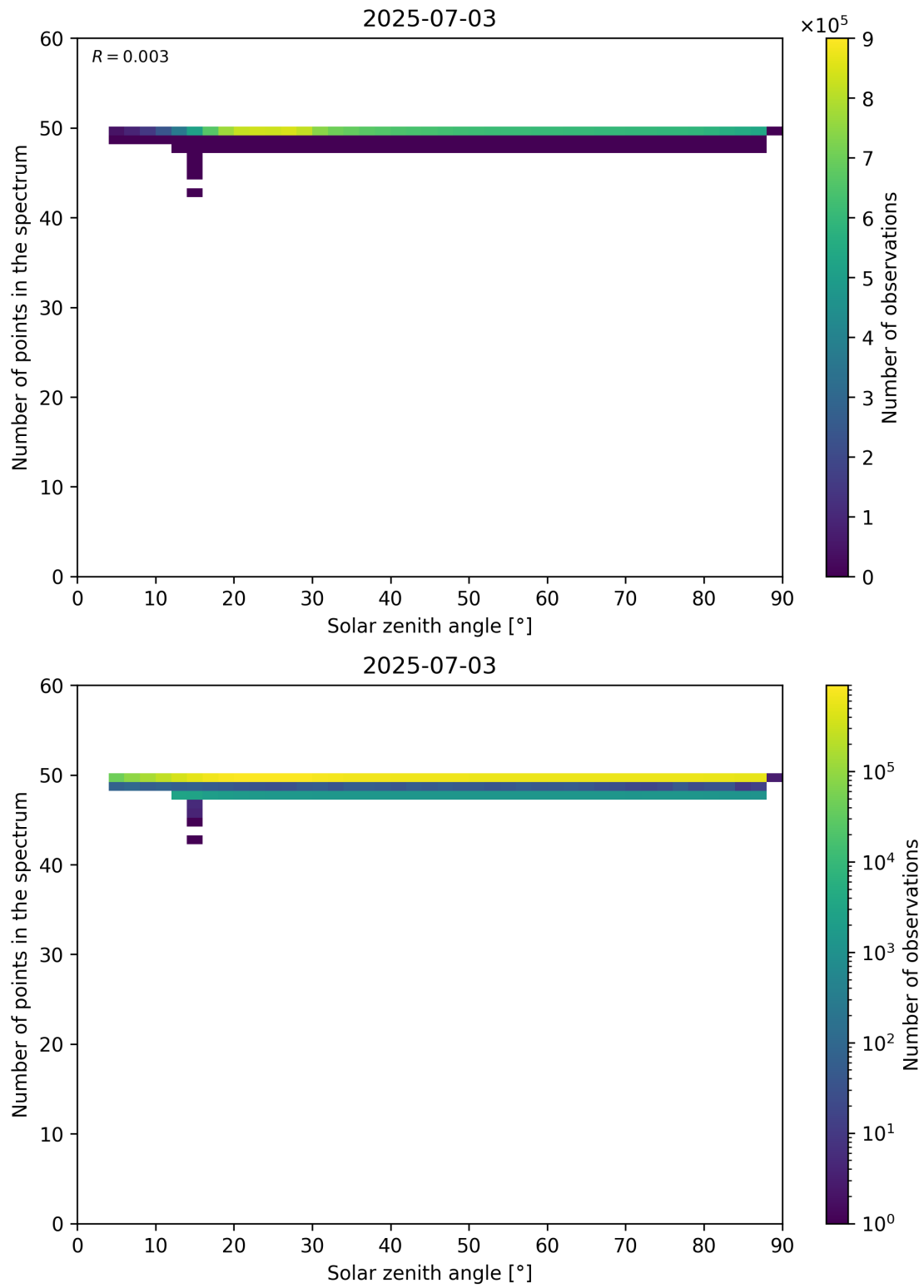
Figure 115: Scatter density plot of “Solar zenith angle” against “Number of points in the spectrum” for 2025-07-03 to 2025-07-04.
