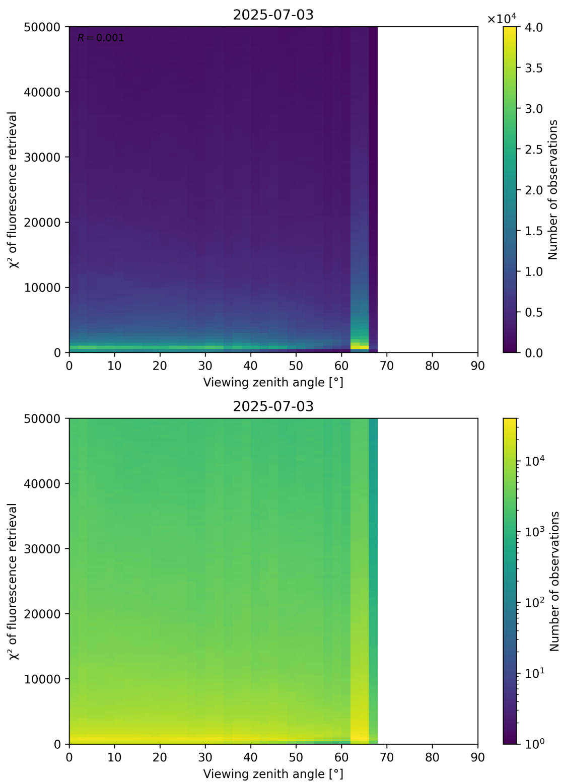
Figure 119: Scatter density plot of “Viewing zenith angle” against “ \chi^2 of fluorescence retrieval” for 2025-07-03 to 2025-07-04.
