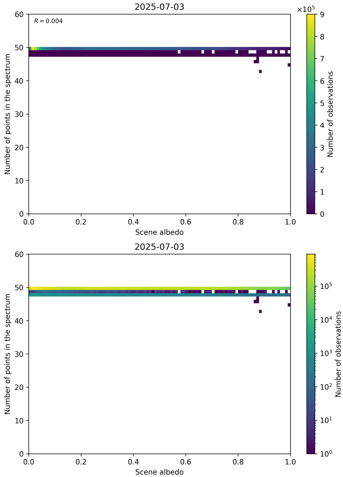
Figure 106: Scatter density plot of “Scene albedo” against “Number of points in the spectrum” for 2025-07-03 to 2025-07-04.
