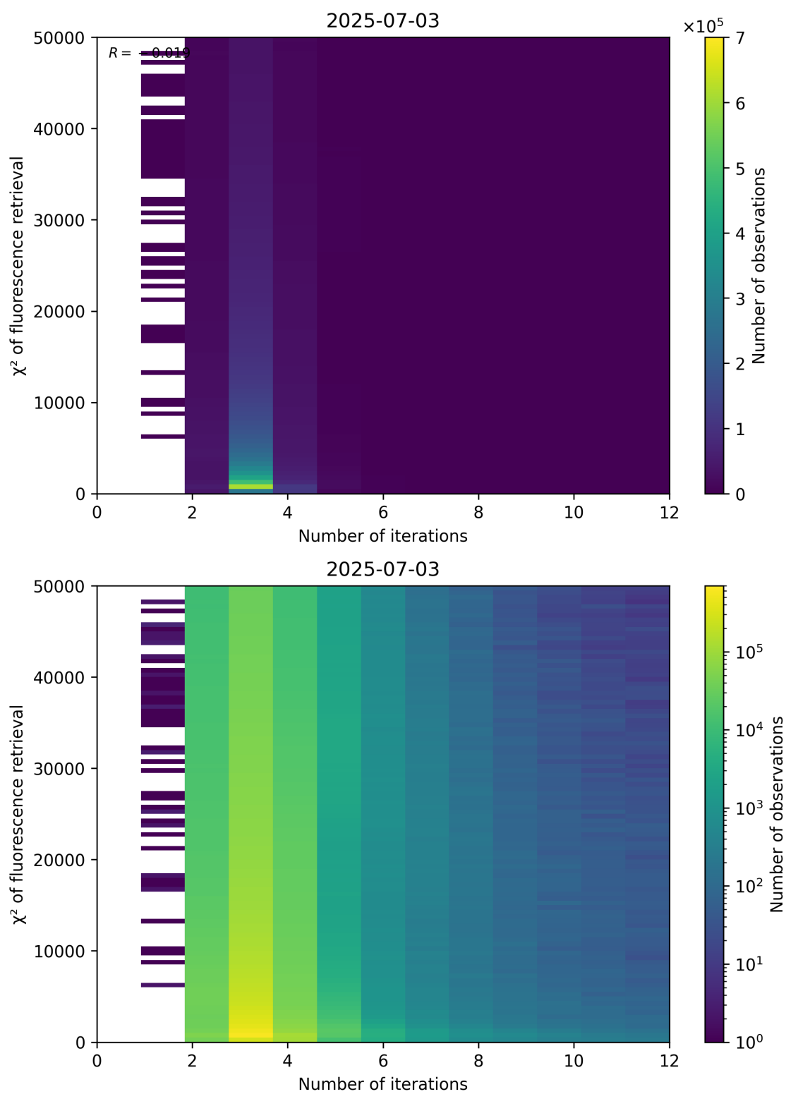
Figure 97: Scatter density plot of “Number of iterations” against “ \chi^2 of fluorescence retrieval” for 2025-07-03 to 2025-07-04.
