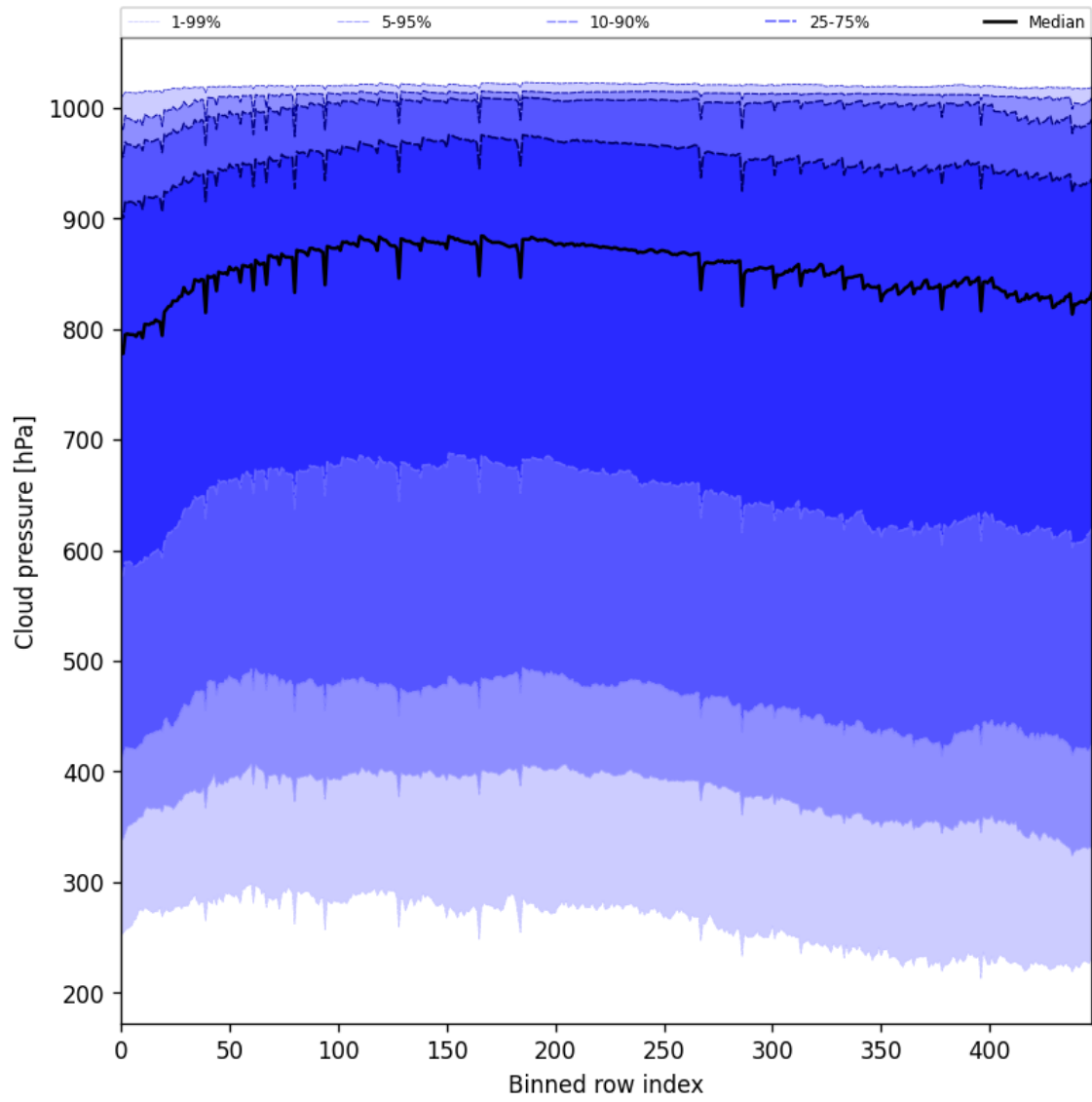
Figure 47: Along track statistics of “Cloud pressure” for 2025-07-03 to 2025-07-04
