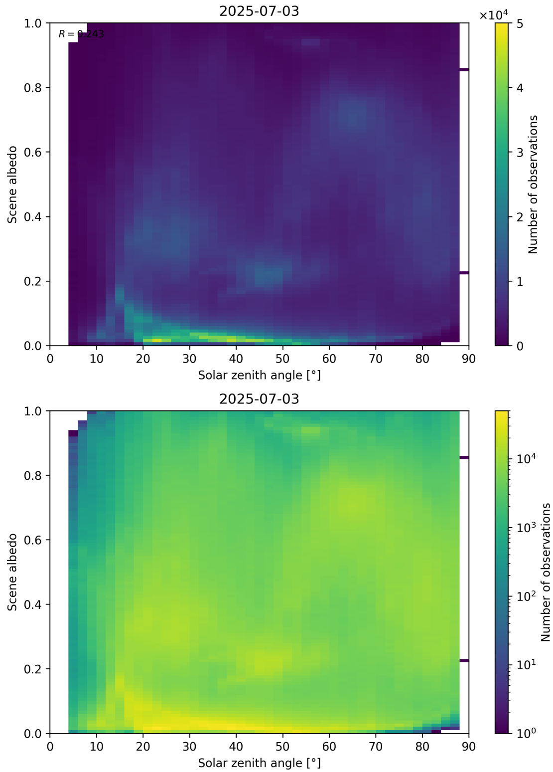
Figure 116: Scatter density plot of “Solar zenith angle” against “Scene albedo” for 2025-07-03 to 2025-07-04.
