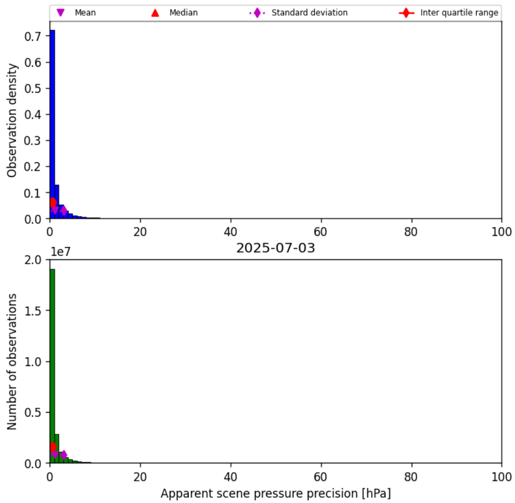
Figure 37: Histogram of “Apparent scene pressure precision” for 2025-07-03 to 2025-07-04
