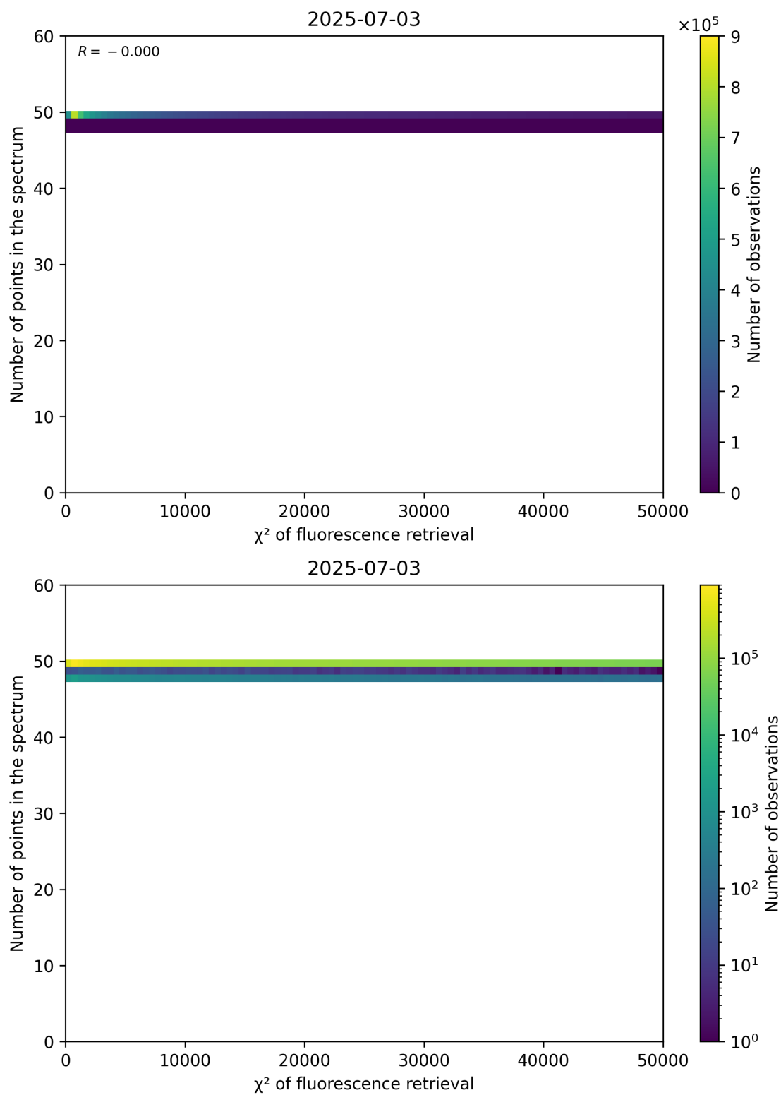
Figure 68: Scatter density plot of “ \chi^2 of fluorescence retrieval” against “Number of points in the spectrum” for 2025-07-03 to 2025-07-04.
