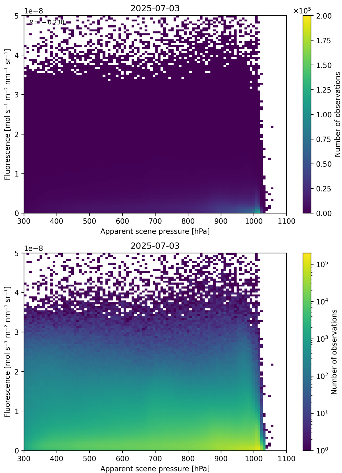
Figure 64: Scatter density plot of “Apparent scene pressure” against “Fluorescence” for 2025-07-03 to 2025-07-04.
