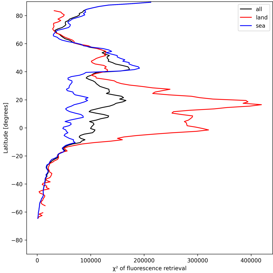
Figure 25: Zonal average of “ \chi^2 of fluorescence retrieval” for 2025-07-03 to 2025-07-04.
