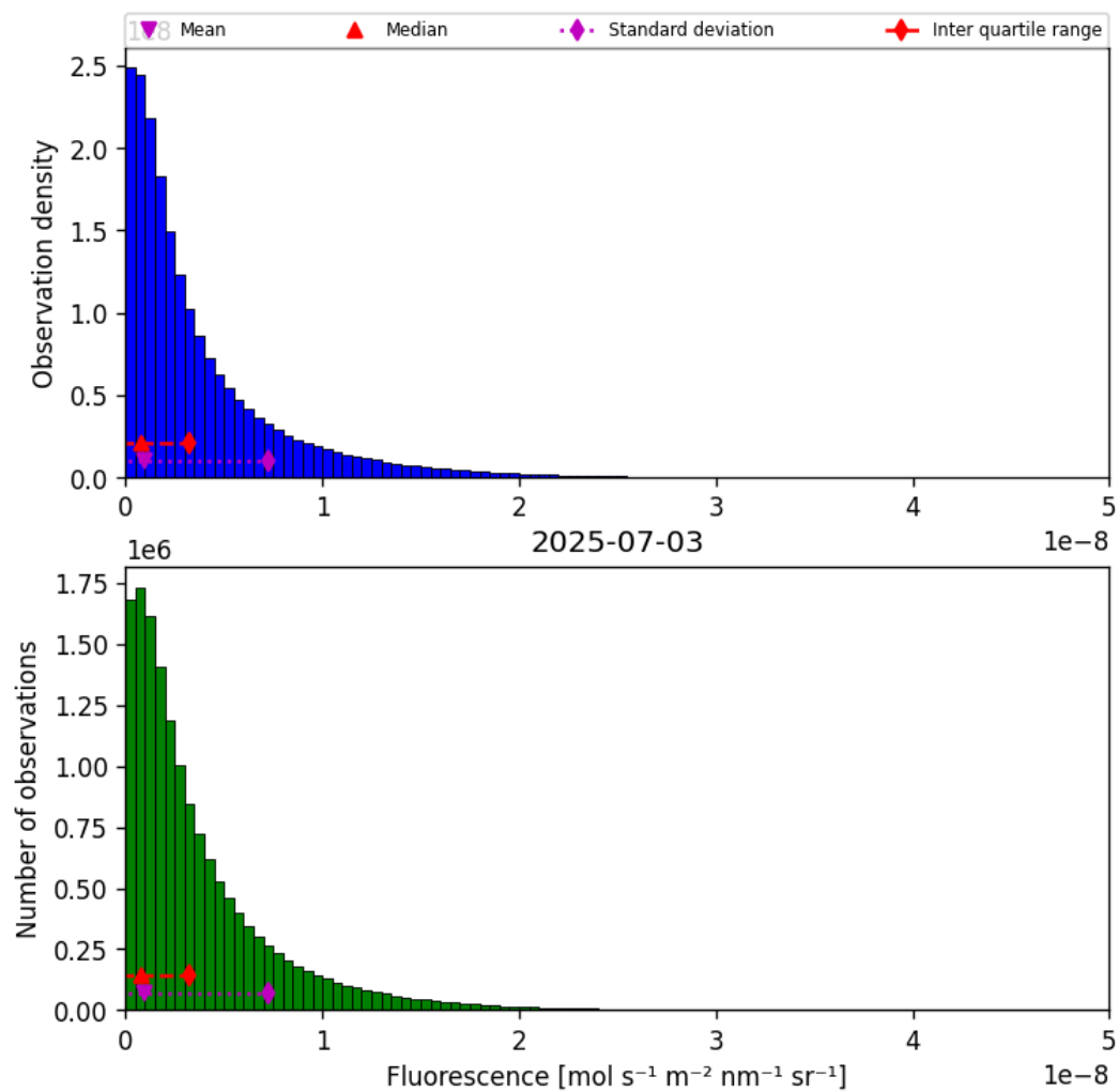
Figure 40: Histogram of “Fluorescence” for 2025-07-03 to 2025-07-04
