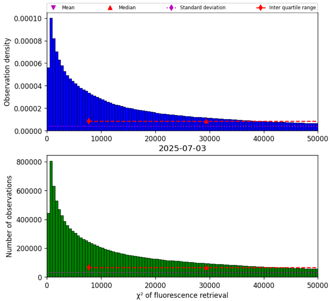
Figure 42: Histogram of “ \chi^2 of fluorescence retrieval” for 2025-07-03 to 2025-07-04
