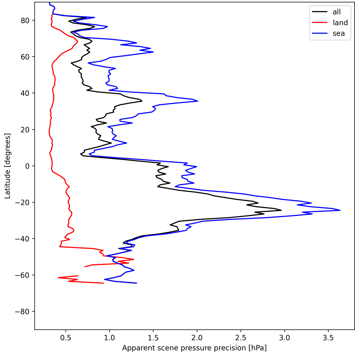
Figure 20: Zonal average of “Apparent scene pressure precision” for 2025-07-03 to 2025-07-04.
