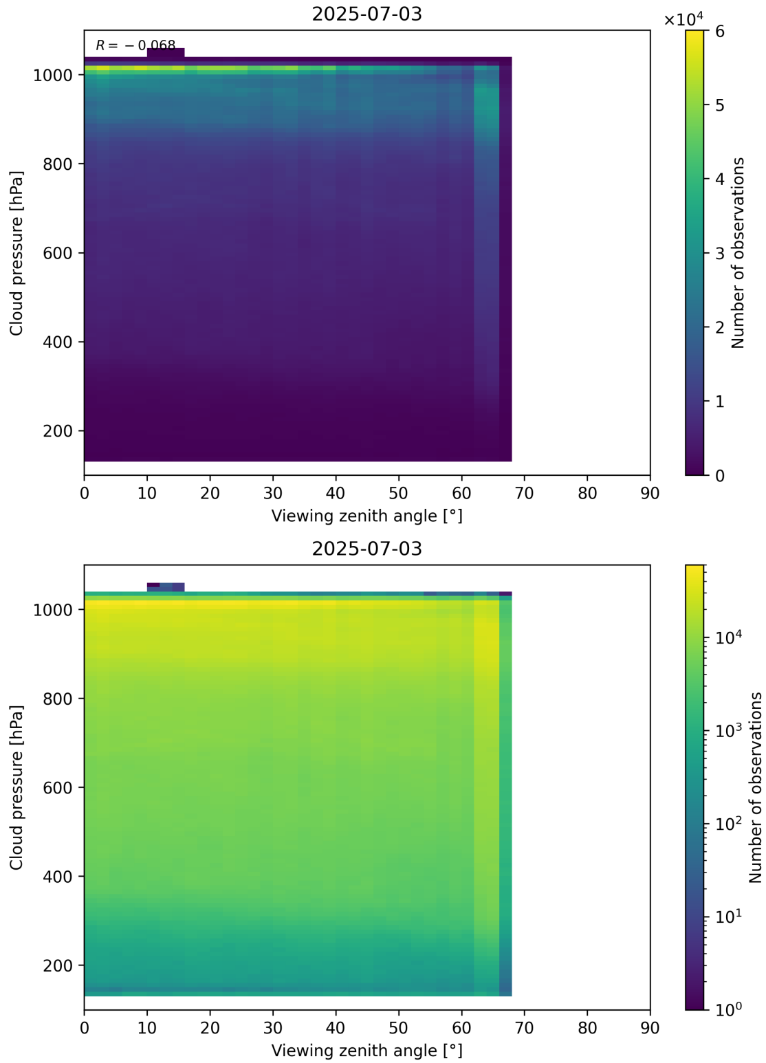
Figure 121: Scatter density plot of “Viewing zenith angle” against “Cloud pressure” for 2025-07-03 to 2025-07-04.
