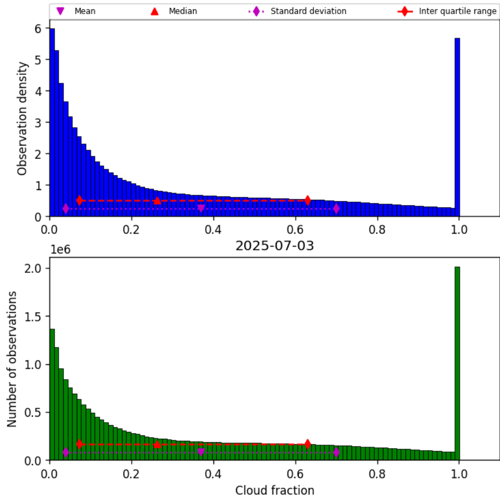
Figure 32: Histogram of “Cloud fraction” for 2025-07-03 to 2025-07-04
