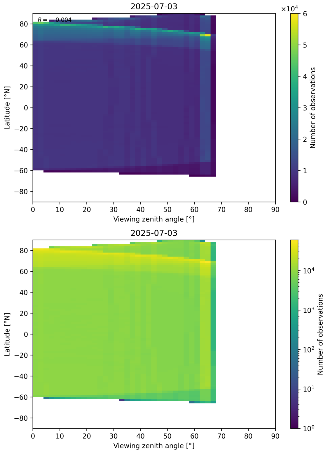
Figure 123: Scatter density plot of “Viewing zenith angle” against “Latitude” for 2025-07-03 to 2025-07-04.
