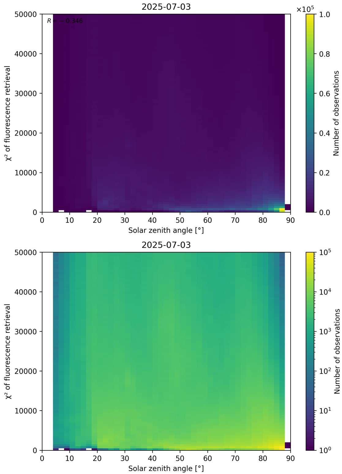
Figure 109: Scatter density plot of “Solar zenith angle” against “ \chi^2 of fluorescence retrieval” for 2025-07-03 to 2025-07-04.
