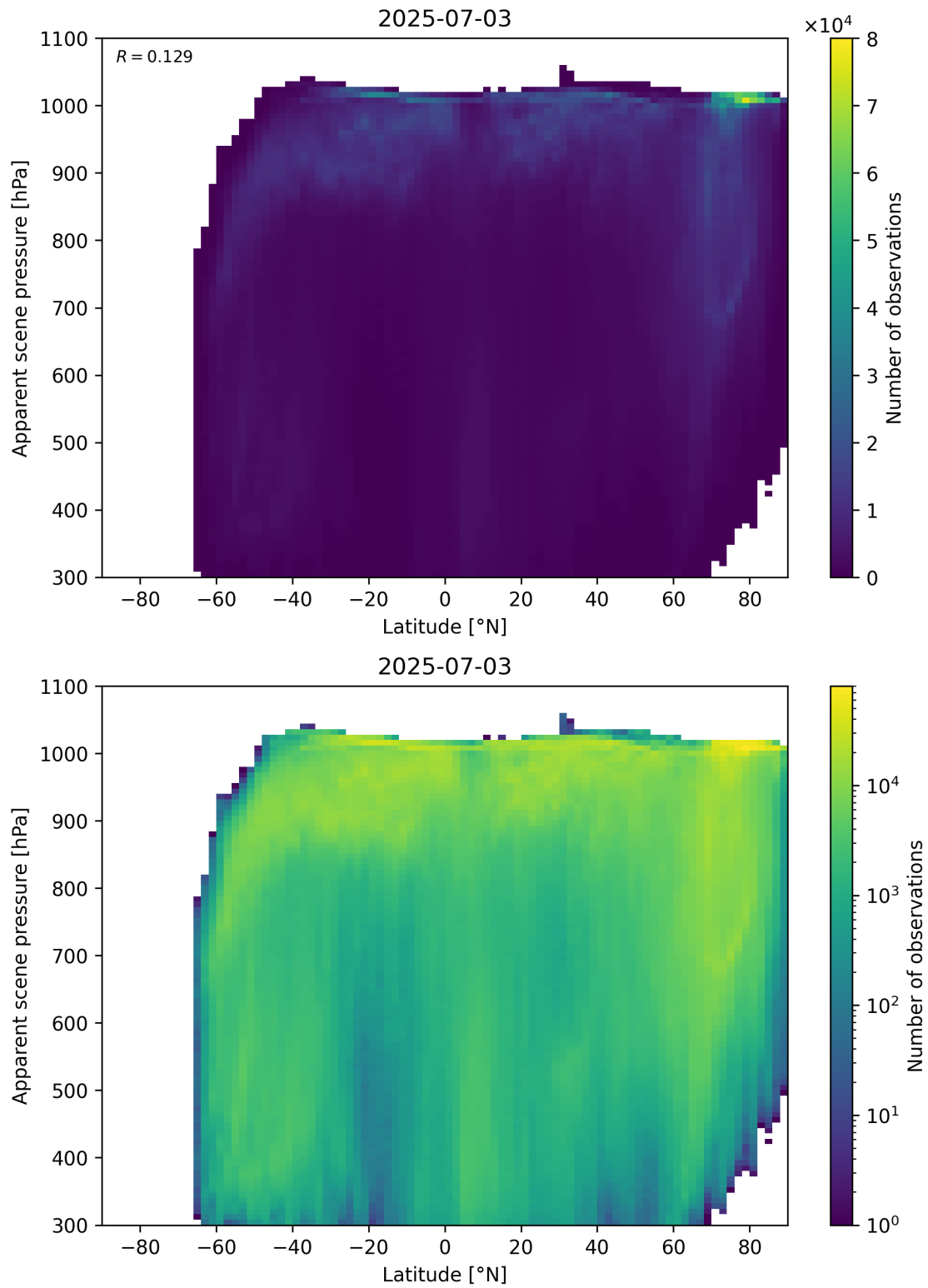
Figure 88: Scatter density plot of “Latitude” against “Apparent scene pressure” for 2025-07-03 to 2025-07-04.
