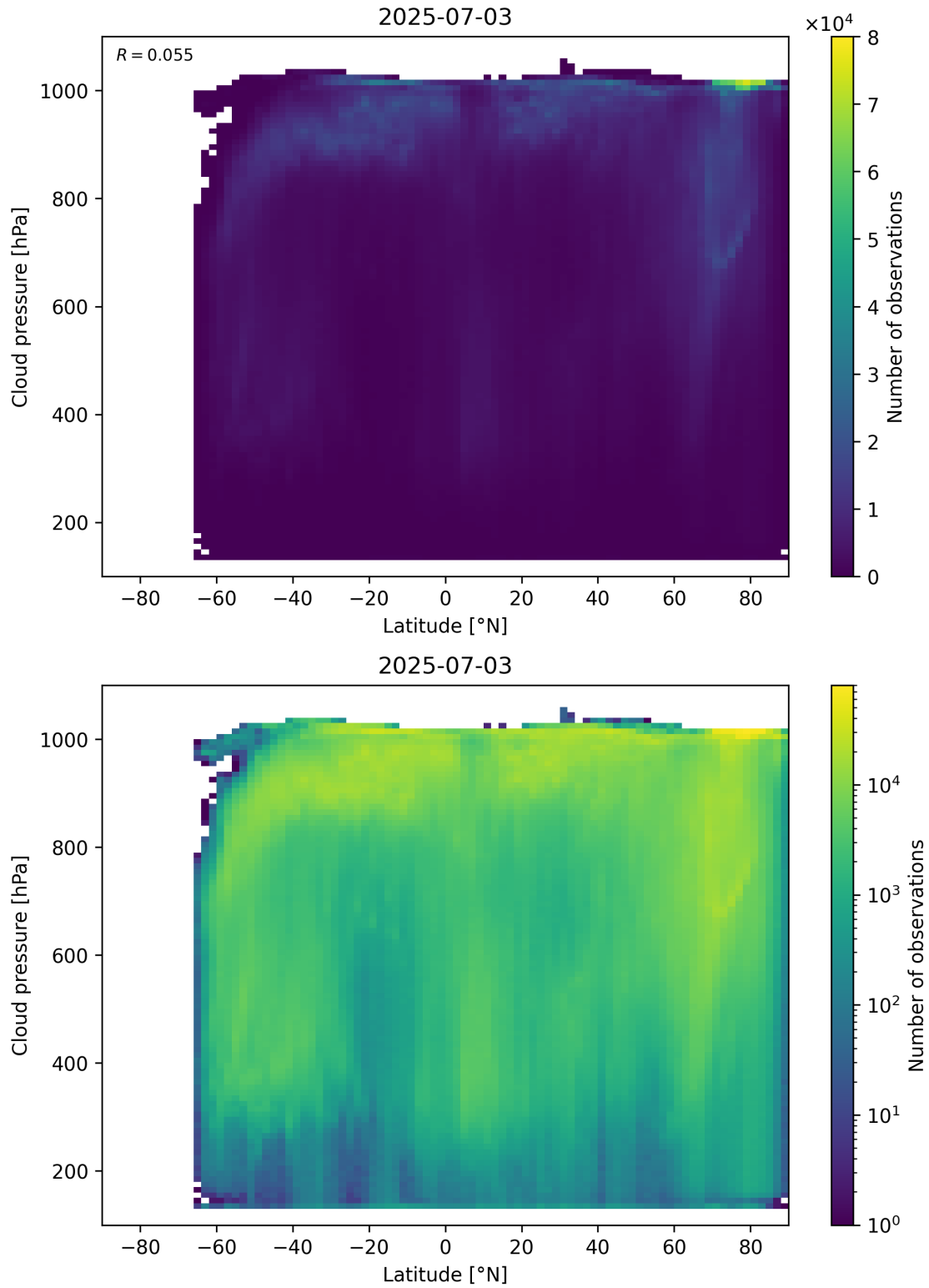
Figure 91: Scatter density plot of “Latitude” against “Cloud pressure” for 2025-07-03 to 2025-07-04.
