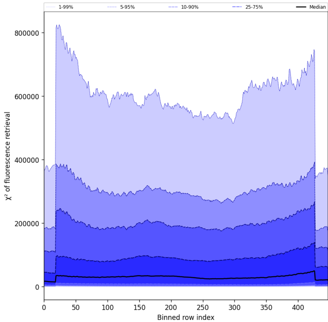
Figure 59: Along track statistics of “ \chi^2 of fluorescence retrieval” for 2025-07-03 to 2025-07-04
