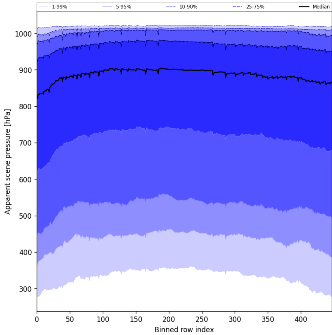
Figure 53: Along track statistics of “Apparent scene pressure” for 2025-07-03 to 2025-07-04
