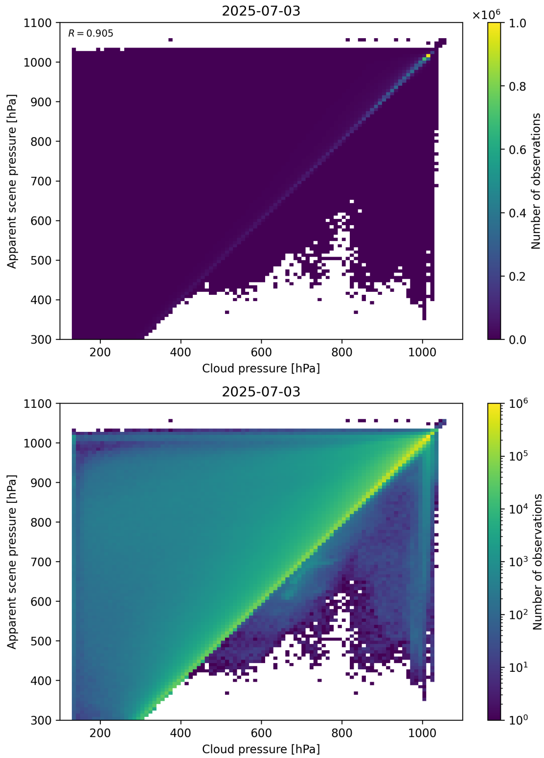
Figure 77: Scatter density plot of “Cloud pressure” against “Apparent scene pressure” for 2025-07-03 to 2025-07-04.
