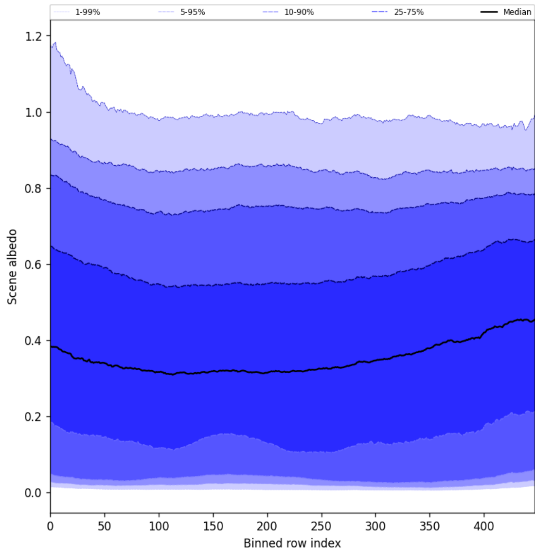
Figure 51: Along track statistics of “Scene albedo” for 2025-07-03 to 2025-07-04
