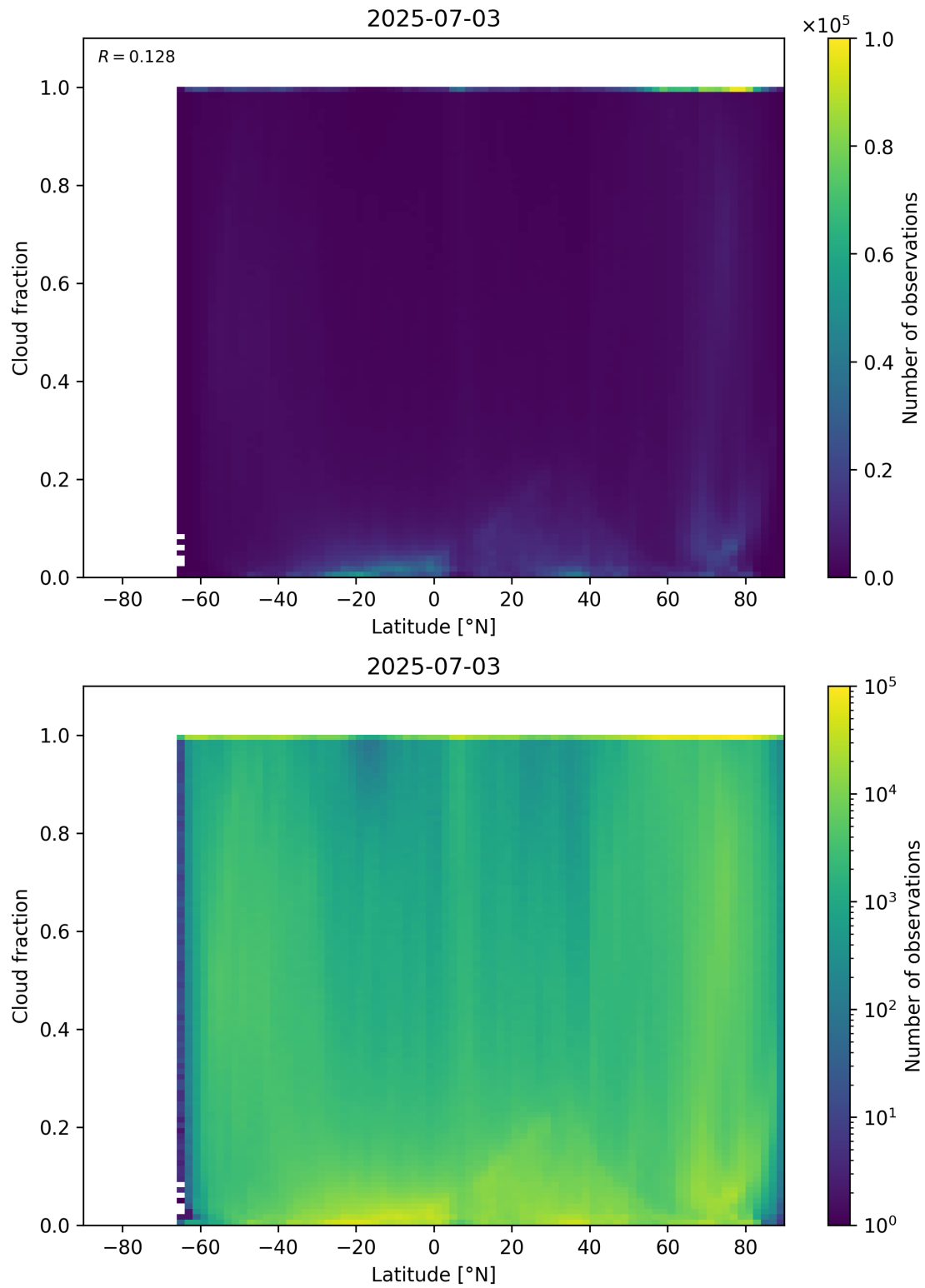
Figure 90: Scatter density plot of “Latitude” against “Cloud fraction” for 2025-07-03 to 2025-07-04.
