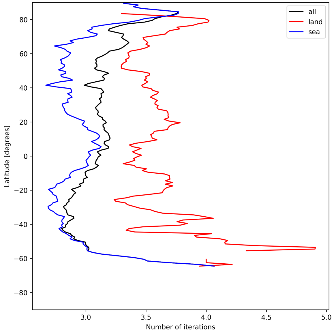
Figure 22: Zonal average of “Number of iterations” for 2025-07-03 to 2025-07-04.
