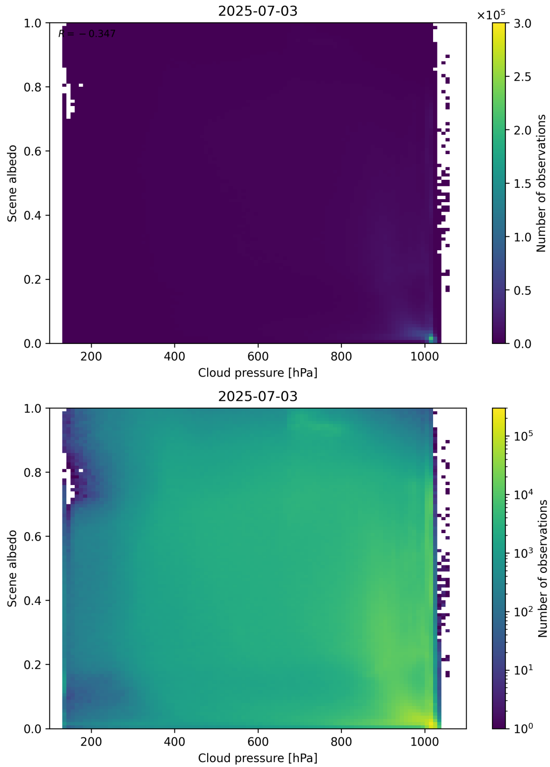
Figure 83: Scatter density plot of “Cloud pressure” against “Scene albedo” for 2025-07-03 to 2025-07-04.
