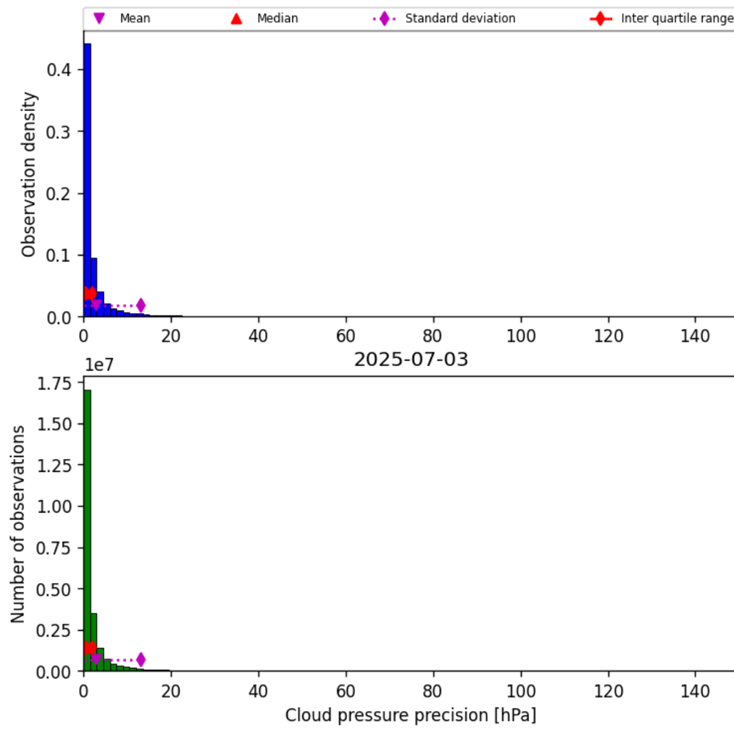
Figure 31: Histogram of “Cloud pressure precision” for 2025-07-03 to 2025-07-04
