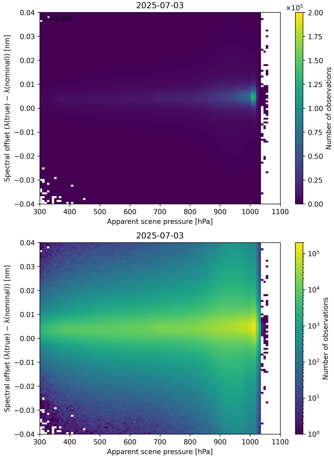
Figure 67: Scatter density plot of “Apparent scene pressure” against “Spectral offset ( \lambda_{\text{true}} - \lambda_{\text{nominal}} )” for 2025-07-03 to 2025-07-04.
