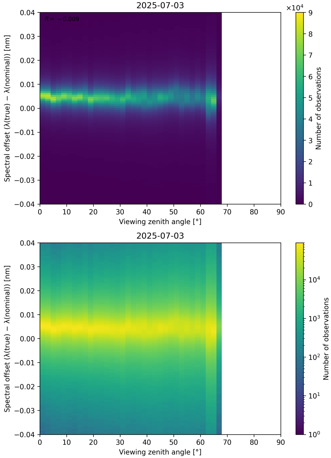
Figure 128: Scatter density plot of “Viewing zenith angle” against “Spectral offset ( \lambda_{\text{true}} - \lambda_{\text{nominal}} )” for 2025-07-03 to 2025-07-04.
