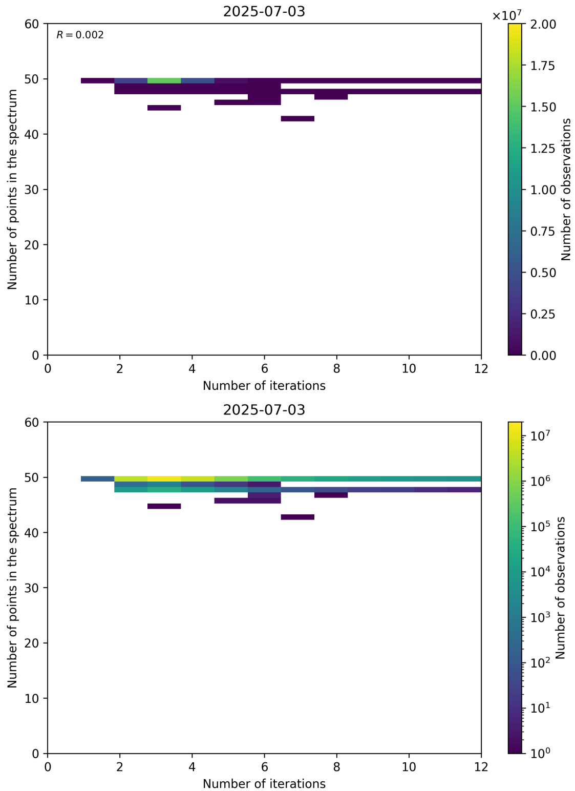
Figure 99: Scatter density plot of “Number of iterations” against “Number of points in the spectrum” for 2025-07-03 to 2025-07-04.
