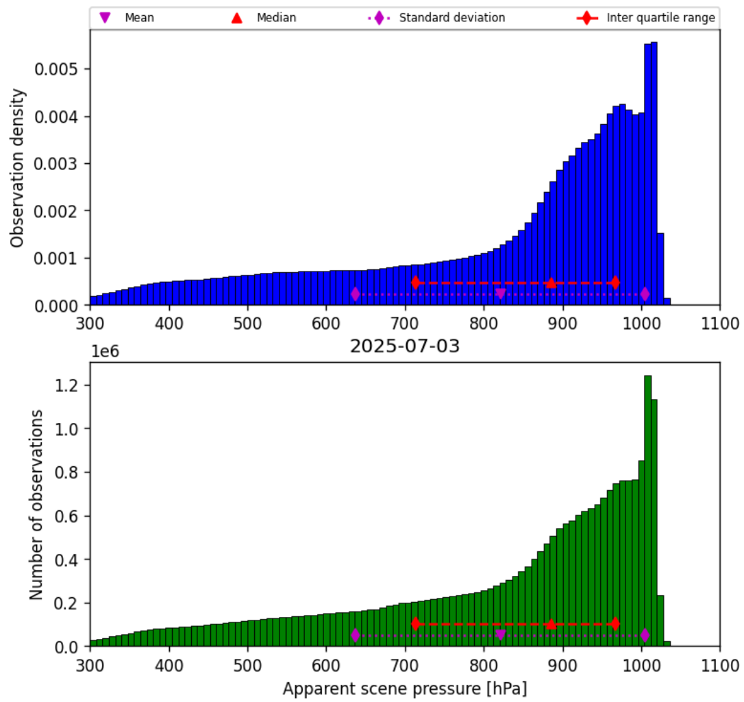
Figure 36: Histogram of “Apparent scene pressure” for 2025-07-03 to 2025-07-04
