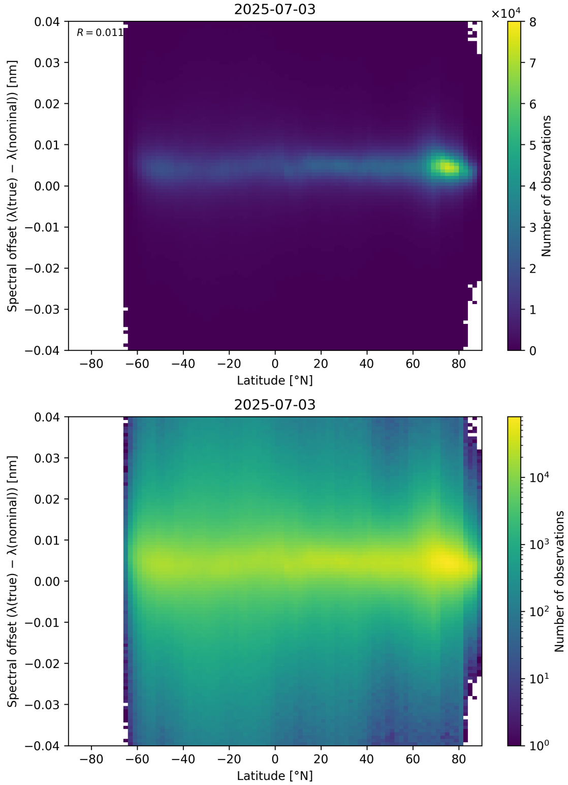
Figure 96: Scatter density plot of “Latitude” against “Spectral offset ( \lambda_{\text{true}} - \lambda_{\text{nominal}} )” for 2025-07-03 to 2025-07-04.
