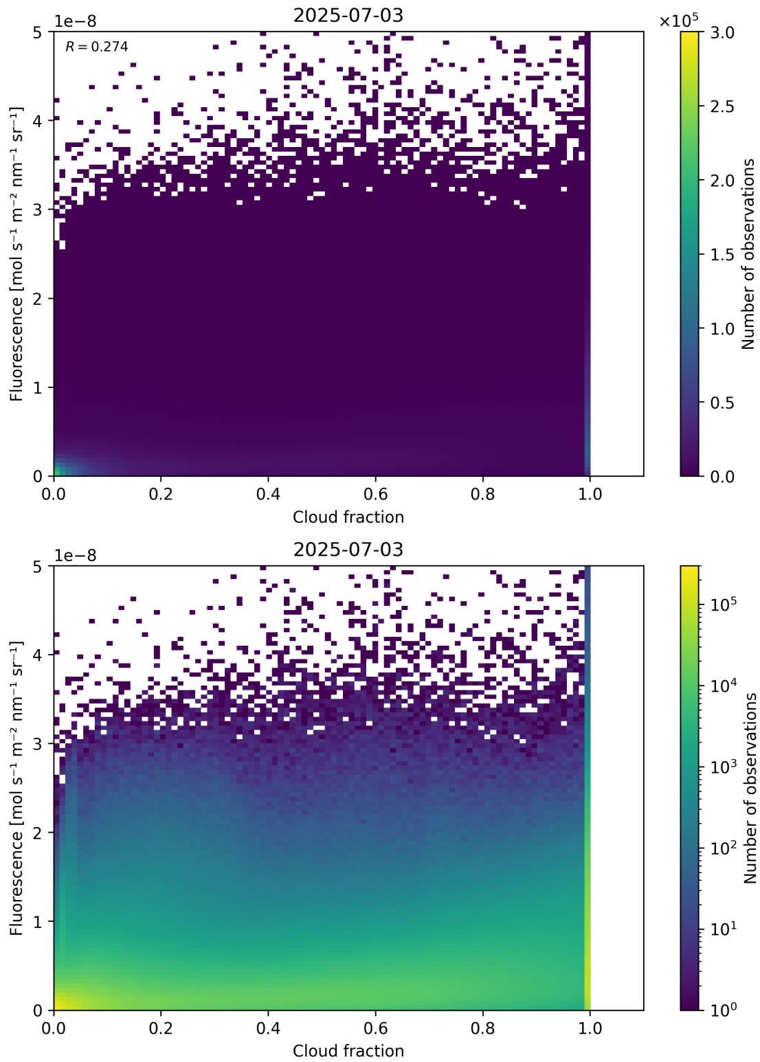
Figure 72: Scatter density plot of “Cloud fraction” against “Fluorescence” for 2025-07-03 to 2025-07-04.
