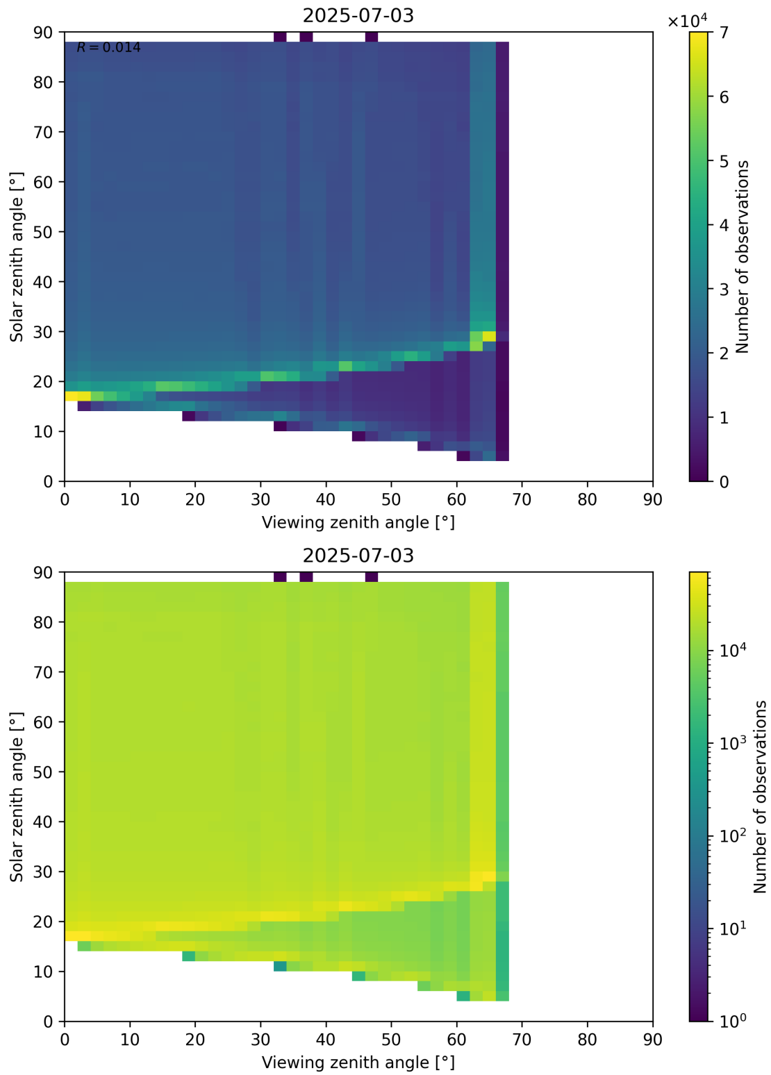
Figure 127: Scatter density plot of “Viewing zenith angle” against “Solar zenith angle” for 2025-07-03 to 2025-07-04.
