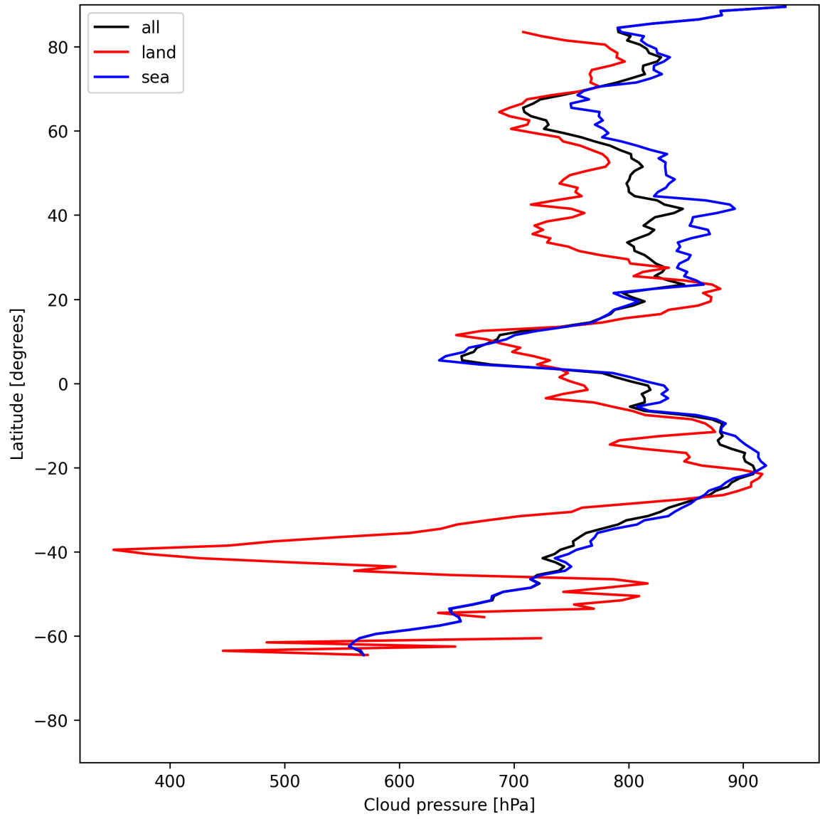
Figure 13: Zonal average of “Cloud pressure” for 2025-07-03 to 2025-07-04.
