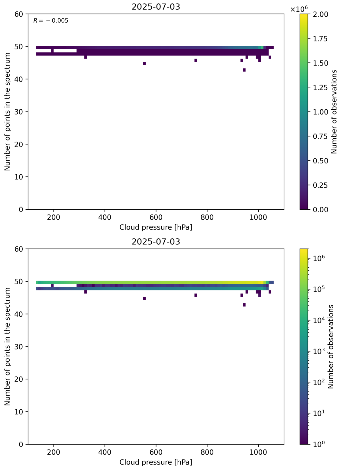
Figure 82: Scatter density plot of “Cloud pressure” against “Number of points in the spectrum” for 2025-07-03 to 2025-07-04.
