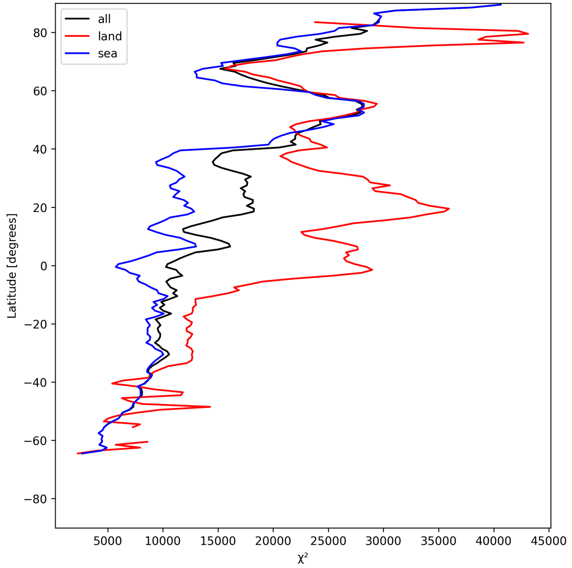
Figure 21: Zonal average of “ \chi^2 ” for 2025-07-03 to 2025-07-04.
