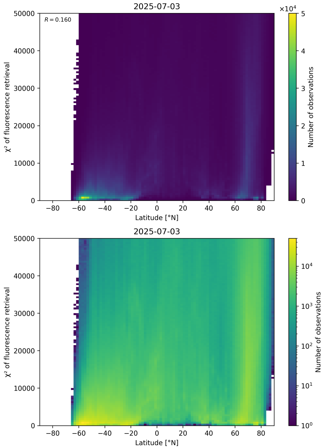
Figure 89: Scatter density plot of “Latitude” against “ \chi^2 of fluorescence retrieval” for 2025-07-03 to 2025-07-04.
