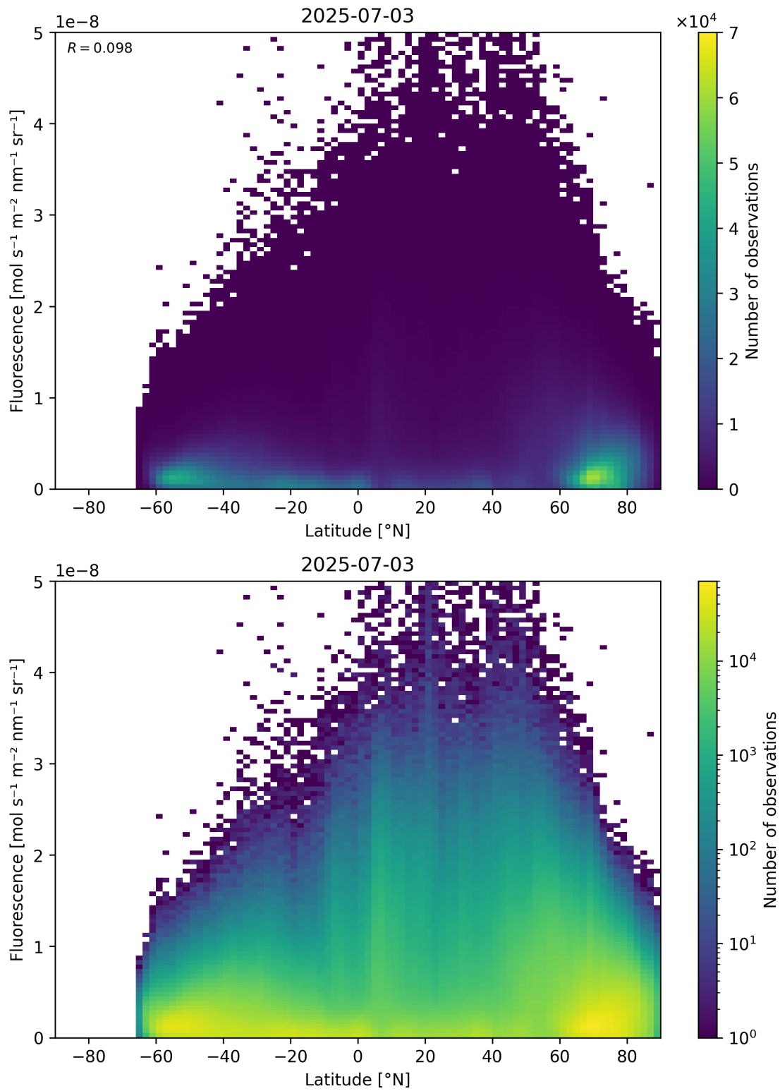
Figure 92: Scatter density plot of “Latitude” against “Fluorescence” for 2025-07-03 to 2025-07-04.
