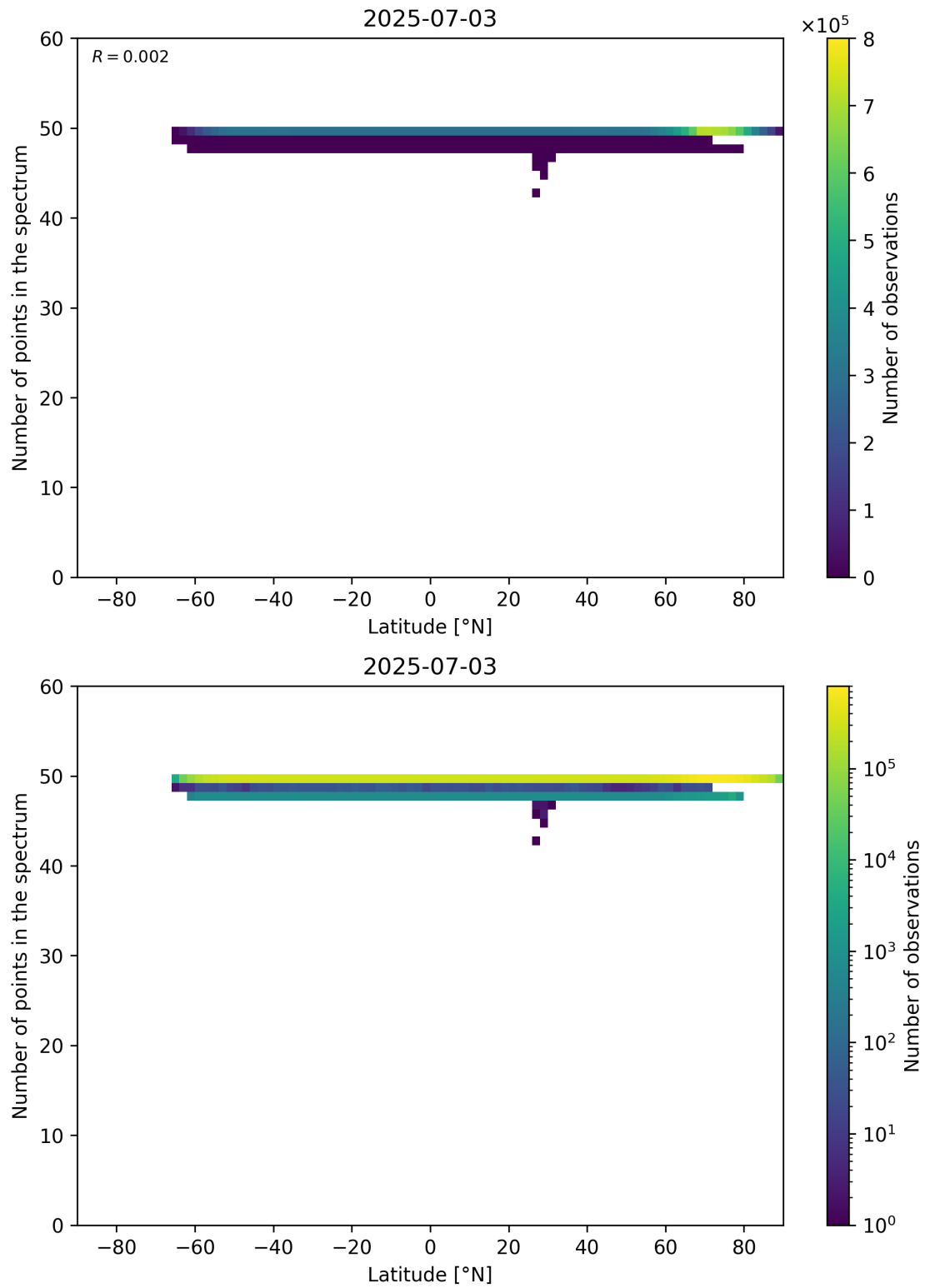
Figure 94: Scatter density plot of “Latitude” against “Number of points in the spectrum” for 2025-07-03 to 2025-07-04.
