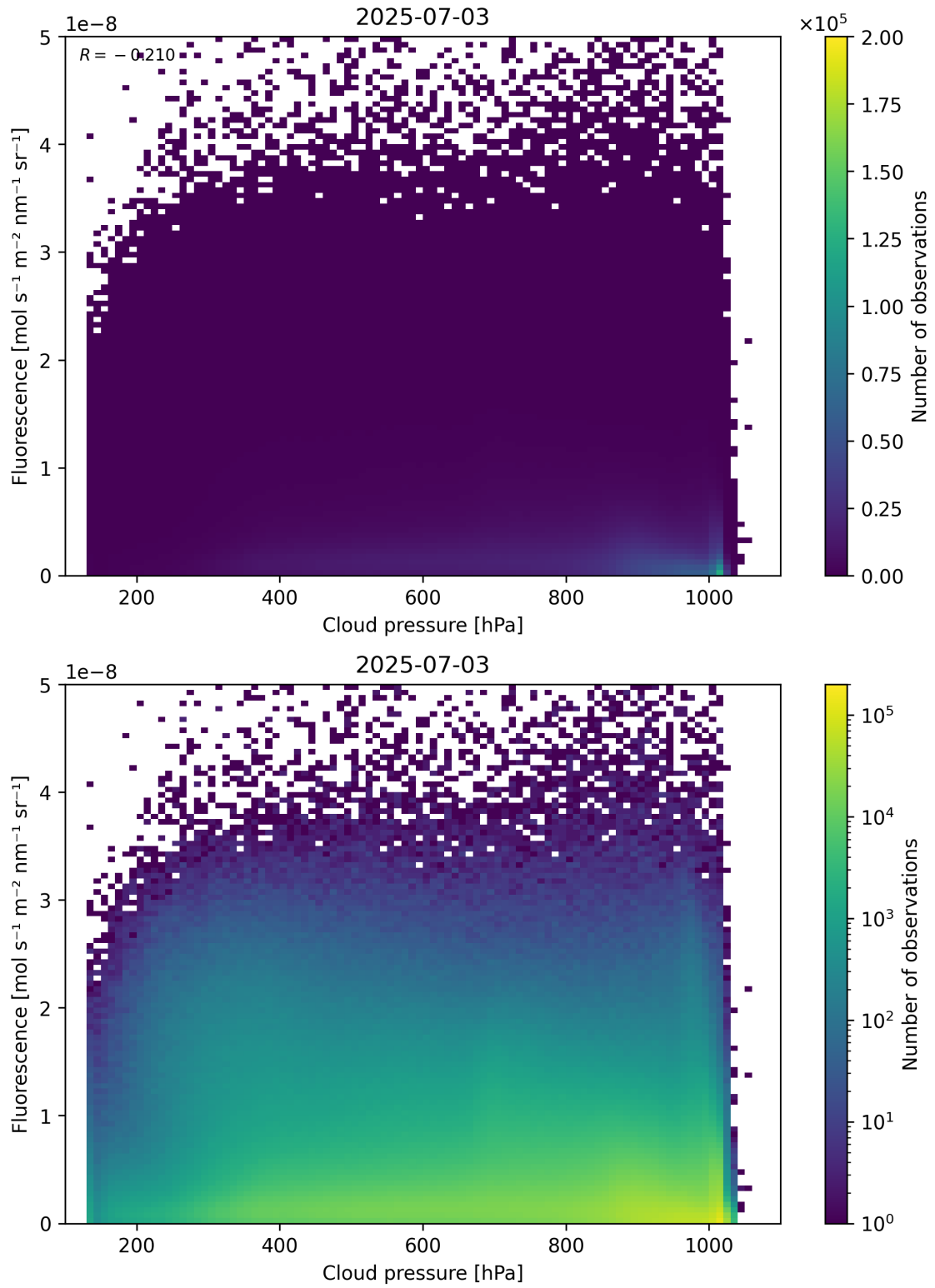
Figure 80: Scatter density plot of “Cloud pressure” against “Fluorescence” for 2025-07-03 to 2025-07-04.
