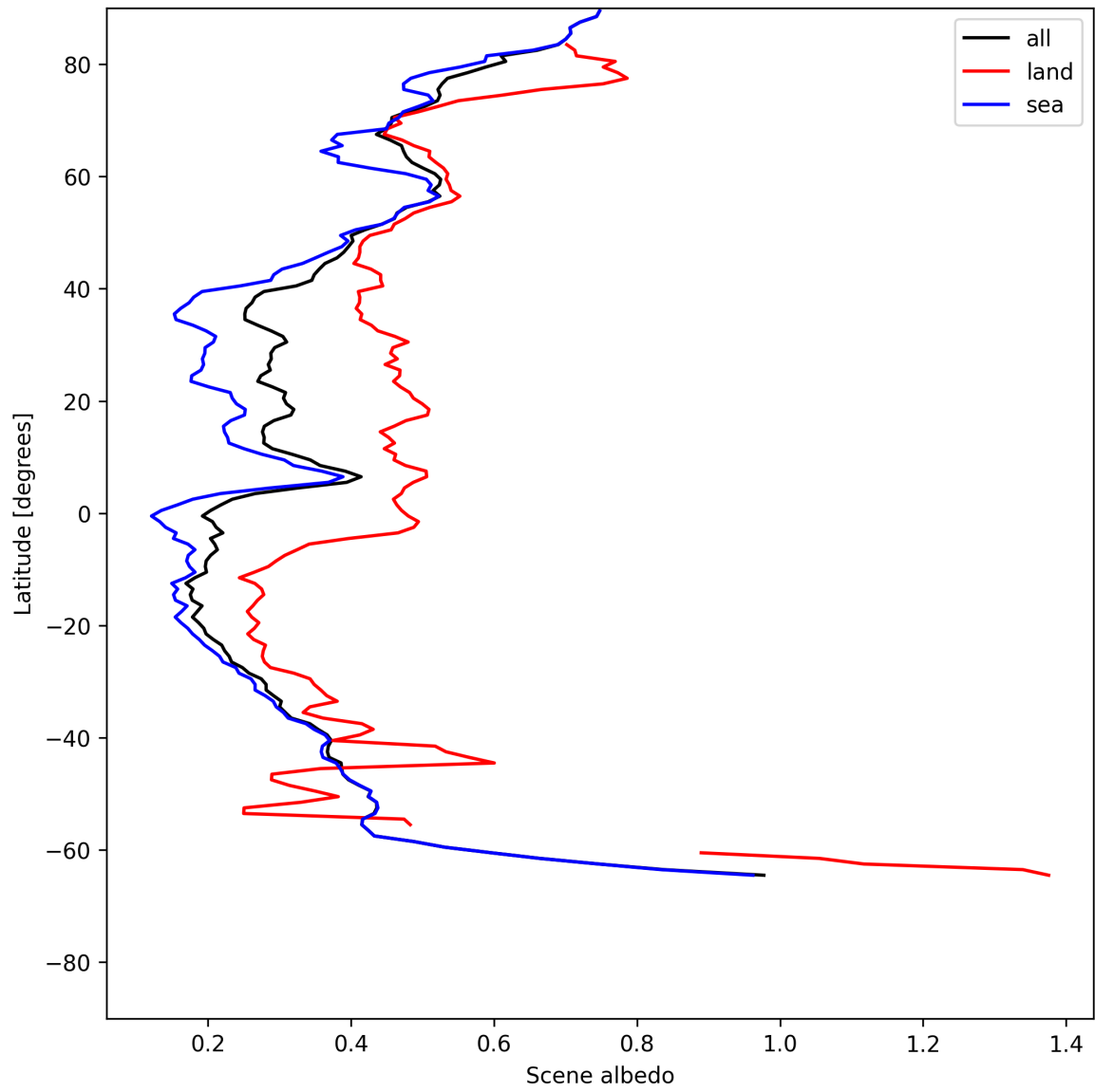
Figure 17: Zonal average of “Scene albedo” for 2025-07-03 to 2025-07-04.
