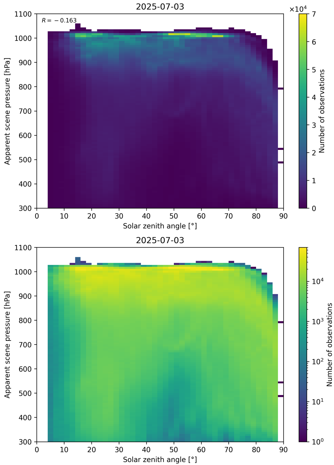
Figure 108: Scatter density plot of “Solar zenith angle” against “Apparent scene pressure” for 2025-07-03 to 2025-07-04.
