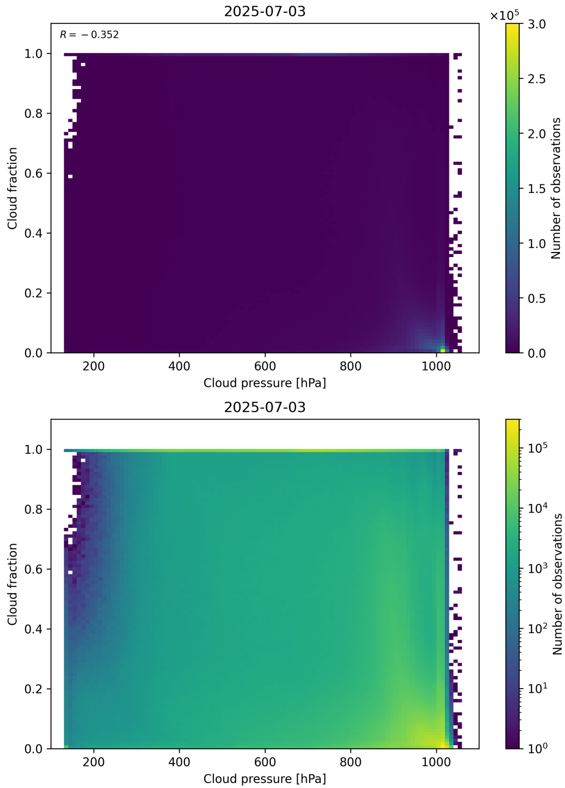
Figure 79: Scatter density plot of “Cloud pressure” against “Cloud fraction” for 2025-07-03 to 2025-07-04.
