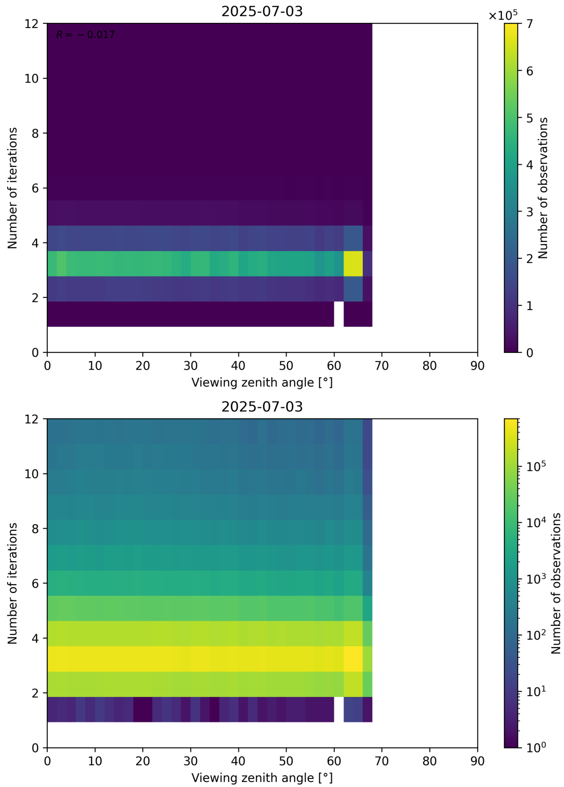
Figure 124: Scatter density plot of “Viewing zenith angle” against “Number of iterations” for 2025-07-03 to 2025-07-04.
