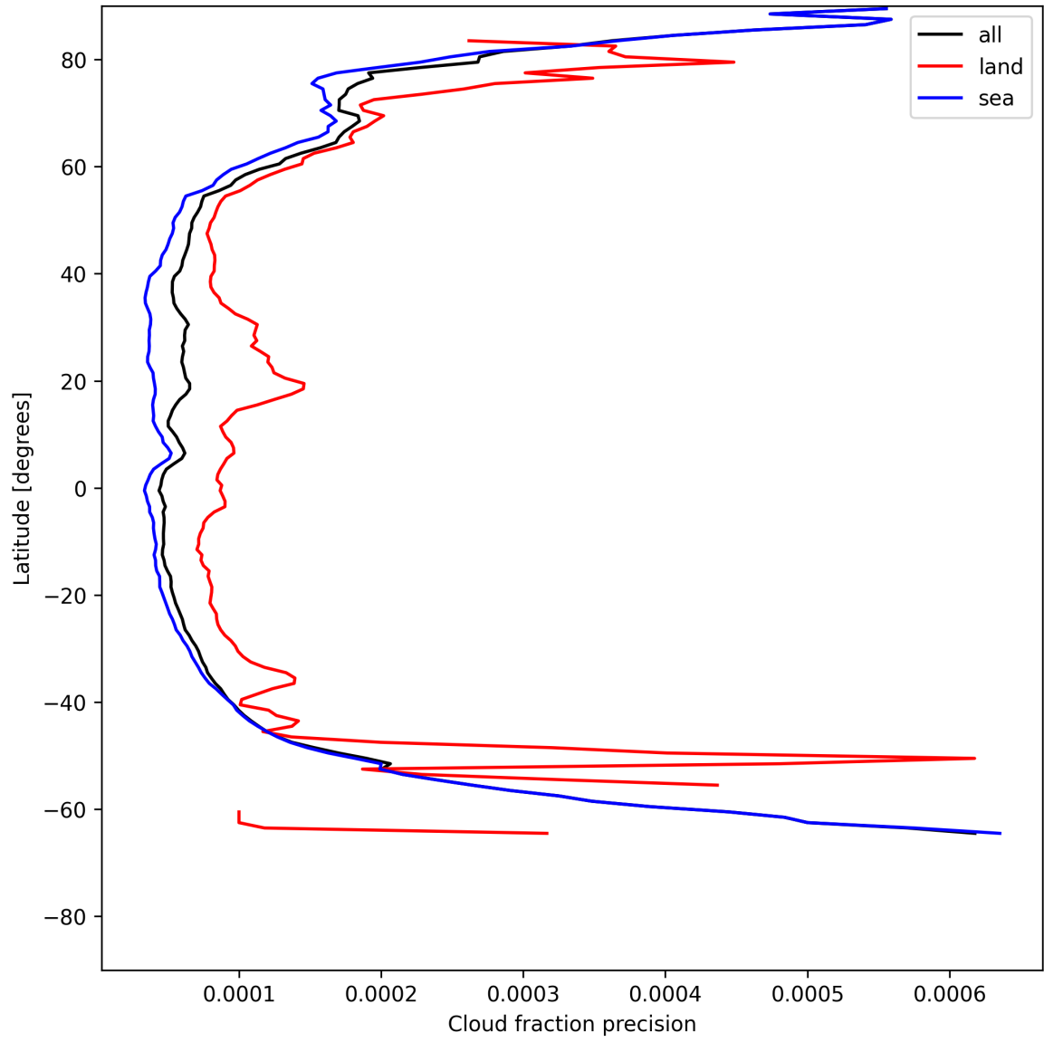
Figure 16: Zonal average of “Cloud fraction precision” for 2025-07-03 to 2025-07-04.
