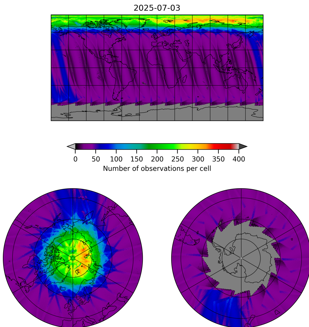
Figure 11: Map of the number of observations for 2025-07-03 to 2025-07-04
