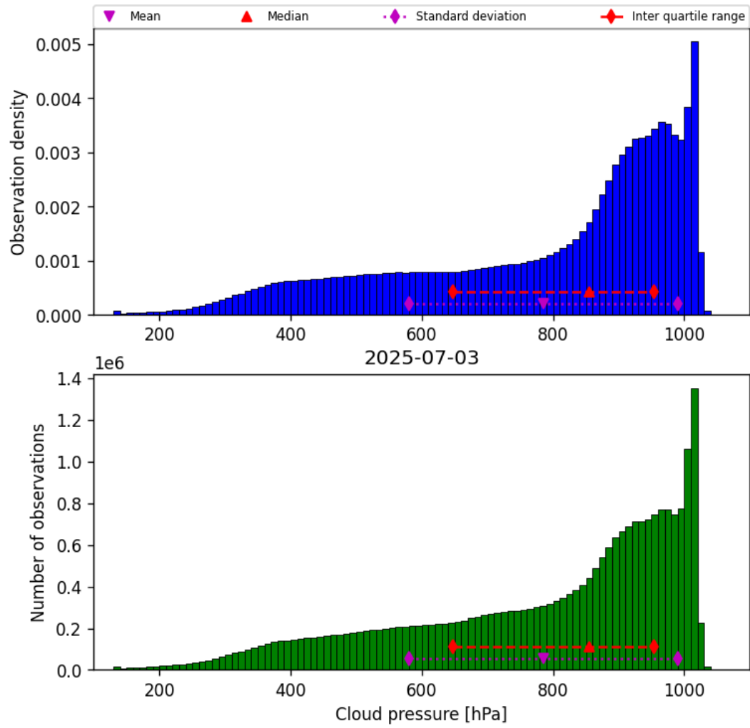
Figure 30: Histogram of “Cloud pressure” for 2025-07-03 to 2025-07-04
