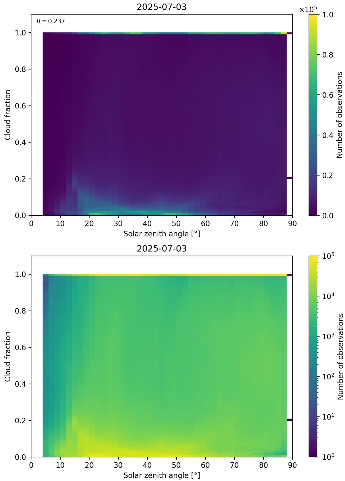
Figure 110: Scatter density plot of “Solar zenith angle” against “Cloud fraction” for 2025-07-03 to 2025-07-04.
