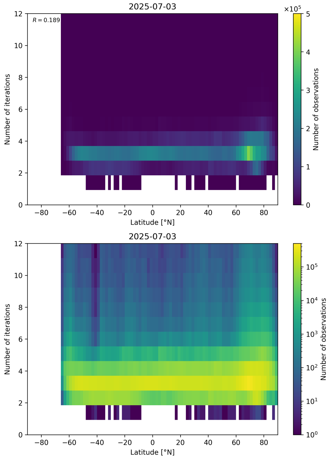
Figure 93: Scatter density plot of “Latitude” against “Number of iterations” for 2025-07-03 to 2025-07-04.
