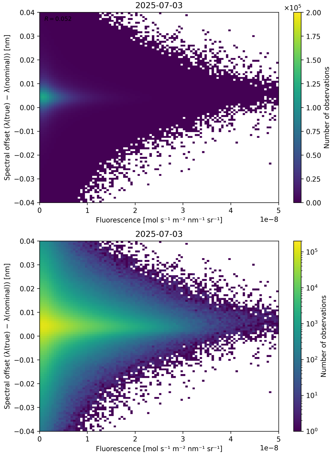
Figure 87: Scatter density plot of “Fluorescence” against “Spectral offset ( \lambda_{\text{true}} - \lambda_{\text{nominal}} )” for 2025-07-03 to 2025-07-04.
