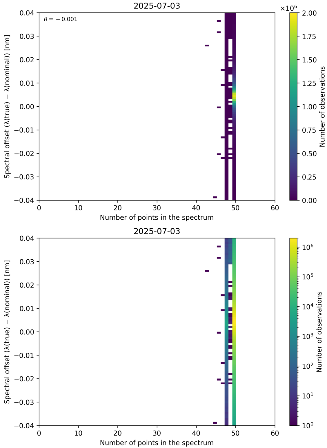
Figure 101: Scatter density plot of “Number of points in the spectrum” against “Spectral offset ( \lambda_{\text{true}} - \lambda_{\text{nominal}} )” for 2025-07-03 to 2025-07-04.
