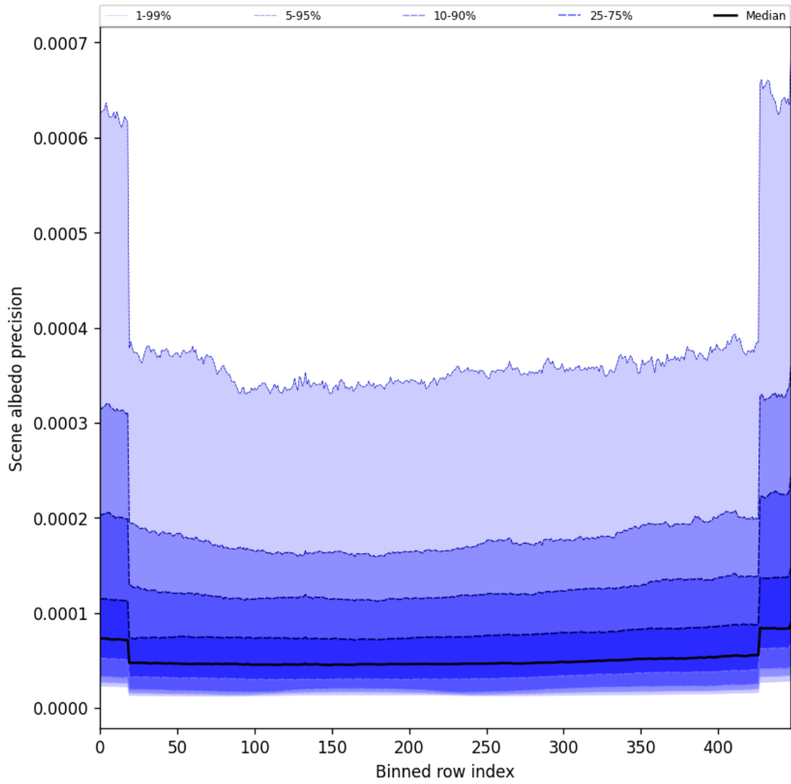
Figure 52: Along track statistics of “Scene albedo precision” for 2025-07-03 to 2025-07-04
