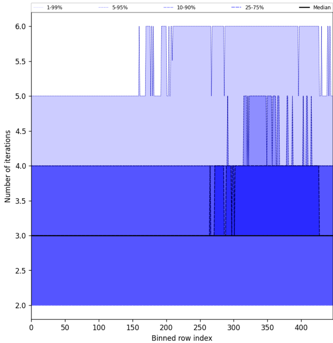
Figure 56: Along track statistics of “Number of iterations” for 2025-07-03 to 2025-07-04
