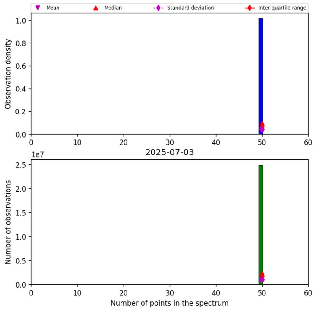
Figure 44: Histogram of “Number of points in the spectrum” for 2025-07-03 to 2025-07-04
