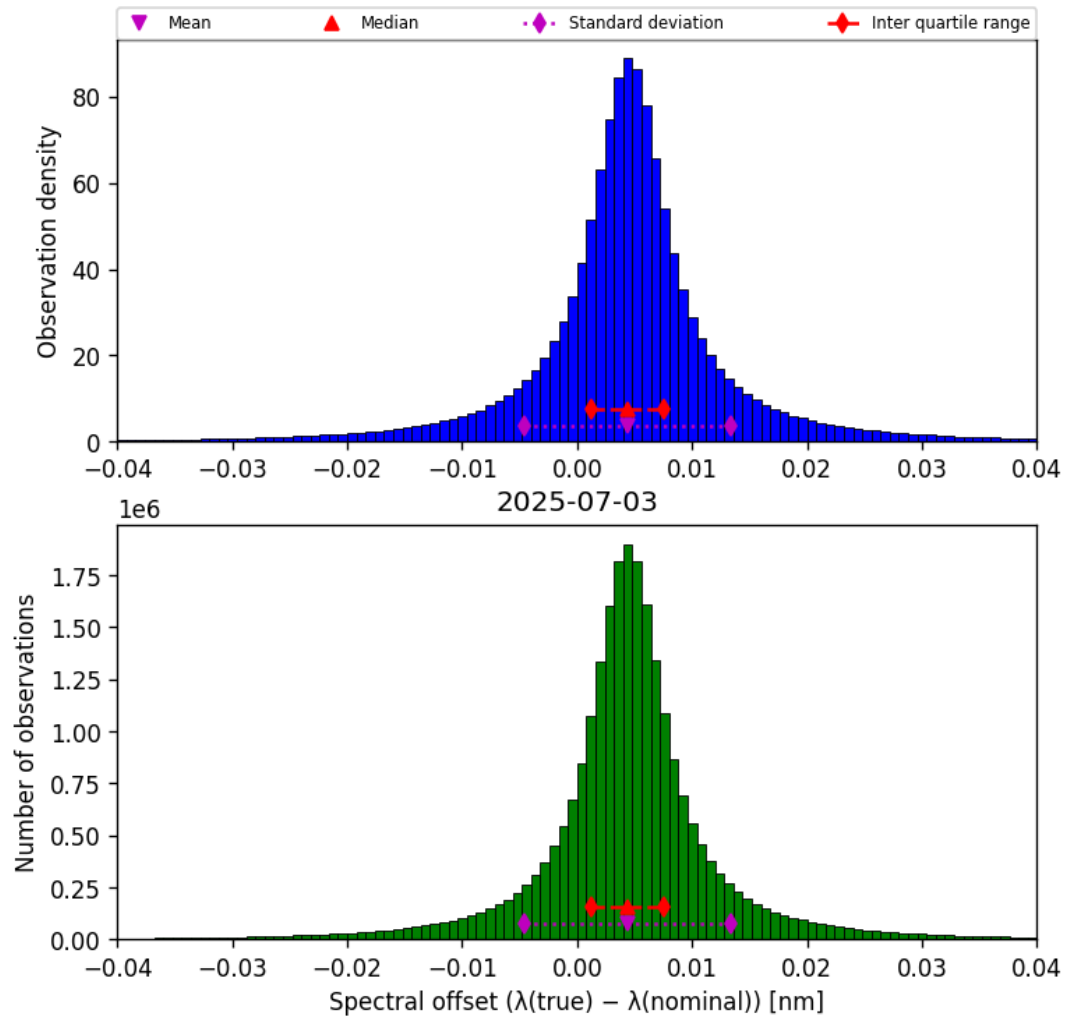
Figure 45: Histogram of “Spectral offset ( \lambda_{\text{true}} - \lambda_{\text{nominal}} )” for 2025-07-03 to 2025-07-04
