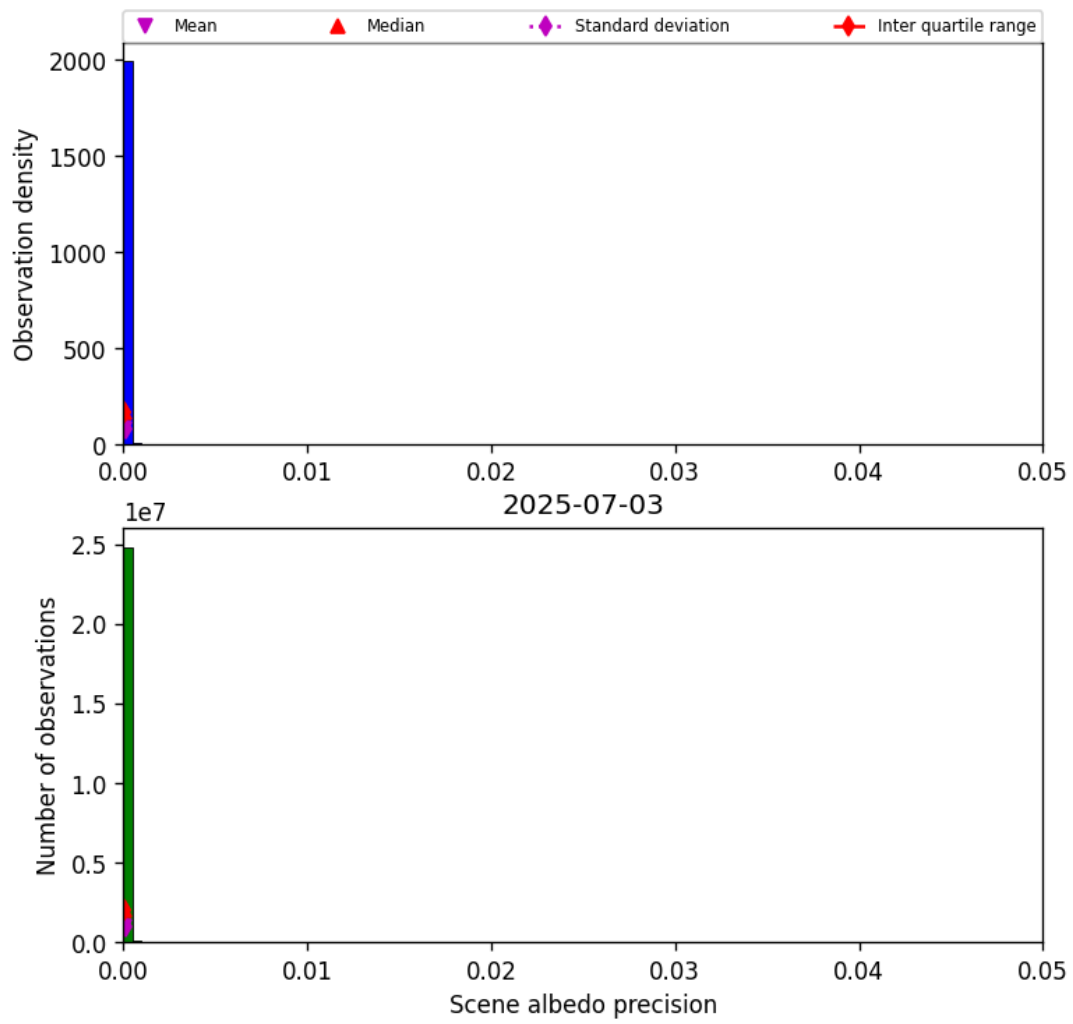
Figure 35: Histogram of “Scene albedo precision” for 2025-07-03 to 2025-07-04
