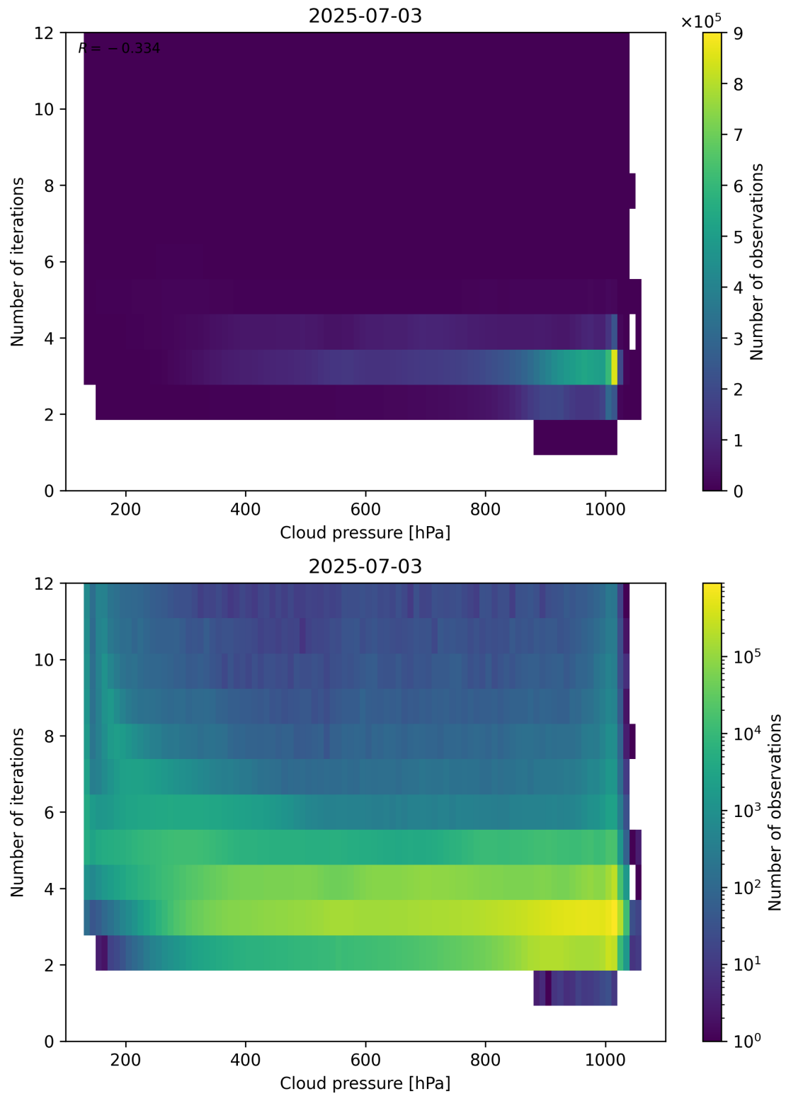
Figure 81: Scatter density plot of “Cloud pressure” against “Number of iterations” for 2025-07-03 to 2025-07-04.
