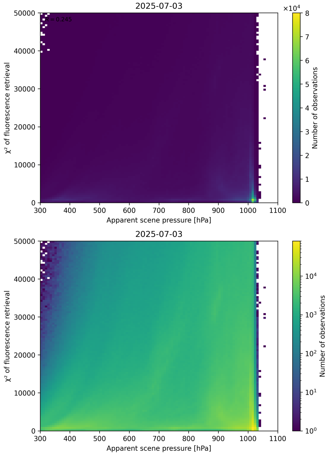
Figure 63: Scatter density plot of “Apparent scene pressure” against “ \chi^2 of fluorescence retrieval” for 2025-07-03 to 2025-07-04.
