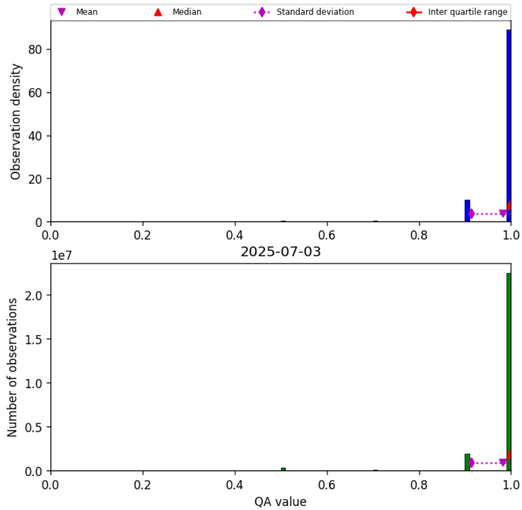
Figure 29: Histogram of “QA value” for 2025-07-03 to 2025-07-04
