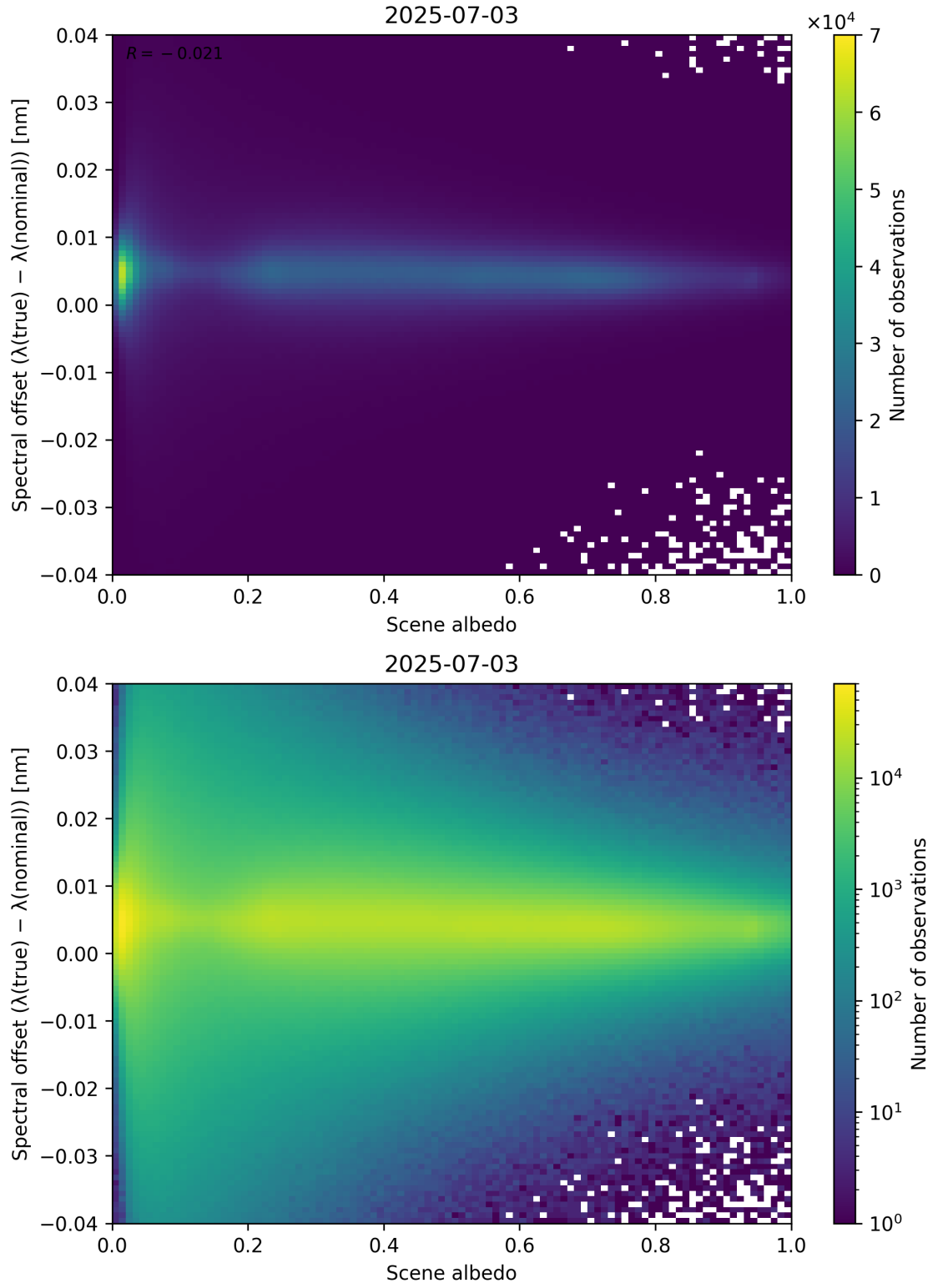
Figure 107: Scatter density plot of “Scene albedo” against “Spectral offset ( \lambda_{\text{true}} - \lambda_{\text{nominal}} )” for 2025-07-03 to 2025-07-04.
