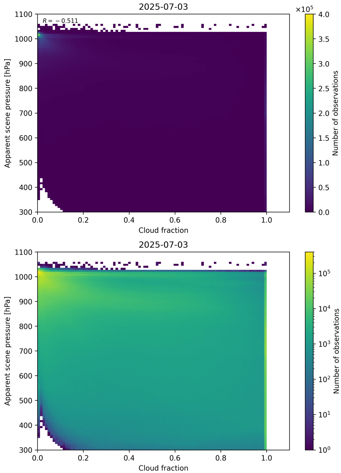
Figure 70: Scatter density plot of “Cloud fraction” against “Apparent scene pressure” for 2025-07-03 to 2025-07-04.
