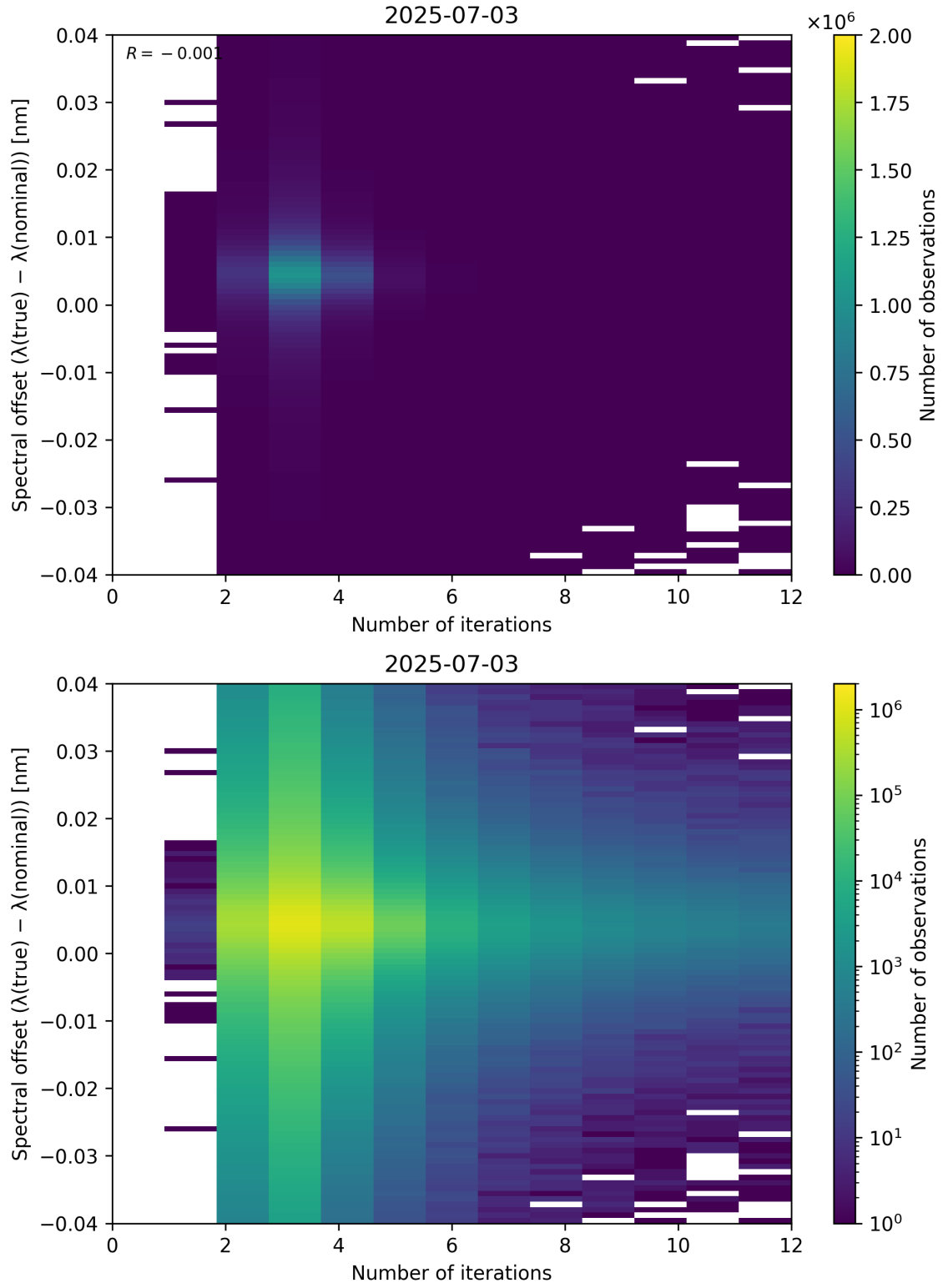
Figure 100: Scatter density plot of “Number of iterations” against “Spectral offset ( \lambda_{\text{true}} - \lambda_{\text{nominal}} )” for 2025-07-03 to 2025-07-04.
