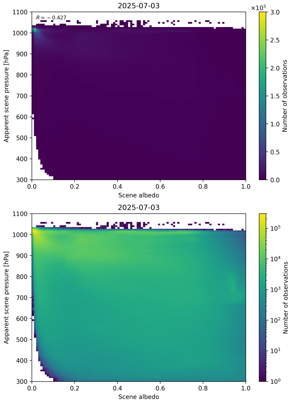
Figure 102: Scatter density plot of “Scene albedo” against “Apparent scene pressure” for 2025-07-03 to 2025-07-04.
