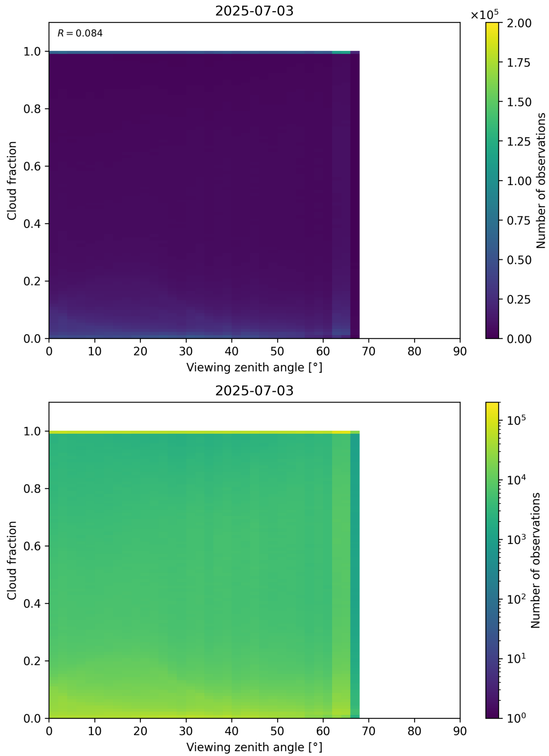
Figure 120: Scatter density plot of “Viewing zenith angle” against “Cloud fraction” for 2025-07-03 to 2025-07-04.
