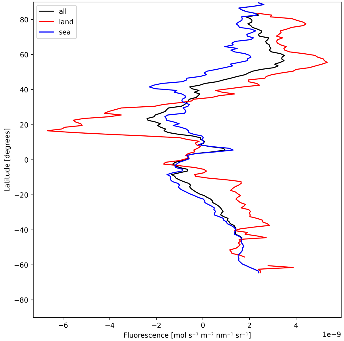
Figure 23: Zonal average of “Fluorescence” for 2025-07-03 to 2025-07-04.
