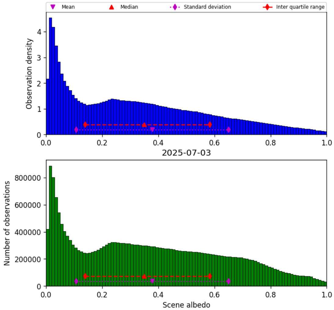
Figure 34: Histogram of “Scene albedo” for 2025-07-03 to 2025-07-04
