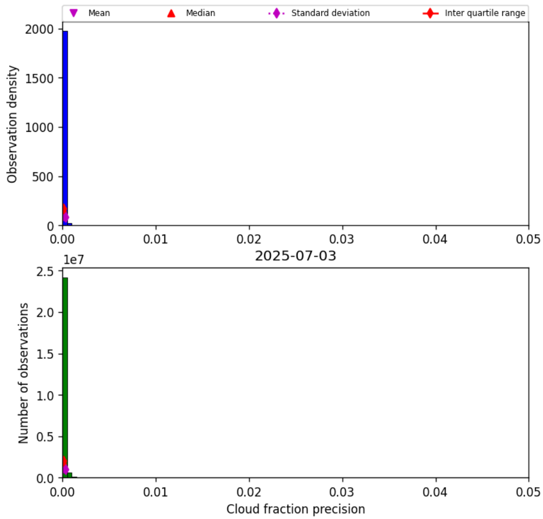
Figure 33: Histogram of “Cloud fraction precision” for 2025-07-03 to 2025-07-04
