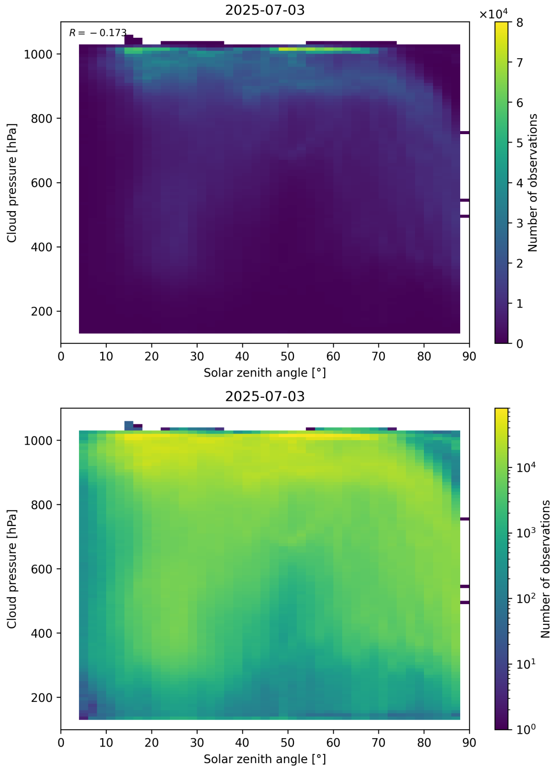
Figure 111: Scatter density plot of “Solar zenith angle” against “Cloud pressure” for 2025-07-03 to 2025-07-04.
