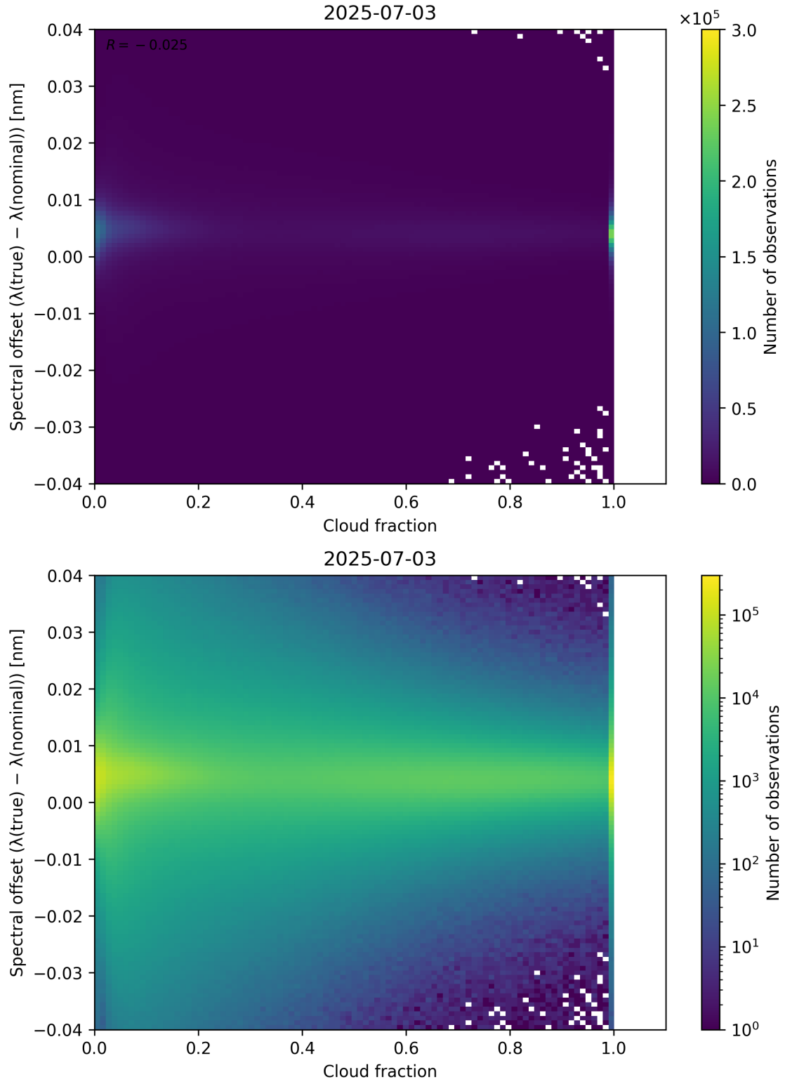
Figure 76: Scatter density plot of “Cloud fraction” against “Spectral offset ( \lambda_{\text{true}} - \lambda_{\text{nominal}} )” for 2025-07-03 to 2025-07-04.
