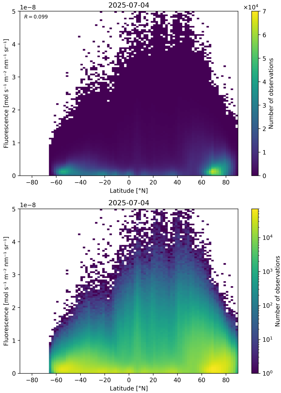
Figure 92: Scatter density plot of “Latitude” against “Fluorescence” for 2025-07-03 to 2025-07-05.
