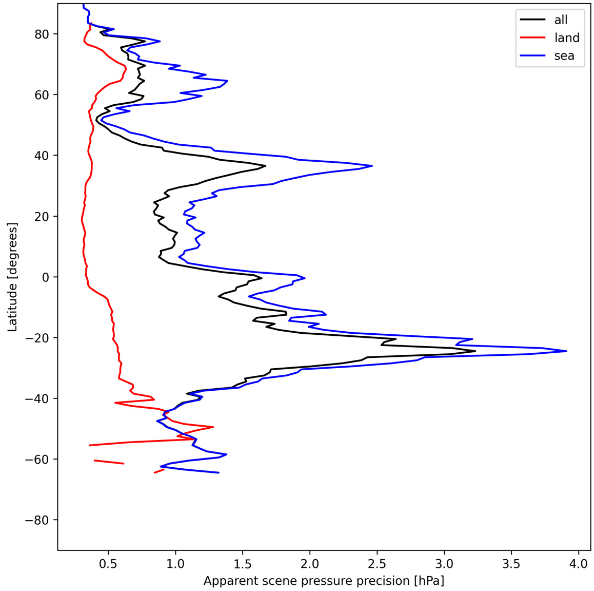
Figure 20: Zonal average of “Apparent scene pressure precision” for 2025-07-03 to 2025-07-05.
