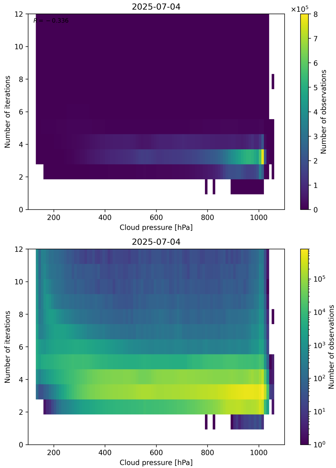
Figure 81: Scatter density plot of “Cloud pressure” against “Number of iterations” for 2025-07-03 to 2025-07-05.
