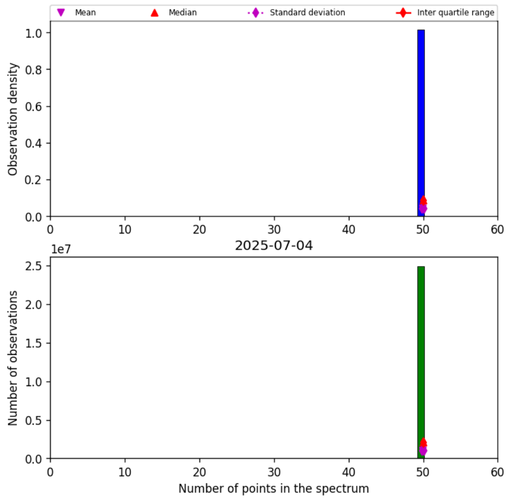
Figure 44: Histogram of “Number of points in the spectrum” for 2025-07-03 to 2025-07-05
