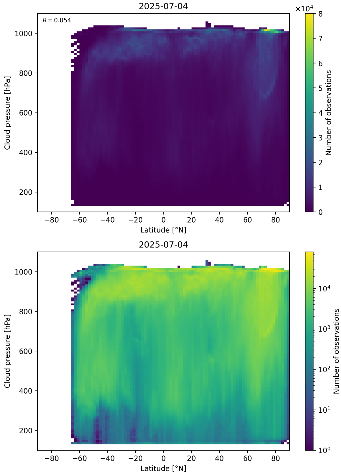
Figure 91: Scatter density plot of “Latitude” against “Cloud pressure” for 2025-07-03 to 2025-07-05.
