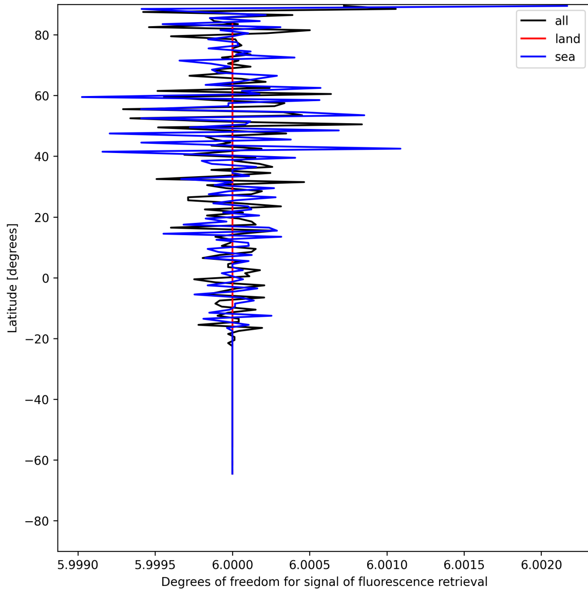
Figure 26: Zonal average of “Degrees of freedom for signal of fluorescence retrieval” for 2025-07-03 to 2025-07-05.
