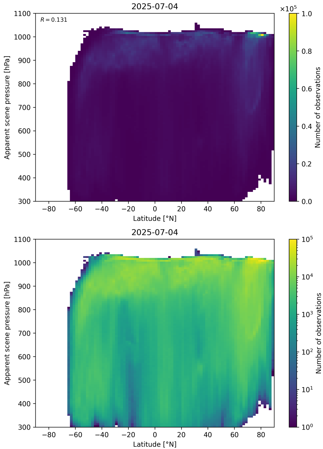
Figure 88: Scatter density plot of “Latitude” against “Apparent scene pressure” for 2025-07-03 to 2025-07-05.
