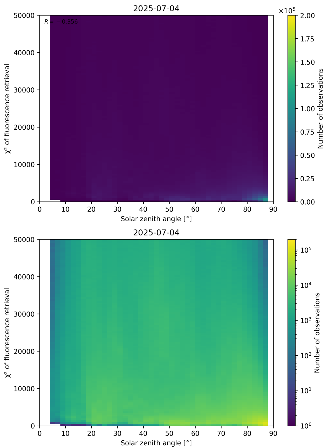
Figure 109: Scatter density plot of “Solar zenith angle” against “ \chi^2 of fluorescence retrieval” for 2025-07-03 to 2025-07-05.
