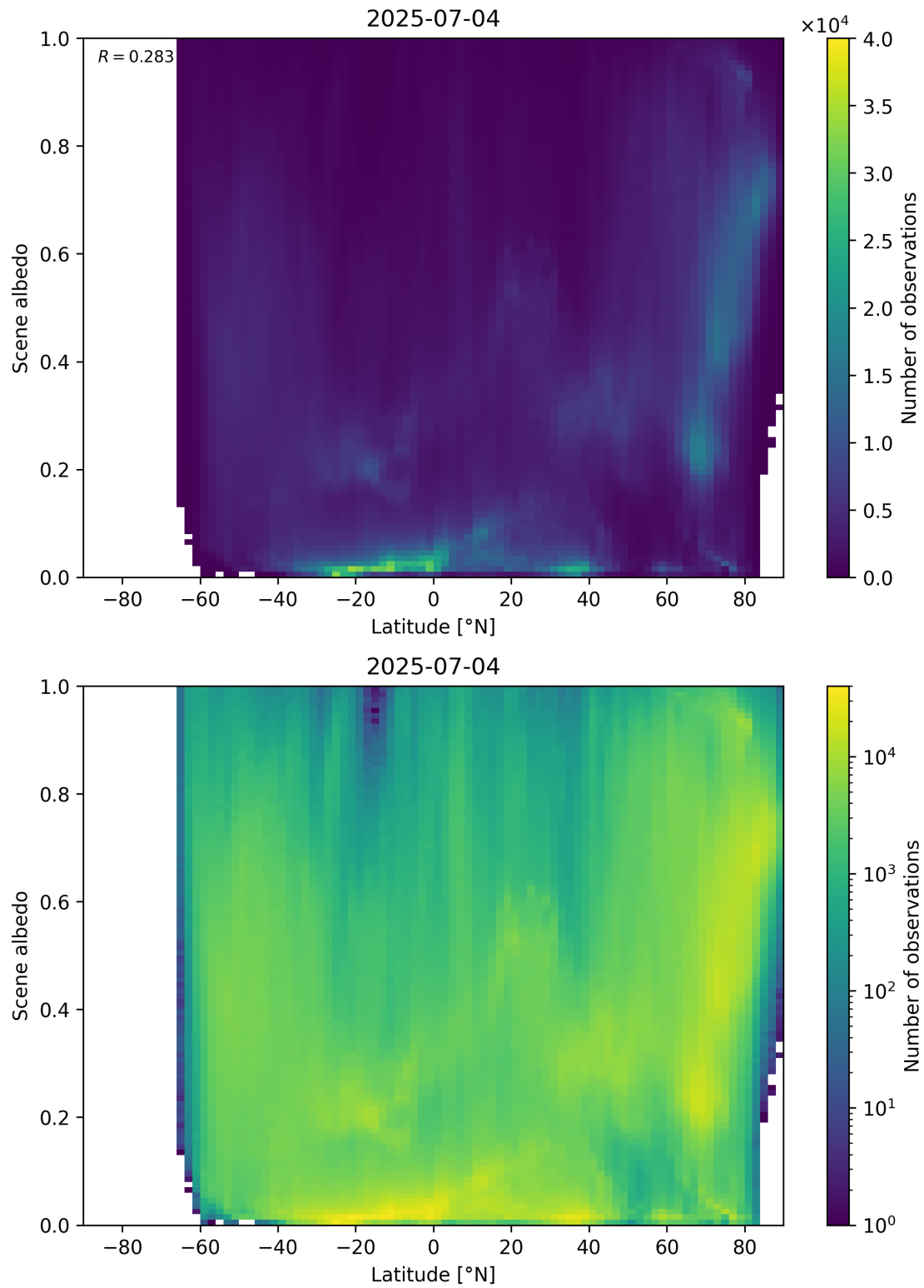
Figure 95: Scatter density plot of “Latitude” against “Scene albedo” for 2025-07-03 to 2025-07-05.
