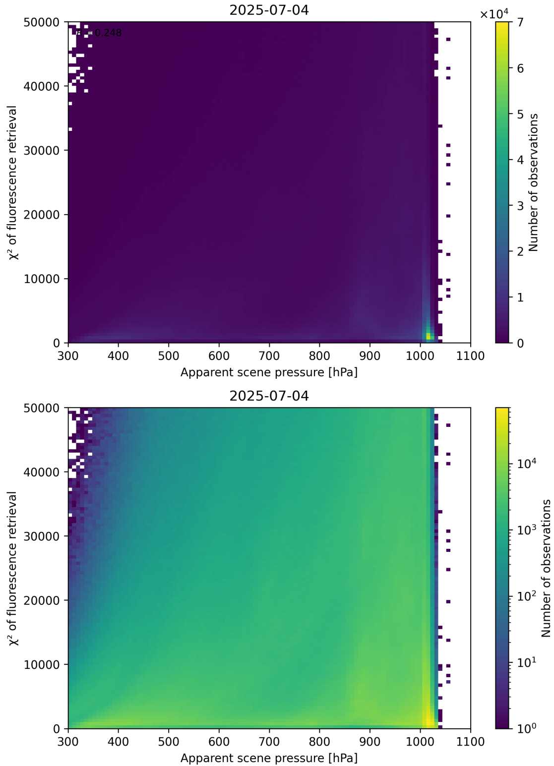
Figure 63: Scatter density plot of “Apparent scene pressure” against “ \chi^2 of fluorescence retrieval” for 2025-07-03 to 2025-07-05.
