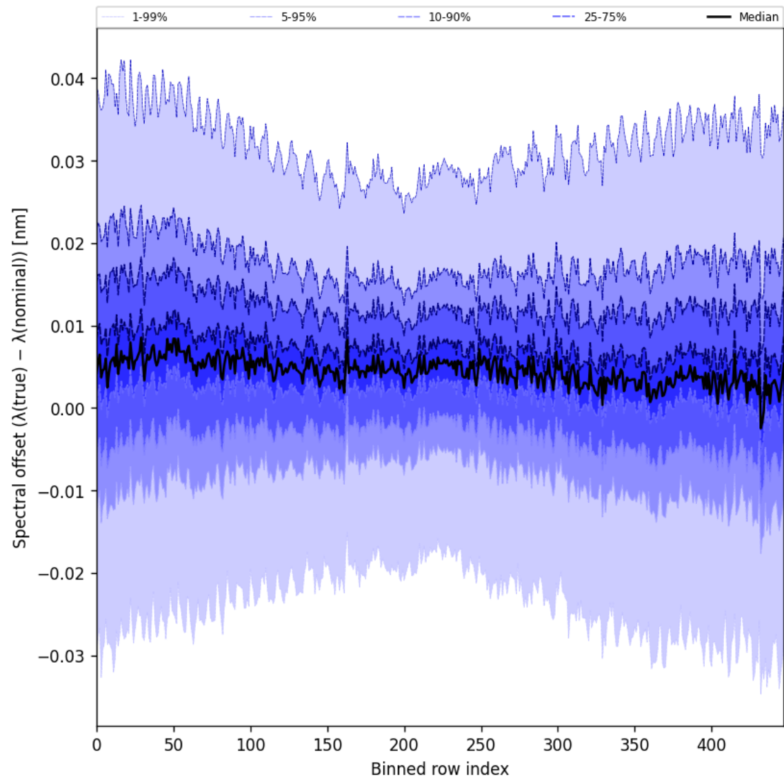
Figure 62: Along track statistics of “Spectral offset ( \lambda_{\text{true}} - \lambda_{\text{nominal}} )” for 2025-07-03 to 2025-07-05
