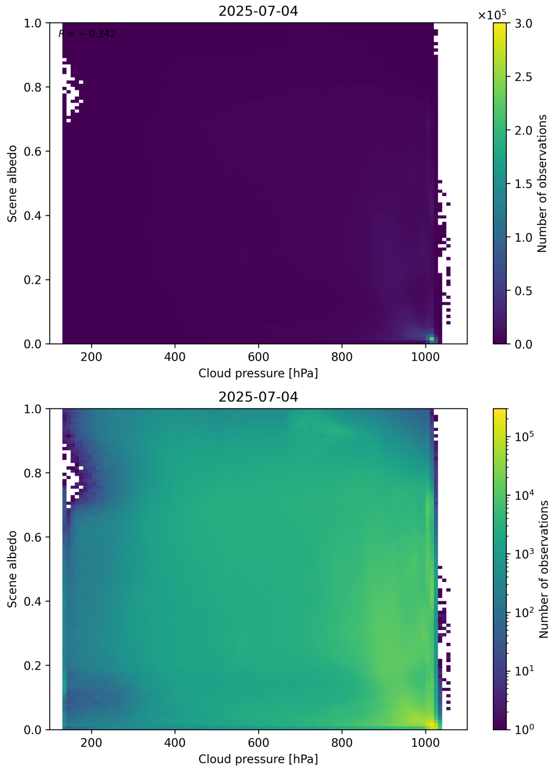
Figure 83: Scatter density plot of “Cloud pressure” against “Scene albedo” for 2025-07-03 to 2025-07-05.
