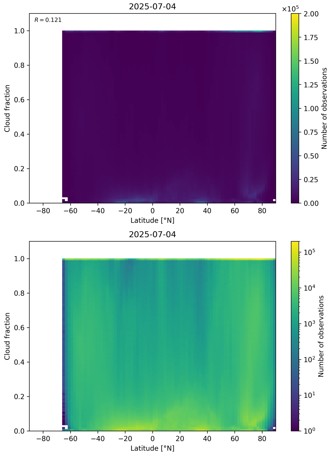
Figure 90: Scatter density plot of “Latitude” against “Cloud fraction” for 2025-07-03 to 2025-07-05.
