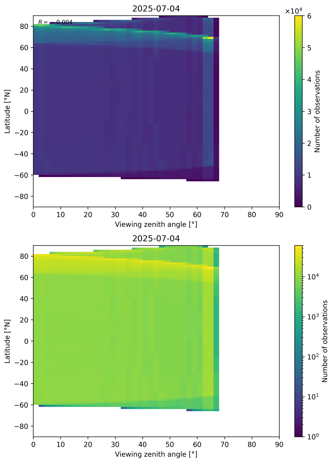
Figure 123: Scatter density plot of “Viewing zenith angle” against “Latitude” for 2025-07-03 to 2025-07-05.
