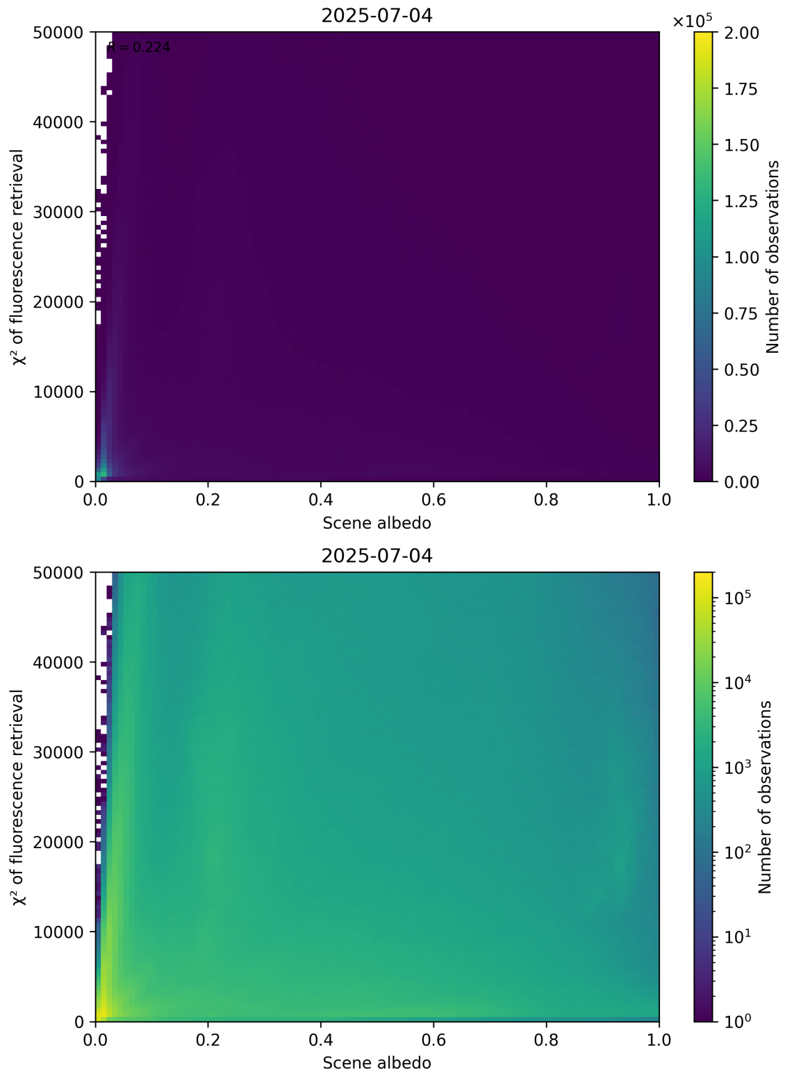
Figure 103: Scatter density plot of “Scene albedo” against “ \chi^2 of fluorescence retrieval” for 2025-07-03 to 2025-07-05.
