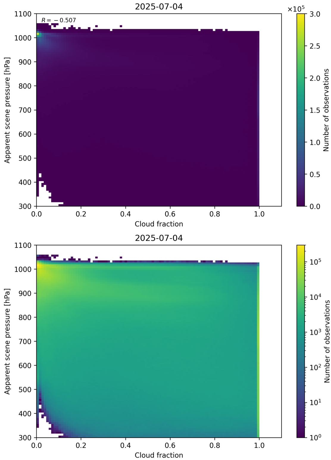
Figure 70: Scatter density plot of “Cloud fraction” against “Apparent scene pressure” for 2025-07-03 to 2025-07-05.
