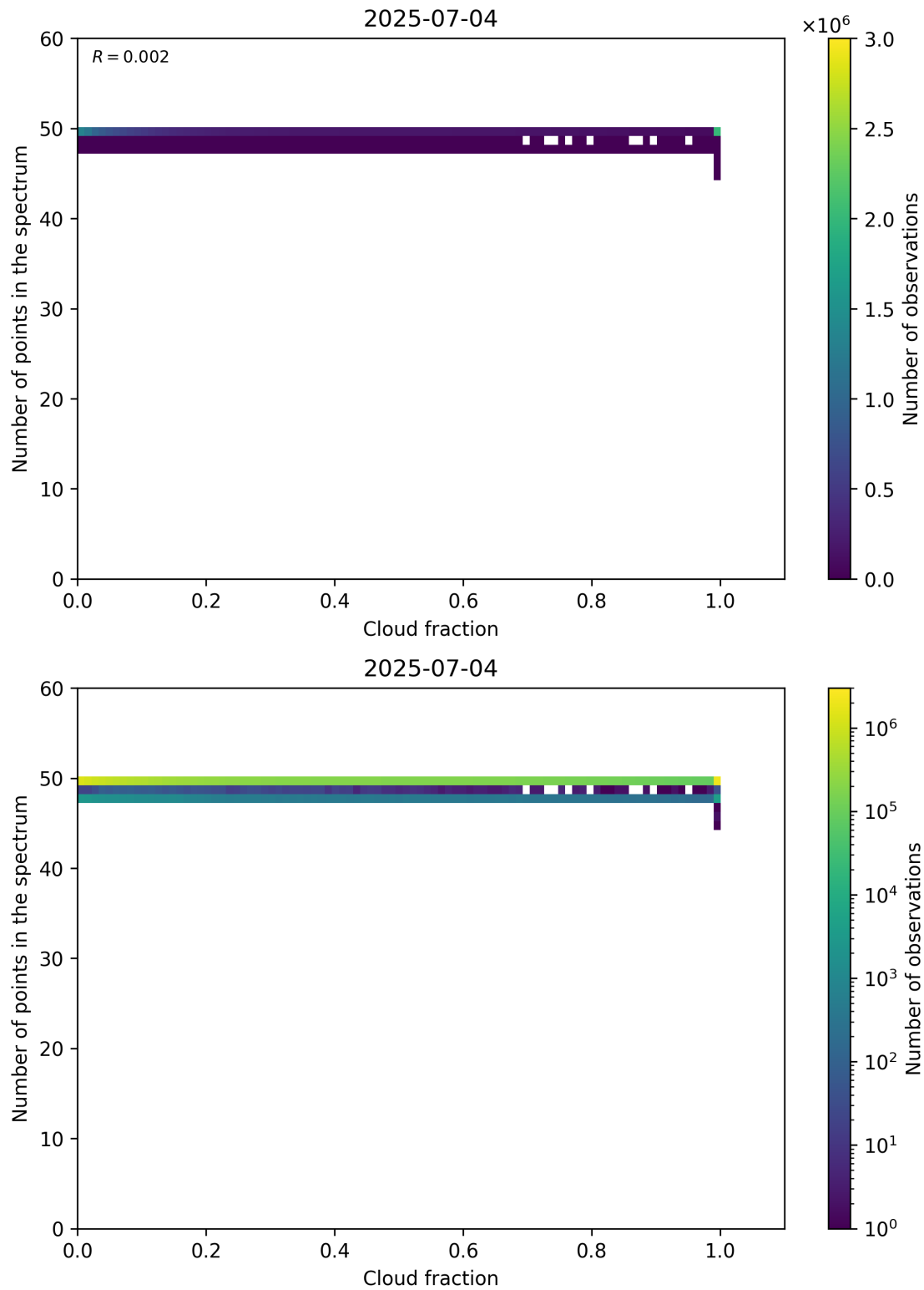
Figure 74: Scatter density plot of “Cloud fraction” against “Number of points in the spectrum” for 2025-07-03 to 2025-07-05.
