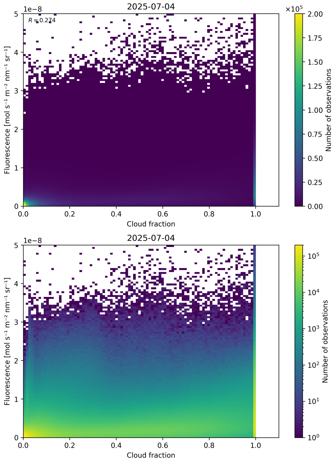
Figure 72: Scatter density plot of “Cloud fraction” against “Fluorescence” for 2025-07-03 to 2025-07-05.
