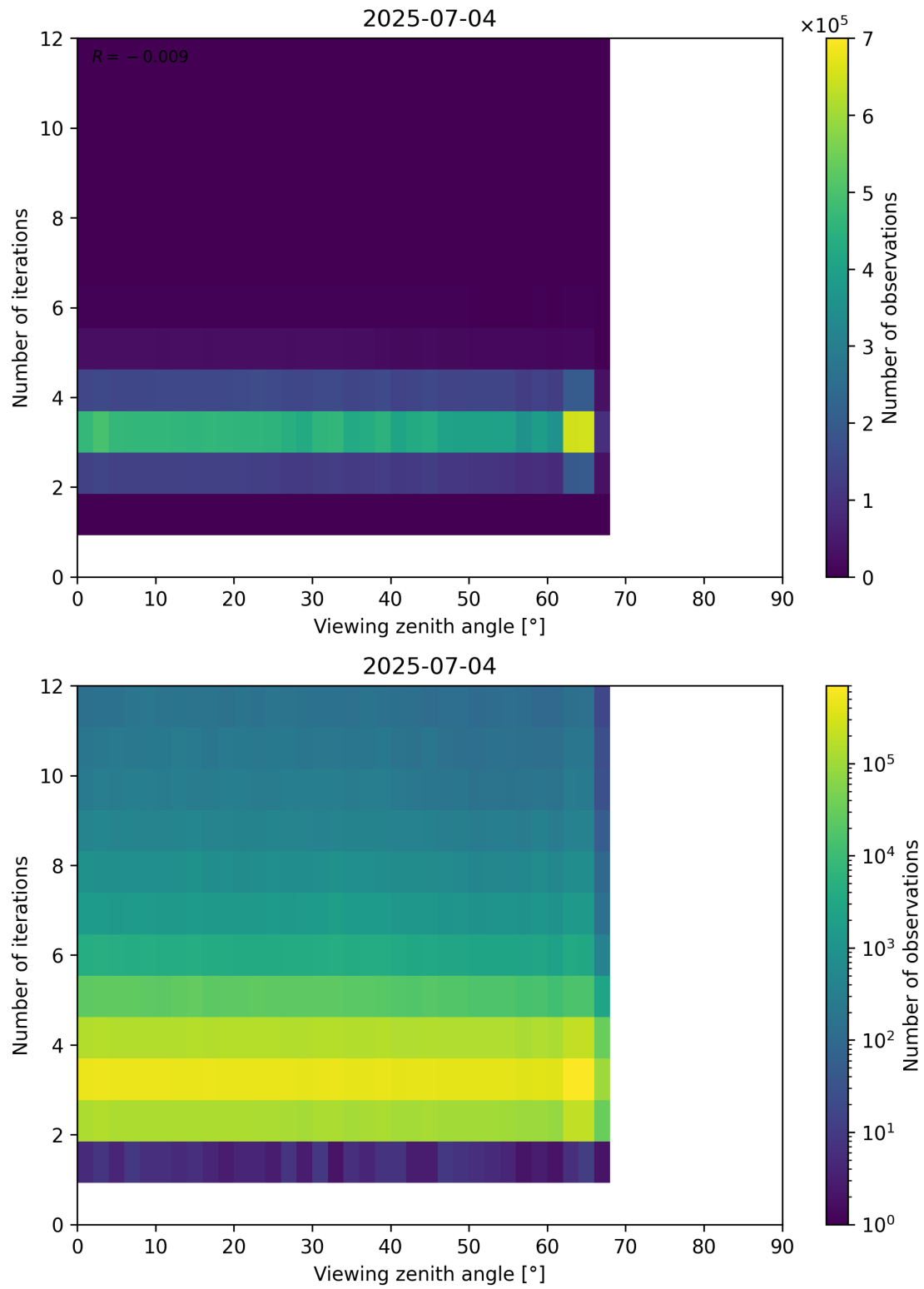
Figure 124: Scatter density plot of “Viewing zenith angle” against “Number of iterations” for 2025-07-03 to 2025-07-05.
