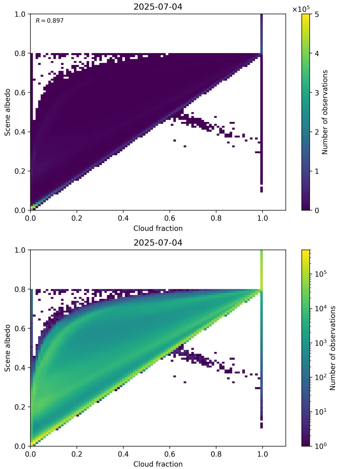
Figure 75: Scatter density plot of “Cloud fraction” against “Scene albedo” for 2025-07-03 to 2025-07-05.
