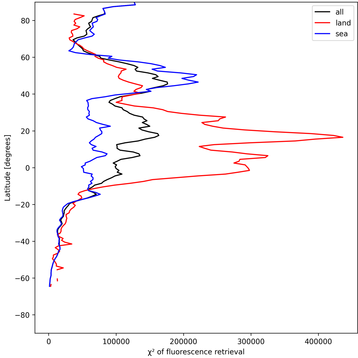
Figure 25: Zonal average of “ \chi^2 of fluorescence retrieval” for 2025-07-03 to 2025-07-05.
