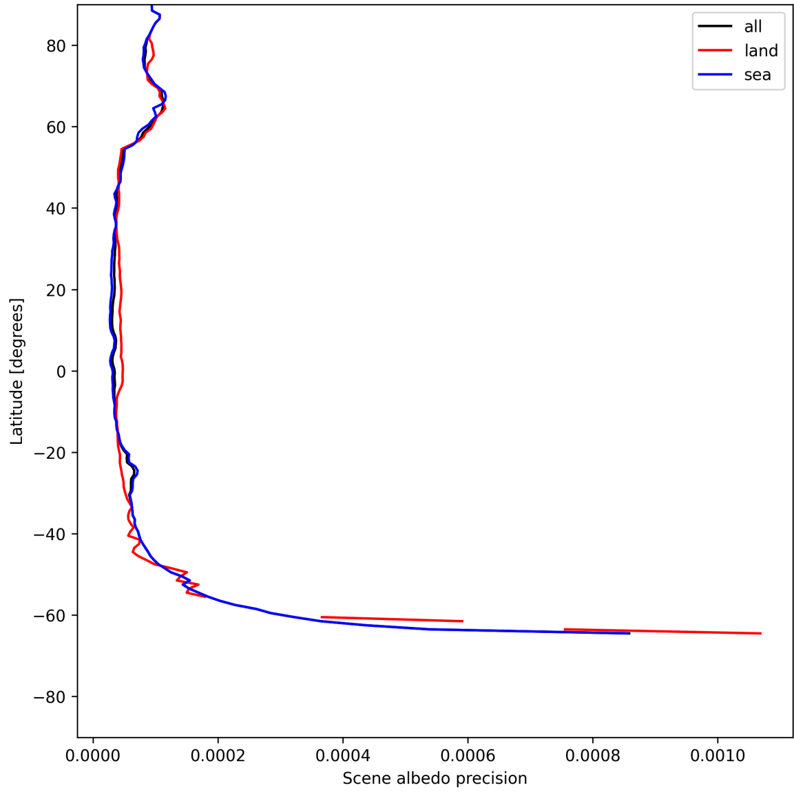
Figure 18: Zonal average of “Scene albedo precision” for 2025-07-03 to 2025-07-05.
