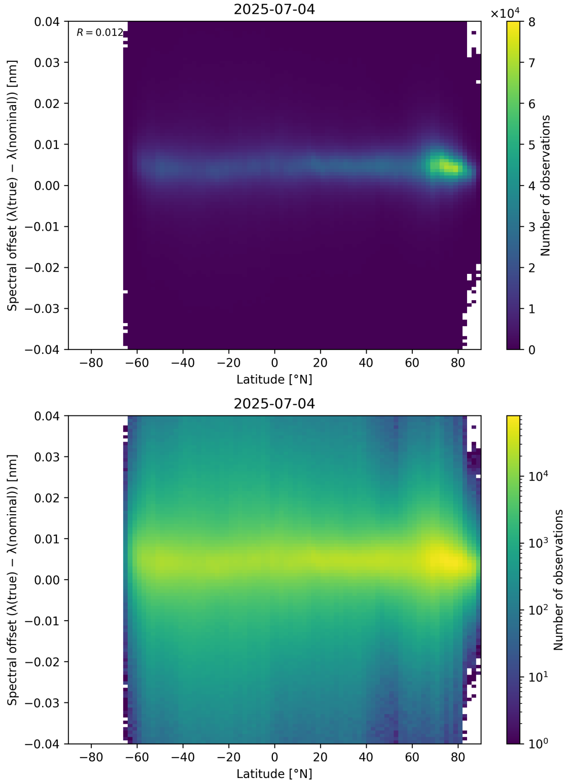
Figure 96: Scatter density plot of “Latitude” against “Spectral offset ( \lambda_{\text{true}} - \lambda_{\text{nominal}} )” for 2025-07-03 to 2025-07-05.
