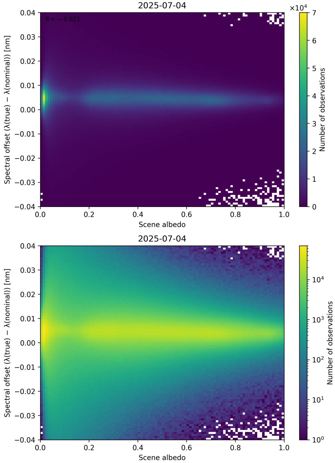
Figure 107: Scatter density plot of “Scene albedo” against “Spectral offset ( \lambda_{\text{true}} - \lambda_{\text{nominal}} )” for 2025-07-03 to 2025-07-05.
