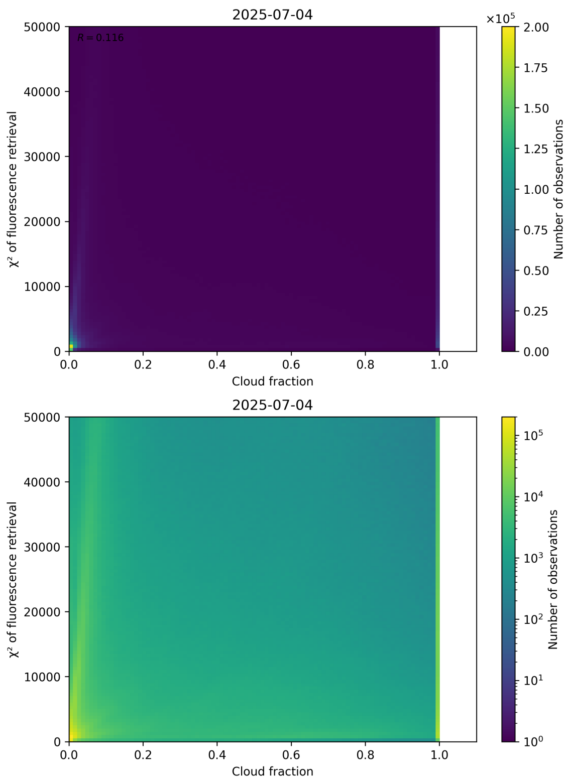
Figure 71: Scatter density plot of “Cloud fraction” against “ \chi^2 of fluorescence retrieval” for 2025-07-03 to 2025-07-05.
