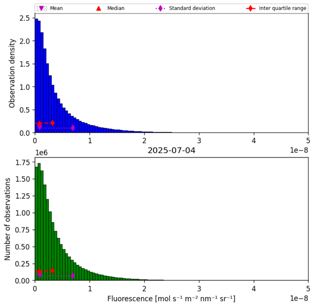
Figure 40: Histogram of “Fluorescence” for 2025-07-03 to 2025-07-05
