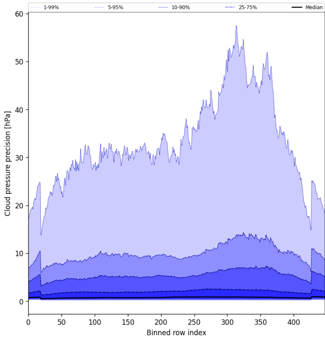
Figure 48: Along track statistics of “Cloud pressure precision” for 2025-07-03 to 2025-07-05
