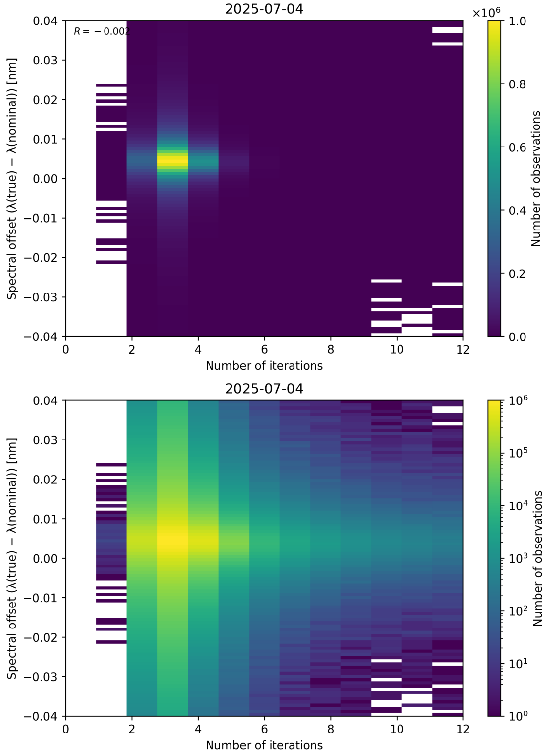
Figure 100: Scatter density plot of “Number of iterations” against “Spectral offset ( \lambda_{\text{true}} - \lambda_{\text{nominal}} )” for 2025-07-03 to 2025-07-05.
