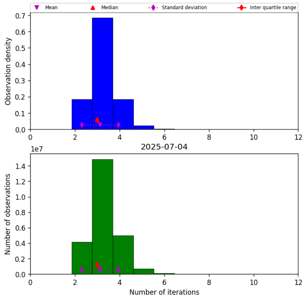
Figure 39: Histogram of “Number of iterations” for 2025-07-03 to 2025-07-05
