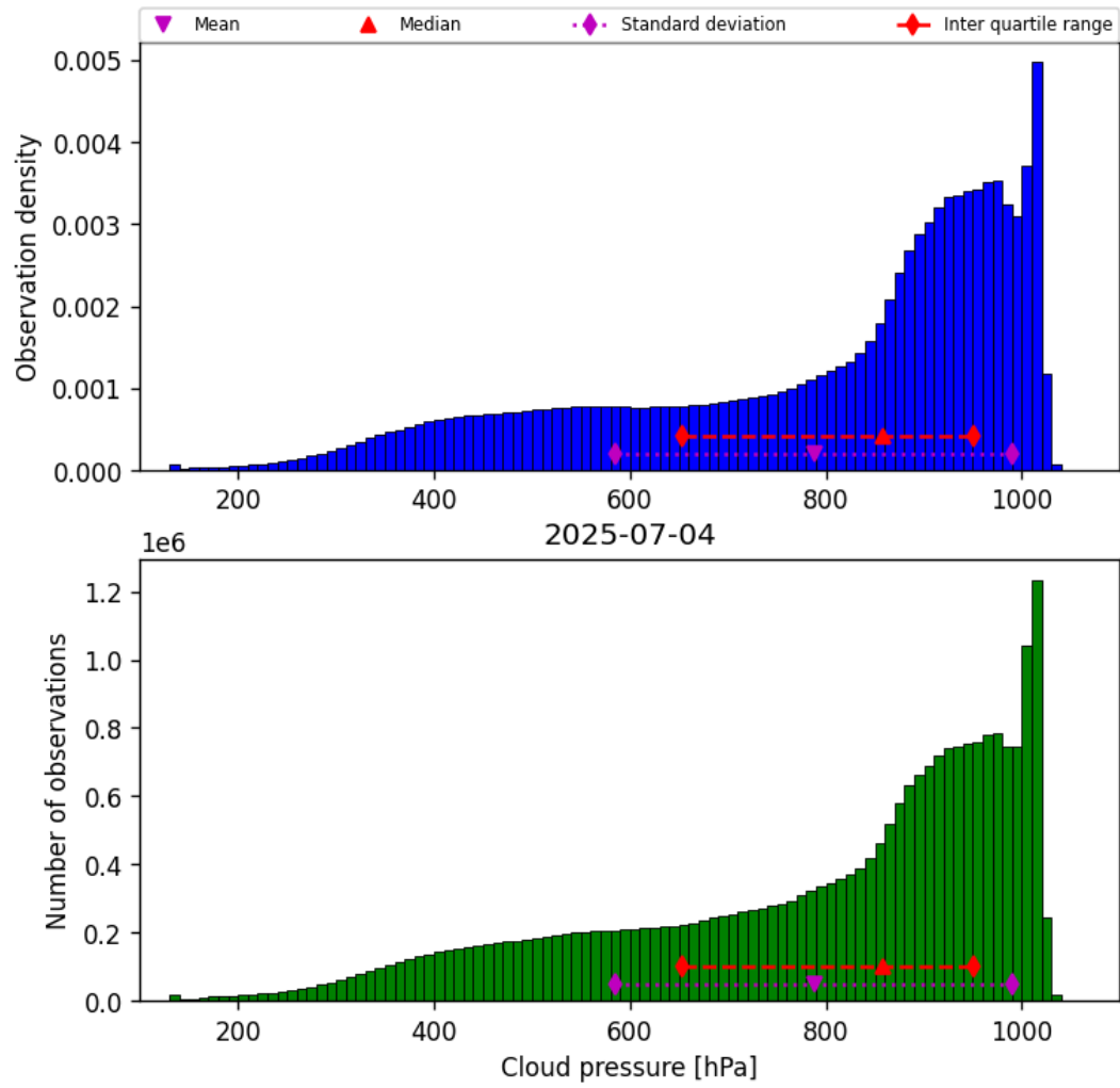
Figure 30: Histogram of “Cloud pressure” for 2025-07-03 to 2025-07-05
