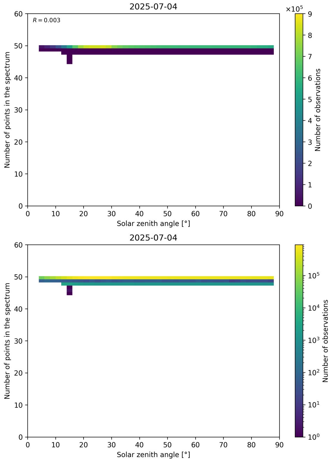
Figure 115: Scatter density plot of “Solar zenith angle” against “Number of points in the spectrum” for 2025-07-03 to 2025-07-05.
