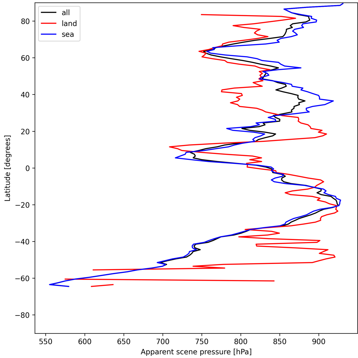
Figure 19: Zonal average of “Apparent scene pressure” for 2025-07-03 to 2025-07-05.
