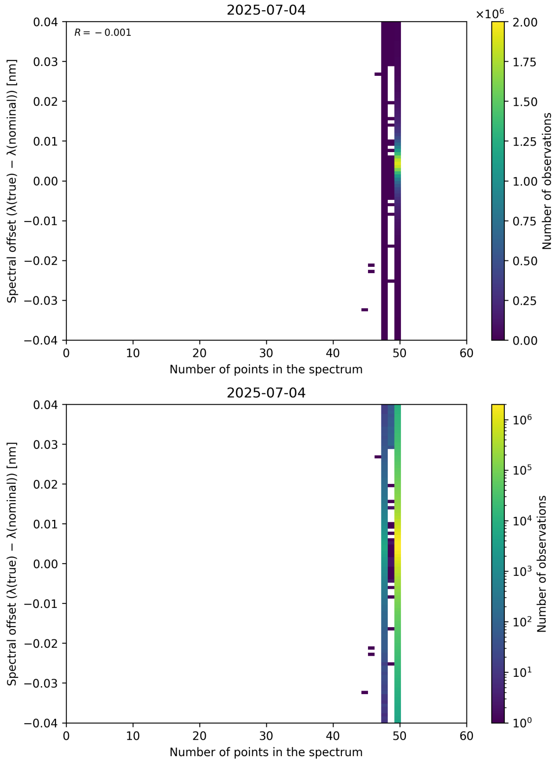
Figure 101: Scatter density plot of “Number of points in the spectrum” against “Spectral offset ( \lambda_{\text{true}} - \lambda_{\text{nominal}} )” for 2025-07-03 to 2025-07-05.
