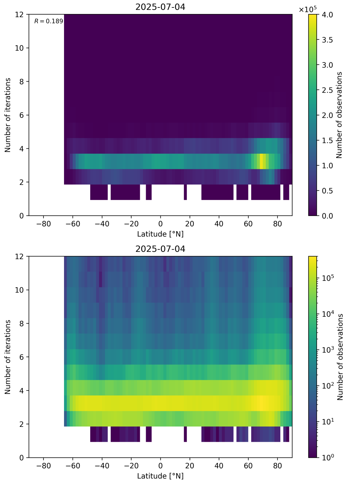
Figure 93: Scatter density plot of “Latitude” against “Number of iterations” for 2025-07-03 to 2025-07-05.
