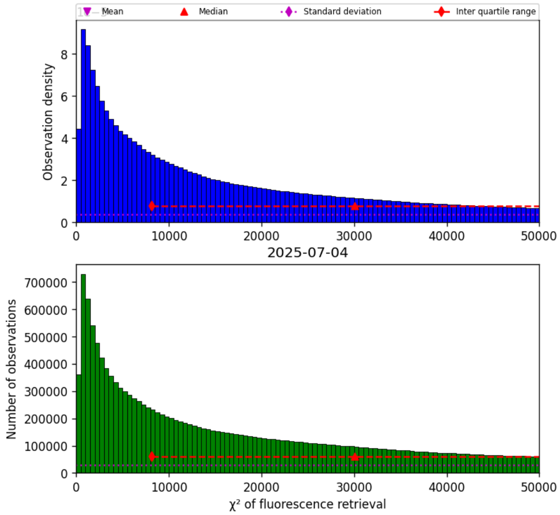
Figure 42: Histogram of “ \chi^2 of fluorescence retrieval” for 2025-07-03 to 2025-07-05
