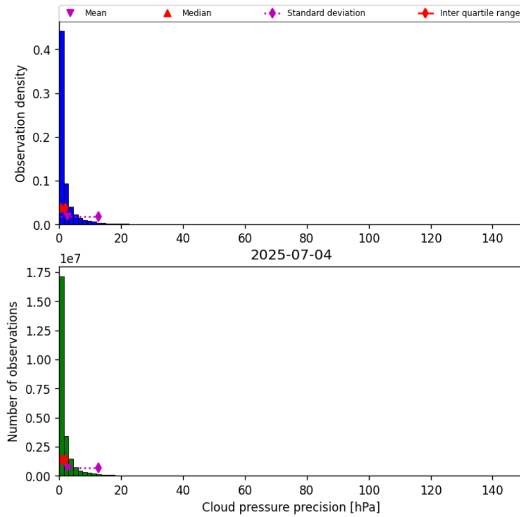
Figure 31: Histogram of “Cloud pressure precision” for 2025-07-03 to 2025-07-05
