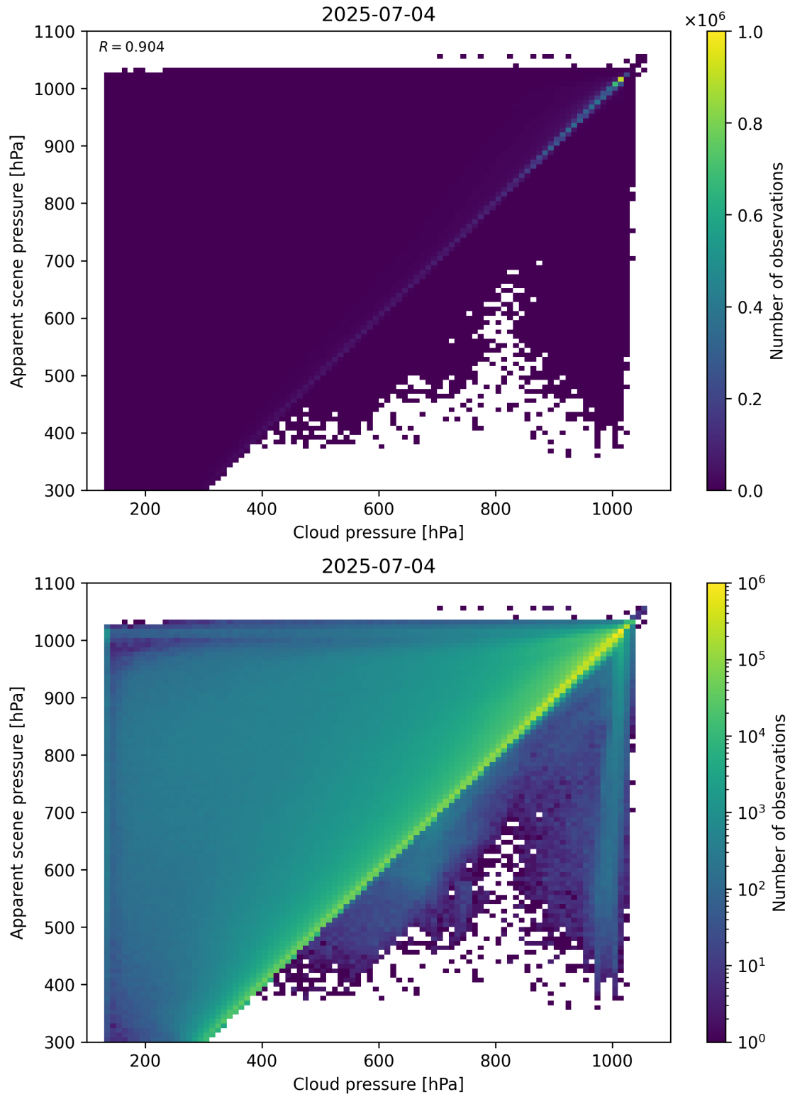
Figure 77: Scatter density plot of “Cloud pressure” against “Apparent scene pressure” for 2025-07-03 to 2025-07-05.
