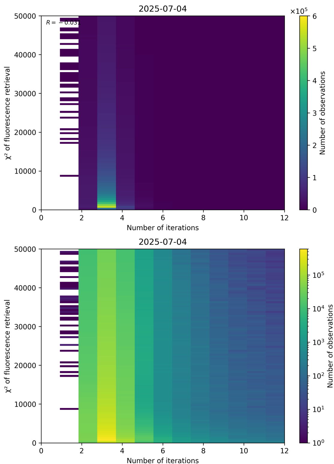
Figure 97: Scatter density plot of “Number of iterations” against “ \chi^2 of fluorescence retrieval” for 2025-07-03 to 2025-07-05.
