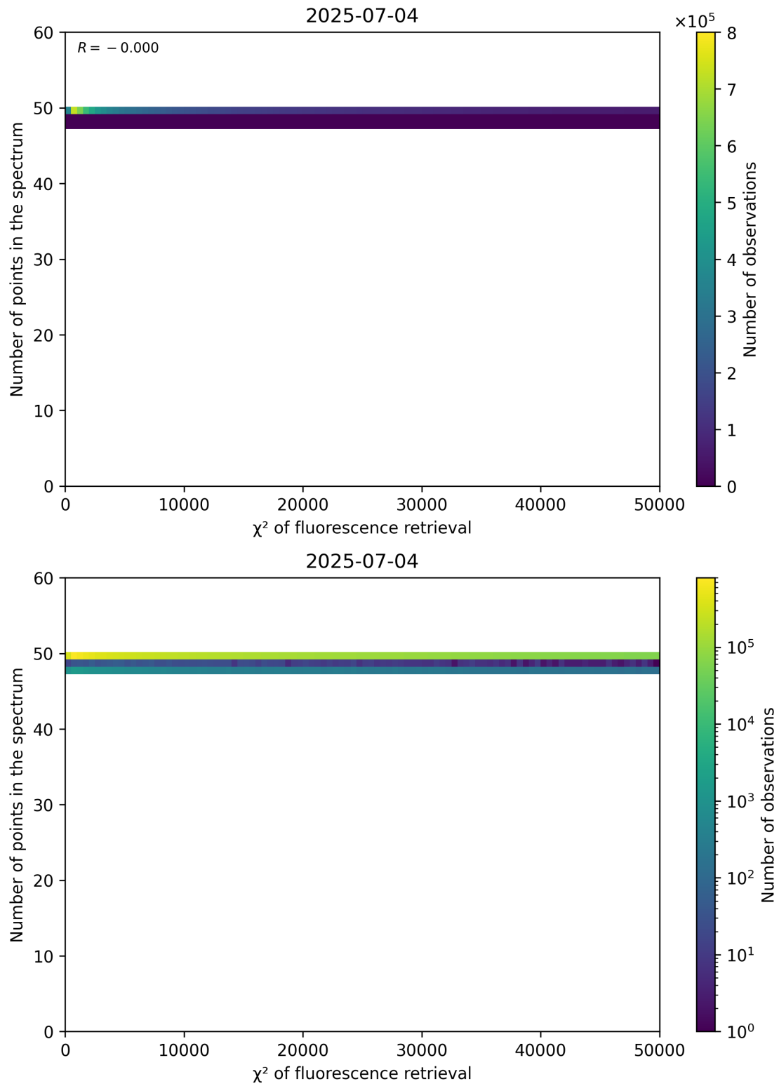
Figure 68: Scatter density plot of “ \chi^2 of fluorescence retrieval” against “Number of points in the spectrum” for 2025-07-03 to 2025-07-05.
