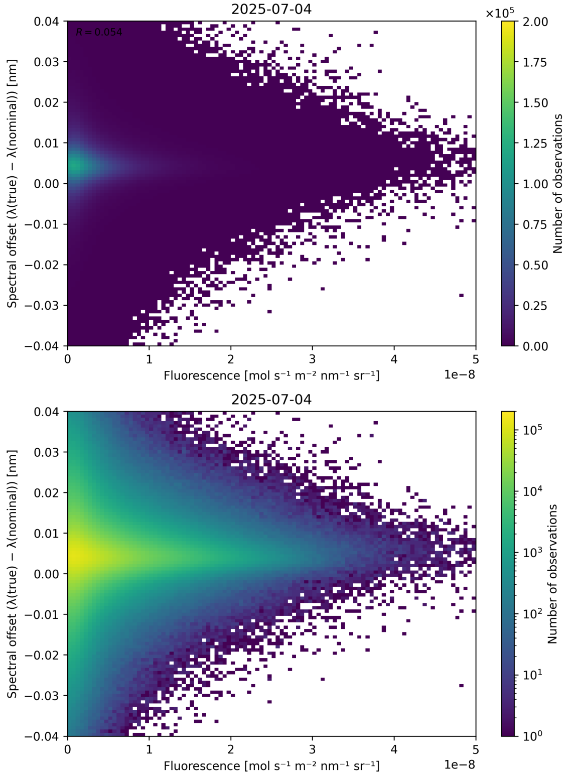
Figure 87: Scatter density plot of “Fluorescence” against “Spectral offset ( \lambda_{\text{true}} - \lambda_{\text{nominal}} )” for 2025-07-03 to 2025-07-05.
