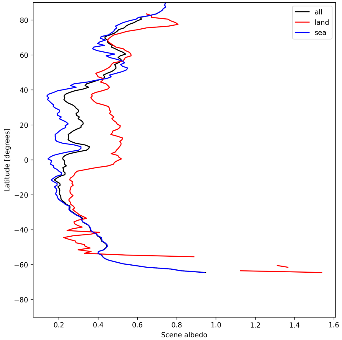
Figure 17: Zonal average of “Scene albedo” for 2025-07-03 to 2025-07-05.
