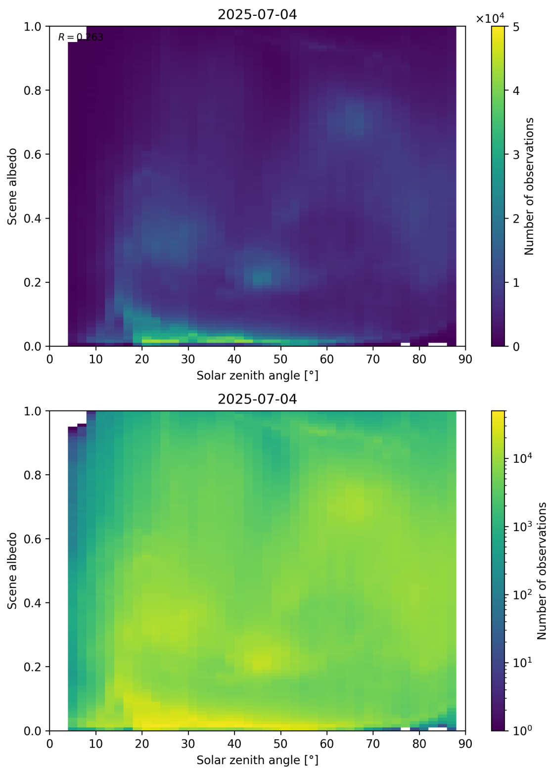
Figure 116: Scatter density plot of “Solar zenith angle” against “Scene albedo” for 2025-07-03 to 2025-07-05.
