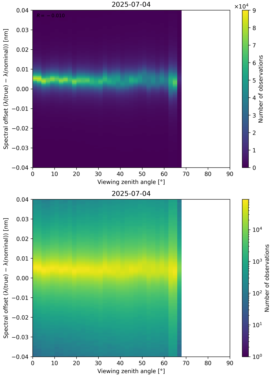
Figure 128: Scatter density plot of “Viewing zenith angle” against “Spectral offset ( \lambda_{\text{true}} - \lambda_{\text{nominal}} )” for 2025-07-03 to 2025-07-05.
