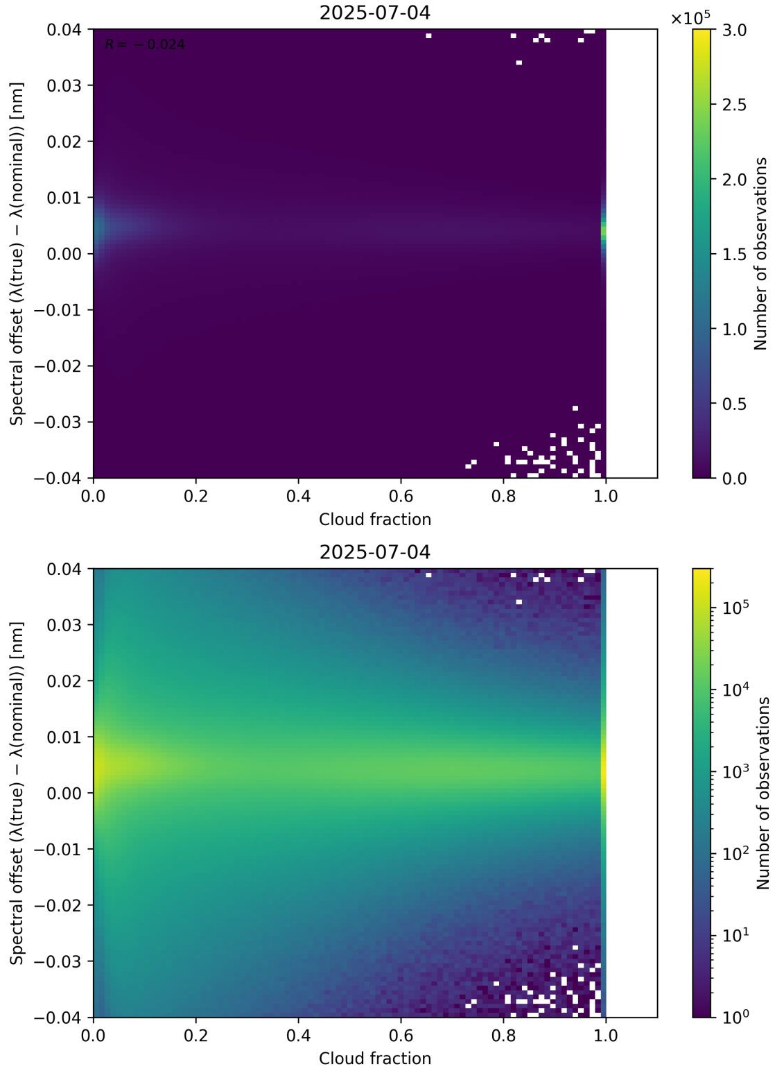
Figure 76: Scatter density plot of “Cloud fraction” against “Spectral offset ( \lambda_{\text{true}} - \lambda_{\text{nominal}} )” for 2025-07-03 to 2025-07-05.
