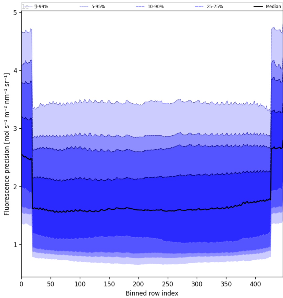
Figure 58: Along track statistics of “Fluorescence precision” for 2025-07-03 to 2025-07-05
