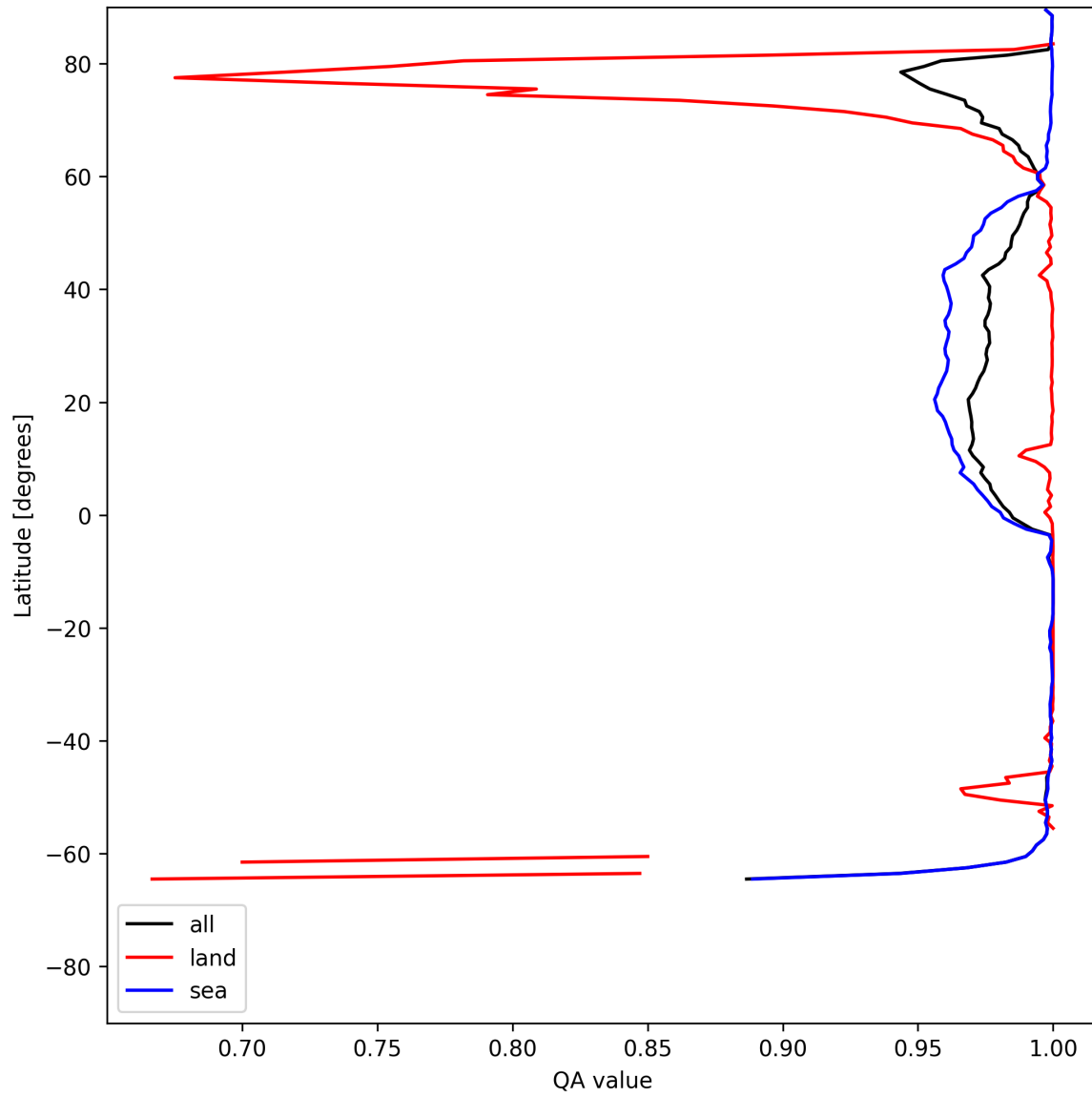
Figure 12: Zonal average of “QA value” for 2025-07-03 to 2025-07-05.
