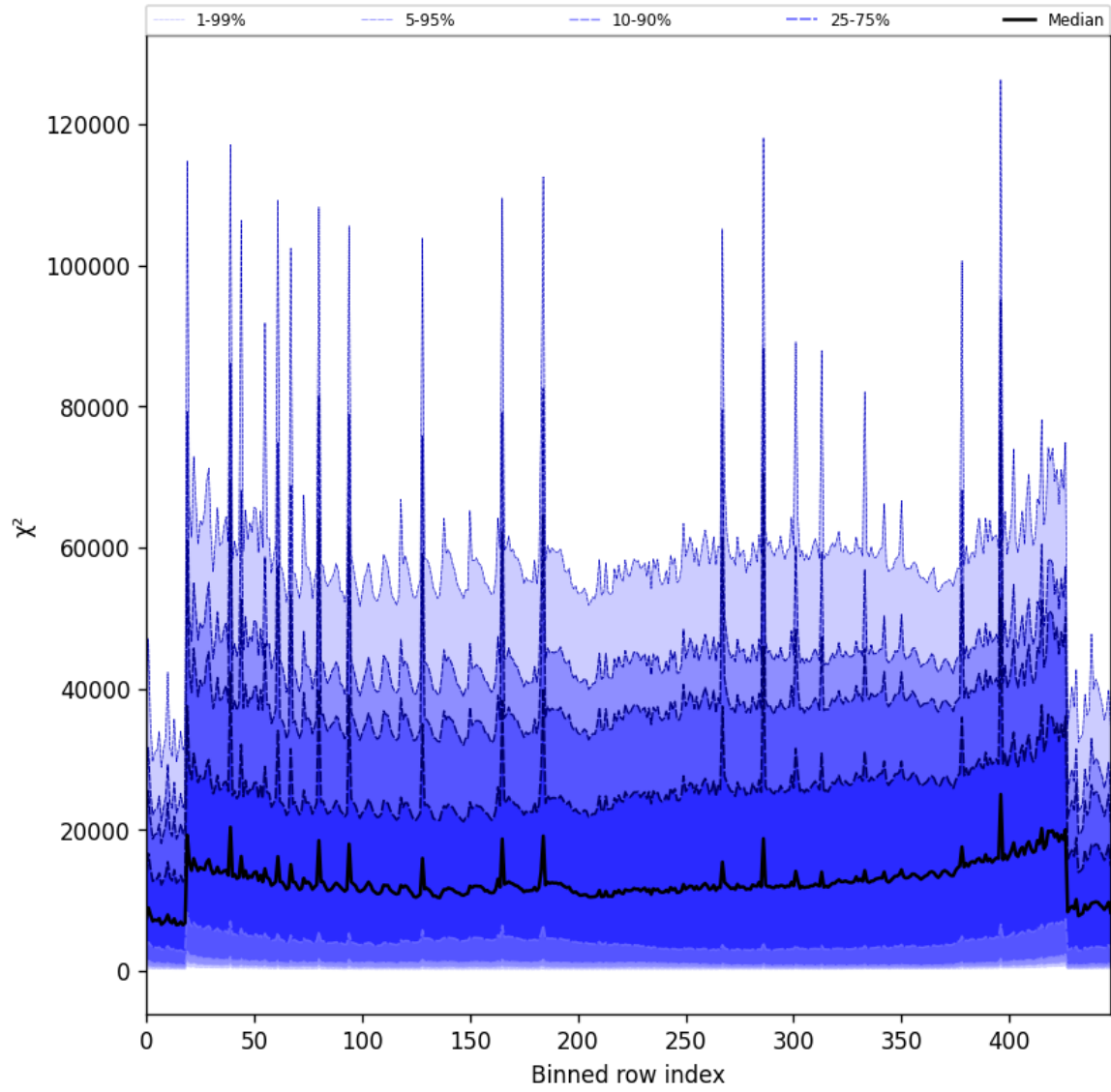
Figure 55: Along track statistics of “ \chi^2 ” for 2025-07-03 to 2025-07-05
