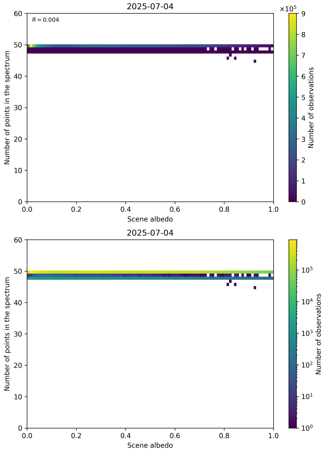
Figure 106: Scatter density plot of “Scene albedo” against “Number of points in the spectrum” for 2025-07-03 to 2025-07-05.
