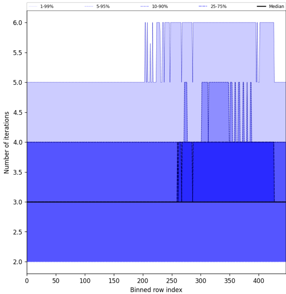
Figure 56: Along track statistics of “Number of iterations” for 2025-07-03 to 2025-07-05
