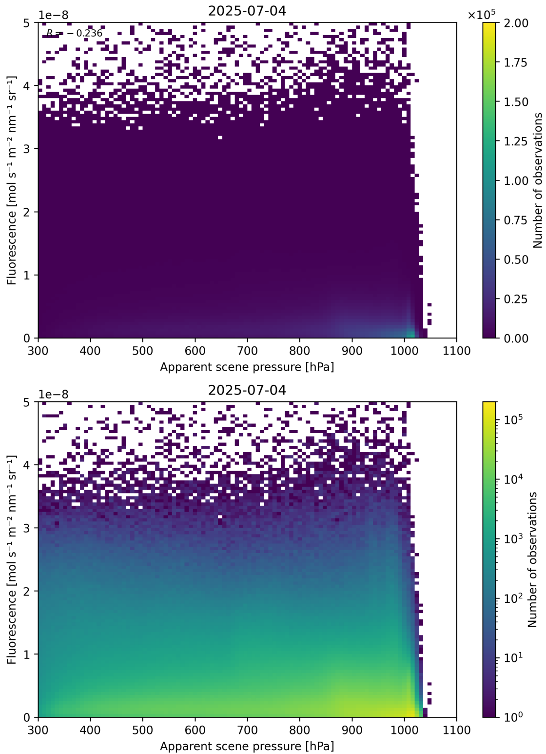
Figure 64: Scatter density plot of “Apparent scene pressure” against “Fluorescence” for 2025-07-03 to 2025-07-05.
