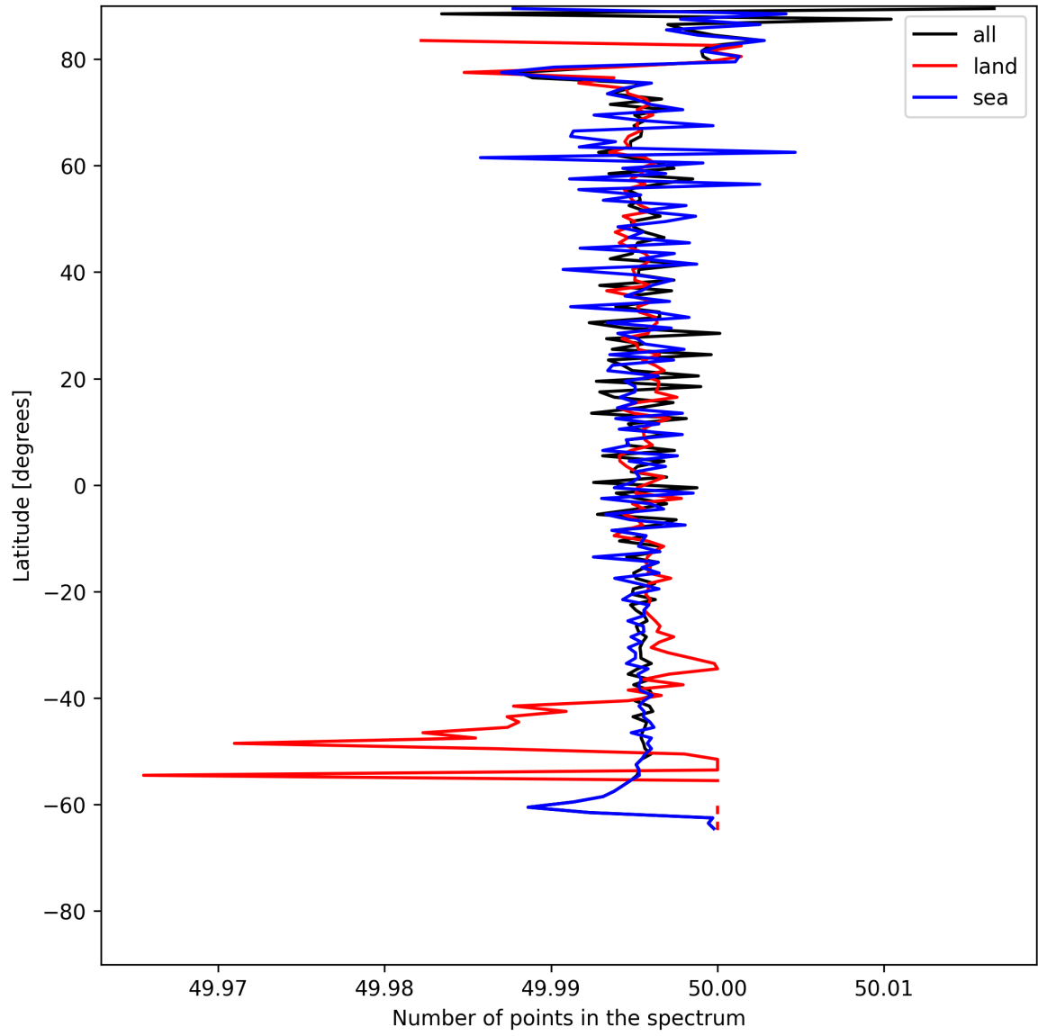
Figure 27: Zonal average of “Number of points in the spectrum” for 2025-07-03 to 2025-07-05.
