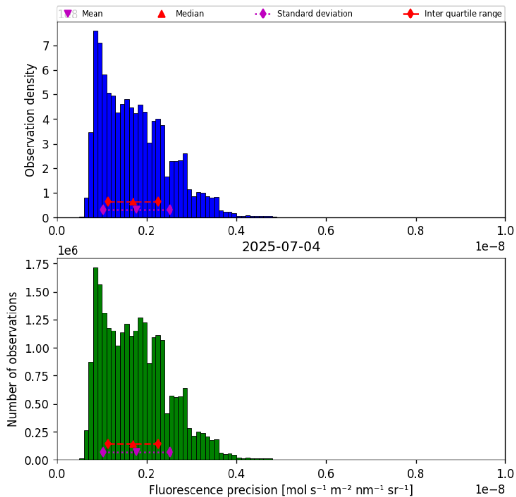
Figure 41: Histogram of “Fluorescence precision” for 2025-07-03 to 2025-07-05
