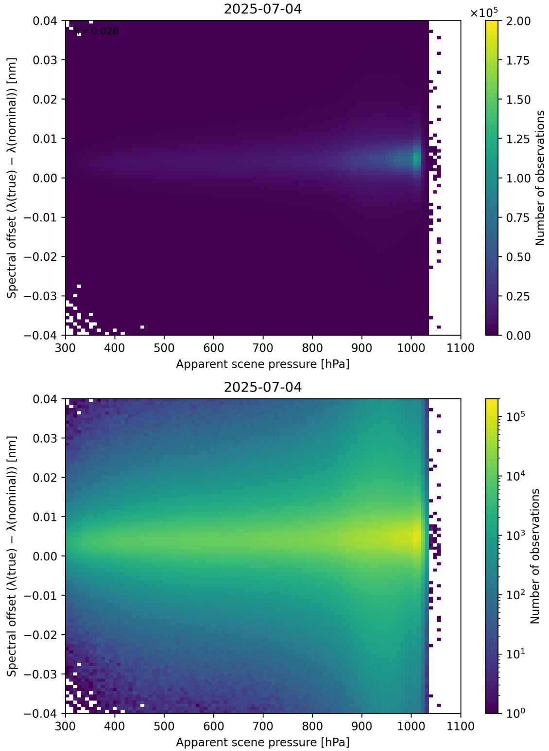
Figure 67: Scatter density plot of “Apparent scene pressure” against “Spectral offset ( \lambda_{\text{true}} - \lambda_{\text{nominal}} )” for 2025-07-03 to 2025-07-05.
