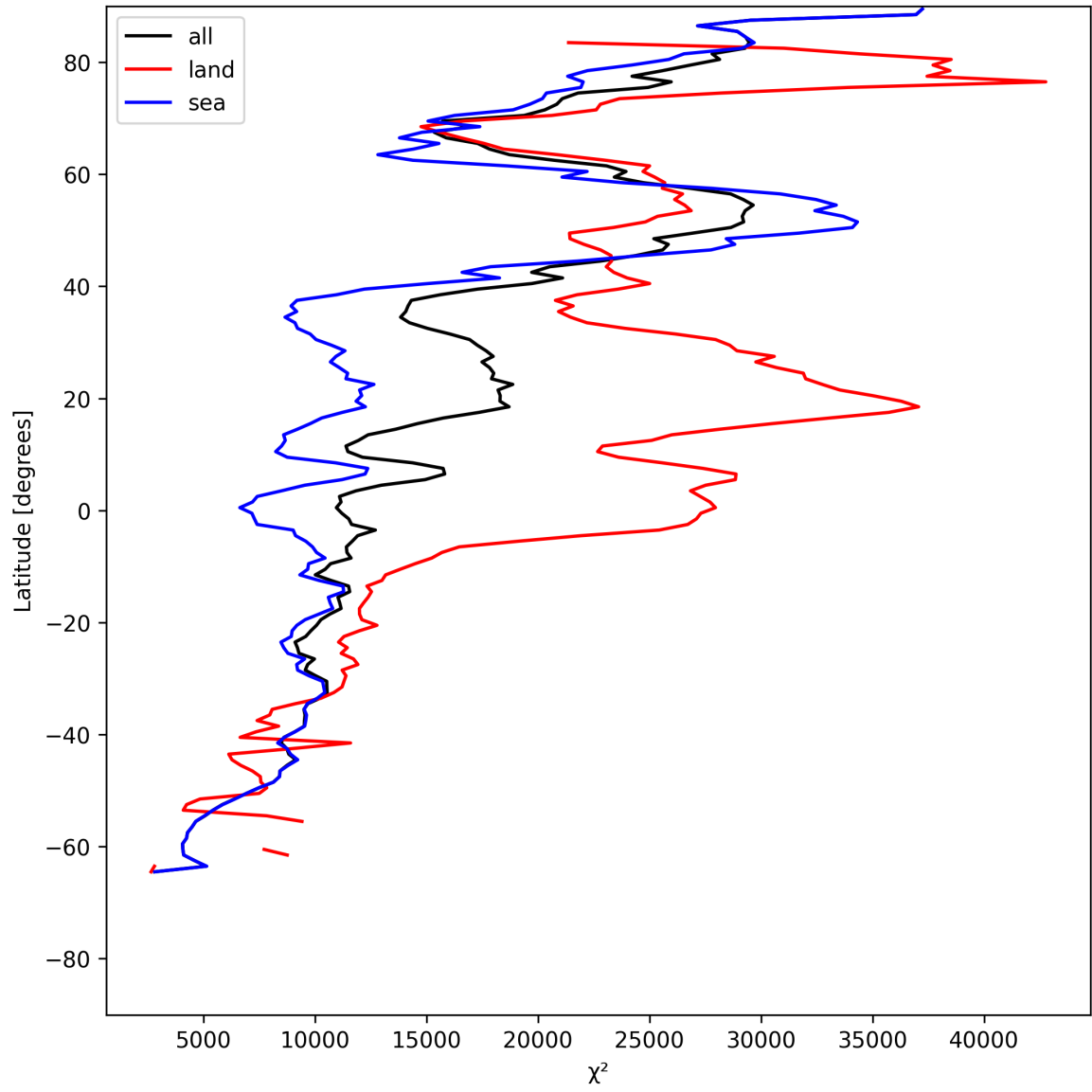
Figure 21: Zonal average of “ \chi^2 ” for 2025-07-03 to 2025-07-05.
