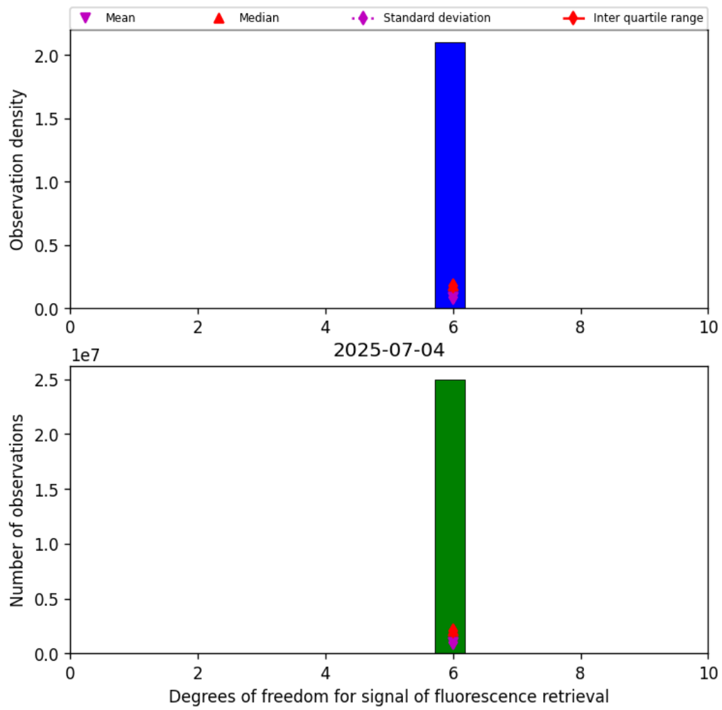
Figure 43: Histogram of “Degrees of freedom for signal of fluorescence retrieval” for 2025-07-03 to 2025-07-05
