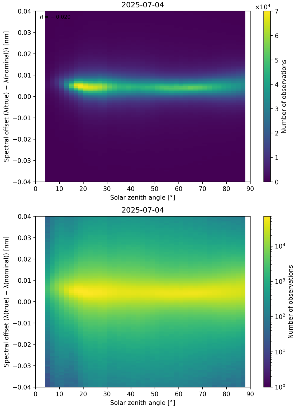
Figure 117: Scatter density plot of “Solar zenith angle” against “Spectral offset ( \lambda_{\text{true}} - \lambda_{\text{nominal}} )” for 2025-07-03 to 2025-07-05.
