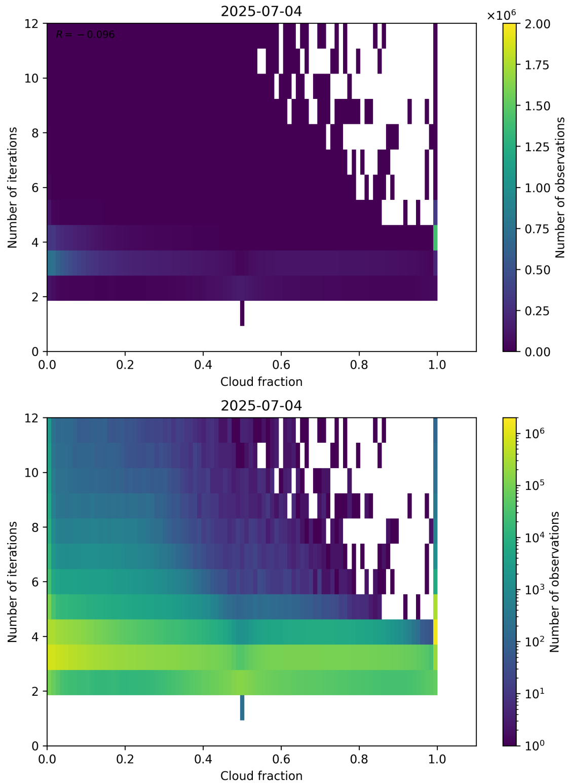
Figure 73: Scatter density plot of “Cloud fraction” against “Number of iterations” for 2025-07-03 to 2025-07-05.
