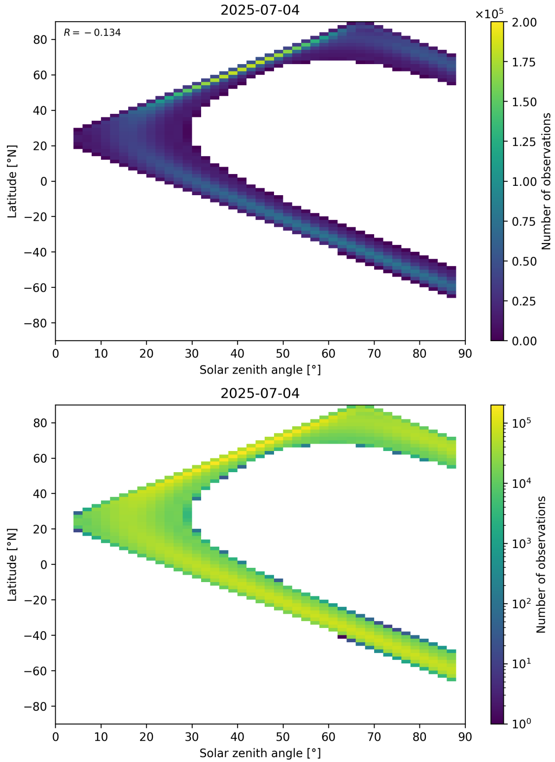
Figure 113: Scatter density plot of “Solar zenith angle” against “Latitude” for 2025-07-03 to 2025-07-05.
