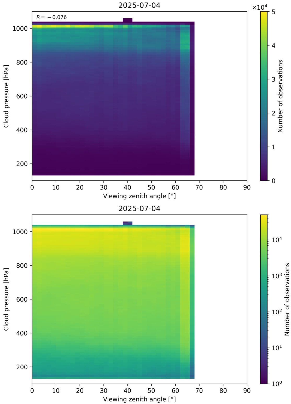
Figure 121: Scatter density plot of “Viewing zenith angle” against “Cloud pressure” for 2025-07-03 to 2025-07-05.
