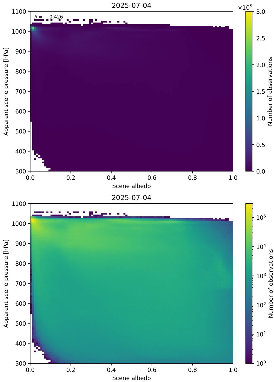
Figure 102: Scatter density plot of “Scene albedo” against “Apparent scene pressure” for 2025-07-03 to 2025-07-05.
