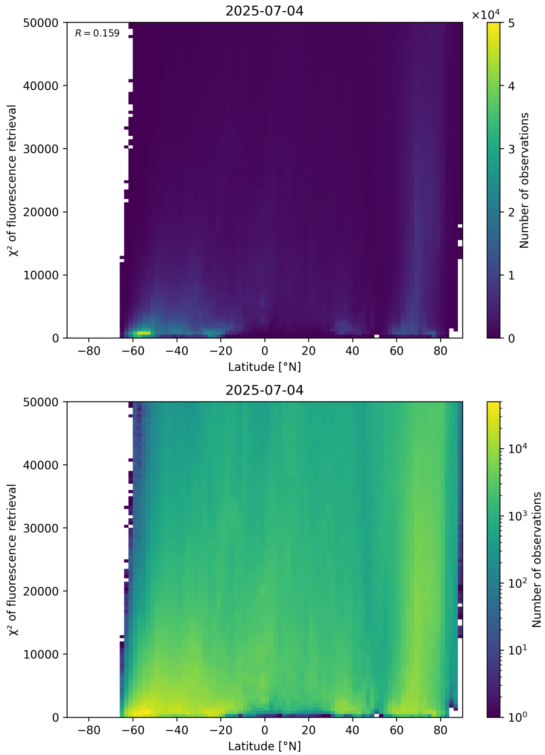
Figure 89: Scatter density plot of “Latitude” against “ \chi^2 of fluorescence retrieval” for 2025-07-03 to 2025-07-05.
