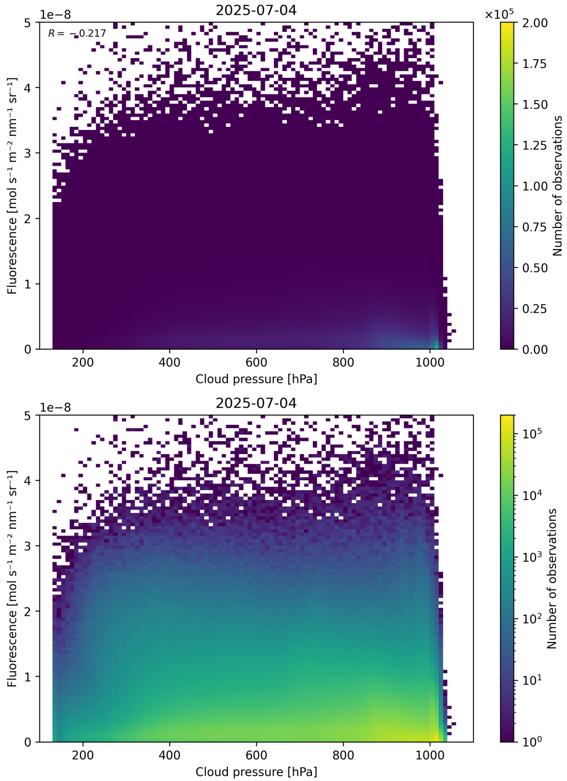
Figure 80: Scatter density plot of “Cloud pressure” against “Fluorescence” for 2025-07-03 to 2025-07-05.
