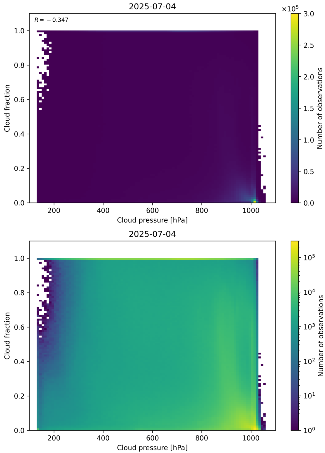
Figure 79: Scatter density plot of “Cloud pressure” against “Cloud fraction” for 2025-07-03 to 2025-07-05.
