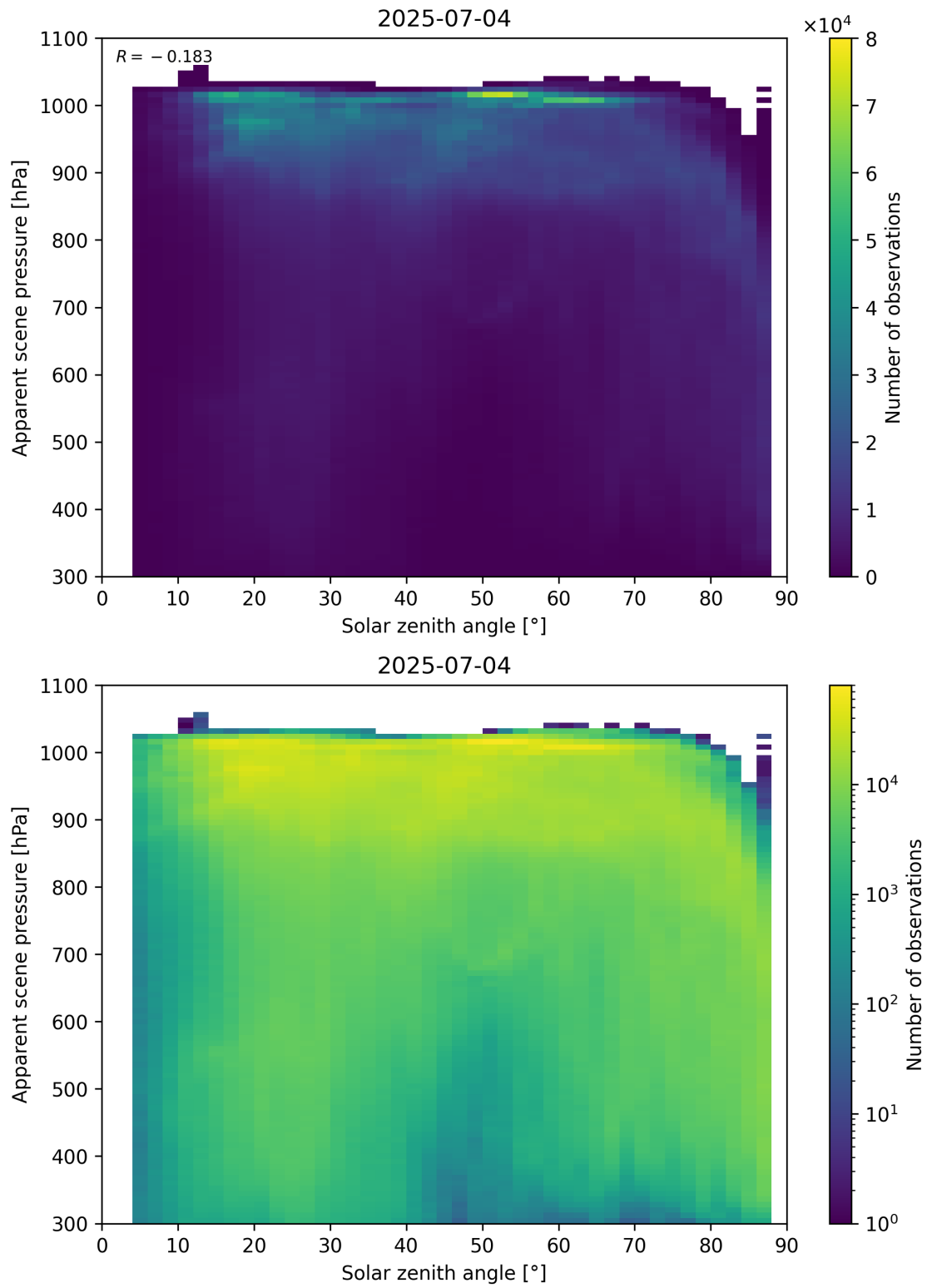
Figure 108: Scatter density plot of “Solar zenith angle” against “Apparent scene pressure” for 2025-07-03 to 2025-07-05.
