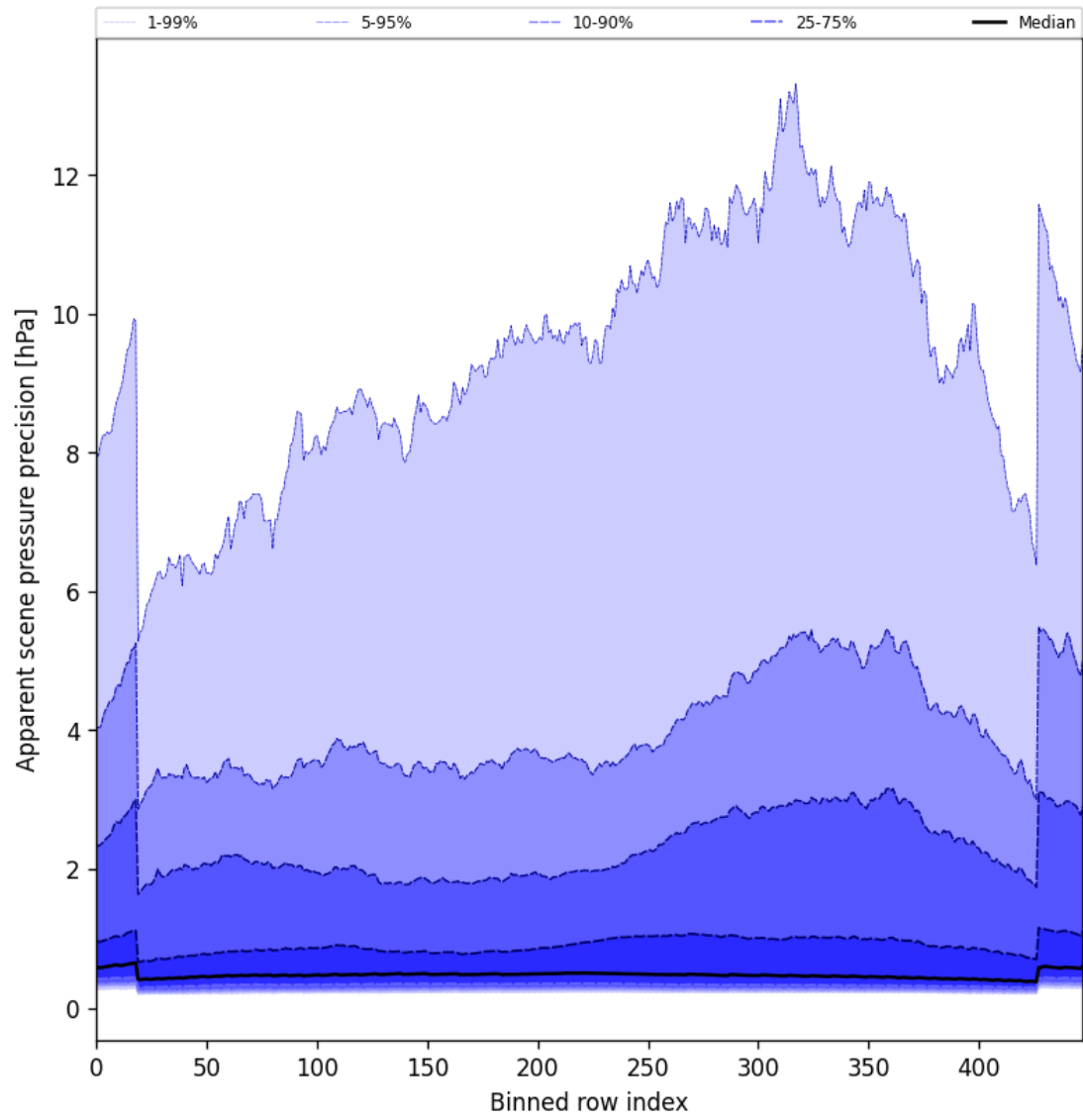
Figure 54: Along track statistics of “Apparent scene pressure precision” for 2025-07-03 to 2025-07-05
