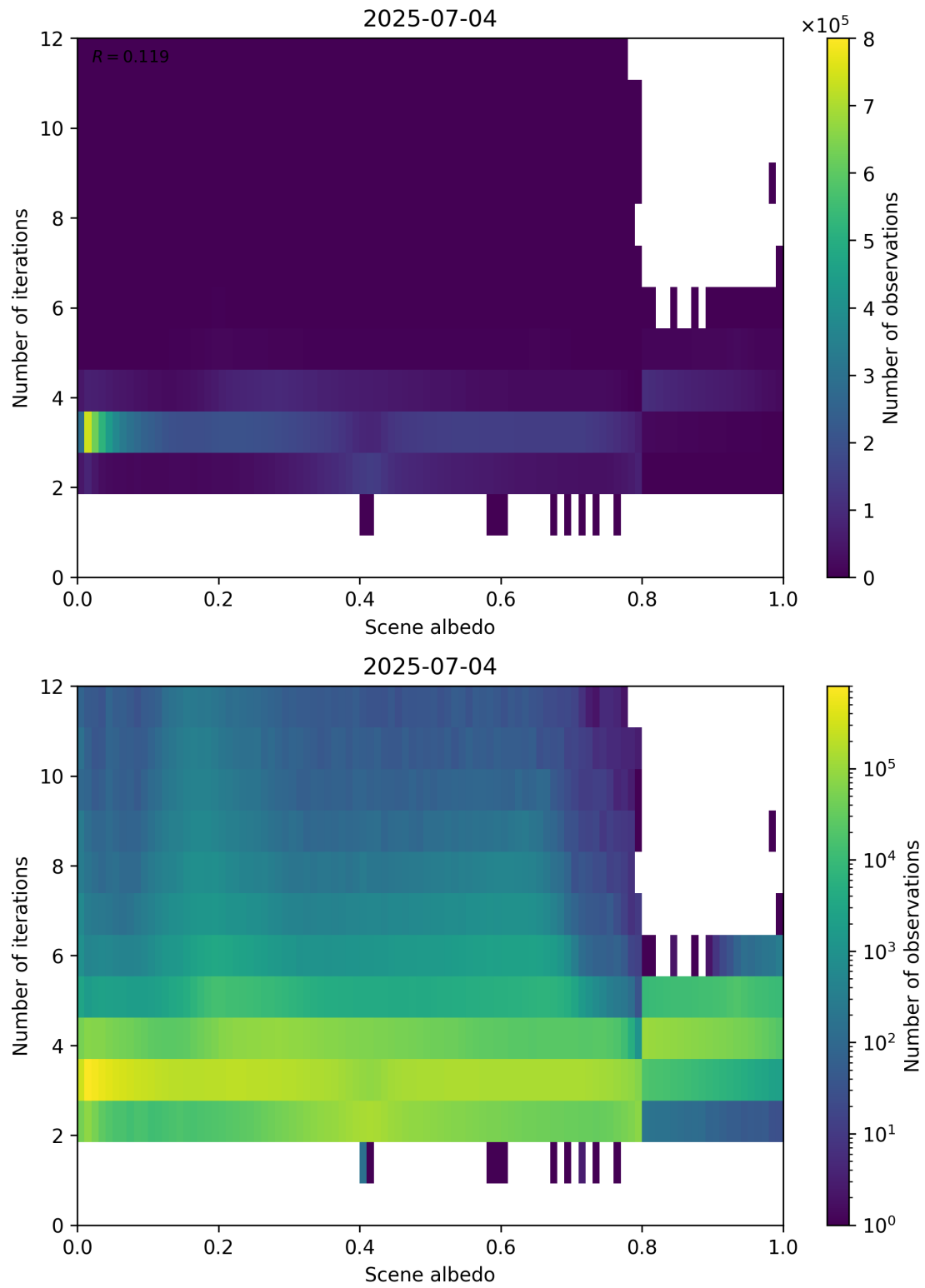
Figure 105: Scatter density plot of “Scene albedo” against “Number of iterations” for 2025-07-03 to 2025-07-05.
