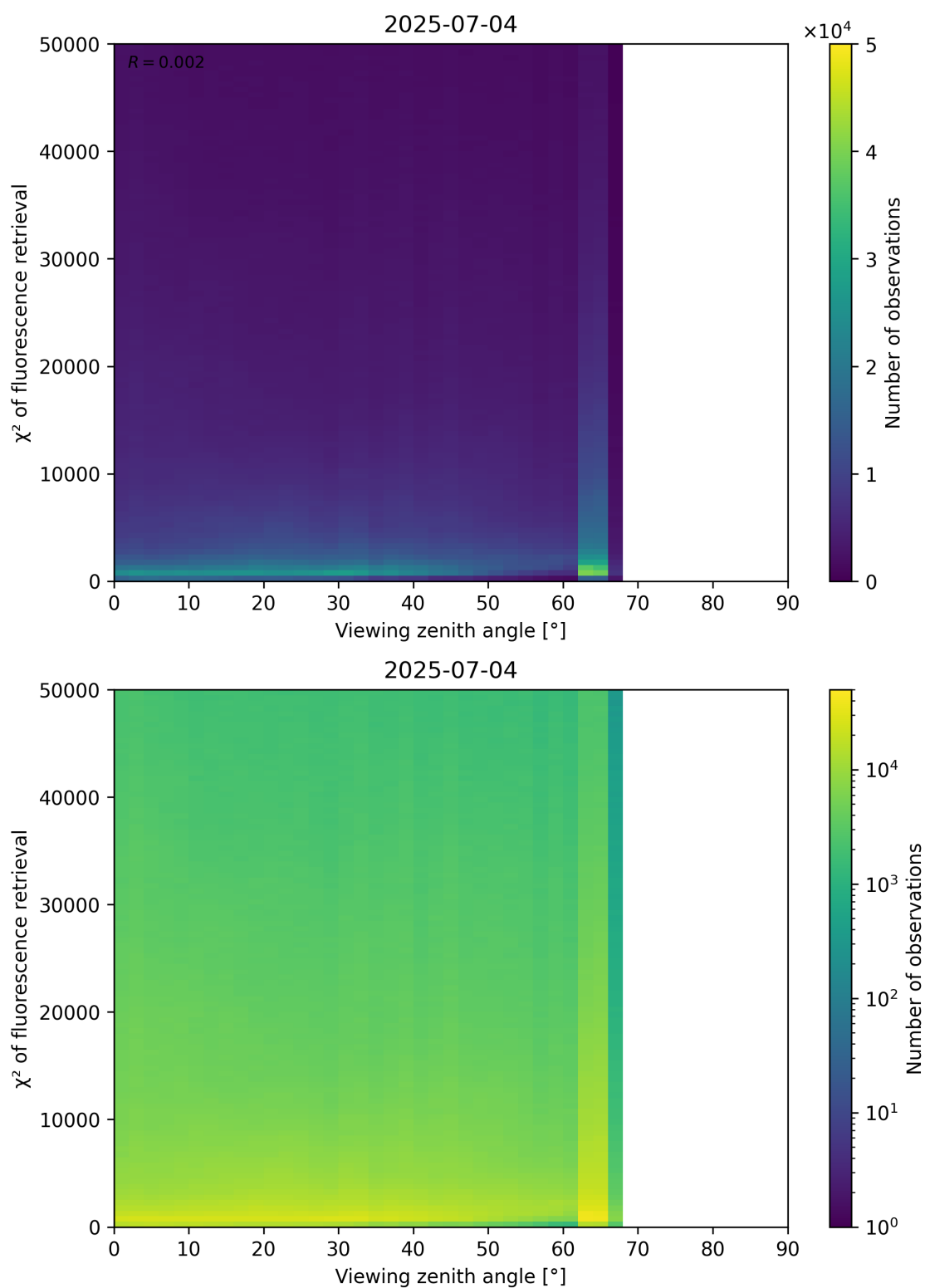
Figure 119: Scatter density plot of “Viewing zenith angle” against “ \chi^2 of fluorescence retrieval” for 2025-07-03 to 2025-07-05.
