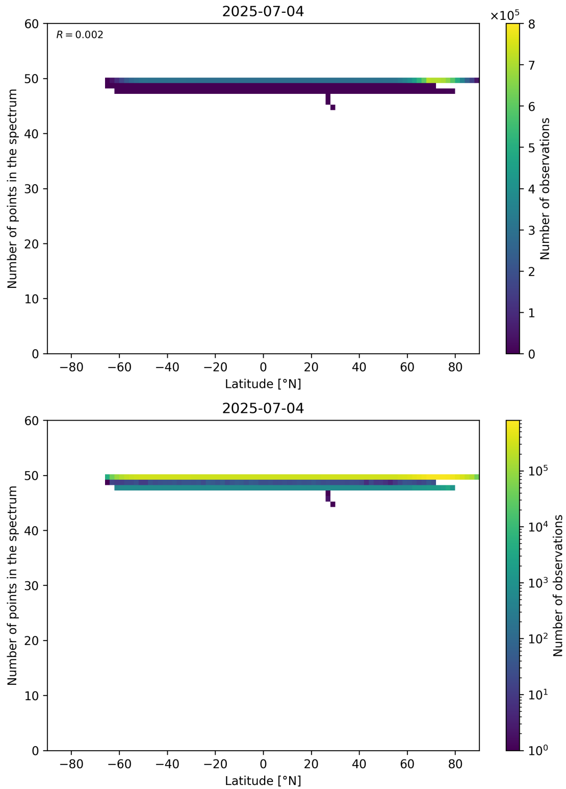
Figure 94: Scatter density plot of “Latitude” against “Number of points in the spectrum” for 2025-07-03 to 2025-07-05.
