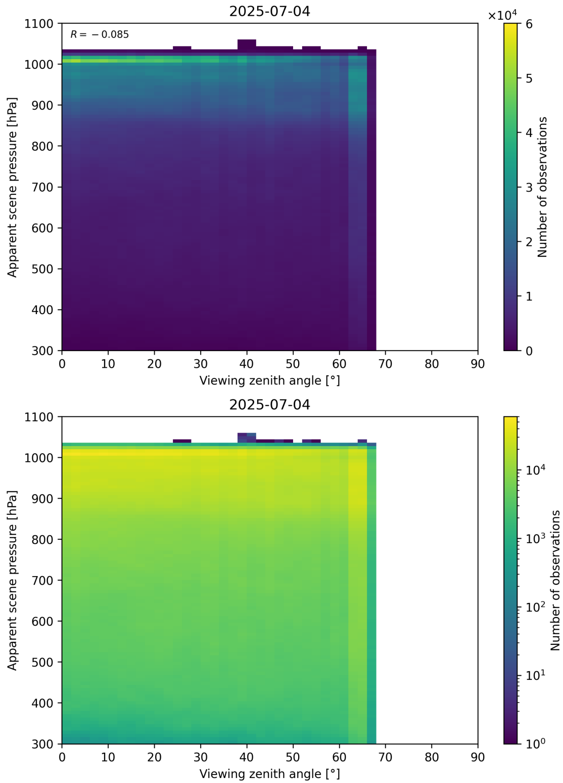
Figure 118: Scatter density plot of “Viewing zenith angle” against “Apparent scene pressure” for 2025-07-03 to 2025-07-05.
