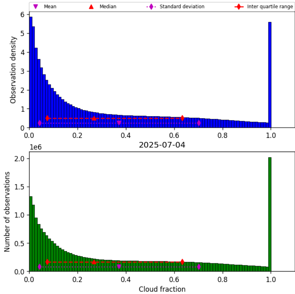
Figure 32: Histogram of “Cloud fraction” for 2025-07-03 to 2025-07-05
