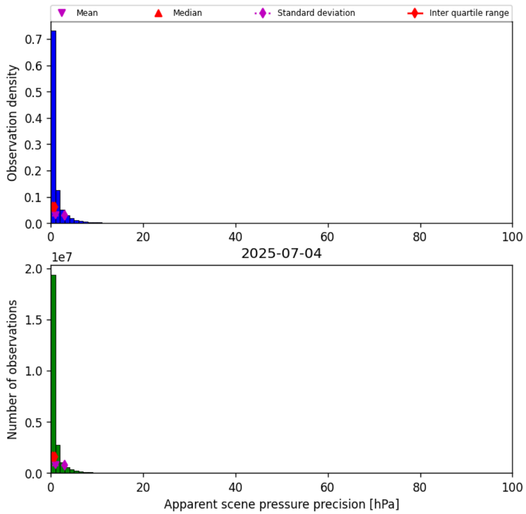
Figure 37: Histogram of “Apparent scene pressure precision” for 2025-07-03 to 2025-07-05
