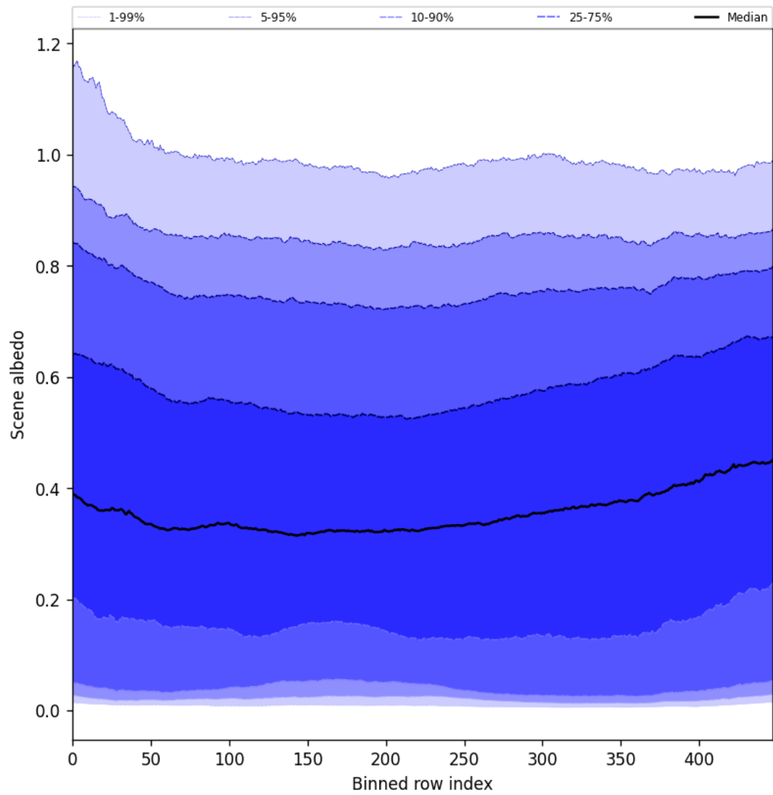
Figure 51: Along track statistics of “Scene albedo” for 2025-07-03 to 2025-07-05
