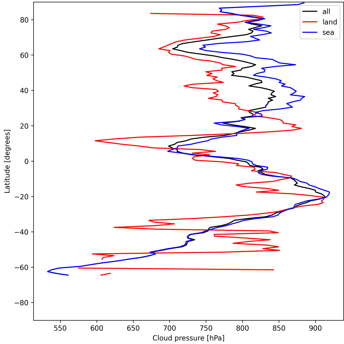
Figure 13: Zonal average of “Cloud pressure” for 2025-07-03 to 2025-07-05.
