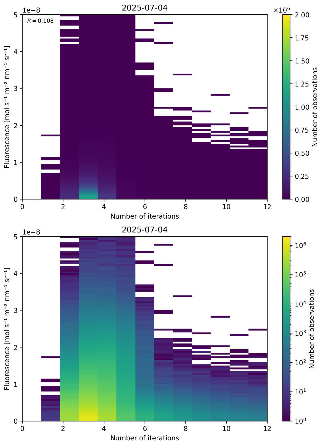
Figure 98: Scatter density plot of “Number of iterations” against “Fluorescence” for 2025-07-03 to 2025-07-05.
