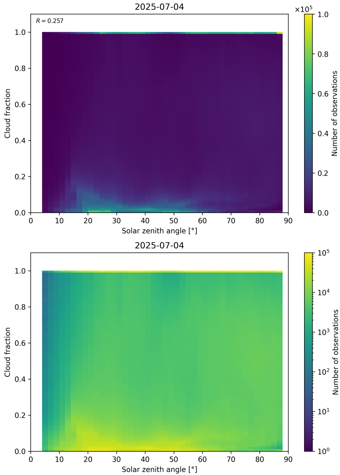
Figure 110: Scatter density plot of “Solar zenith angle” against “Cloud fraction” for 2025-07-03 to 2025-07-05.
