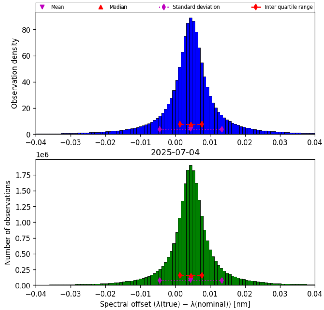
Figure 45: Histogram of “Spectral offset ( \lambda_{\text{true}} - \lambda_{\text{nominal}} )” for 2025-07-03 to 2025-07-05
