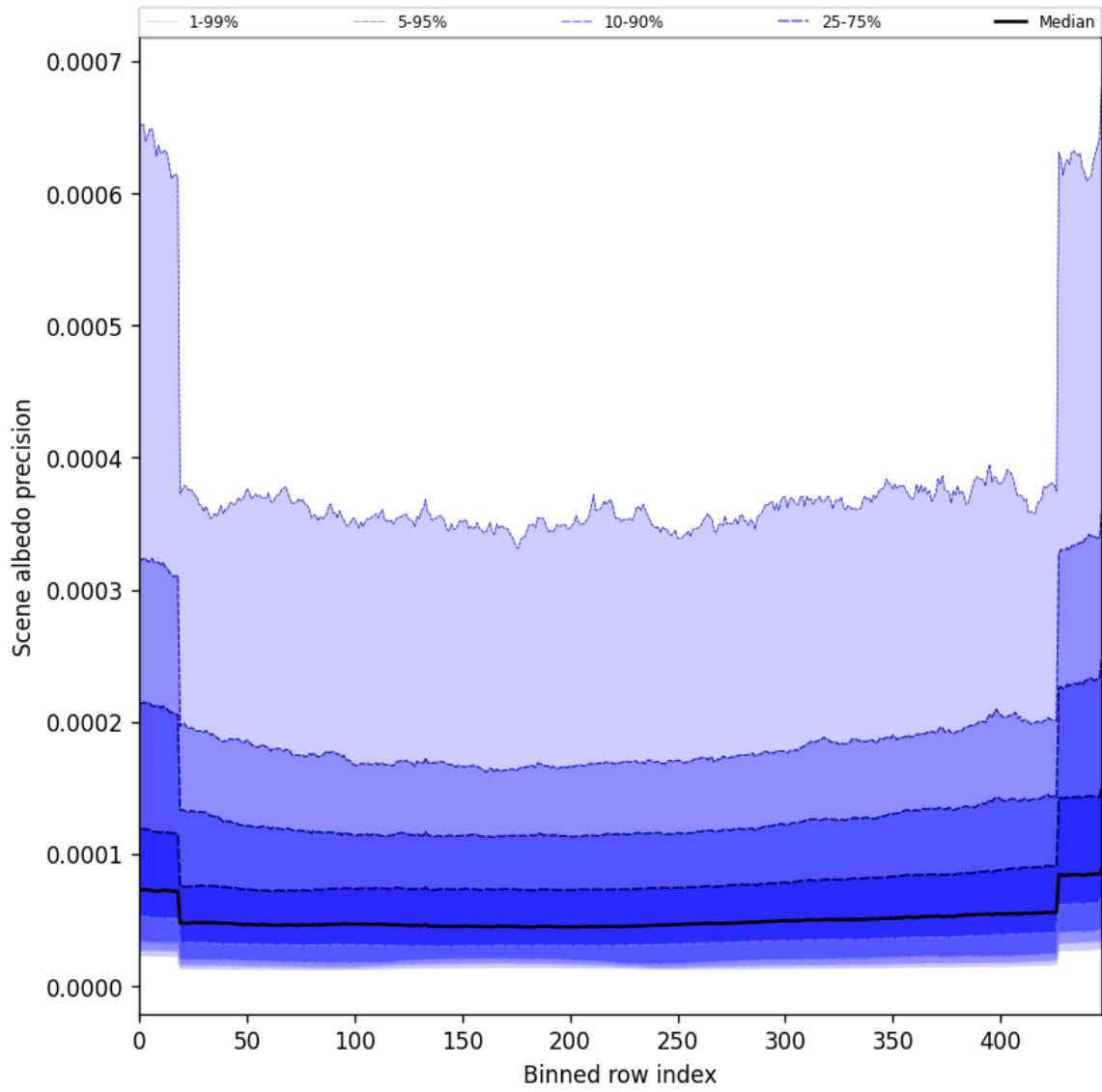
Figure 52: Along track statistics of “Scene albedo precision” for 2025-07-03 to 2025-07-05
