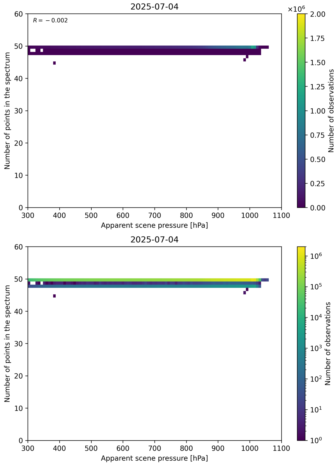
Figure 66: Scatter density plot of “Apparent scene pressure” against “Number of points in the spectrum” for 2025-07-03 to 2025-07-05.
