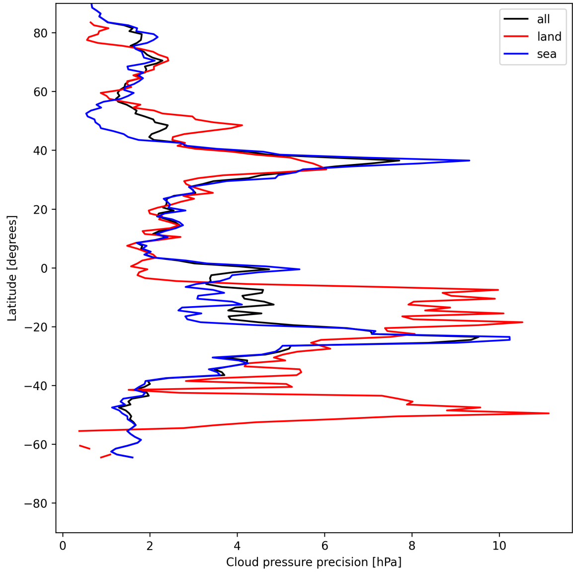
Figure 14: Zonal average of “Cloud pressure precision” for 2025-07-03 to 2025-07-05.
