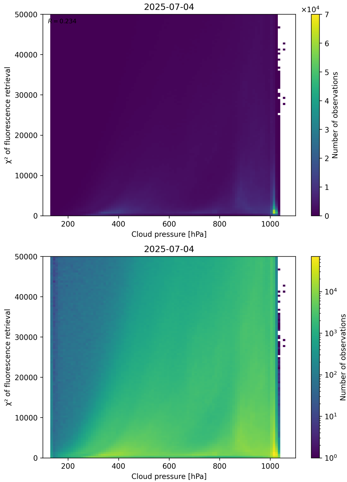
Figure 78: Scatter density plot of “Cloud pressure” against “ \chi^2 of fluorescence retrieval” for 2025-07-03 to 2025-07-05.
