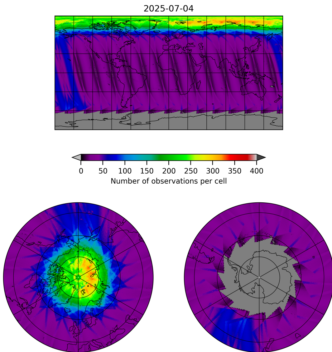
Figure 11: Map of the number of observations for 2025-07-03 to 2025-07-05
