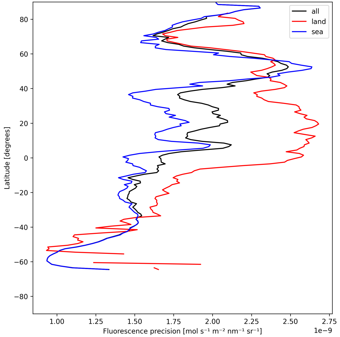
Figure 24: Zonal average of “Fluorescence precision” for 2025-07-03 to 2025-07-05.
