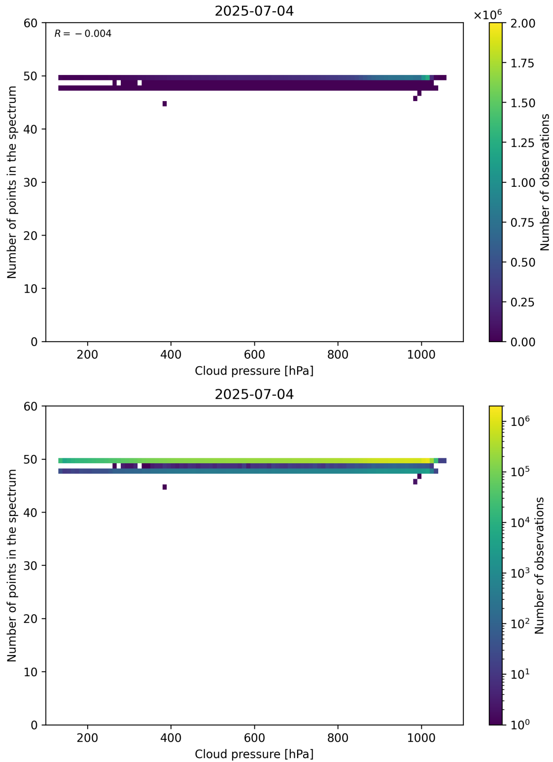
Figure 82: Scatter density plot of “Cloud pressure” against “Number of points in the spectrum” for 2025-07-03 to 2025-07-05.
