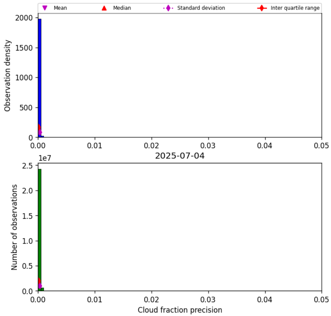
Figure 33: Histogram of “Cloud fraction precision” for 2025-07-03 to 2025-07-05
