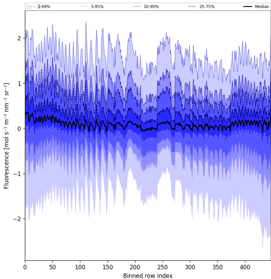
Figure 57: Along track statistics of “Fluorescence” for 2025-07-03 to 2025-07-05
