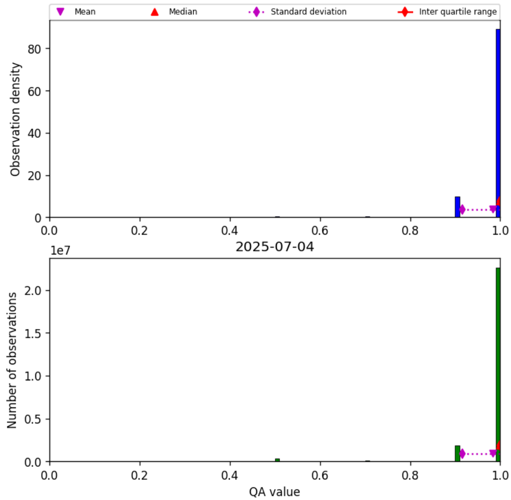
Figure 29: Histogram of “QA value” for 2025-07-03 to 2025-07-05
