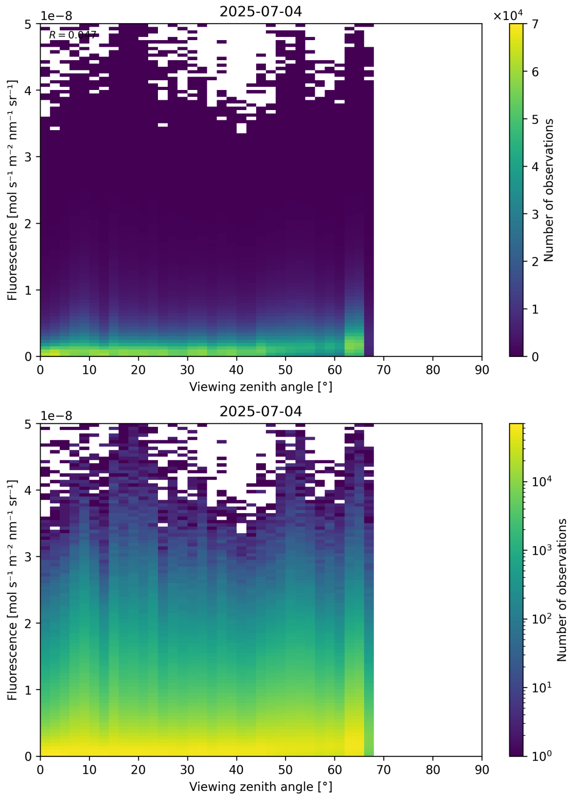
Figure 122: Scatter density plot of “Viewing zenith angle” against “Fluorescence” for 2025-07-03 to 2025-07-05.
