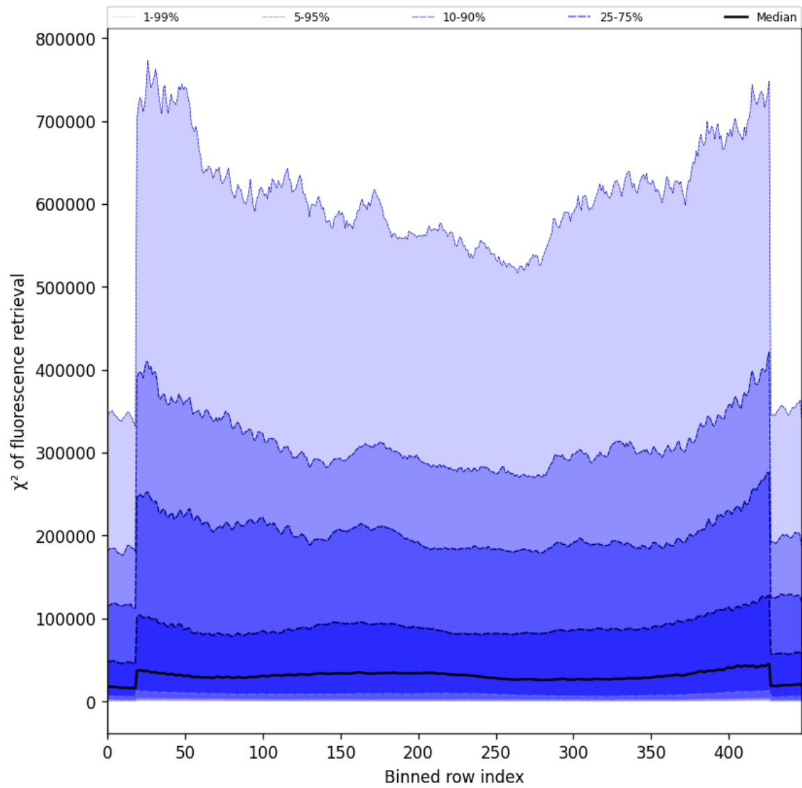
Figure 59: Along track statistics of “ \chi^2 of fluorescence retrieval” for 2025-07-03 to 2025-07-05
