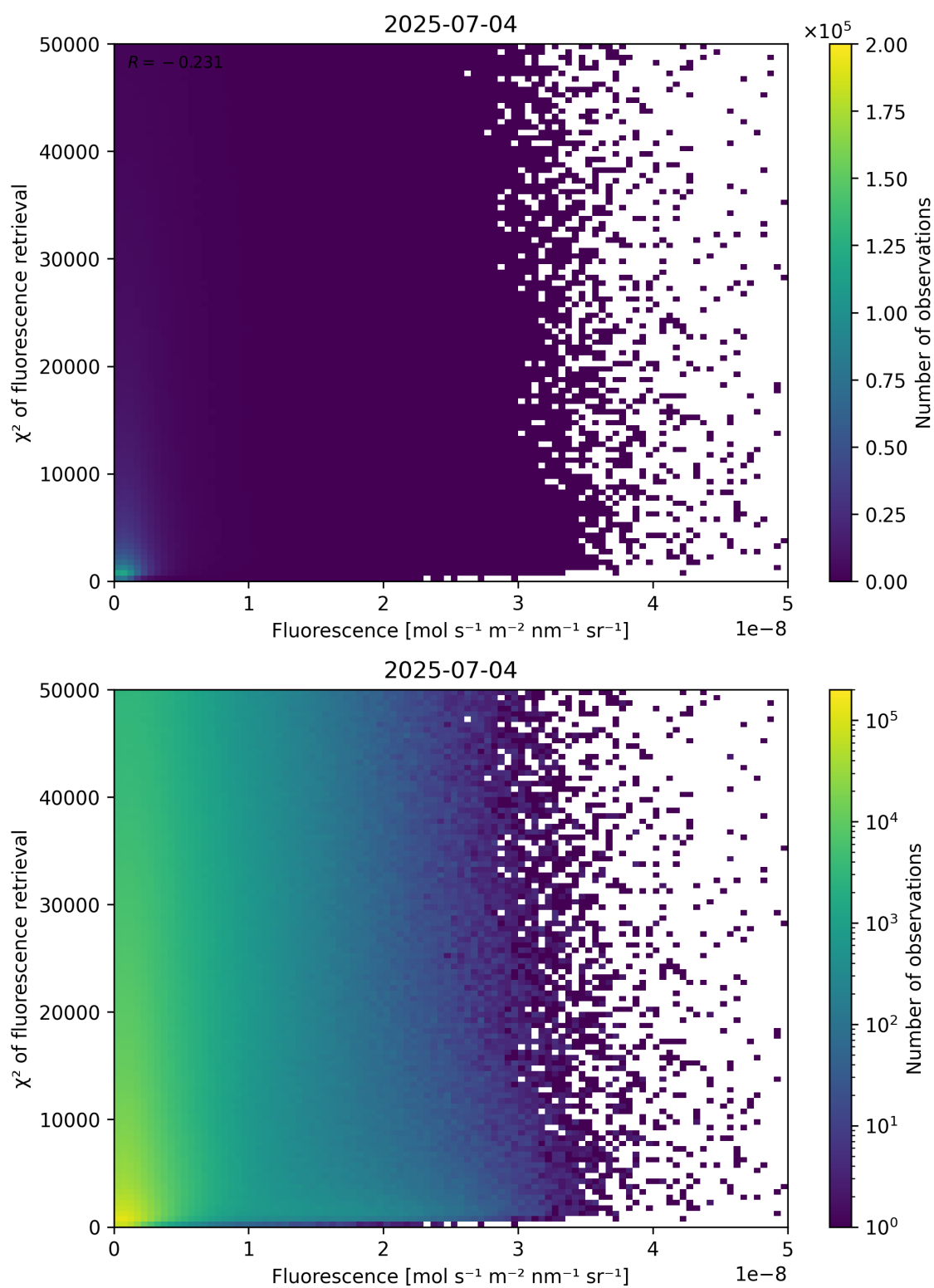
Figure 85: Scatter density plot of “Fluorescence” against “ \chi^2 of fluorescence retrieval” for 2025-07-03 to 2025-07-05.
