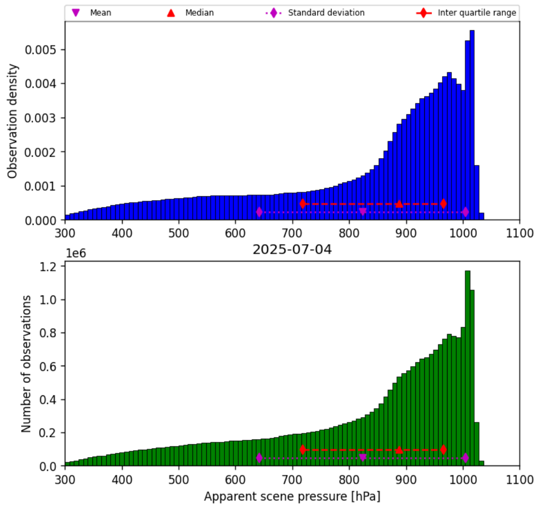
Figure 36: Histogram of “Apparent scene pressure” for 2025-07-03 to 2025-07-05
