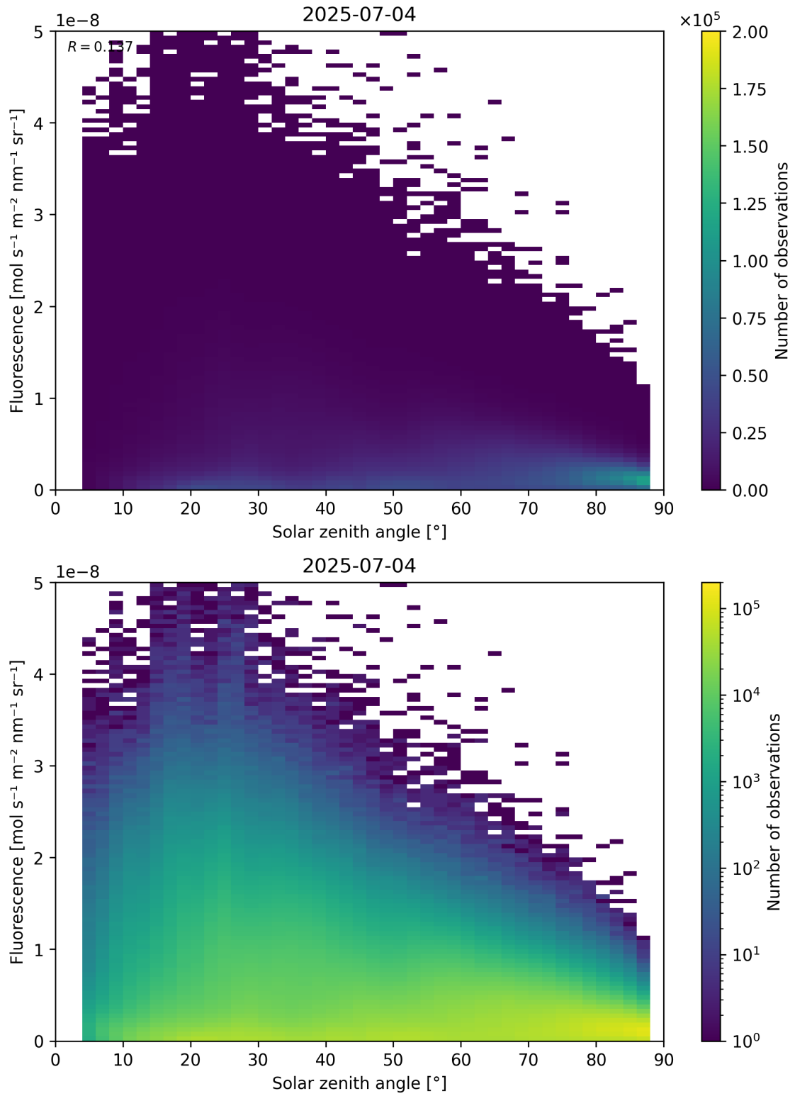
Figure 112: Scatter density plot of “Solar zenith angle” against “Fluorescence” for 2025-07-03 to 2025-07-05.
