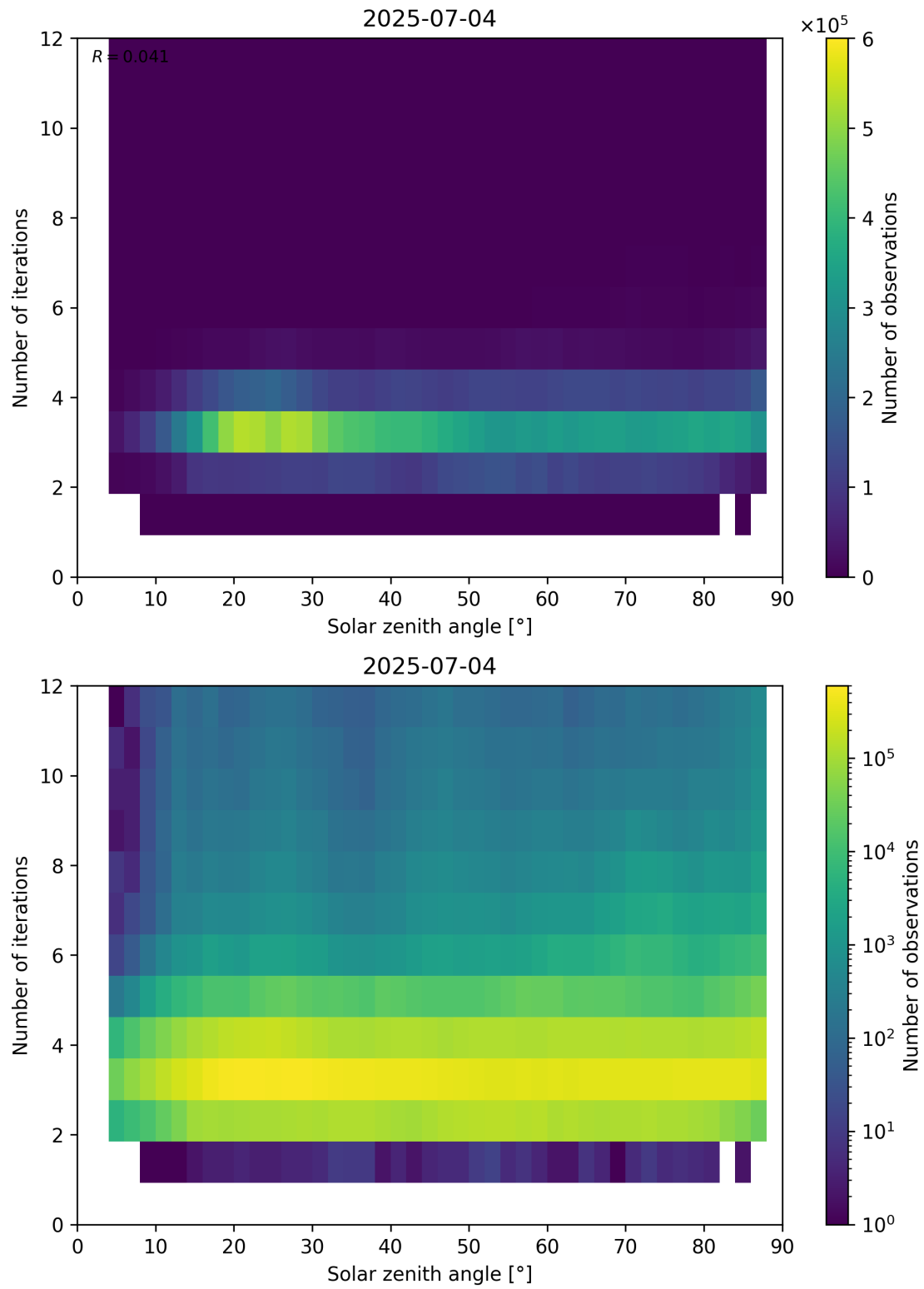
Figure 114: Scatter density plot of “Solar zenith angle” against “Number of iterations” for 2025-07-03 to 2025-07-05.
