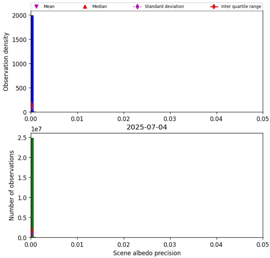
Figure 35: Histogram of “Scene albedo precision” for 2025-07-03 to 2025-07-05
