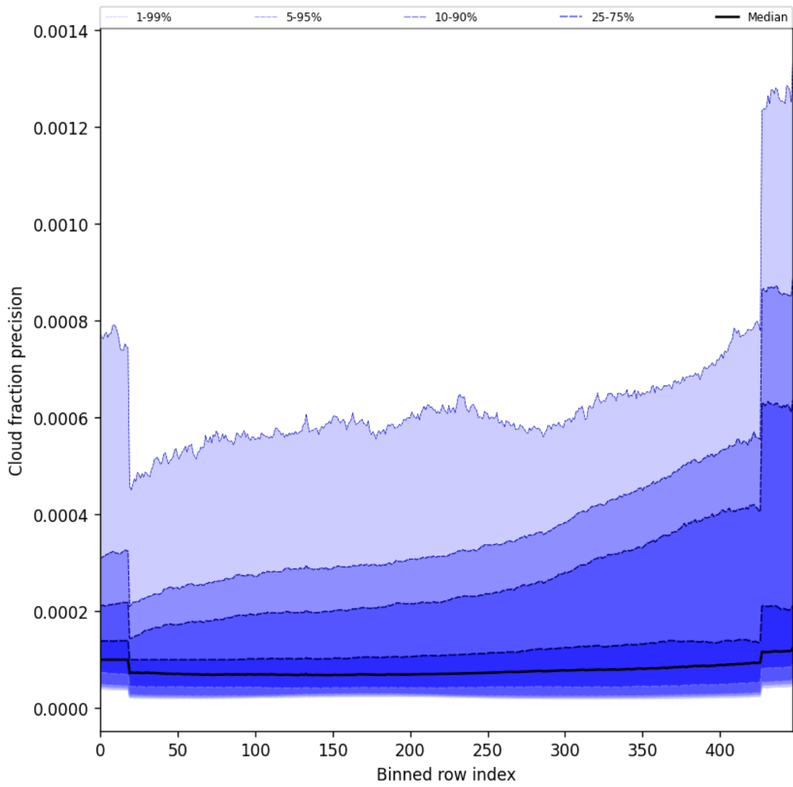
Figure 50: Along track statistics of “Cloud fraction precision” for 2025-07-03 to 2025-07-05
