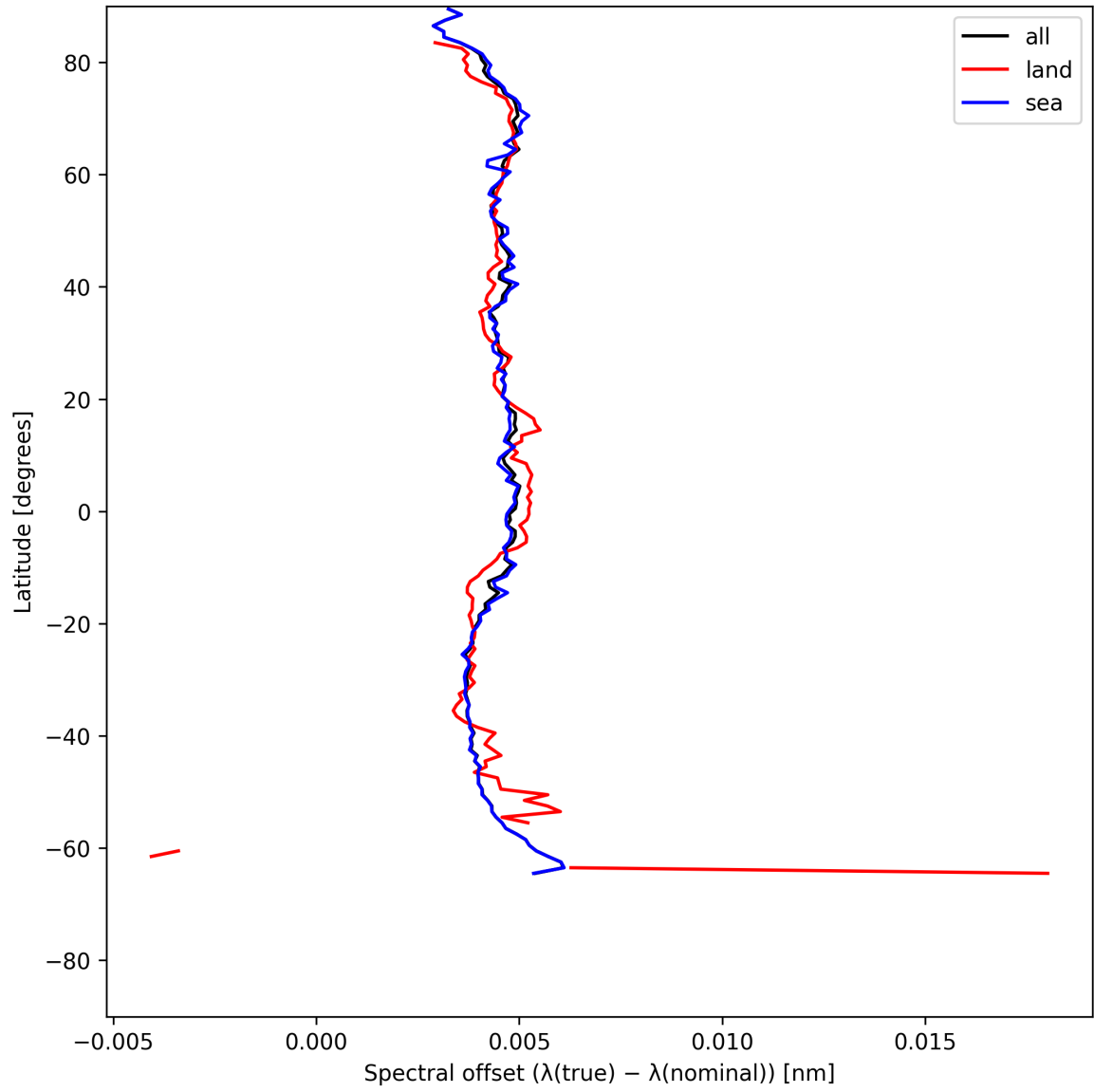
Figure 28: Zonal average of “Spectral offset ( \lambda_{\text{true}} - \lambda_{\text{nominal}} )” for 2025-07-03 to 2025-07-05.
