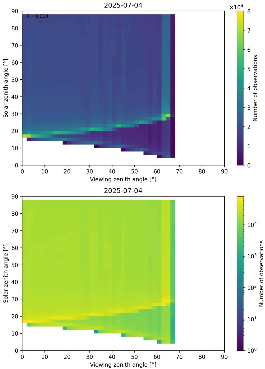
Figure 127: Scatter density plot of “Viewing zenith angle” against “Solar zenith angle” for 2025-07-03 to 2025-07-05.
