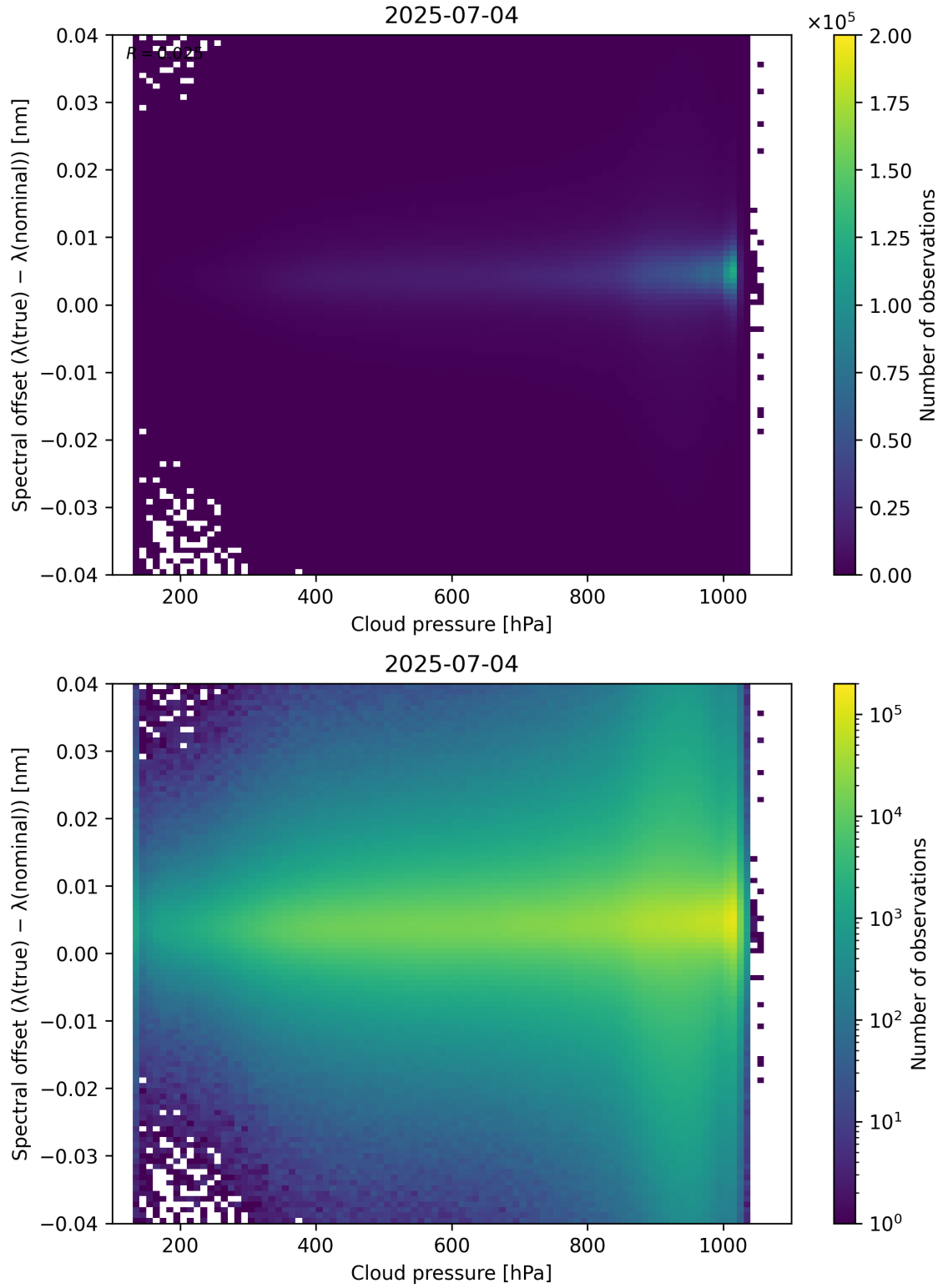
Figure 84: Scatter density plot of “Cloud pressure” against “Spectral offset ( \lambda_{\text{true}} - \lambda_{\text{nominal}} )” for 2025-07-03 to 2025-07-05.
