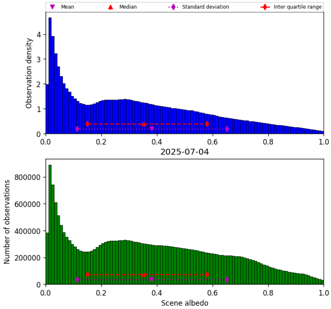
Figure 34: Histogram of “Scene albedo” for 2025-07-03 to 2025-07-05
