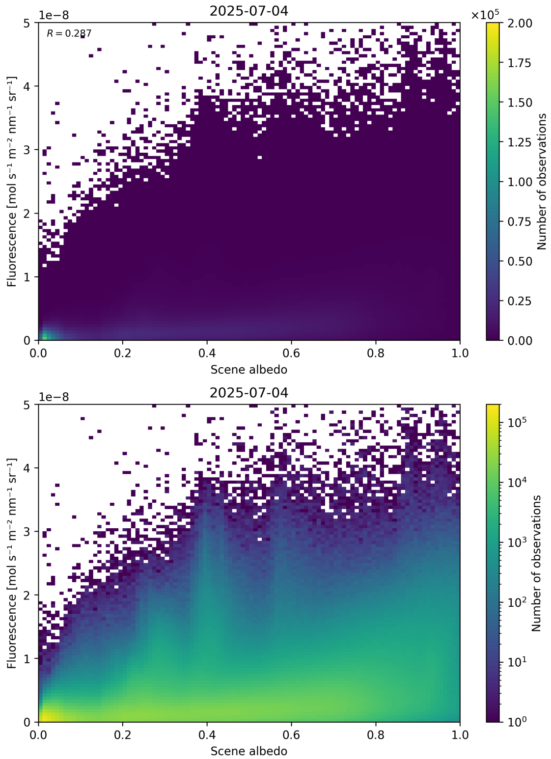
Figure 104: Scatter density plot of “Scene albedo” against “Fluorescence” for 2025-07-03 to 2025-07-05.
