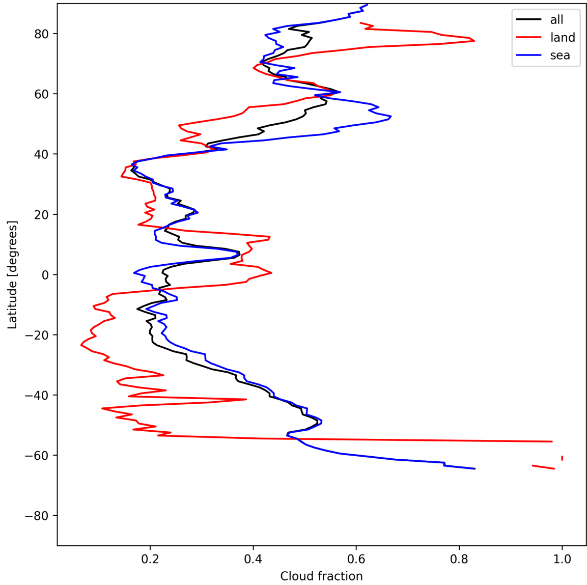
Figure 15: Zonal average of “Cloud fraction” for 2025-07-03 to 2025-07-05.
