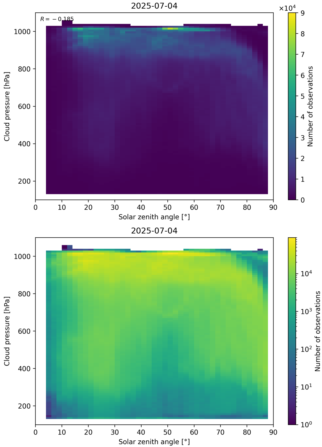
Figure 111: Scatter density plot of “Solar zenith angle” against “Cloud pressure” for 2025-07-03 to 2025-07-05.
