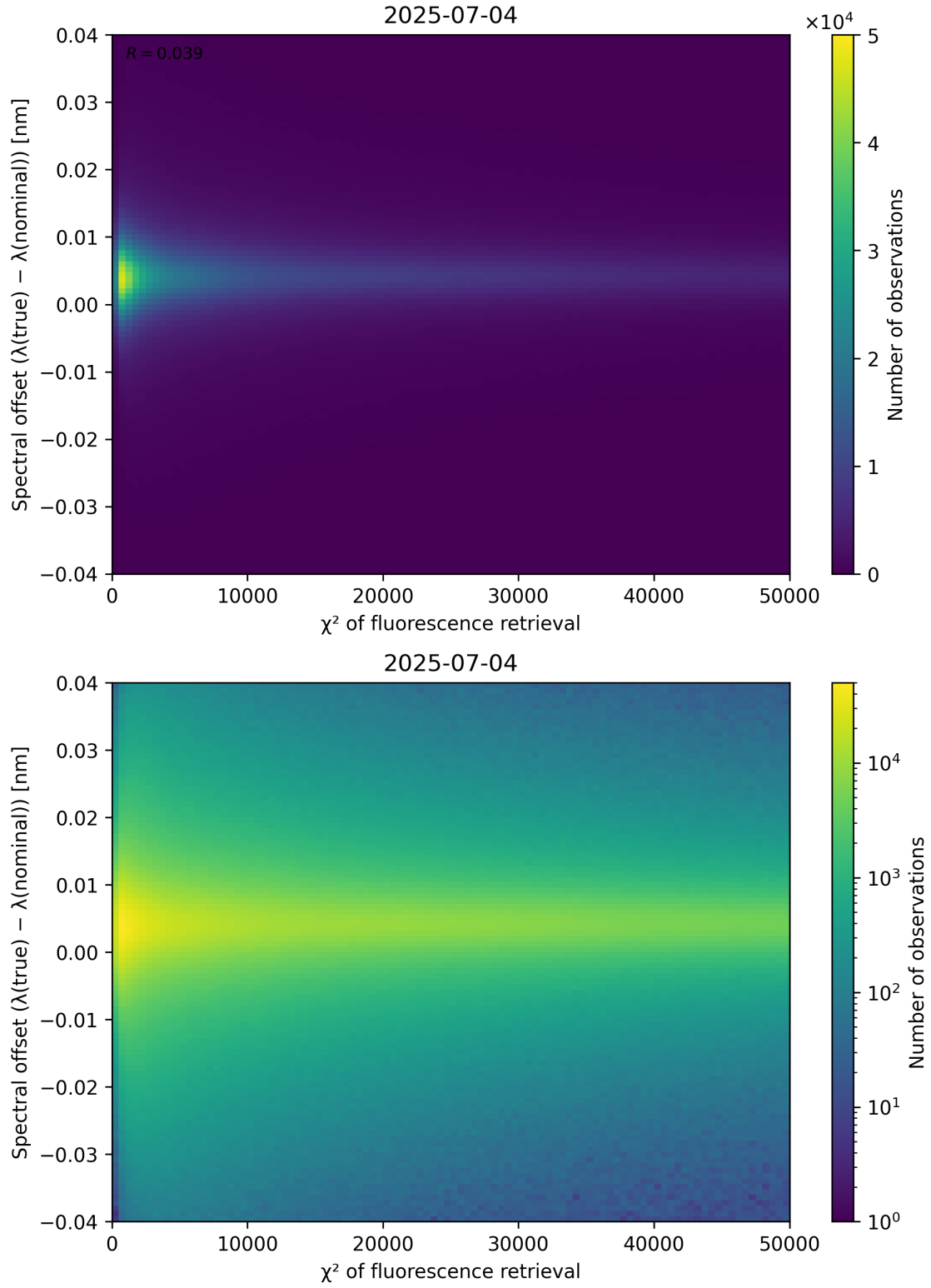
Figure 69: Scatter density plot of “ \chi^2 of fluorescence retrieval” against “Spectral offset ( \lambda_{\text{true}} - \lambda_{\text{nominal}} )” for 2025-07-03 to 2025-07-05.
