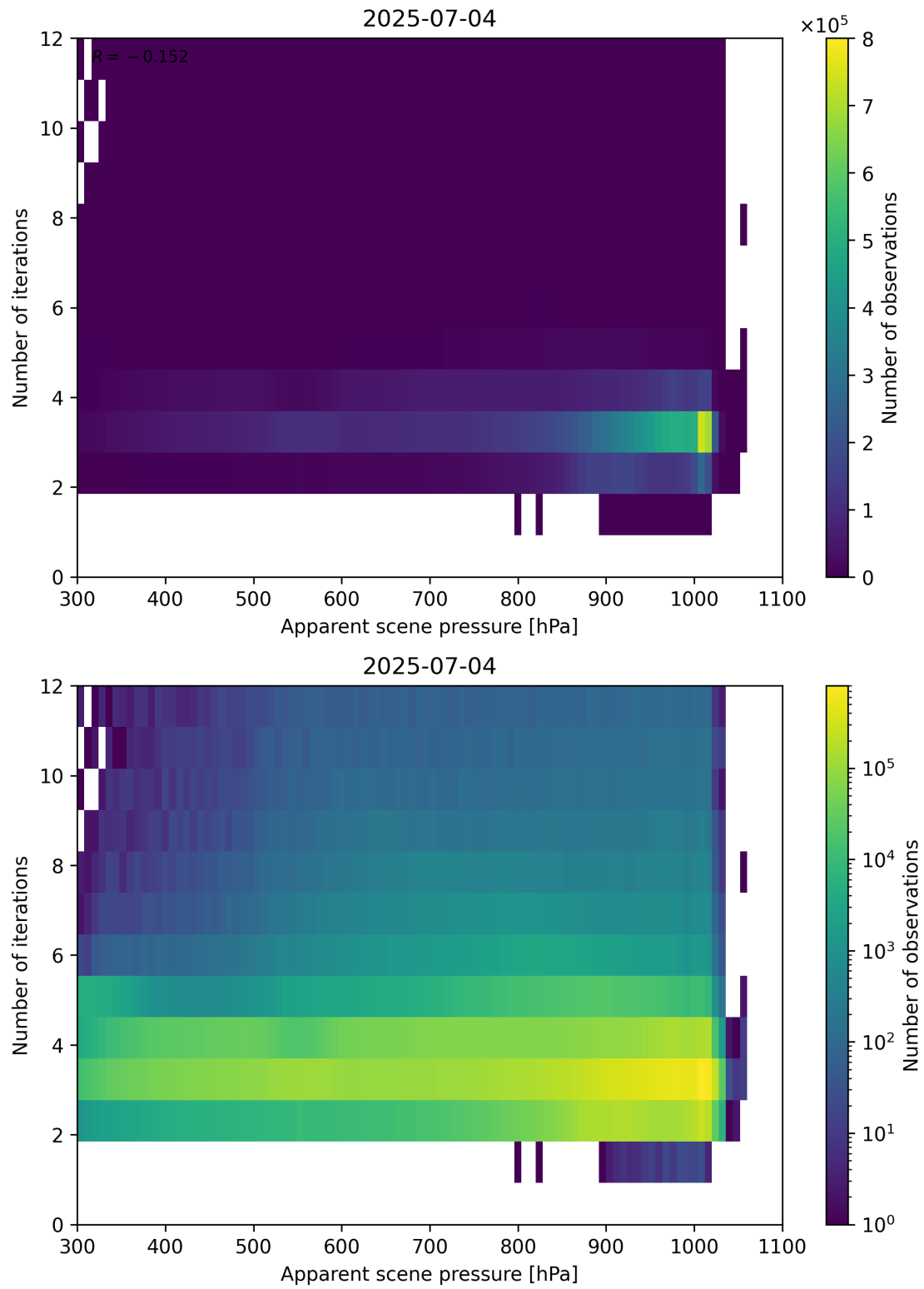
Figure 65: Scatter density plot of “Apparent scene pressure” against “Number of iterations” for 2025-07-03 to 2025-07-05.
