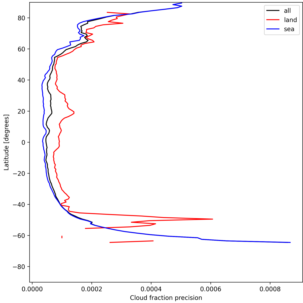
Figure 16: Zonal average of “Cloud fraction precision” for 2025-07-03 to 2025-07-05.
