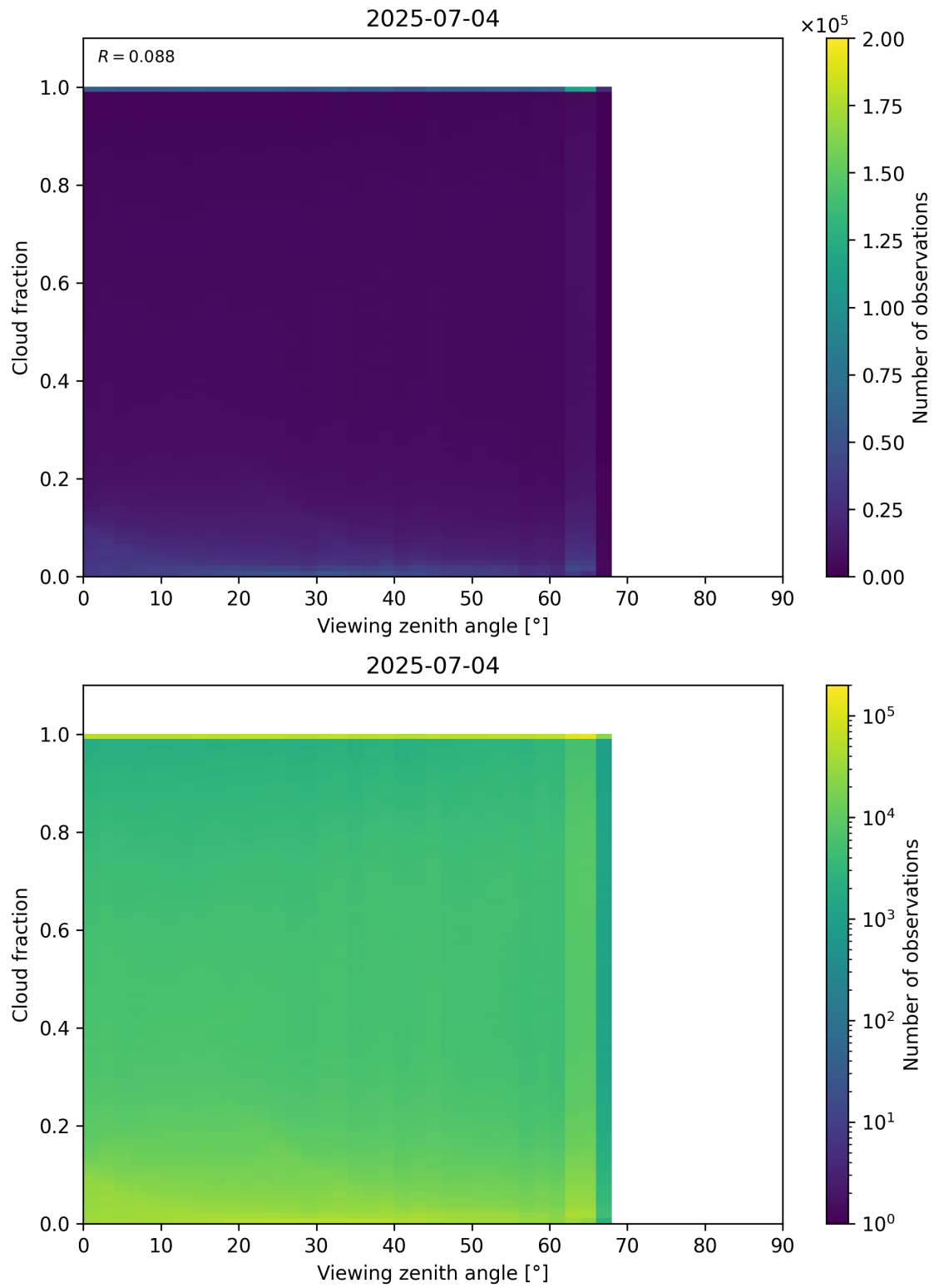
Figure 120: Scatter density plot of “Viewing zenith angle” against “Cloud fraction” for 2025-07-03 to 2025-07-05.
