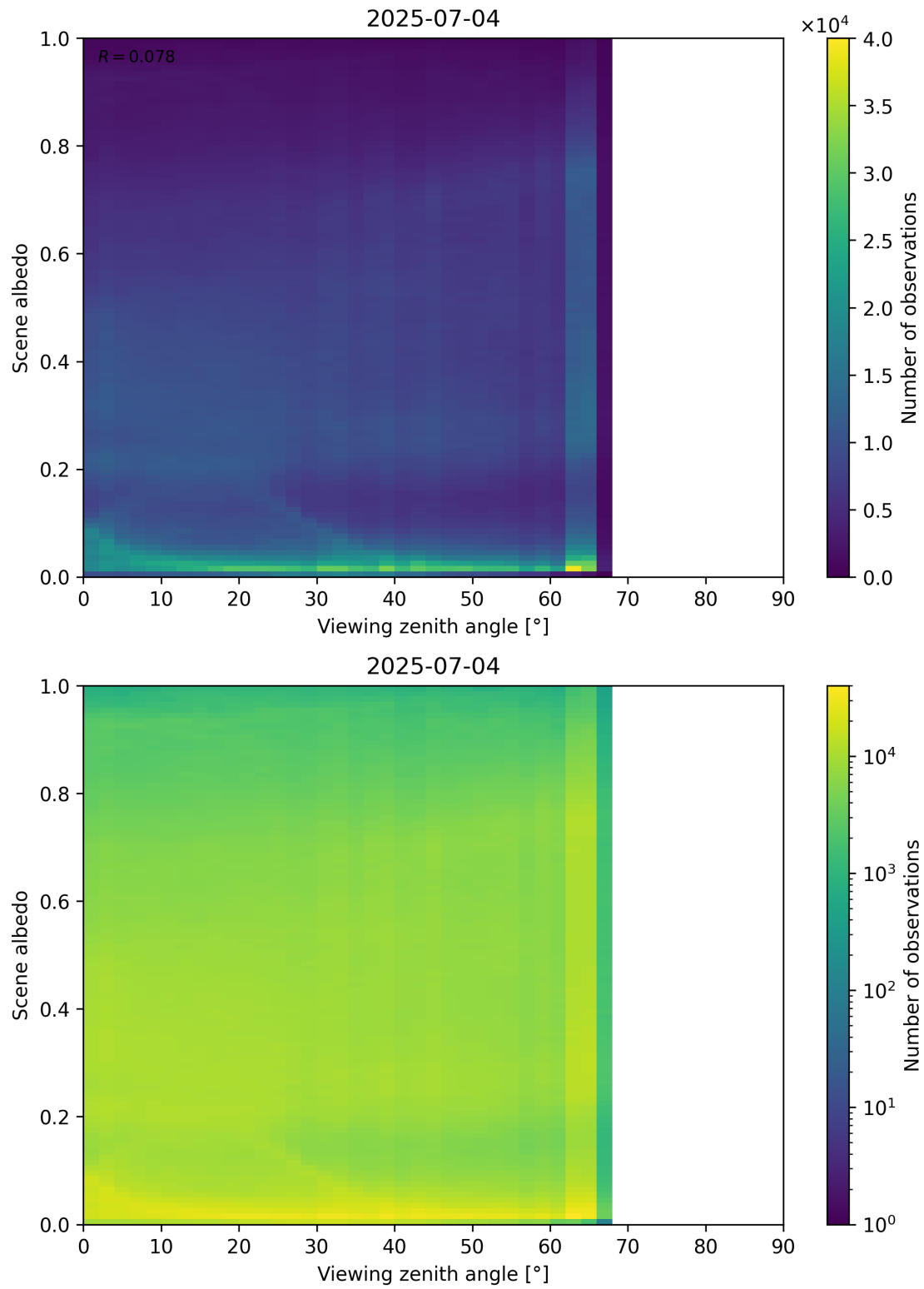
Figure 126: Scatter density plot of “Viewing zenith angle” against “Scene albedo” for 2025-07-03 to 2025-07-05.
