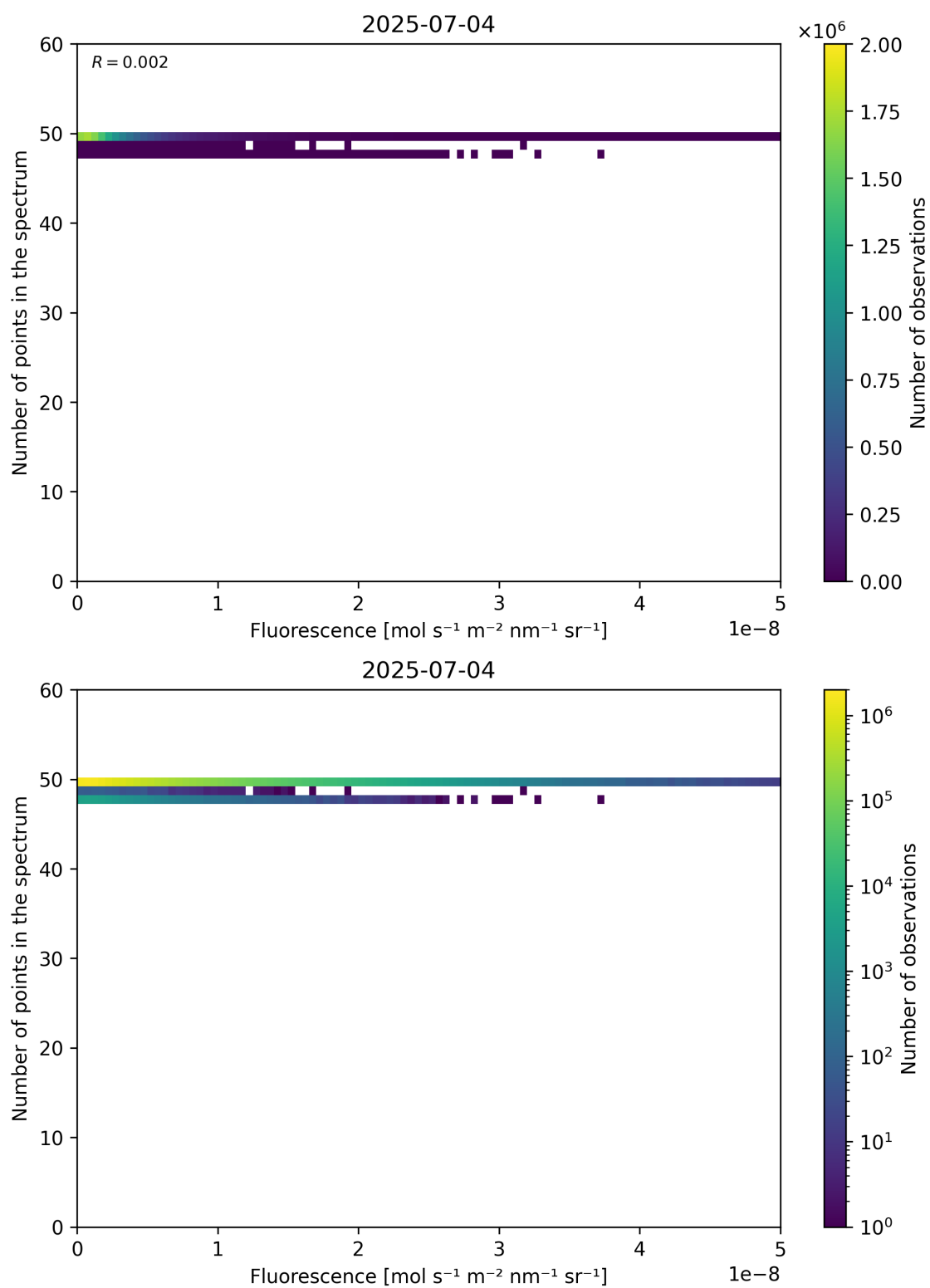
Figure 86: Scatter density plot of “Fluorescence” against “Number of points in the spectrum” for 2025-07-03 to 2025-07-05.
