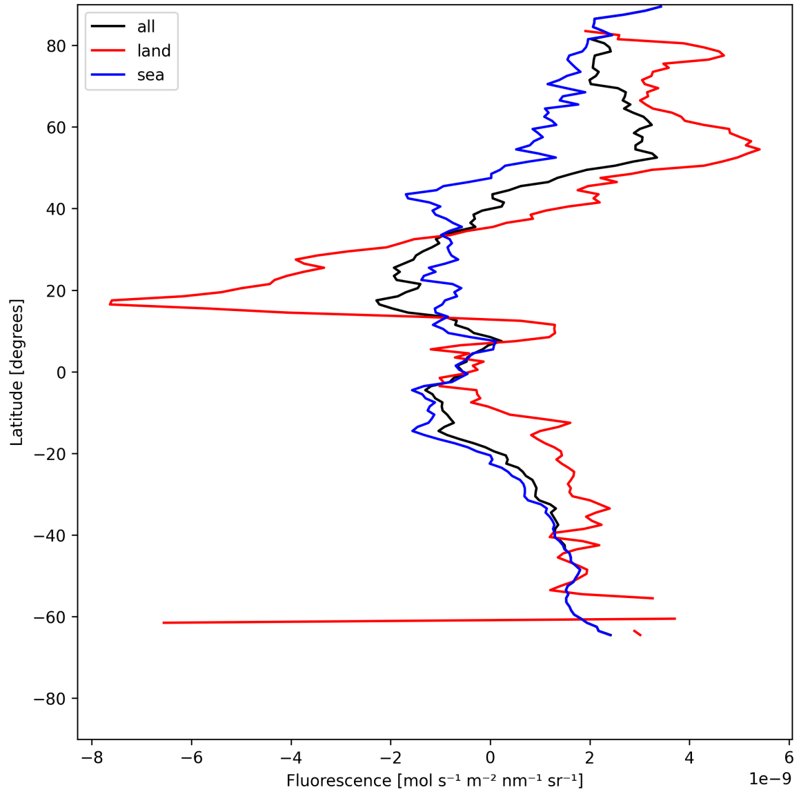
Figure 23: Zonal average of “Fluorescence” for 2025-07-03 to 2025-07-05.
