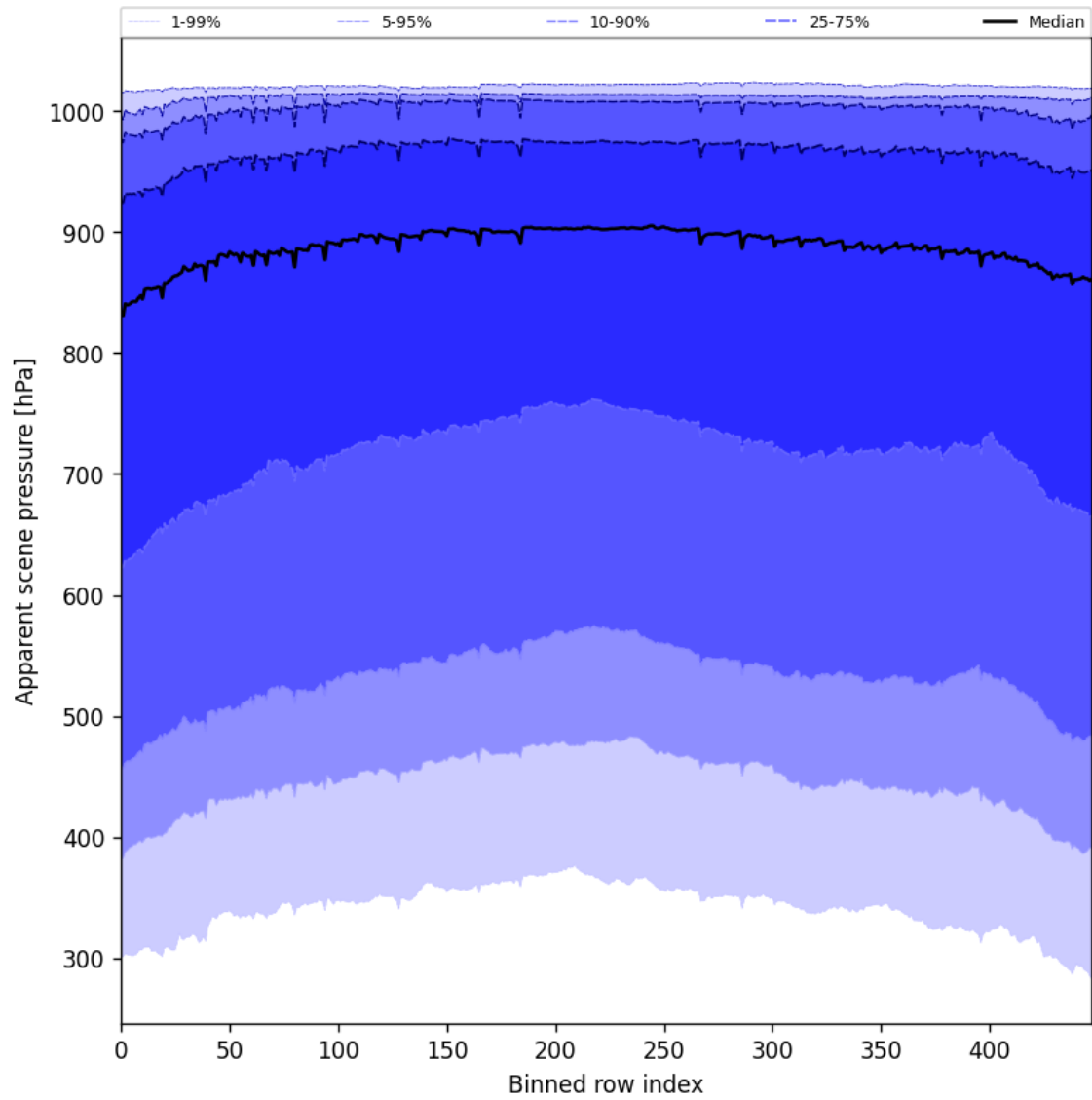
Figure 53: Along track statistics of “Apparent scene pressure” for 2025-07-03 to 2025-07-05
