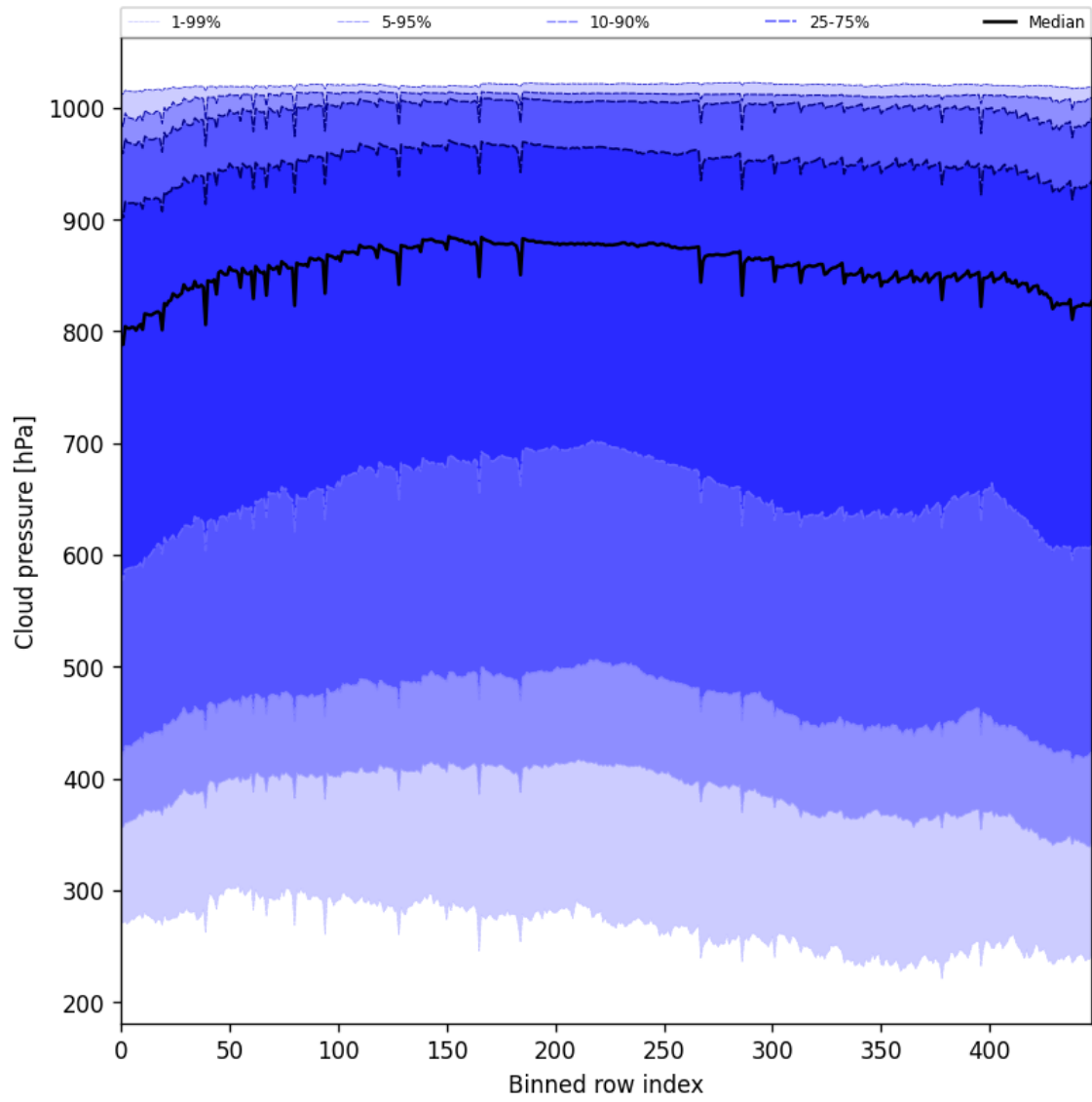
Figure 47: Along track statistics of “Cloud pressure” for 2025-07-03 to 2025-07-05
