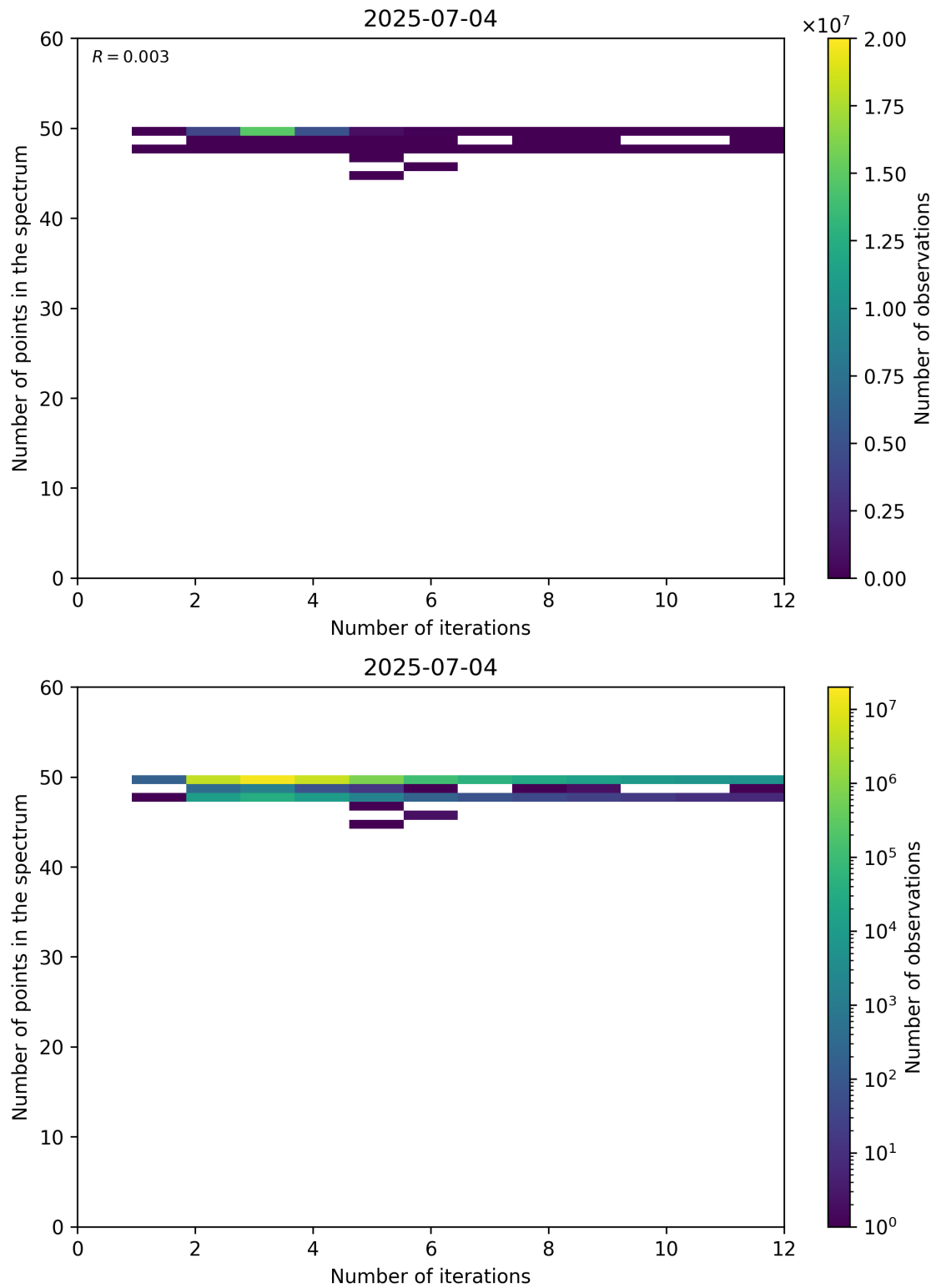
Figure 99: Scatter density plot of “Number of iterations” against “Number of points in the spectrum” for 2025-07-03 to 2025-07-05.
