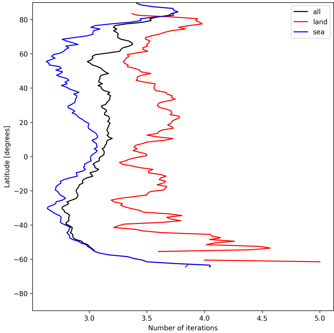
Figure 22: Zonal average of “Number of iterations” for 2025-07-03 to 2025-07-05.
