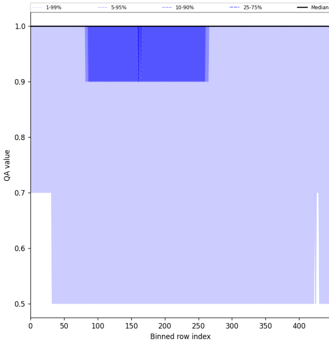
Figure 46: Along track statistics of “QA value” for 2025-07-03 to 2025-07-05
