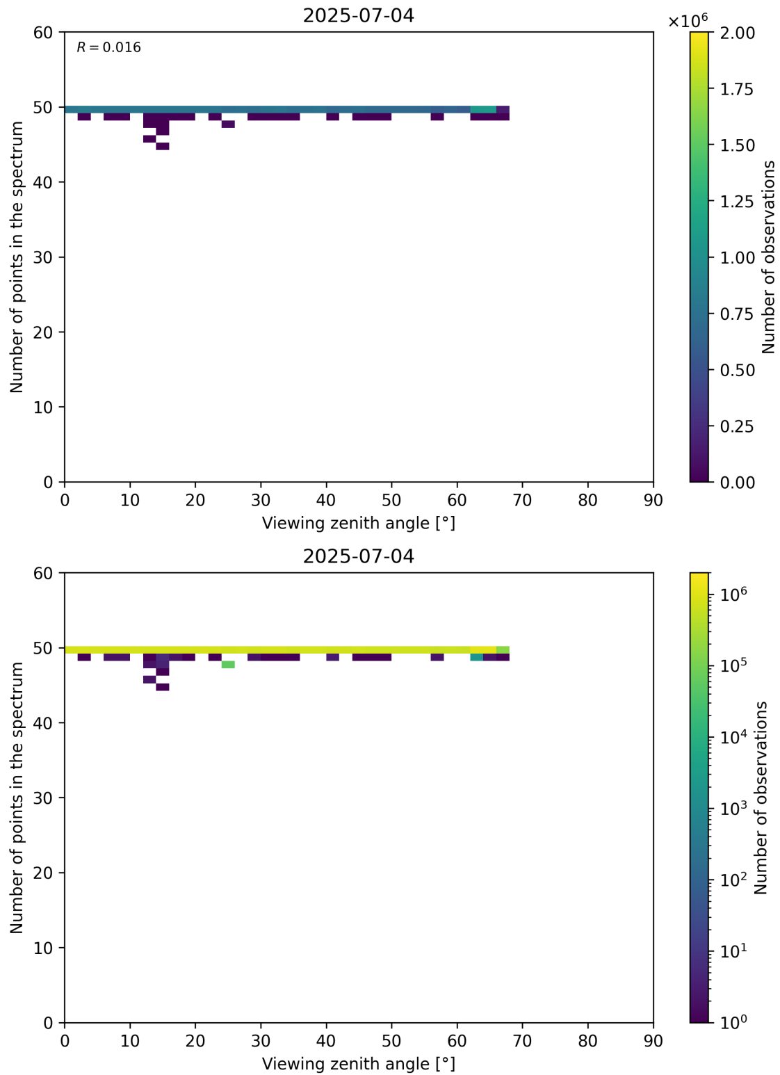
Figure 125: Scatter density plot of “Viewing zenith angle” against “Number of points in the spectrum” for 2025-07-03 to 2025-07-05.
