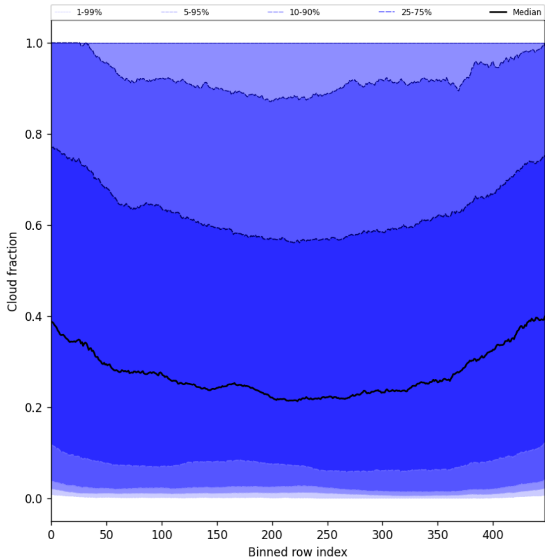
Figure 49: Along track statistics of “Cloud fraction” for 2025-07-03 to 2025-07-05
