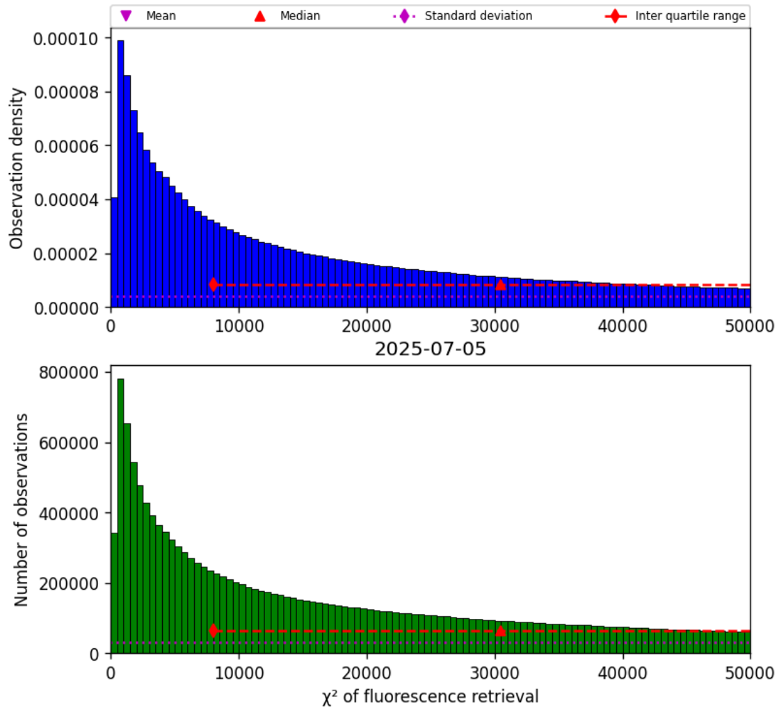
Figure 42: Histogram of “ \chi^2 of fluorescence retrieval” for 2025-07-04 to 2025-07-06
