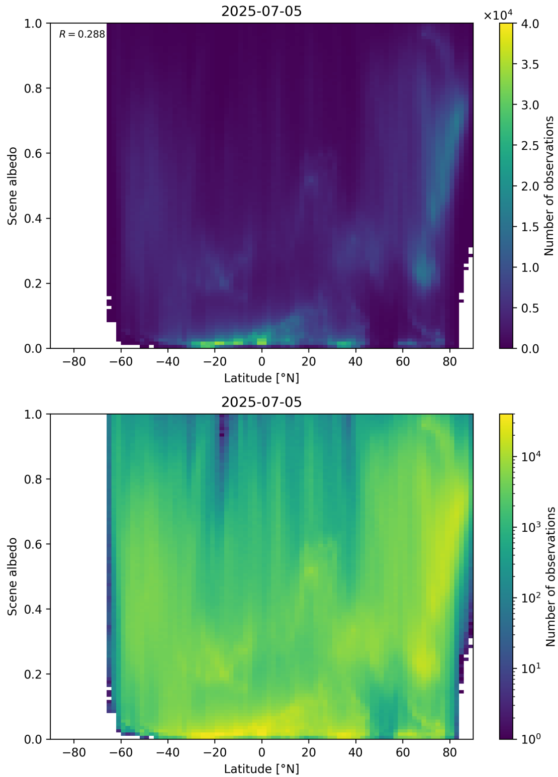
Figure 95: Scatter density plot of “Latitude” against “Scene albedo” for 2025-07-04 to 2025-07-06.
