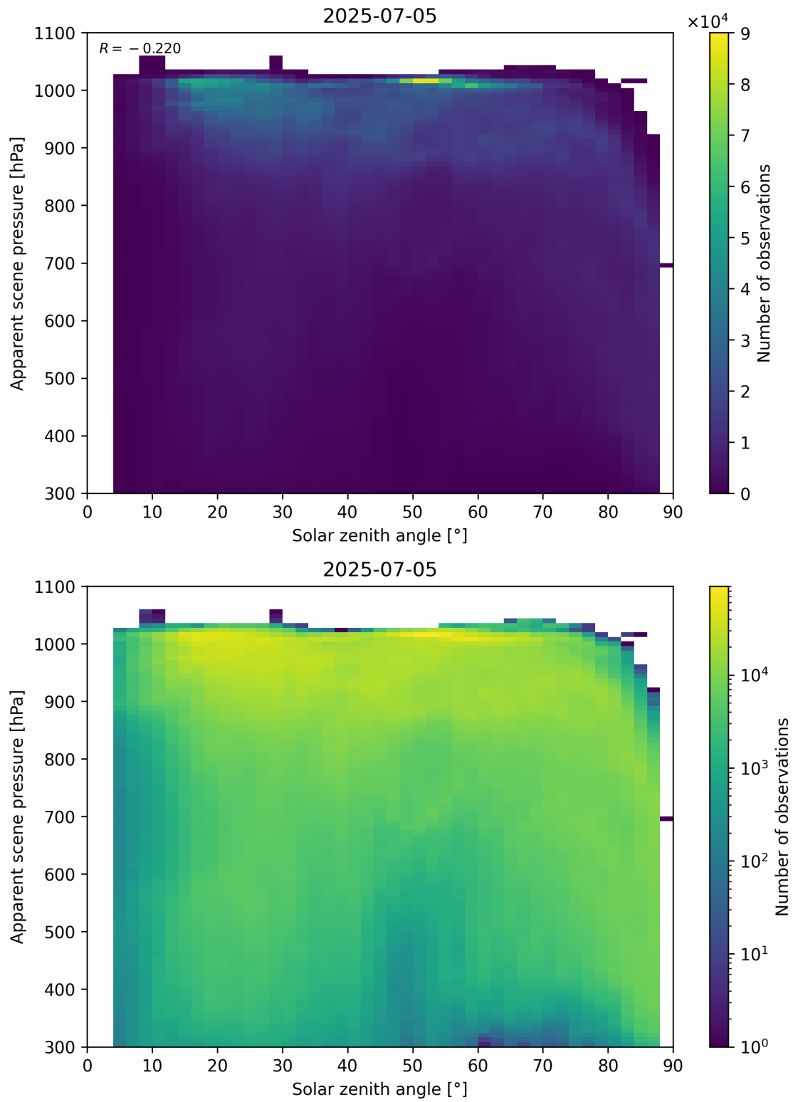
Figure 108: Scatter density plot of “Solar zenith angle” against “Apparent scene pressure” for 2025-07-04 to 2025-07-06.
