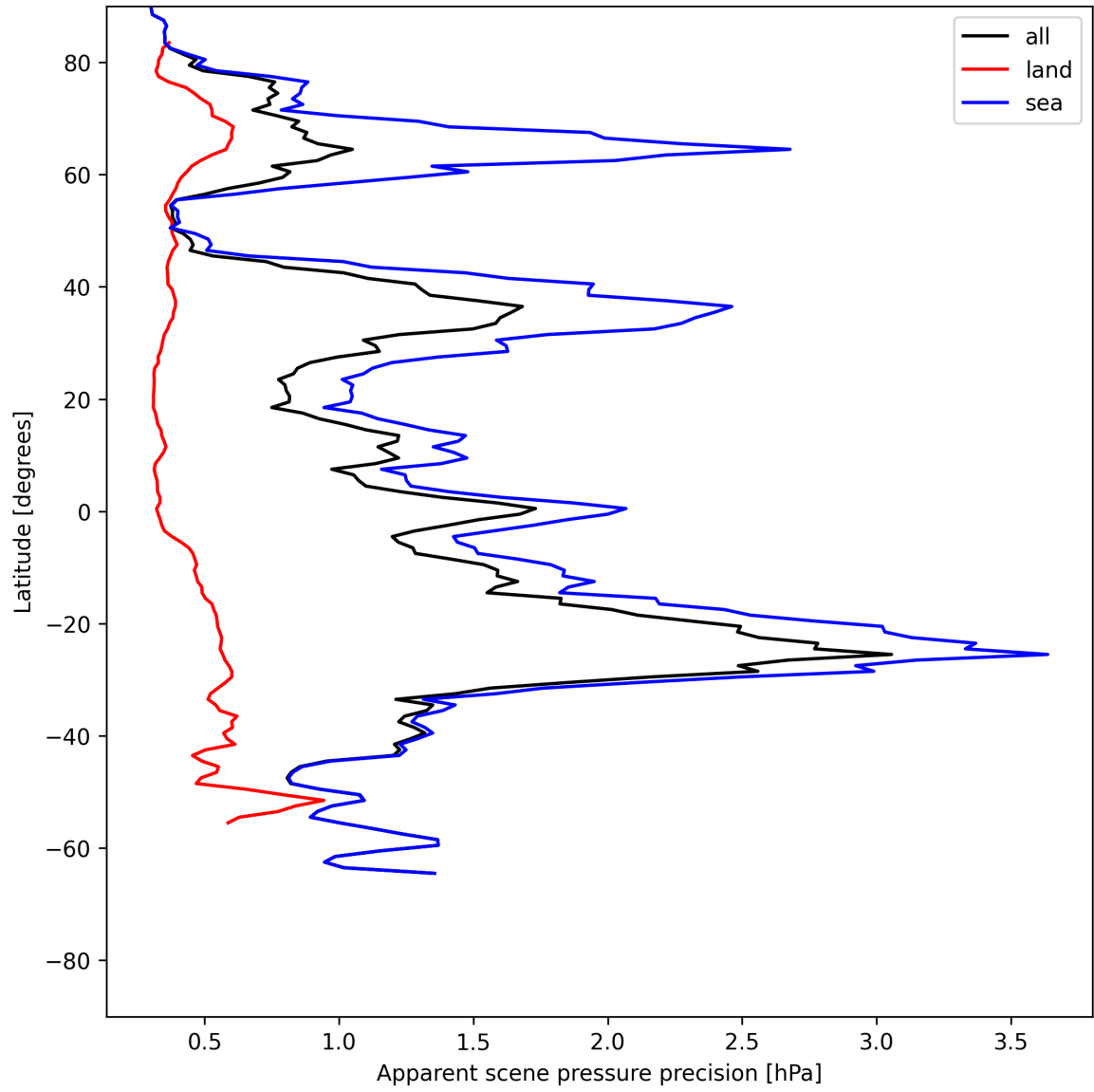
Figure 20: Zonal average of “Apparent scene pressure precision” for 2025-07-04 to 2025-07-06.
