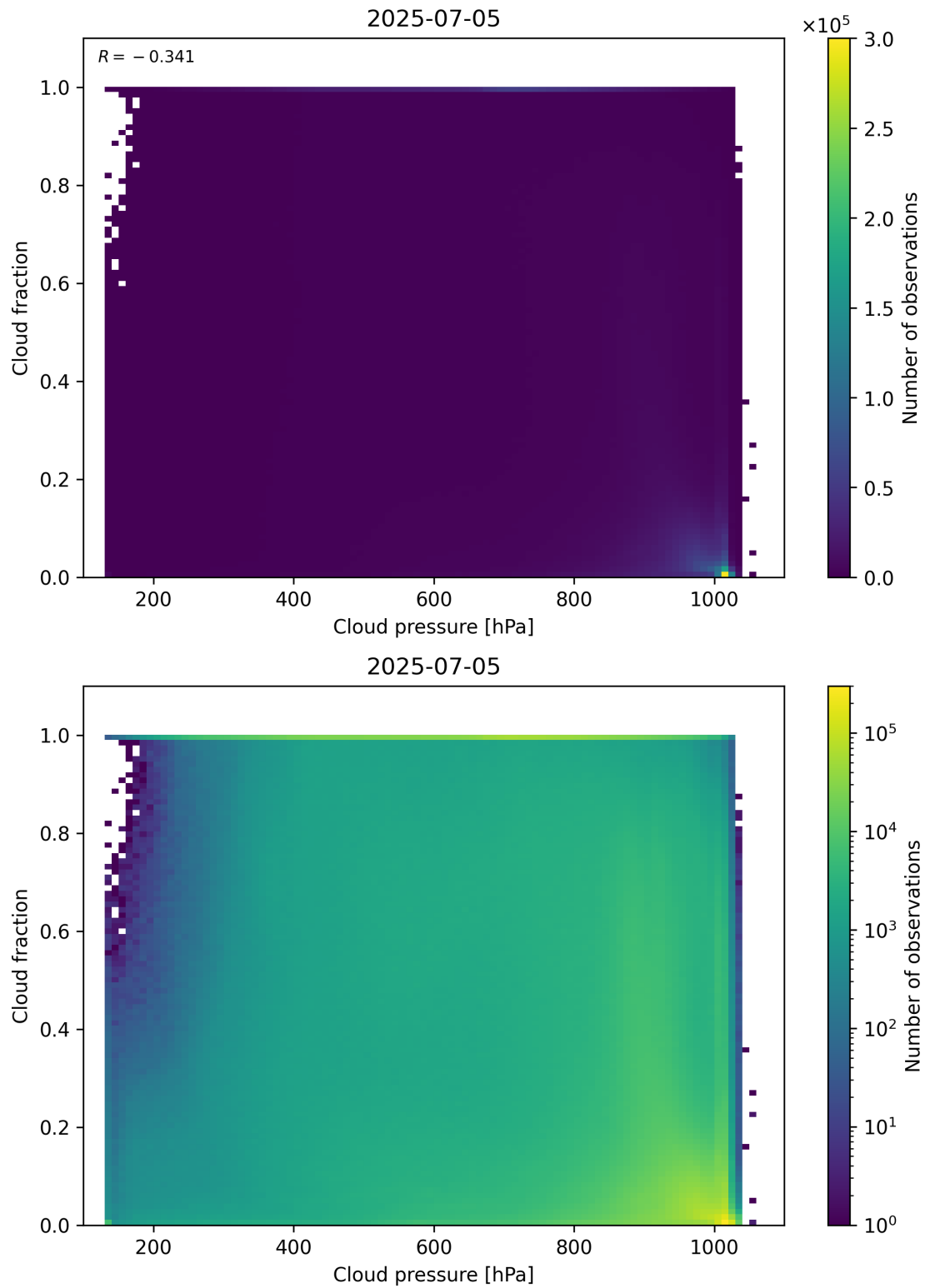
Figure 79: Scatter density plot of “Cloud pressure” against “Cloud fraction” for 2025-07-04 to 2025-07-06.
