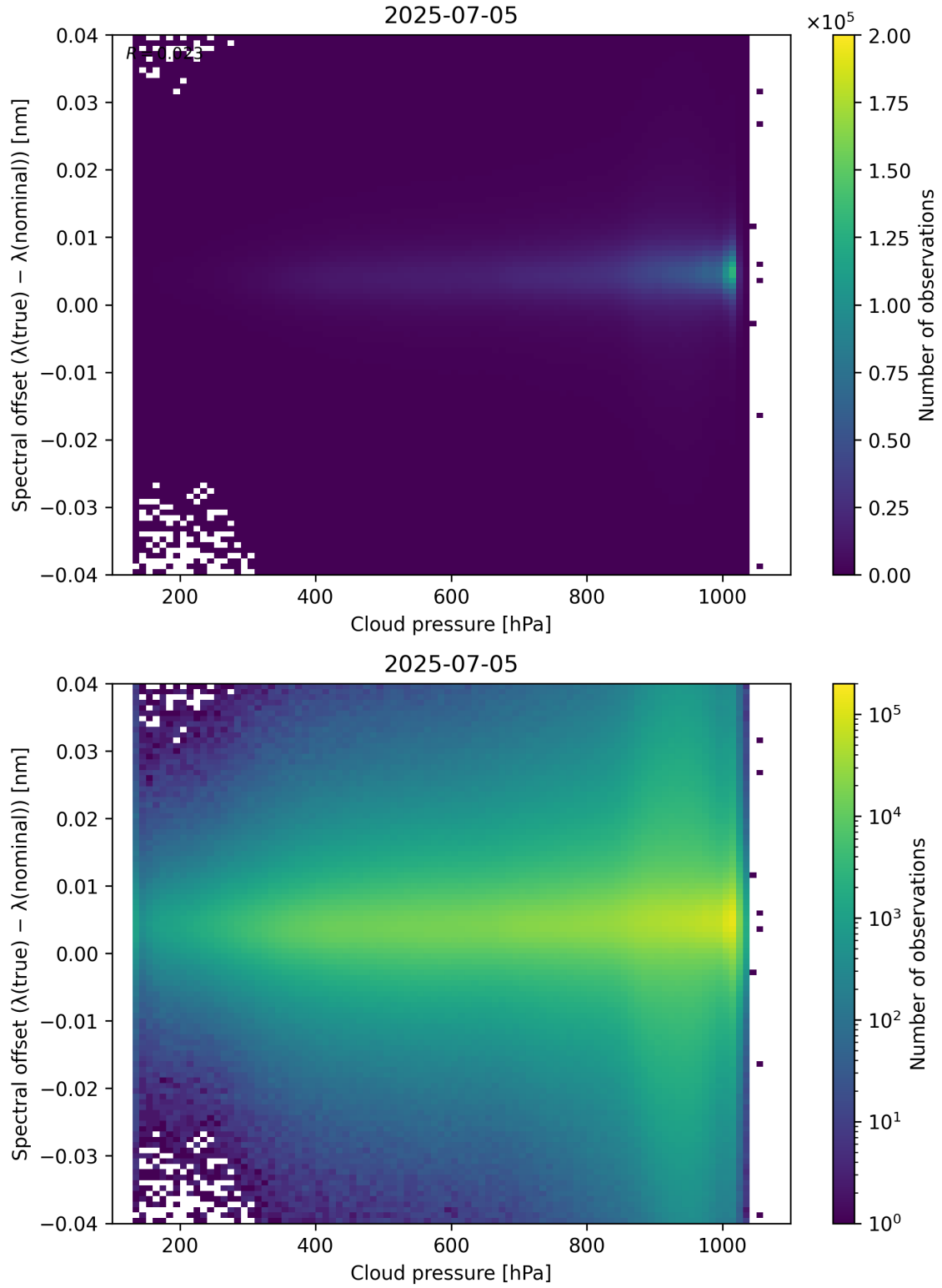
Figure 84: Scatter density plot of “Cloud pressure” against “Spectral offset ( \lambda_{\text{true}} - \lambda_{\text{nominal}} )” for 2025-07-04 to 2025-07-06.
