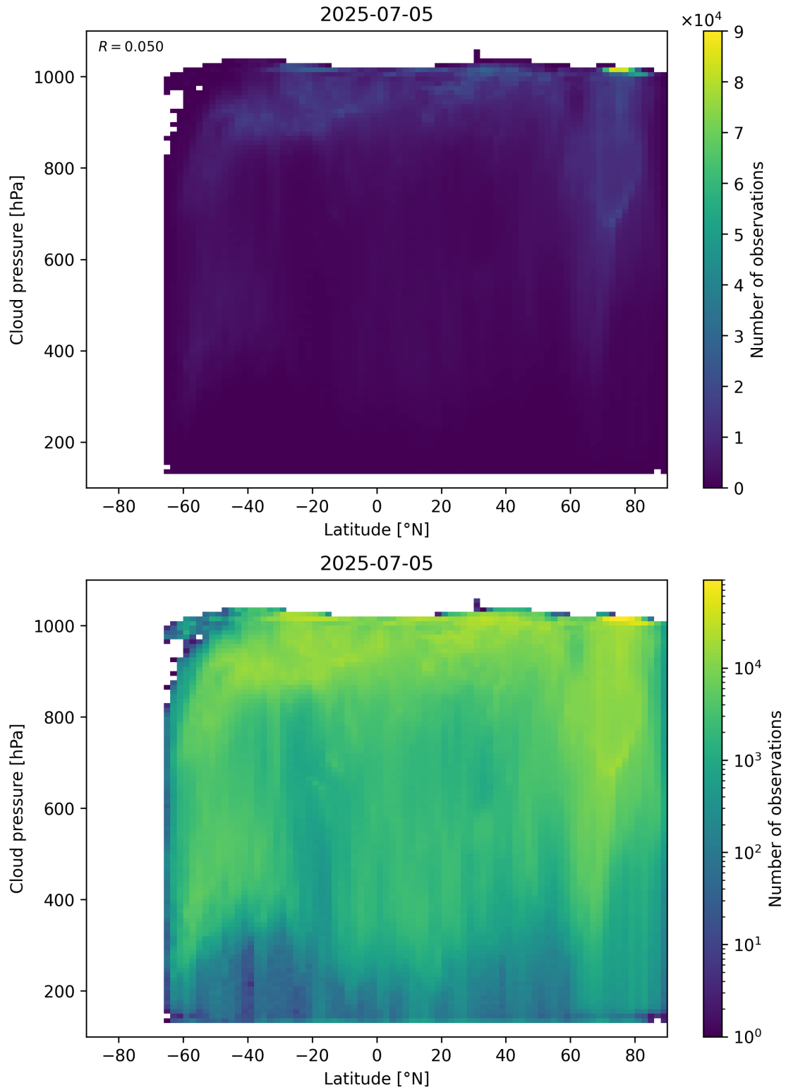
Figure 91: Scatter density plot of “Latitude” against “Cloud pressure” for 2025-07-04 to 2025-07-06.
