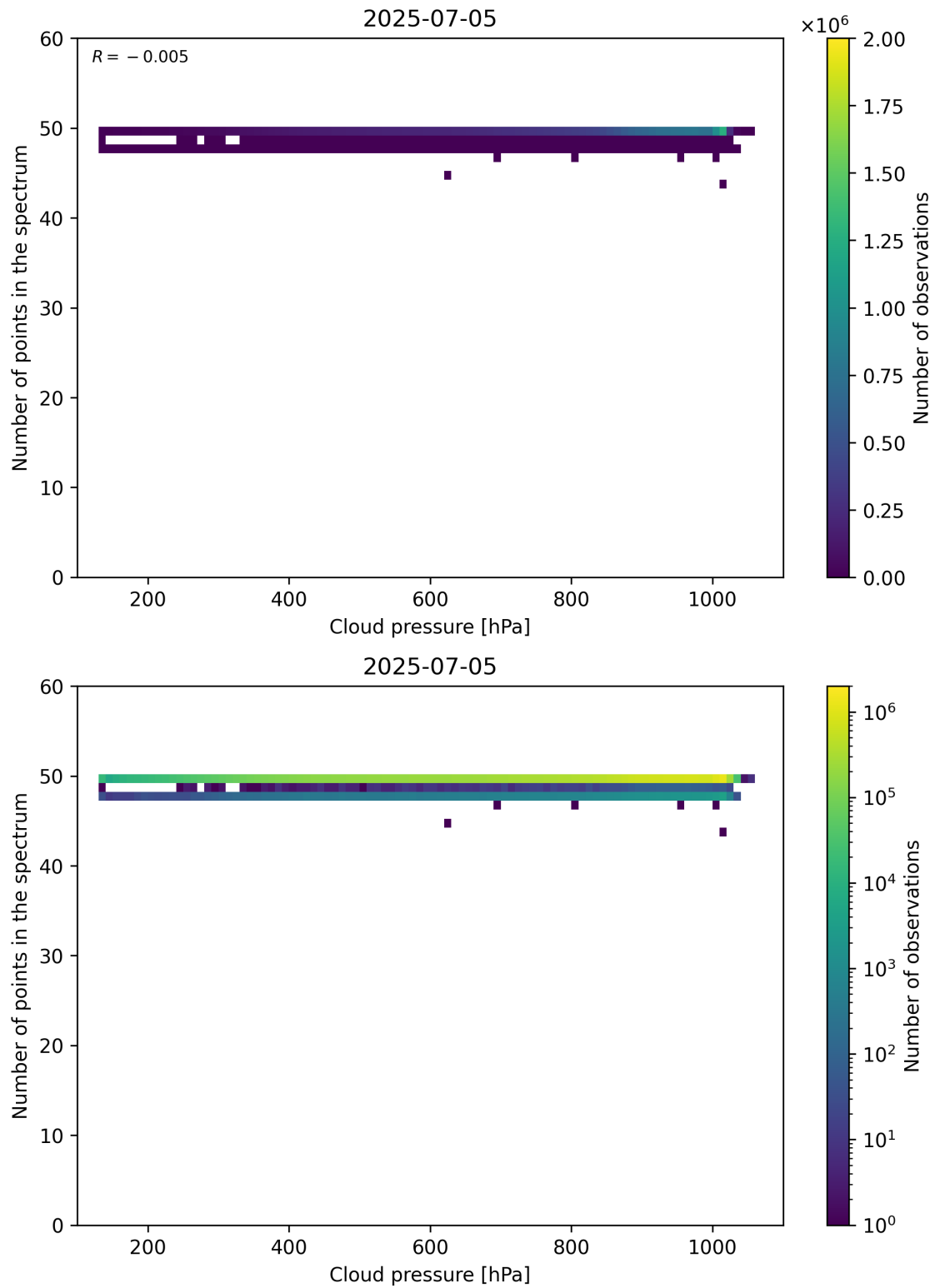
Figure 82: Scatter density plot of “Cloud pressure” against “Number of points in the spectrum” for 2025-07-04 to 2025-07-06.
