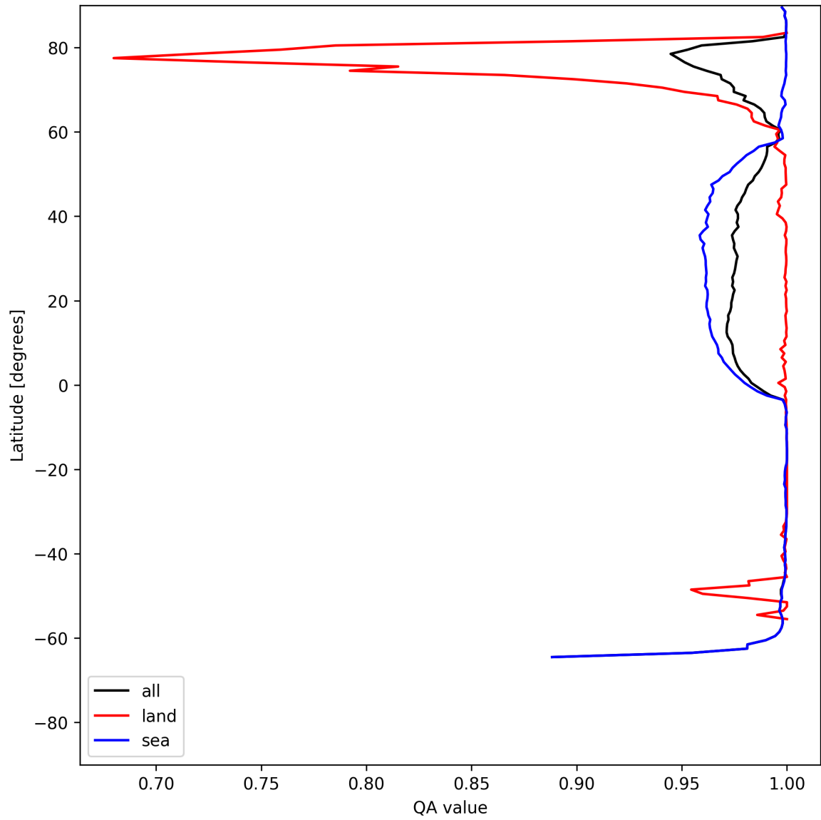
Figure 12: Zonal average of “QA value” for 2025-07-04 to 2025-07-06.
