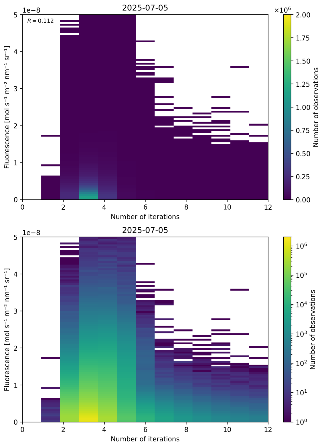
Figure 98: Scatter density plot of “Number of iterations” against “Fluorescence” for 2025-07-04 to 2025-07-06.
