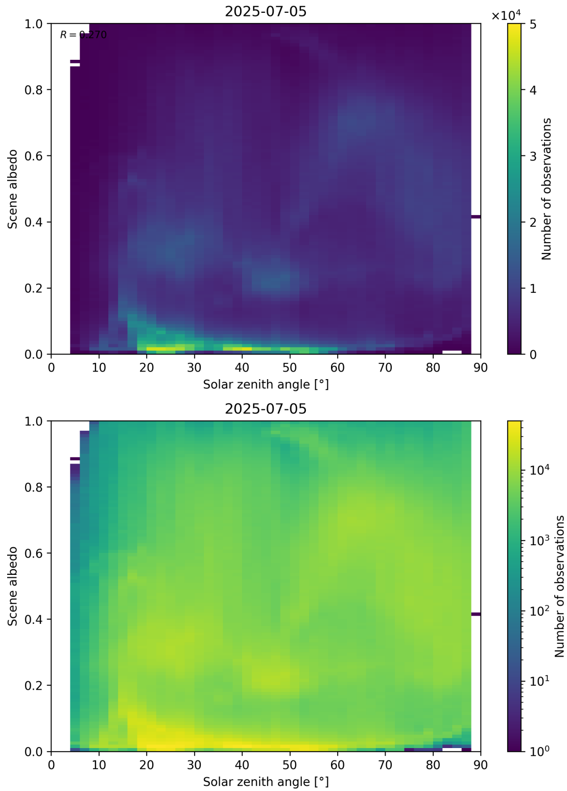
Figure 116: Scatter density plot of “Solar zenith angle” against “Scene albedo” for 2025-07-04 to 2025-07-06.
