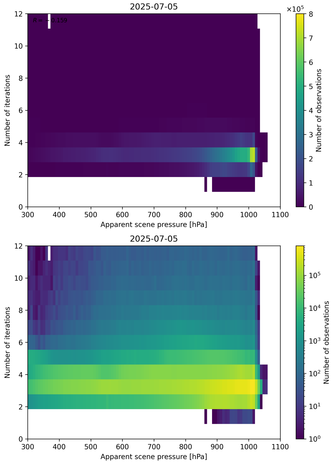
Figure 65: Scatter density plot of “Apparent scene pressure” against “Number of iterations” for 2025-07-04 to 2025-07-06.
