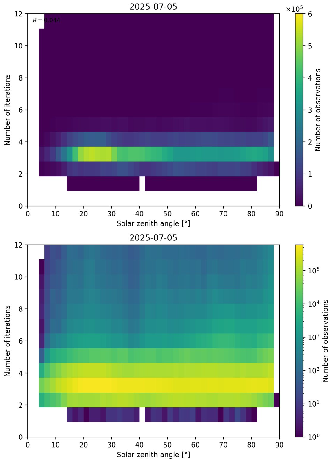
Figure 114: Scatter density plot of “Solar zenith angle” against “Number of iterations” for 2025-07-04 to 2025-07-06.
