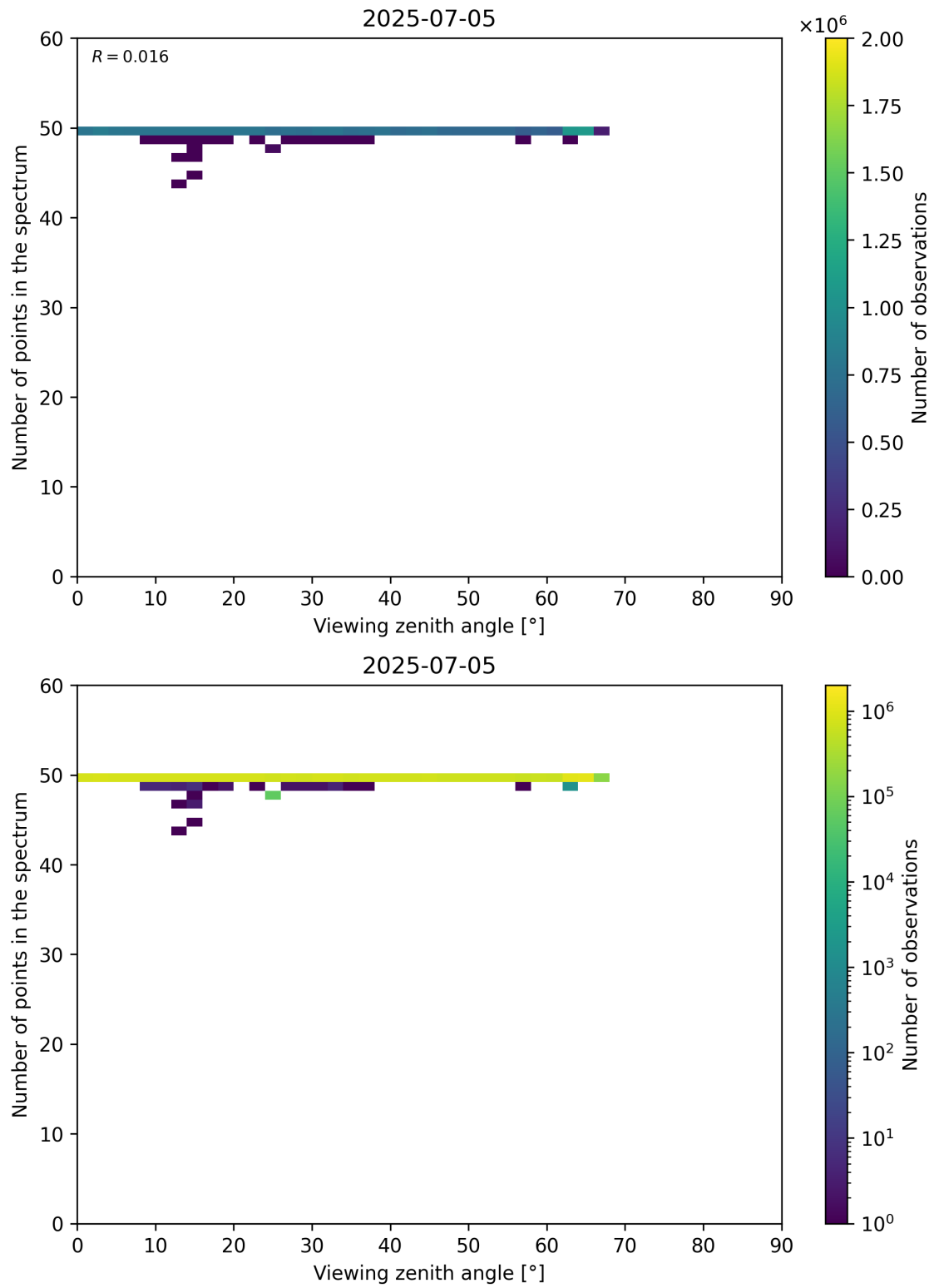
Figure 125: Scatter density plot of “Viewing zenith angle” against “Number of points in the spectrum” for 2025-07-04 to 2025-07-06.
