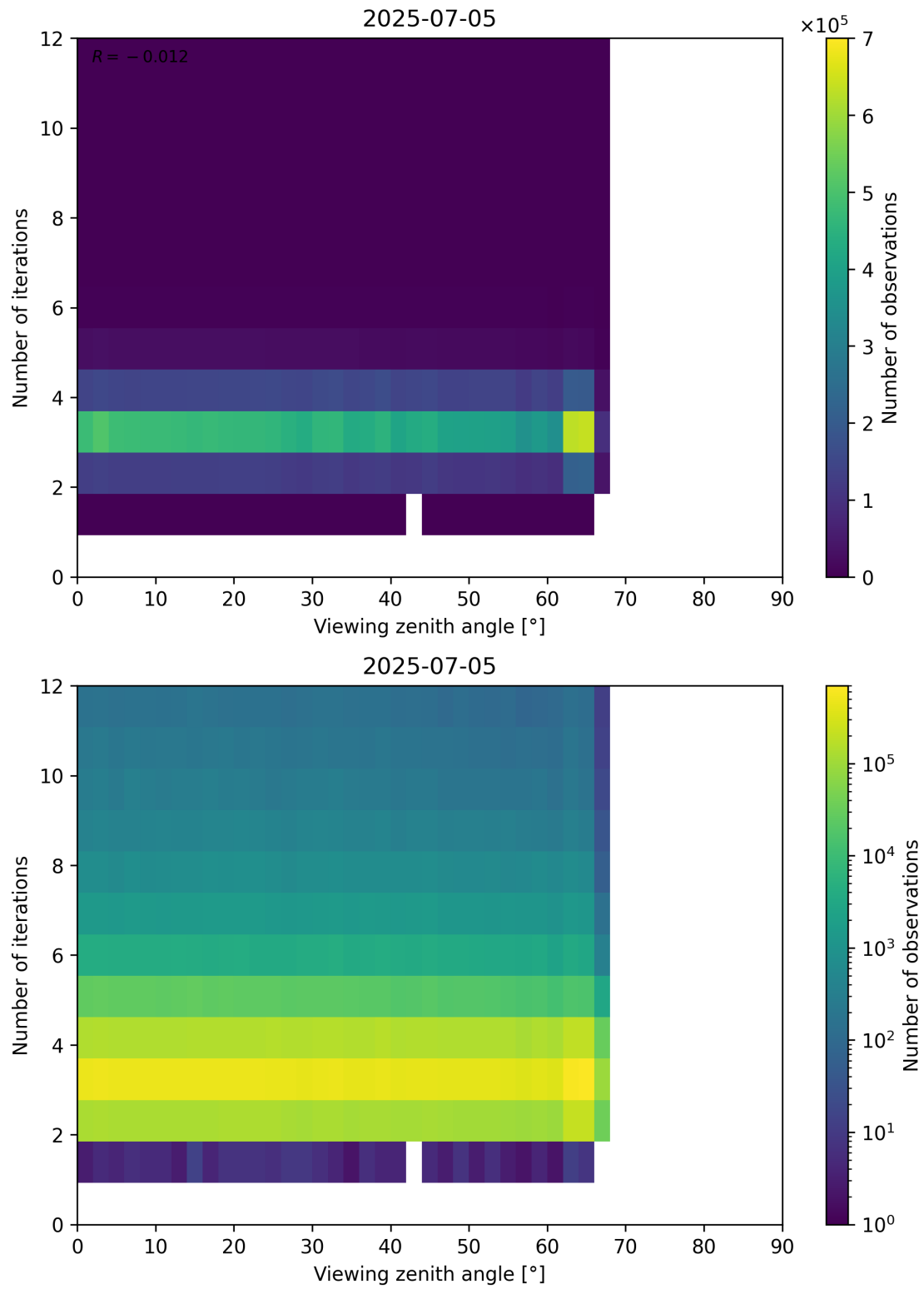
Figure 124: Scatter density plot of “Viewing zenith angle” against “Number of iterations” for 2025-07-04 to 2025-07-06.
