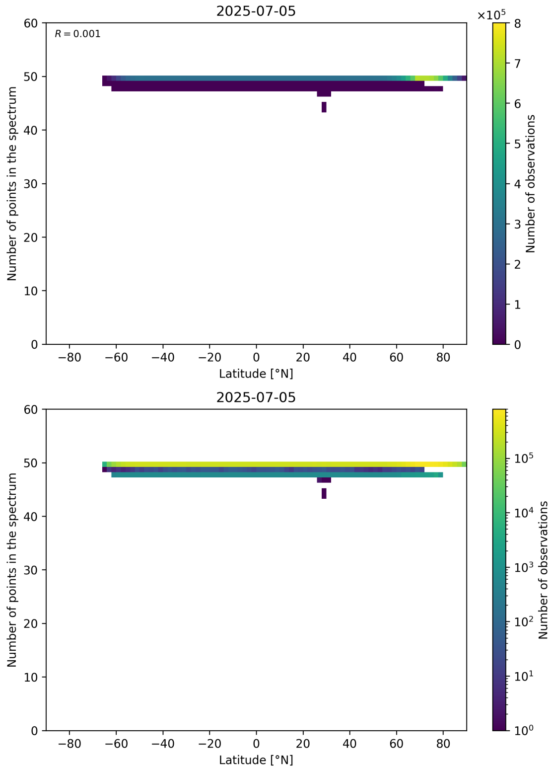
Figure 94: Scatter density plot of “Latitude” against “Number of points in the spectrum” for 2025-07-04 to 2025-07-06.
