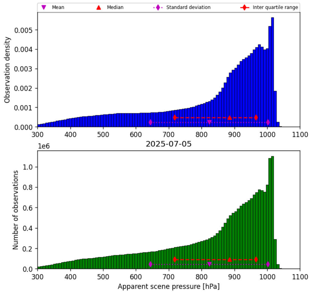
Figure 36: Histogram of “Apparent scene pressure” for 2025-07-04 to 2025-07-06
