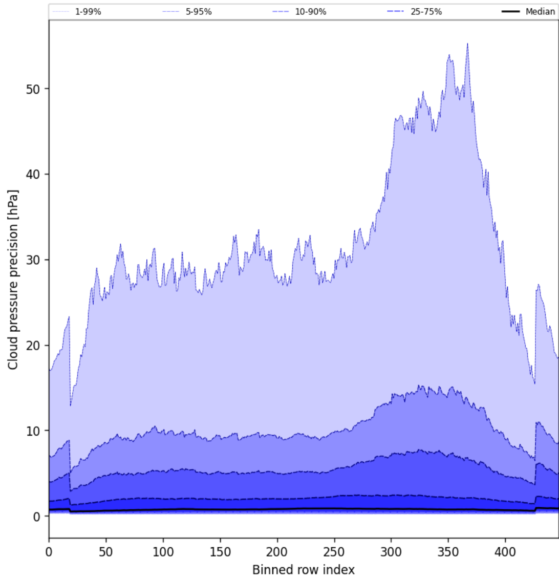
Figure 48: Along track statistics of “Cloud pressure precision” for 2025-07-04 to 2025-07-06
