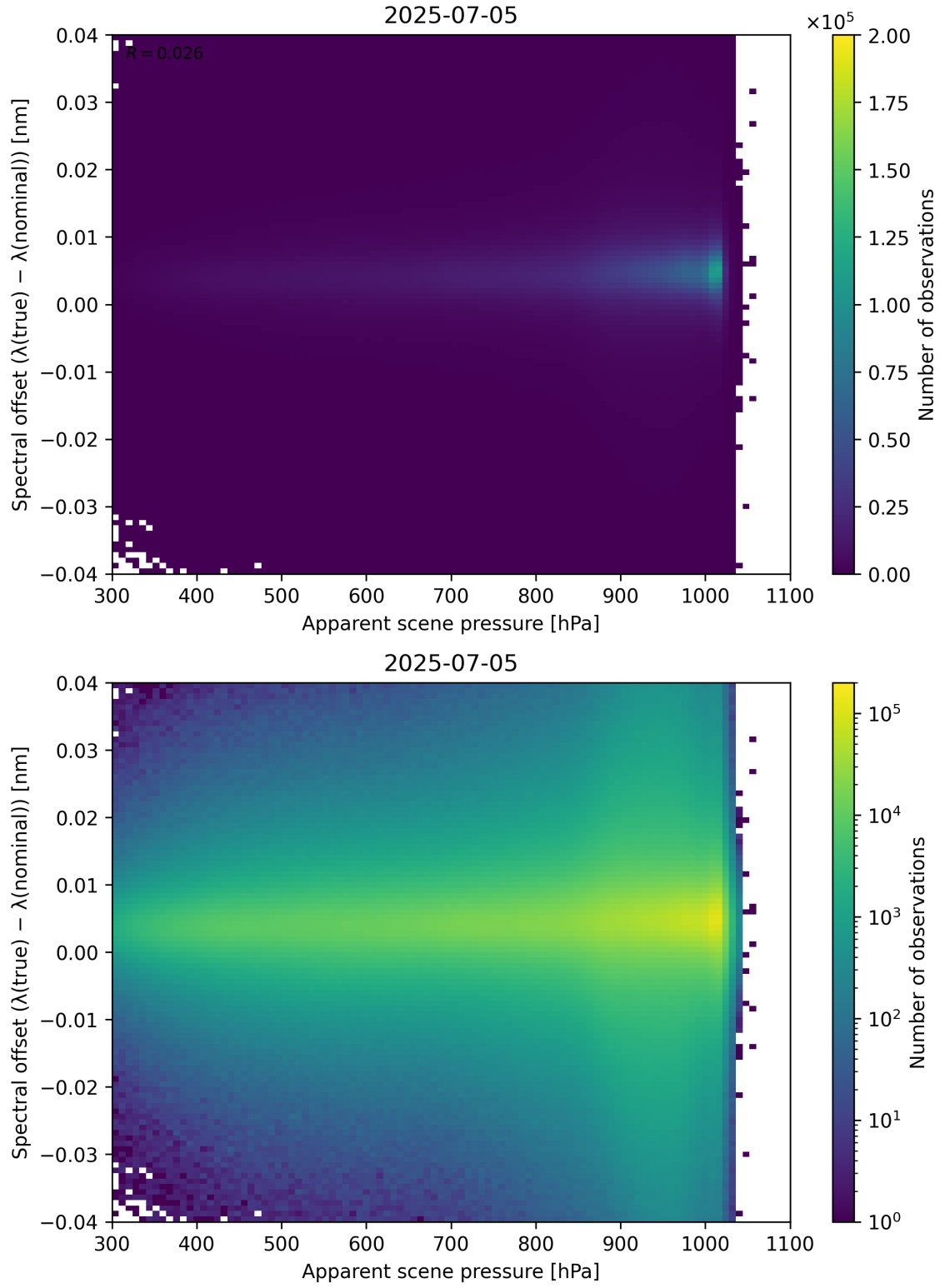
Figure 67: Scatter density plot of “Apparent scene pressure” against “Spectral offset ( \lambda_{\text{true}} - \lambda_{\text{nominal}} )” for 2025-07-04 to 2025-07-06.
