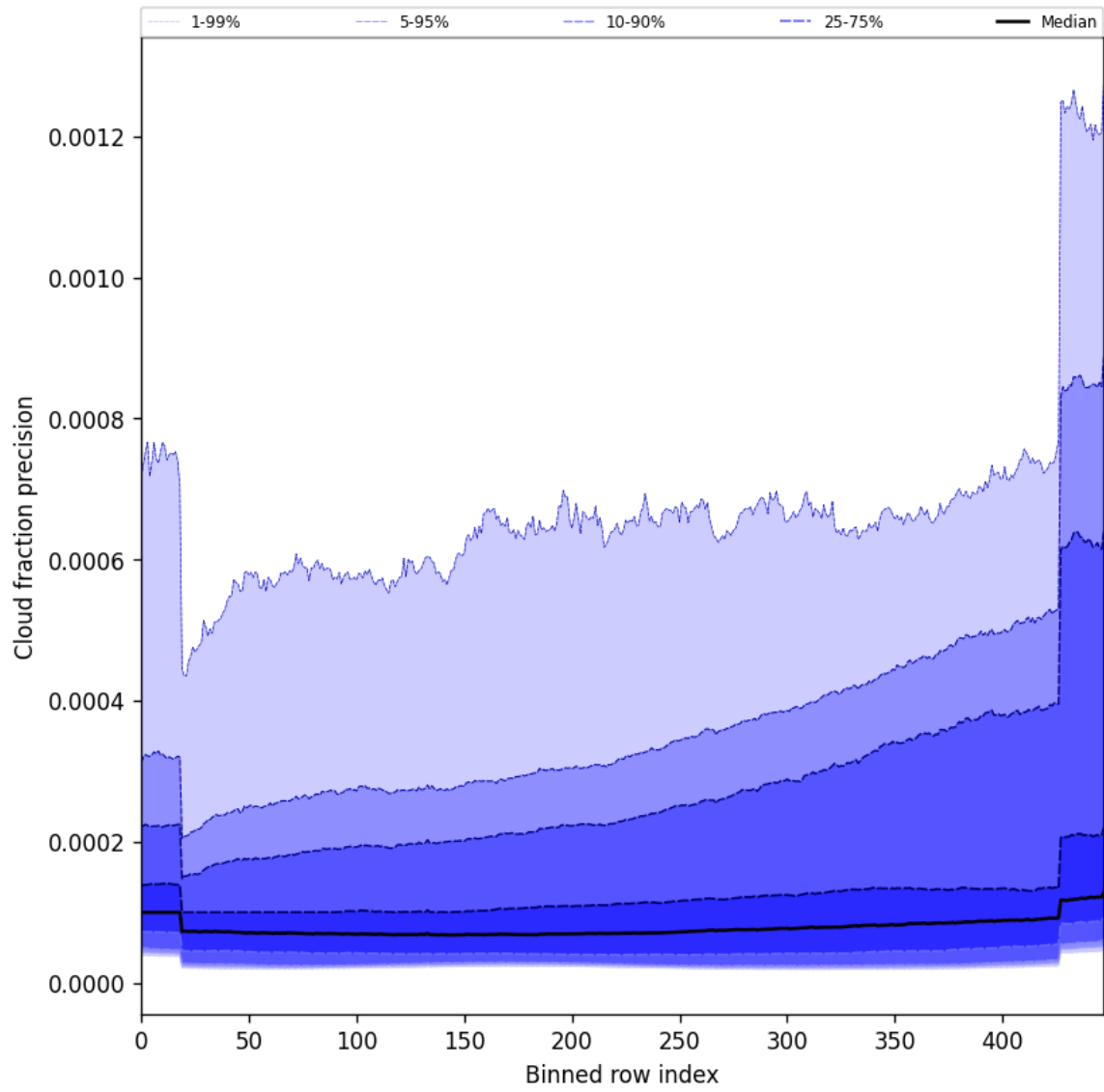
Figure 50: Along track statistics of “Cloud fraction precision” for 2025-07-04 to 2025-07-06
