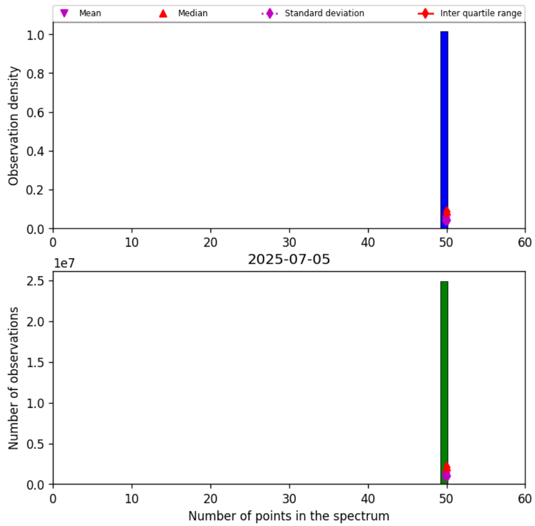
Figure 44: Histogram of “Number of points in the spectrum” for 2025-07-04 to 2025-07-06
