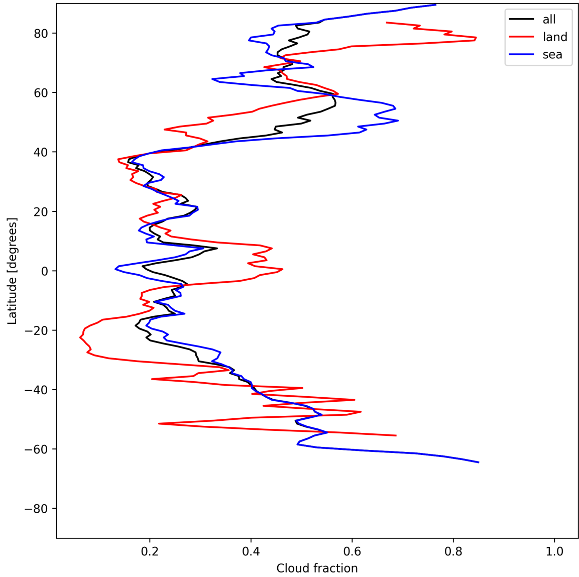
Figure 15: Zonal average of “Cloud fraction” for 2025-07-04 to 2025-07-06.
