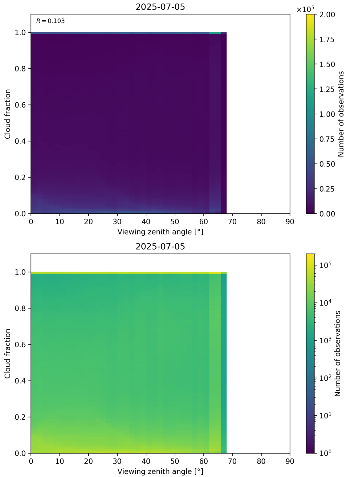
Figure 120: Scatter density plot of “Viewing zenith angle” against “Cloud fraction” for 2025-07-04 to 2025-07-06.
