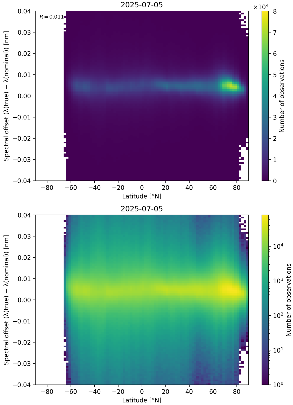
Figure 96: Scatter density plot of “Latitude” against “Spectral offset ( \lambda_{\text{true}} - \lambda_{\text{nominal}} )” for 2025-07-04 to 2025-07-06.
