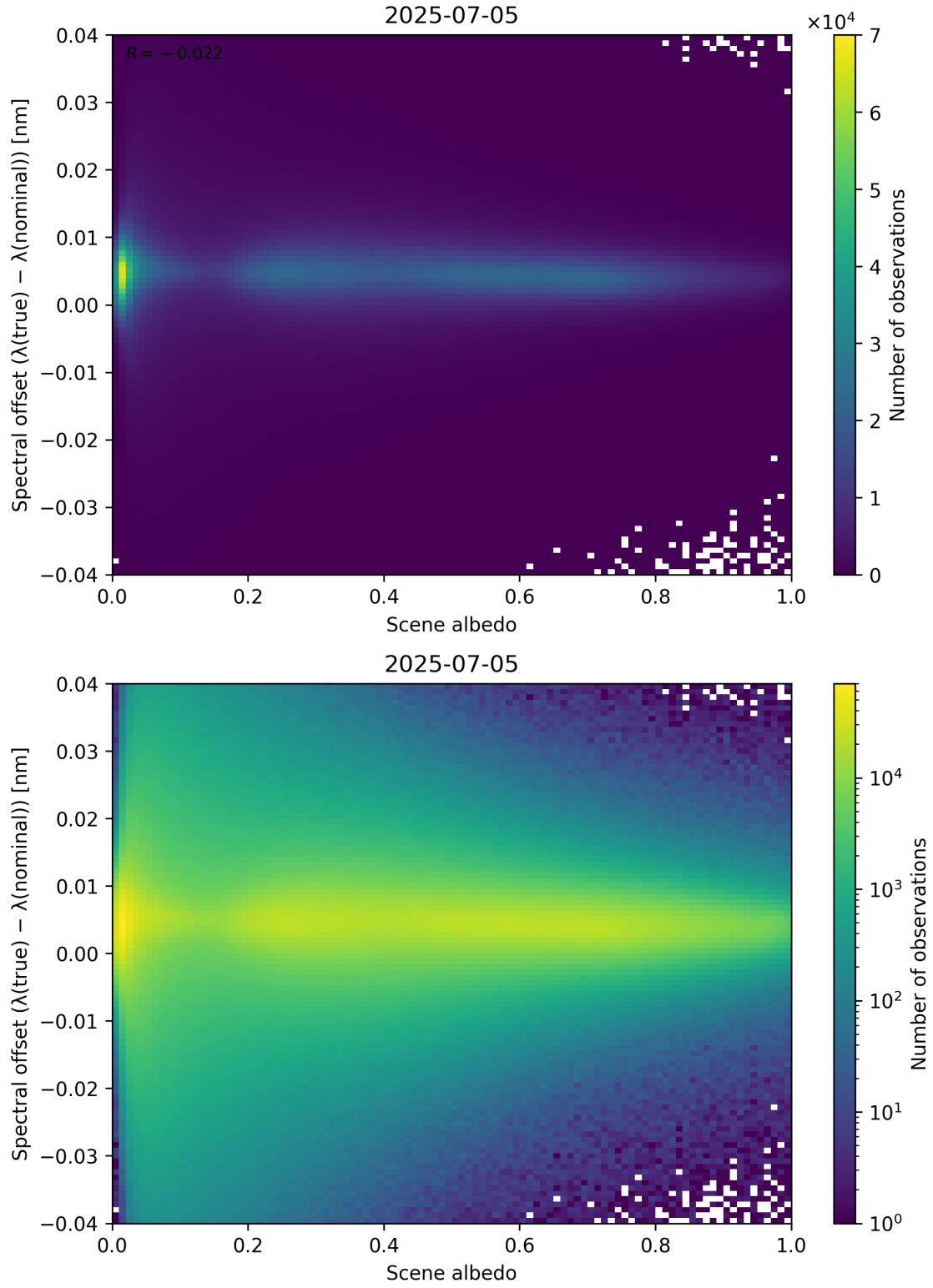
Figure 107: Scatter density plot of “Scene albedo” against “Spectral offset ( \lambda_{\text{true}} - \lambda_{\text{nominal}} )” for 2025-07-04 to 2025-07-06.
