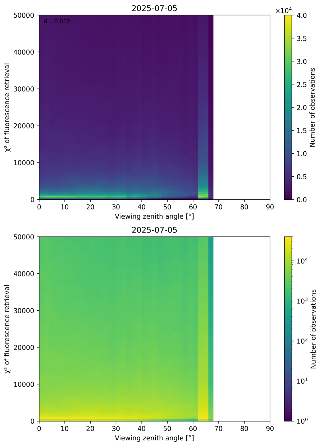
Figure 119: Scatter density plot of “Viewing zenith angle” against “ \chi^2 of fluorescence retrieval” for 2025-07-04 to 2025-07-06.
