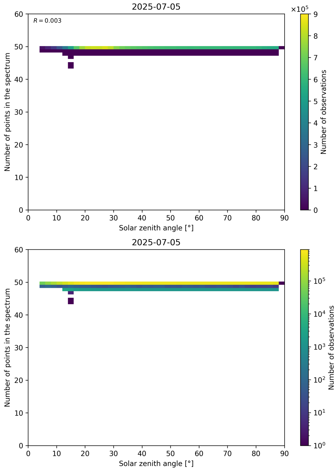
Figure 115: Scatter density plot of “Solar zenith angle” against “Number of points in the spectrum” for 2025-07-04 to 2025-07-06.
