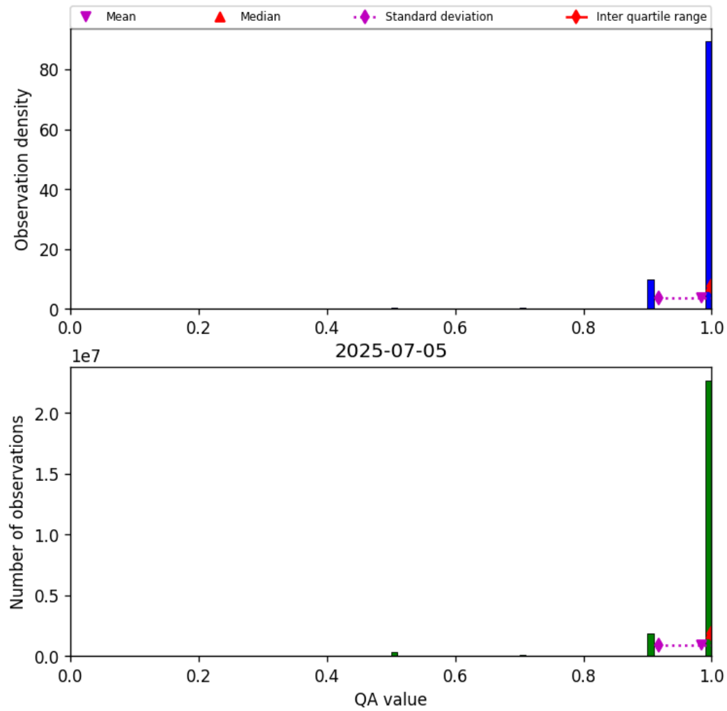
Figure 29: Histogram of “QA value” for 2025-07-04 to 2025-07-06
