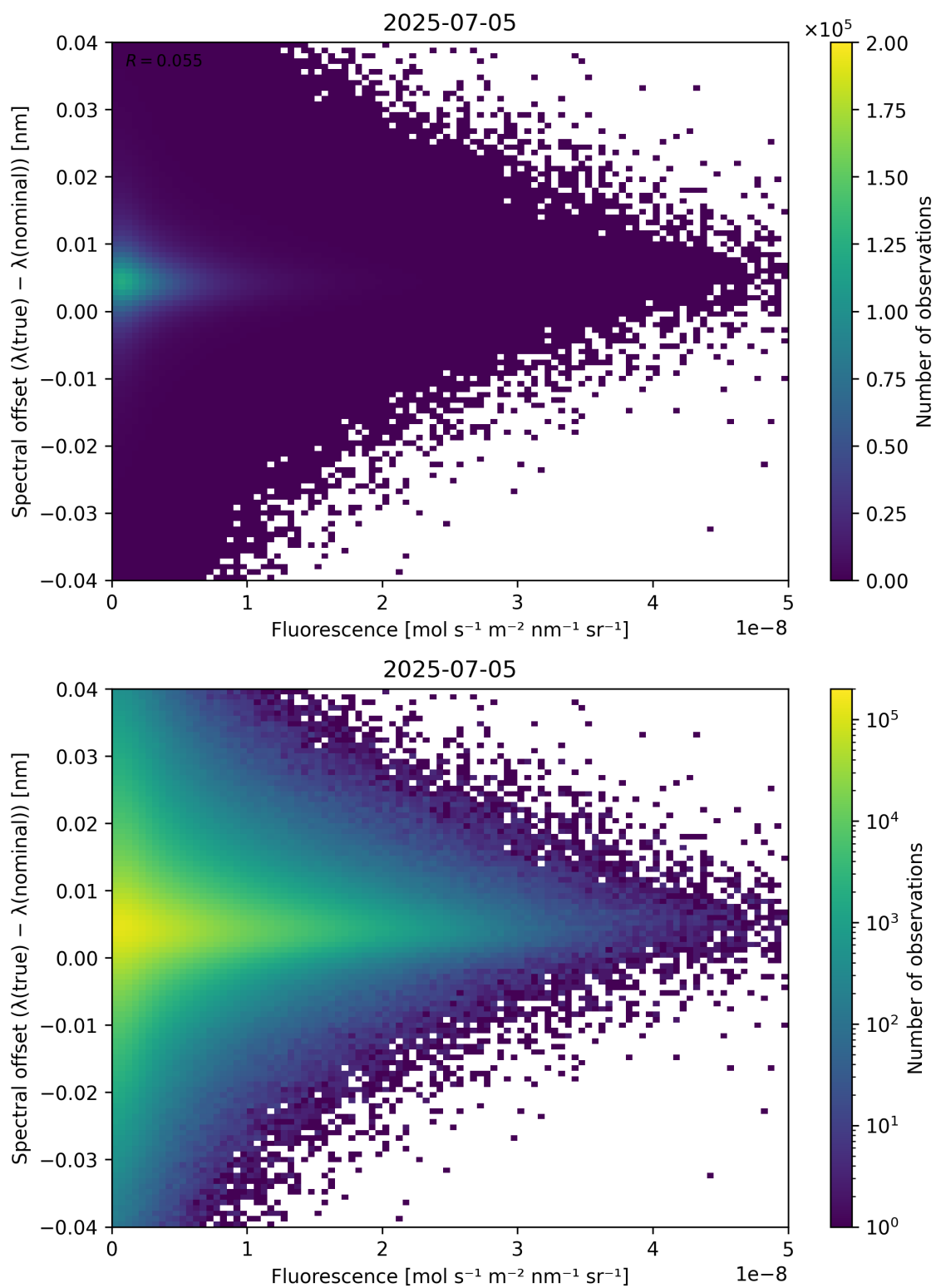
Figure 87: Scatter density plot of “Fluorescence” against “Spectral offset ( \lambda_{\text{true}} - \lambda_{\text{nominal}} )” for 2025-07-04 to 2025-07-06.
