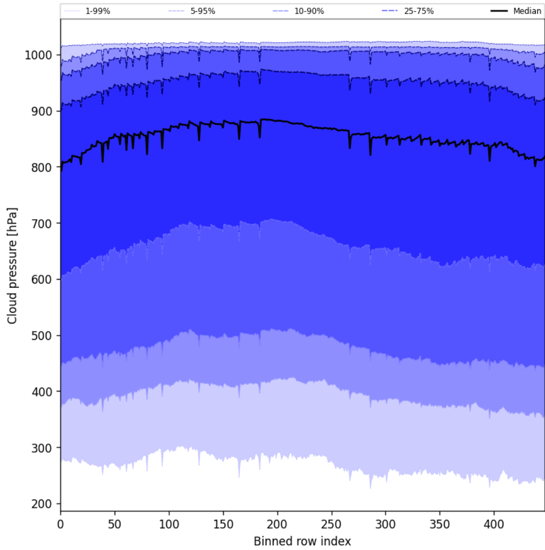
Figure 47: Along track statistics of “Cloud pressure” for 2025-07-04 to 2025-07-06
