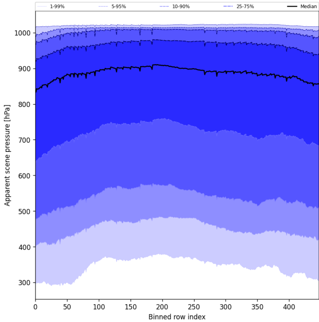
Figure 53: Along track statistics of “Apparent scene pressure” for 2025-07-04 to 2025-07-06
