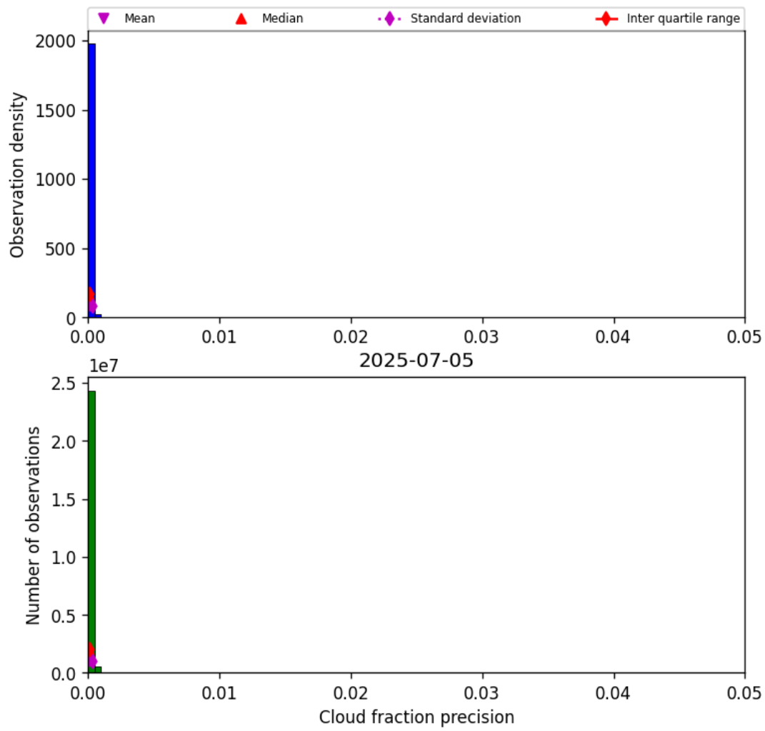
Figure 33: Histogram of “Cloud fraction precision” for 2025-07-04 to 2025-07-06
