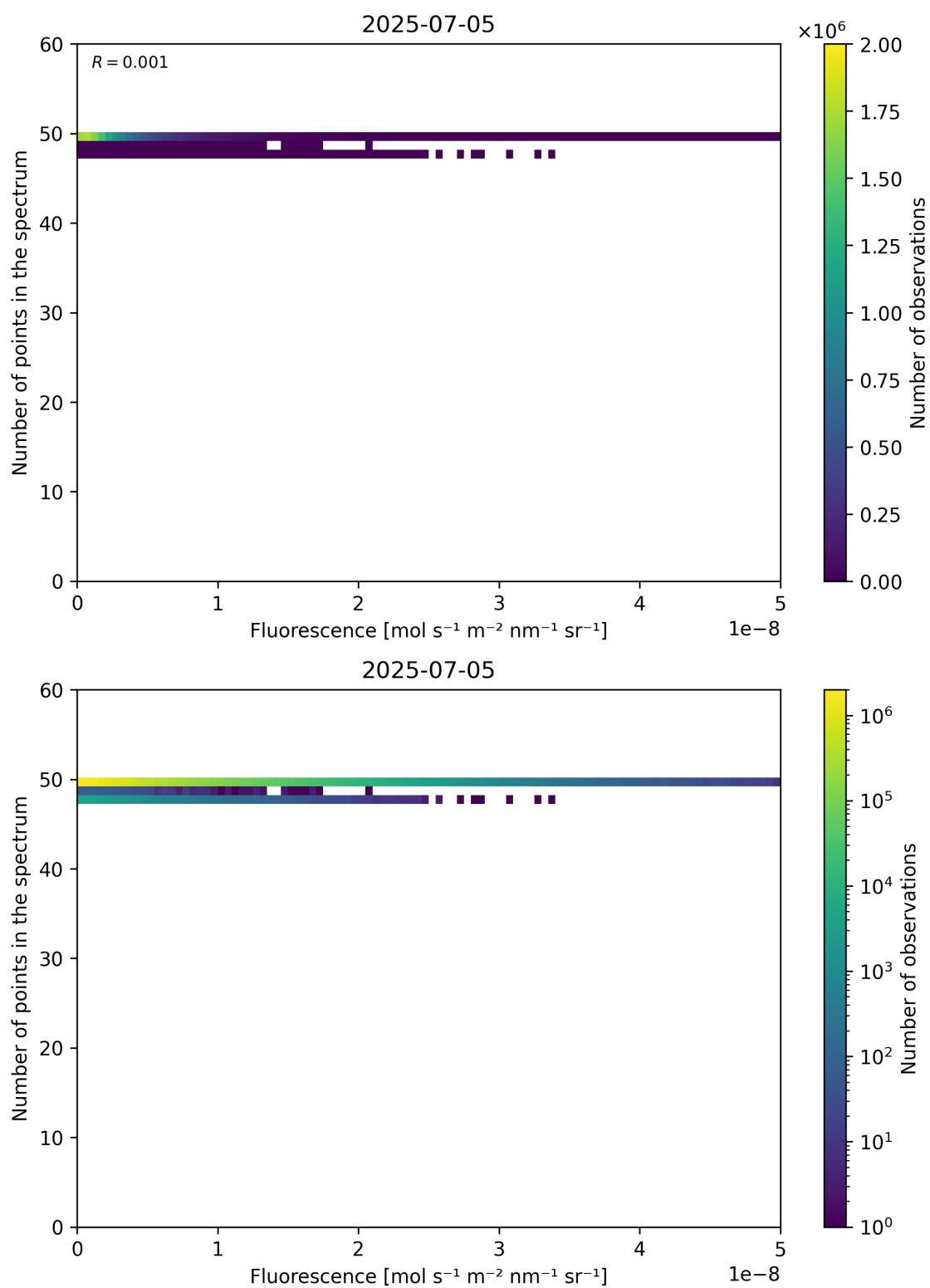
Figure 86: Scatter density plot of “Fluorescence” against “Number of points in the spectrum” for 2025-07-04 to 2025-07-06.
