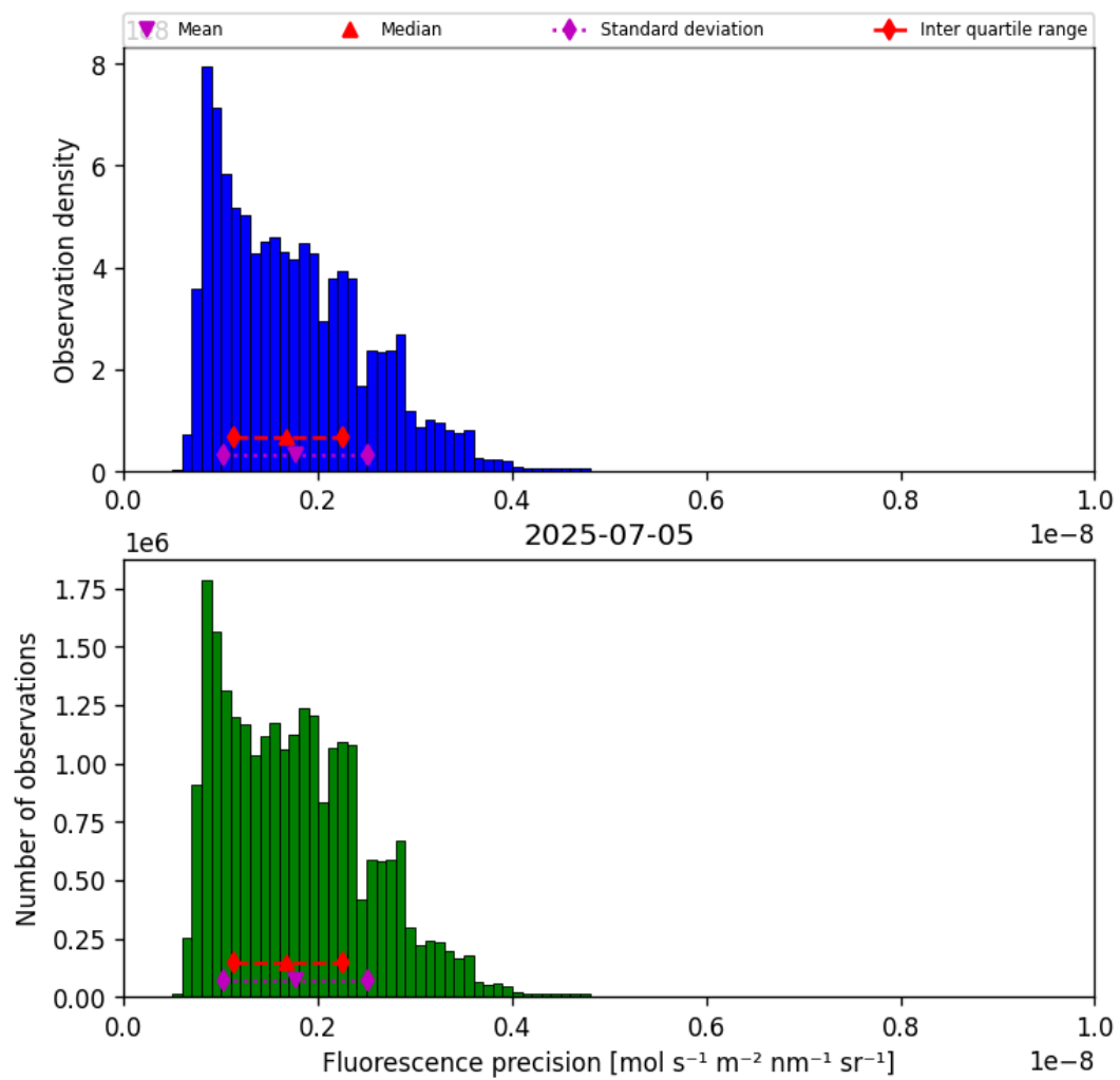
Figure 41: Histogram of “Fluorescence precision” for 2025-07-04 to 2025-07-06
