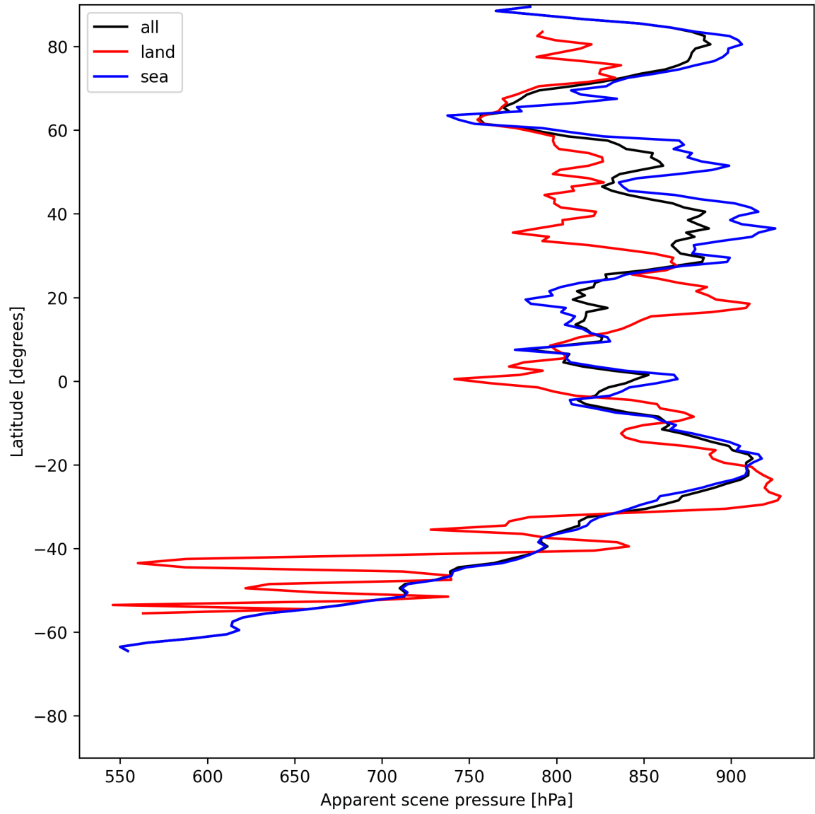
Figure 19: Zonal average of “Apparent scene pressure” for 2025-07-04 to 2025-07-06.
