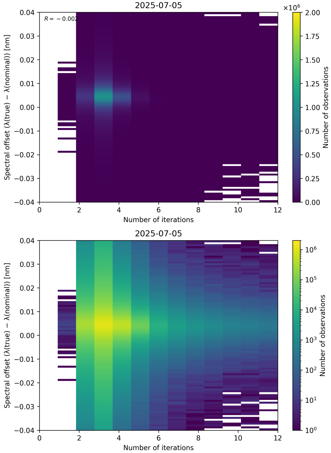
Figure 100: Scatter density plot of “Number of iterations” against “Spectral offset ( \lambda_{\text{true}} - \lambda_{\text{nominal}} )” for 2025-07-04 to 2025-07-06.
