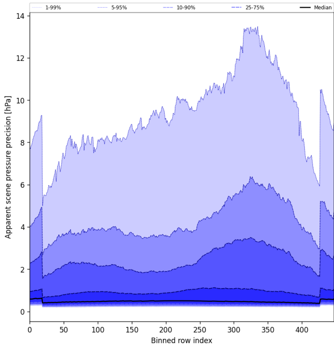
Figure 54: Along track statistics of “Apparent scene pressure precision” for 2025-07-04 to 2025-07-06
