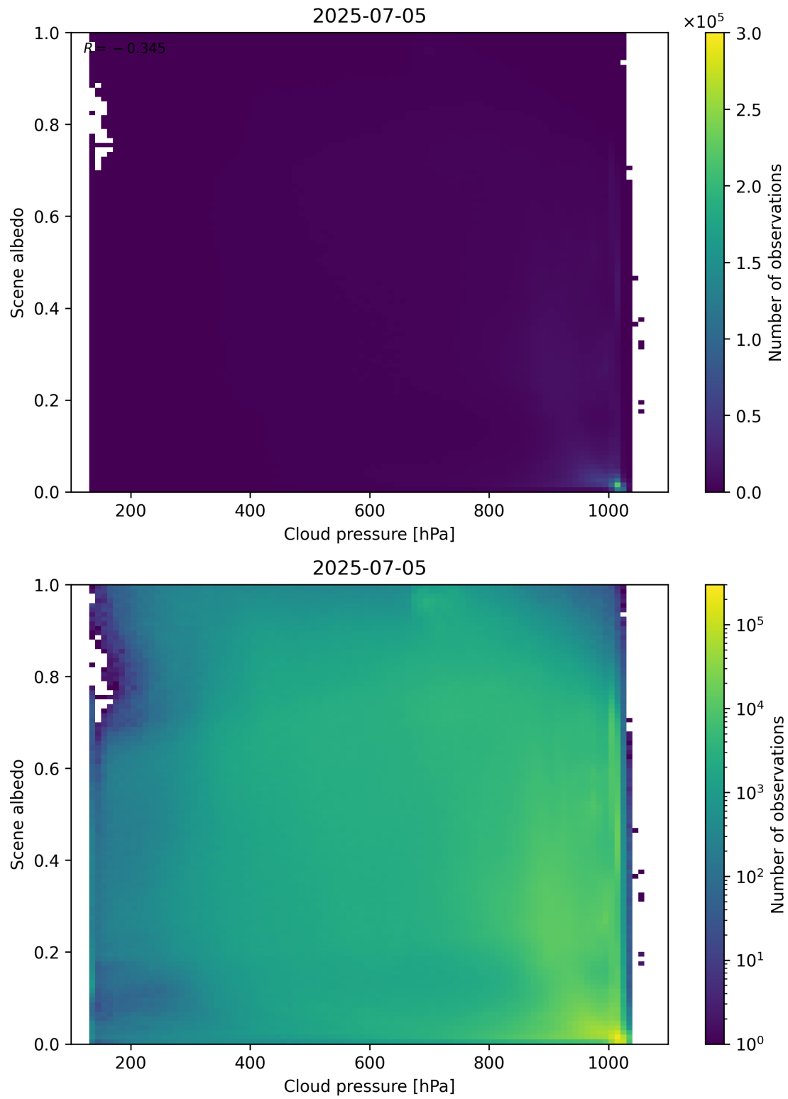
Figure 83: Scatter density plot of “Cloud pressure” against “Scene albedo” for 2025-07-04 to 2025-07-06.
