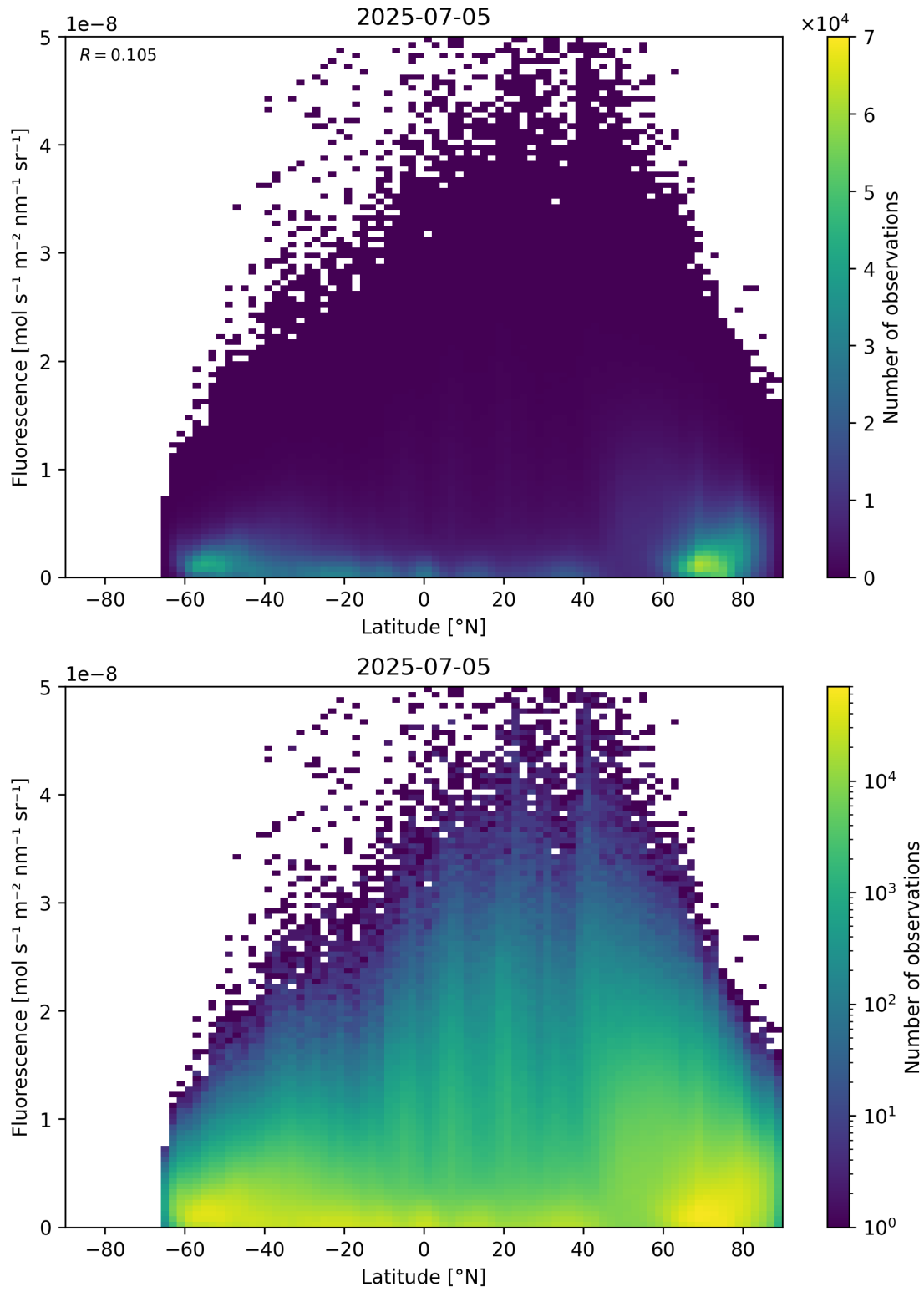
Figure 92: Scatter density plot of “Latitude” against “Fluorescence” for 2025-07-04 to 2025-07-06.
