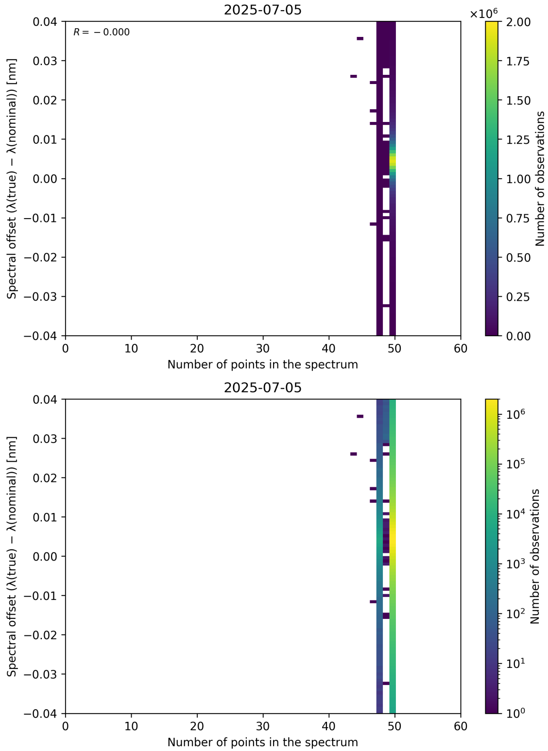
Figure 101: Scatter density plot of “Number of points in the spectrum” against “Spectral offset ( \lambda_{\text{true}} - \lambda_{\text{nominal}} )” for 2025-07-04 to 2025-07-06.
