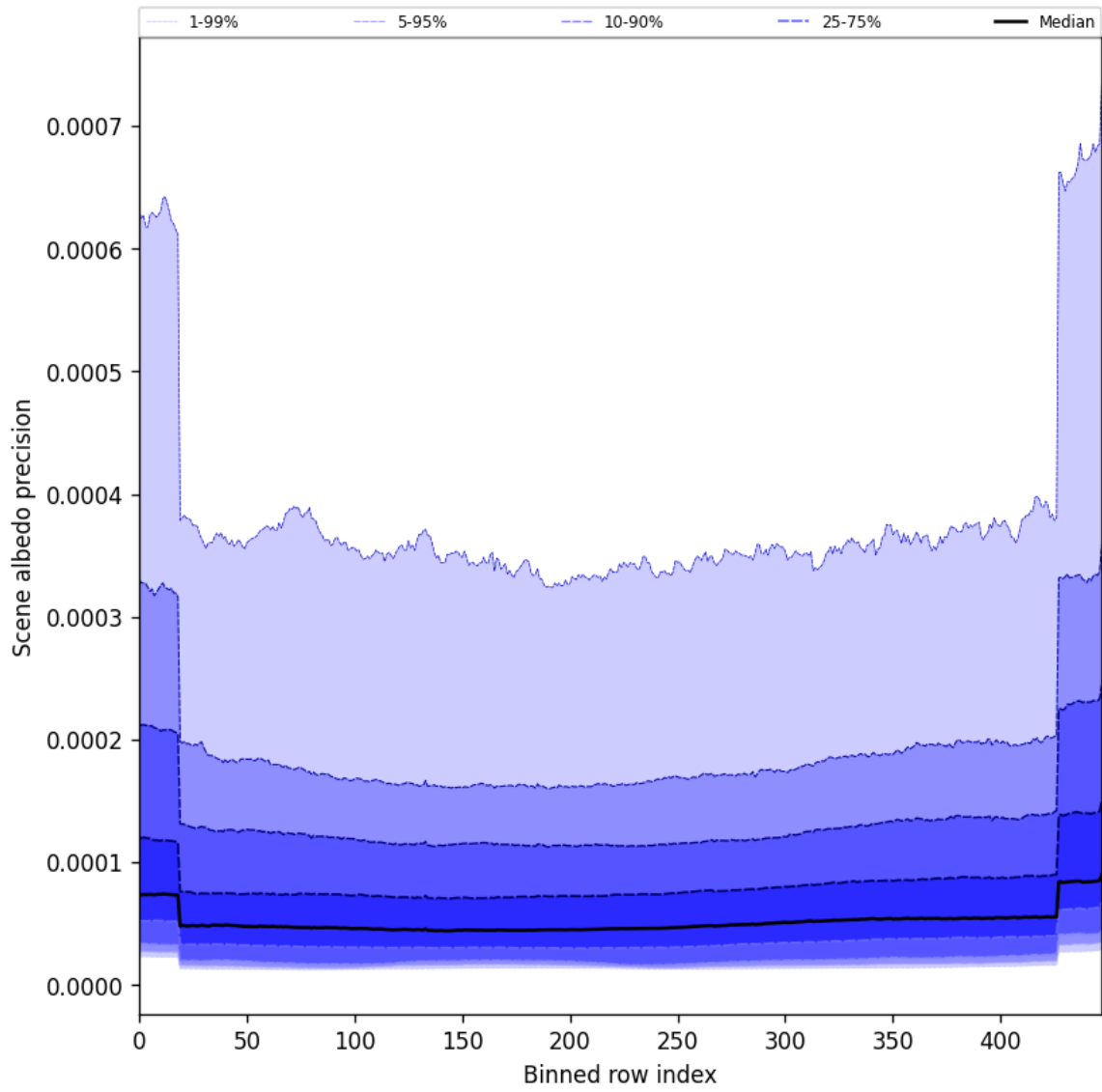
Figure 52: Along track statistics of “Scene albedo precision” for 2025-07-04 to 2025-07-06
