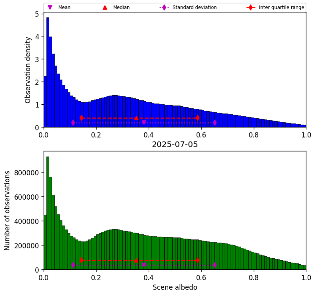
Figure 34: Histogram of “Scene albedo” for 2025-07-04 to 2025-07-06
