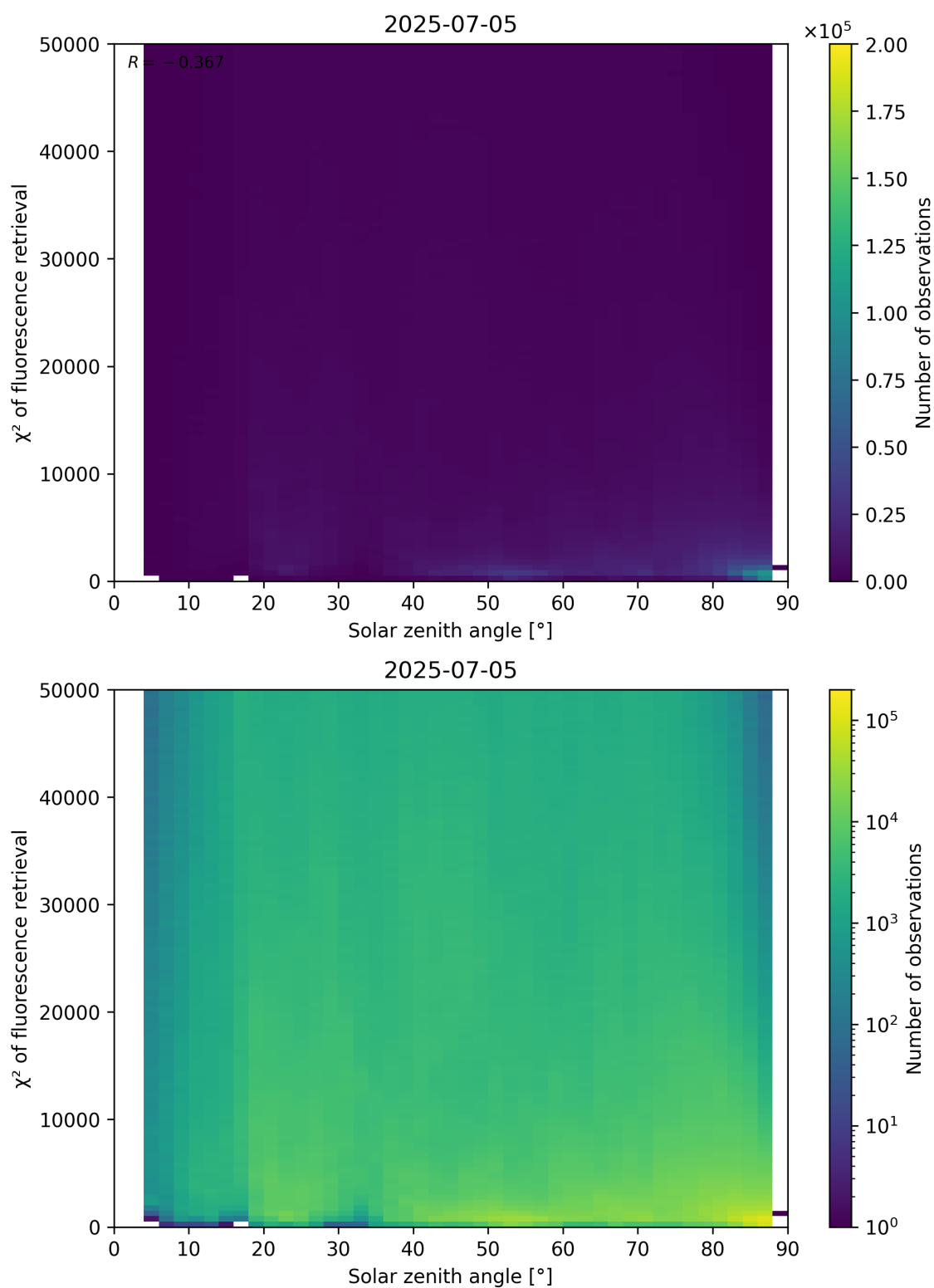
Figure 109: Scatter density plot of “Solar zenith angle” against “ \chi^2 of fluorescence retrieval” for 2025-07-04 to 2025-07-06.
