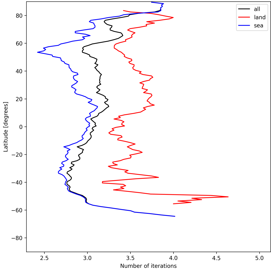
Figure 22: Zonal average of “Number of iterations” for 2025-07-04 to 2025-07-06.
