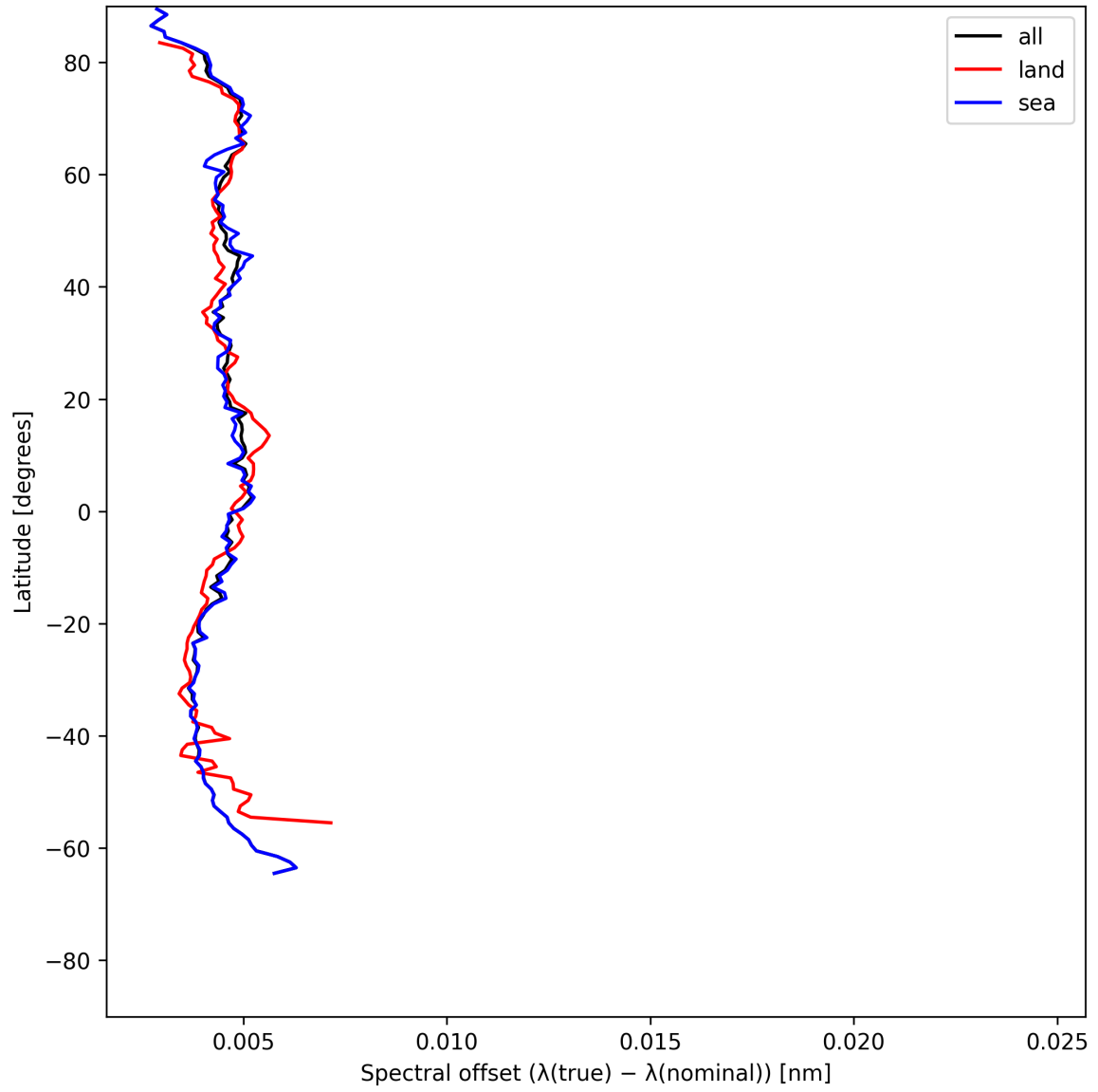
Figure 28: Zonal average of “Spectral offset ( \lambda_{\text{true}} - \lambda_{\text{nominal}} )” for 2025-07-04 to 2025-07-06.
