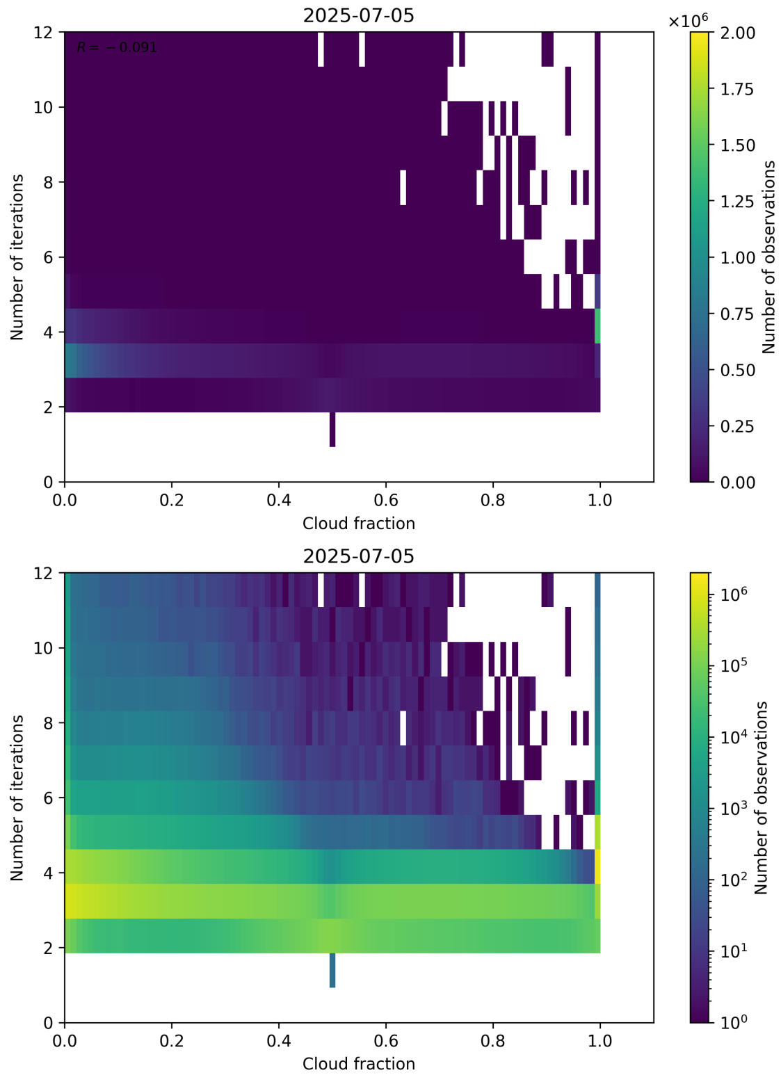
Figure 73: Scatter density plot of “Cloud fraction” against “Number of iterations” for 2025-07-04 to 2025-07-06.
