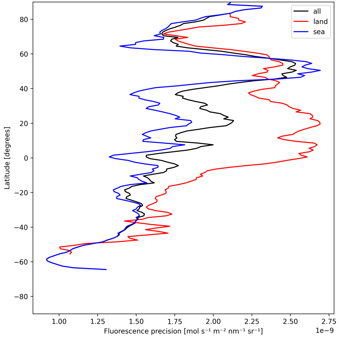
Figure 24: Zonal average of “Fluorescence precision” for 2025-07-04 to 2025-07-06.
