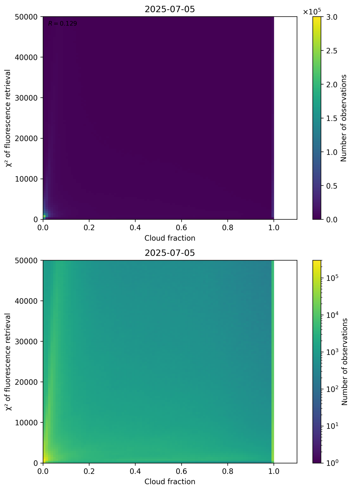
Figure 71: Scatter density plot of “Cloud fraction” against “ \chi^2 of fluorescence retrieval” for 2025-07-04 to 2025-07-06.
