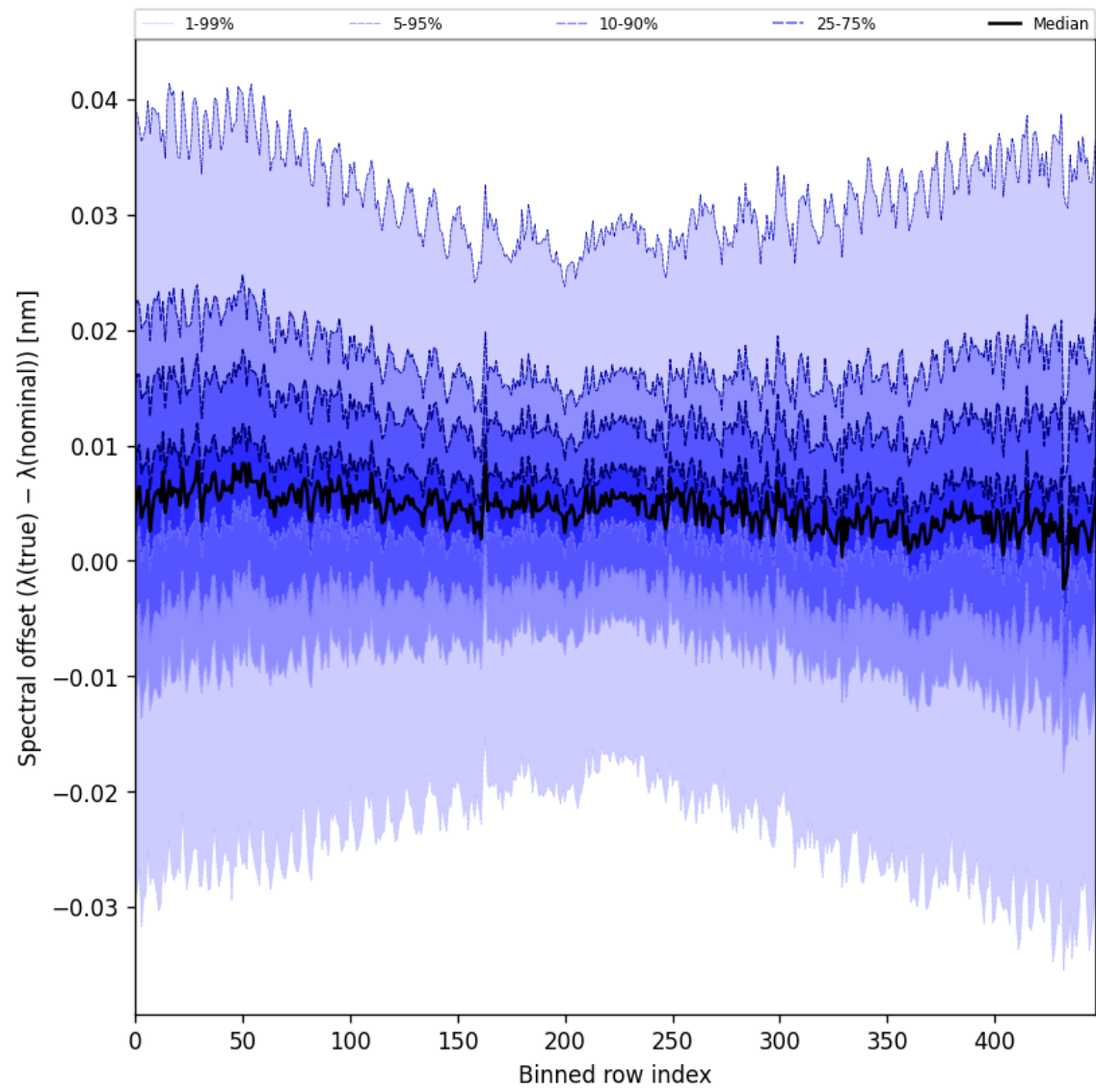
Figure 62: Along track statistics of “Spectral offset ( \lambda_{\text{true}} - \lambda_{\text{nominal}} )” for 2025-07-04 to 2025-07-06
