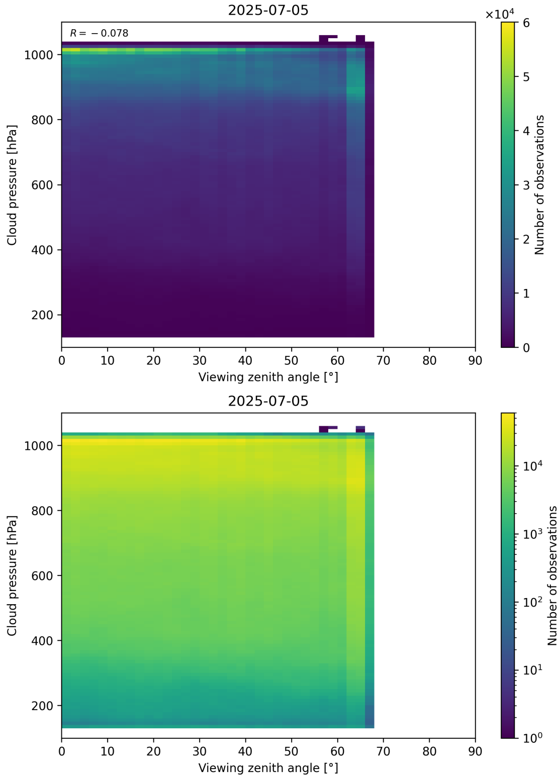
Figure 121: Scatter density plot of “Viewing zenith angle” against “Cloud pressure” for 2025-07-04 to 2025-07-06.
