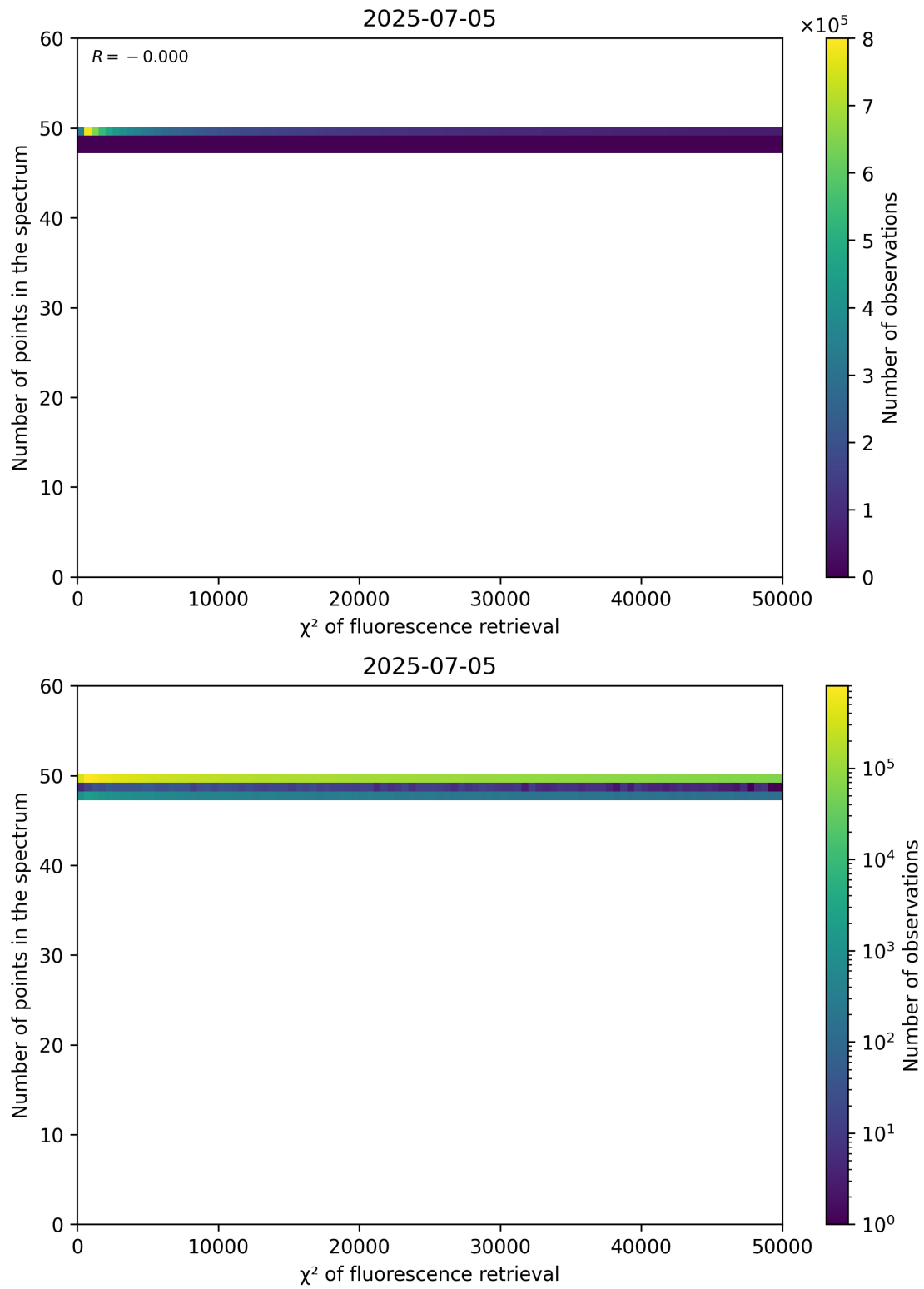
Figure 68: Scatter density plot of “ \chi^2 of fluorescence retrieval” against “Number of points in the spectrum” for 2025-07-04 to 2025-07-06.
