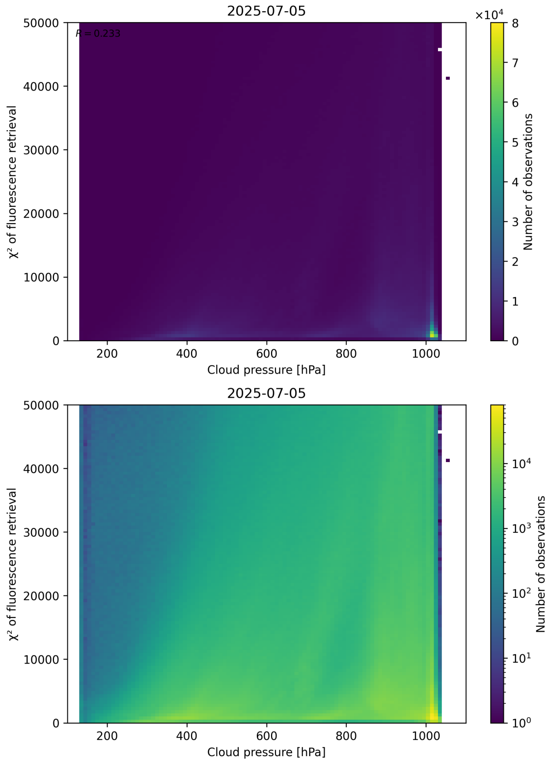
Figure 78: Scatter density plot of “Cloud pressure” against “ \chi^2 of fluorescence retrieval” for 2025-07-04 to 2025-07-06.
