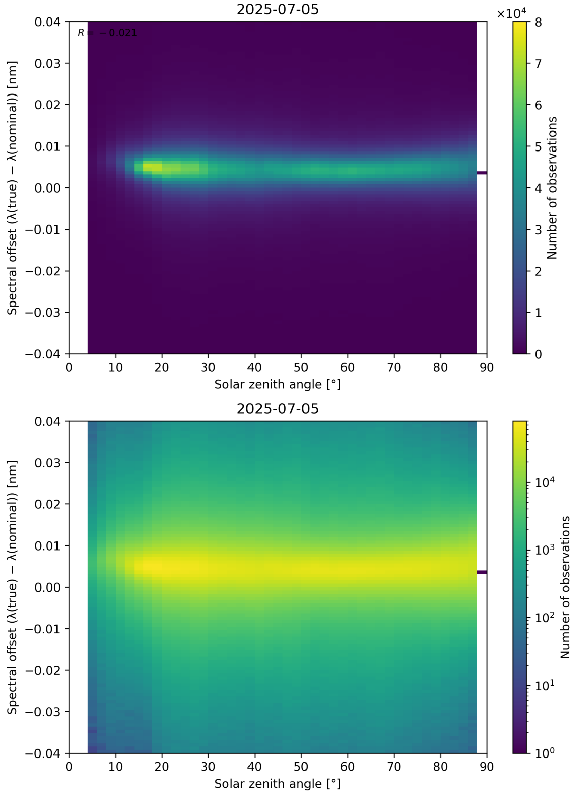
Figure 117: Scatter density plot of “Solar zenith angle” against “Spectral offset ( \lambda_{\text{true}} - \lambda_{\text{nominal}} )” for 2025-07-04 to 2025-07-06.
