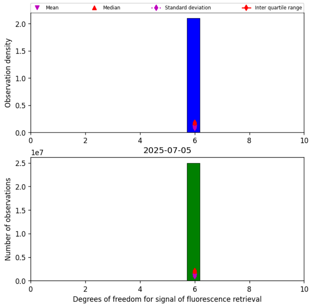
Figure 43: Histogram of “Degrees of freedom for signal of fluorescence retrieval” for 2025-07-04 to 2025-07-06
