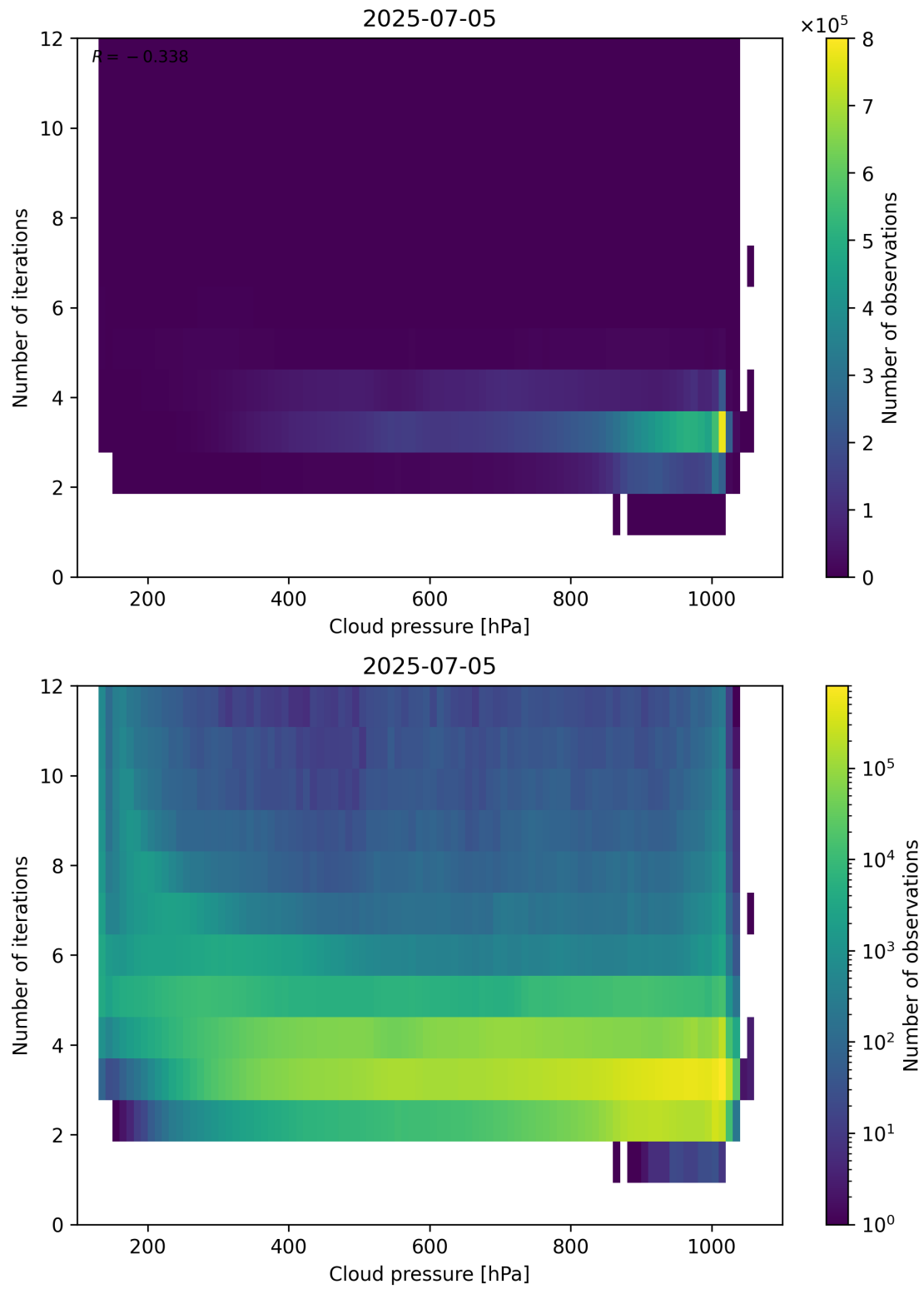
Figure 81: Scatter density plot of “Cloud pressure” against “Number of iterations” for 2025-07-04 to 2025-07-06.
