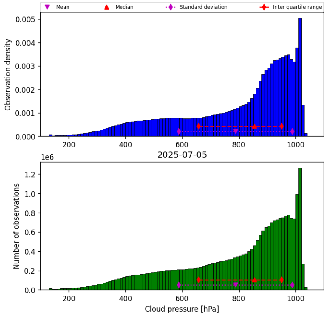
Figure 30: Histogram of “Cloud pressure” for 2025-07-04 to 2025-07-06
