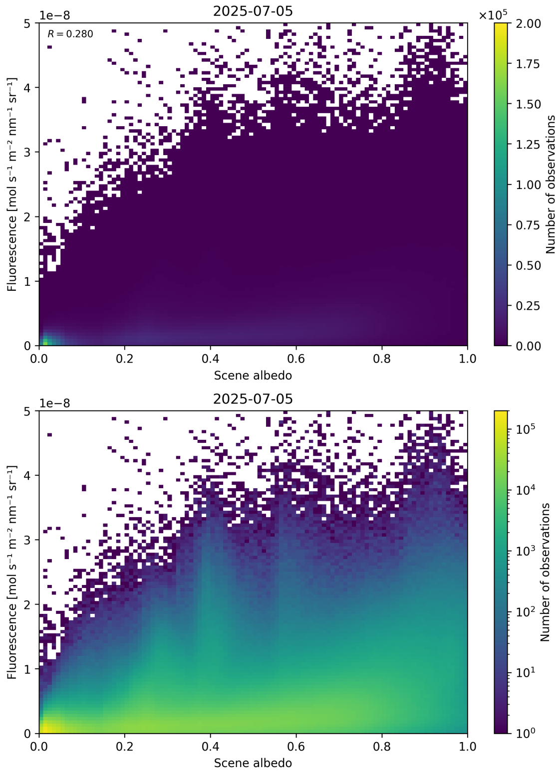
Figure 104: Scatter density plot of “Scene albedo” against “Fluorescence” for 2025-07-04 to 2025-07-06.
