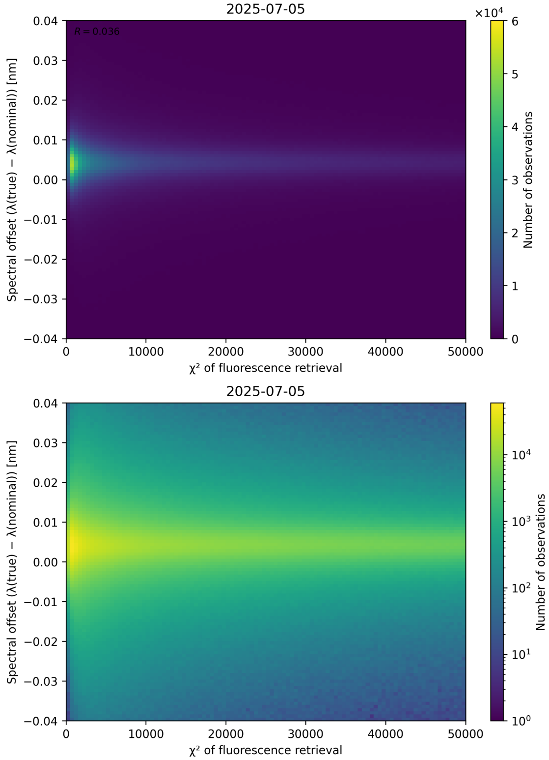
Figure 69: Scatter density plot of “ \chi^2 of fluorescence retrieval” against “Spectral offset ( \lambda_{\text{true}} - \lambda_{\text{nominal}} )” for 2025-07-04 to 2025-07-06.
