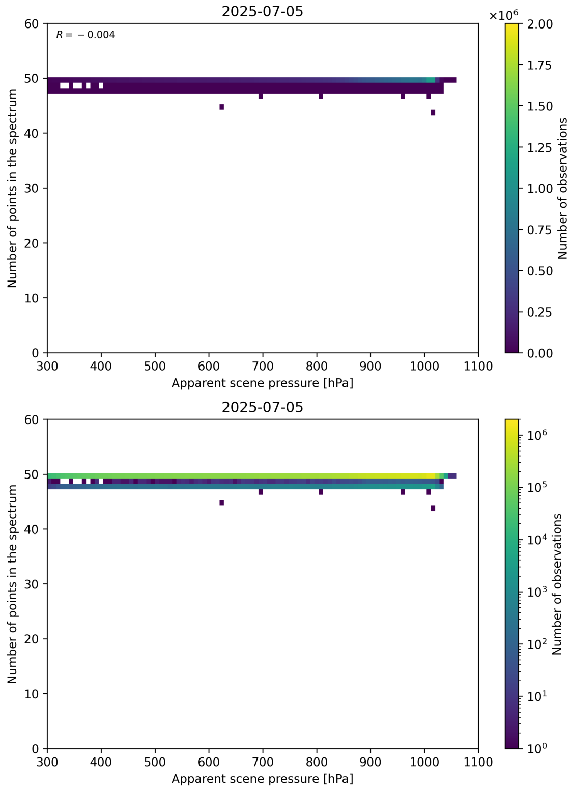
Figure 66: Scatter density plot of “Apparent scene pressure” against “Number of points in the spectrum” for 2025-07-04 to 2025-07-06.
