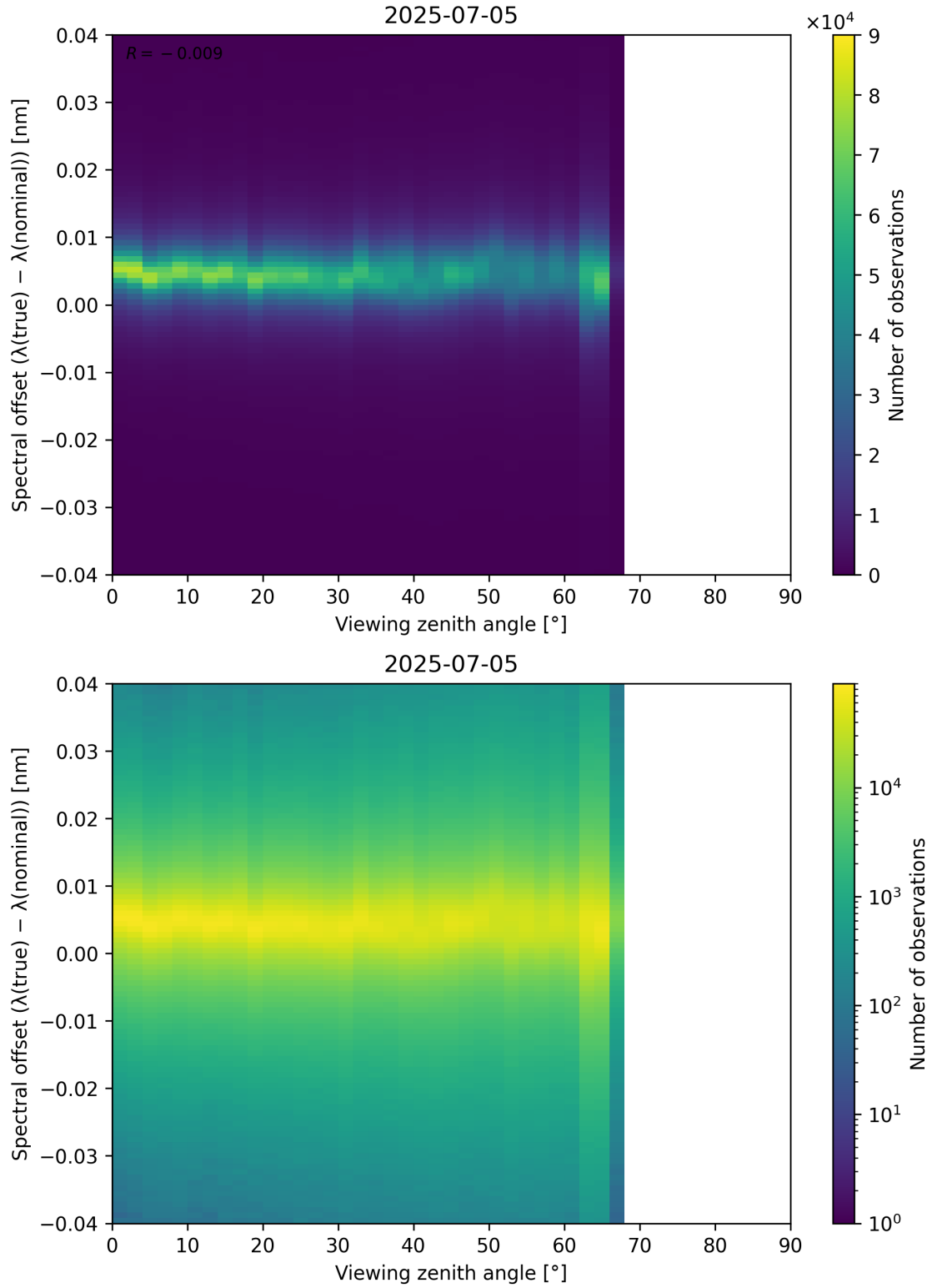
Figure 128: Scatter density plot of “Viewing zenith angle” against “Spectral offset ( \lambda_{\text{true}} - \lambda_{\text{nominal}} )” for 2025-07-04 to 2025-07-06.
