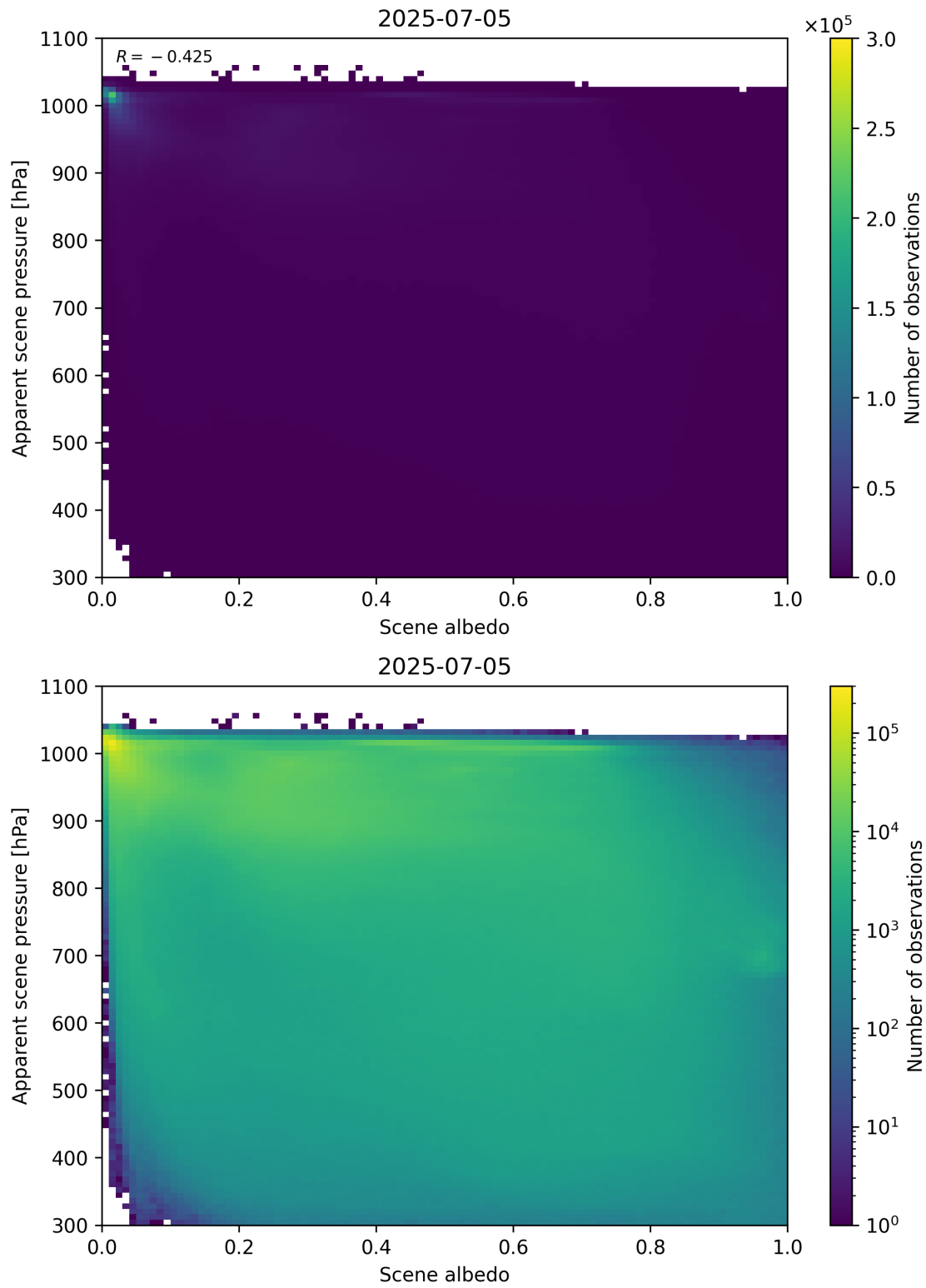
Figure 102: Scatter density plot of “Scene albedo” against “Apparent scene pressure” for 2025-07-04 to 2025-07-06.
