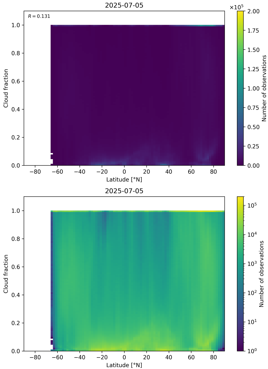
Figure 90: Scatter density plot of “Latitude” against “Cloud fraction” for 2025-07-04 to 2025-07-06.
