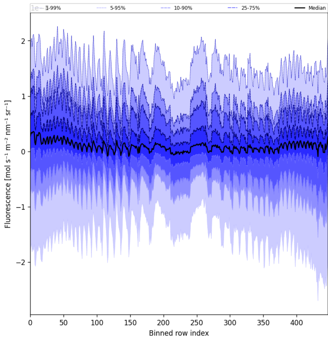
Figure 57: Along track statistics of “Fluorescence” for 2025-07-04 to 2025-07-06
