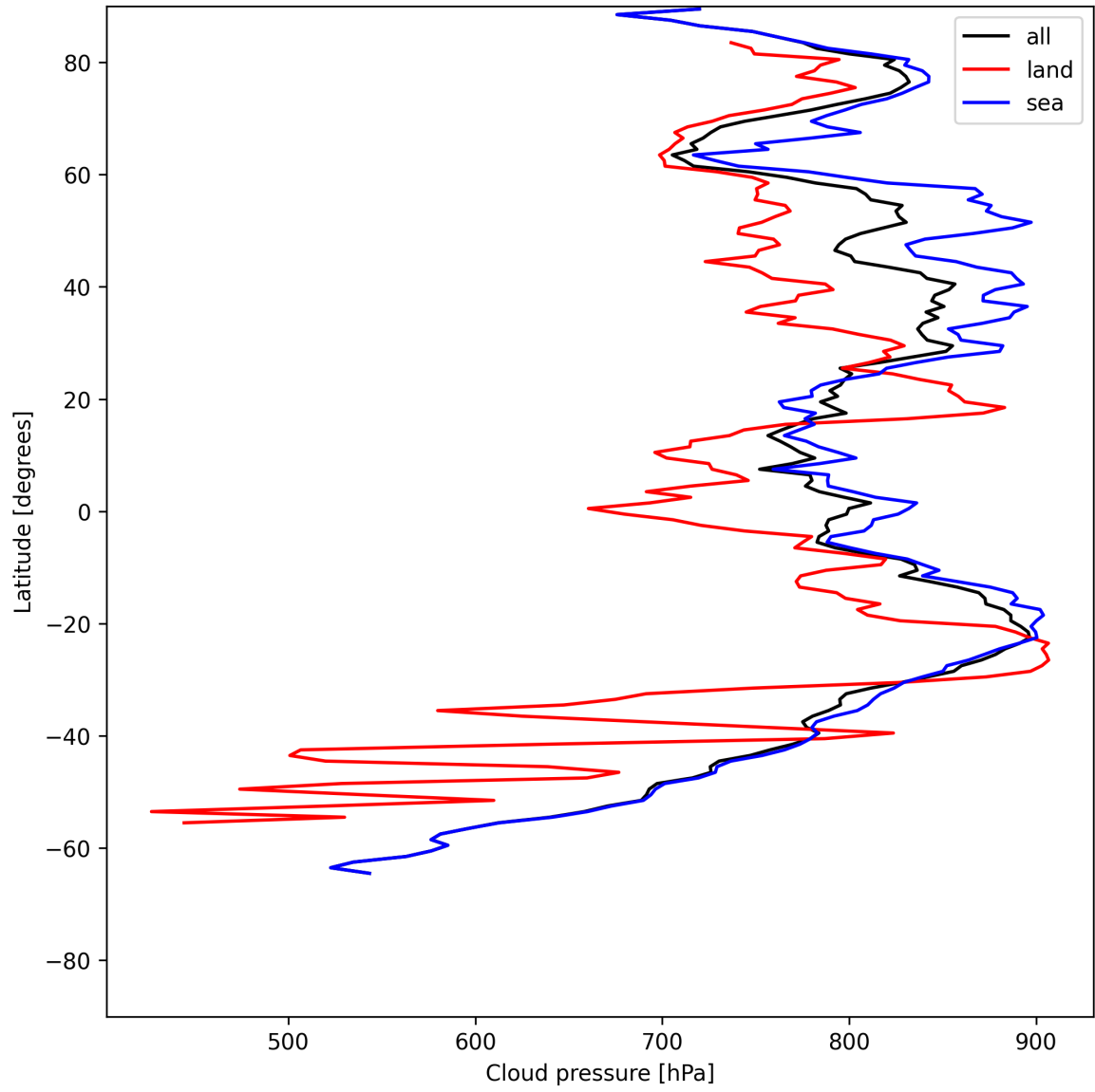
Figure 13: Zonal average of “Cloud pressure” for 2025-07-04 to 2025-07-06.
