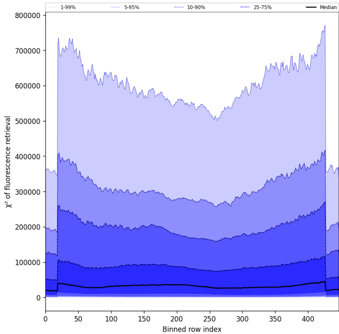
Figure 59: Along track statistics of “ \chi^2 of fluorescence retrieval” for 2025-07-04 to 2025-07-06
