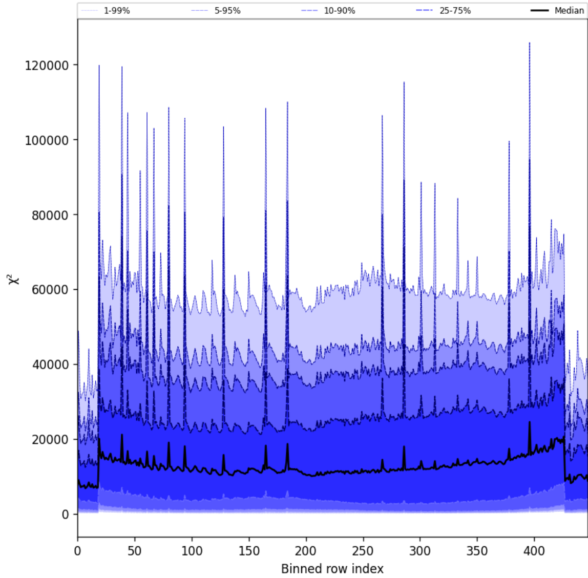
Figure 55: Along track statistics of “ \chi^2 ” for 2025-07-04 to 2025-07-06
