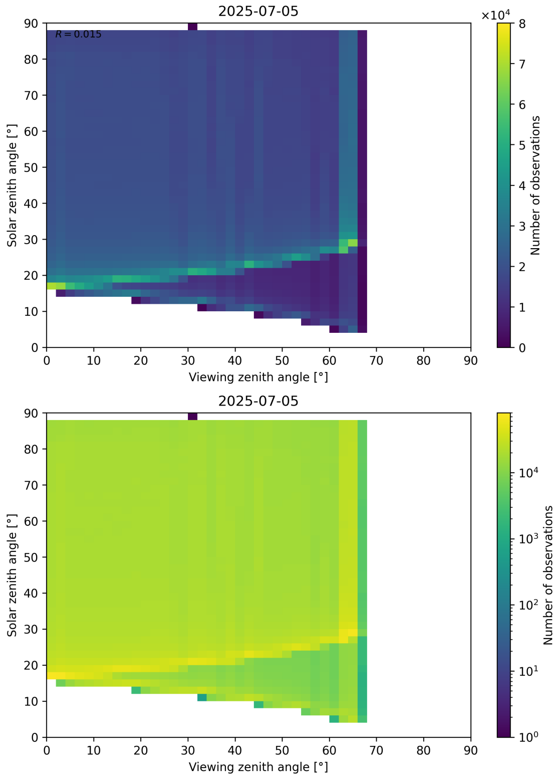
Figure 127: Scatter density plot of “Viewing zenith angle” against “Solar zenith angle” for 2025-07-04 to 2025-07-06.
