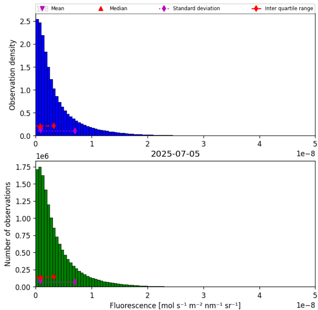
Figure 40: Histogram of “Fluorescence” for 2025-07-04 to 2025-07-06
