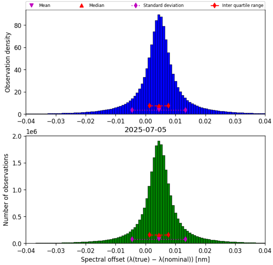
Figure 45: Histogram of “Spectral offset ( \lambda_{\text{true}} - \lambda_{\text{nominal}} )” for 2025-07-04 to 2025-07-06
