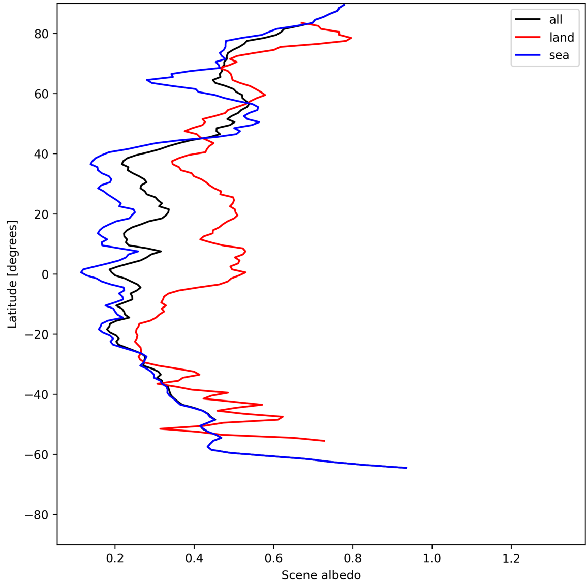
Figure 17: Zonal average of “Scene albedo” for 2025-07-04 to 2025-07-06.
