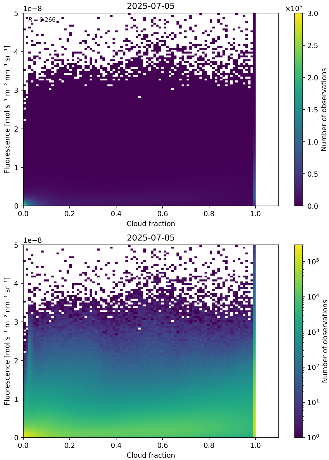
Figure 72: Scatter density plot of “Cloud fraction” against “Fluorescence” for 2025-07-04 to 2025-07-06.
