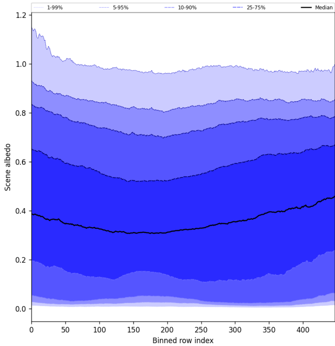
Figure 51: Along track statistics of “Scene albedo” for 2025-07-04 to 2025-07-06
