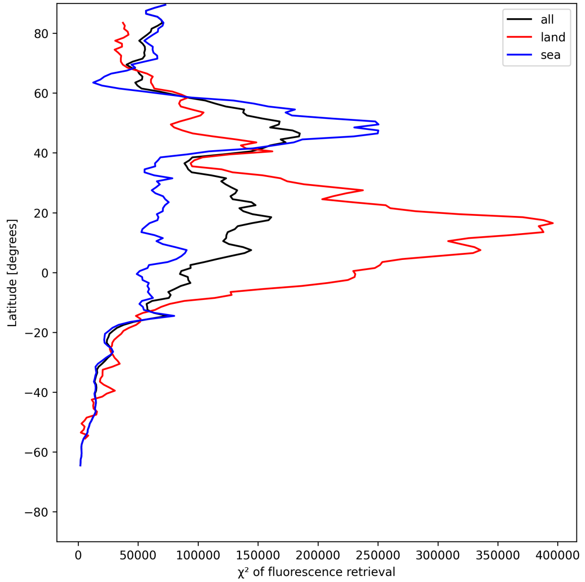
Figure 25: Zonal average of “ \chi^2 of fluorescence retrieval” for 2025-07-04 to 2025-07-06.
