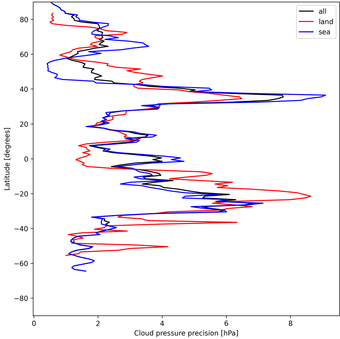
Figure 14: Zonal average of “Cloud pressure precision” for 2025-07-04 to 2025-07-06.
