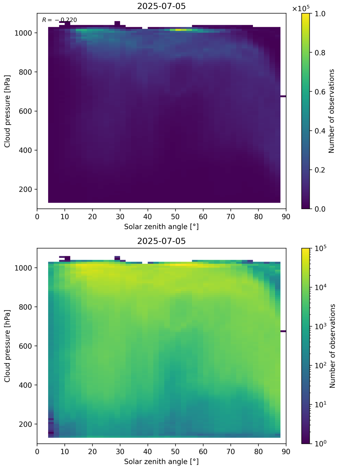
Figure 111: Scatter density plot of “Solar zenith angle” against “Cloud pressure” for 2025-07-04 to 2025-07-06.
