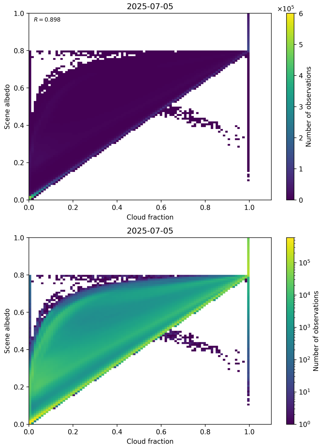
Figure 75: Scatter density plot of “Cloud fraction” against “Scene albedo” for 2025-07-04 to 2025-07-06.
