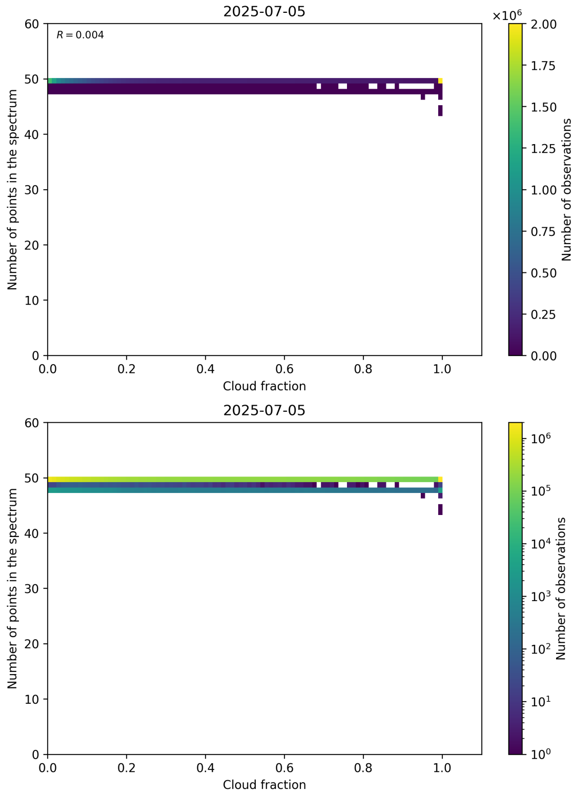
Figure 74: Scatter density plot of “Cloud fraction” against “Number of points in the spectrum” for 2025-07-04 to 2025-07-06.
