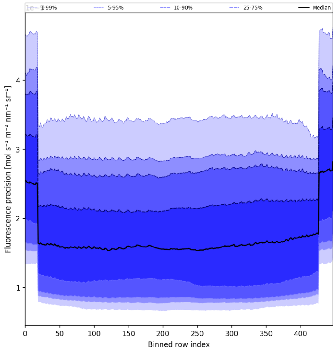
Figure 58: Along track statistics of “Fluorescence precision” for 2025-07-04 to 2025-07-06
