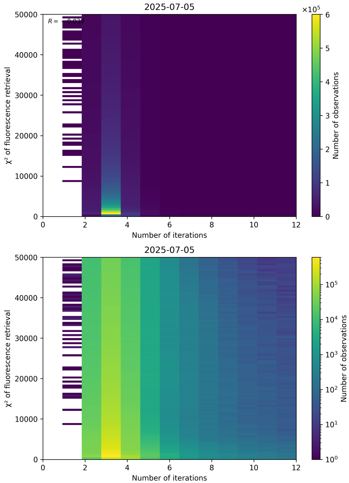
Figure 97: Scatter density plot of “Number of iterations” against “ \chi^2 of fluorescence retrieval” for 2025-07-04 to 2025-07-06.
