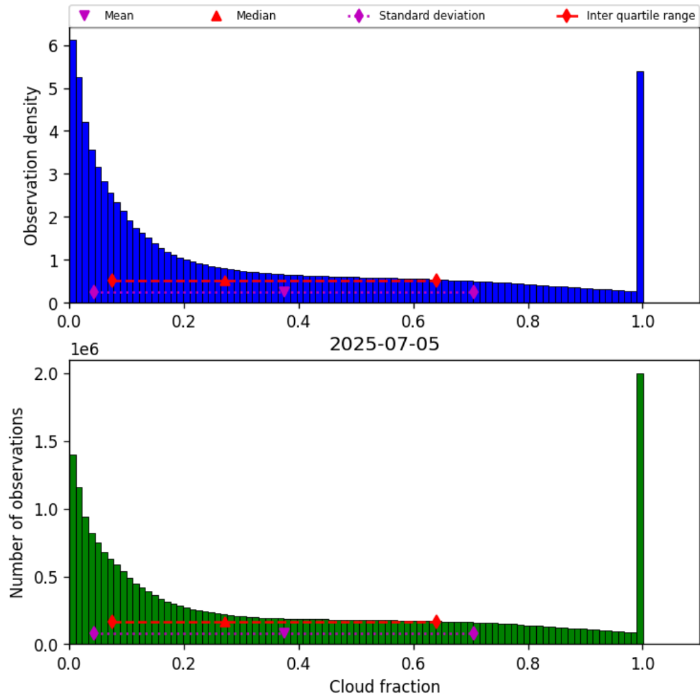
Figure 32: Histogram of “Cloud fraction” for 2025-07-04 to 2025-07-06
