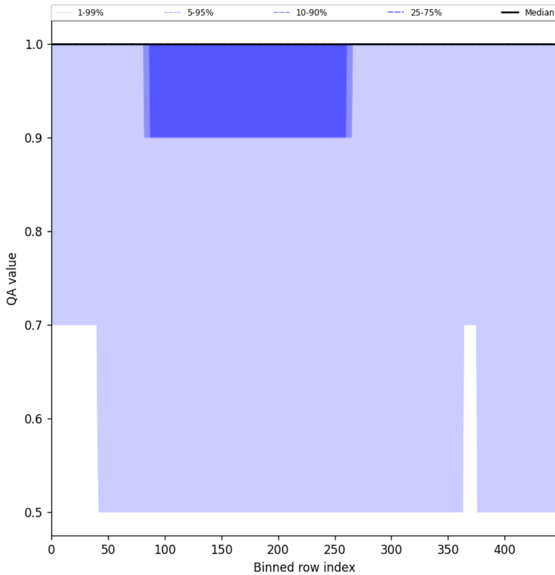
Figure 46: Along track statistics of “QA value” for 2025-07-04 to 2025-07-06
