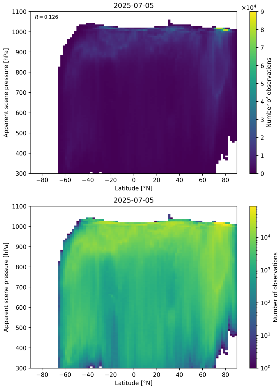
Figure 88: Scatter density plot of “Latitude” against “Apparent scene pressure” for 2025-07-04 to 2025-07-06.
