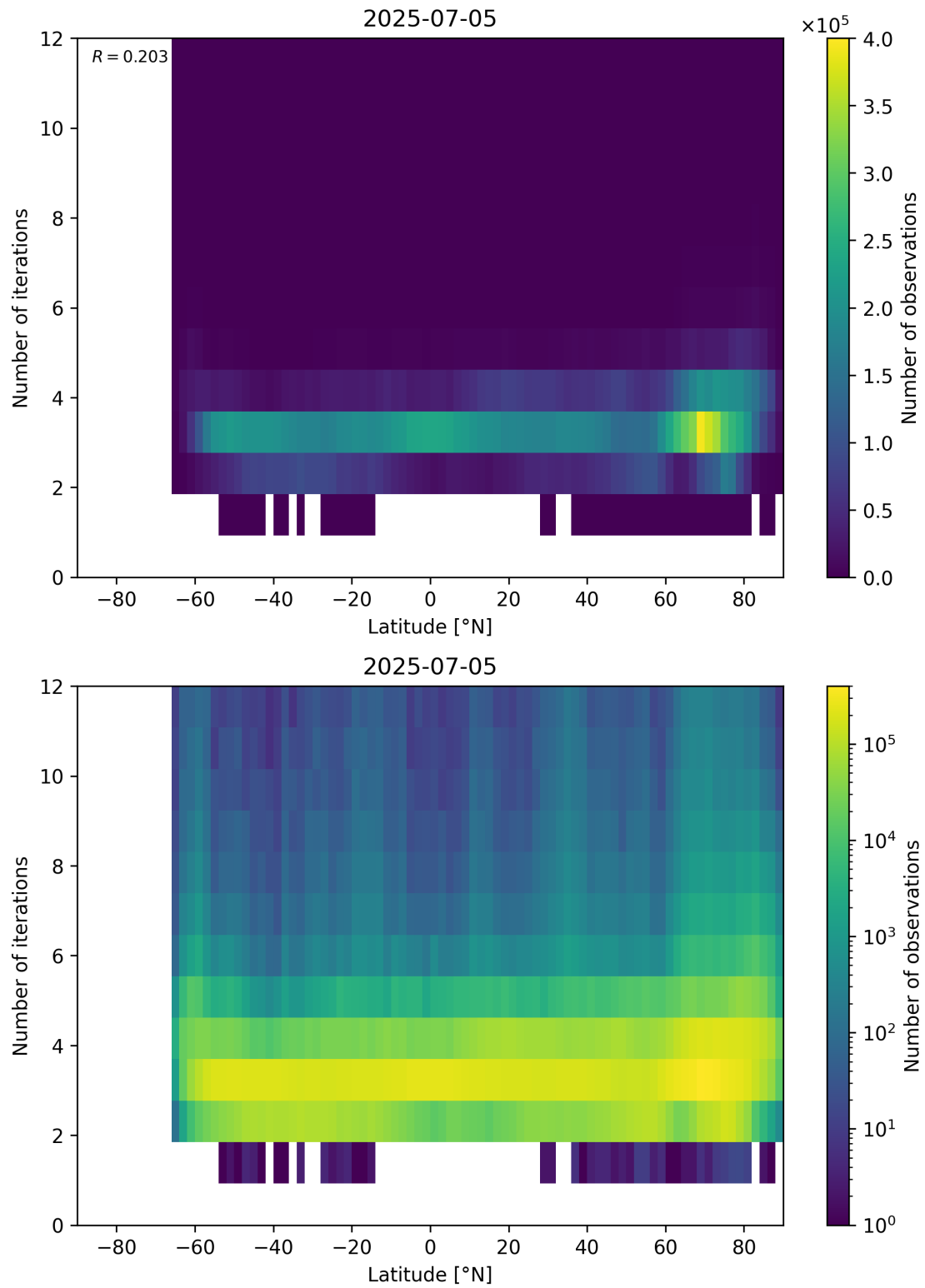
Figure 93: Scatter density plot of “Latitude” against “Number of iterations” for 2025-07-04 to 2025-07-06.
