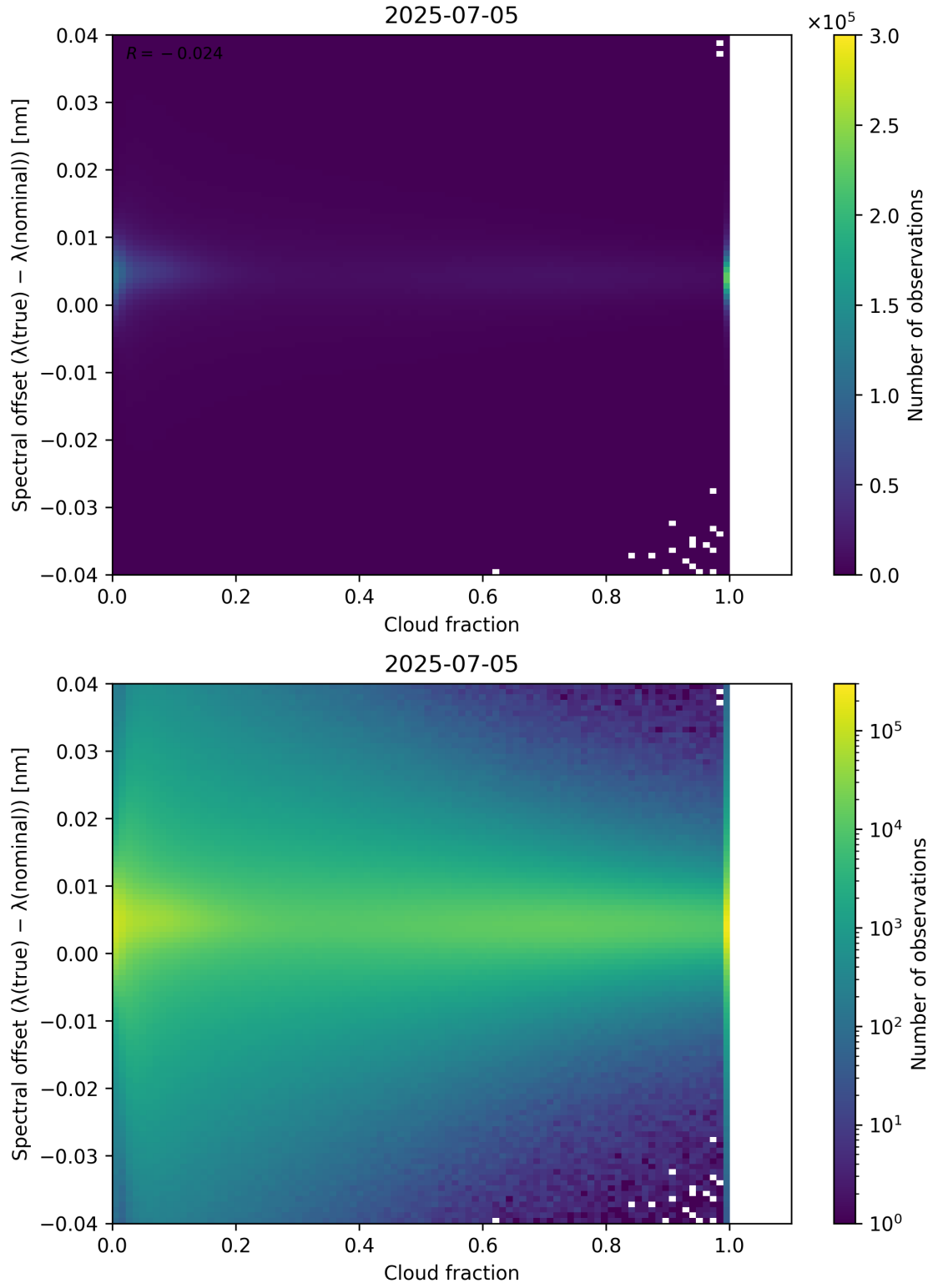
Figure 76: Scatter density plot of “Cloud fraction” against “Spectral offset ( \lambda_{\text{true}} - \lambda_{\text{nominal}} )” for 2025-07-04 to 2025-07-06.
