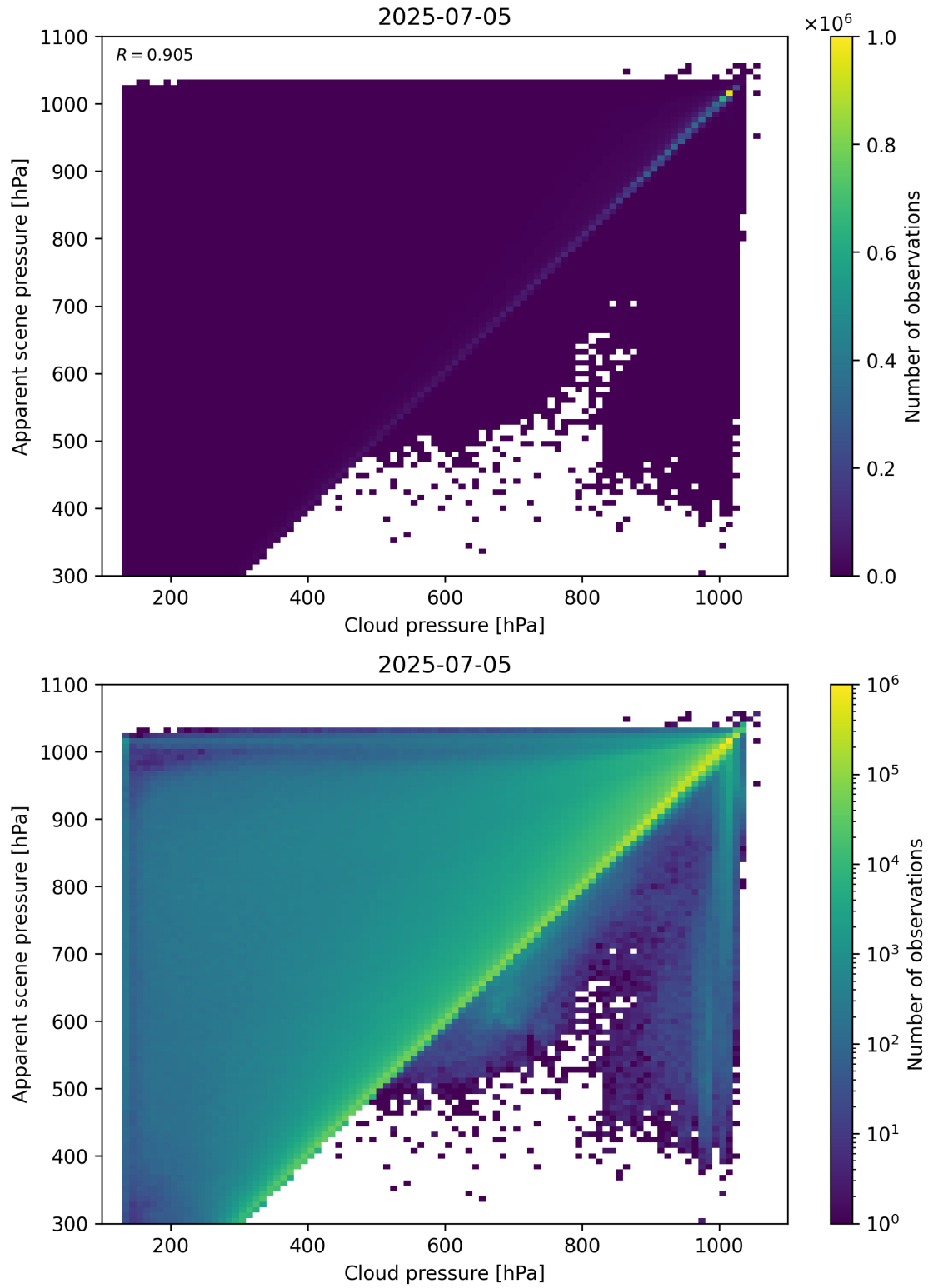
Figure 77: Scatter density plot of “Cloud pressure” against “Apparent scene pressure” for 2025-07-04 to 2025-07-06.
