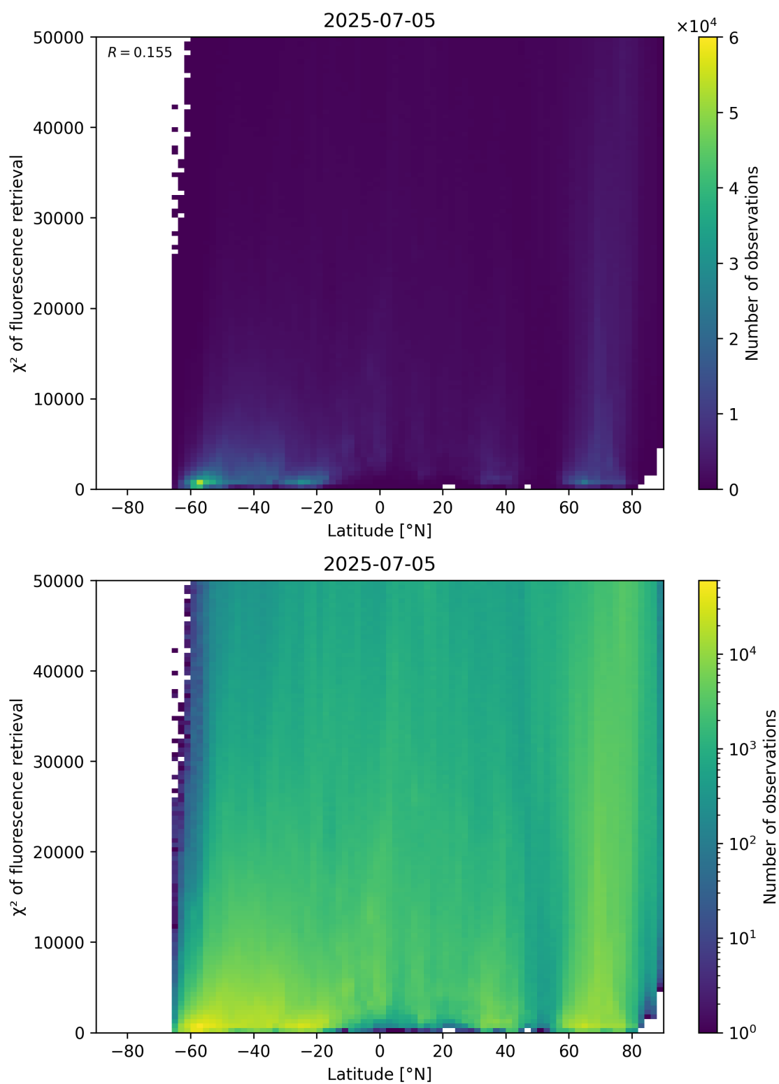
Figure 89: Scatter density plot of “Latitude” against “ \chi^2 of fluorescence retrieval” for 2025-07-04 to 2025-07-06.
