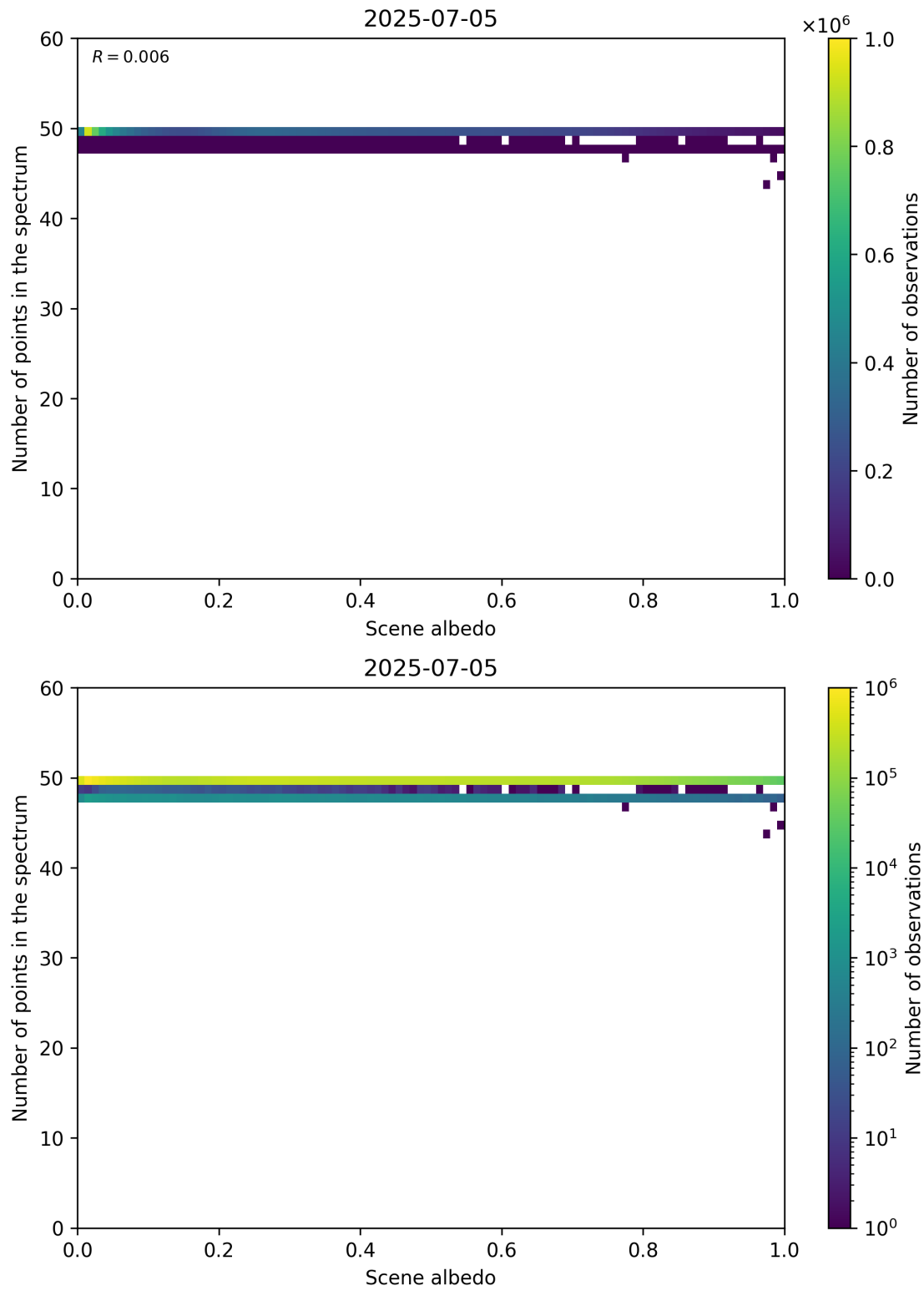
Figure 106: Scatter density plot of “Scene albedo” against “Number of points in the spectrum” for 2025-07-04 to 2025-07-06.
