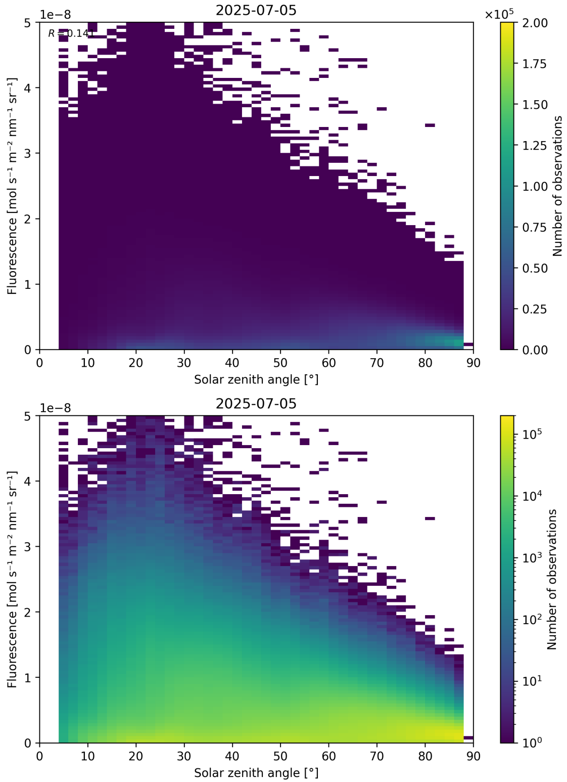
Figure 112: Scatter density plot of “Solar zenith angle” against “Fluorescence” for 2025-07-04 to 2025-07-06.
