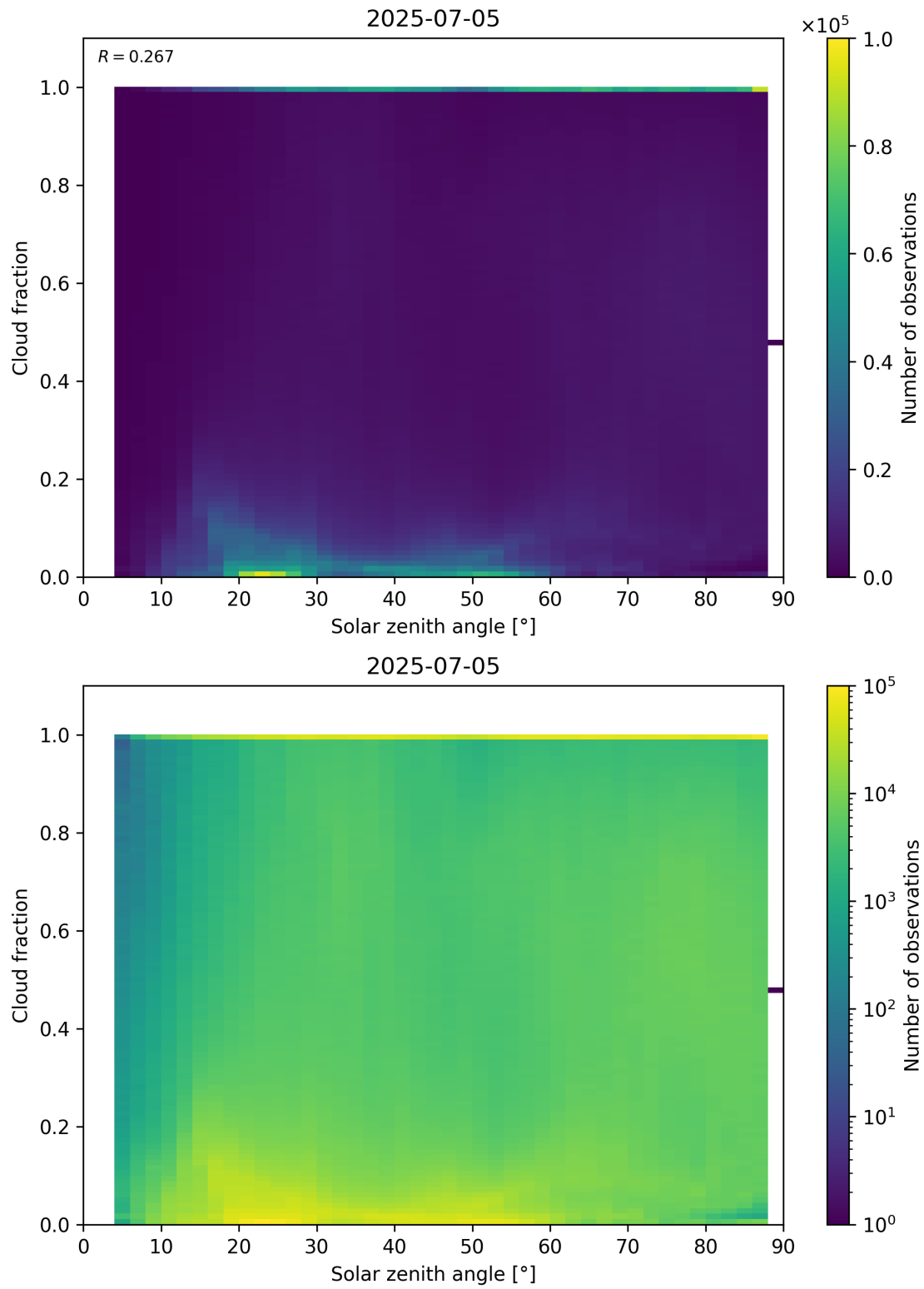
Figure 110: Scatter density plot of “Solar zenith angle” against “Cloud fraction” for 2025-07-04 to 2025-07-06.
