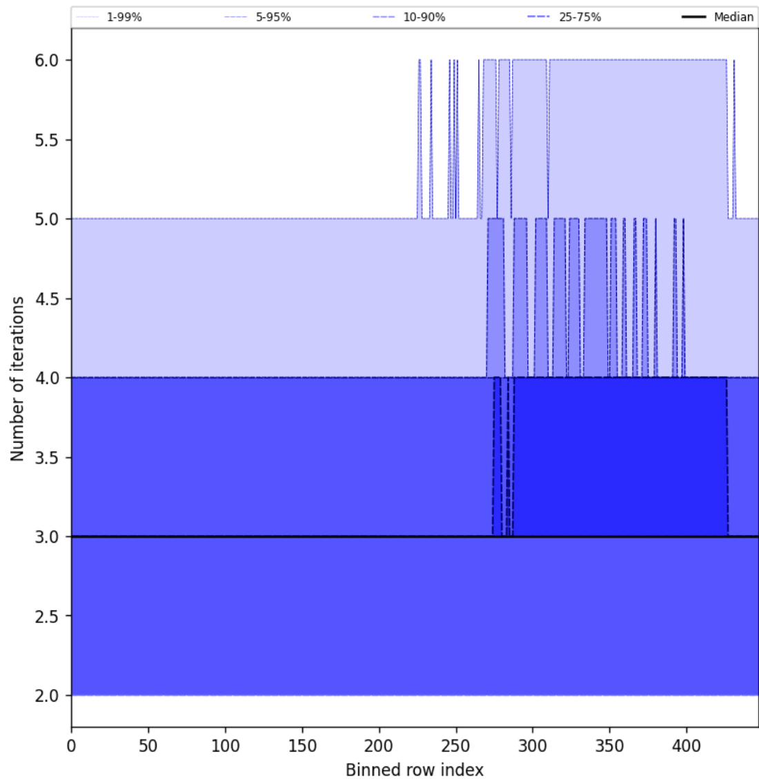
Figure 56: Along track statistics of “Number of iterations” for 2025-07-04 to 2025-07-06
