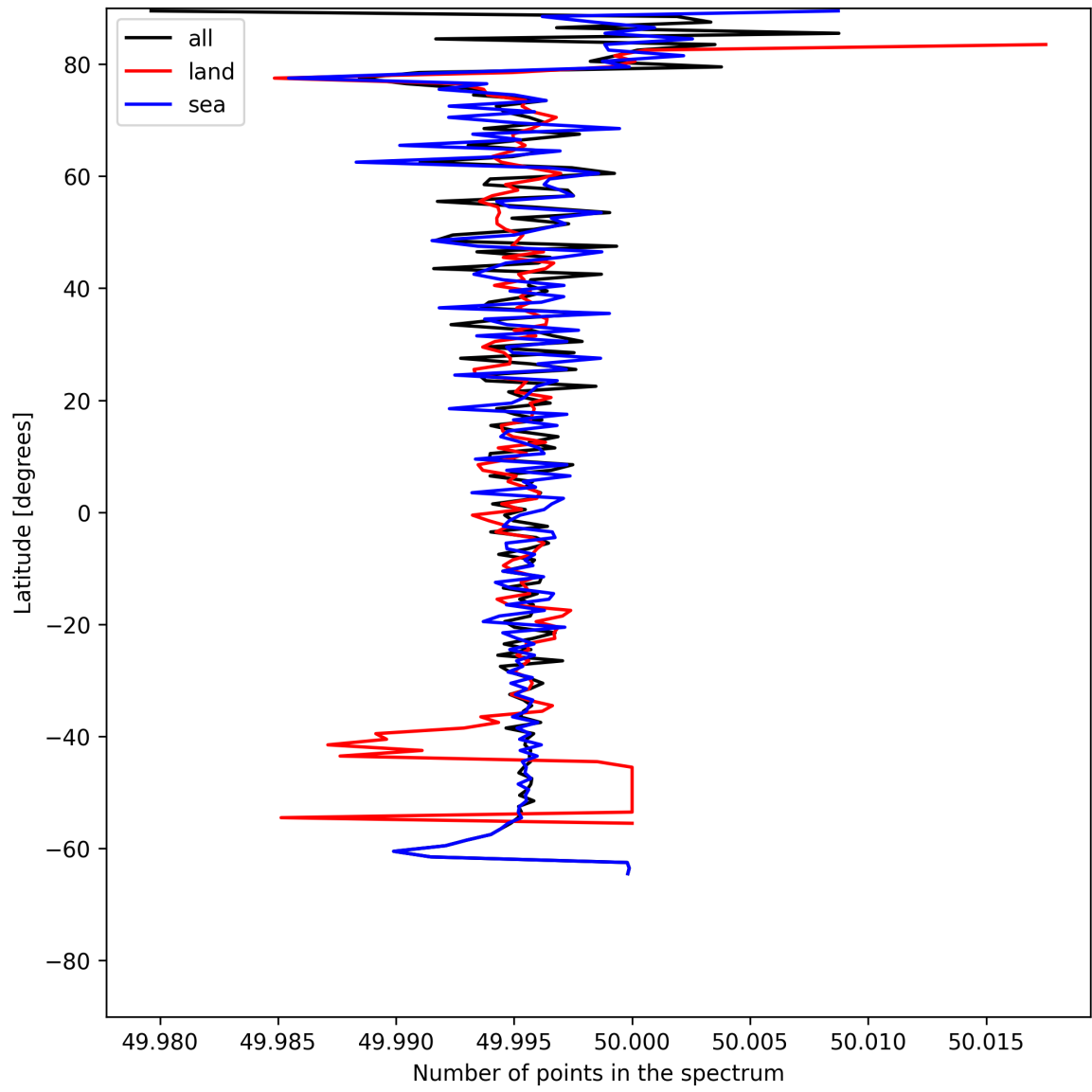
Figure 27: Zonal average of “Number of points in the spectrum” for 2025-07-04 to 2025-07-06.
