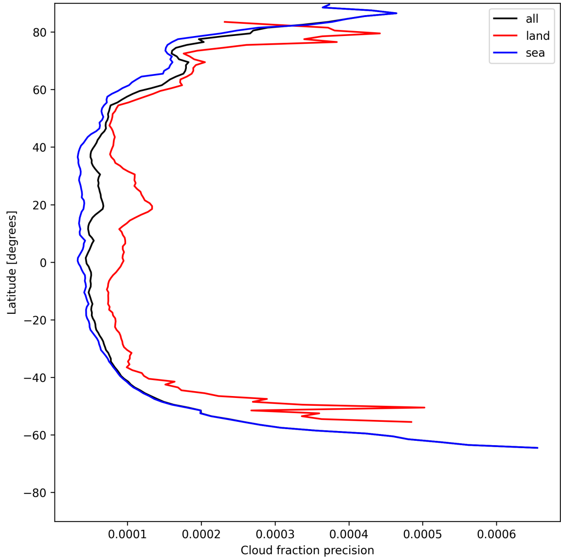
Figure 16: Zonal average of “Cloud fraction precision” for 2025-07-04 to 2025-07-06.
