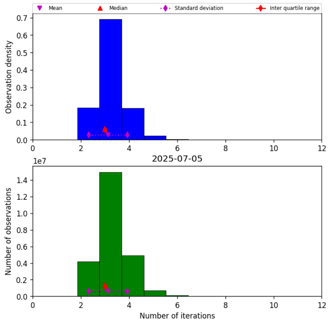
Figure 39: Histogram of “Number of iterations” for 2025-07-04 to 2025-07-06
