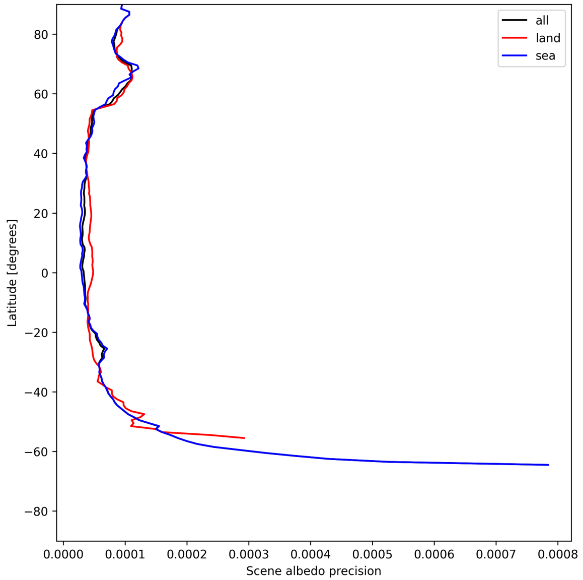
Figure 18: Zonal average of “Scene albedo precision” for 2025-07-04 to 2025-07-06.
