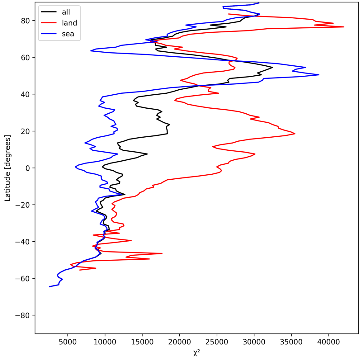
Figure 21: Zonal average of “ \chi^2 ” for 2025-07-04 to 2025-07-06.
