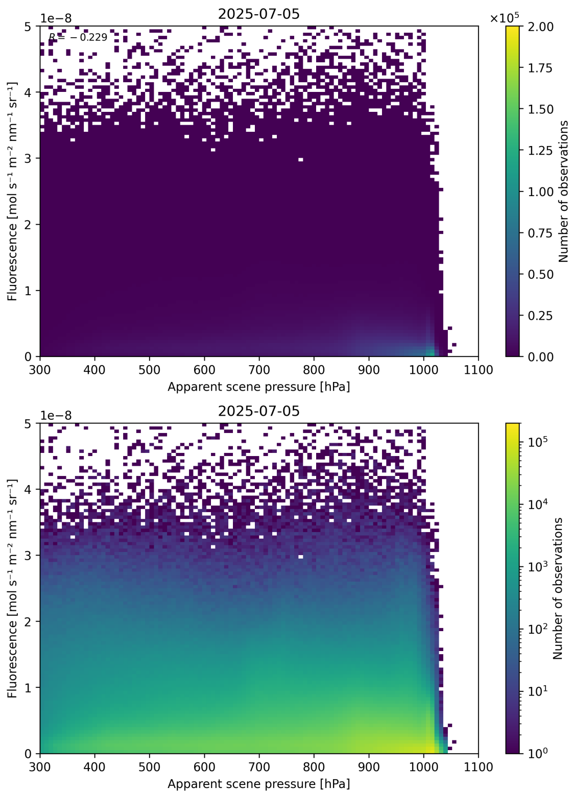
Figure 64: Scatter density plot of “Apparent scene pressure” against “Fluorescence” for 2025-07-04 to 2025-07-06.
