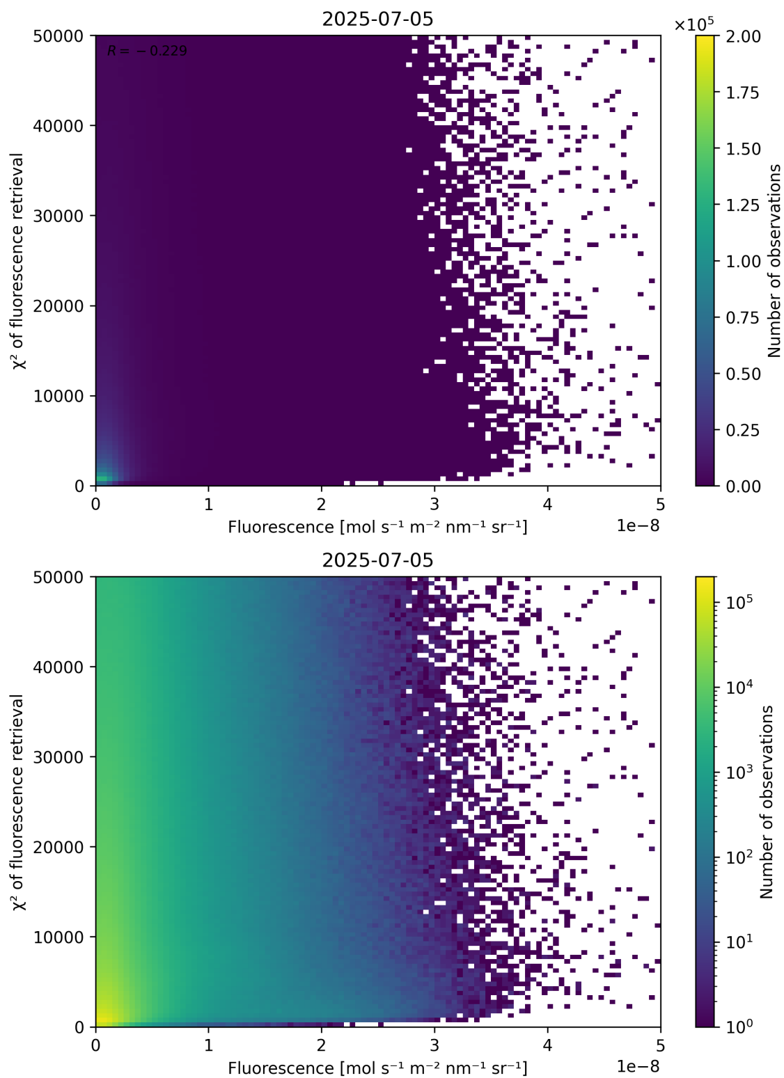
Figure 85: Scatter density plot of “Fluorescence” against “ \chi^2 of fluorescence retrieval” for 2025-07-04 to 2025-07-06.
