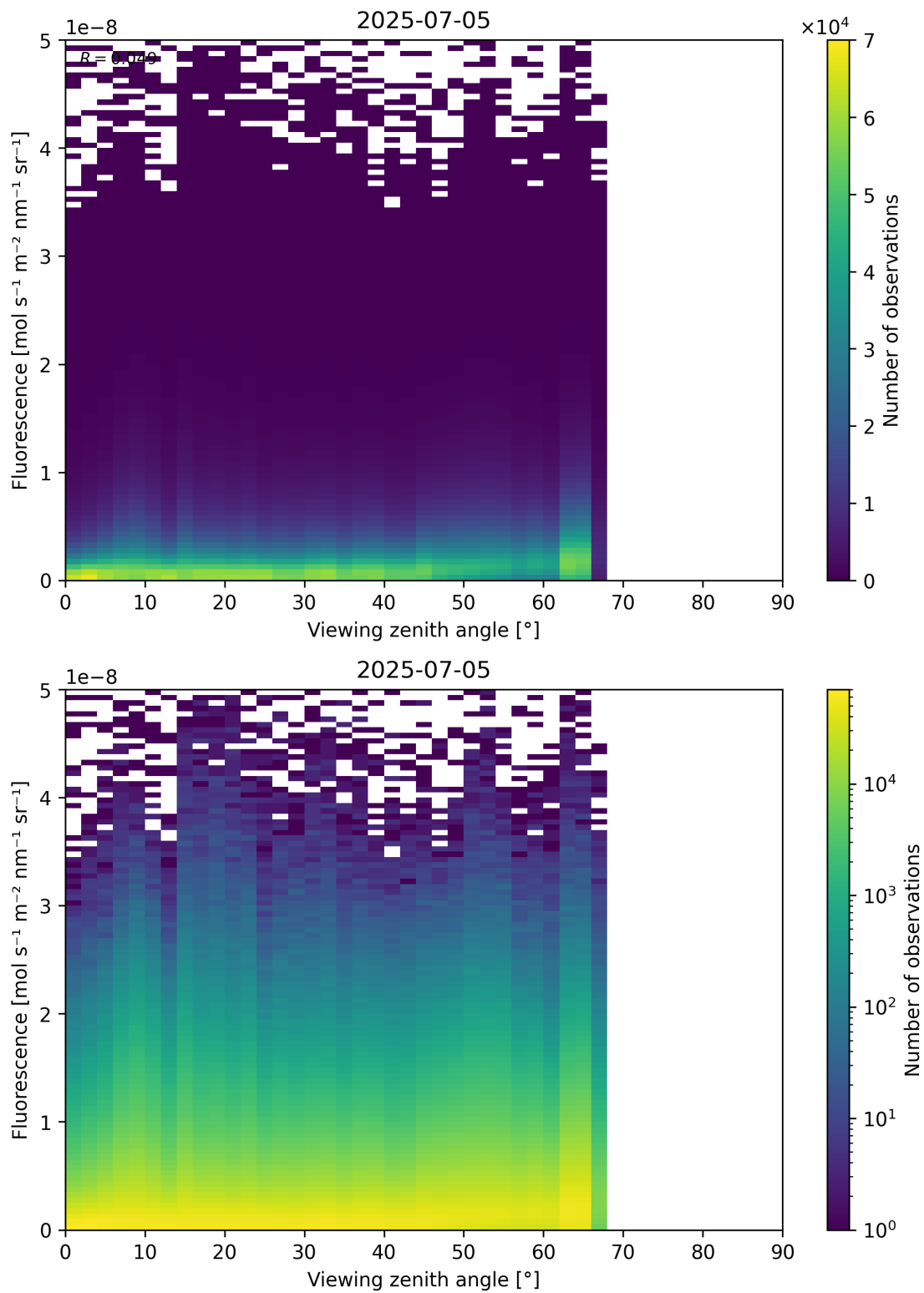
Figure 122: Scatter density plot of “Viewing zenith angle” against “Fluorescence” for 2025-07-04 to 2025-07-06.
