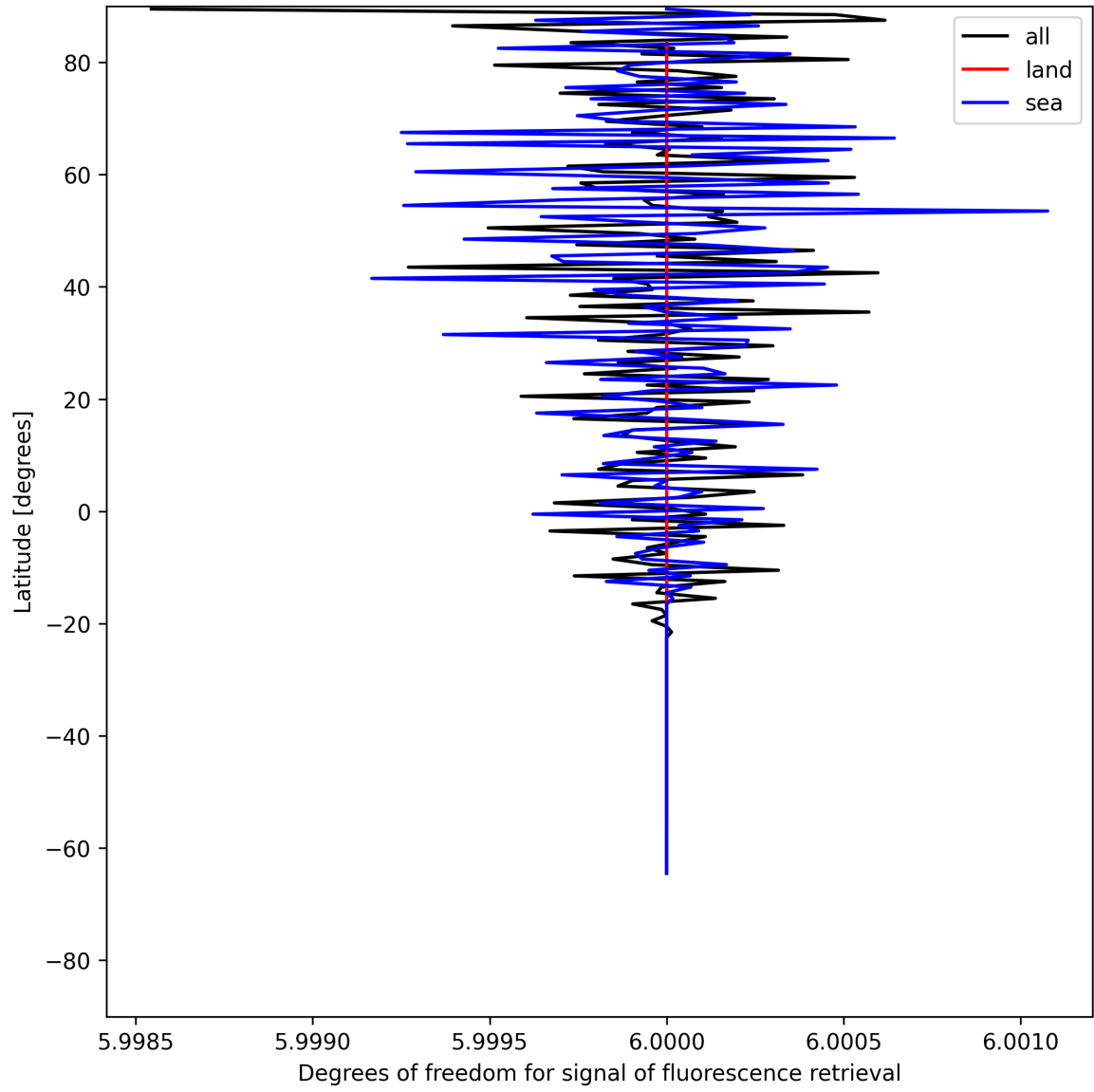
Figure 26: Zonal average of “Degrees of freedom for signal of fluorescence retrieval” for 2025-07-04 to 2025-07-06.
