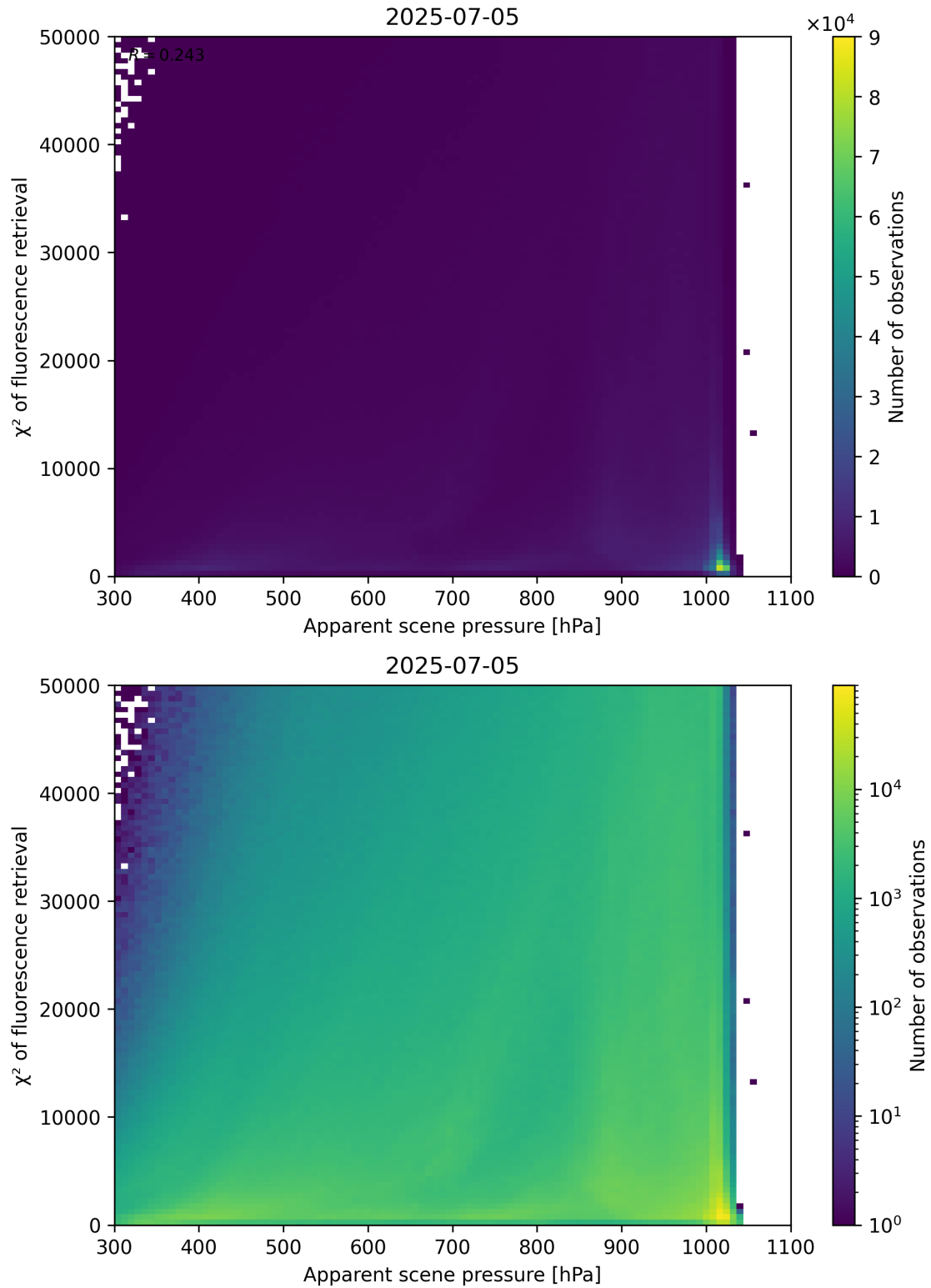
Figure 63: Scatter density plot of “Apparent scene pressure” against “ \chi^2 of fluorescence retrieval” for 2025-07-04 to 2025-07-06.
