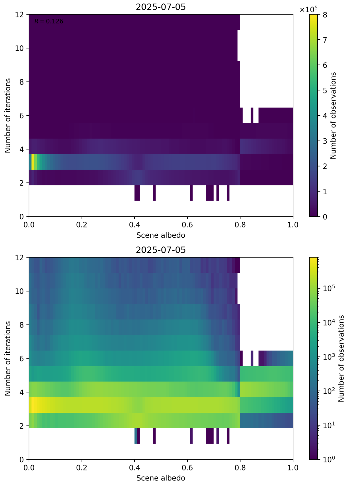
Figure 105: Scatter density plot of “Scene albedo” against “Number of iterations” for 2025-07-04 to 2025-07-06.
