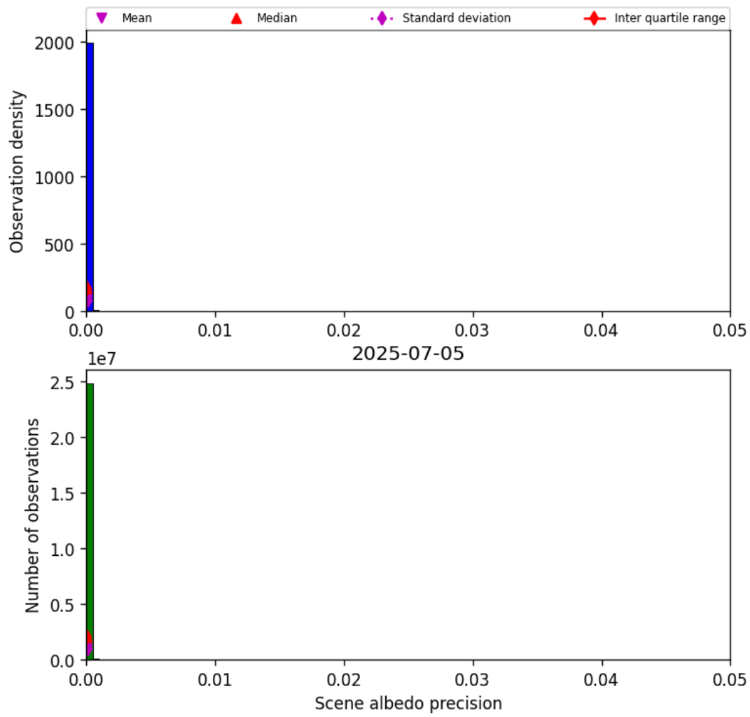
Figure 35: Histogram of “Scene albedo precision” for 2025-07-04 to 2025-07-06
