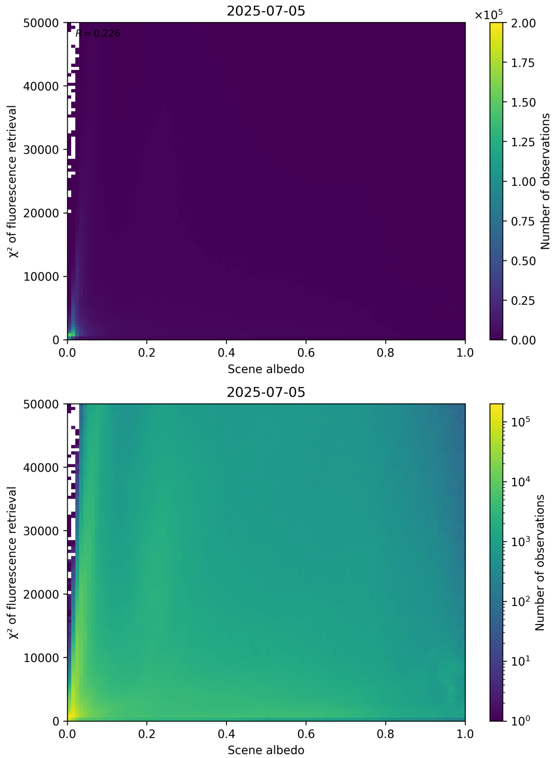
Figure 103: Scatter density plot of “Scene albedo” against “ \chi^2 of fluorescence retrieval” for 2025-07-04 to 2025-07-06.
