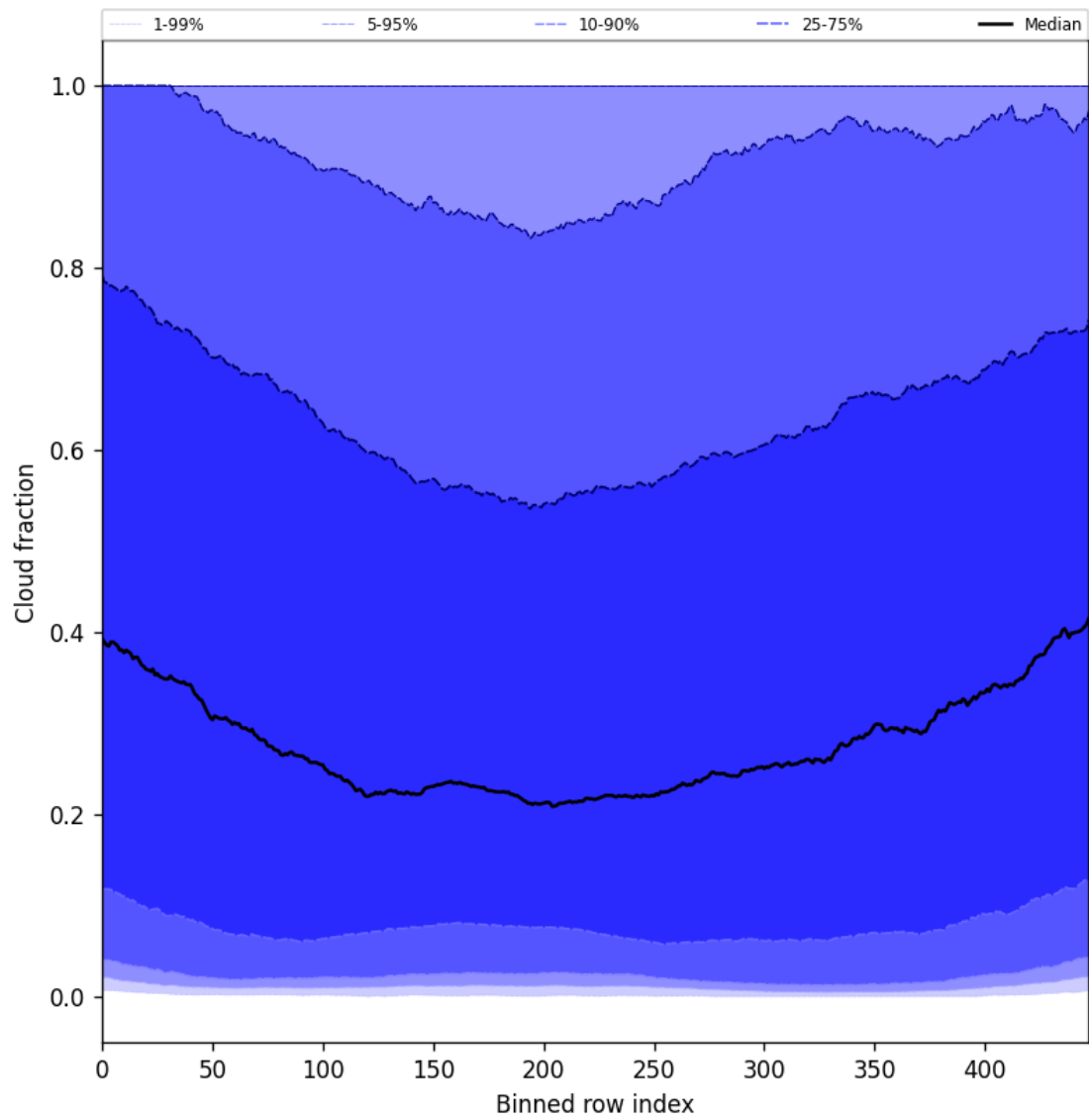
Figure 49: Along track statistics of “Cloud fraction” for 2025-07-04 to 2025-07-06
