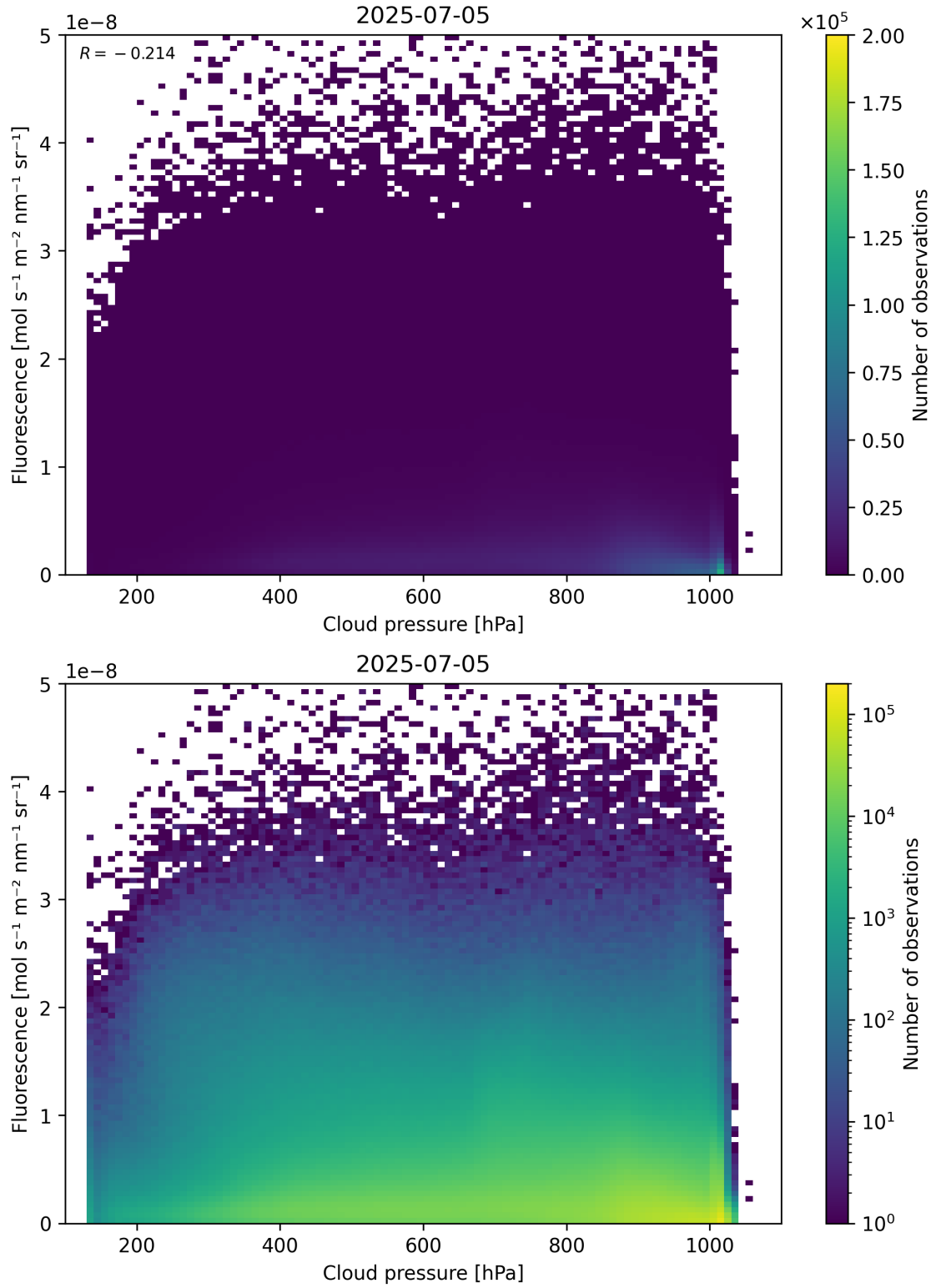
Figure 80: Scatter density plot of “Cloud pressure” against “Fluorescence” for 2025-07-04 to 2025-07-06.
