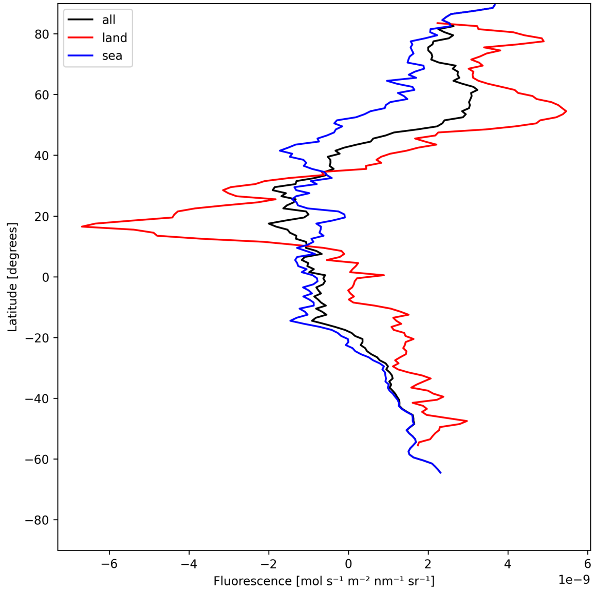
Figure 23: Zonal average of “Fluorescence” for 2025-07-04 to 2025-07-06.
