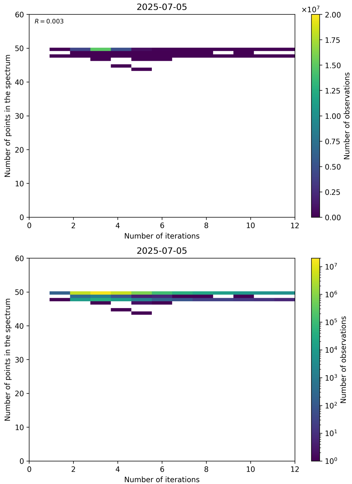
Figure 99: Scatter density plot of “Number of iterations” against “Number of points in the spectrum” for 2025-07-04 to 2025-07-06.
