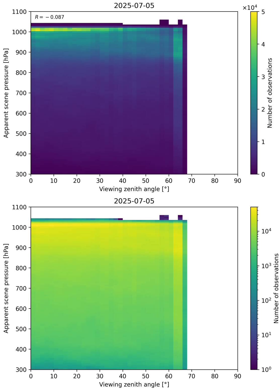
Figure 118: Scatter density plot of “Viewing zenith angle” against “Apparent scene pressure” for 2025-07-04 to 2025-07-06.
