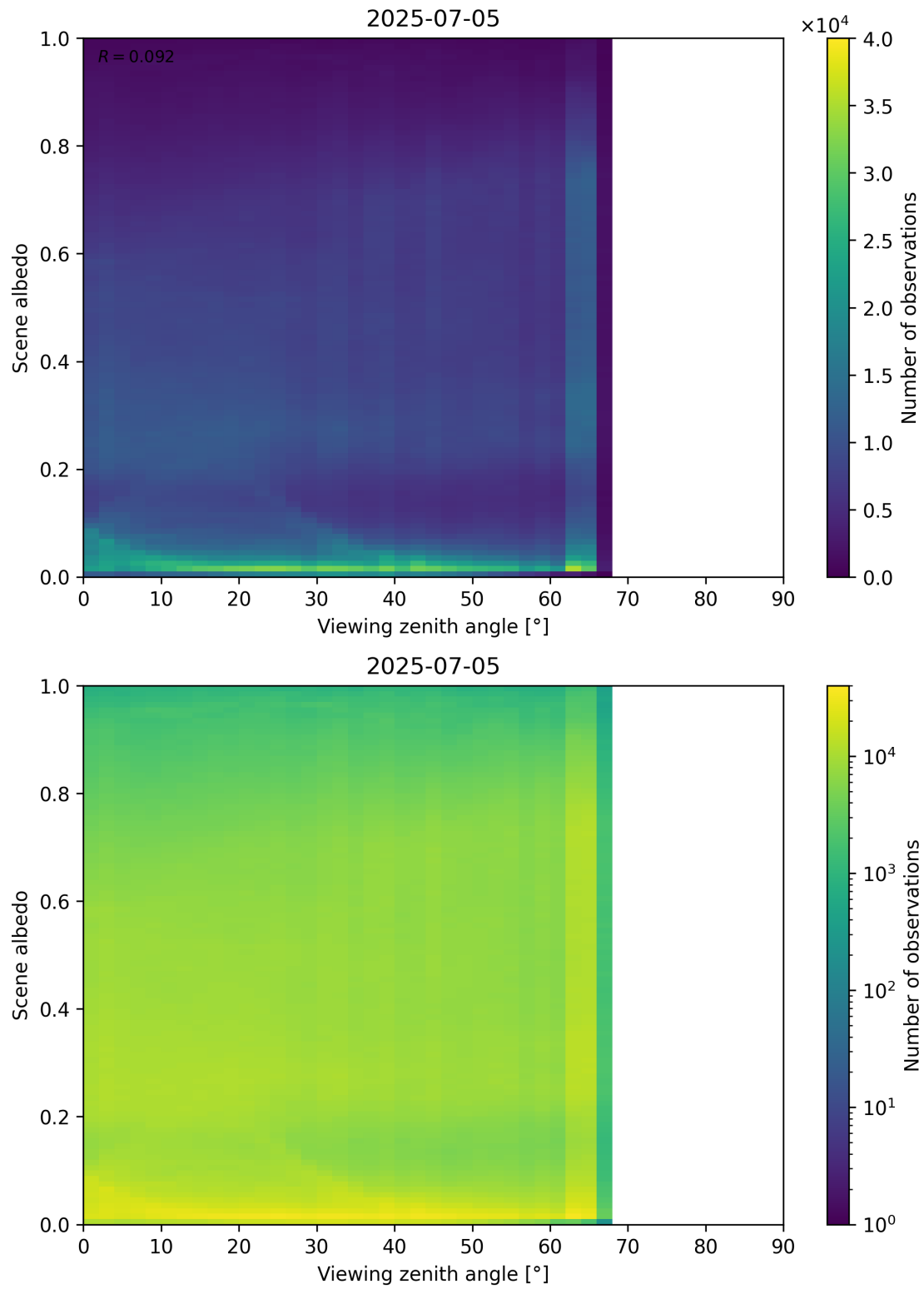
Figure 126: Scatter density plot of “Viewing zenith angle” against “Scene albedo” for 2025-07-04 to 2025-07-06.
