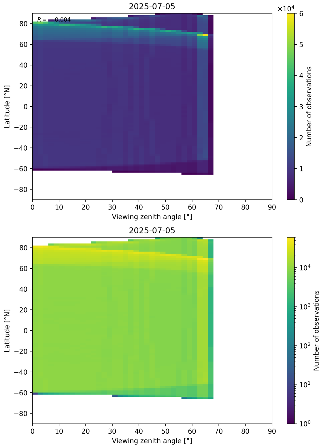
Figure 123: Scatter density plot of “Viewing zenith angle” against “Latitude” for 2025-07-04 to 2025-07-06.
