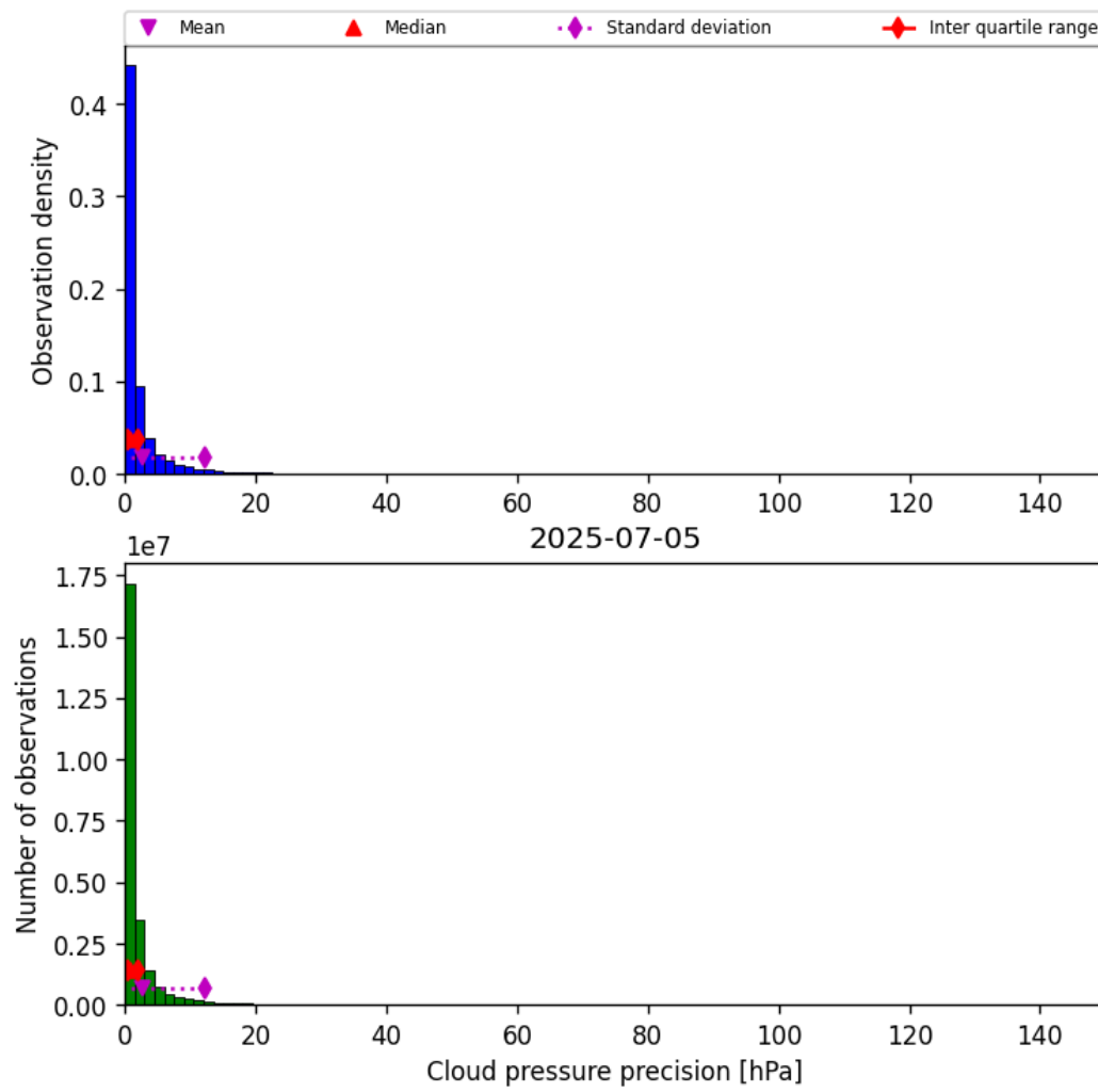
Figure 31: Histogram of “Cloud pressure precision” for 2025-07-04 to 2025-07-06
