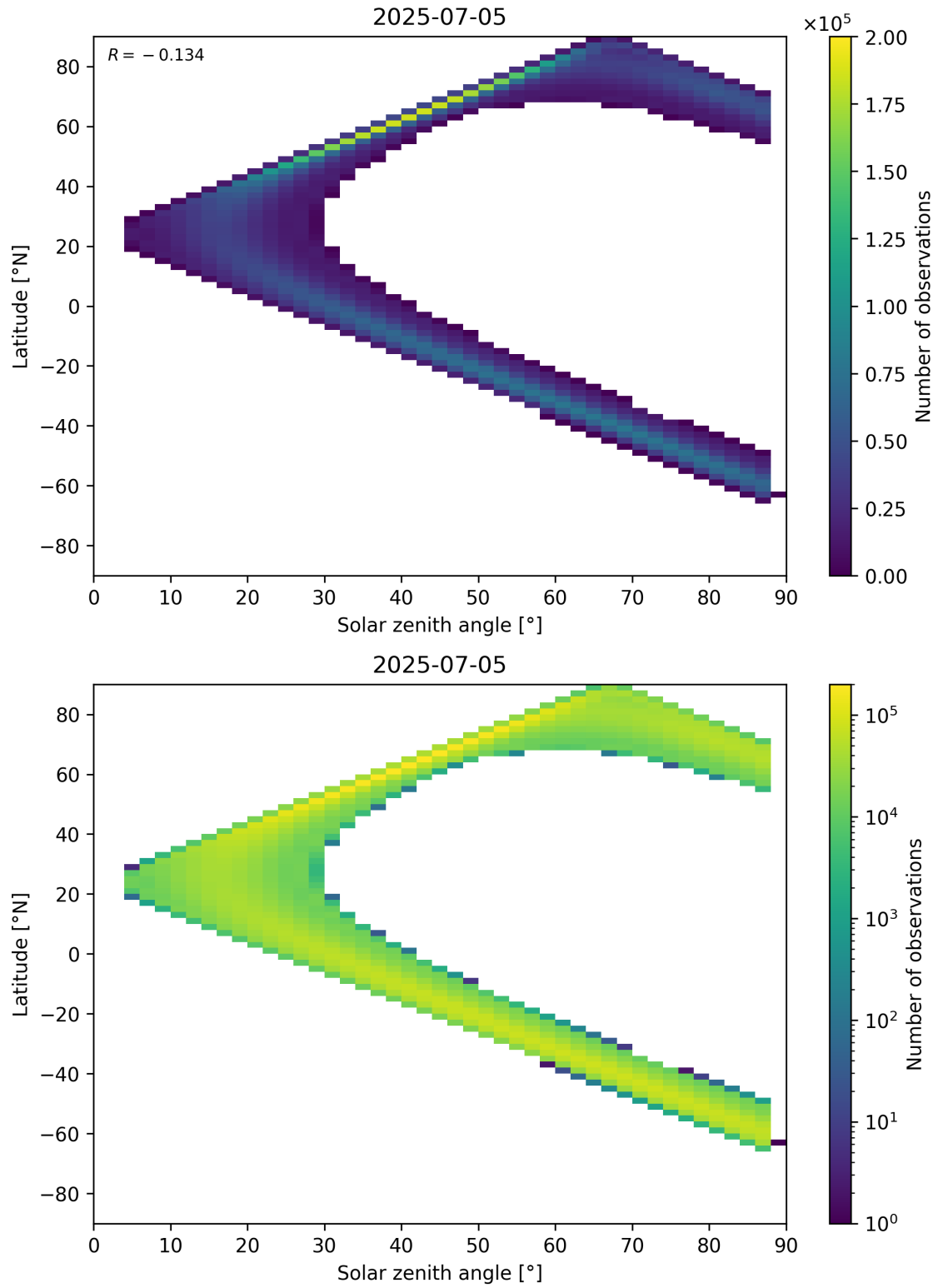
Figure 113: Scatter density plot of “Solar zenith angle” against “Latitude” for 2025-07-04 to 2025-07-06.
