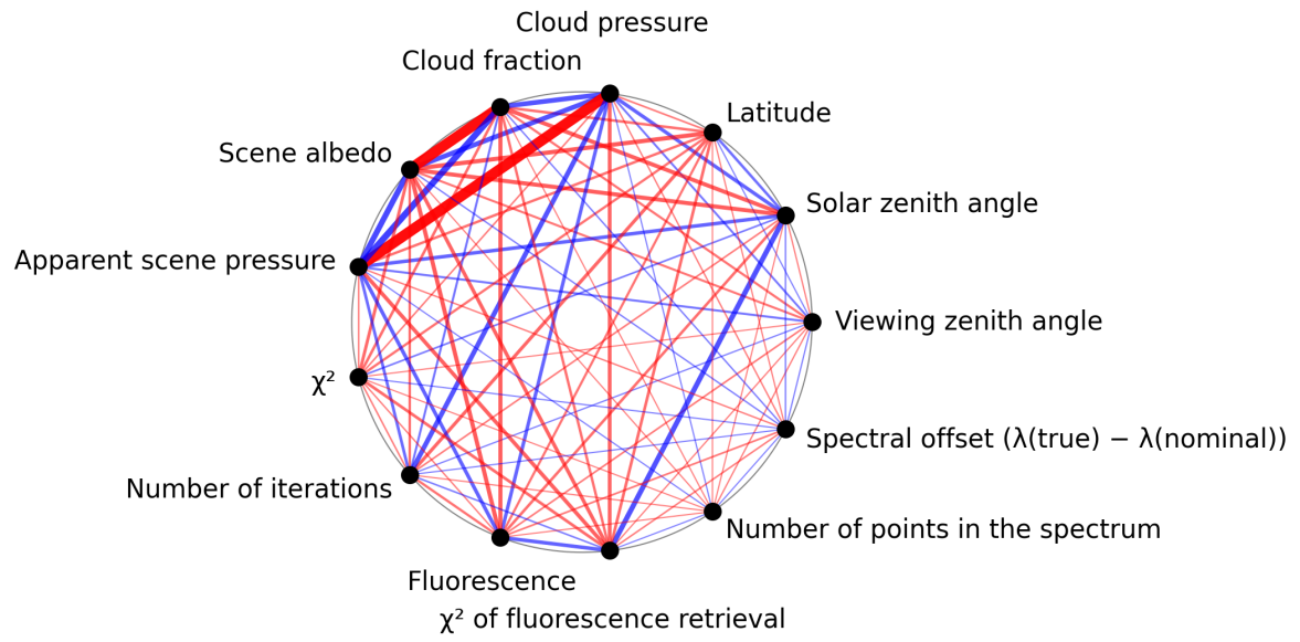
Figure 1: Map of correlation graph for 2025-07-04 to 2025-07-06.
