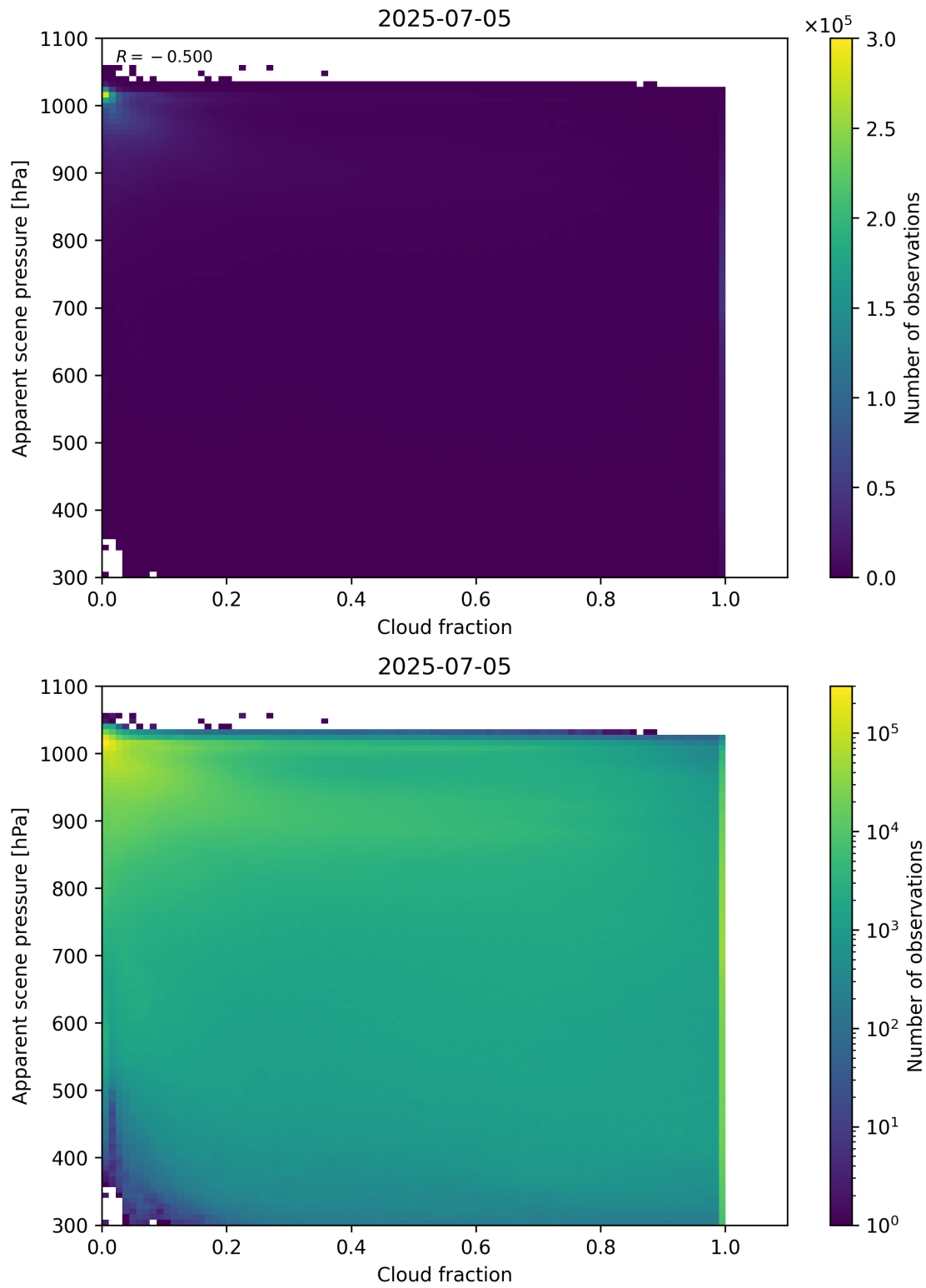
Figure 70: Scatter density plot of “Cloud fraction” against “Apparent scene pressure” for 2025-07-04 to 2025-07-06.
