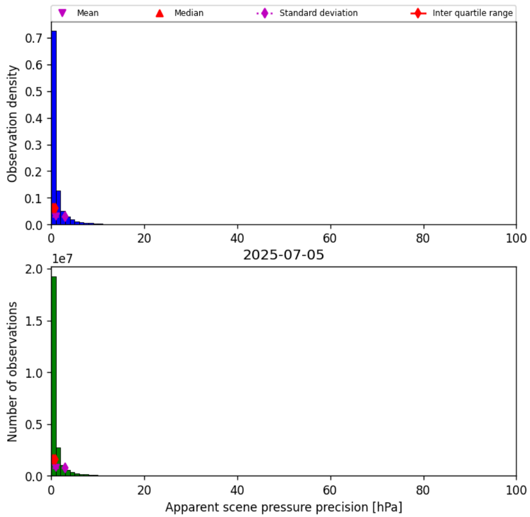
Figure 37: Histogram of “Apparent scene pressure precision” for 2025-07-04 to 2025-07-06
