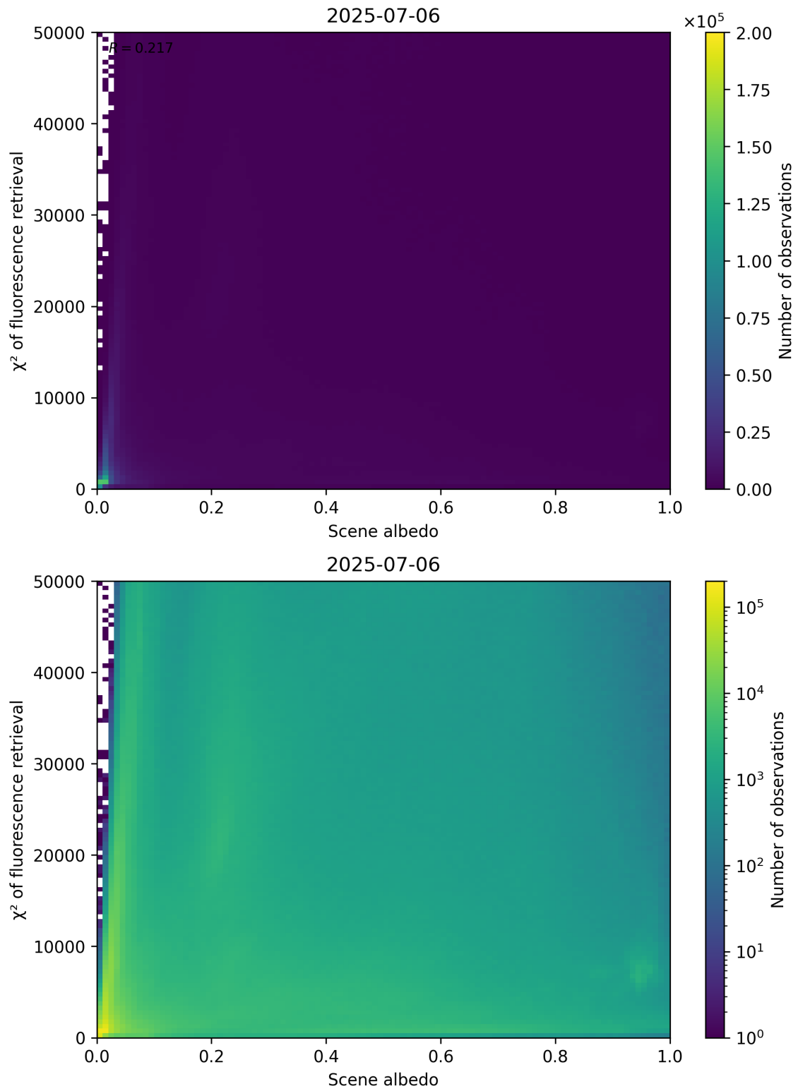
Figure 103: Scatter density plot of “Scene albedo” against “ \chi^2 of fluorescence retrieval” for 2025-07-05 to 2025-07-07.
