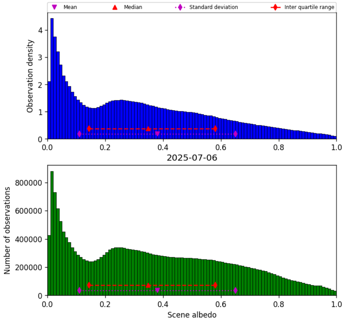
Figure 34: Histogram of “Scene albedo” for 2025-07-05 to 2025-07-07
