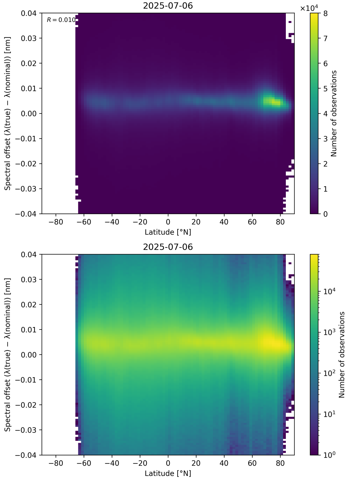
Figure 96: Scatter density plot of “Latitude” against “Spectral offset ( \lambda_{\text{true}} - \lambda_{\text{nominal}} )” for 2025-07-05 to 2025-07-07.
