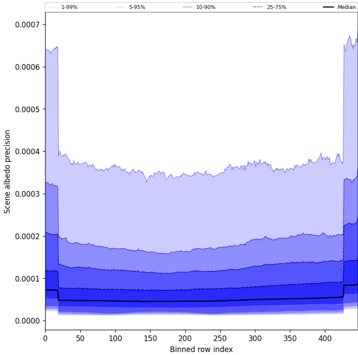
Figure 52: Along track statistics of “Scene albedo precision” for 2025-07-05 to 2025-07-07
