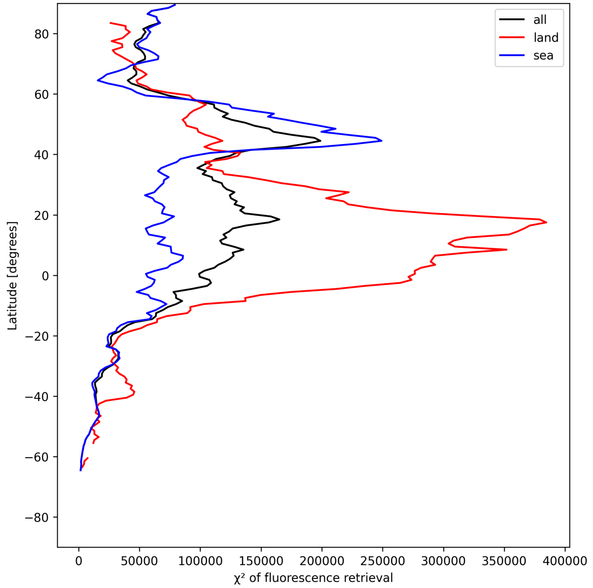
Figure 25: Zonal average of “ \chi^2 of fluorescence retrieval” for 2025-07-05 to 2025-07-07.
