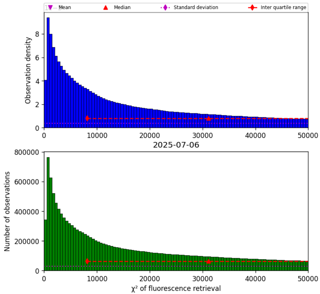
Figure 42: Histogram of “ \chi^2 of fluorescence retrieval” for 2025-07-05 to 2025-07-07
