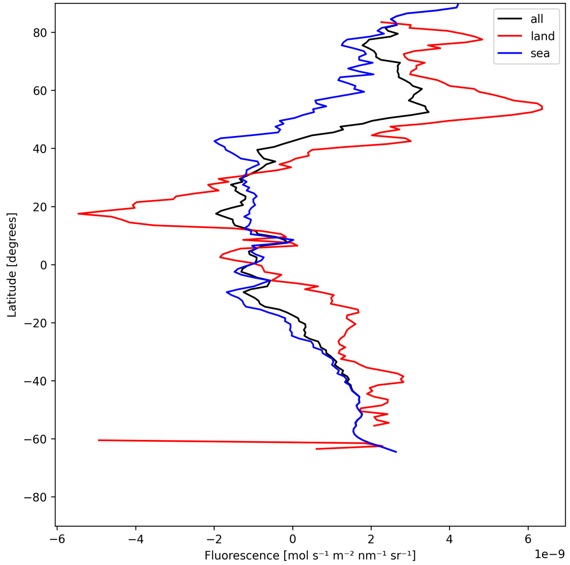
Figure 23: Zonal average of “Fluorescence” for 2025-07-05 to 2025-07-07.
