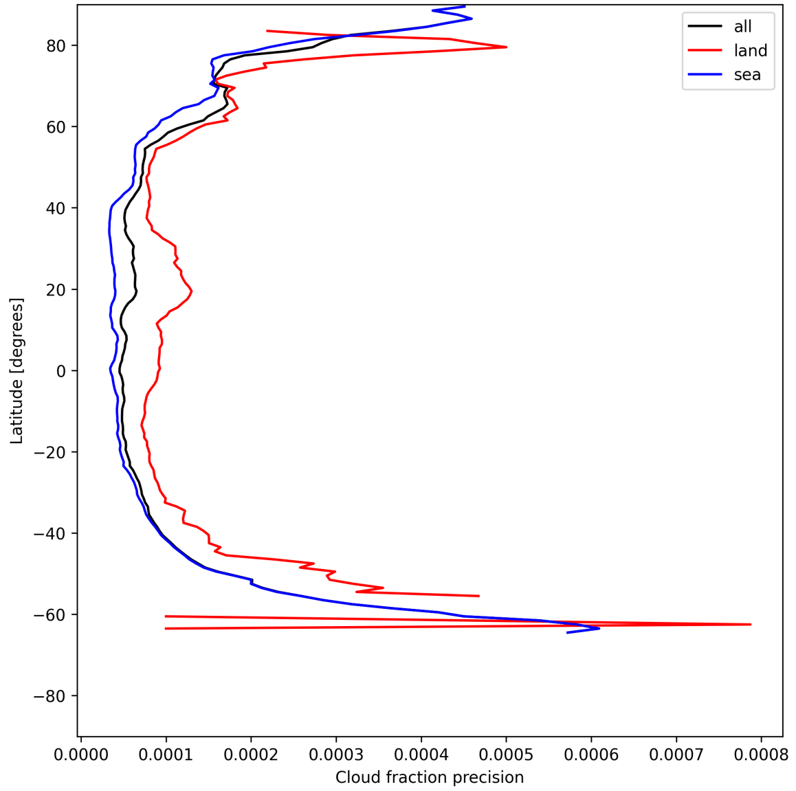
Figure 16: Zonal average of “Cloud fraction precision” for 2025-07-05 to 2025-07-07.
