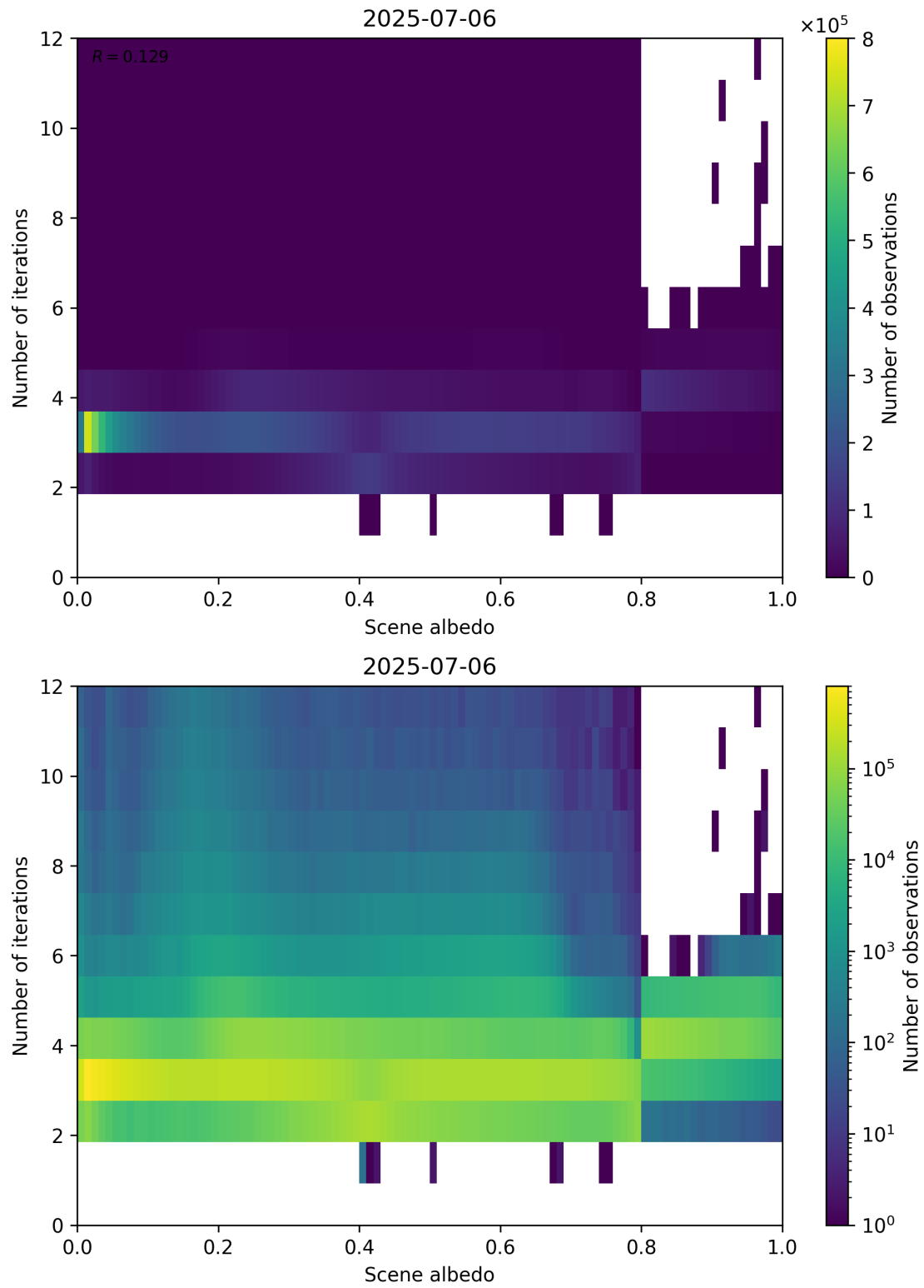
Figure 105: Scatter density plot of “Scene albedo” against “Number of iterations” for 2025-07-05 to 2025-07-07.
