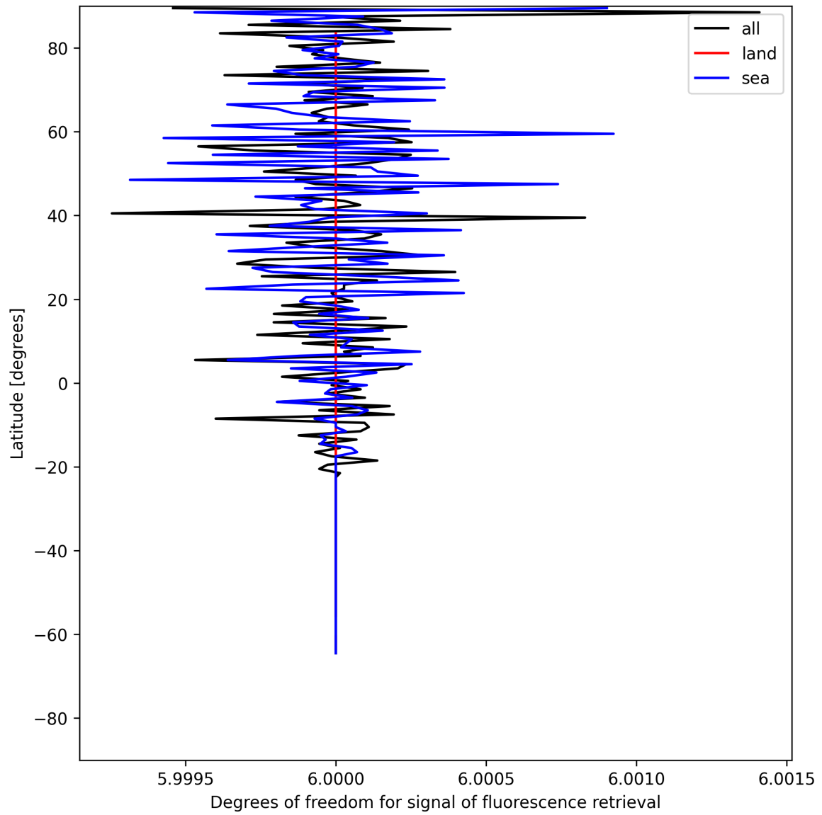
Figure 26: Zonal average of “Degrees of freedom for signal of fluorescence retrieval” for 2025-07-05 to 2025-07-07.
