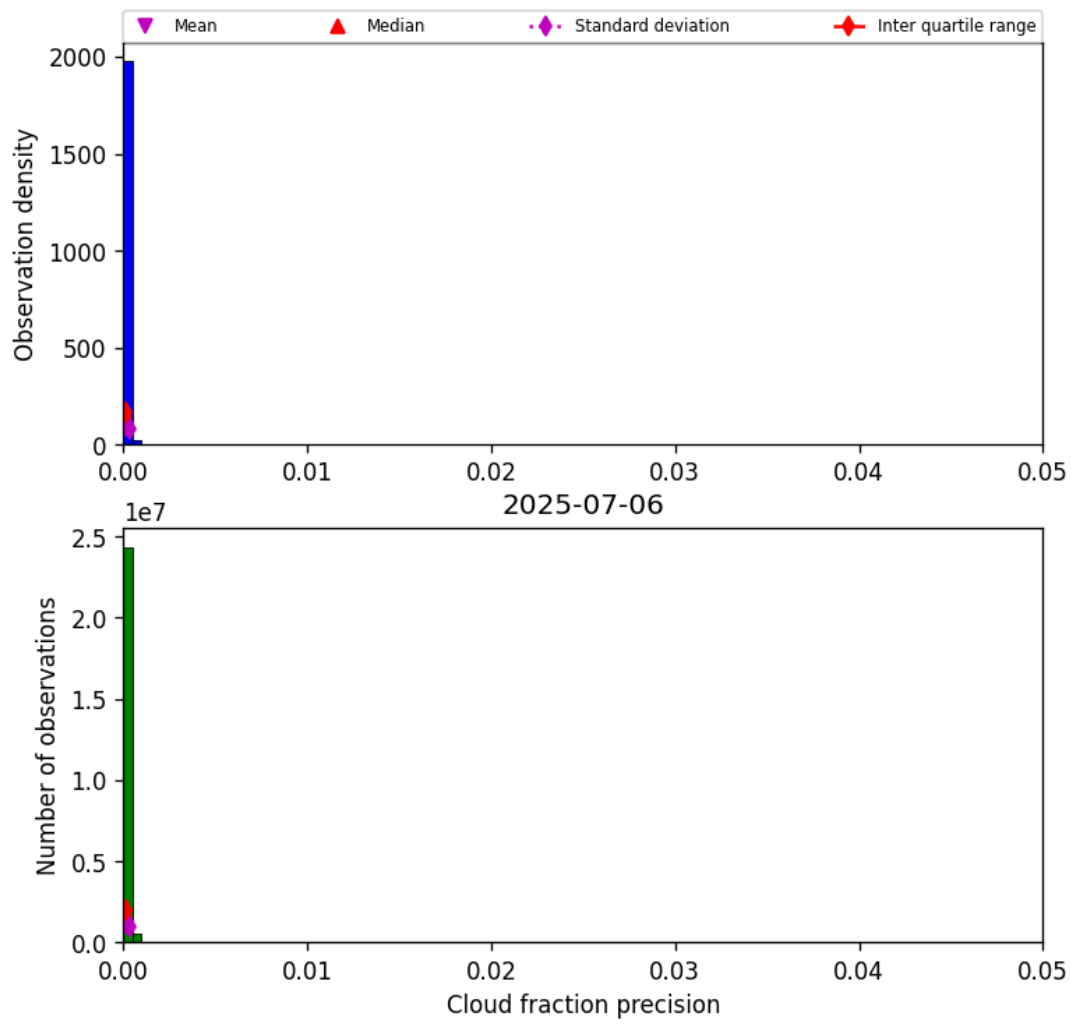
Figure 33: Histogram of “Cloud fraction precision” for 2025-07-05 to 2025-07-07
