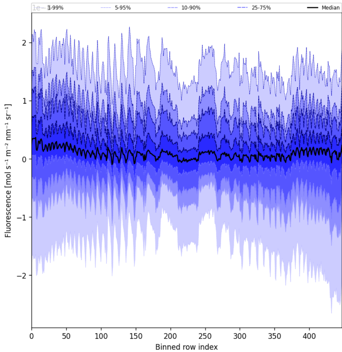
Figure 57: Along track statistics of “Fluorescence” for 2025-07-05 to 2025-07-07
