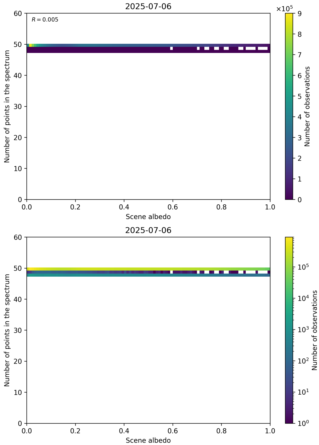
Figure 106: Scatter density plot of “Scene albedo” against “Number of points in the spectrum” for 2025-07-05 to 2025-07-07.
