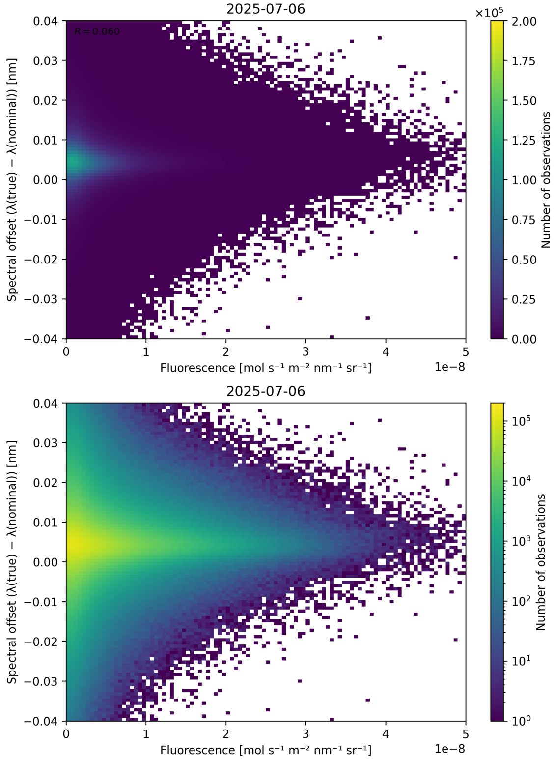
Figure 87: Scatter density plot of “Fluorescence” against “Spectral offset ( \lambda_{\text{true}} - \lambda_{\text{nominal}} )” for 2025-07-05 to 2025-07-07.
