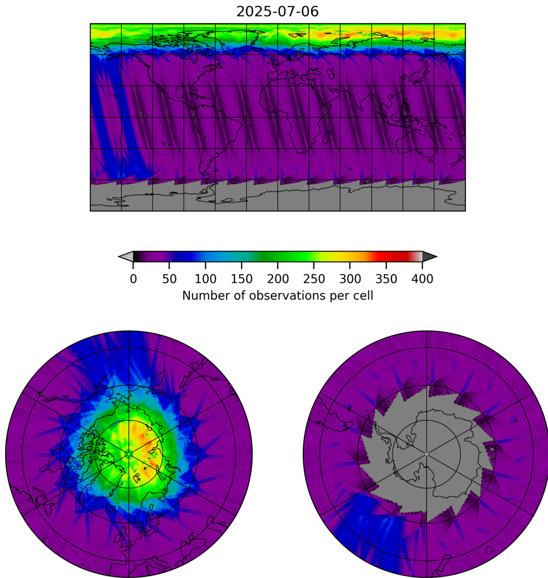
Figure 11: Map of the number of observations for 2025-07-05 to 2025-07-07
