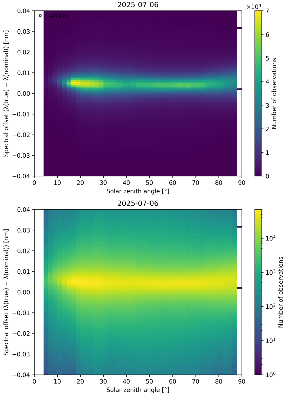
Figure 117: Scatter density plot of “Solar zenith angle” against “Spectral offset ( \lambda_{\text{true}} - \lambda_{\text{nominal}} )” for 2025-07-05 to 2025-07-07.
