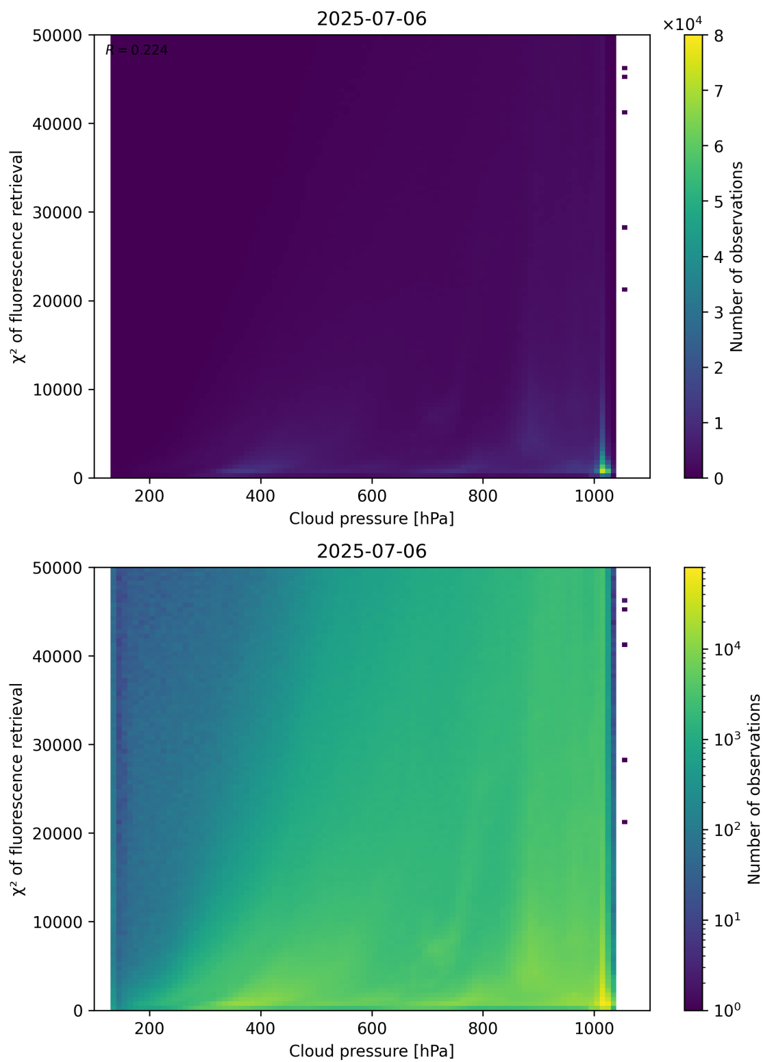
Figure 78: Scatter density plot of “Cloud pressure” against “ \chi^2 of fluorescence retrieval” for 2025-07-05 to 2025-07-07.
