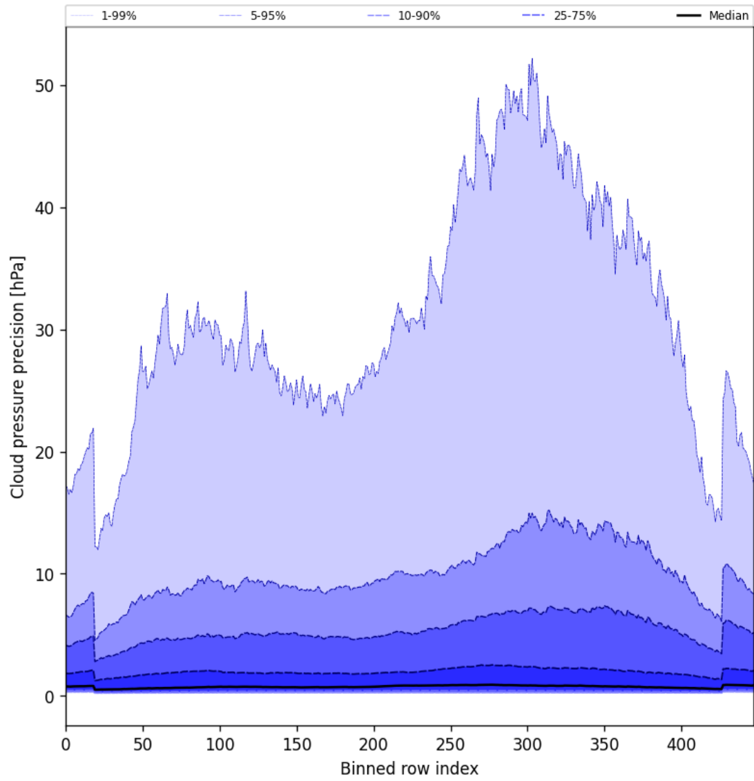
Figure 48: Along track statistics of “Cloud pressure precision” for 2025-07-05 to 2025-07-07
