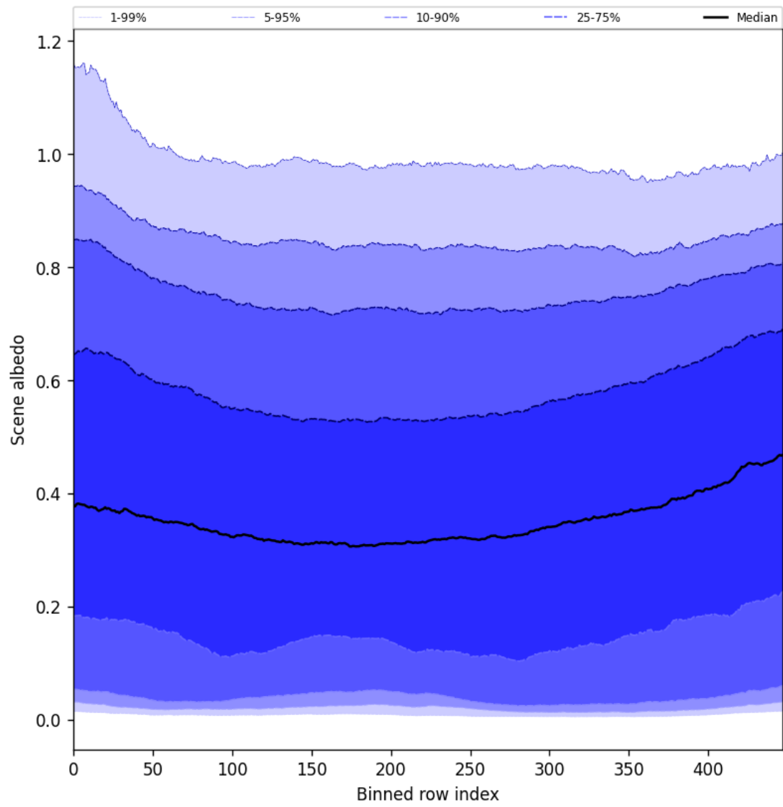
Figure 51: Along track statistics of “Scene albedo” for 2025-07-05 to 2025-07-07
