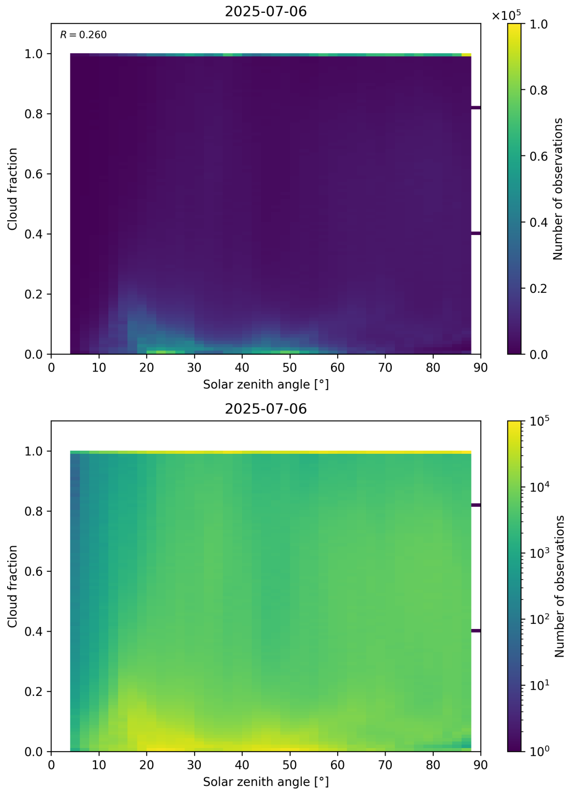
Figure 110: Scatter density plot of “Solar zenith angle” against “Cloud fraction” for 2025-07-05 to 2025-07-07.
