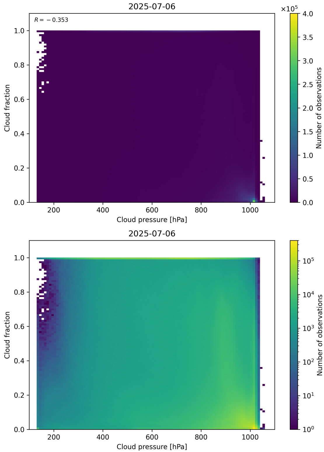
Figure 79: Scatter density plot of “Cloud pressure” against “Cloud fraction” for 2025-07-05 to 2025-07-07.
