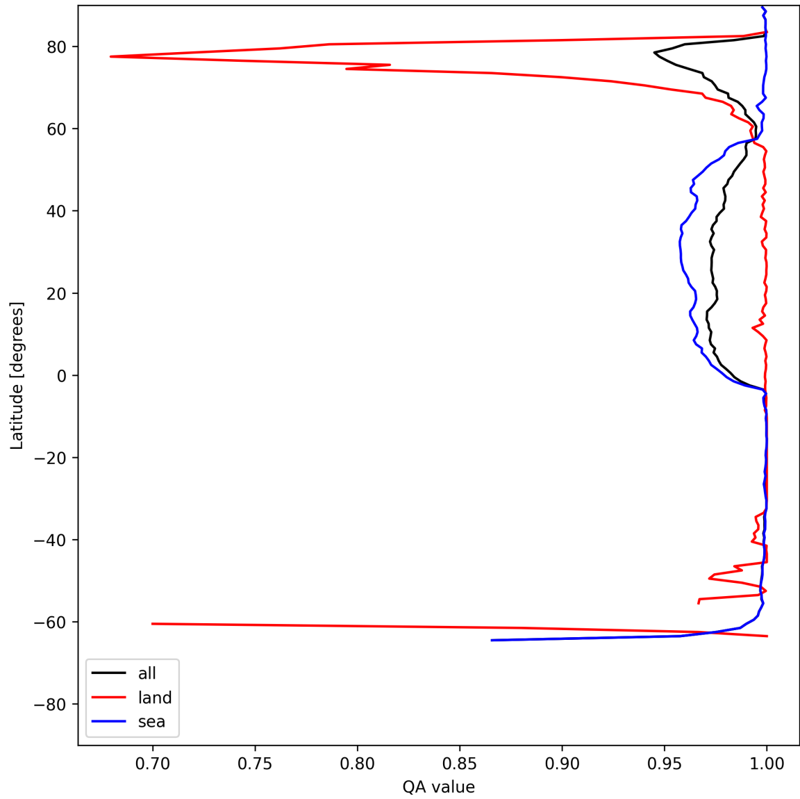
Figure 12: Zonal average of “QA value” for 2025-07-05 to 2025-07-07.
