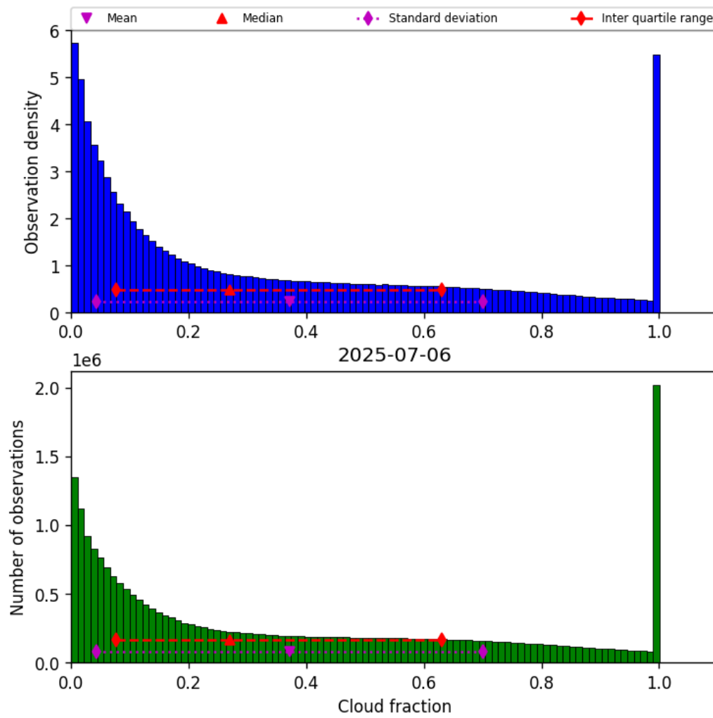
Figure 32: Histogram of “Cloud fraction” for 2025-07-05 to 2025-07-07
