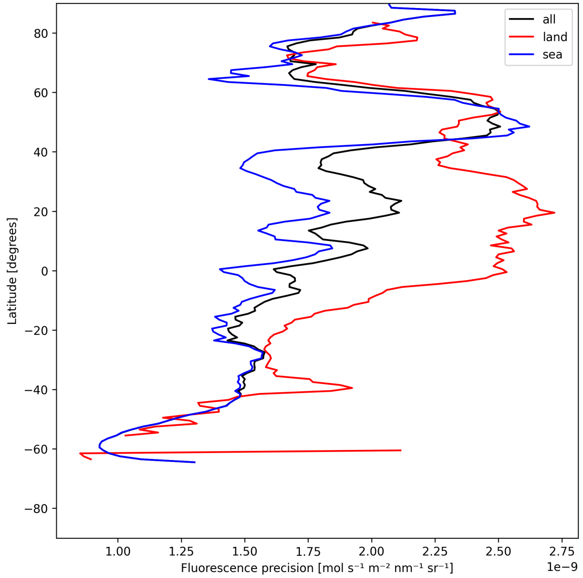
Figure 24: Zonal average of “Fluorescence precision” for 2025-07-05 to 2025-07-07.
