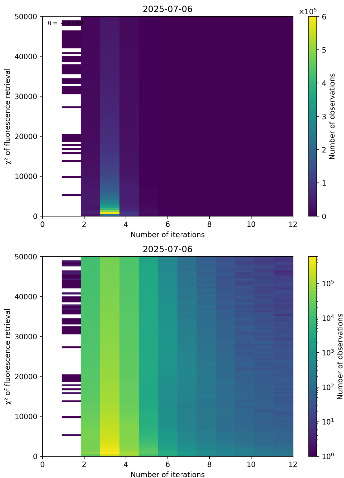
Figure 97: Scatter density plot of “Number of iterations” against “ \chi^2 of fluorescence retrieval” for 2025-07-05 to 2025-07-07.
