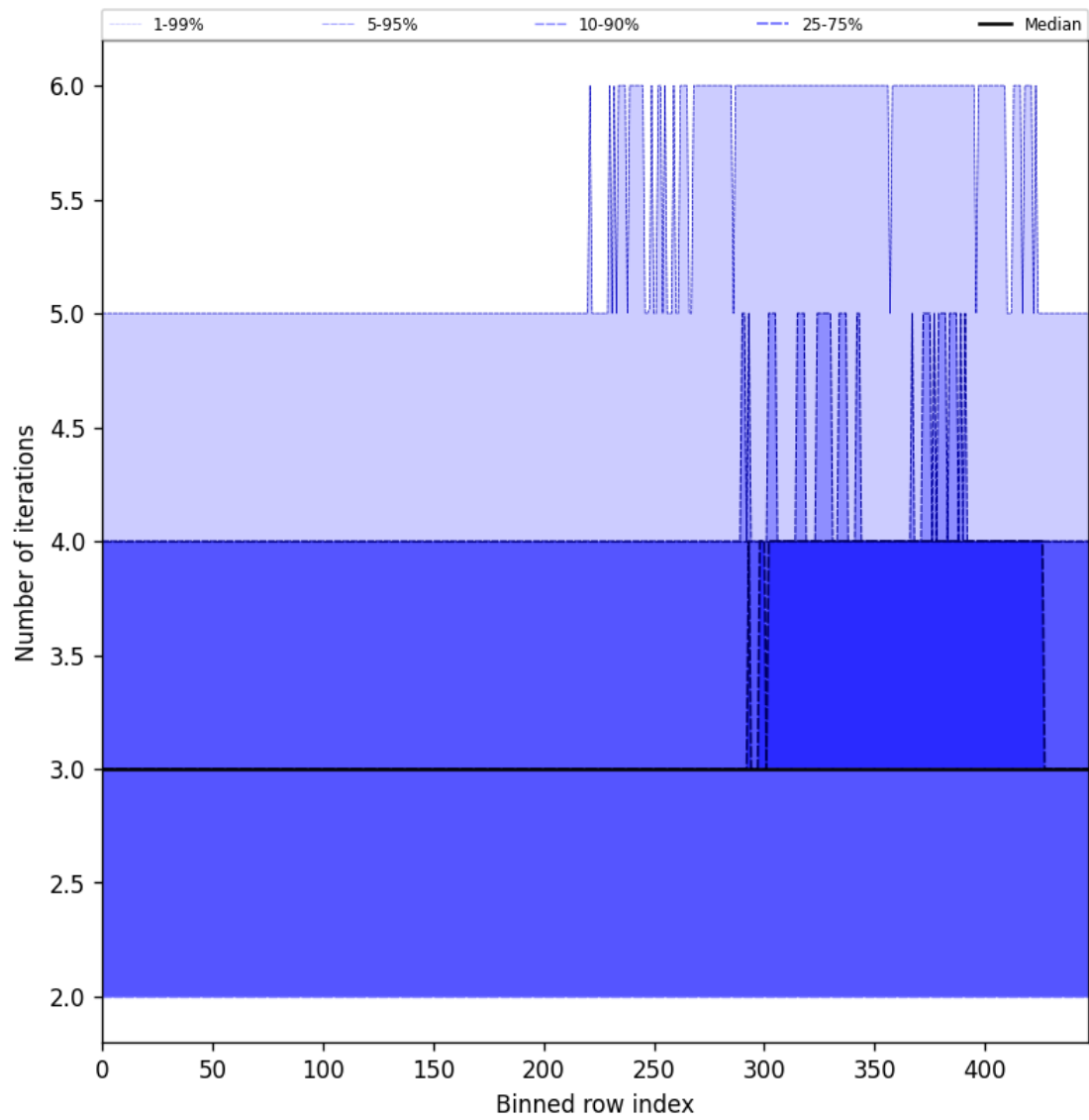
Figure 56: Along track statistics of “Number of iterations” for 2025-07-05 to 2025-07-07
