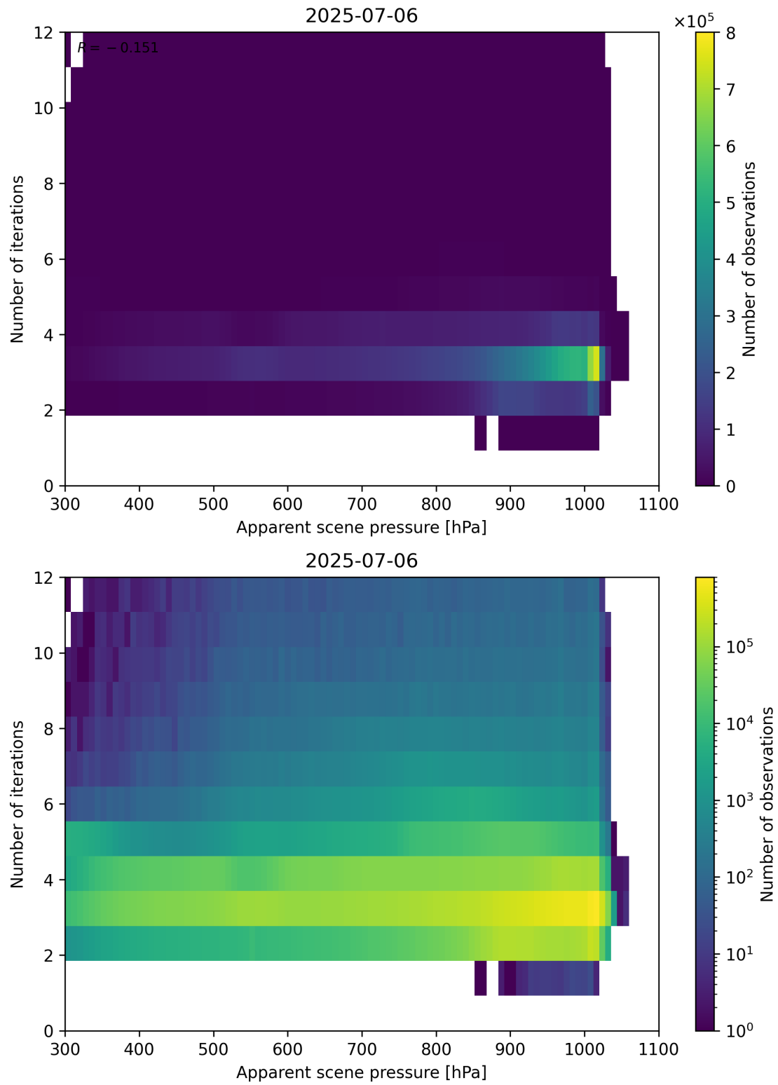
Figure 65: Scatter density plot of “Apparent scene pressure” against “Number of iterations” for 2025-07-05 to 2025-07-07.
