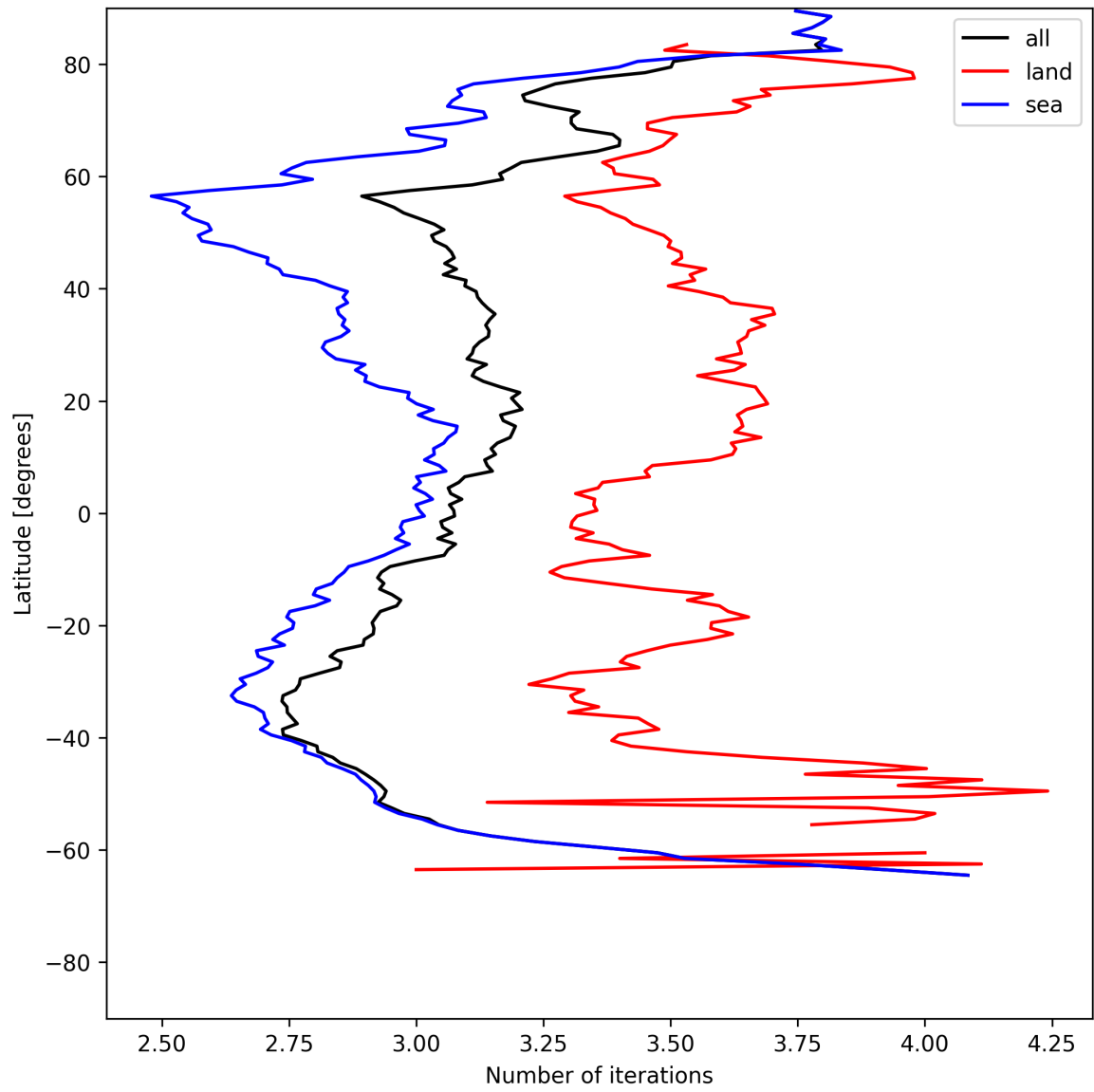
Figure 22: Zonal average of “Number of iterations” for 2025-07-05 to 2025-07-07.
