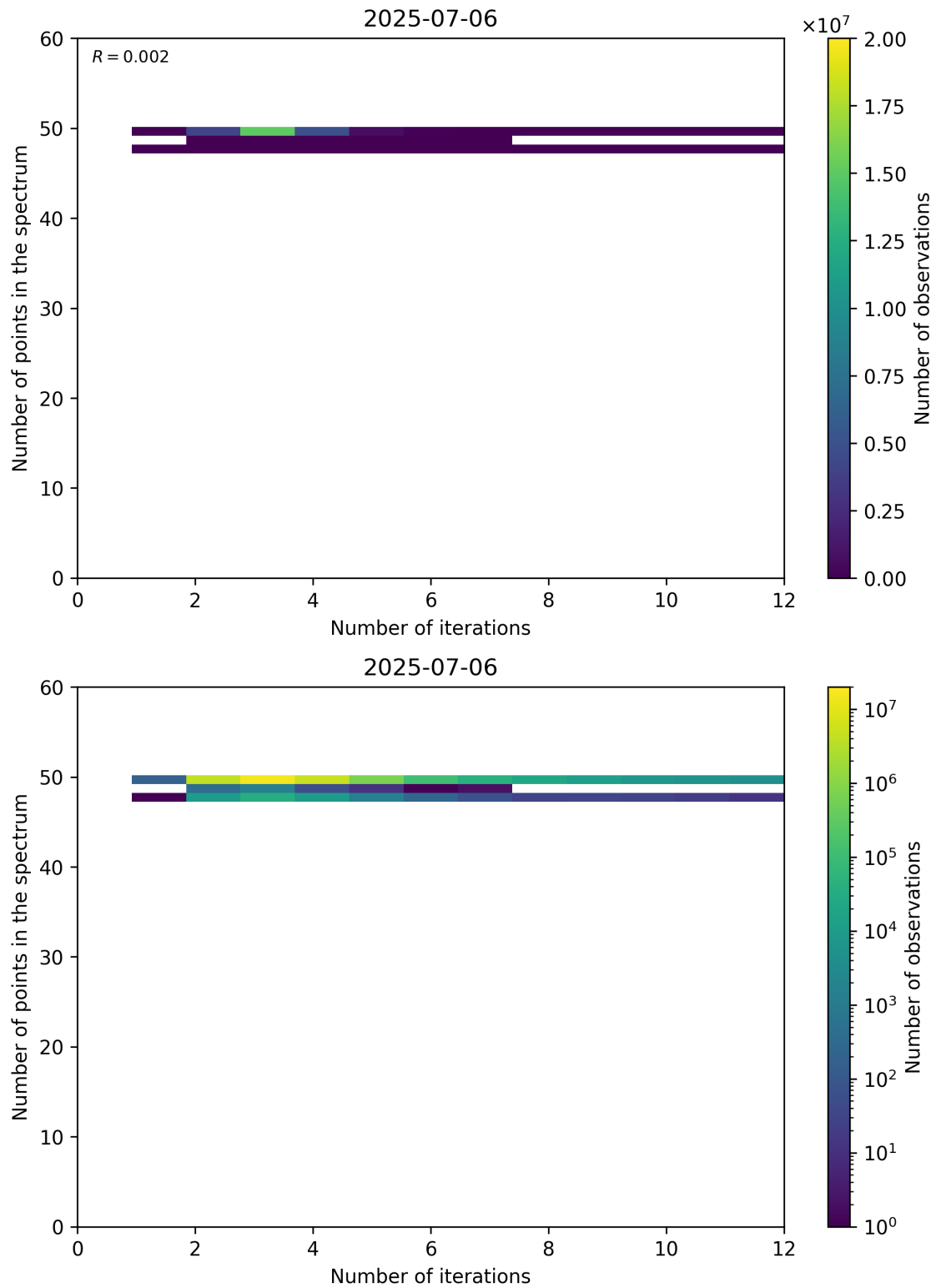
Figure 99: Scatter density plot of “Number of iterations” against “Number of points in the spectrum” for 2025-07-05 to 2025-07-07.
