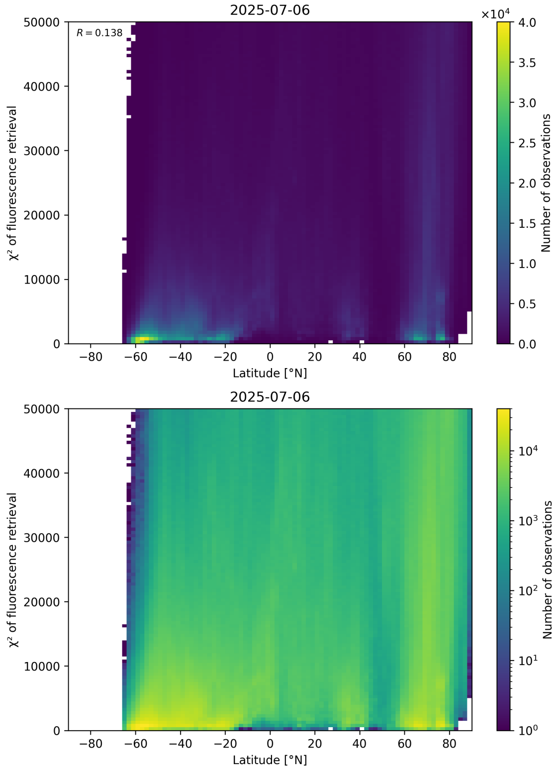
Figure 89: Scatter density plot of “Latitude” against “ \chi^2 of fluorescence retrieval” for 2025-07-05 to 2025-07-07.
