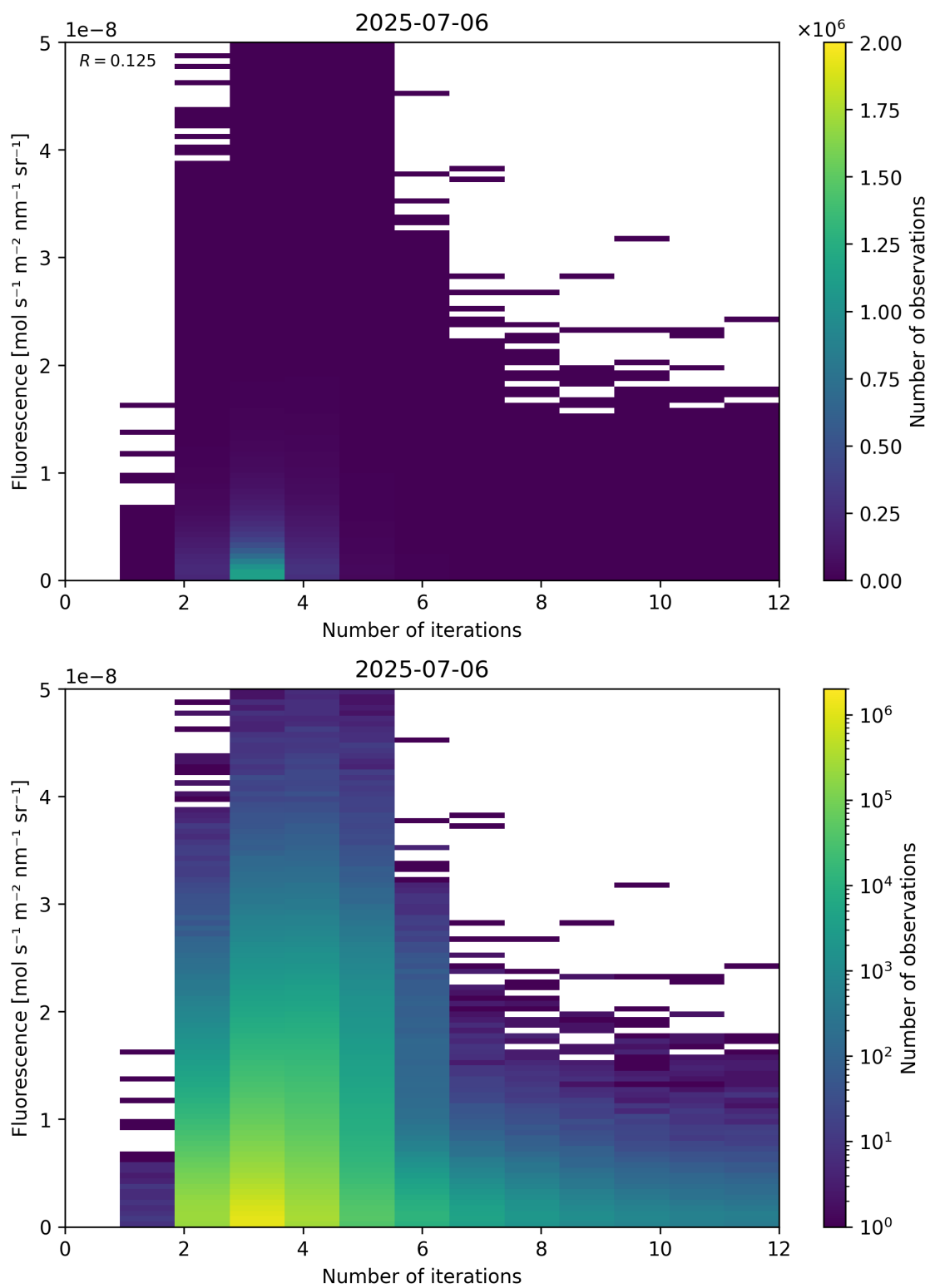
Figure 98: Scatter density plot of “Number of iterations” against “Fluorescence” for 2025-07-05 to 2025-07-07.
