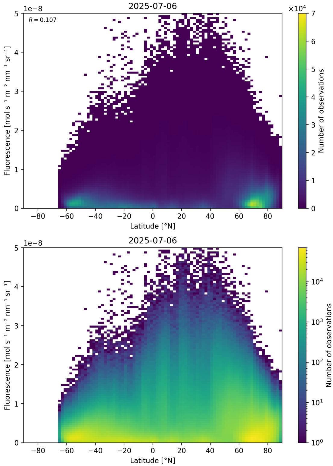
Figure 92: Scatter density plot of “Latitude” against “Fluorescence” for 2025-07-05 to 2025-07-07.
