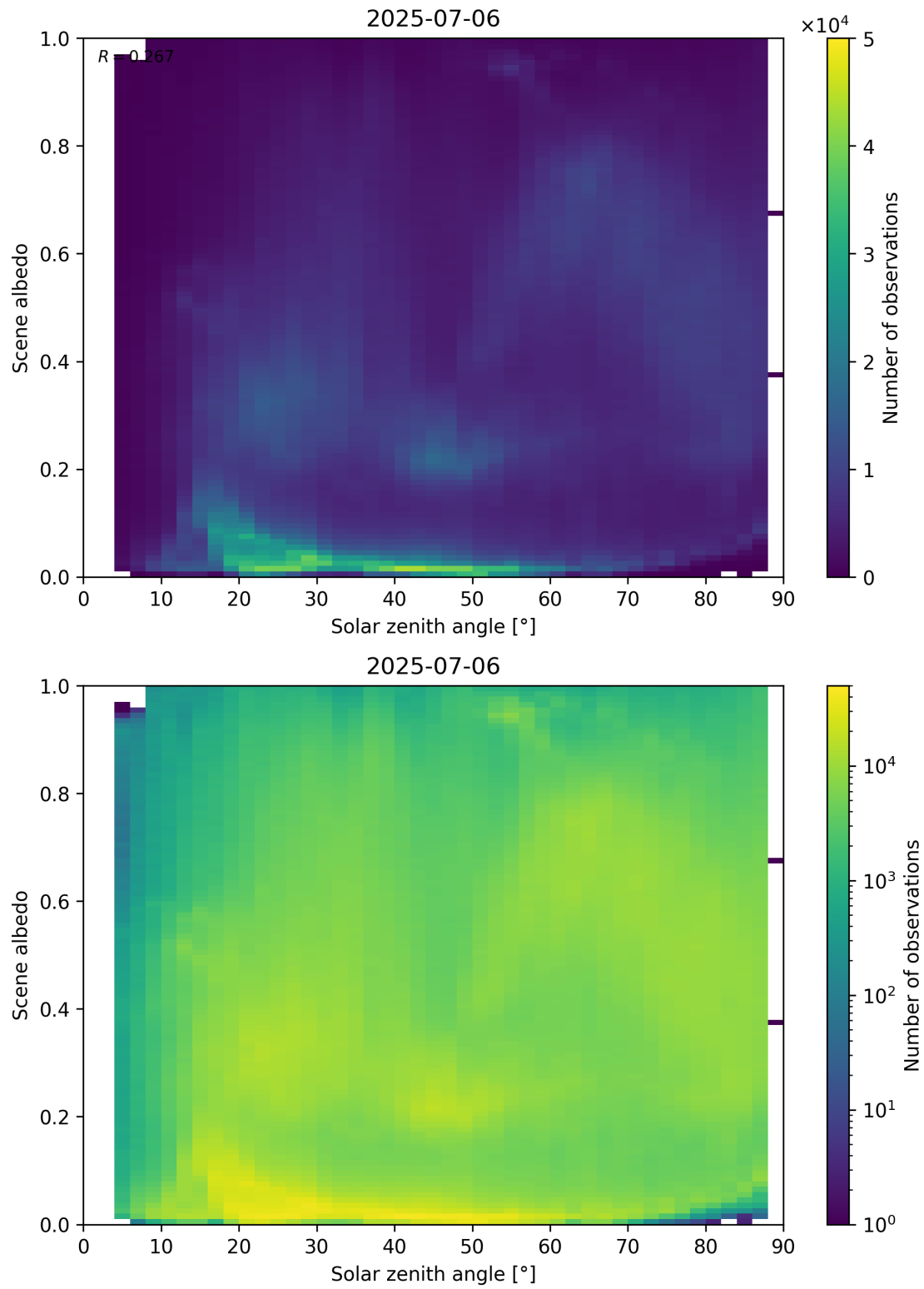
Figure 116: Scatter density plot of “Solar zenith angle” against “Scene albedo” for 2025-07-05 to 2025-07-07.
