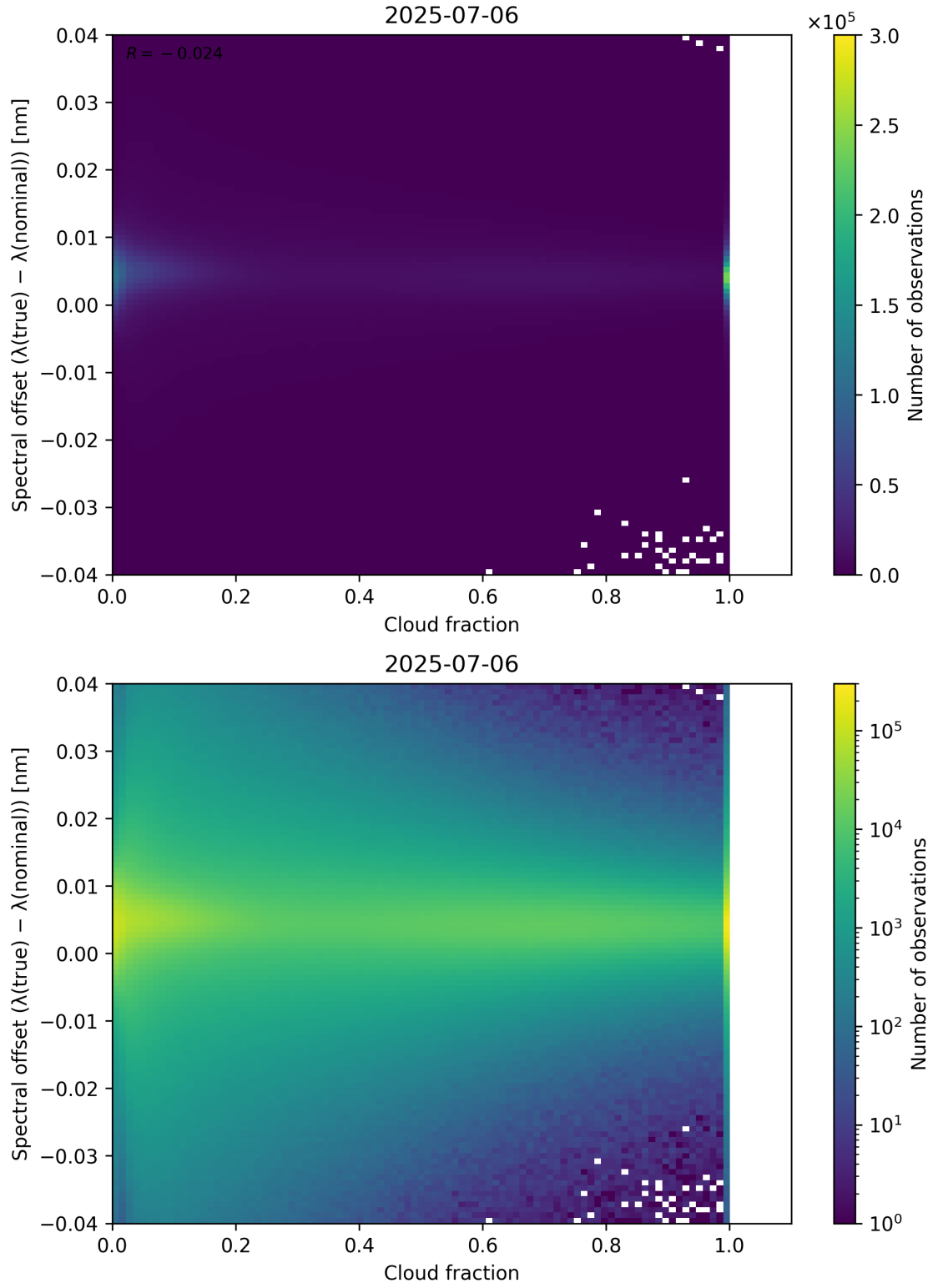
Figure 76: Scatter density plot of “Cloud fraction” against “Spectral offset ( \lambda_{\text{true}} - \lambda_{\text{nominal}} )” for 2025-07-05 to 2025-07-07.
