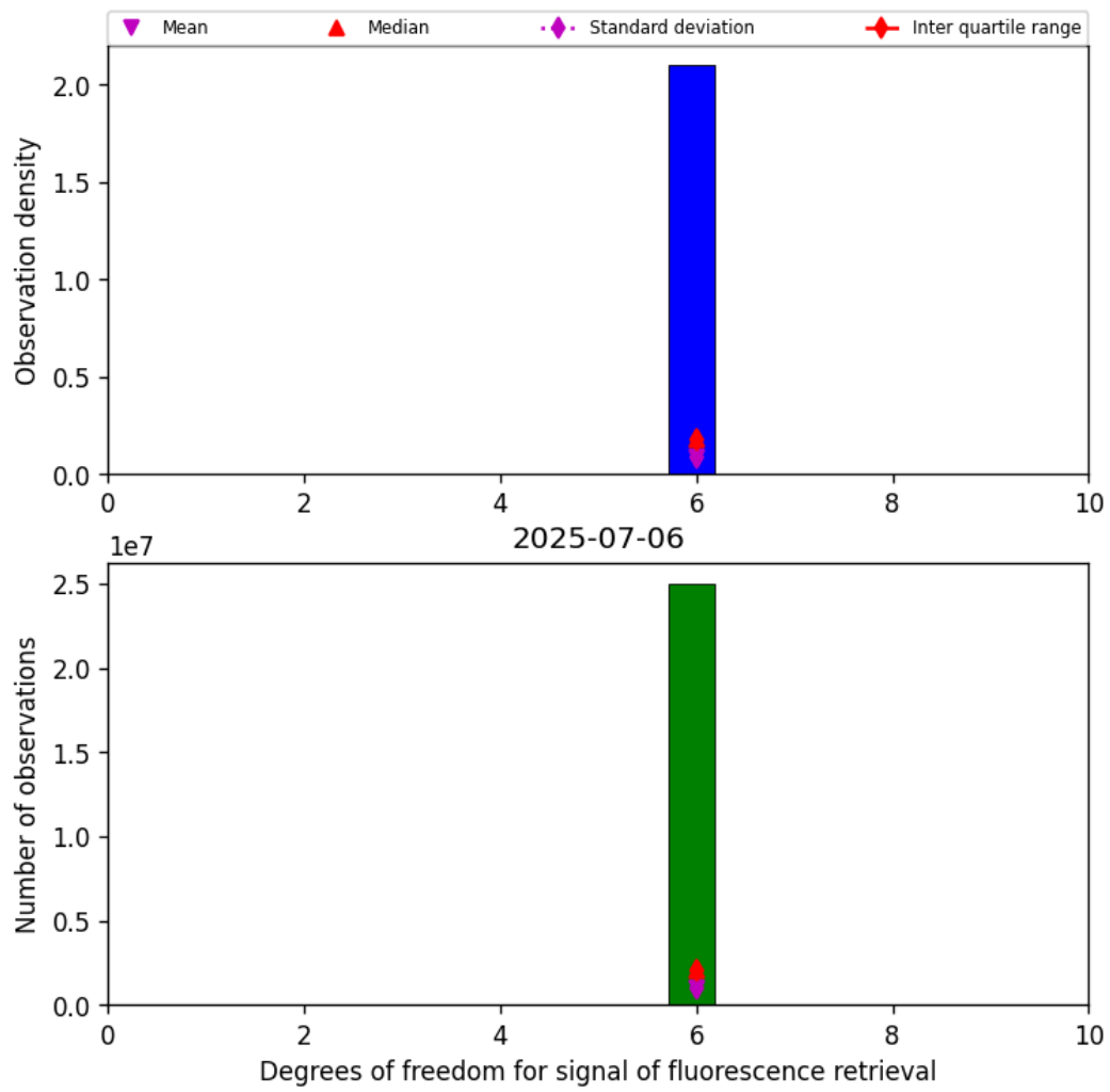
Figure 43: Histogram of “Degrees of freedom for signal of fluorescence retrieval” for 2025-07-05 to 2025-07-07
