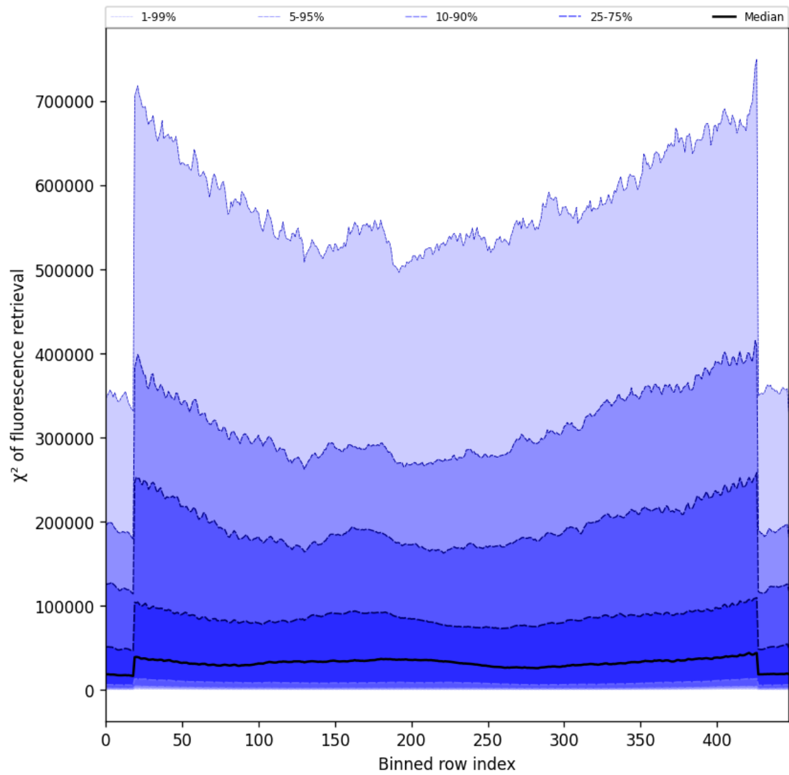
Figure 59: Along track statistics of “ \chi^2 of fluorescence retrieval” for 2025-07-05 to 2025-07-07
