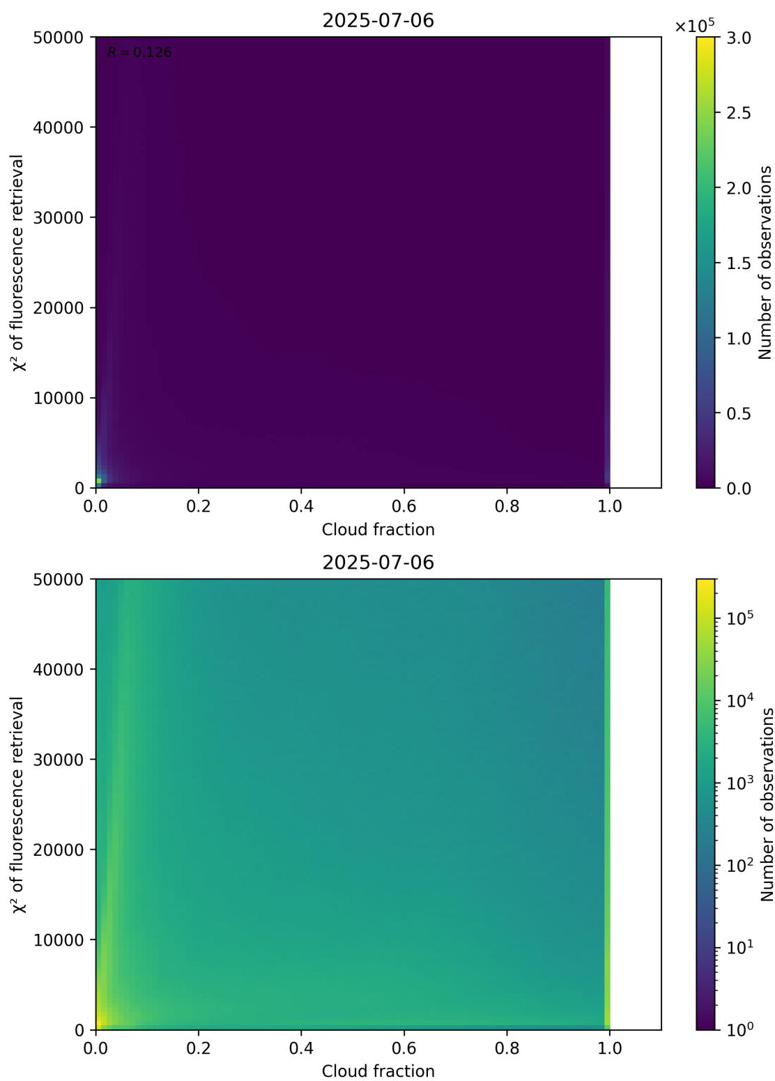
Figure 71: Scatter density plot of “Cloud fraction” against “ \chi^2 of fluorescence retrieval” for 2025-07-05 to 2025-07-07.
