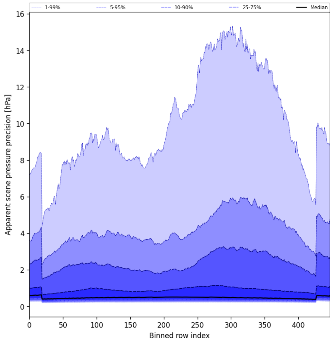
Figure 54: Along track statistics of “Apparent scene pressure precision” for 2025-07-05 to 2025-07-07
