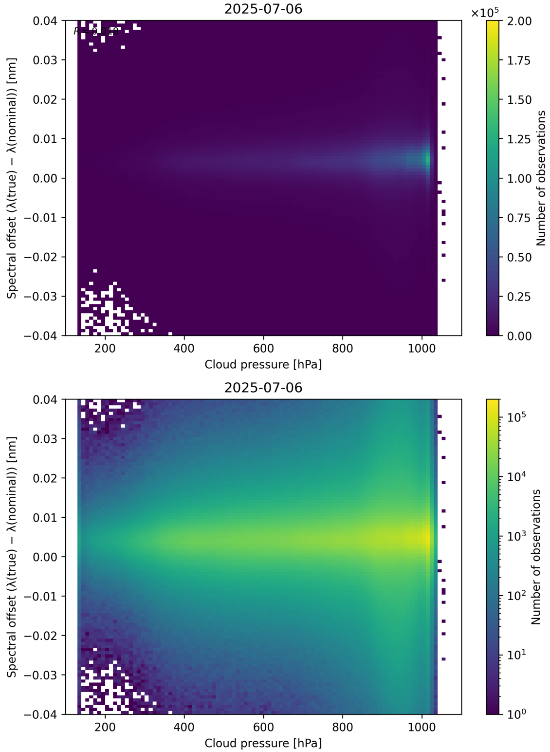
Figure 84: Scatter density plot of “Cloud pressure” against “Spectral offset ( \lambda_{\text{true}} - \lambda_{\text{nominal}} )” for 2025-07-05 to 2025-07-07.
