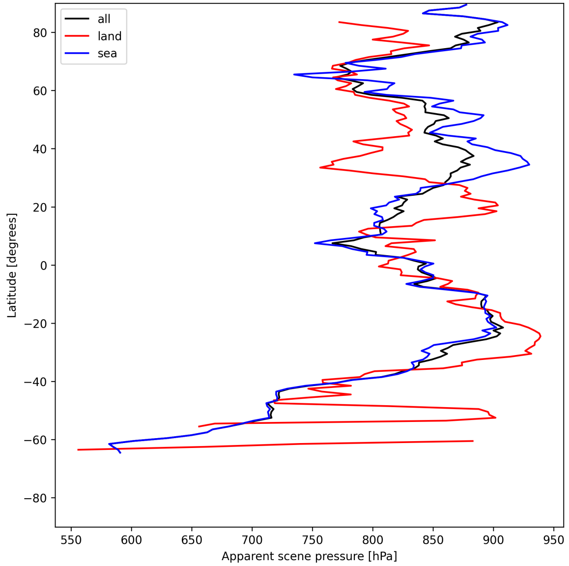
Figure 19: Zonal average of “Apparent scene pressure” for 2025-07-05 to 2025-07-07.
