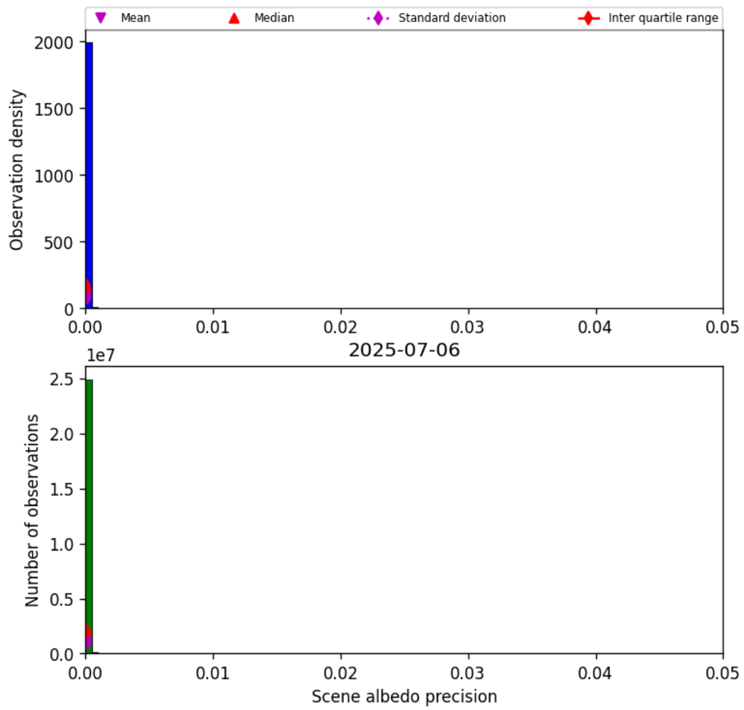
Figure 35: Histogram of “Scene albedo precision” for 2025-07-05 to 2025-07-07
