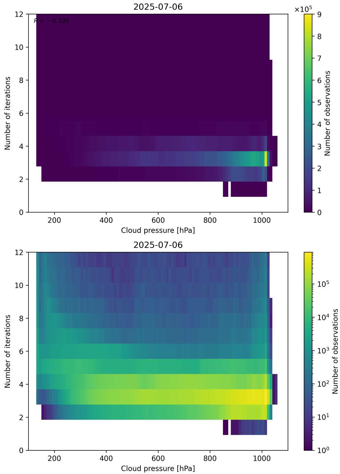
Figure 81: Scatter density plot of “Cloud pressure” against “Number of iterations” for 2025-07-05 to 2025-07-07.
