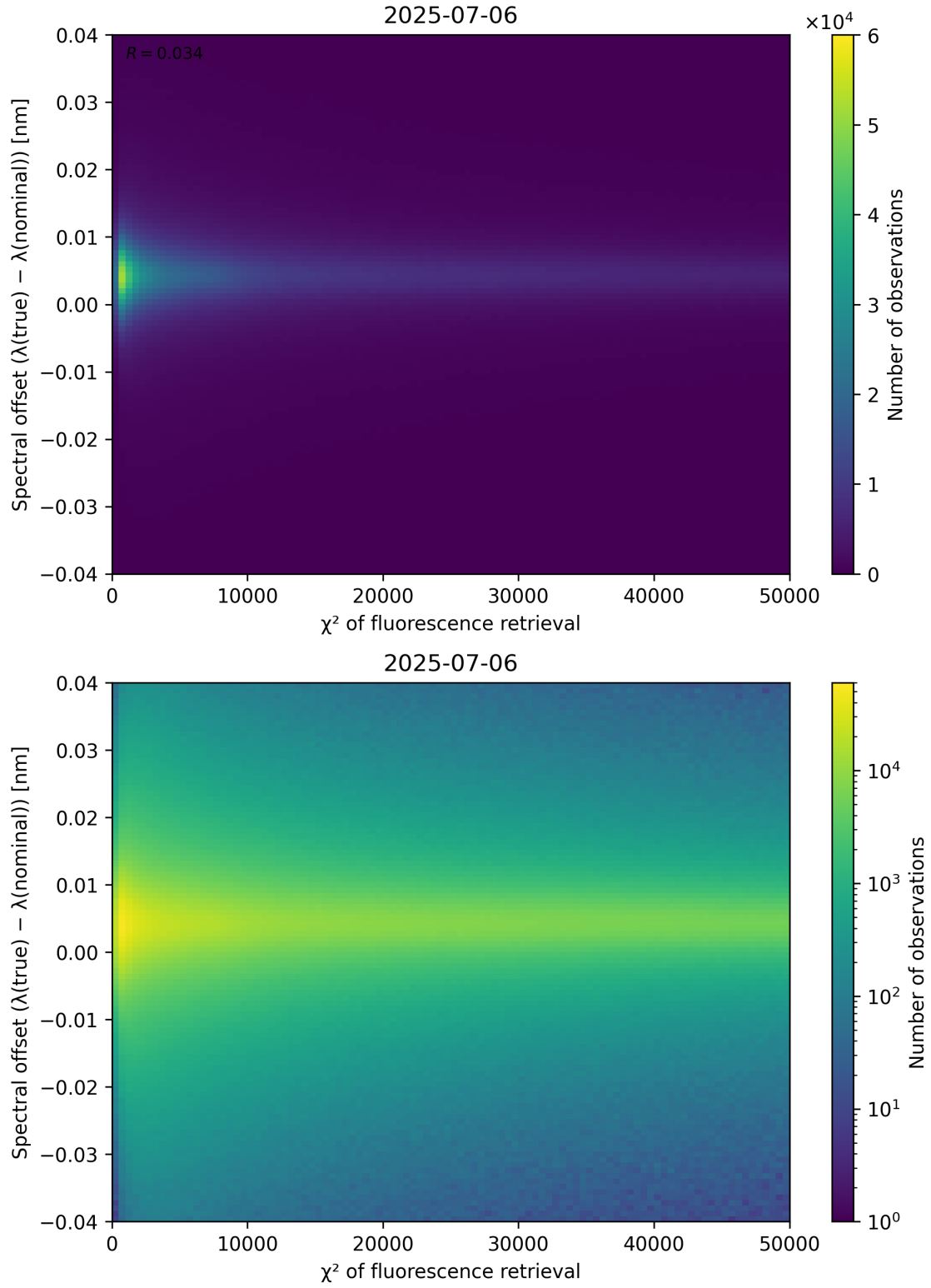
Figure 69: Scatter density plot of “ \chi^2 of fluorescence retrieval” against “Spectral offset ( \lambda_{\text{true}} - \lambda_{\text{nominal}} )” for 2025-07-05 to 2025-07-07.
