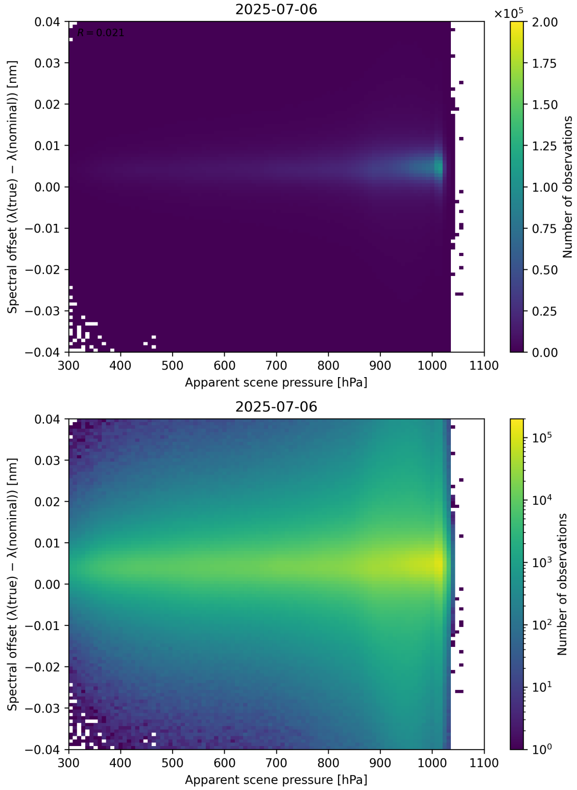
Figure 67: Scatter density plot of “Apparent scene pressure” against “Spectral offset ( \lambda_{\text{true}} - \lambda_{\text{nominal}} )” for 2025-07-05 to 2025-07-07.
