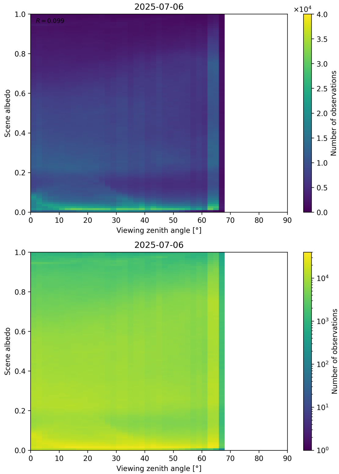
Figure 126: Scatter density plot of “Viewing zenith angle” against “Scene albedo” for 2025-07-05 to 2025-07-07.
