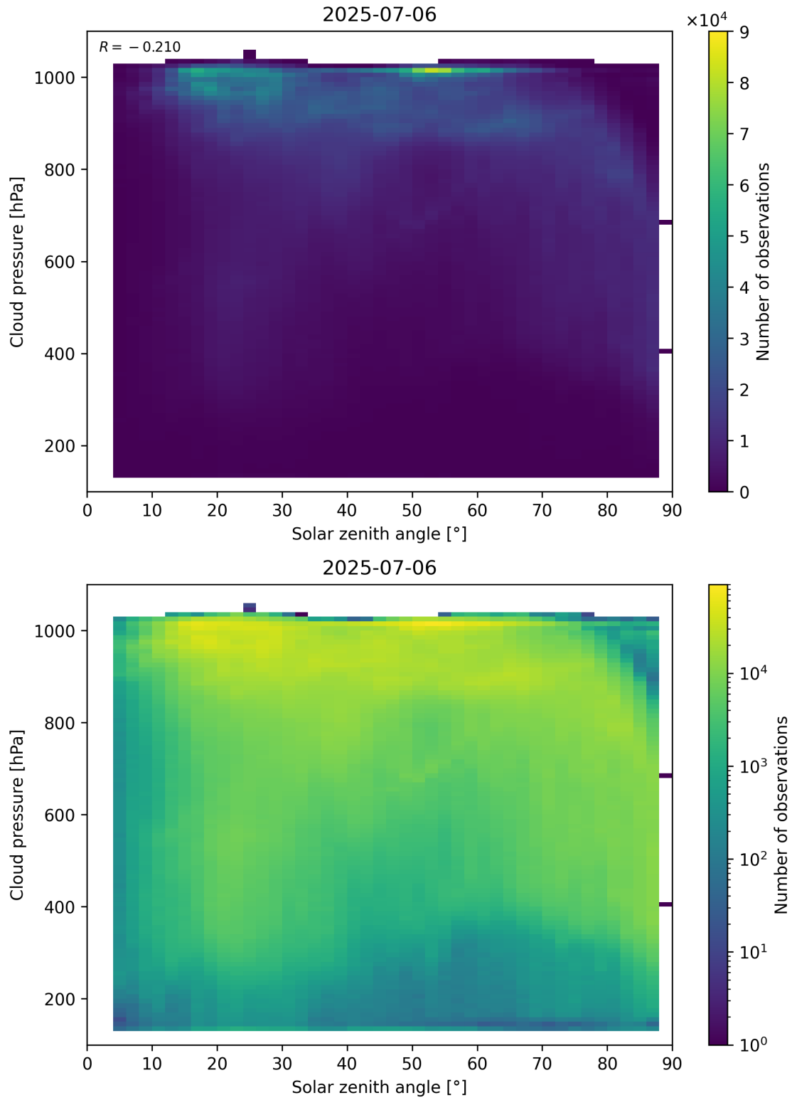
Figure 111: Scatter density plot of “Solar zenith angle” against “Cloud pressure” for 2025-07-05 to 2025-07-07.
