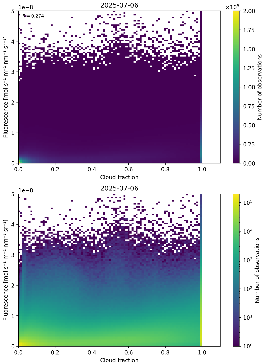
Figure 72: Scatter density plot of “Cloud fraction” against “Fluorescence” for 2025-07-05 to 2025-07-07.
