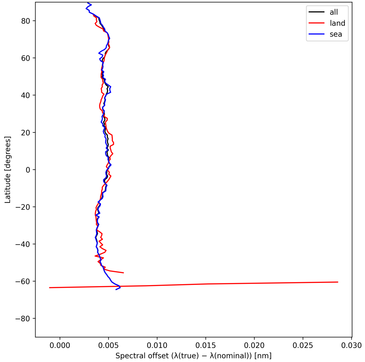
Figure 28: Zonal average of “Spectral offset ( \lambda_{\text{true}} - \lambda_{\text{nominal}} )” for 2025-07-05 to 2025-07-07.
