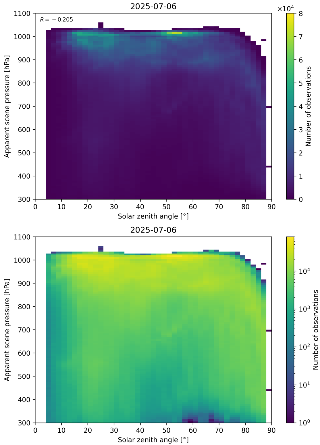
Figure 108: Scatter density plot of “Solar zenith angle” against “Apparent scene pressure” for 2025-07-05 to 2025-07-07.
