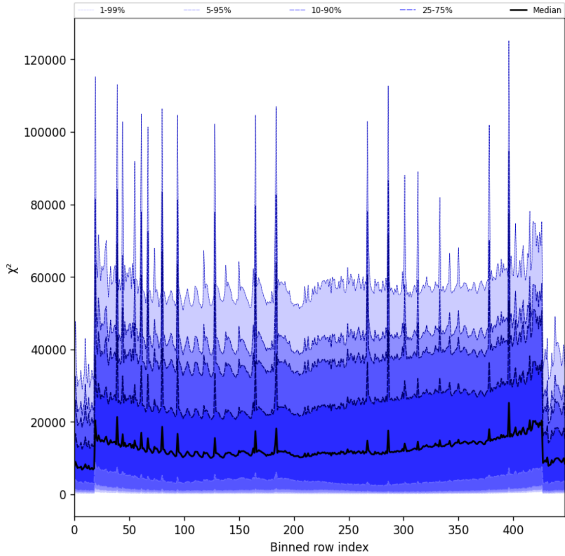
Figure 55: Along track statistics of “ \chi^2 ” for 2025-07-05 to 2025-07-07
