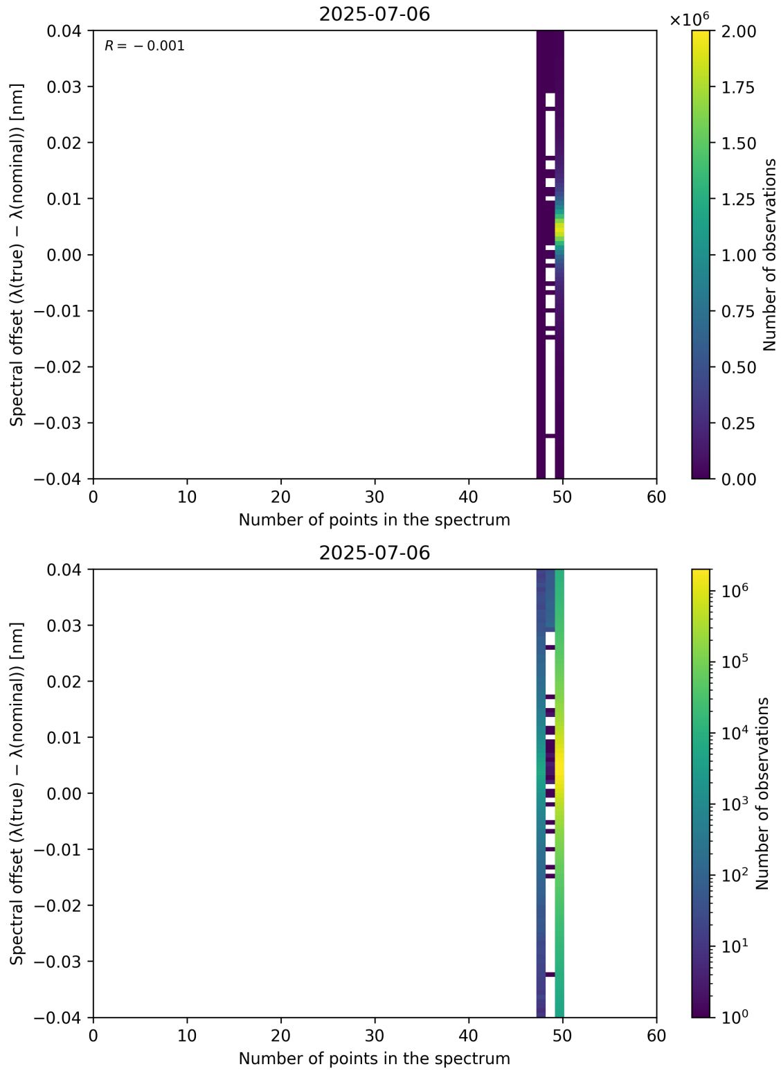
Figure 101: Scatter density plot of “Number of points in the spectrum” against “Spectral offset ( \lambda_{\text{true}} - \lambda_{\text{nominal}} )” for 2025-07-05 to 2025-07-07.
