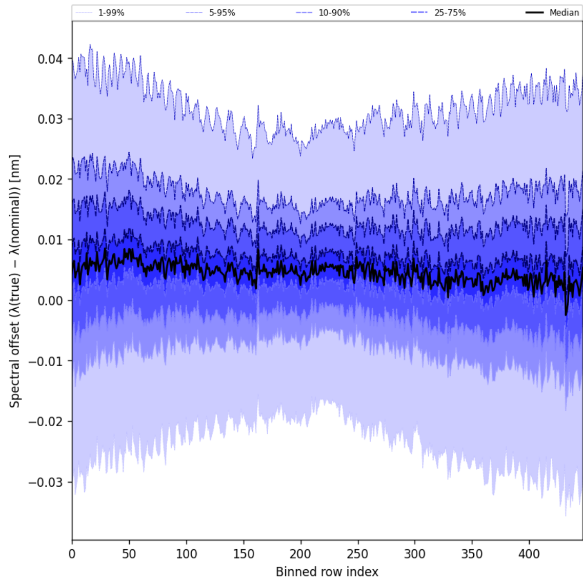
Figure 62: Along track statistics of “Spectral offset ( \lambda_{\text{true}} - \lambda_{\text{nominal}} )” for 2025-07-05 to 2025-07-07
