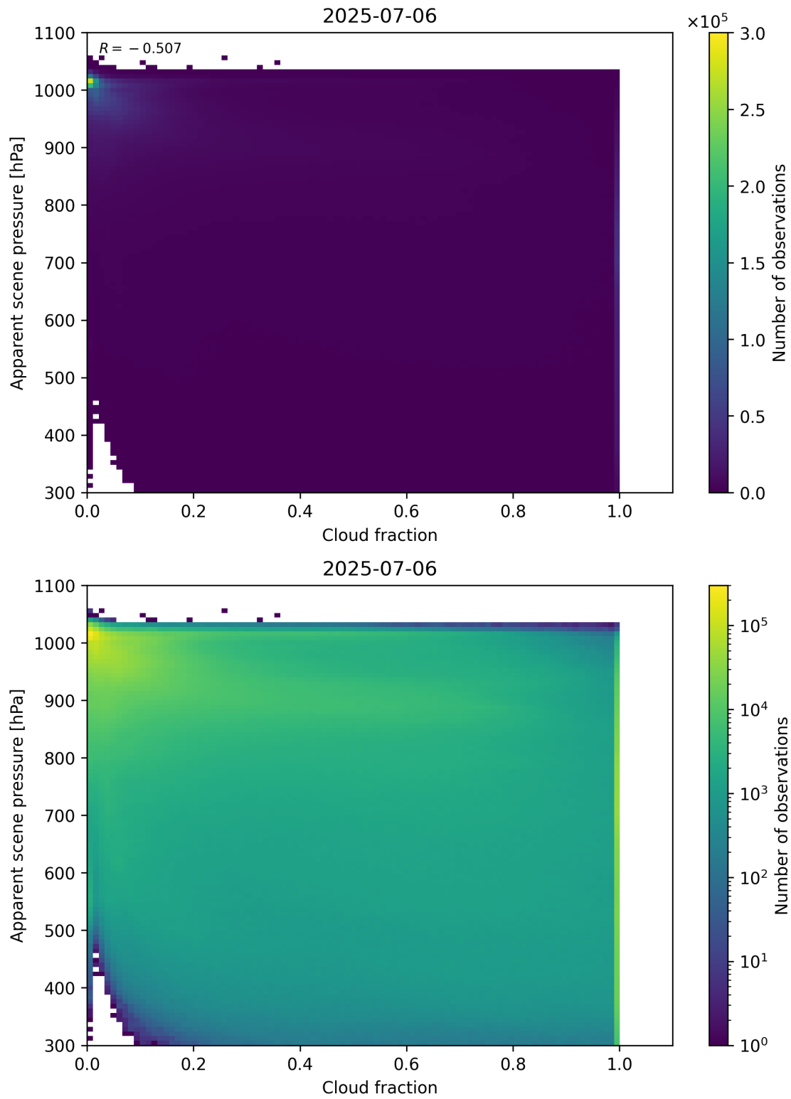
Figure 70: Scatter density plot of “Cloud fraction” against “Apparent scene pressure” for 2025-07-05 to 2025-07-07.
