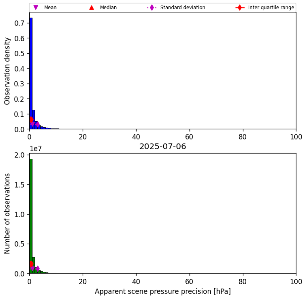
Figure 37: Histogram of “Apparent scene pressure precision” for 2025-07-05 to 2025-07-07
