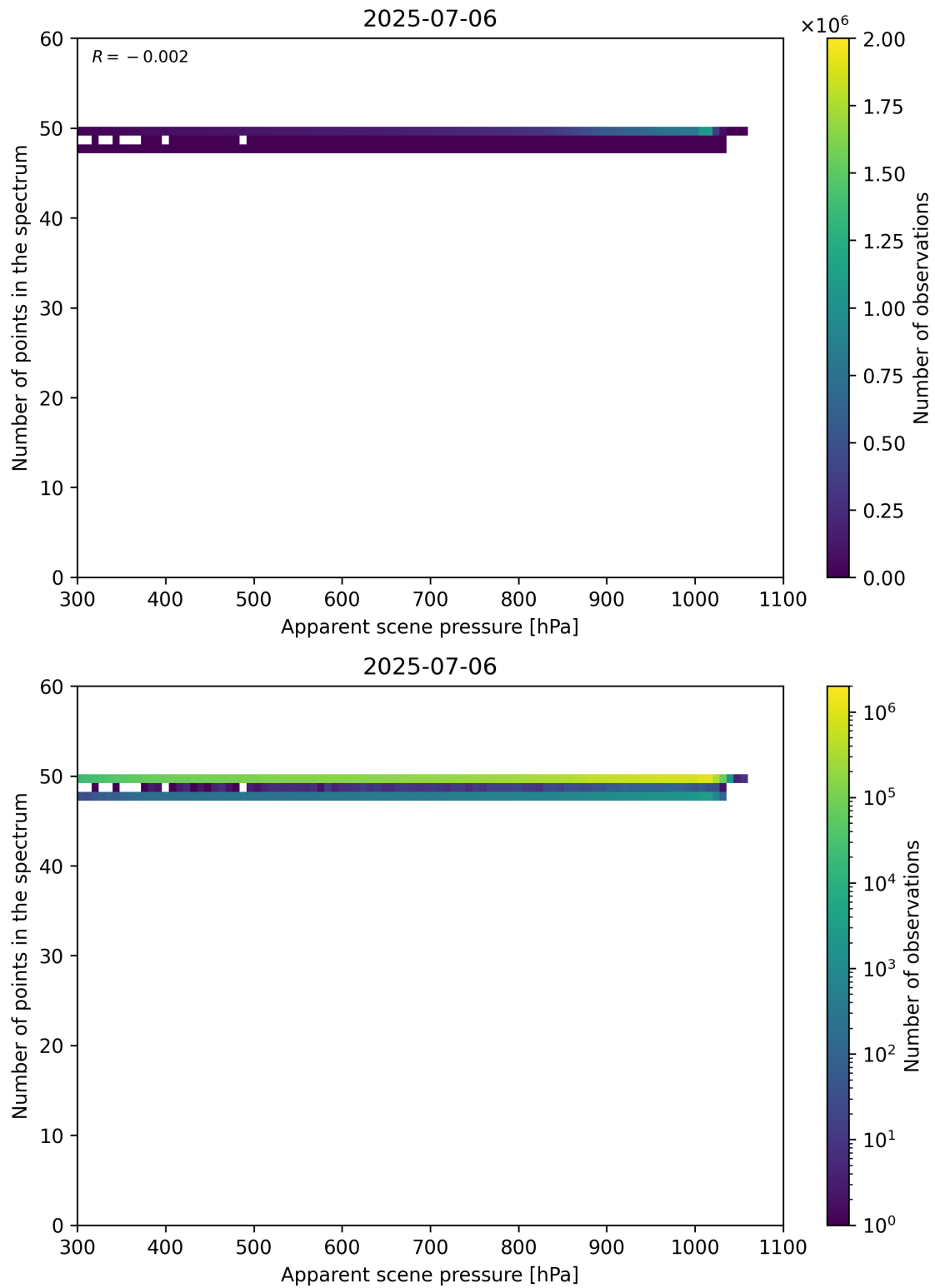
Figure 66: Scatter density plot of “Apparent scene pressure” against “Number of points in the spectrum” for 2025-07-05 to 2025-07-07.
