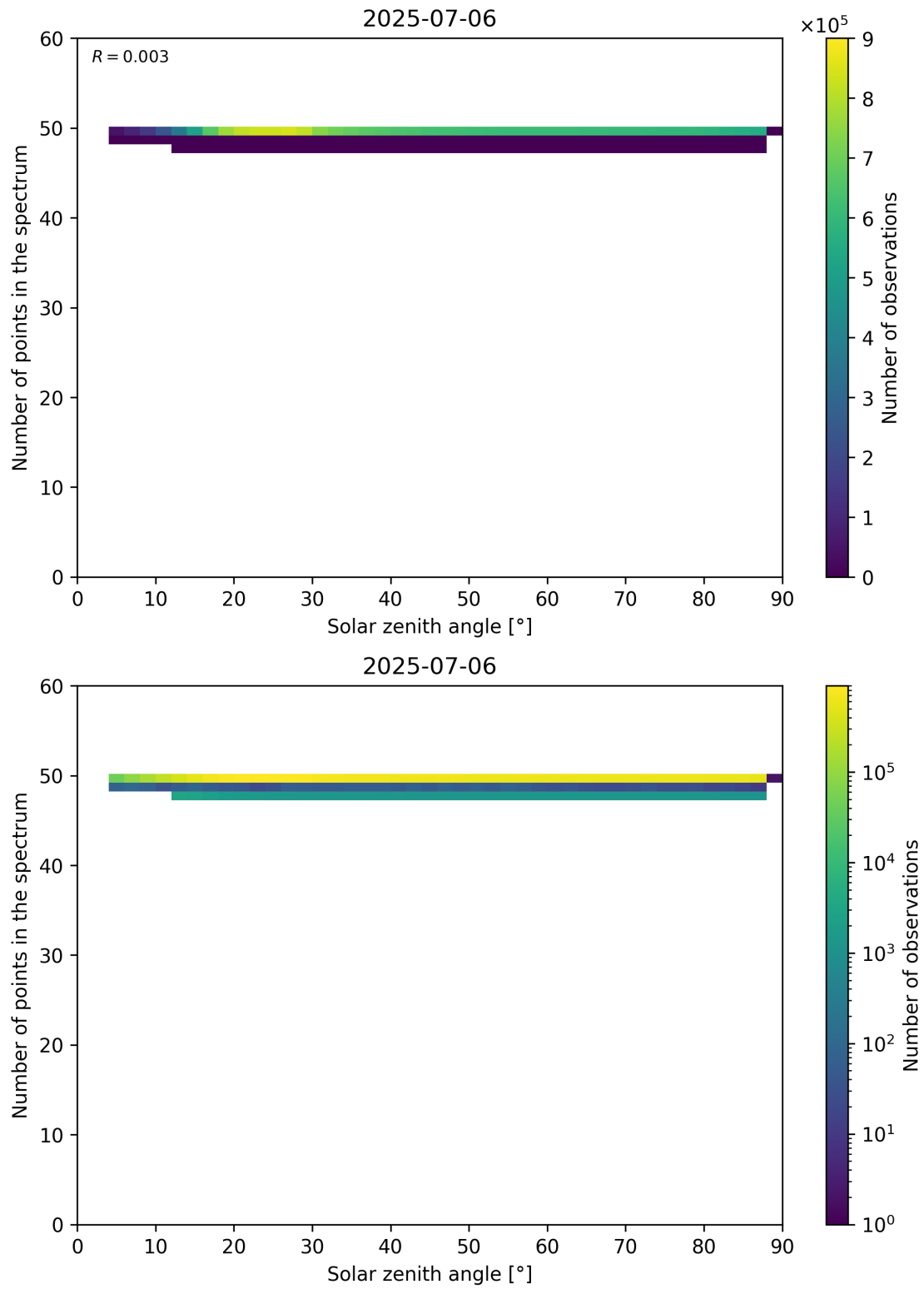
Figure 115: Scatter density plot of “Solar zenith angle” against “Number of points in the spectrum” for 2025-07-05 to 2025-07-07.
