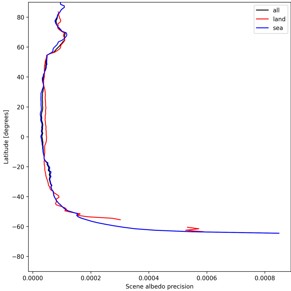
Figure 18: Zonal average of “Scene albedo precision” for 2025-07-05 to 2025-07-07.
