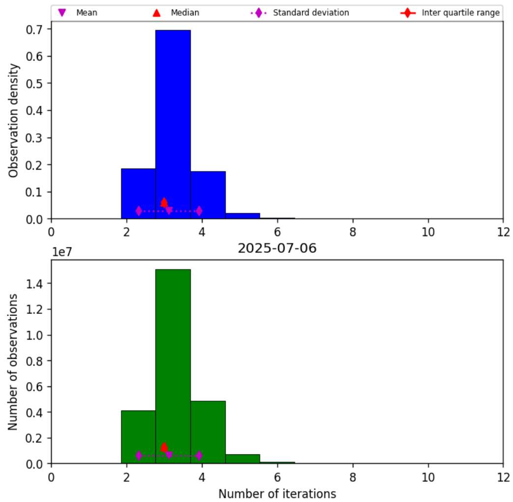
Figure 39: Histogram of “Number of iterations” for 2025-07-05 to 2025-07-07
