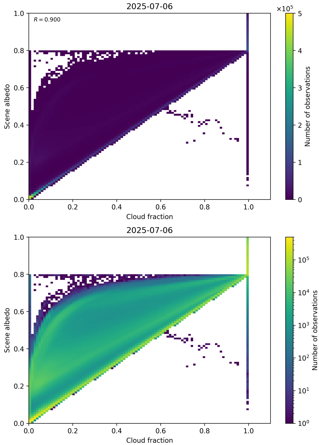
Figure 75: Scatter density plot of “Cloud fraction” against “Scene albedo” for 2025-07-05 to 2025-07-07.
