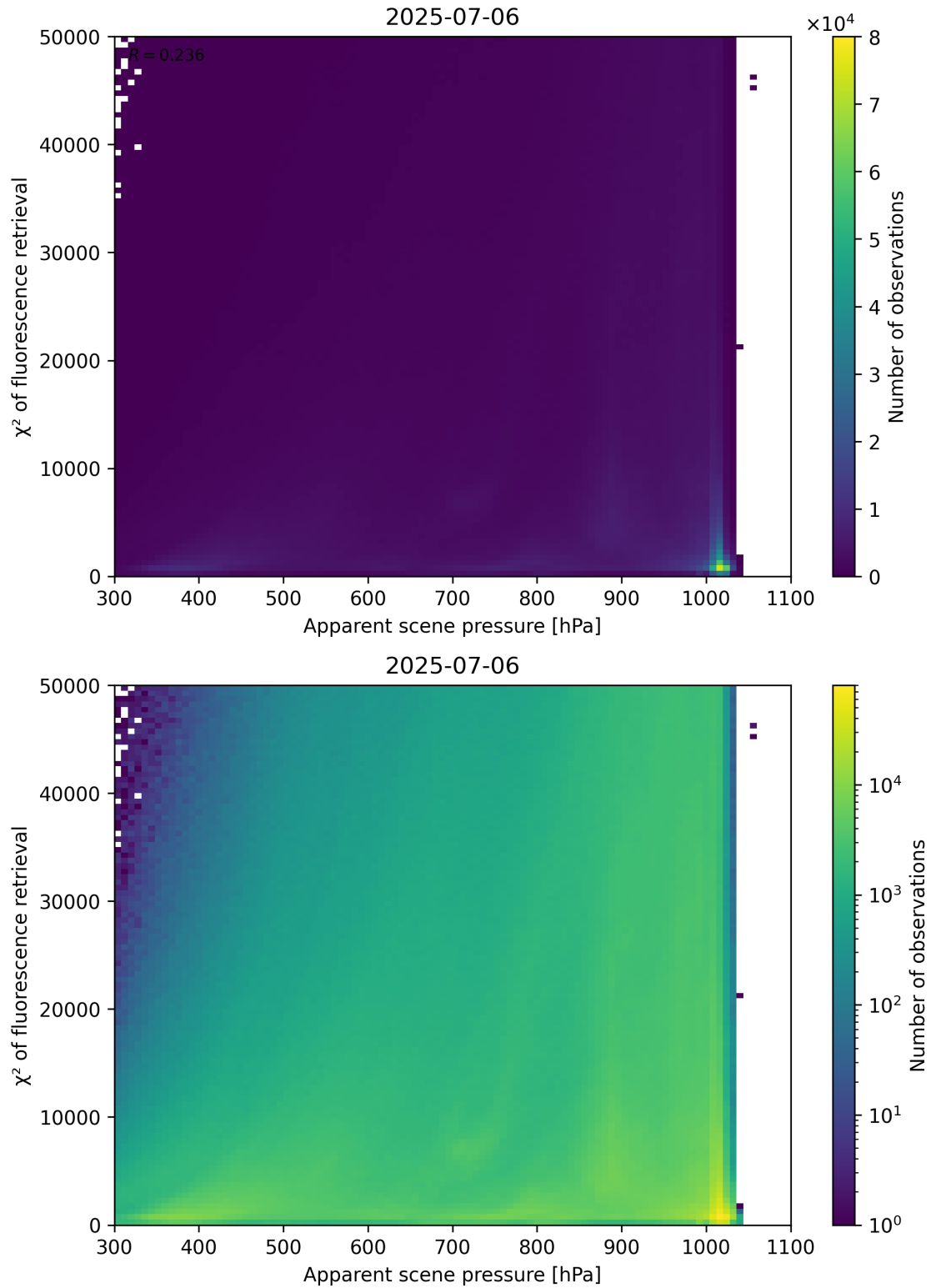
Figure 63: Scatter density plot of “Apparent scene pressure” against “ \chi^2 of fluorescence retrieval” for 2025-07-05 to 2025-07-07.
