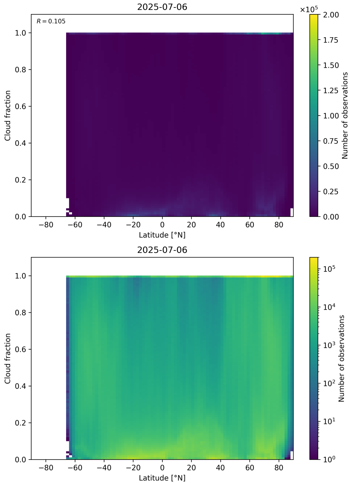
Figure 90: Scatter density plot of “Latitude” against “Cloud fraction” for 2025-07-05 to 2025-07-07.
