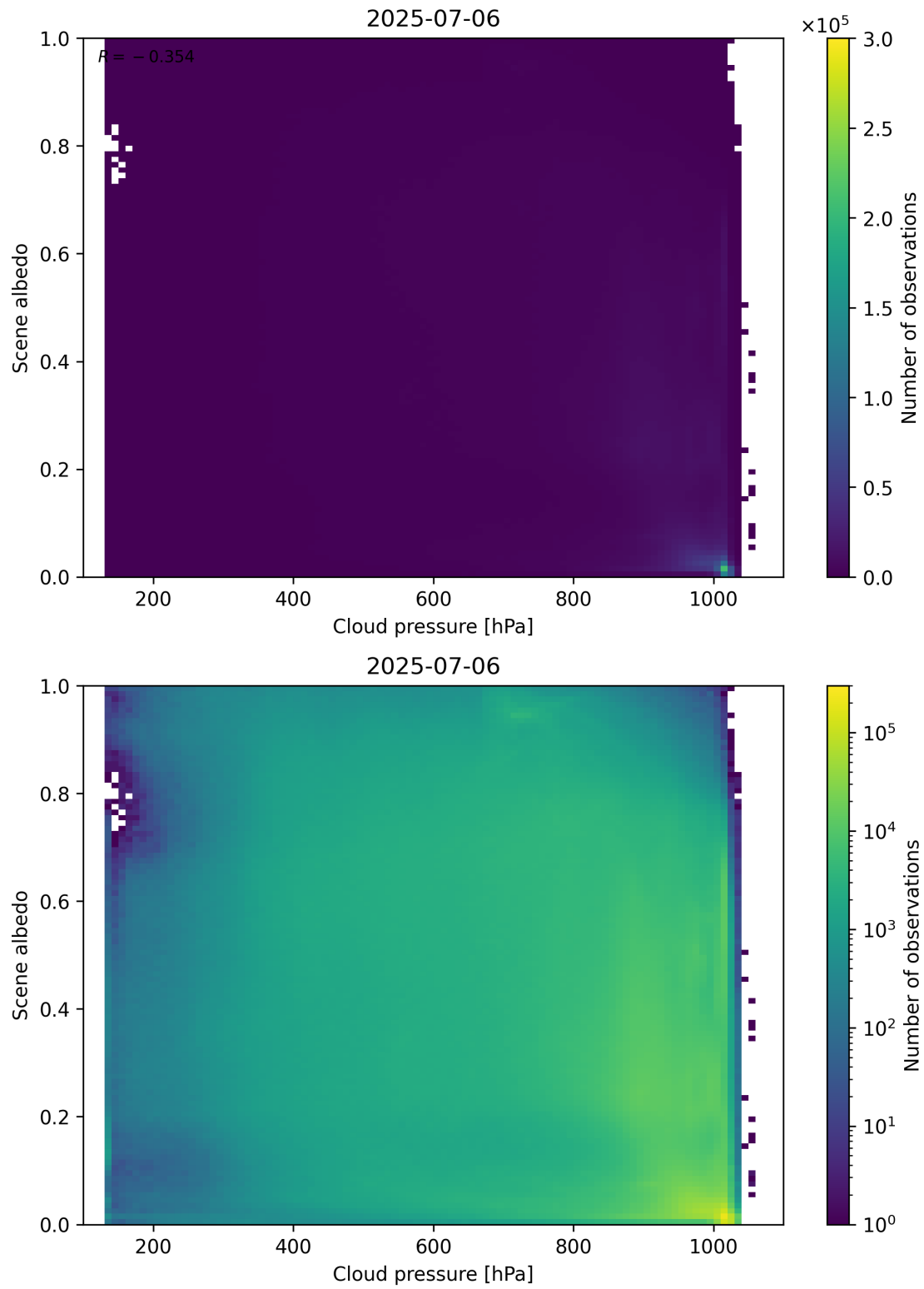
Figure 83: Scatter density plot of “Cloud pressure” against “Scene albedo” for 2025-07-05 to 2025-07-07.
