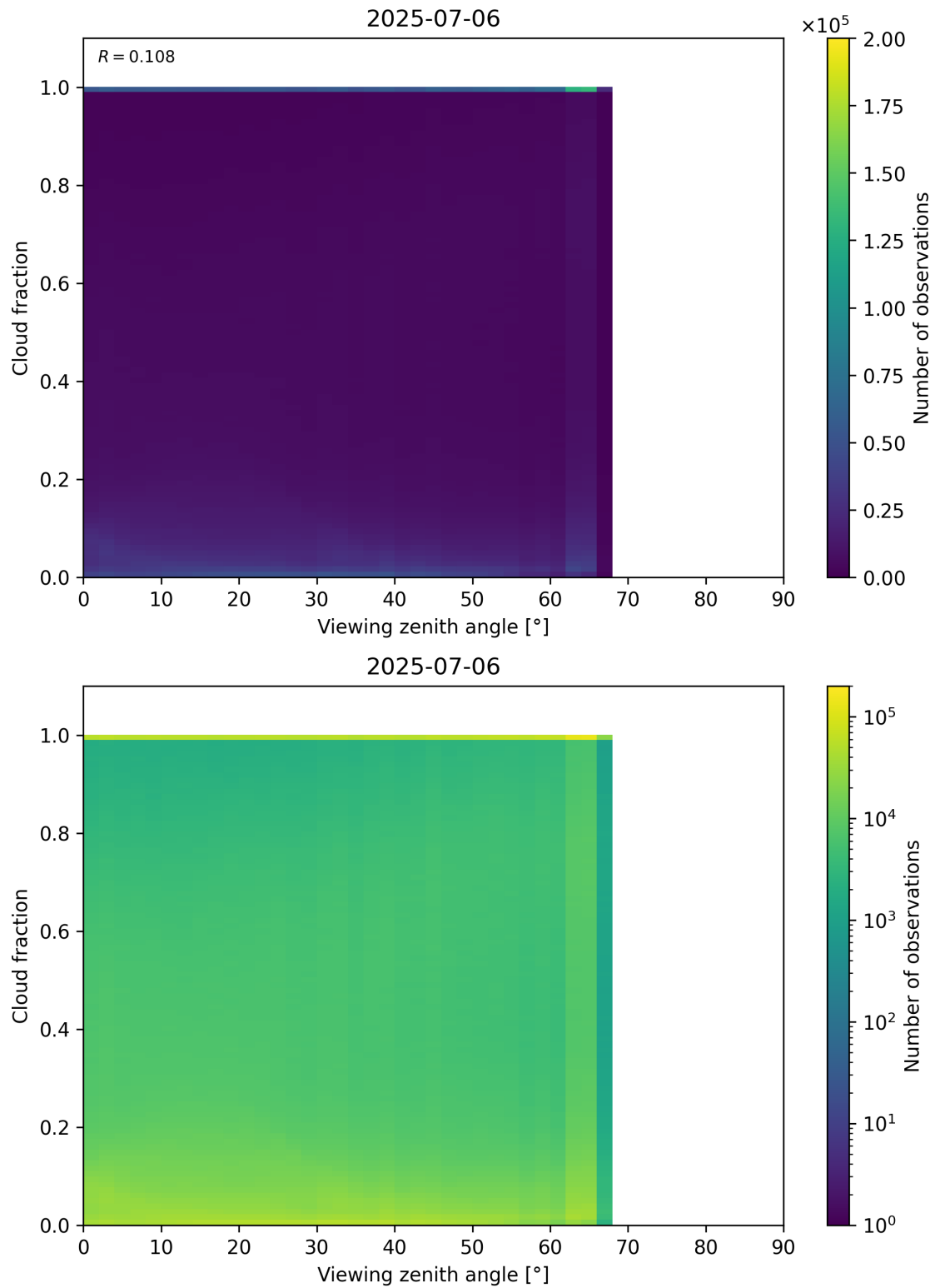
Figure 120: Scatter density plot of “Viewing zenith angle” against “Cloud fraction” for 2025-07-05 to 2025-07-07.
