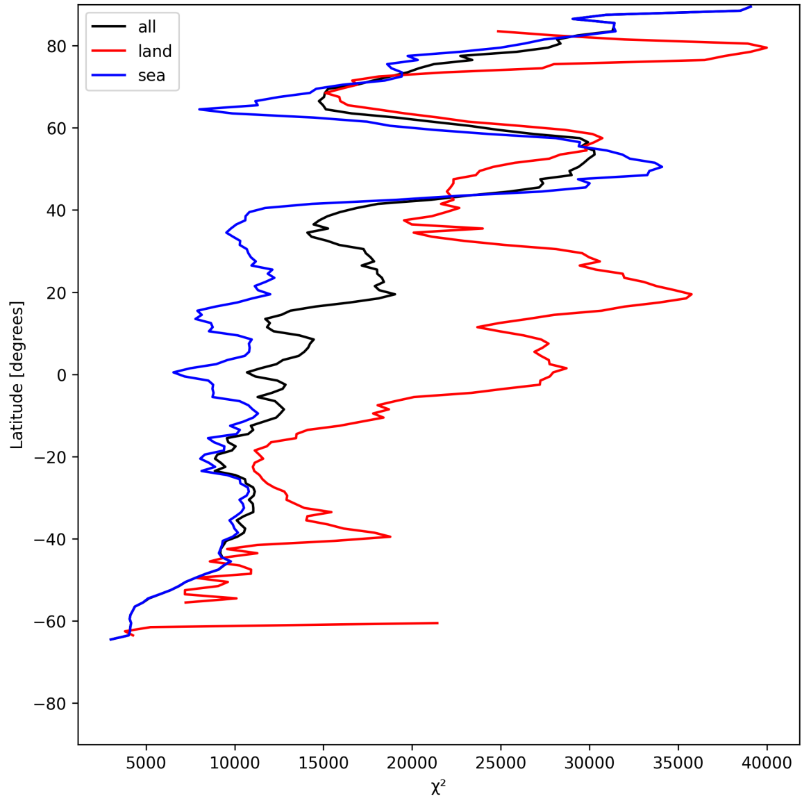
Figure 21: Zonal average of “ \chi^2 ” for 2025-07-05 to 2025-07-07.
