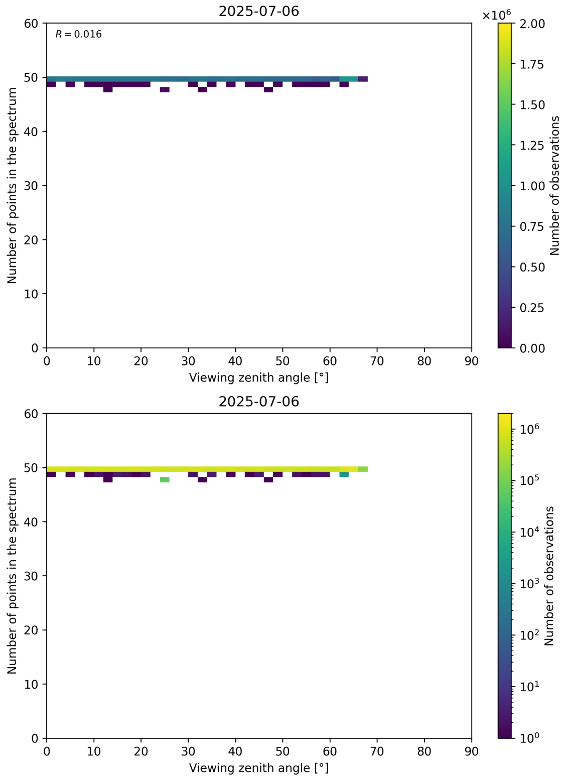
Figure 125: Scatter density plot of “Viewing zenith angle” against “Number of points in the spectrum” for 2025-07-05 to 2025-07-07.
