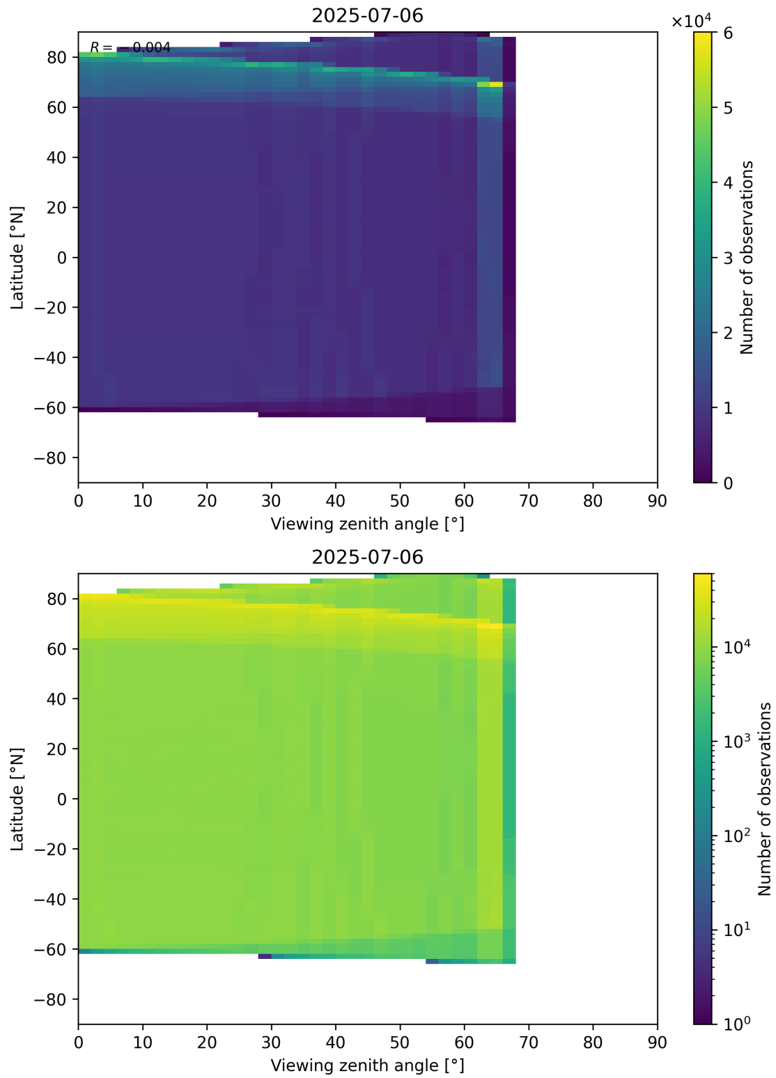
Figure 123: Scatter density plot of “Viewing zenith angle” against “Latitude” for 2025-07-05 to 2025-07-07.
