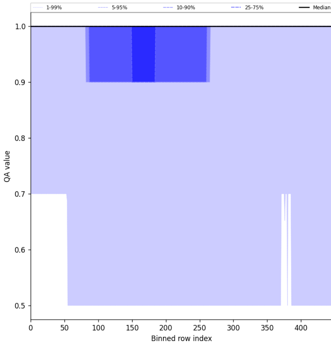
Figure 46: Along track statistics of “QA value” for 2025-07-05 to 2025-07-07
