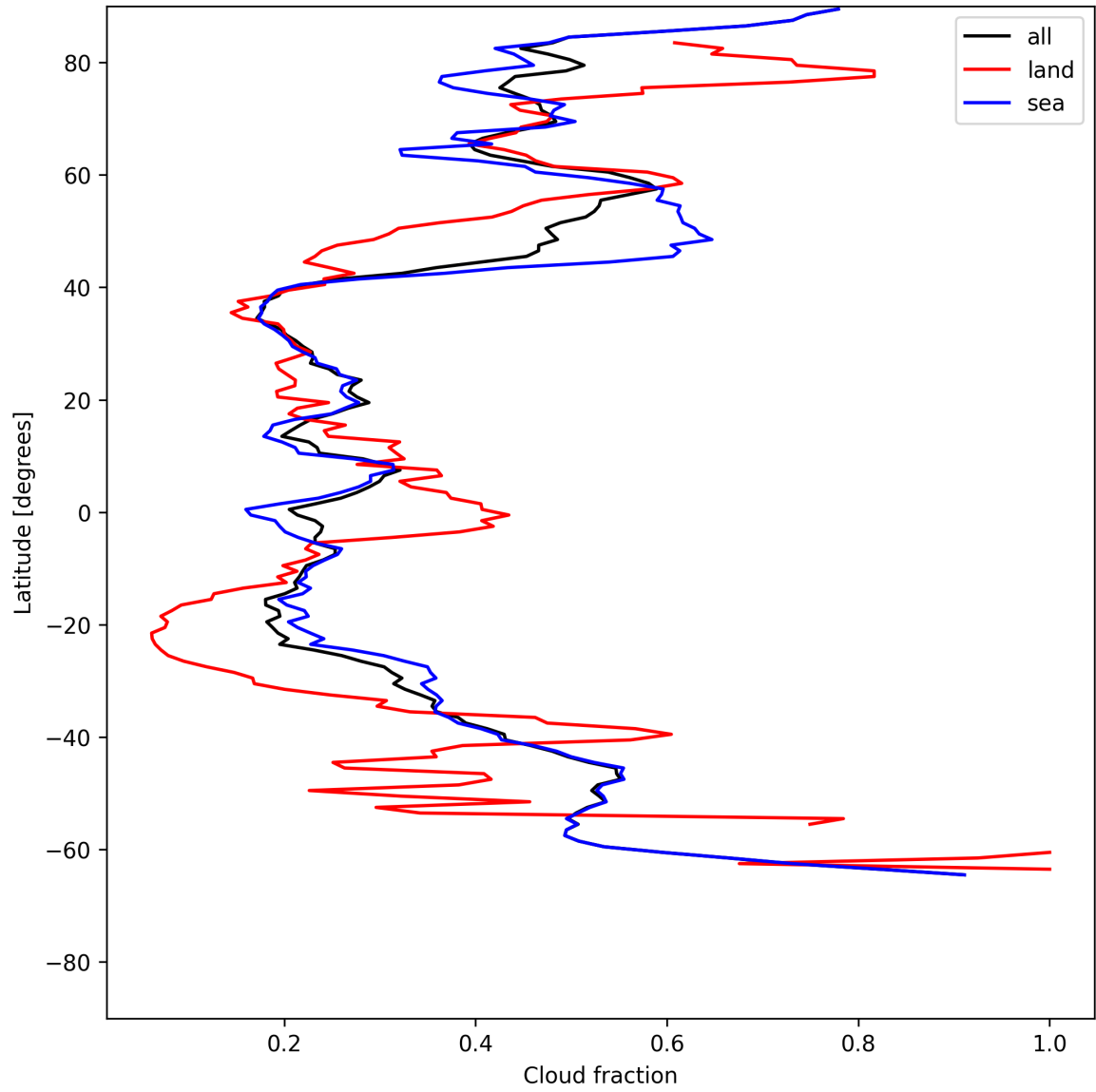
Figure 15: Zonal average of “Cloud fraction” for 2025-07-05 to 2025-07-07.
