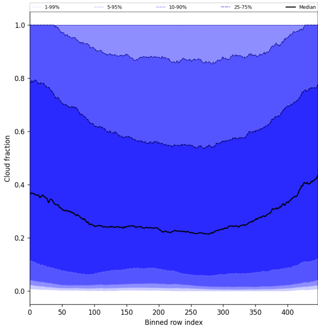
Figure 49: Along track statistics of “Cloud fraction” for 2025-07-05 to 2025-07-07
