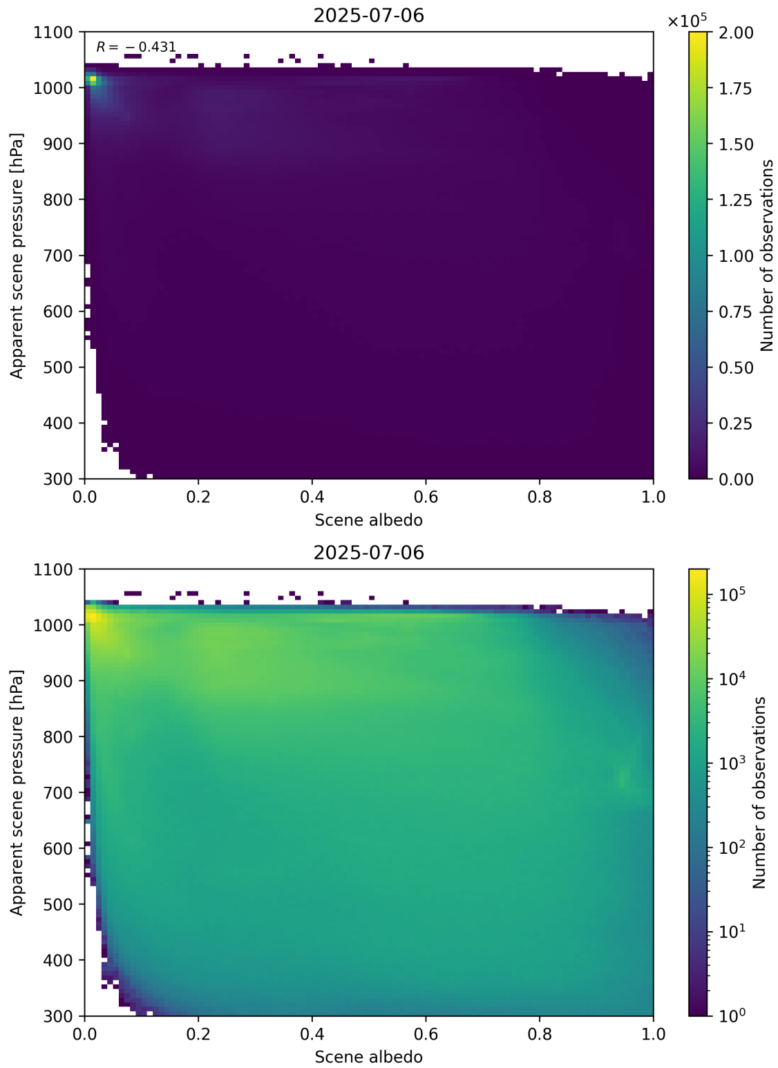
Figure 102: Scatter density plot of “Scene albedo” against “Apparent scene pressure” for 2025-07-05 to 2025-07-07.
