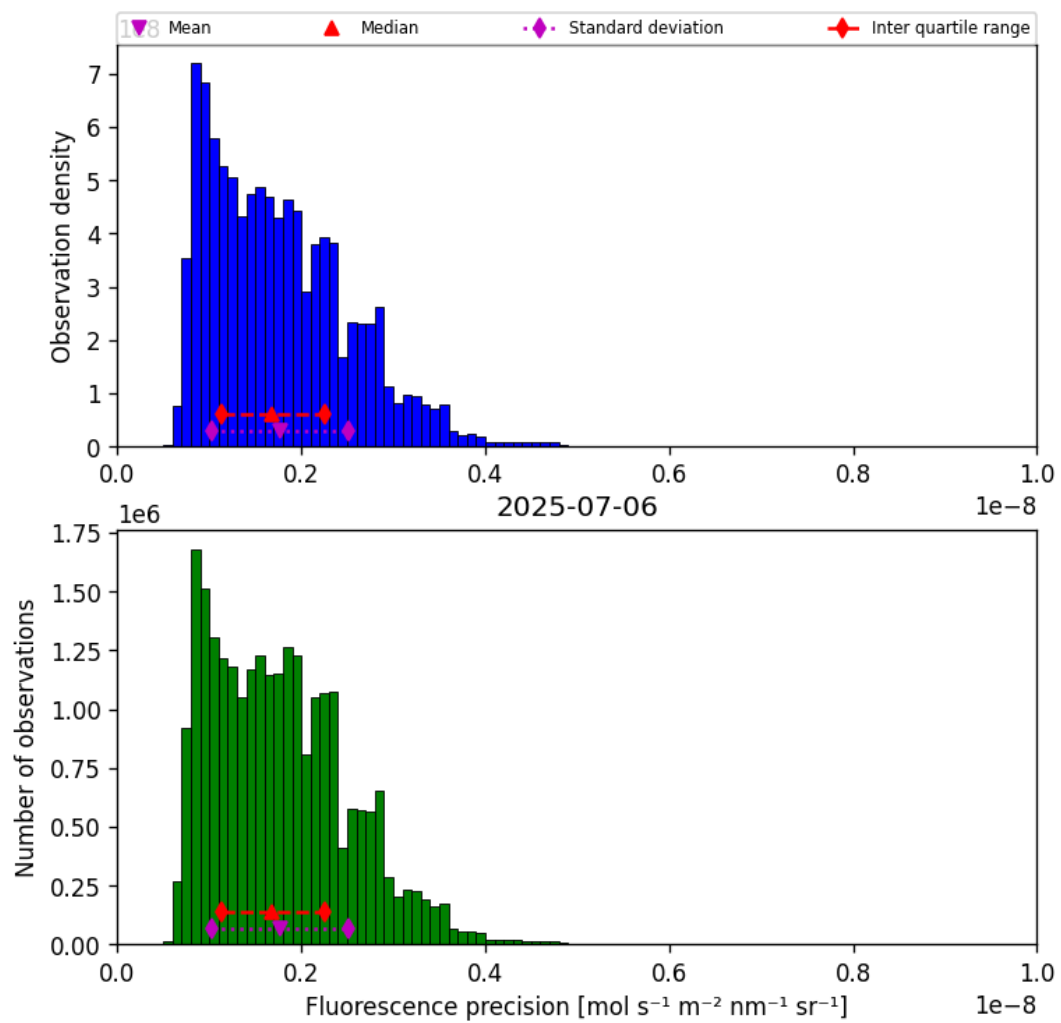
Figure 41: Histogram of “Fluorescence precision” for 2025-07-05 to 2025-07-07
