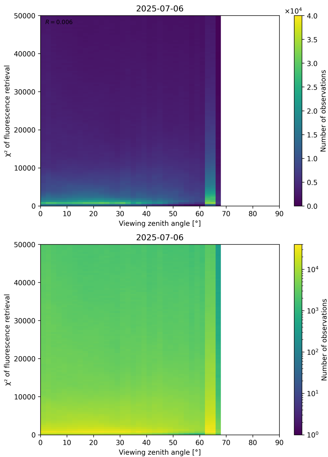
Figure 119: Scatter density plot of “Viewing zenith angle” against “ \chi^2 of fluorescence retrieval” for 2025-07-05 to 2025-07-07.
