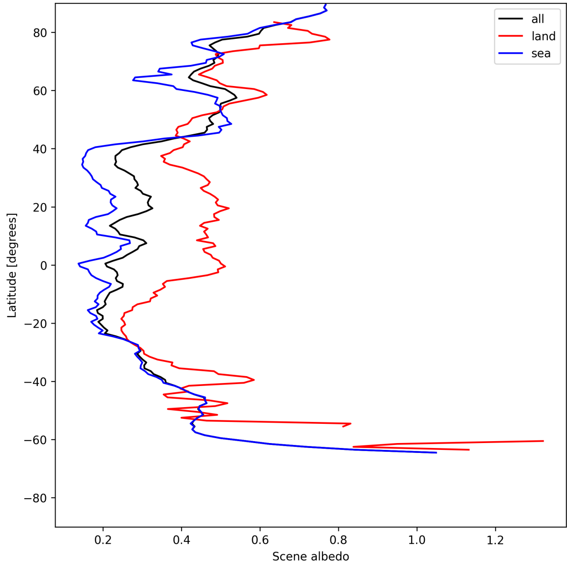
Figure 17: Zonal average of “Scene albedo” for 2025-07-05 to 2025-07-07.
