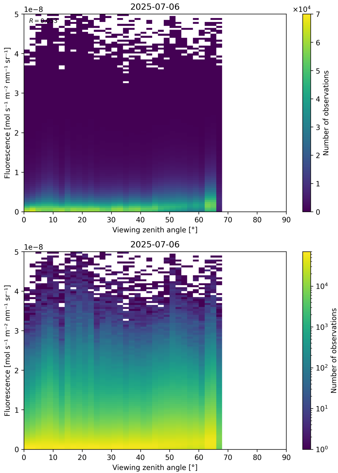
Figure 122: Scatter density plot of “Viewing zenith angle” against “Fluorescence” for 2025-07-05 to 2025-07-07.
