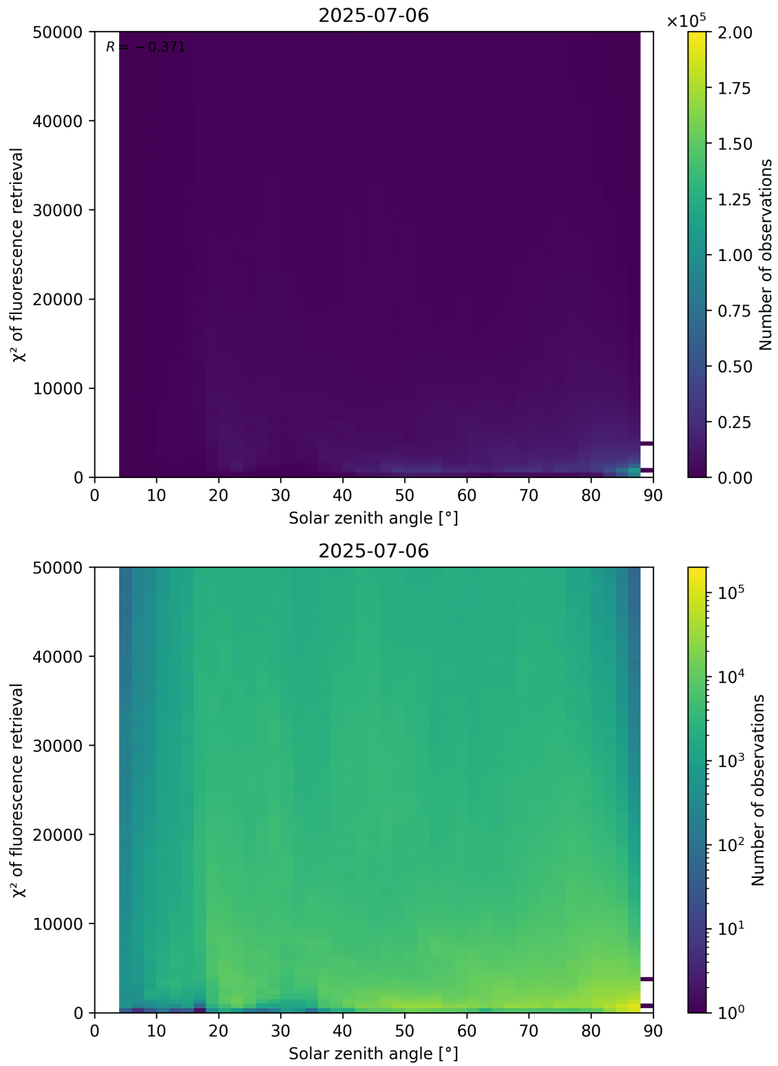
Figure 109: Scatter density plot of “Solar zenith angle” against “ \chi^2 of fluorescence retrieval” for 2025-07-05 to 2025-07-07.
