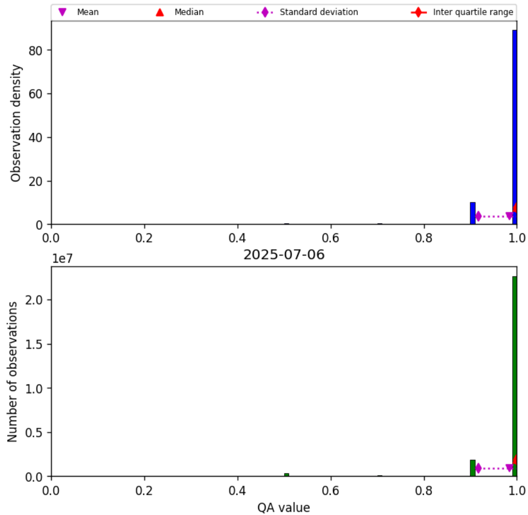
Figure 29: Histogram of “QA value” for 2025-07-05 to 2025-07-07
