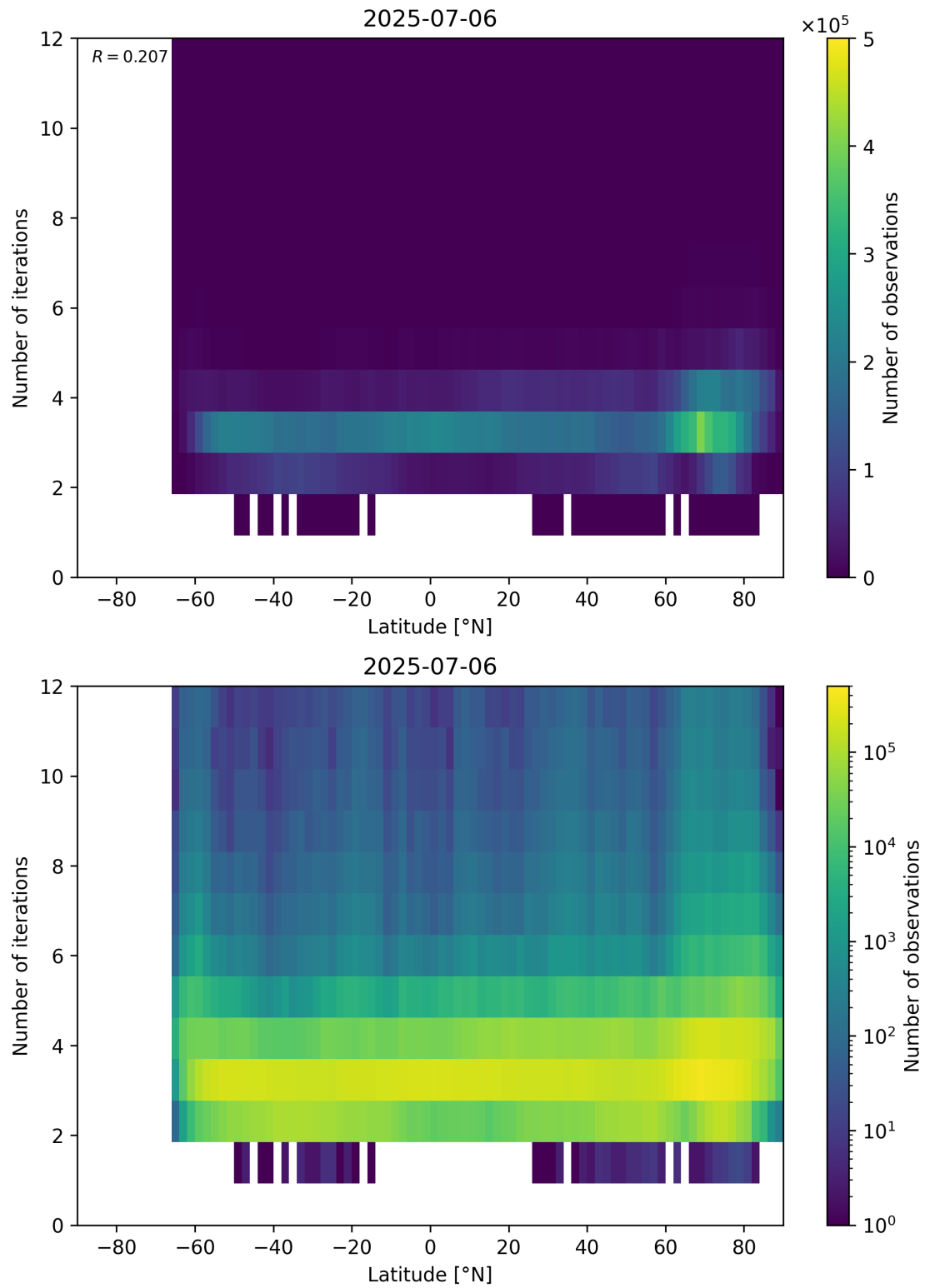
Figure 93: Scatter density plot of “Latitude” against “Number of iterations” for 2025-07-05 to 2025-07-07.
