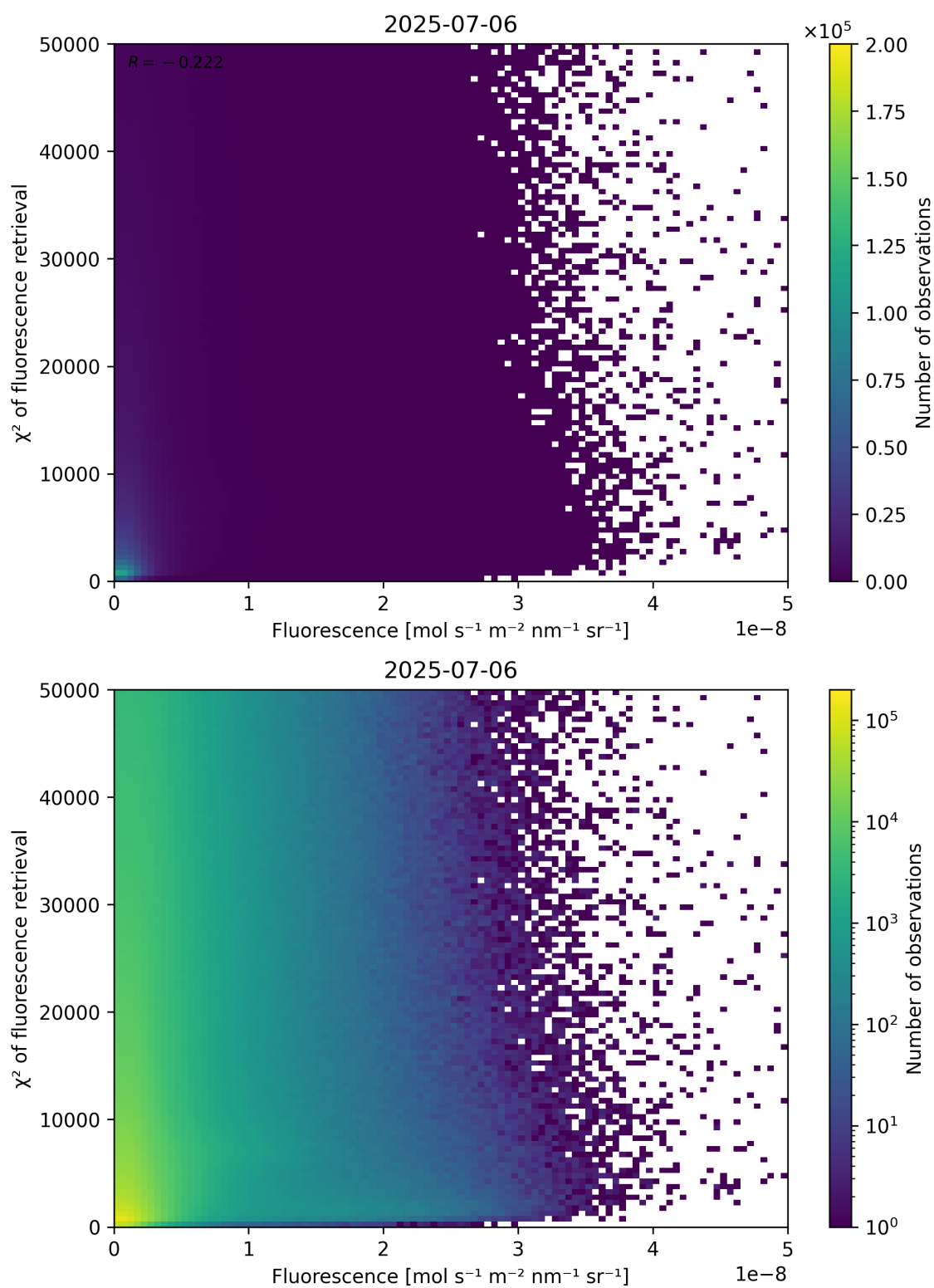
Figure 85: Scatter density plot of “Fluorescence” against “ \chi^2 of fluorescence retrieval” for 2025-07-05 to 2025-07-07.
