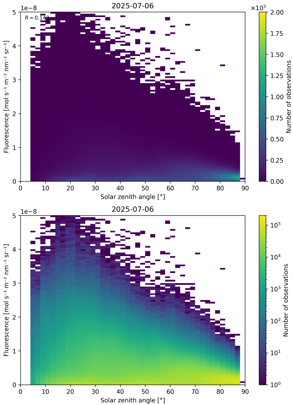
Figure 112: Scatter density plot of “Solar zenith angle” against “Fluorescence” for 2025-07-05 to 2025-07-07.
