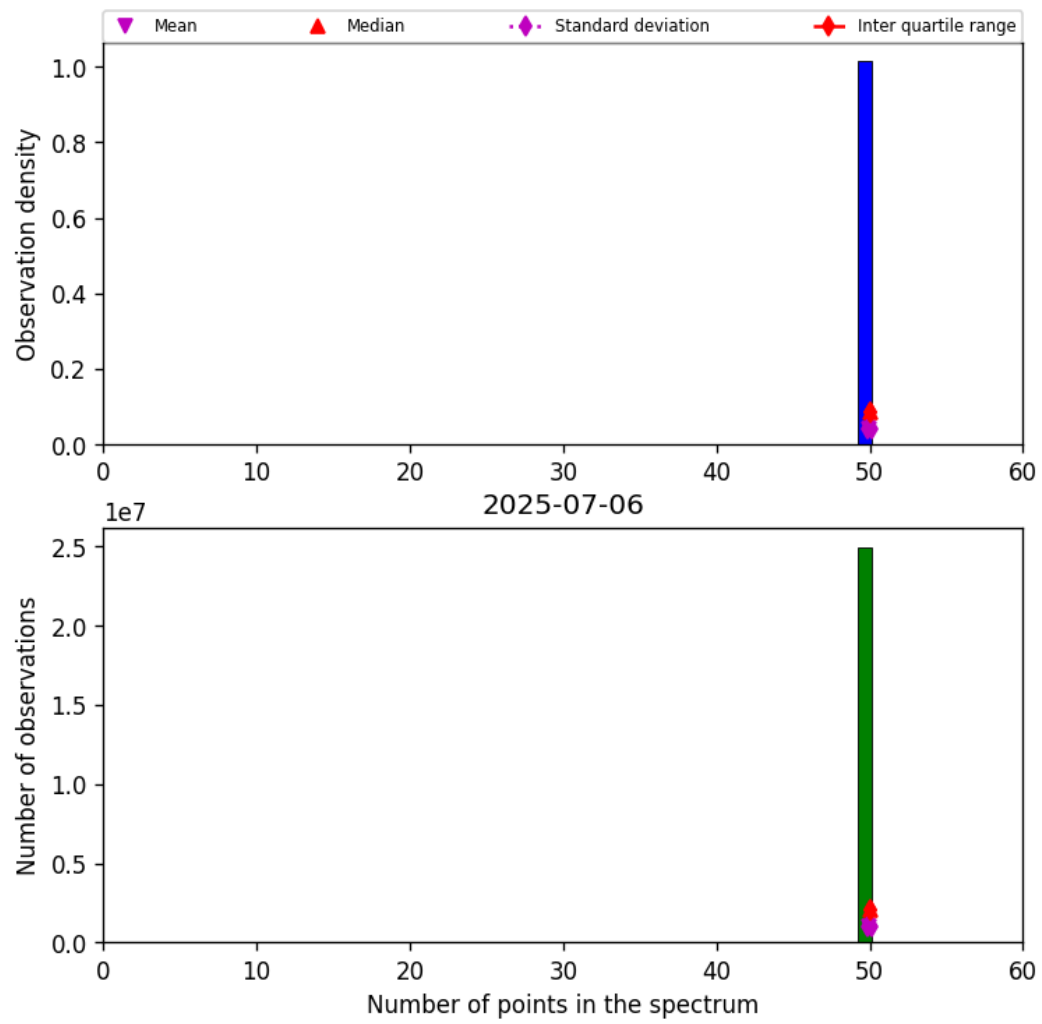
Figure 44: Histogram of "Number of points in the spectrum" for 2025-07-05 to 2025-07-07
