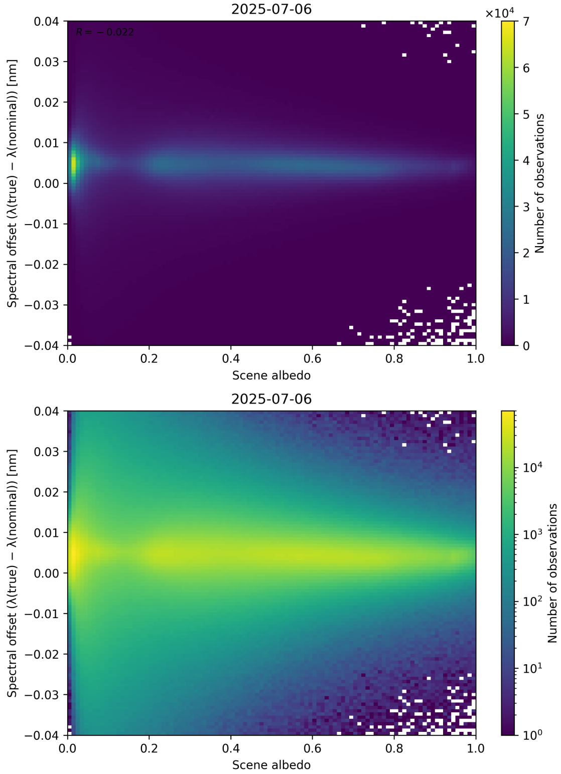
Figure 107: Scatter density plot of “Scene albedo” against “Spectral offset ( \lambda_{\text{true}} - \lambda_{\text{nominal}} )” for 2025-07-05 to 2025-07-07.
