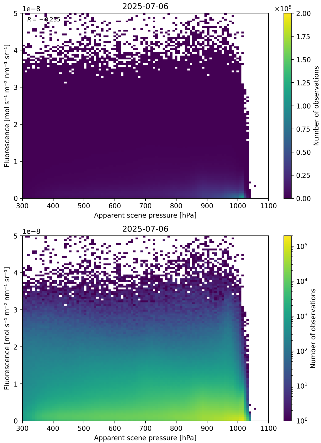
Figure 64: Scatter density plot of “Apparent scene pressure” against “Fluorescence” for 2025-07-05 to 2025-07-07.
