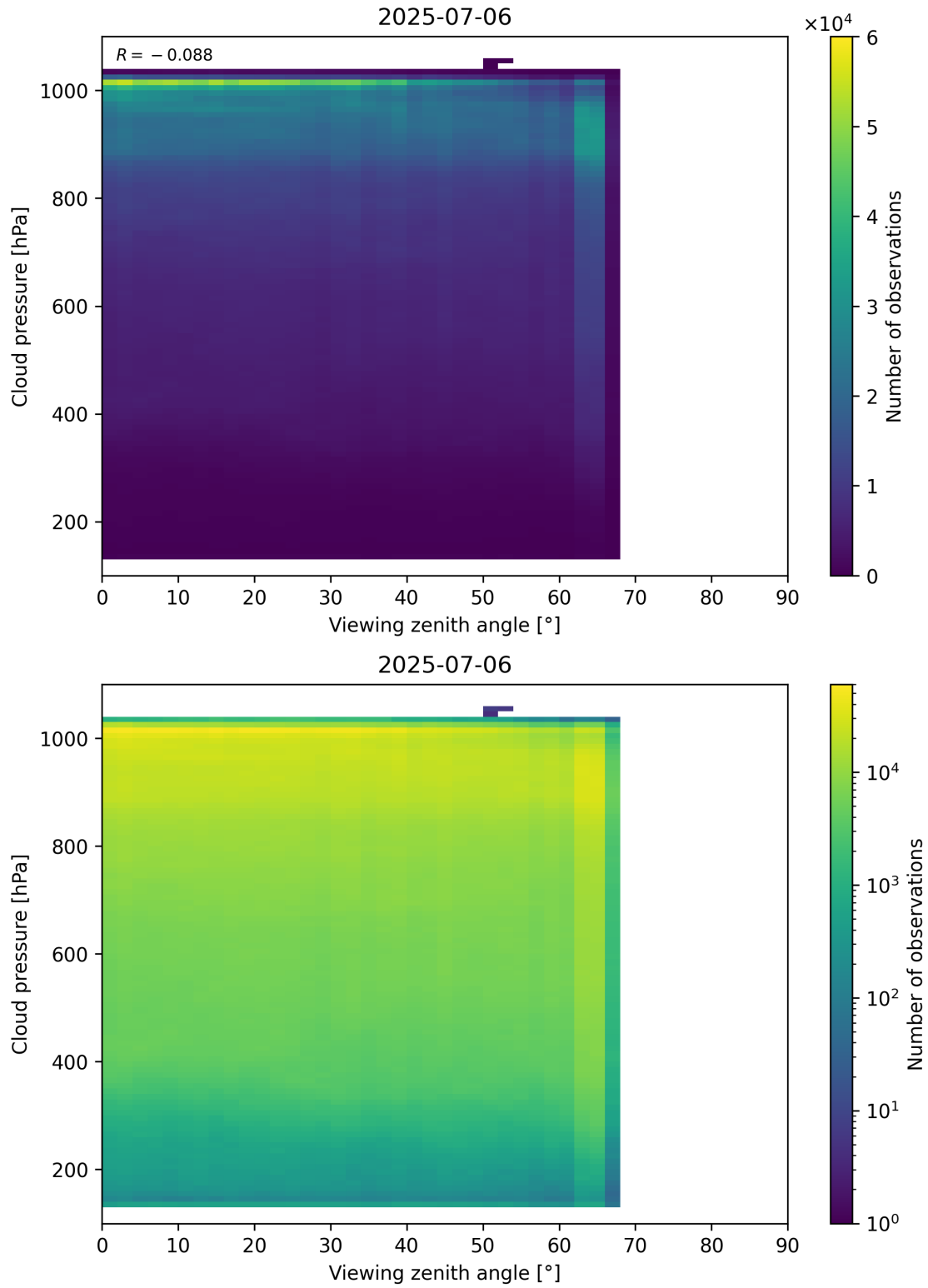
Figure 121: Scatter density plot of “Viewing zenith angle” against “Cloud pressure” for 2025-07-05 to 2025-07-07.
