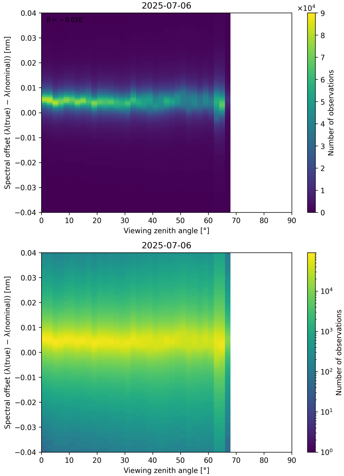
Figure 128: Scatter density plot of “Viewing zenith angle” against “Spectral offset ( \lambda_{\text{true}} - \lambda_{\text{nominal}} )” for 2025-07-05 to 2025-07-07.
