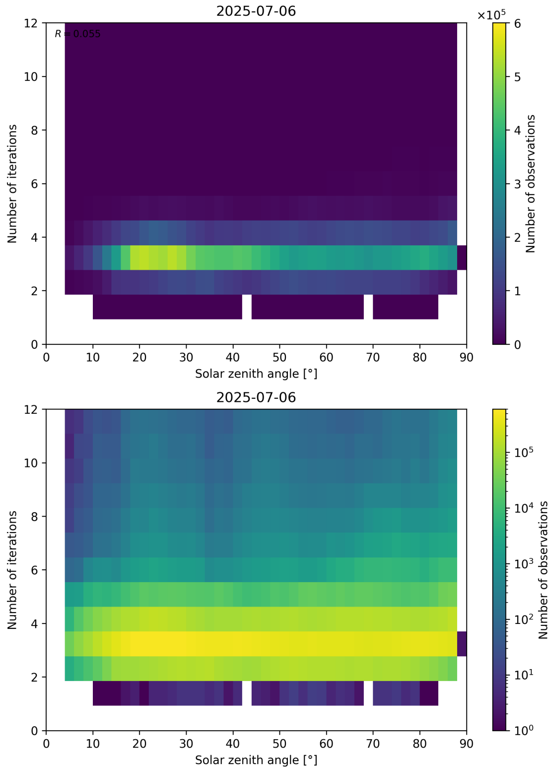
Figure 114: Scatter density plot of “Solar zenith angle” against “Number of iterations” for 2025-07-05 to 2025-07-07.
