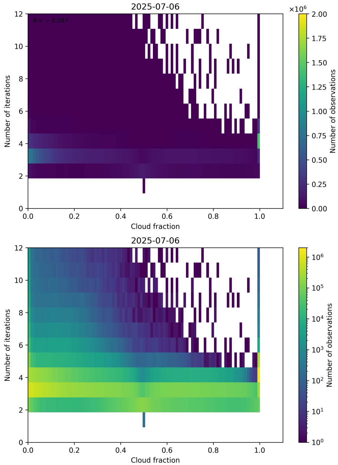
Figure 73: Scatter density plot of “Cloud fraction” against “Number of iterations” for 2025-07-05 to 2025-07-07.
