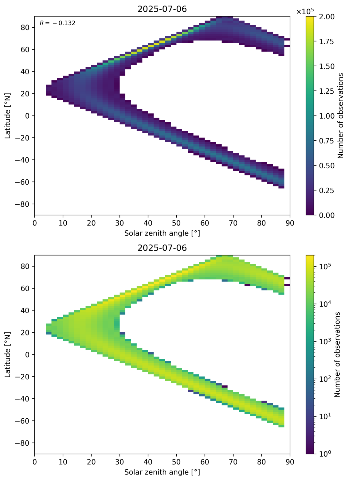
Figure 113: Scatter density plot of “Solar zenith angle” against “Latitude” for 2025-07-05 to 2025-07-07.
