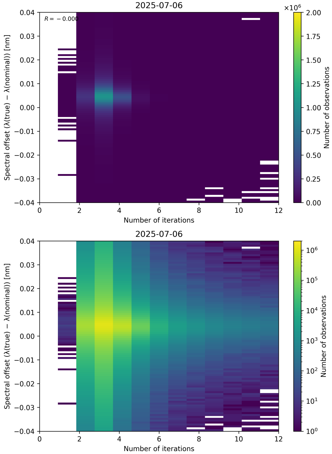
Figure 100: Scatter density plot of “Number of iterations” against “Spectral offset ( \lambda_{\text{true}} - \lambda_{\text{nominal}} )” for 2025-07-05 to 2025-07-07.
