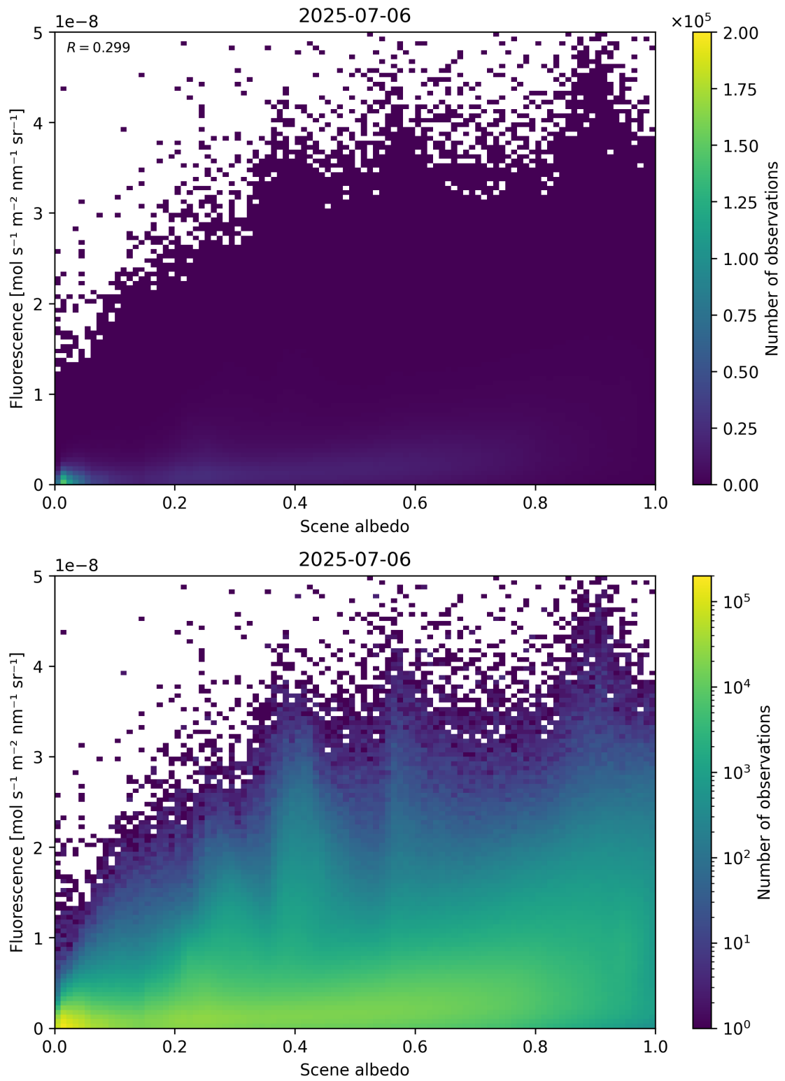
Figure 104: Scatter density plot of “Scene albedo” against “Fluorescence” for 2025-07-05 to 2025-07-07.
