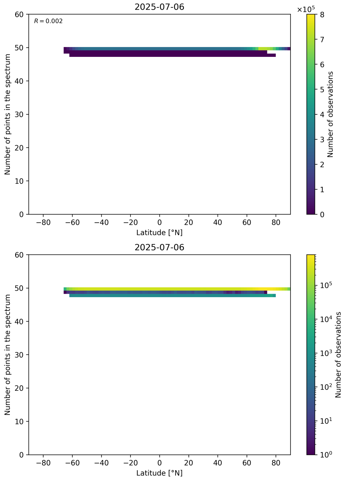
Figure 94: Scatter density plot of “Latitude” against “Number of points in the spectrum” for 2025-07-05 to 2025-07-07.
