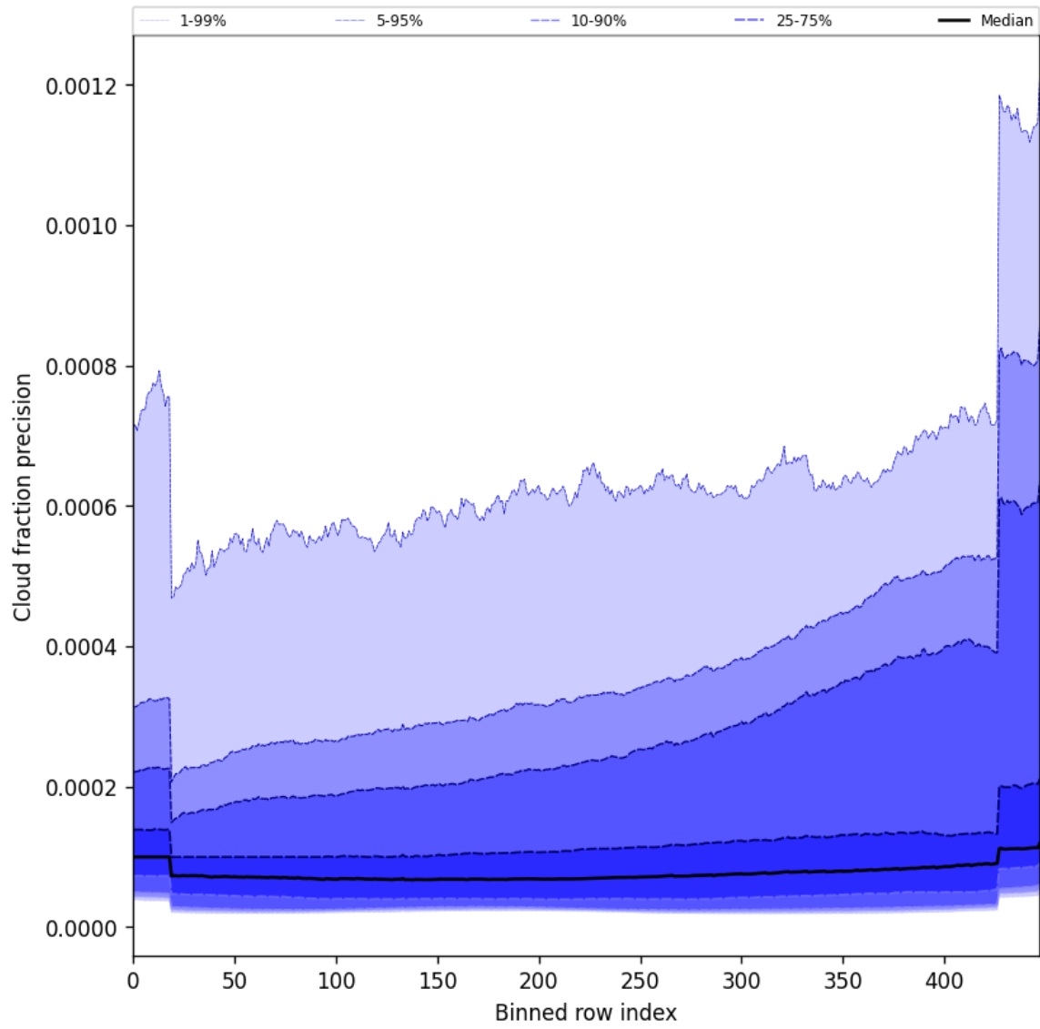
Figure 50: Along track statistics of “Cloud fraction precision” for 2025-07-05 to 2025-07-07
