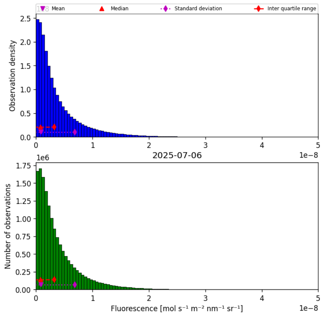
Figure 40: Histogram of “Fluorescence” for 2025-07-05 to 2025-07-07
