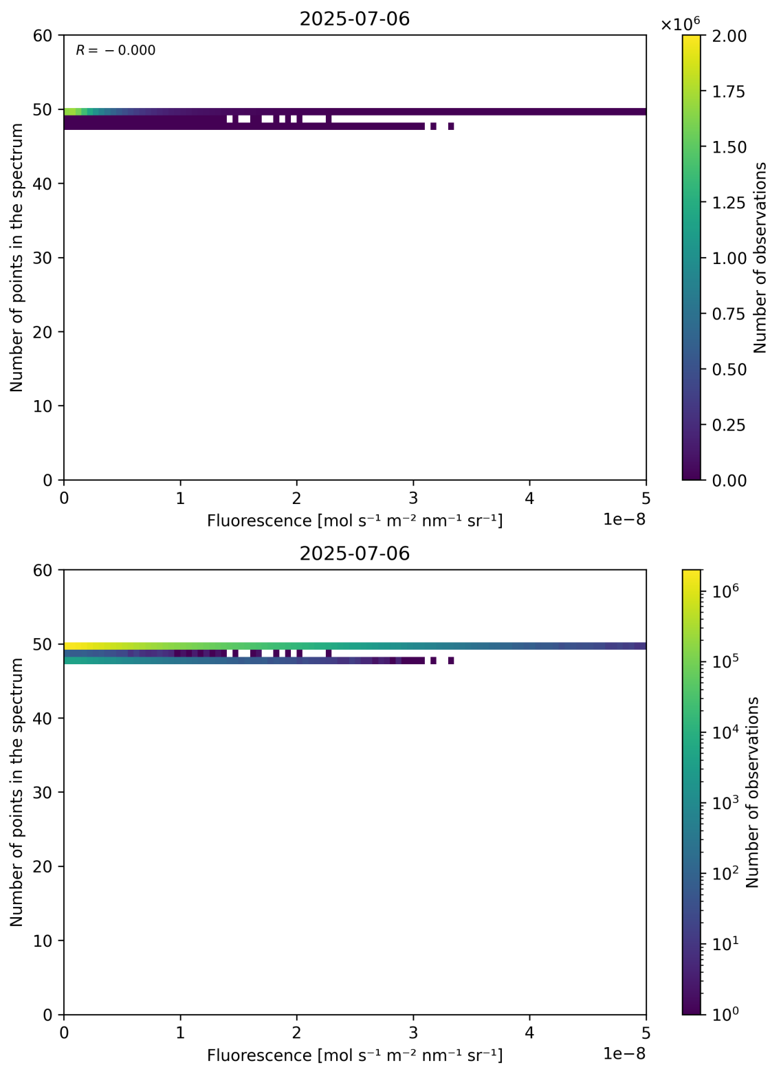
Figure 86: Scatter density plot of “Fluorescence” against “Number of points in the spectrum” for 2025-07-05 to 2025-07-07.
