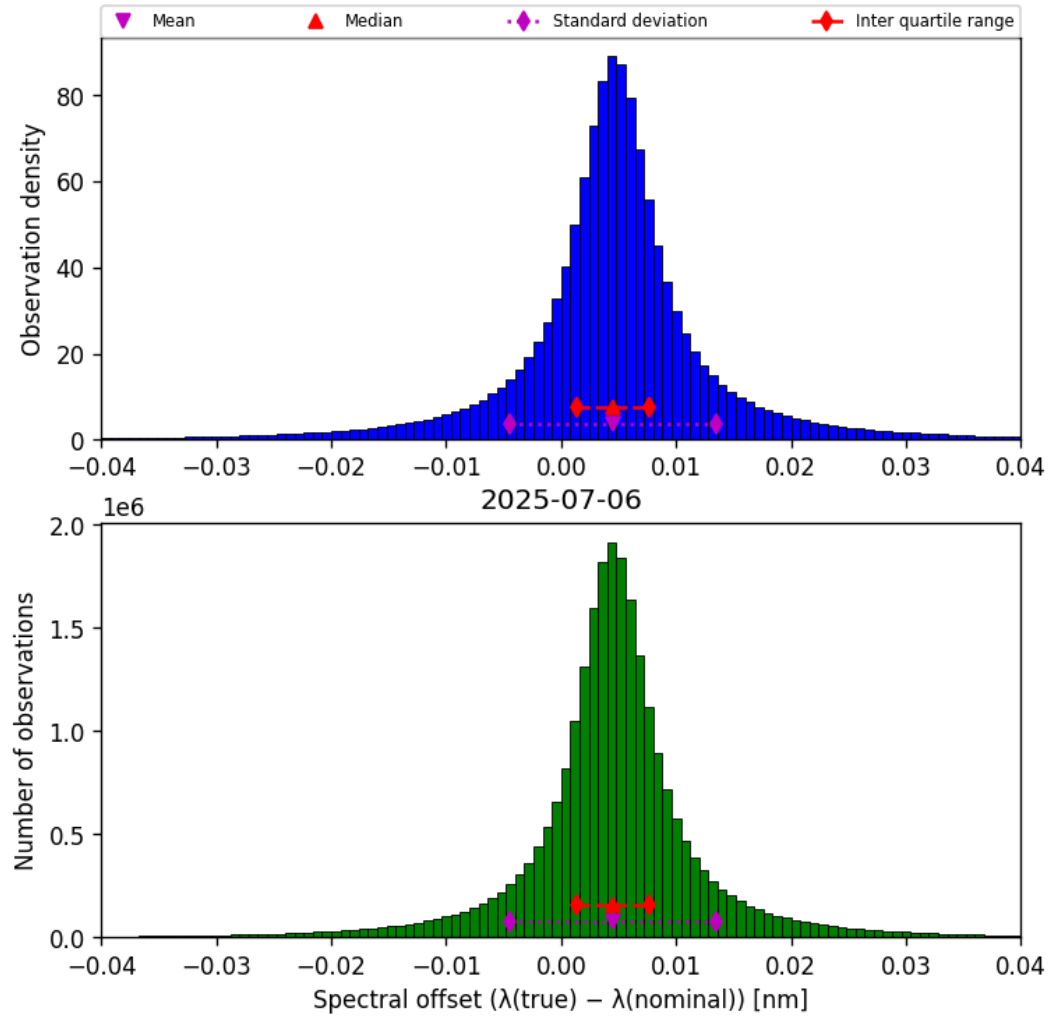
Figure 45: Histogram of “Spectral offset ( \lambda_{\text{true}} - \lambda_{\text{nominal}} )” for 2025-07-05 to 2025-07-07
