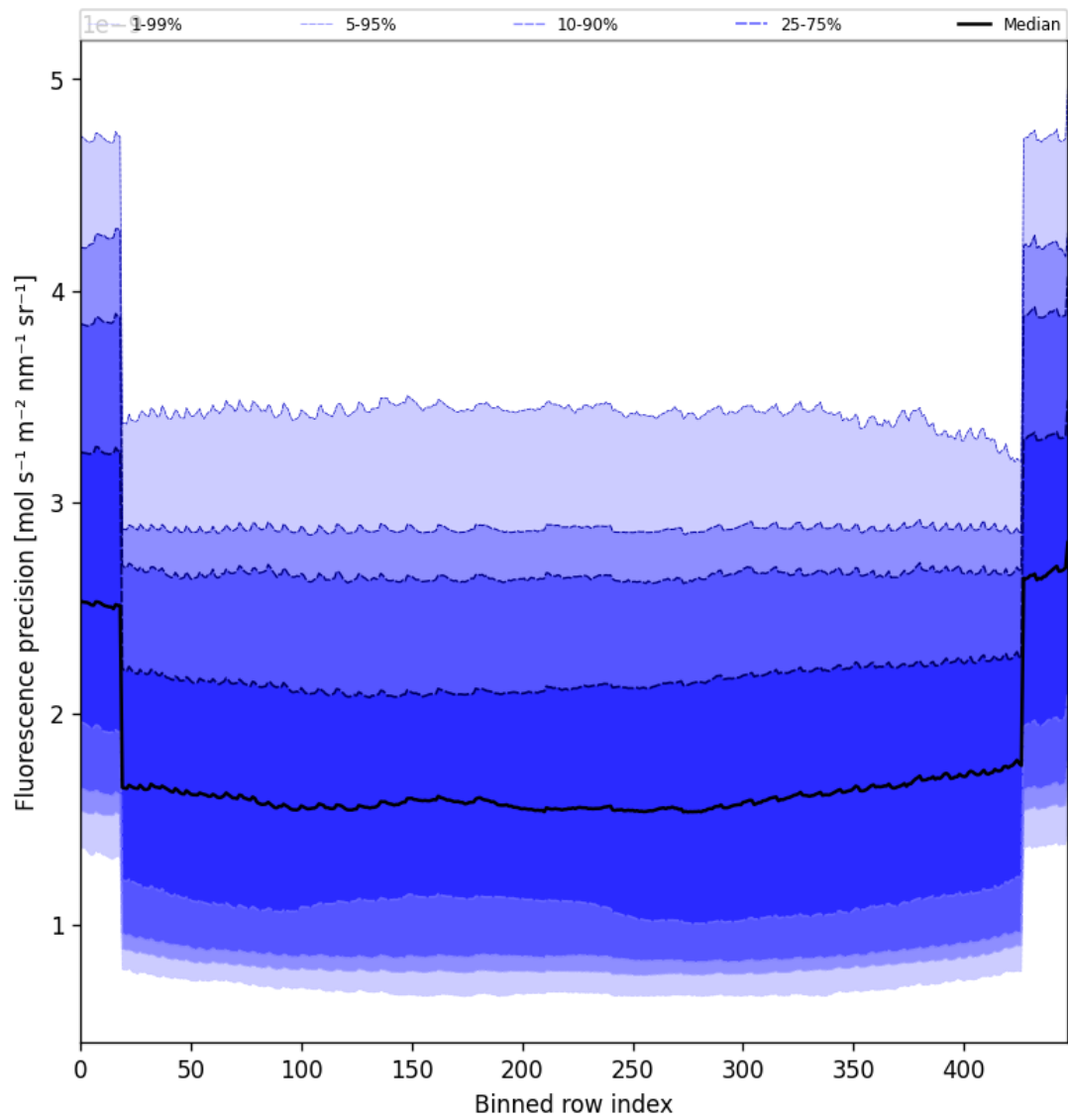
Figure 58: Along track statistics of “Fluorescence precision” for 2025-07-05 to 2025-07-07
