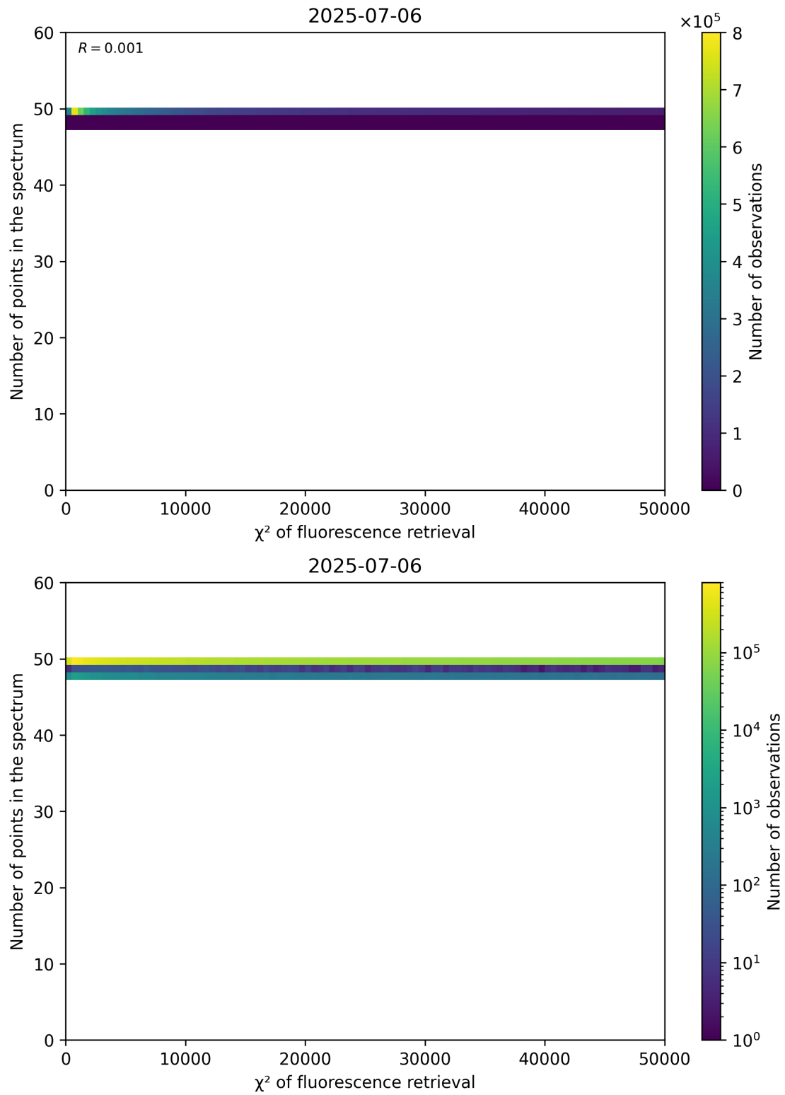
Figure 68: Scatter density plot of " \chi^2 of fluorescence retrieval" against "Number of points in the spectrum" for 2025-07-05 to 2025-07-07.
