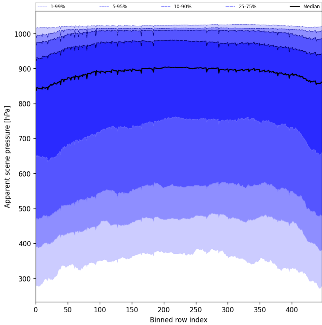
Figure 53: Along track statistics of “Apparent scene pressure” for 2025-07-05 to 2025-07-07
