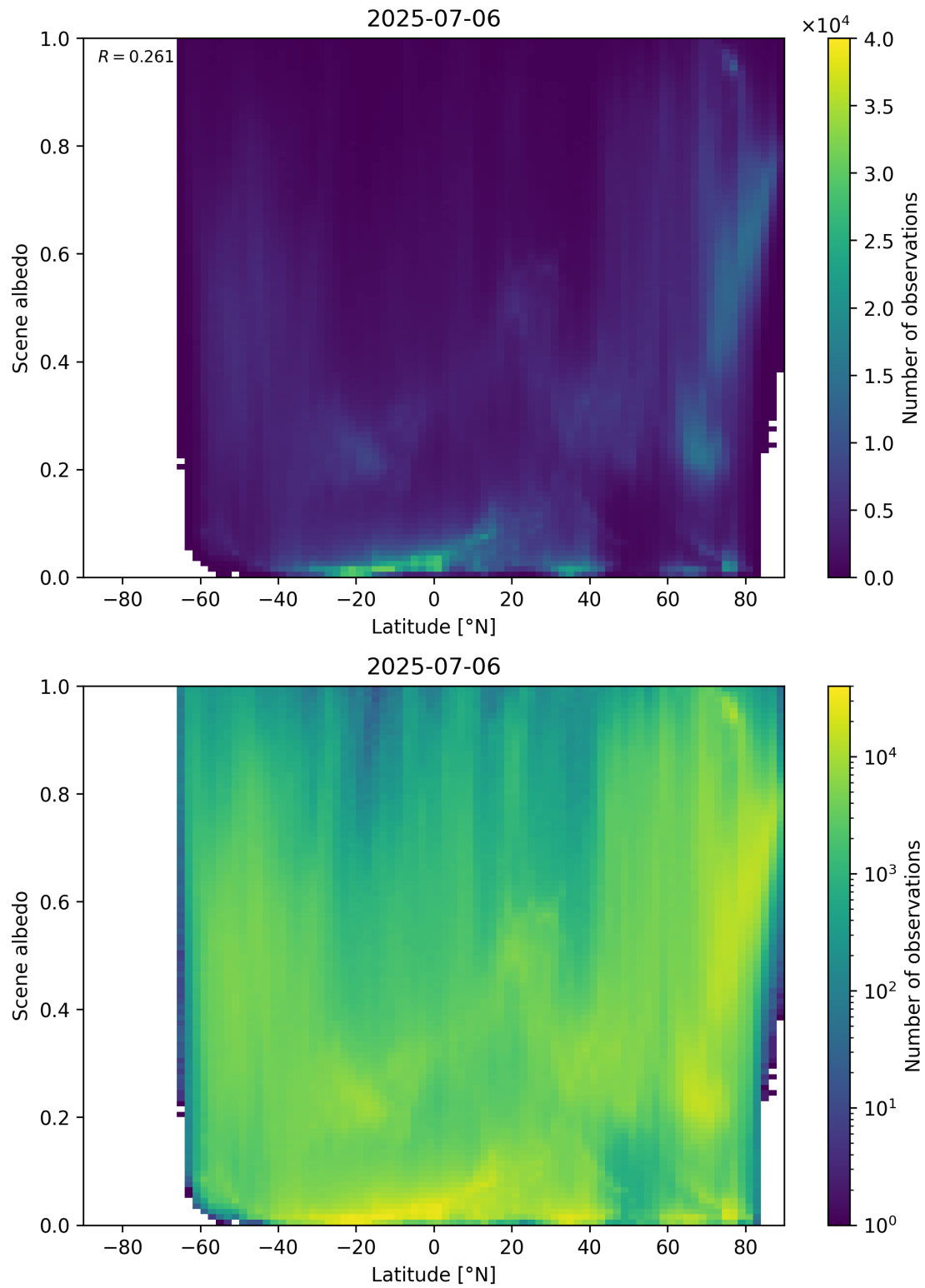
Figure 95: Scatter density plot of “Latitude” against “Scene albedo” for 2025-07-05 to 2025-07-07.
