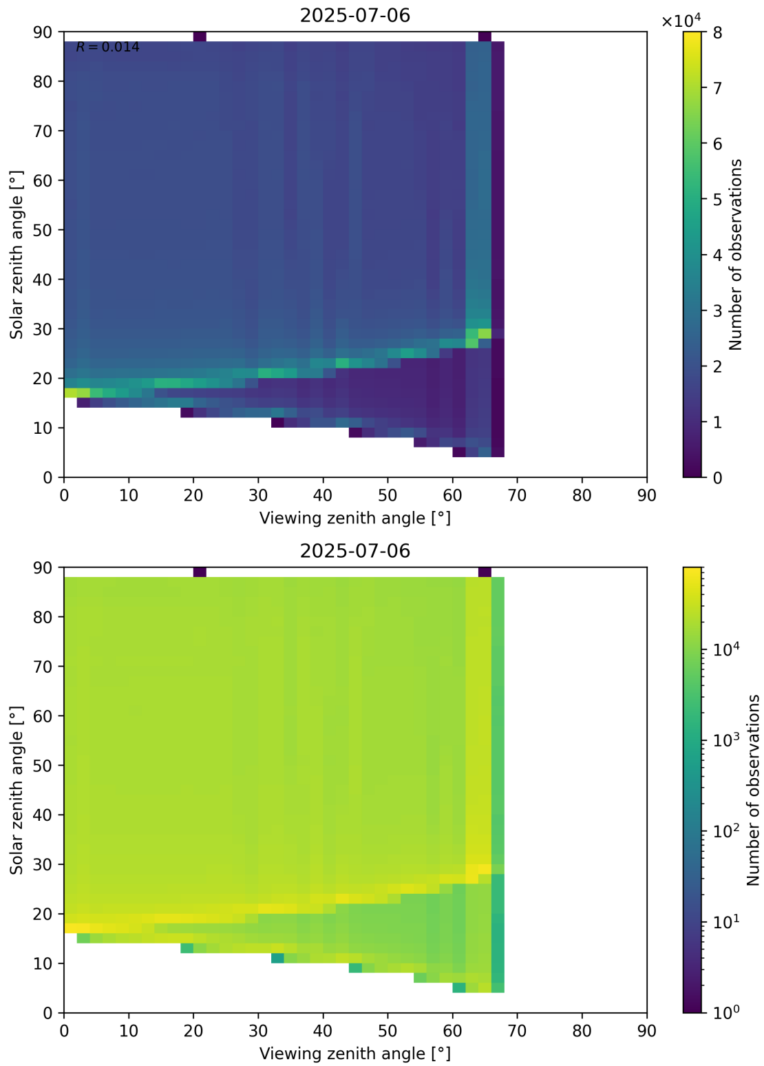
Figure 127: Scatter density plot of “Viewing zenith angle” against “Solar zenith angle” for 2025-07-05 to 2025-07-07.
