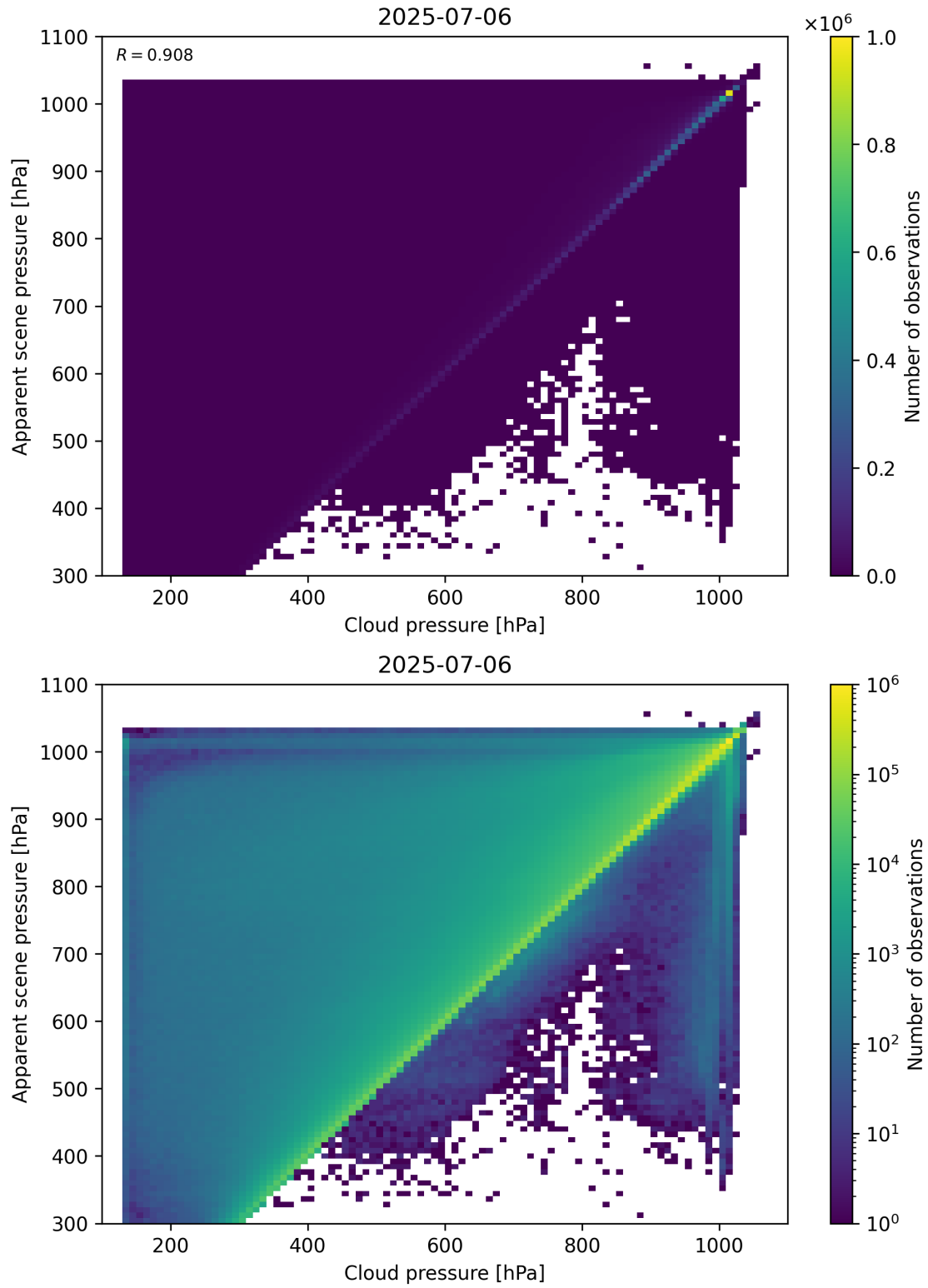
Figure 77: Scatter density plot of “Cloud pressure” against “Apparent scene pressure” for 2025-07-05 to 2025-07-07.
