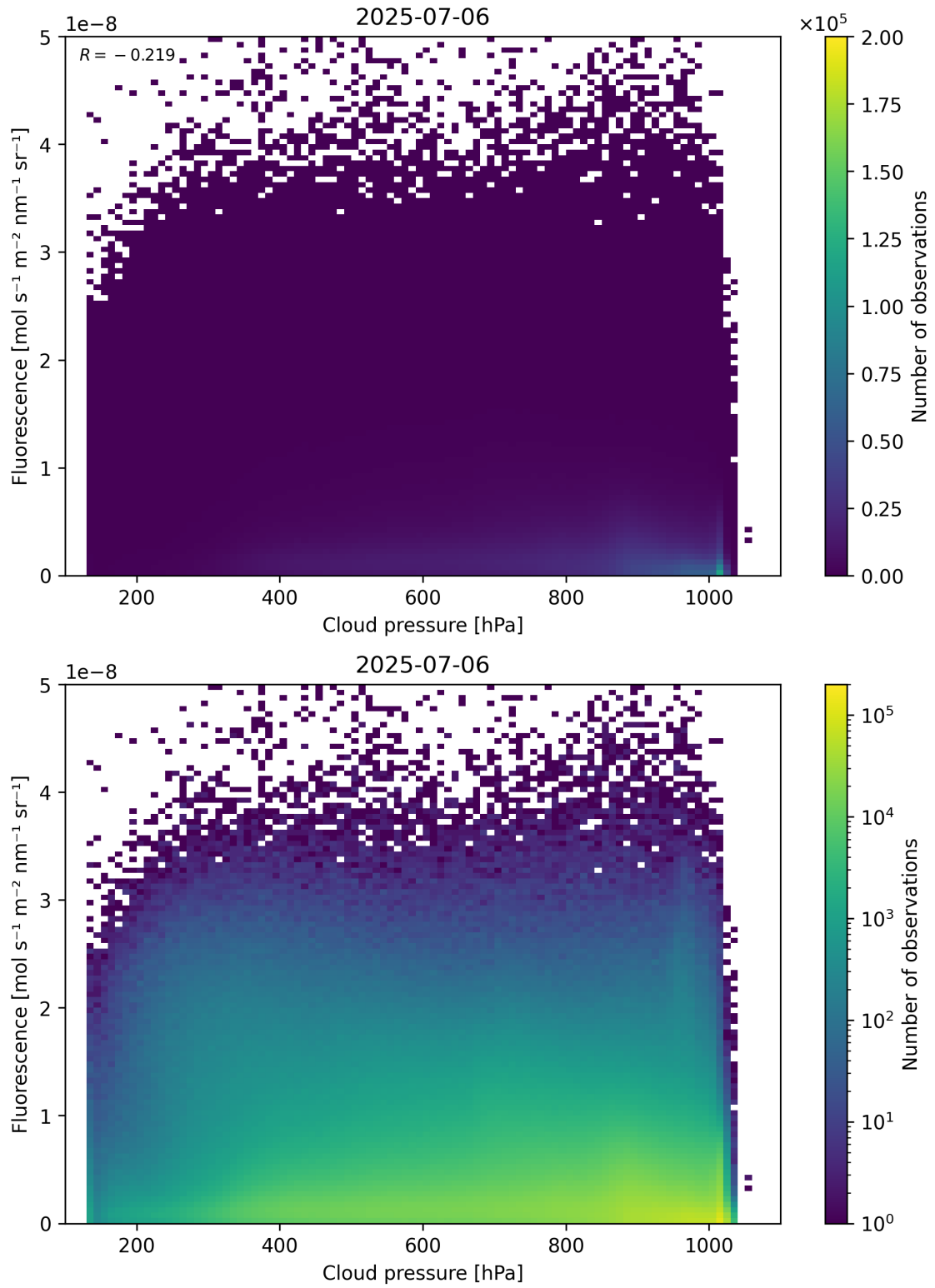
Figure 80: Scatter density plot of “Cloud pressure” against “Fluorescence” for 2025-07-05 to 2025-07-07.
