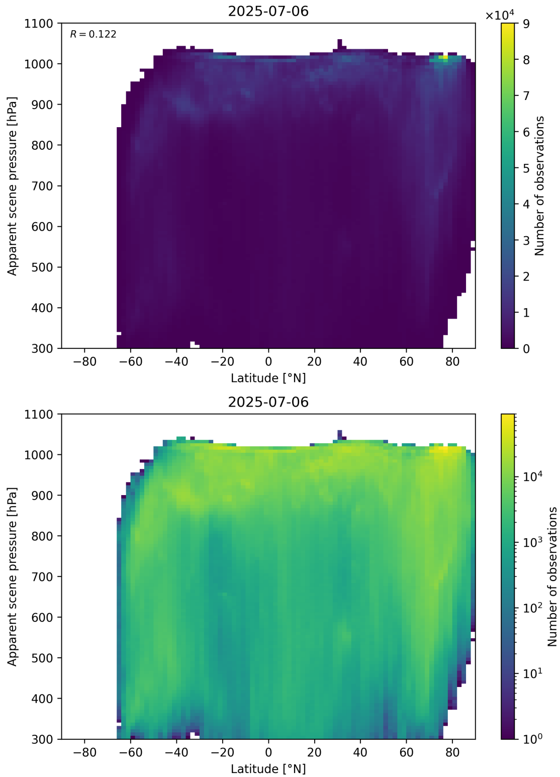
Figure 88: Scatter density plot of “Latitude” against “Apparent scene pressure” for 2025-07-05 to 2025-07-07.
