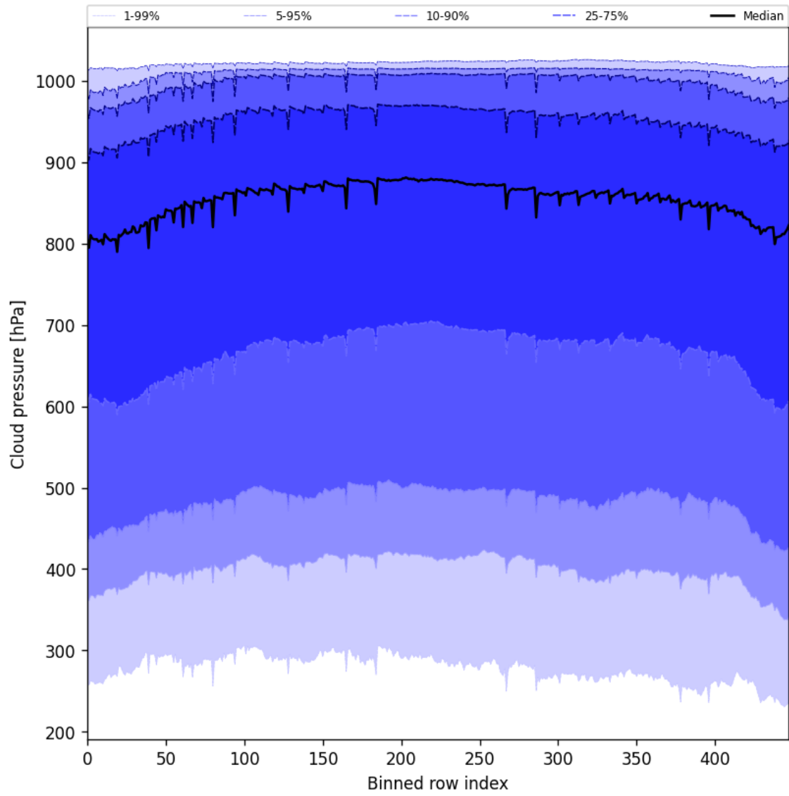
Figure 47: Along track statistics of “Cloud pressure” for 2025-07-05 to 2025-07-07
