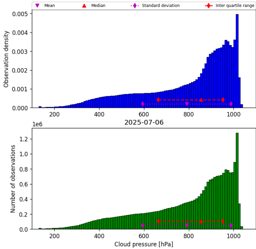
Figure 30: Histogram of “Cloud pressure” for 2025-07-05 to 2025-07-07
