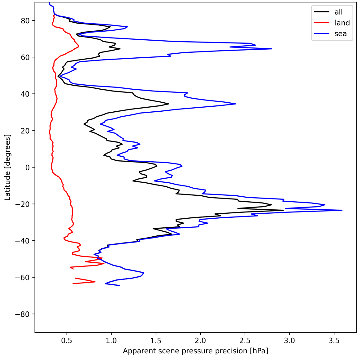
Figure 20: Zonal average of “Apparent scene pressure precision” for 2025-07-05 to 2025-07-07.
