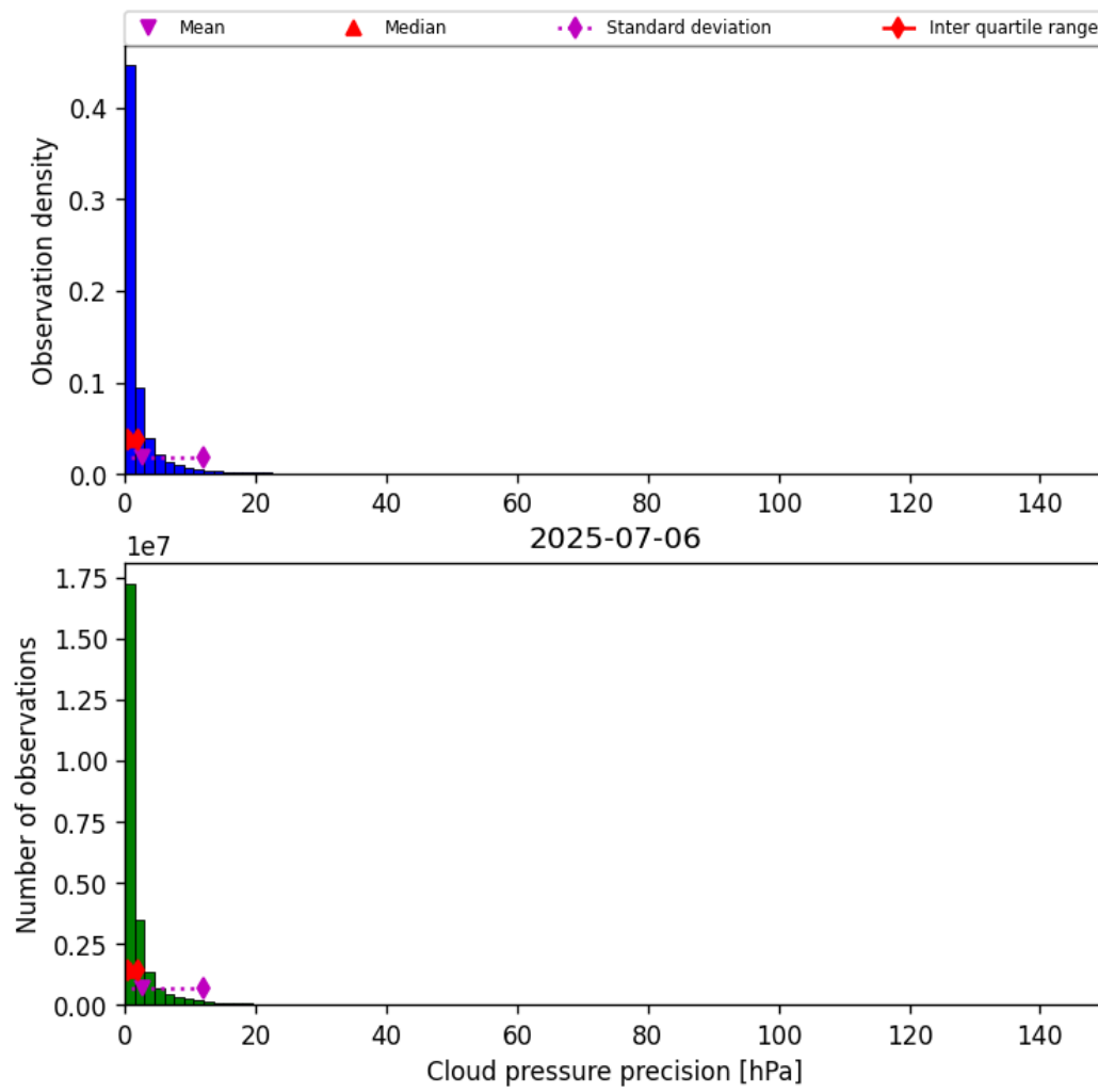
Figure 31: Histogram of “Cloud pressure precision” for 2025-07-05 to 2025-07-07
