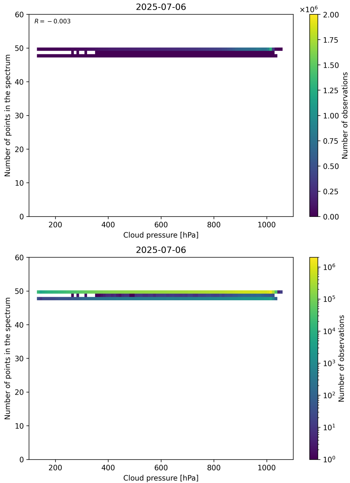
Figure 82: Scatter density plot of “Cloud pressure” against “Number of points in the spectrum” for 2025-07-05 to 2025-07-07.
