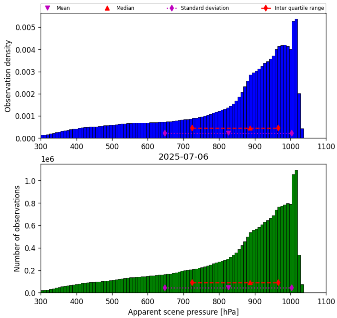
Figure 36: Histogram of “Apparent scene pressure” for 2025-07-05 to 2025-07-07
