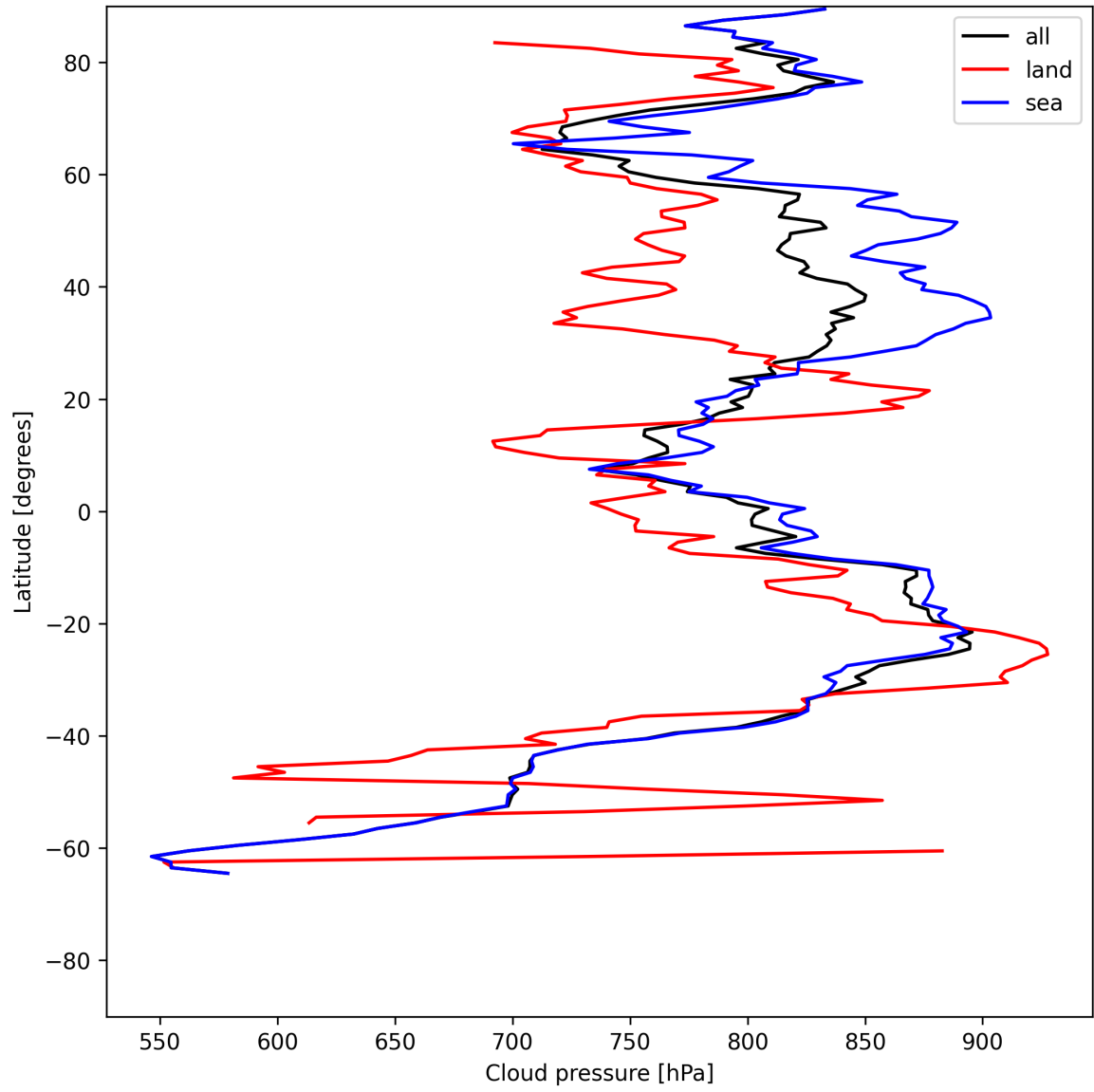
Figure 13: Zonal average of “Cloud pressure” for 2025-07-05 to 2025-07-07.
