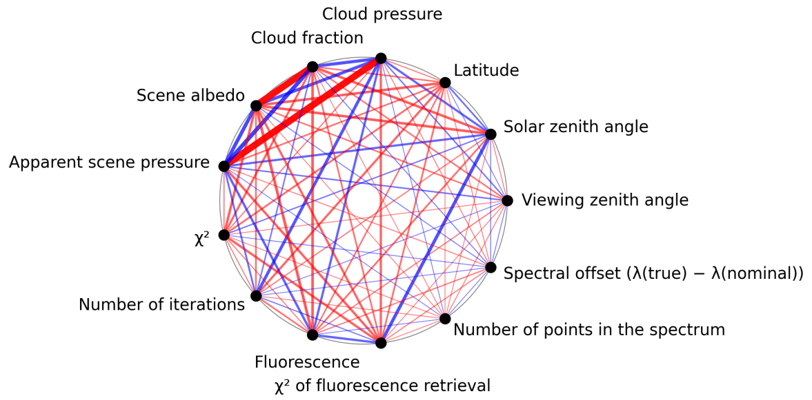
Figure 1: Map of correlation graph for 2025-07-05 to 2025-07-07.
