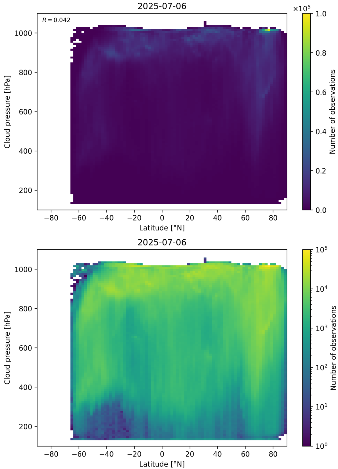
Figure 91: Scatter density plot of “Latitude” against “Cloud pressure” for 2025-07-05 to 2025-07-07.
