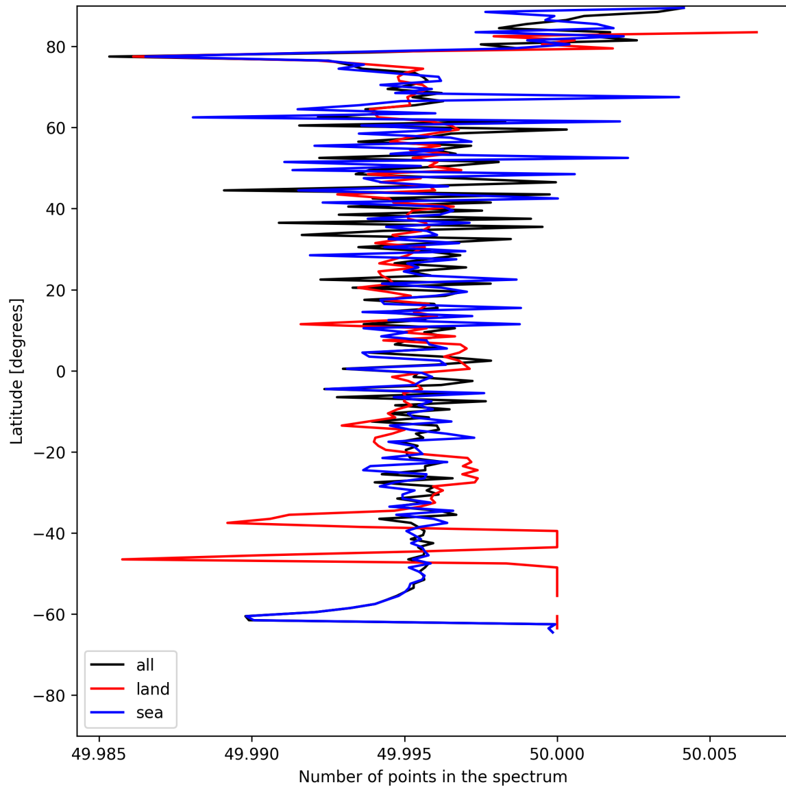
Figure 27: Zonal average of “Number of points in the spectrum” for 2025-07-05 to 2025-07-07.
