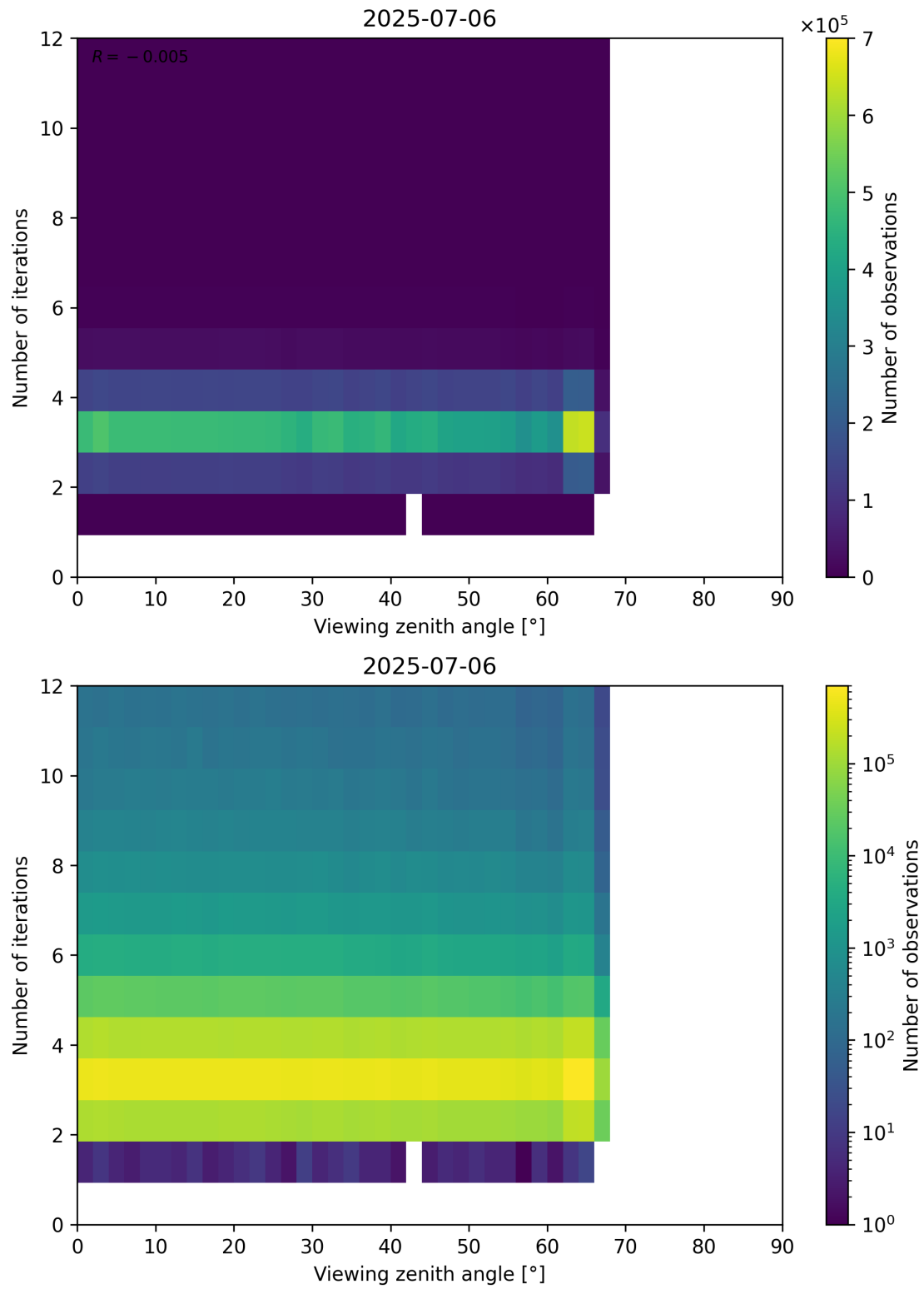
Figure 124: Scatter density plot of “Viewing zenith angle” against “Number of iterations” for 2025-07-05 to 2025-07-07.
