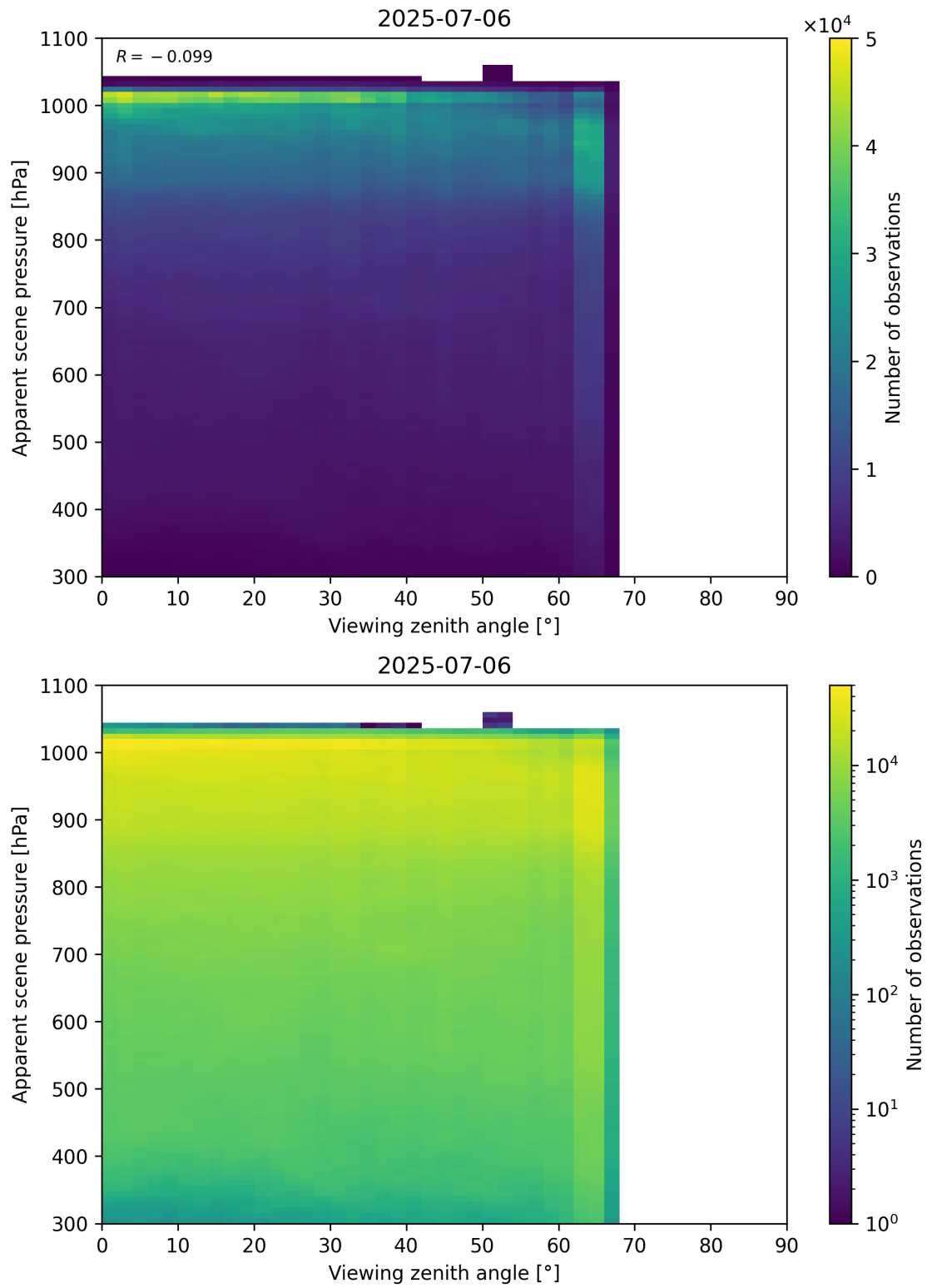
Figure 118: Scatter density plot of “Viewing zenith angle” against “Apparent scene pressure” for 2025-07-05 to 2025-07-07.
