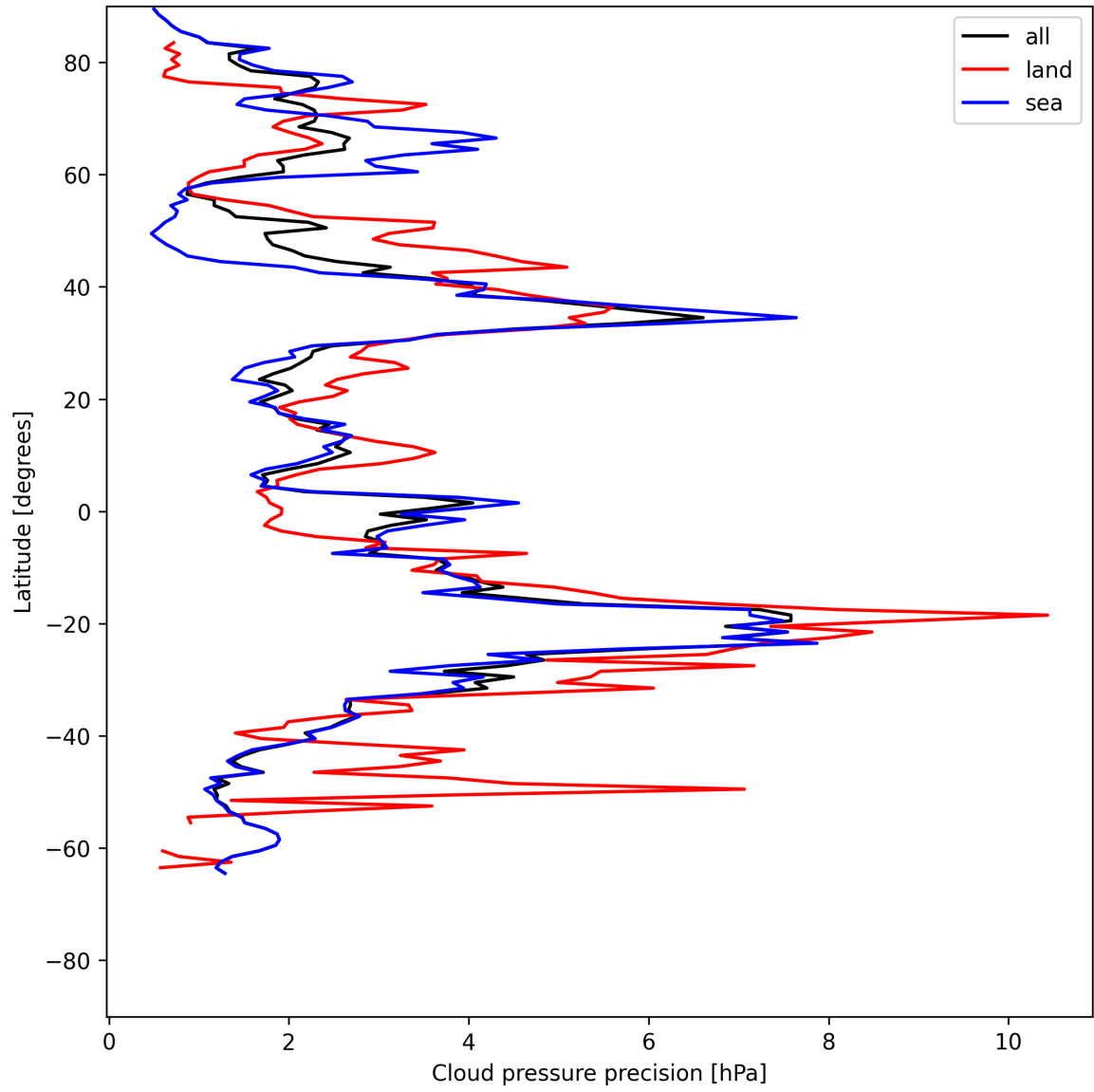
Figure 14: Zonal average of “Cloud pressure precision” for 2025-07-05 to 2025-07-07.
