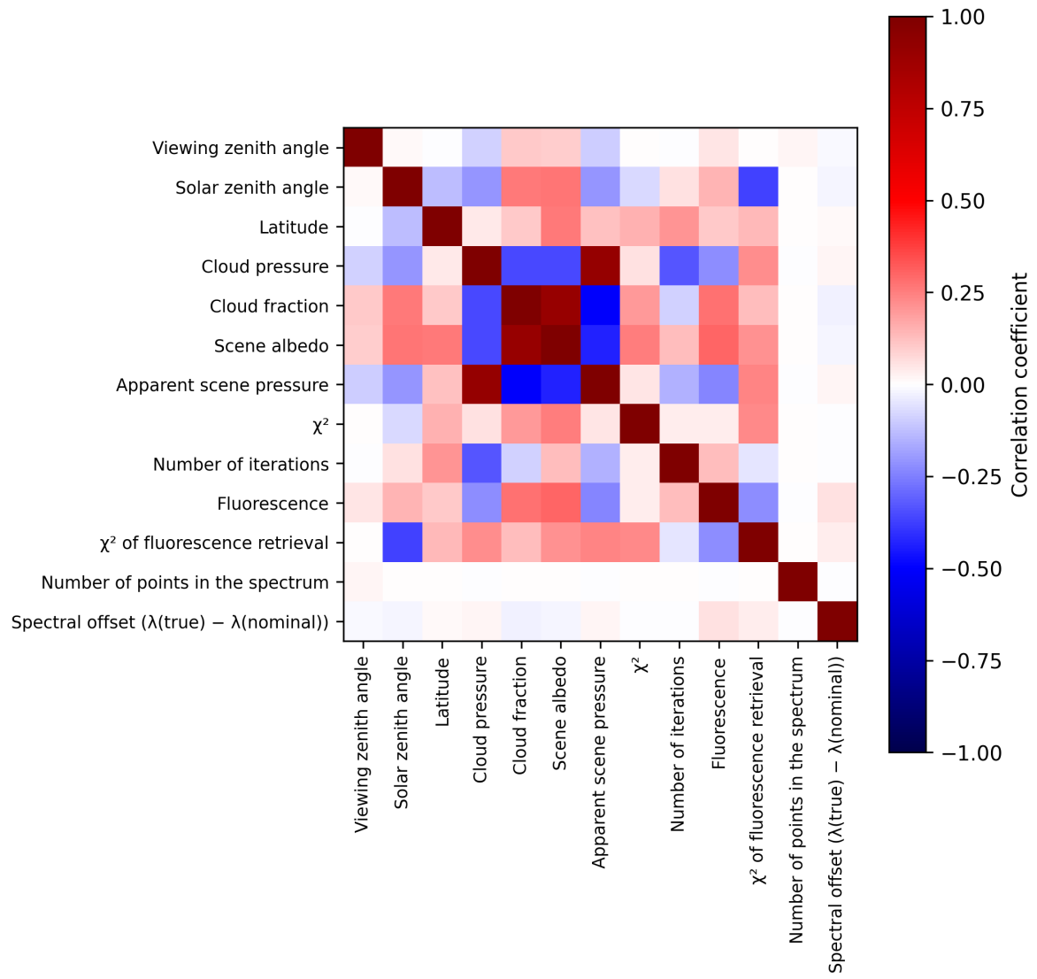
Figure 2: Map of correlation matrix for 2025-07-05 to 2025-07-07.
