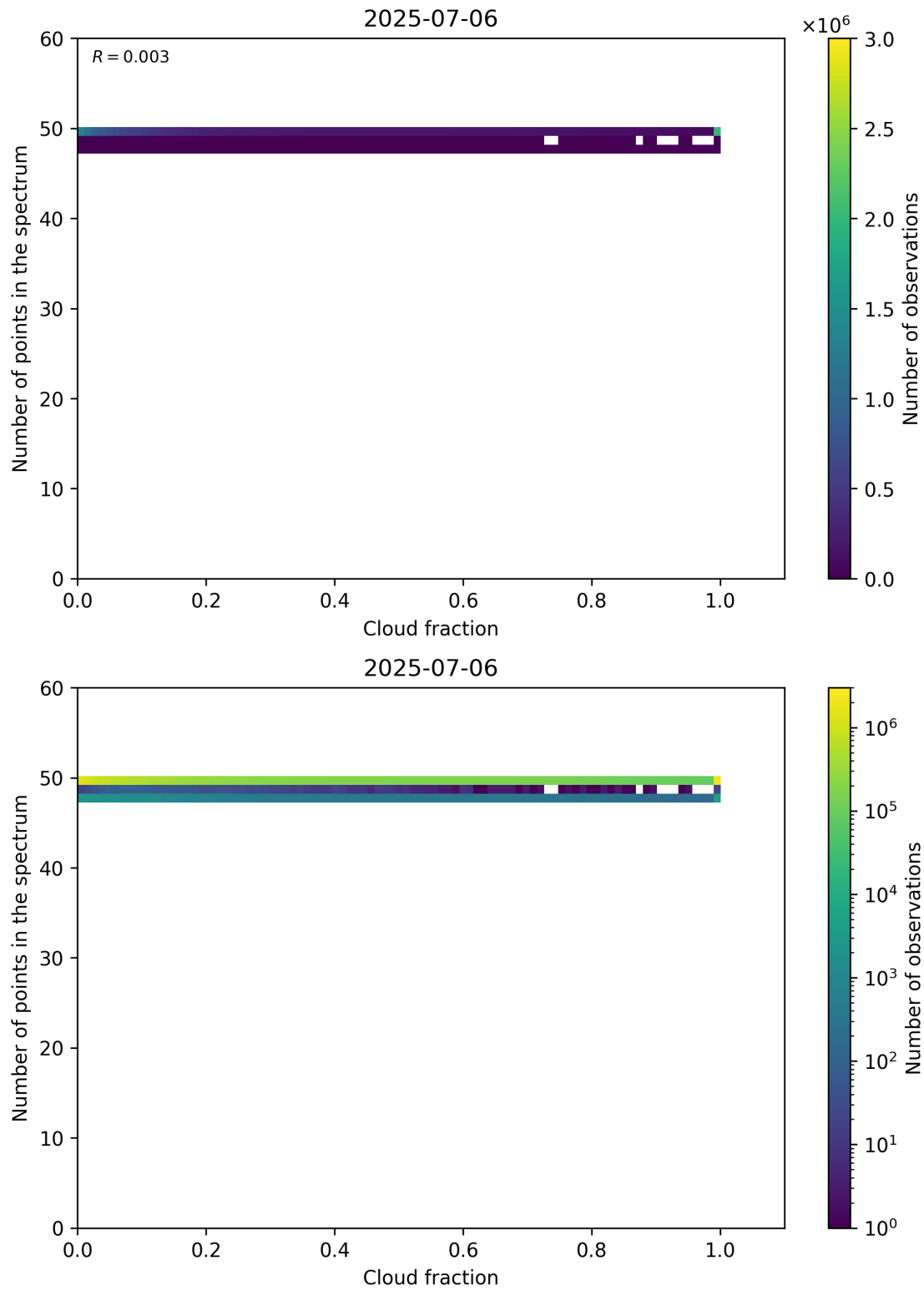
Figure 74: Scatter density plot of “Cloud fraction” against “Number of points in the spectrum” for 2025-07-05 to 2025-07-07.
