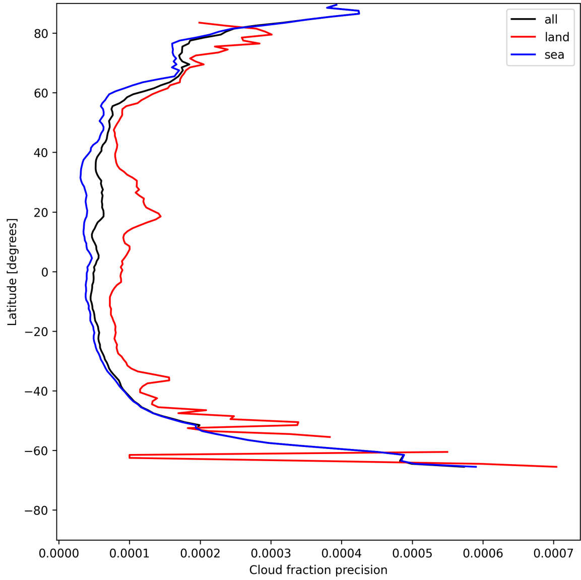
Figure 16: Zonal average of “Cloud fraction precision” for 2025-07-08 to 2025-07-09.
