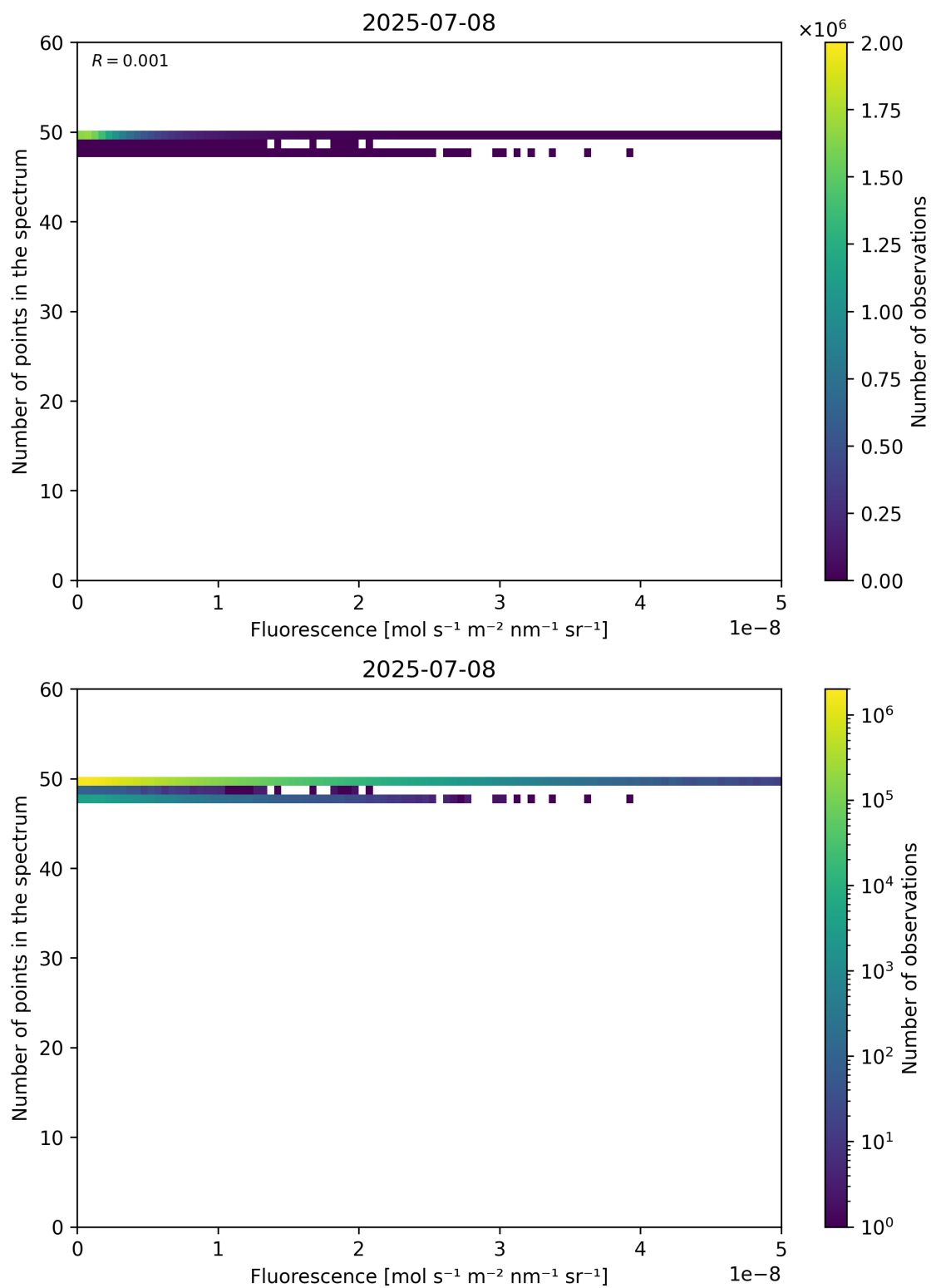
Figure 86: Scatter density plot of “Fluorescence” against “Number of points in the spectrum” for 2025-07-08 to 2025-07-09.
