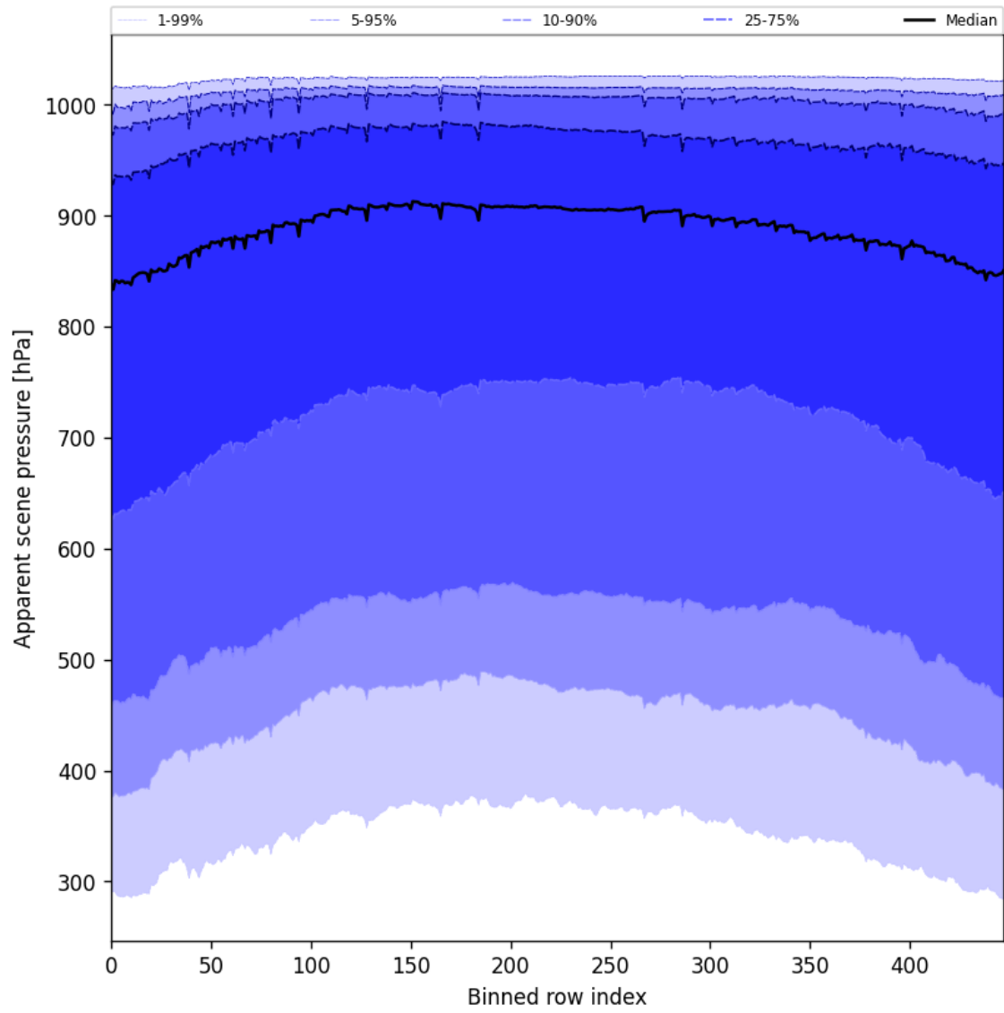
Figure 53: Along track statistics of “Apparent scene pressure” for 2025-07-08 to 2025-07-09
