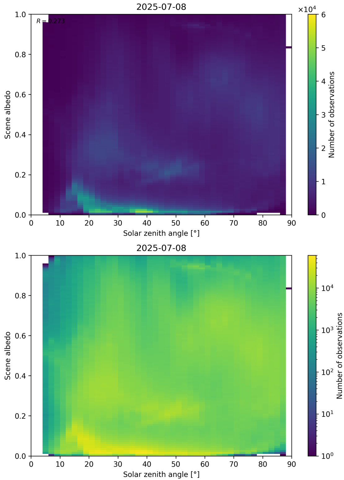
Figure 116: Scatter density plot of “Solar zenith angle” against “Scene albedo” for 2025-07-08 to 2025-07-09.
