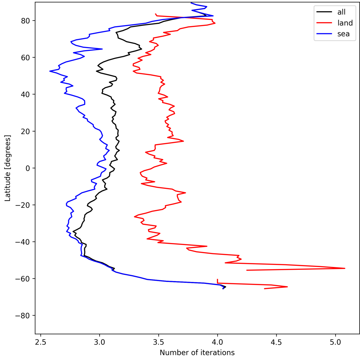
Figure 22: Zonal average of “Number of iterations” for 2025-07-08 to 2025-07-09.
