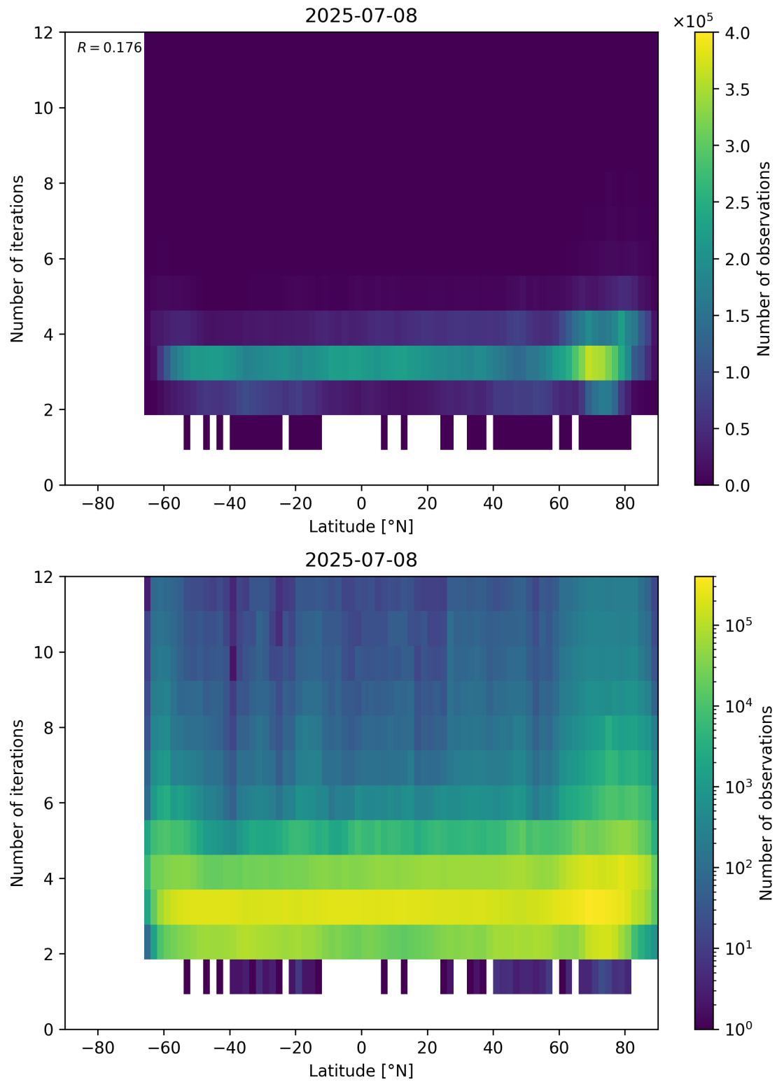
Figure 93: Scatter density plot of “Latitude” against “Number of iterations” for 2025-07-08 to 2025-07-09.
