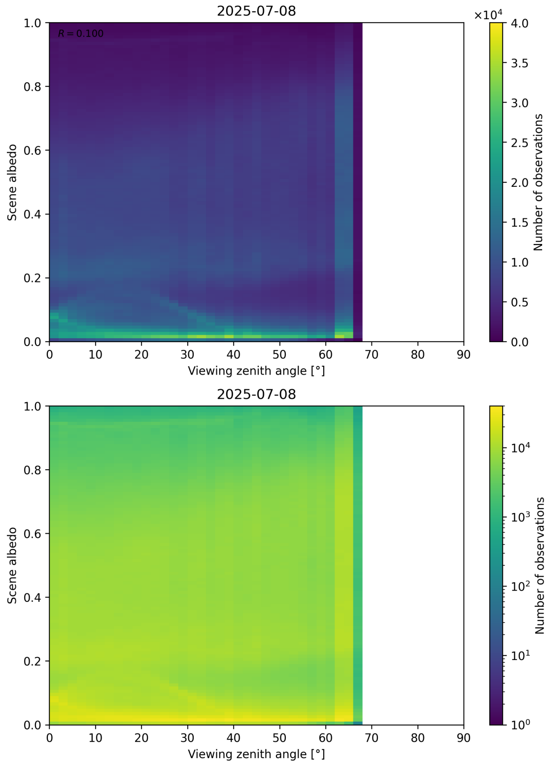
Figure 126: Scatter density plot of “Viewing zenith angle” against “Scene albedo” for 2025-07-08 to 2025-07-09.
