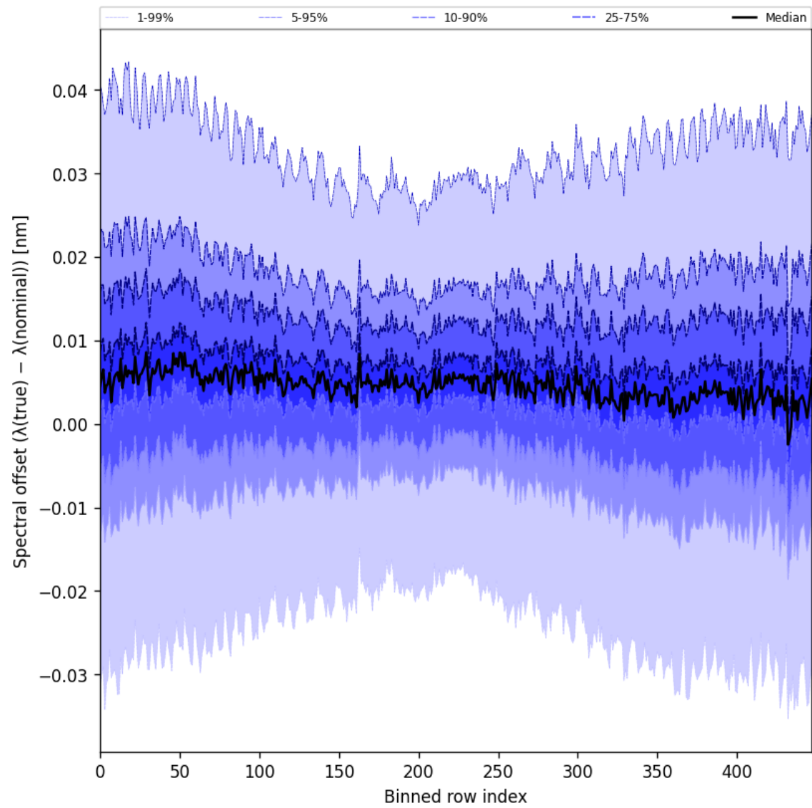
Figure 62: Along track statistics of “Spectral offset ( \lambda_{\text{true}} - \lambda_{\text{nominal}} )” for 2025-07-08 to 2025-07-09
