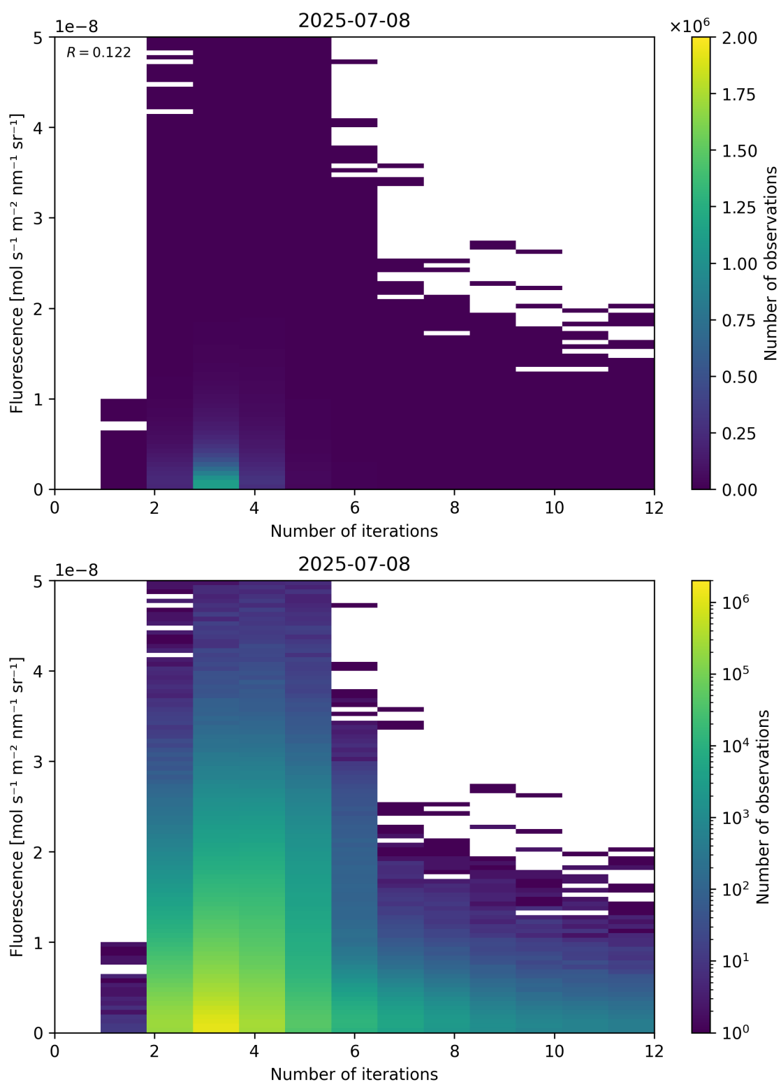
Figure 98: Scatter density plot of “Number of iterations” against “Fluorescence” for 2025-07-08 to 2025-07-09.
