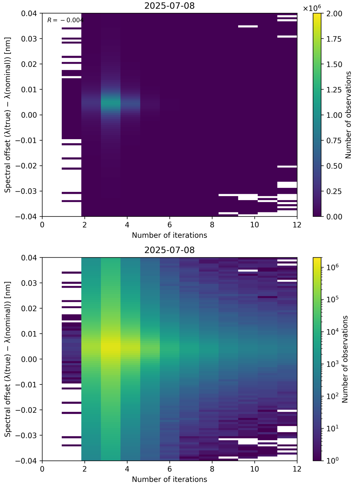
Figure 100: Scatter density plot of “Number of iterations” against “Spectral offset ( \lambda_{\text{true}} - \lambda_{\text{nominal}} )” for 2025-07-08 to 2025-07-09.
