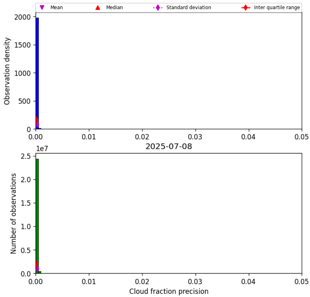
Figure 33: Histogram of “Cloud fraction precision” for 2025-07-08 to 2025-07-09
