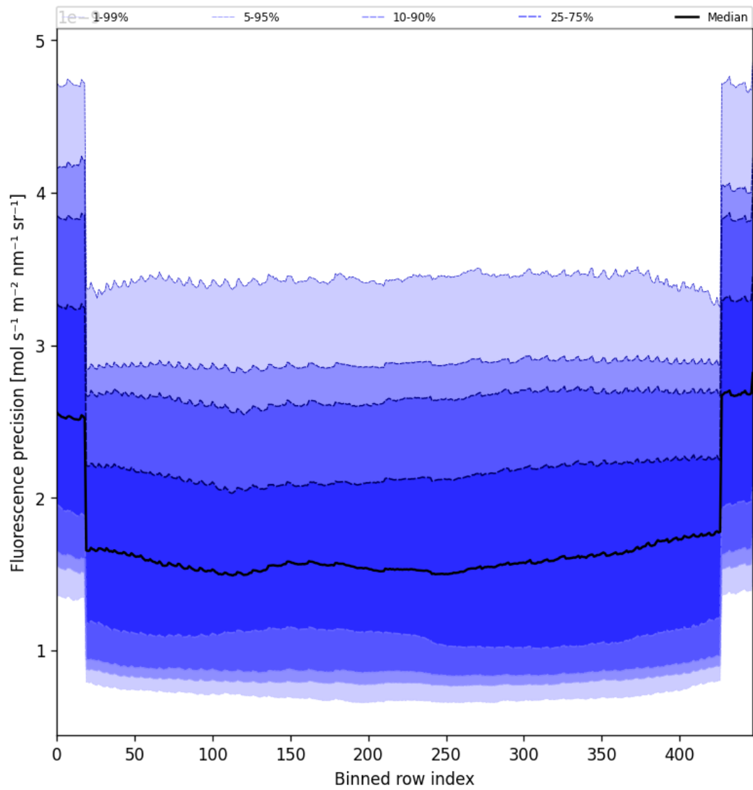
Figure 58: Along track statistics of “Fluorescence precision” for 2025-07-08 to 2025-07-09
