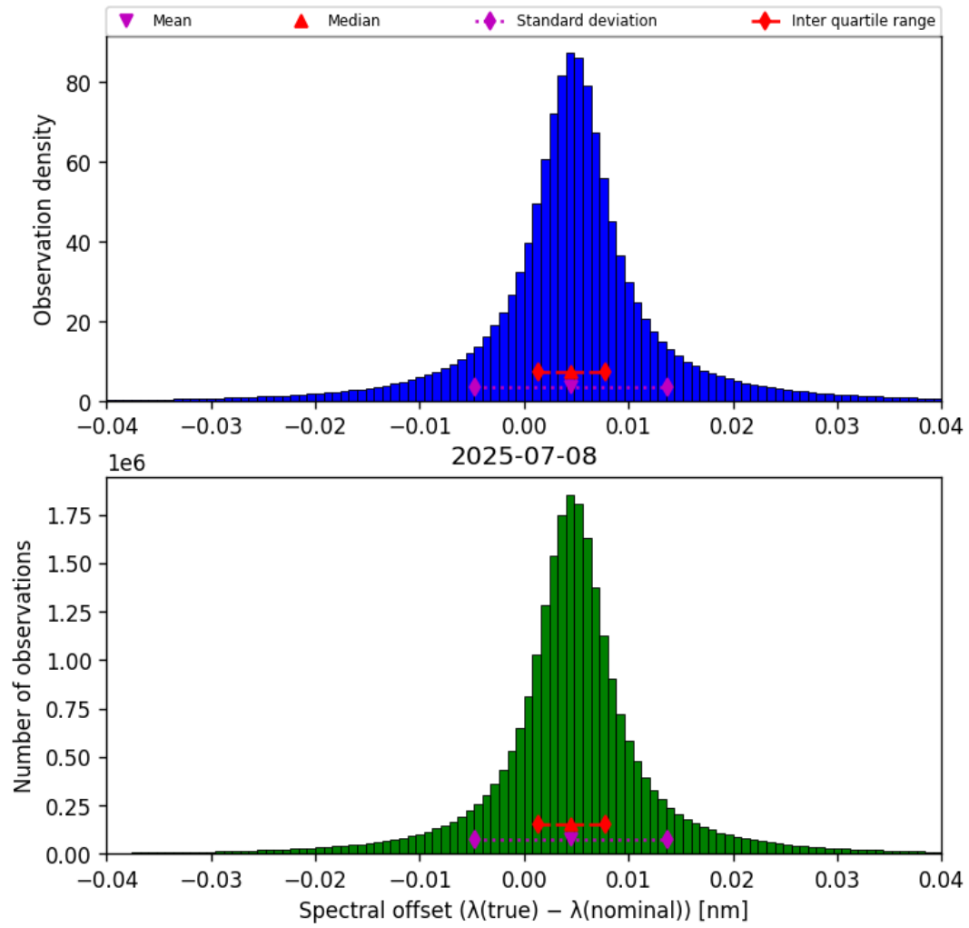
Figure 45: Histogram of “Spectral offset ( \lambda_{\text{true}} - \lambda_{\text{nominal}} )” for 2025-07-08 to 2025-07-09
