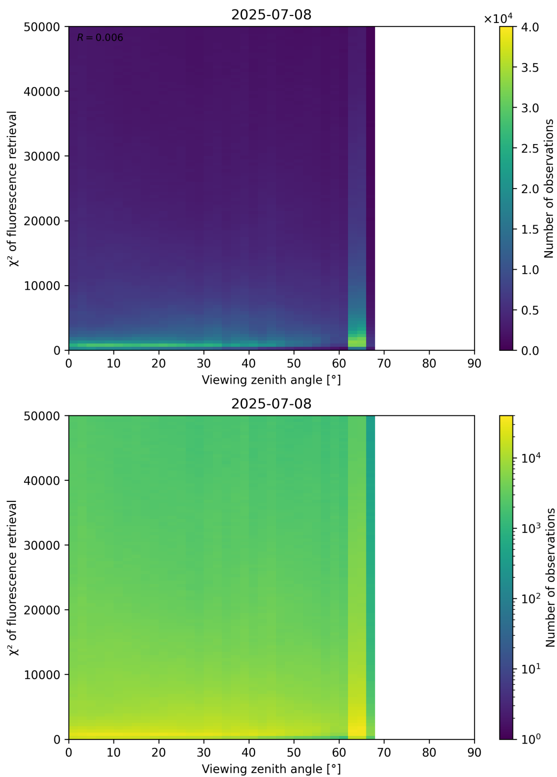
Figure 119: Scatter density plot of “Viewing zenith angle” against “ \chi^2 of fluorescence retrieval” for 2025-07-08 to 2025-07-09.
