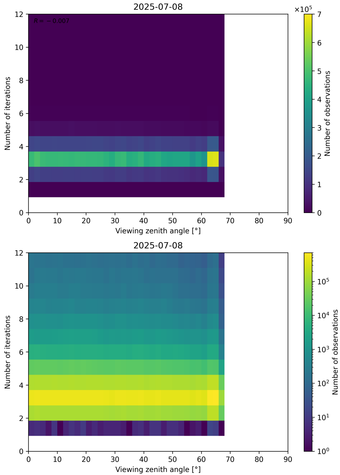
Figure 124: Scatter density plot of “Viewing zenith angle” against “Number of iterations” for 2025-07-08 to 2025-07-09.
