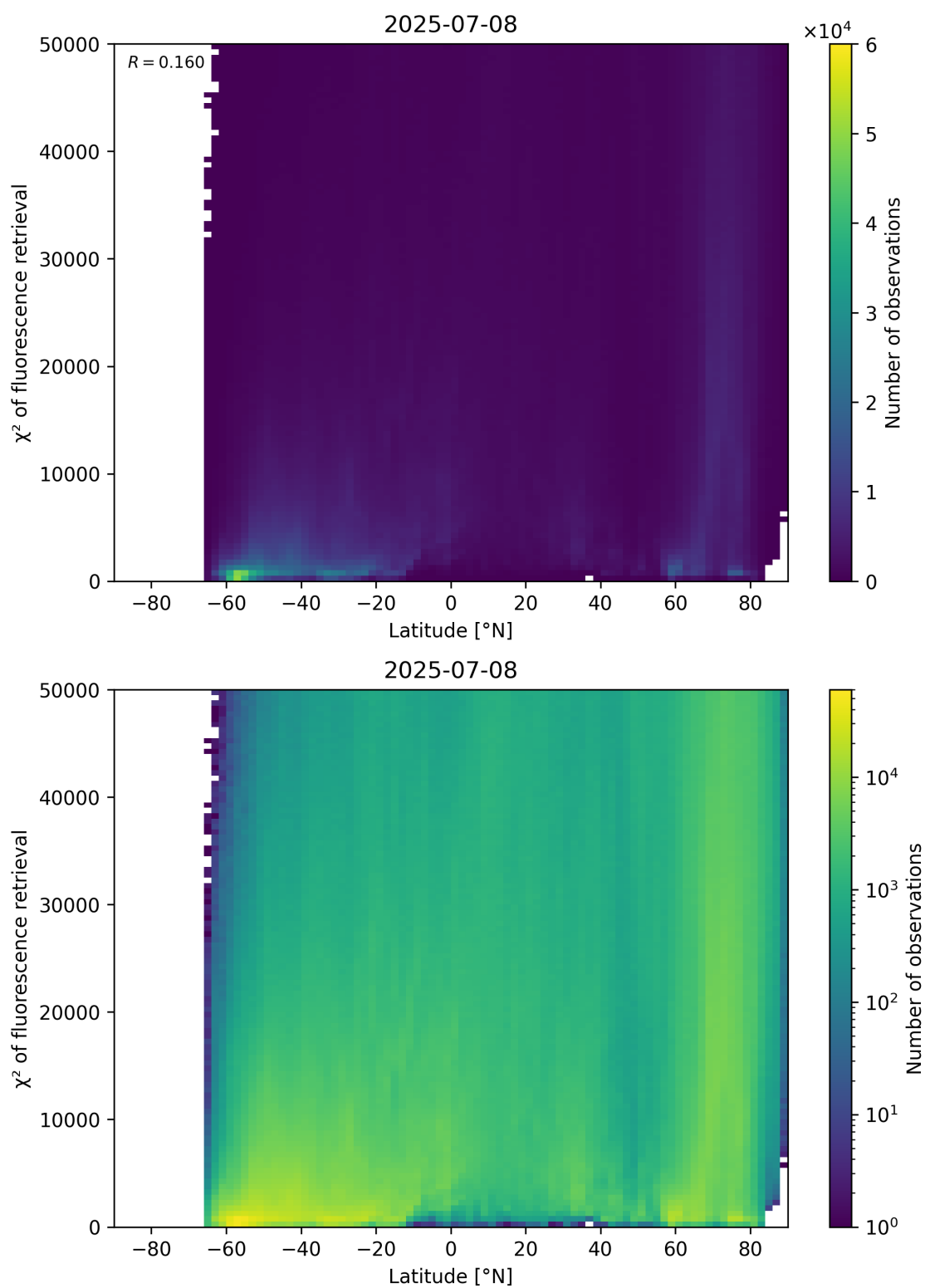
Figure 89: Scatter density plot of “Latitude” against “ \chi^2 of fluorescence retrieval” for 2025-07-08 to 2025-07-09.
