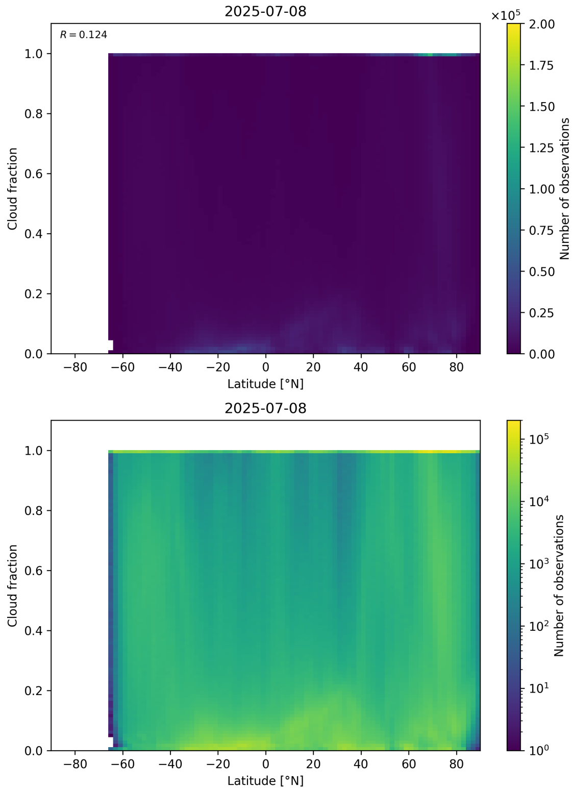
Figure 90: Scatter density plot of “Latitude” against “Cloud fraction” for 2025-07-08 to 2025-07-09.
