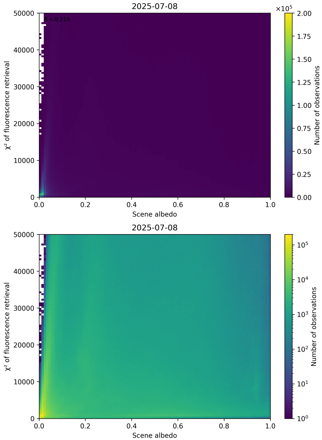
Figure 103: Scatter density plot of “Scene albedo” against “ \chi^2 of fluorescence retrieval” for 2025-07-08 to 2025-07-09.
