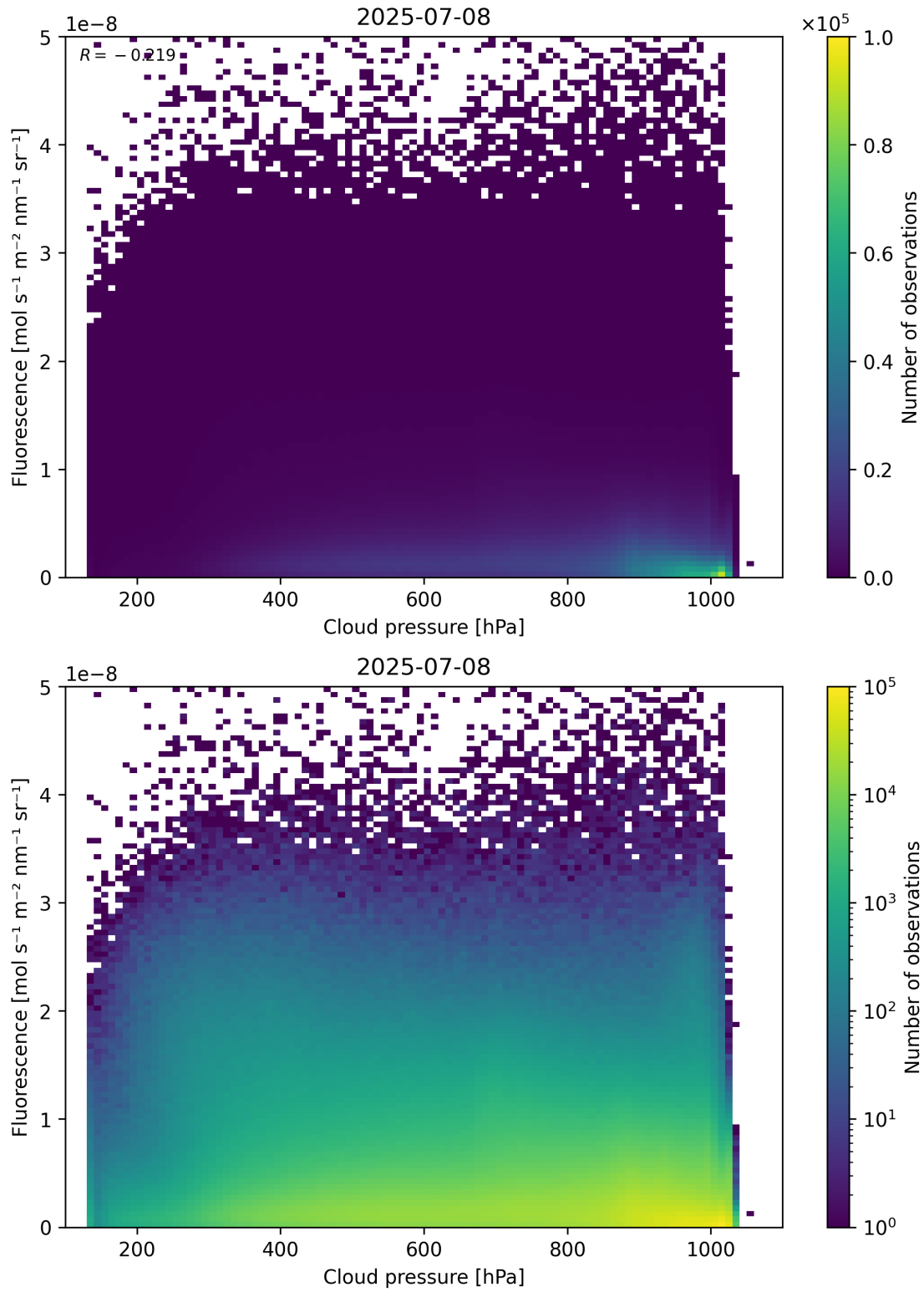
Figure 80: Scatter density plot of “Cloud pressure” against “Fluorescence” for 2025-07-08 to 2025-07-09.
