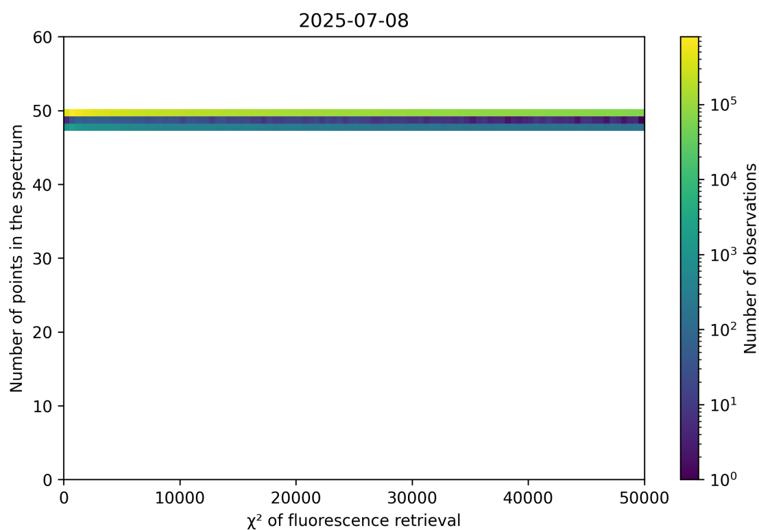
Figure 68: Scatter density plot of “ \chi^2 of fluorescence retrieval” against “Number of points in the spectrum” for 2025-07-08 to 2025-07-09.
