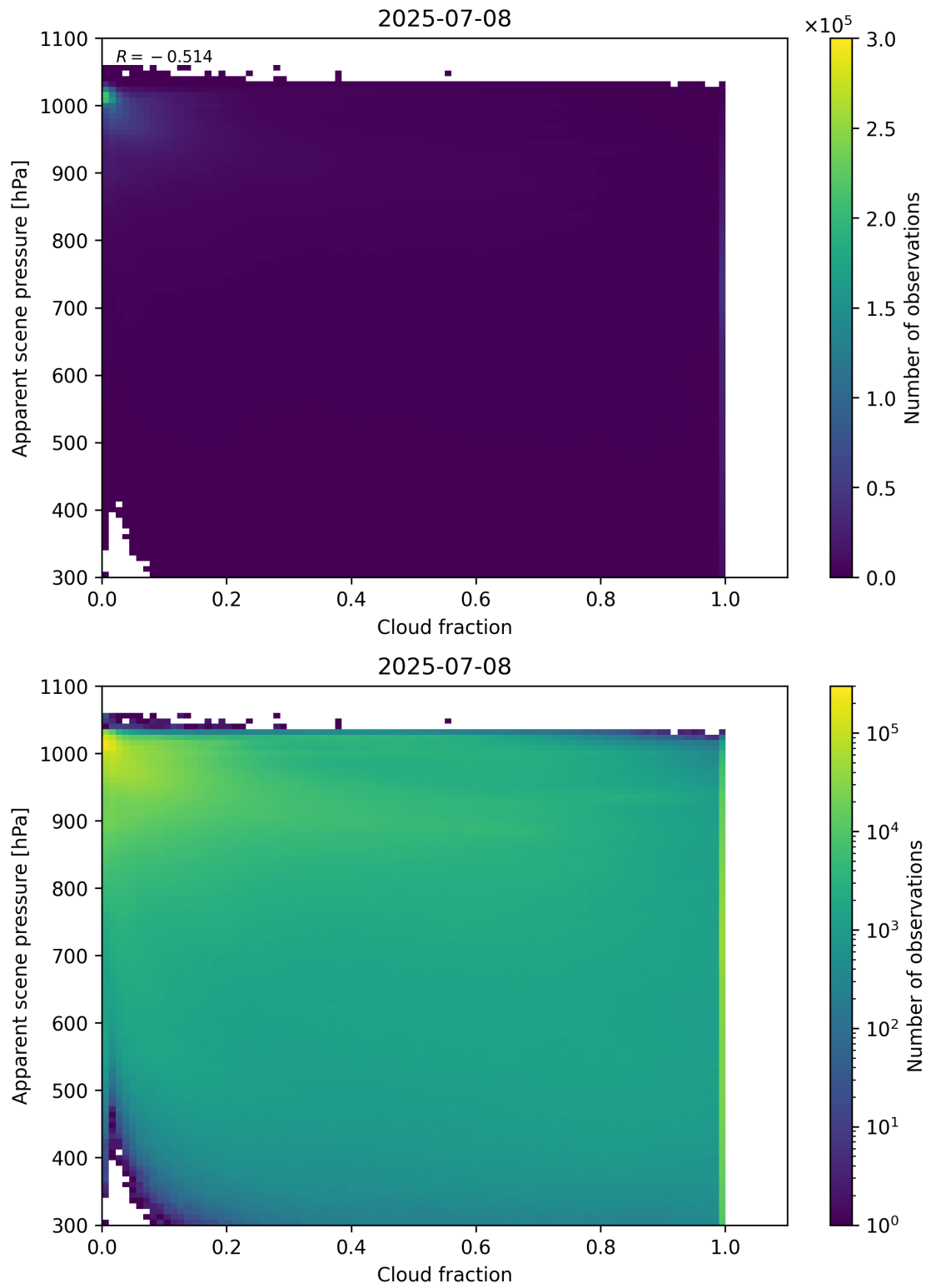
Figure 70: Scatter density plot of “Cloud fraction” against “Apparent scene pressure” for 2025-07-08 to 2025-07-09.
