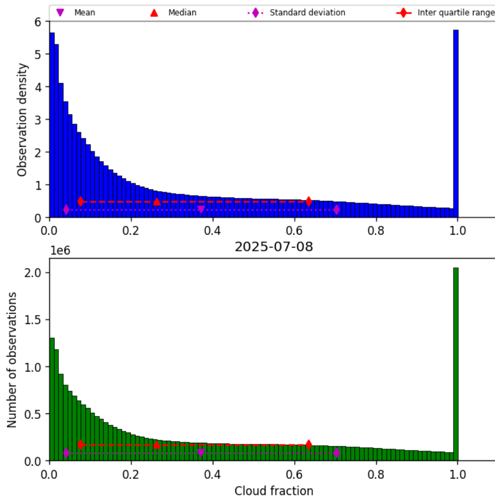
Figure 32: Histogram of “Cloud fraction” for 2025-07-08 to 2025-07-09
