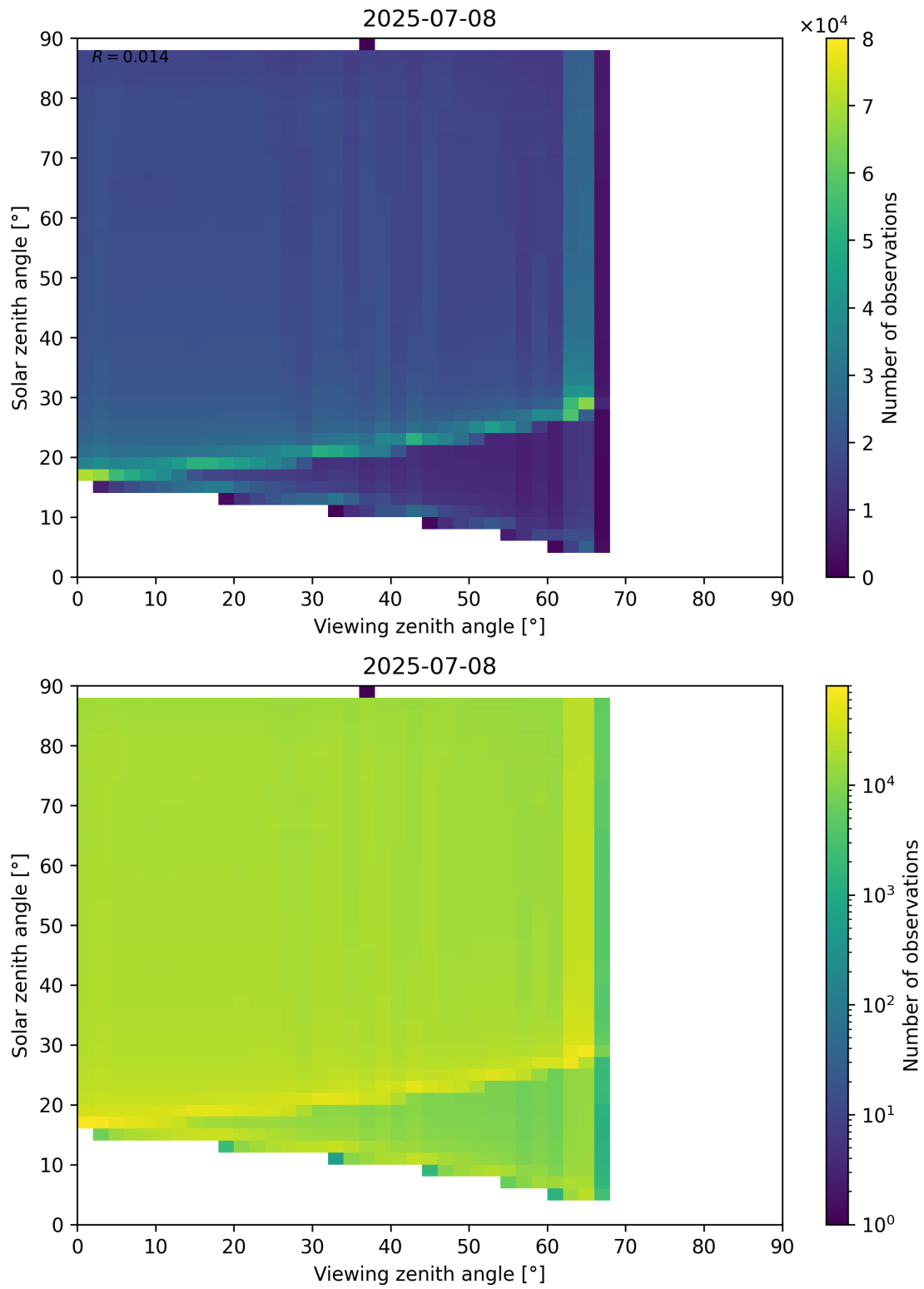
Figure 127: Scatter density plot of “Viewing zenith angle” against “Solar zenith angle” for 2025-07-08 to 2025-07-09.
