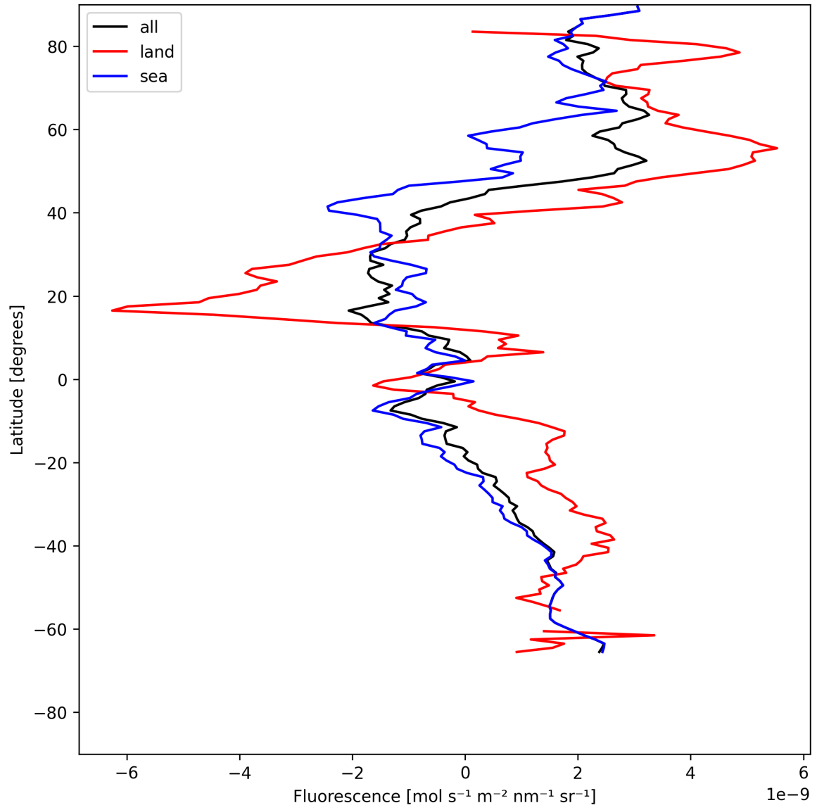
Figure 23: Zonal average of “Fluorescence” for 2025-07-08 to 2025-07-09.
