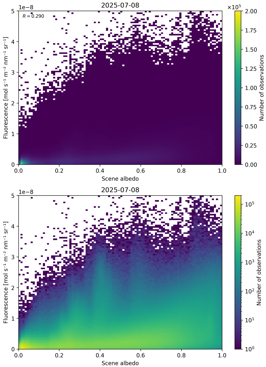
Figure 104: Scatter density plot of “Scene albedo” against “Fluorescence” for 2025-07-08 to 2025-07-09.
