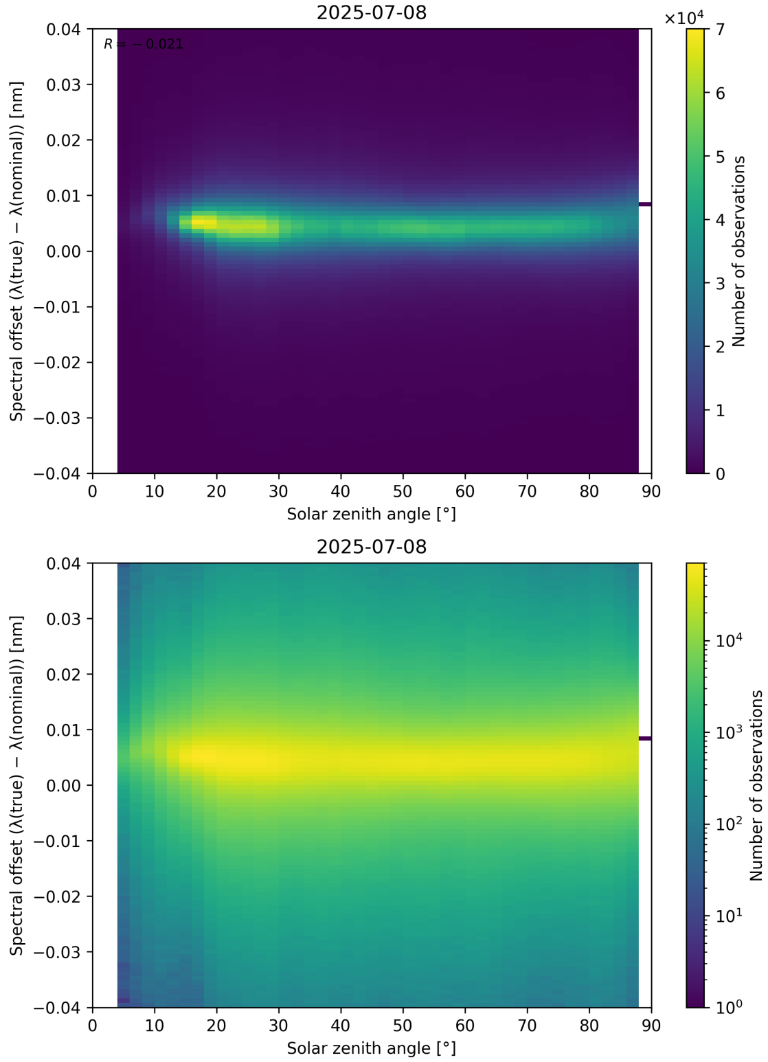
Figure 117: Scatter density plot of “Solar zenith angle” against “Spectral offset ( \lambda_{\text{true}} - \lambda_{\text{nominal}} )” for 2025-07-08 to 2025-07-09.
