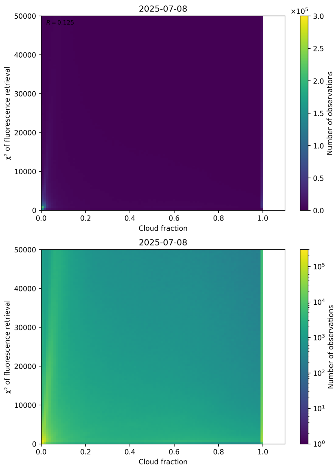
Figure 71: Scatter density plot of “Cloud fraction” against “ \chi^2 of fluorescence retrieval” for 2025-07-08 to 2025-07-09.
