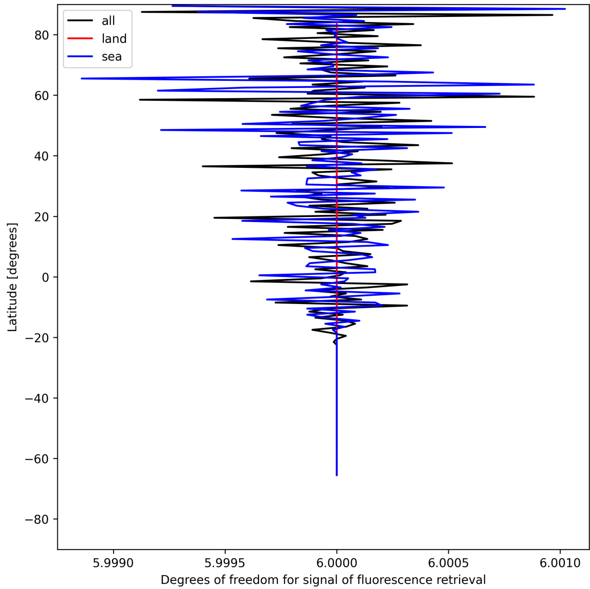
Figure 26: Zonal average of “Degrees of freedom for signal of fluorescence retrieval” for 2025-07-08 to 2025-07-09.
