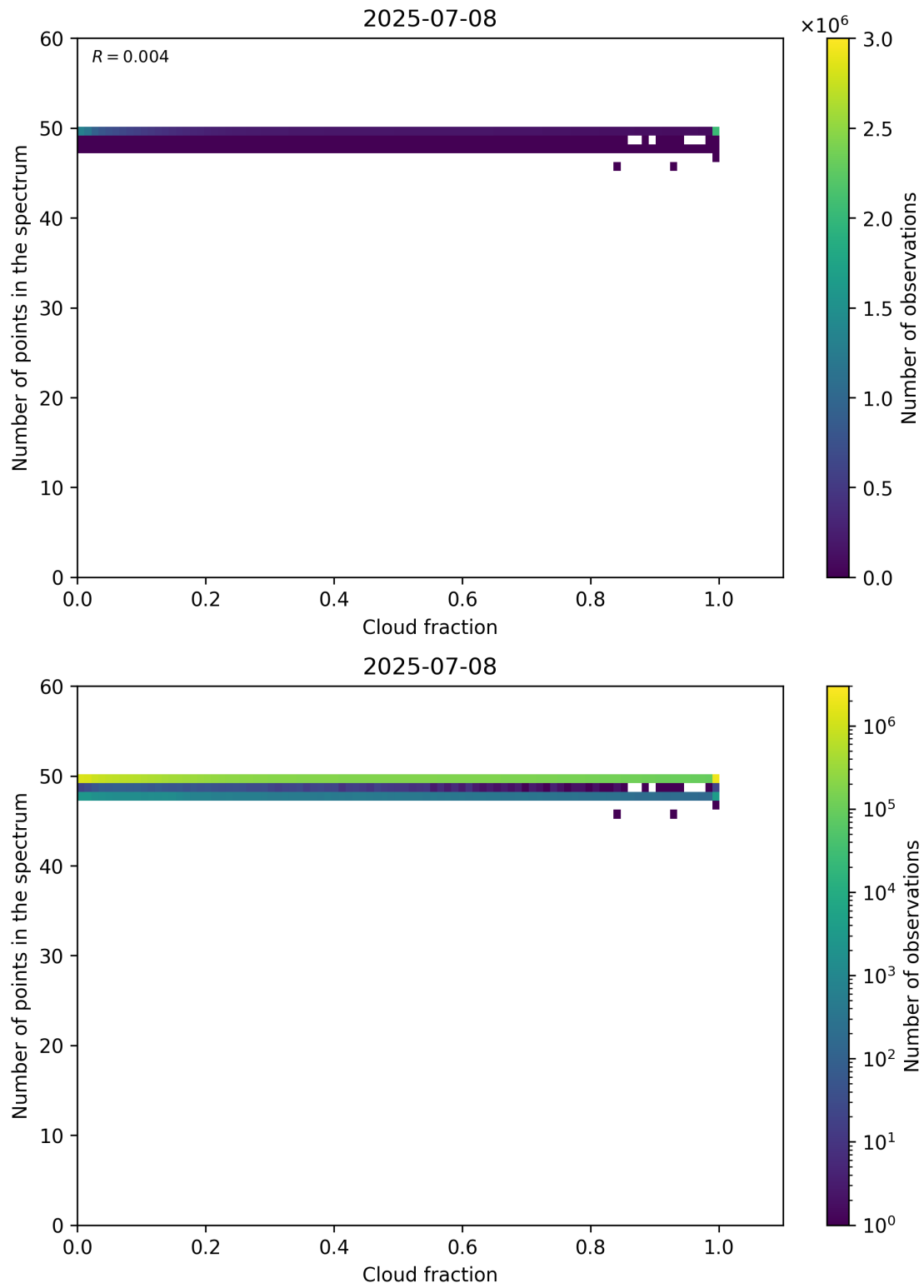
Figure 74: Scatter density plot of “Cloud fraction” against “Number of points in the spectrum” for 2025-07-08 to 2025-07-09.
