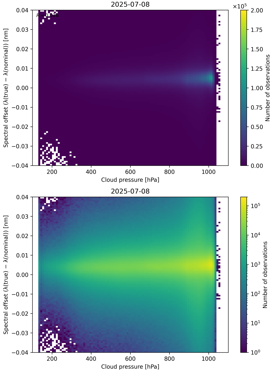
Figure 84: Scatter density plot of “Cloud pressure” against “Spectral offset ( \lambda_{\text{true}} - \lambda_{\text{nominal}} )” for 2025-07-08 to 2025-07-09.
