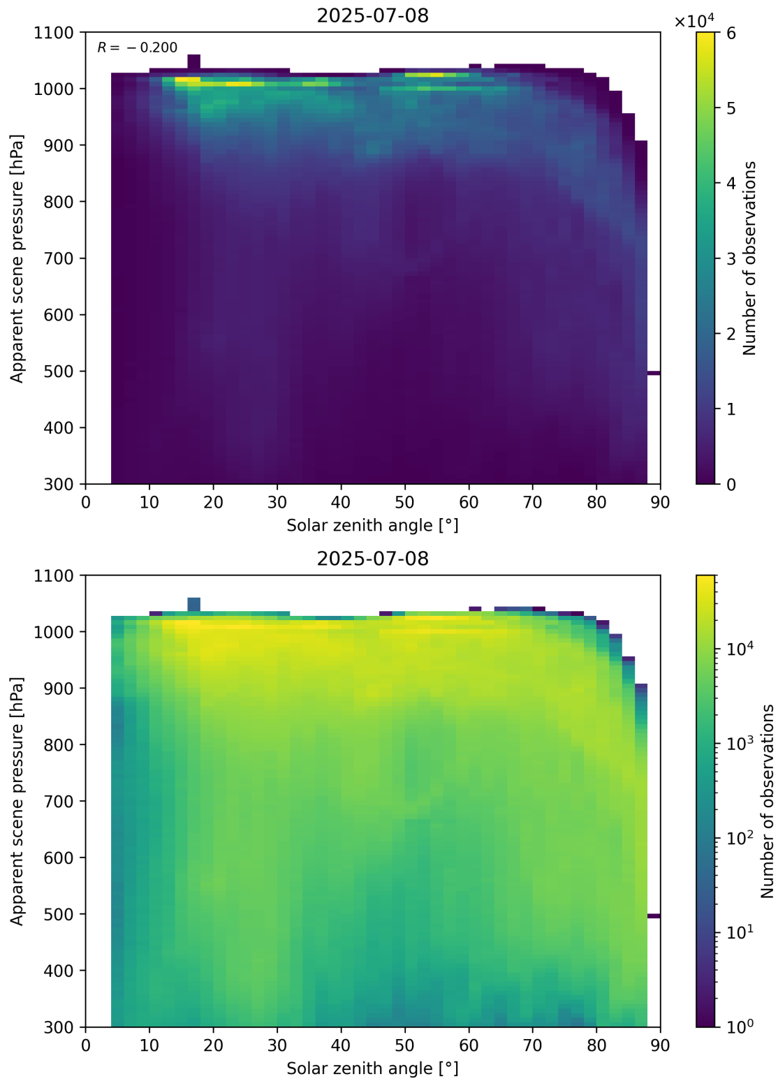
Figure 108: Scatter density plot of “Solar zenith angle” against “Apparent scene pressure” for 2025-07-08 to 2025-07-09.
