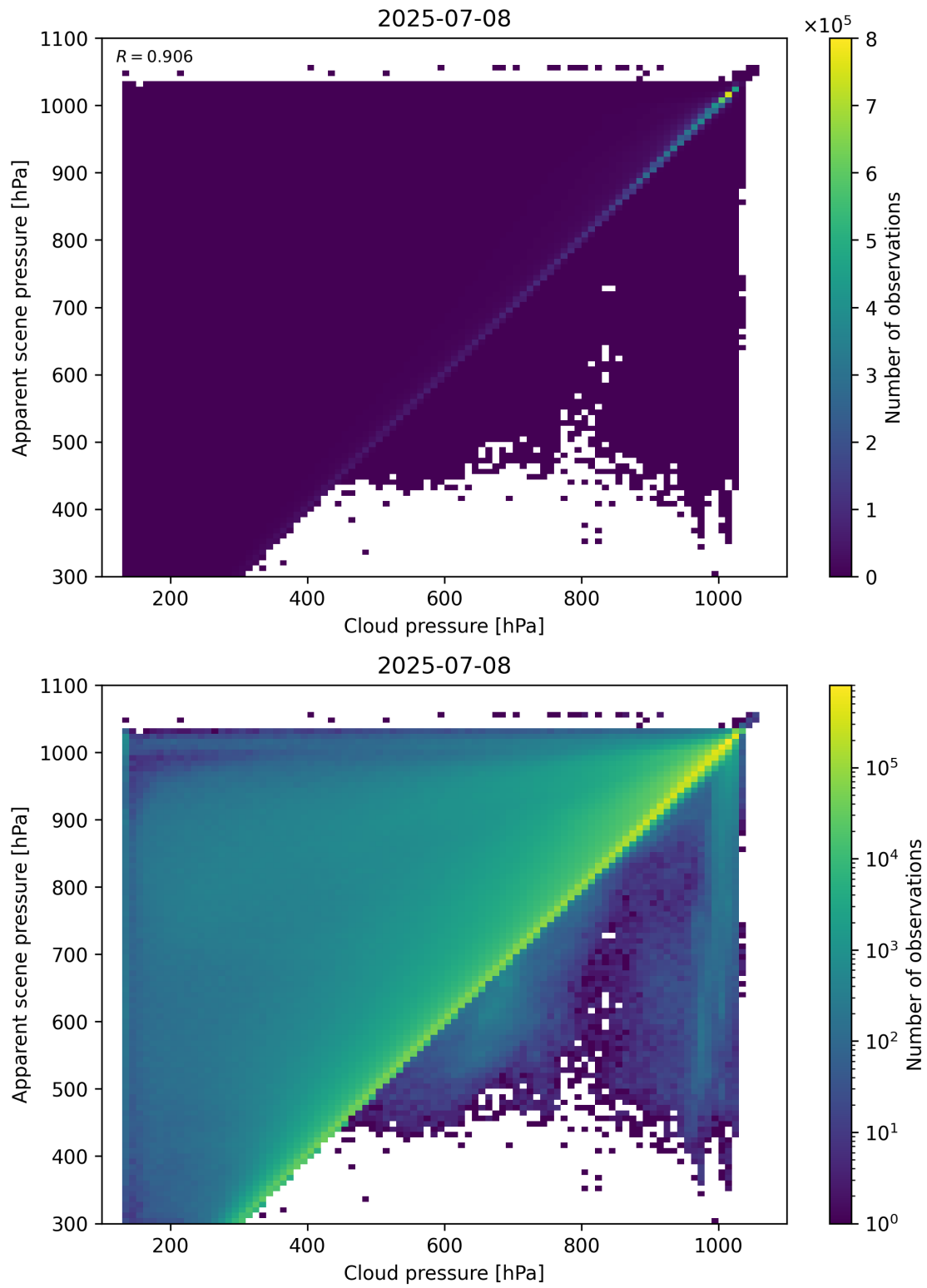
Figure 77: Scatter density plot of “Cloud pressure” against “Apparent scene pressure” for 2025-07-08 to 2025-07-09.
