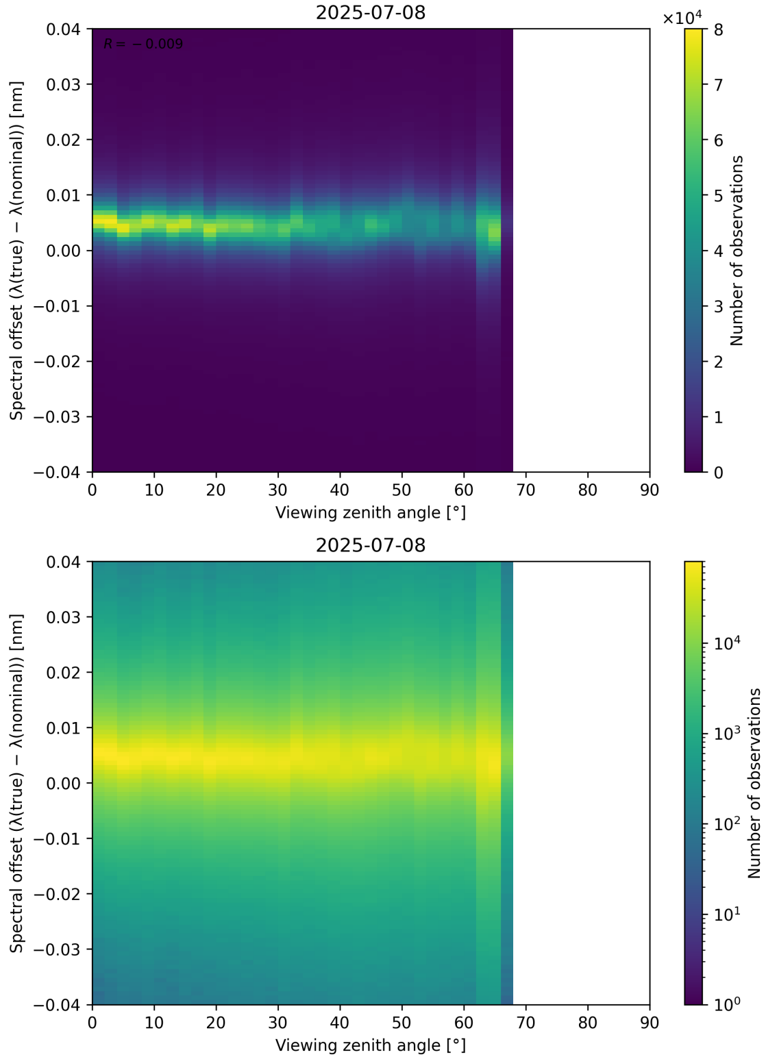
Figure 128: Scatter density plot of “Viewing zenith angle” against “Spectral offset ( \lambda_{\text{true}} - \lambda_{\text{nominal}} )” for 2025-07-08 to 2025-07-09.
