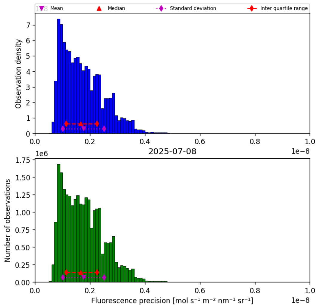
Figure 41: Histogram of “Fluorescence precision” for 2025-07-08 to 2025-07-09
