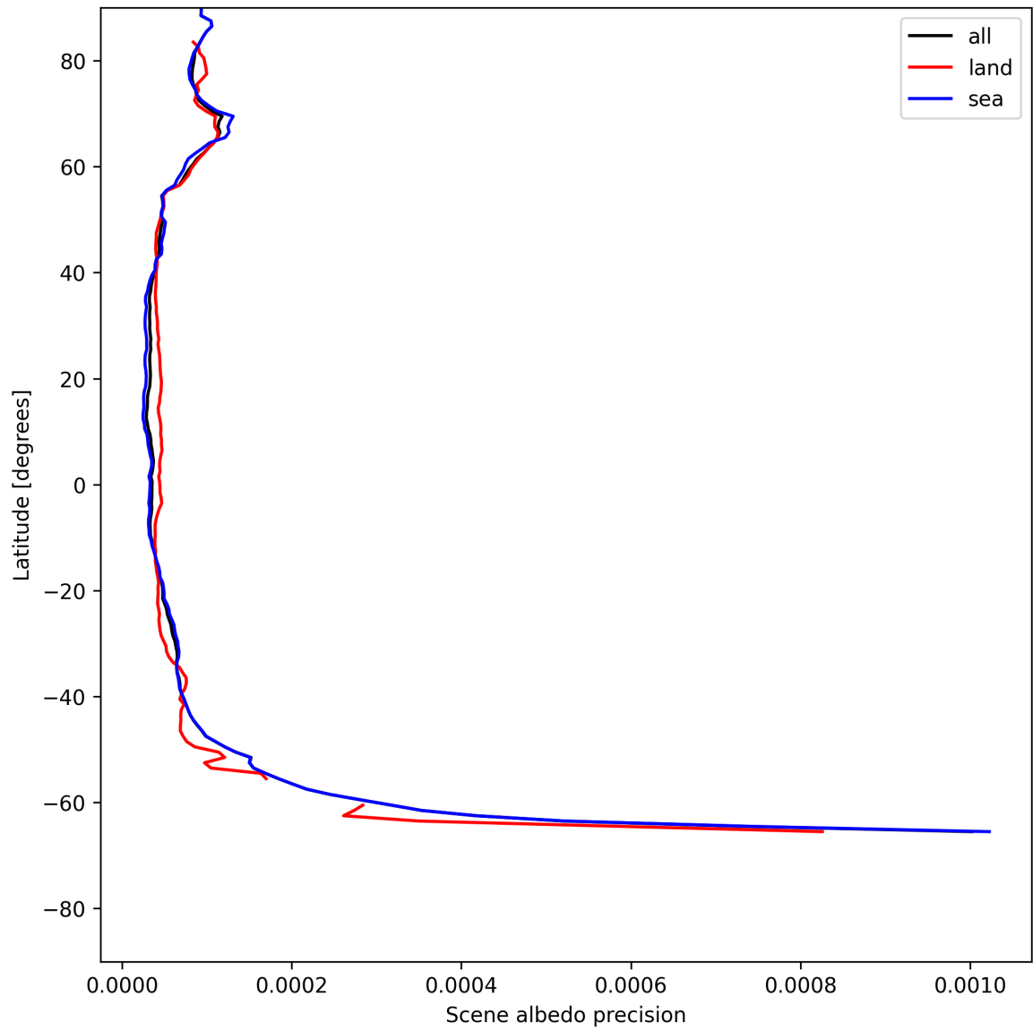
Figure 18: Zonal average of “Scene albedo precision” for 2025-07-08 to 2025-07-09.
