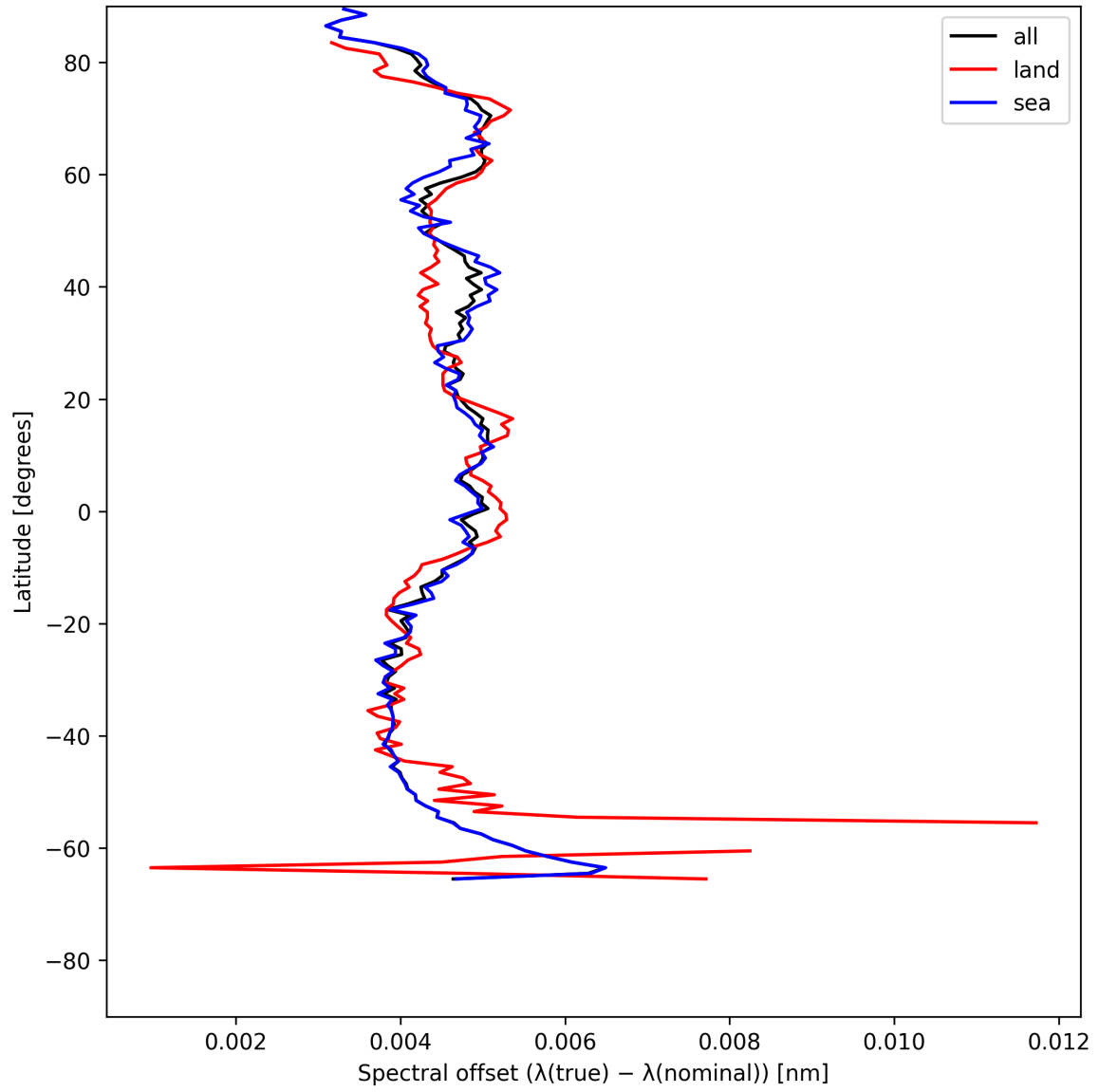
Figure 28: Zonal average of “Spectral offset ( \lambda_{\text{true}} - \lambda_{\text{nominal}} )” for 2025-07-08 to 2025-07-09.
