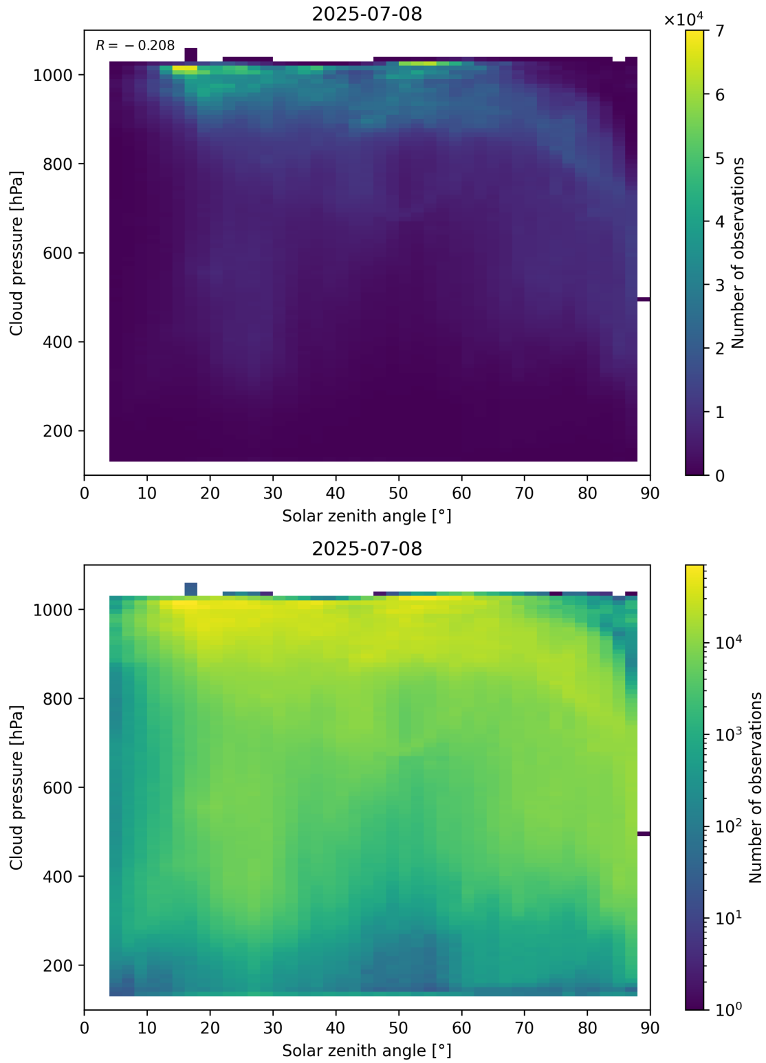
Figure 111: Scatter density plot of “Solar zenith angle” against “Cloud pressure” for 2025-07-08 to 2025-07-09.
