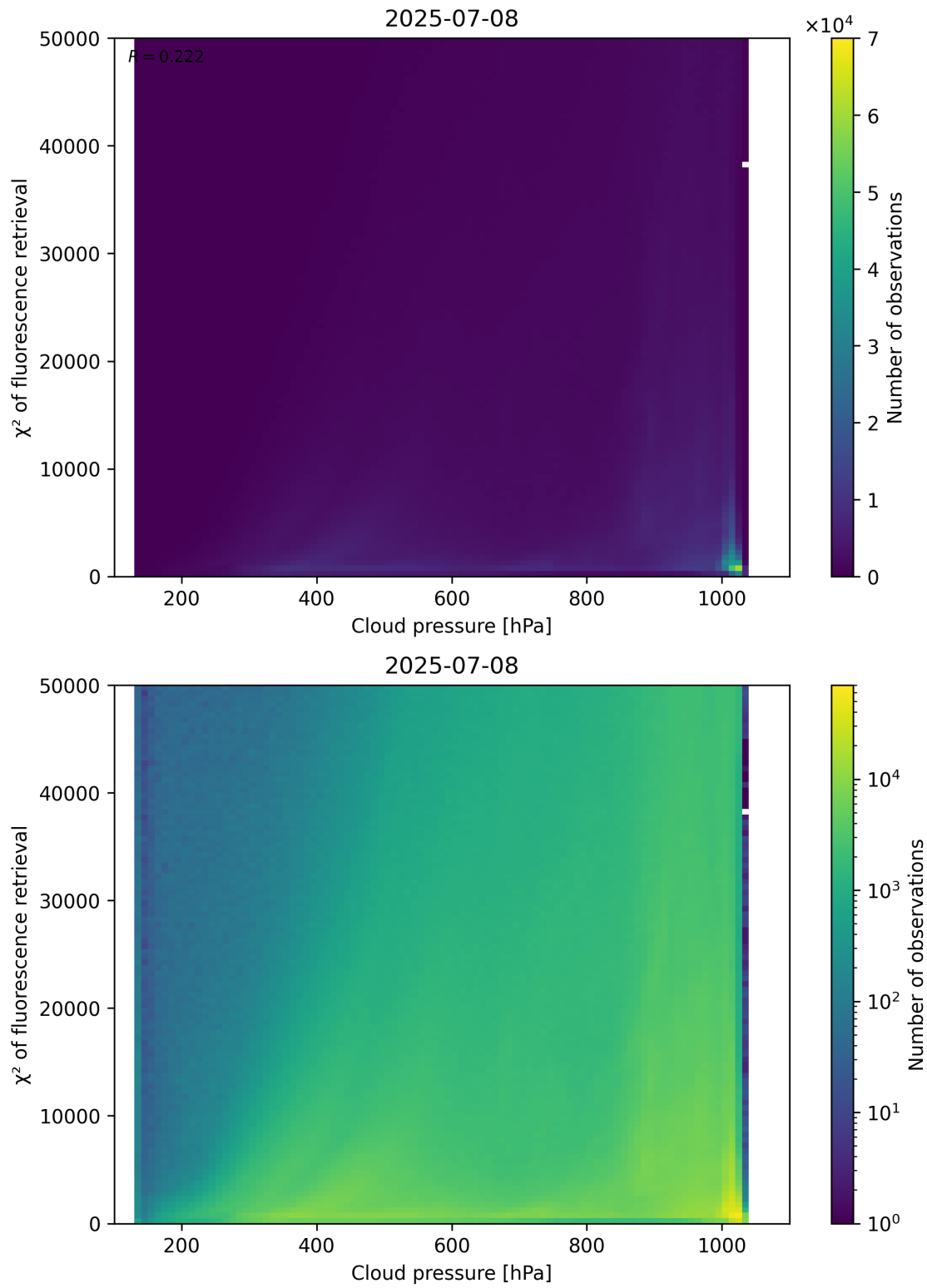
Figure 78: Scatter density plot of “Cloud pressure” against “ \chi^2 of fluorescence retrieval” for 2025-07-08 to 2025-07-09.
