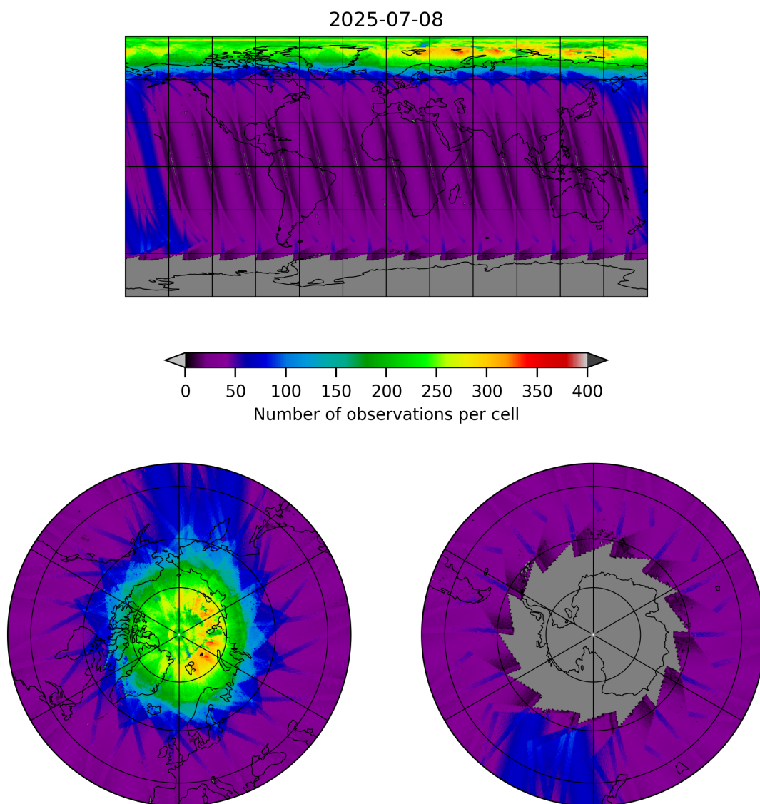
Figure 11: Map of the number of observations for 2025-07-08 to 2025-07-09
