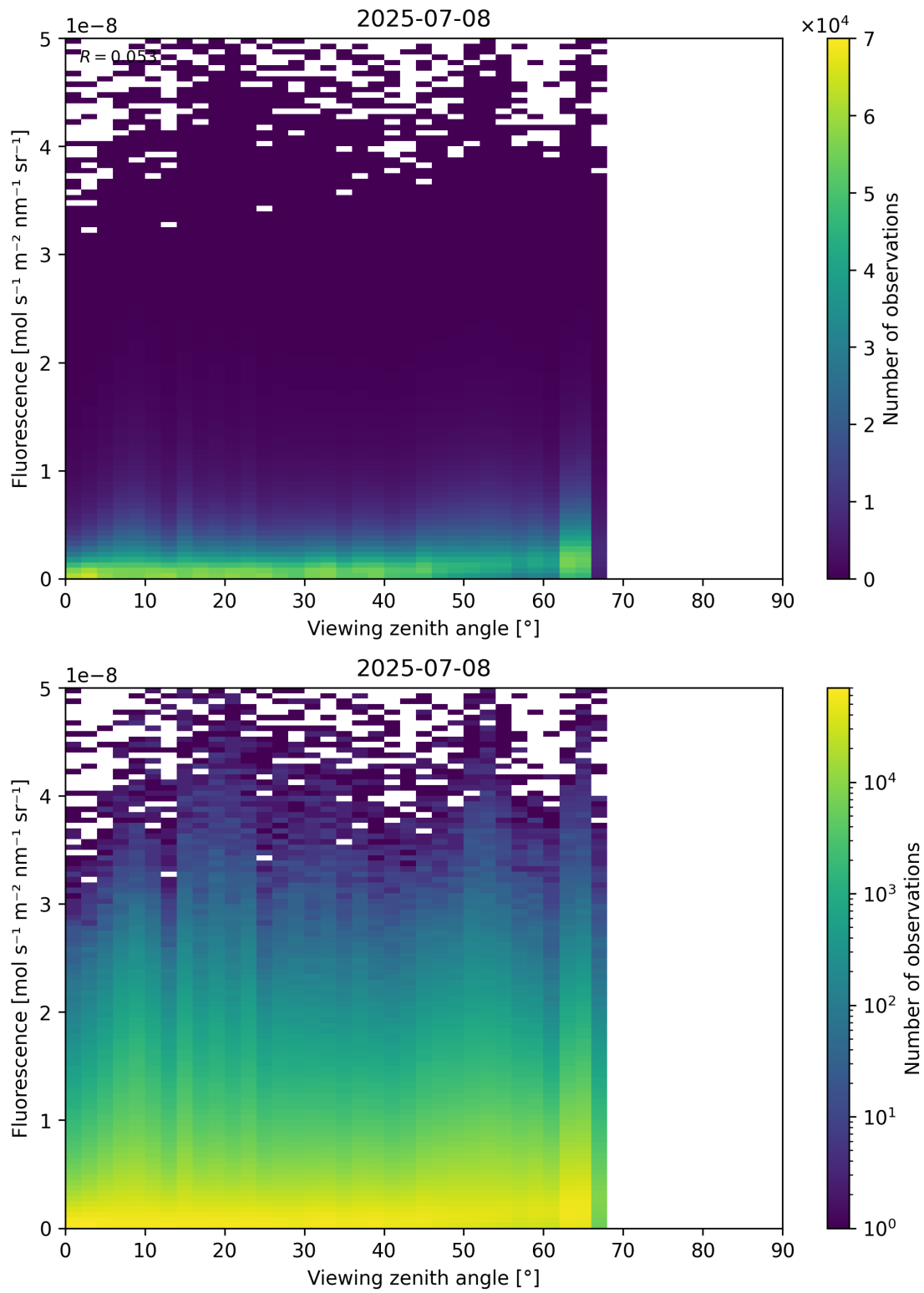
Figure 122: Scatter density plot of “Viewing zenith angle” against “Fluorescence” for 2025-07-08 to 2025-07-09.
