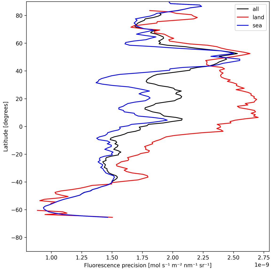
Figure 24: Zonal average of “Fluorescence precision” for 2025-07-08 to 2025-07-09.
