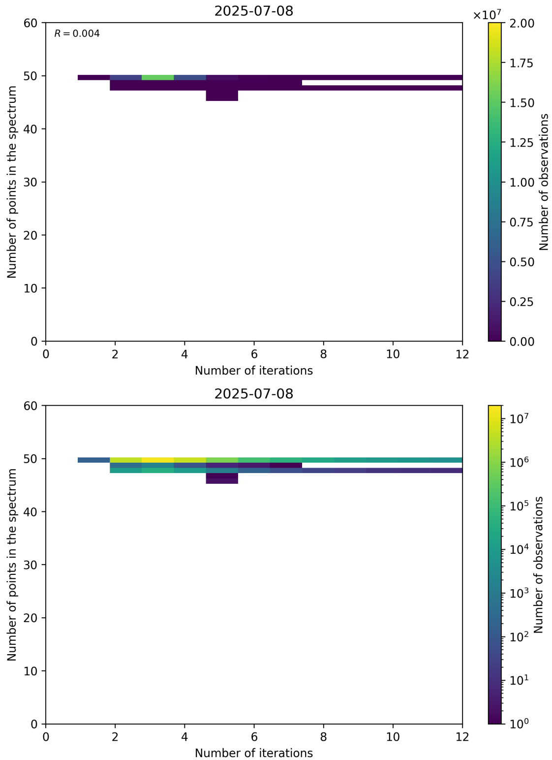
Figure 99: Scatter density plot of “Number of iterations” against “Number of points in the spectrum” for 2025-07-08 to 2025-07-09.
