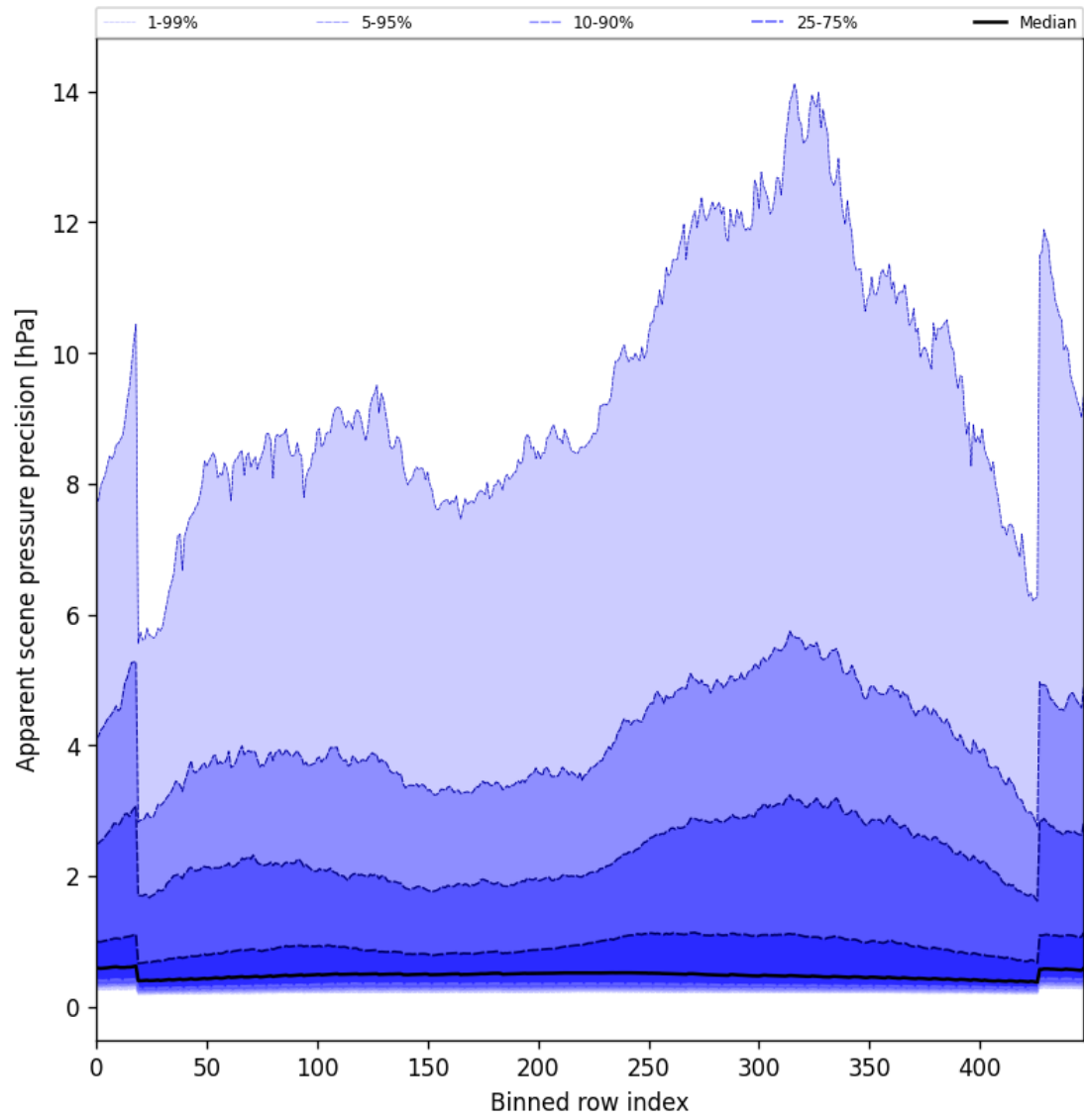
Figure 54: Along track statistics of “Apparent scene pressure precision” for 2025-07-08 to 2025-07-09
