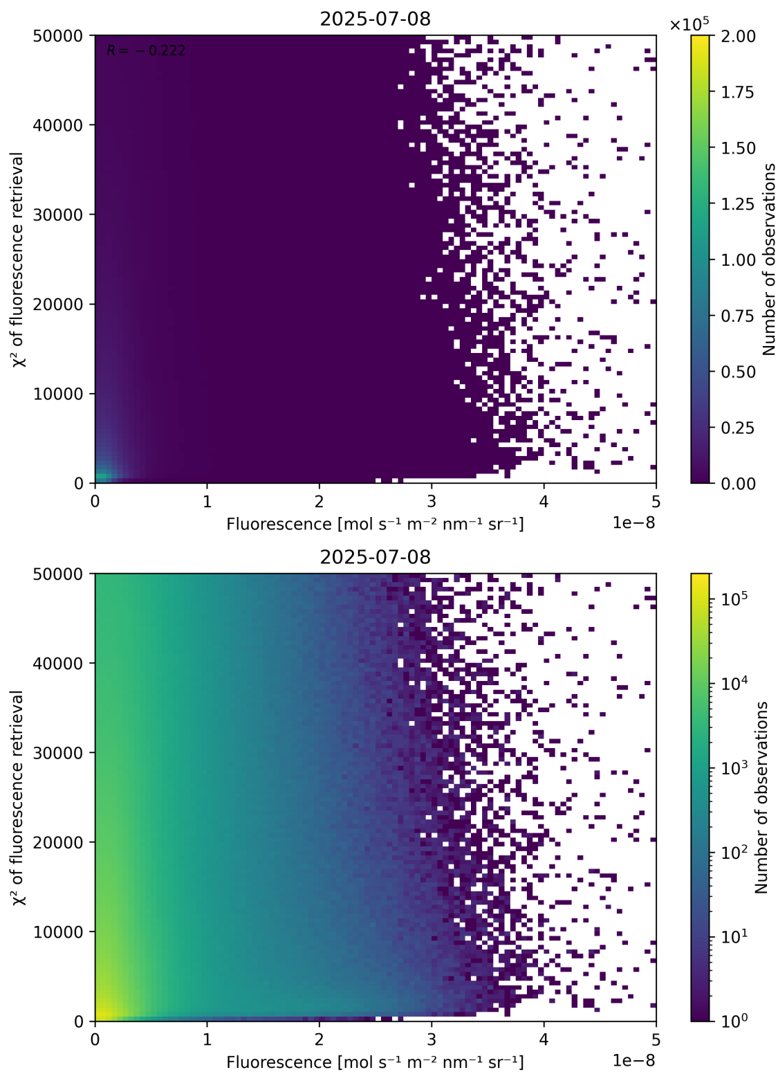
Figure 85: Scatter density plot of “Fluorescence” against “ \chi^2 of fluorescence retrieval” for 2025-07-08 to 2025-07-09.
