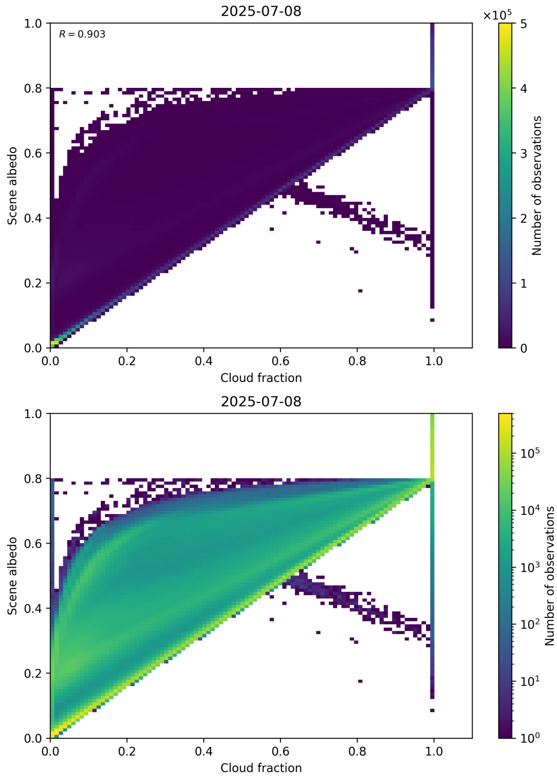
Figure 75: Scatter density plot of “Cloud fraction” against “Scene albedo” for 2025-07-08 to 2025-07-09.
