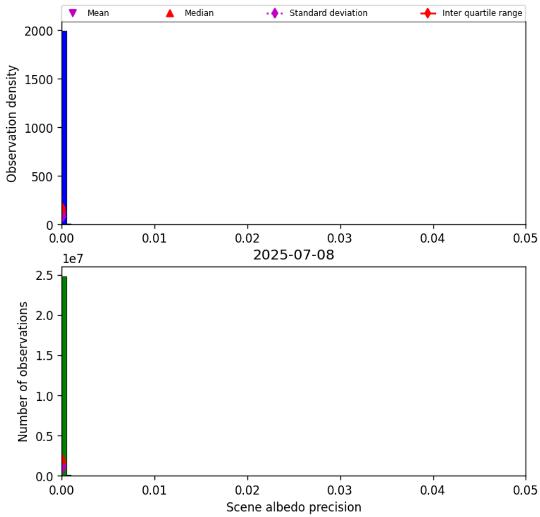
Figure 35: Histogram of “Scene albedo precision” for 2025-07-08 to 2025-07-09
