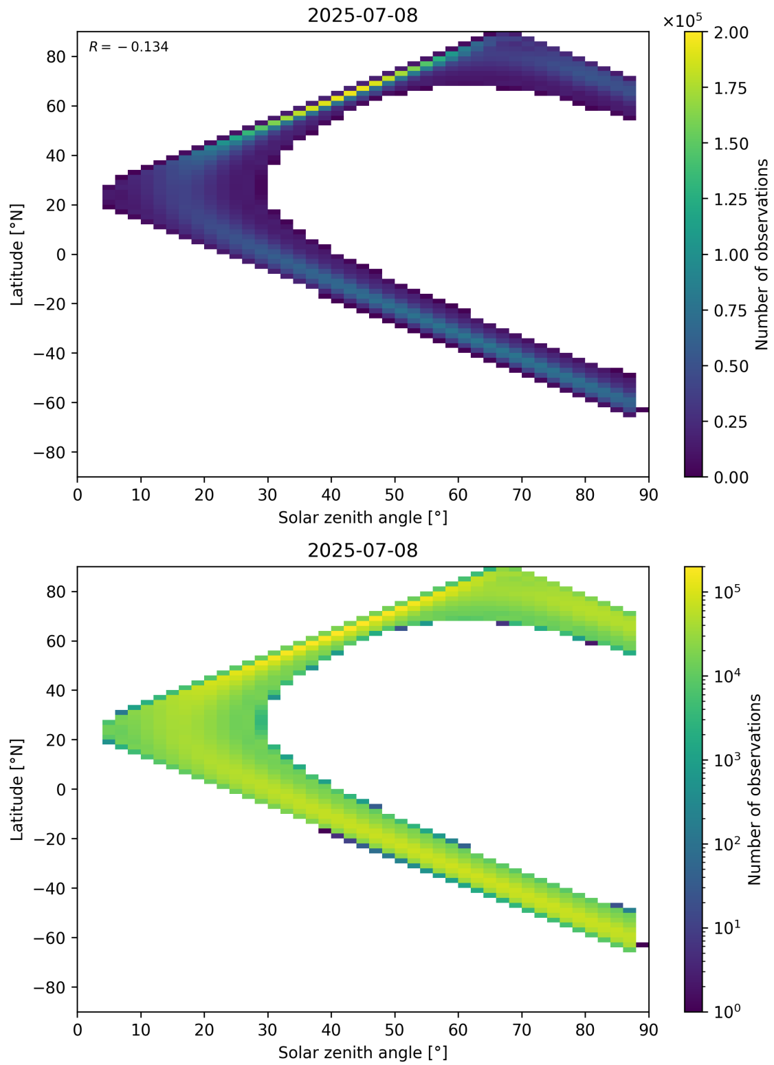
Figure 113: Scatter density plot of “Solar zenith angle” against “Latitude” for 2025-07-08 to 2025-07-09.
