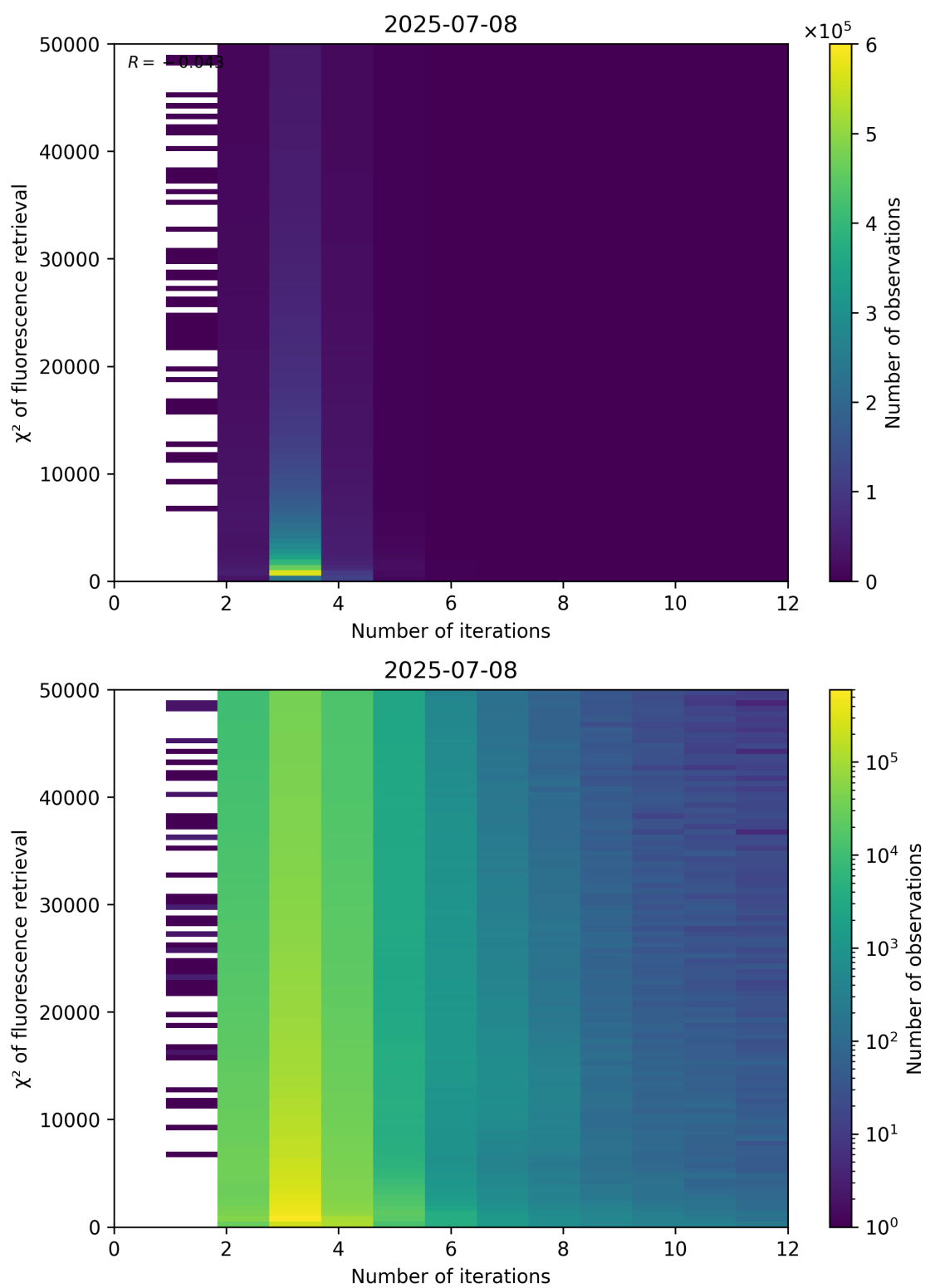
Figure 97: Scatter density plot of “Number of iterations” against “ \chi^2 of fluorescence retrieval” for 2025-07-08 to 2025-07-09.
