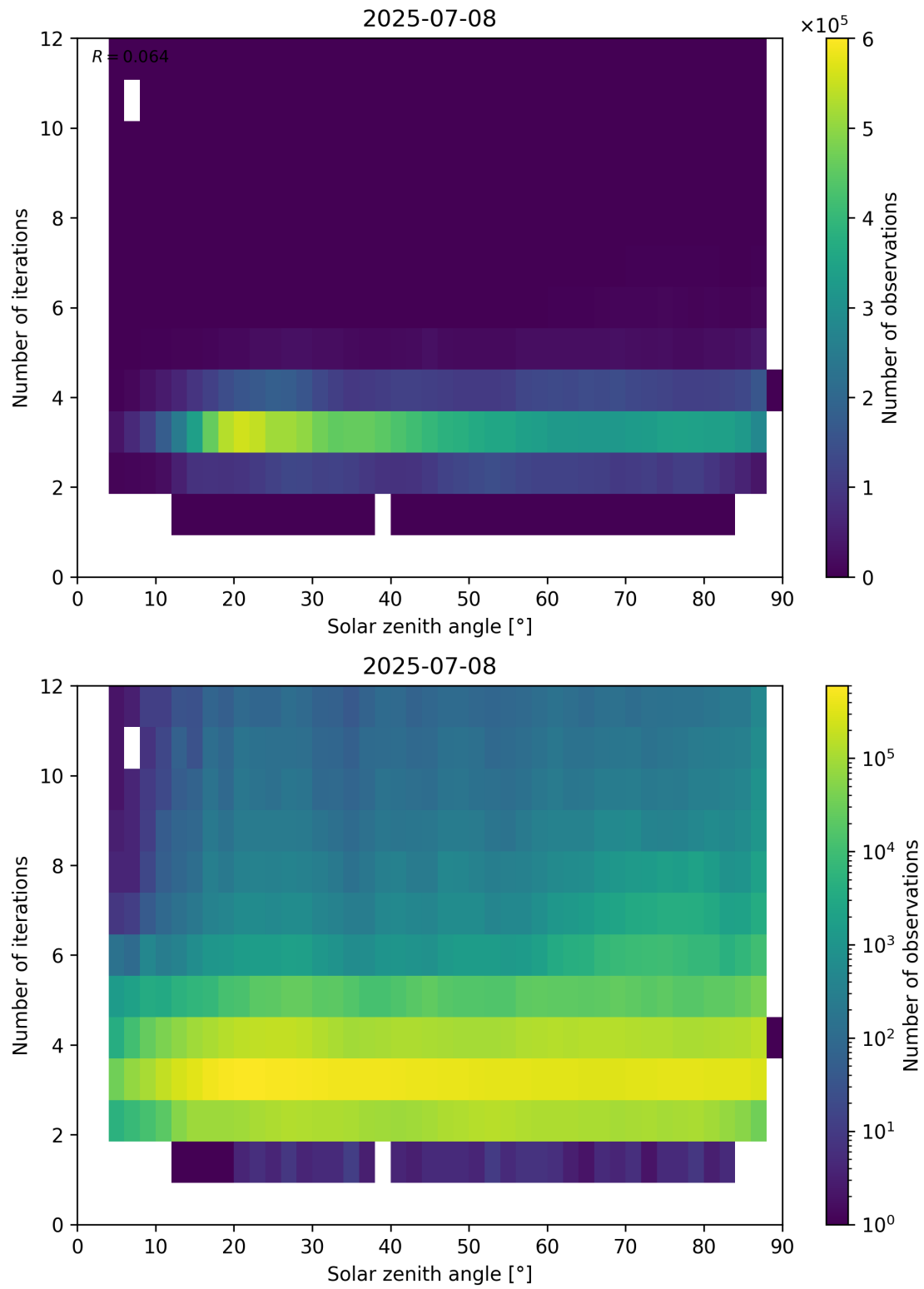
Figure 114: Scatter density plot of “Solar zenith angle” against “Number of iterations” for 2025-07-08 to 2025-07-09.
