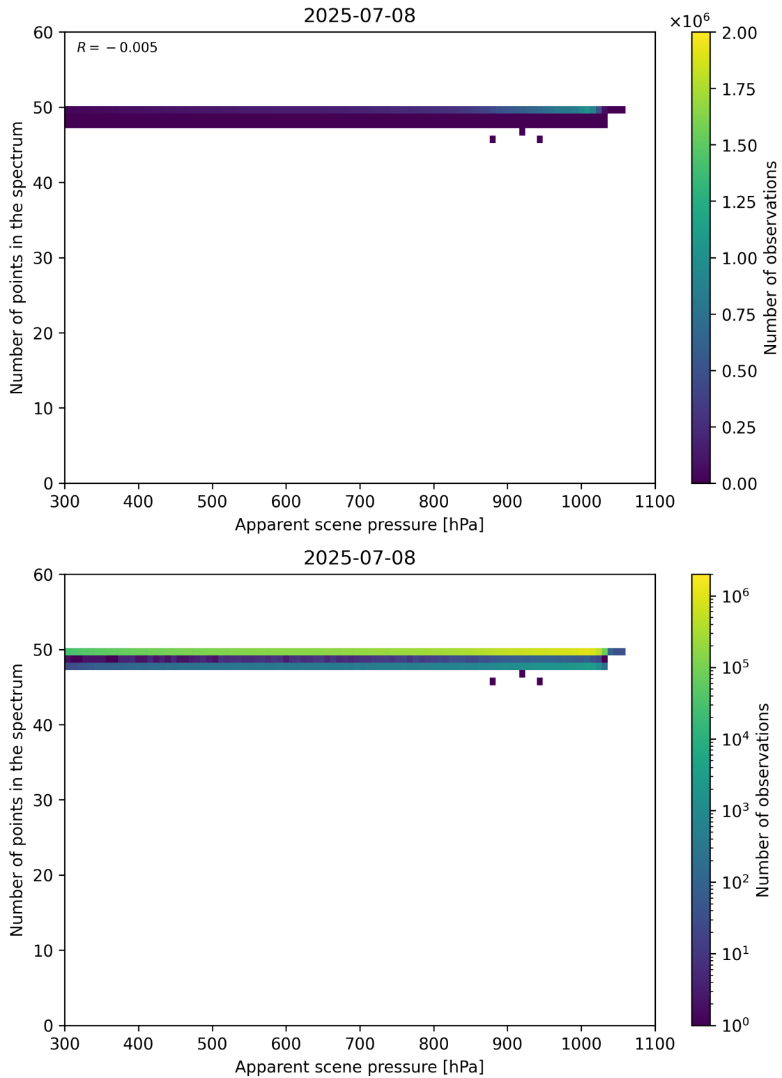
Figure 66: Scatter density plot of “Apparent scene pressure” against “Number of points in the spectrum” for 2025-07-08 to 2025-07-09.
