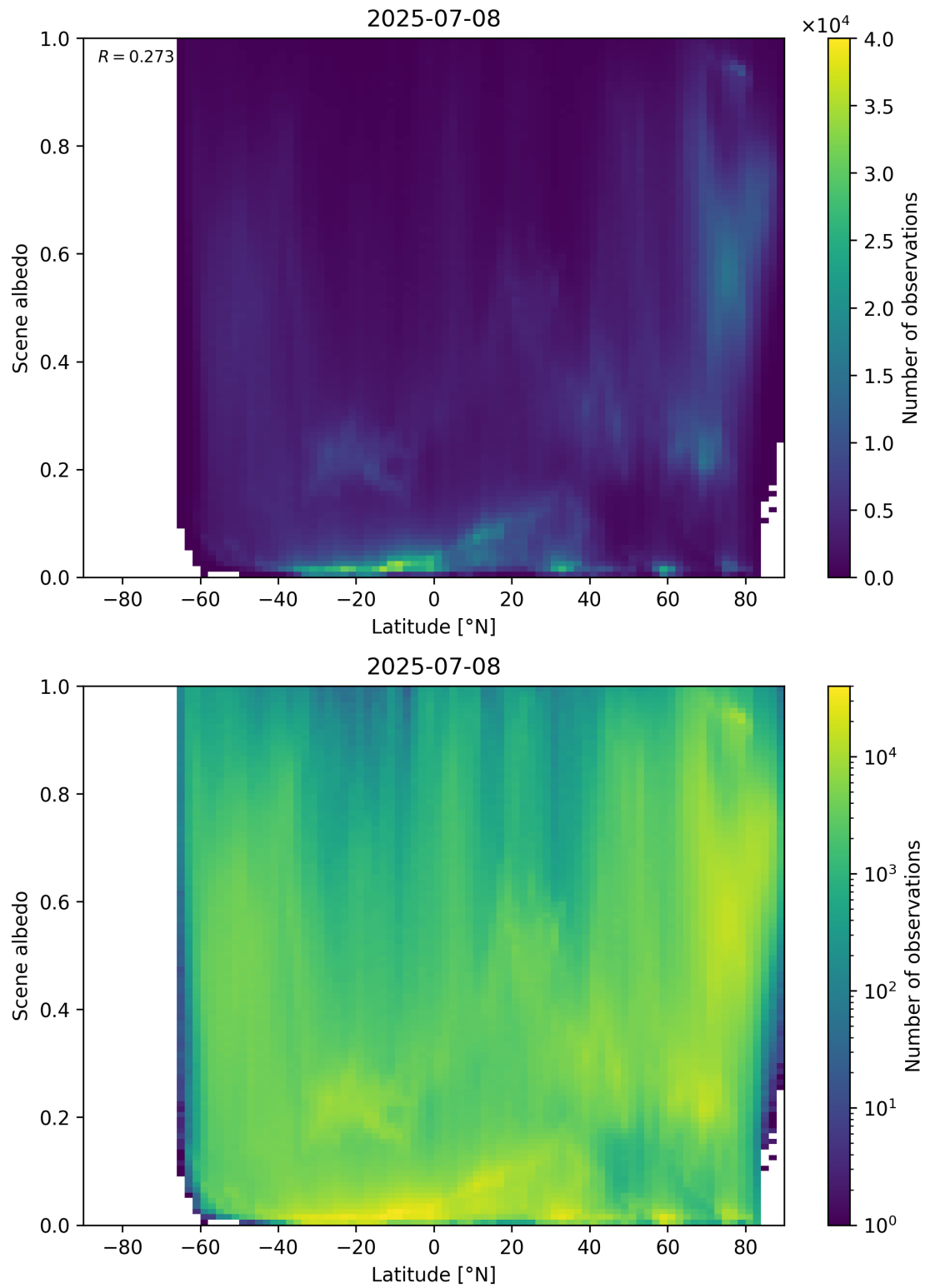
Figure 95: Scatter density plot of “Latitude” against “Scene albedo” for 2025-07-08 to 2025-07-09.
