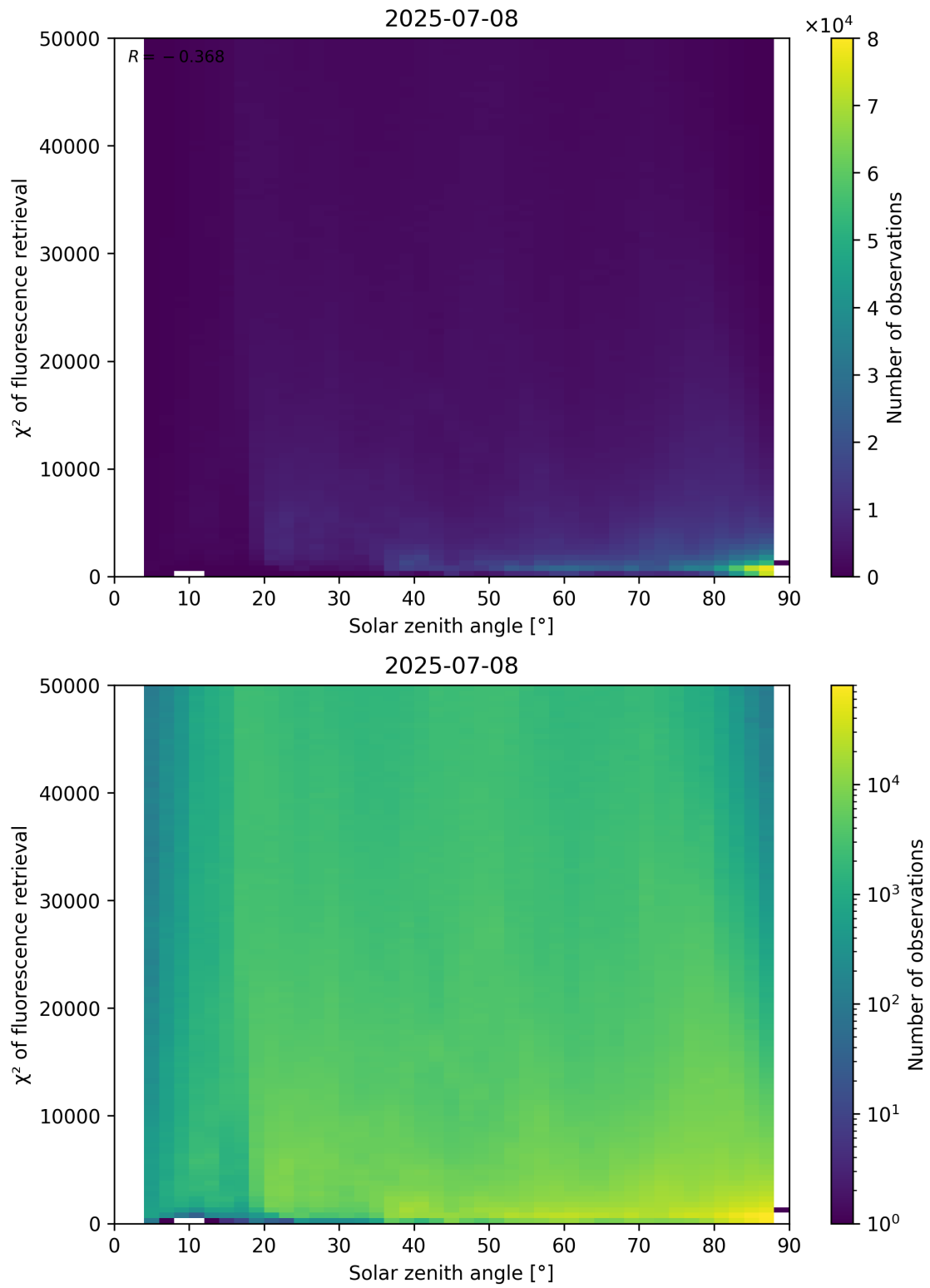
Figure 109: Scatter density plot of “Solar zenith angle” against “ \chi^2 of fluorescence retrieval” for 2025-07-08 to 2025-07-09.
