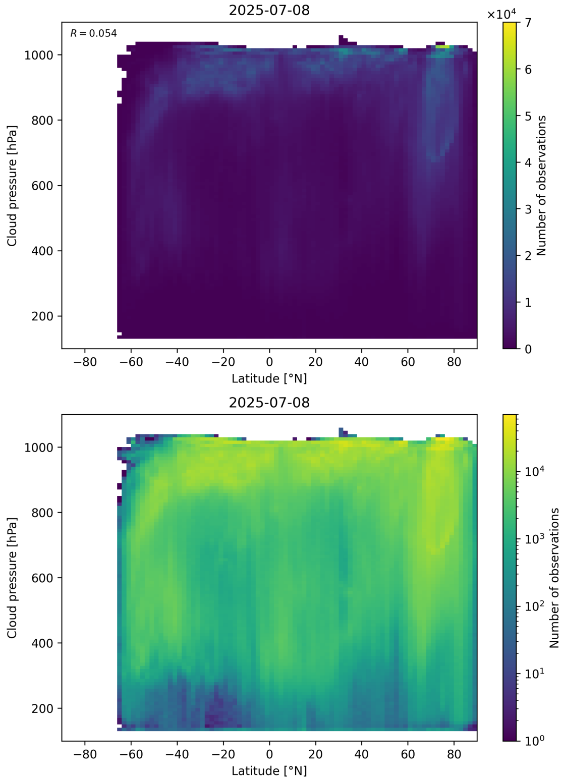
Figure 91: Scatter density plot of “Latitude” against “Cloud pressure” for 2025-07-08 to 2025-07-09.
