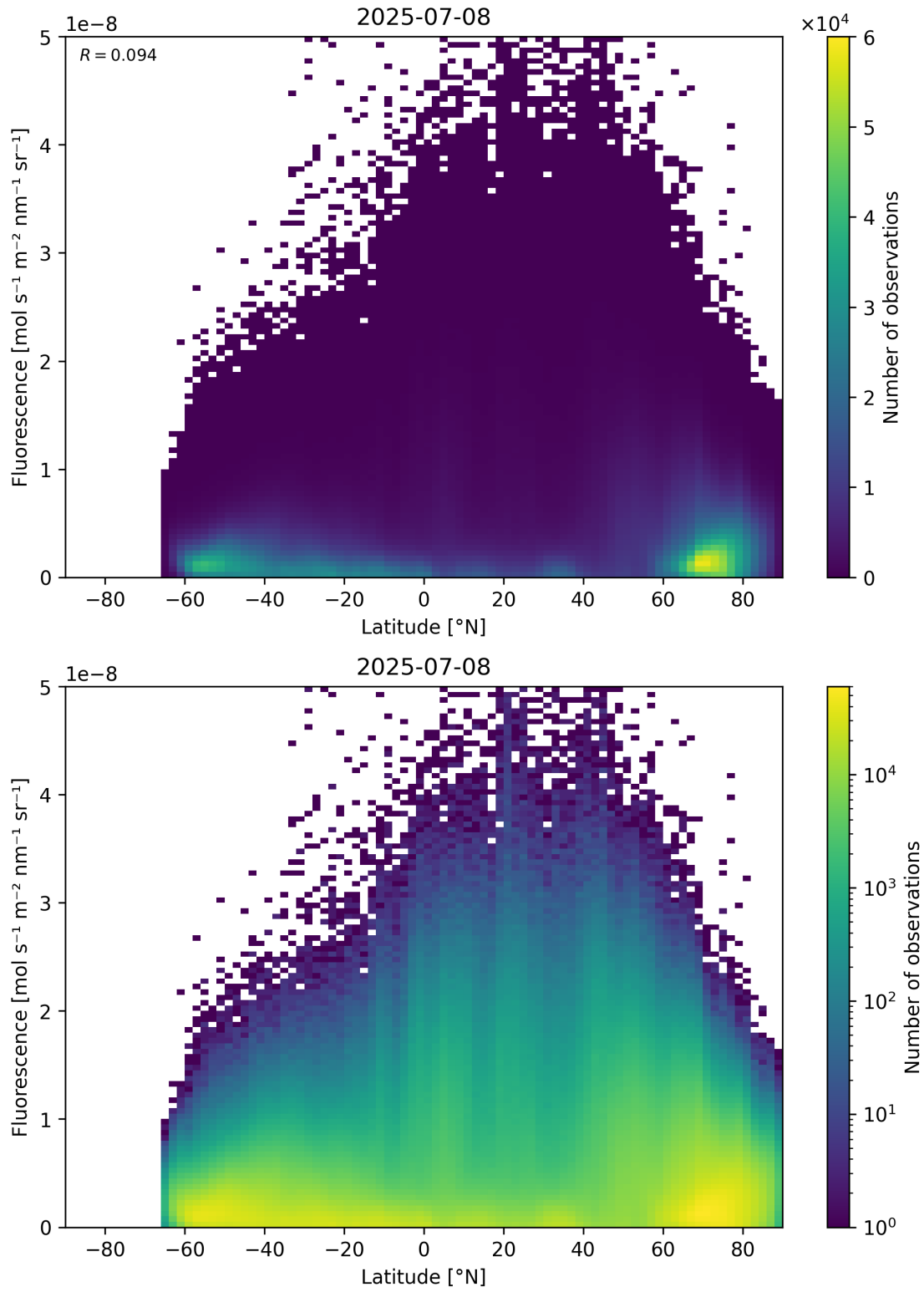
Figure 92: Scatter density plot of “Latitude” against “Fluorescence” for 2025-07-08 to 2025-07-09.
