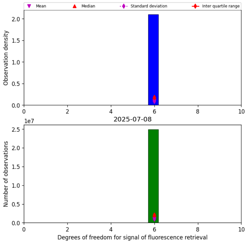
Figure 43: Histogram of “Degrees of freedom for signal of fluorescence retrieval” for 2025-07-08 to 2025-07-09
