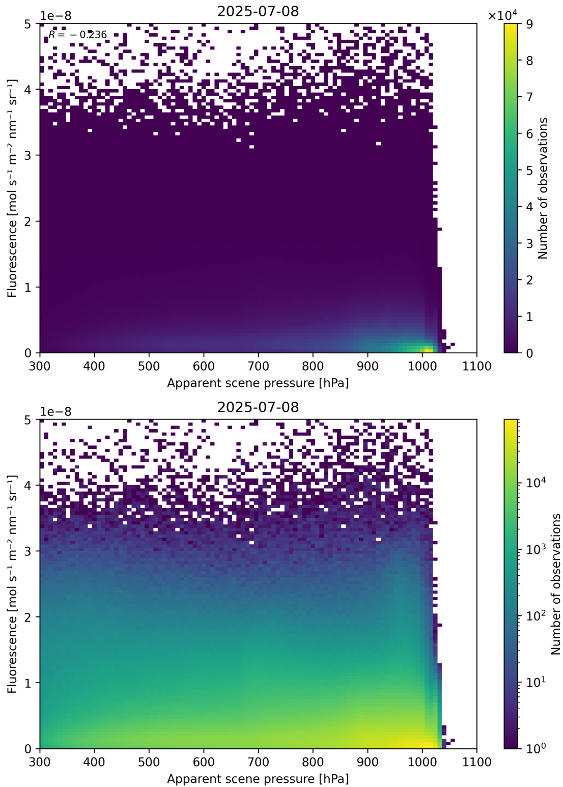
Figure 64: Scatter density plot of “Apparent scene pressure” against “Fluorescence” for 2025-07-08 to 2025-07-09.
