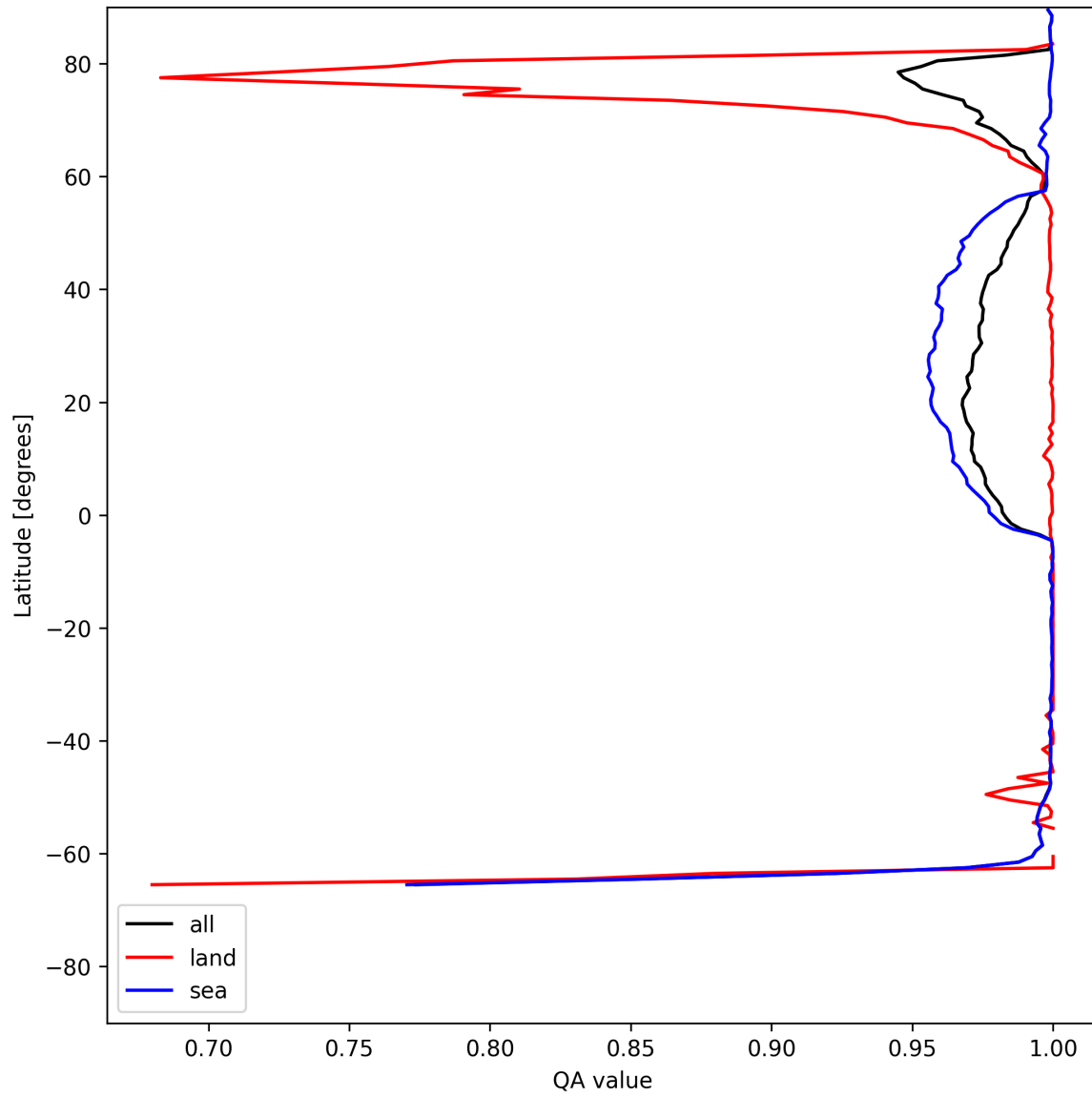
Figure 12: Zonal average of “QA value” for 2025-07-08 to 2025-07-09.
