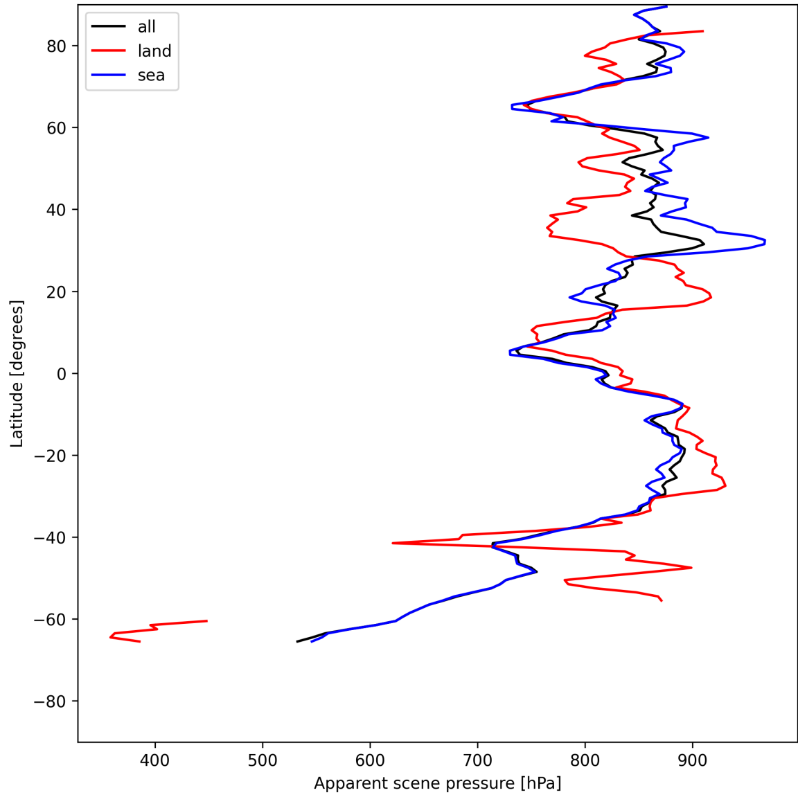
Figure 19: Zonal average of “Apparent scene pressure” for 2025-07-08 to 2025-07-09.
