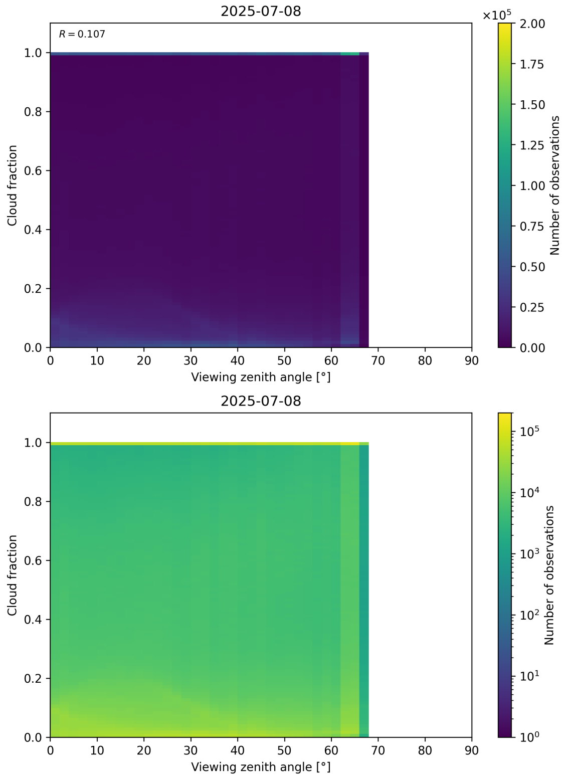
Figure 120: Scatter density plot of “Viewing zenith angle” against “Cloud fraction” for 2025-07-08 to 2025-07-09.
