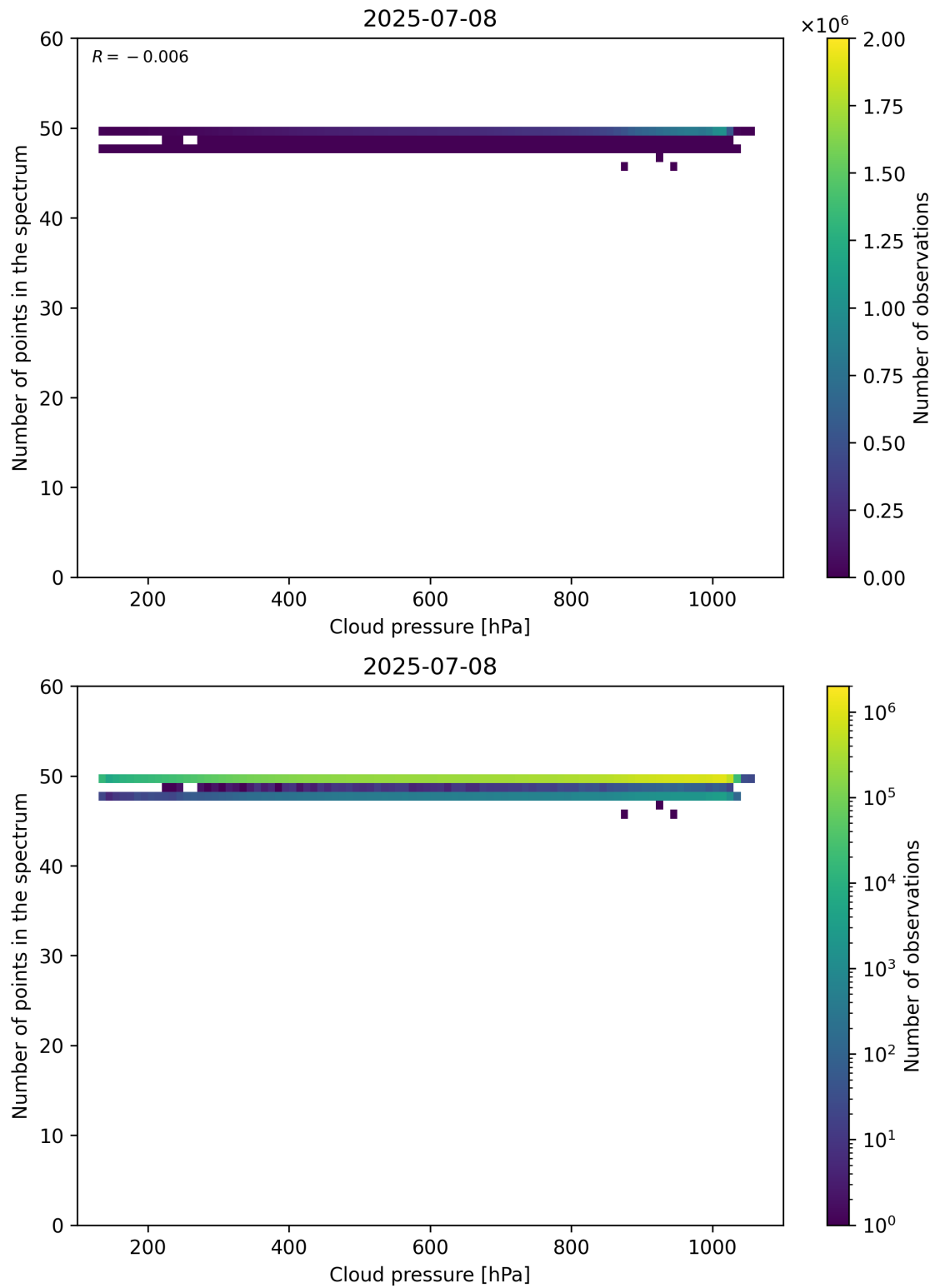
Figure 82: Scatter density plot of “Cloud pressure” against “Number of points in the spectrum” for 2025-07-08 to 2025-07-09.
