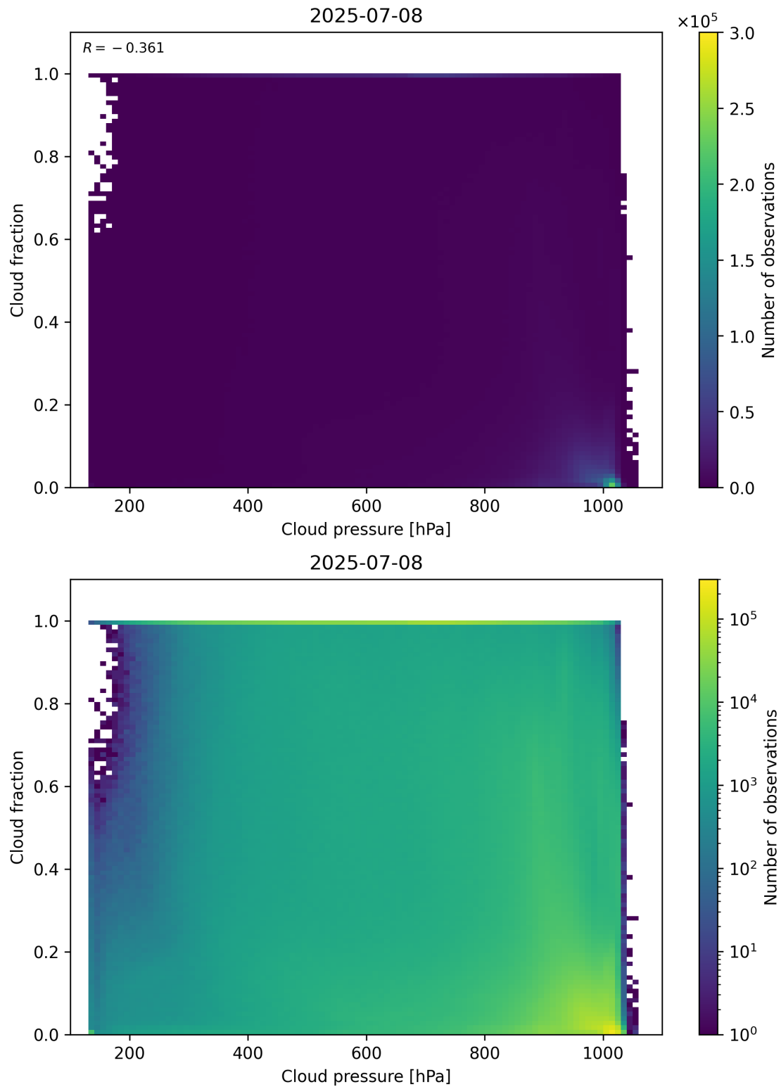
Figure 79: Scatter density plot of “Cloud pressure” against “Cloud fraction” for 2025-07-08 to 2025-07-09.
