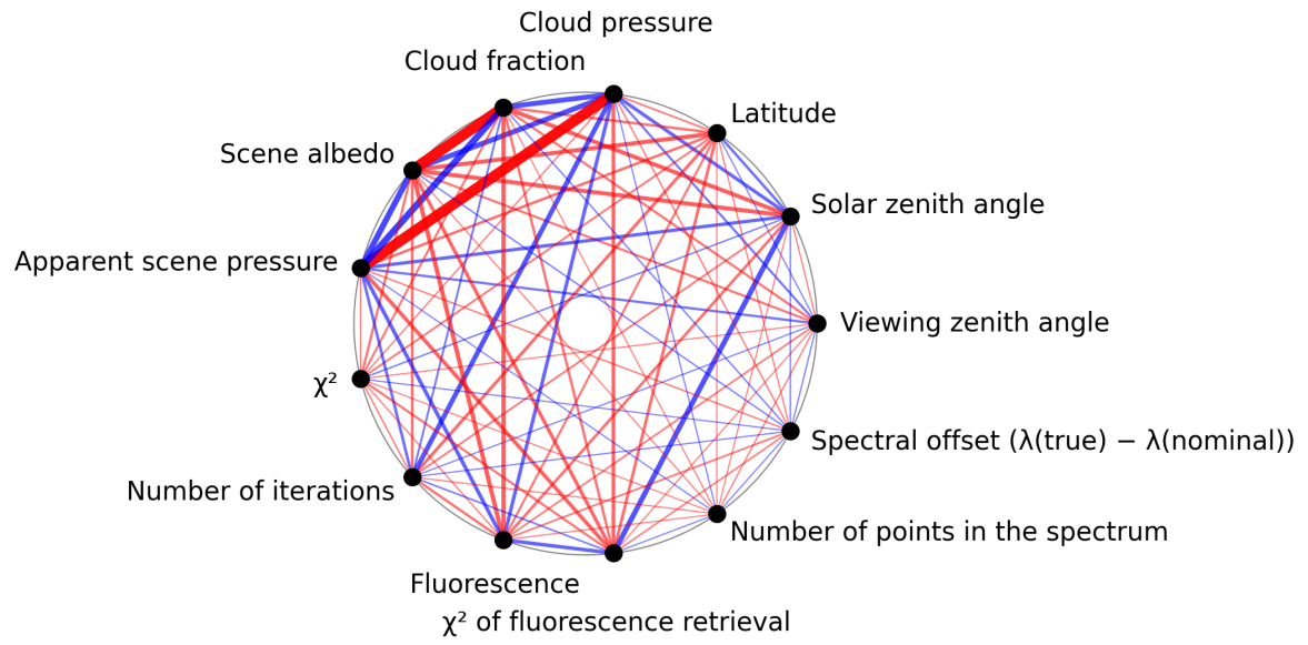
Figure 1: Map of correlation graph for 2025-07-08 to 2025-07-09.
