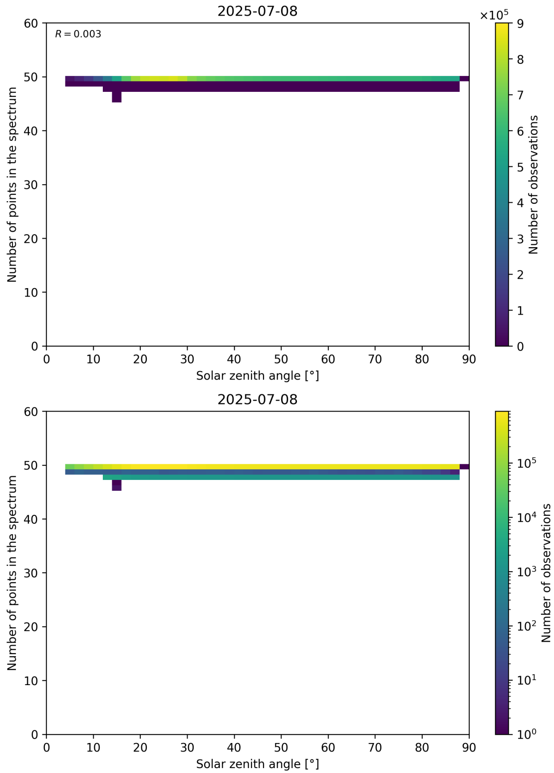
Figure 115: Scatter density plot of “Solar zenith angle” against “Number of points in the spectrum” for 2025-07-08 to 2025-07-09.
