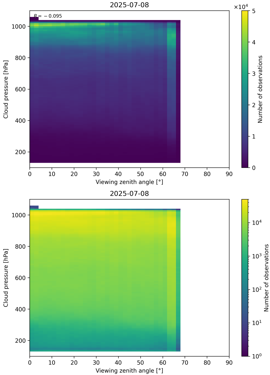
Figure 121: Scatter density plot of “Viewing zenith angle” against “Cloud pressure” for 2025-07-08 to 2025-07-09.
