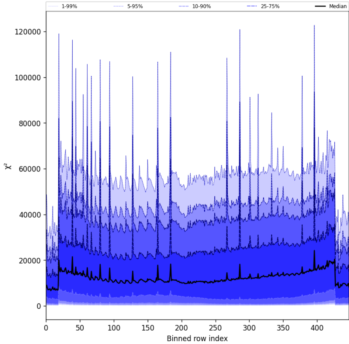
Figure 55: Along track statistics of “ \chi^2 ” for 2025-07-08 to 2025-07-09
