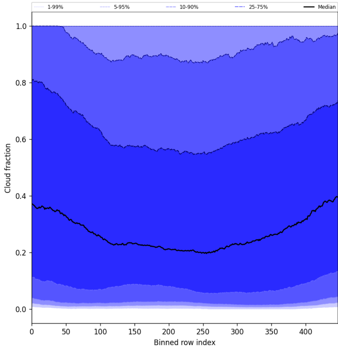
Figure 49: Along track statistics of “Cloud fraction” for 2025-07-08 to 2025-07-09
