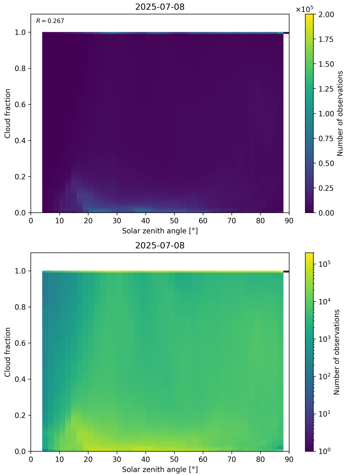
Figure 110: Scatter density plot of “Solar zenith angle” against “Cloud fraction” for 2025-07-08 to 2025-07-09.
