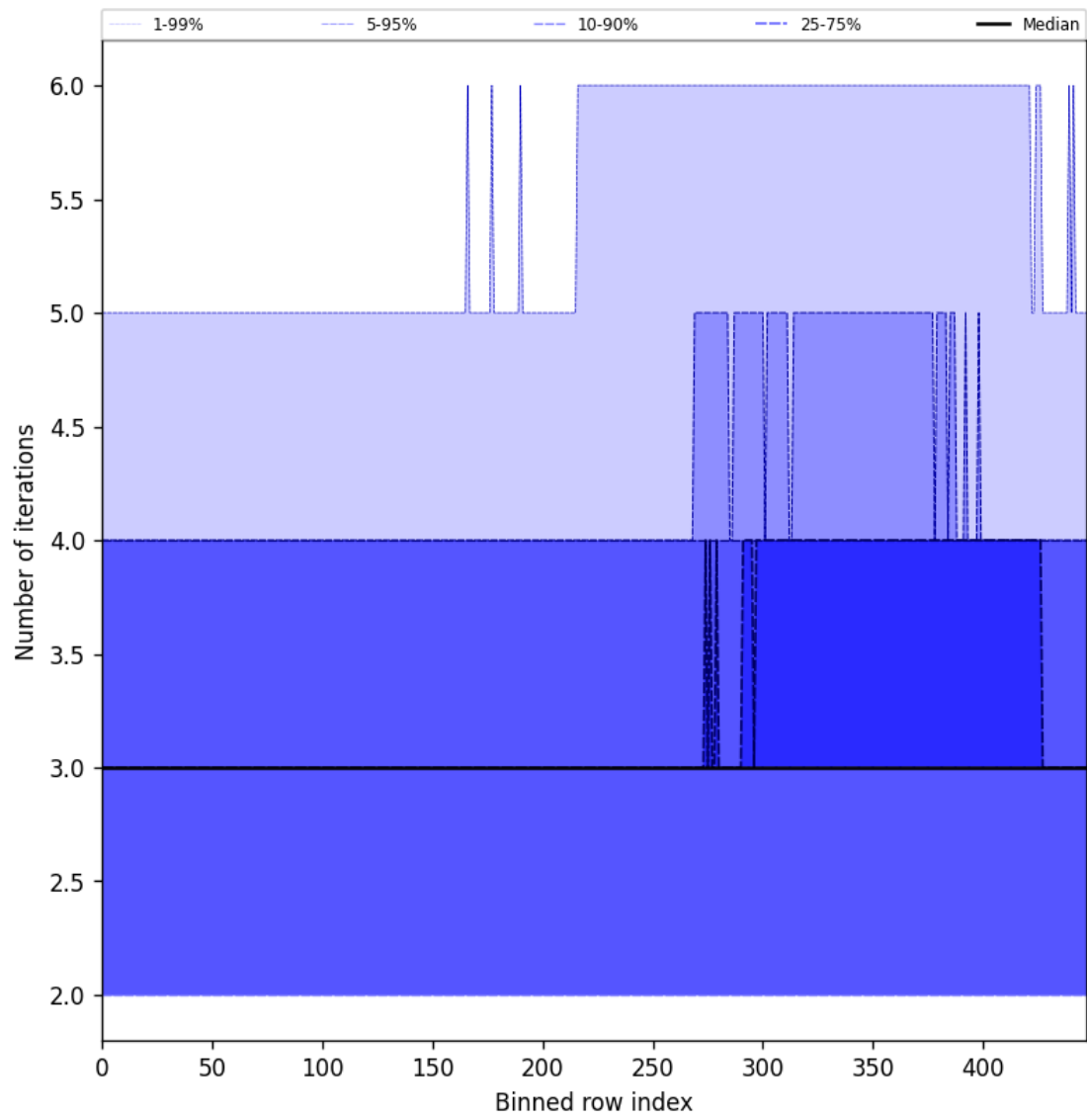
Figure 56: Along track statistics of “Number of iterations” for 2025-07-08 to 2025-07-09
