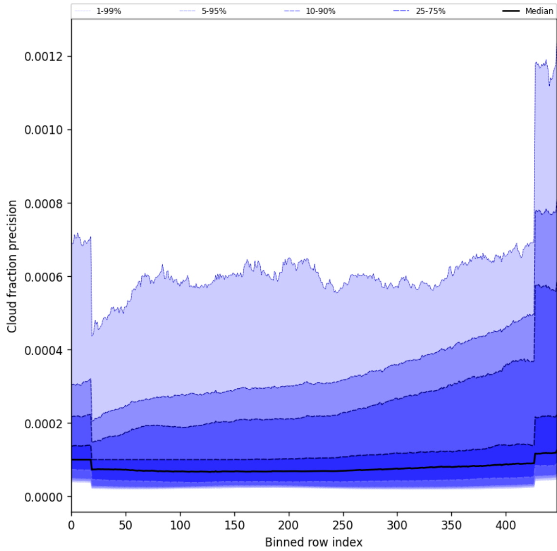
Figure 50: Along track statistics of “Cloud fraction precision” for 2025-07-08 to 2025-07-09
