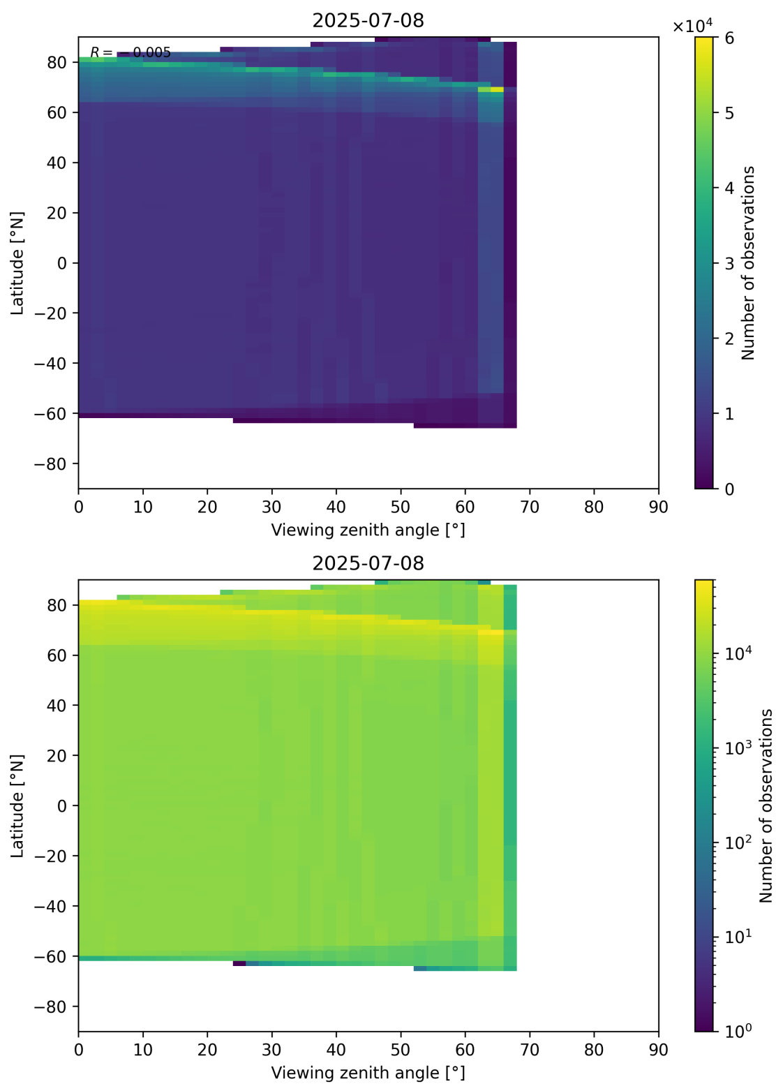
Figure 123: Scatter density plot of “Viewing zenith angle” against “Latitude” for 2025-07-08 to 2025-07-09.
