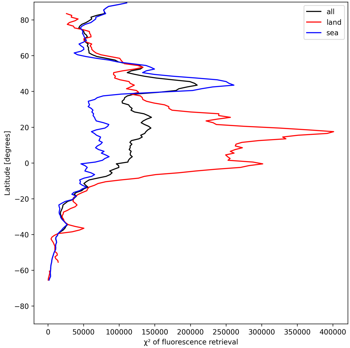
Figure 25: Zonal average of “ \chi^2 of fluorescence retrieval” for 2025-07-08 to 2025-07-09.
