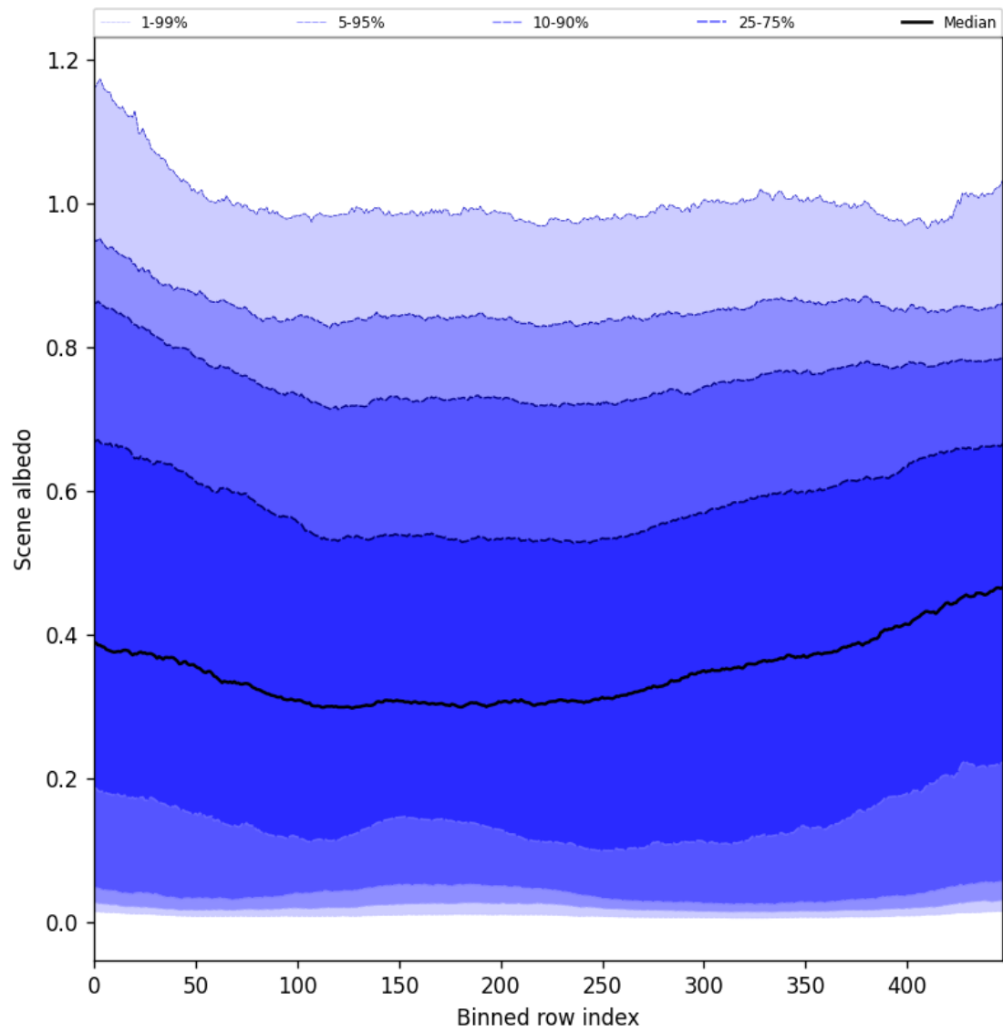
Figure 51: Along track statistics of “Scene albedo” for 2025-07-08 to 2025-07-09
