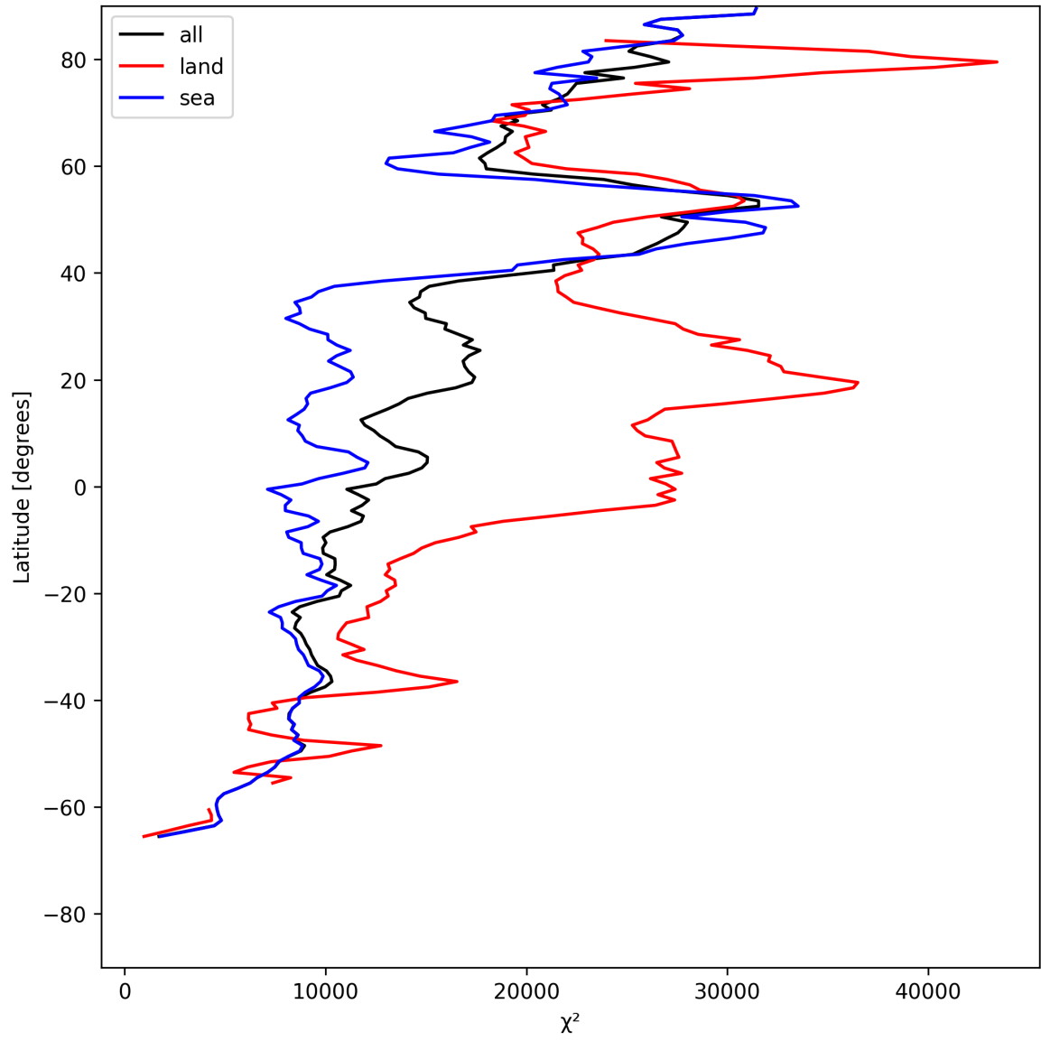
Figure 21: Zonal average of “ \chi^2 ” for 2025-07-08 to 2025-07-09.
