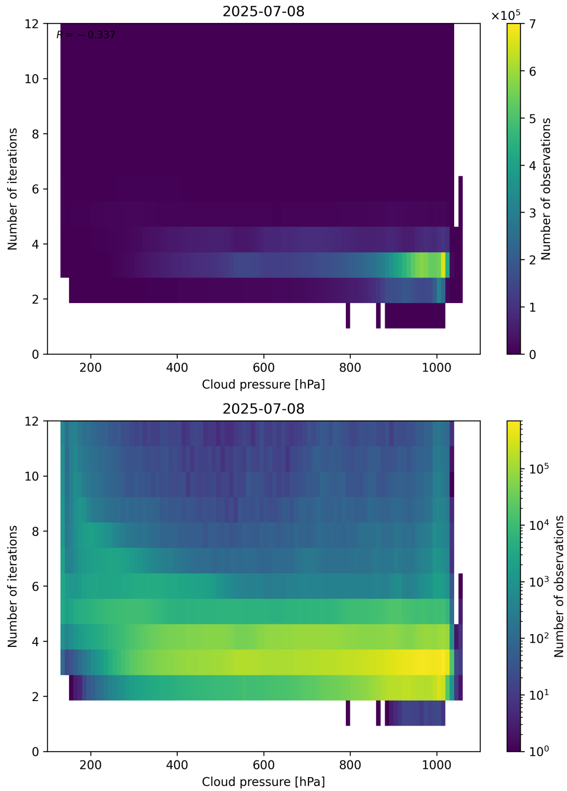
Figure 81: Scatter density plot of “Cloud pressure” against “Number of iterations” for 2025-07-08 to 2025-07-09.
