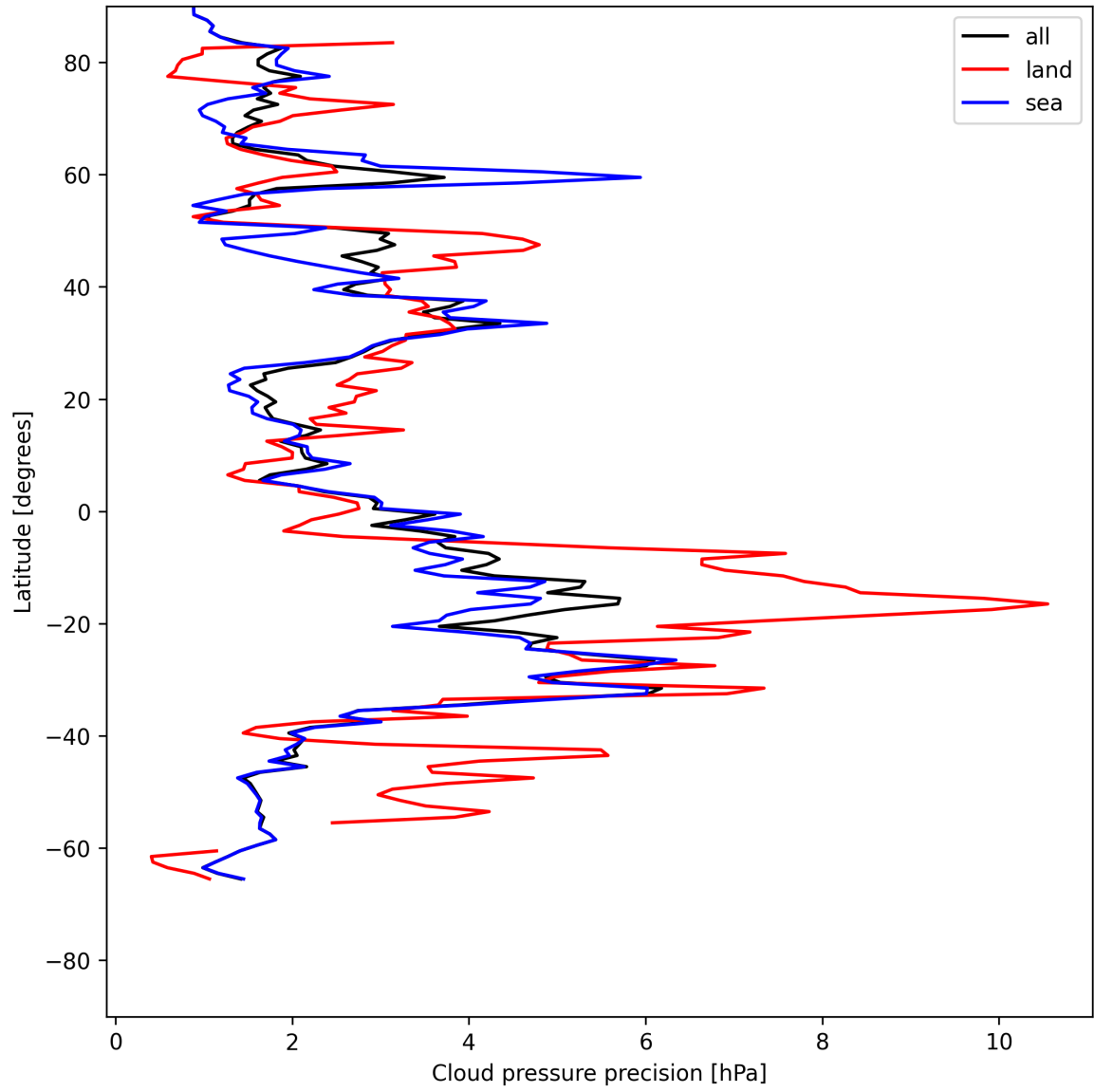
Figure 14: Zonal average of "Cloud pressure precision" for 2025-07-08 to 2025-07-09.
