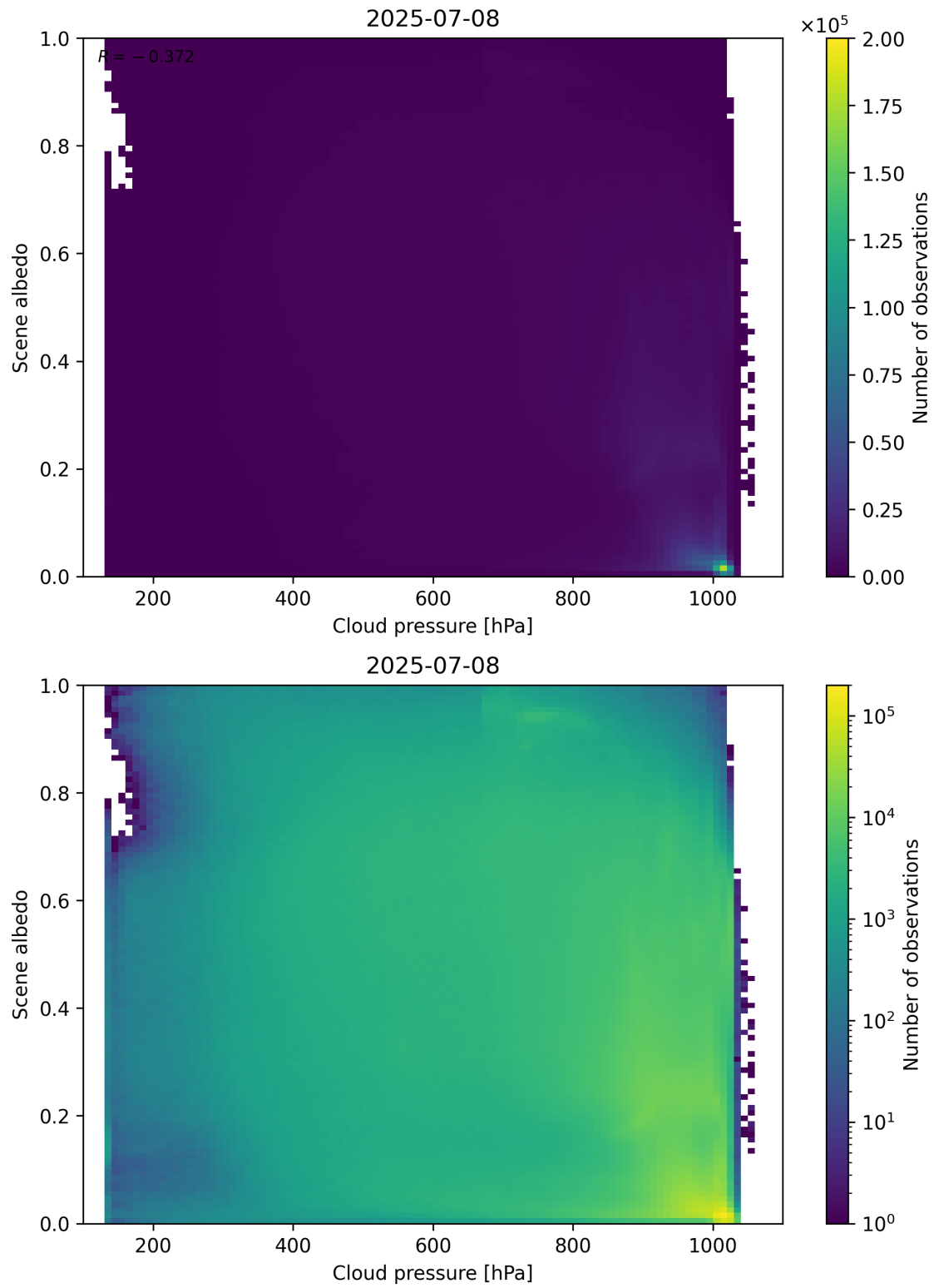
Figure 83: Scatter density plot of “Cloud pressure” against “Scene albedo” for 2025-07-08 to 2025-07-09.
