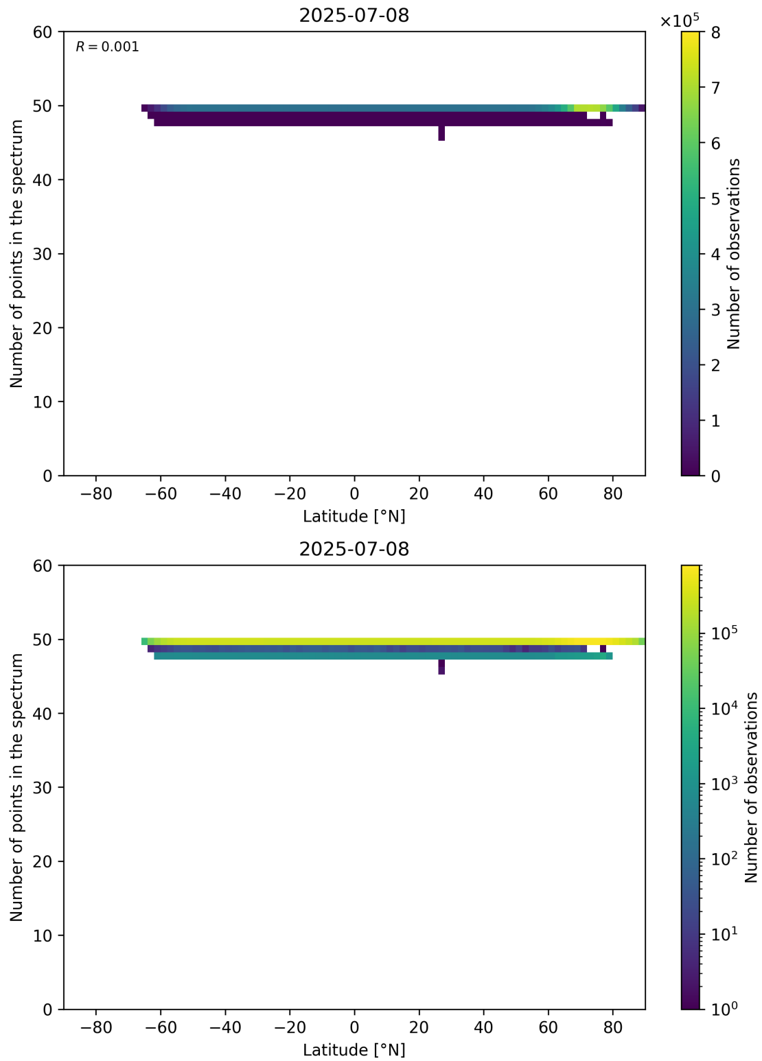
Figure 94: Scatter density plot of “Latitude” against “Number of points in the spectrum” for 2025-07-08 to 2025-07-09.
