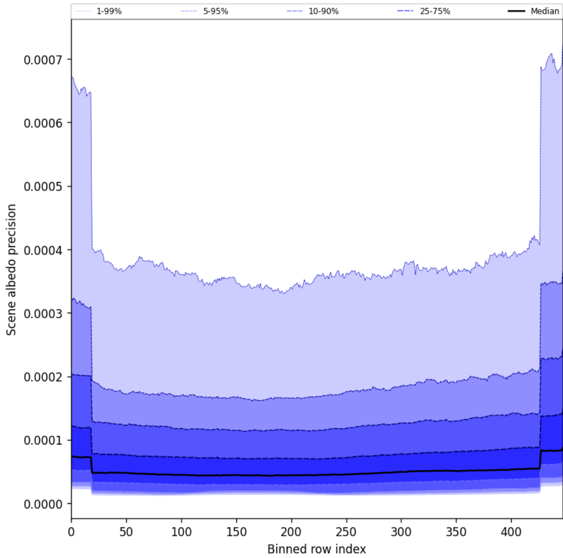
Figure 52: Along track statistics of “Scene albedo precision” for 2025-07-08 to 2025-07-09
