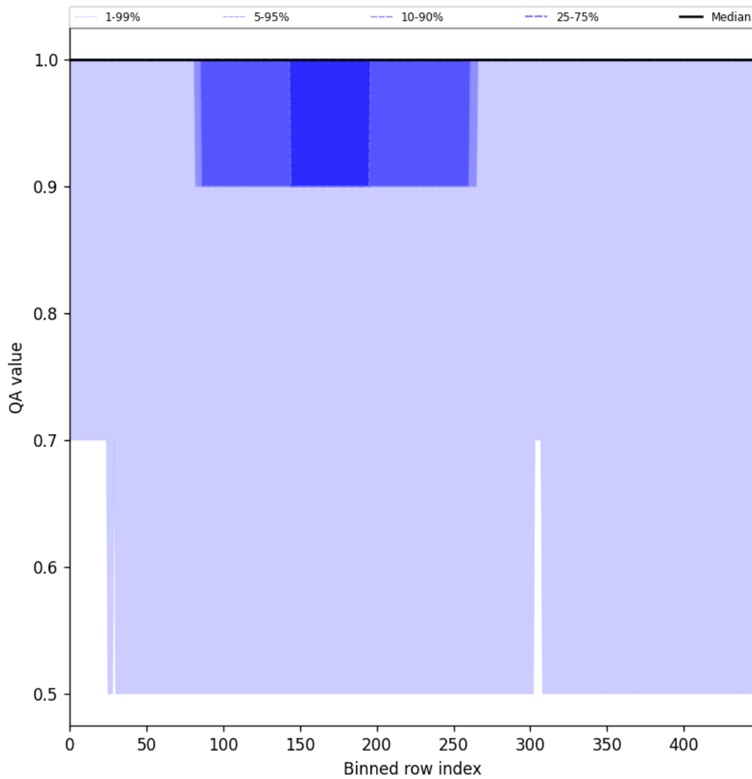
Figure 46: Along track statistics of “QA value” for 2025-07-08 to 2025-07-09
