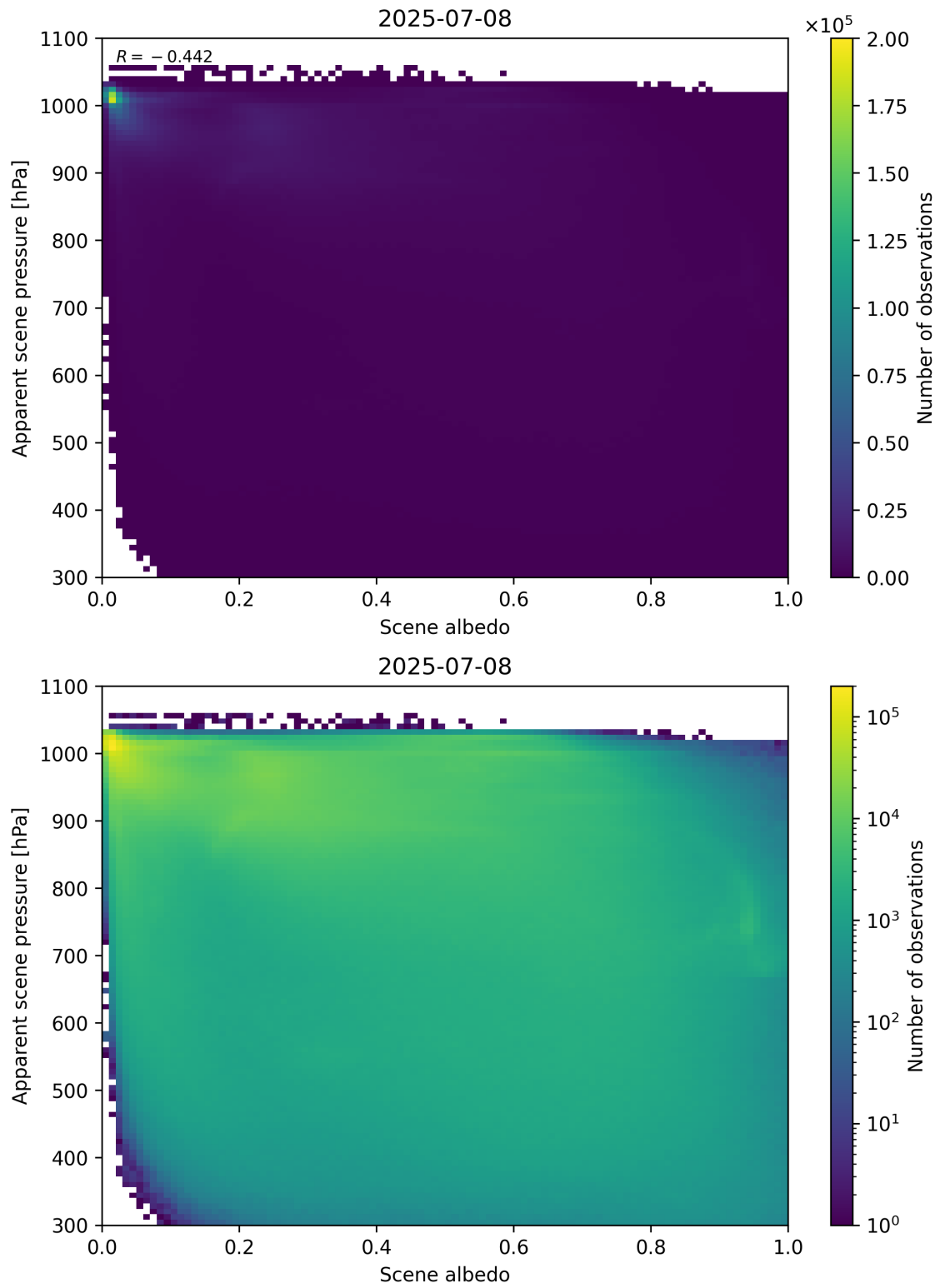
Figure 102: Scatter density plot of “Scene albedo” against “Apparent scene pressure” for 2025-07-08 to 2025-07-09.
