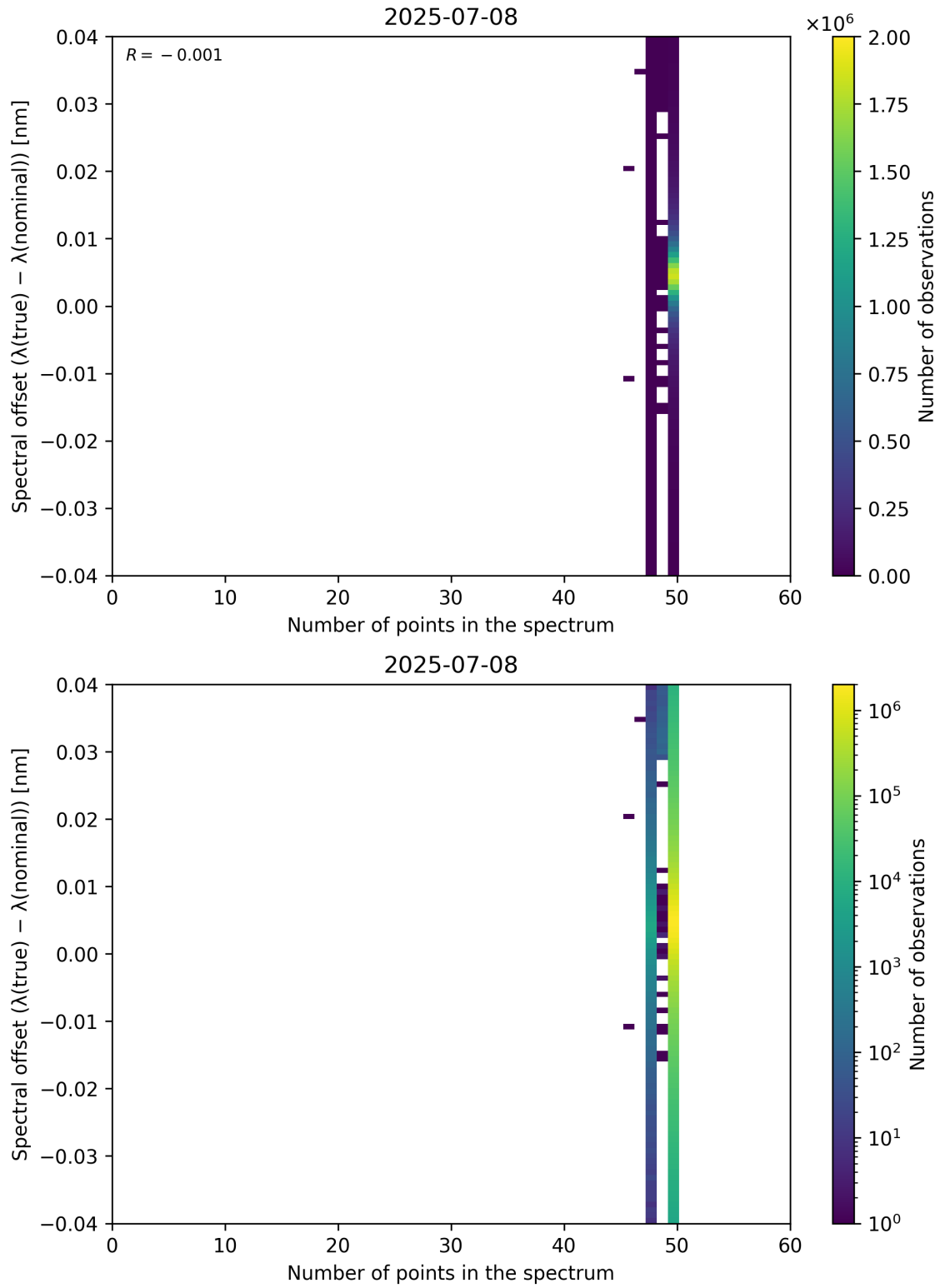
Figure 101: Scatter density plot of “Number of points in the spectrum” against “Spectral offset ( \lambda_{\text{true}} - \lambda_{\text{nominal}} )” for 2025-07-08 to 2025-07-09.
