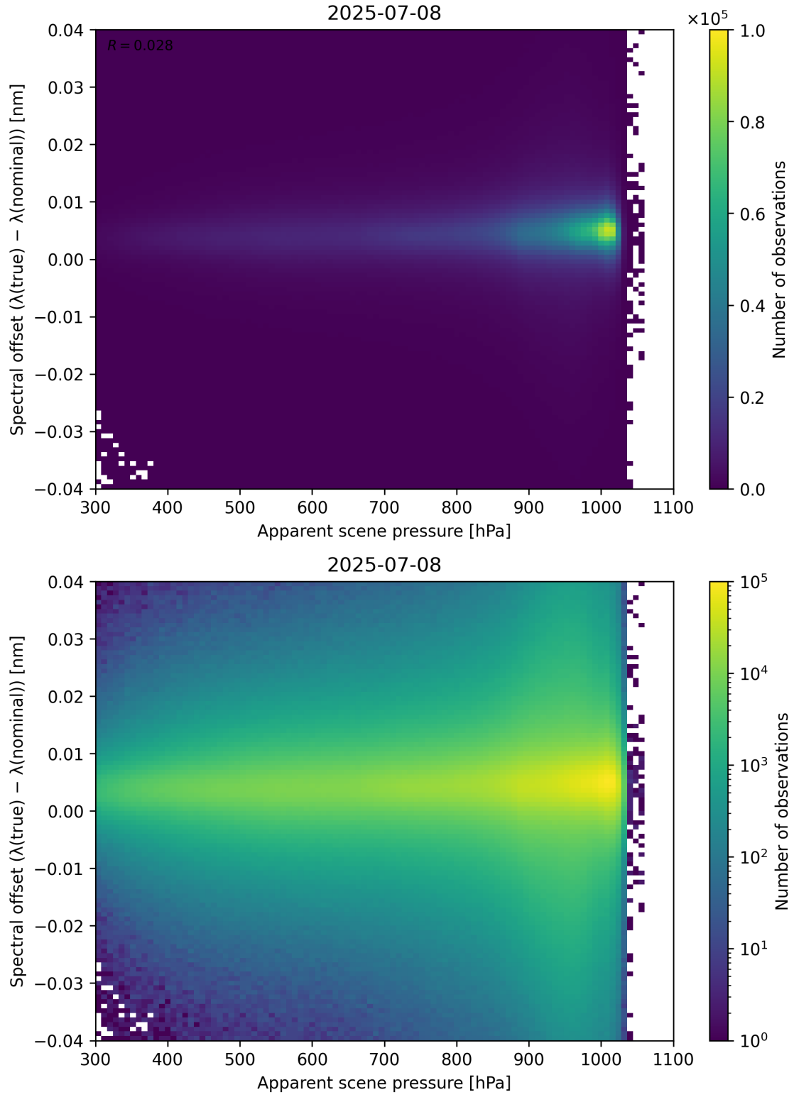
Figure 67: Scatter density plot of “Apparent scene pressure” against “Spectral offset ( \lambda_{\text{true}} - \lambda_{\text{nominal}} )” for 2025-07-08 to 2025-07-09.
