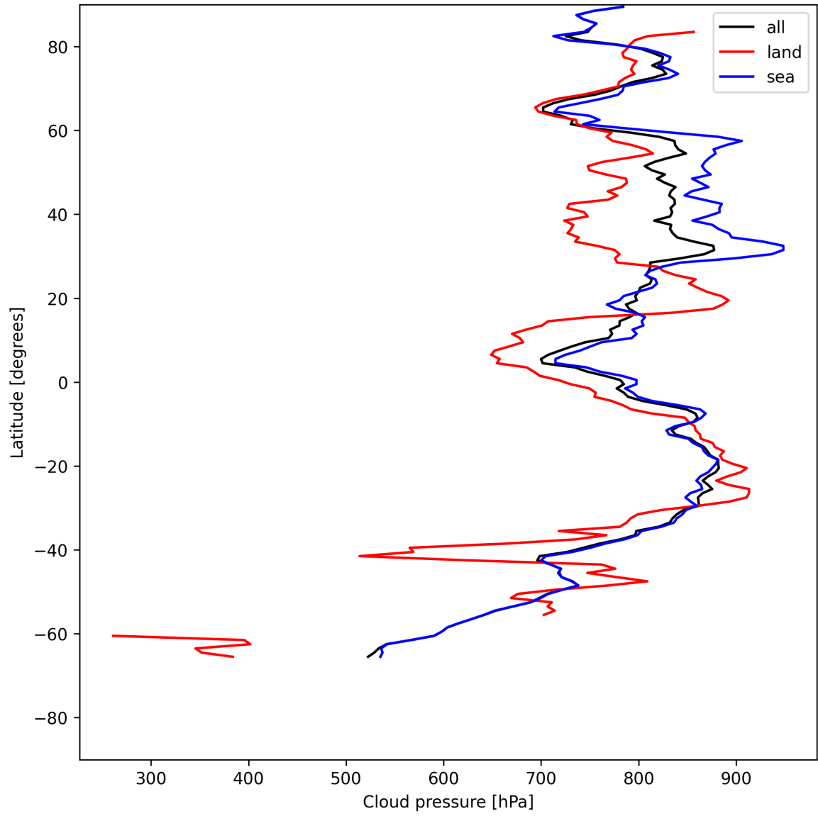
Figure 13: Zonal average of “Cloud pressure” for 2025-07-08 to 2025-07-09.
