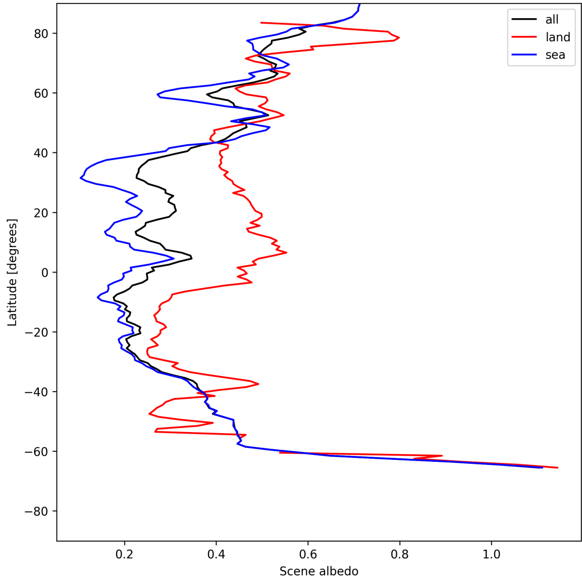
Figure 17: Zonal average of “Scene albedo” for 2025-07-08 to 2025-07-09.
