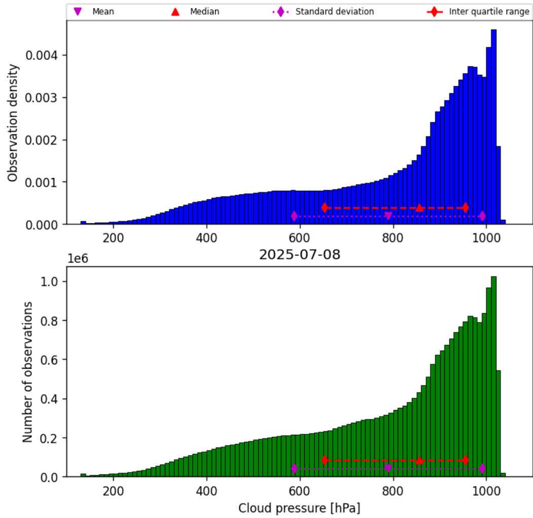
Figure 30: Histogram of “Cloud pressure” for 2025-07-08 to 2025-07-09
