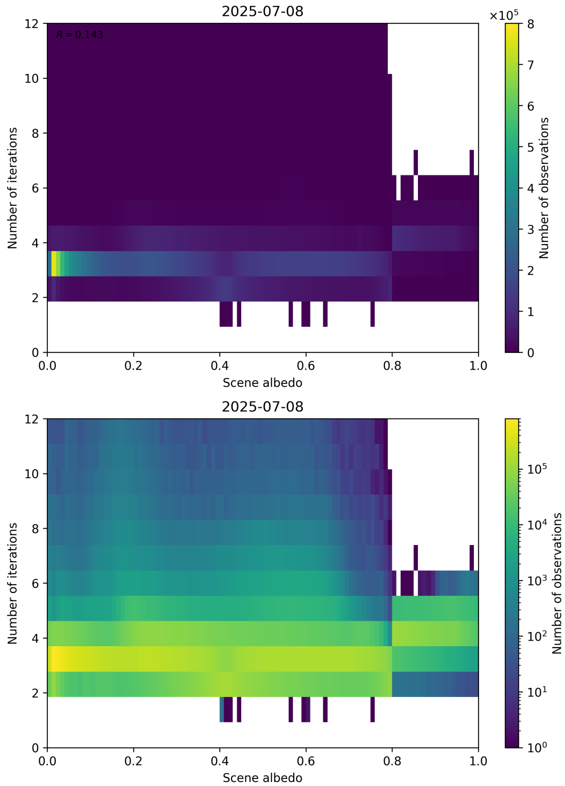
Figure 105: Scatter density plot of “Scene albedo” against “Number of iterations” for 2025-07-08 to 2025-07-09.
