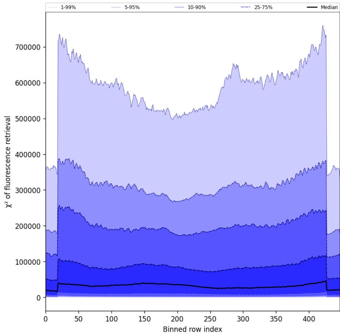
Figure 59: Along track statistics of “ \chi^2 of fluorescence retrieval” for 2025-07-08 to 2025-07-09
