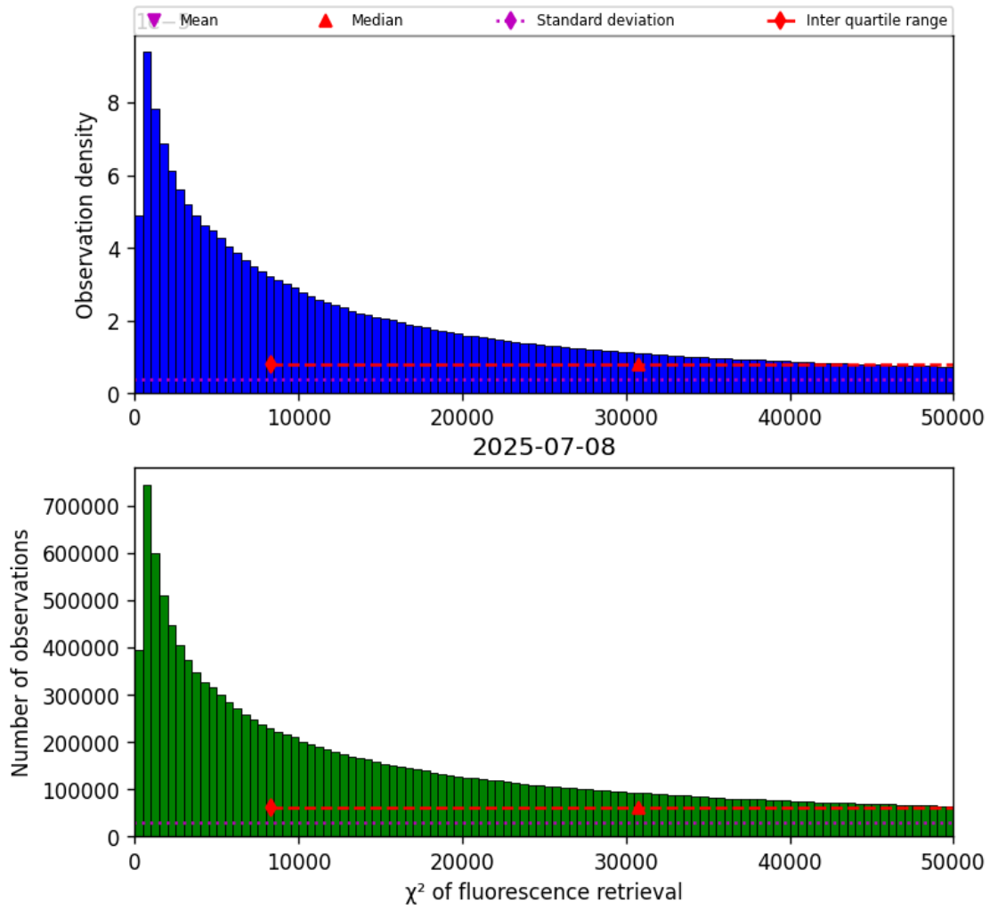
Figure 42: Histogram of “ \chi^2 of fluorescence retrieval” for 2025-07-08 to 2025-07-09
