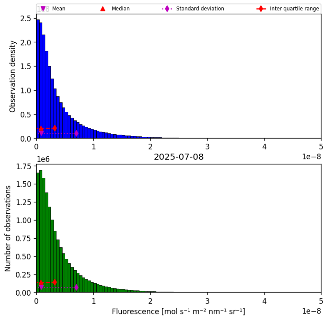
Figure 40: Histogram of “Fluorescence” for 2025-07-08 to 2025-07-09
