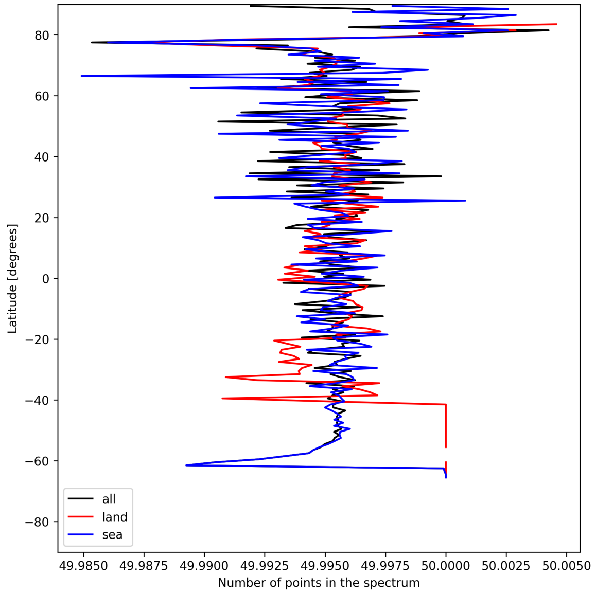
Figure 27: Zonal average of “Number of points in the spectrum” for 2025-07-08 to 2025-07-09.
