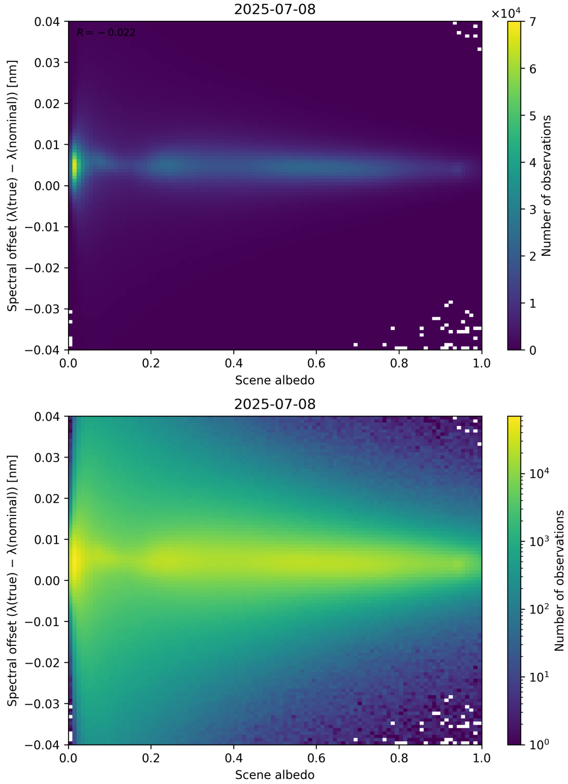
Figure 107: Scatter density plot of “Scene albedo” against “Spectral offset ( \lambda_{\text{true}} - \lambda_{\text{nominal}} )” for 2025-07-08 to 2025-07-09.
