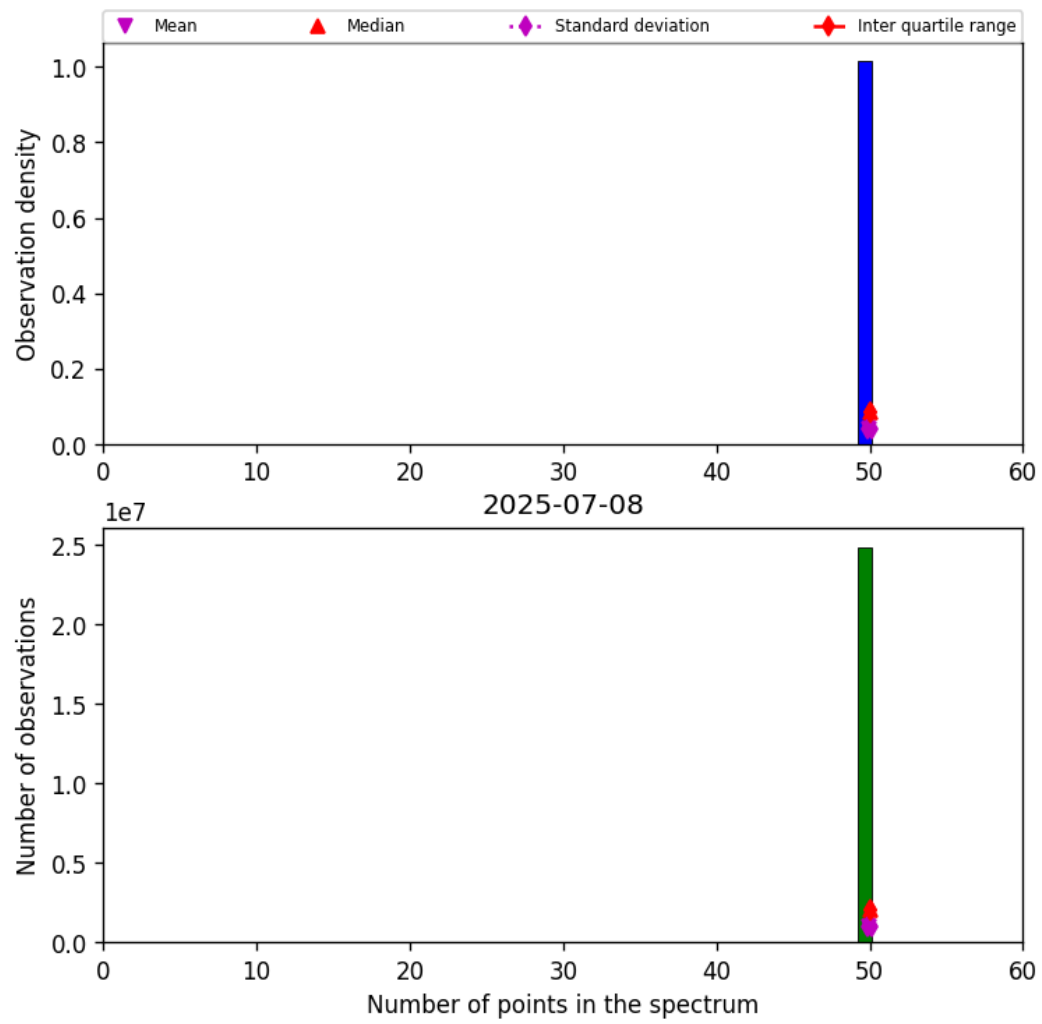
Figure 44: Histogram of “Number of points in the spectrum” for 2025-07-08 to 2025-07-09
