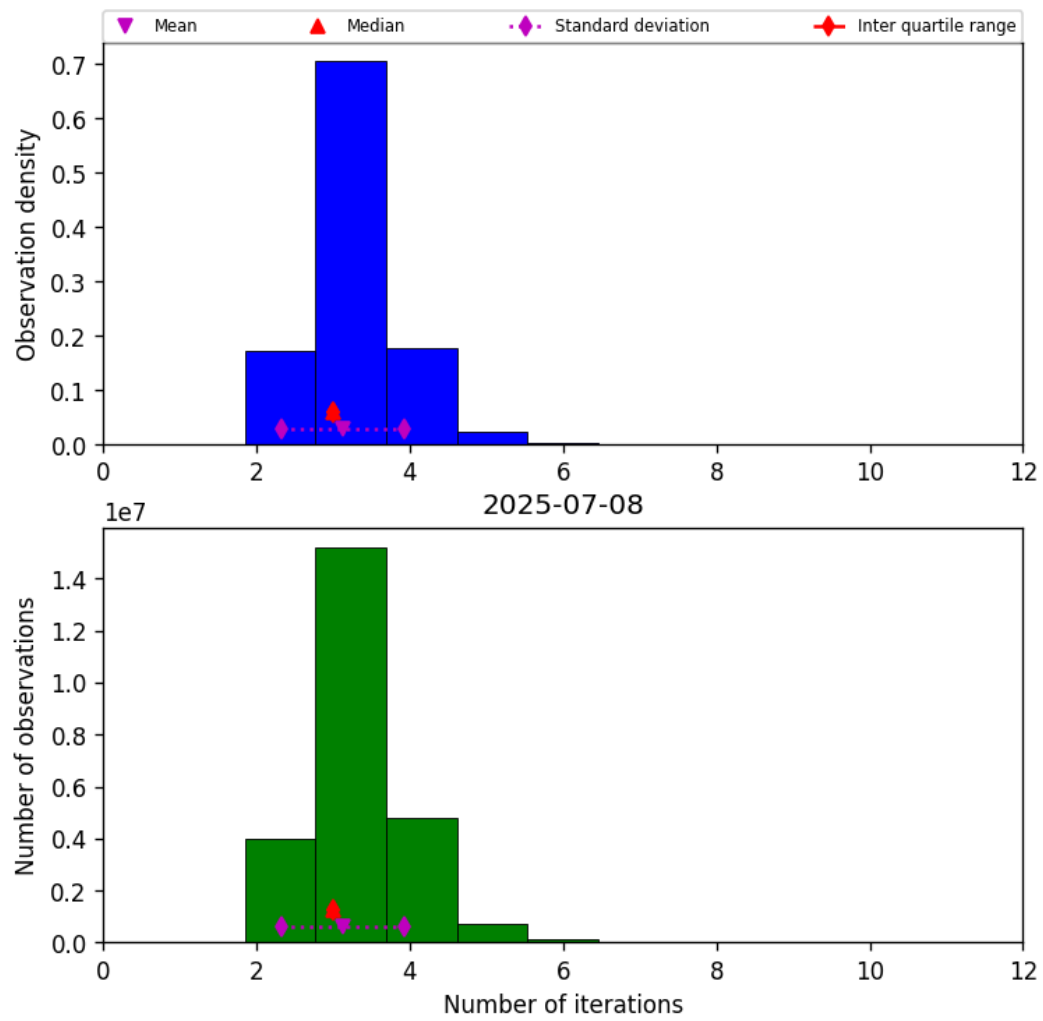
Figure 39: Histogram of “Number of iterations” for 2025-07-08 to 2025-07-09
