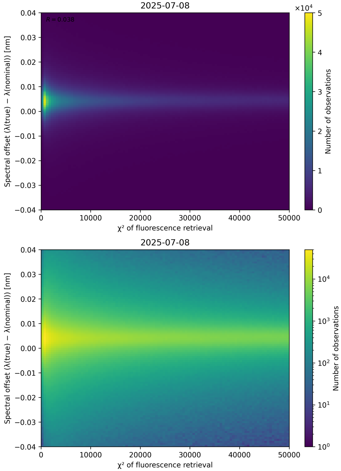
Figure 69: Scatter density plot of “ \chi^2 of fluorescence retrieval” against “Spectral offset ( \lambda_{\text{true}} - \lambda_{\text{nominal}} )” for 2025-07-08 to 2025-07-09.
