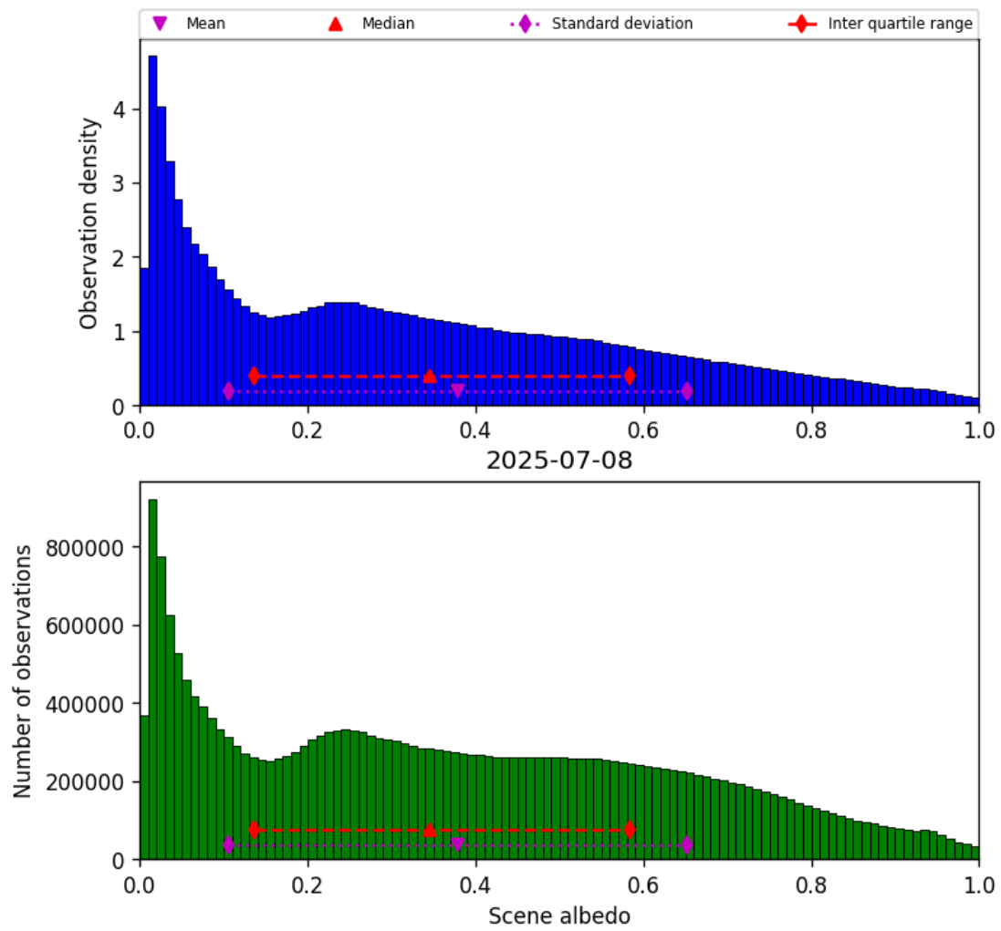
Figure 34: Histogram of “Scene albedo” for 2025-07-08 to 2025-07-09
