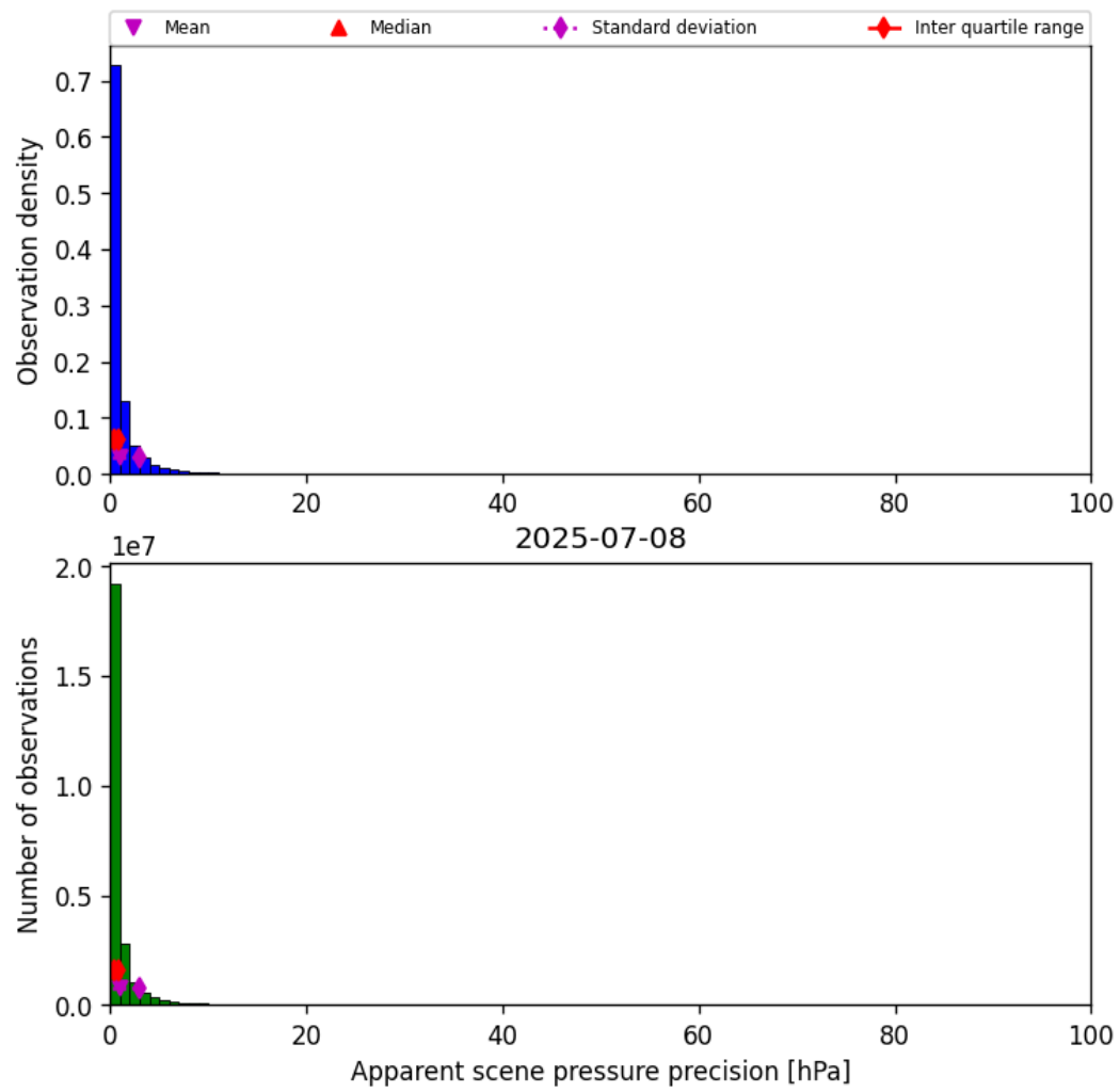
Figure 37: Histogram of “Apparent scene pressure precision” for 2025-07-08 to 2025-07-09
