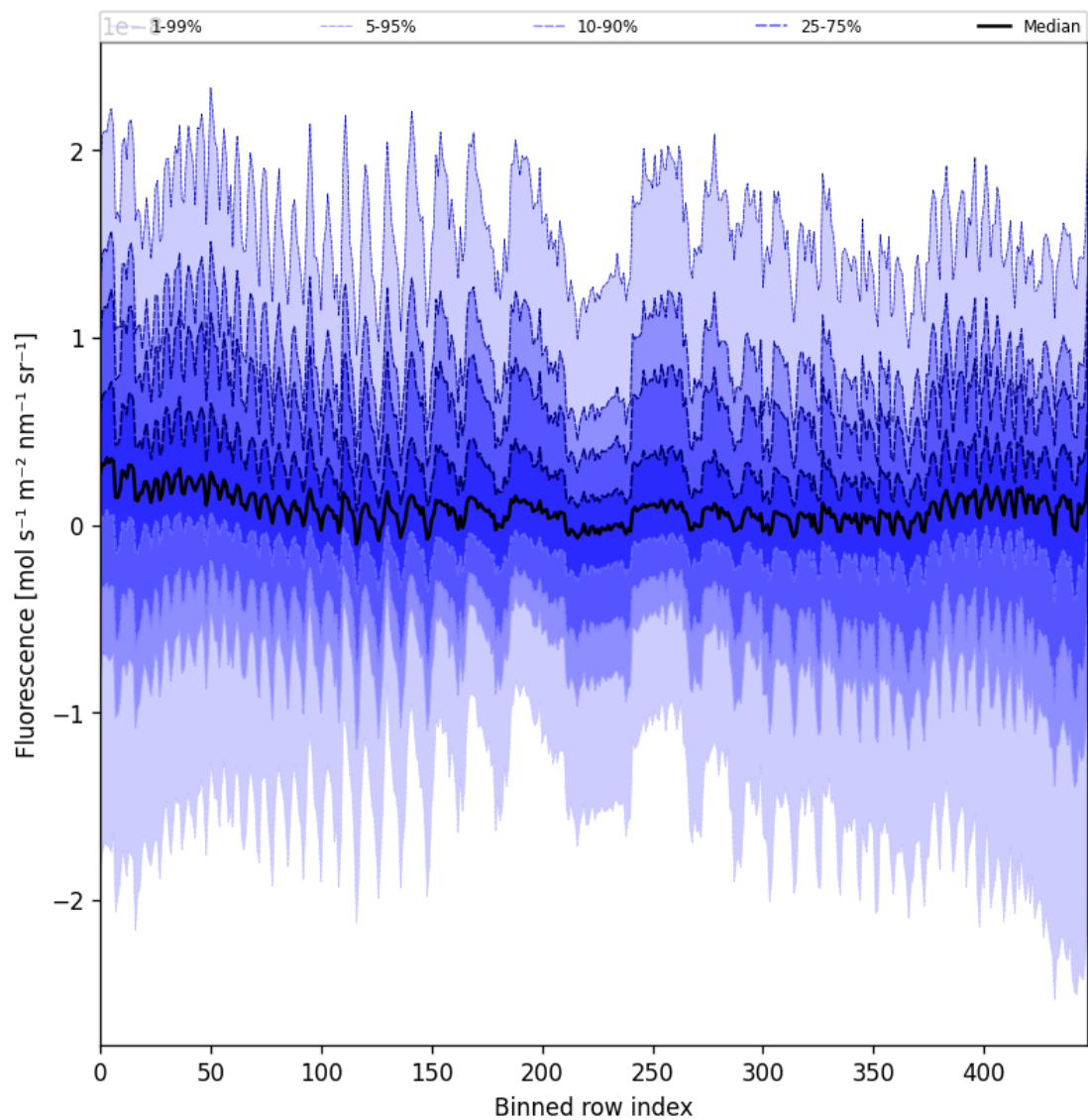
Figure 57: Along track statistics of “Fluorescence” for 2025-07-08 to 2025-07-09
