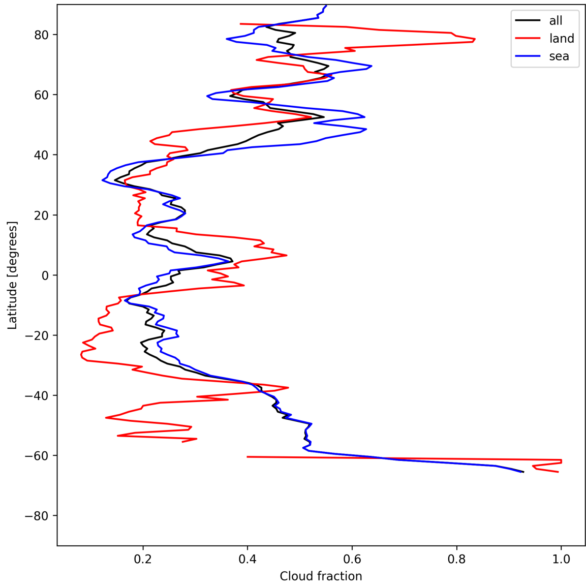
Figure 15: Zonal average of “Cloud fraction” for 2025-07-08 to 2025-07-09.
