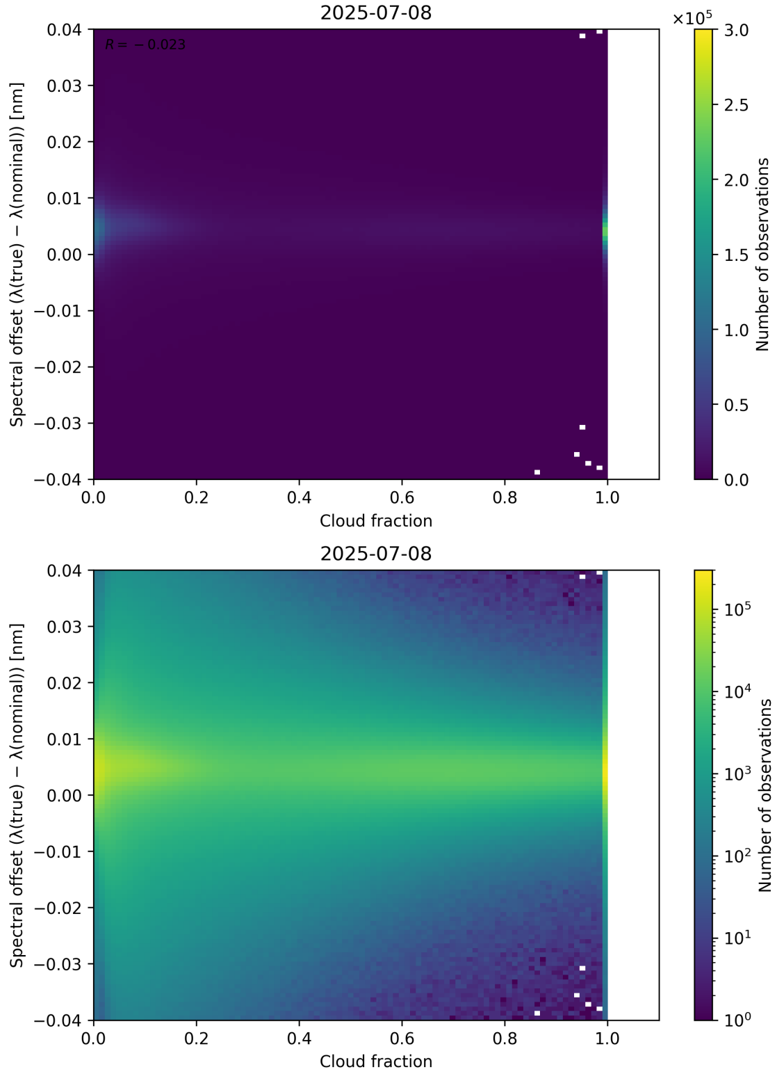
Figure 76: Scatter density plot of “Cloud fraction” against “Spectral offset ( \lambda_{\text{true}} - \lambda_{\text{nominal}} )” for 2025-07-08 to 2025-07-09.
