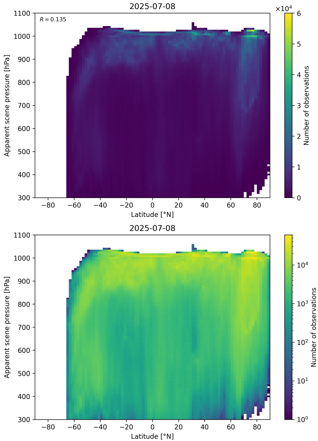
Figure 88: Scatter density plot of “Latitude” against “Apparent scene pressure” for 2025-07-08 to 2025-07-09.
