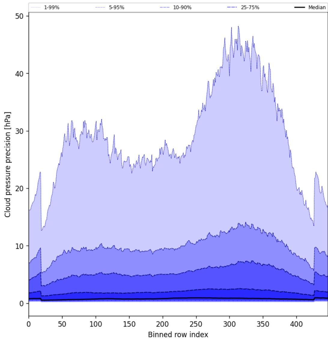
Figure 48: Along track statistics of “Cloud pressure precision” for 2025-07-08 to 2025-07-09
