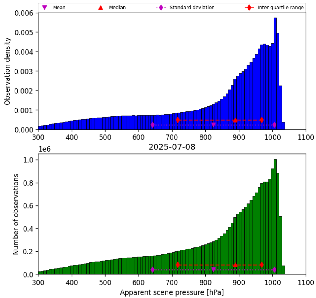
Figure 36: Histogram of “Apparent scene pressure” for 2025-07-08 to 2025-07-09
