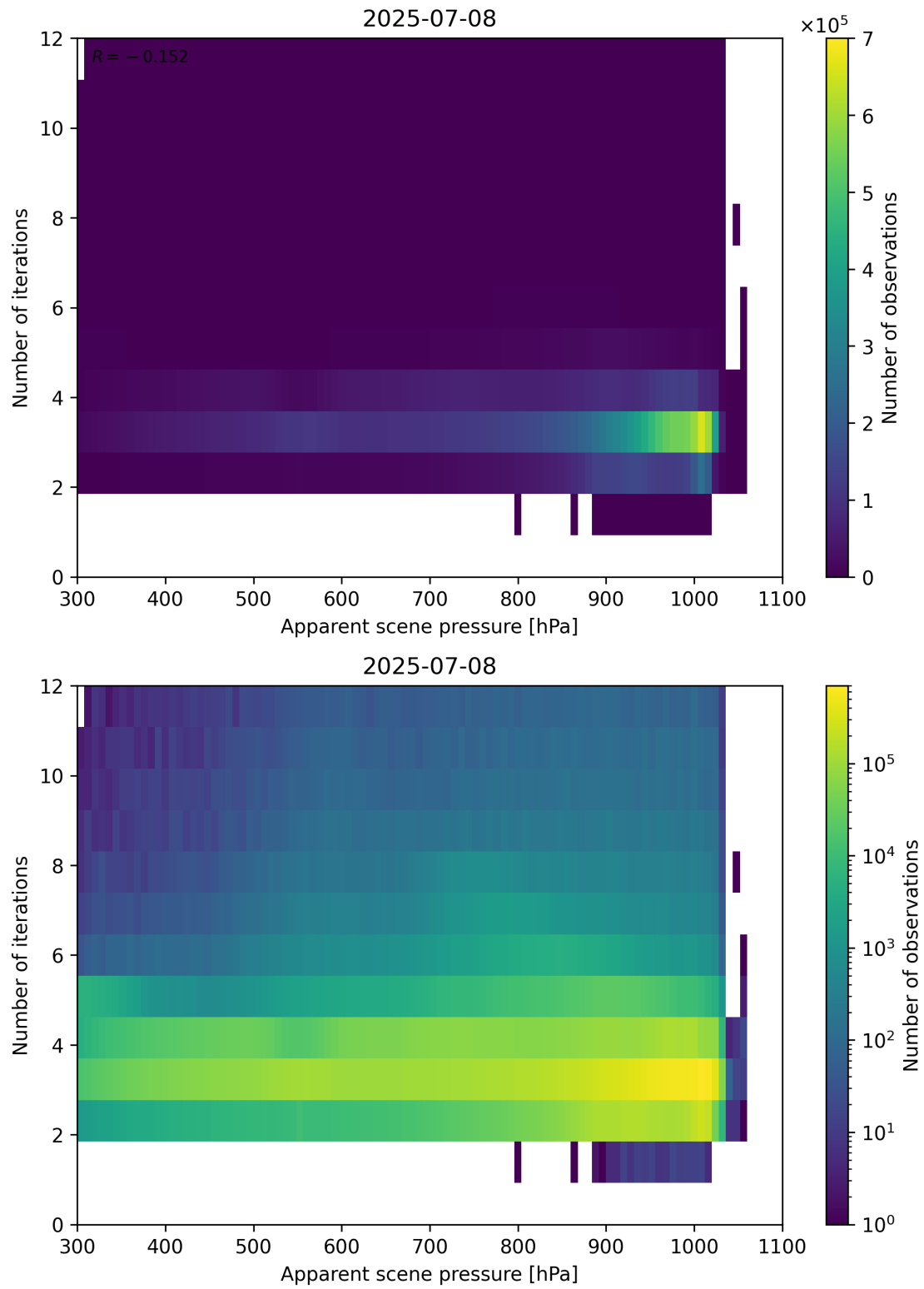
Figure 65: Scatter density plot of “Apparent scene pressure” against “Number of iterations” for 2025-07-08 to 2025-07-09.
