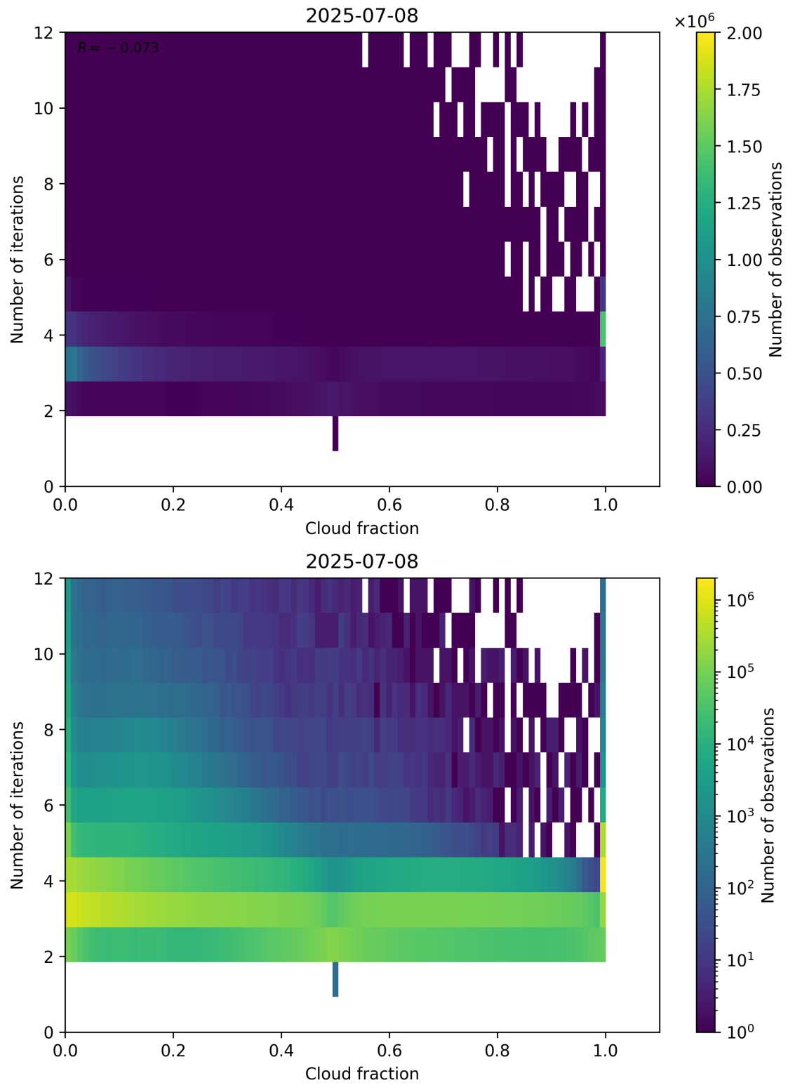
Figure 73: Scatter density plot of “Cloud fraction” against “Number of iterations” for 2025-07-08 to 2025-07-09.
