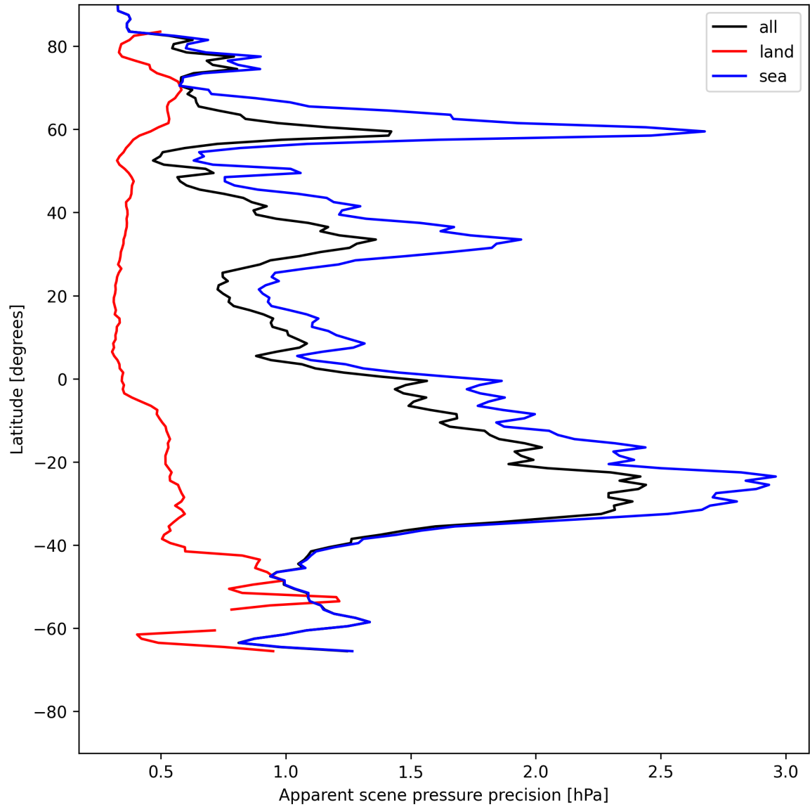
Figure 20: Zonal average of “Apparent scene pressure precision” for 2025-07-08 to 2025-07-09.
