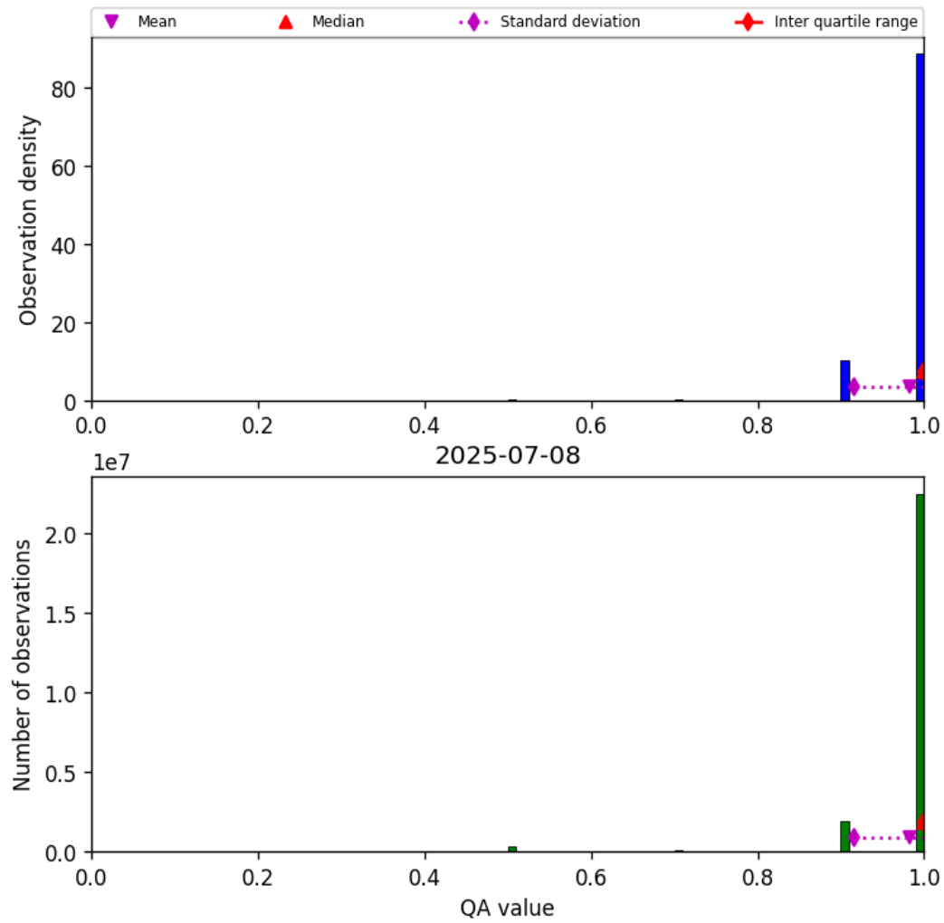
Figure 29: Histogram of “QA value” for 2025-07-08 to 2025-07-09
