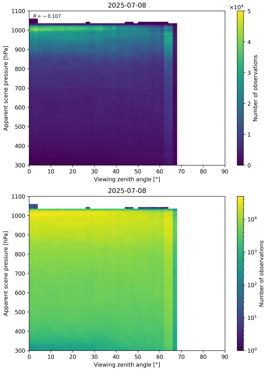
Figure 118: Scatter density plot of “Viewing zenith angle” against “Apparent scene pressure” for 2025-07-08 to 2025-07-09.
