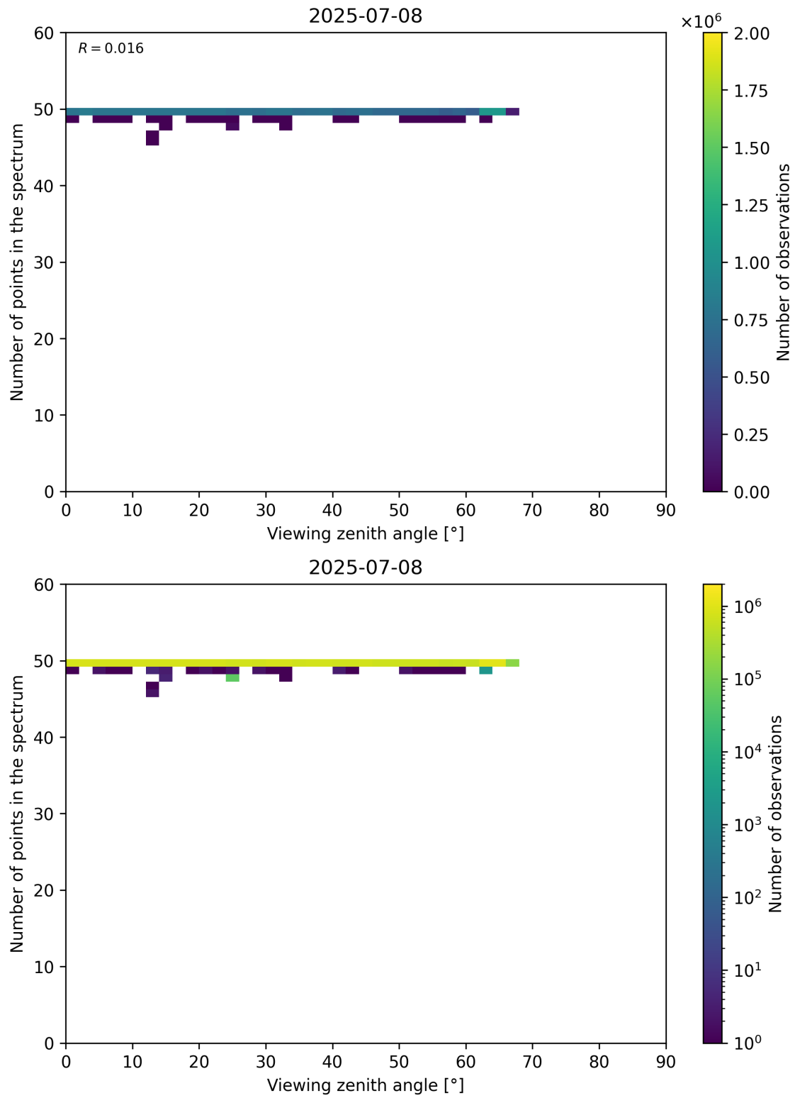
Figure 125: Scatter density plot of “Viewing zenith angle” against “Number of points in the spectrum” for 2025-07-08 to 2025-07-09.
