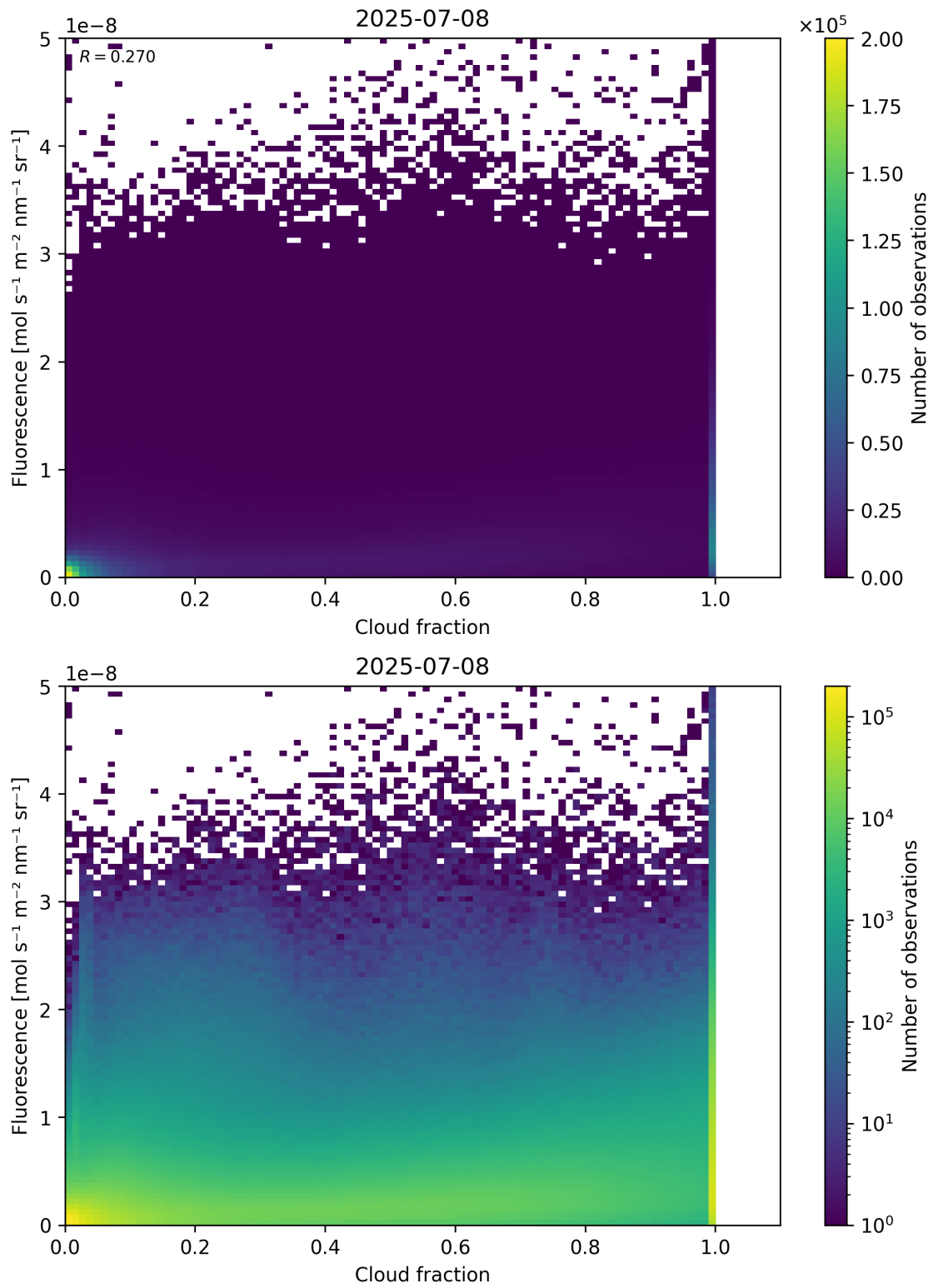
Figure 72: Scatter density plot of “Cloud fraction” against “Fluorescence” for 2025-07-08 to 2025-07-09.
