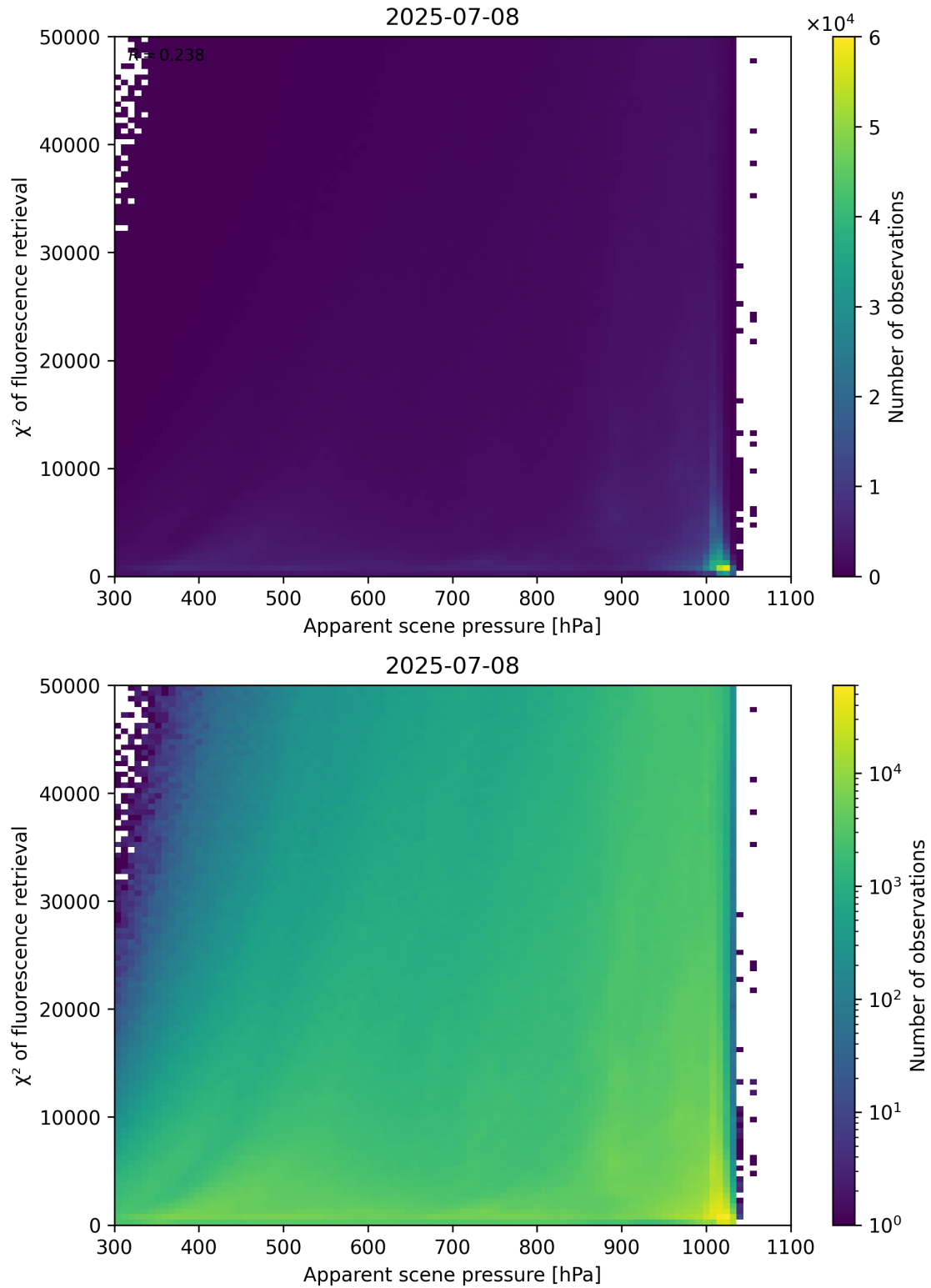
Figure 63: Scatter density plot of “Apparent scene pressure” against “ \chi^2 of fluorescence retrieval” for 2025-07-08 to 2025-07-09.
