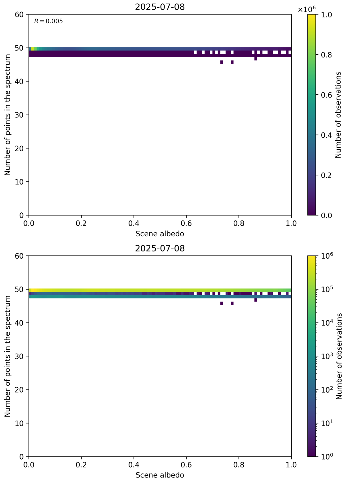
Figure 106: Scatter density plot of “Scene albedo” against “Number of points in the spectrum” for 2025-07-08 to 2025-07-09.
