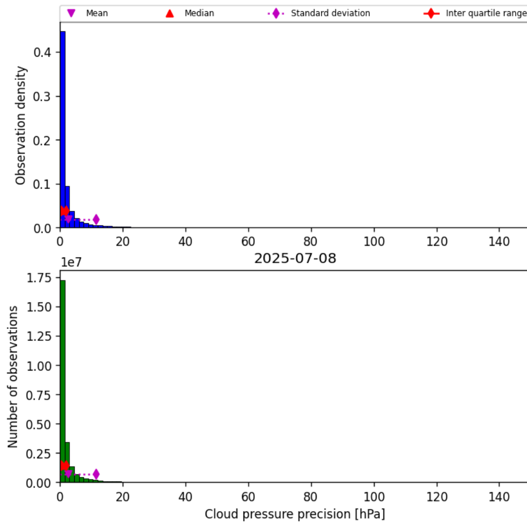
Figure 31: Histogram of “Cloud pressure precision” for 2025-07-08 to 2025-07-09
