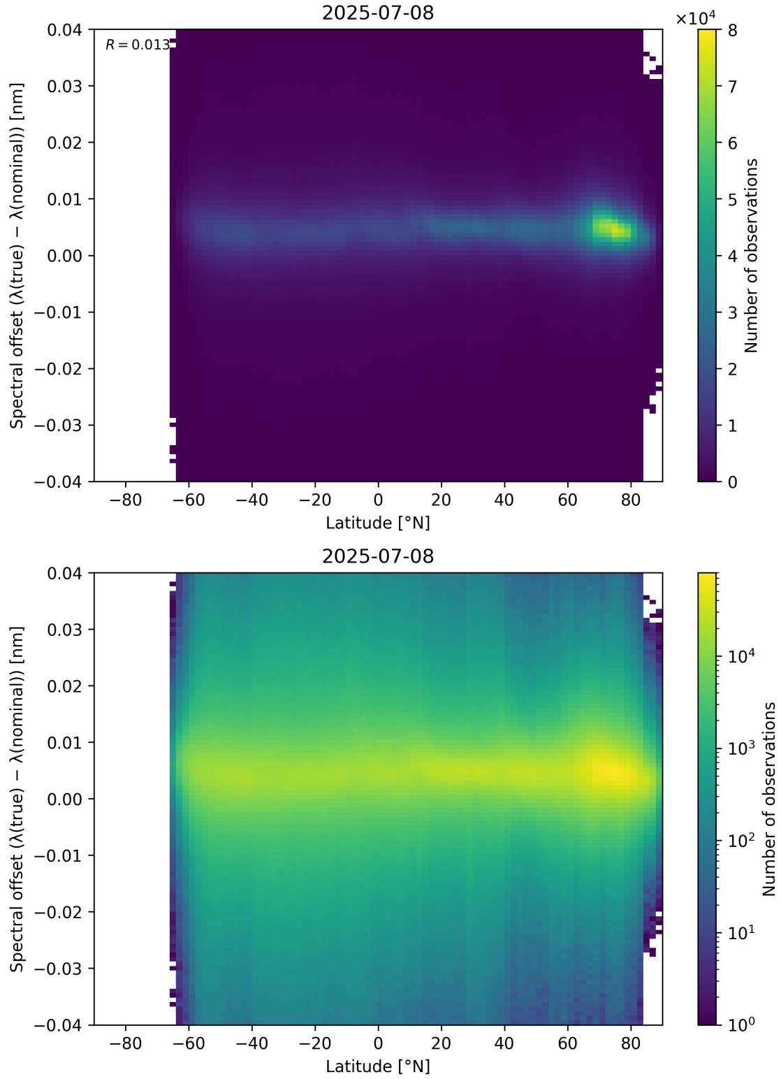
Figure 96: Scatter density plot of “Latitude” against “Spectral offset ( \lambda_{\text{true}} - \lambda_{\text{nominal}} )” for 2025-07-08 to 2025-07-09.
