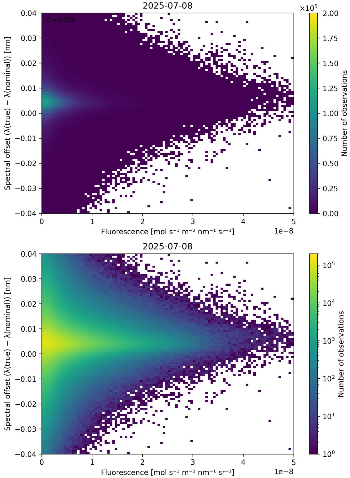
Figure 87: Scatter density plot of “Fluorescence” against “Spectral offset ( \lambda_{\text{true}} - \lambda_{\text{nominal}} )” for 2025-07-08 to 2025-07-09.
