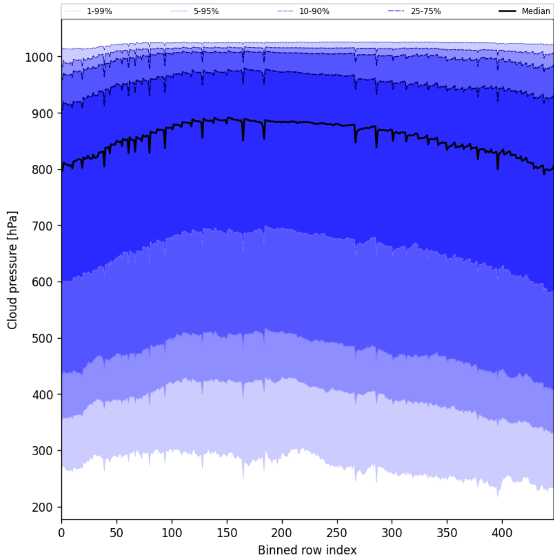
Figure 47: Along track statistics of “Cloud pressure” for 2025-07-08 to 2025-07-09
