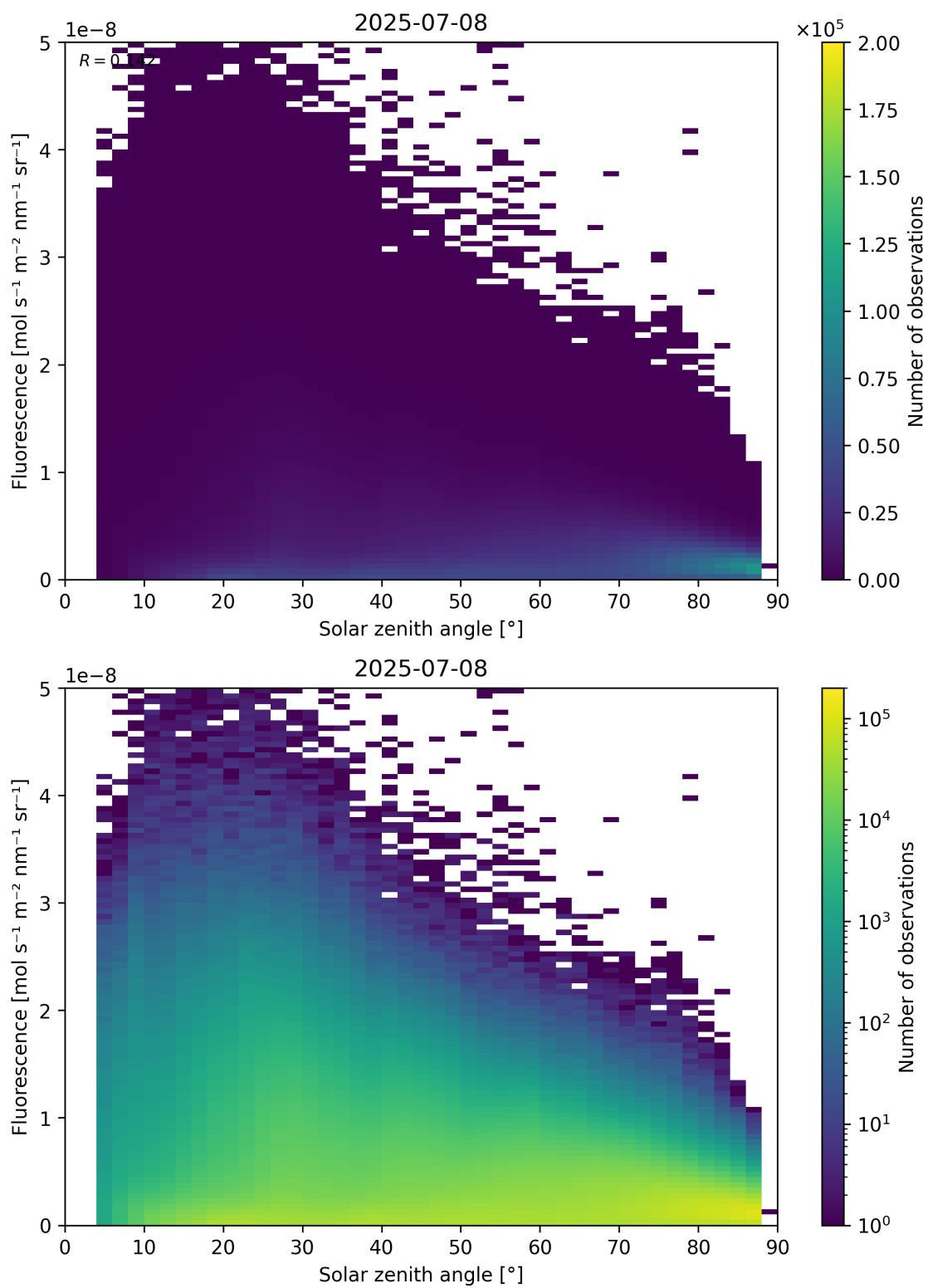
Figure 112: Scatter density plot of “Solar zenith angle” against “Fluorescence” for 2025-07-08 to 2025-07-09.
