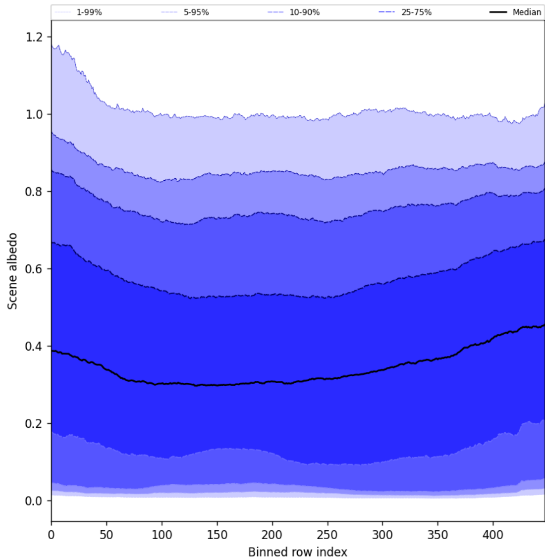
Figure 51: Along track statistics of “Scene albedo” for 2025-07-08 to 2025-07-10
