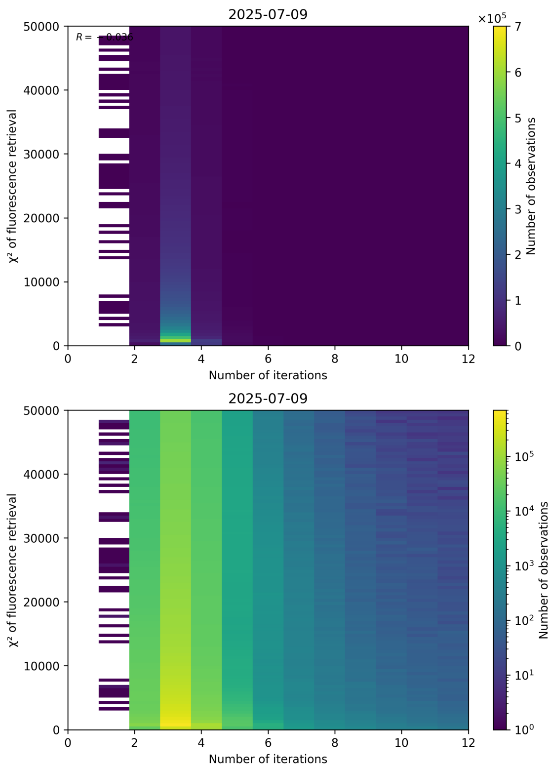
Figure 97: Scatter density plot of “Number of iterations” against “ \chi^2 of fluorescence retrieval” for 2025-07-08 to 2025-07-10.
