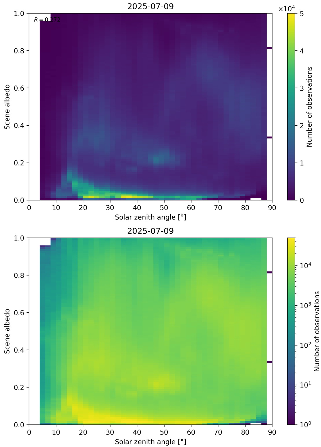
Figure 116: Scatter density plot of “Solar zenith angle” against “Scene albedo” for 2025-07-08 to 2025-07-10.
