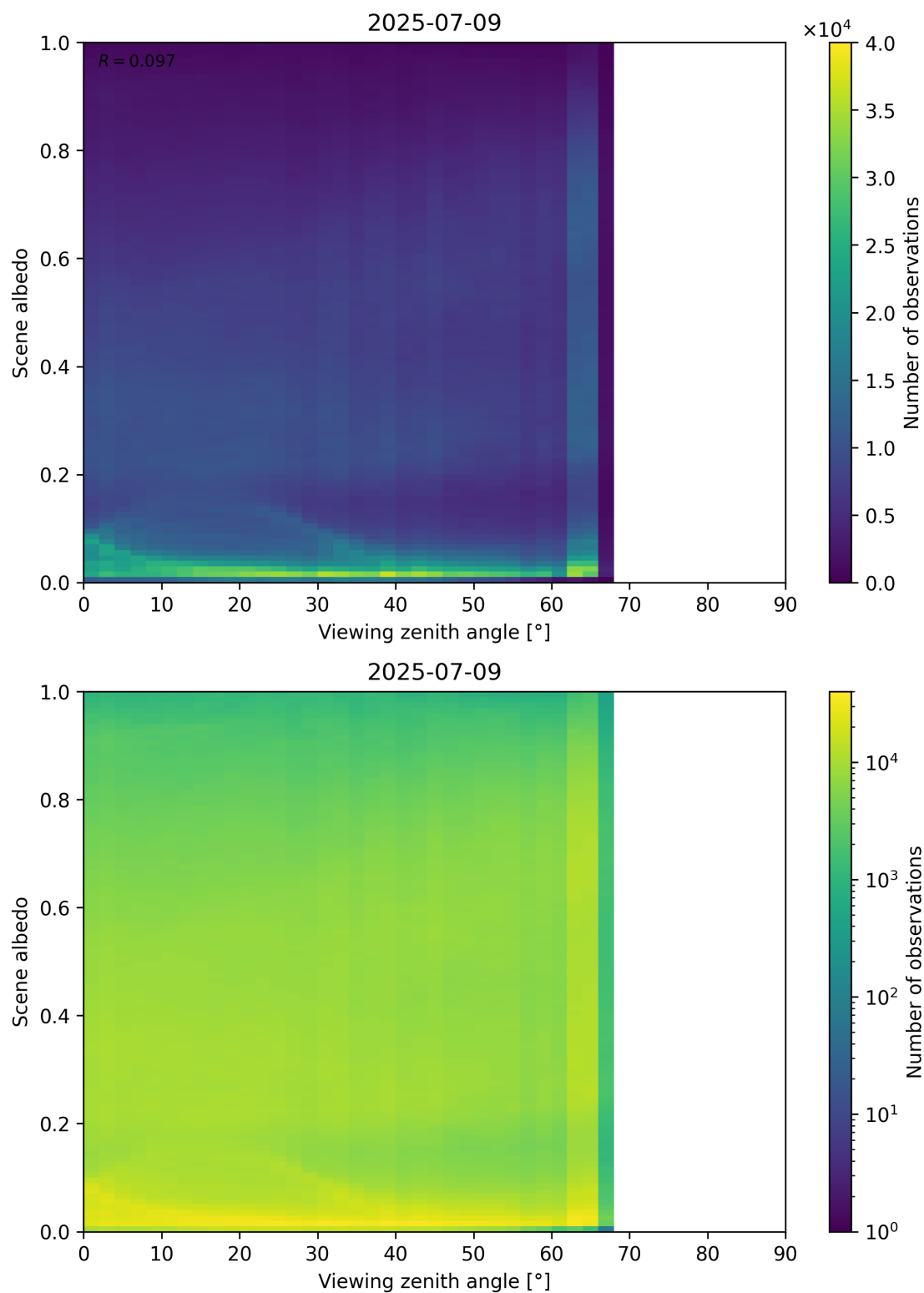
Figure 126: Scatter density plot of “Viewing zenith angle” against “Scene albedo” for 2025-07-08 to 2025-07-10.
