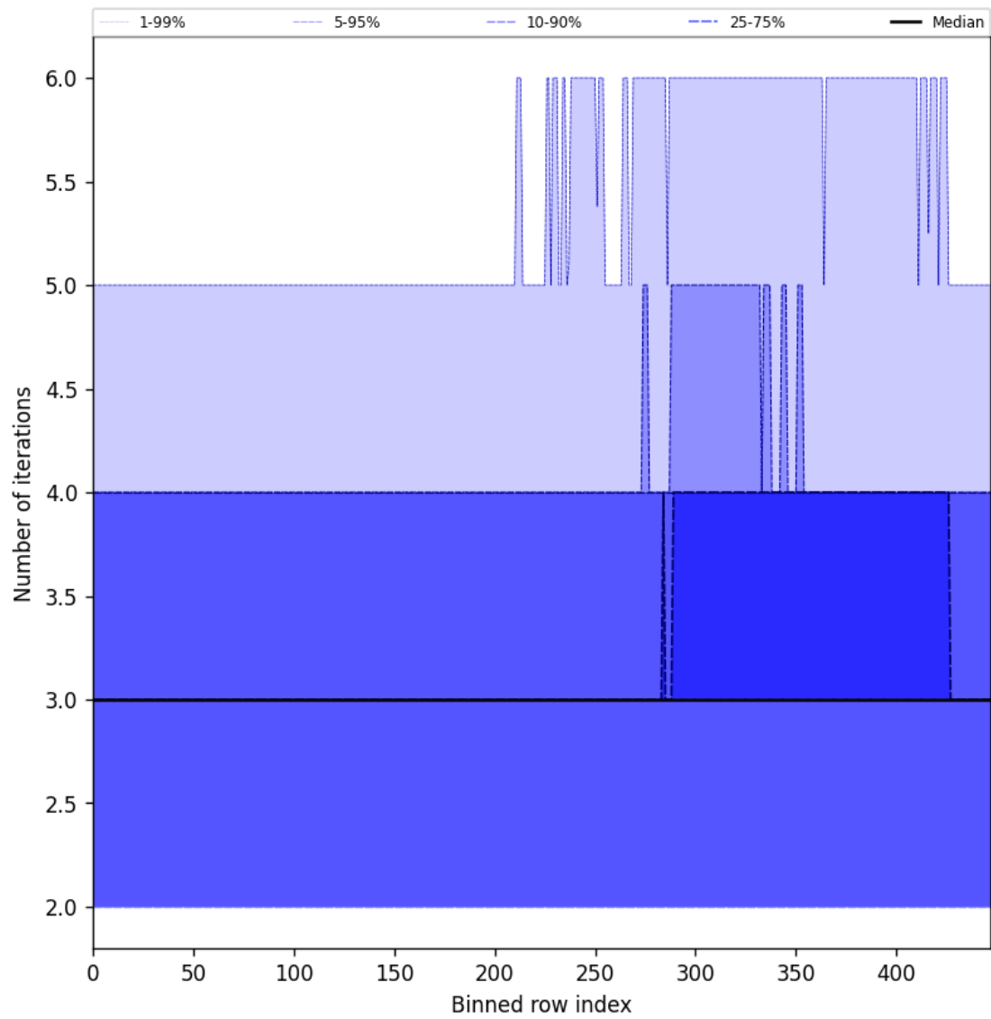
Figure 56: Along track statistics of "Number of iterations" for 2025-07-08 to 2025-07-10
