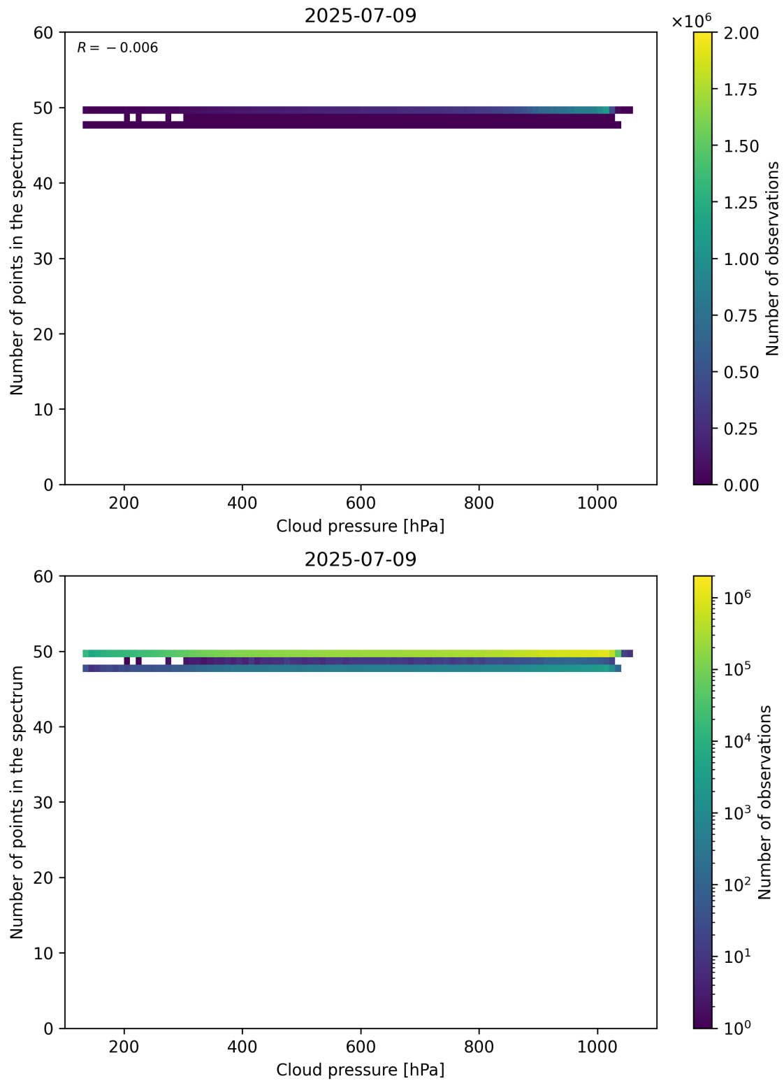
Figure 82: Scatter density plot of “Cloud pressure” against “Number of points in the spectrum” for 2025-07-08 to 2025-07-10.
