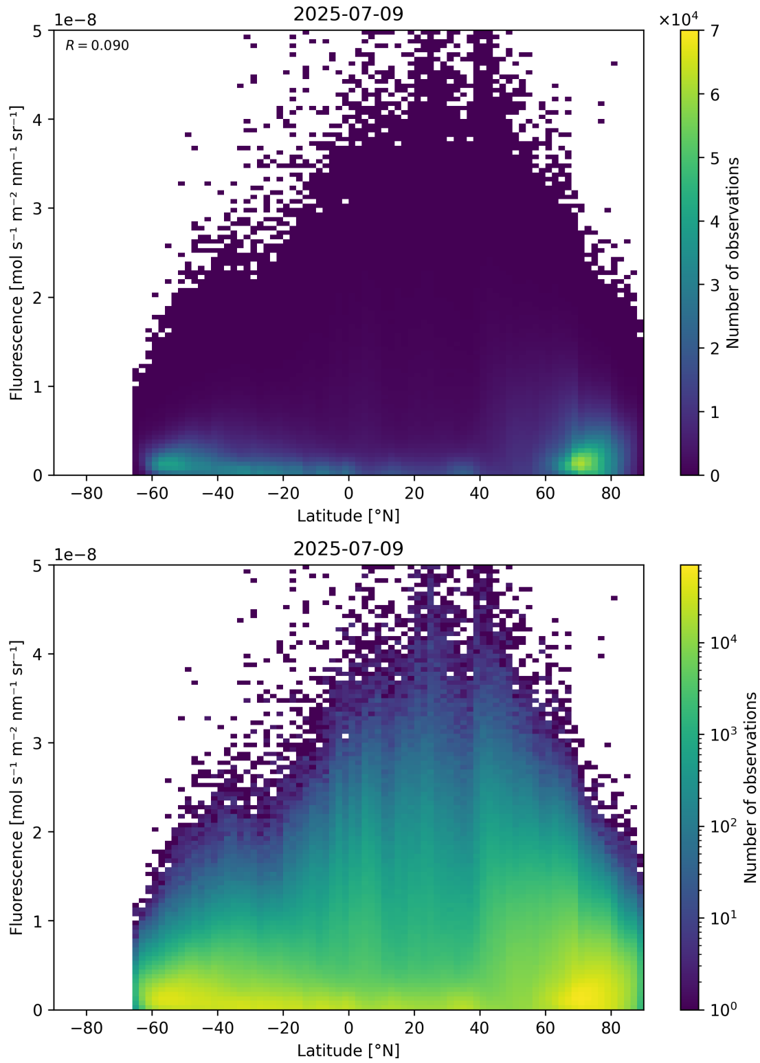
Figure 92: Scatter density plot of “Latitude” against “Fluorescence” for 2025-07-08 to 2025-07-10.
