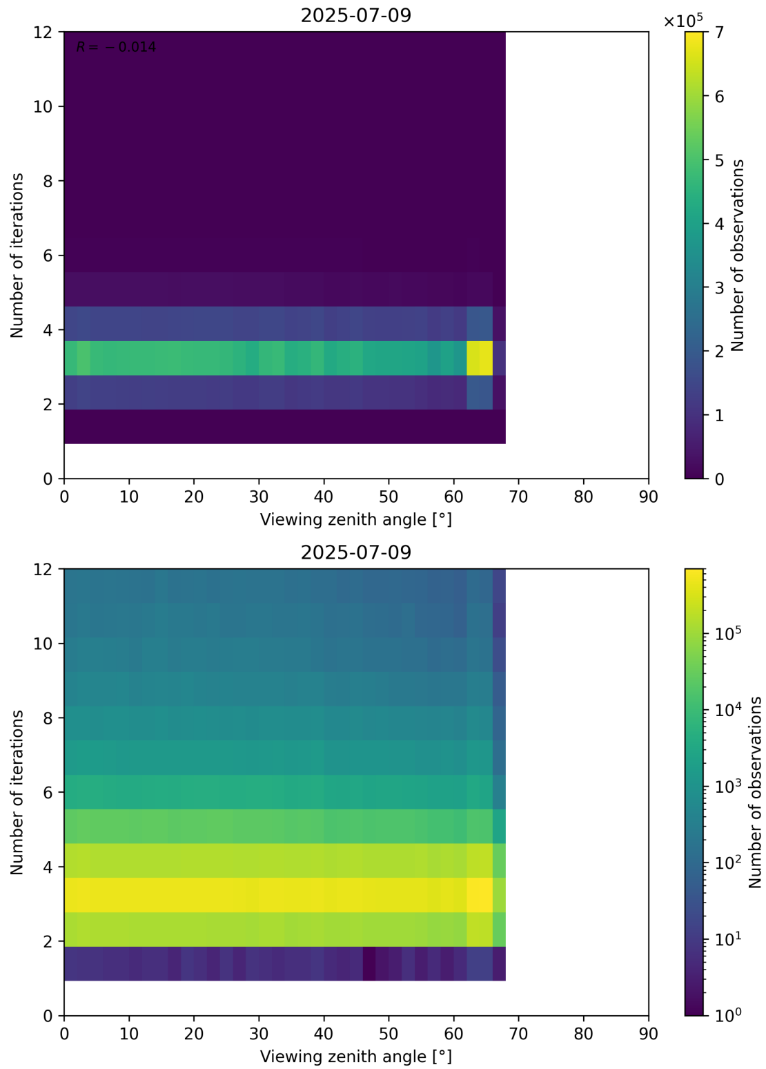
Figure 124: Scatter density plot of “Viewing zenith angle” against “Number of iterations” for 2025-07-08 to 2025-07-10.
