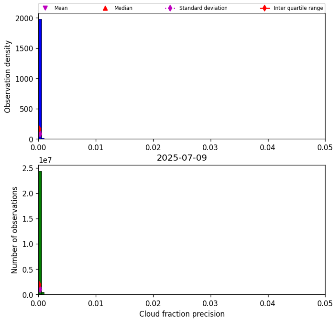
Figure 33: Histogram of “Cloud fraction precision” for 2025-07-08 to 2025-07-10
