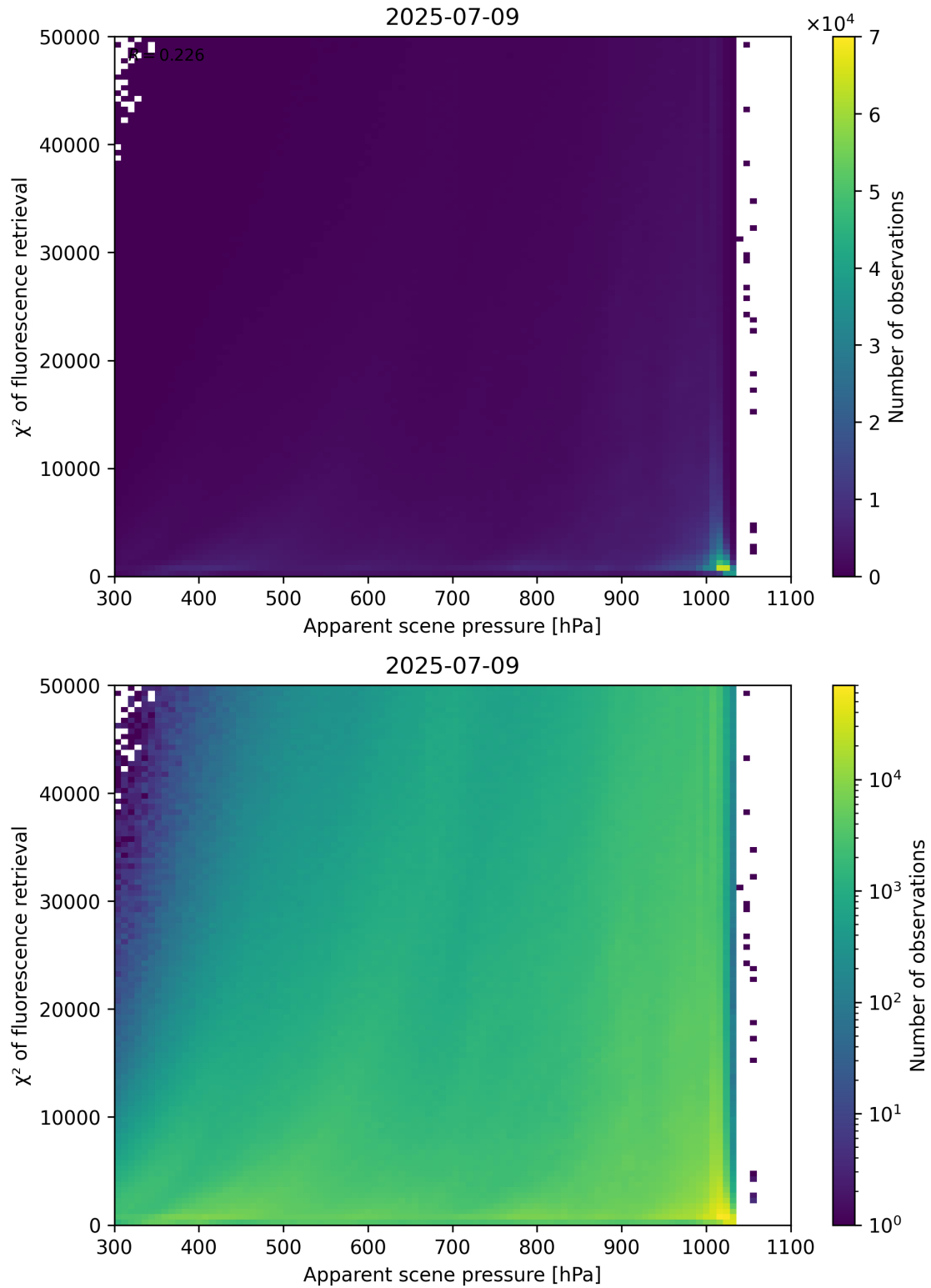
Figure 63: Scatter density plot of “Apparent scene pressure” against “ \chi^2 of fluorescence retrieval” for 2025-07-08 to 2025-07-10.
