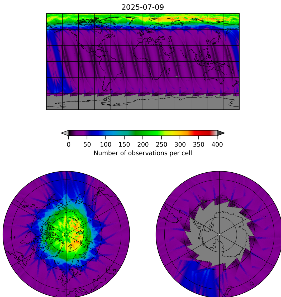
Figure 11: Map of the number of observations for 2025-07-08 to 2025-07-10
