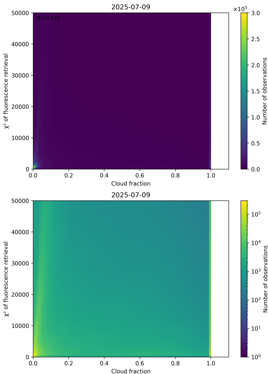
Figure 71: Scatter density plot of “Cloud fraction” against “ \chi^2 of fluorescence retrieval” for 2025-07-08 to 2025-07-10.
