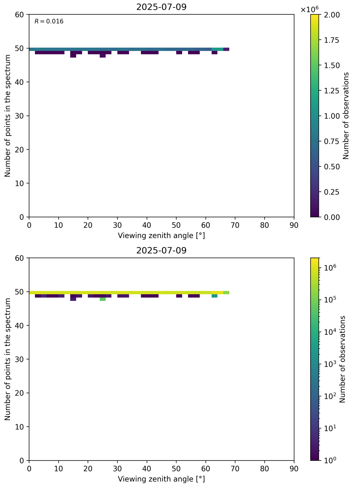
Figure 125: Scatter density plot of “Viewing zenith angle” against “Number of points in the spectrum” for 2025-07-08 to 2025-07-10.
