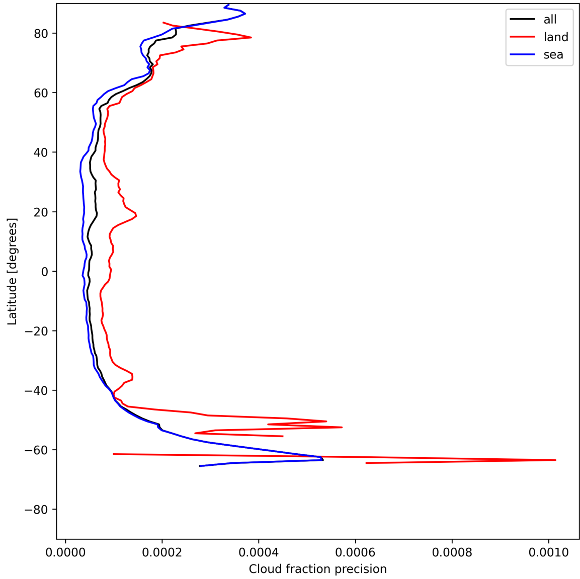
Figure 16: Zonal average of “Cloud fraction precision” for 2025-07-08 to 2025-07-10.
