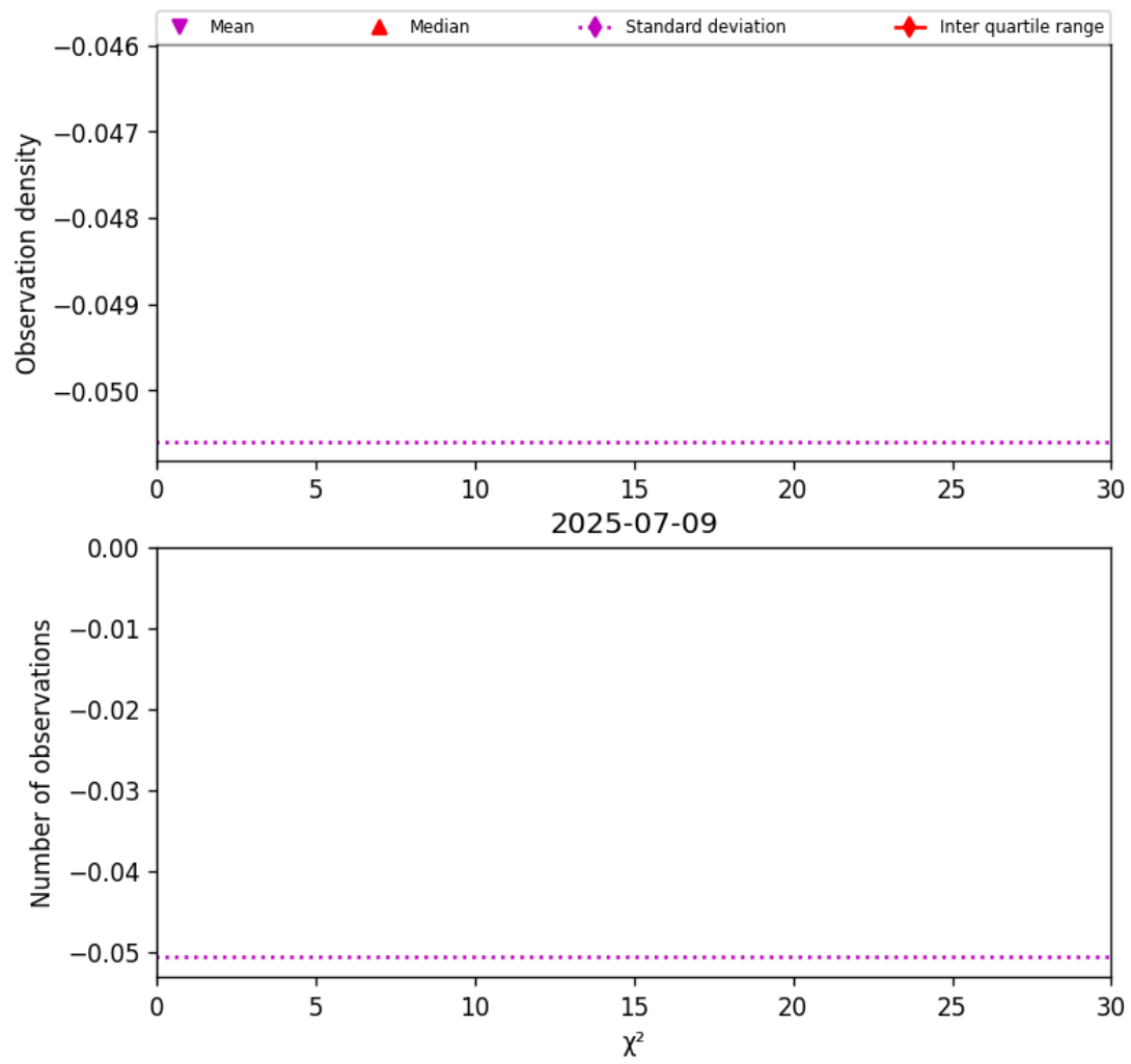
Figure 38: Histogram of " \chi^2 " for 2025-07-08 to 2025-07-10
