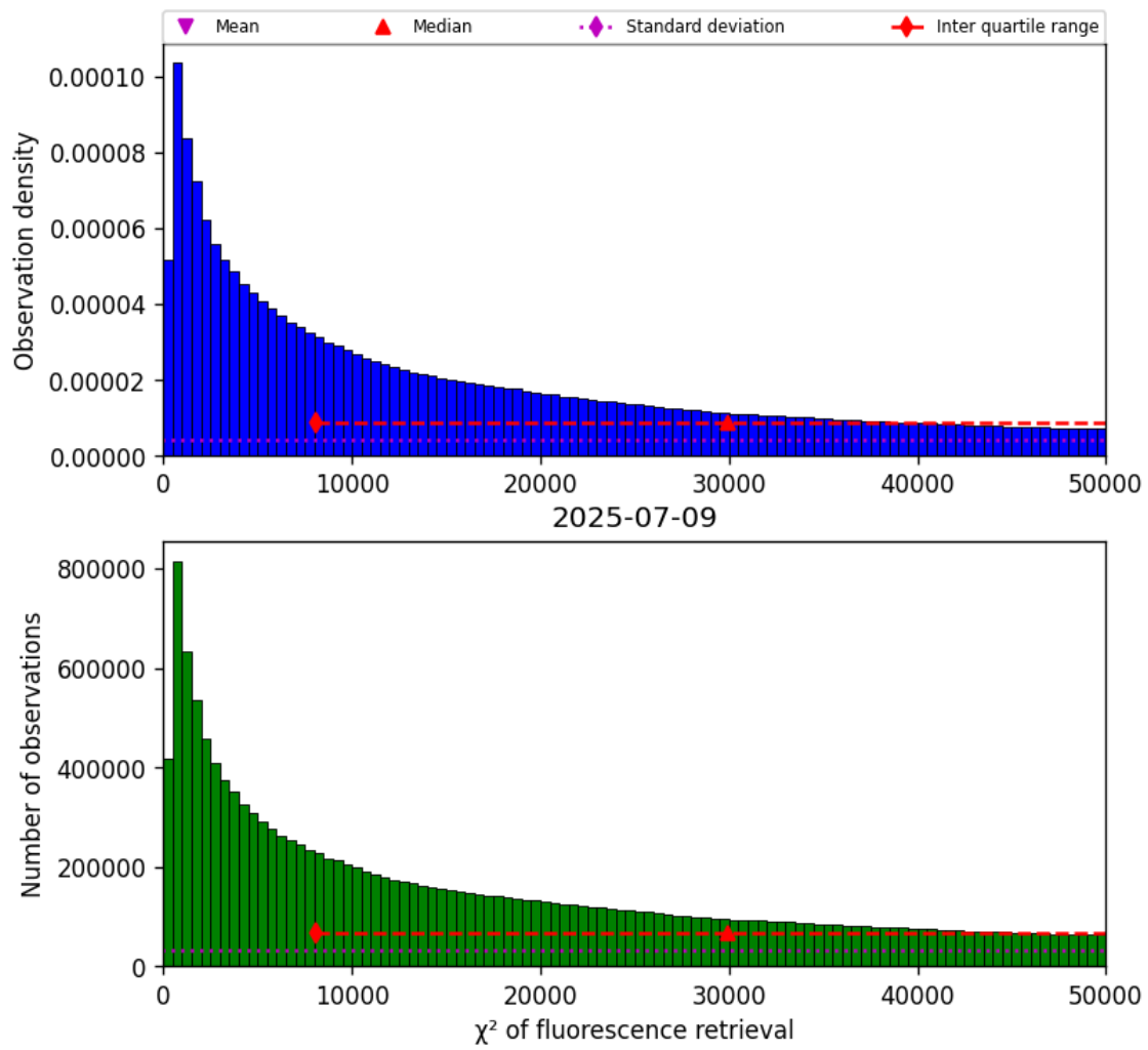
Figure 42: Histogram of “ \chi^2 of fluorescence retrieval” for 2025-07-08 to 2025-07-10
