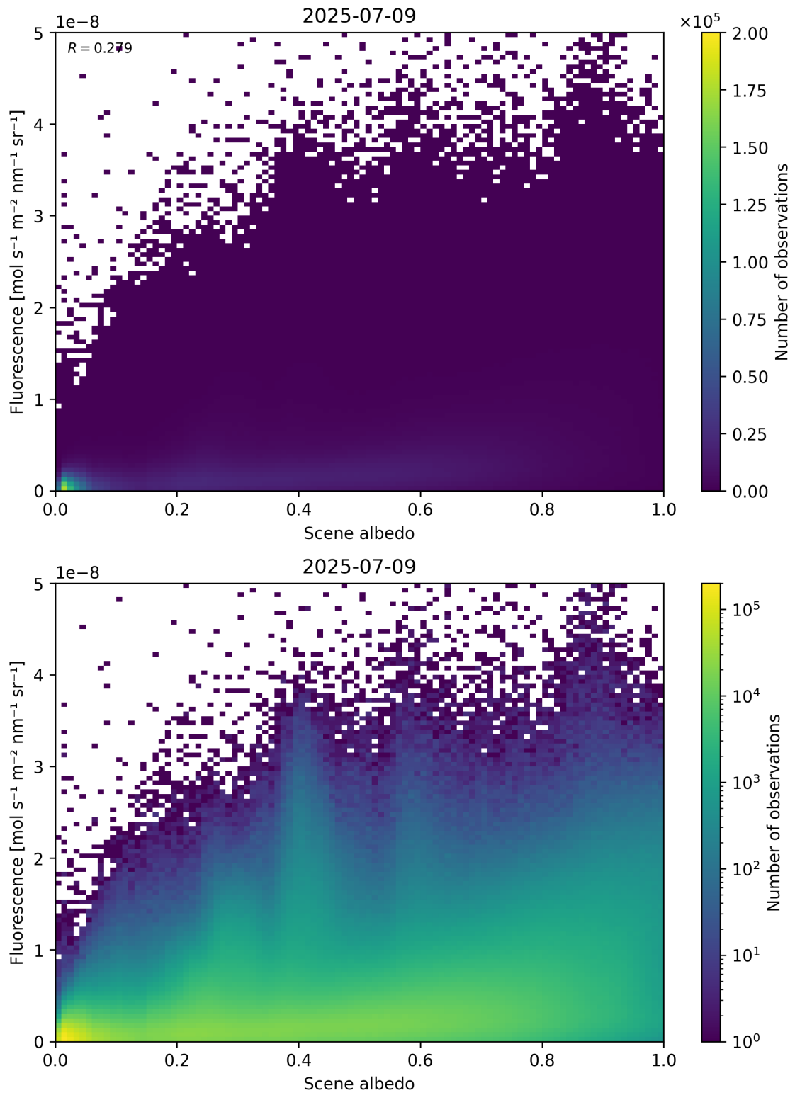
Figure 104: Scatter density plot of “Scene albedo” against “Fluorescence” for 2025-07-08 to 2025-07-10.
