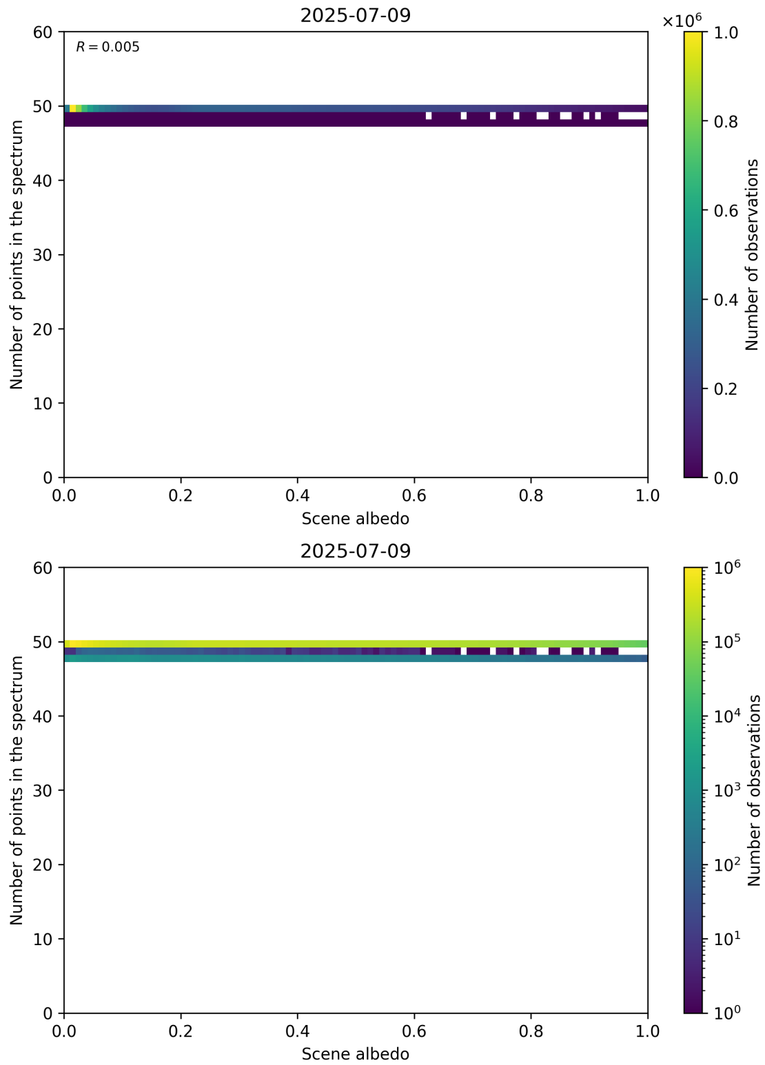
Figure 106: Scatter density plot of “Scene albedo” against “Number of points in the spectrum” for 2025-07-08 to 2025-07-10.
