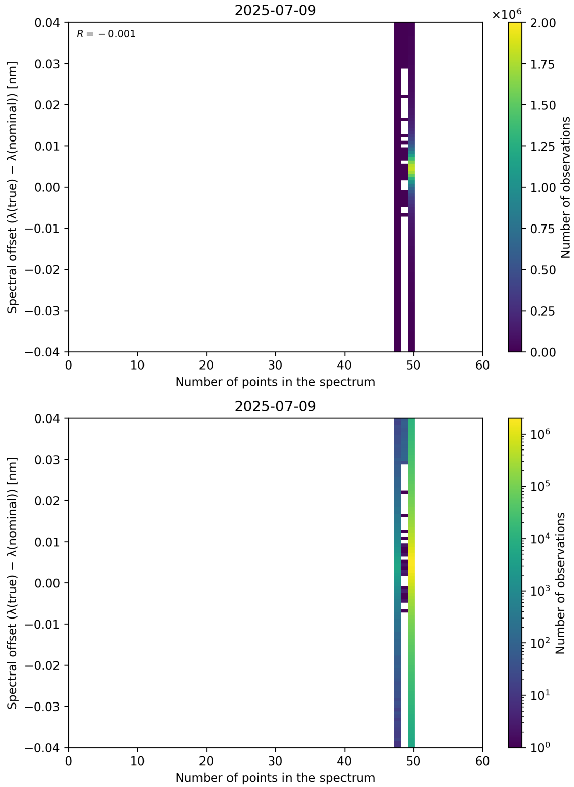
Figure 101: Scatter density plot of “Number of points in the spectrum” against “Spectral offset ( \lambda_{\text{true}} - \lambda_{\text{nominal}} )” for 2025-07-08 to 2025-07-10.
