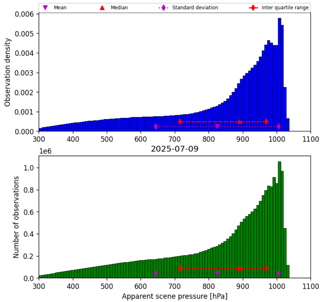
Figure 36: Histogram of “Apparent scene pressure” for 2025-07-08 to 2025-07-10
