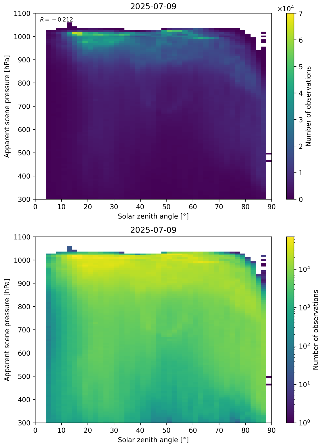
Figure 108: Scatter density plot of “Solar zenith angle” against “Apparent scene pressure” for 2025-07-08 to 2025-07-10.
