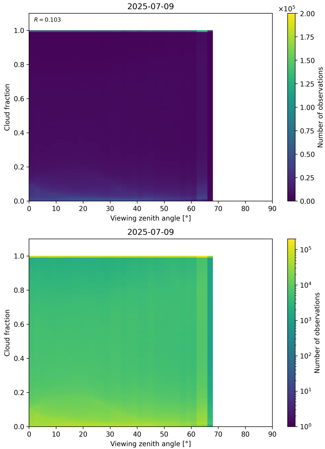
Figure 120: Scatter density plot of “Viewing zenith angle” against “Cloud fraction” for 2025-07-08 to 2025-07-10.
