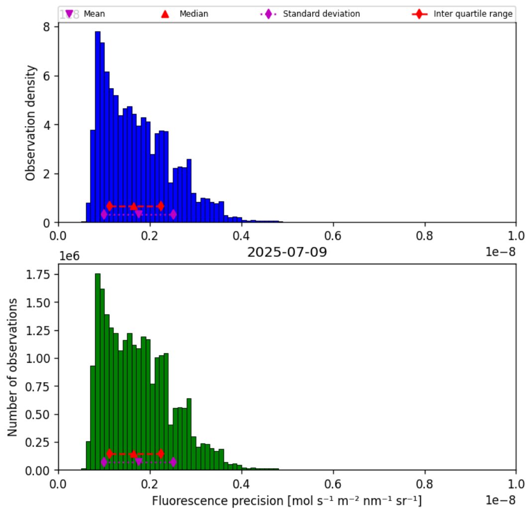
Figure 41: Histogram of “Fluorescence precision” for 2025-07-08 to 2025-07-10
