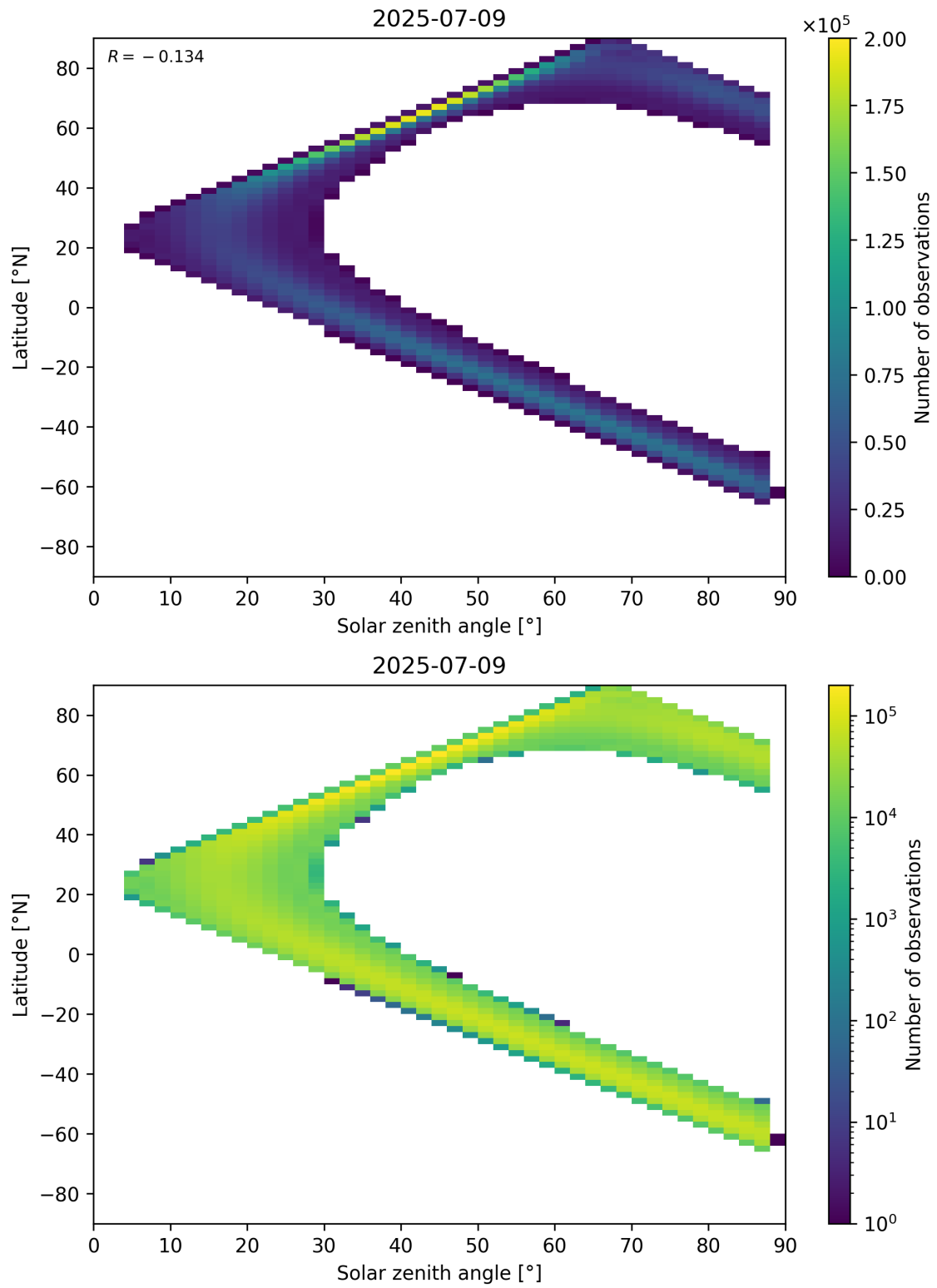
Figure 113: Scatter density plot of “Solar zenith angle” against “Latitude” for 2025-07-08 to 2025-07-10.
