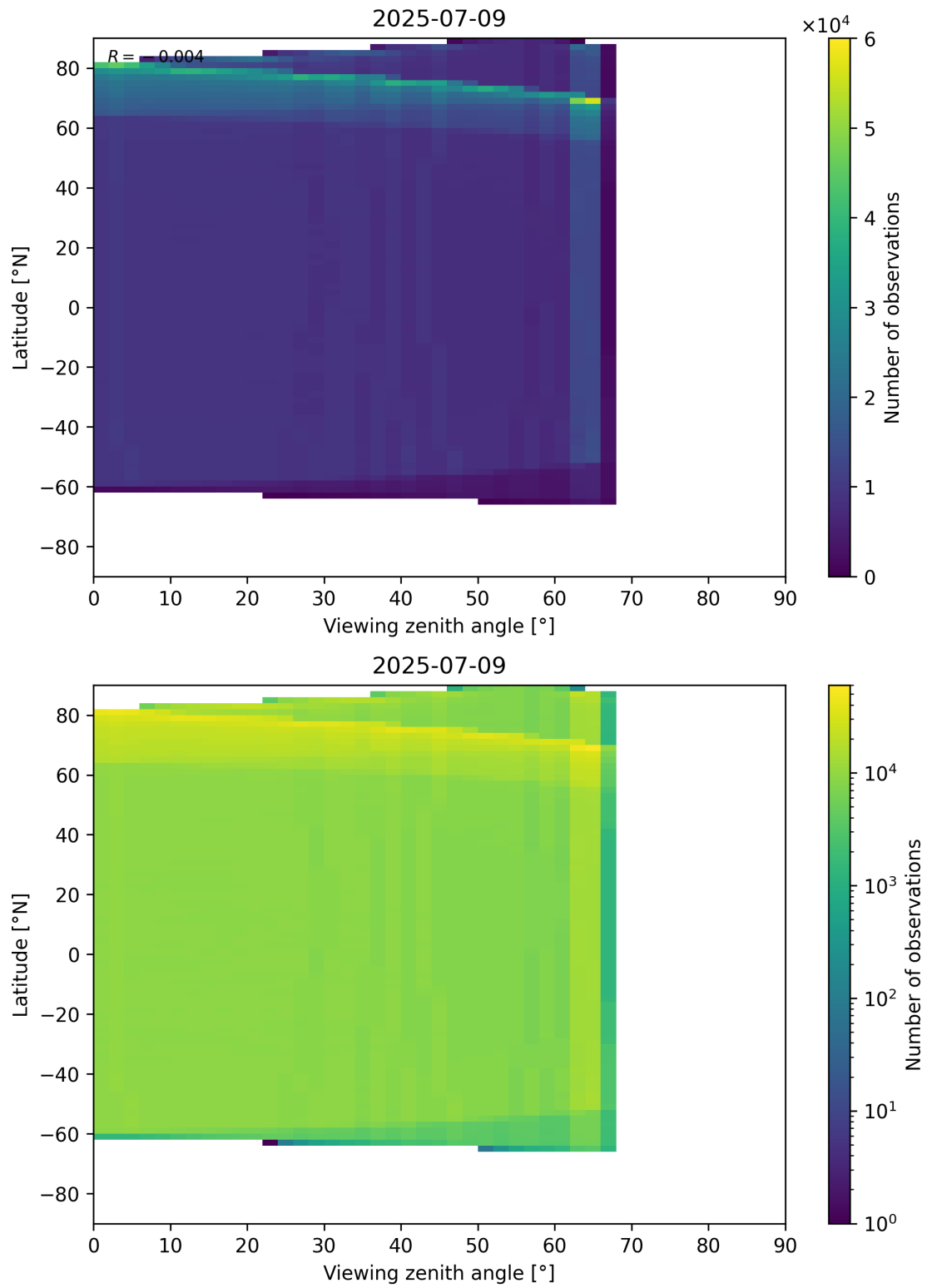
Figure 123: Scatter density plot of “Viewing zenith angle” against “Latitude” for 2025-07-08 to 2025-07-10.
