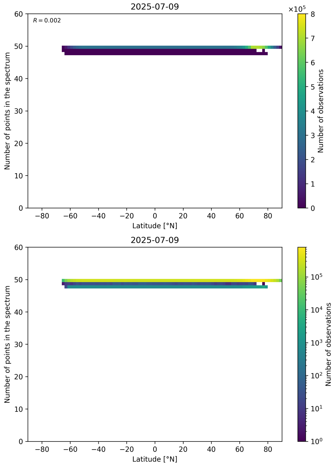
Figure 94: Scatter density plot of “Latitude” against “Number of points in the spectrum” for 2025-07-08 to 2025-07-10.
