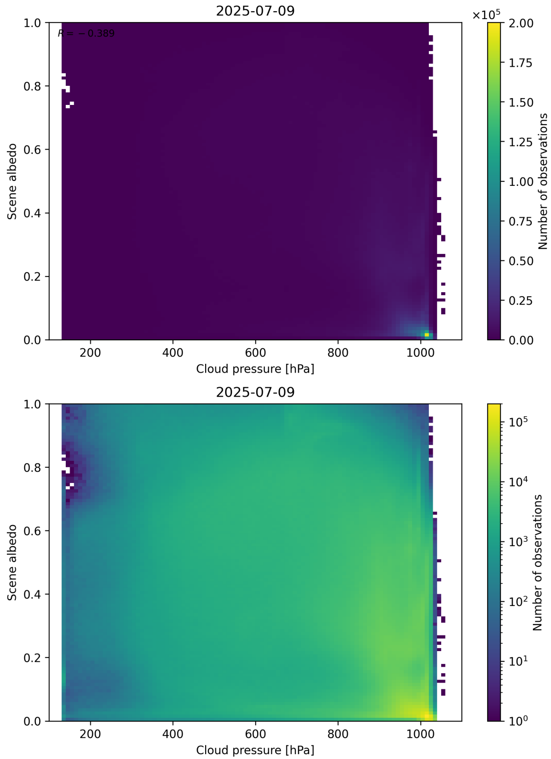
Figure 83: Scatter density plot of “Cloud pressure” against “Scene albedo” for 2025-07-08 to 2025-07-10.
