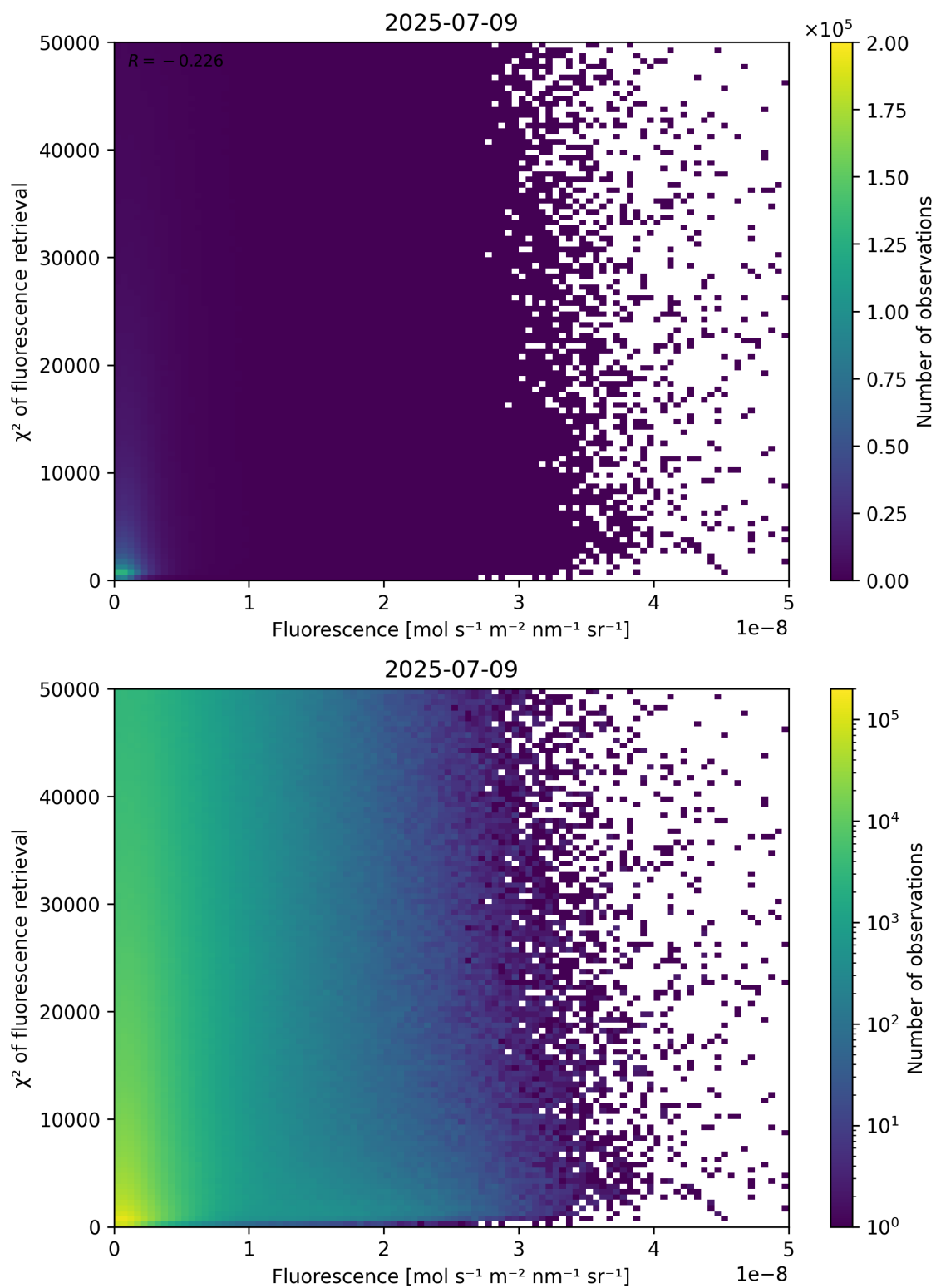
Figure 85: Scatter density plot of “Fluorescence” against “ \chi^2 of fluorescence retrieval” for 2025-07-08 to 2025-07-10.
