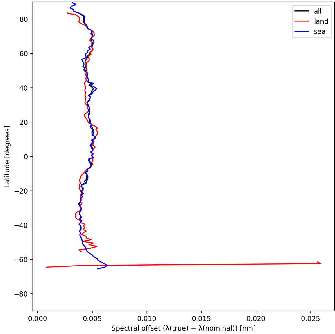
Figure 28: Zonal average of “Spectral offset ( \lambda_{\text{true}} - \lambda_{\text{nominal}} )” for 2025-07-08 to 2025-07-10.
