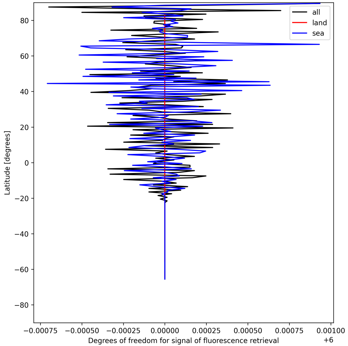
Figure 26: Zonal average of “Degrees of freedom for signal of fluorescence retrieval” for 2025-07-08 to 2025-07-10.
