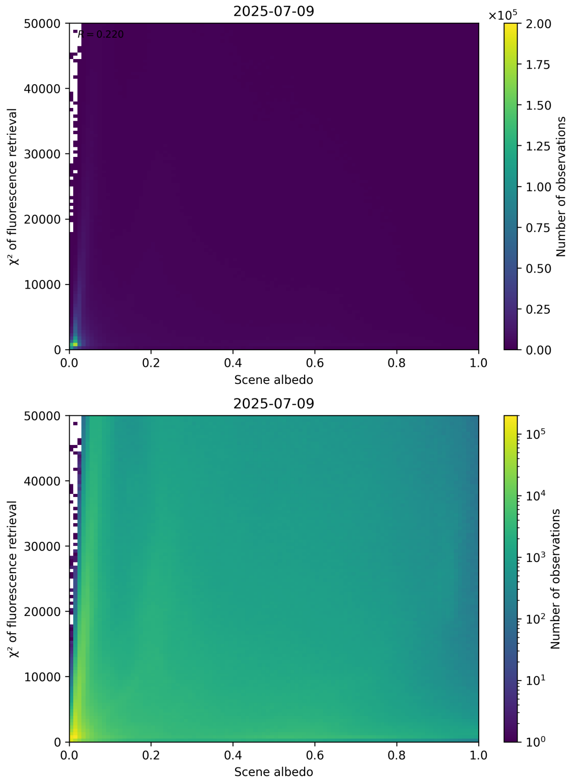
Figure 103: Scatter density plot of “Scene albedo” against “ \chi^2 of fluorescence retrieval” for 2025-07-08 to 2025-07-10.
