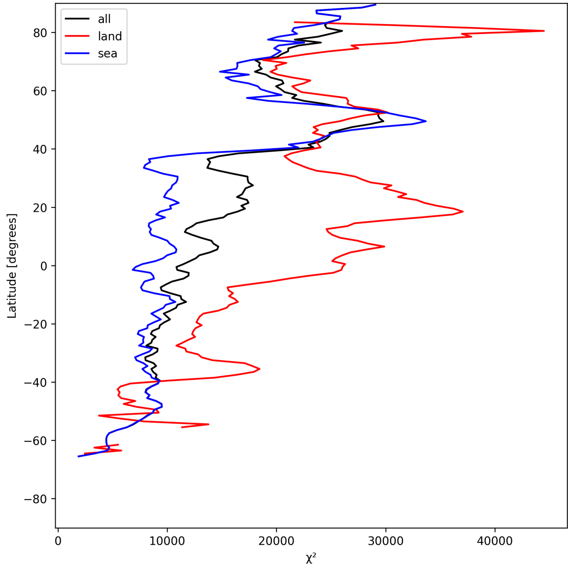
Figure 21: Zonal average of “ \chi^2 ” for 2025-07-08 to 2025-07-10.
