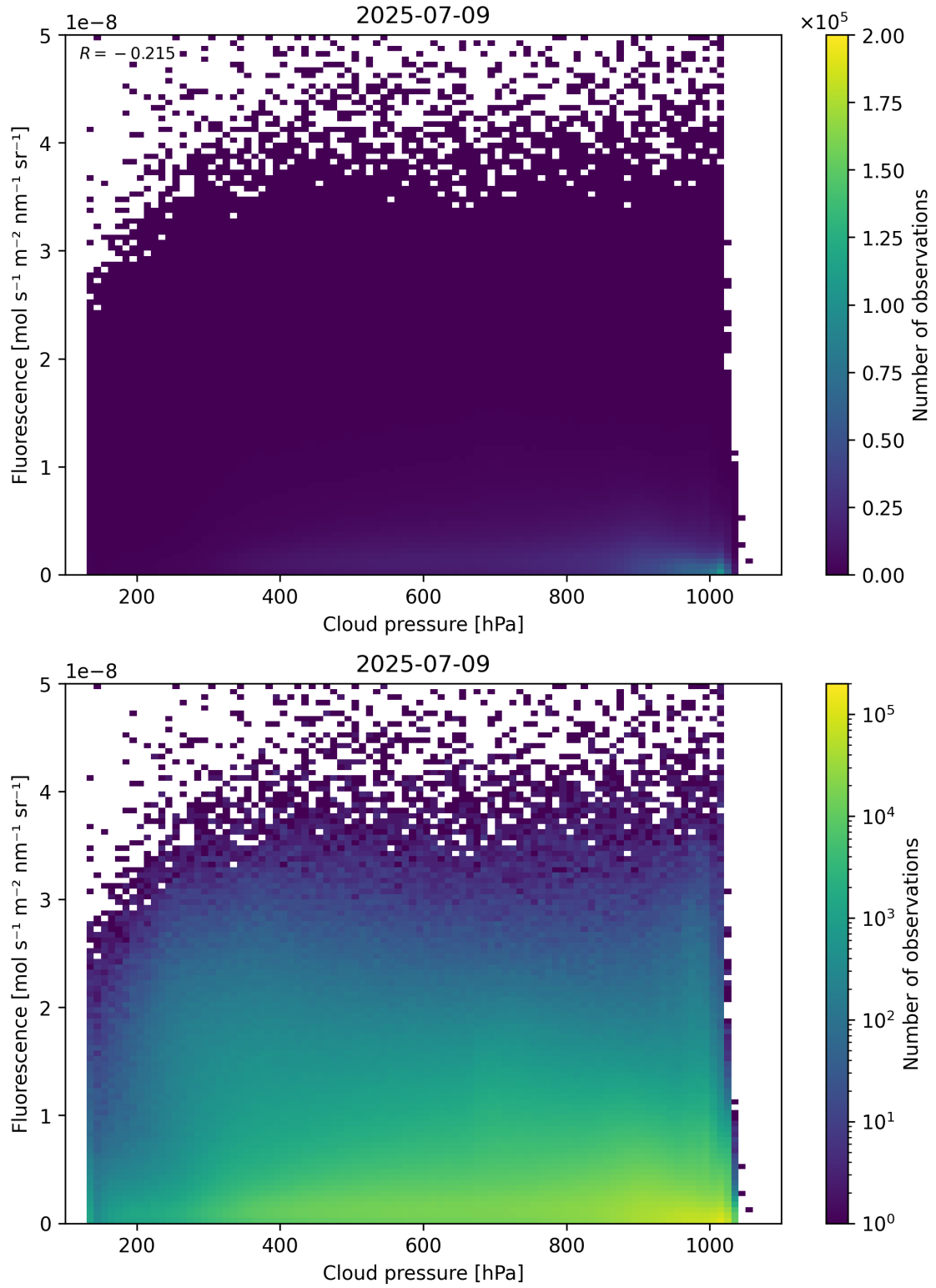
Figure 80: Scatter density plot of “Cloud pressure” against “Fluorescence” for 2025-07-08 to 2025-07-10.
