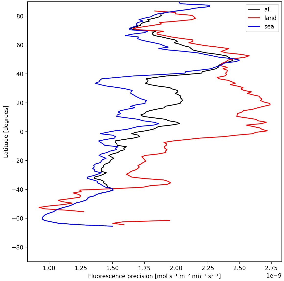
Figure 24: Zonal average of “Fluorescence precision” for 2025-07-08 to 2025-07-10.
