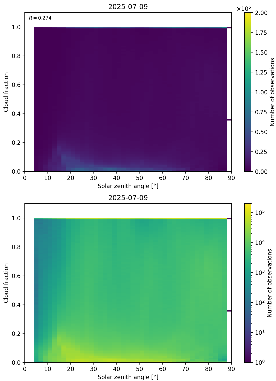
Figure 110: Scatter density plot of “Solar zenith angle” against “Cloud fraction” for 2025-07-08 to 2025-07-10.
