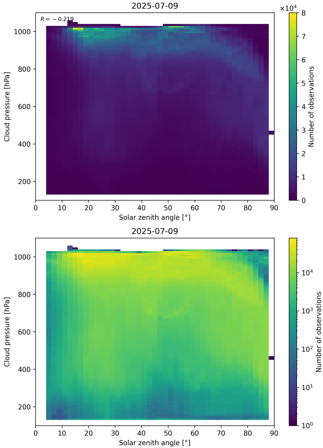
Figure 111: Scatter density plot of “Solar zenith angle” against “Cloud pressure” for 2025-07-08 to 2025-07-10.
