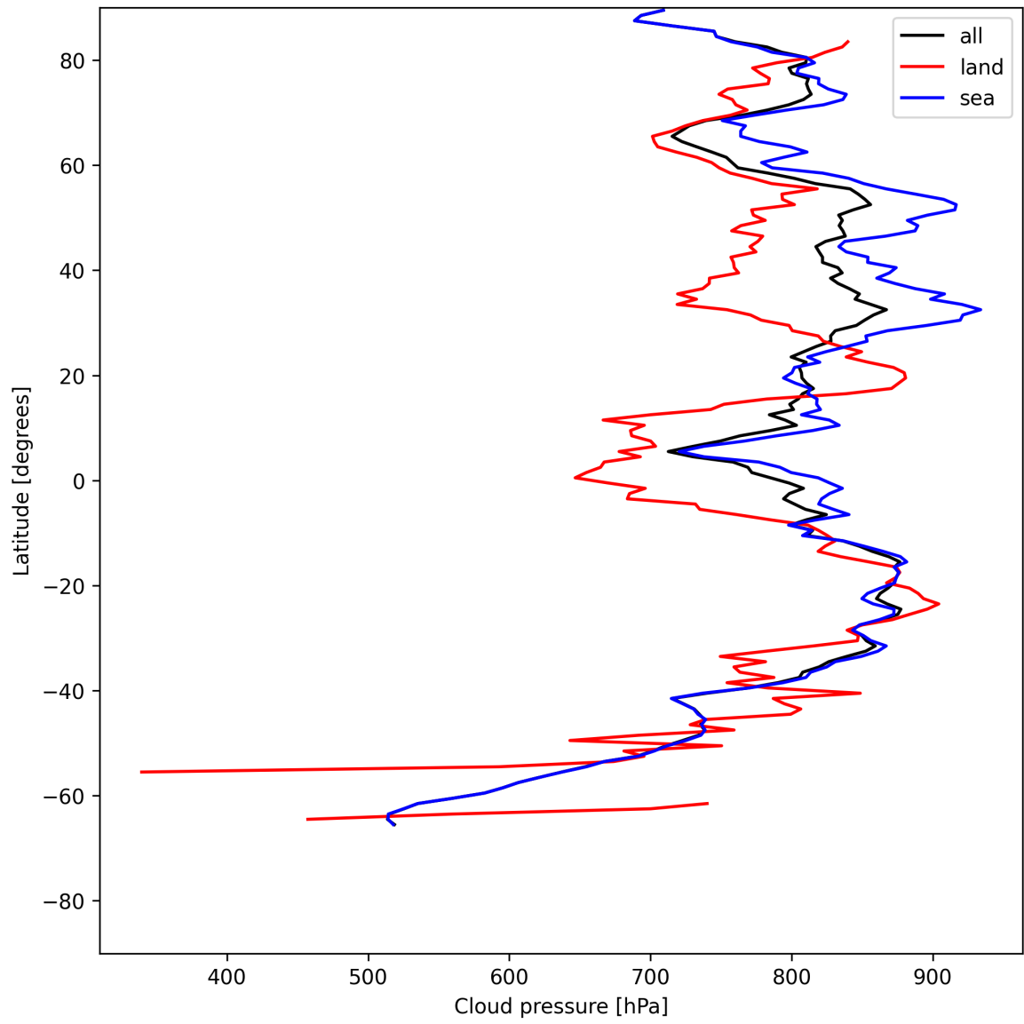
Figure 13: Zonal average of “Cloud pressure” for 2025-07-08 to 2025-07-10.
