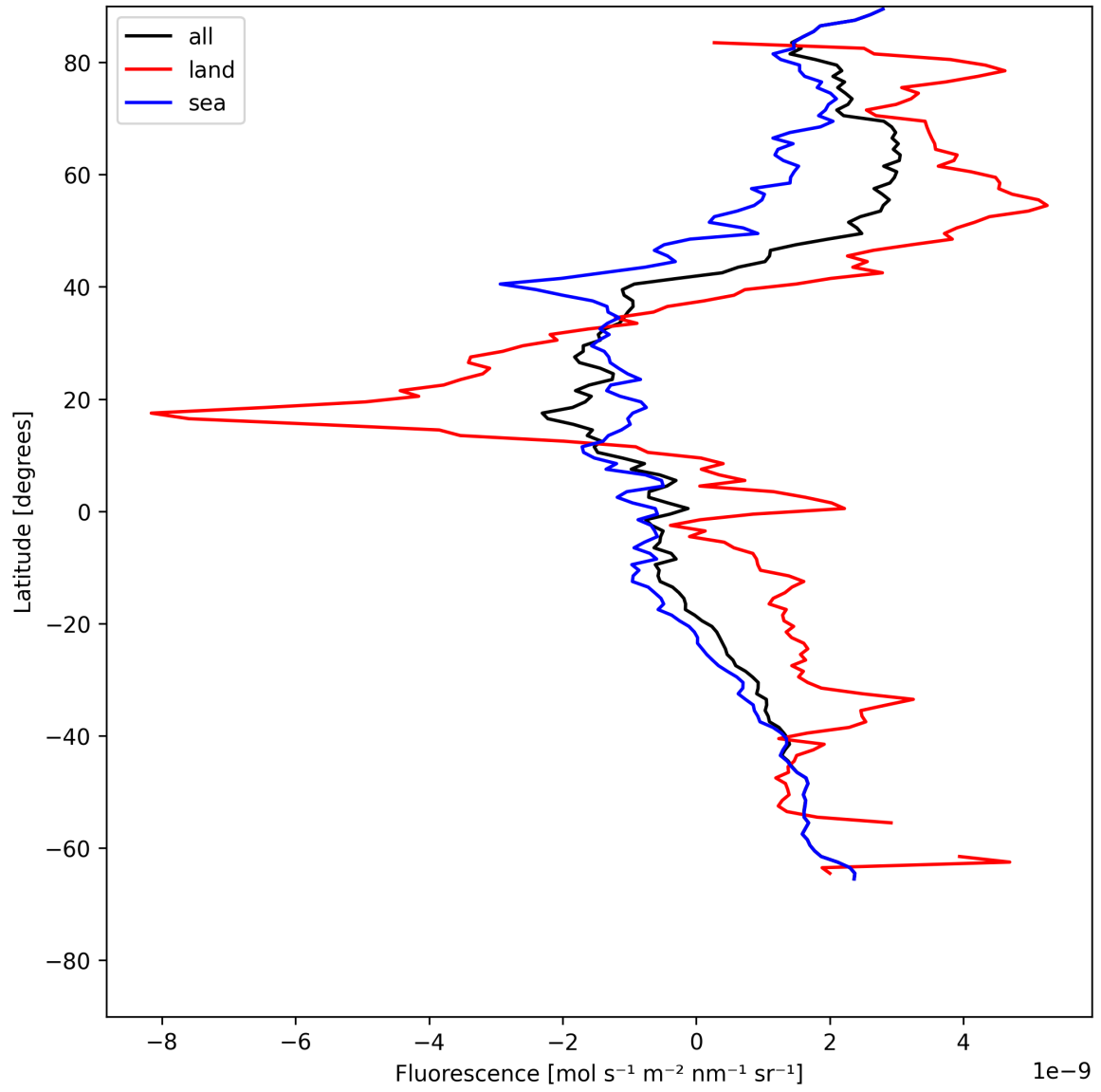
Figure 23: Zonal average of “Fluorescence” for 2025-07-08 to 2025-07-10.
