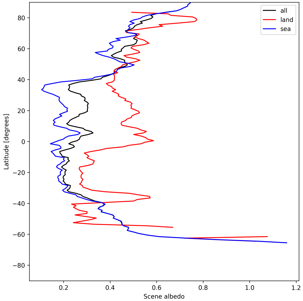
Figure 17: Zonal average of “Scene albedo” for 2025-07-08 to 2025-07-10.
