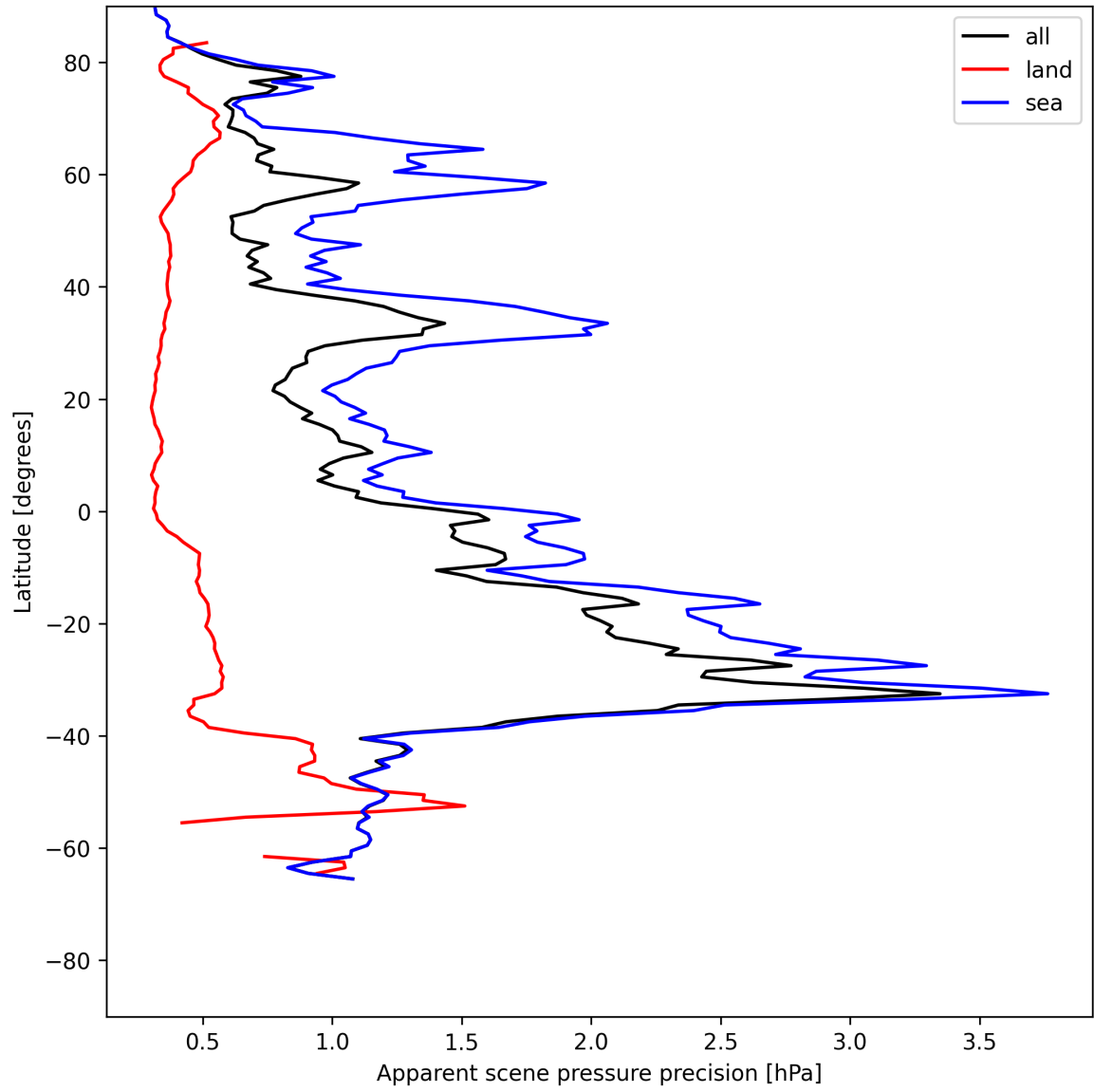
Figure 20: Zonal average of “Apparent scene pressure precision” for 2025-07-08 to 2025-07-10.
