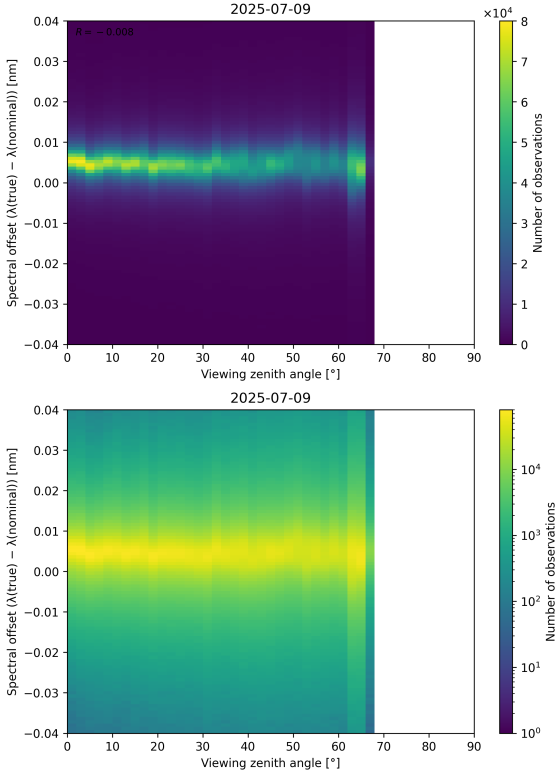
Figure 128: Scatter density plot of “Viewing zenith angle” against “Spectral offset ( \lambda_{\text{true}} - \lambda_{\text{nominal}} )” for 2025-07-08 to 2025-07-10.
