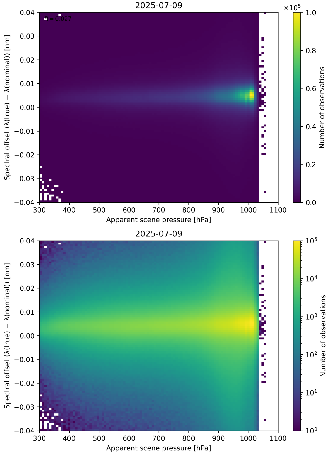
Figure 67: Scatter density plot of “Apparent scene pressure” against “Spectral offset ( \lambda_{\text{true}} - \lambda_{\text{nominal}} )” for 2025-07-08 to 2025-07-10.
