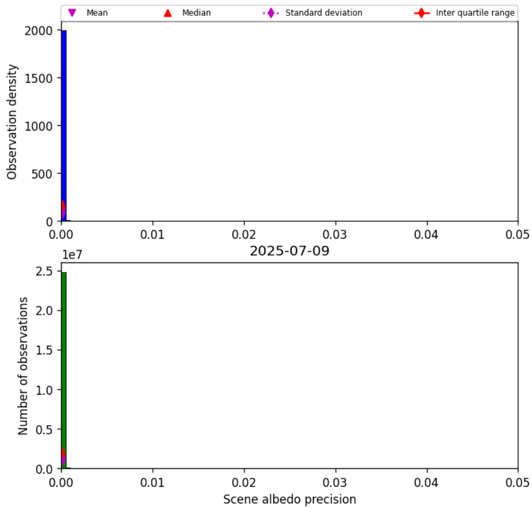
Figure 35: Histogram of “Scene albedo precision” for 2025-07-08 to 2025-07-10
