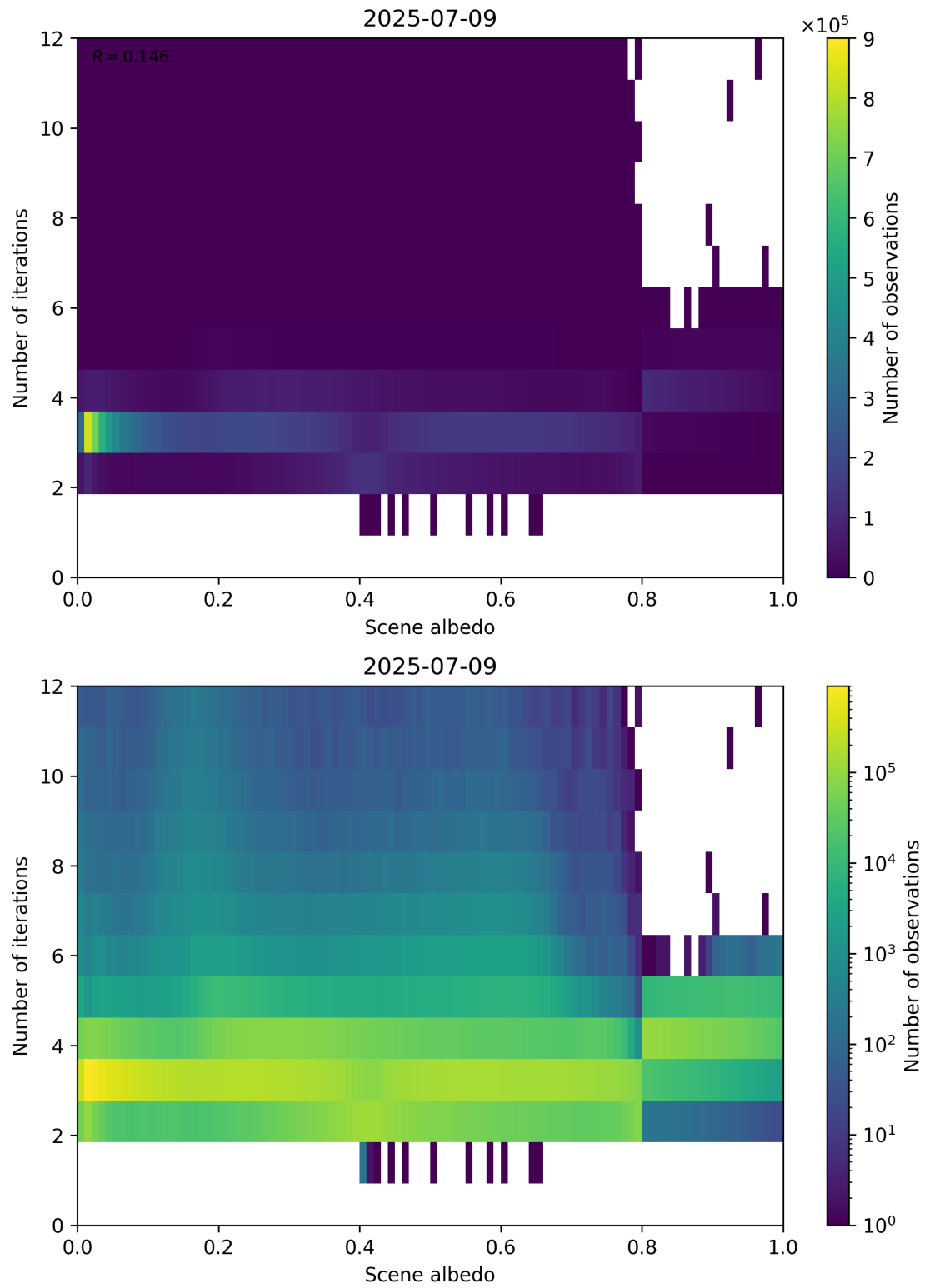
Figure 105: Scatter density plot of “Scene albedo” against “Number of iterations” for 2025-07-08 to 2025-07-10.
