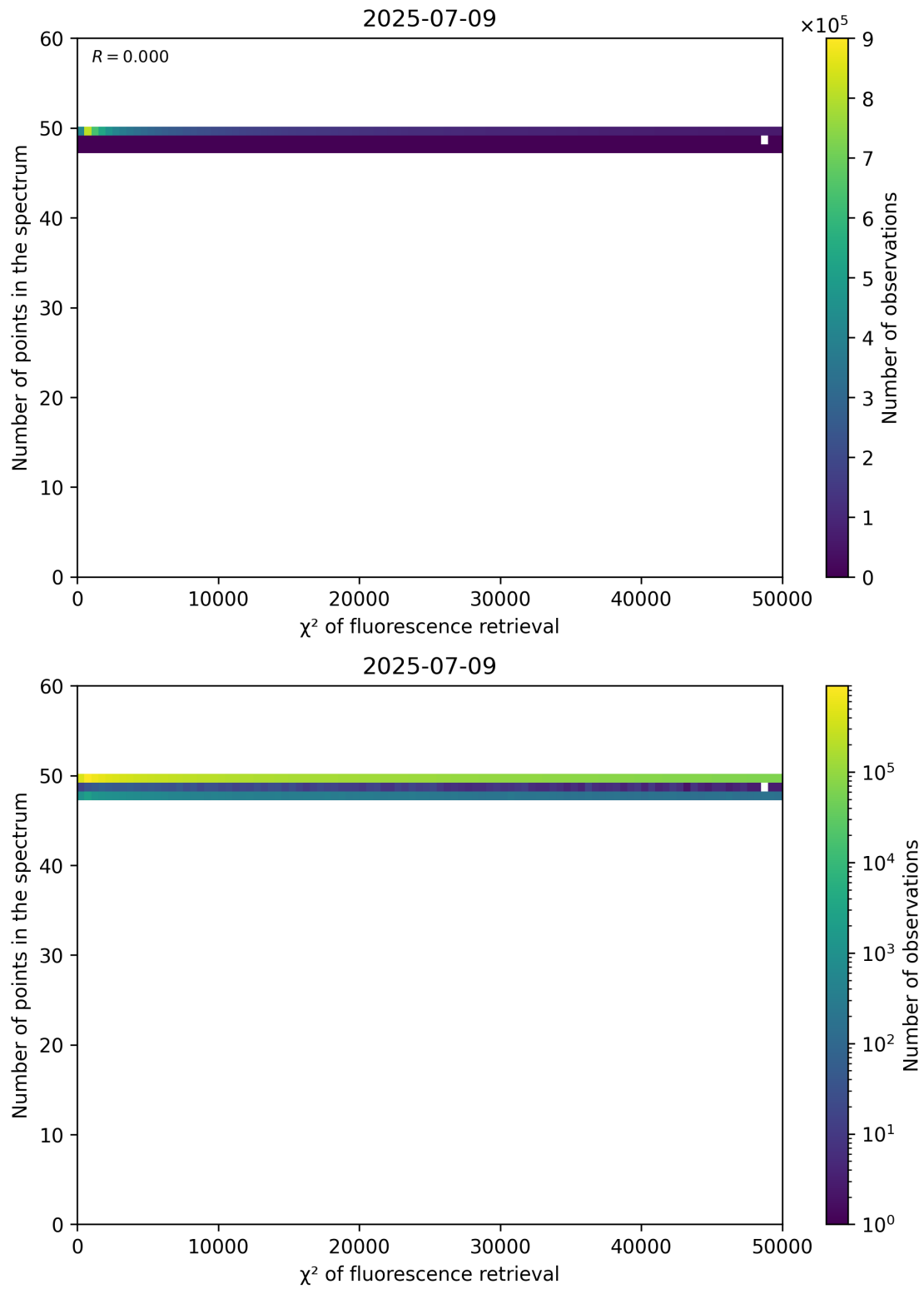
Figure 68: Scatter density plot of " \chi^2 of fluorescence retrieval" against "Number of points in the spectrum" for 2025-07-08 to 2025-07-10.
