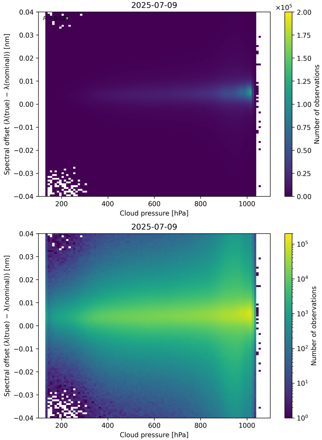
Figure 84: Scatter density plot of “Cloud pressure” against “Spectral offset ( \lambda_{\text{true}} - \lambda_{\text{nominal}} )” for 2025-07-08 to 2025-07-10.
