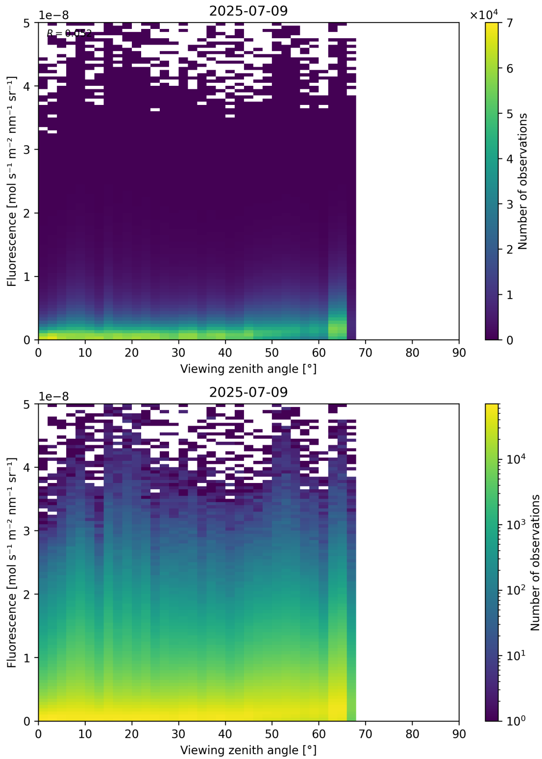
Figure 122: Scatter density plot of “Viewing zenith angle” against “Fluorescence” for 2025-07-08 to 2025-07-10.
