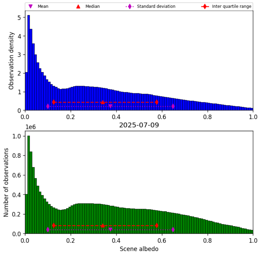
Figure 34: Histogram of “Scene albedo” for 2025-07-08 to 2025-07-10
