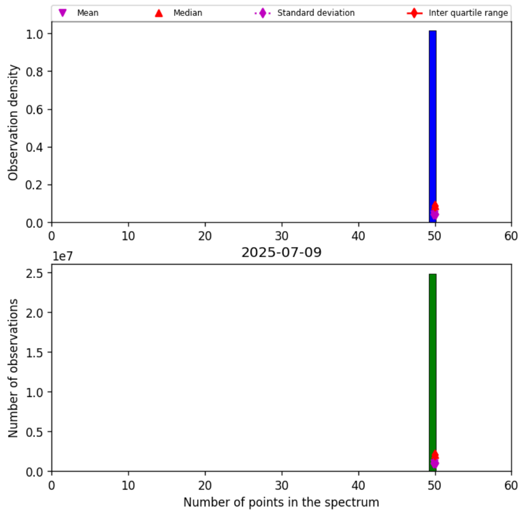
Figure 44: Histogram of “Number of points in the spectrum” for 2025-07-08 to 2025-07-10
