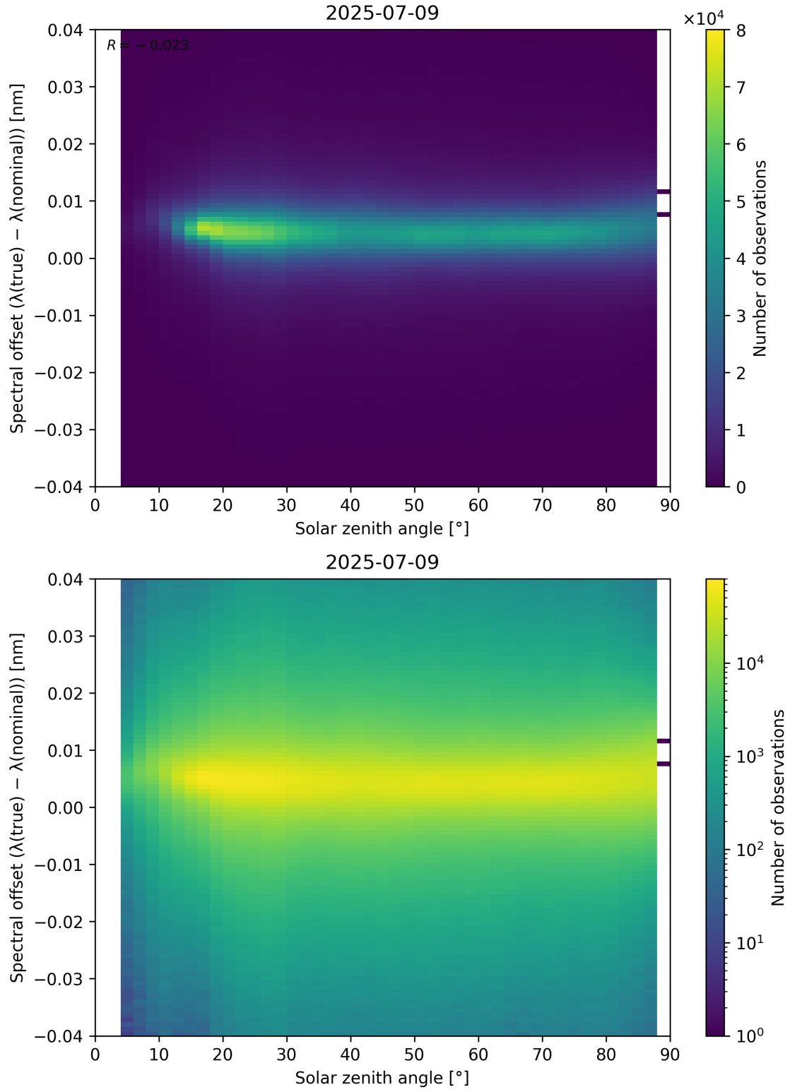
Figure 117: Scatter density plot of “Solar zenith angle” against “Spectral offset ( \lambda_{\text{true}} - \lambda_{\text{nominal}} )” for 2025-07-08 to 2025-07-10.
