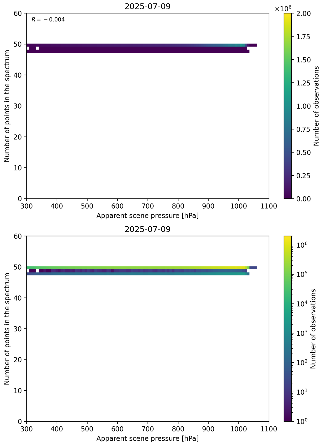
Figure 66: Scatter density plot of “Apparent scene pressure” against “Number of points in the spectrum” for 2025-07-08 to 2025-07-10.
