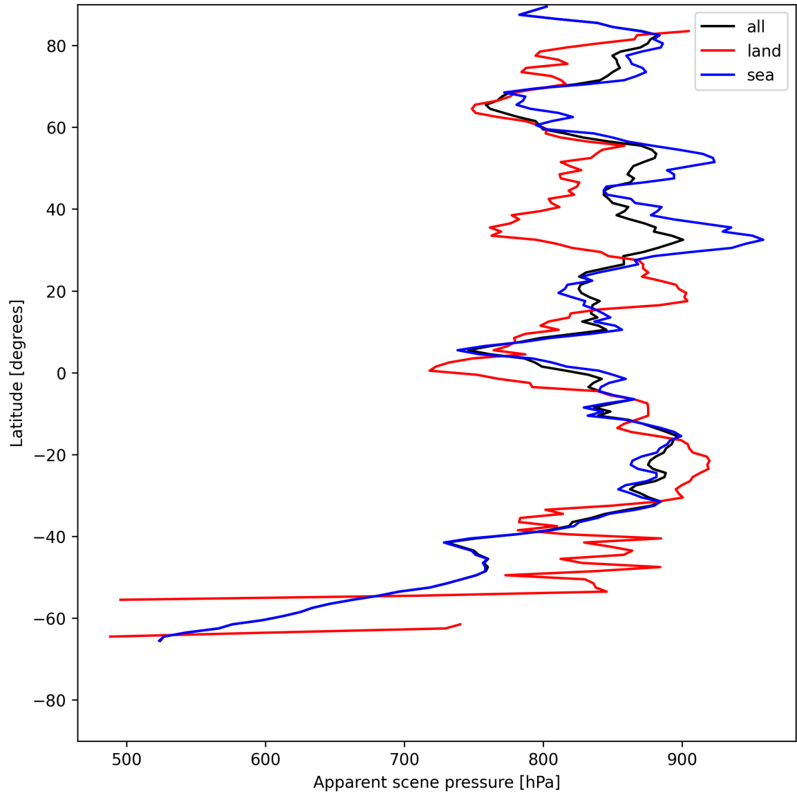
Figure 19: Zonal average of “Apparent scene pressure” for 2025-07-08 to 2025-07-10.
