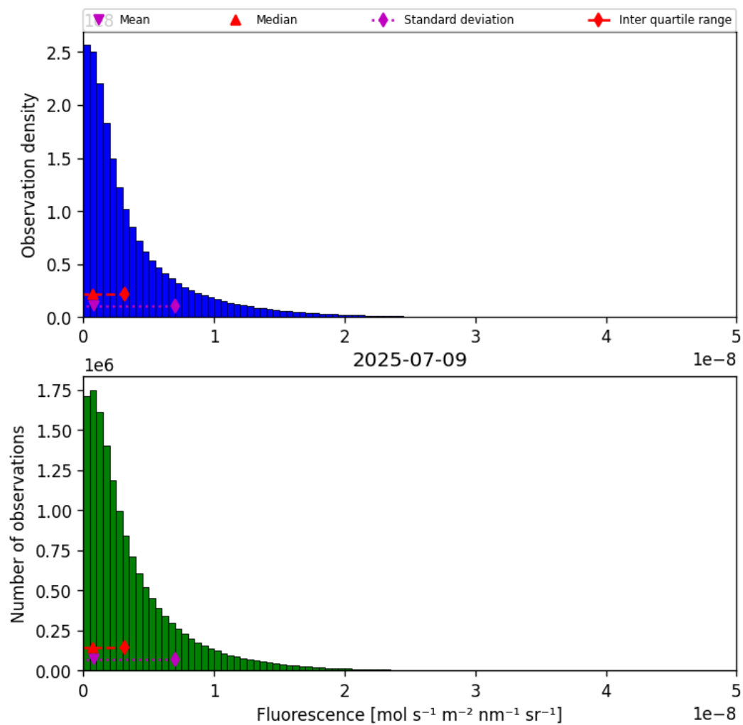
Figure 40: Histogram of “Fluorescence” for 2025-07-08 to 2025-07-10
