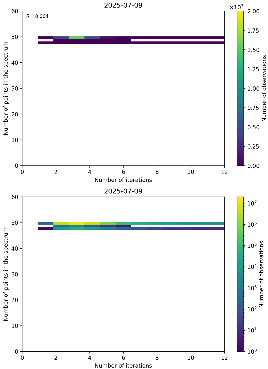
Figure 99: Scatter density plot of “Number of iterations” against “Number of points in the spectrum” for 2025-07-08 to 2025-07-10.
