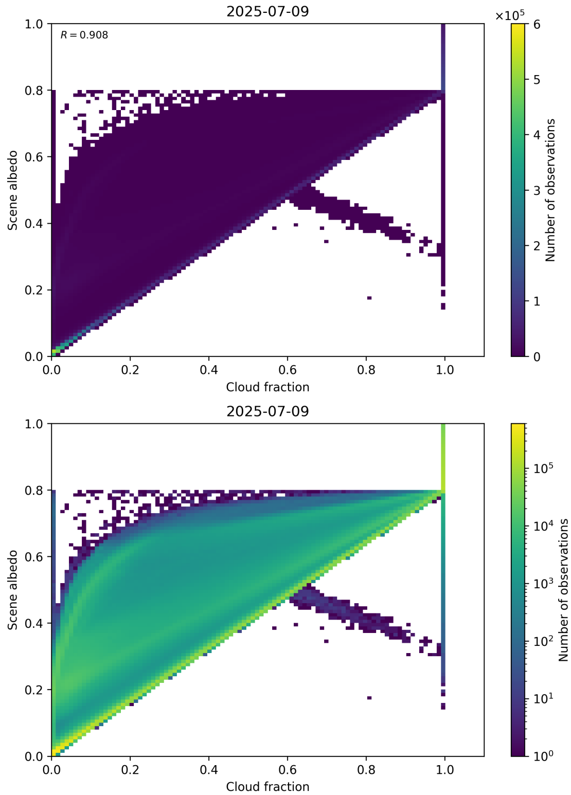
Figure 75: Scatter density plot of “Cloud fraction” against “Scene albedo” for 2025-07-08 to 2025-07-10.
