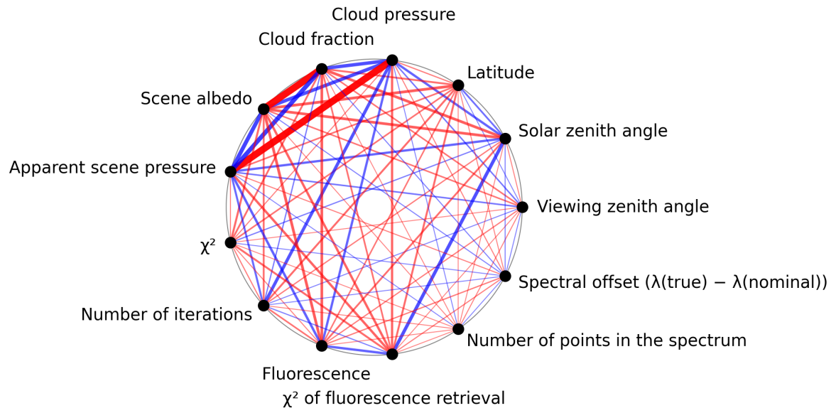
Figure 1: Map of correlation graph for 2025-07-08 to 2025-07-10.
