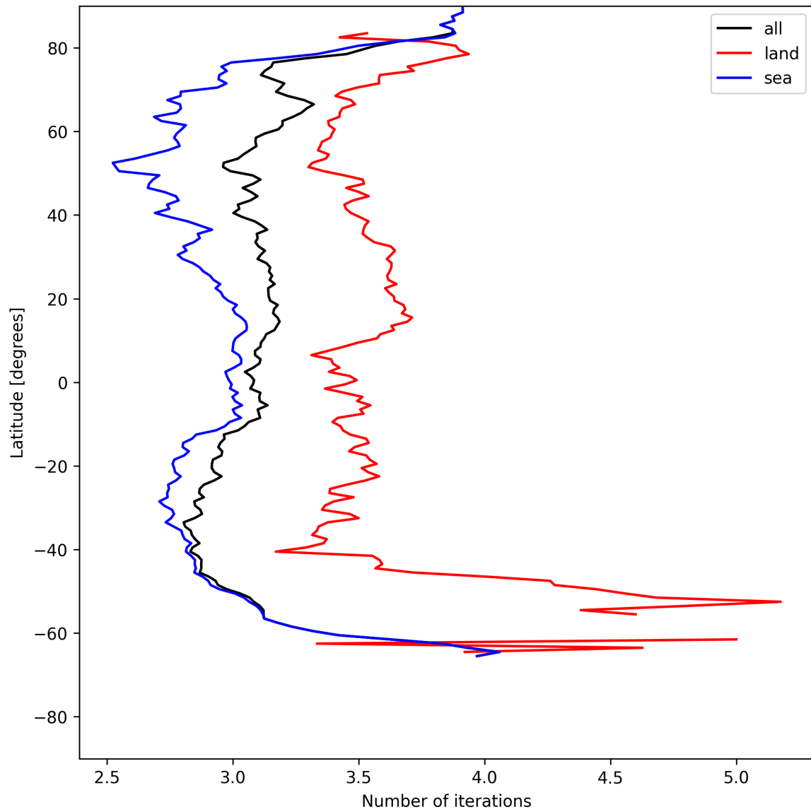
Figure 22: Zonal average of “Number of iterations” for 2025-07-08 to 2025-07-10.
