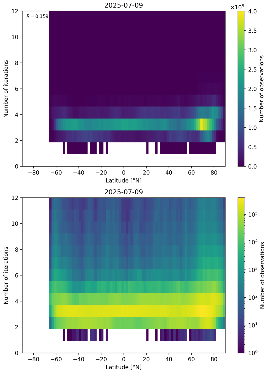
Figure 93: Scatter density plot of “Latitude” against “Number of iterations” for 2025-07-08 to 2025-07-10.
