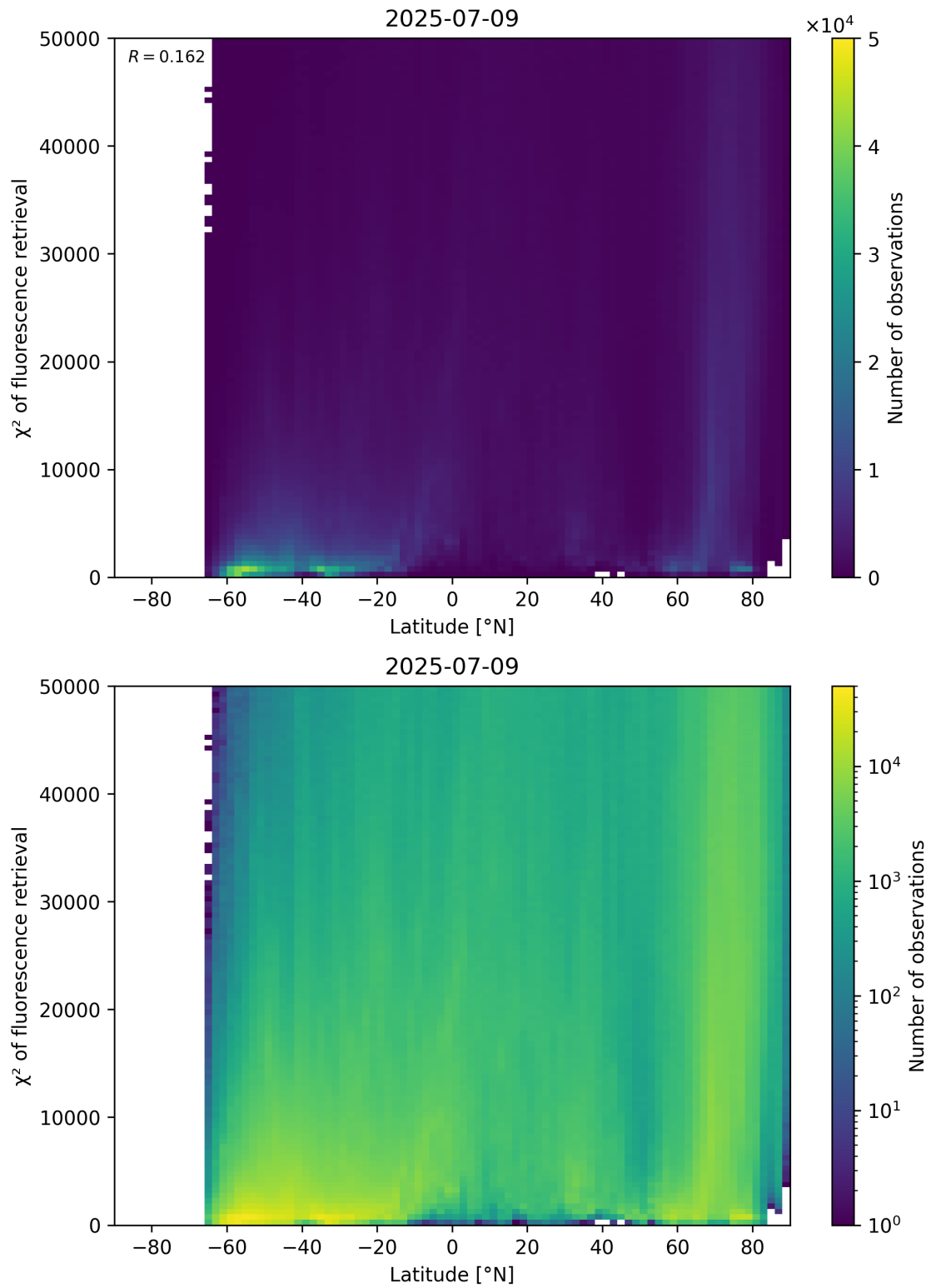
Figure 89: Scatter density plot of “Latitude” against “ \chi^2 of fluorescence retrieval” for 2025-07-08 to 2025-07-10.
