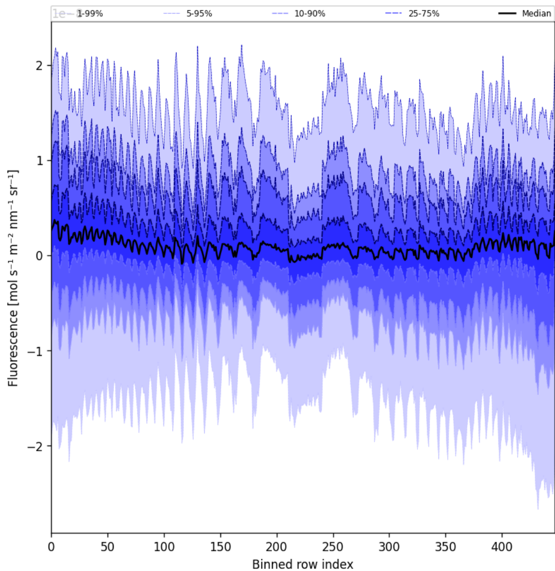
Figure 57: Along track statistics of “Fluorescence” for 2025-07-08 to 2025-07-10
