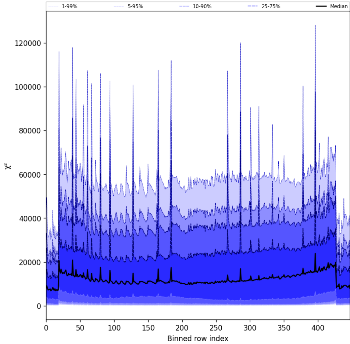
Figure 55: Along track statistics of “ \chi^2 ” for 2025-07-08 to 2025-07-10
