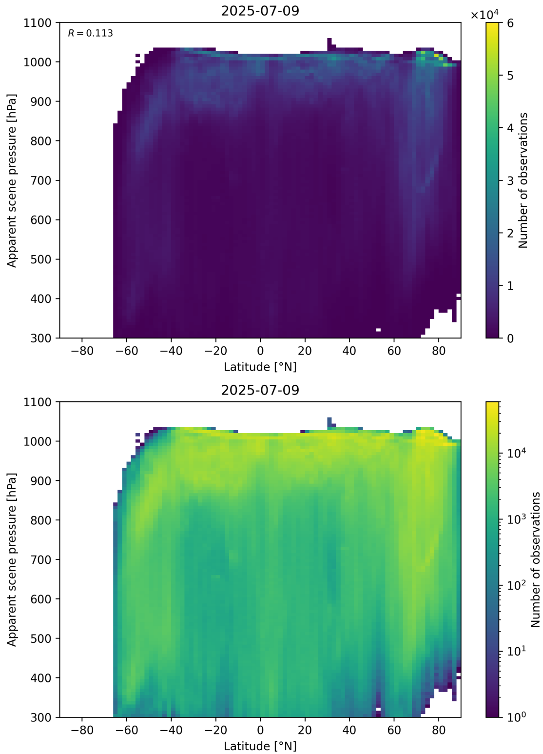
Figure 88: Scatter density plot of “Latitude” against “Apparent scene pressure” for 2025-07-08 to 2025-07-10.
