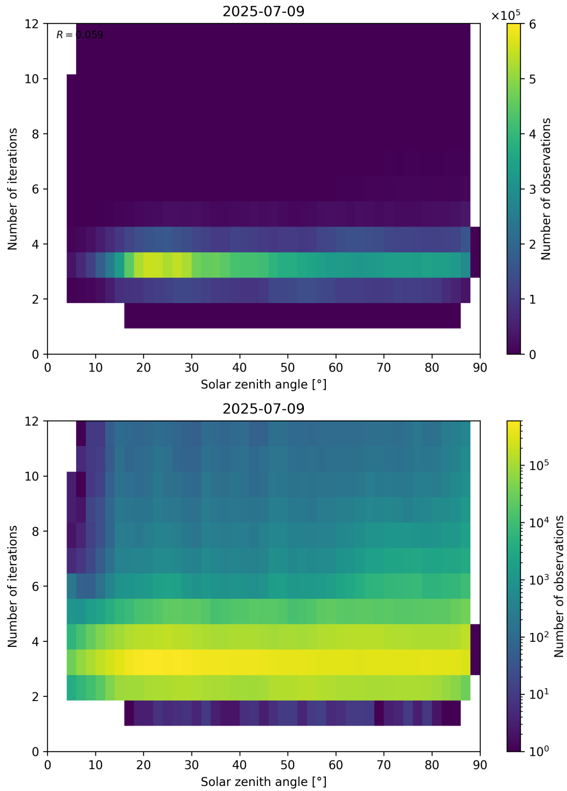
Figure 114: Scatter density plot of “Solar zenith angle” against “Number of iterations” for 2025-07-08 to 2025-07-10.
