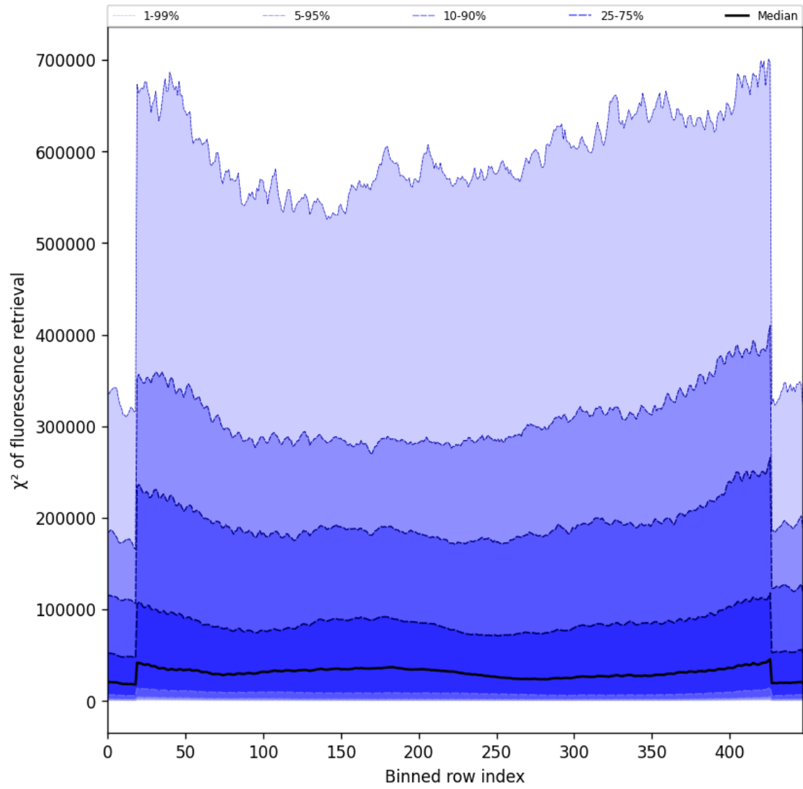
Figure 59: Along track statistics of “ \chi^2 of fluorescence retrieval” for 2025-07-08 to 2025-07-10
