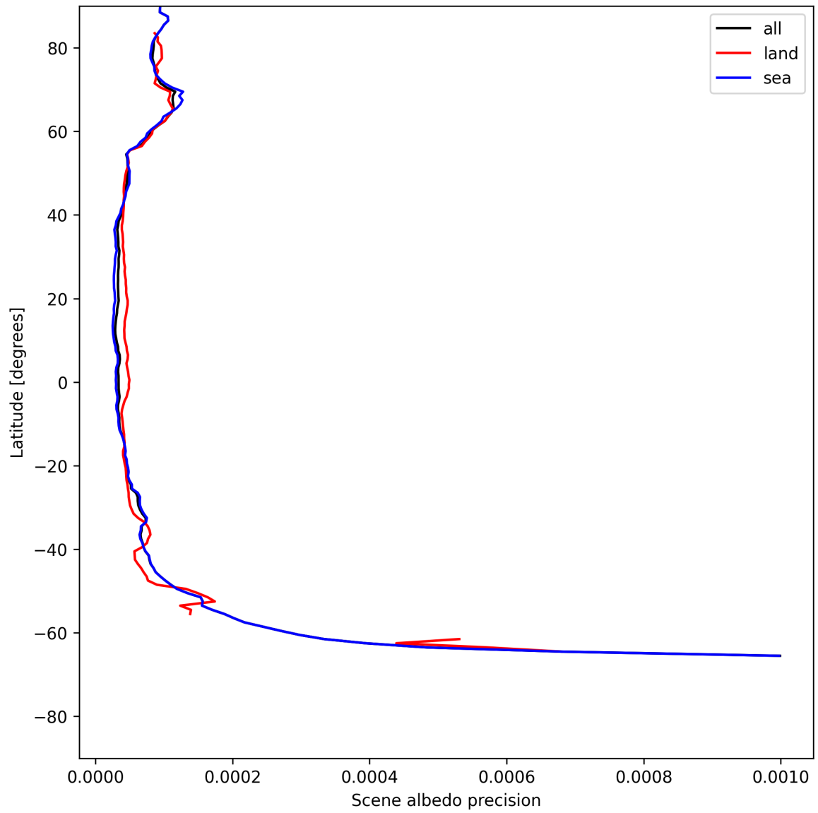
Figure 18: Zonal average of “Scene albedo precision” for 2025-07-08 to 2025-07-10.
