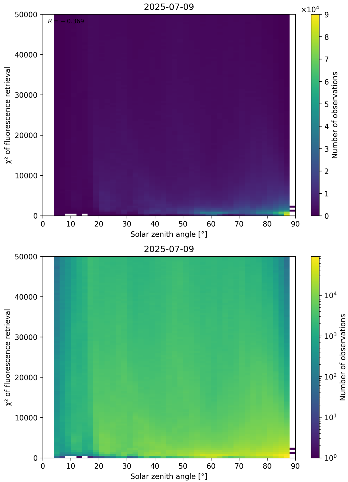
Figure 109: Scatter density plot of “Solar zenith angle” against “ \chi^2 of fluorescence retrieval” for 2025-07-08 to 2025-07-10.
