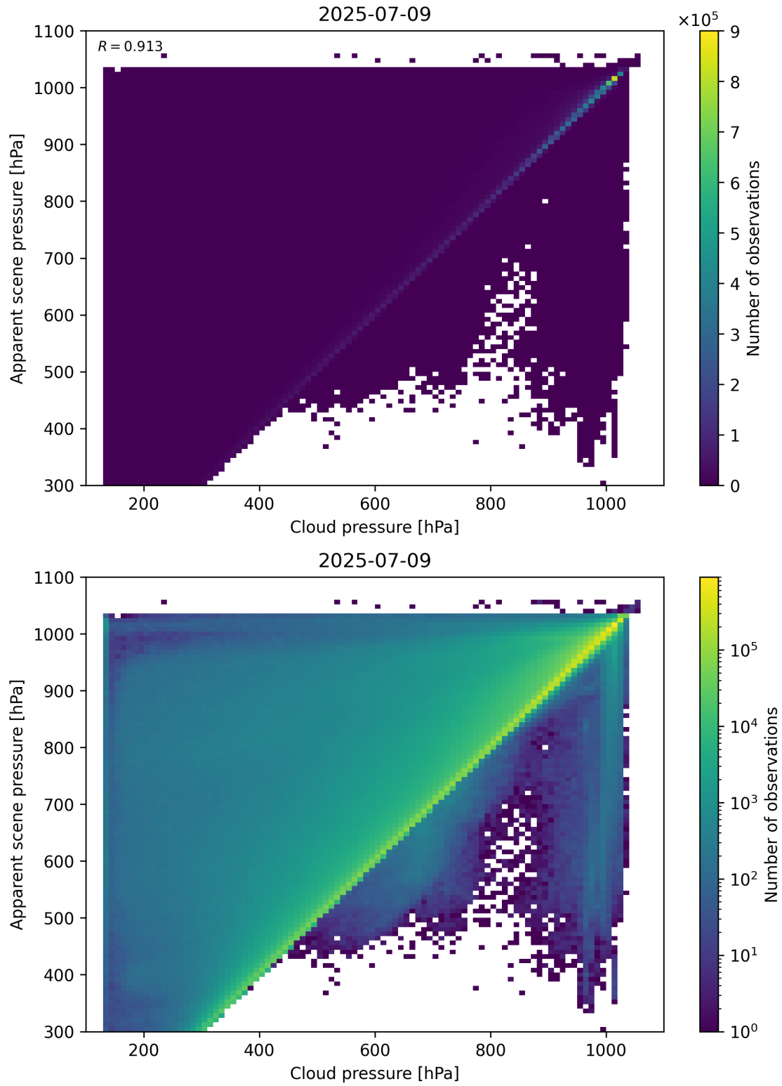
Figure 77: Scatter density plot of “Cloud pressure” against “Apparent scene pressure” for 2025-07-08 to 2025-07-10.
