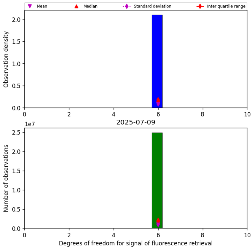
Figure 43: Histogram of “Degrees of freedom for signal of fluorescence retrieval” for 2025-07-08 to 2025-07-10
