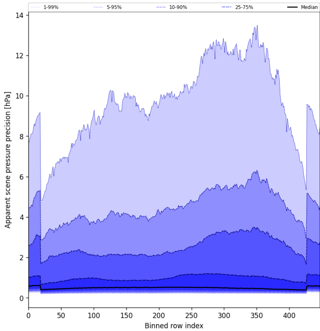
Figure 54: Along track statistics of “Apparent scene pressure precision” for 2025-07-08 to 2025-07-10
