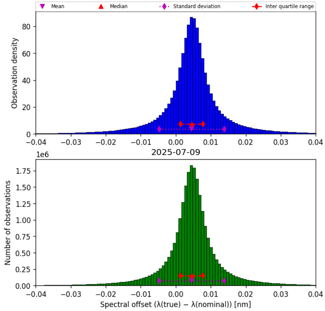
Figure 45: Histogram of “Spectral offset ( \lambda_{\text{true}} - \lambda_{\text{nominal}} )” for 2025-07-08 to 2025-07-10
