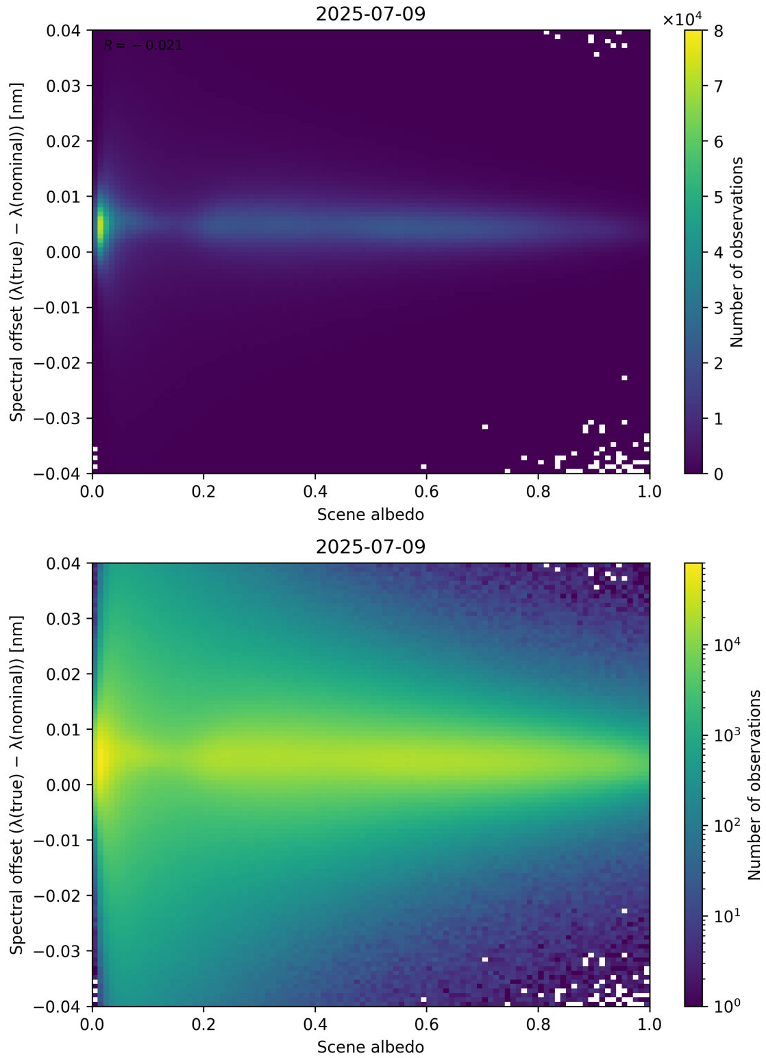
Figure 107: Scatter density plot of “Scene albedo” against “Spectral offset ( \lambda_{\text{true}} - \lambda_{\text{nominal}} )” for 2025-07-08 to 2025-07-10.
