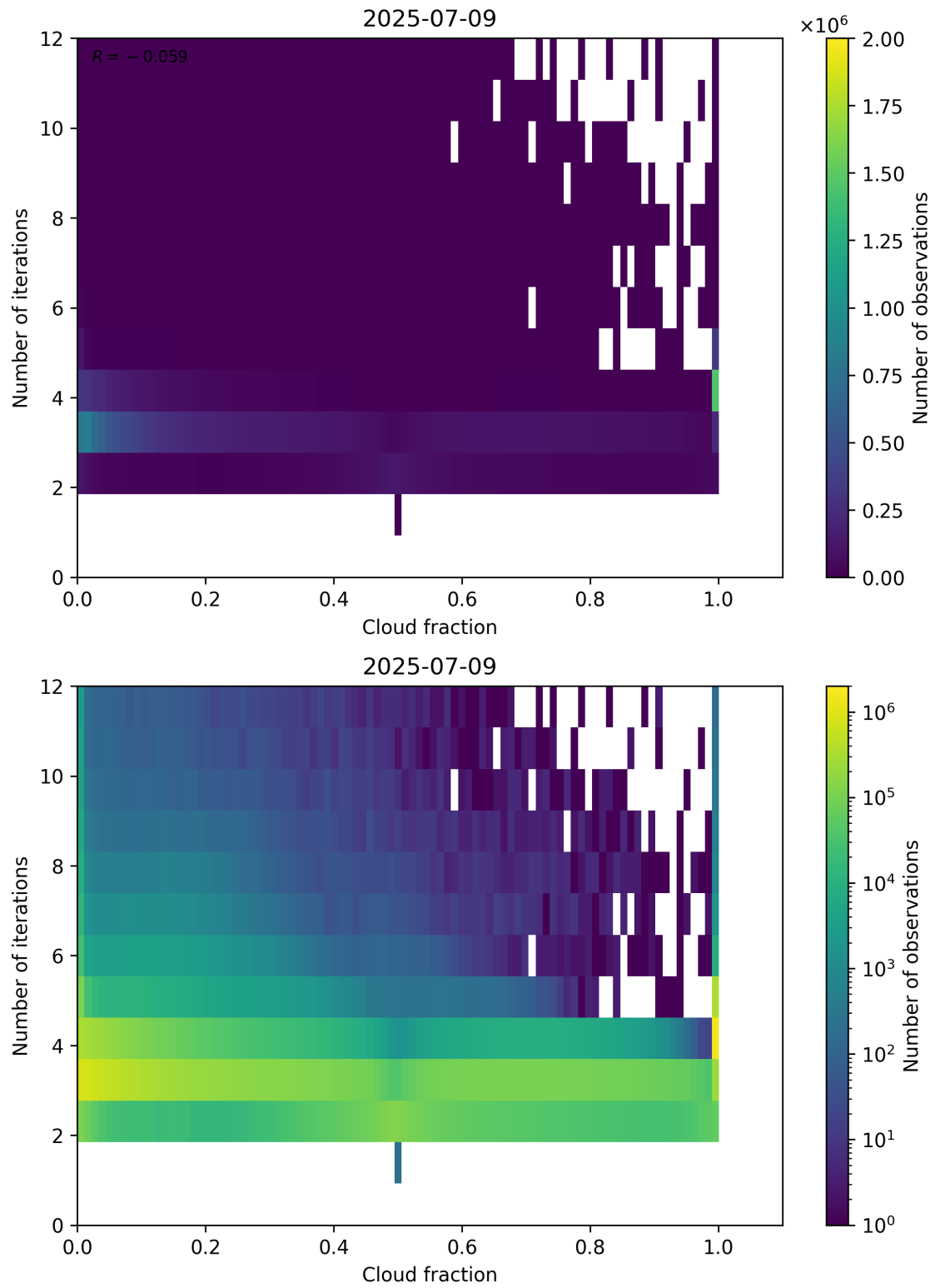
Figure 73: Scatter density plot of “Cloud fraction” against “Number of iterations” for 2025-07-08 to 2025-07-10.
