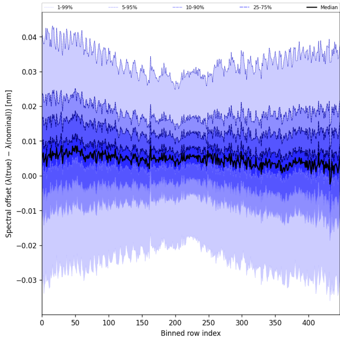
Figure 62: Along track statistics of “Spectral offset ( \lambda_{\text{true}} - \lambda_{\text{nominal}} )” for 2025-07-08 to 2025-07-10
