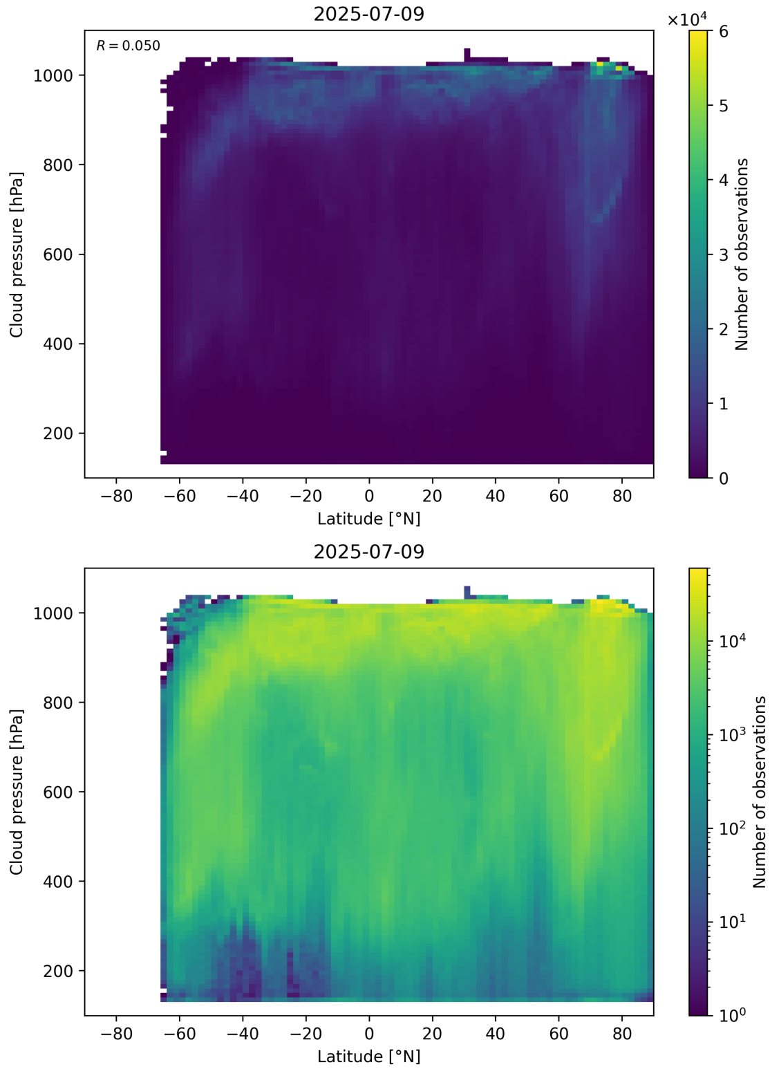
Figure 91: Scatter density plot of “Latitude” against “Cloud pressure” for 2025-07-08 to 2025-07-10.
