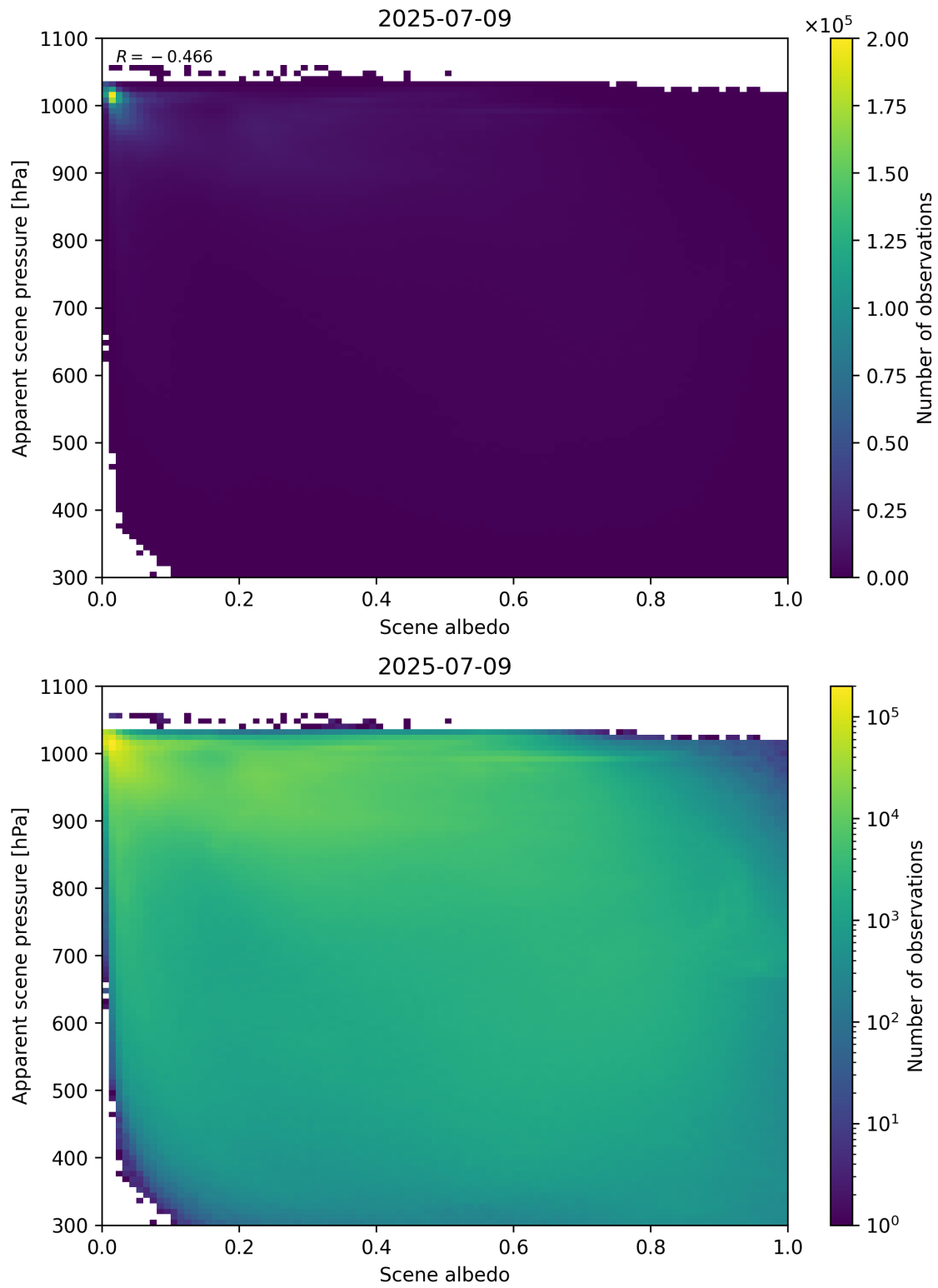
Figure 102: Scatter density plot of “Scene albedo” against “Apparent scene pressure” for 2025-07-08 to 2025-07-10.
