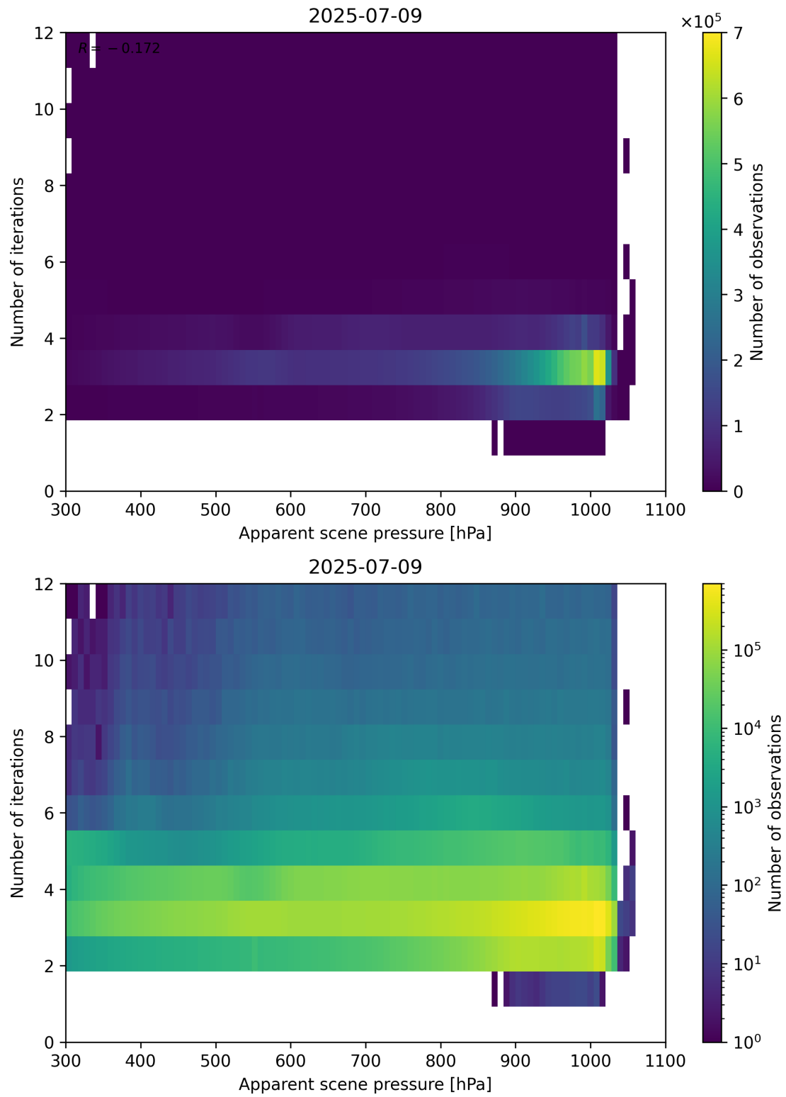
Figure 65: Scatter density plot of “Apparent scene pressure” against “Number of iterations” for 2025-07-08 to 2025-07-10.
