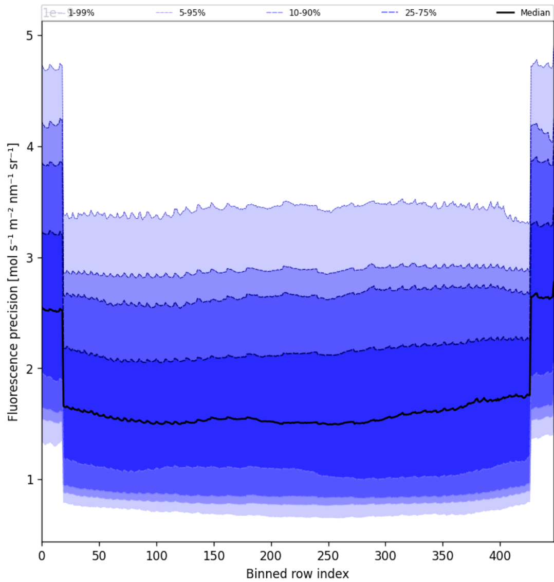
Figure 58: Along track statistics of “Fluorescence precision” for 2025-07-08 to 2025-07-10
