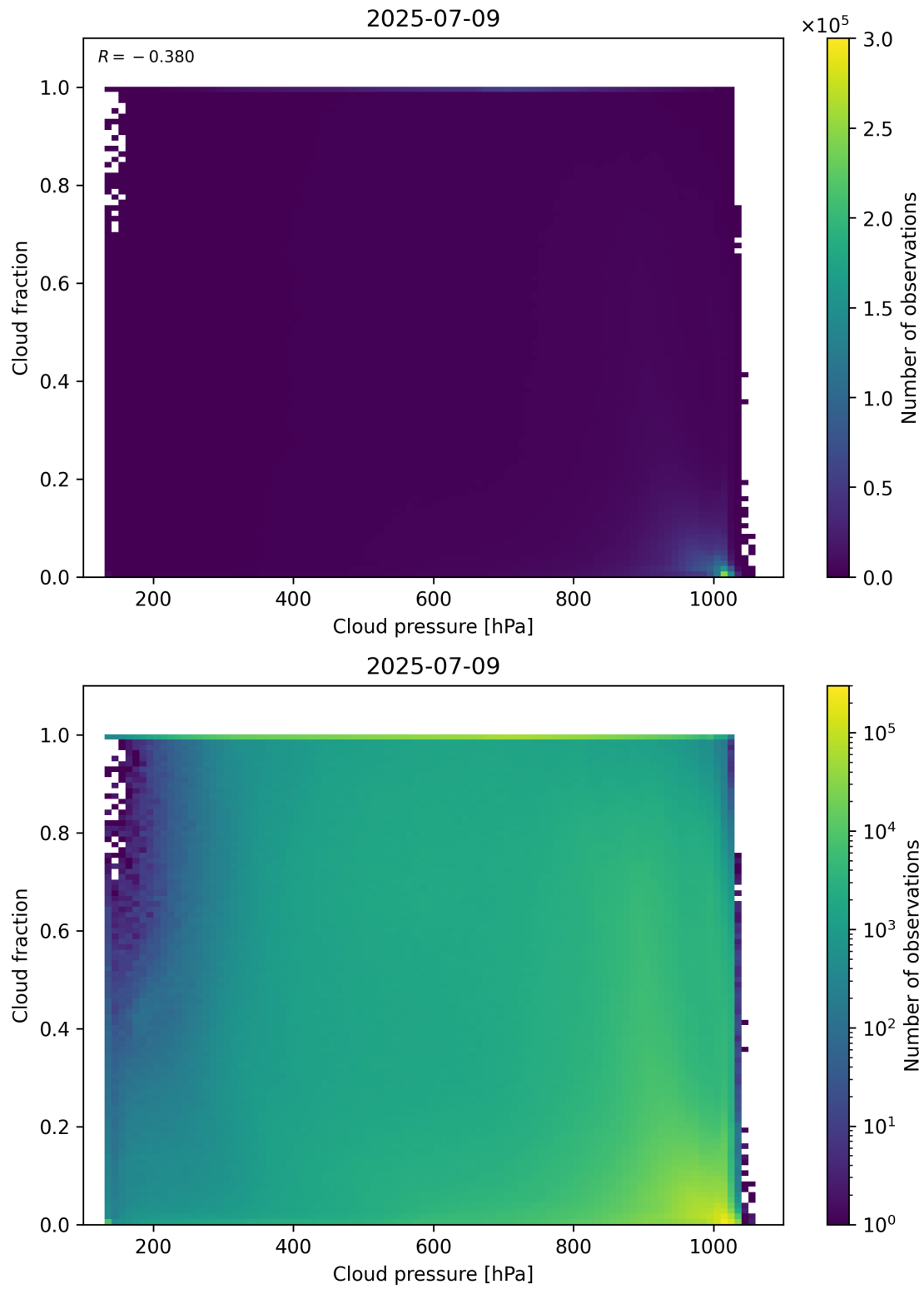
Figure 79: Scatter density plot of “Cloud pressure” against “Cloud fraction” for 2025-07-08 to 2025-07-10.
