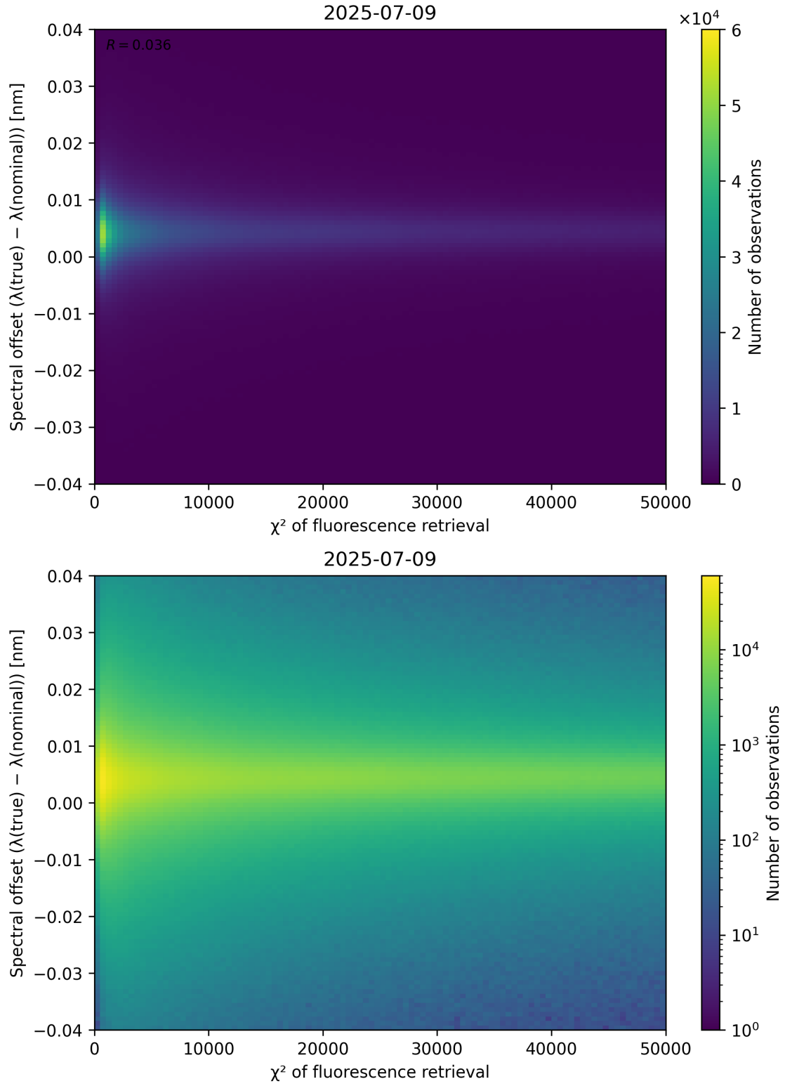
Figure 69: Scatter density plot of “ \chi^2 of fluorescence retrieval” against “Spectral offset ( \lambda_{\text{true}} - \lambda_{\text{nominal}} )” for 2025-07-08 to 2025-07-10.
