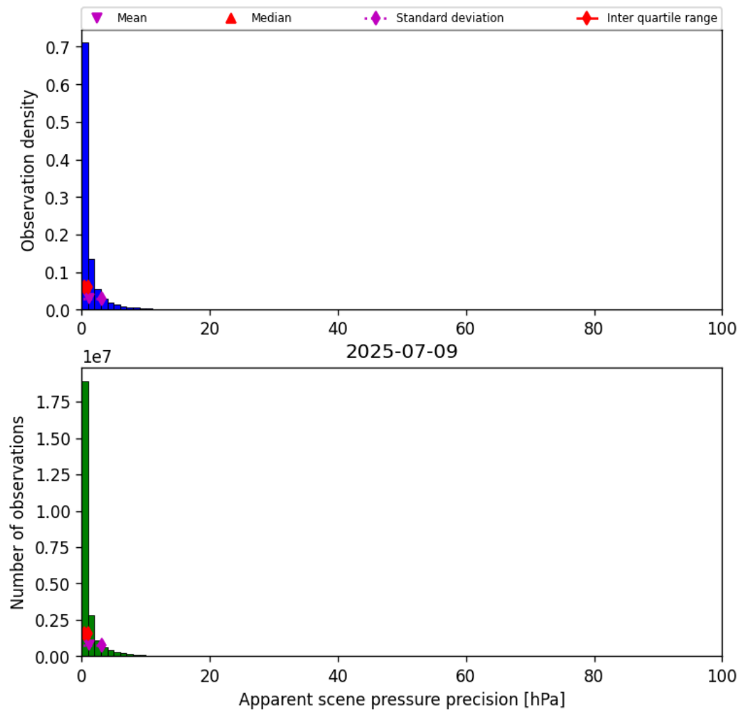
Figure 37: Histogram of “Apparent scene pressure precision” for 2025-07-08 to 2025-07-10
