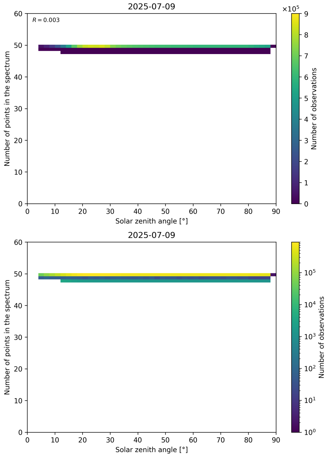
Figure 115: Scatter density plot of “Solar zenith angle” against “Number of points in the spectrum” for 2025-07-08 to 2025-07-10.
