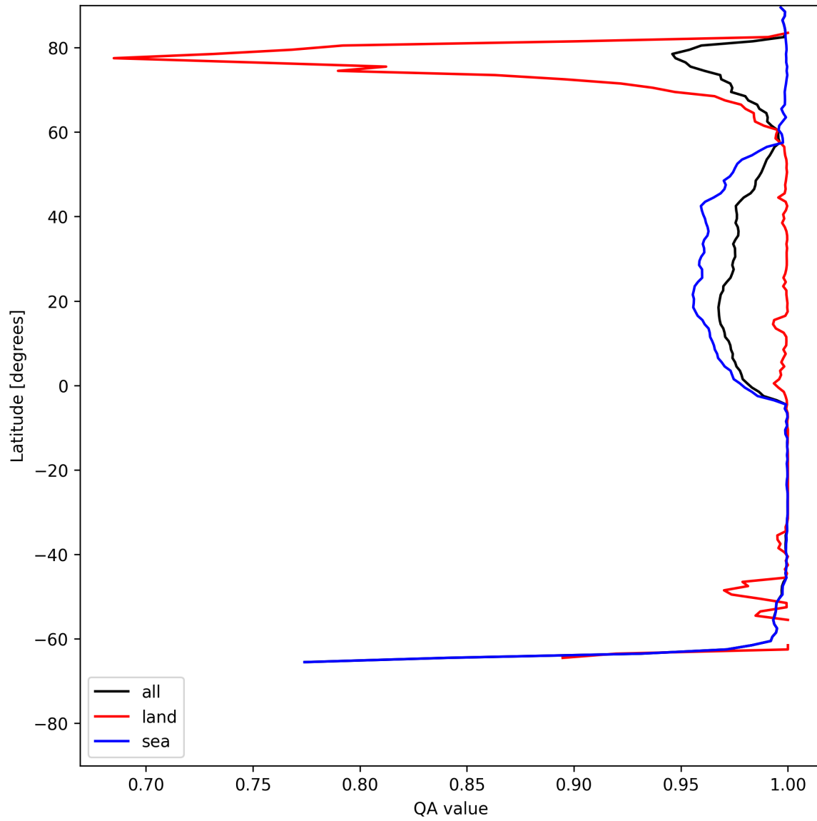
Figure 12: Zonal average of “QA value” for 2025-07-08 to 2025-07-10.
