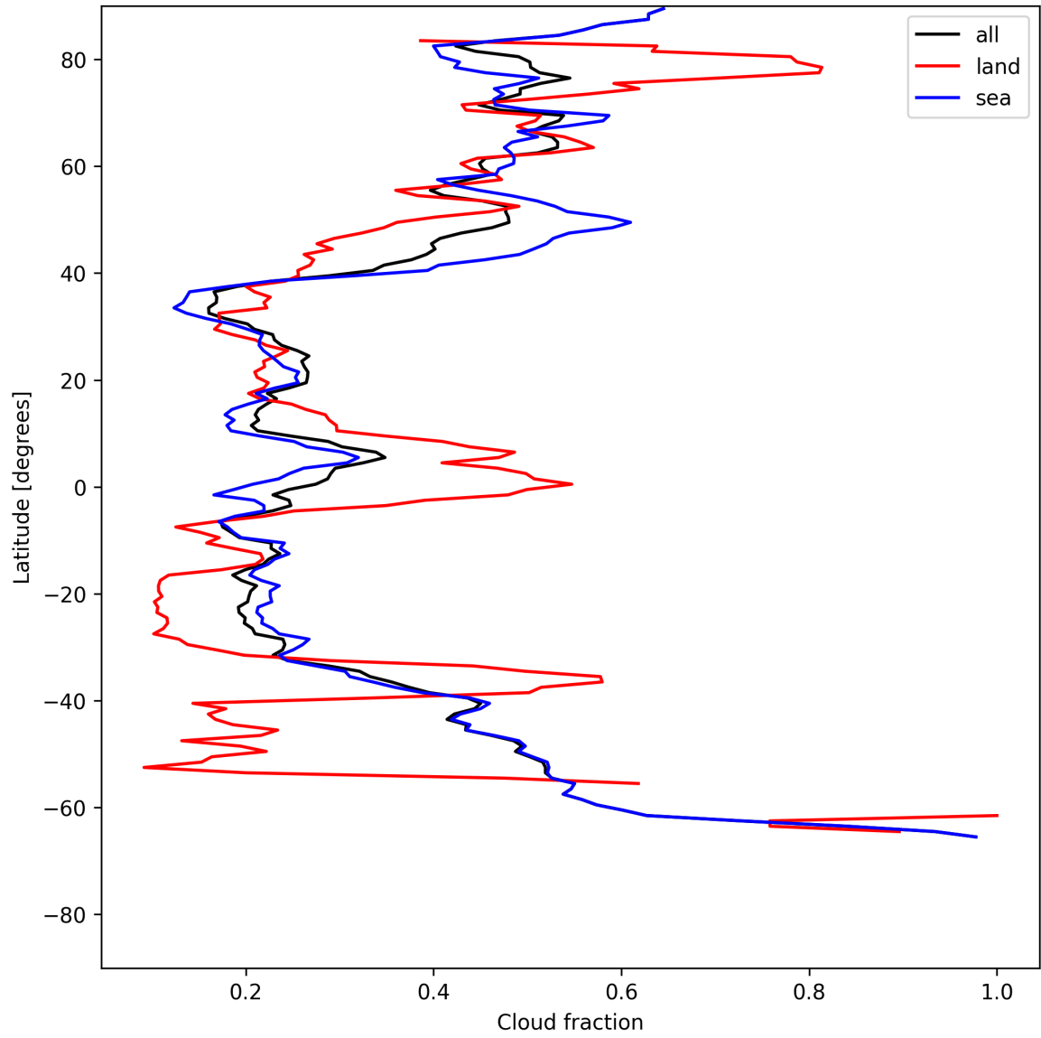
Figure 15: Zonal average of “Cloud fraction” for 2025-07-08 to 2025-07-10.
