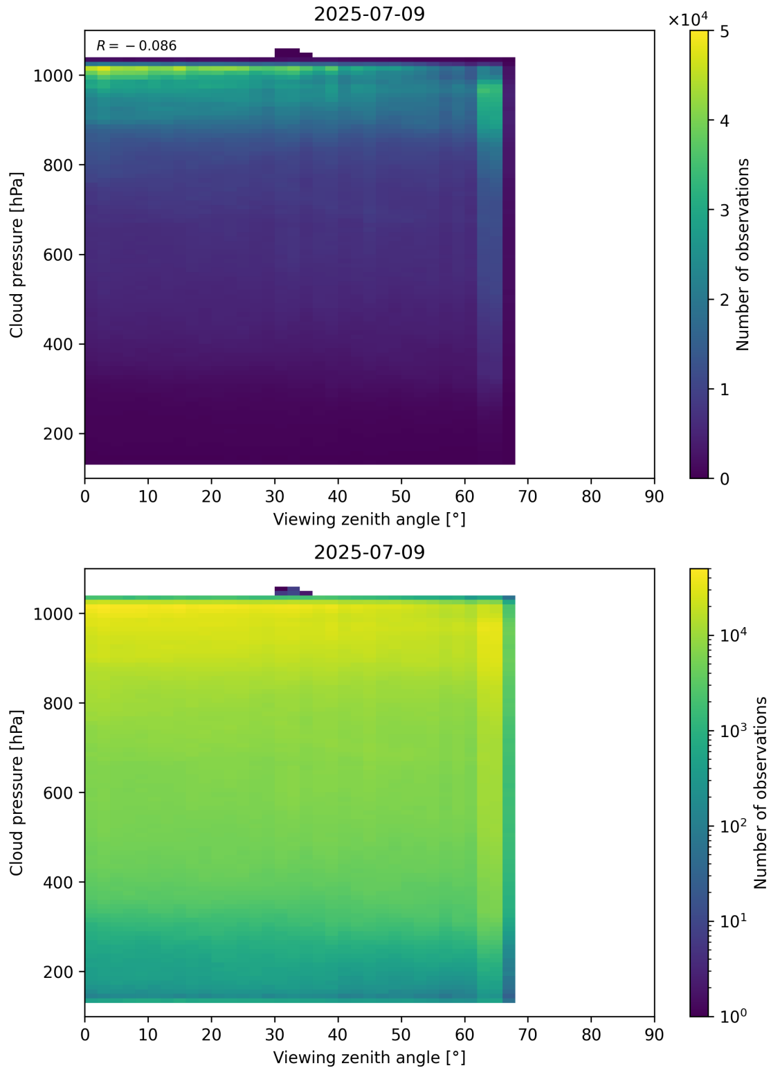
Figure 121: Scatter density plot of “Viewing zenith angle” against “Cloud pressure” for 2025-07-08 to 2025-07-10.
