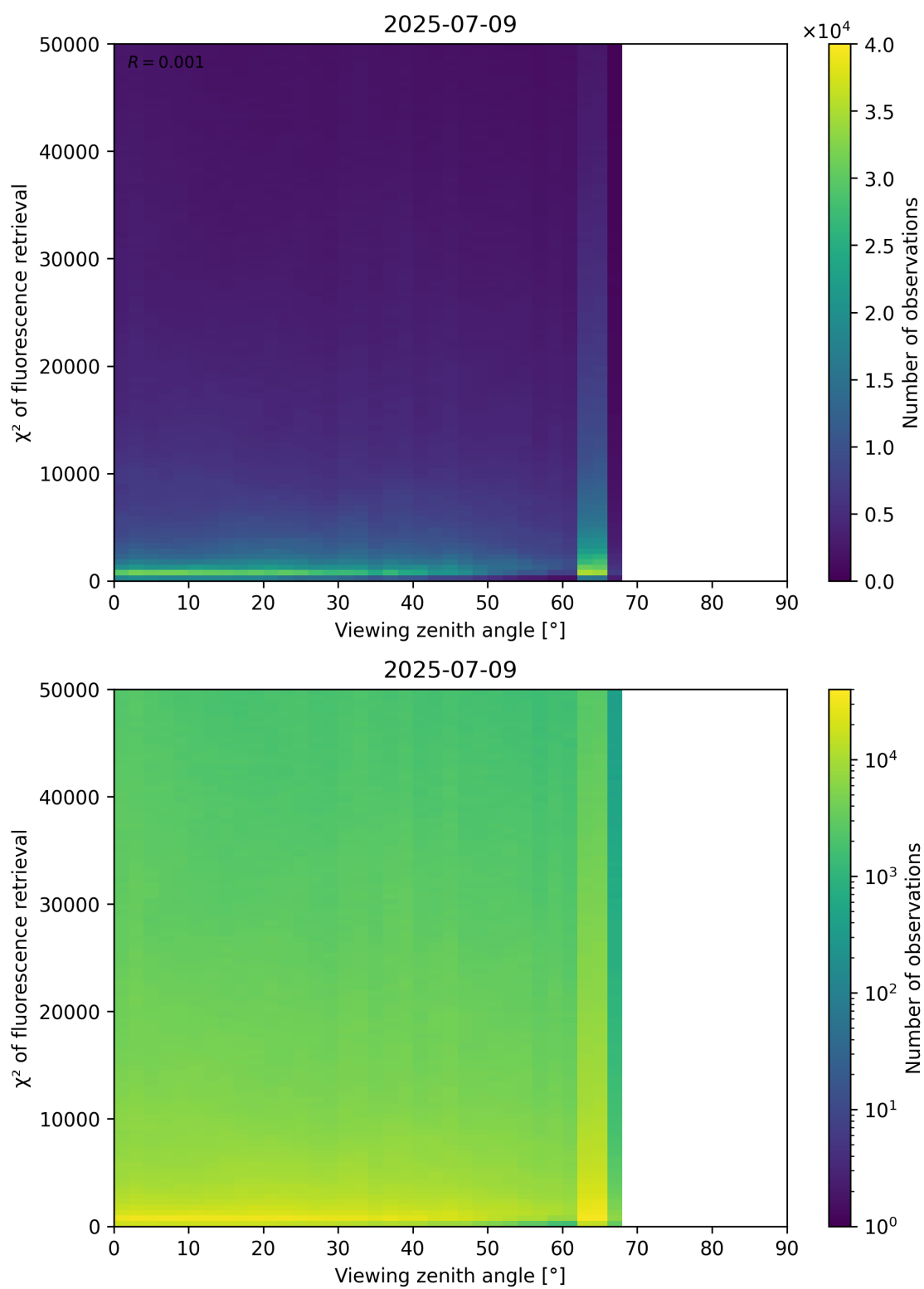
Figure 119: Scatter density plot of “Viewing zenith angle” against “ \chi^2 of fluorescence retrieval” for 2025-07-08 to 2025-07-10.
