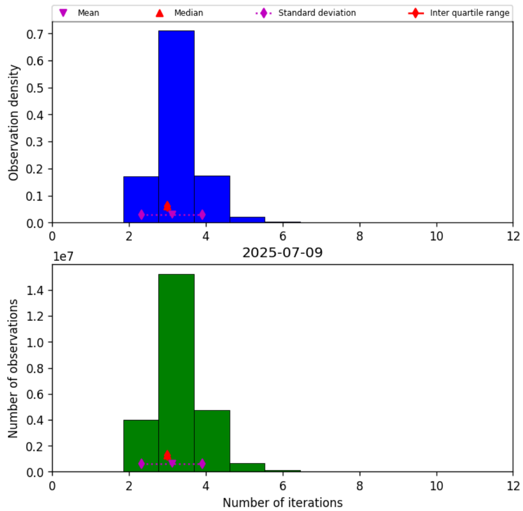
Figure 39: Histogram of “Number of iterations” for 2025-07-08 to 2025-07-10
