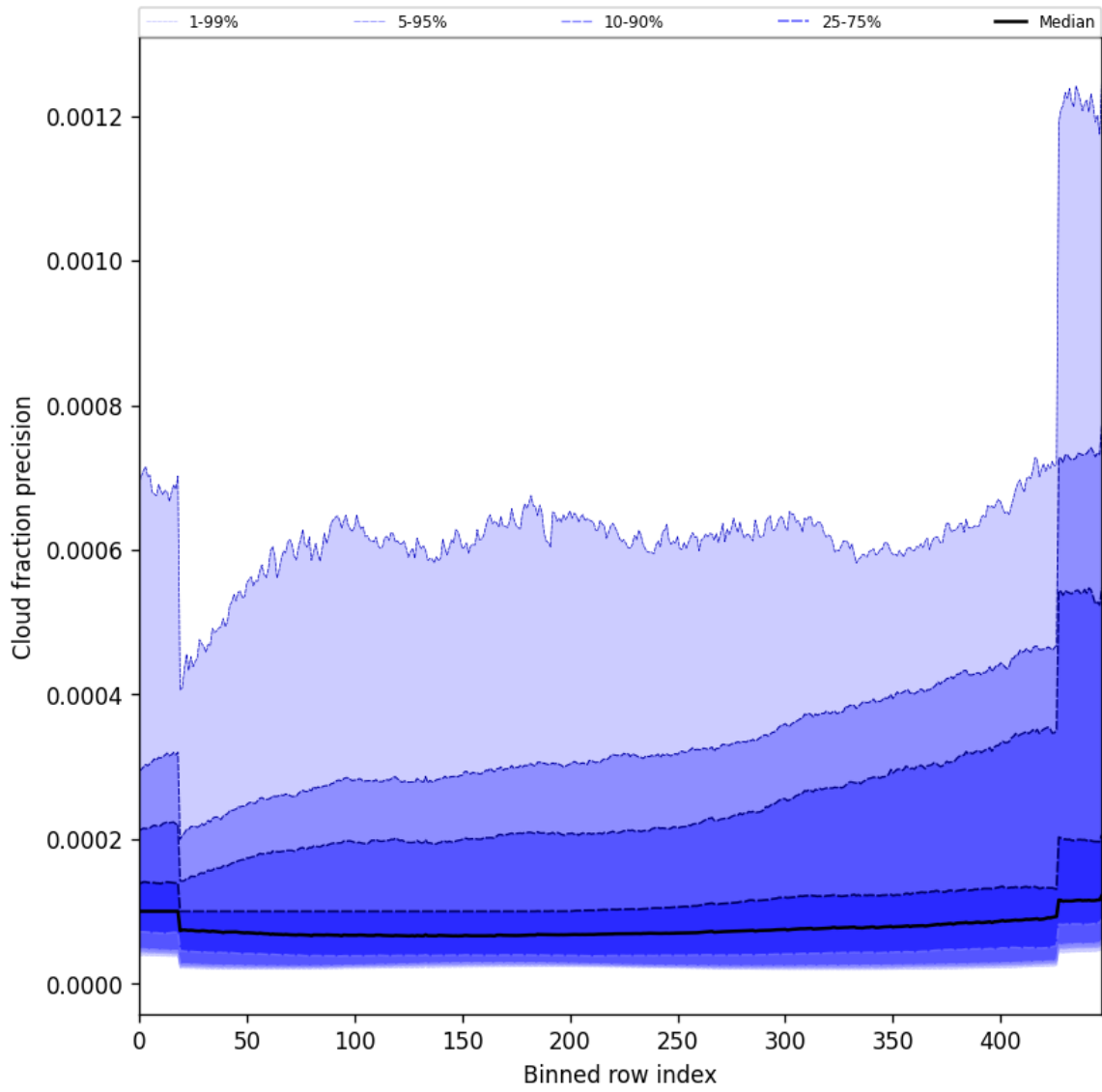
Figure 50: Along track statistics of “Cloud fraction precision” for 2025-07-08 to 2025-07-10
