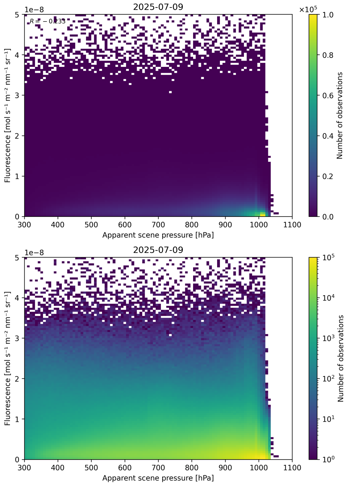
Figure 64: Scatter density plot of “Apparent scene pressure” against “Fluorescence” for 2025-07-08 to 2025-07-10.
