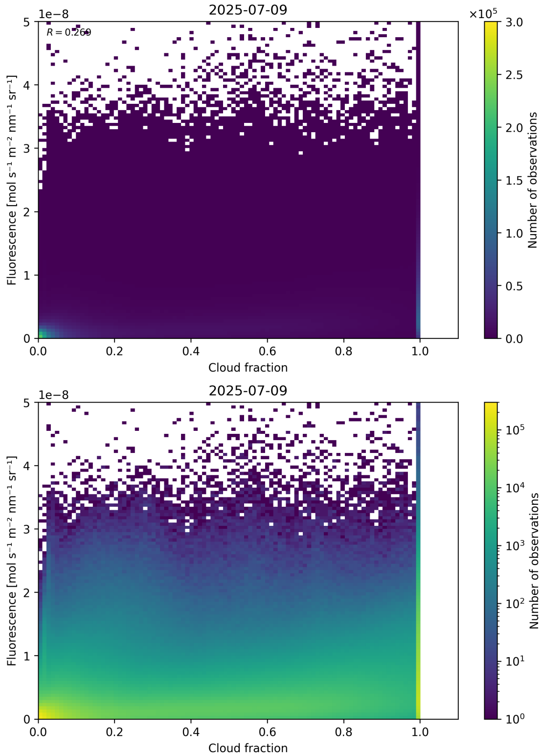
Figure 72: Scatter density plot of “Cloud fraction” against “Fluorescence” for 2025-07-08 to 2025-07-10.
