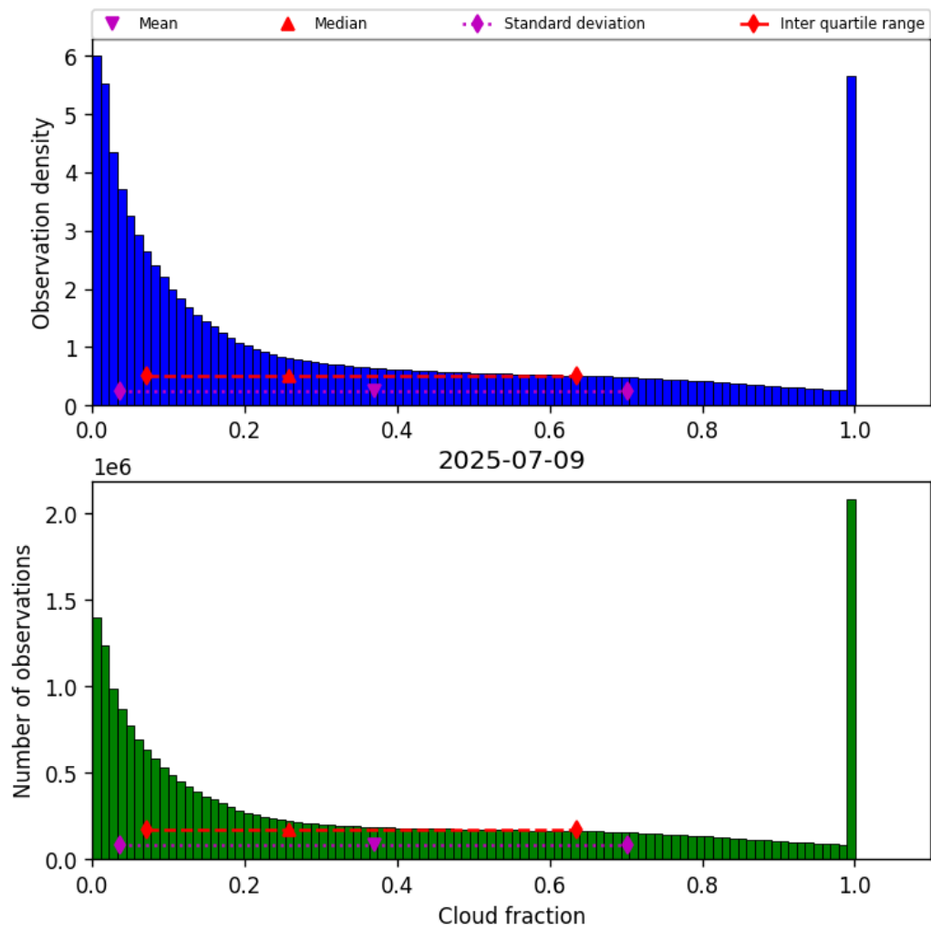
Figure 32: Histogram of “Cloud fraction” for 2025-07-08 to 2025-07-10
