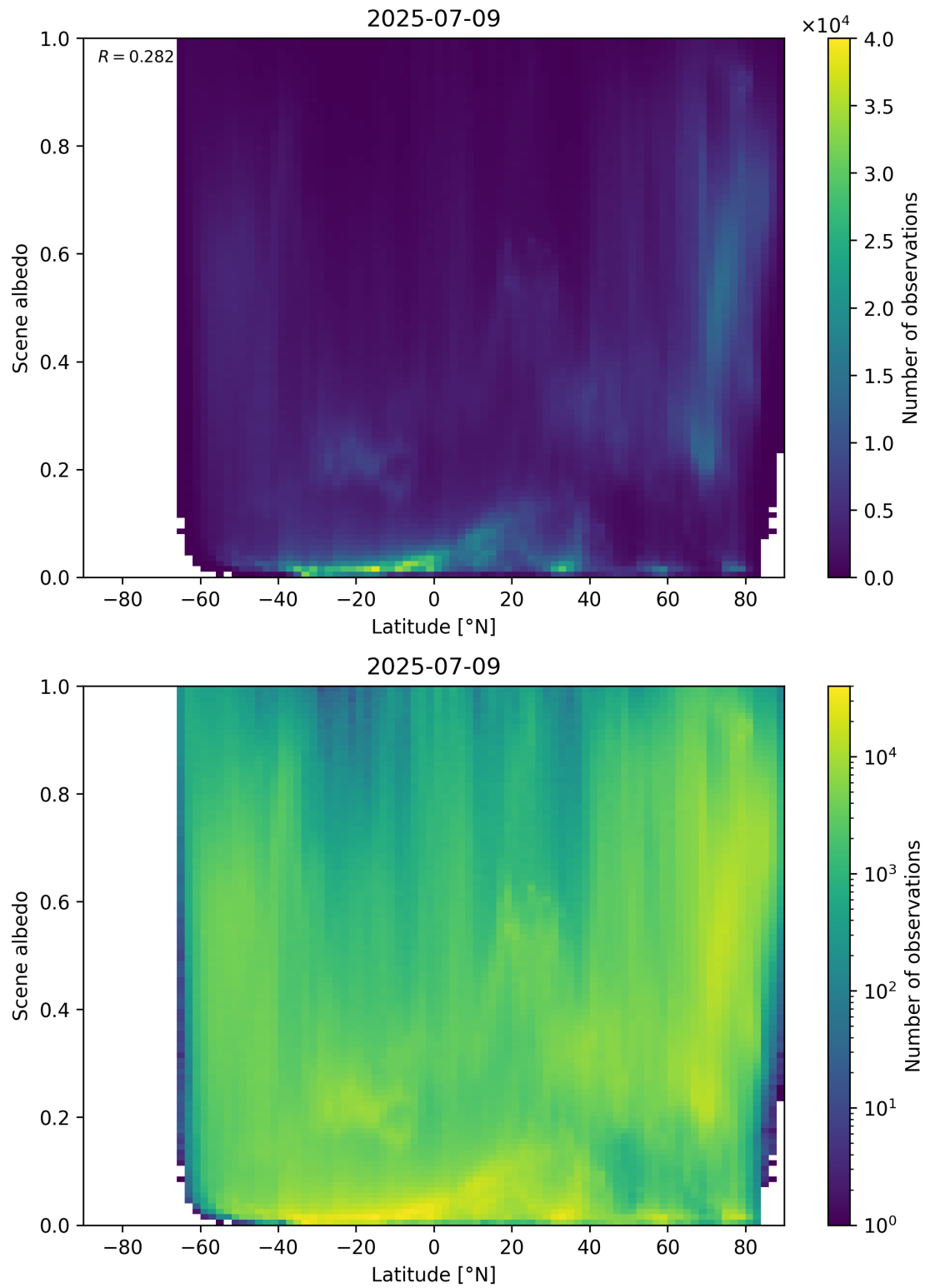
Figure 95: Scatter density plot of “Latitude” against “Scene albedo” for 2025-07-08 to 2025-07-10.
