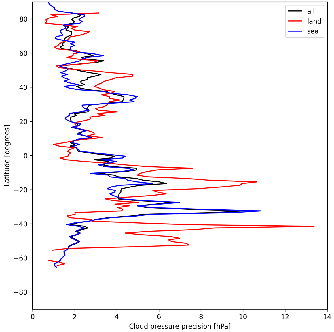
Figure 14: Zonal average of “Cloud pressure precision” for 2025-07-08 to 2025-07-10.
