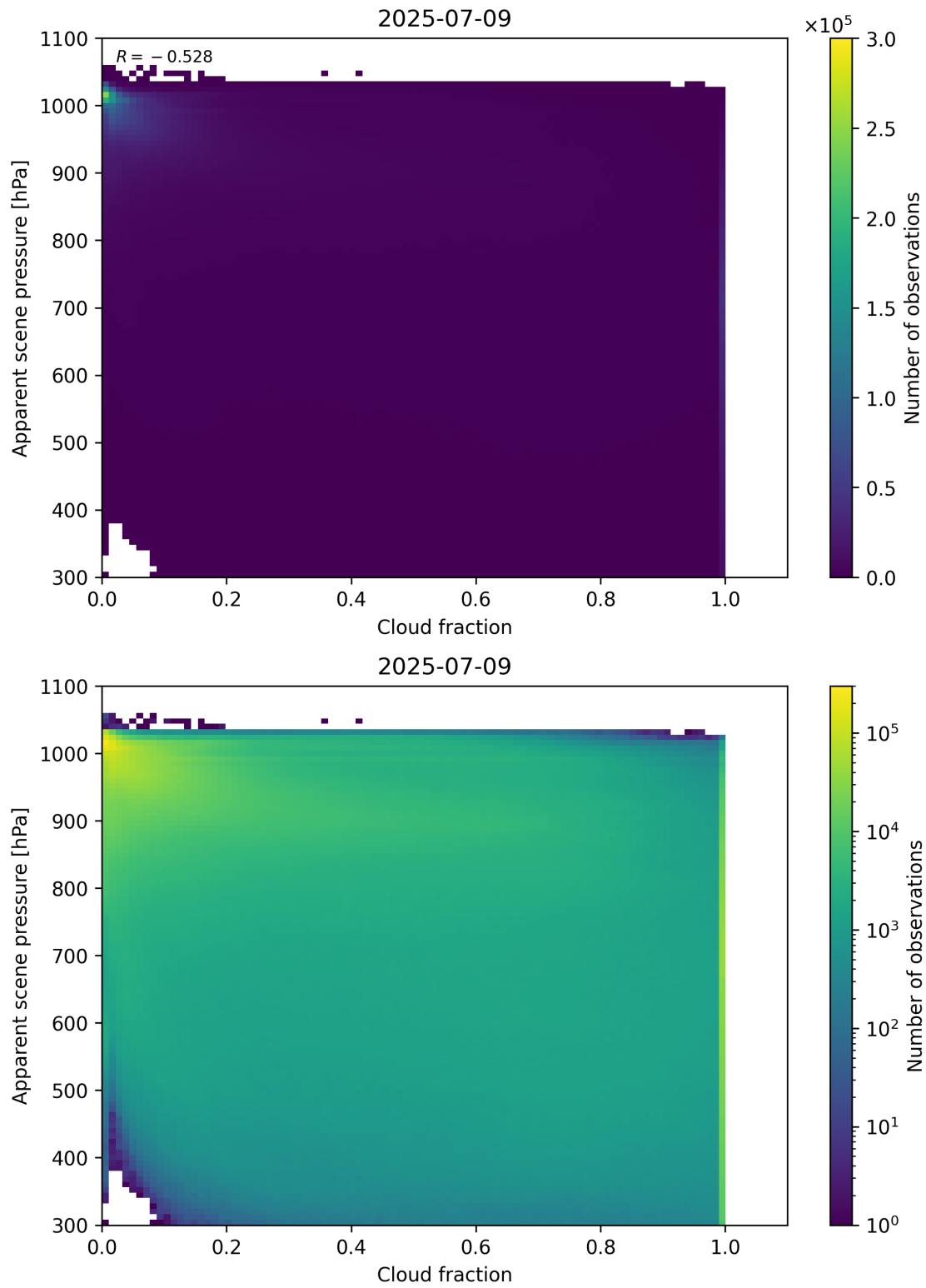
Figure 70: Scatter density plot of “Cloud fraction” against “Apparent scene pressure” for 2025-07-08 to 2025-07-10.
