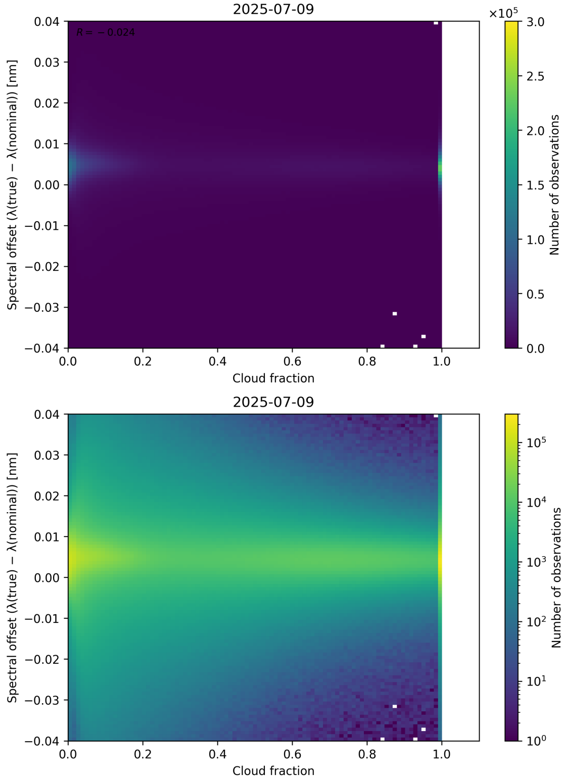
Figure 76: Scatter density plot of “Cloud fraction” against “Spectral offset ( \lambda_{\text{true}} - \lambda_{\text{nominal}} )” for 2025-07-08 to 2025-07-10.
