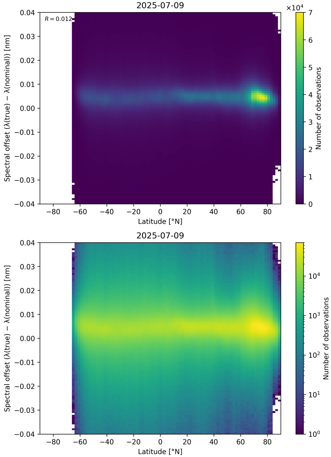
Figure 96: Scatter density plot of “Latitude” against “Spectral offset ( \lambda_{\text{true}} - \lambda_{\text{nominal}} )” for 2025-07-08 to 2025-07-10.
