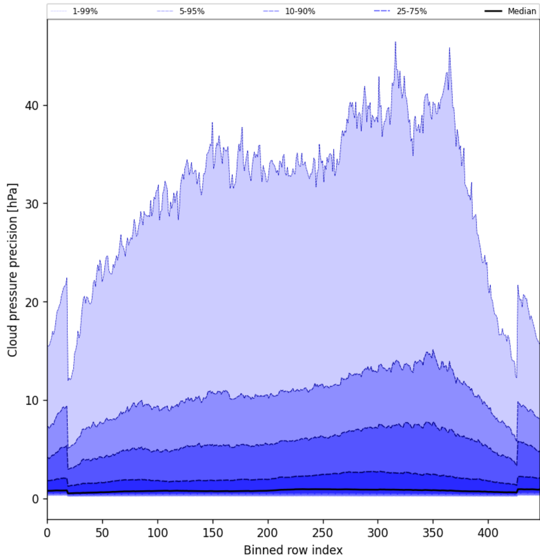
Figure 48: Along track statistics of “Cloud pressure precision” for 2025-07-08 to 2025-07-10
