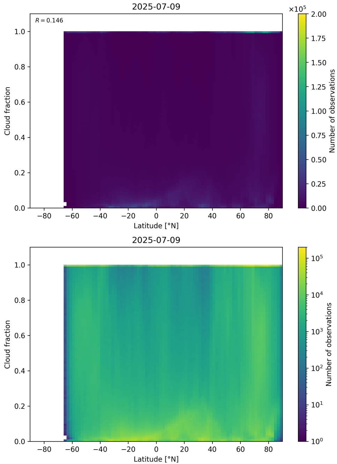
Figure 90: Scatter density plot of “Latitude” against “Cloud fraction” for 2025-07-08 to 2025-07-10.
