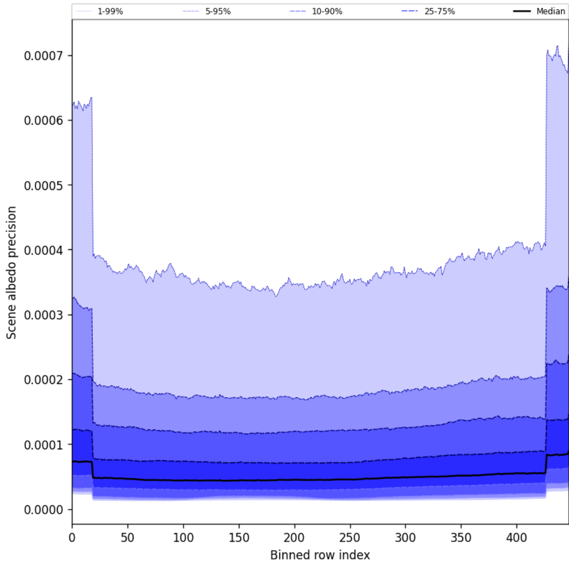
Figure 52: Along track statistics of “Scene albedo precision” for 2025-07-08 to 2025-07-10
