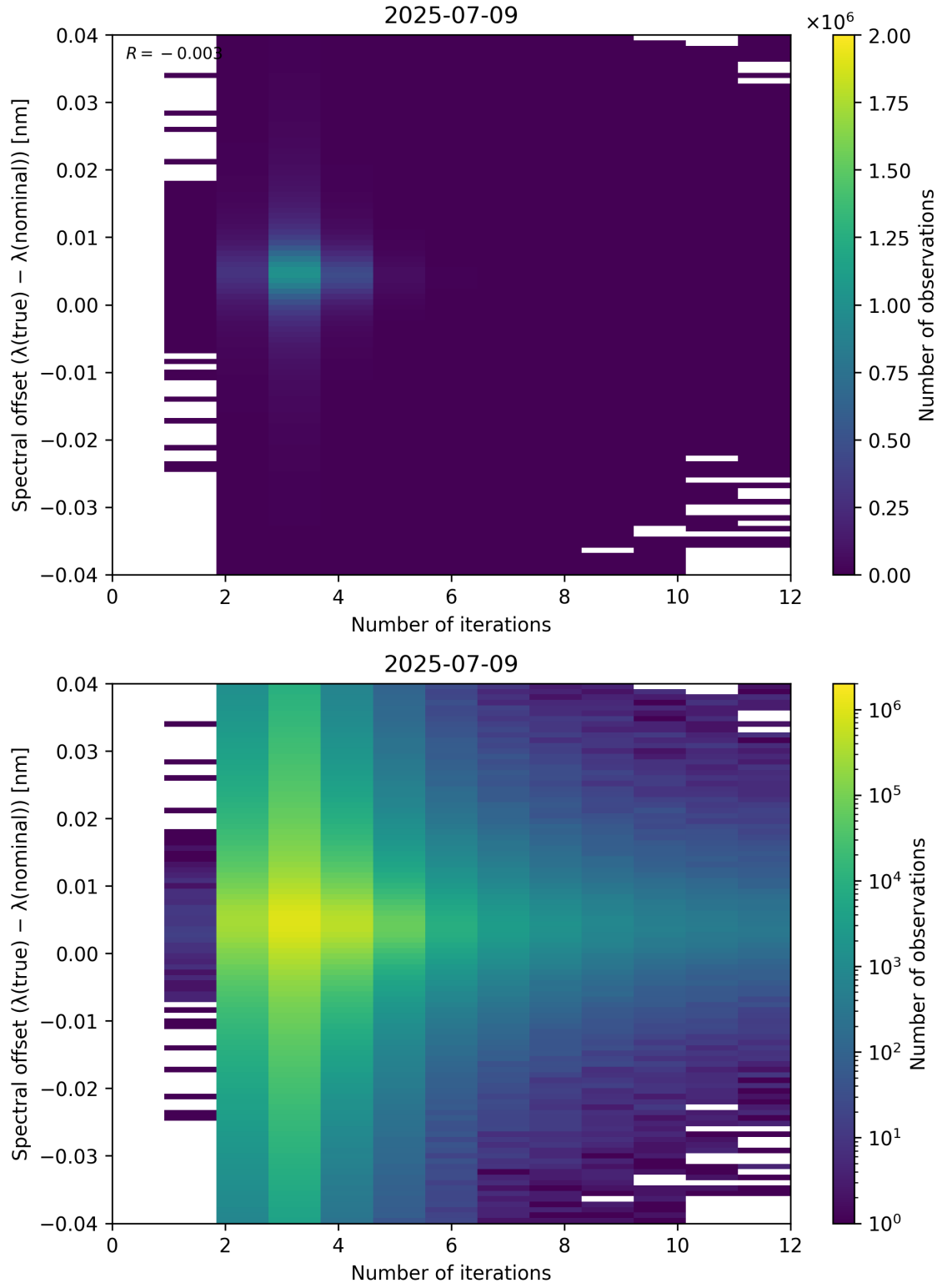
Figure 100: Scatter density plot of “Number of iterations” against “Spectral offset ( \lambda_{\text{true}} - \lambda_{\text{nominal}} )” for 2025-07-08 to 2025-07-10.
