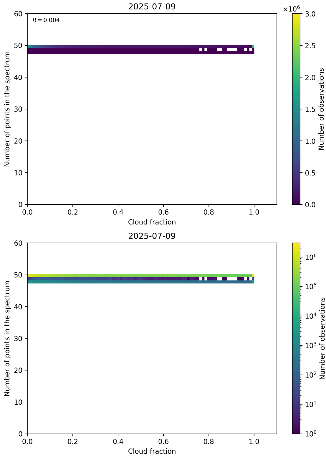
Figure 74: Scatter density plot of “Cloud fraction” against “Number of points in the spectrum” for 2025-07-08 to 2025-07-10.
