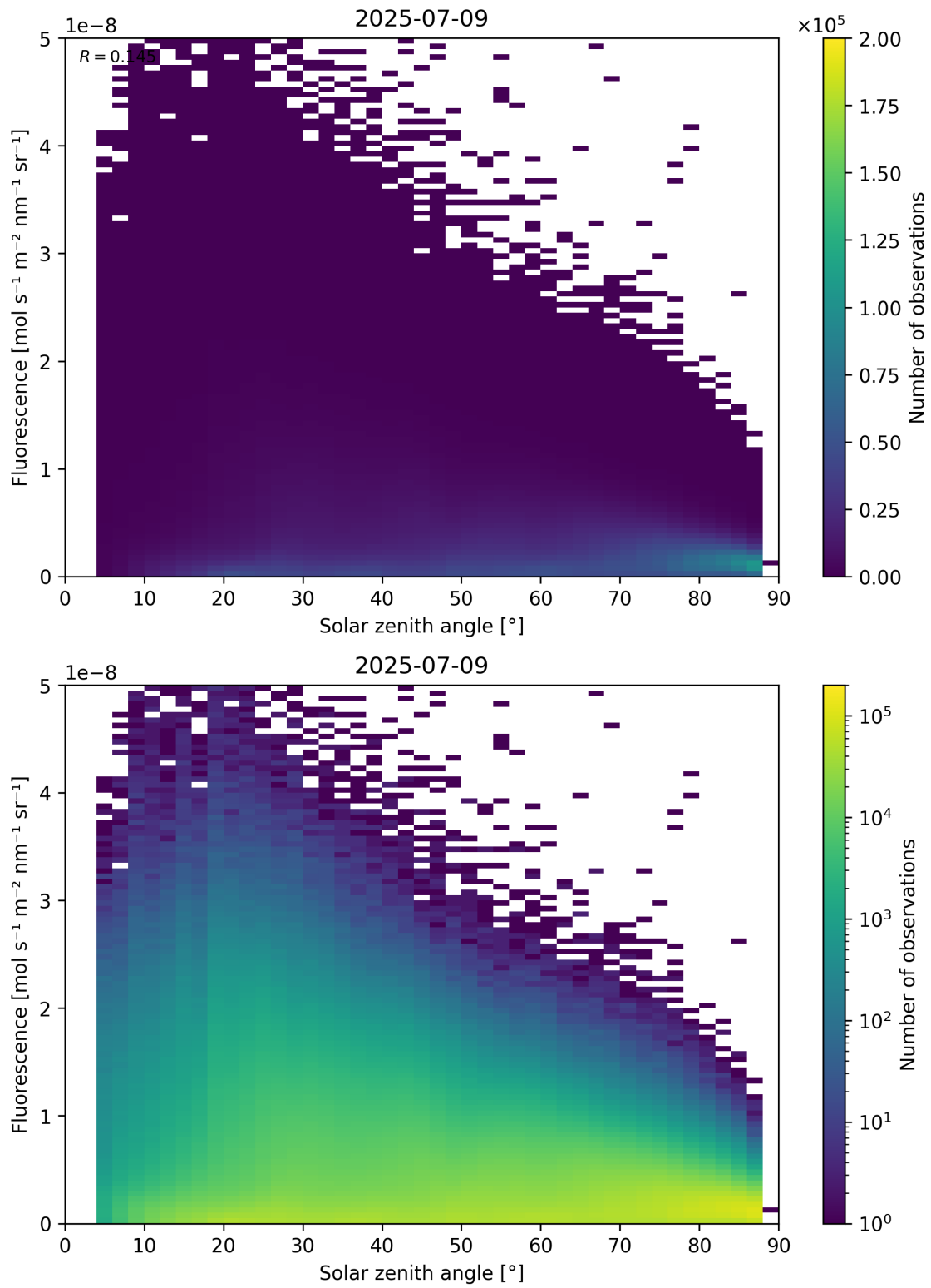
Figure 112: Scatter density plot of “Solar zenith angle” against “Fluorescence” for 2025-07-08 to 2025-07-10.
