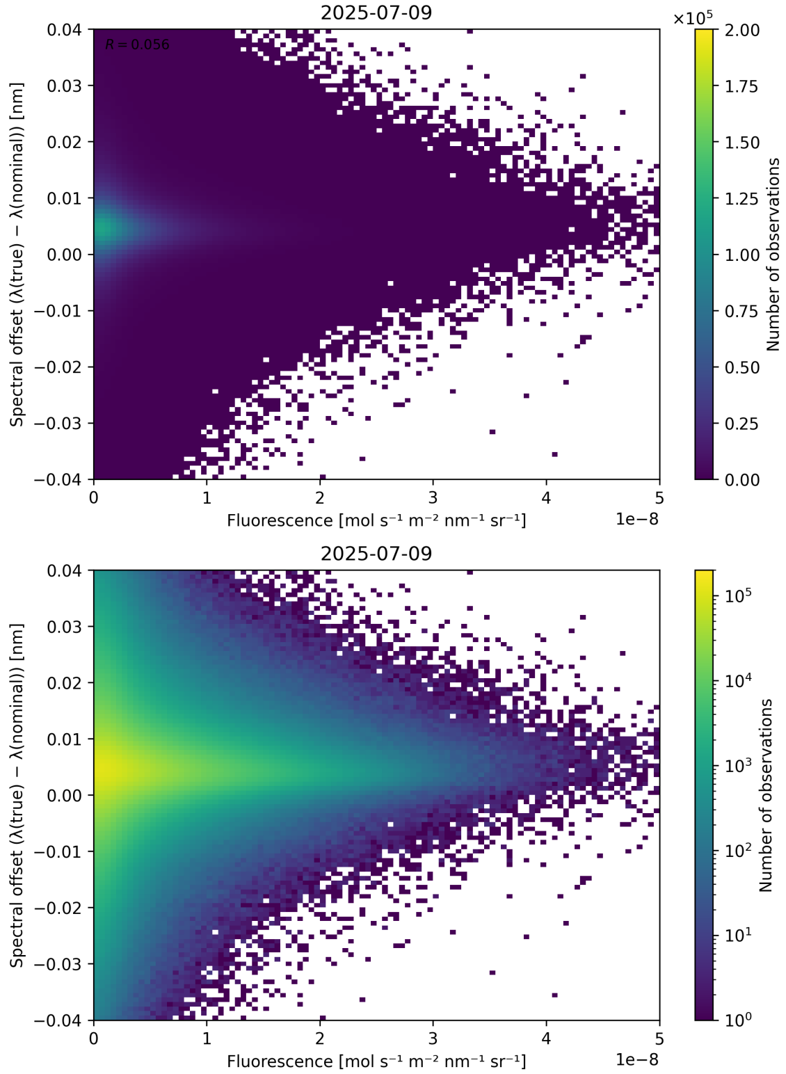
Figure 87: Scatter density plot of “Fluorescence” against “Spectral offset ( \lambda_{\text{true}} - \lambda_{\text{nominal}} )” for 2025-07-08 to 2025-07-10.
