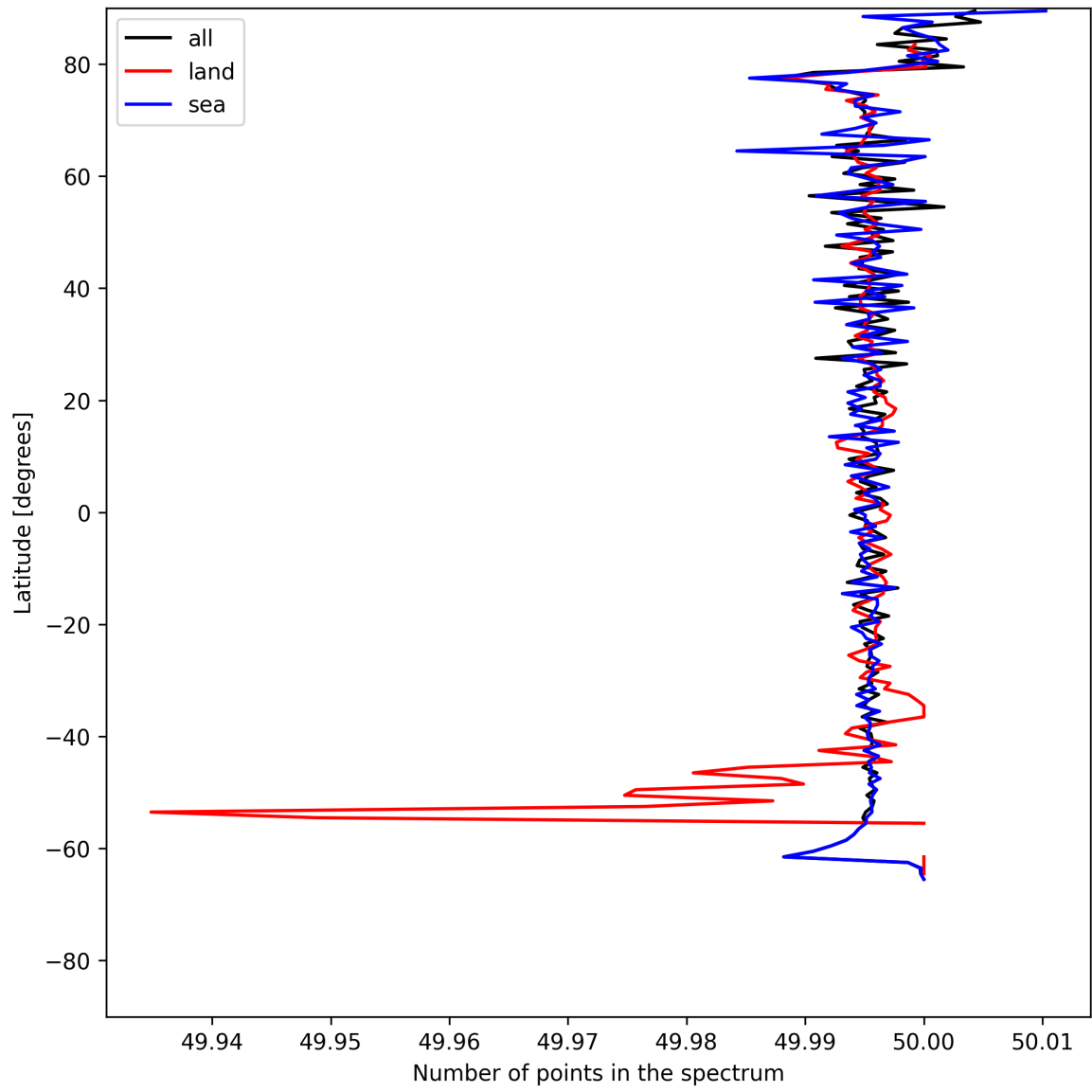
Figure 27: Zonal average of “Number of points in the spectrum” for 2025-07-08 to 2025-07-10.
