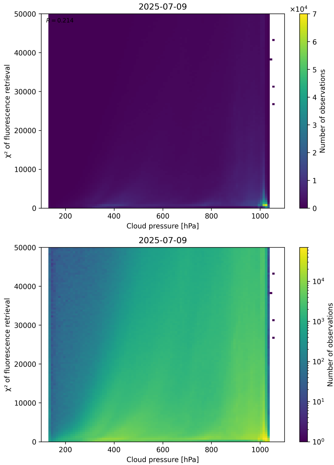
Figure 78: Scatter density plot of “Cloud pressure” against “ \chi^2 of fluorescence retrieval” for 2025-07-08 to 2025-07-10.
