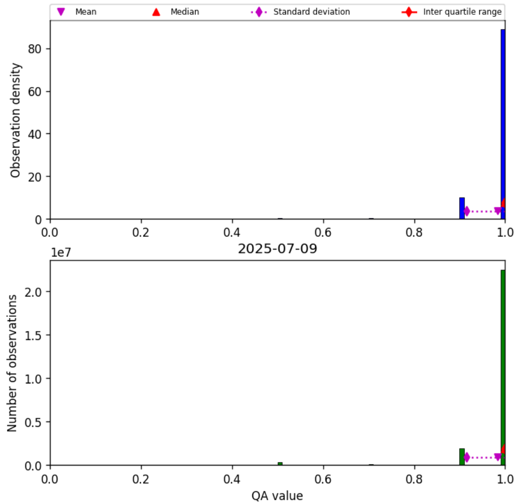
Figure 29: Histogram of “QA value” for 2025-07-08 to 2025-07-10
