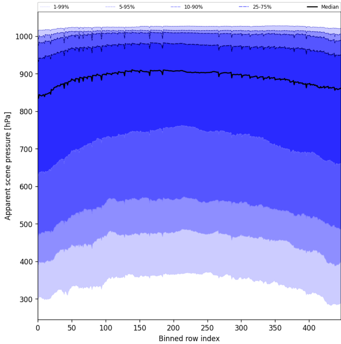
Figure 53: Along track statistics of “Apparent scene pressure” for 2025-07-08 to 2025-07-10
