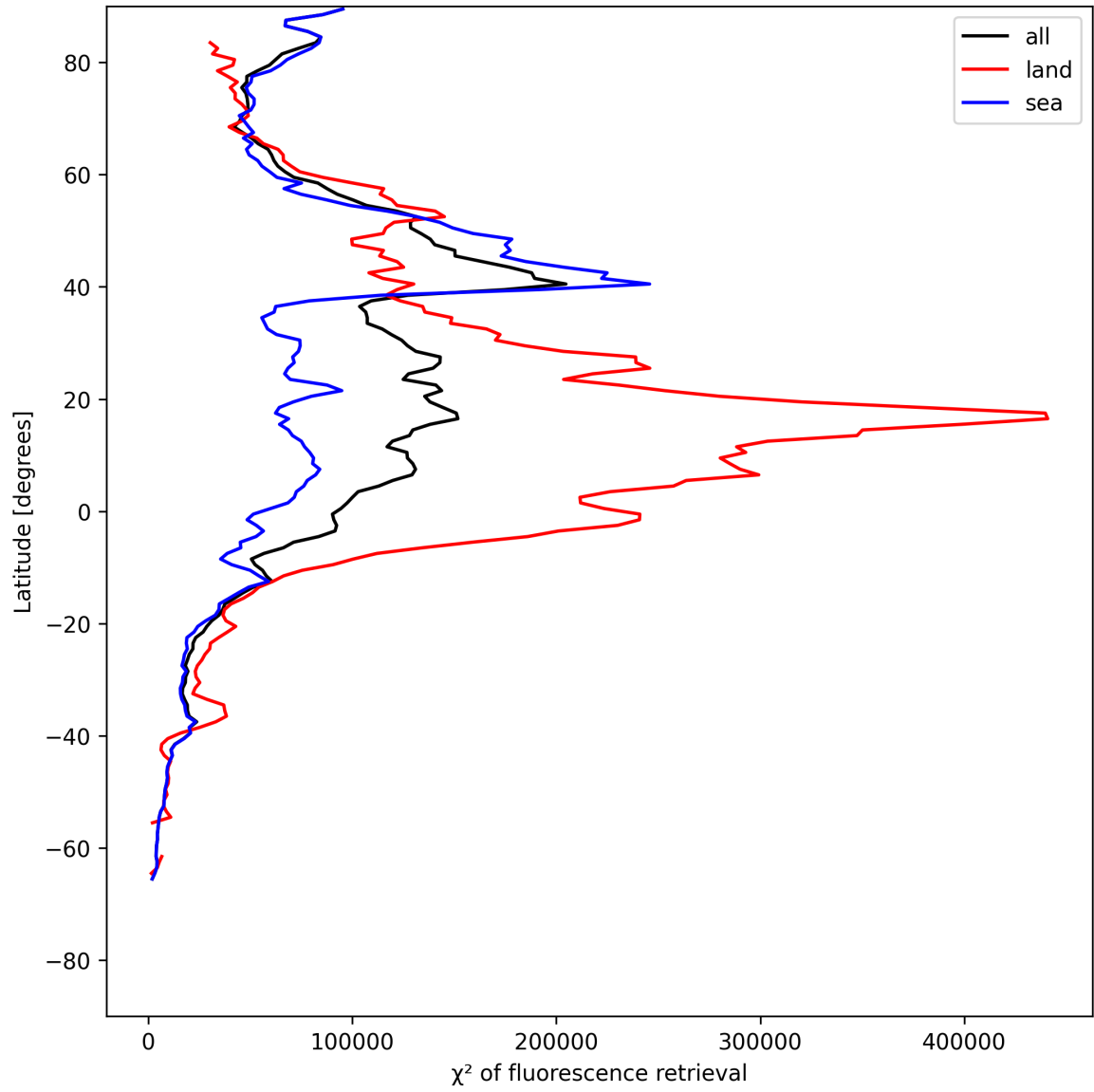
Figure 25: Zonal average of “ \chi^2 of fluorescence retrieval” for 2025-07-08 to 2025-07-10.
