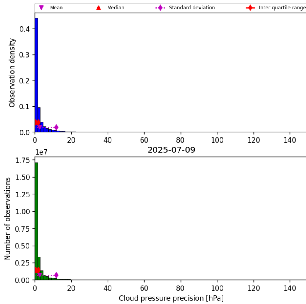
Figure 31: Histogram of “Cloud pressure precision” for 2025-07-08 to 2025-07-10
