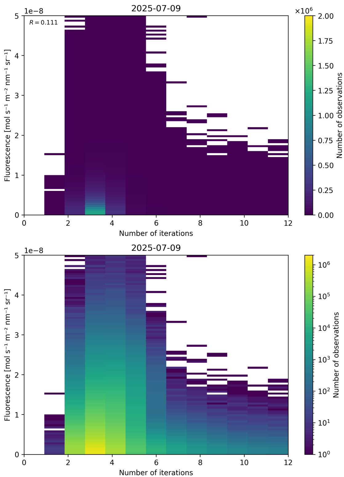
Figure 98: Scatter density plot of “Number of iterations” against “Fluorescence” for 2025-07-08 to 2025-07-10.
