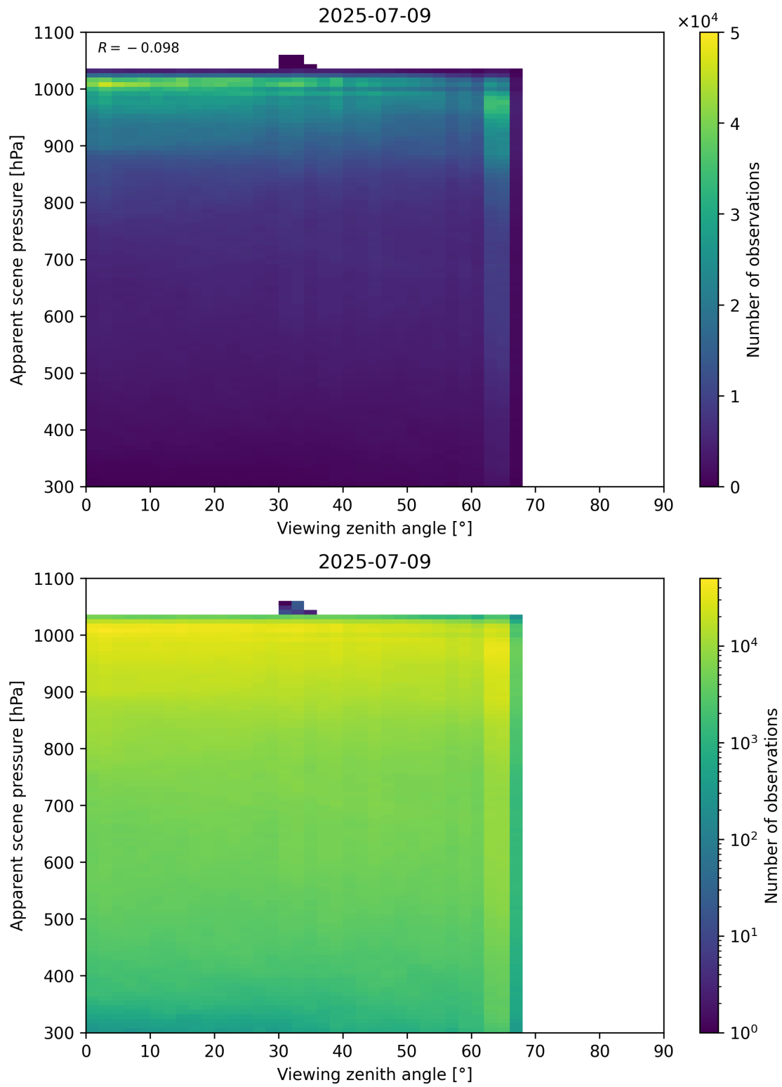
Figure 118: Scatter density plot of “Viewing zenith angle” against “Apparent scene pressure” for 2025-07-08 to 2025-07-10.
