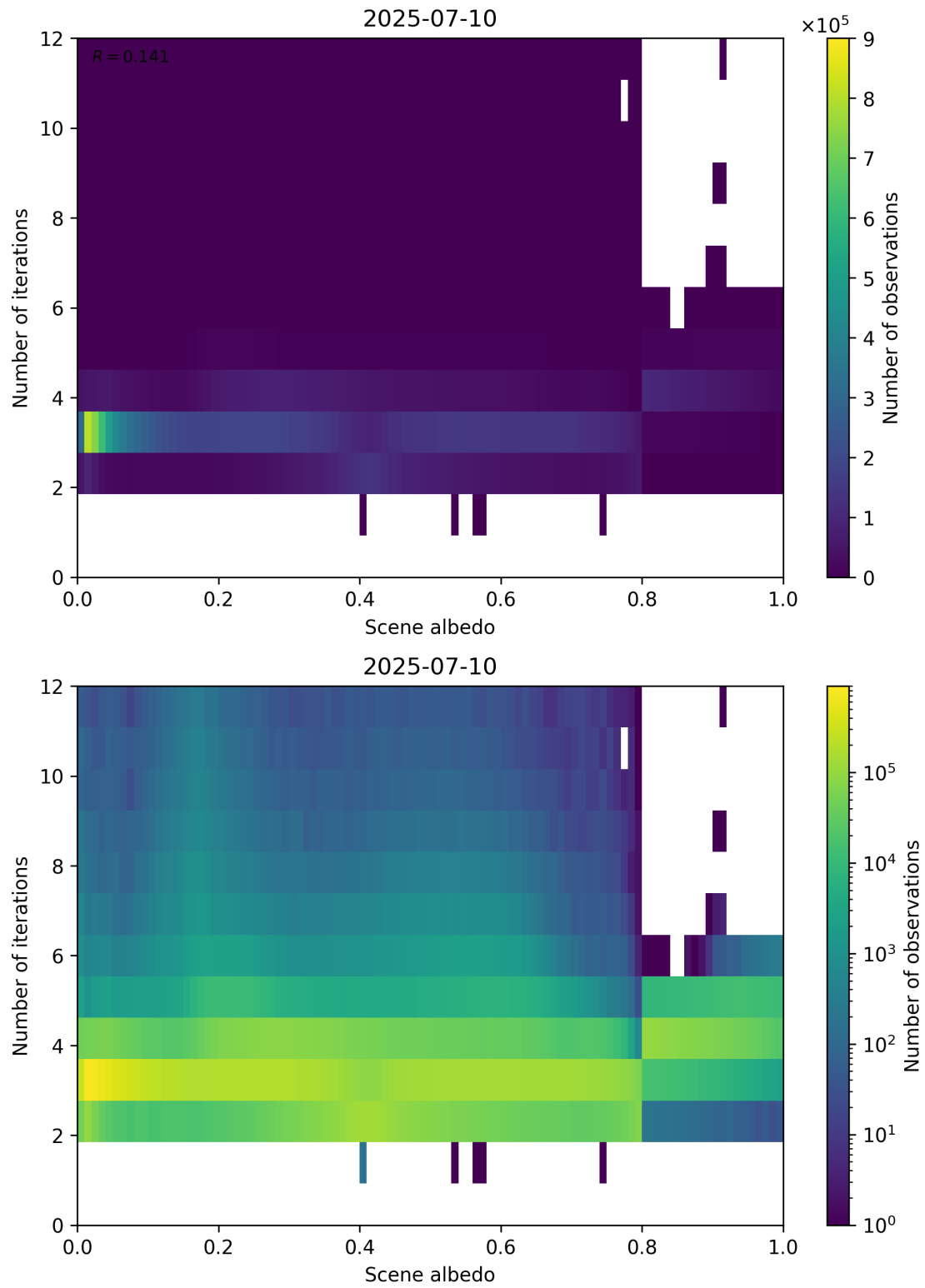
Figure 105: Scatter density plot of “Scene albedo” against “Number of iterations” for 2025-07-09 to 2025-07-11.
