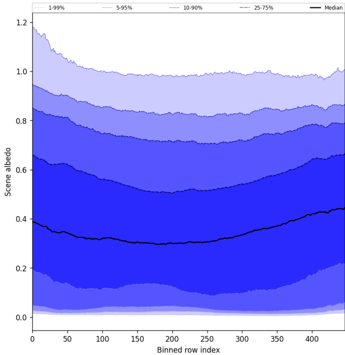
Figure 51: Along track statistics of “Scene albedo” for 2025-07-09 to 2025-07-11
