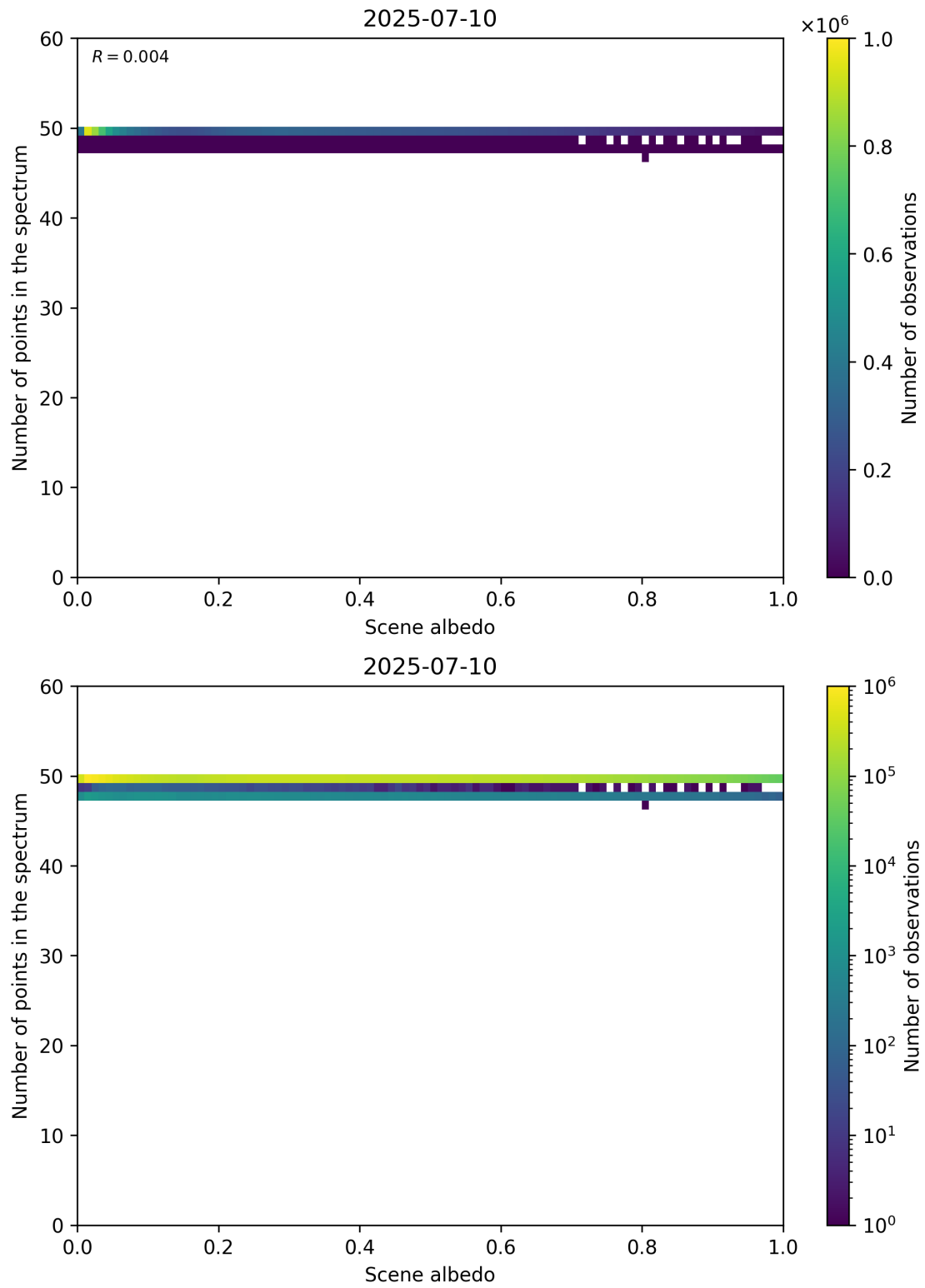
Figure 106: Scatter density plot of “Scene albedo” against “Number of points in the spectrum” for 2025-07-09 to 2025-07-11.
