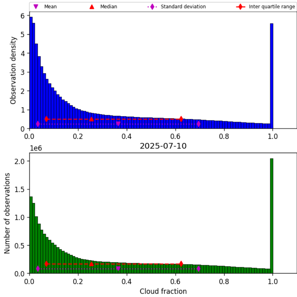
Figure 32: Histogram of “Cloud fraction” for 2025-07-09 to 2025-07-11
