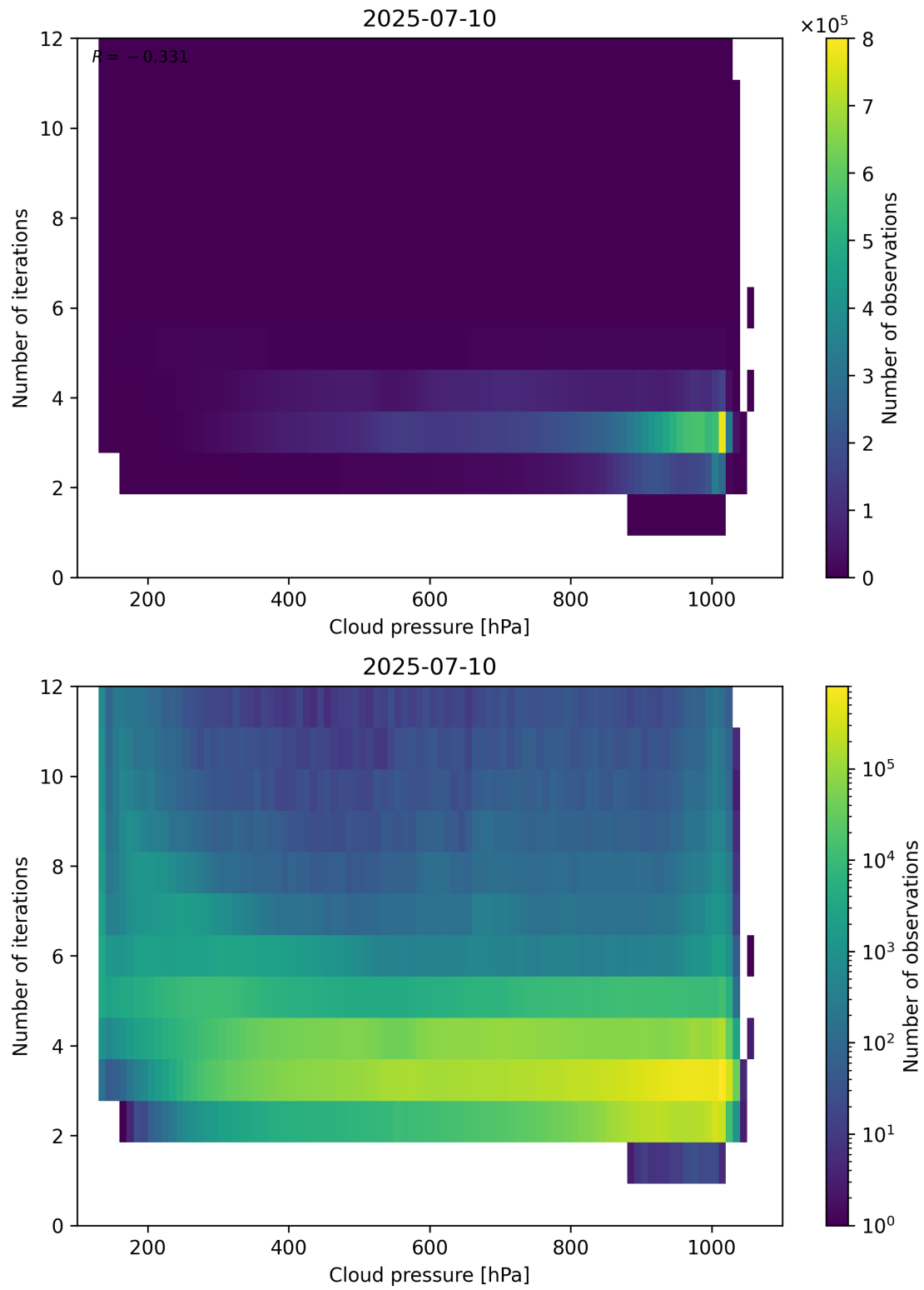
Figure 81: Scatter density plot of “Cloud pressure” against “Number of iterations” for 2025-07-09 to 2025-07-11.
