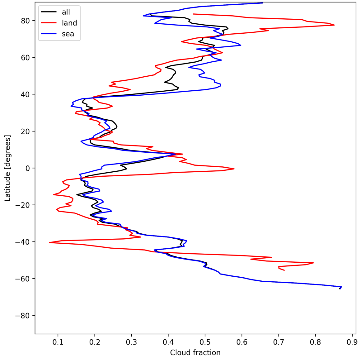
Figure 15: Zonal average of “Cloud fraction” for 2025-07-09 to 2025-07-11.
