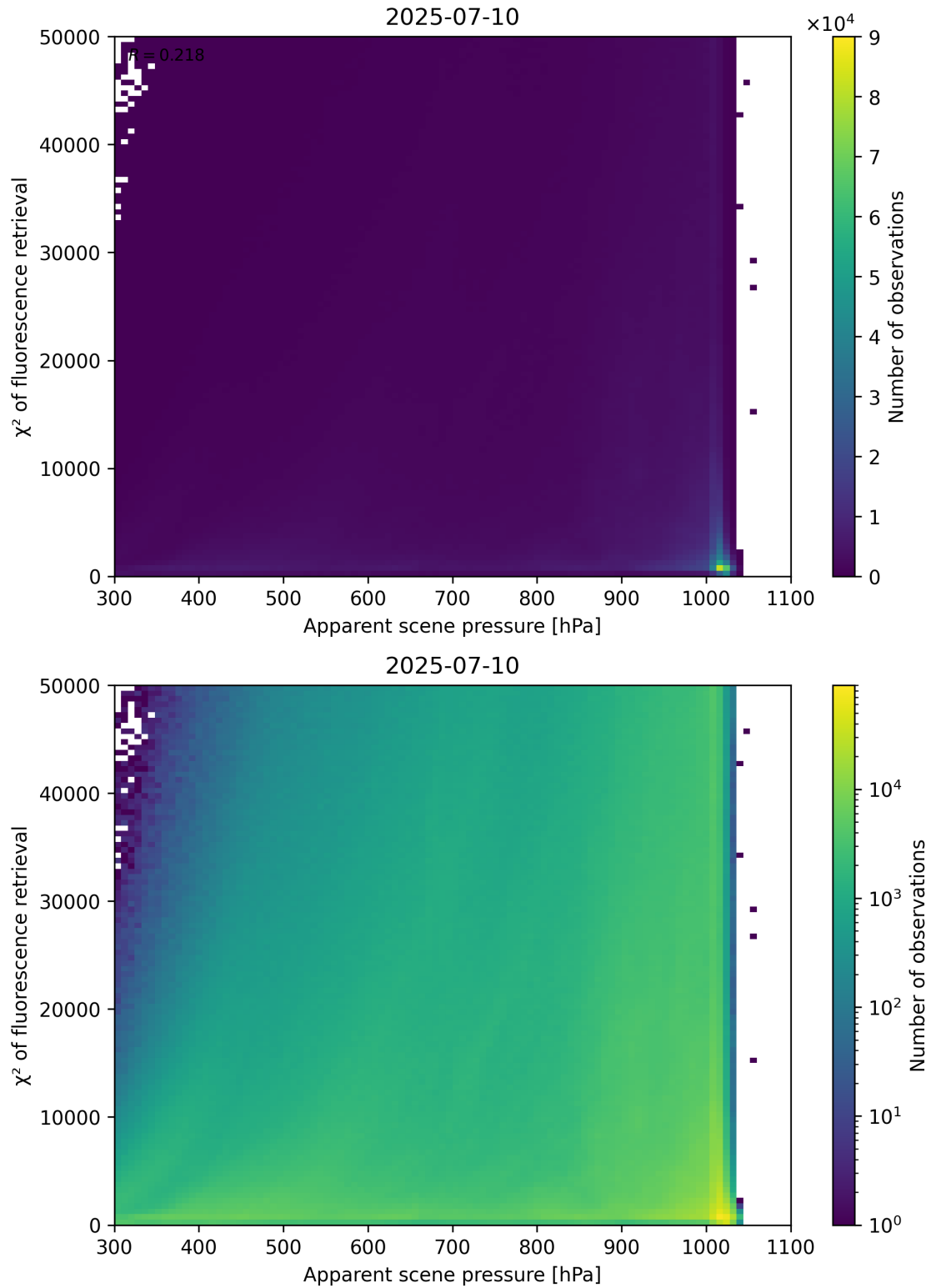
Figure 63: Scatter density plot of “Apparent scene pressure” against “ \chi^2 of fluorescence retrieval” for 2025-07-09 to 2025-07-11.
