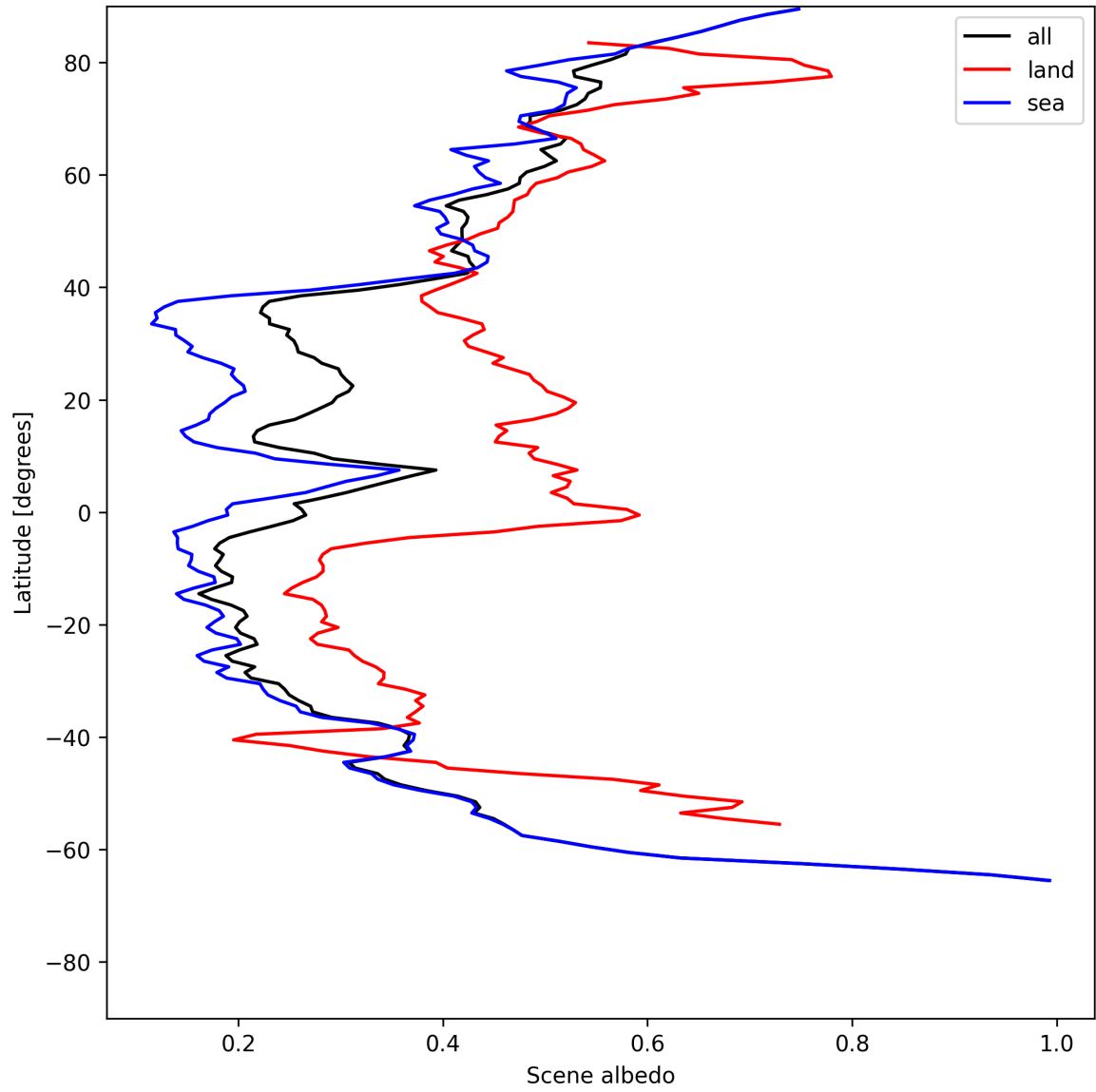
Figure 17: Zonal average of “Scene albedo” for 2025-07-09 to 2025-07-11.
