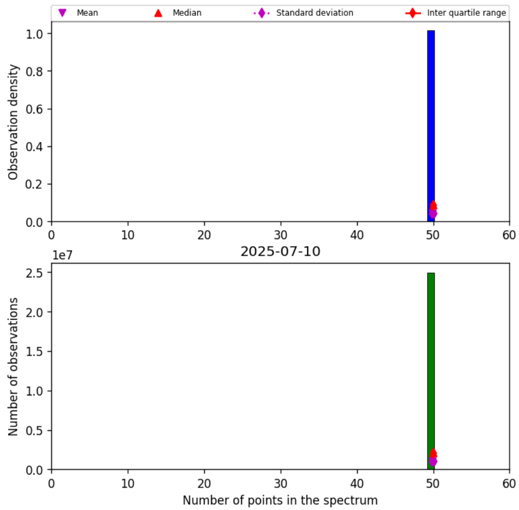
Figure 44: Histogram of “Number of points in the spectrum” for 2025-07-09 to 2025-07-11
