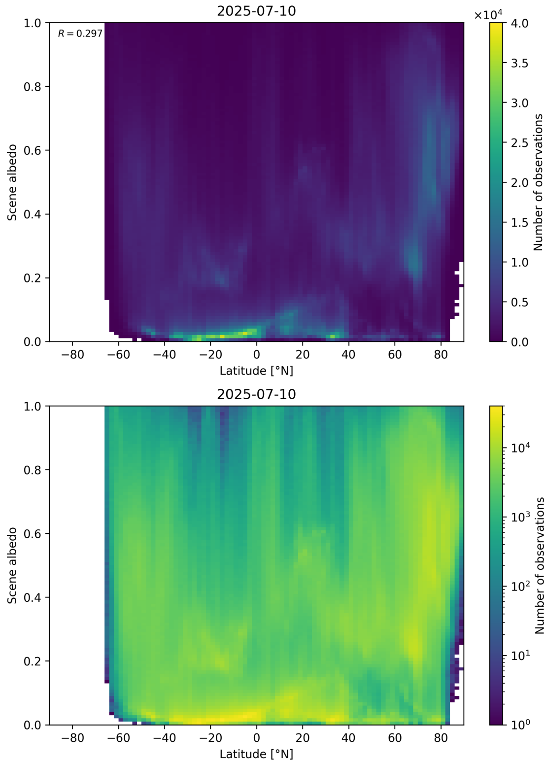
Figure 95: Scatter density plot of “Latitude” against “Scene albedo” for 2025-07-09 to 2025-07-11.
