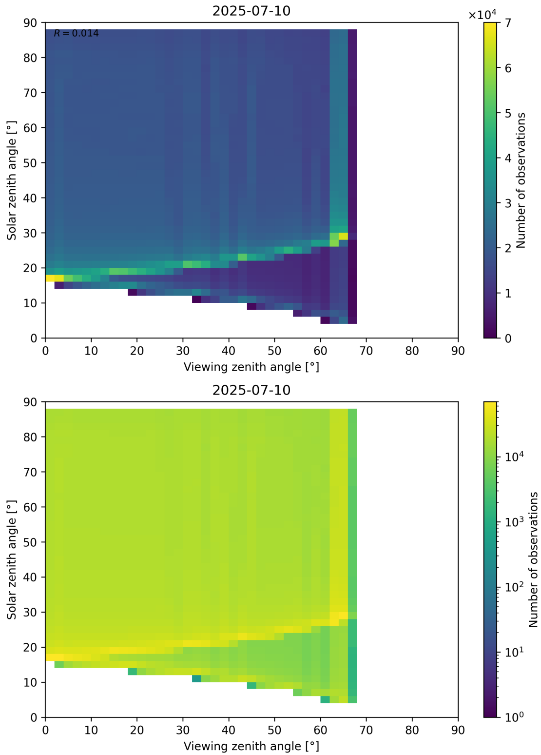
Figure 127: Scatter density plot of “Viewing zenith angle” against “Solar zenith angle” for 2025-07-09 to 2025-07-11.
