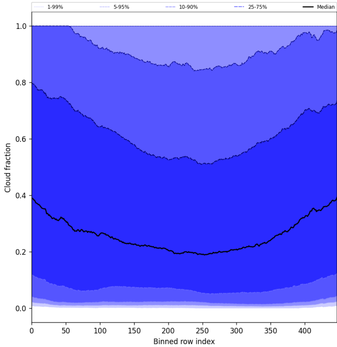
Figure 49: Along track statistics of “Cloud fraction” for 2025-07-09 to 2025-07-11
