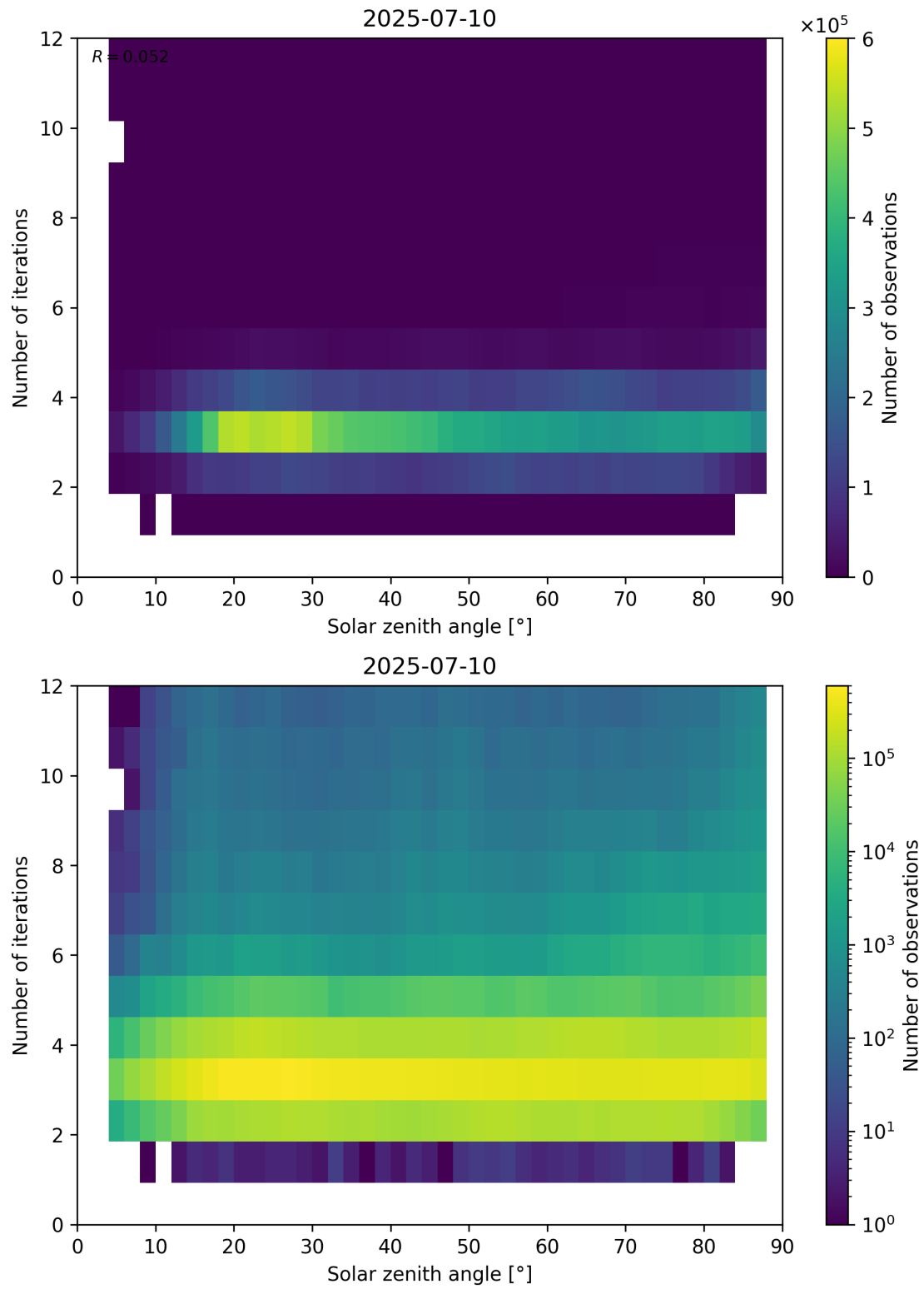
Figure 114: Scatter density plot of “Solar zenith angle” against “Number of iterations” for 2025-07-09 to 2025-07-11.
