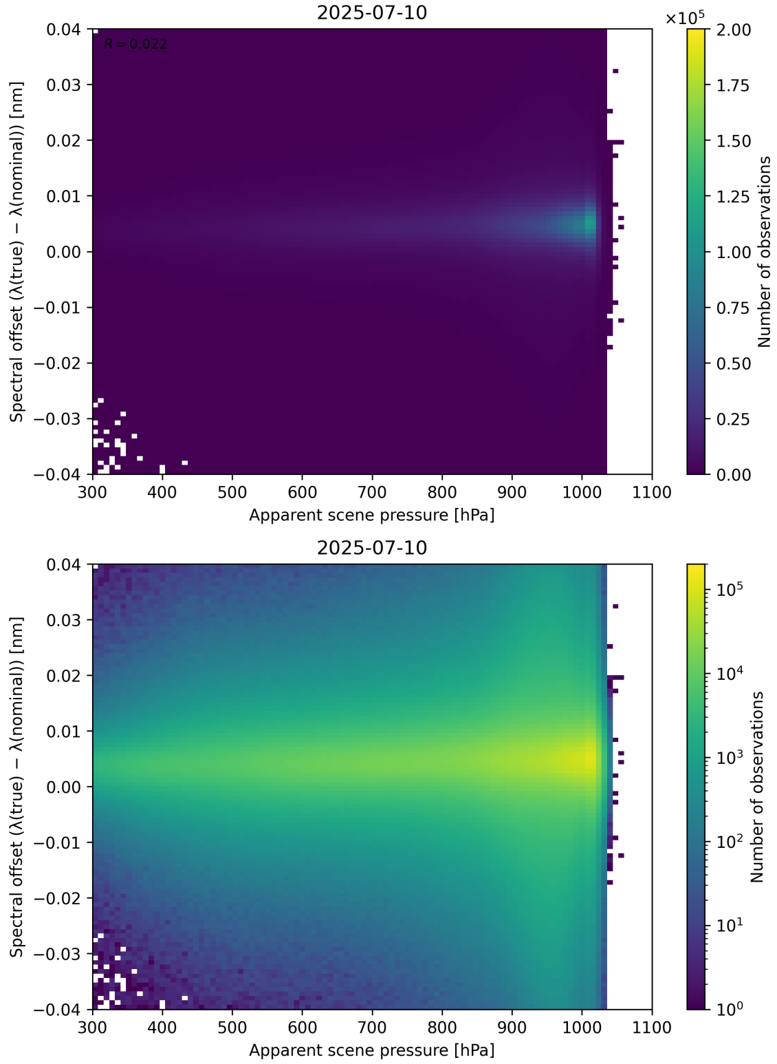
Figure 67: Scatter density plot of “Apparent scene pressure” against “Spectral offset ( \lambda_{\text{true}} - \lambda_{\text{nominal}} )” for 2025-07-09 to 2025-07-11.
