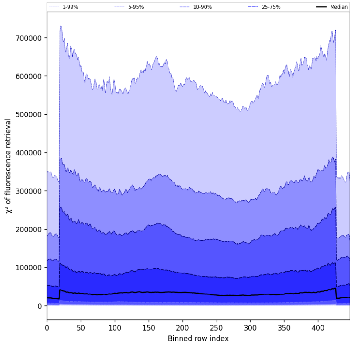
Figure 59: Along track statistics of “ \chi^2 of fluorescence retrieval” for 2025-07-09 to 2025-07-11
