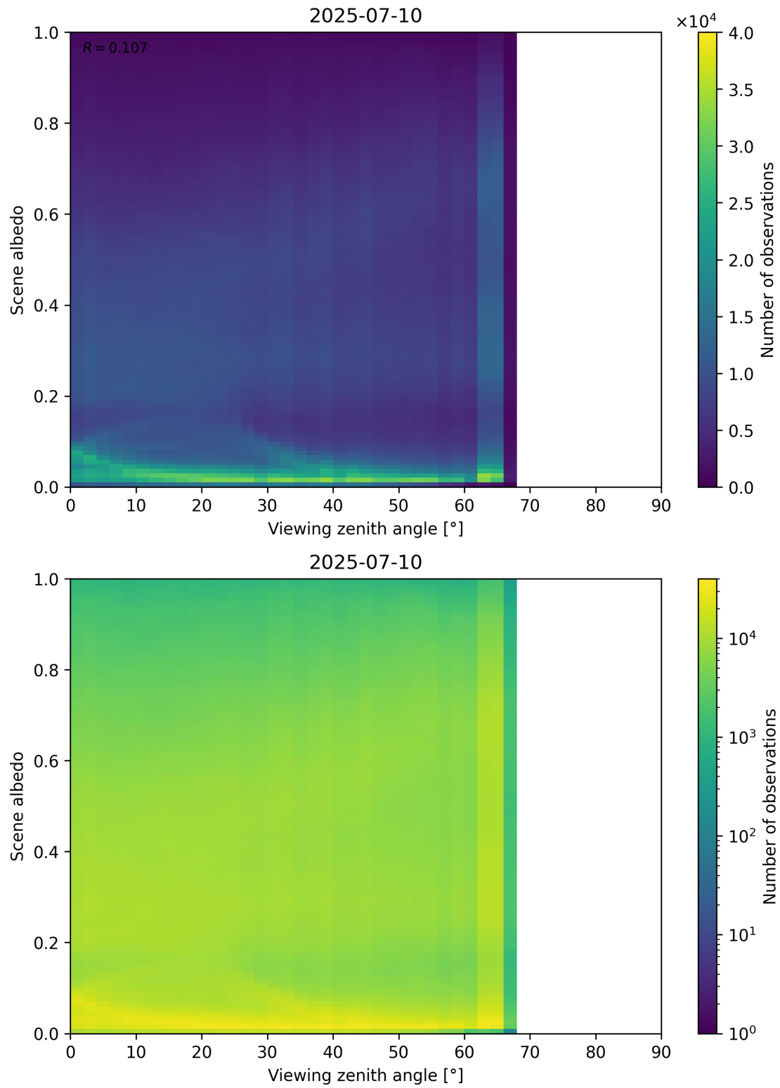
Figure 126: Scatter density plot of “Viewing zenith angle” against “Scene albedo” for 2025-07-09 to 2025-07-11.
