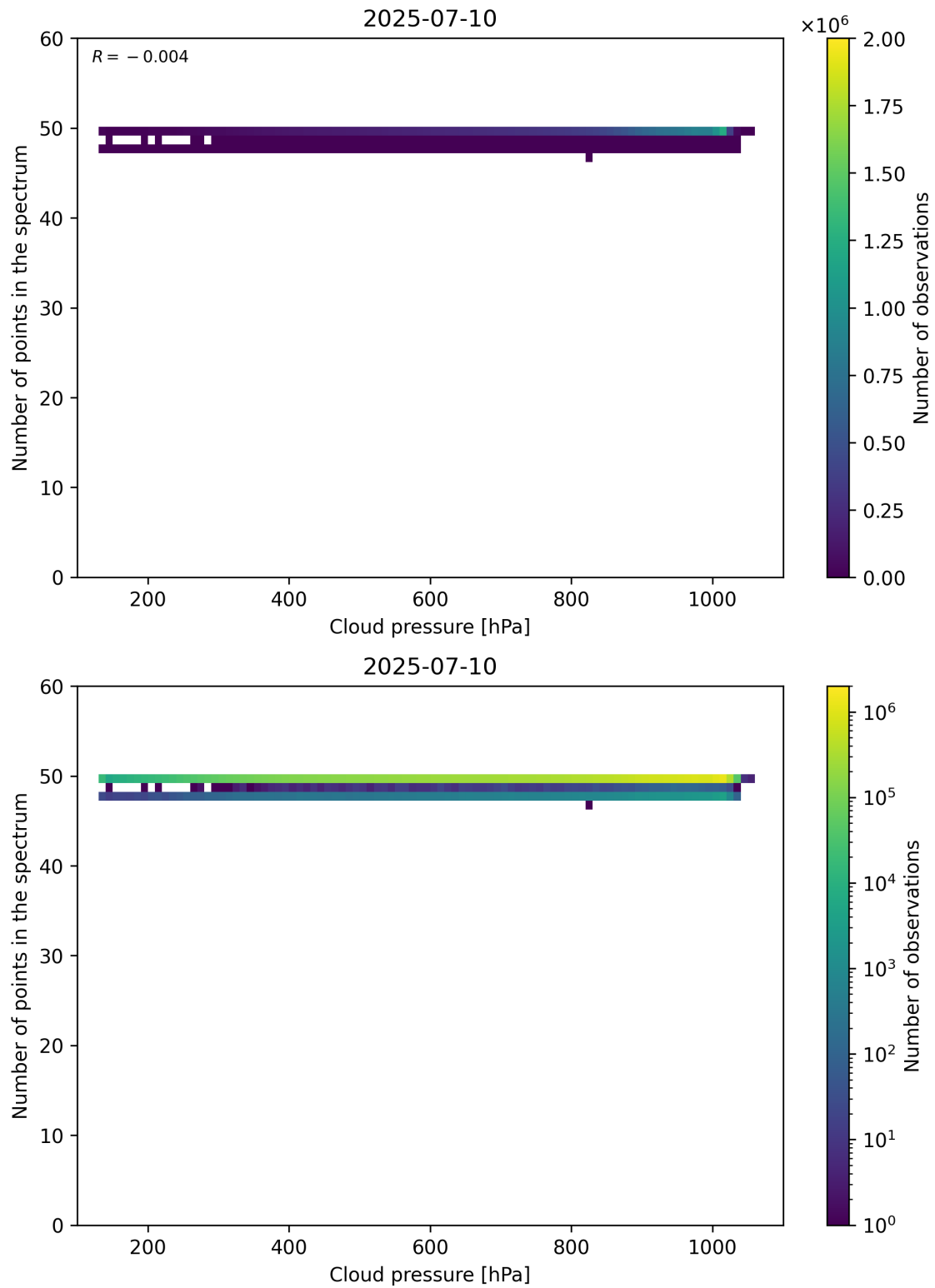
Figure 82: Scatter density plot of “Cloud pressure” against “Number of points in the spectrum” for 2025-07-09 to 2025-07-11.
