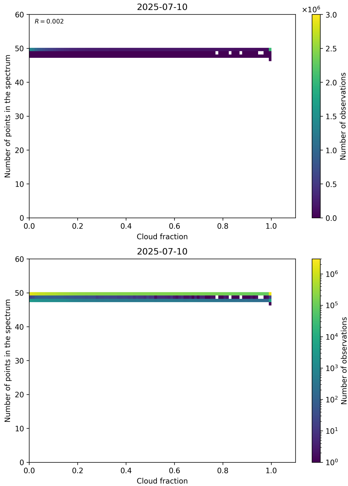
Figure 74: Scatter density plot of “Cloud fraction” against “Number of points in the spectrum” for 2025-07-09 to 2025-07-11.
