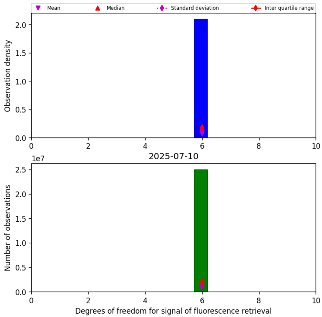
Figure 43: Histogram of "Degrees of freedom for signal of fluorescence retrieval" for 2025-07-09 to 2025-07-11
