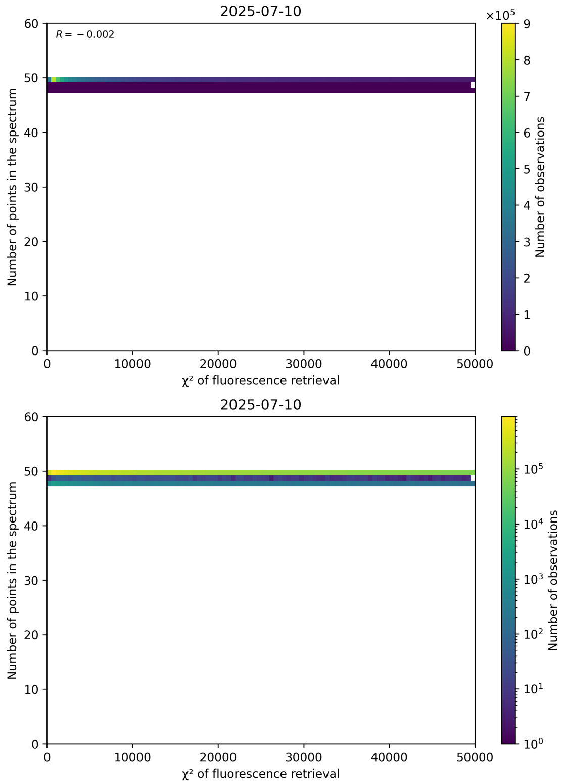
Figure 68: Scatter density plot of “ \chi^2 of fluorescence retrieval” against “Number of points in the spectrum” for 2025-07-09 to 2025-07-11.
