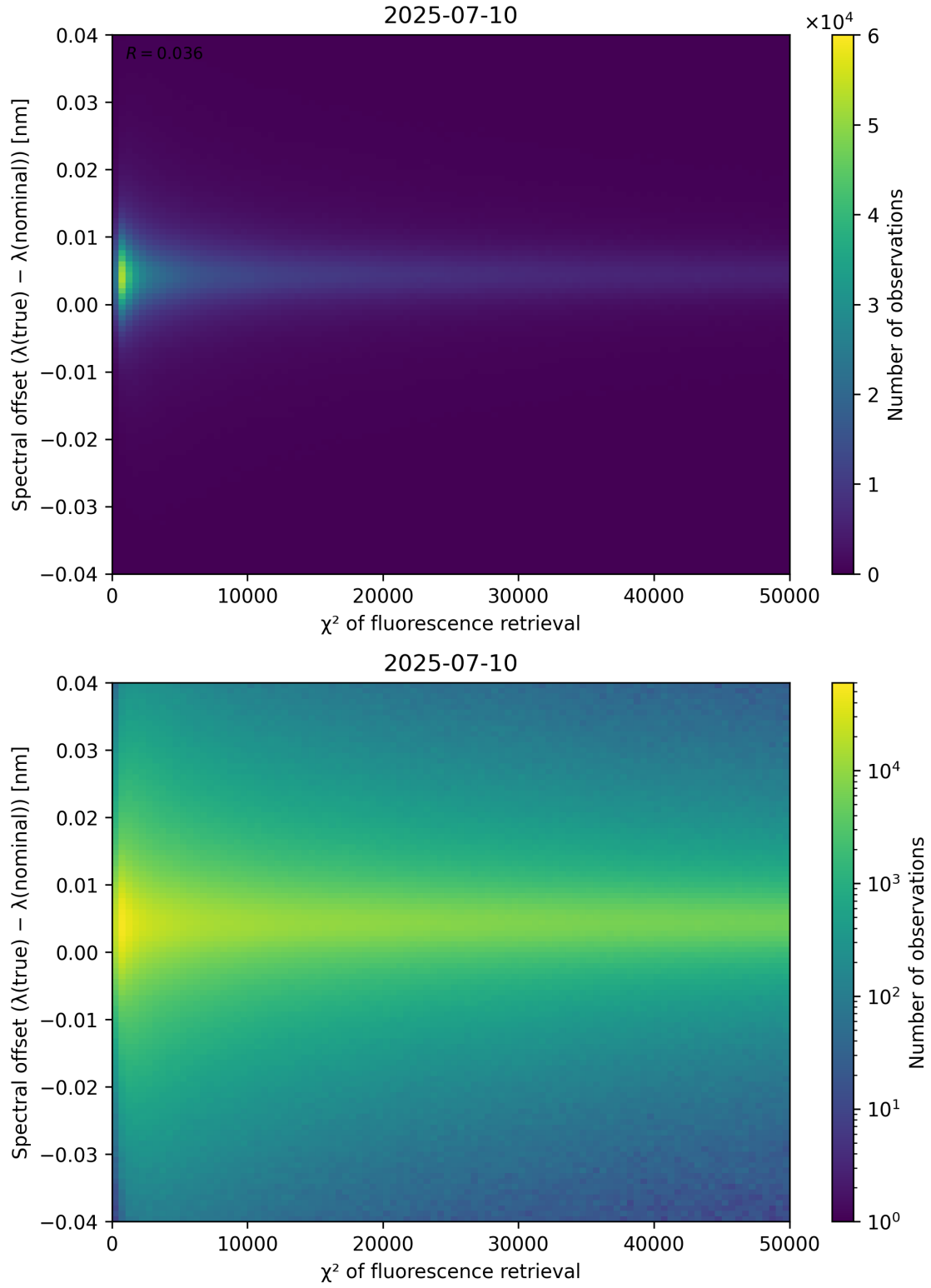
Figure 69: Scatter density plot of “ \chi^2 of fluorescence retrieval” against “Spectral offset ( \lambda_{\text{true}} - \lambda_{\text{nominal}} )” for 2025-07-09 to 2025-07-11.
