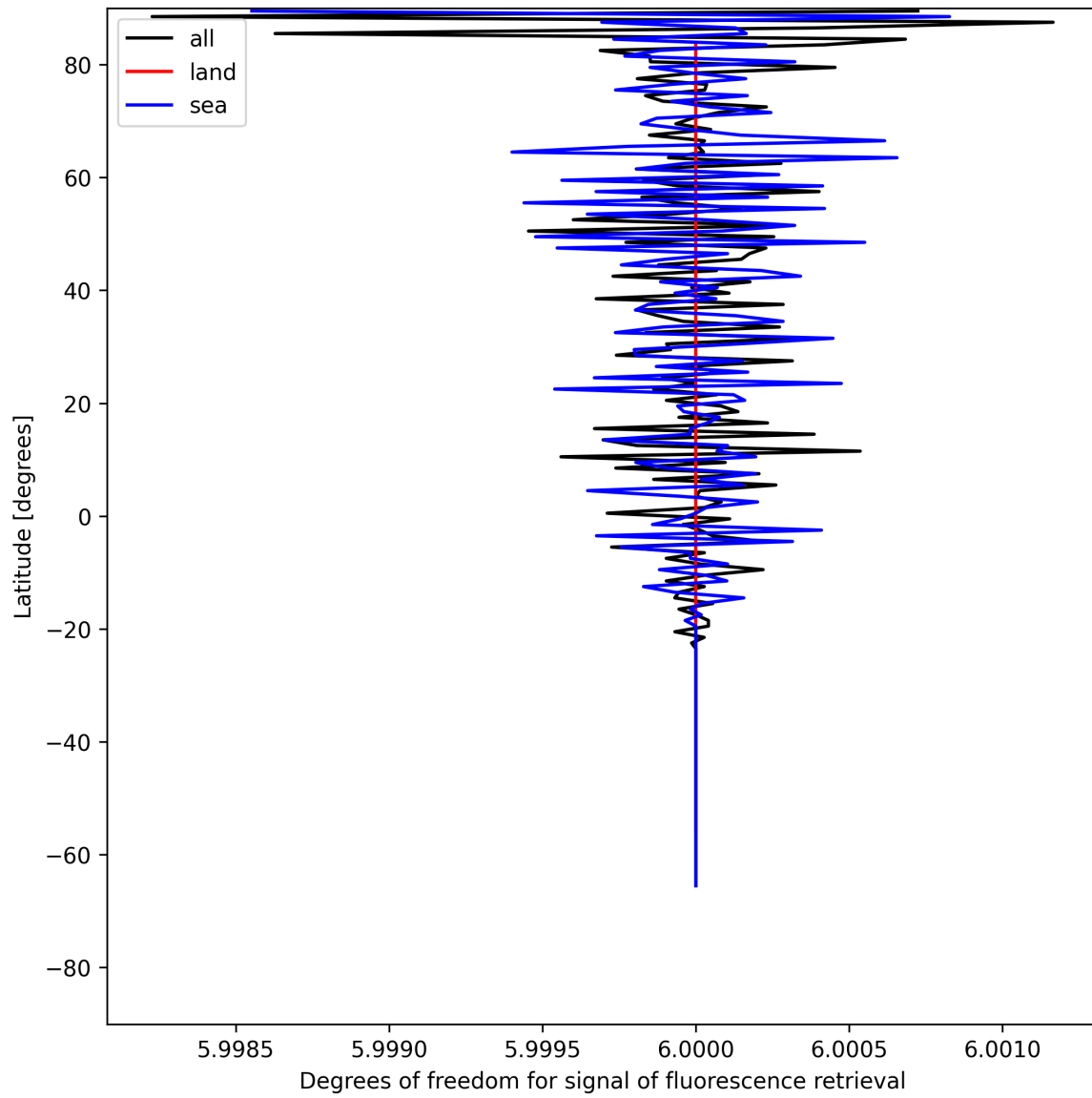
Figure 26: Zonal average of “Degrees of freedom for signal of fluorescence retrieval” for 2025-07-09 to 2025-07-11.
