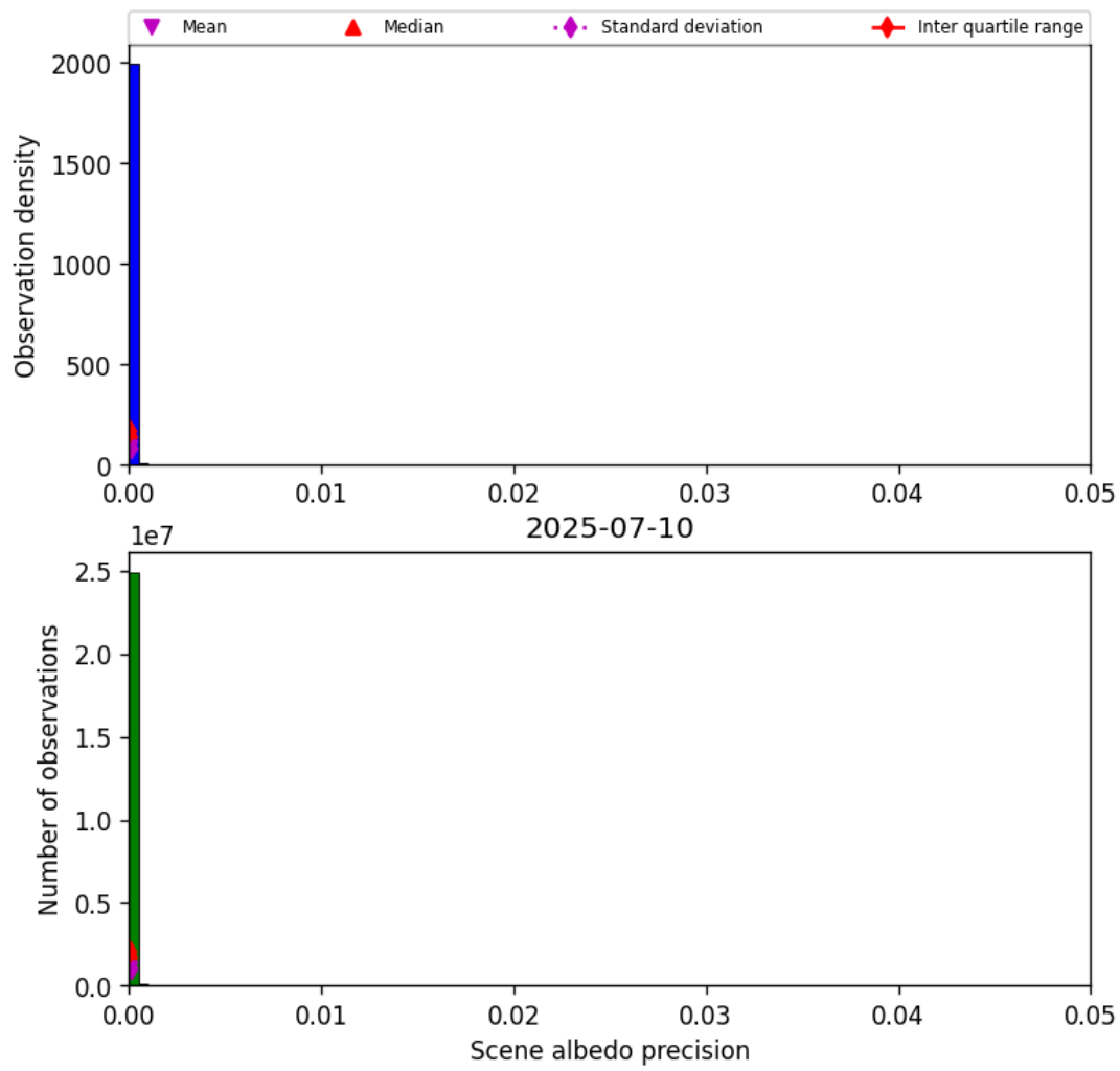
Figure 35: Histogram of “Scene albedo precision” for 2025-07-09 to 2025-07-11
