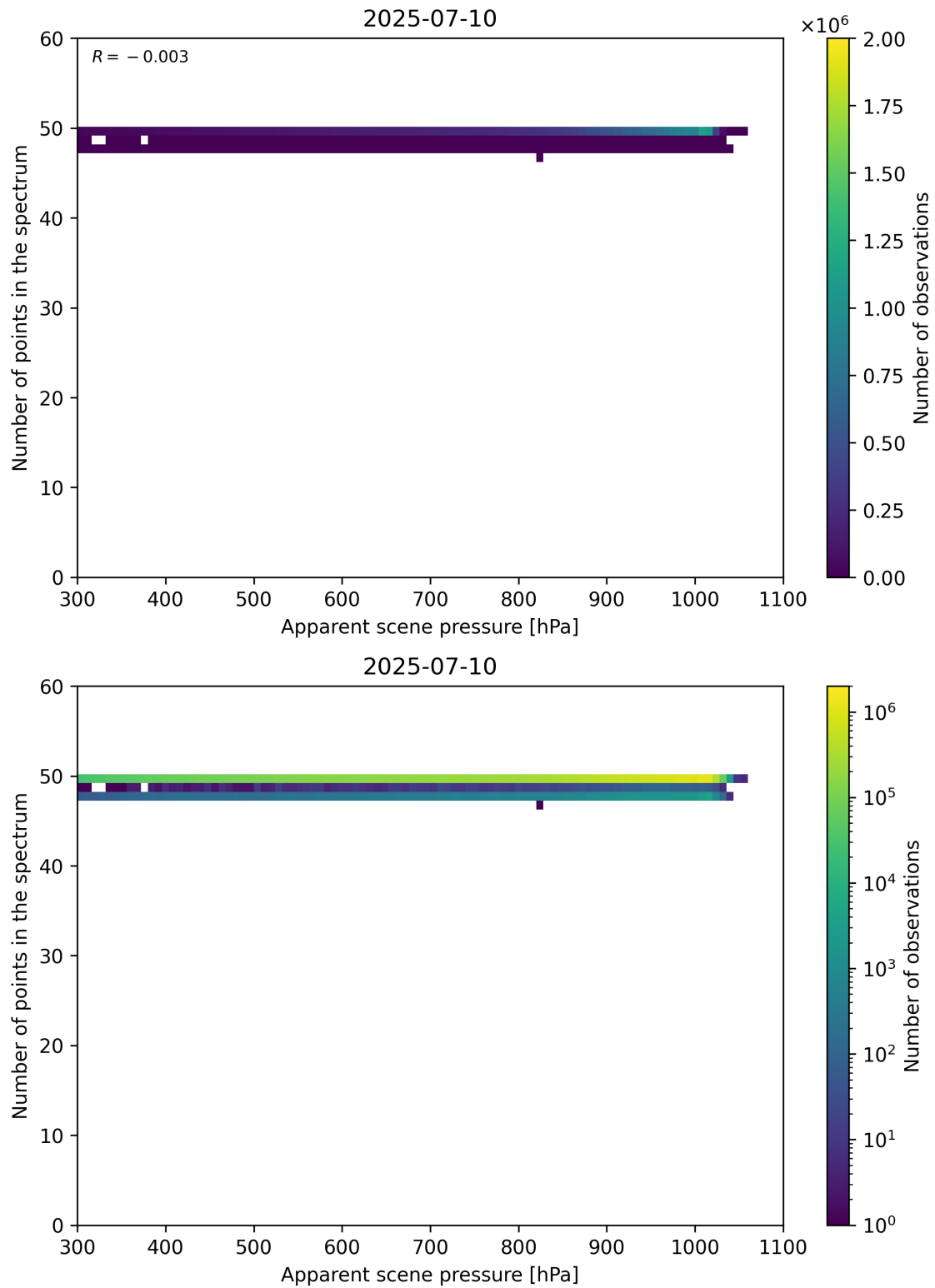
Figure 66: Scatter density plot of “Apparent scene pressure” against “Number of points in the spectrum” for 2025-07-09 to 2025-07-11.
