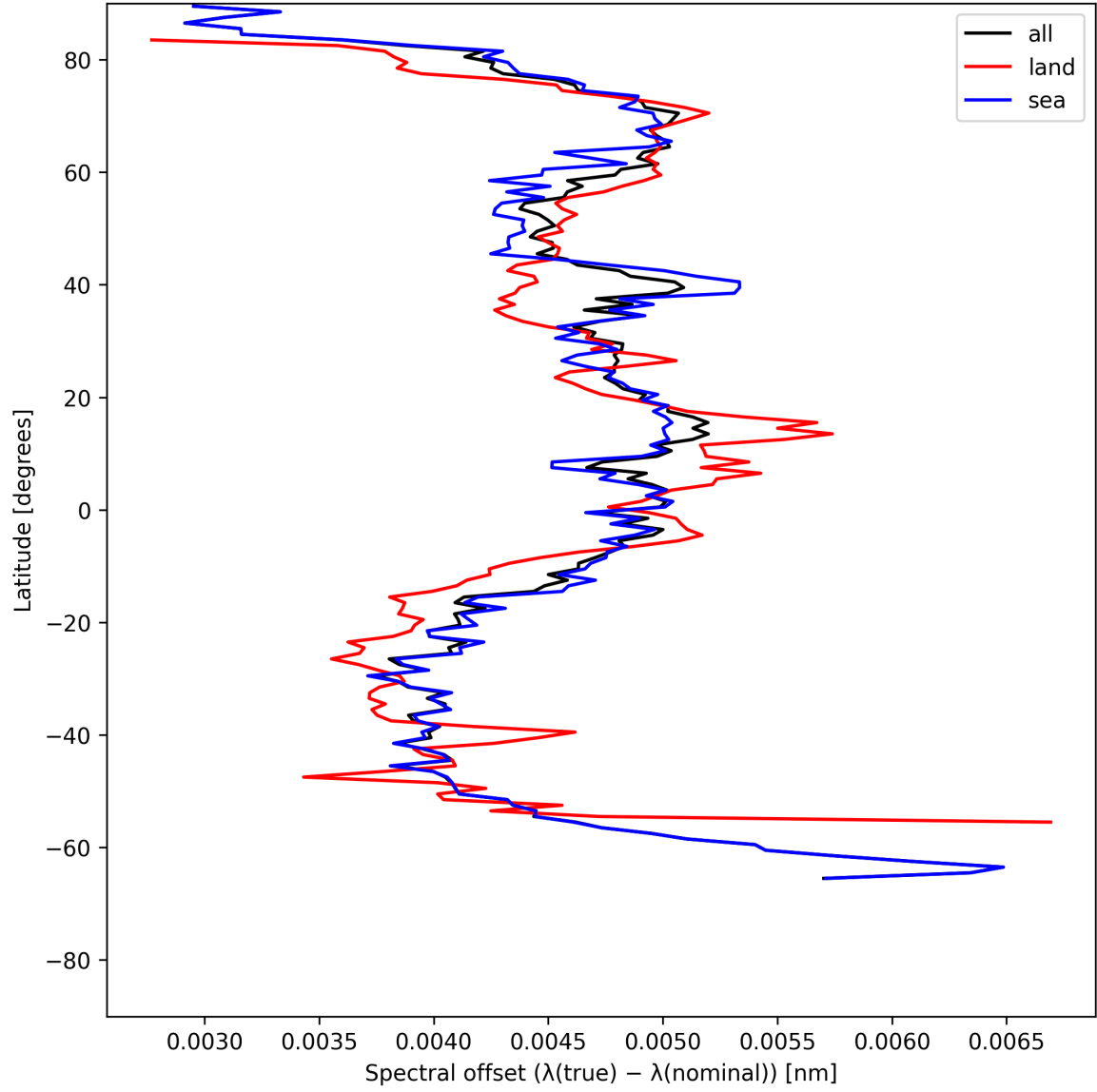
Figure 28: Zonal average of “Spectral offset ( \lambda_{\text{true}} - \lambda_{\text{nominal}} )” for 2025-07-09 to 2025-07-11.
