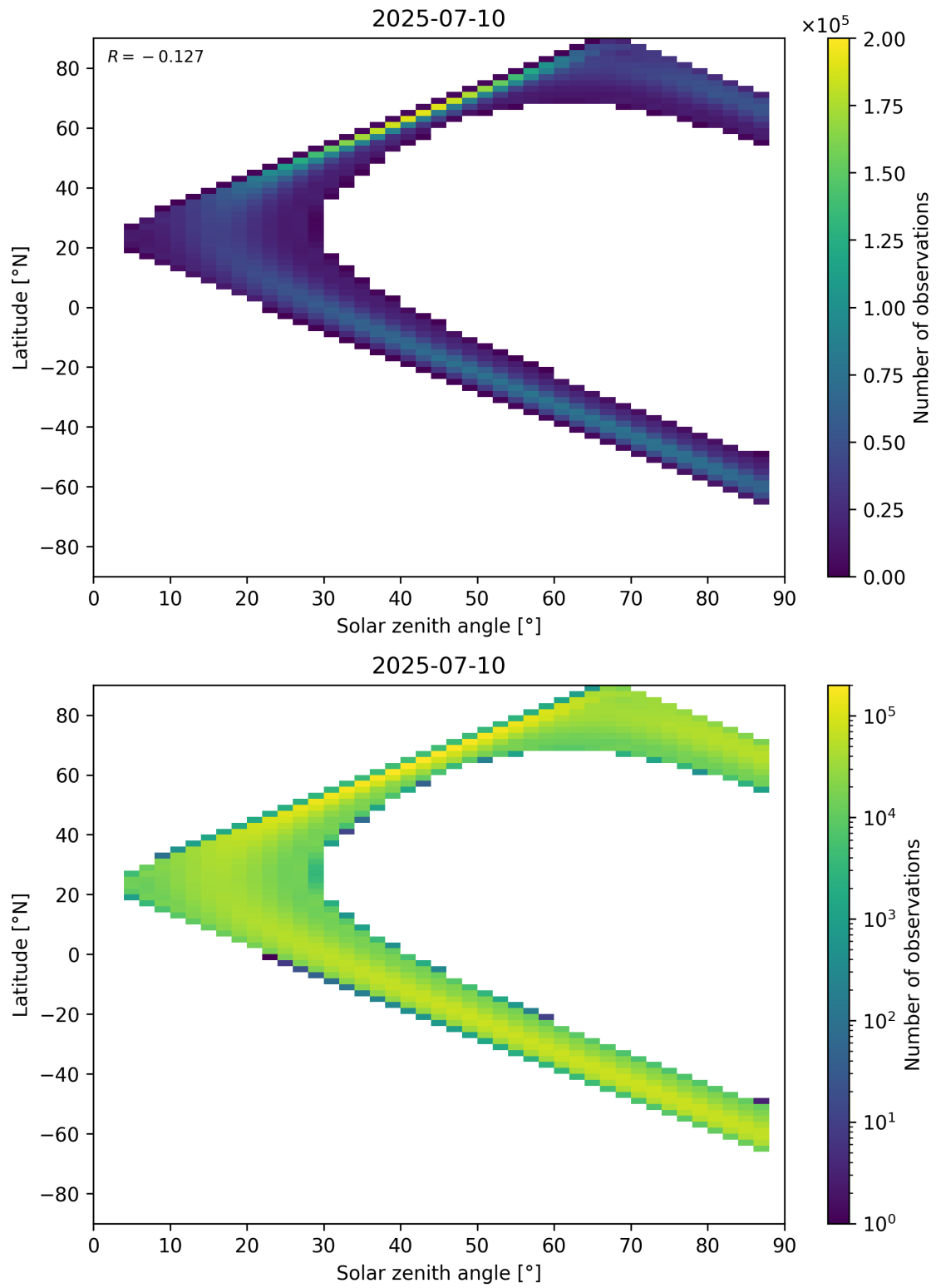
Figure 113: Scatter density plot of “Solar zenith angle” against “Latitude” for 2025-07-09 to 2025-07-11.
