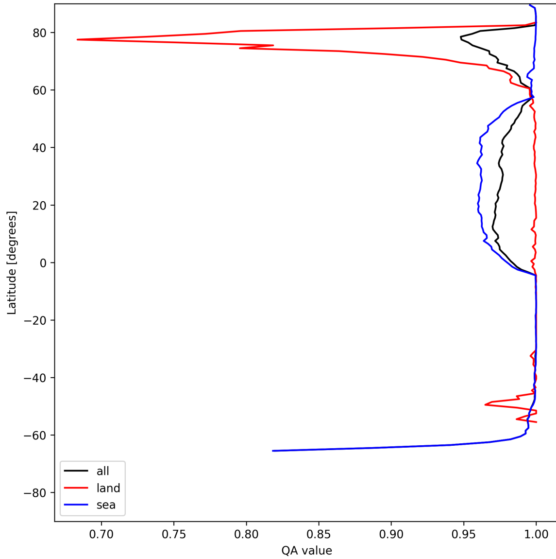
Figure 12: Zonal average of “QA value” for 2025-07-09 to 2025-07-11.
