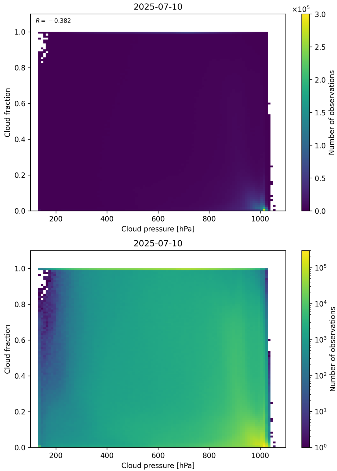
Figure 79: Scatter density plot of “Cloud pressure” against “Cloud fraction” for 2025-07-09 to 2025-07-11.
