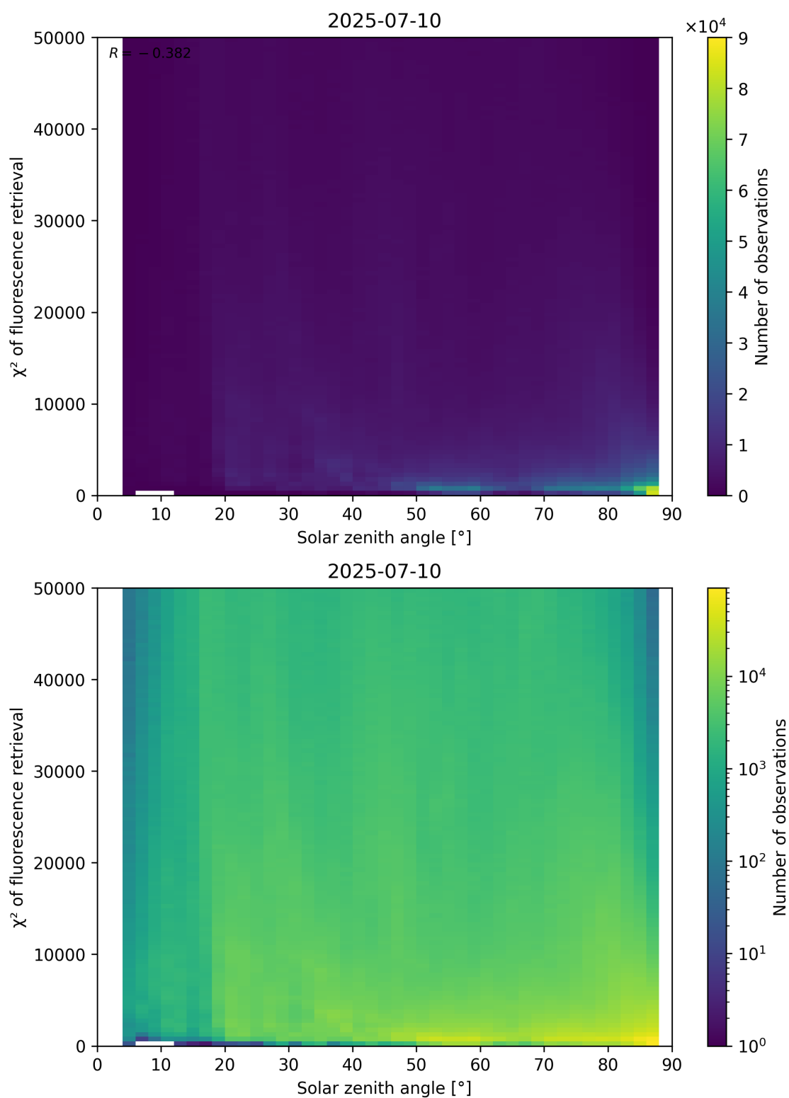
Figure 109: Scatter density plot of “Solar zenith angle” against “ \chi^2 of fluorescence retrieval” for 2025-07-09 to 2025-07-11.
