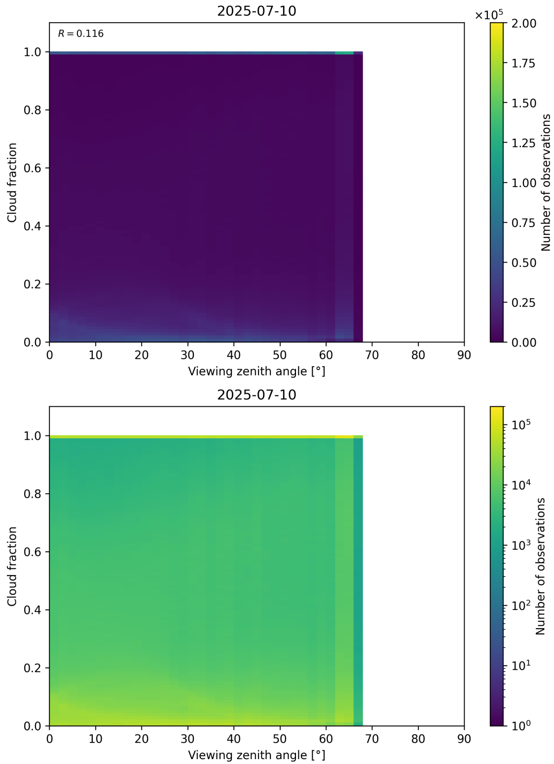
Figure 120: Scatter density plot of “Viewing zenith angle” against “Cloud fraction” for 2025-07-09 to 2025-07-11.
