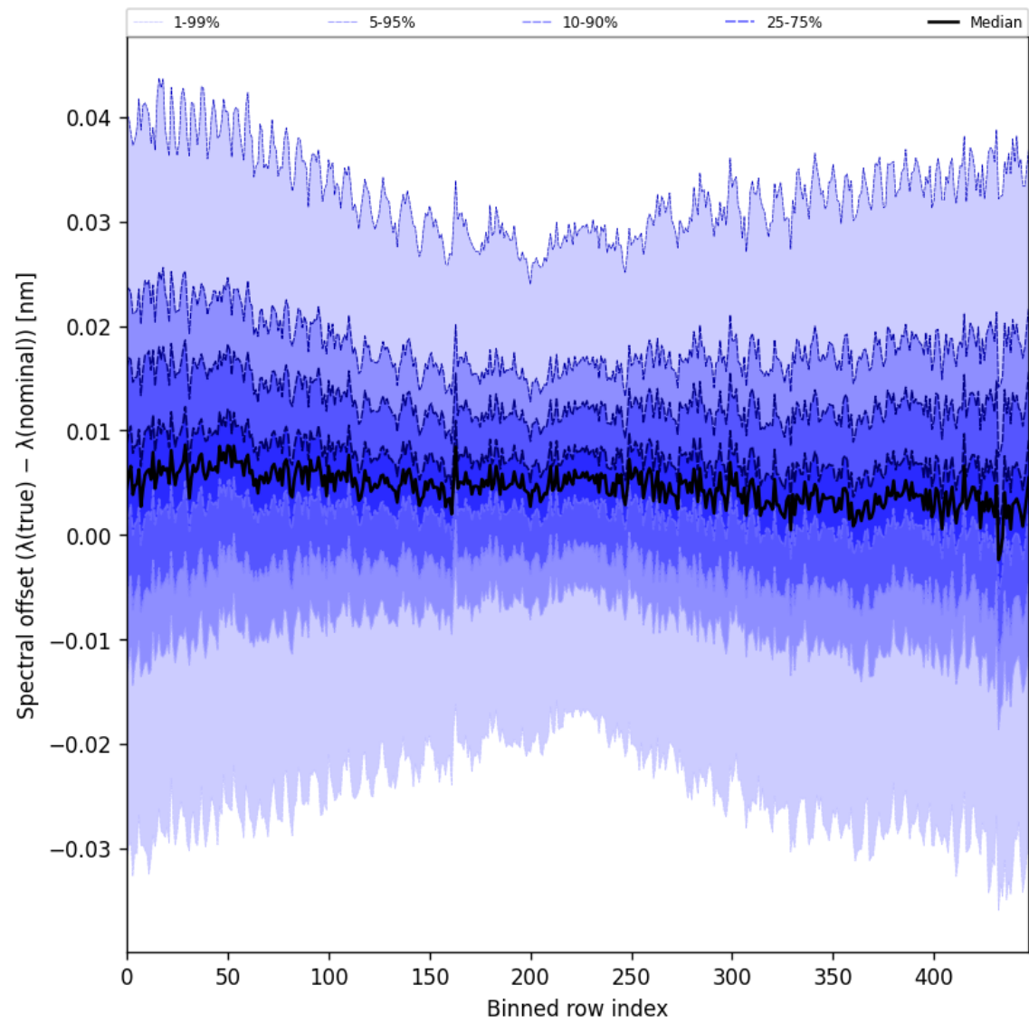
Figure 62: Along track statistics of “Spectral offset ( \lambda_{\text{true}} - \lambda_{\text{nominal}} )” for 2025-07-09 to 2025-07-11
