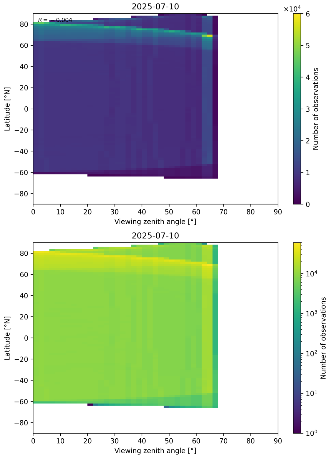
Figure 123: Scatter density plot of “Viewing zenith angle” against “Latitude” for 2025-07-09 to 2025-07-11.
