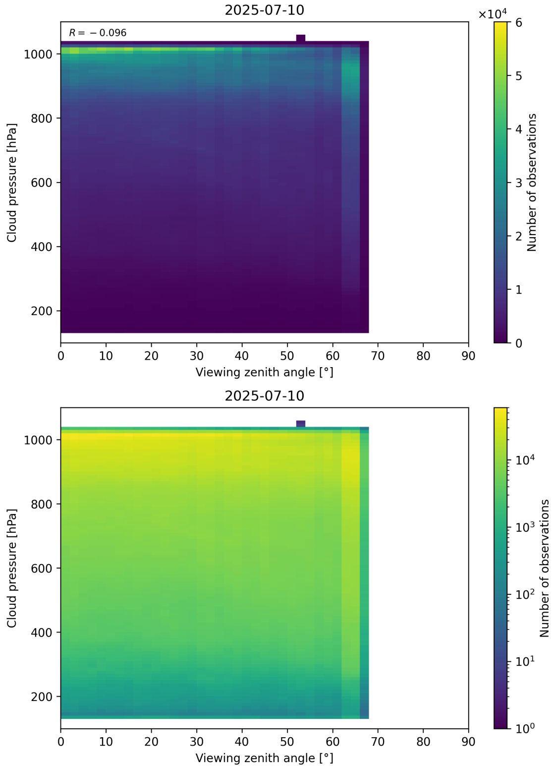
Figure 121: Scatter density plot of “Viewing zenith angle” against “Cloud pressure” for 2025-07-09 to 2025-07-11.
