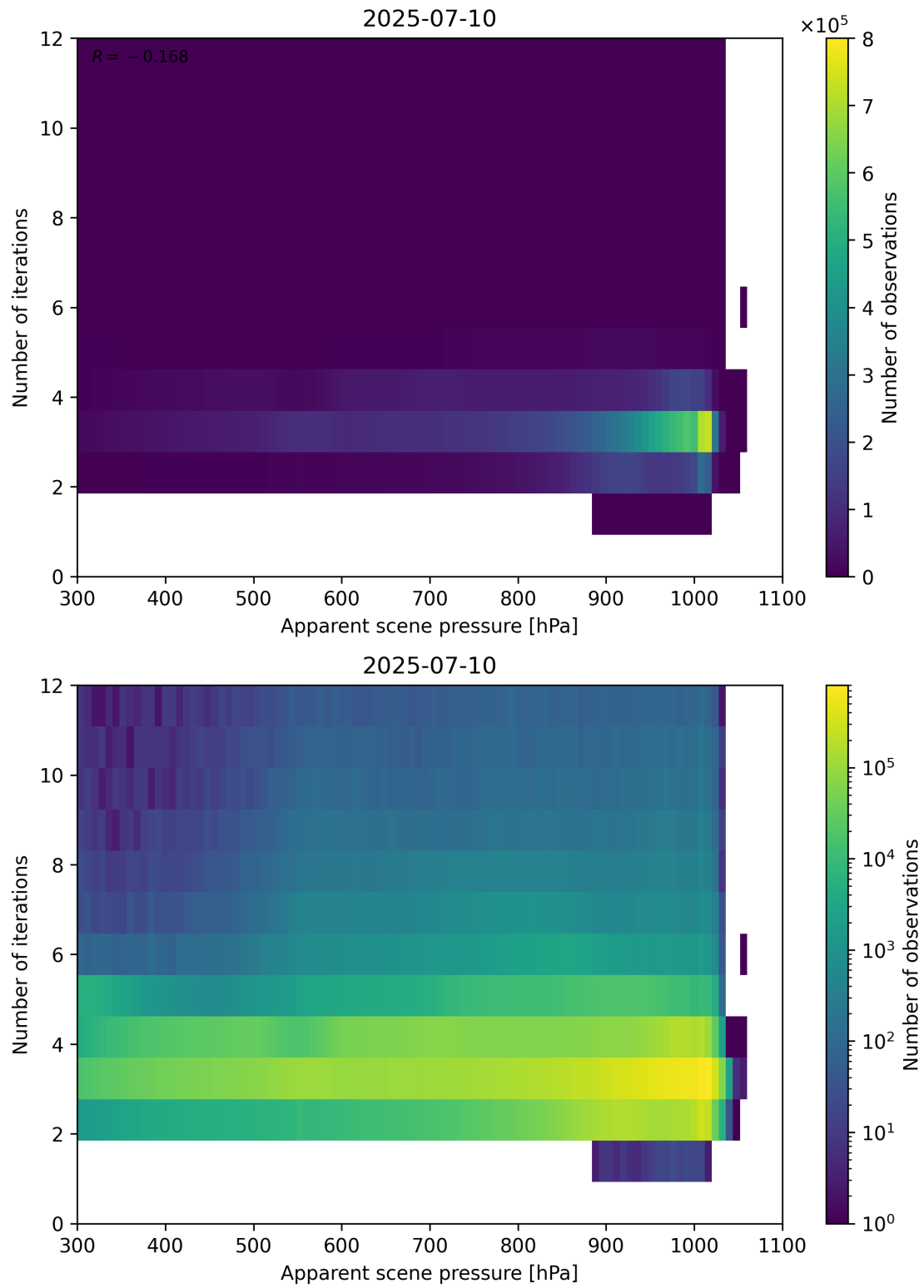
Figure 65: Scatter density plot of “Apparent scene pressure” against “Number of iterations” for 2025-07-09 to 2025-07-11.
