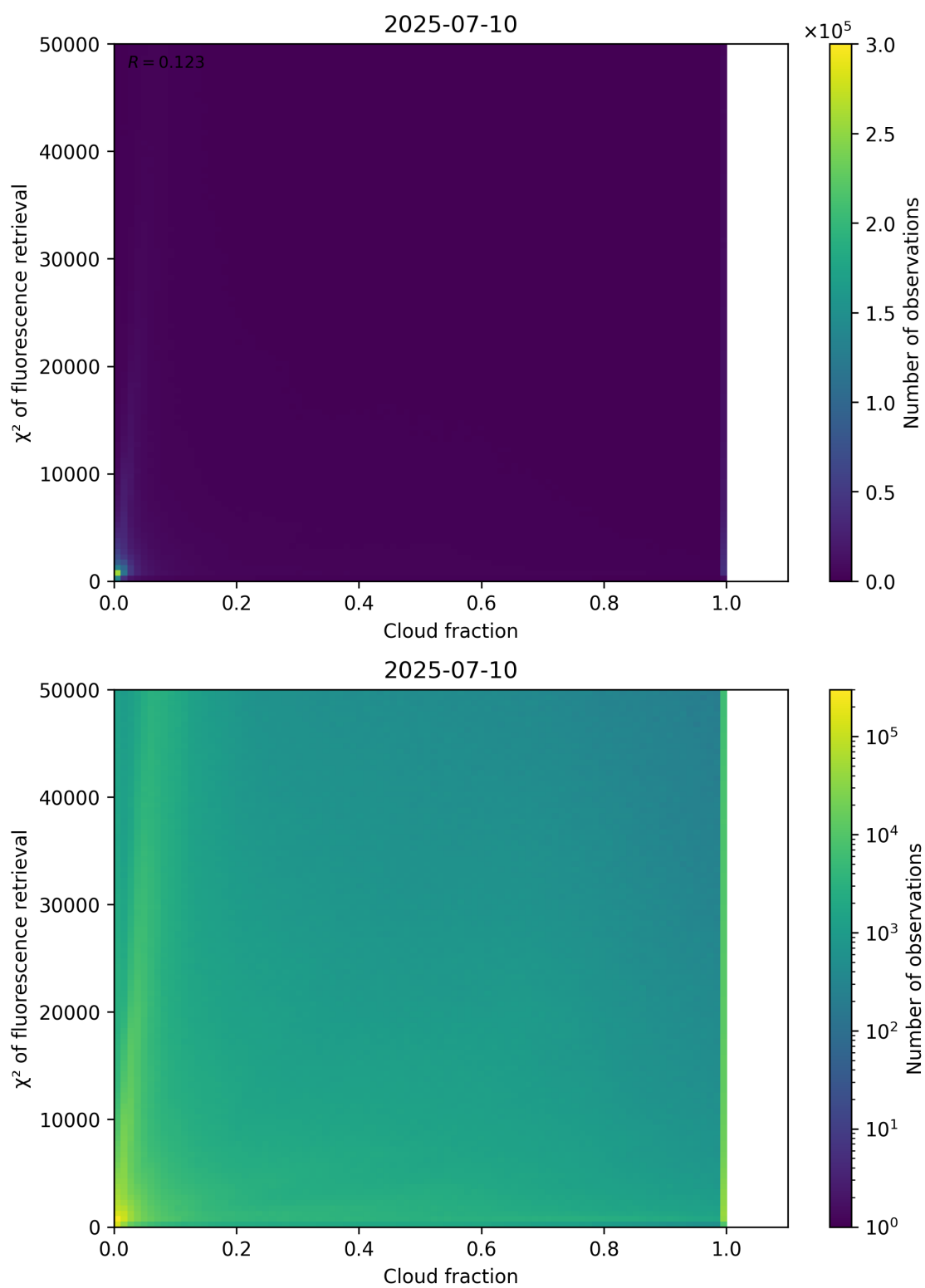
Figure 71: Scatter density plot of “Cloud fraction” against “ \chi^2 of fluorescence retrieval” for 2025-07-09 to 2025-07-11.
