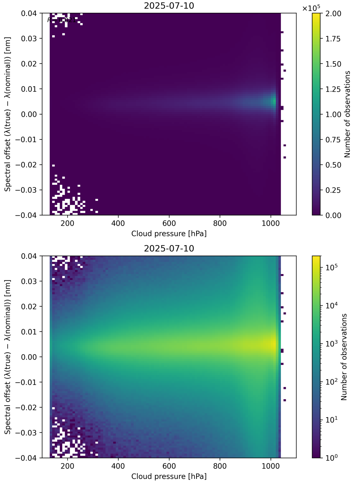
Figure 84: Scatter density plot of “Cloud pressure” against “Spectral offset ( \lambda_{\text{true}} - \lambda_{\text{nominal}} )” for 2025-07-09 to 2025-07-11.
