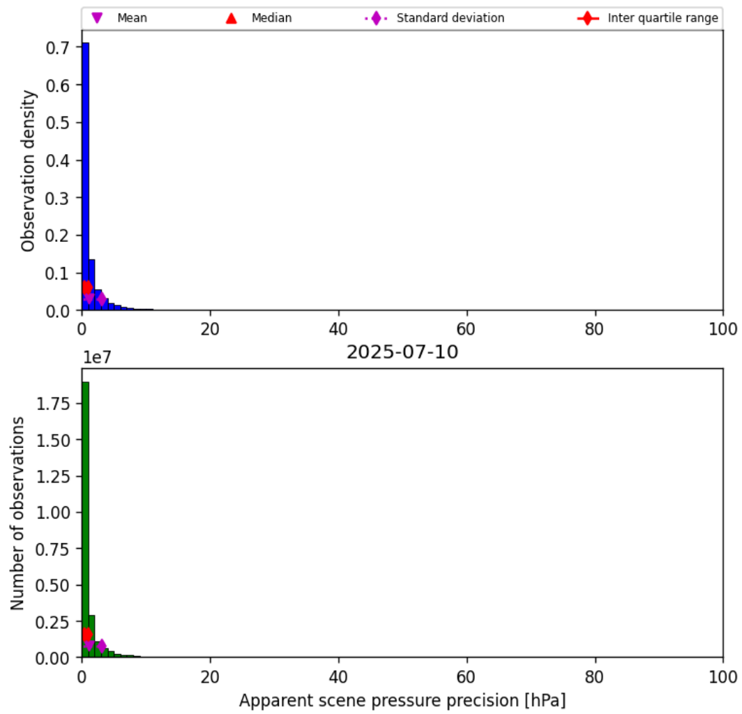
Figure 37: Histogram of “Apparent scene pressure precision” for 2025-07-09 to 2025-07-11
