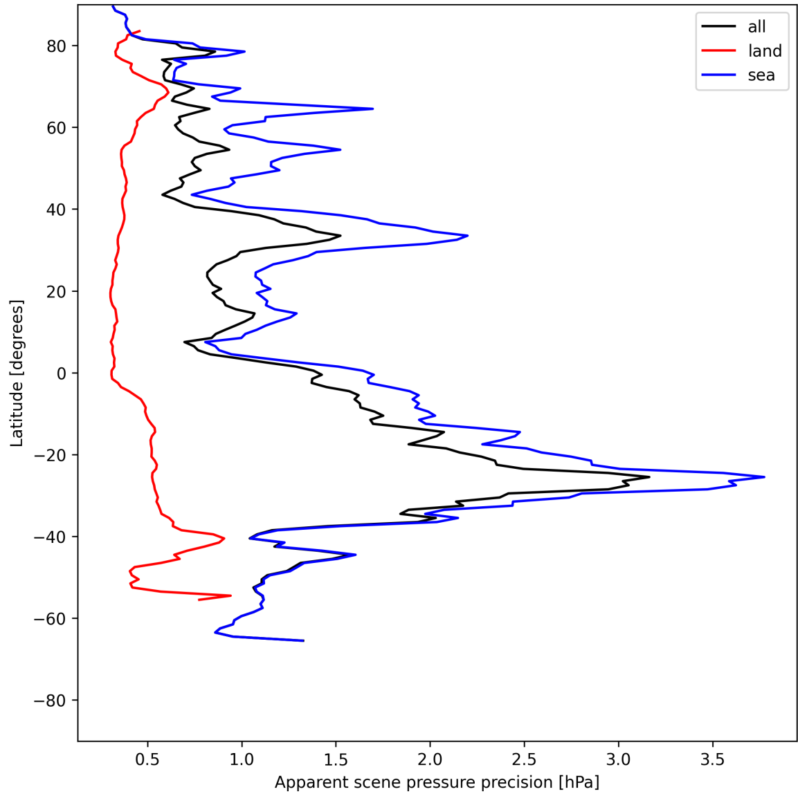
Figure 20: Zonal average of “Apparent scene pressure precision” for 2025-07-09 to 2025-07-11.
