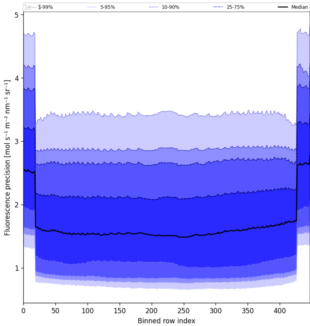
Figure 58: Along track statistics of “Fluorescence precision” for 2025-07-09 to 2025-07-11
