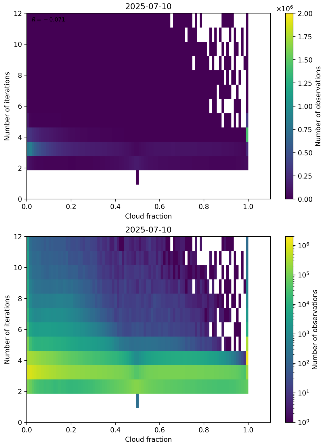
Figure 73: Scatter density plot of “Cloud fraction” against “Number of iterations” for 2025-07-09 to 2025-07-11.
