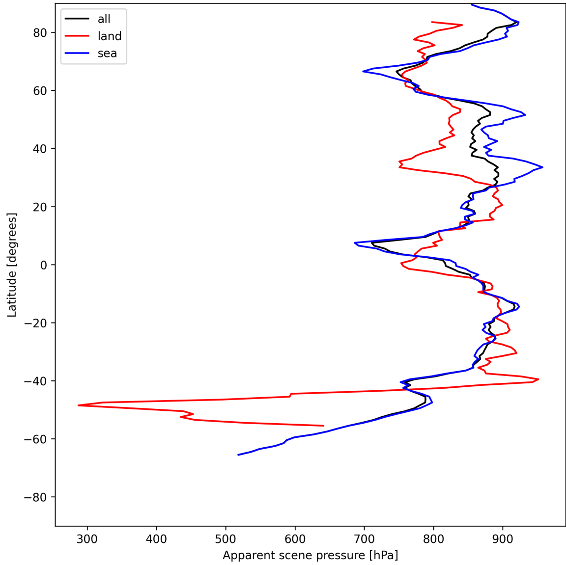
Figure 19: Zonal average of “Apparent scene pressure” for 2025-07-09 to 2025-07-11.
