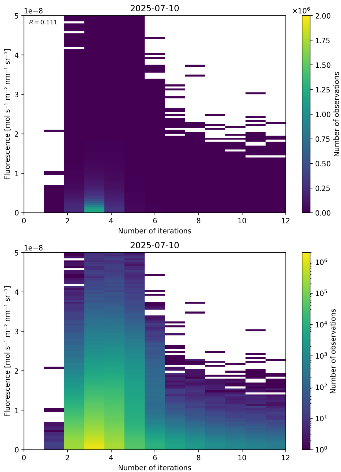
Figure 98: Scatter density plot of “Number of iterations” against “Fluorescence” for 2025-07-09 to 2025-07-11.
