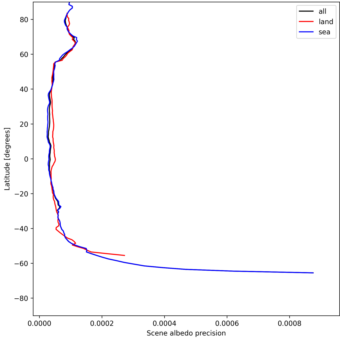
Figure 18: Zonal average of “Scene albedo precision” for 2025-07-09 to 2025-07-11.
