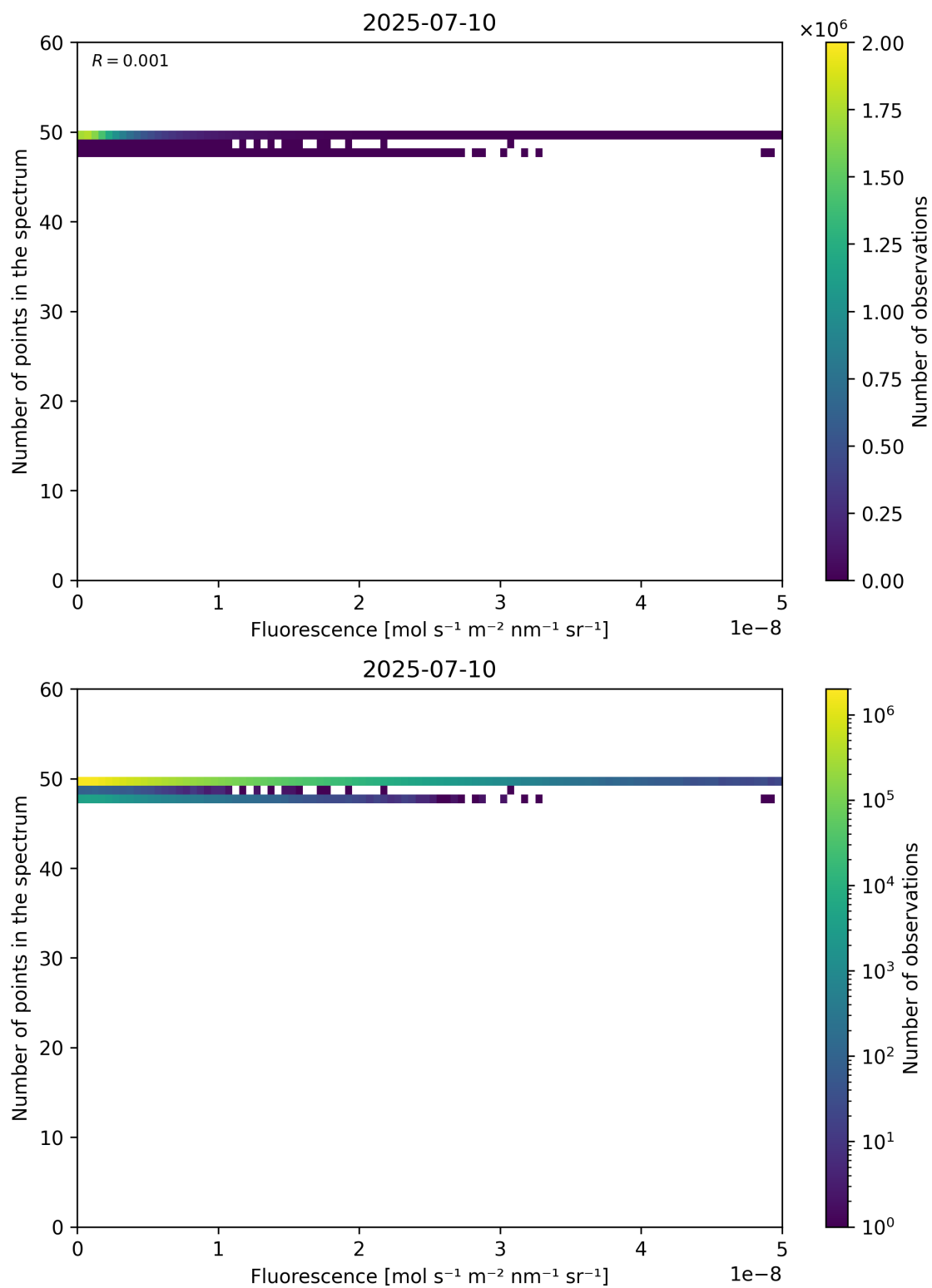
Figure 86: Scatter density plot of “Fluorescence” against “Number of points in the spectrum” for 2025-07-09 to 2025-07-11.
