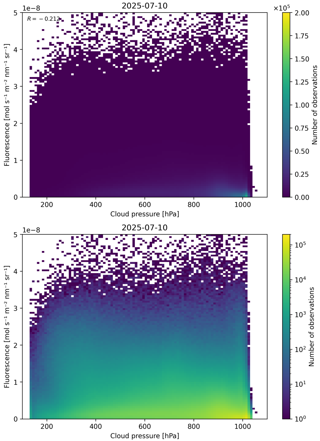
Figure 80: Scatter density plot of “Cloud pressure” against “Fluorescence” for 2025-07-09 to 2025-07-11.
