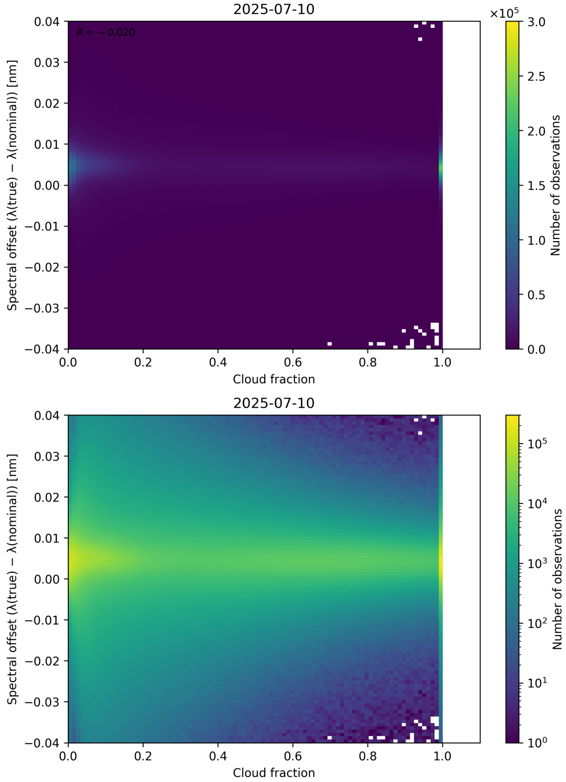
Figure 76: Scatter density plot of “Cloud fraction” against “Spectral offset ( \lambda_{\text{true}} - \lambda_{\text{nominal}} )” for 2025-07-09 to 2025-07-11.
