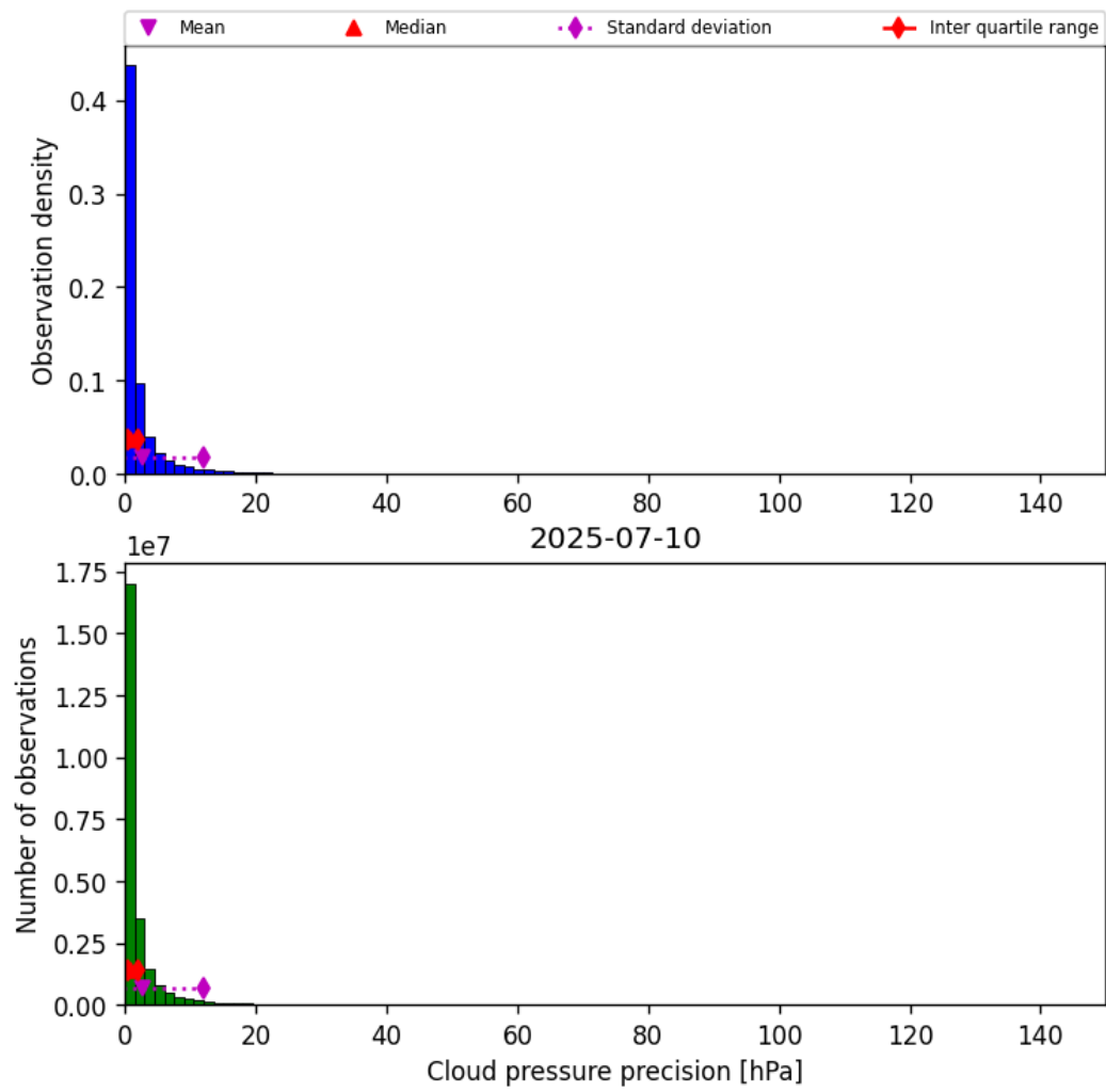
Figure 31: Histogram of “Cloud pressure precision” for 2025-07-09 to 2025-07-11
