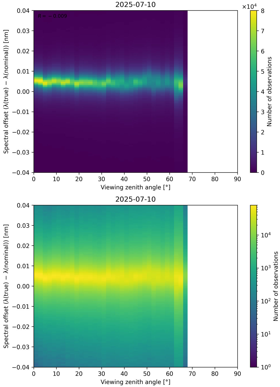
Figure 128: Scatter density plot of “Viewing zenith angle” against “Spectral offset ( \lambda_{\text{true}} - \lambda_{\text{nominal}} )” for 2025-07-09 to 2025-07-11.
