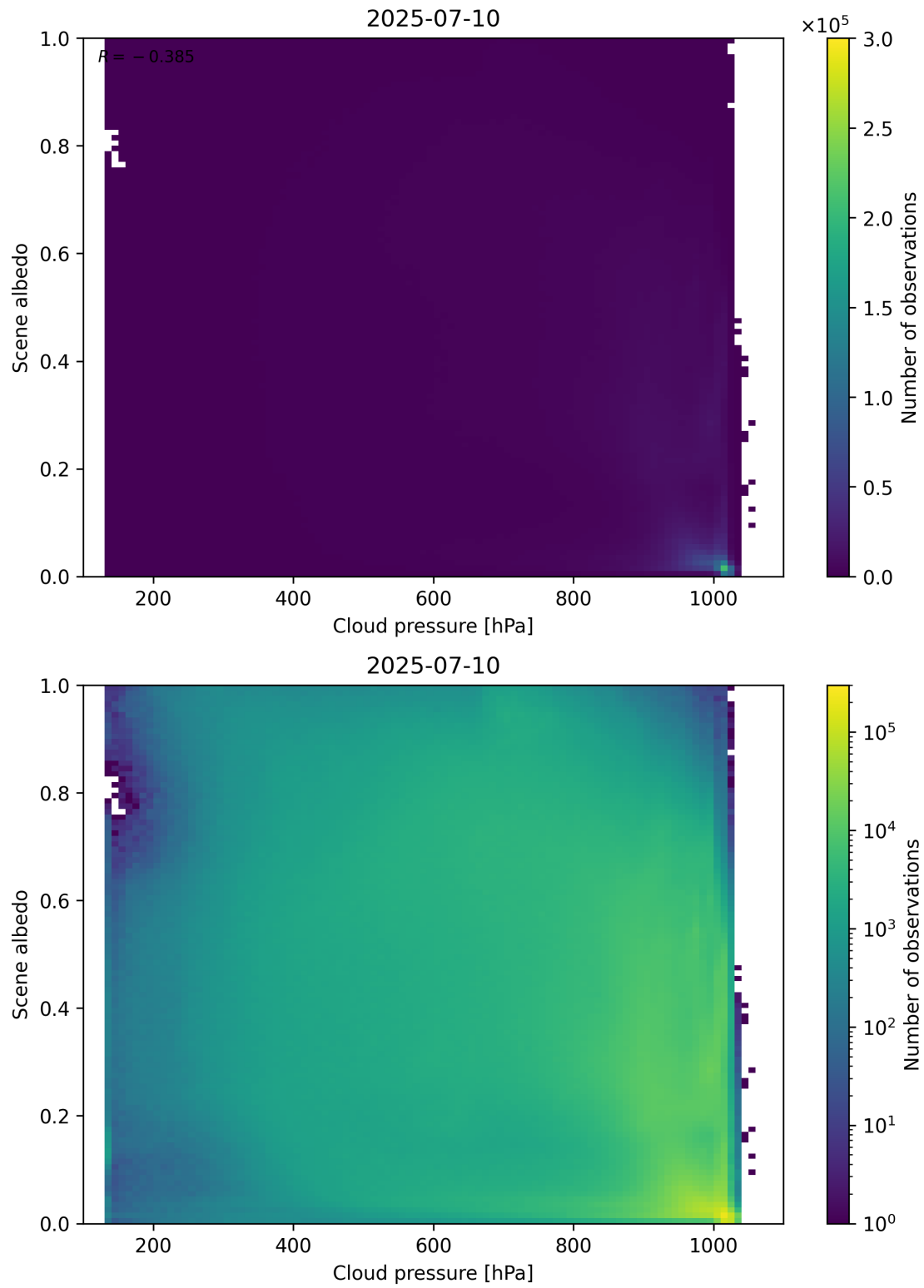
Figure 83: Scatter density plot of “Cloud pressure” against “Scene albedo” for 2025-07-09 to 2025-07-11.
