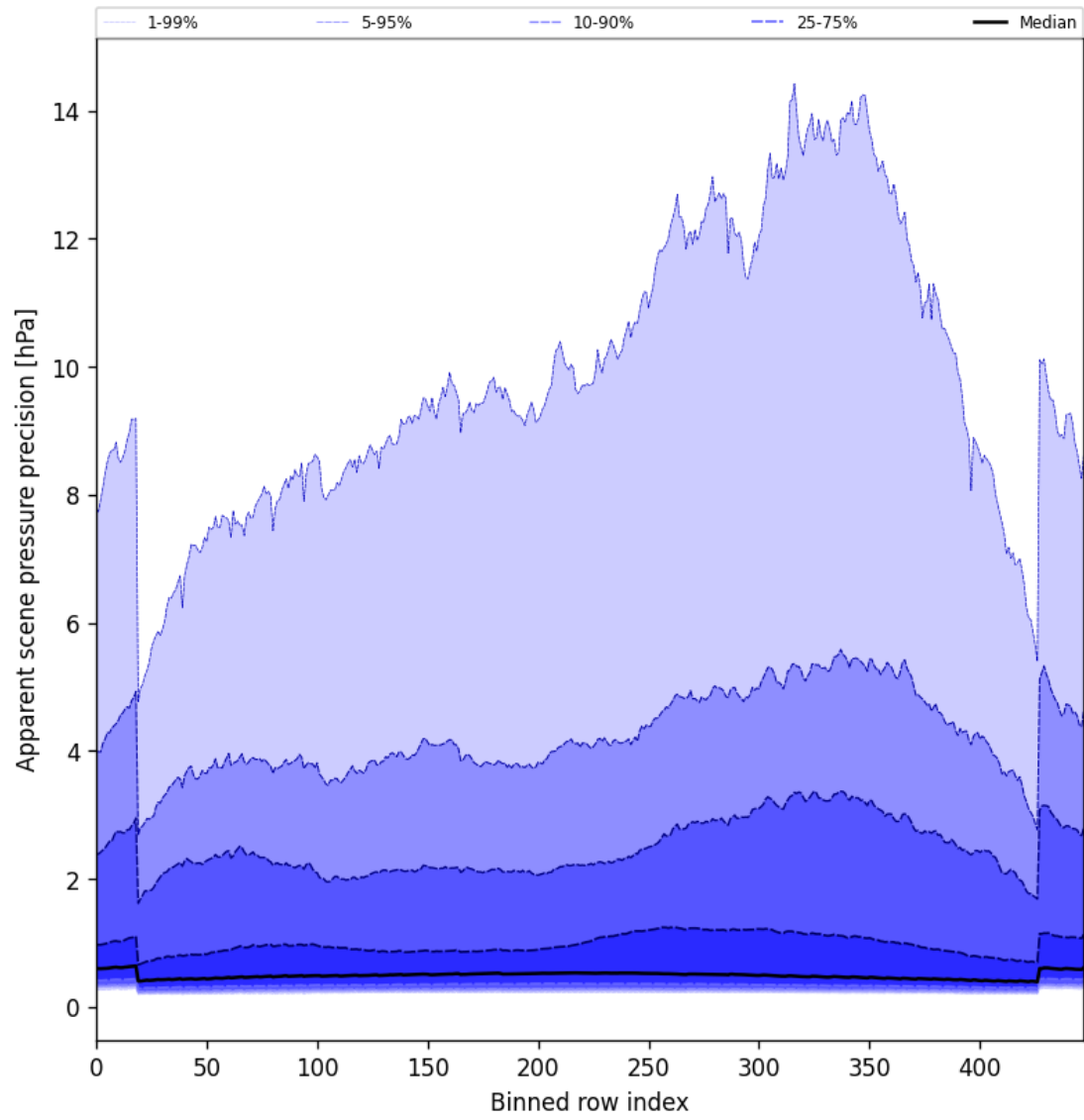
Figure 54: Along track statistics of “Apparent scene pressure precision” for 2025-07-09 to 2025-07-11
