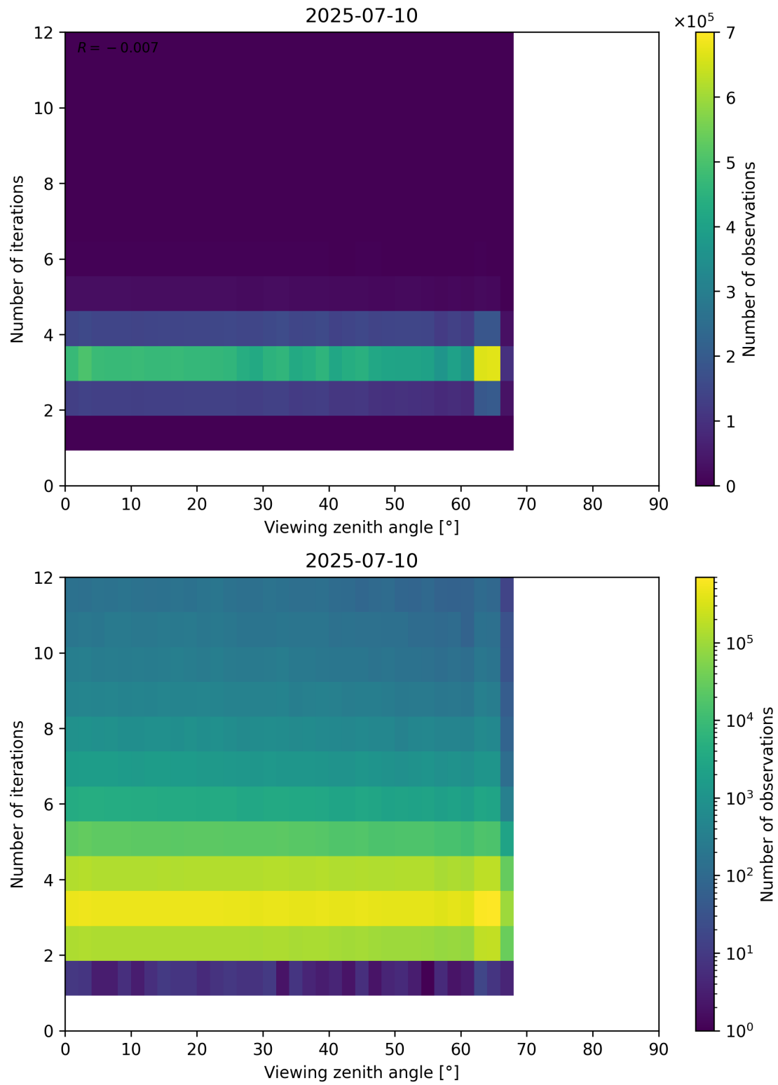
Figure 124: Scatter density plot of “Viewing zenith angle” against “Number of iterations” for 2025-07-09 to 2025-07-11.
