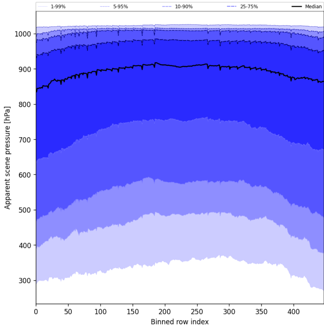
Figure 53: Along track statistics of “Apparent scene pressure” for 2025-07-09 to 2025-07-11
