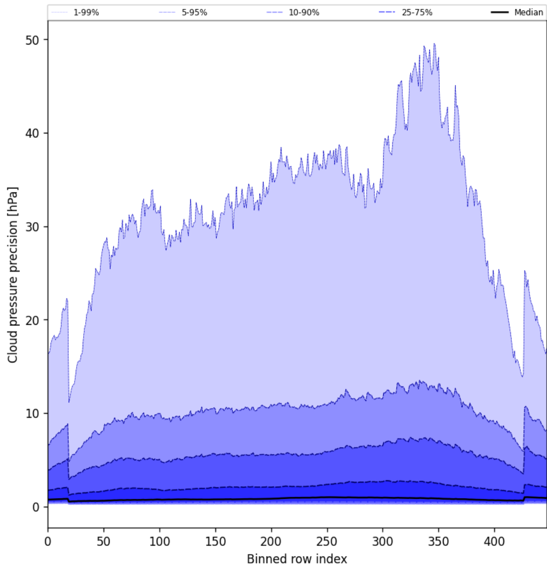
Figure 48: Along track statistics of “Cloud pressure precision” for 2025-07-09 to 2025-07-11
