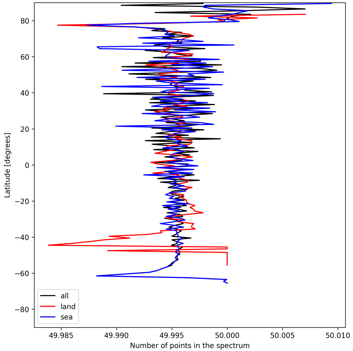
Figure 27: Zonal average of “Number of points in the spectrum” for 2025-07-09 to 2025-07-11.
