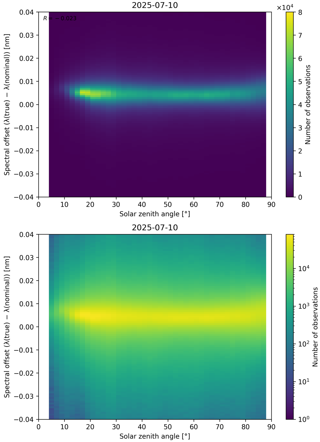
Figure 117: Scatter density plot of “Solar zenith angle” against “Spectral offset ( \lambda_{\text{true}} - \lambda_{\text{nominal}} )” for 2025-07-09 to 2025-07-11.
