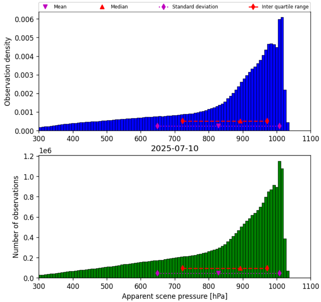
Figure 36: Histogram of “Apparent scene pressure” for 2025-07-09 to 2025-07-11
