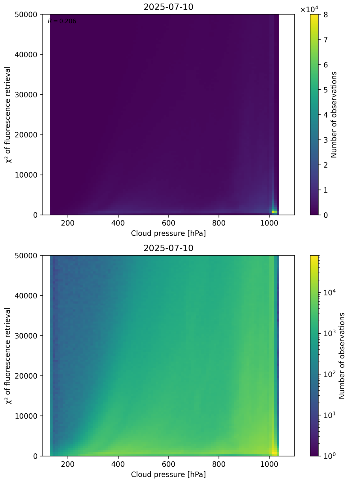
Figure 78: Scatter density plot of “Cloud pressure” against “ \chi^2 of fluorescence retrieval” for 2025-07-09 to 2025-07-11.
