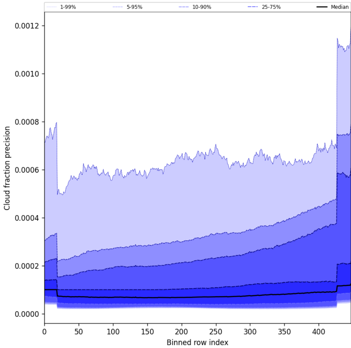
Figure 50: Along track statistics of “Cloud fraction precision” for 2025-07-09 to 2025-07-11
