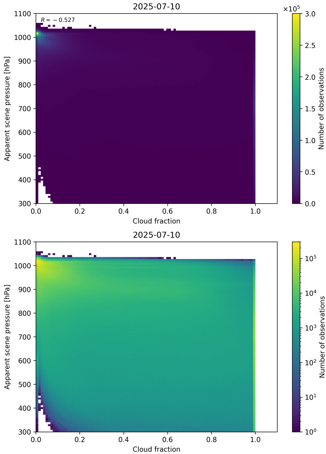
Figure 70: Scatter density plot of “Cloud fraction” against “Apparent scene pressure” for 2025-07-09 to 2025-07-11.
