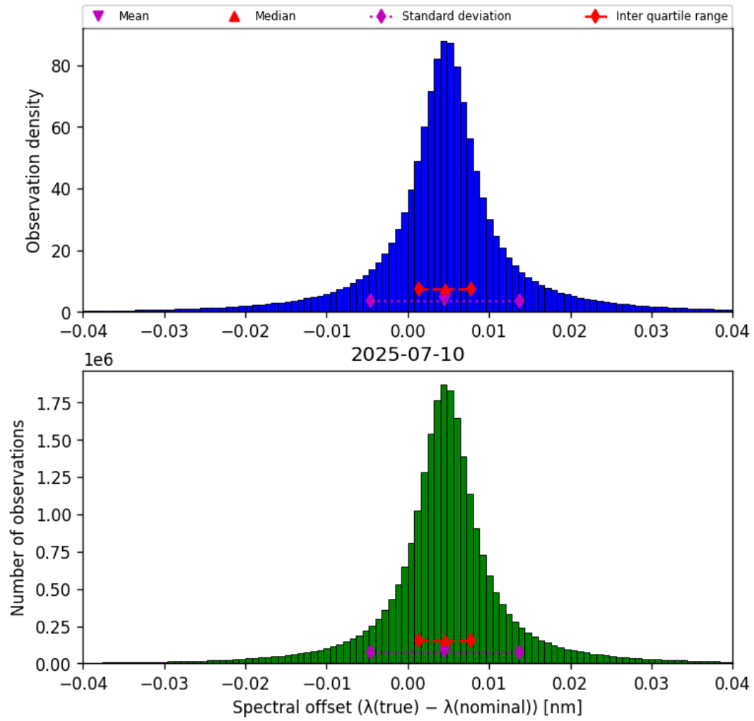
Figure 45: Histogram of “Spectral offset ( \lambda_{\text{true}} - \lambda_{\text{nominal}} )” for 2025-07-09 to 2025-07-11
