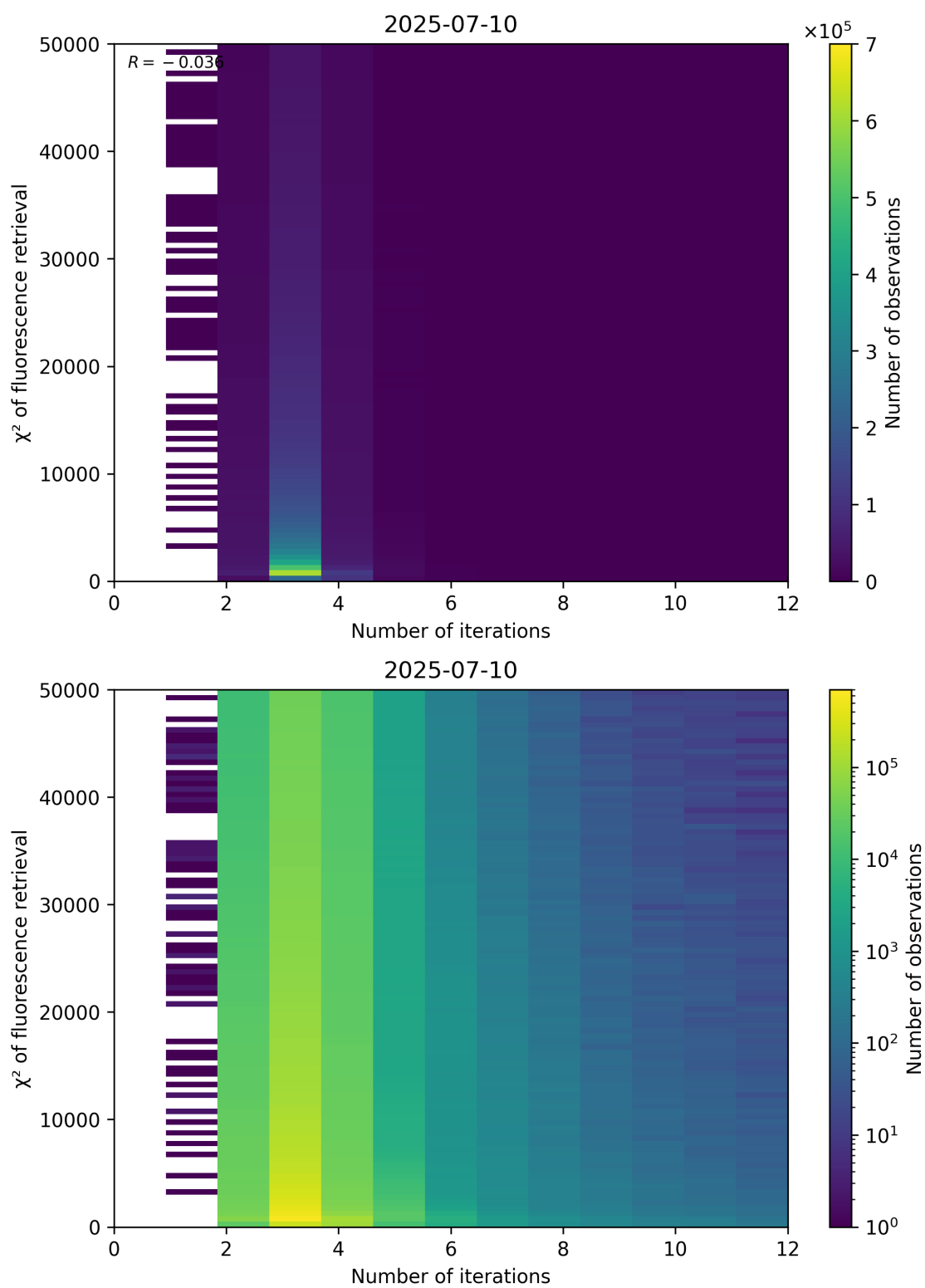
Figure 97: Scatter density plot of “Number of iterations” against “ \chi^2 of fluorescence retrieval” for 2025-07-09 to 2025-07-11.
