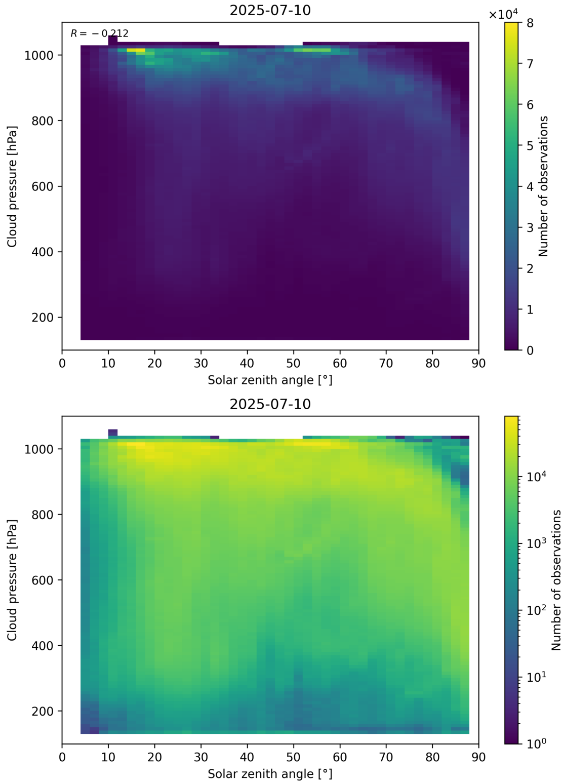
Figure 111: Scatter density plot of “Solar zenith angle” against “Cloud pressure” for 2025-07-09 to 2025-07-11.
