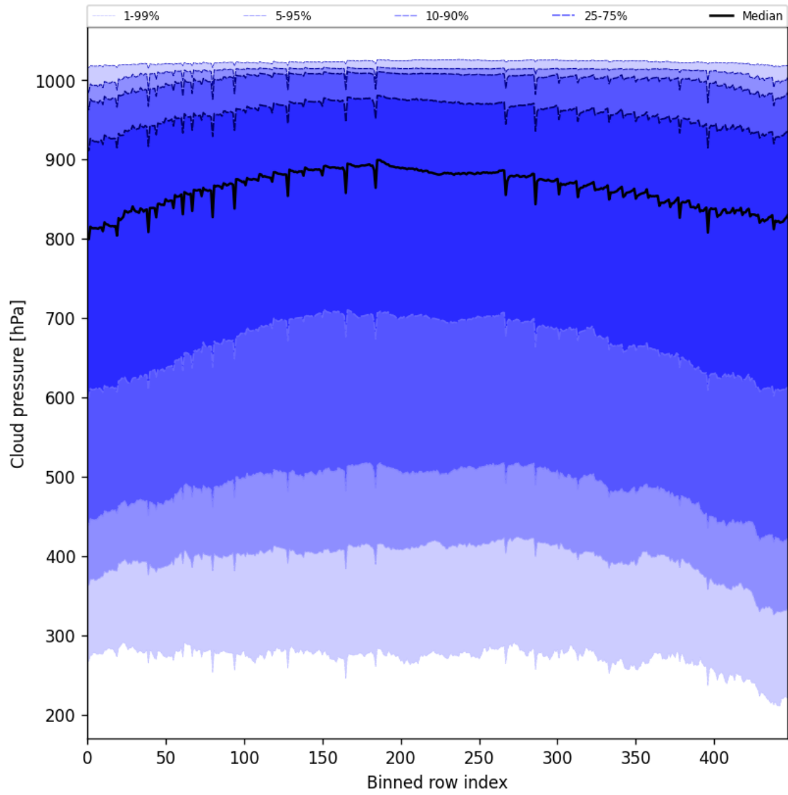
Figure 47: Along track statistics of “Cloud pressure” for 2025-07-09 to 2025-07-11
