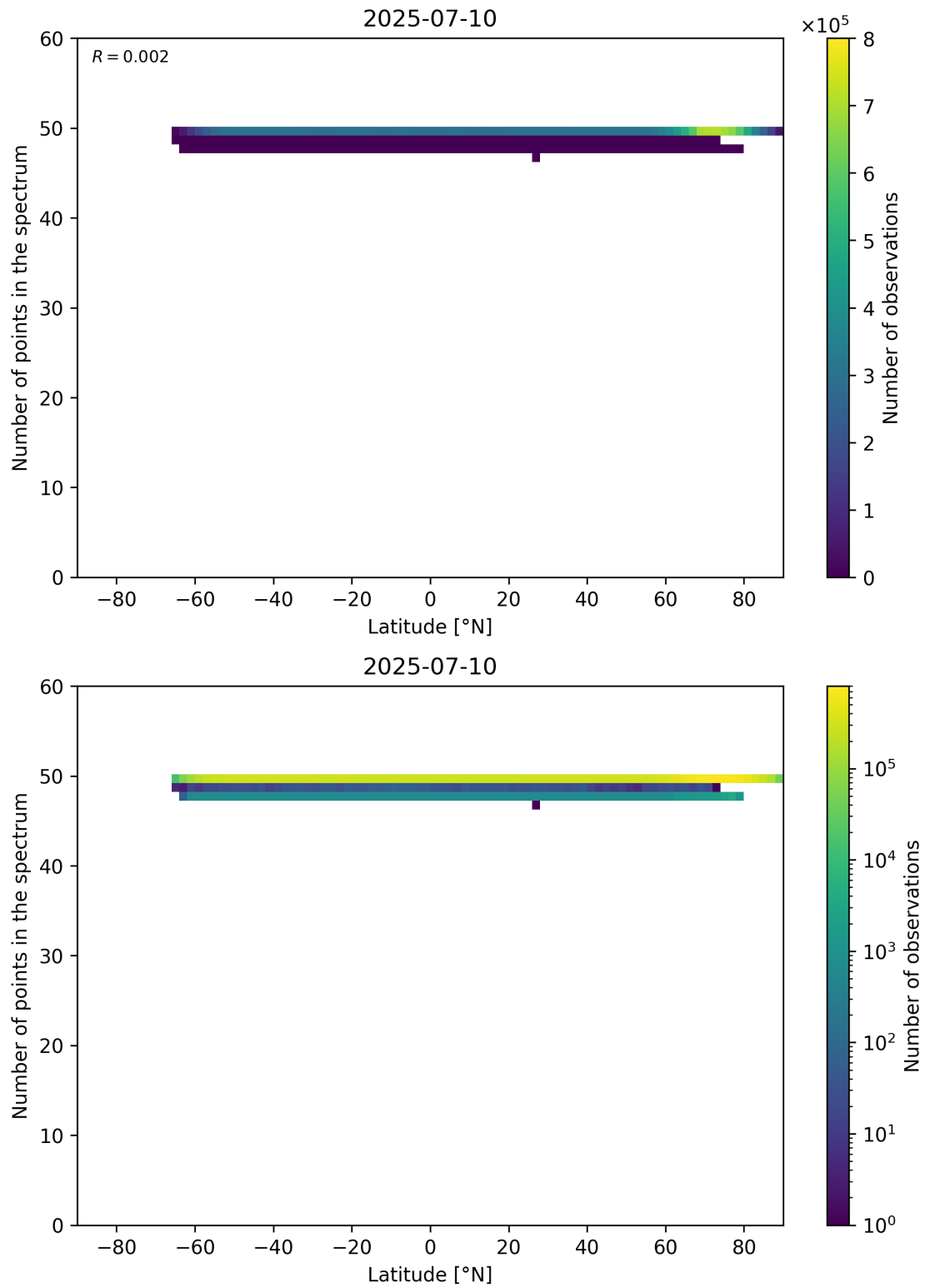
Figure 94: Scatter density plot of “Latitude” against “Number of points in the spectrum” for 2025-07-09 to 2025-07-11.
