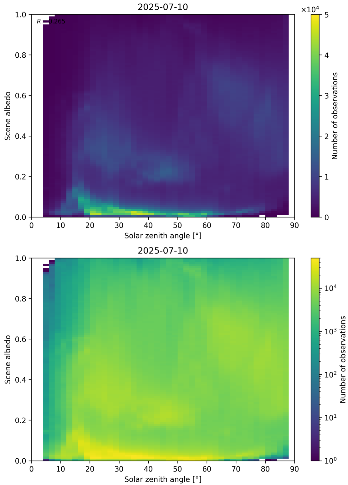
Figure 116: Scatter density plot of “Solar zenith angle” against “Scene albedo” for 2025-07-09 to 2025-07-11.
