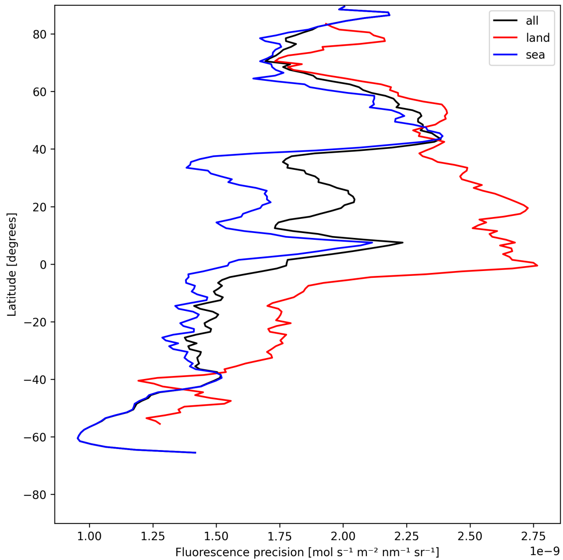
Figure 24: Zonal average of “Fluorescence precision” for 2025-07-09 to 2025-07-11.
