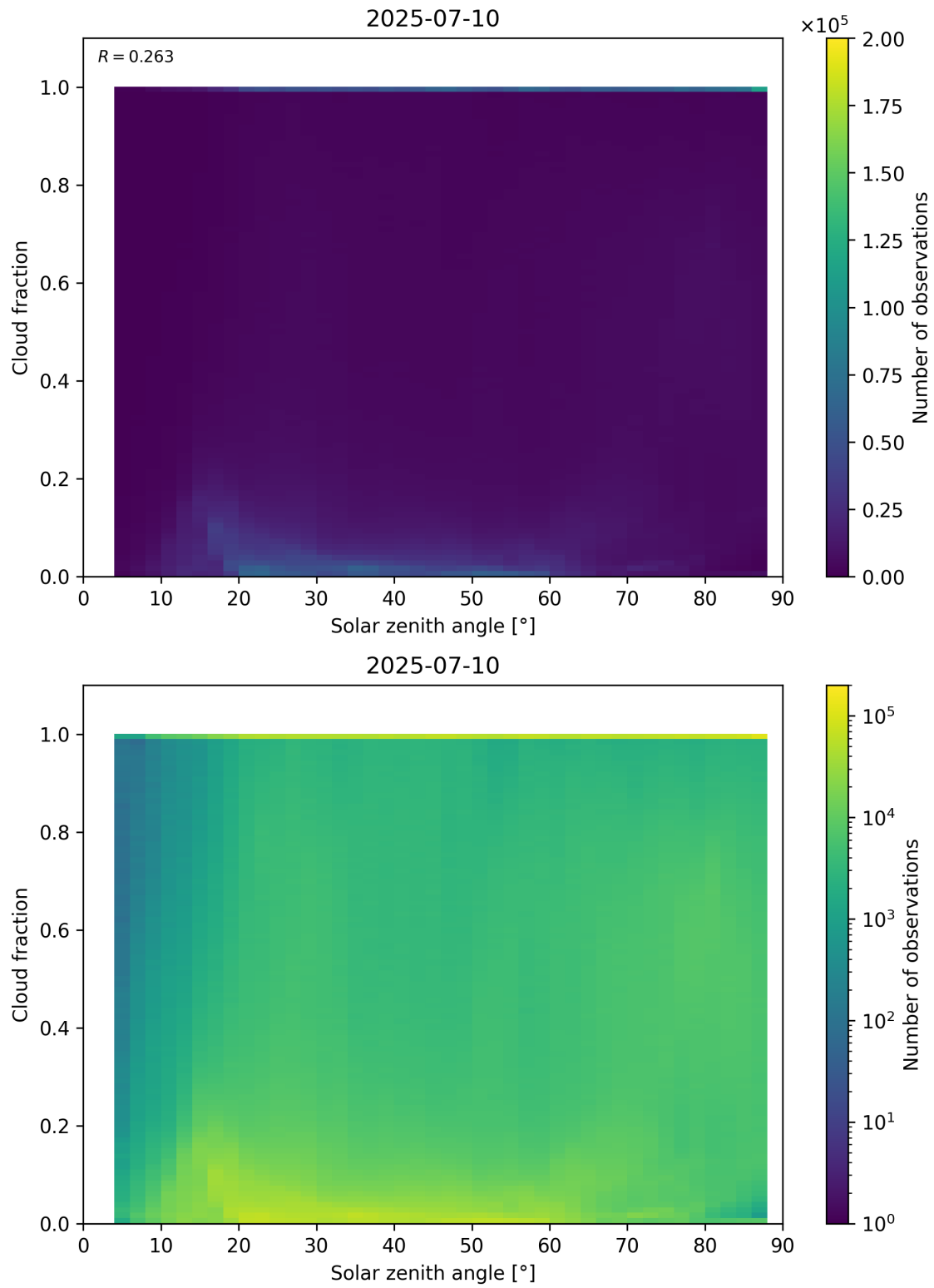
Figure 110: Scatter density plot of “Solar zenith angle” against “Cloud fraction” for 2025-07-09 to 2025-07-11.
