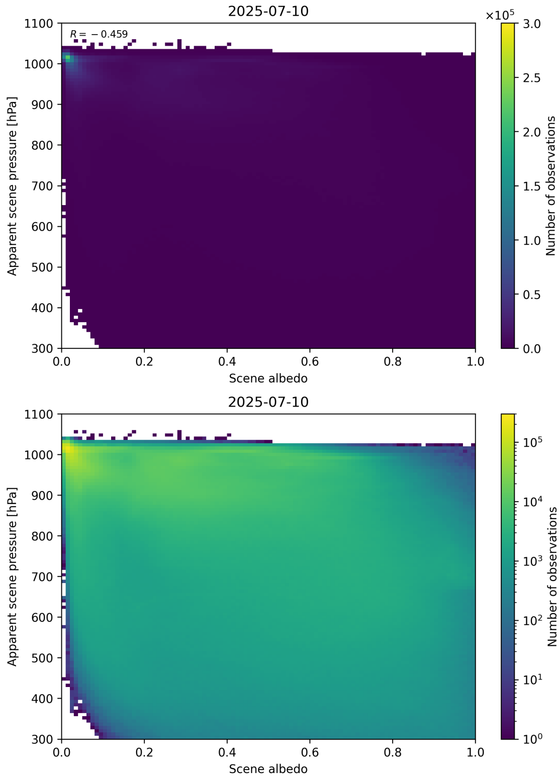
Figure 102: Scatter density plot of “Scene albedo” against “Apparent scene pressure” for 2025-07-09 to 2025-07-11.
