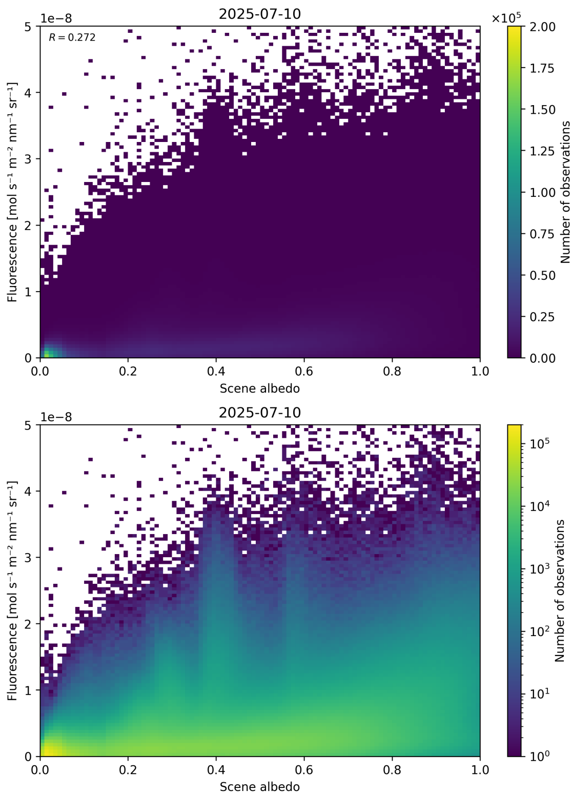
Figure 104: Scatter density plot of “Scene albedo” against “Fluorescence” for 2025-07-09 to 2025-07-11.
