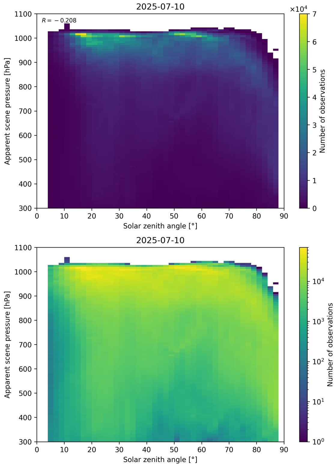
Figure 108: Scatter density plot of “Solar zenith angle” against “Apparent scene pressure” for 2025-07-09 to 2025-07-11.
