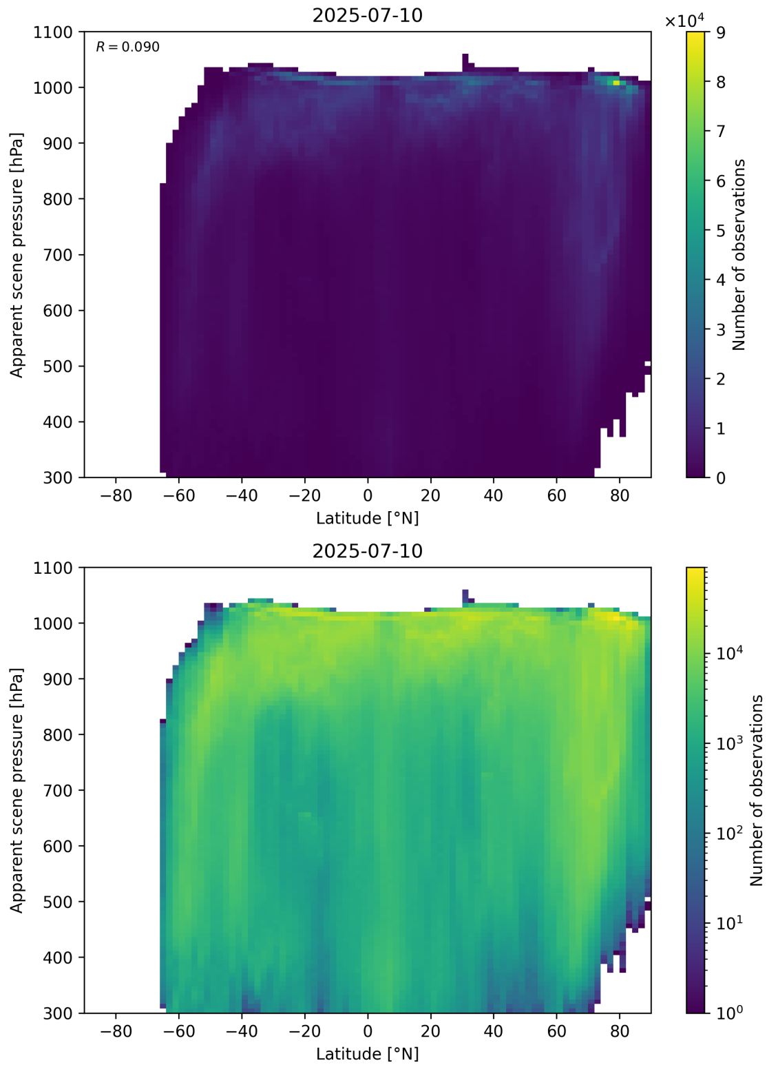
Figure 88: Scatter density plot of “Latitude” against “Apparent scene pressure” for 2025-07-09 to 2025-07-11.
