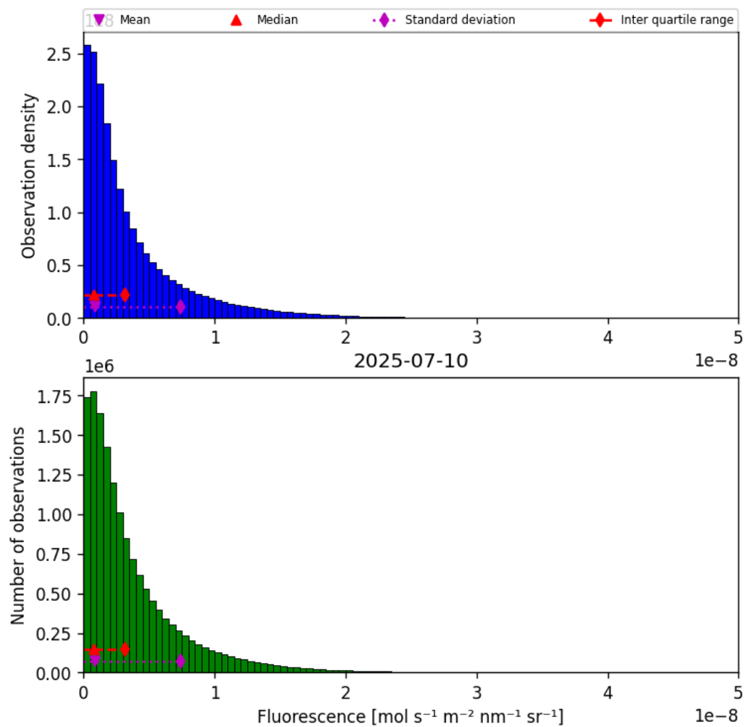
Figure 40: Histogram of “Fluorescence” for 2025-07-09 to 2025-07-11
