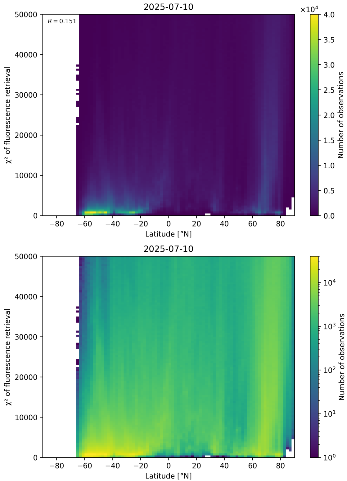
Figure 89: Scatter density plot of “Latitude” against “ \chi^2 of fluorescence retrieval” for 2025-07-09 to 2025-07-11.
