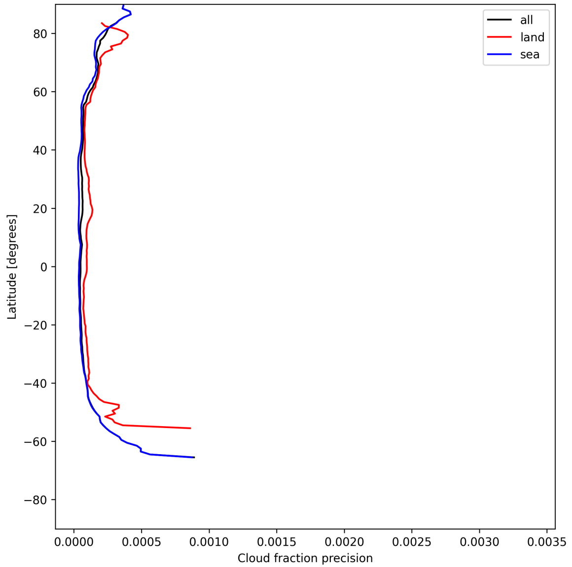
Figure 16: Zonal average of “Cloud fraction precision” for 2025-07-09 to 2025-07-11.
