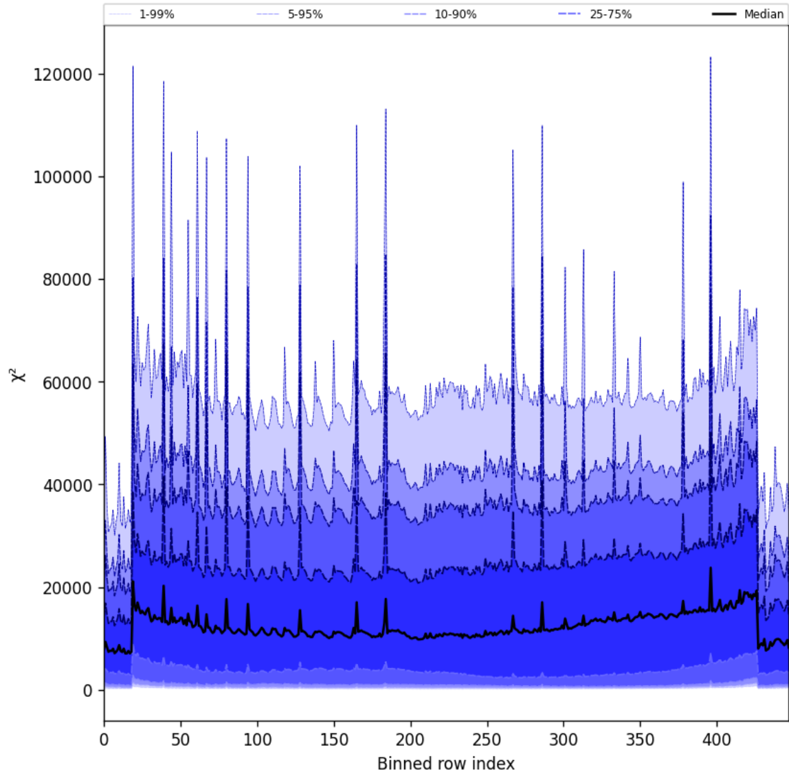
Figure 55: Along track statistics of “ \chi^2 ” for 2025-07-09 to 2025-07-11
