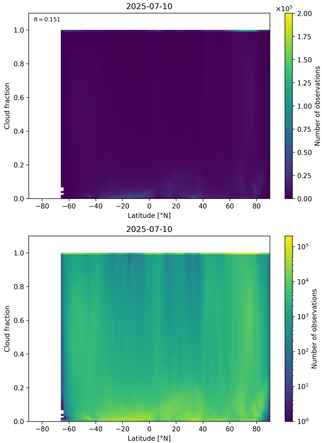
Figure 90: Scatter density plot of “Latitude” against “Cloud fraction” for 2025-07-09 to 2025-07-11.
