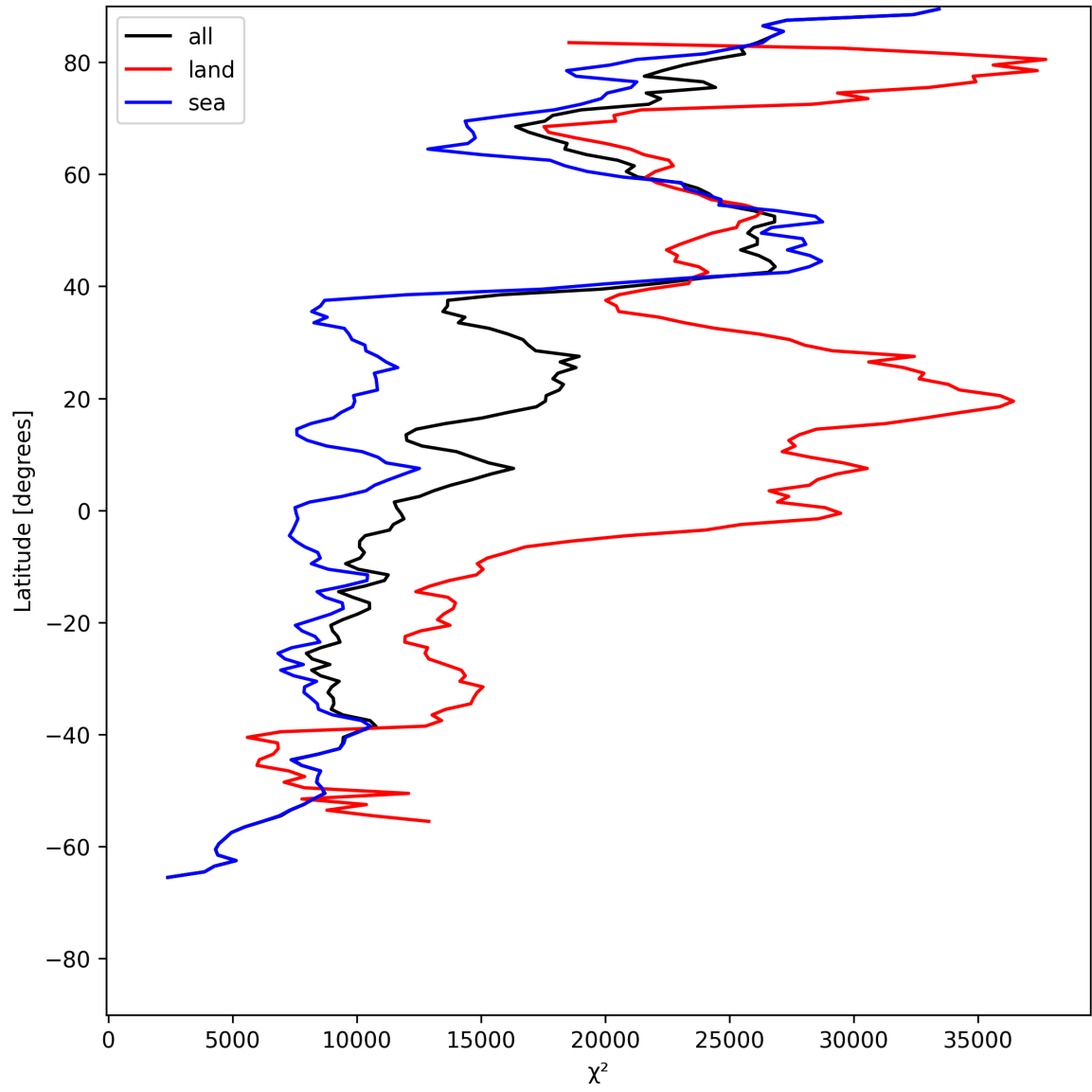
Figure 21: Zonal average of “ \chi^2 ” for 2025-07-09 to 2025-07-11.
