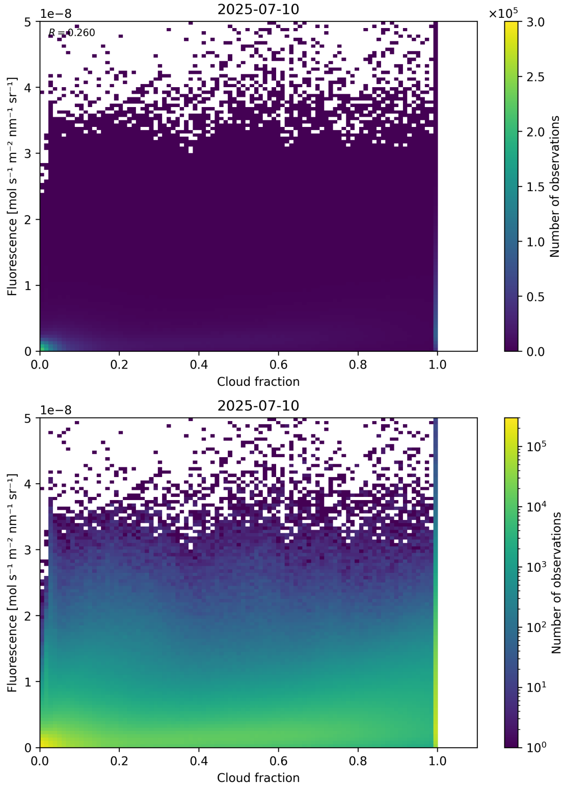
Figure 72: Scatter density plot of “Cloud fraction” against “Fluorescence” for 2025-07-09 to 2025-07-11.
