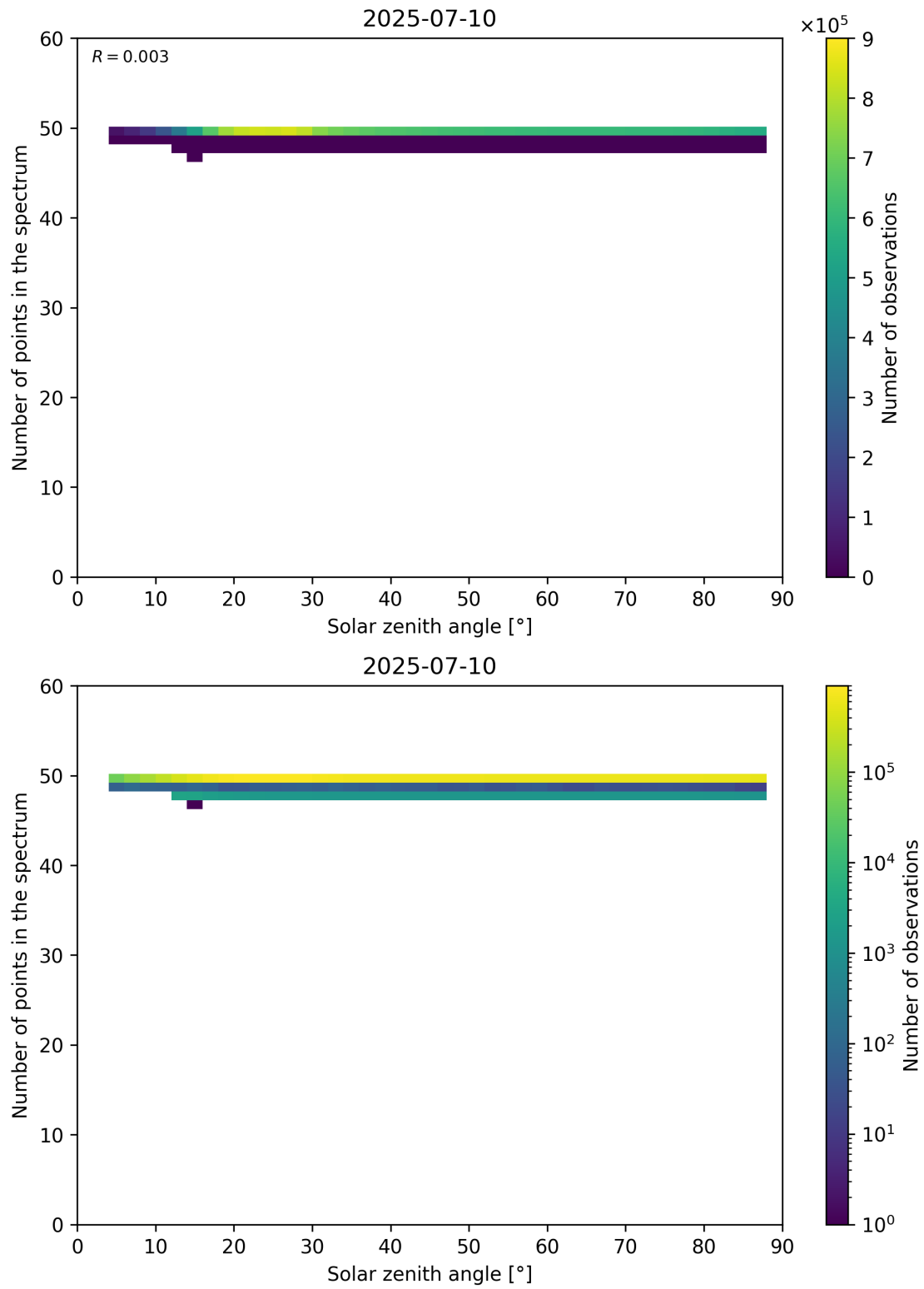
Figure 115: Scatter density plot of “Solar zenith angle” against “Number of points in the spectrum” for 2025-07-09 to 2025-07-11.
