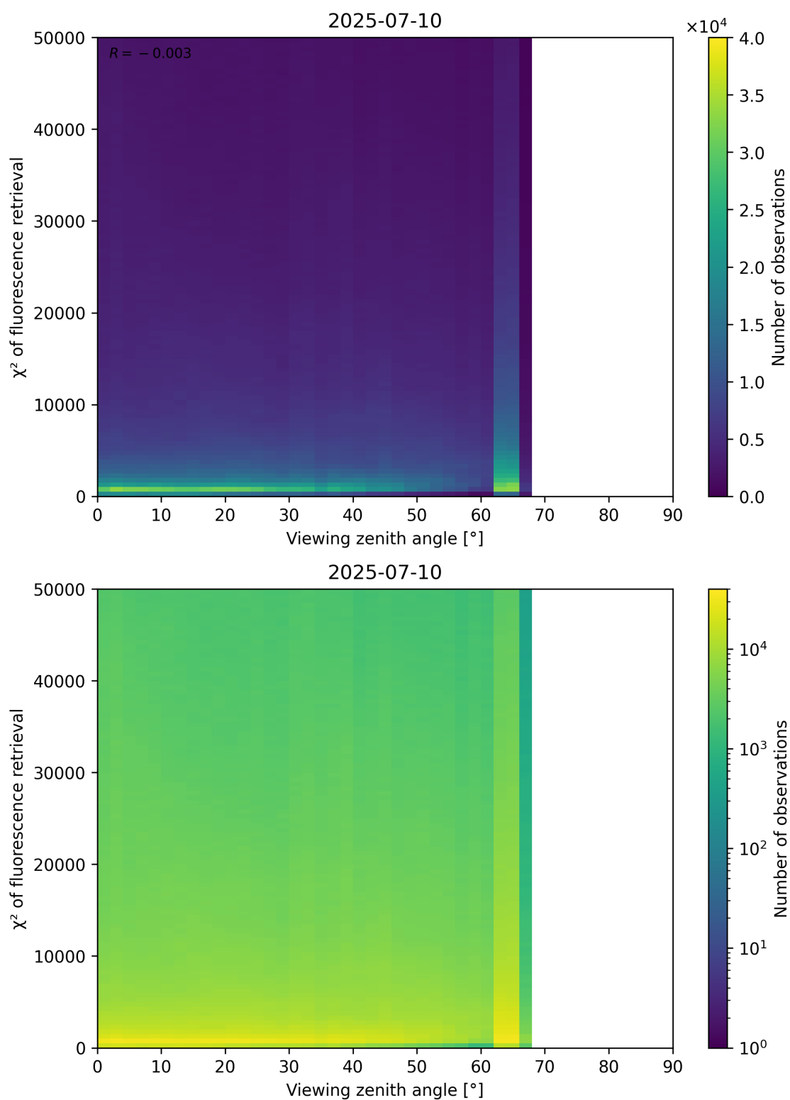
Figure 119: Scatter density plot of “Viewing zenith angle” against “ \chi^2 of fluorescence retrieval” for 2025-07-09 to 2025-07-11.
