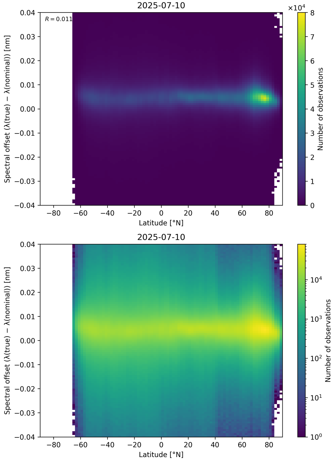
Figure 96: Scatter density plot of “Latitude” against “Spectral offset ( \lambda_{\text{true}} - \lambda_{\text{nominal}} )” for 2025-07-09 to 2025-07-11.
