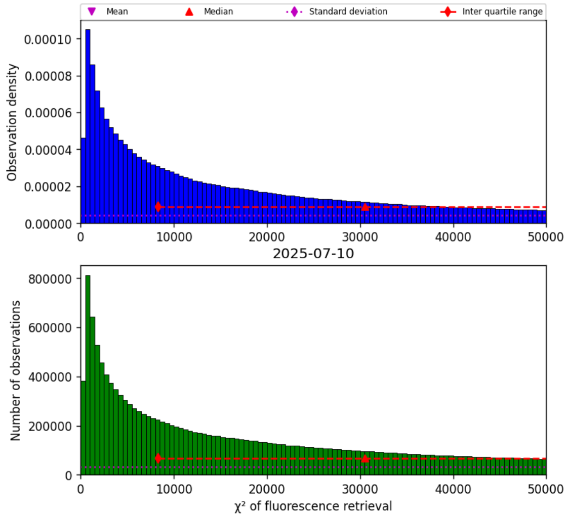
Figure 42: Histogram of “ \chi^2 of fluorescence retrieval” for 2025-07-09 to 2025-07-11
