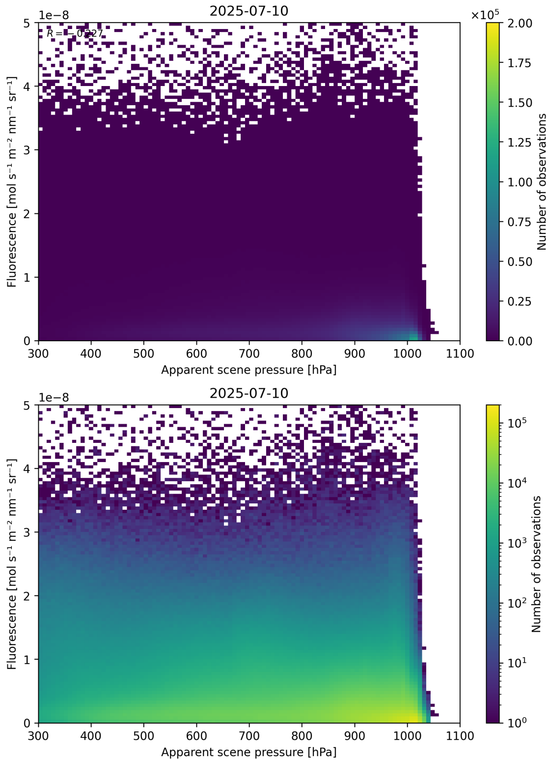
Figure 64: Scatter density plot of “Apparent scene pressure” against “Fluorescence” for 2025-07-09 to 2025-07-11.
