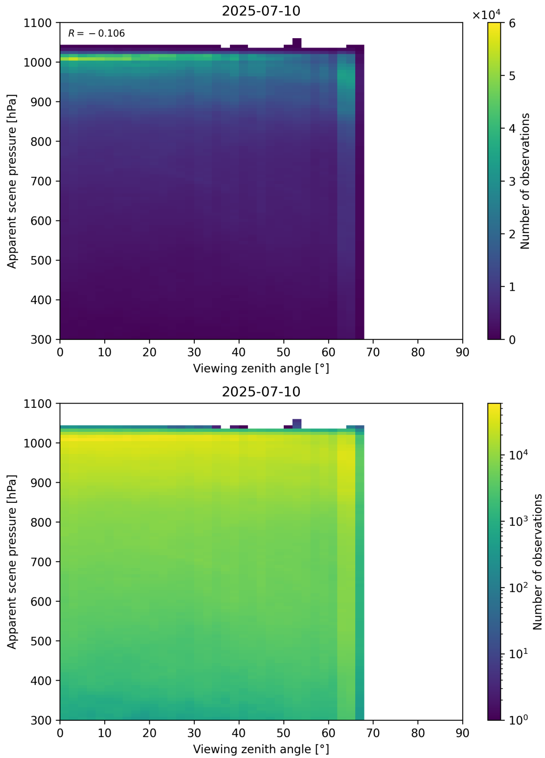
Figure 118: Scatter density plot of “Viewing zenith angle” against “Apparent scene pressure” for 2025-07-09 to 2025-07-11.
