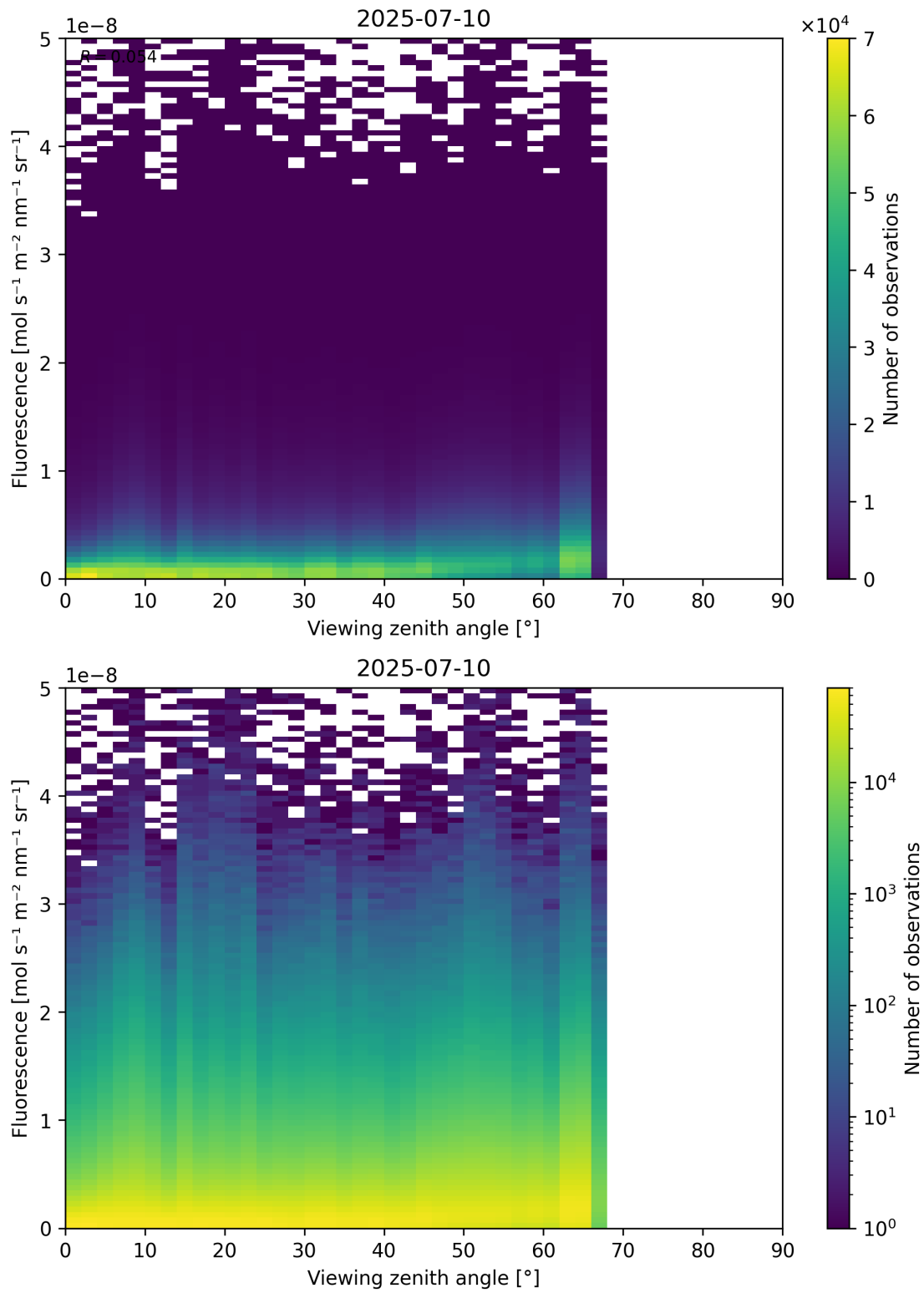
Figure 122: Scatter density plot of “Viewing zenith angle” against “Fluorescence” for 2025-07-09 to 2025-07-11.
