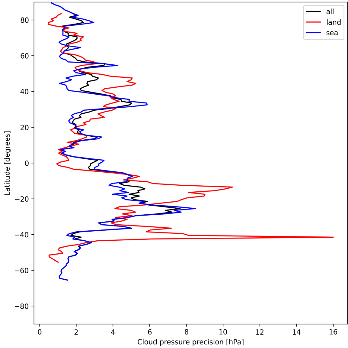
Figure 14: Zonal average of “Cloud pressure precision” for 2025-07-09 to 2025-07-11.
