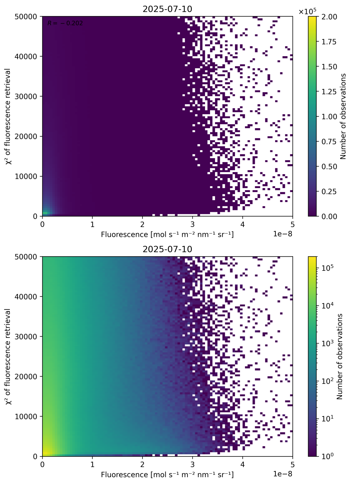
Figure 85: Scatter density plot of “Fluorescence” against “ \chi^2 of fluorescence retrieval” for 2025-07-09 to 2025-07-11.
