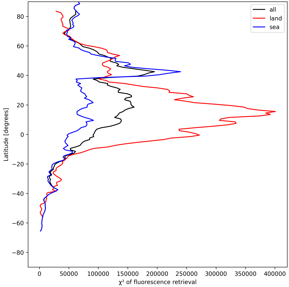
Figure 25: Zonal average of “ \chi^2 of fluorescence retrieval” for 2025-07-09 to 2025-07-11.
