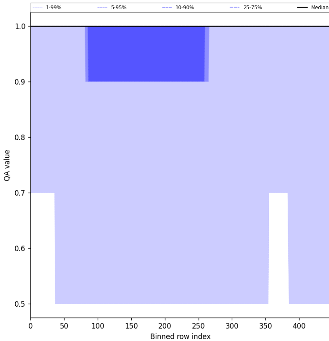
Figure 46: Along track statistics of “QA value” for 2025-07-09 to 2025-07-11
