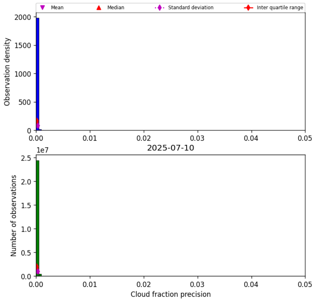
Figure 33: Histogram of “Cloud fraction precision” for 2025-07-09 to 2025-07-11
