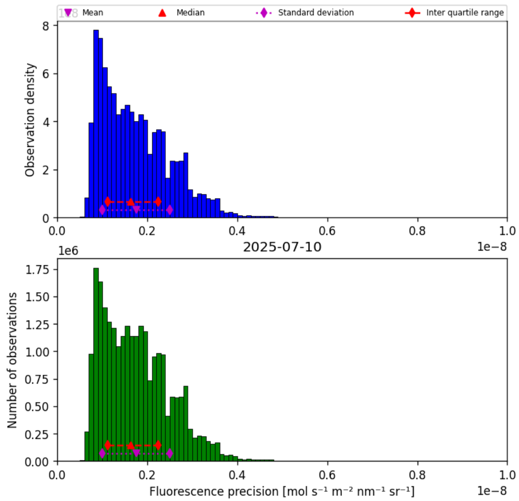
Figure 41: Histogram of “Fluorescence precision” for 2025-07-09 to 2025-07-11
