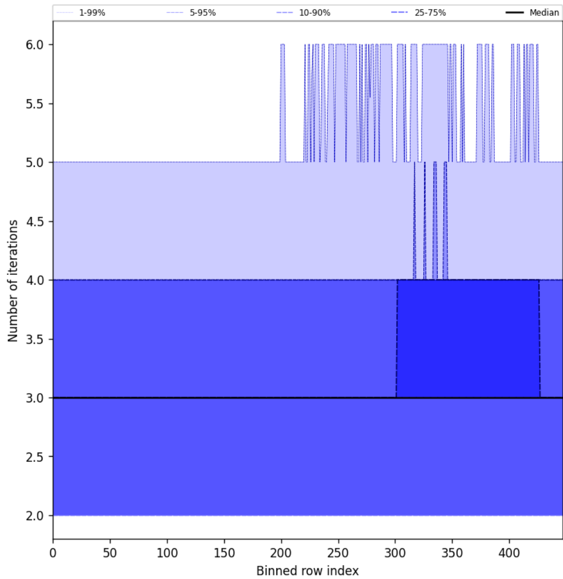
Figure 56: Along track statistics of “Number of iterations” for 2025-07-09 to 2025-07-11
