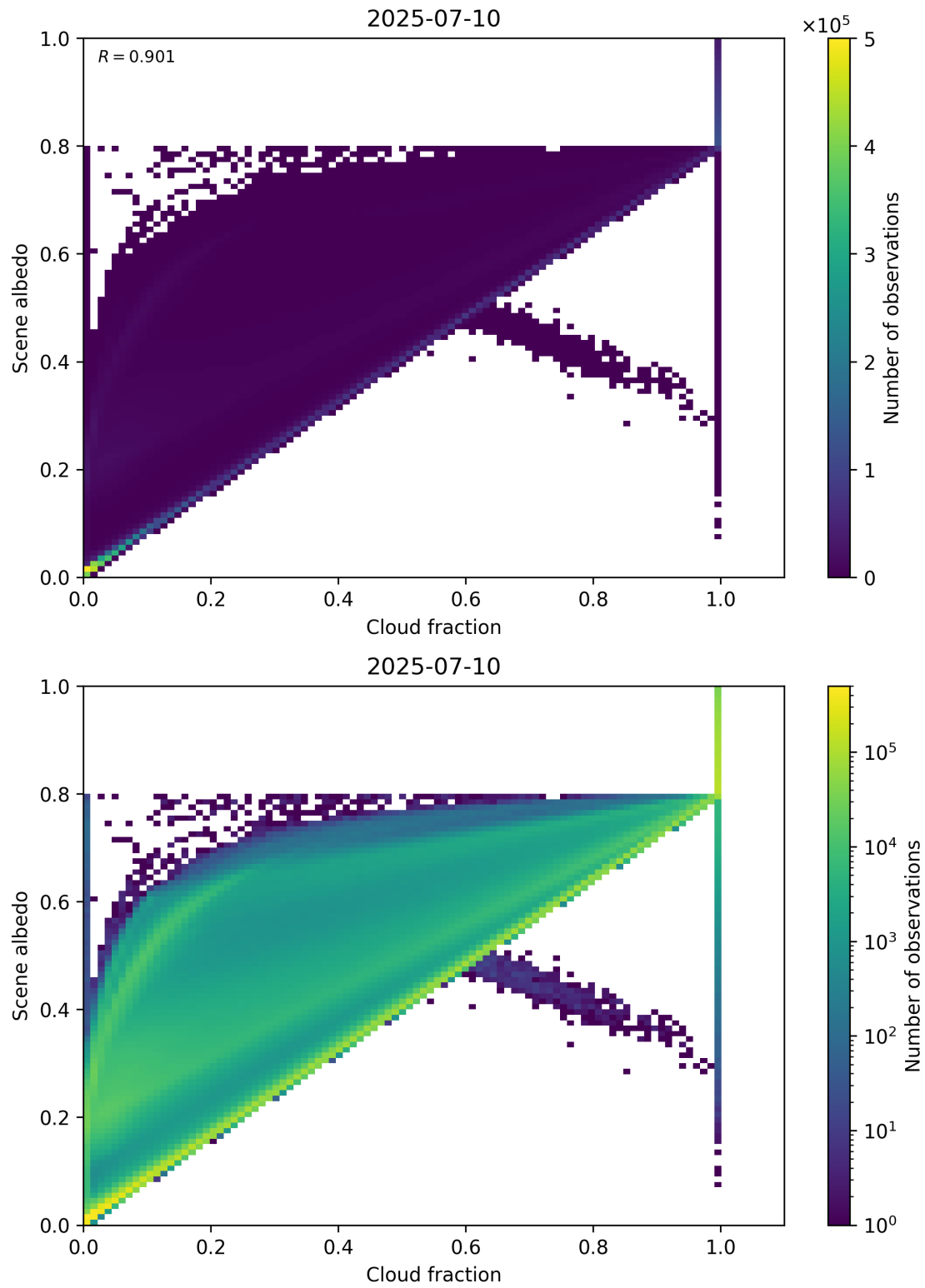
Figure 75: Scatter density plot of “Cloud fraction” against “Scene albedo” for 2025-07-09 to 2025-07-11.
