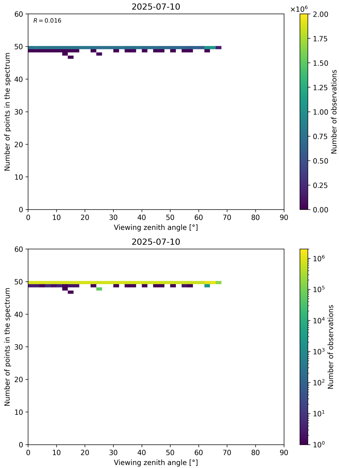
Figure 125: Scatter density plot of “Viewing zenith angle” against “Number of points in the spectrum” for 2025-07-09 to 2025-07-11.
