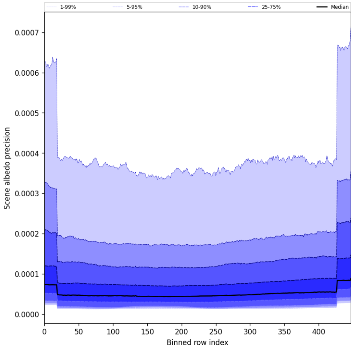
Figure 52: Along track statistics of “Scene albedo precision” for 2025-07-09 to 2025-07-11
