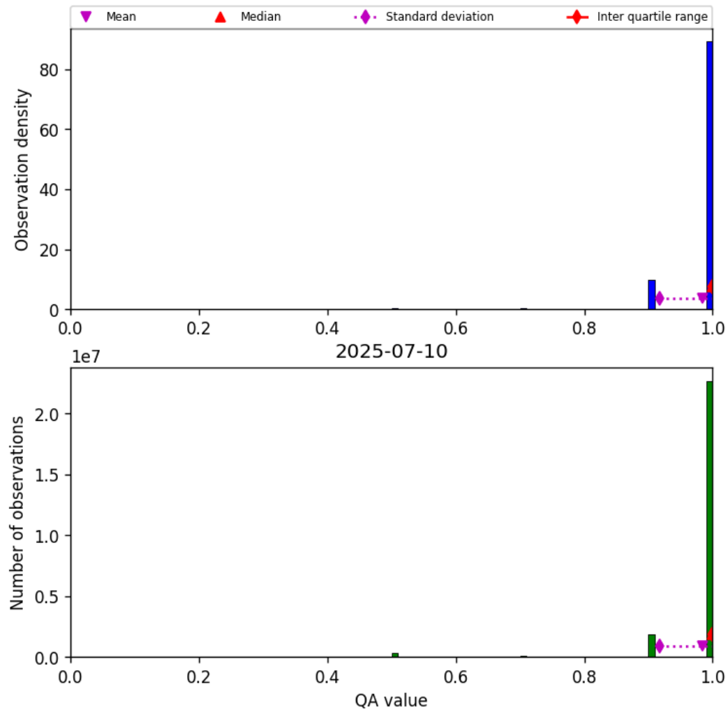
Figure 29: Histogram of “QA value” for 2025-07-09 to 2025-07-11
