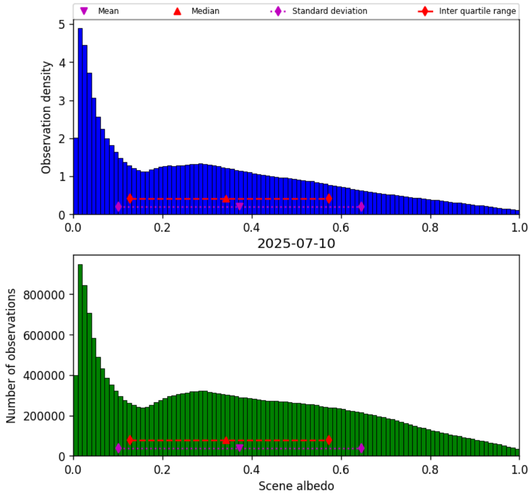
Figure 34: Histogram of “Scene albedo” for 2025-07-09 to 2025-07-11
