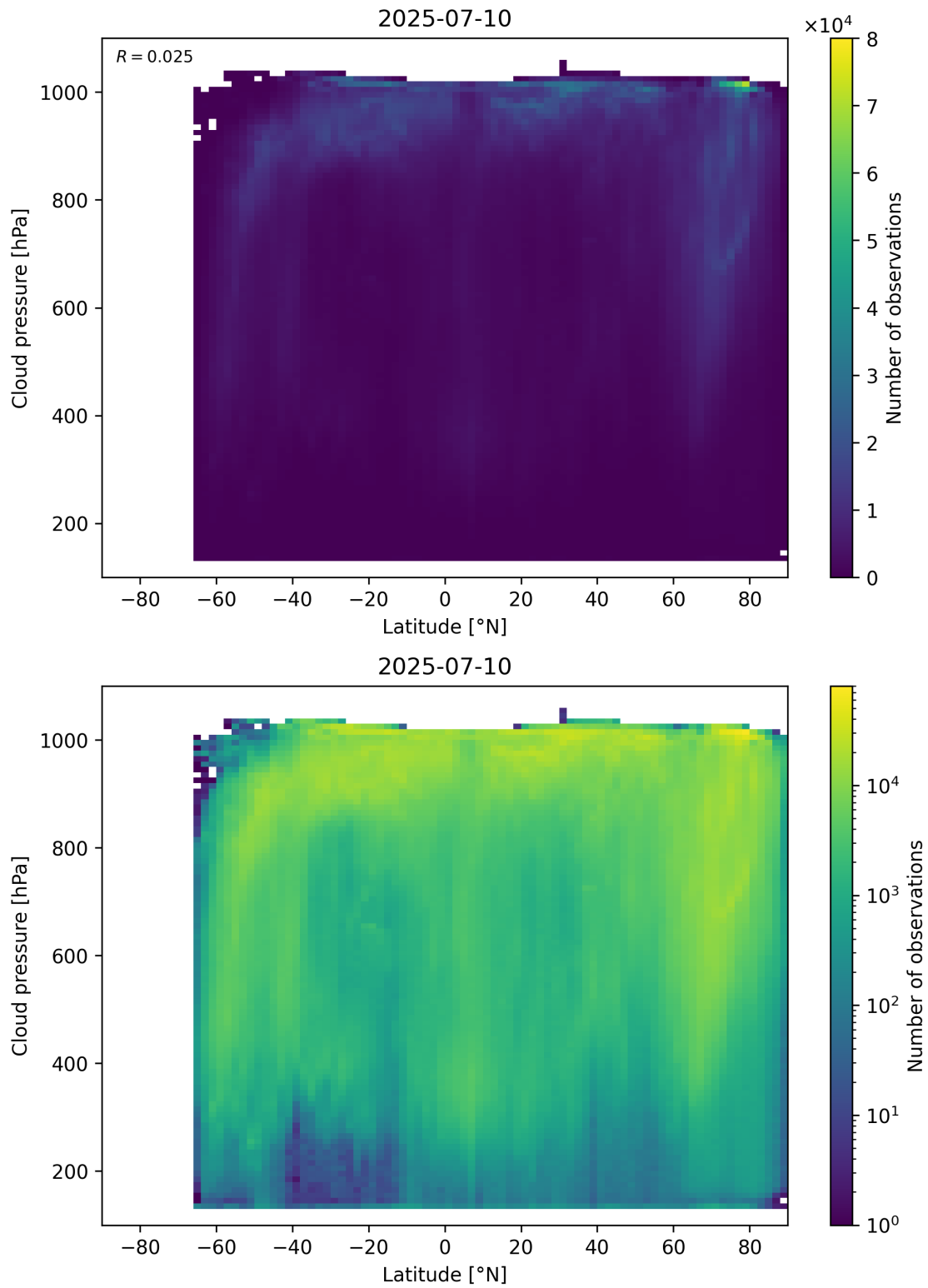
Figure 91: Scatter density plot of “Latitude” against “Cloud pressure” for 2025-07-09 to 2025-07-11.
