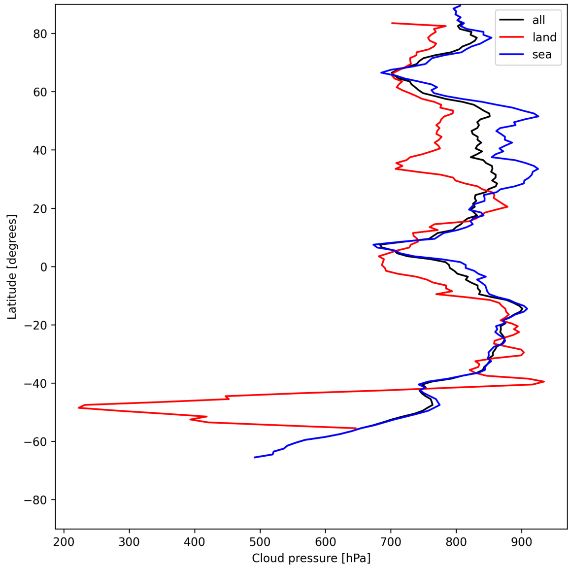
Figure 13: Zonal average of “Cloud pressure” for 2025-07-09 to 2025-07-11.
