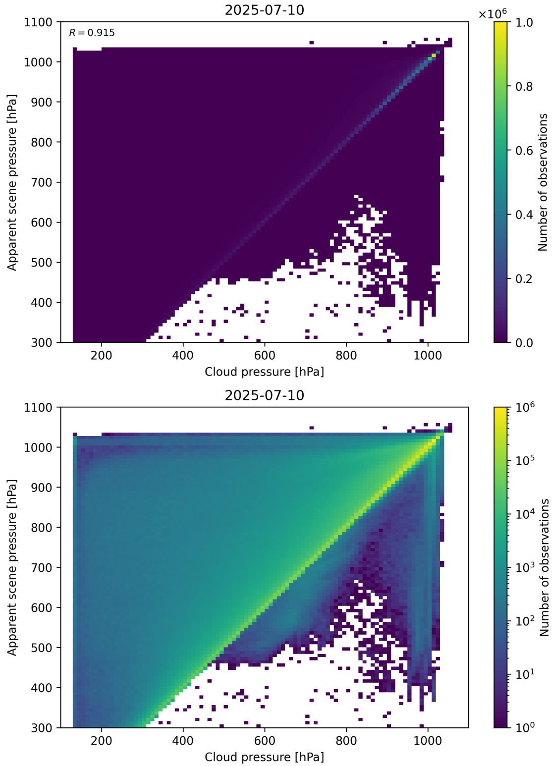
Figure 77: Scatter density plot of “Cloud pressure” against “Apparent scene pressure” for 2025-07-09 to 2025-07-11.
