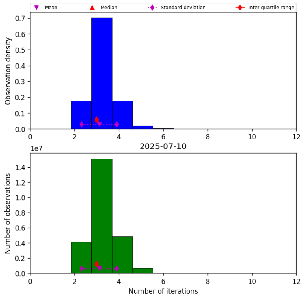
Figure 39: Histogram of “Number of iterations” for 2025-07-09 to 2025-07-11
