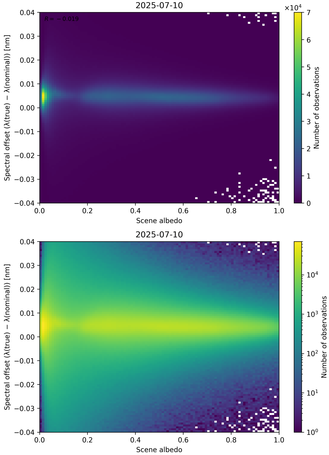
Figure 107: Scatter density plot of “Scene albedo” against “Spectral offset ( \lambda_{\text{true}} - \lambda_{\text{nominal}} )” for 2025-07-09 to 2025-07-11.
