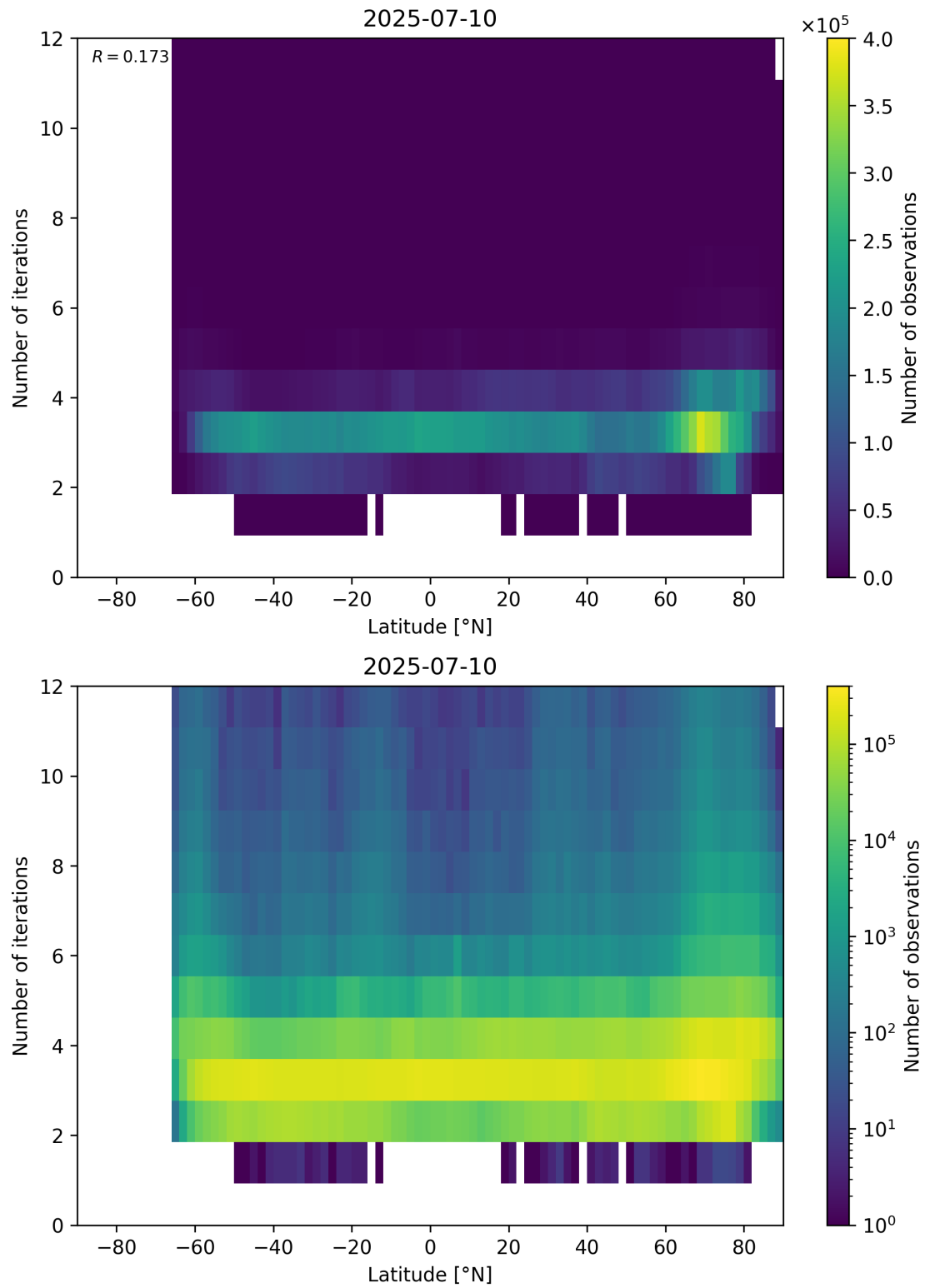
Figure 93: Scatter density plot of “Latitude” against “Number of iterations” for 2025-07-09 to 2025-07-11.
