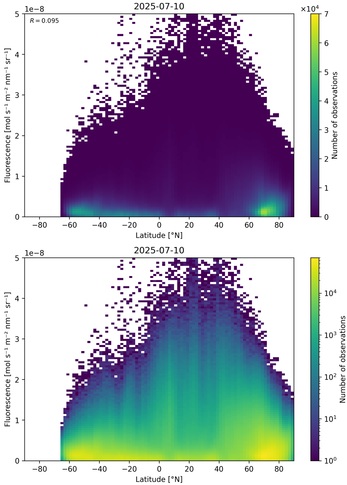
Figure 92: Scatter density plot of “Latitude” against “Fluorescence” for 2025-07-09 to 2025-07-11.
