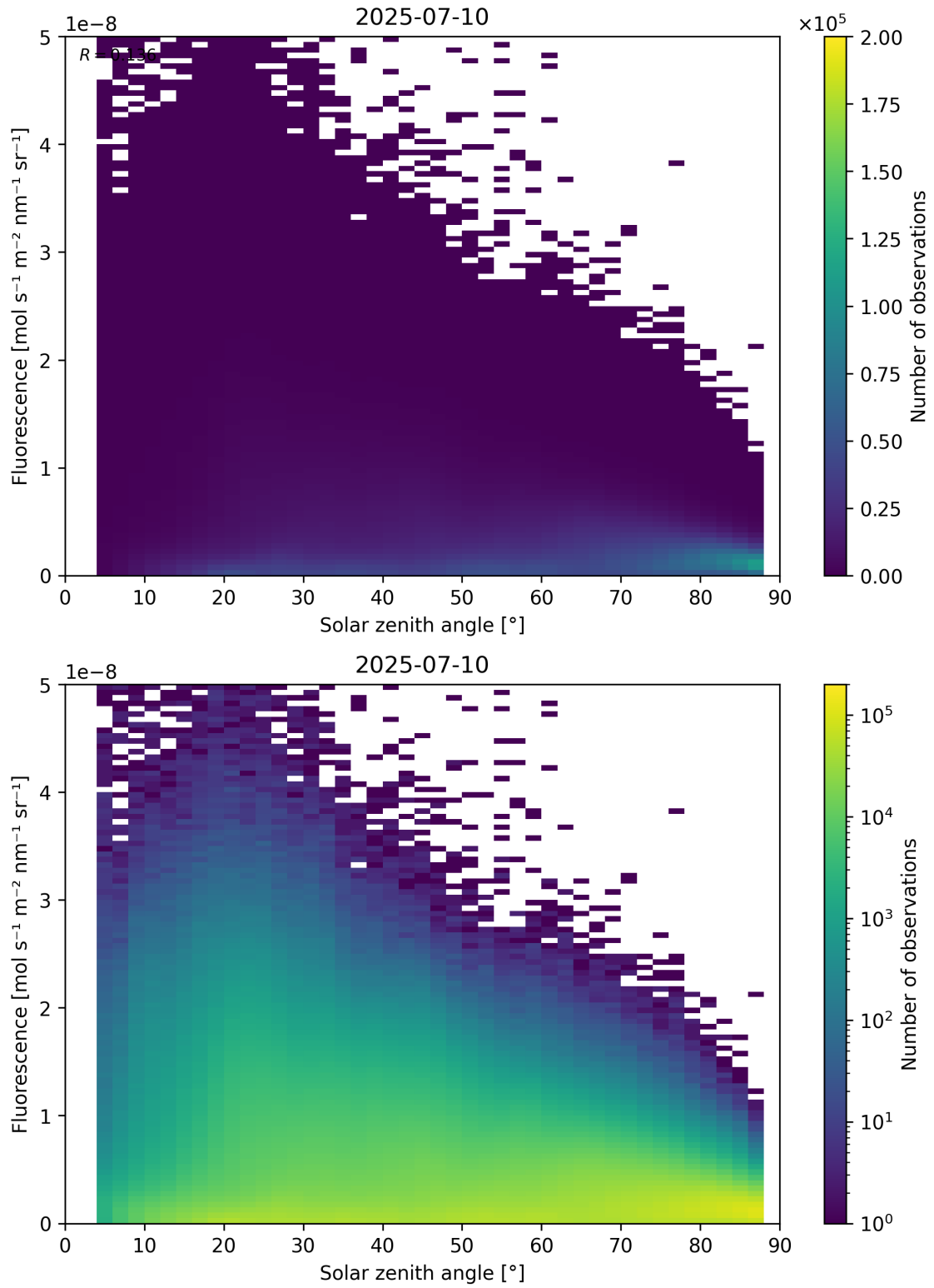
Figure 112: Scatter density plot of “Solar zenith angle” against “Fluorescence” for 2025-07-09 to 2025-07-11.
