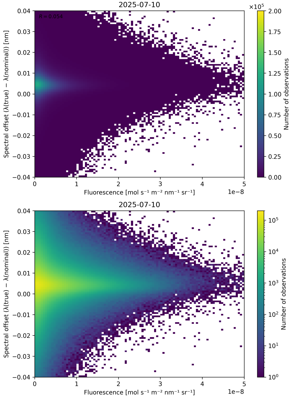
Figure 87: Scatter density plot of “Fluorescence” against “Spectral offset ( \lambda_{\text{true}} - \lambda_{\text{nominal}} )” for 2025-07-09 to 2025-07-11.
