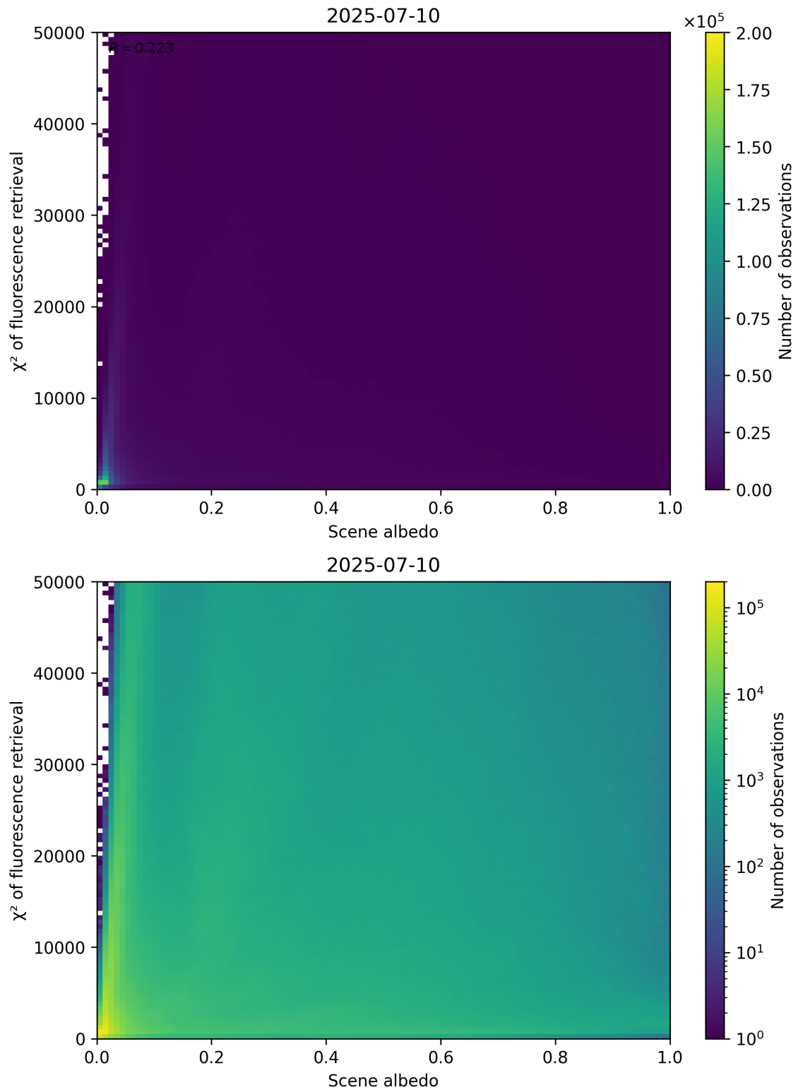
Figure 103: Scatter density plot of “Scene albedo” against “ \chi^2 of fluorescence retrieval” for 2025-07-09 to 2025-07-11.
