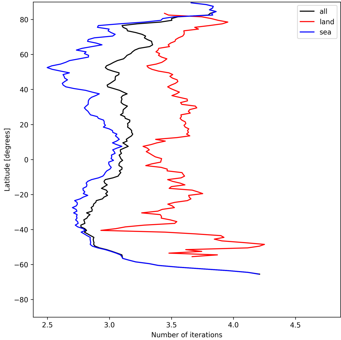
Figure 22: Zonal average of “Number of iterations” for 2025-07-09 to 2025-07-11.
