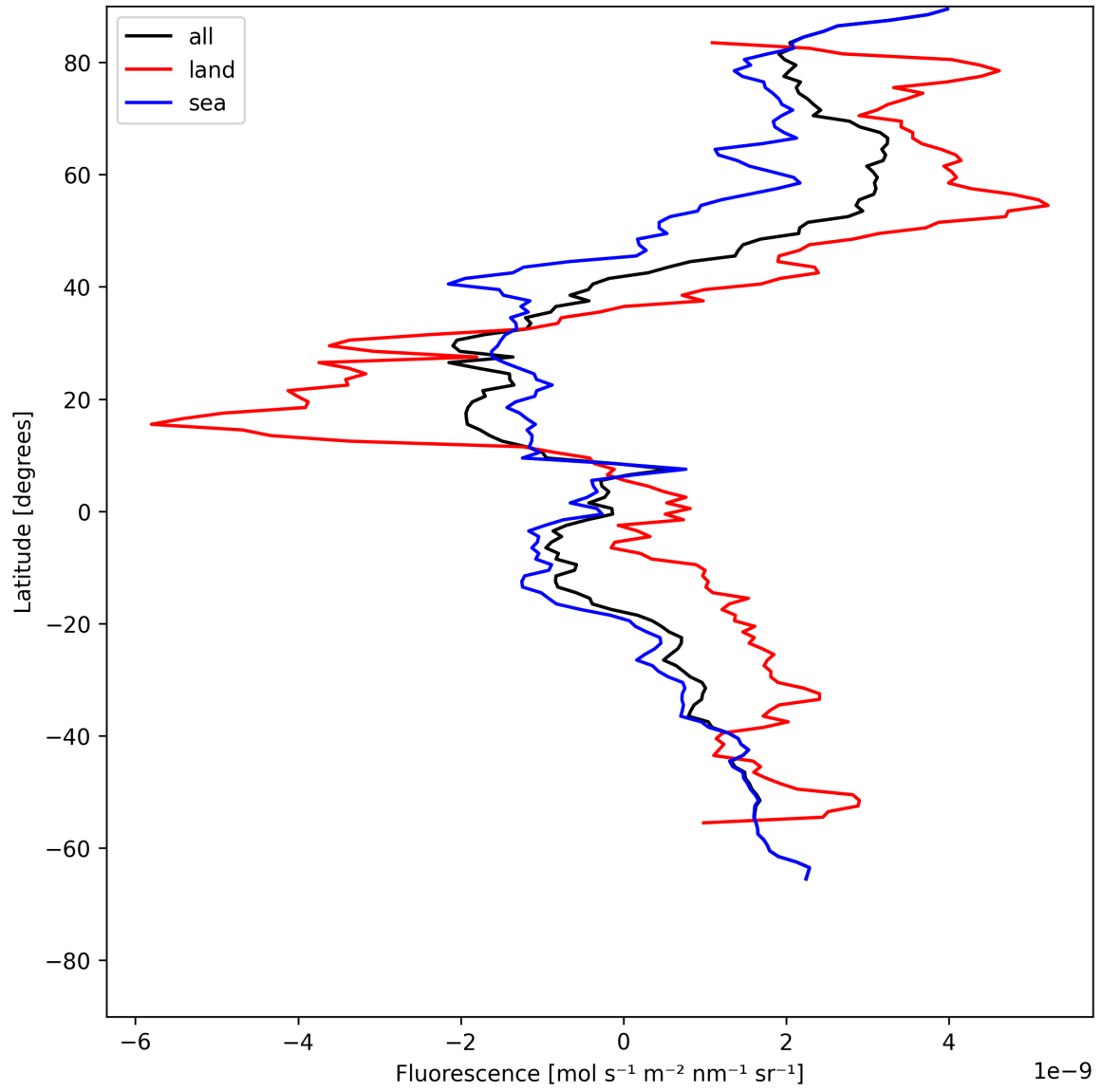
Figure 23: Zonal average of “Fluorescence” for 2025-07-09 to 2025-07-11.
