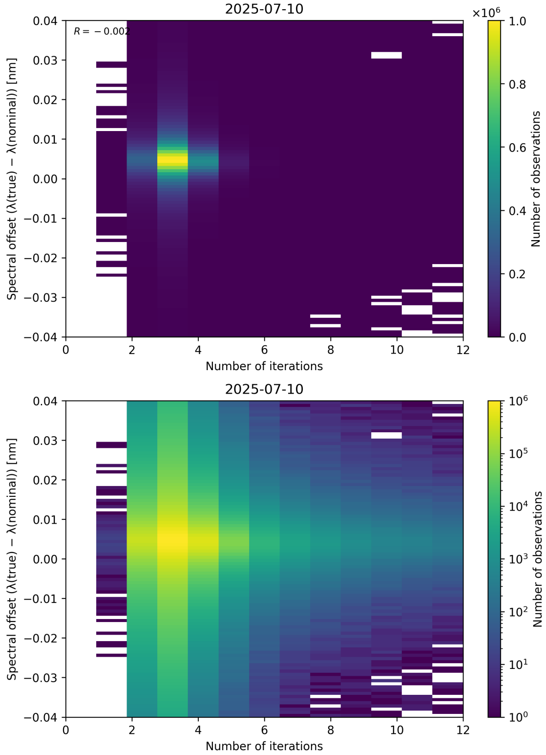
Figure 100: Scatter density plot of “Number of iterations” against “Spectral offset ( \lambda_{\text{true}} - \lambda_{\text{nominal}} )” for 2025-07-09 to 2025-07-11.
