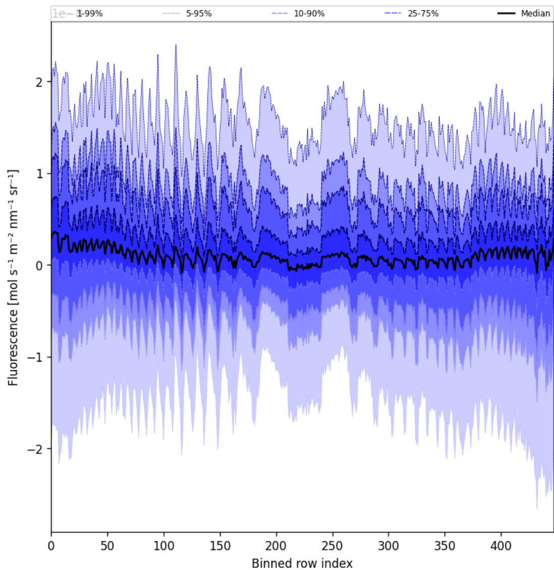
Figure 57: Along track statistics of “Fluorescence” for 2025-07-09 to 2025-07-11
