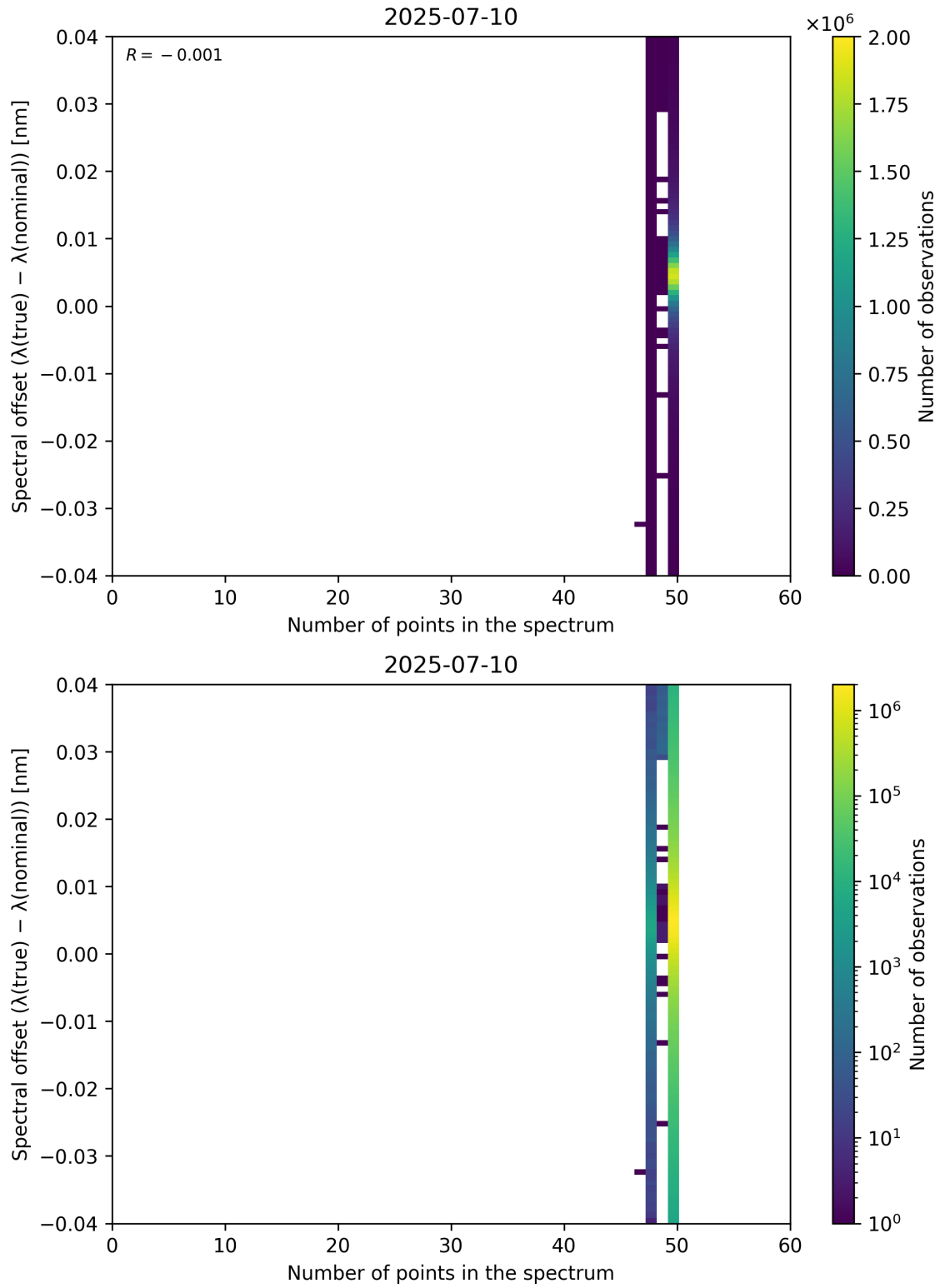
Figure 101: Scatter density plot of “Number of points in the spectrum” against “Spectral offset ( \lambda_{\text{true}} - \lambda_{\text{nominal}} )” for 2025-07-09 to 2025-07-11.
