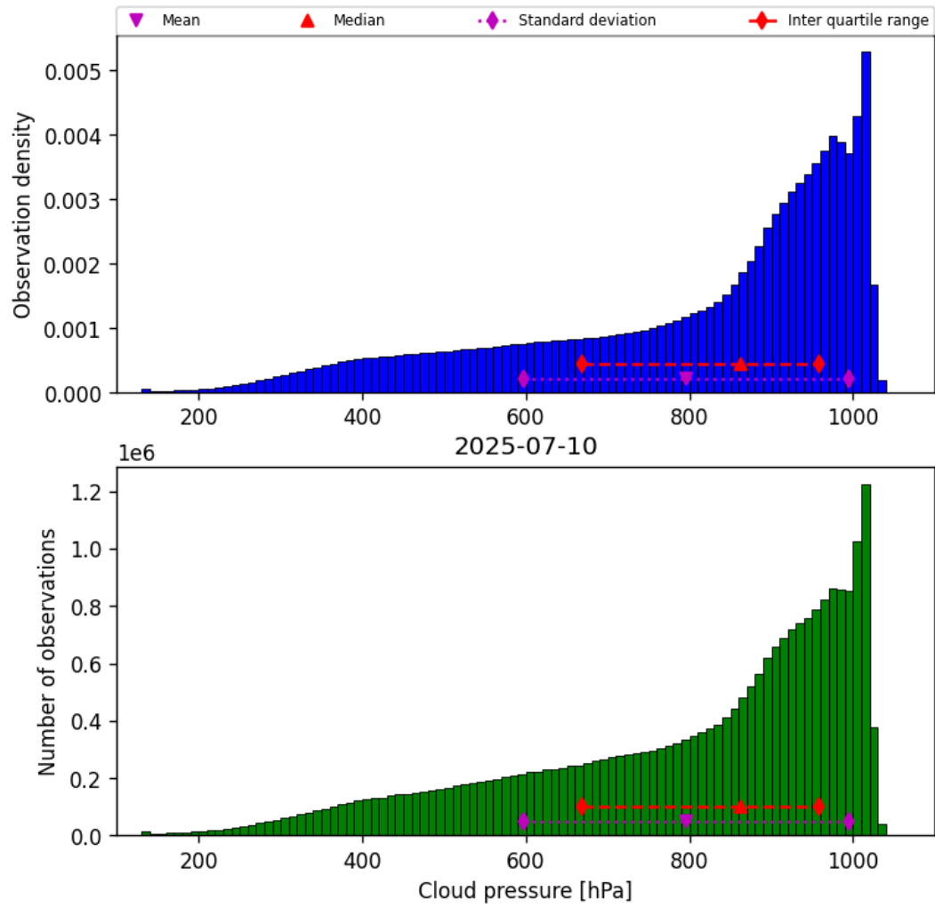
Figure 30: Histogram of “Cloud pressure” for 2025-07-09 to 2025-07-11
