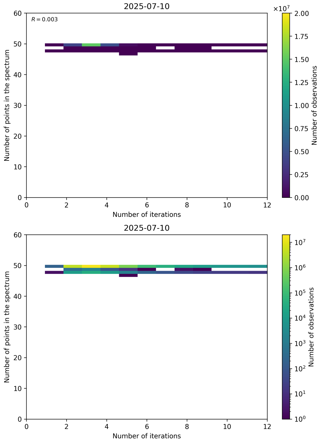
Figure 99: Scatter density plot of “Number of iterations” against “Number of points in the spectrum” for 2025-07-09 to 2025-07-11.
