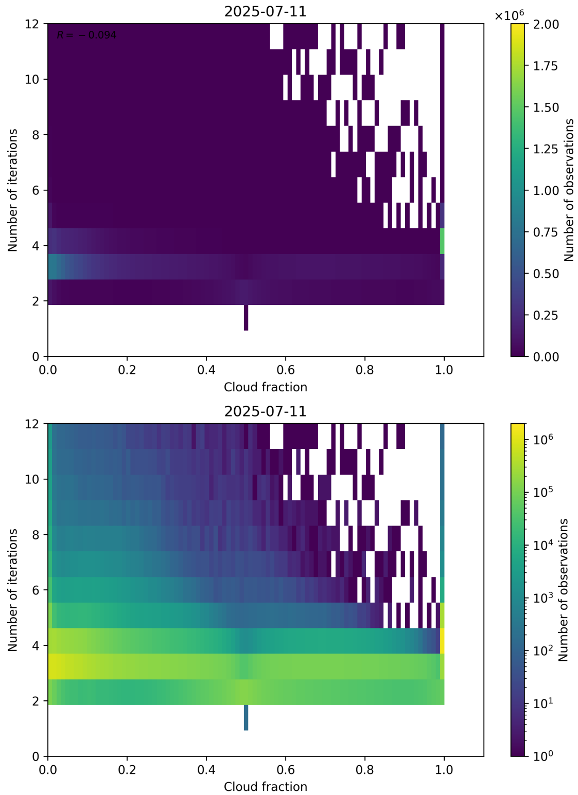
Figure 73: Scatter density plot of “Cloud fraction” against “Number of iterations” for 2025-07-10 to 2025-07-12.
