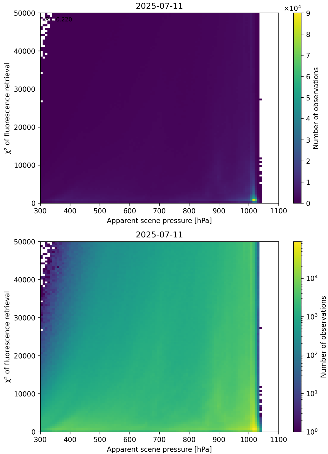
Figure 63: Scatter density plot of “Apparent scene pressure” against “ \chi^2 of fluorescence retrieval” for 2025-07-10 to 2025-07-12.
