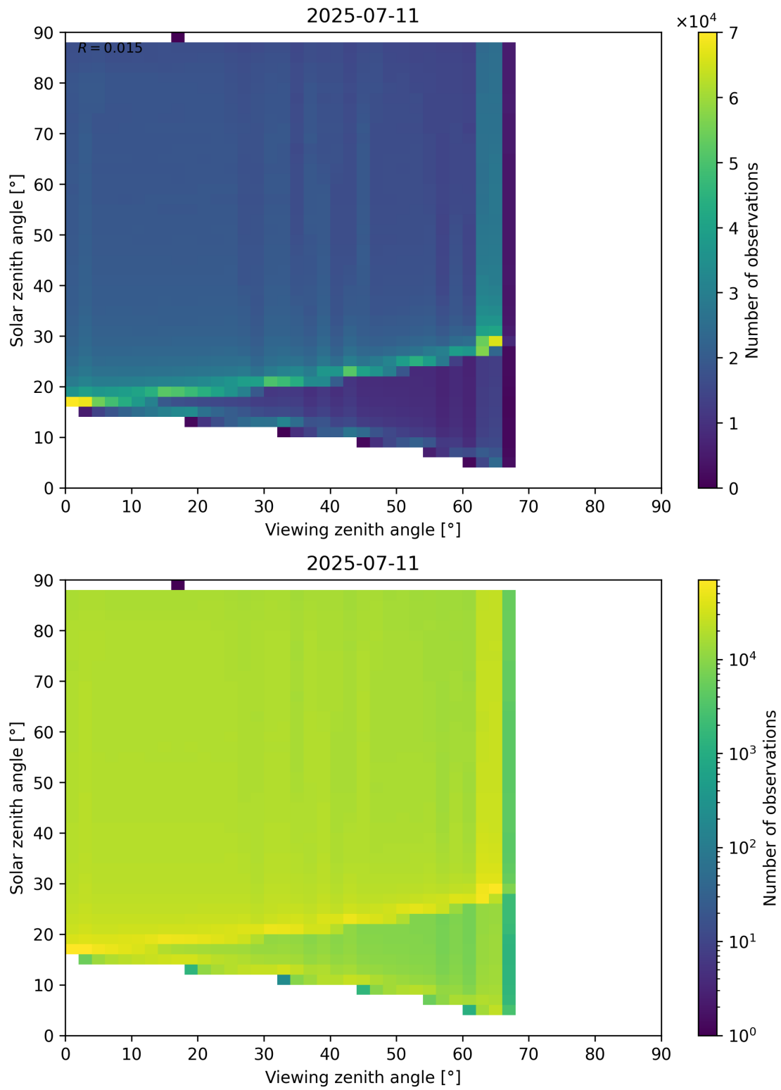
Figure 127: Scatter density plot of “Viewing zenith angle” against “Solar zenith angle” for 2025-07-10 to 2025-07-12.
