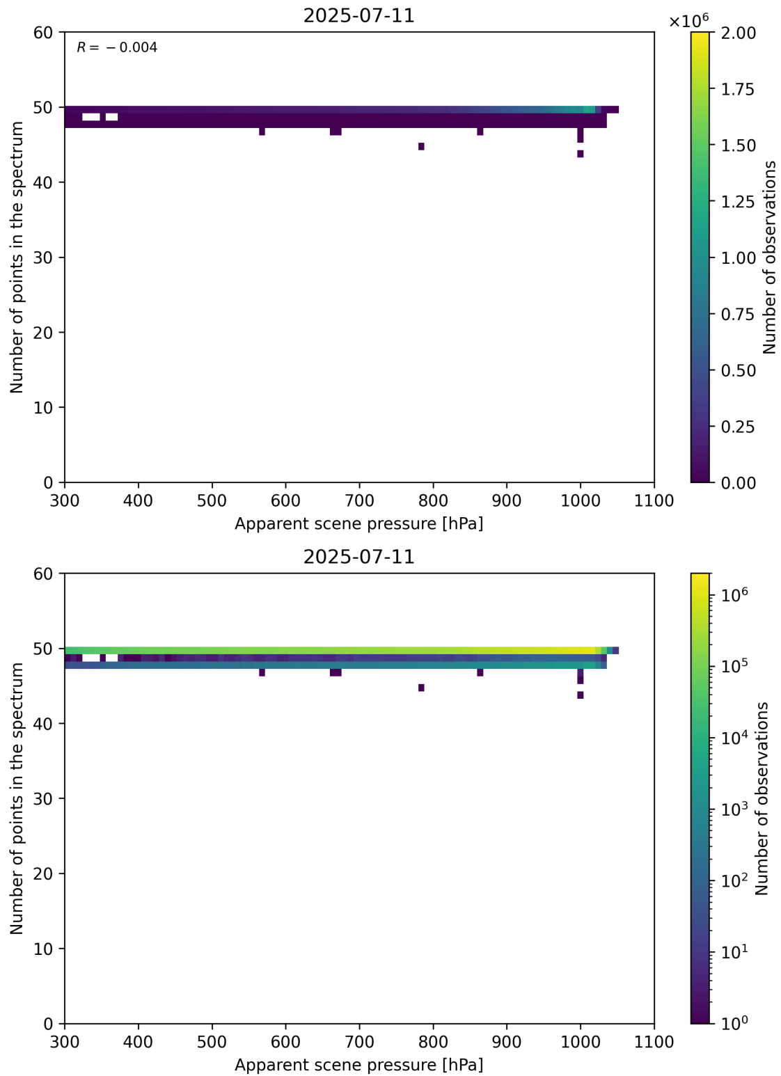
Figure 66: Scatter density plot of “Apparent scene pressure” against “Number of points in the spectrum” for 2025-07-10 to 2025-07-12.
