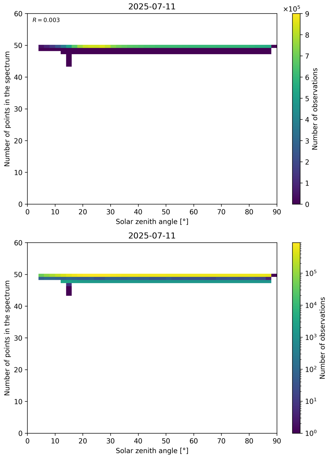
Figure 115: Scatter density plot of “Solar zenith angle” against “Number of points in the spectrum” for 2025-07-10 to 2025-07-12.
