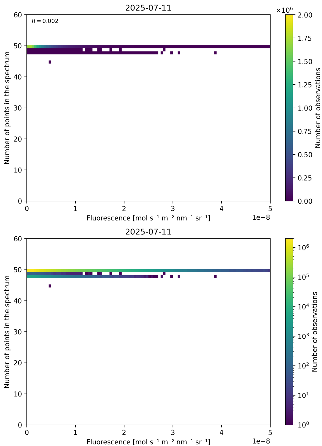
Figure 86: Scatter density plot of “Fluorescence” against “Number of points in the spectrum” for 2025-07-10 to 2025-07-12.
