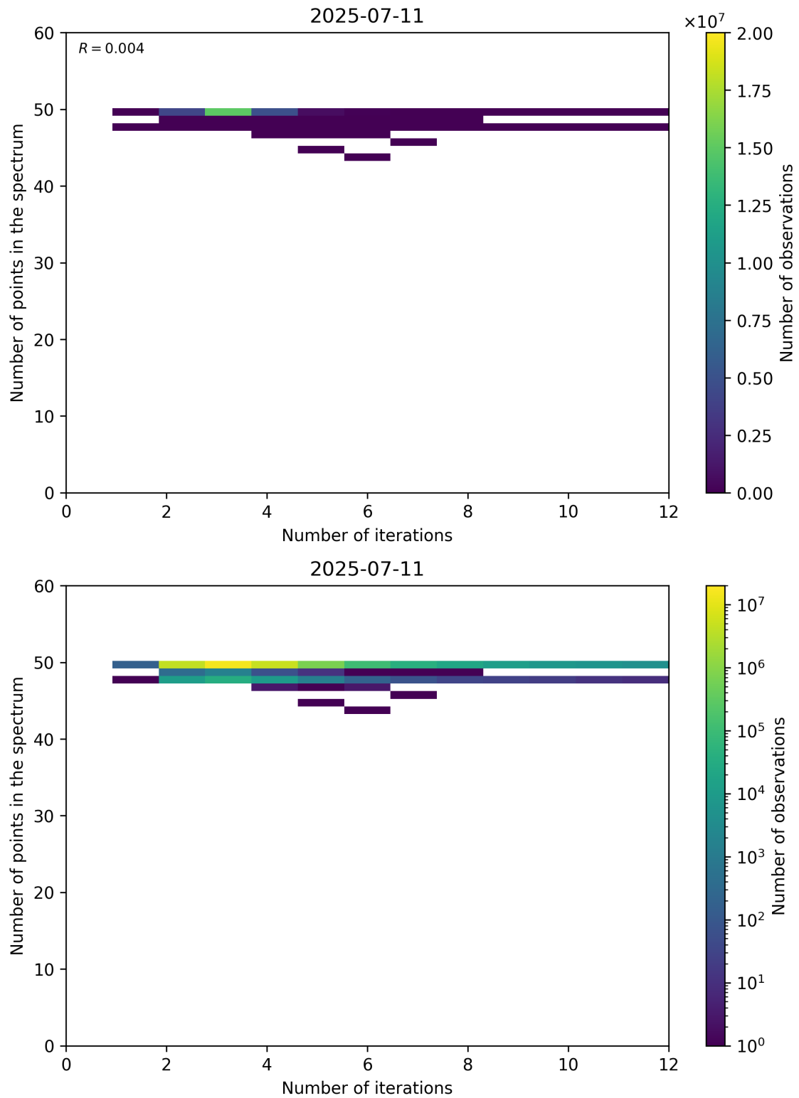
Figure 99: Scatter density plot of “Number of iterations” against “Number of points in the spectrum” for 2025-07-10 to 2025-07-12.
