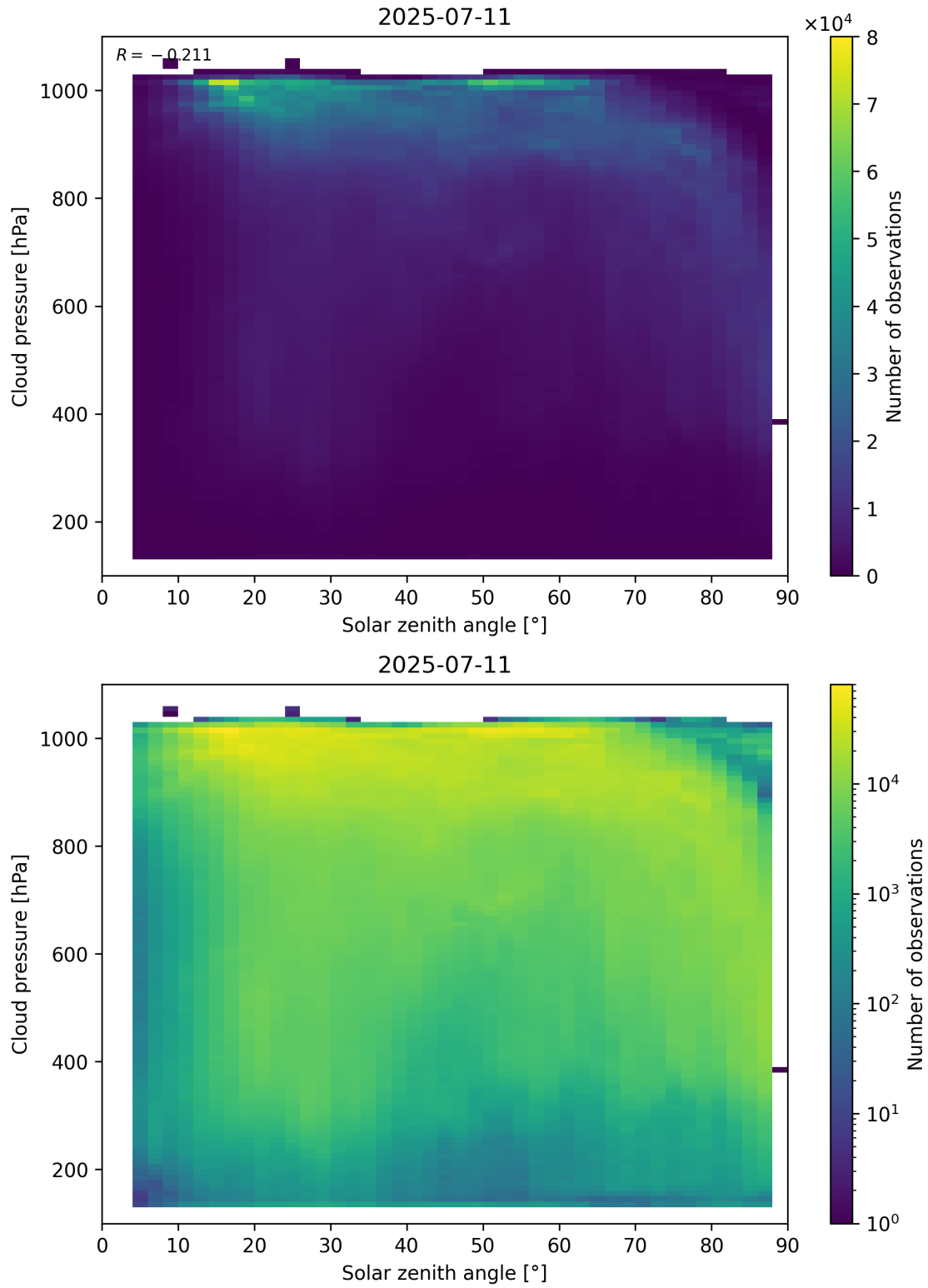
Figure 111: Scatter density plot of “Solar zenith angle” against “Cloud pressure” for 2025-07-10 to 2025-07-12.
