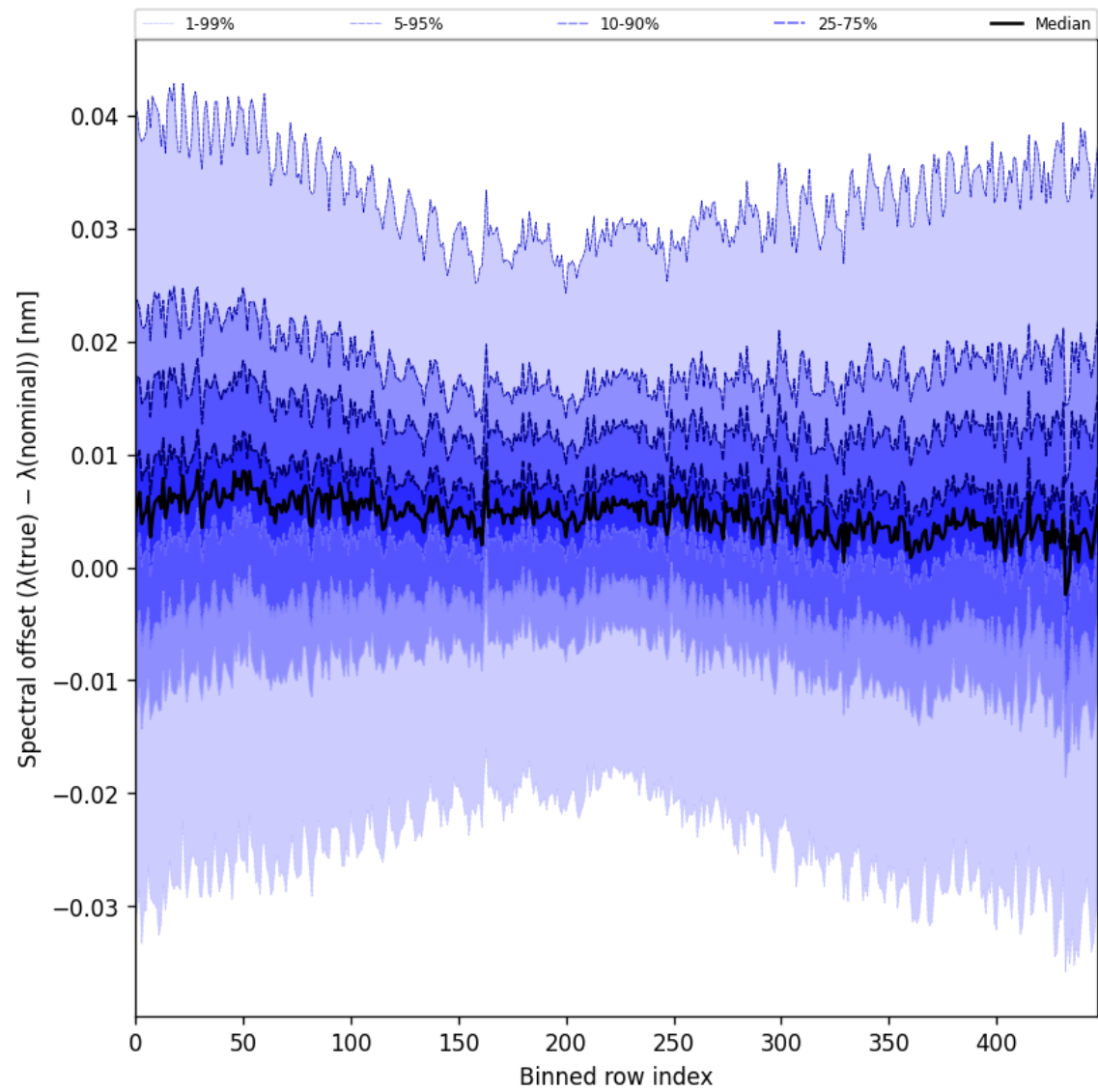
Figure 62: Along track statistics of “Spectral offset ( \lambda_{\text{true}} - \lambda_{\text{nominal}} )” for 2025-07-10 to 2025-07-12
