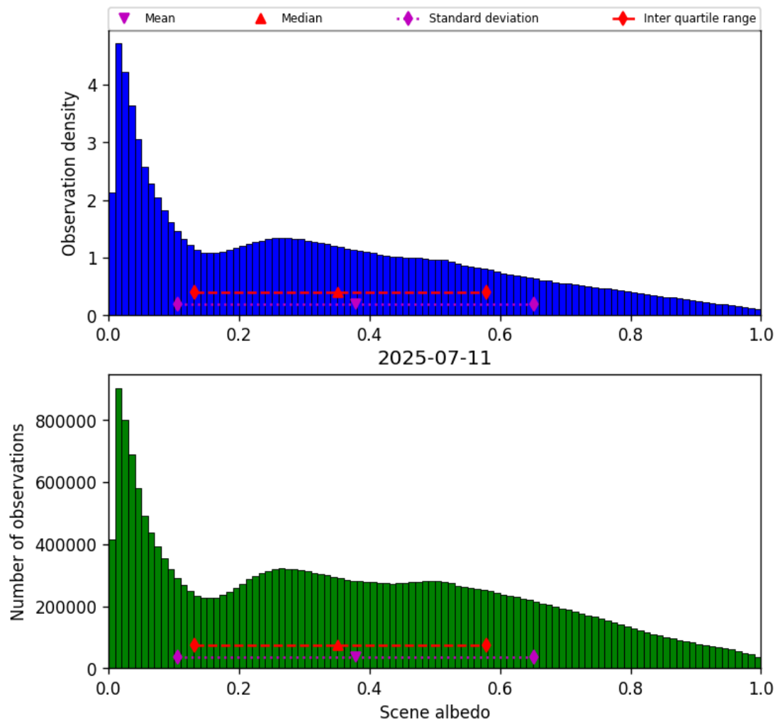
Figure 34: Histogram of “Scene albedo” for 2025-07-10 to 2025-07-12
