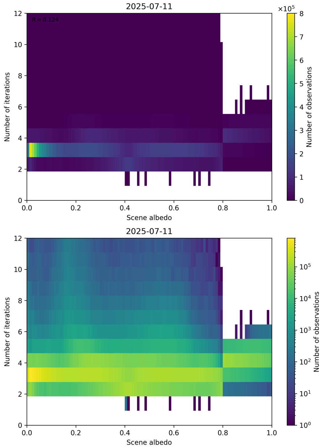
Figure 105: Scatter density plot of “Scene albedo” against “Number of iterations” for 2025-07-10 to 2025-07-12.
