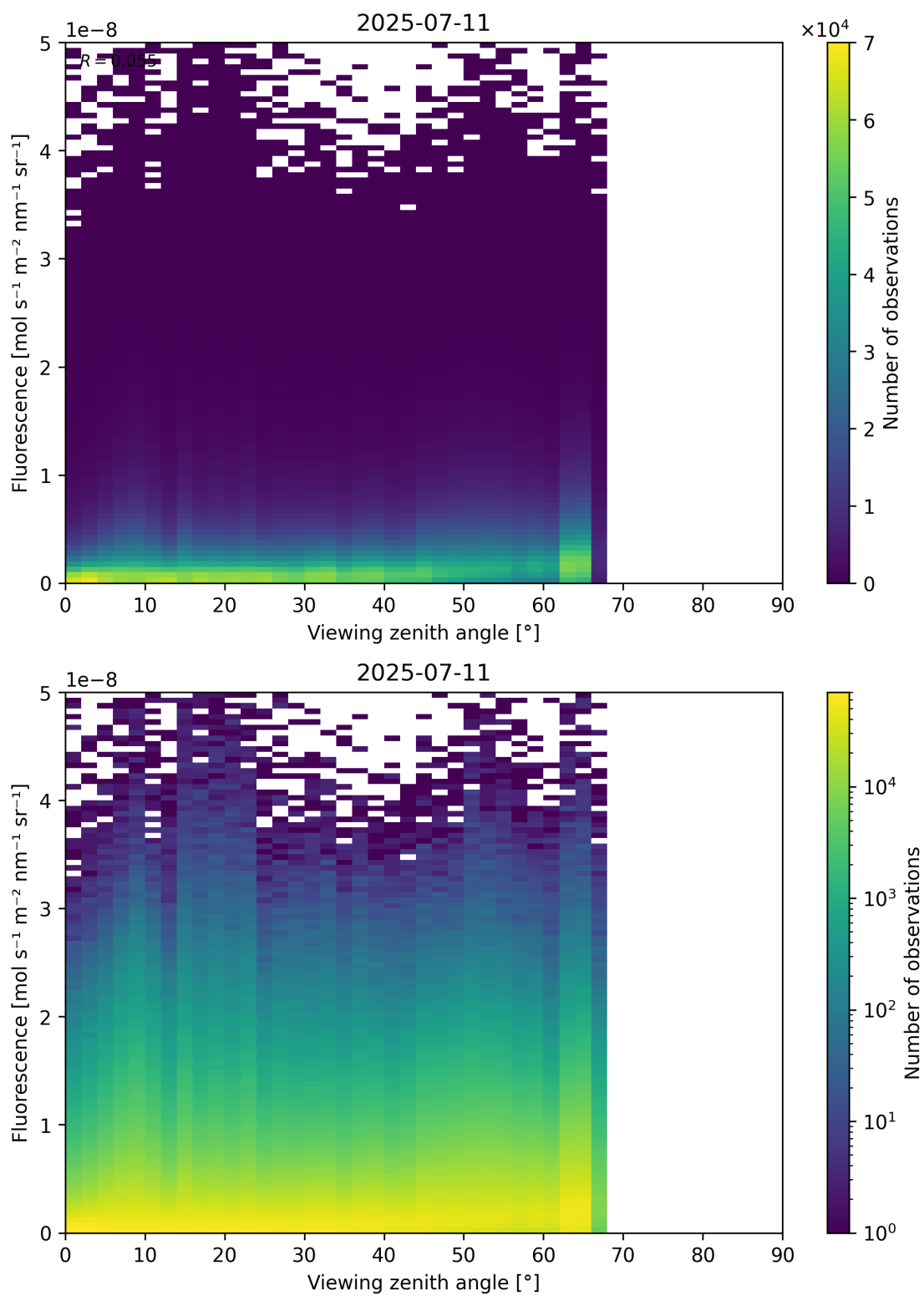
Figure 122: Scatter density plot of “Viewing zenith angle” against “Fluorescence” for 2025-07-10 to 2025-07-12.
