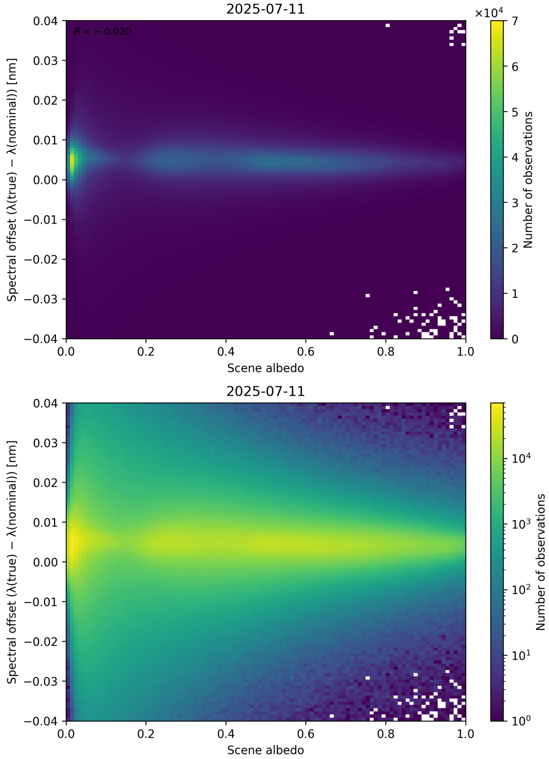
Figure 107: Scatter density plot of “Scene albedo” against “Spectral offset ( \lambda_{\text{true}} - \lambda_{\text{nominal}} )” for 2025-07-10 to 2025-07-12.
