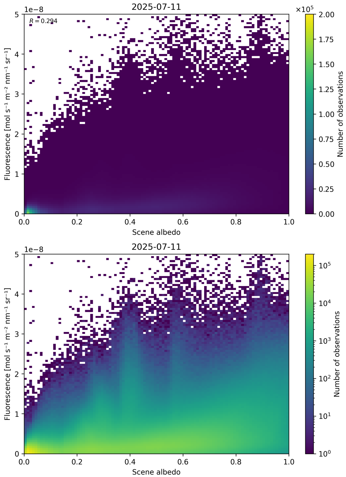
Figure 104: Scatter density plot of “Scene albedo” against “Fluorescence” for 2025-07-10 to 2025-07-12.
