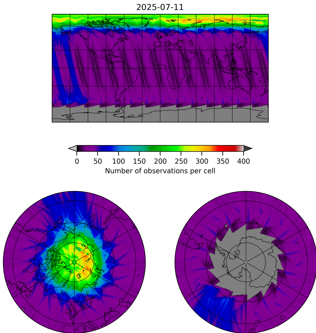
Figure 11: Map of the number of observations for 2025-07-10 to 2025-07-12
