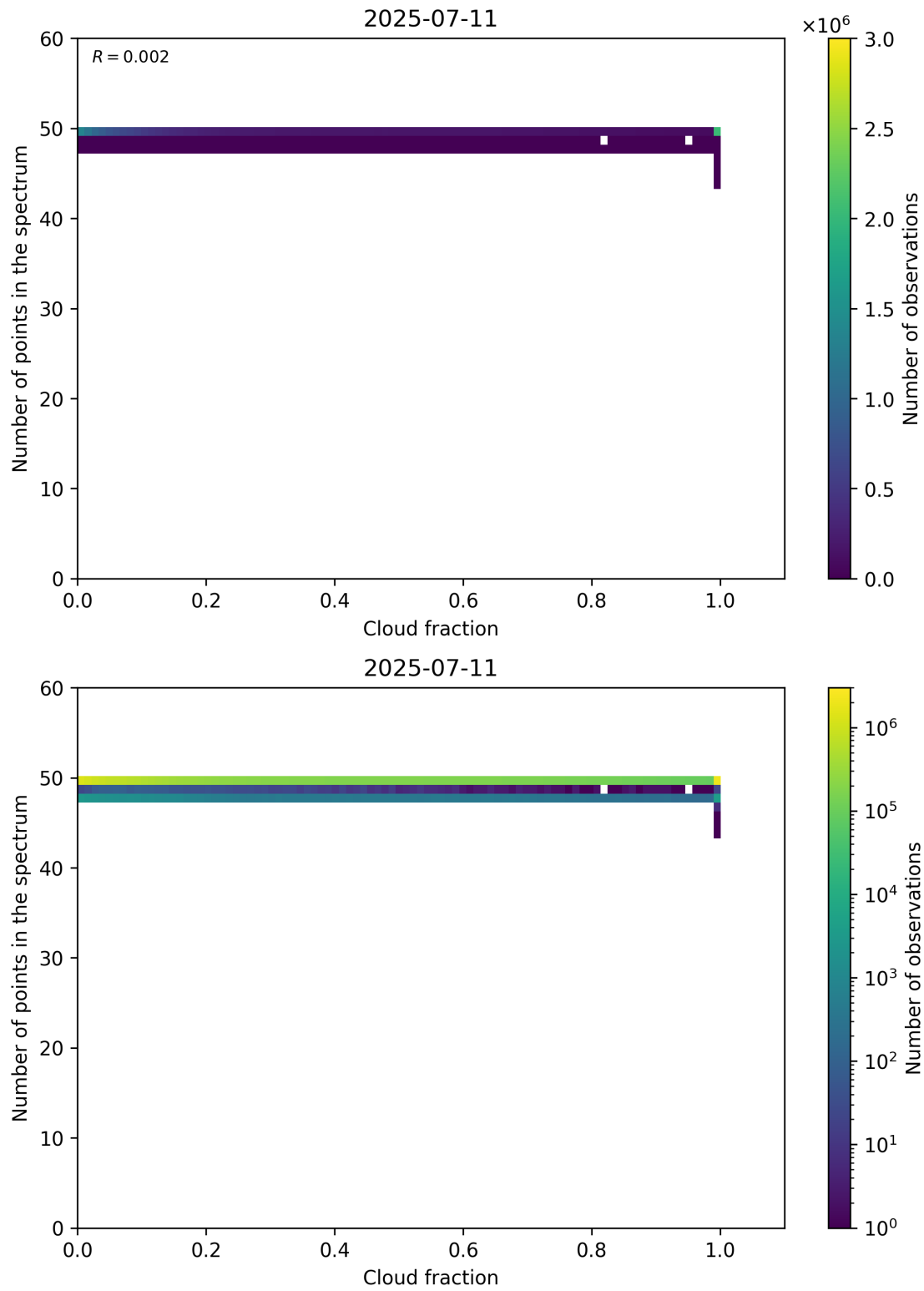
Figure 74: Scatter density plot of “Cloud fraction” against “Number of points in the spectrum” for 2025-07-10 to 2025-07-12.
