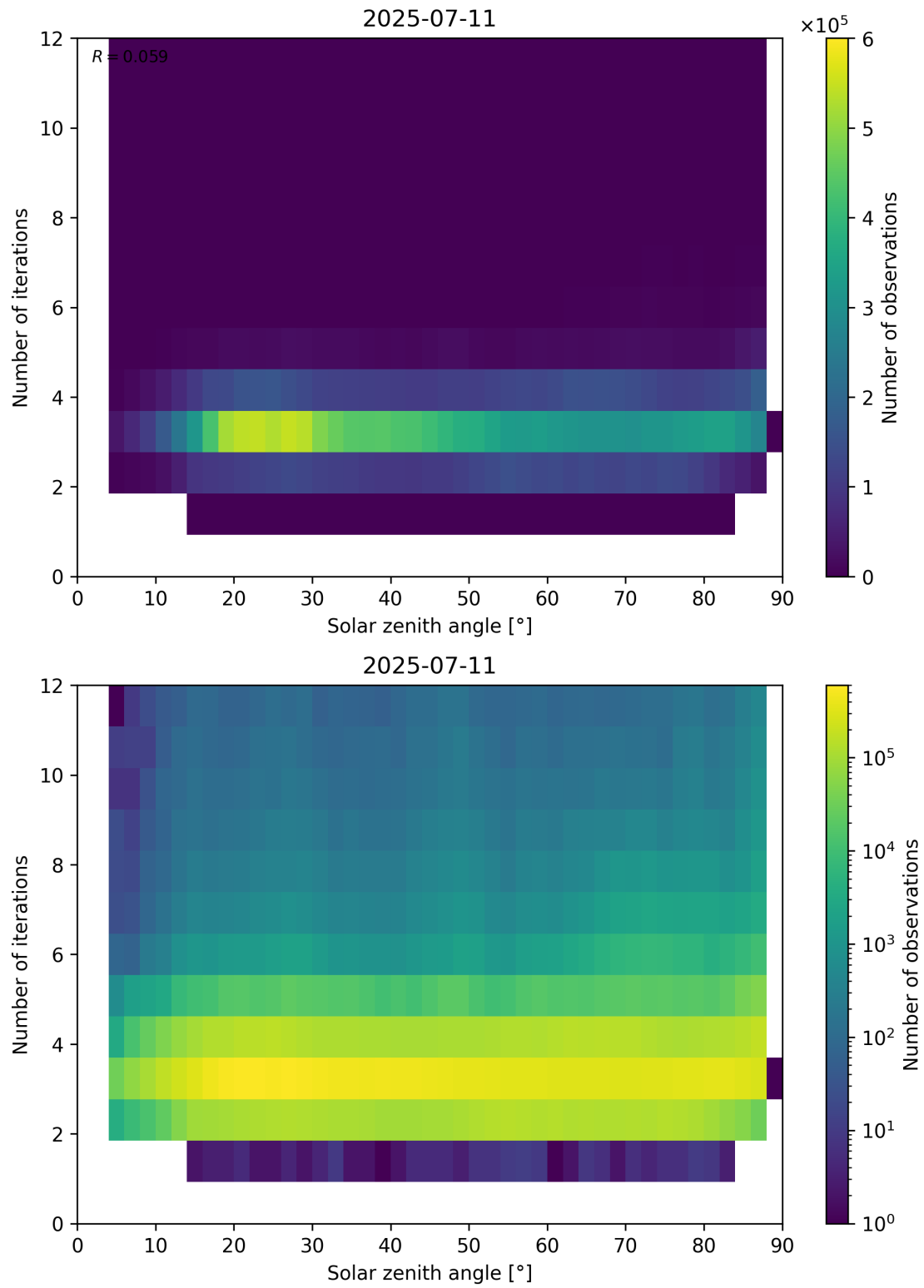
Figure 114: Scatter density plot of “Solar zenith angle” against “Number of iterations” for 2025-07-10 to 2025-07-12.
