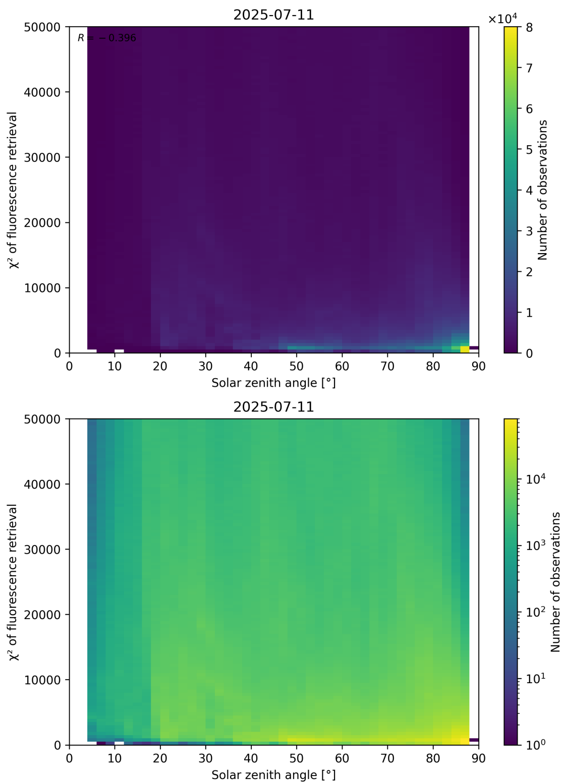
Figure 109: Scatter density plot of “Solar zenith angle” against “ \chi^2 of fluorescence retrieval” for 2025-07-10 to 2025-07-12.
