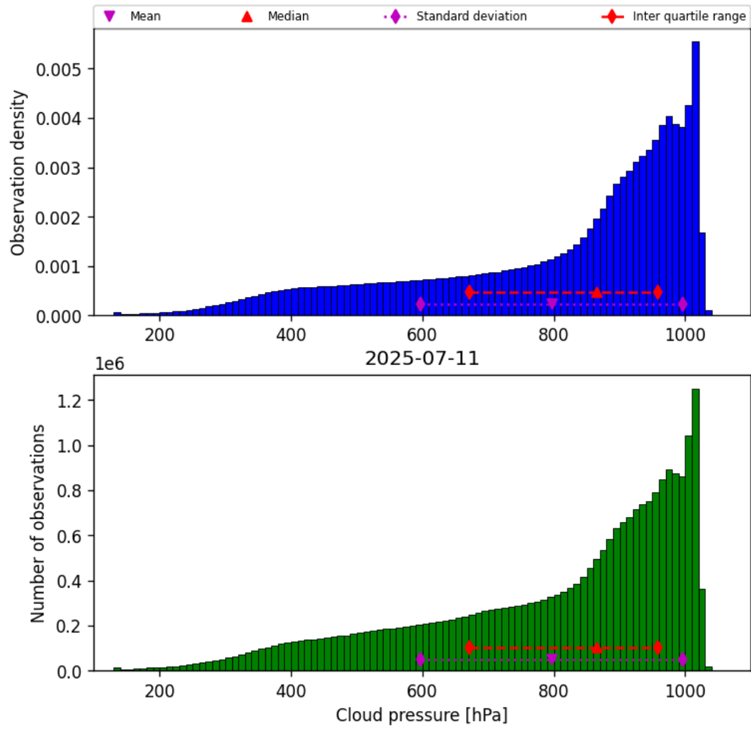
Figure 30: Histogram of “Cloud pressure” for 2025-07-10 to 2025-07-12
