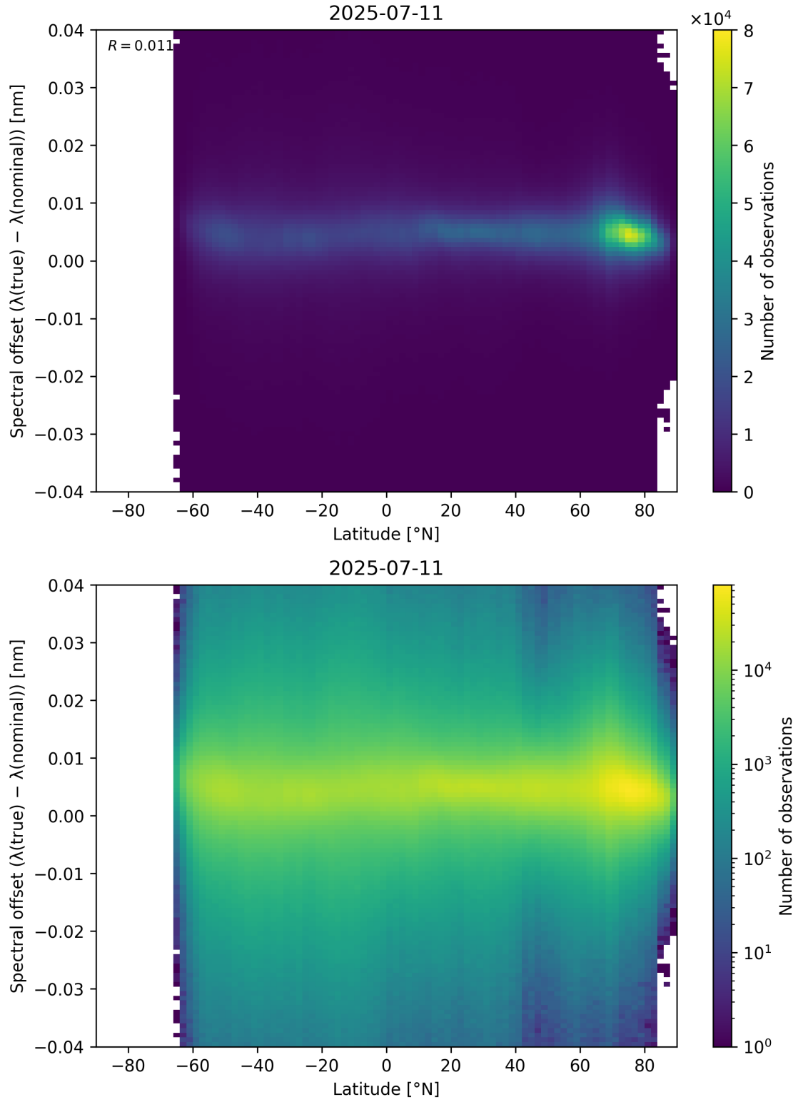
Figure 96: Scatter density plot of “Latitude” against “Spectral offset ( \lambda_{\text{true}} - \lambda_{\text{nominal}} )” for 2025-07-10 to 2025-07-12.
