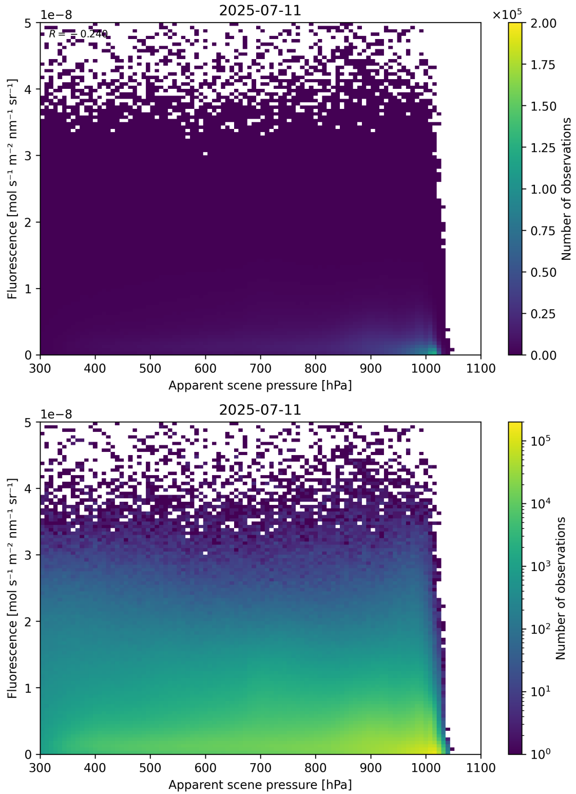
Figure 64: Scatter density plot of “Apparent scene pressure” against “Fluorescence” for 2025-07-10 to 2025-07-12.
