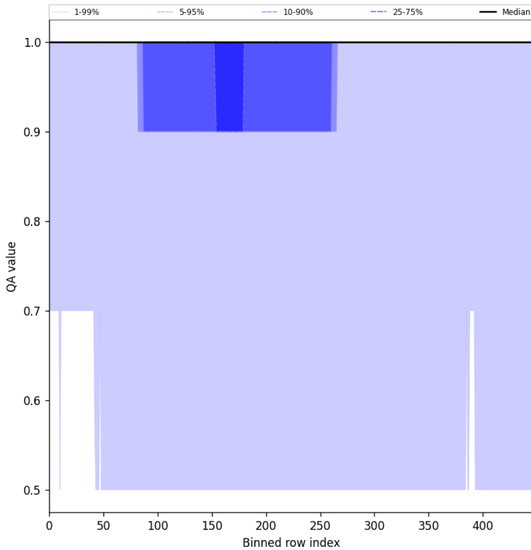
Figure 46: Along track statistics of “QA value” for 2025-07-10 to 2025-07-12
