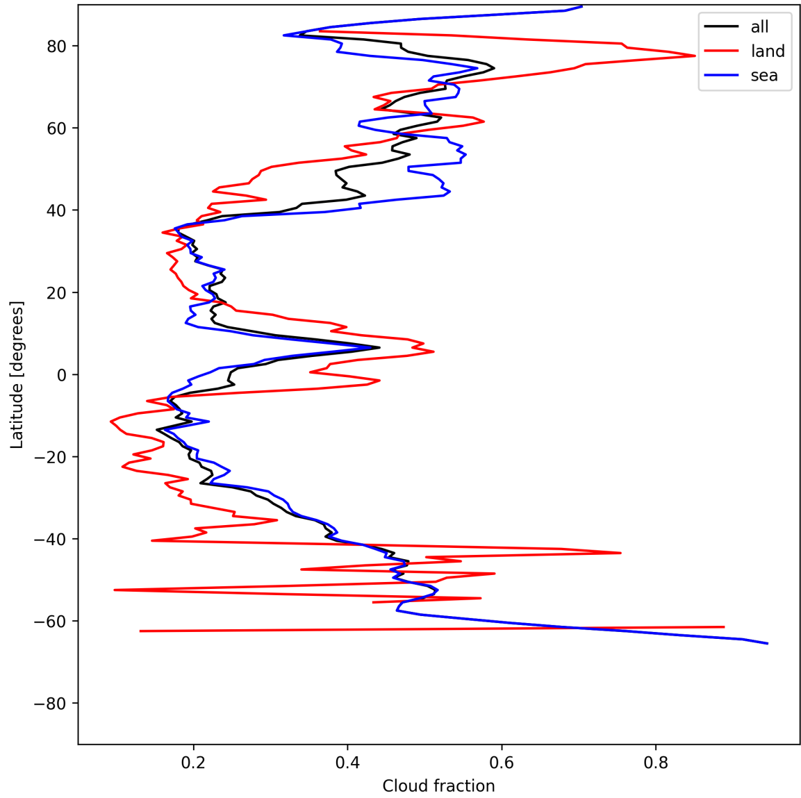
Figure 15: Zonal average of “Cloud fraction” for 2025-07-10 to 2025-07-12.
