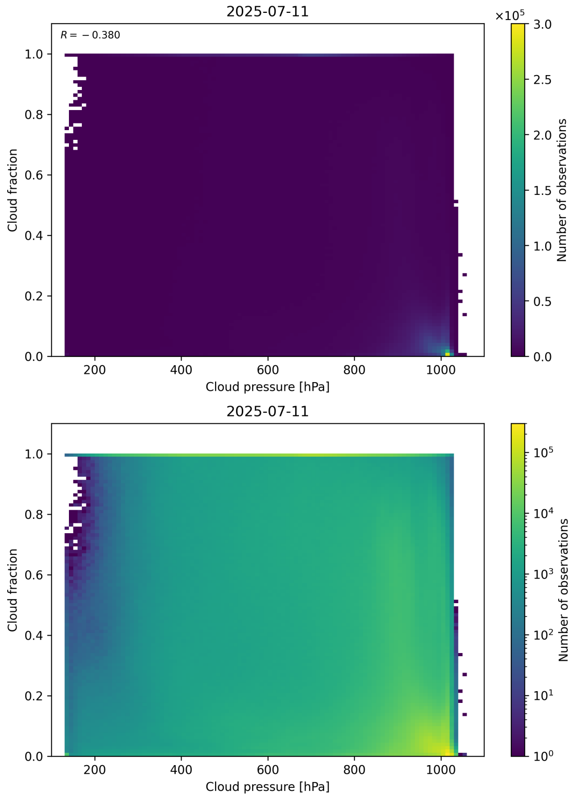
Figure 79: Scatter density plot of “Cloud pressure” against “Cloud fraction” for 2025-07-10 to 2025-07-12.
