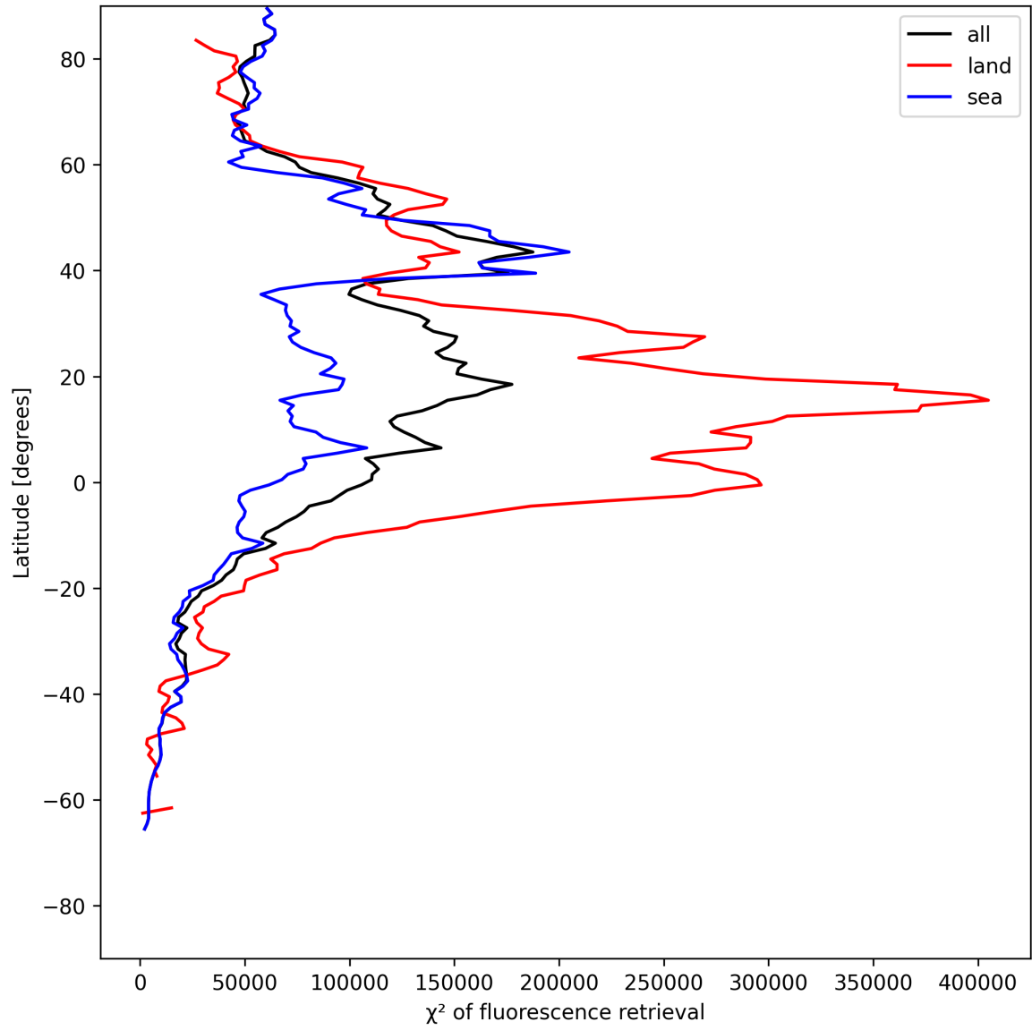
Figure 25: Zonal average of “ \chi^2 of fluorescence retrieval” for 2025-07-10 to 2025-07-12.
