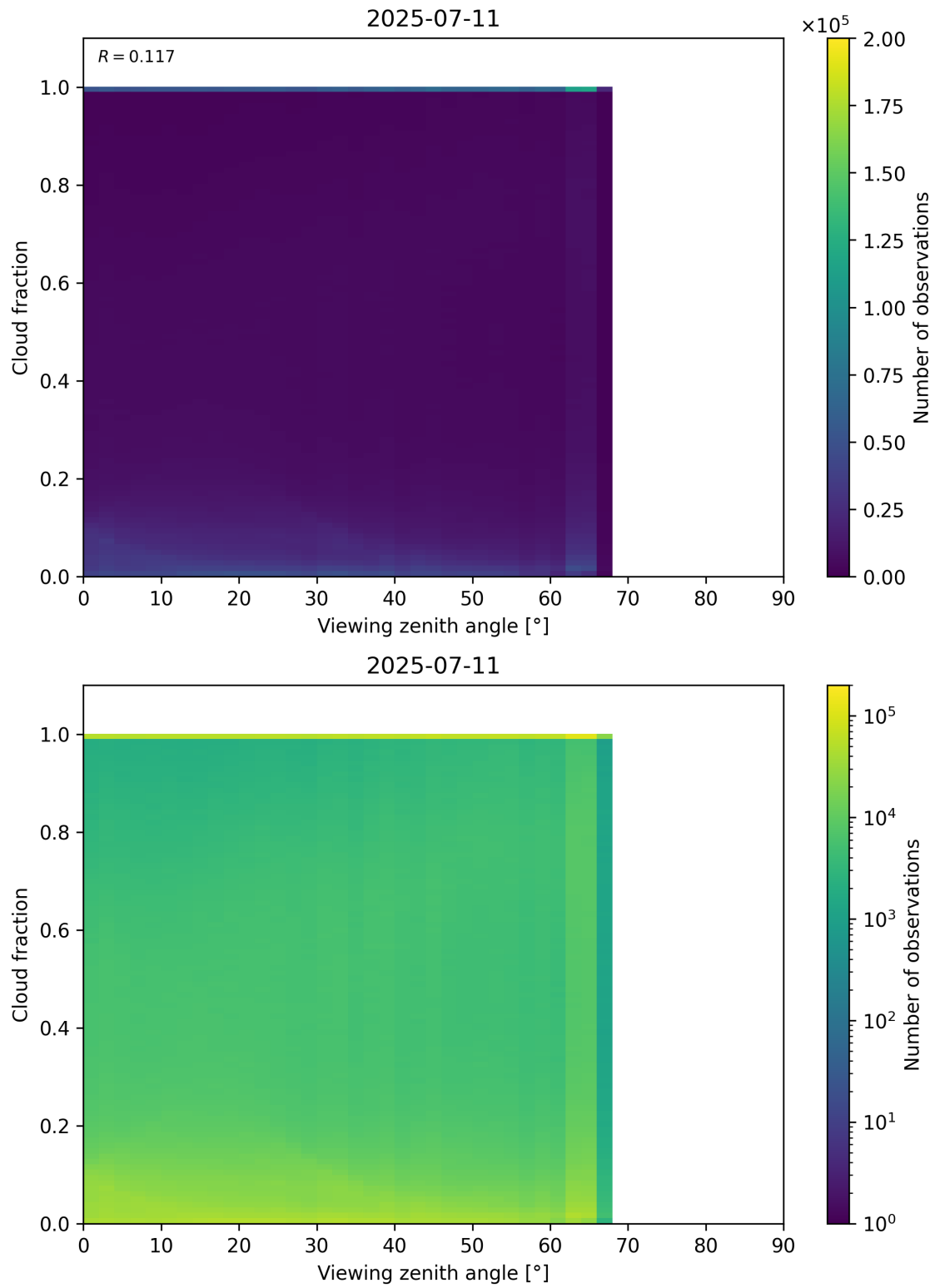
Figure 120: Scatter density plot of “Viewing zenith angle” against “Cloud fraction” for 2025-07-10 to 2025-07-12.
