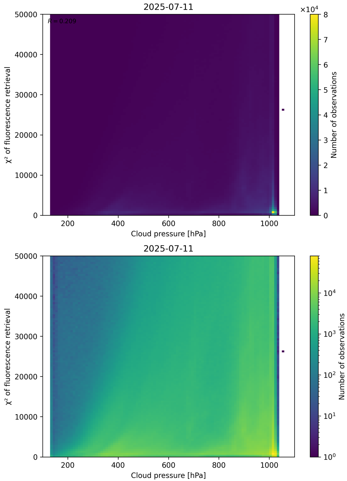
Figure 78: Scatter density plot of “Cloud pressure” against “ \chi^2 of fluorescence retrieval” for 2025-07-10 to 2025-07-12.
