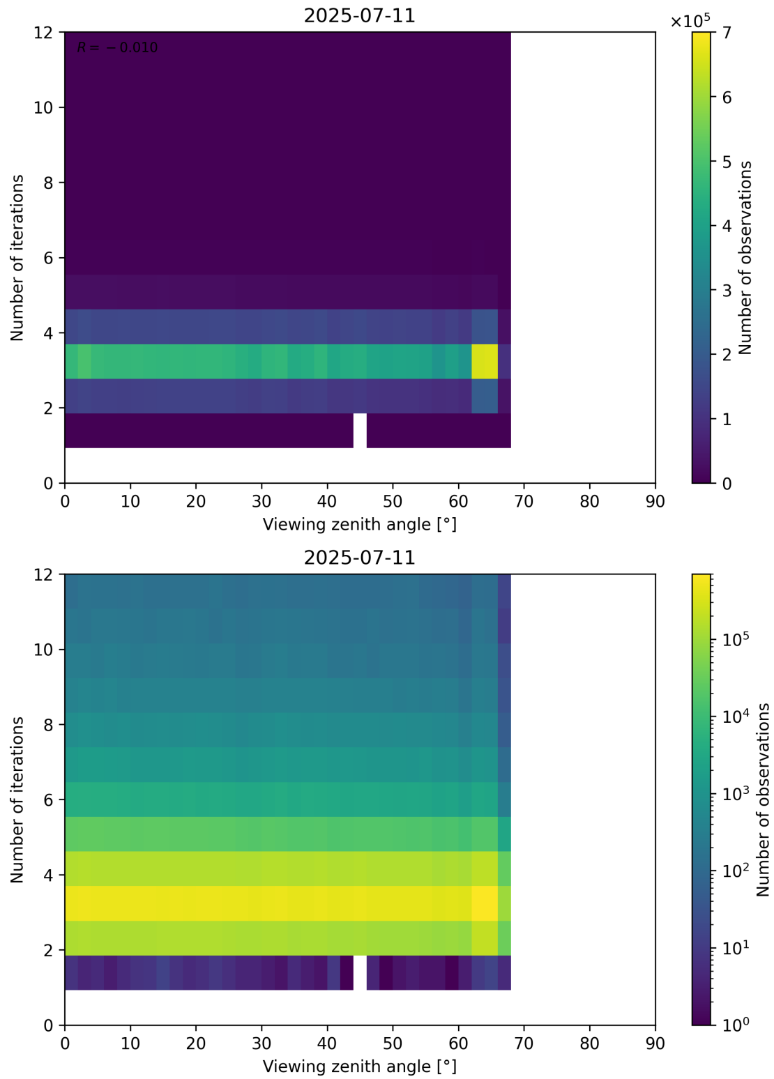
Figure 124: Scatter density plot of “Viewing zenith angle” against “Number of iterations” for 2025-07-10 to 2025-07-12.
