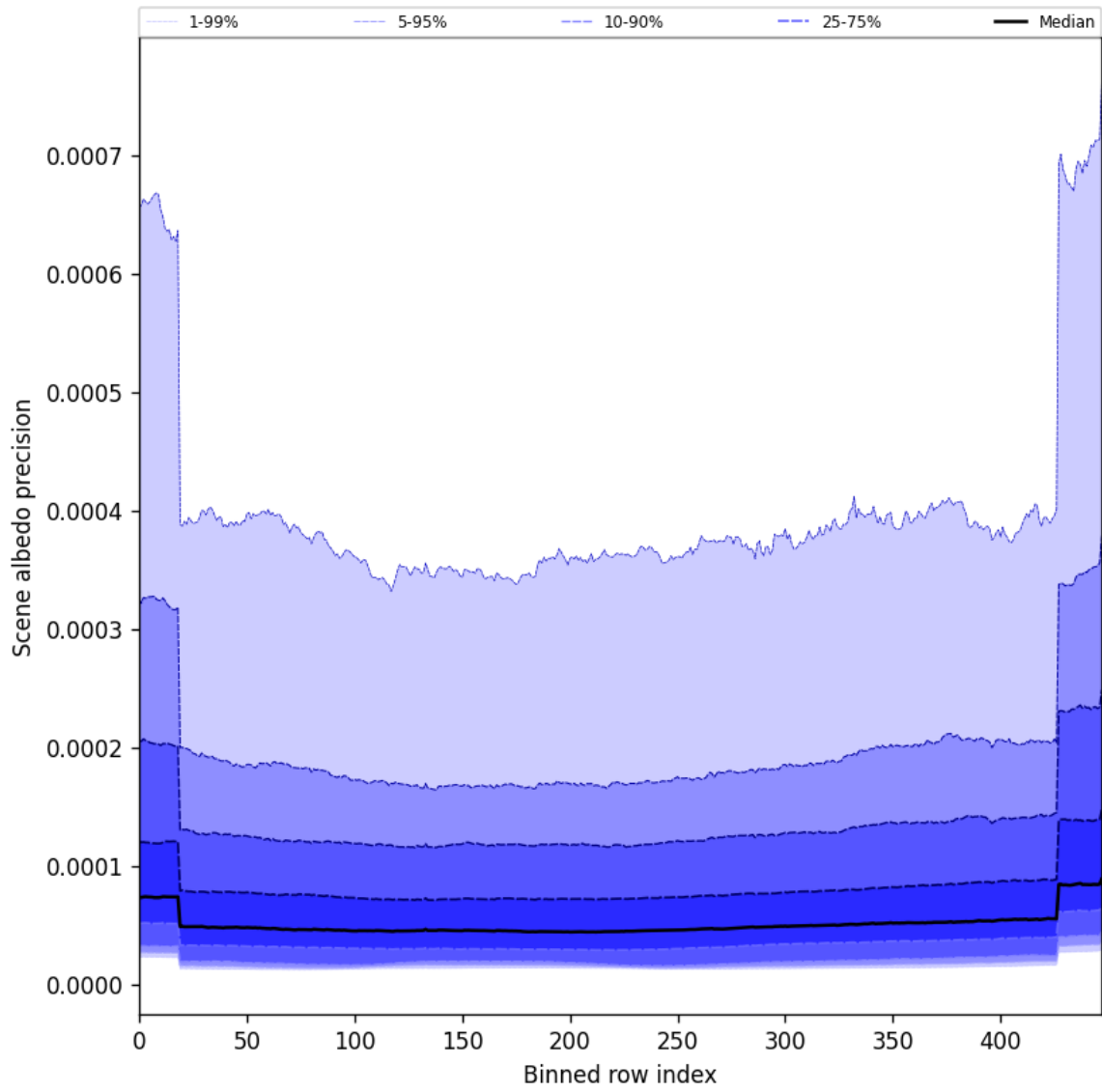
Figure 52: Along track statistics of “Scene albedo precision” for 2025-07-10 to 2025-07-12
