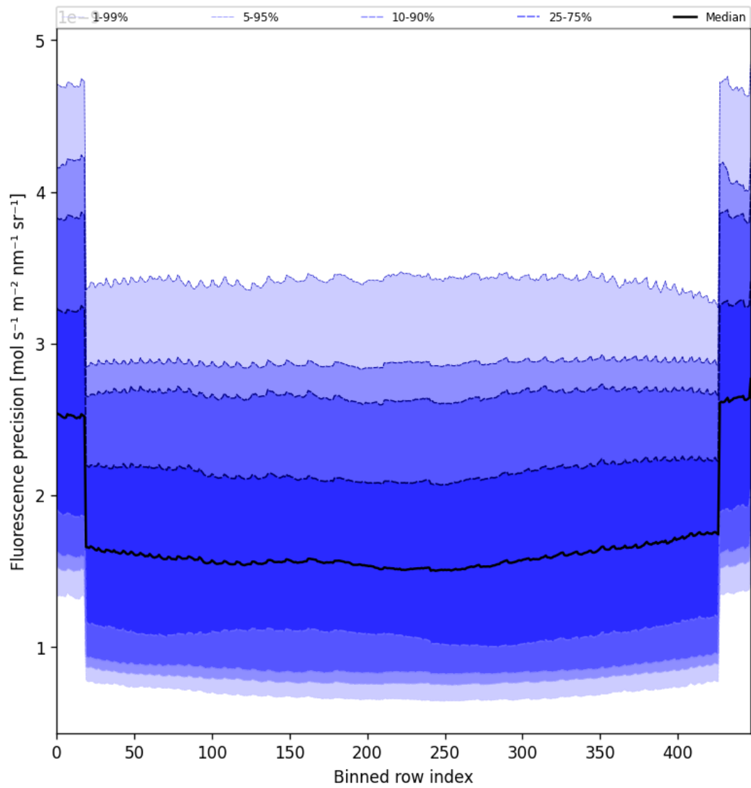
Figure 58: Along track statistics of “Fluorescence precision” for 2025-07-10 to 2025-07-12
