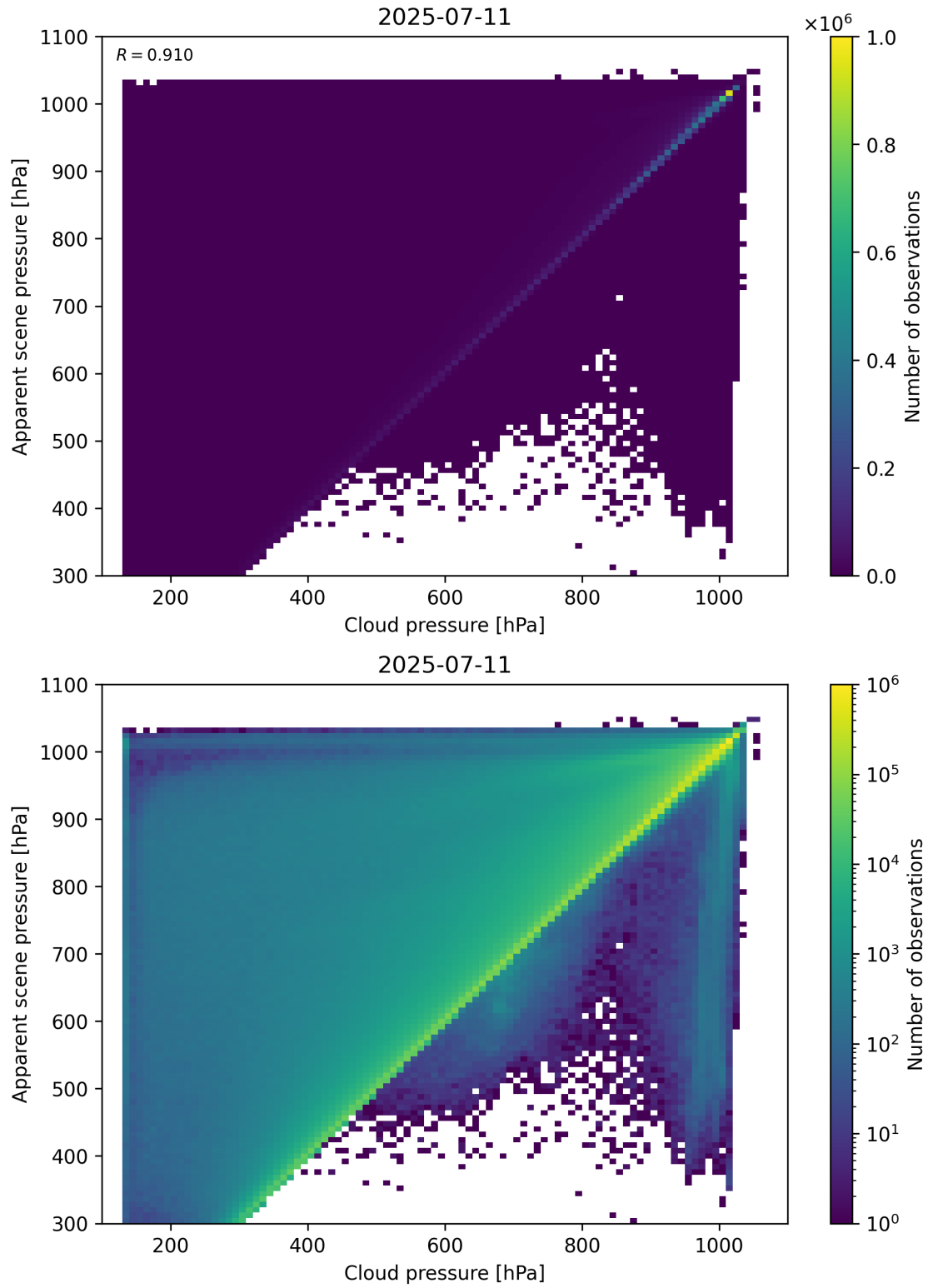
Figure 77: Scatter density plot of “Cloud pressure” against “Apparent scene pressure” for 2025-07-10 to 2025-07-12.
