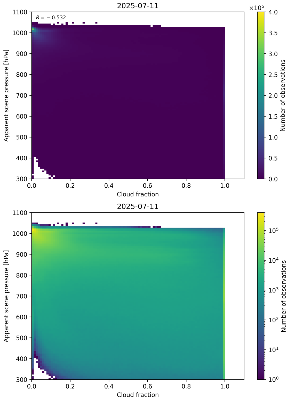
Figure 70: Scatter density plot of “Cloud fraction” against “Apparent scene pressure” for 2025-07-10 to 2025-07-12.
