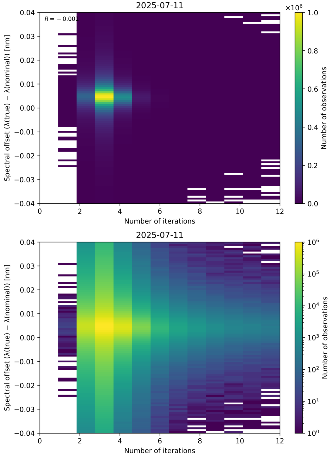
Figure 100: Scatter density plot of “Number of iterations” against “Spectral offset ( \lambda_{\text{true}} - \lambda_{\text{nominal}} )” for 2025-07-10 to 2025-07-12.
