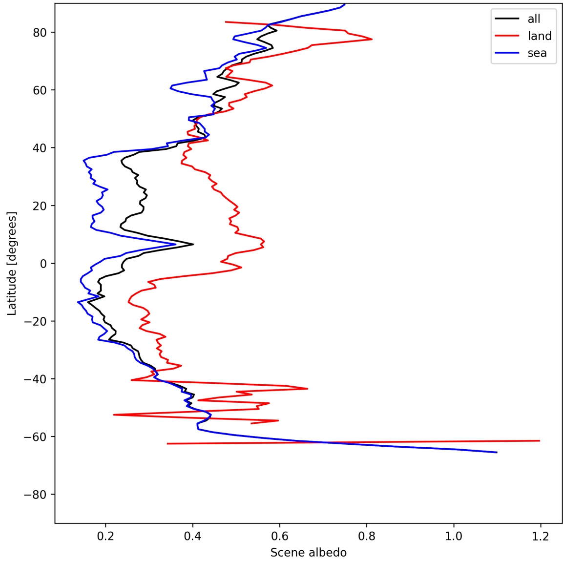
Figure 17: Zonal average of “Scene albedo” for 2025-07-10 to 2025-07-12.
