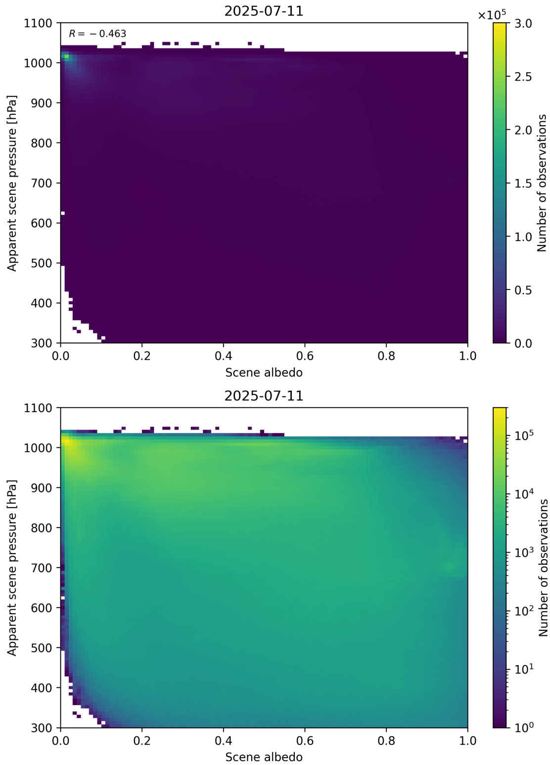
Figure 102: Scatter density plot of “Scene albedo” against “Apparent scene pressure” for 2025-07-10 to 2025-07-12.
