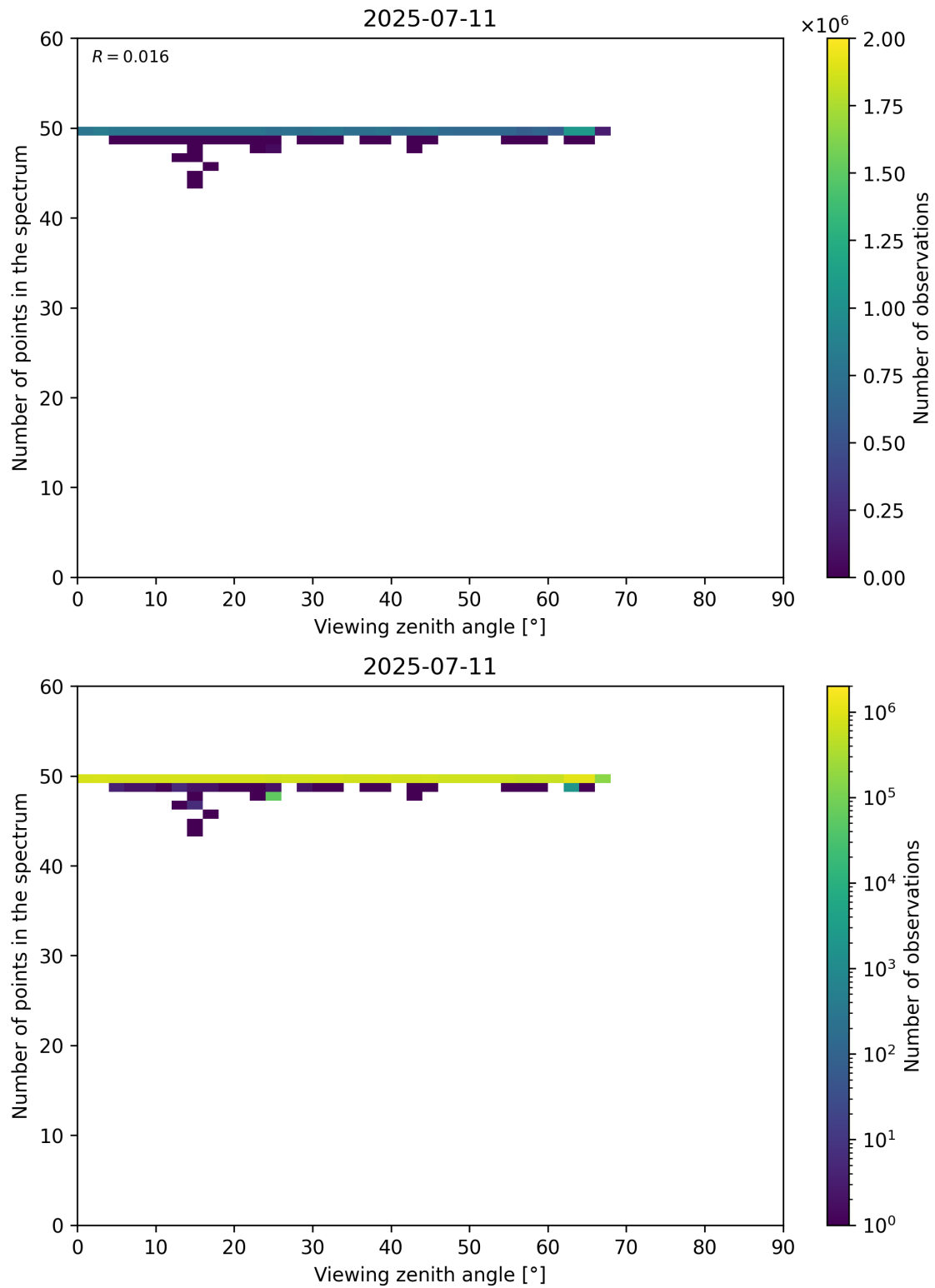
Figure 125: Scatter density plot of “Viewing zenith angle” against “Number of points in the spectrum” for 2025-07-10 to 2025-07-12.
