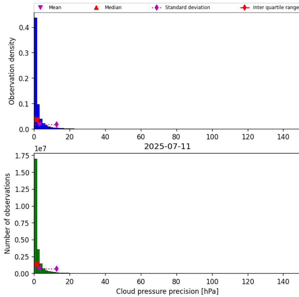
Figure 31: Histogram of “Cloud pressure precision” for 2025-07-10 to 2025-07-12
