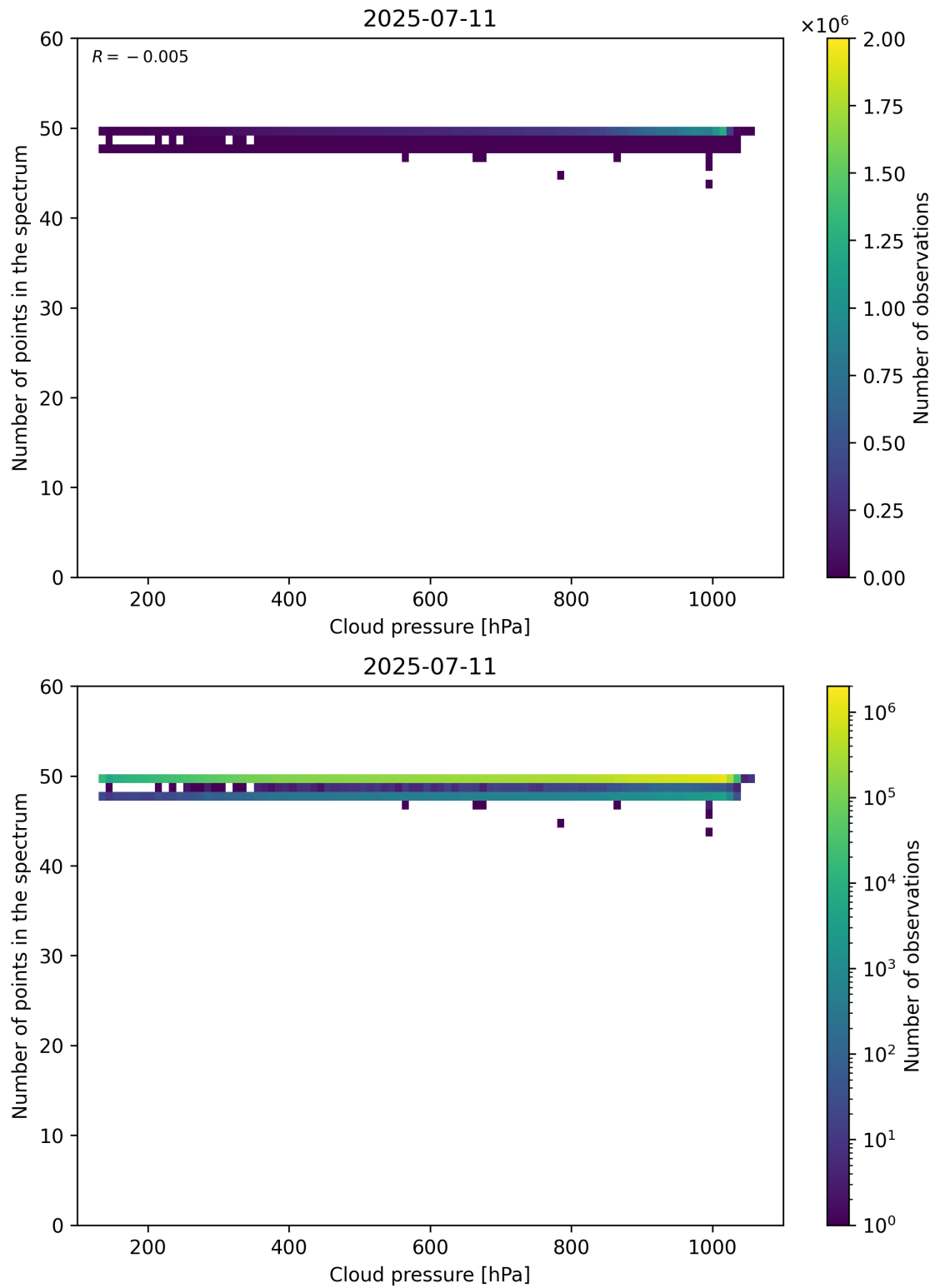
Figure 82: Scatter density plot of “Cloud pressure” against “Number of points in the spectrum” for 2025-07-10 to 2025-07-12.
