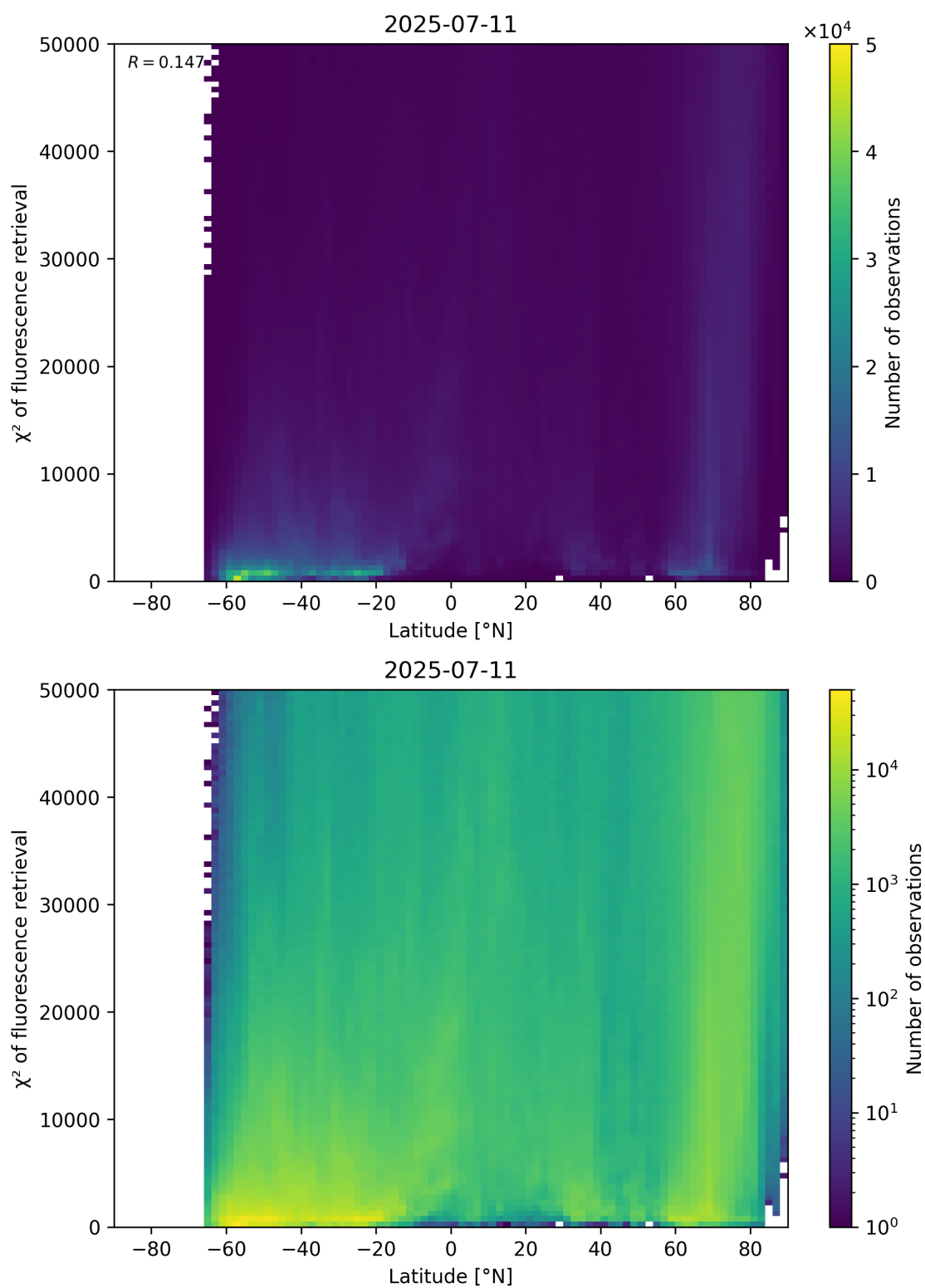
Figure 89: Scatter density plot of “Latitude” against “ \chi^2 of fluorescence retrieval” for 2025-07-10 to 2025-07-12.
