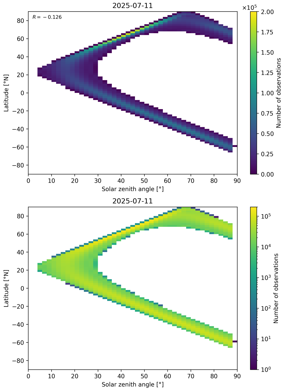
Figure 113: Scatter density plot of “Solar zenith angle” against “Latitude” for 2025-07-10 to 2025-07-12.
