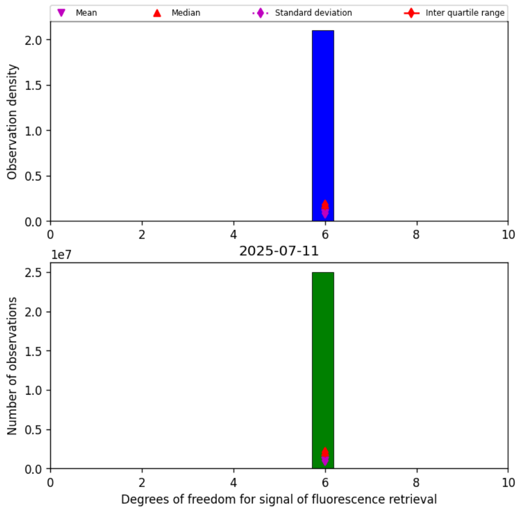
Figure 43: Histogram of “Degrees of freedom for signal of fluorescence retrieval” for 2025-07-10 to 2025-07-12
