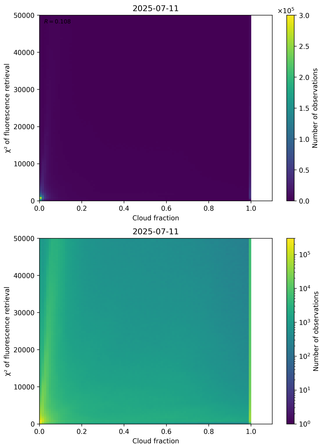
Figure 71: Scatter density plot of “Cloud fraction” against “ \chi^2 of fluorescence retrieval” for 2025-07-10 to 2025-07-12.
