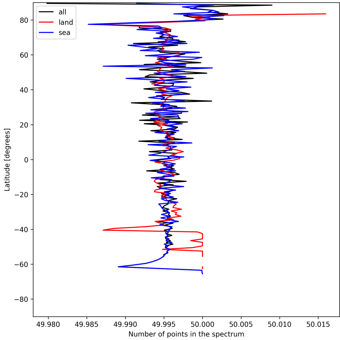
Figure 27: Zonal average of “Number of points in the spectrum” for 2025-07-10 to 2025-07-12.
