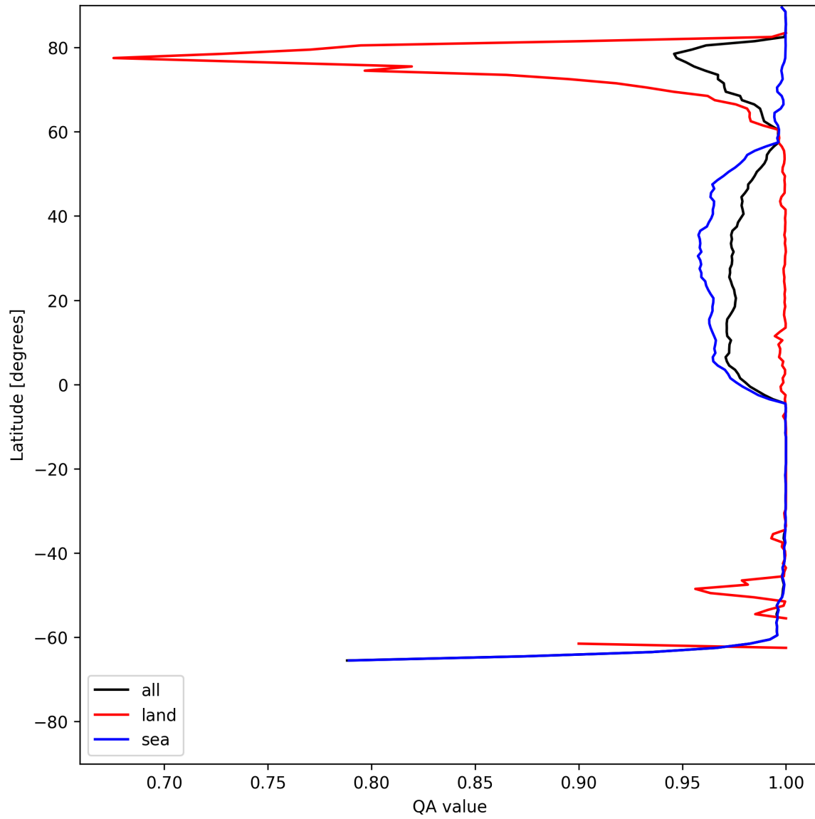
Figure 12: Zonal average of “QA value” for 2025-07-10 to 2025-07-12.
