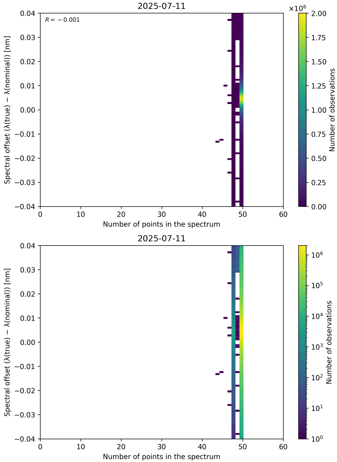
Figure 101: Scatter density plot of “Number of points in the spectrum” against “Spectral offset ( \lambda_{\text{true}} - \lambda_{\text{nominal}} )” for 2025-07-10 to 2025-07-12.
