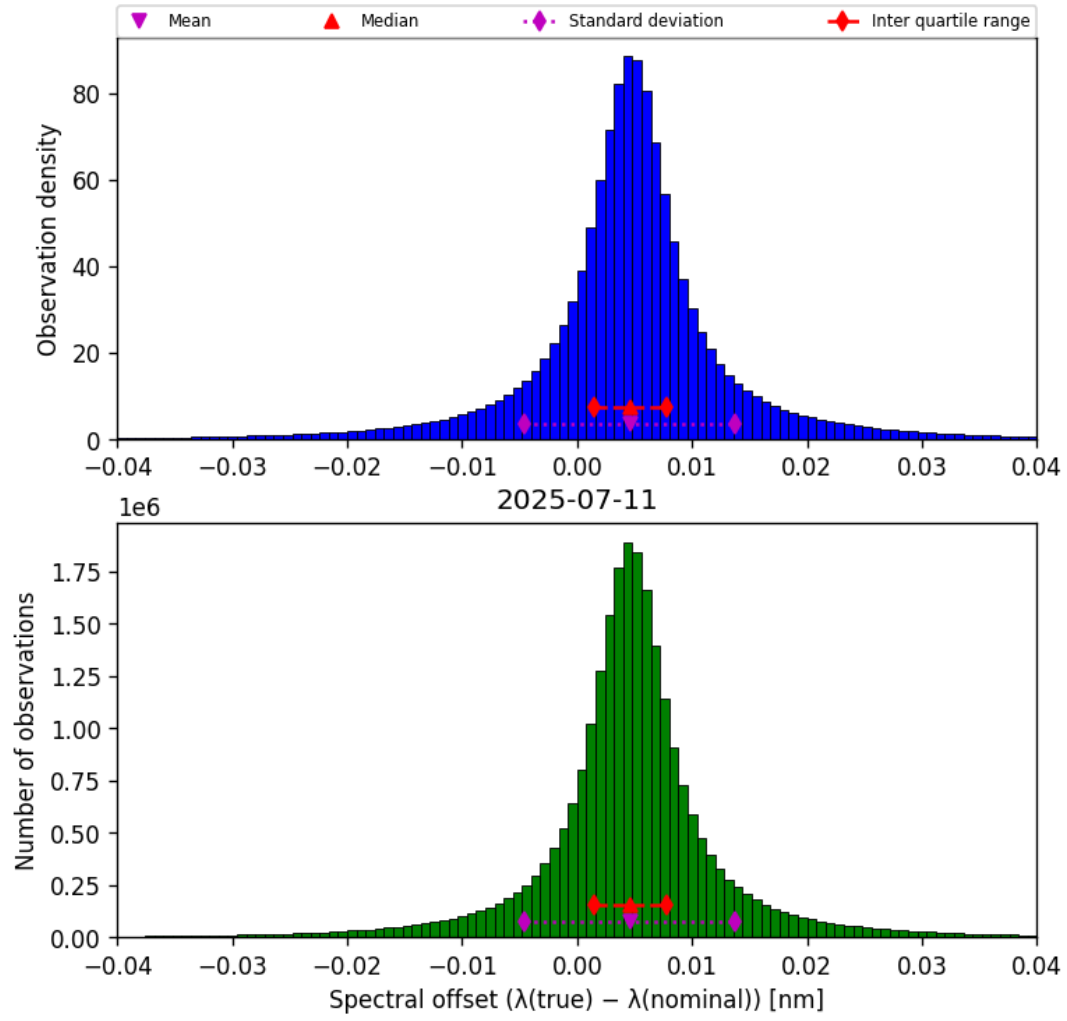
Figure 45: Histogram of “Spectral offset ( \lambda_{\text{true}} - \lambda_{\text{nominal}} )” for 2025-07-10 to 2025-07-12
