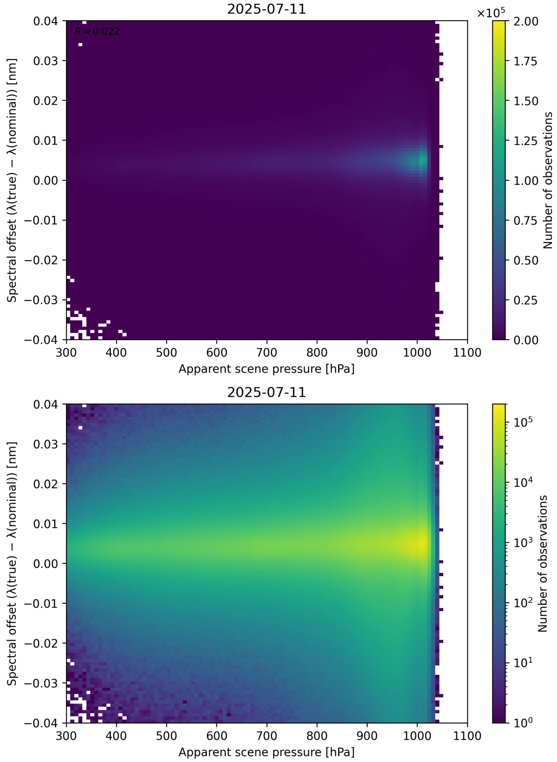
Figure 67: Scatter density plot of “Apparent scene pressure” against “Spectral offset ( \lambda_{\text{true}} - \lambda_{\text{nominal}} )” for 2025-07-10 to 2025-07-12.
