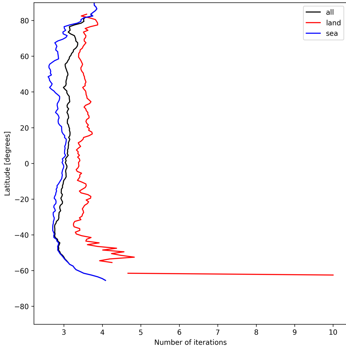
Figure 22: Zonal average of “Number of iterations” for 2025-07-10 to 2025-07-12.
