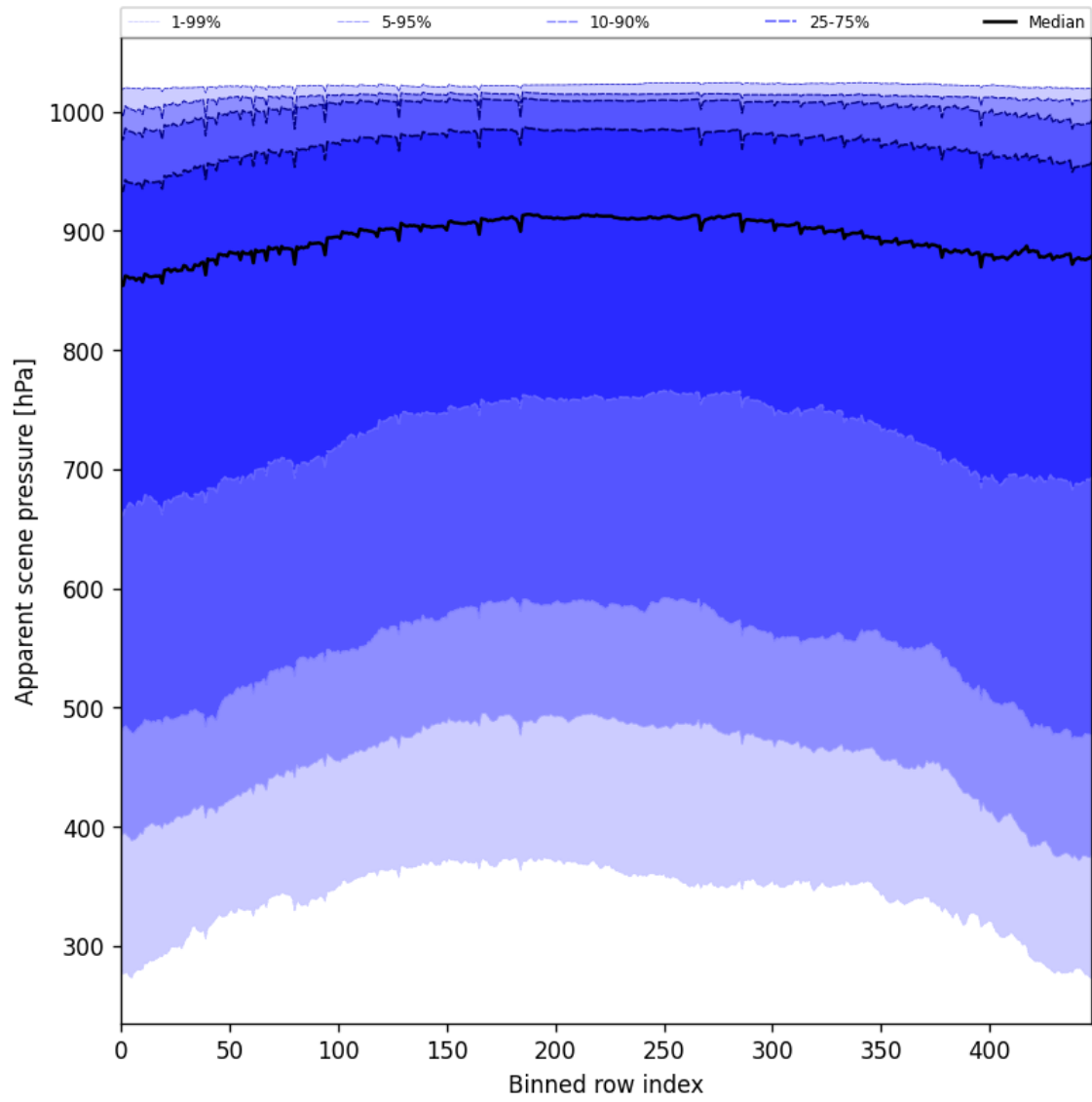
Figure 53: Along track statistics of “Apparent scene pressure” for 2025-07-10 to 2025-07-12
