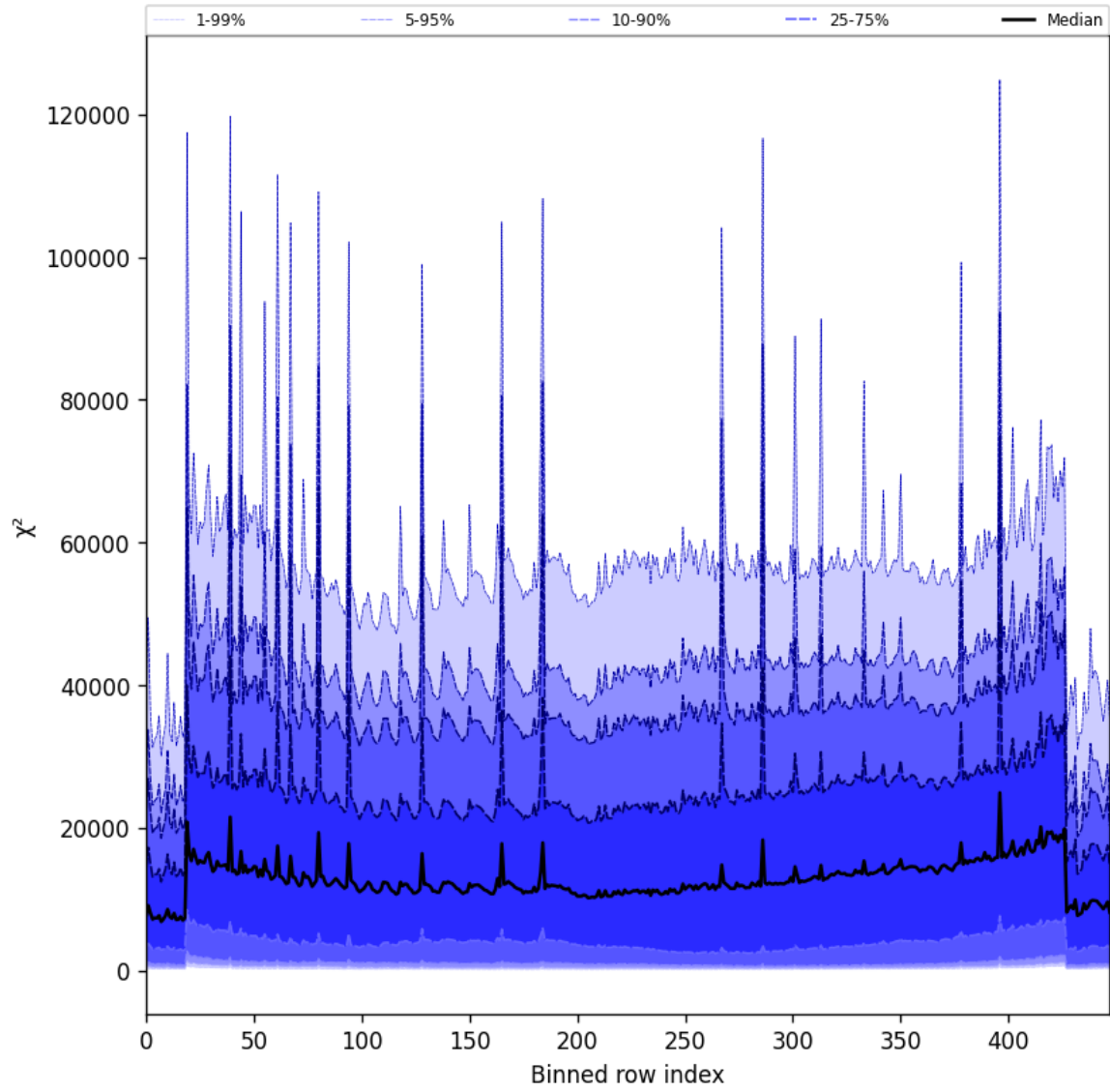
Figure 55: Along track statistics of " \chi^2 " for 2025-07-10 to 2025-07-12
