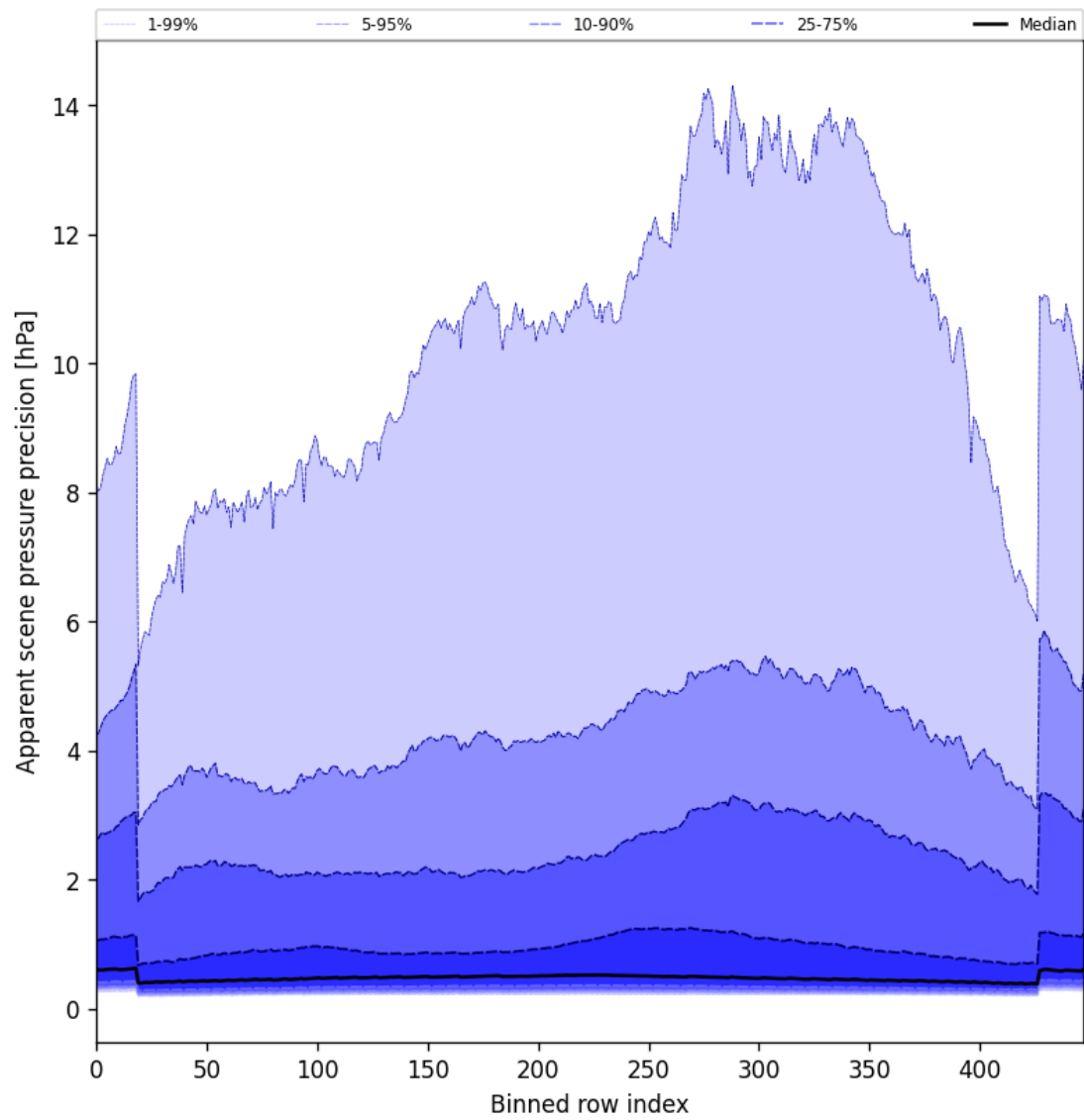
Figure 54: Along track statistics of “Apparent scene pressure precision” for 2025-07-10 to 2025-07-12
