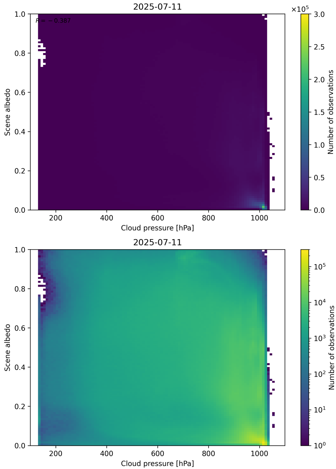
Figure 83: Scatter density plot of “Cloud pressure” against “Scene albedo” for 2025-07-10 to 2025-07-12.
