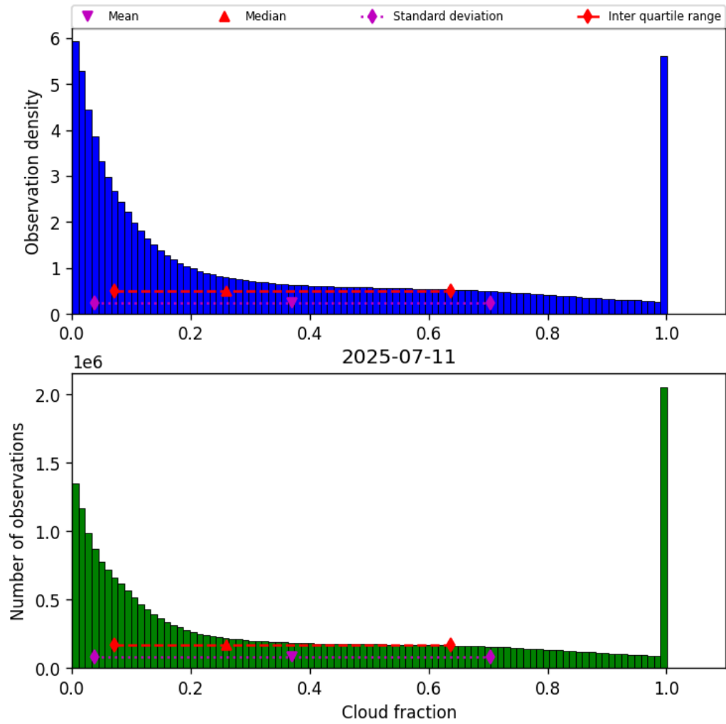
Figure 32: Histogram of “Cloud fraction” for 2025-07-10 to 2025-07-12
