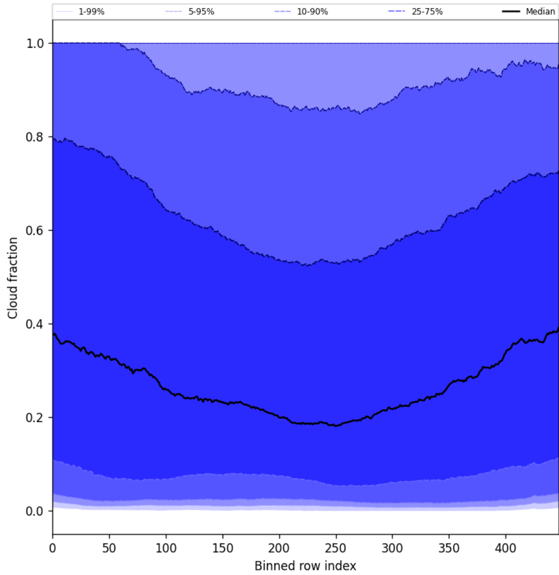
Figure 49: Along track statistics of “Cloud fraction” for 2025-07-10 to 2025-07-12
