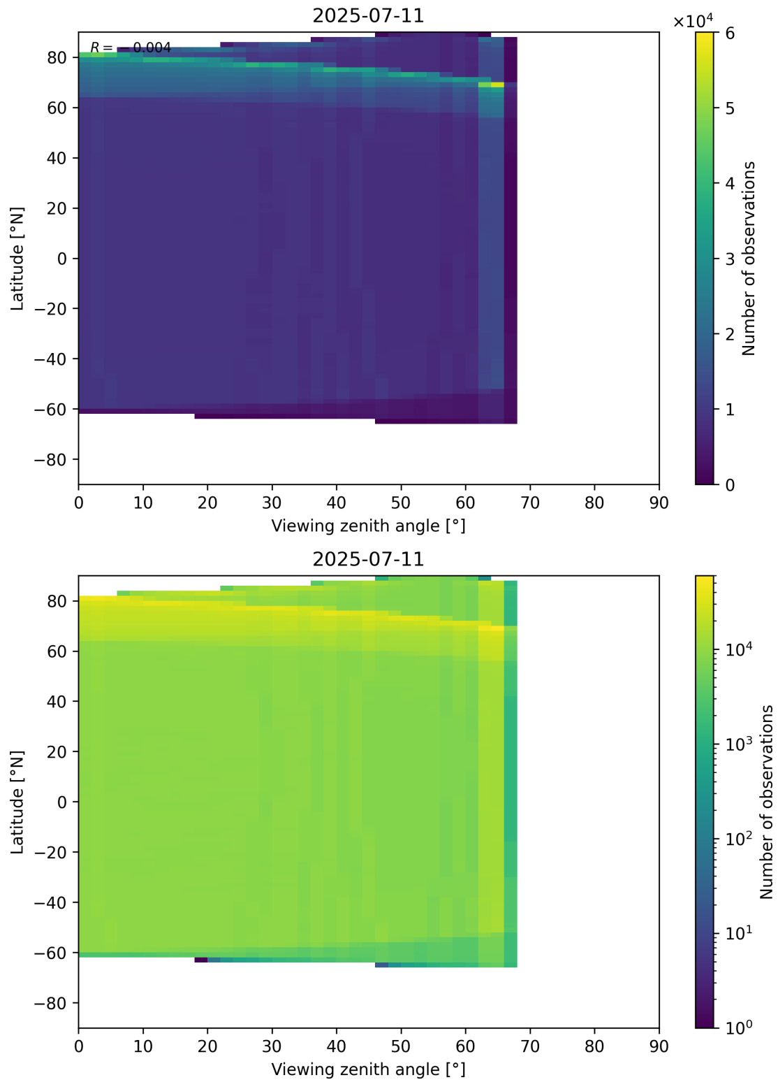
Figure 123: Scatter density plot of “Viewing zenith angle” against “Latitude” for 2025-07-10 to 2025-07-12.
