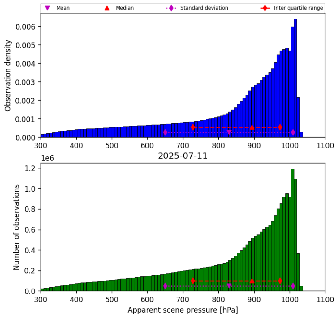
Figure 36: Histogram of “Apparent scene pressure” for 2025-07-10 to 2025-07-12
