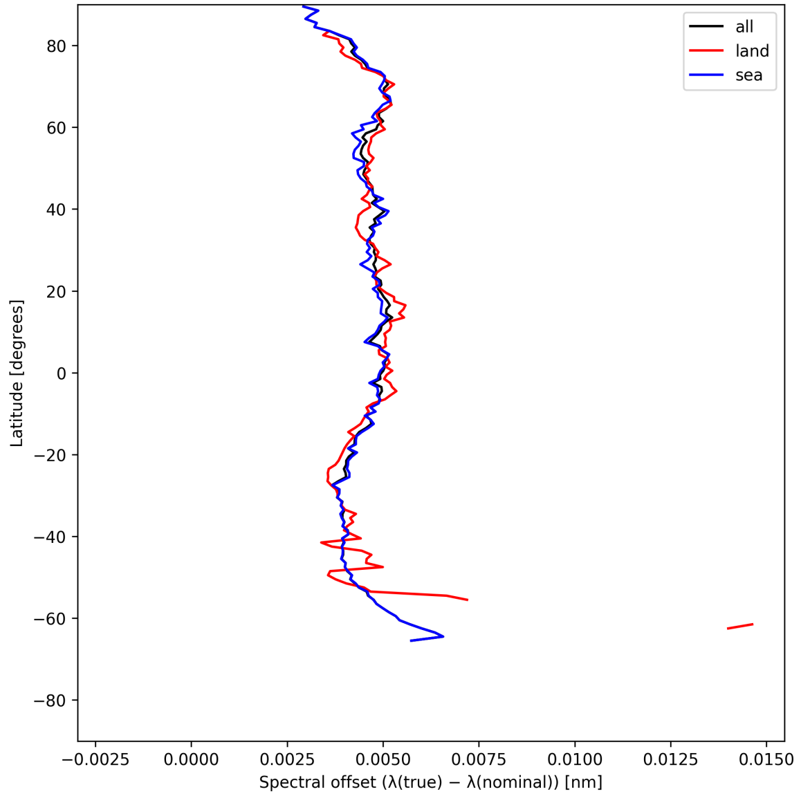
Figure 28: Zonal average of “Spectral offset ( \lambda_{\text{true}} - \lambda_{\text{nominal}} )” for 2025-07-10 to 2025-07-12.
