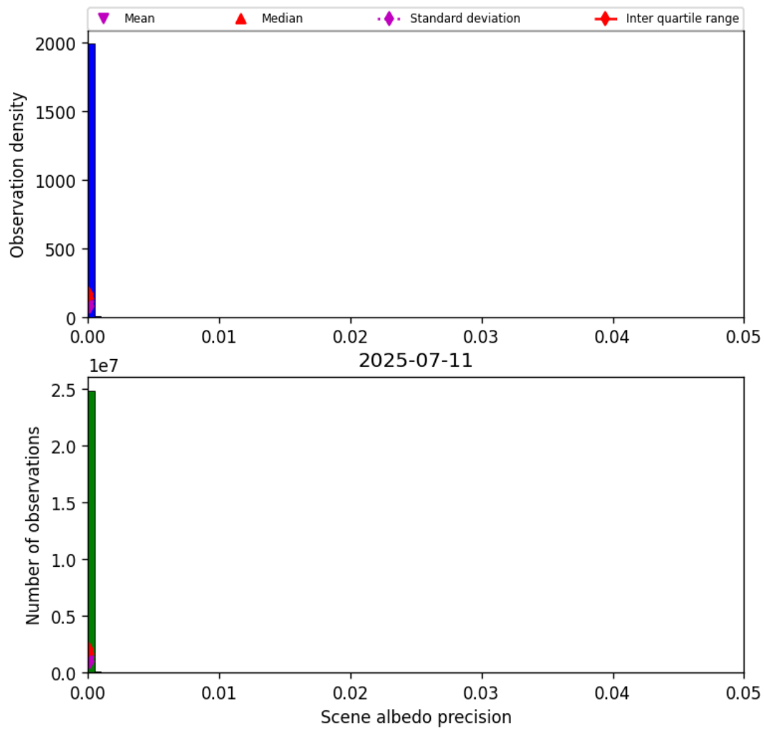
Figure 35: Histogram of “Scene albedo precision” for 2025-07-10 to 2025-07-12
