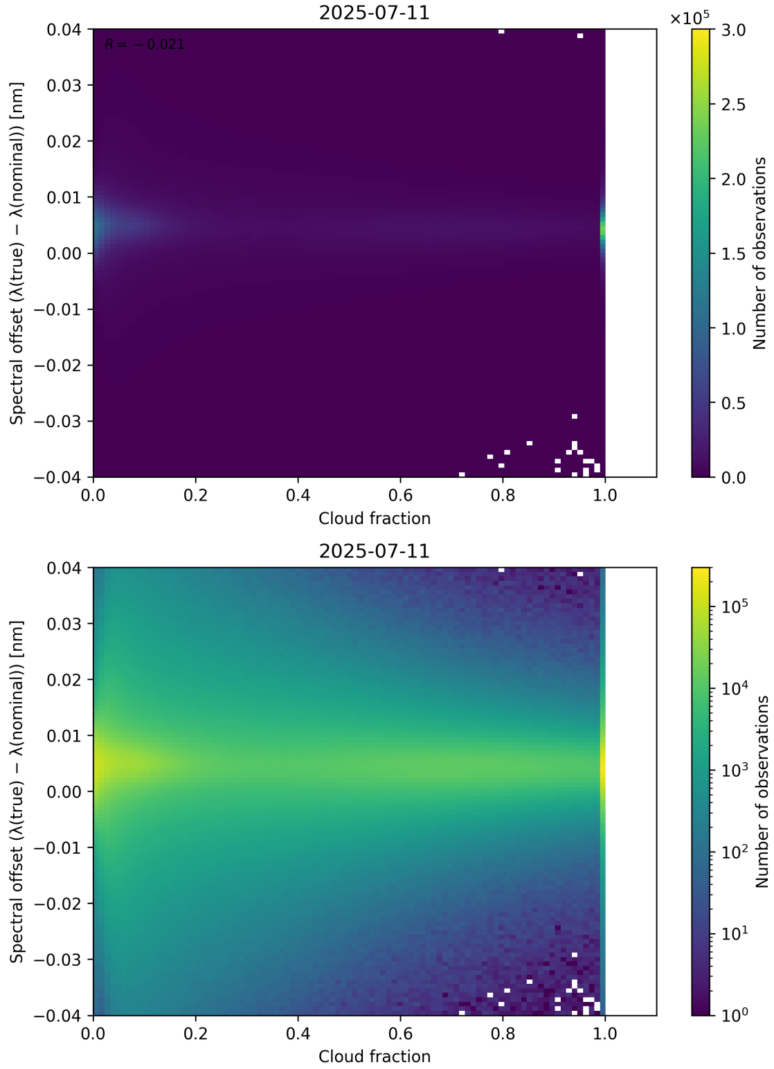
Figure 76: Scatter density plot of “Cloud fraction” against “Spectral offset ( \lambda_{\text{true}} - \lambda_{\text{nominal}} )” for 2025-07-10 to 2025-07-12.
