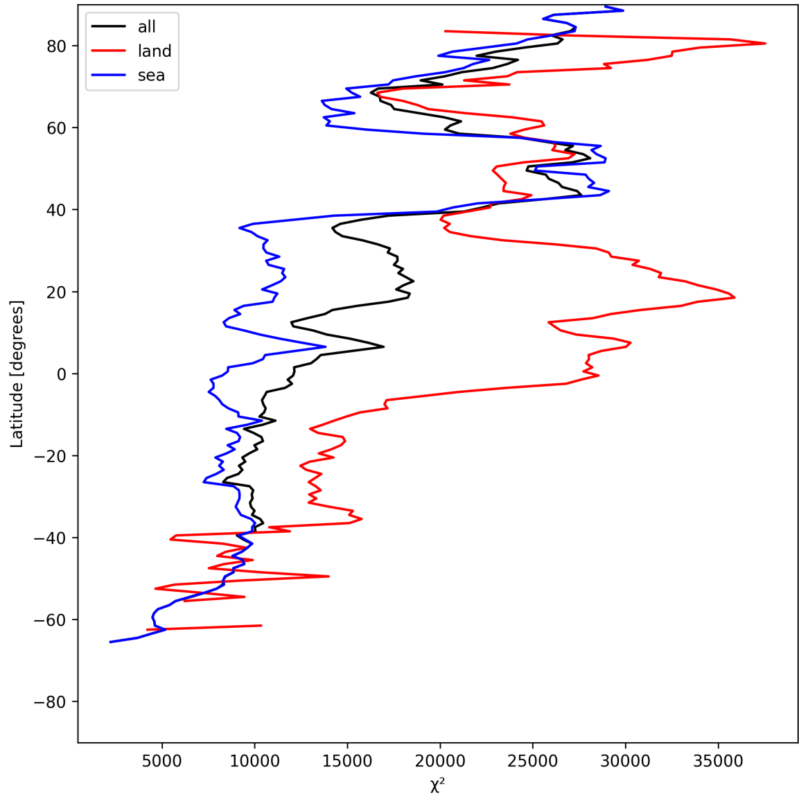
Figure 21: Zonal average of “ \chi^2 ” for 2025-07-10 to 2025-07-12.
