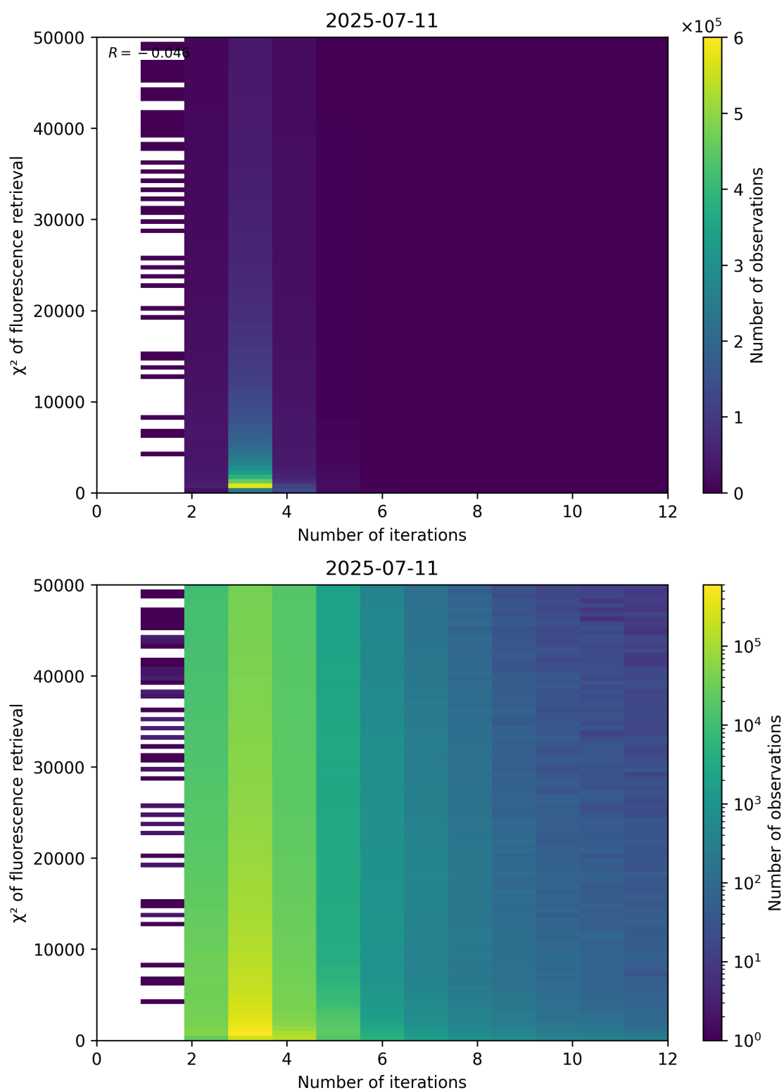
Figure 97: Scatter density plot of “Number of iterations” against “ \chi^2 of fluorescence retrieval” for 2025-07-10 to 2025-07-12.
