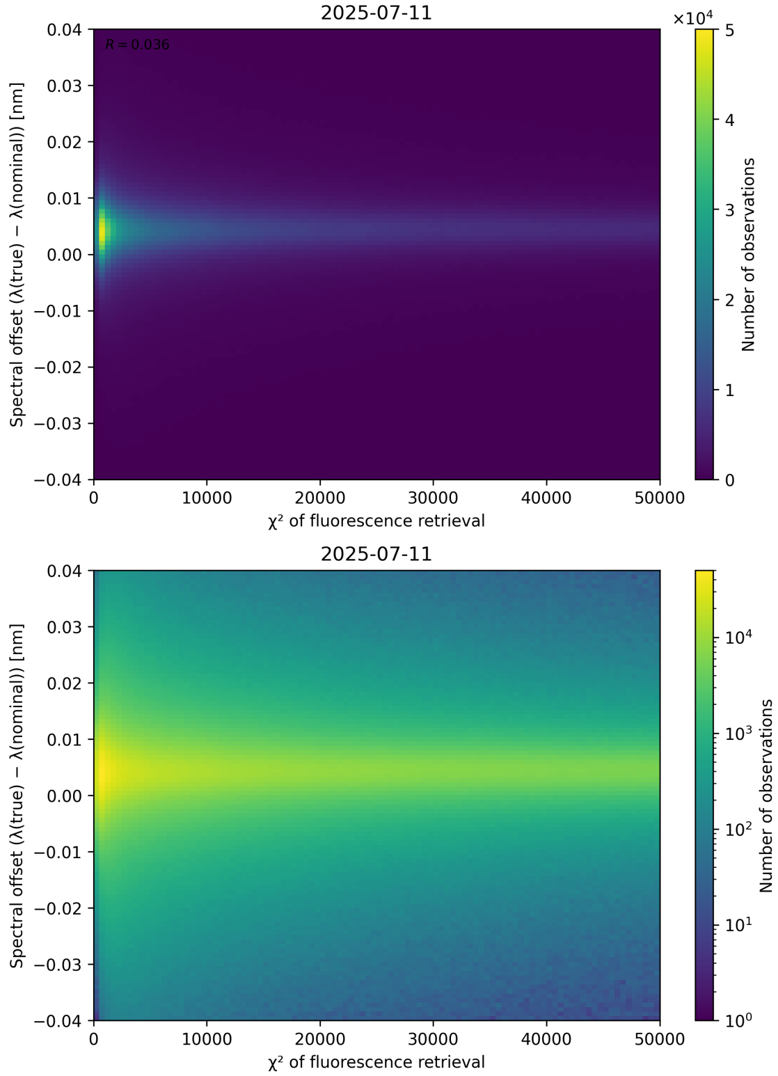
Figure 69: Scatter density plot of “ \chi^2 of fluorescence retrieval” against “Spectral offset ( \lambda_{\text{true}} - \lambda_{\text{nominal}} )” for 2025-07-10 to 2025-07-12.
