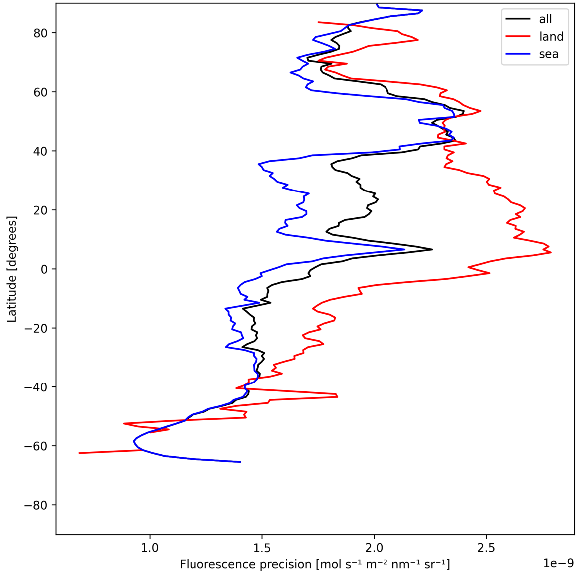
Figure 24: Zonal average of "Fluorescence precision" for 2025-07-10 to 2025-07-12.
