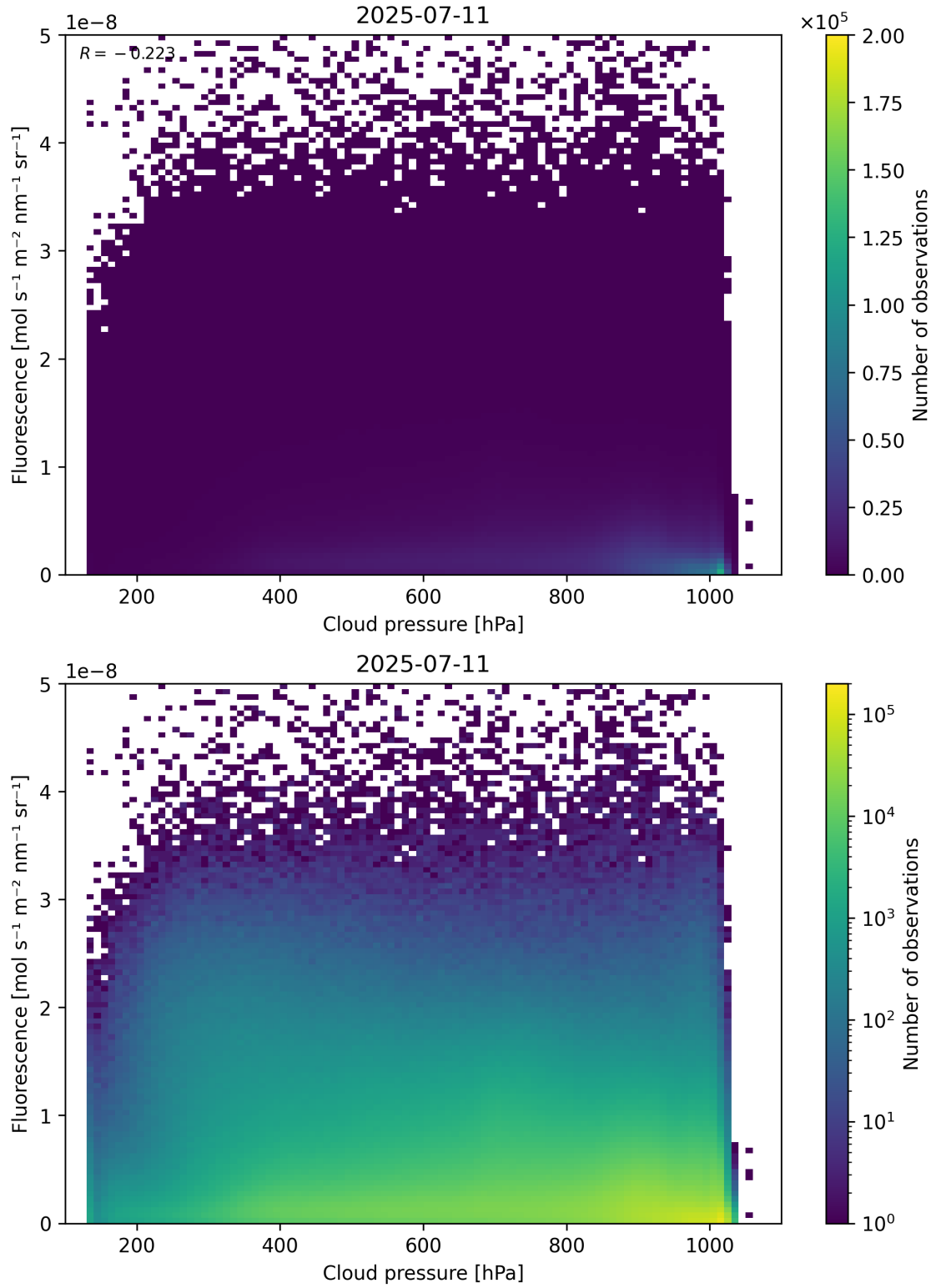
Figure 80: Scatter density plot of “Cloud pressure” against “Fluorescence” for 2025-07-10 to 2025-07-12.
