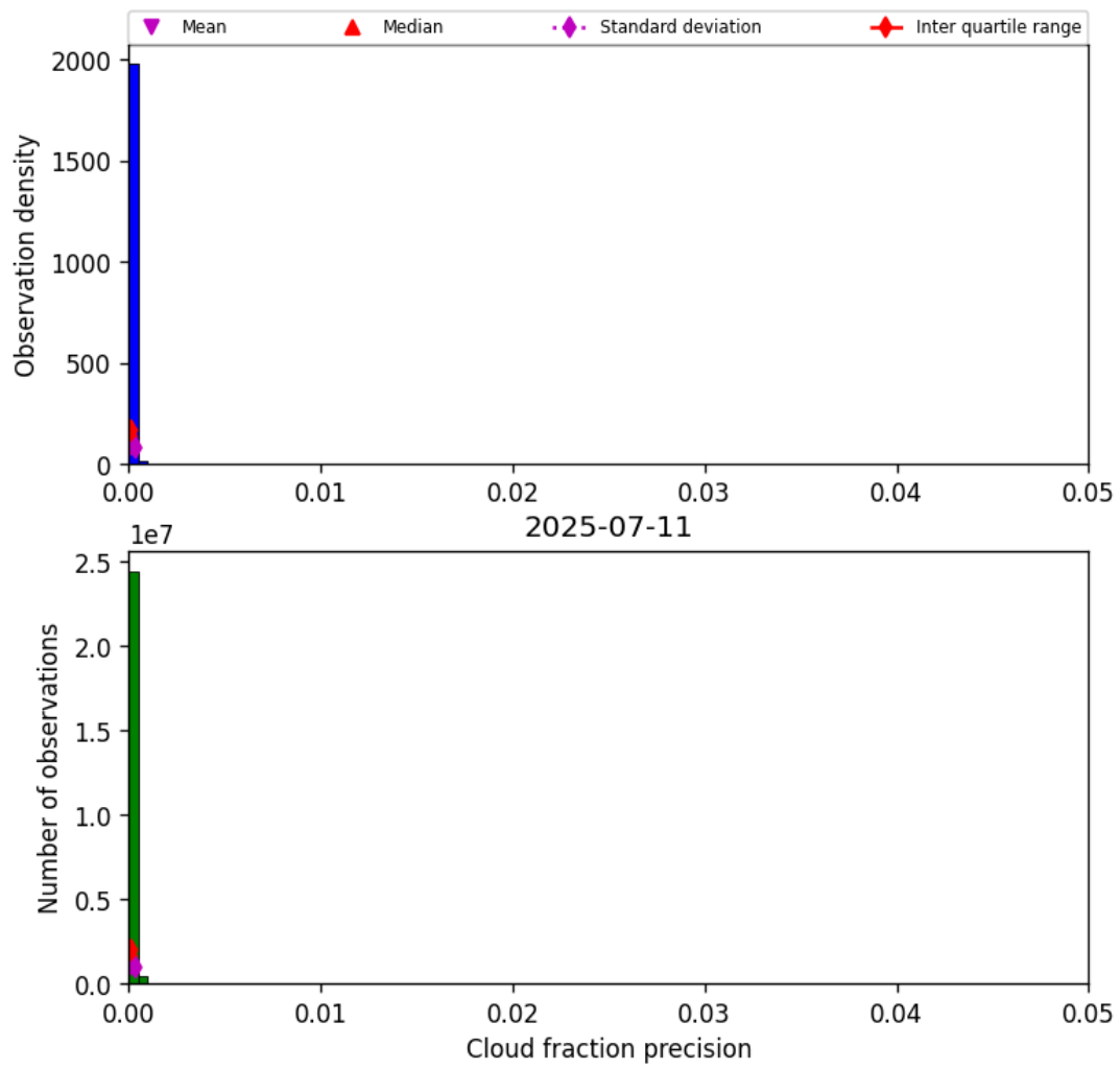
Figure 33: Histogram of “Cloud fraction precision” for 2025-07-10 to 2025-07-12
