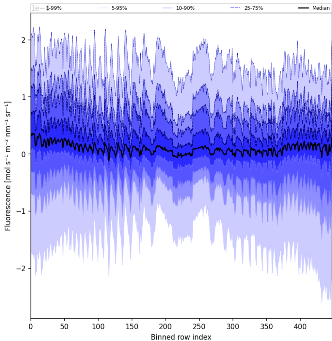
Figure 57: Along track statistics of “Fluorescence” for 2025-07-10 to 2025-07-12
