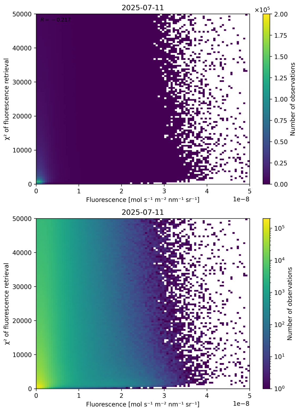
Figure 85: Scatter density plot of “Fluorescence” against “ \chi^2 of fluorescence retrieval” for 2025-07-10 to 2025-07-12.
