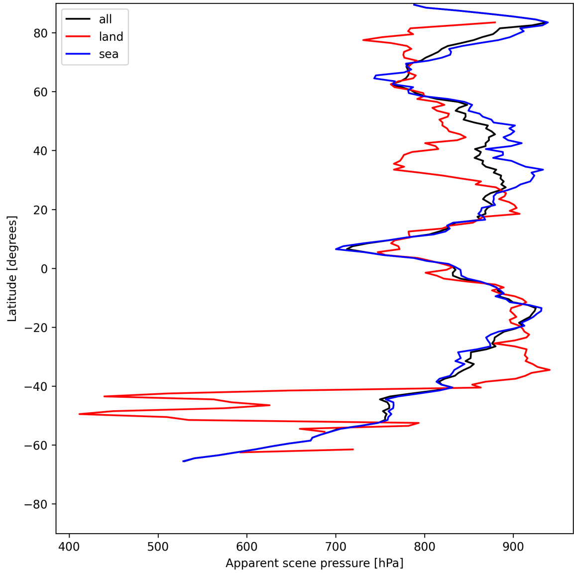
Figure 19: Zonal average of “Apparent scene pressure” for 2025-07-10 to 2025-07-12.
