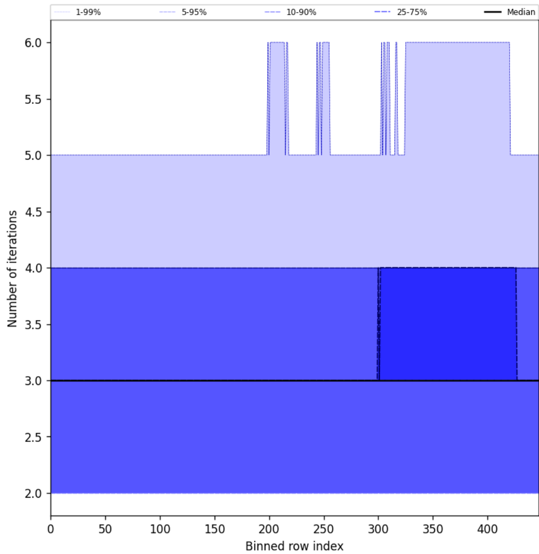
Figure 56: Along track statistics of “Number of iterations” for 2025-07-10 to 2025-07-12
