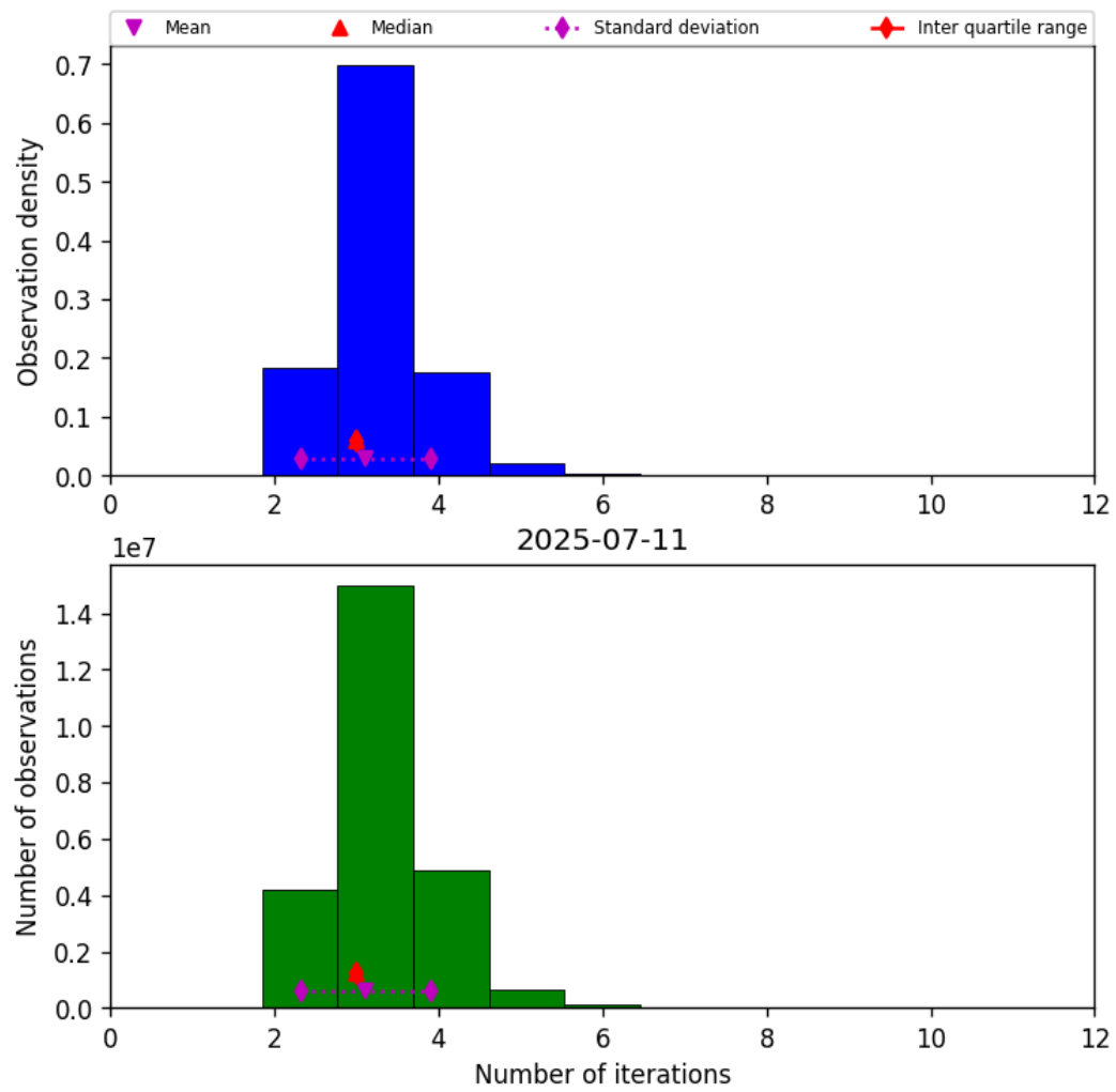
Figure 39: Histogram of “Number of iterations” for 2025-07-10 to 2025-07-12
