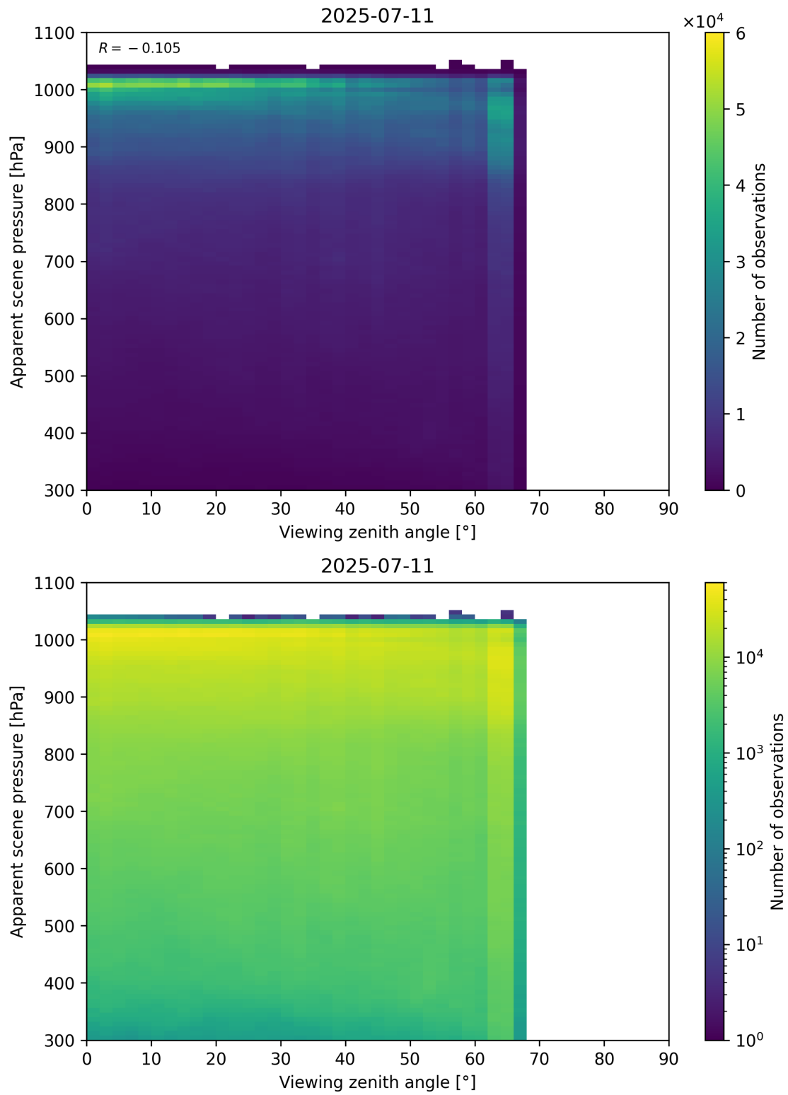
Figure 118: Scatter density plot of “Viewing zenith angle” against “Apparent scene pressure” for 2025-07-10 to 2025-07-12.
