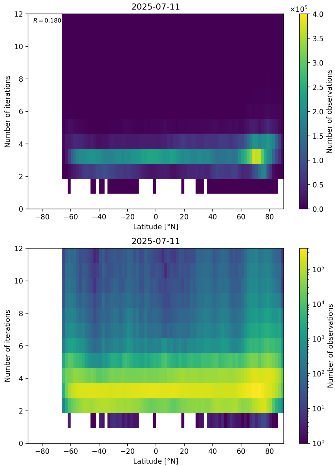
Figure 93: Scatter density plot of “Latitude” against “Number of iterations” for 2025-07-10 to 2025-07-12.
