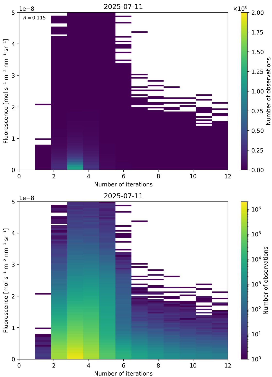
Figure 98: Scatter density plot of “Number of iterations” against “Fluorescence” for 2025-07-10 to 2025-07-12.
