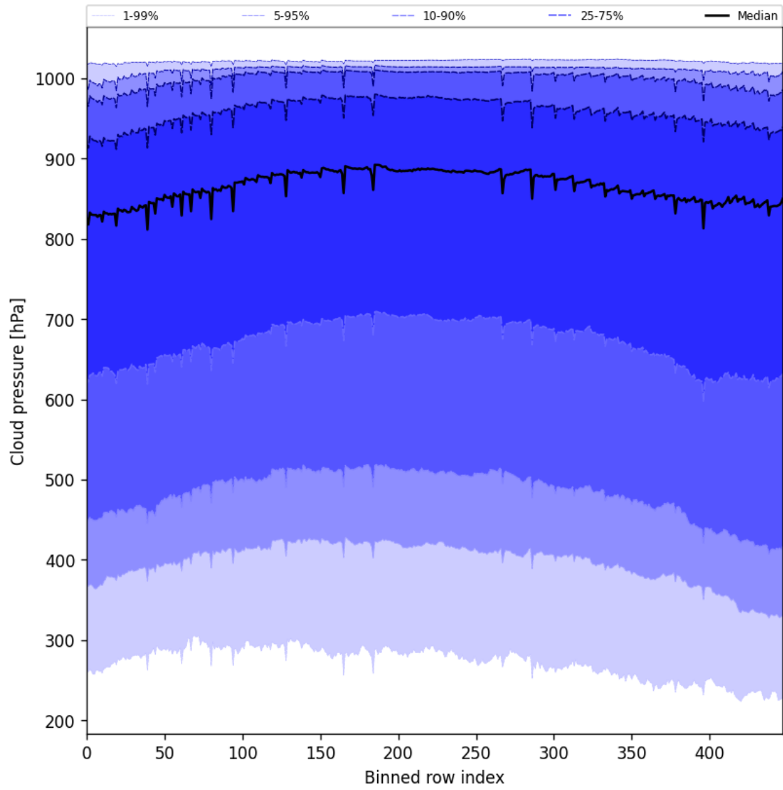
Figure 47: Along track statistics of “Cloud pressure” for 2025-07-10 to 2025-07-12
