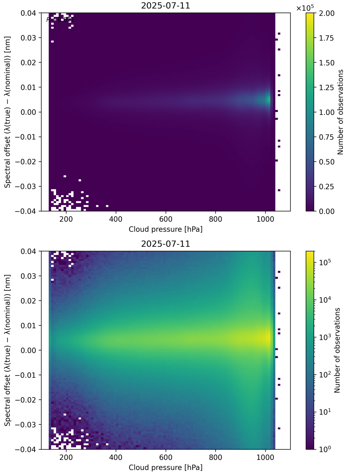
Figure 84: Scatter density plot of “Cloud pressure” against “Spectral offset ( \lambda_{\text{true}} - \lambda_{\text{nominal}} )” for 2025-07-10 to 2025-07-12.
