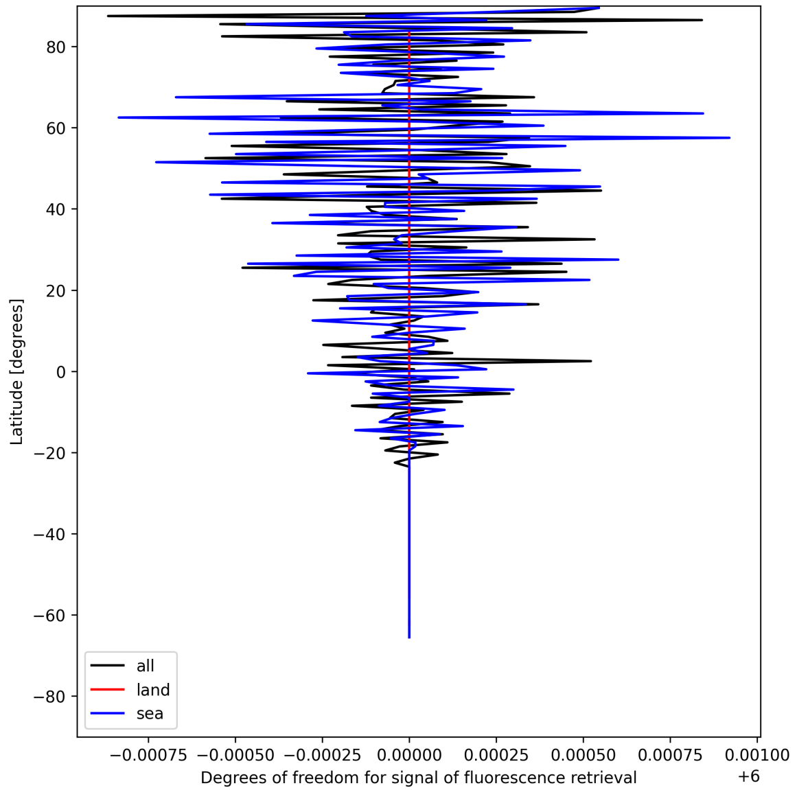
Figure 26: Zonal average of “Degrees of freedom for signal of fluorescence retrieval” for 2025-07-10 to 2025-07-12.
