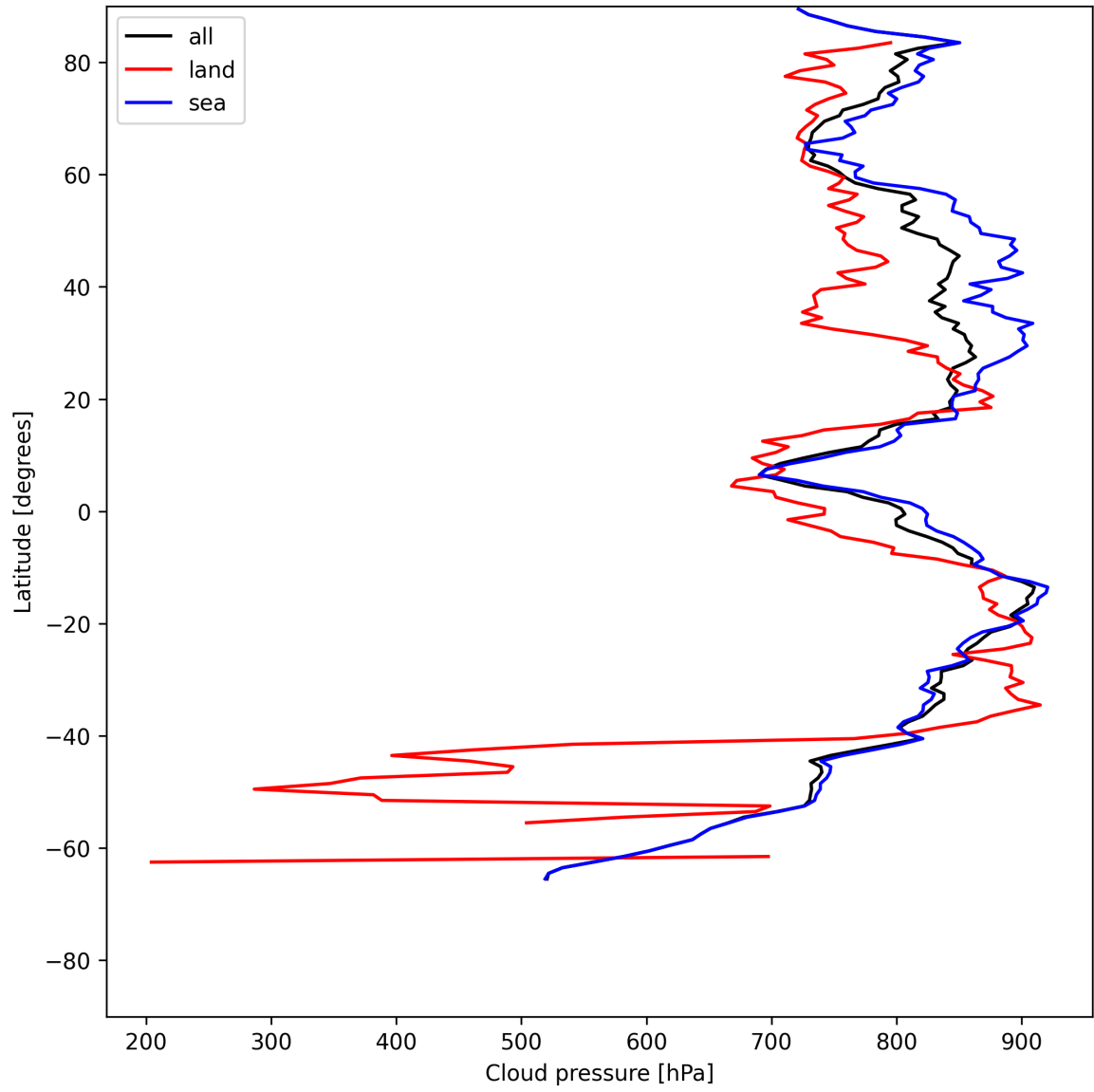
Figure 13: Zonal average of “Cloud pressure” for 2025-07-10 to 2025-07-12.
