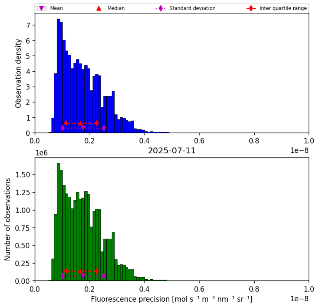
Figure 41: Histogram of “Fluorescence precision” for 2025-07-10 to 2025-07-12
