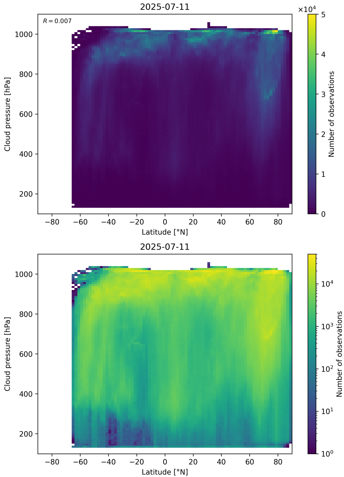
Figure 91: Scatter density plot of “Latitude” against “Cloud pressure” for 2025-07-10 to 2025-07-12.
