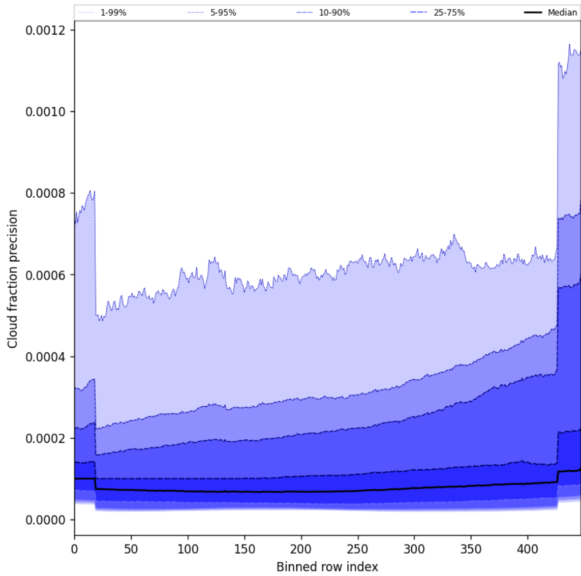
Figure 50: Along track statistics of “Cloud fraction precision” for 2025-07-10 to 2025-07-12
