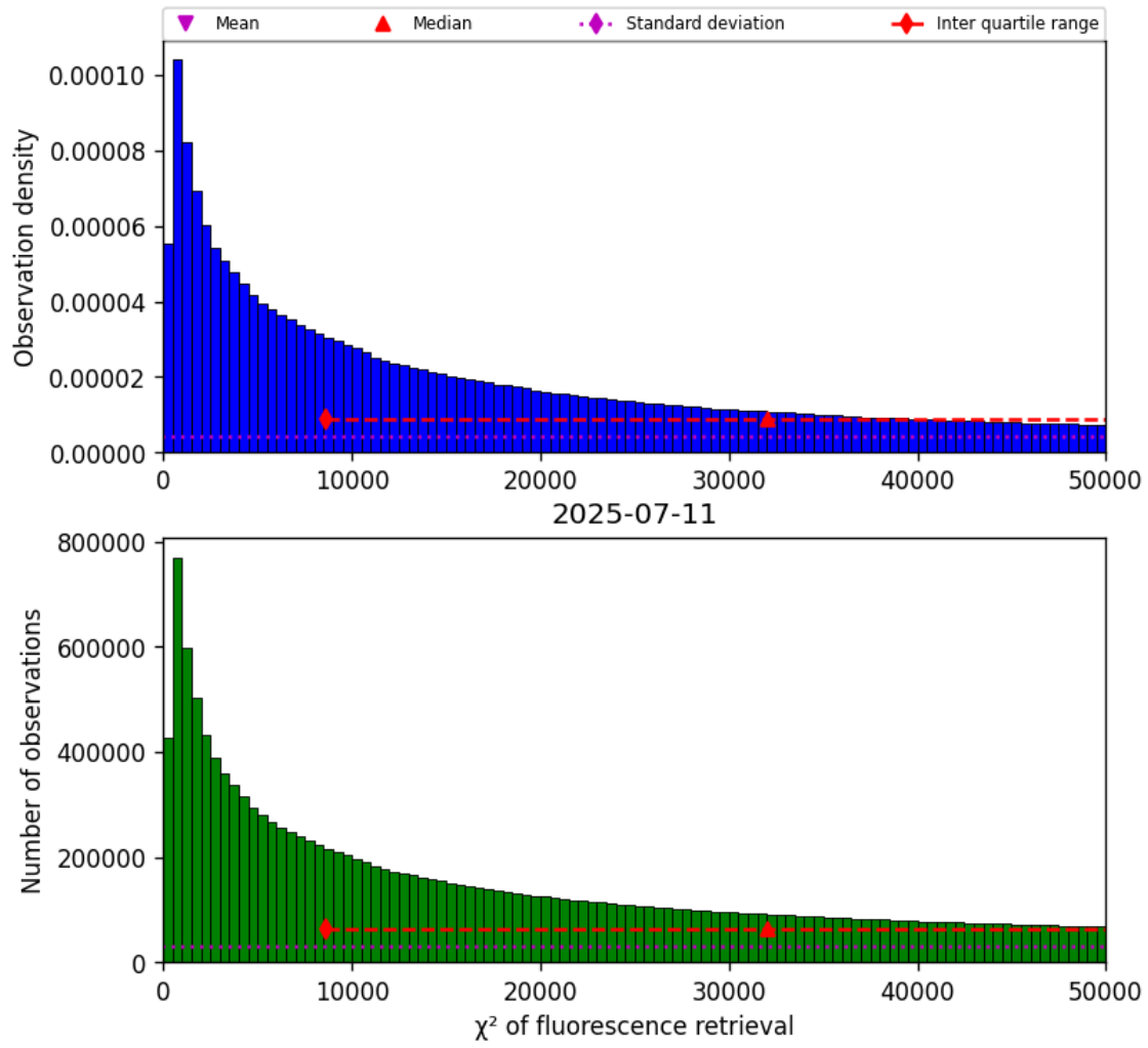
Figure 42: Histogram of “ \chi^2 of fluorescence retrieval” for 2025-07-10 to 2025-07-12
