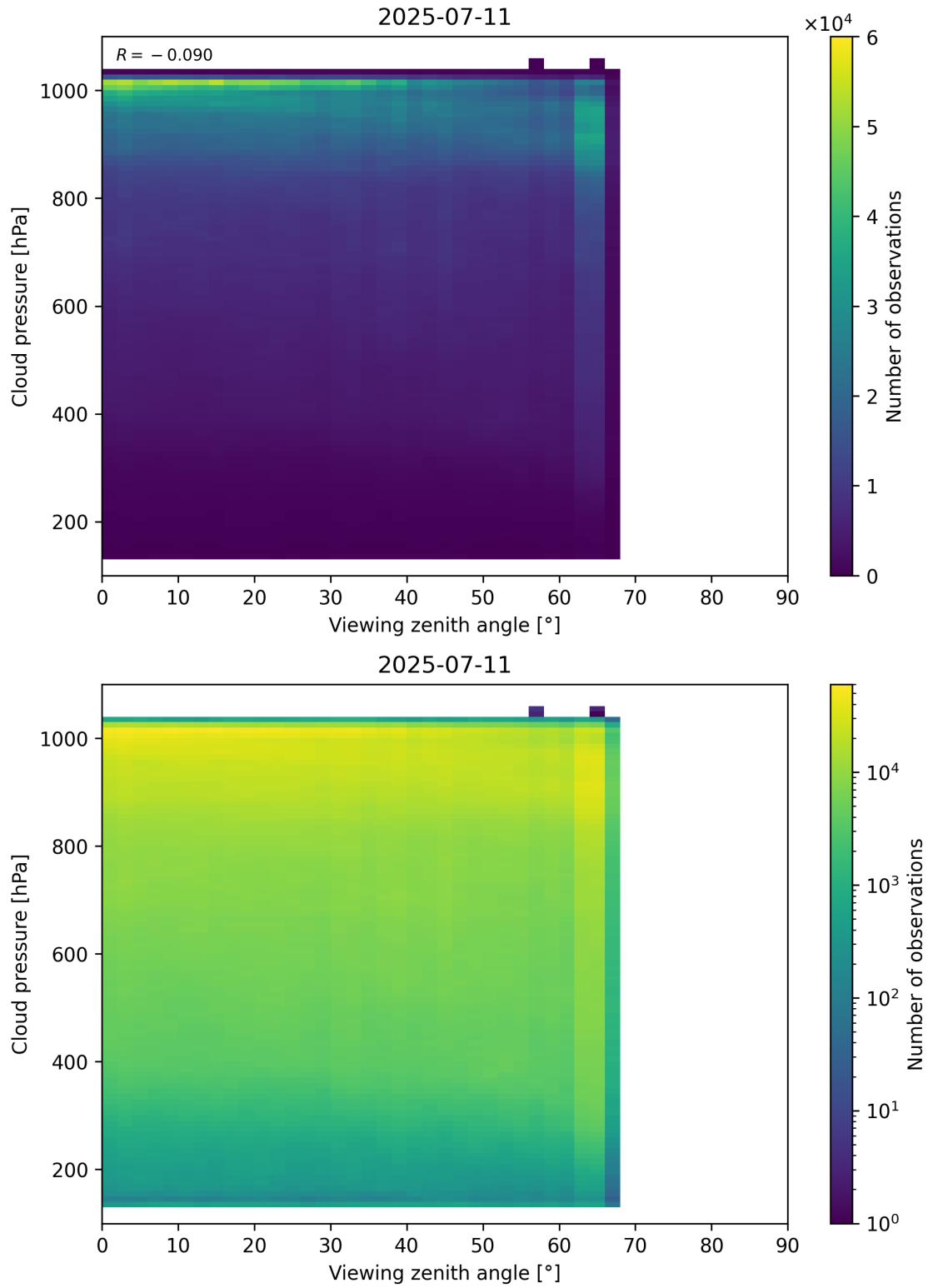
Figure 121: Scatter density plot of “Viewing zenith angle” against “Cloud pressure” for 2025-07-10 to 2025-07-12.
