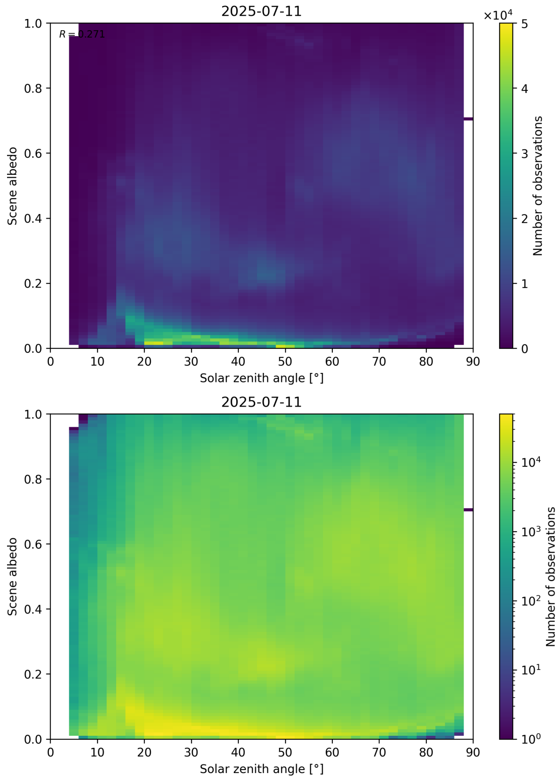
Figure 116: Scatter density plot of “Solar zenith angle” against “Scene albedo” for 2025-07-10 to 2025-07-12.
