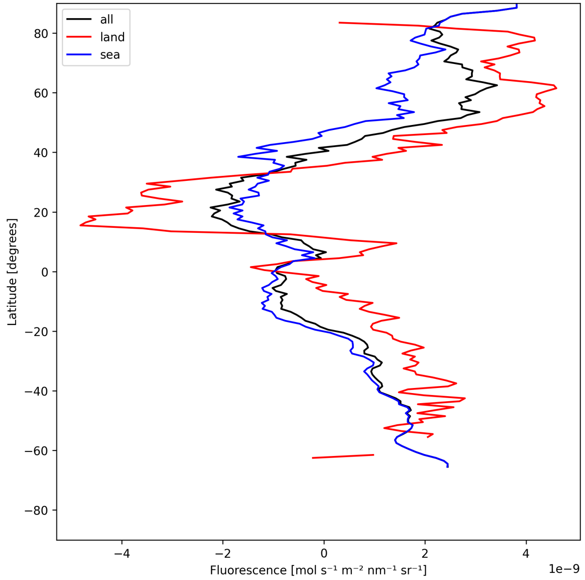
Figure 23: Zonal average of “Fluorescence” for 2025-07-10 to 2025-07-12.
