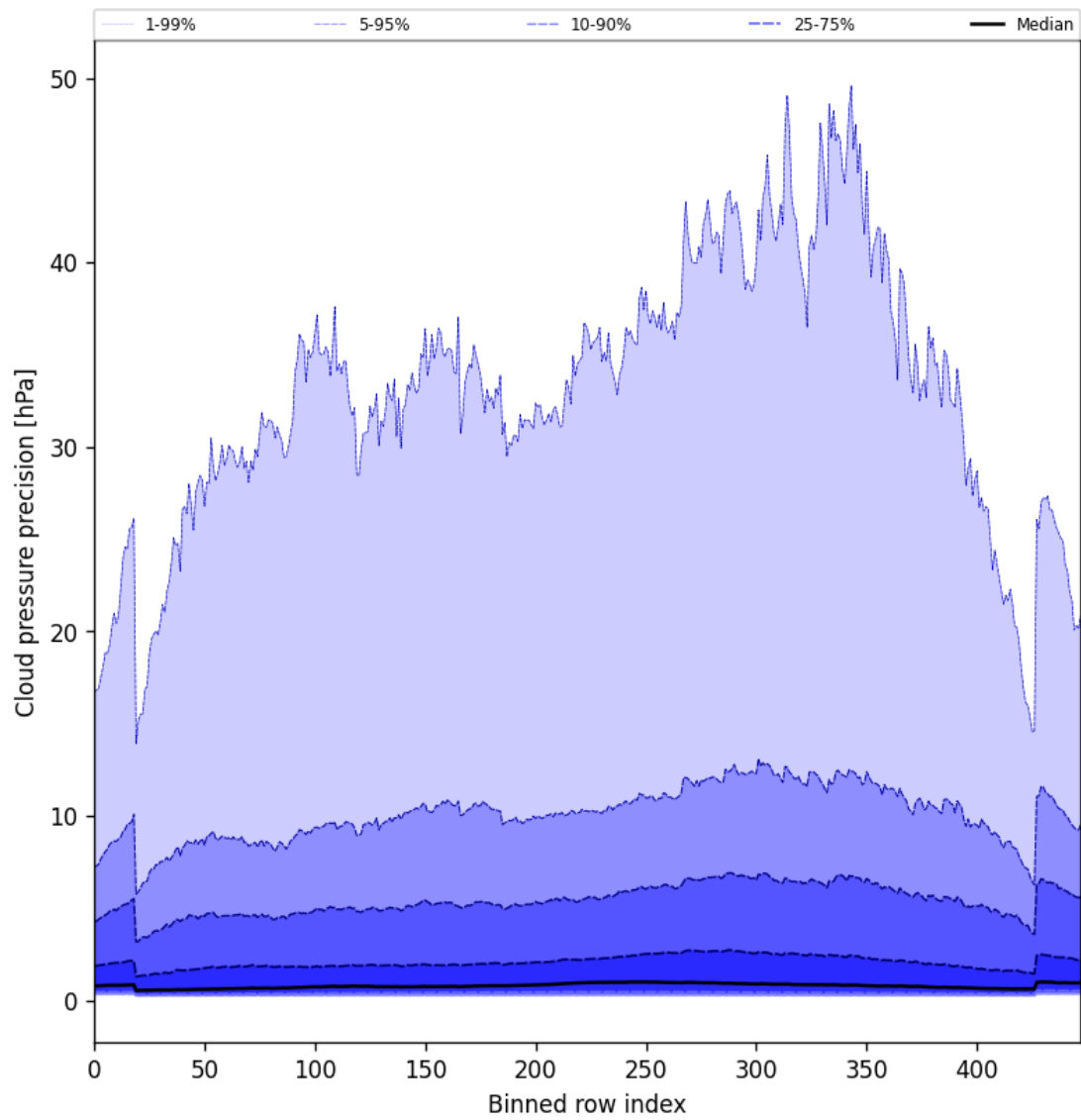
Figure 48: Along track statistics of “Cloud pressure precision” for 2025-07-10 to 2025-07-12
