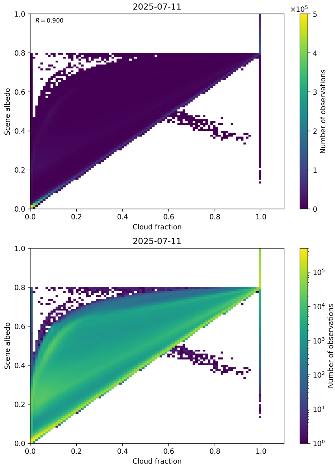
Figure 75: Scatter density plot of “Cloud fraction” against “Scene albedo” for 2025-07-10 to 2025-07-12.
