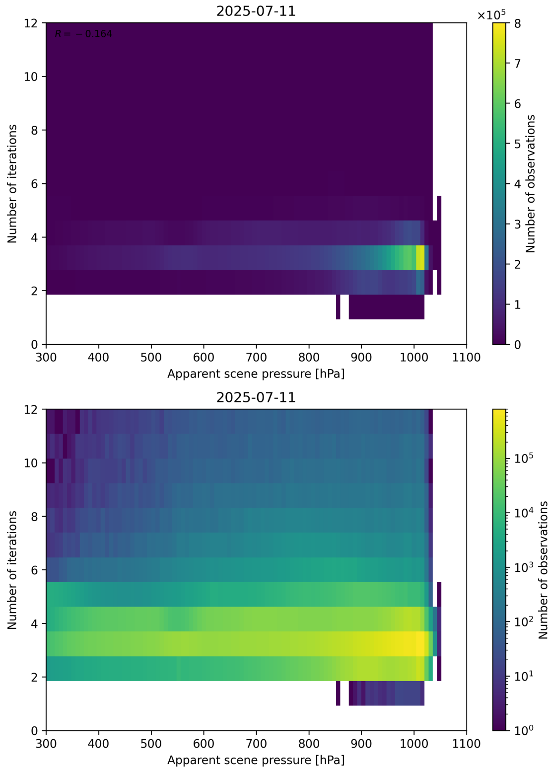
Figure 65: Scatter density plot of “Apparent scene pressure” against “Number of iterations” for 2025-07-10 to 2025-07-12.
