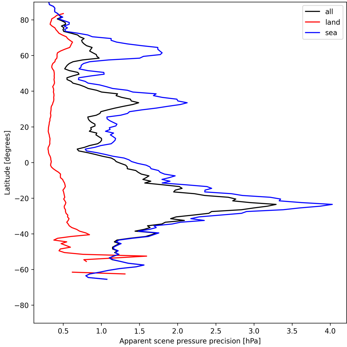
Figure 20: Zonal average of “Apparent scene pressure precision” for 2025-07-10 to 2025-07-12.
