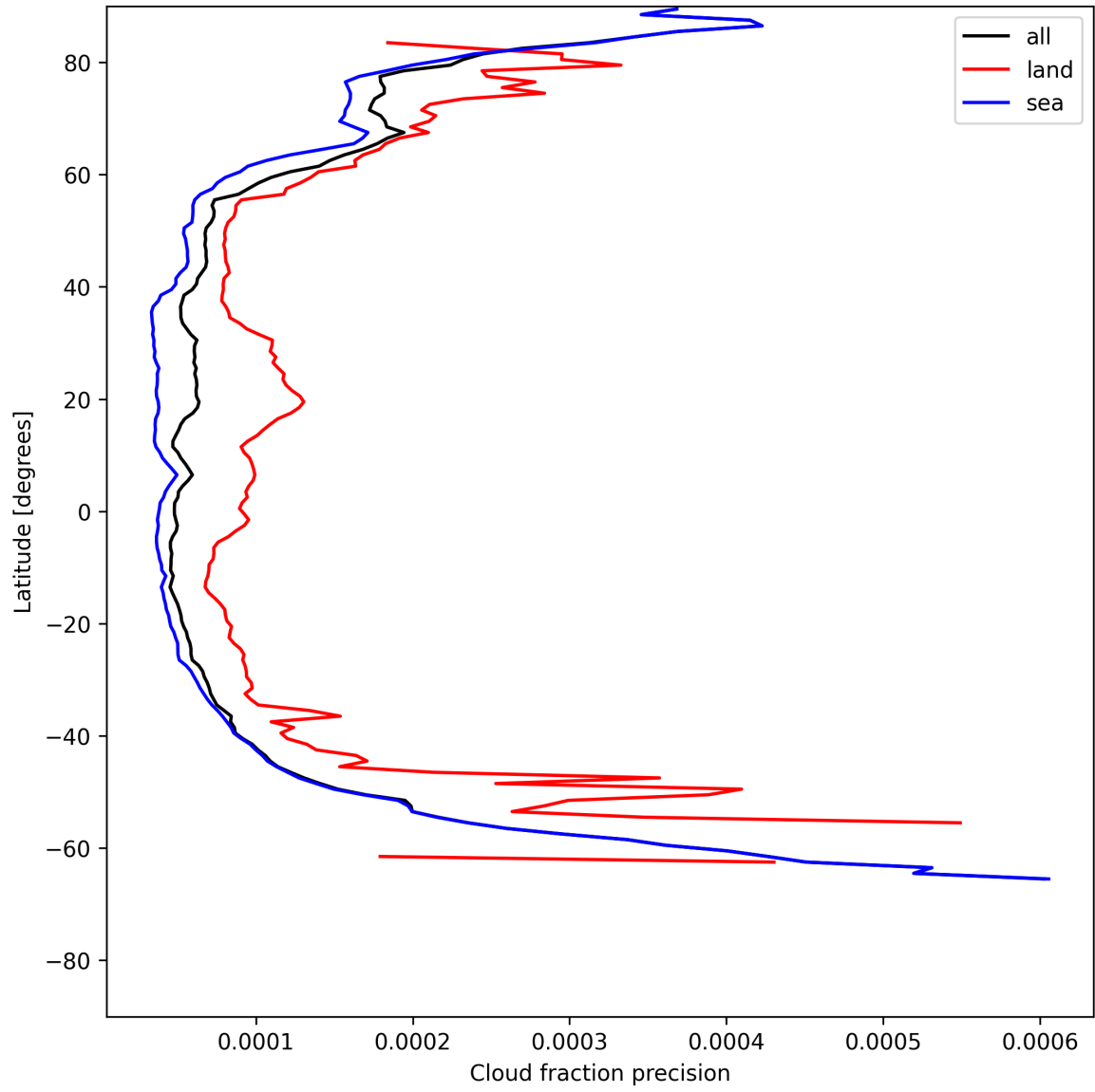
Figure 16: Zonal average of “Cloud fraction precision” for 2025-07-10 to 2025-07-12.
