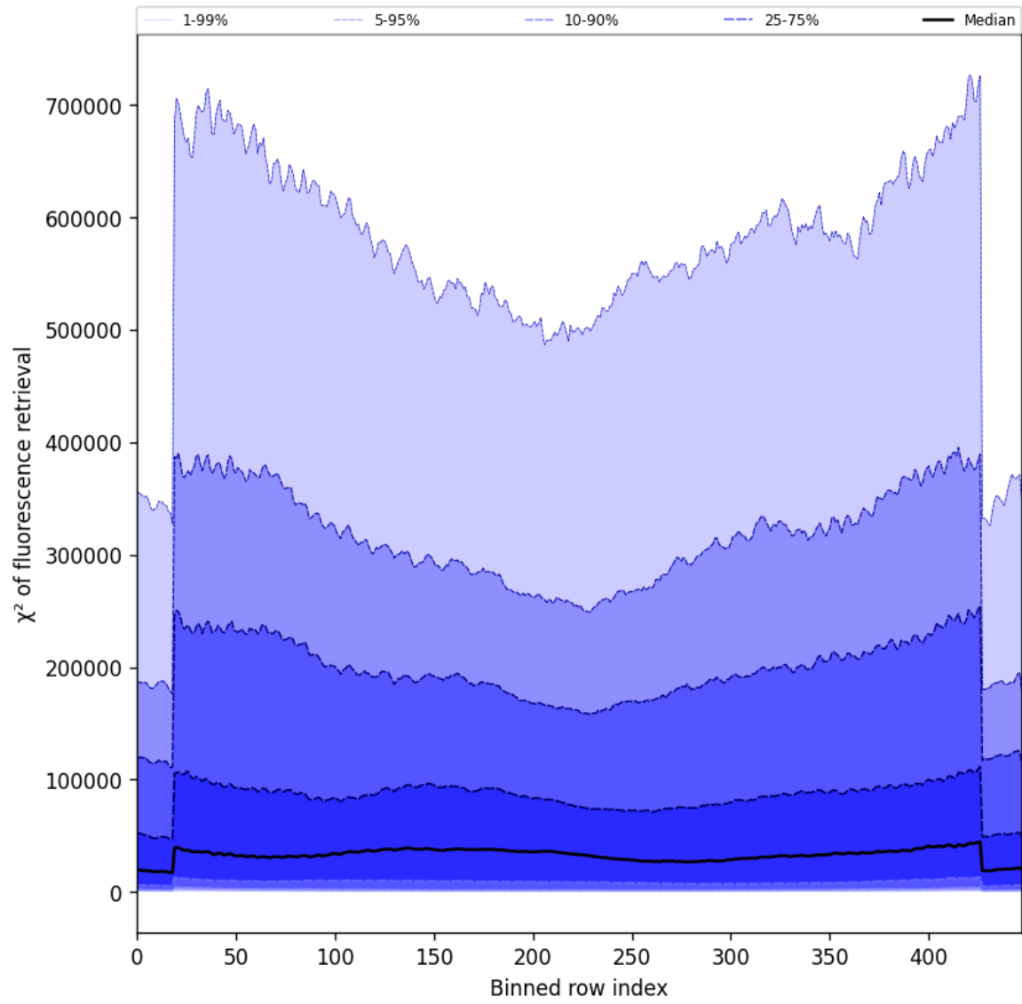
Figure 59: Along track statistics of “ \chi^2 of fluorescence retrieval” for 2025-07-10 to 2025-07-12
