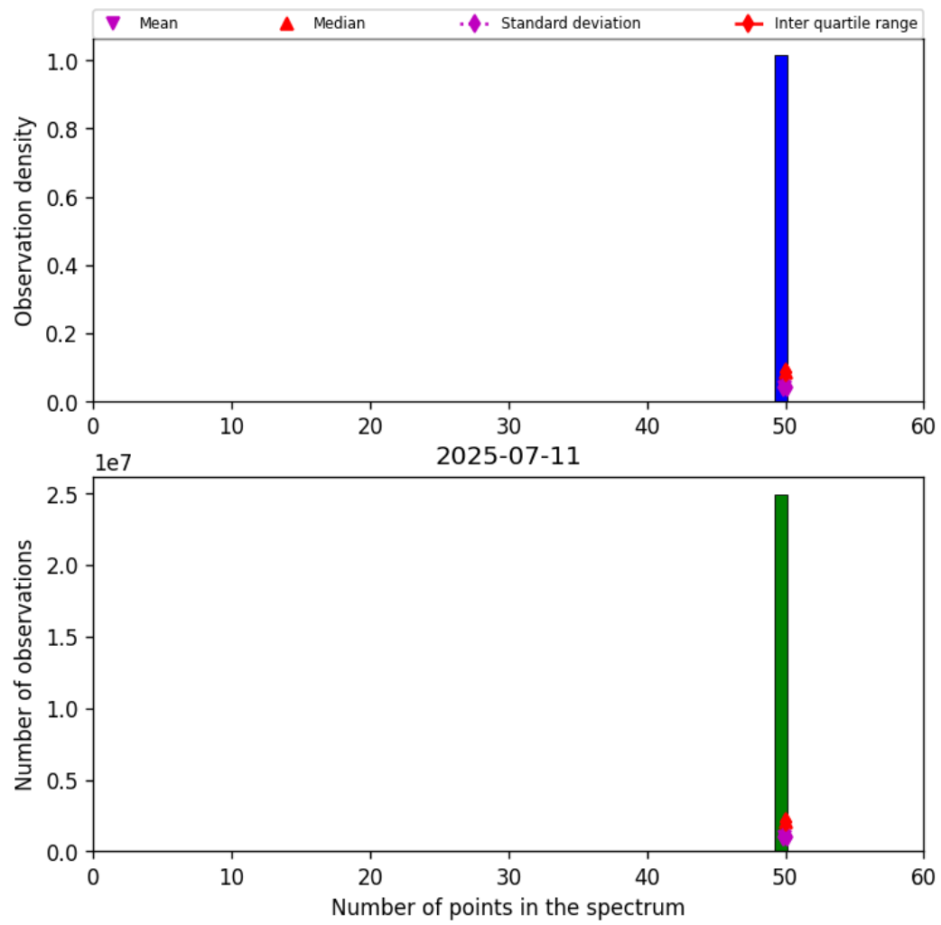
Figure 44: Histogram of "Number of points in the spectrum" for 2025-07-10 to 2025-07-12
