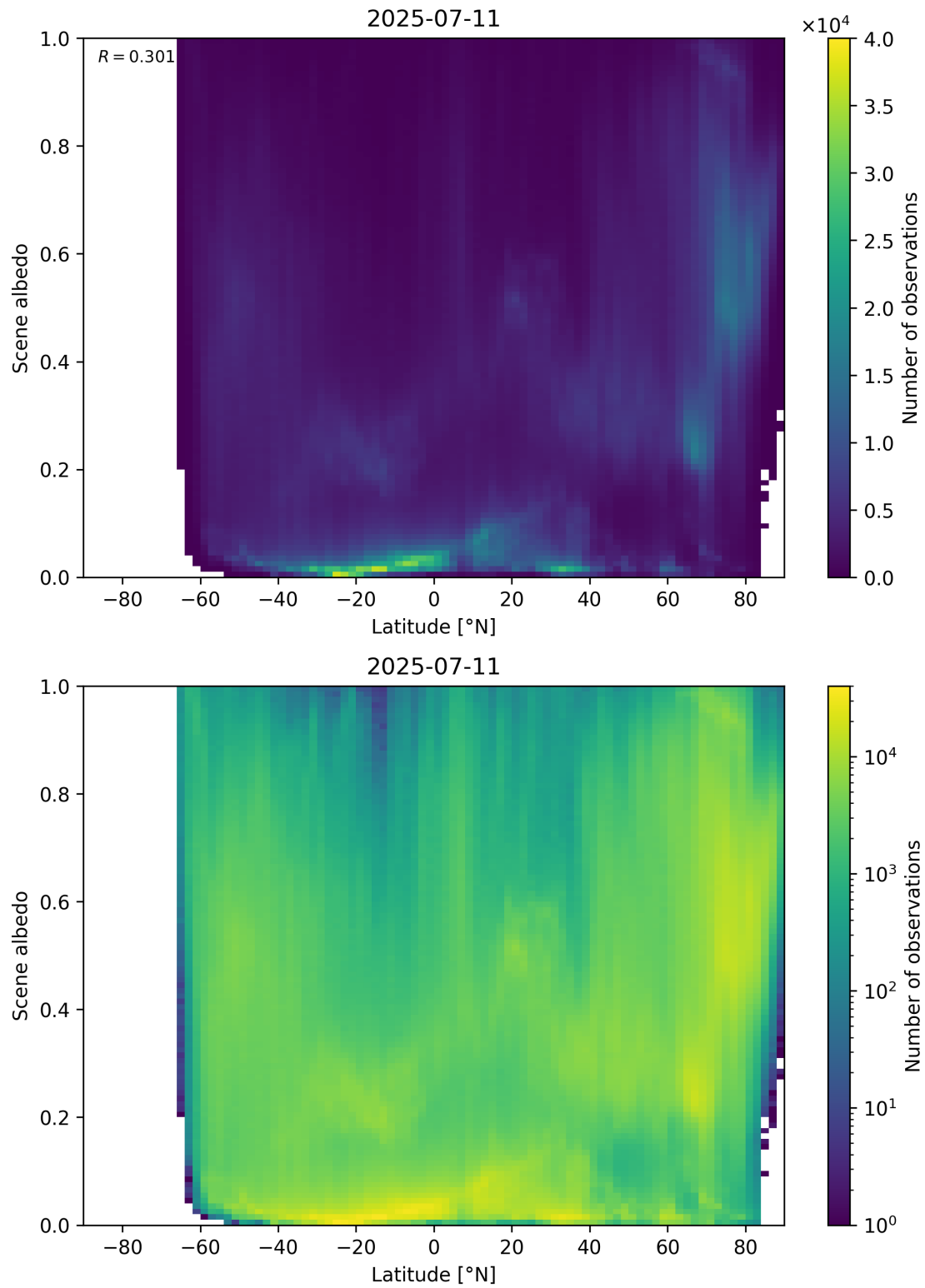
Figure 95: Scatter density plot of “Latitude” against “Scene albedo” for 2025-07-10 to 2025-07-12.
