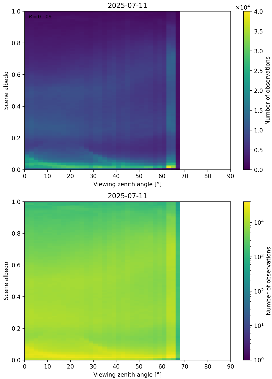
Figure 126: Scatter density plot of “Viewing zenith angle” against “Scene albedo” for 2025-07-10 to 2025-07-12.
