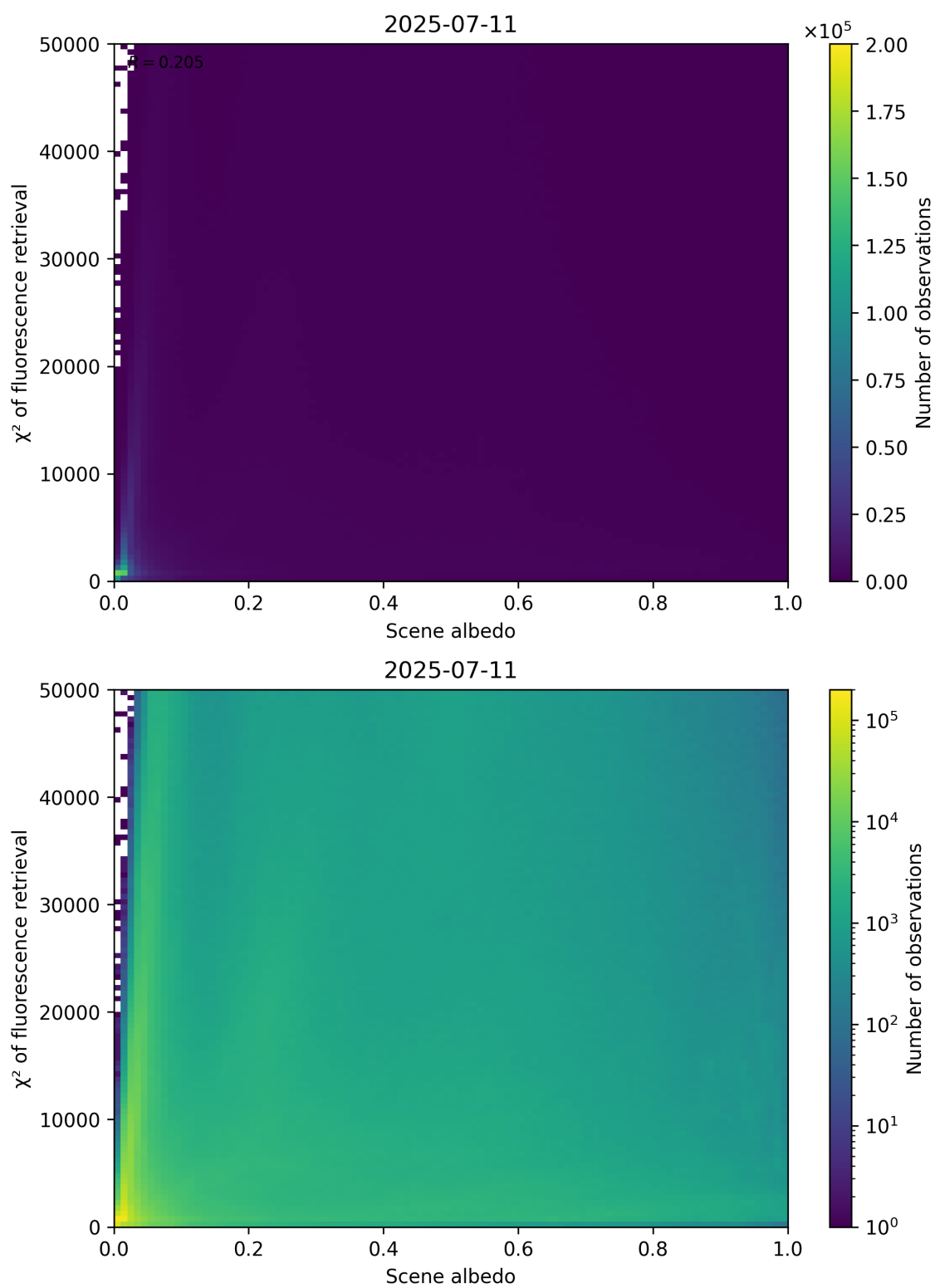
Figure 103: Scatter density plot of “Scene albedo” against “ \chi^2 of fluorescence retrieval” for 2025-07-10 to 2025-07-12.
