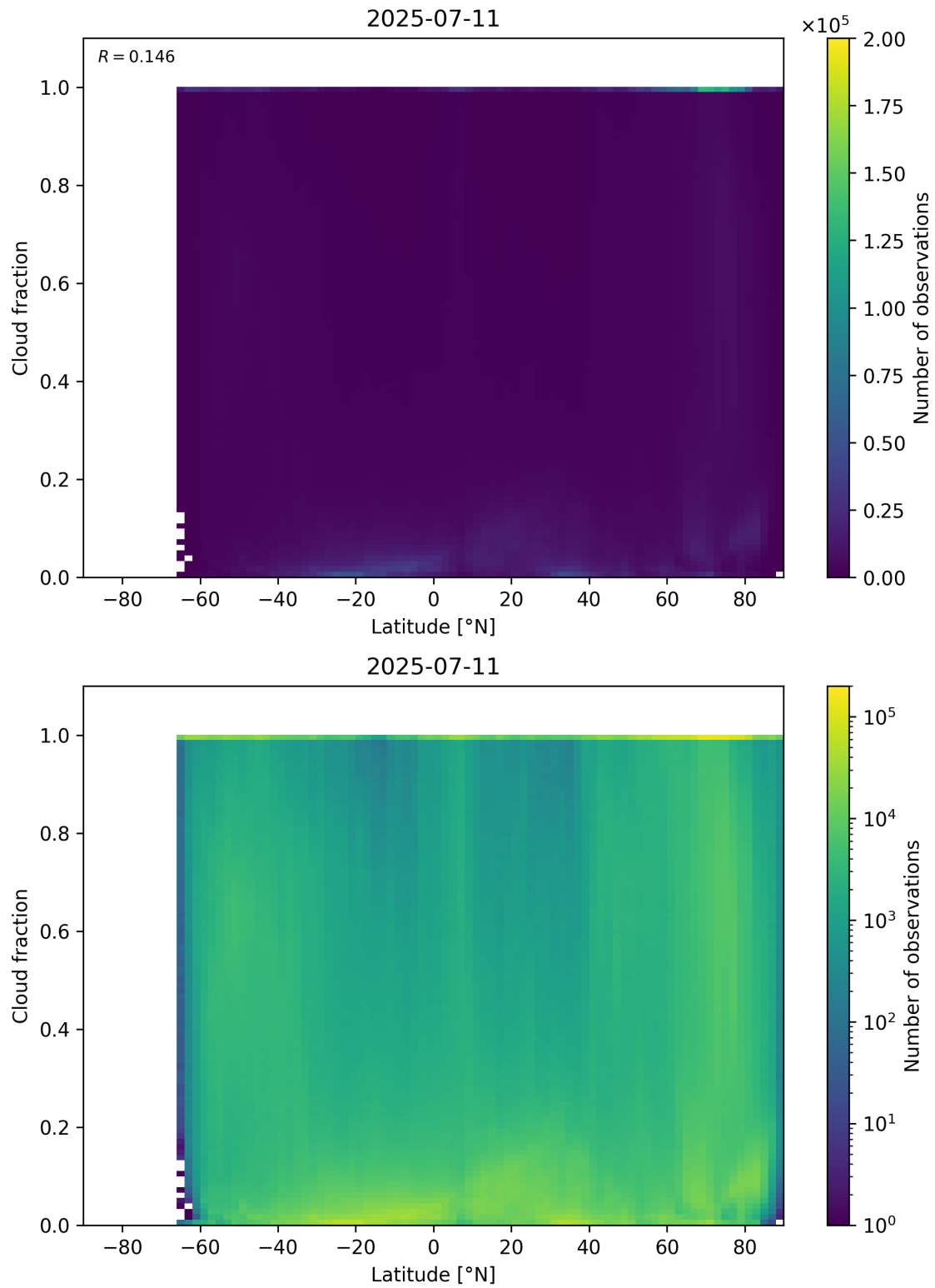
Figure 90: Scatter density plot of “Latitude” against “Cloud fraction” for 2025-07-10 to 2025-07-12.
