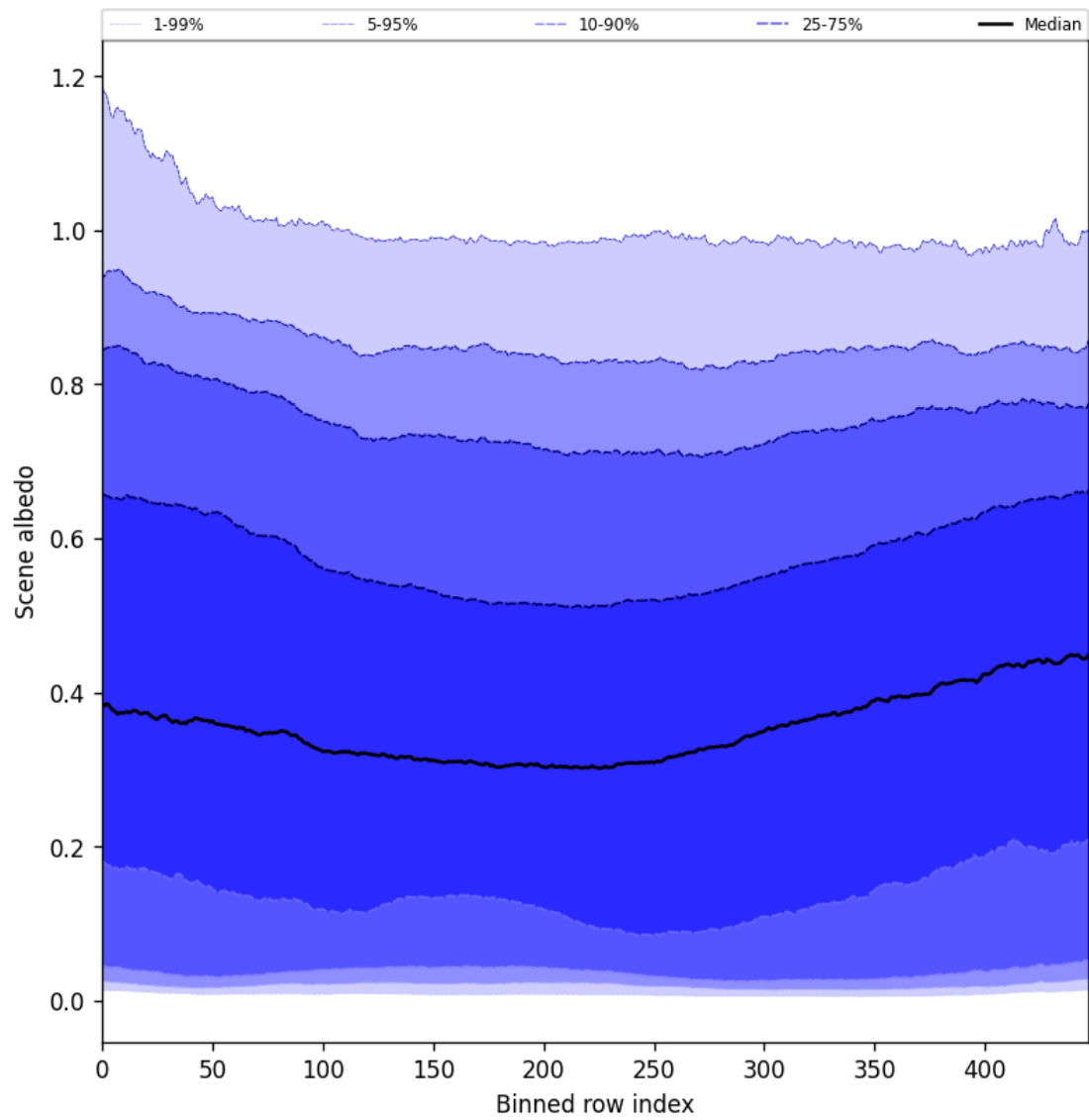
Figure 51: Along track statistics of “Scene albedo” for 2025-07-10 to 2025-07-12
