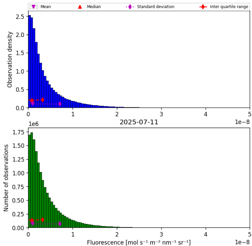
Figure 40: Histogram of “Fluorescence” for 2025-07-10 to 2025-07-12
