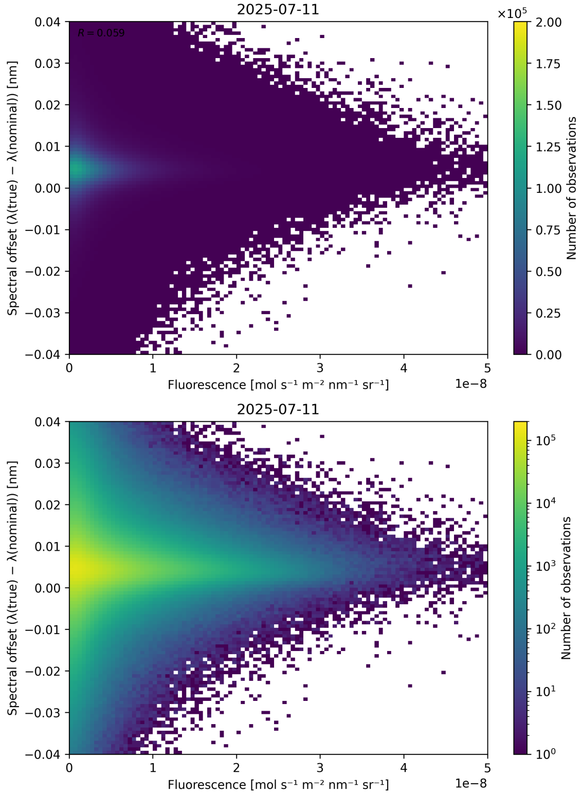
Figure 87: Scatter density plot of “Fluorescence” against “Spectral offset ( \lambda_{\text{true}} - \lambda_{\text{nominal}} )” for 2025-07-10 to 2025-07-12.
