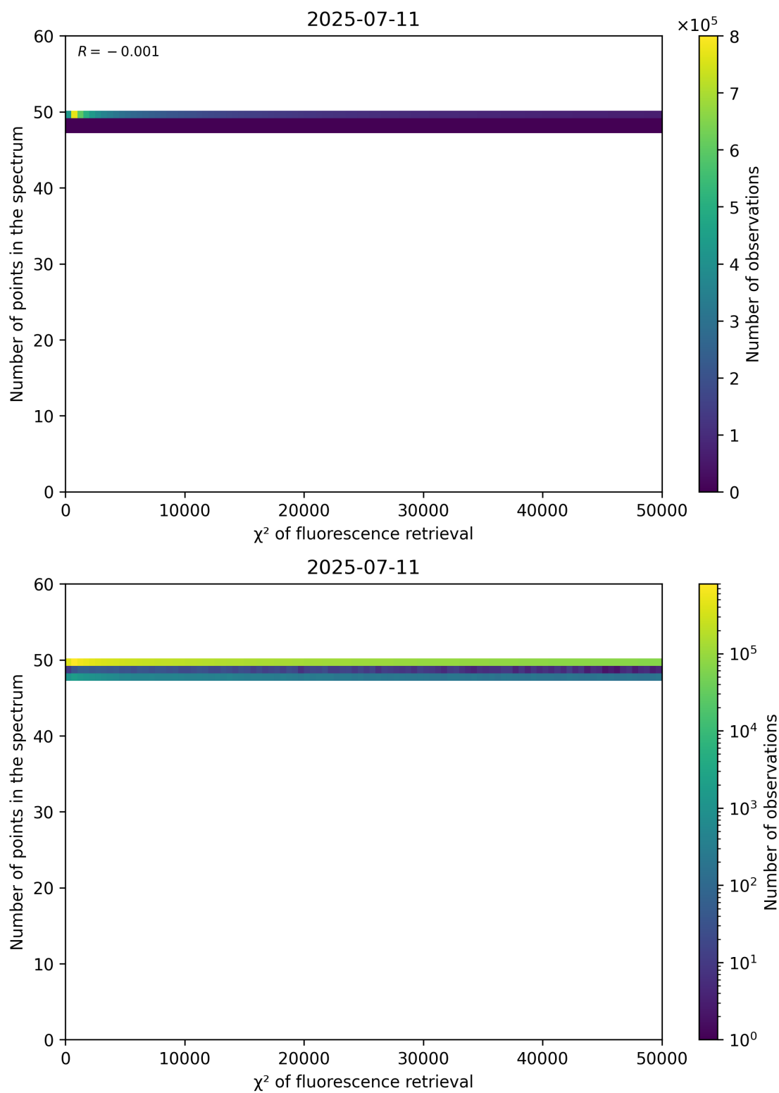
Figure 68: Scatter density plot of " \chi^2 of fluorescence retrieval" against "Number of points in the spectrum" for 2025-07-10 to 2025-07-12.
