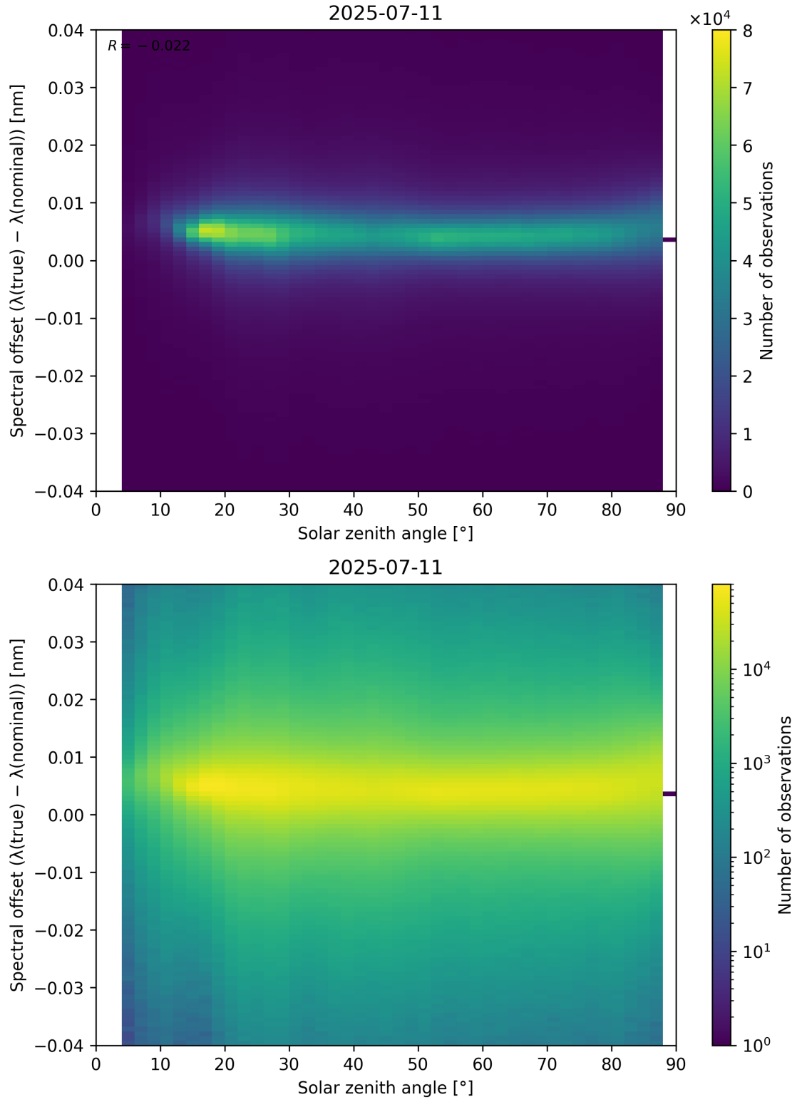
Figure 117: Scatter density plot of “Solar zenith angle” against “Spectral offset ( \lambda_{\text{true}} - \lambda_{\text{nominal}} )” for 2025-07-10 to 2025-07-12.
