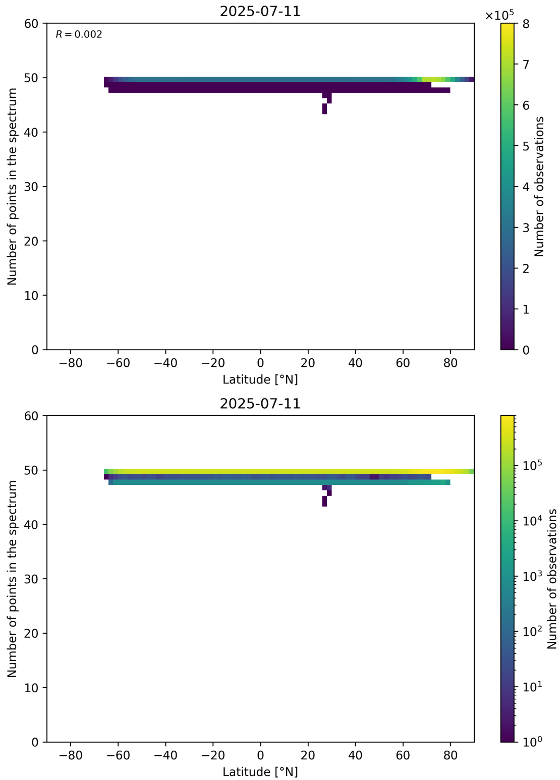
Figure 94: Scatter density plot of “Latitude” against “Number of points in the spectrum” for 2025-07-10 to 2025-07-12.
