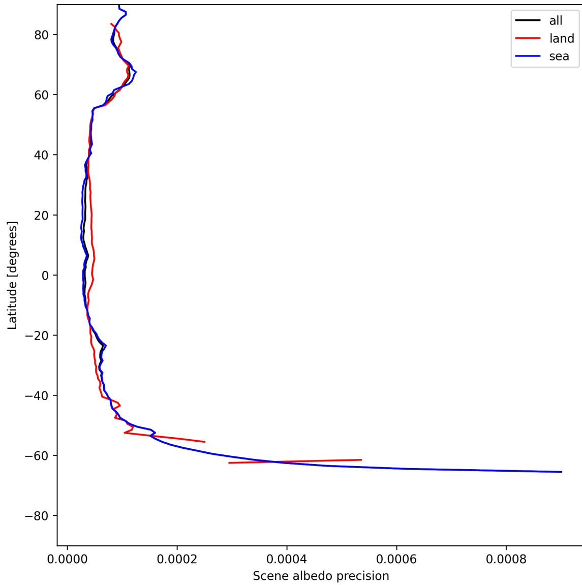
Figure 18: Zonal average of “Scene albedo precision” for 2025-07-10 to 2025-07-12.
