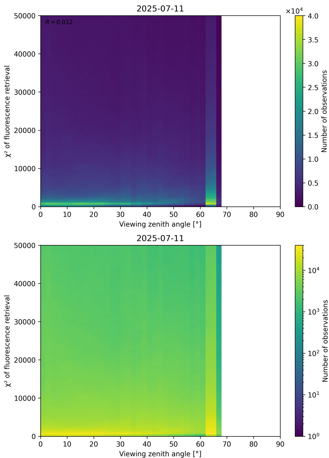
Figure 119: Scatter density plot of “Viewing zenith angle” against “ \chi^2 of fluorescence retrieval” for 2025-07-10 to 2025-07-12.
