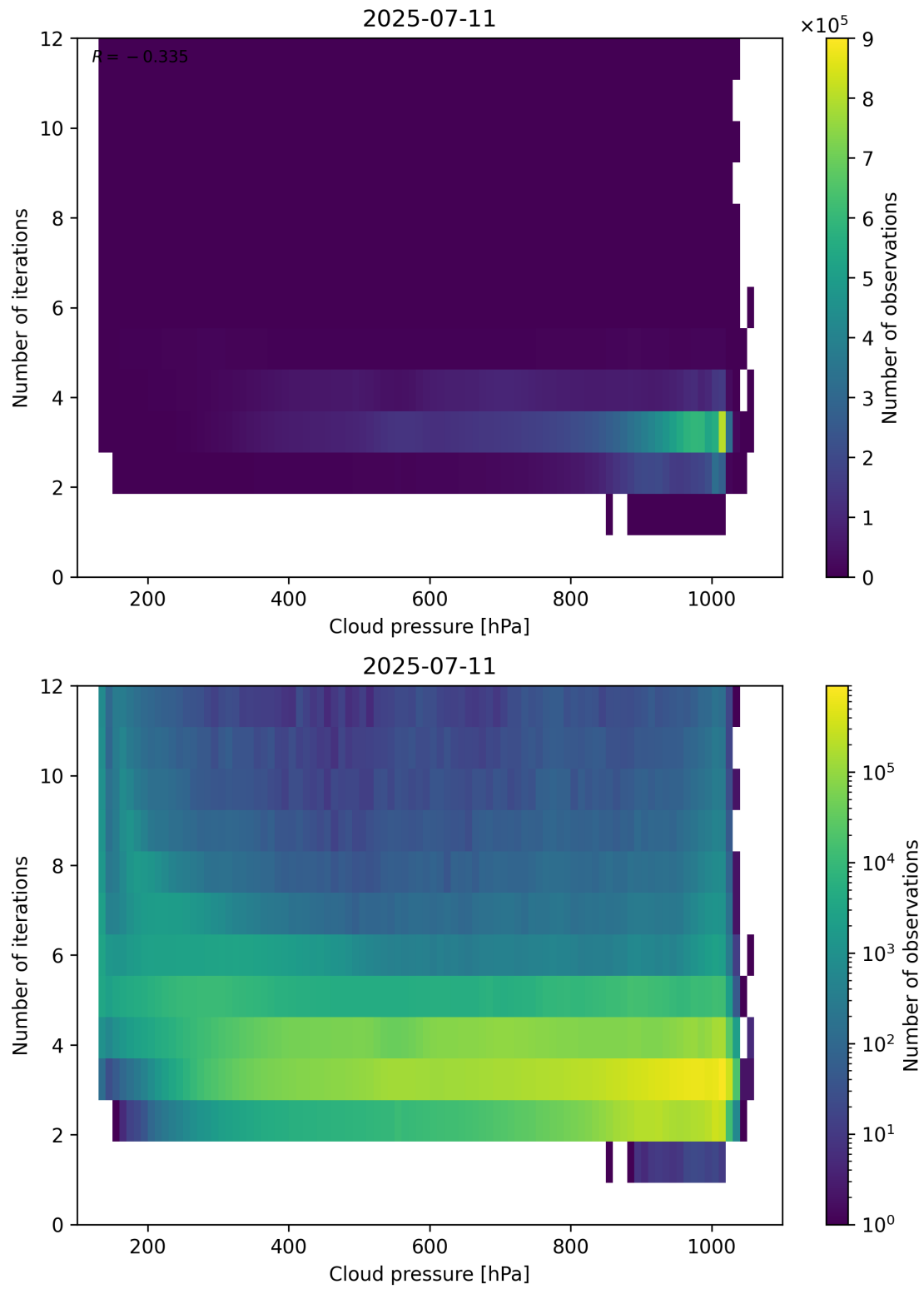
Figure 81: Scatter density plot of “Cloud pressure” against “Number of iterations” for 2025-07-10 to 2025-07-12.
