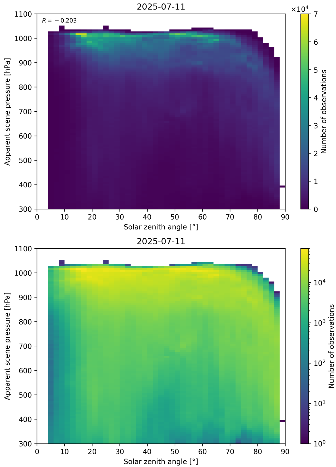
Figure 108: Scatter density plot of “Solar zenith angle” against “Apparent scene pressure” for 2025-07-10 to 2025-07-12.
