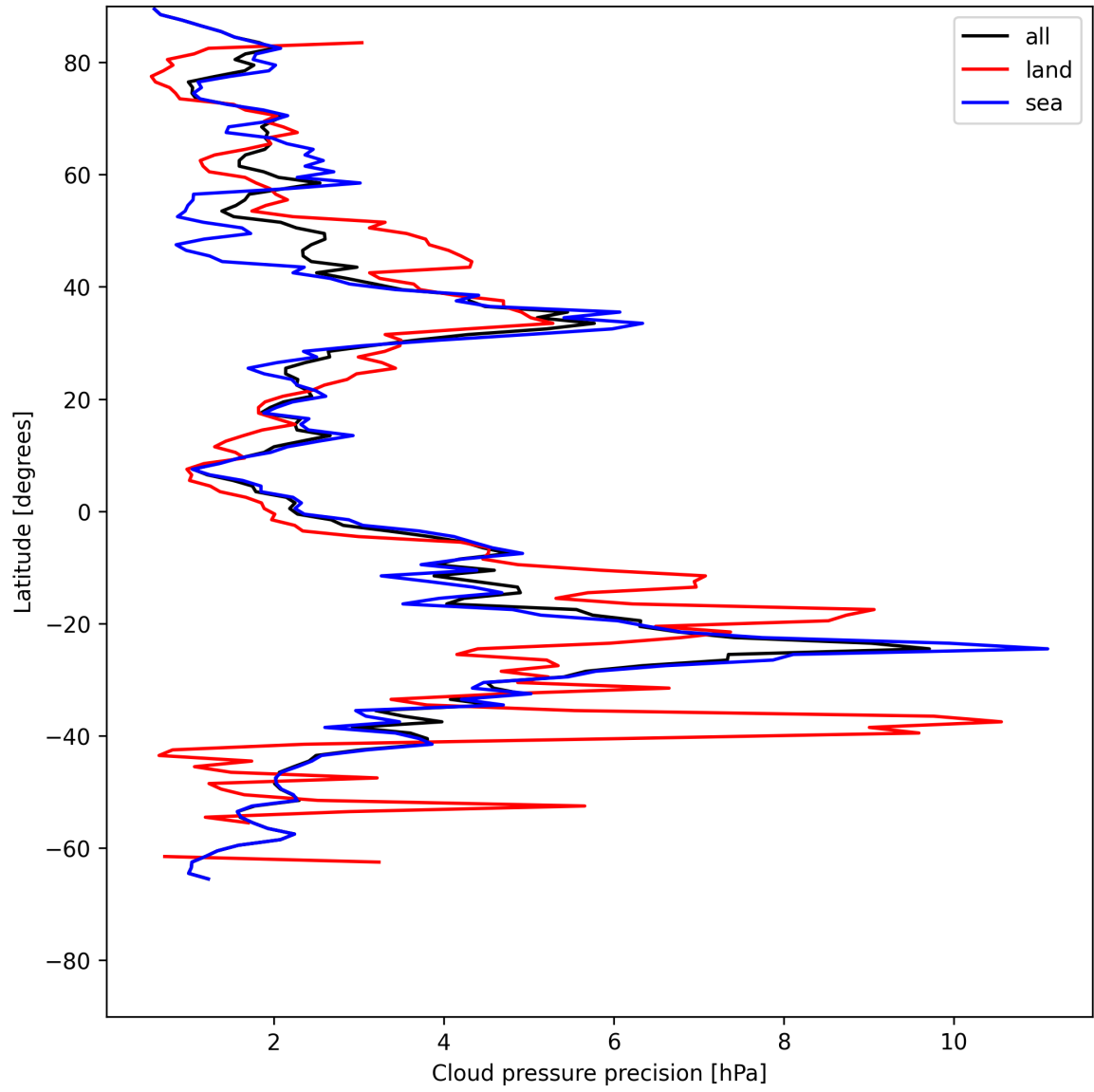
Figure 14: Zonal average of “Cloud pressure precision” for 2025-07-10 to 2025-07-12.
