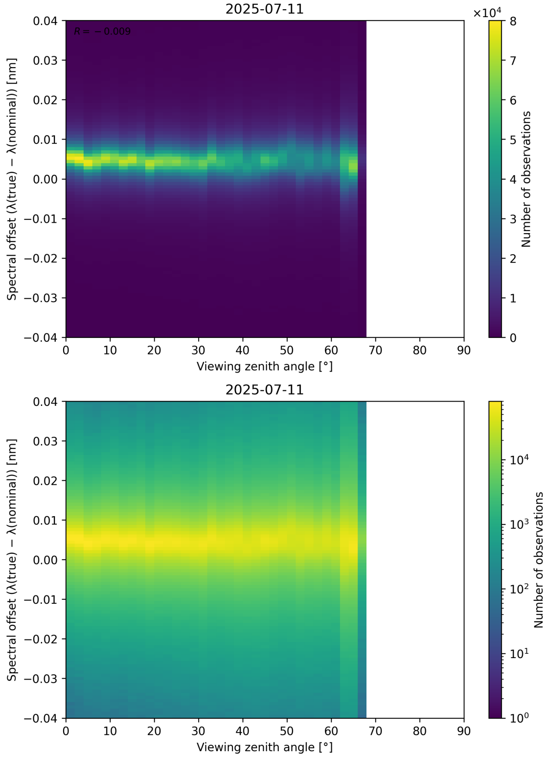
Figure 128: Scatter density plot of “Viewing zenith angle” against “Spectral offset ( \lambda_{\text{true}} - \lambda_{\text{nominal}} )” for 2025-07-10 to 2025-07-12.
