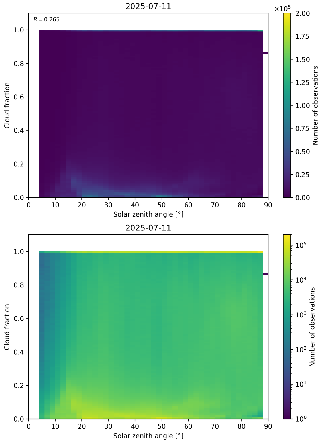
Figure 110: Scatter density plot of “Solar zenith angle” against “Cloud fraction” for 2025-07-10 to 2025-07-12.
