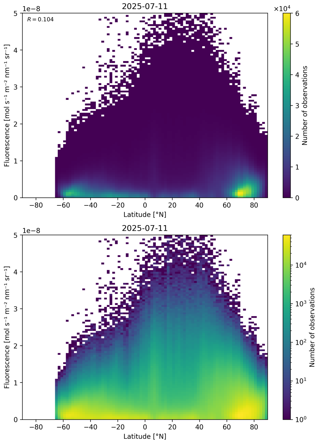
Figure 92: Scatter density plot of “Latitude” against “Fluorescence” for 2025-07-10 to 2025-07-12.
