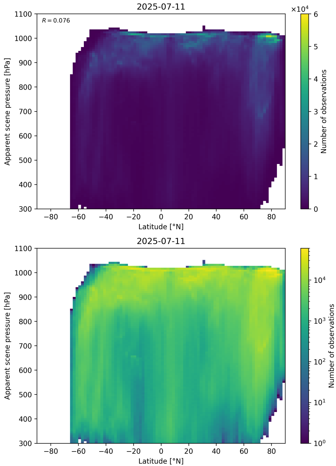
Figure 88: Scatter density plot of “Latitude” against “Apparent scene pressure” for 2025-07-10 to 2025-07-12.
