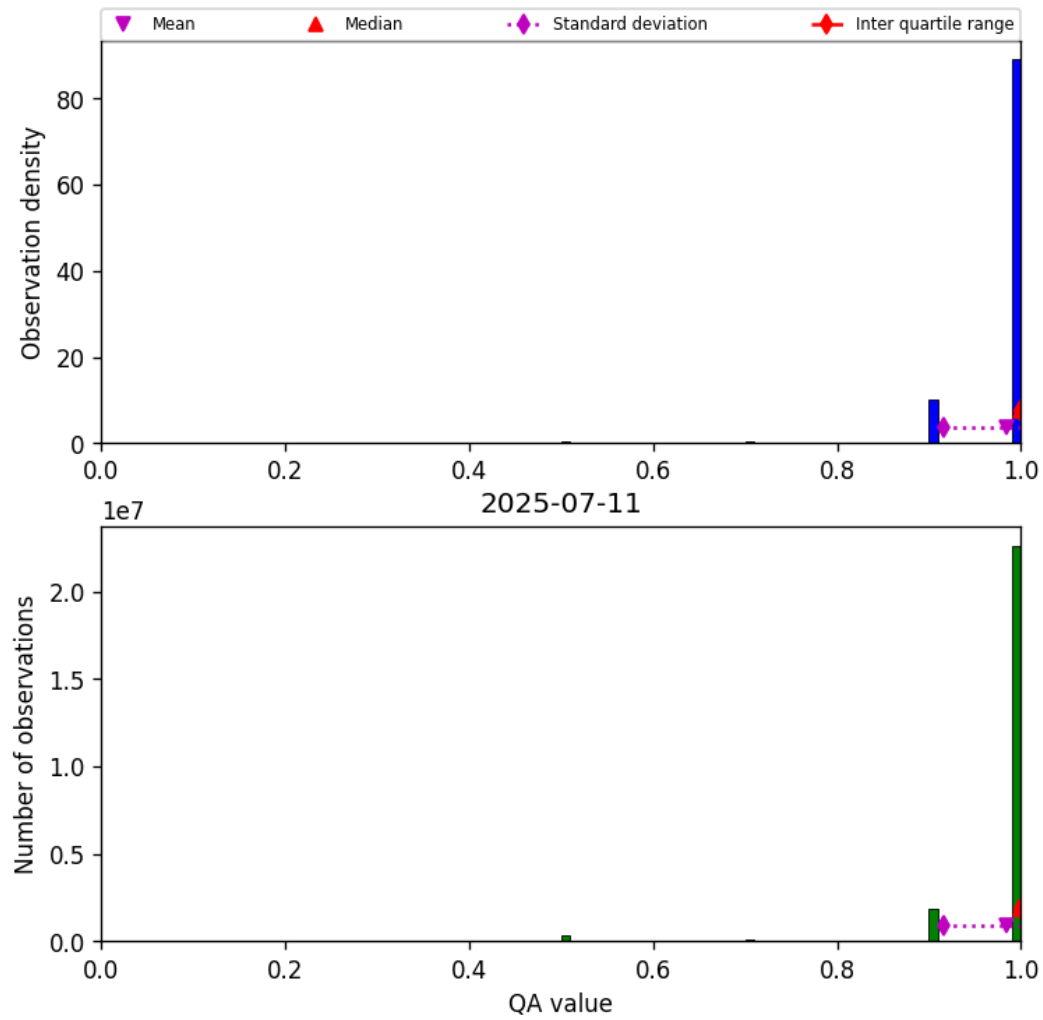
Figure 29: Histogram of “QA value” for 2025-07-10 to 2025-07-12
