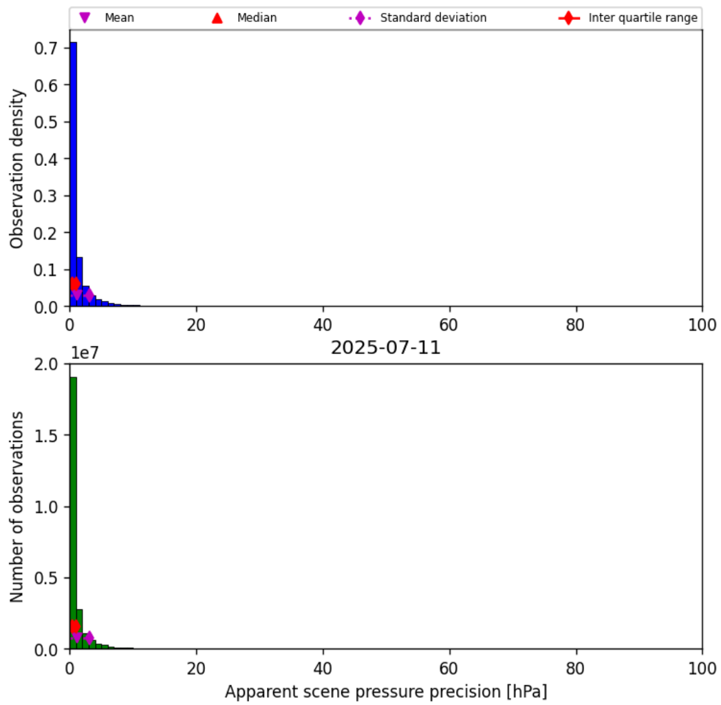
Figure 37: Histogram of “Apparent scene pressure precision” for 2025-07-10 to 2025-07-12
