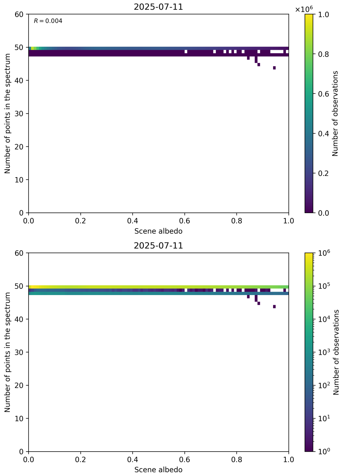
Figure 106: Scatter density plot of “Scene albedo” against “Number of points in the spectrum” for 2025-07-10 to 2025-07-12.
