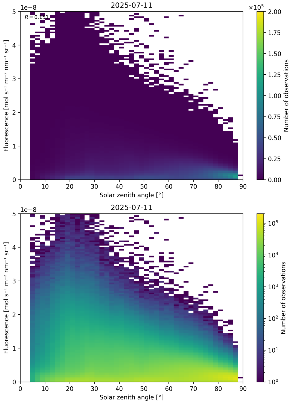
Figure 112: Scatter density plot of “Solar zenith angle” against “Fluorescence” for 2025-07-10 to 2025-07-12.
