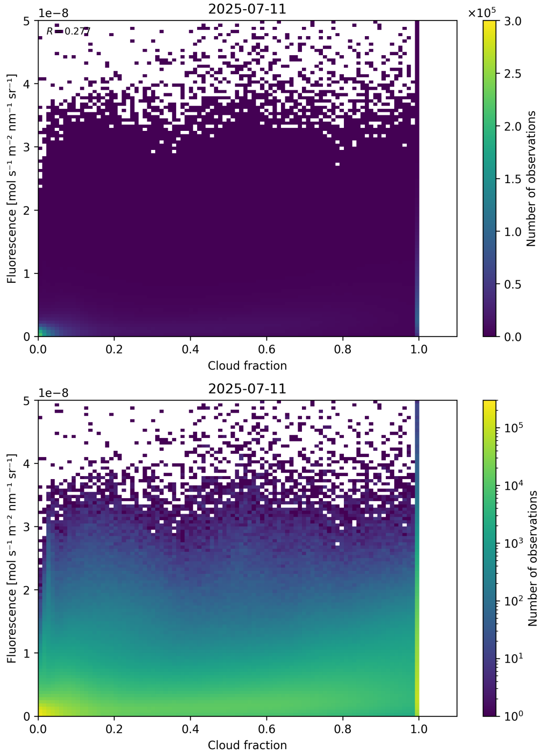
Figure 72: Scatter density plot of “Cloud fraction” against “Fluorescence” for 2025-07-10 to 2025-07-12.
