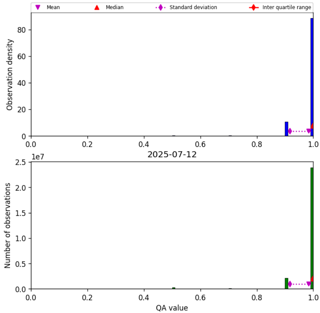
Figure 29: Histogram of “QA value” for 2025-07-11 to 2025-07-13
