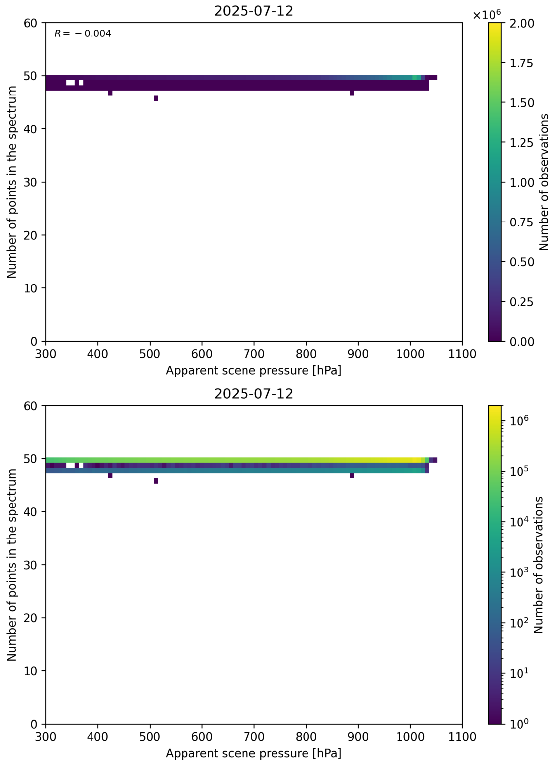
Figure 66: Scatter density plot of “Apparent scene pressure” against “Number of points in the spectrum” for 2025-07-11 to 2025-07-13.
