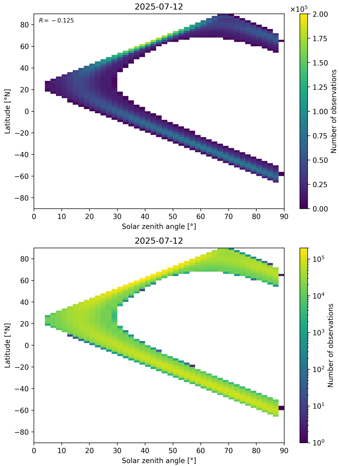
Figure 113: Scatter density plot of “Solar zenith angle” against “Latitude” for 2025-07-11 to 2025-07-13.
