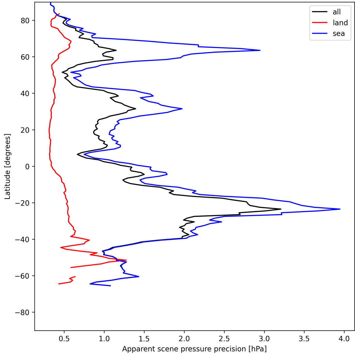
Figure 20: Zonal average of “Apparent scene pressure precision” for 2025-07-11 to 2025-07-13.
