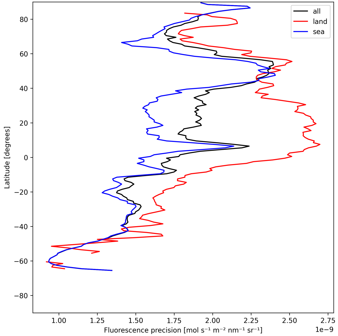
Figure 24: Zonal average of “Fluorescence precision” for 2025-07-11 to 2025-07-13.
