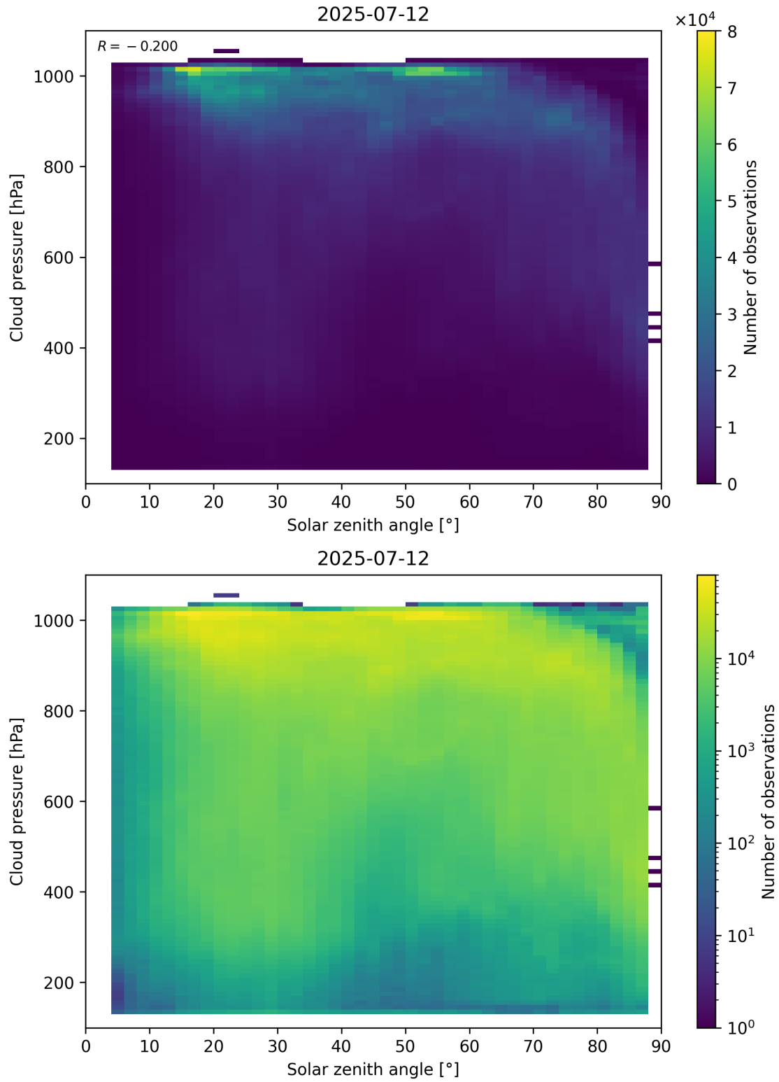
Figure 111: Scatter density plot of “Solar zenith angle” against “Cloud pressure” for 2025-07-11 to 2025-07-13.
