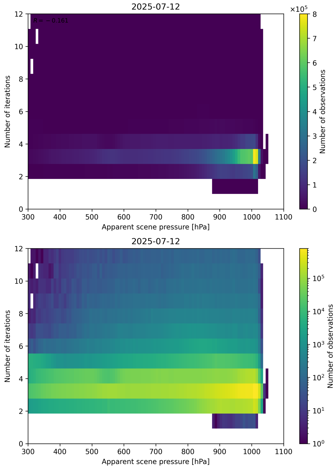
Figure 65: Scatter density plot of “Apparent scene pressure” against “Number of iterations” for 2025-07-11 to 2025-07-13.
