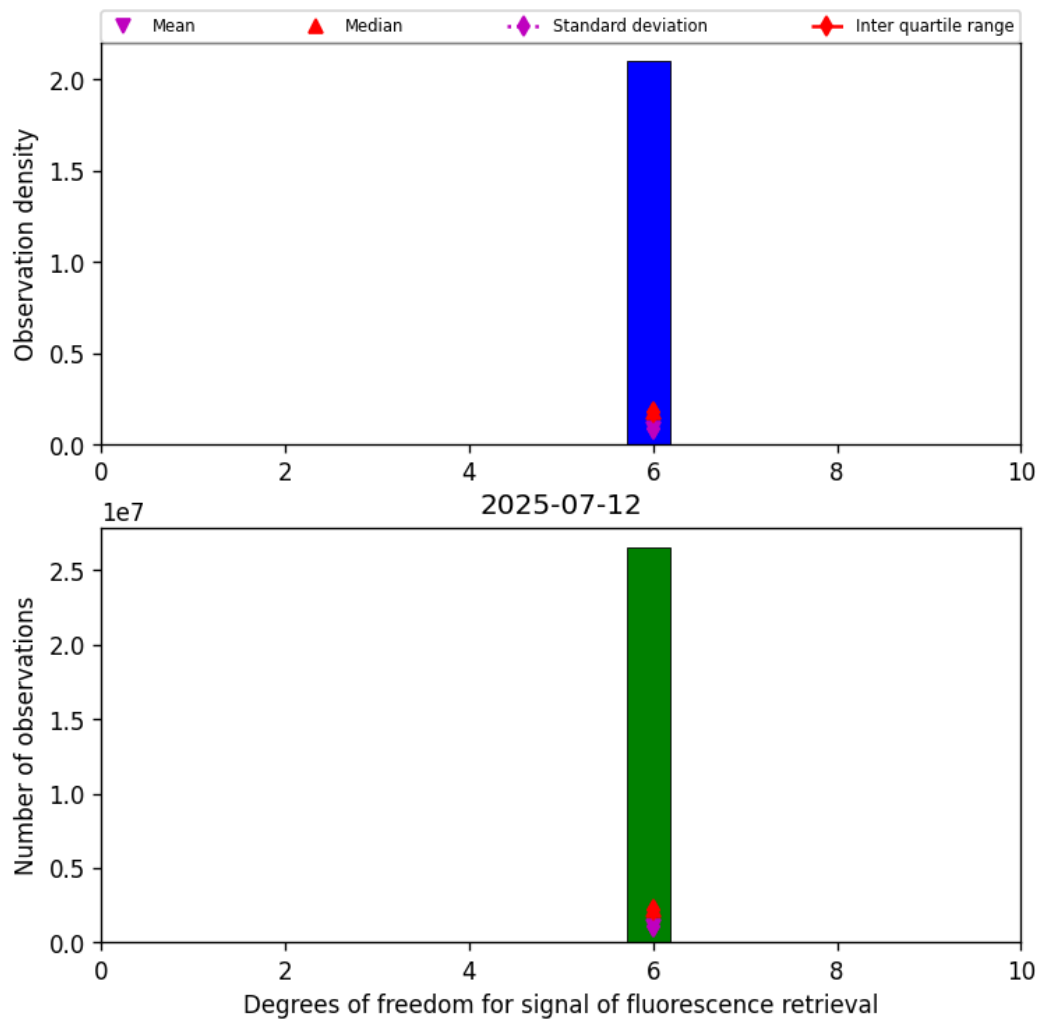
Figure 43: Histogram of "Degrees of freedom for signal of fluorescence retrieval" for 2025-07-11 to 2025-07-13
