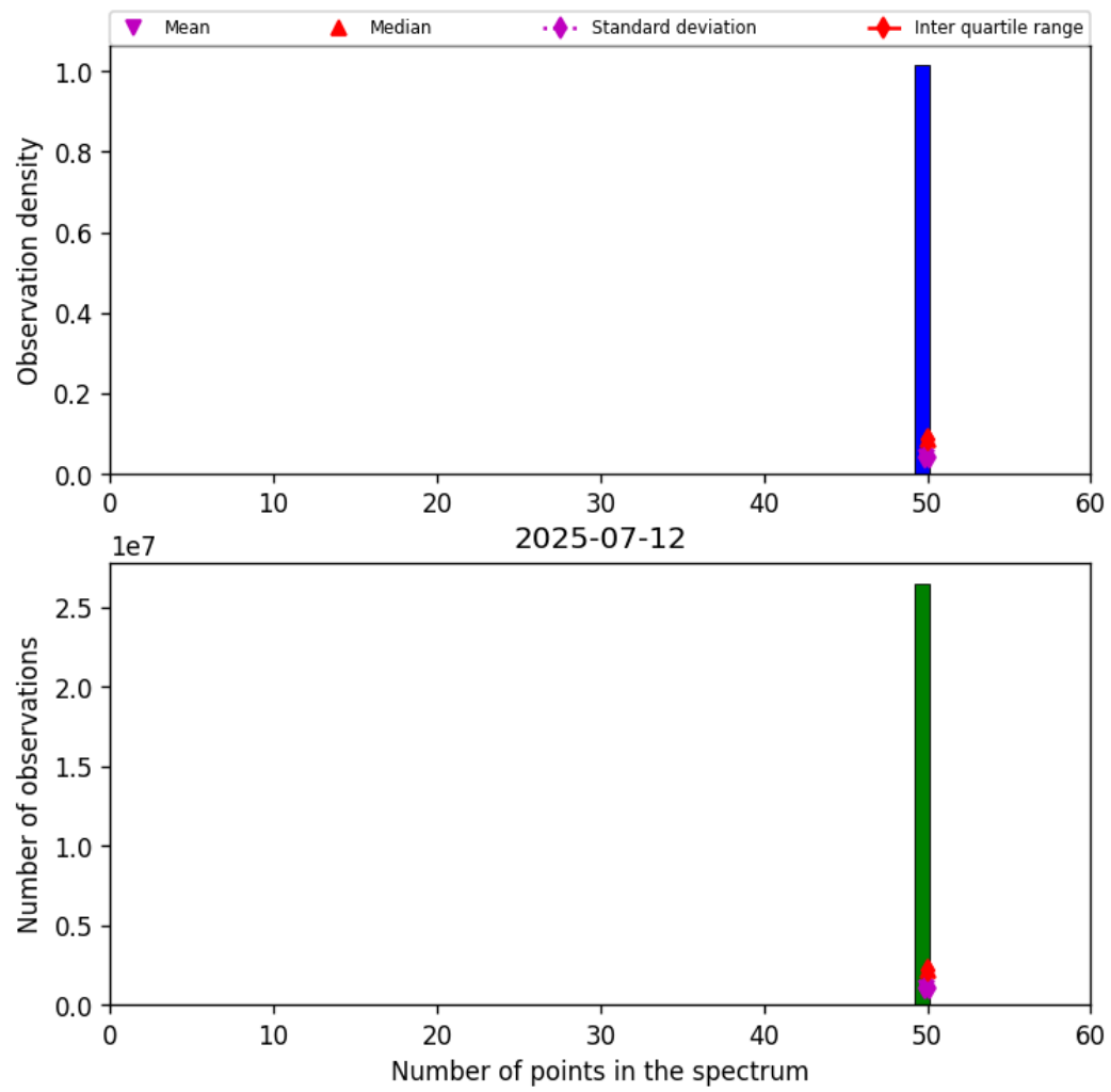
Figure 44: Histogram of “Number of points in the spectrum” for 2025-07-11 to 2025-07-13
