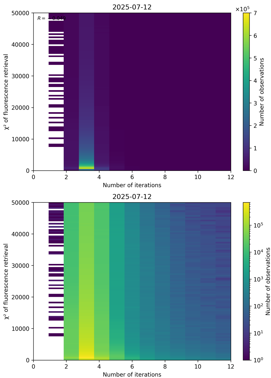
Figure 97: Scatter density plot of “Number of iterations” against “ \chi^2 of fluorescence retrieval” for 2025-07-11 to 2025-07-13.
