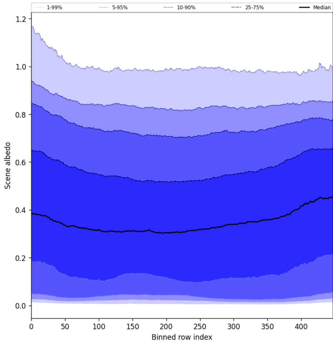
Figure 51: Along track statistics of “Scene albedo” for 2025-07-11 to 2025-07-13
