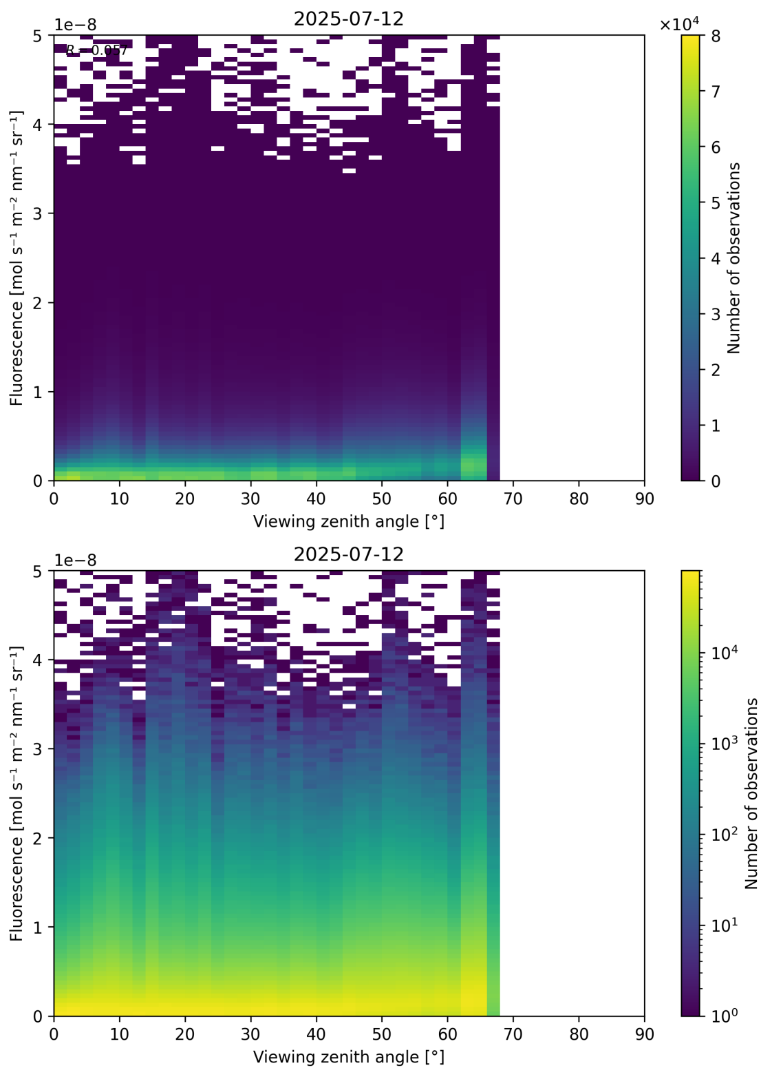
Figure 122: Scatter density plot of “Viewing zenith angle” against “Fluorescence” for 2025-07-11 to 2025-07-13.
