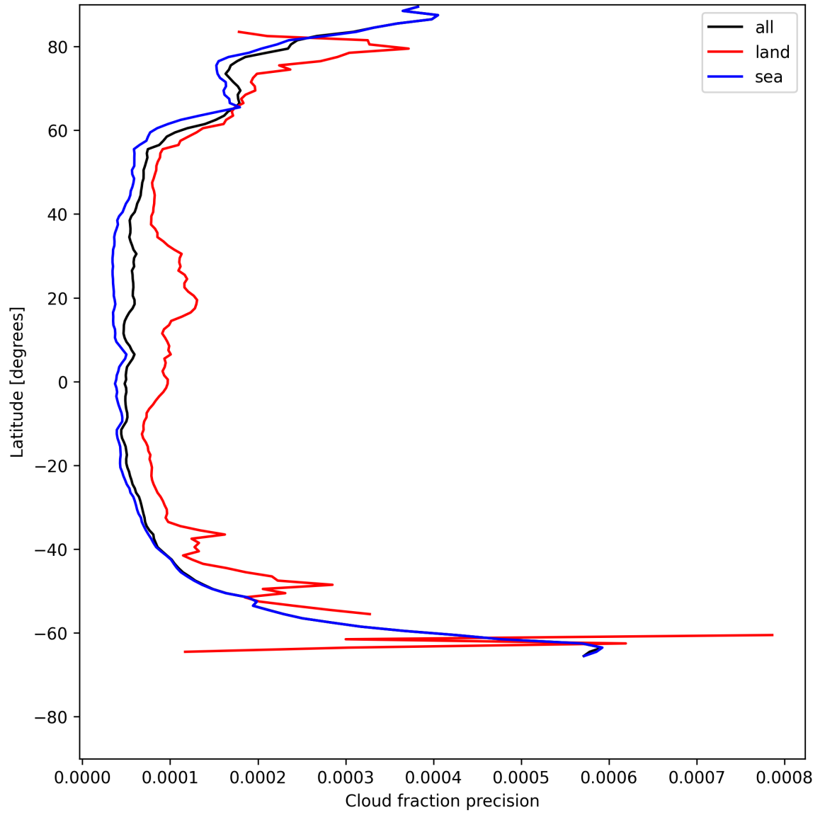
Figure 16: Zonal average of “Cloud fraction precision” for 2025-07-11 to 2025-07-13.
