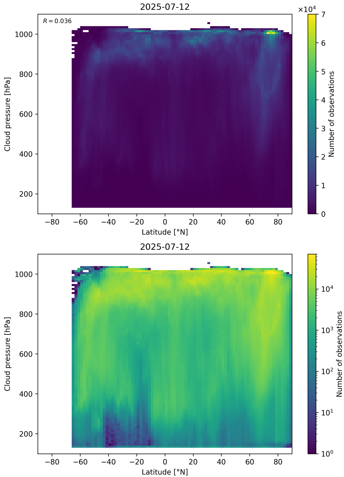
Figure 91: Scatter density plot of “Latitude” against “Cloud pressure” for 2025-07-11 to 2025-07-13.
