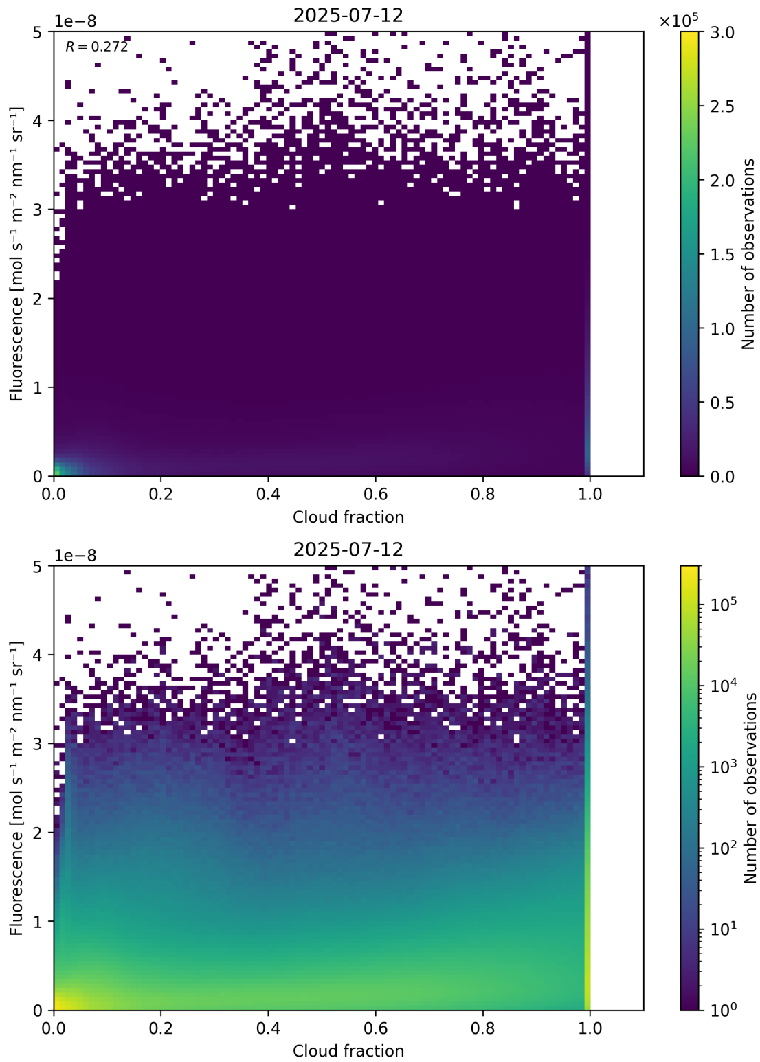
Figure 72: Scatter density plot of “Cloud fraction” against “Fluorescence” for 2025-07-11 to 2025-07-13.
