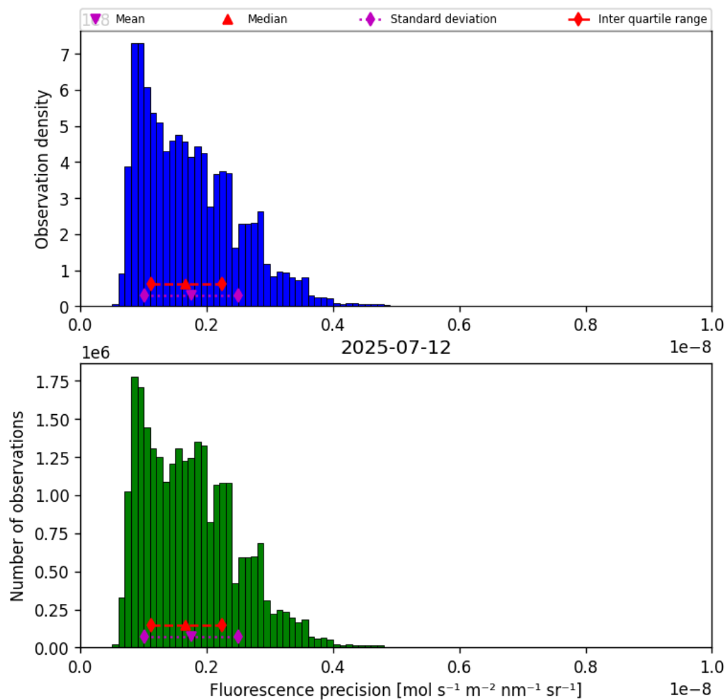
Figure 41: Histogram of “Fluorescence precision” for 2025-07-11 to 2025-07-13
