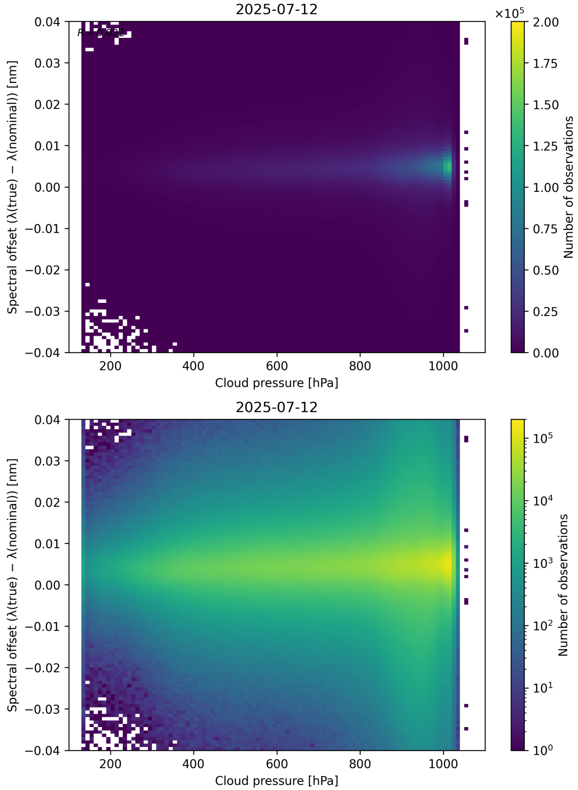
Figure 84: Scatter density plot of “Cloud pressure” against “Spectral offset ( \lambda_{\text{true}} - \lambda_{\text{nominal}} )” for 2025-07-11 to 2025-07-13.
