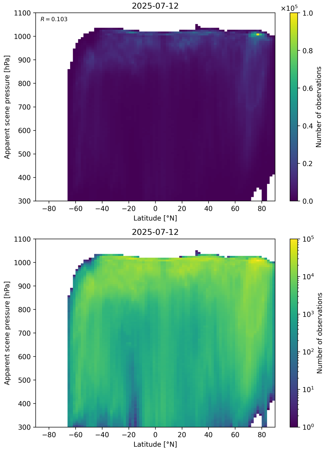
Figure 88: Scatter density plot of “Latitude” against “Apparent scene pressure” for 2025-07-11 to 2025-07-13.
