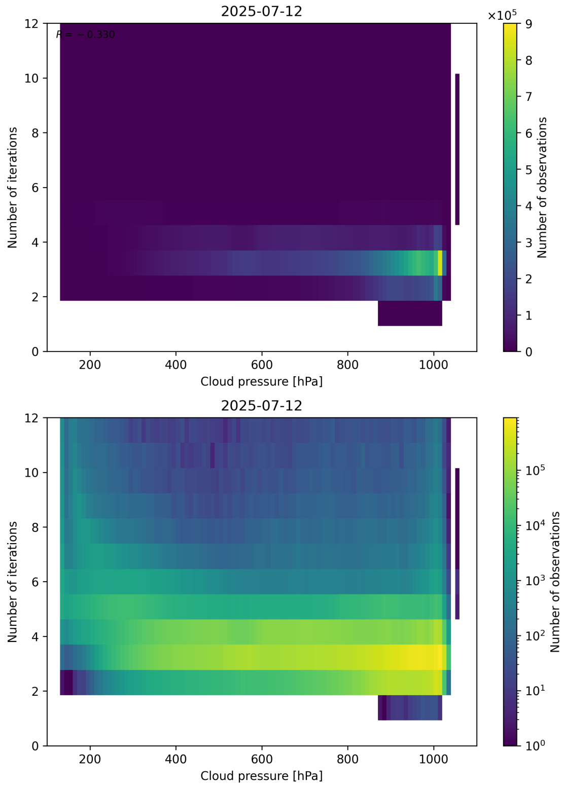
Figure 81: Scatter density plot of “Cloud pressure” against “Number of iterations” for 2025-07-11 to 2025-07-13.
