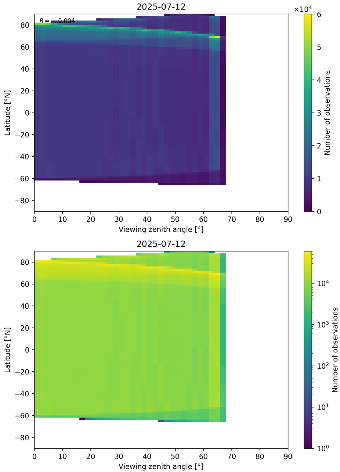
Figure 123: Scatter density plot of “Viewing zenith angle” against “Latitude” for 2025-07-11 to 2025-07-13.
