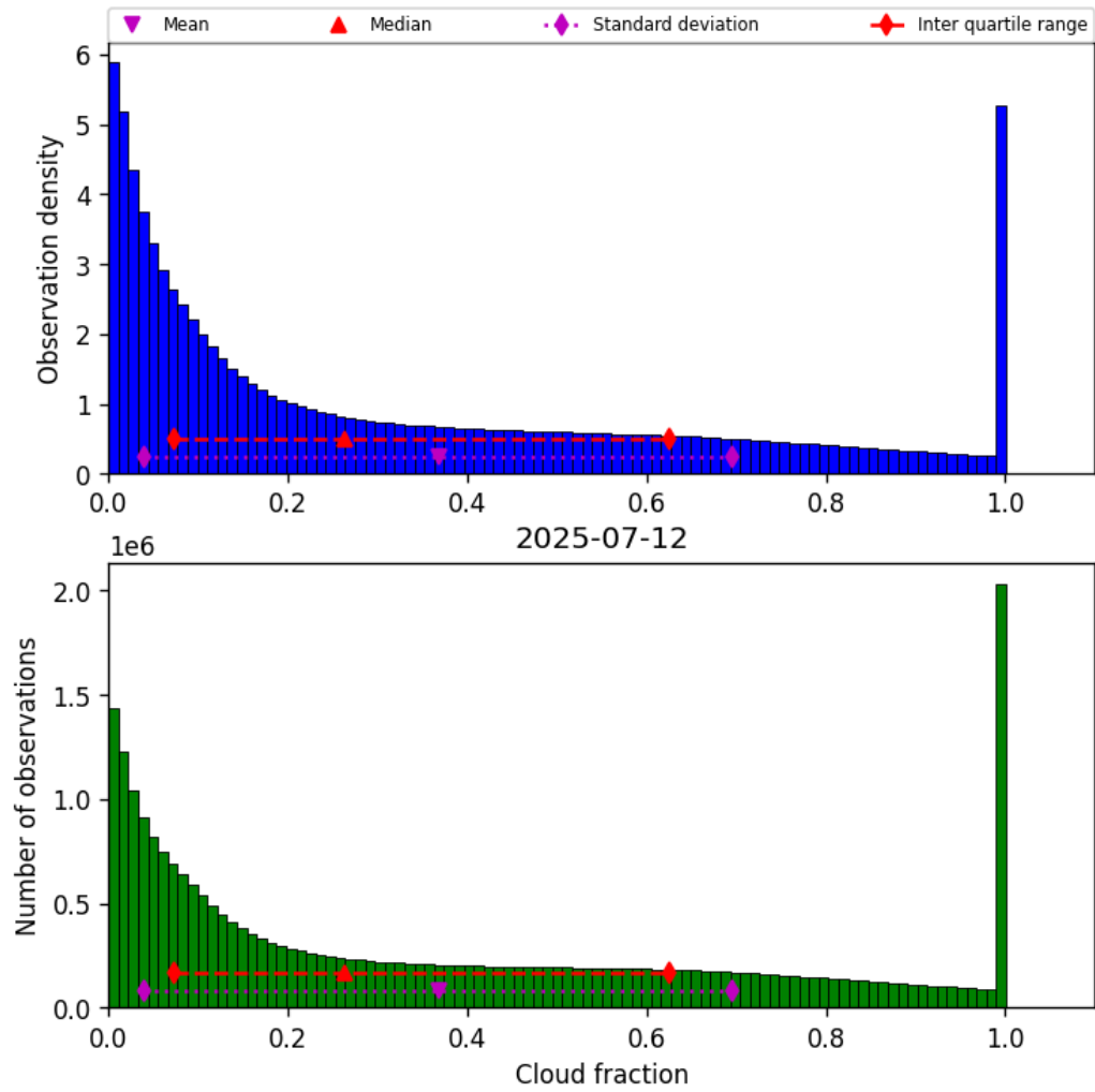
Figure 32: Histogram of “Cloud fraction” for 2025-07-11 to 2025-07-13
