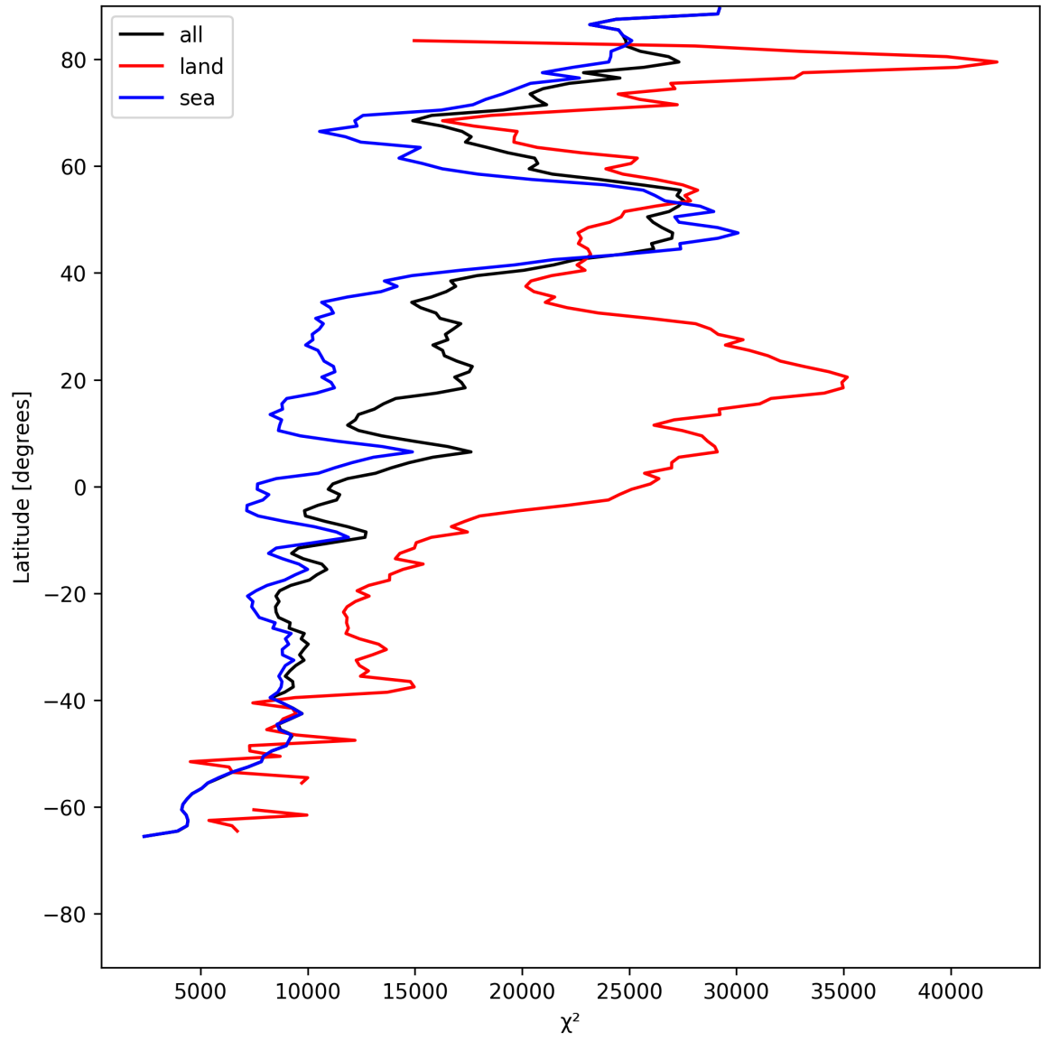
Figure 21: Zonal average of “ \chi^2 ” for 2025-07-11 to 2025-07-13.
