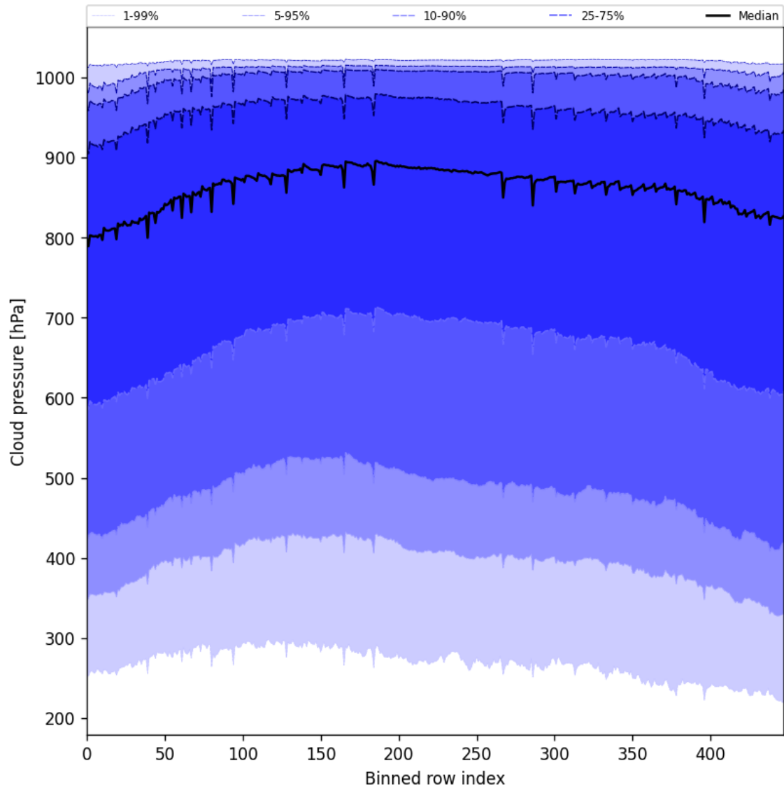
Figure 47: Along track statistics of “Cloud pressure” for 2025-07-11 to 2025-07-13
