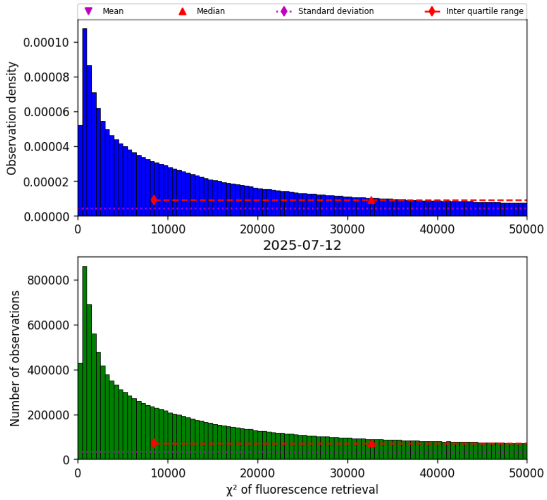
Figure 42: Histogram of “ \chi^2 of fluorescence retrieval” for 2025-07-11 to 2025-07-13
