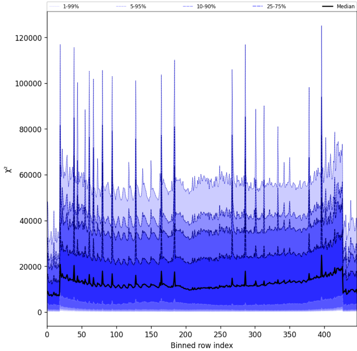
Figure 55: Along track statistics of “ \chi^2 ” for 2025-07-11 to 2025-07-13
