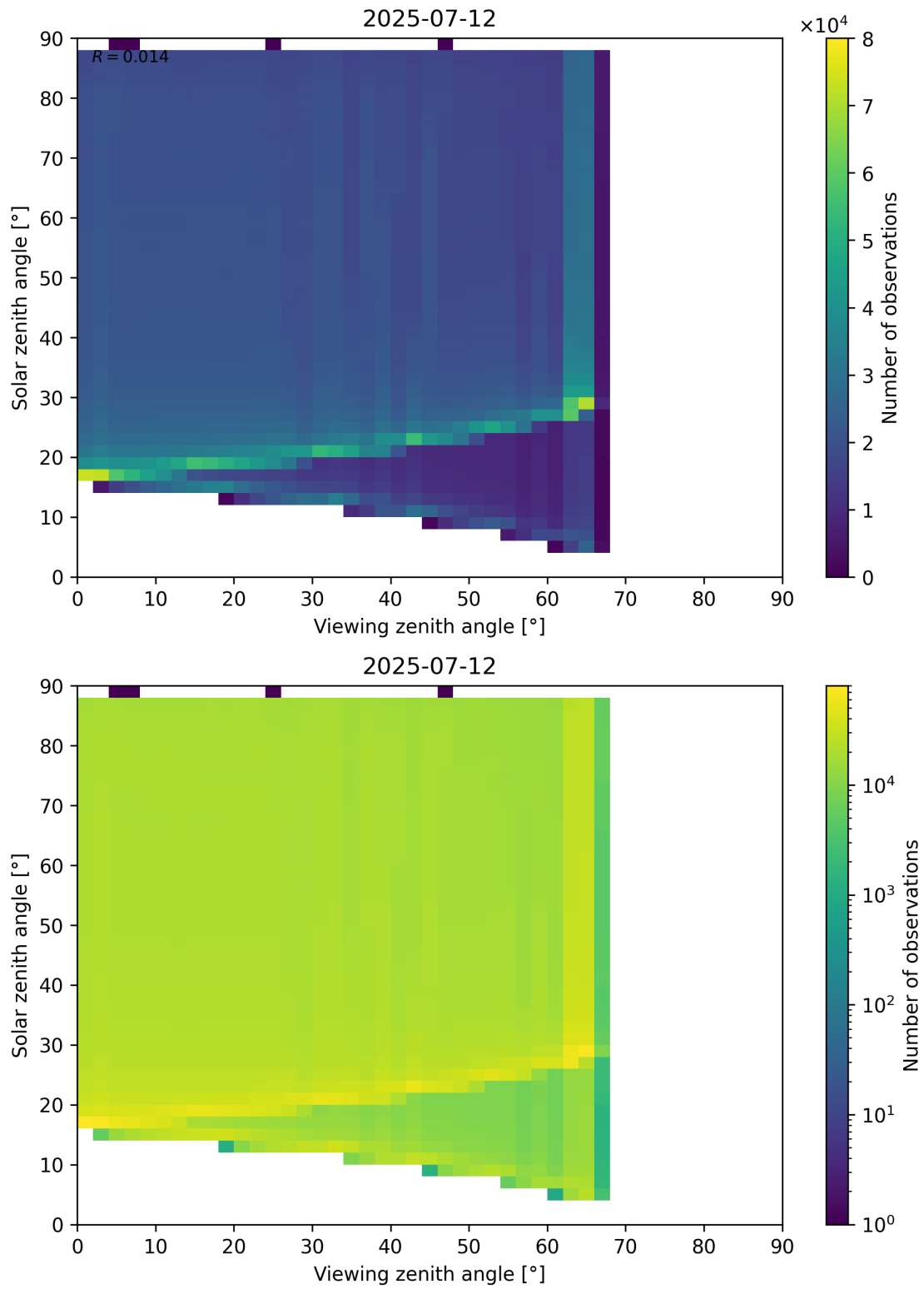
Figure 127: Scatter density plot of “Viewing zenith angle” against “Solar zenith angle” for 2025-07-11 to 2025-07-13.
