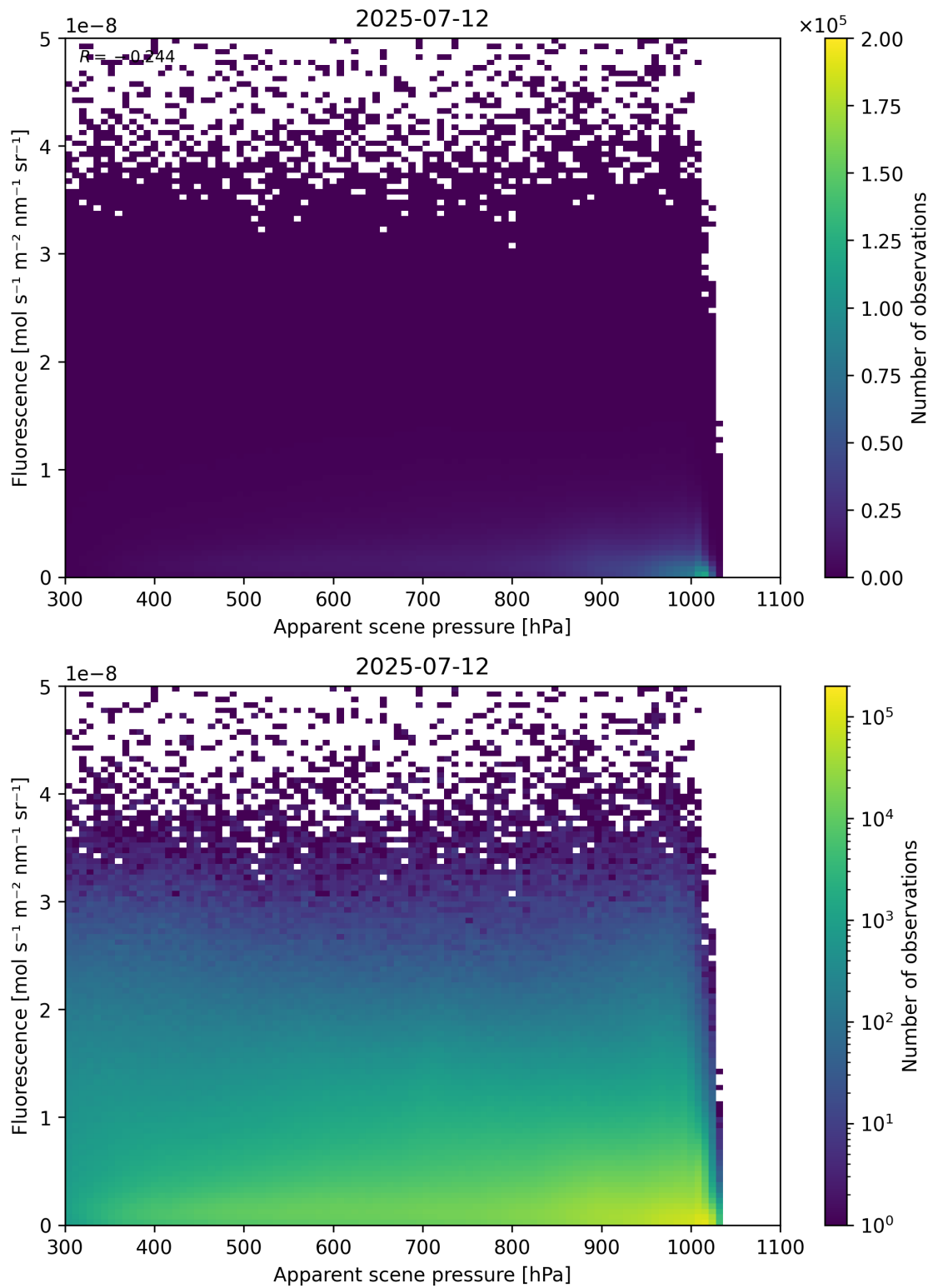
Figure 64: Scatter density plot of “Apparent scene pressure” against “Fluorescence” for 2025-07-11 to 2025-07-13.
