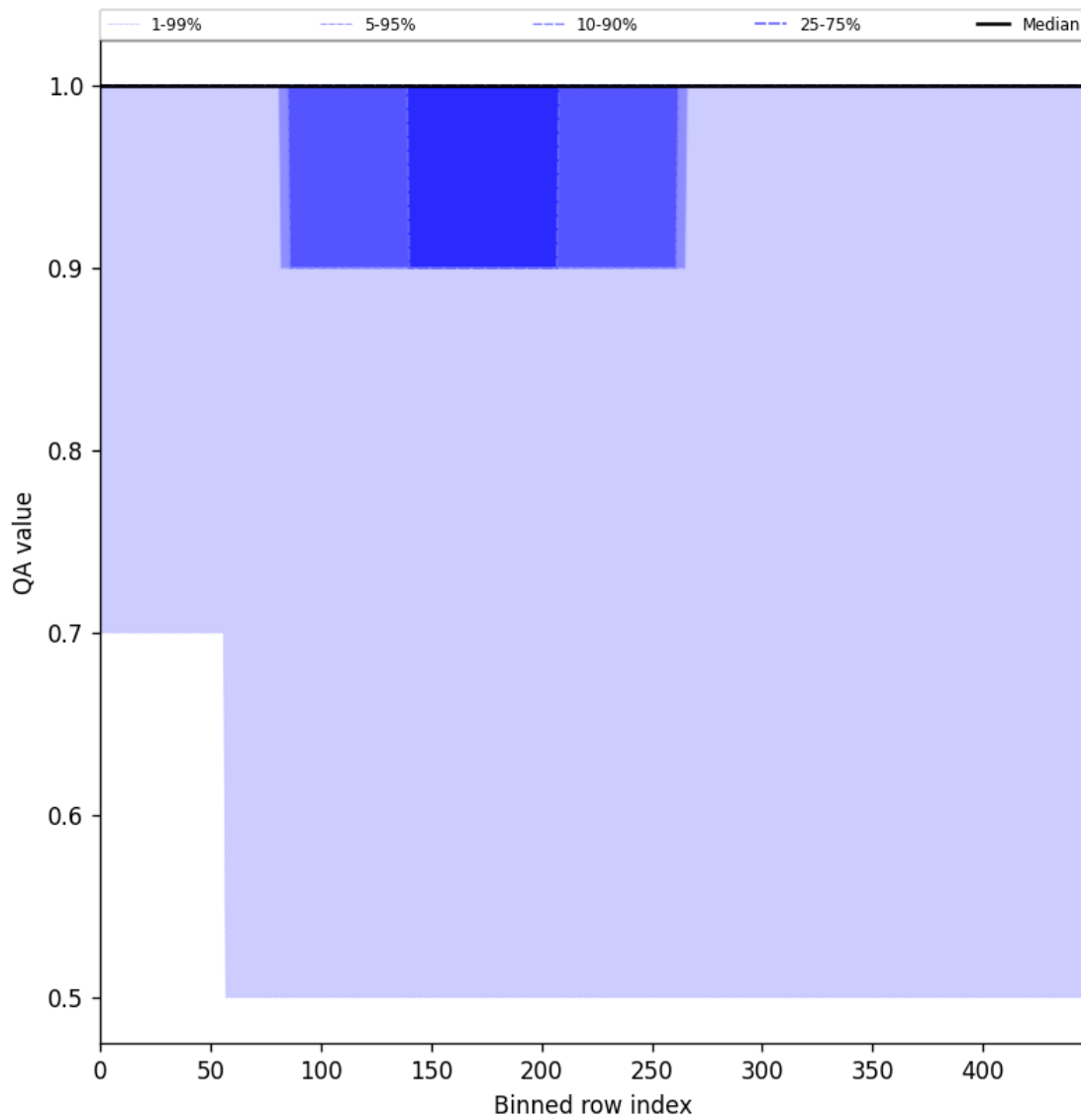
Figure 46: Along track statistics of “QA value” for 2025-07-11 to 2025-07-13
