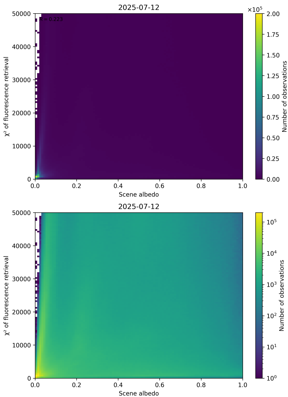
Figure 103: Scatter density plot of “Scene albedo” against “ \chi^2 of fluorescence retrieval” for 2025-07-11 to 2025-07-13.
