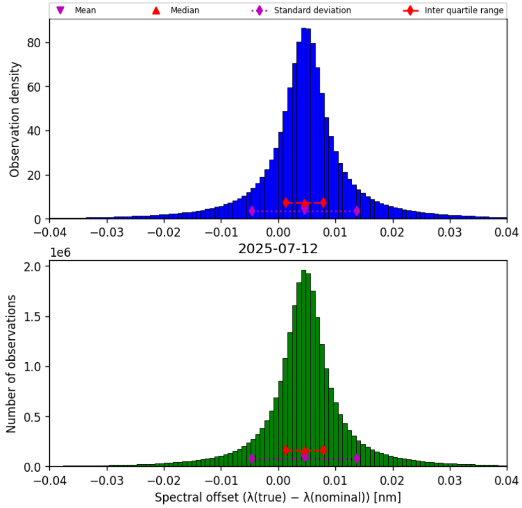
Figure 45: Histogram of “Spectral offset ( \lambda_{\text{true}} - \lambda_{\text{nominal}} )” for 2025-07-11 to 2025-07-13
