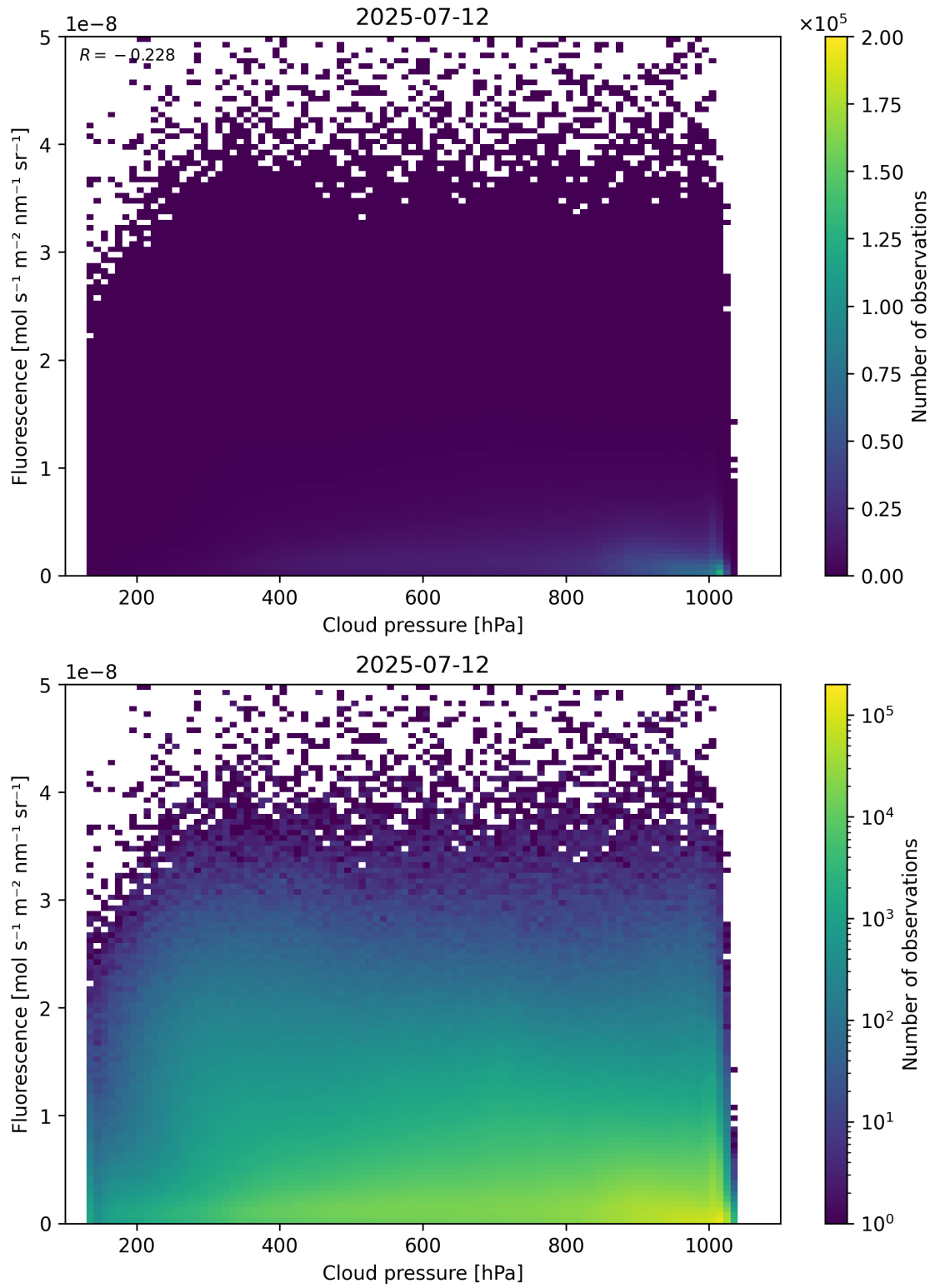
Figure 80: Scatter density plot of “Cloud pressure” against “Fluorescence” for 2025-07-11 to 2025-07-13.
