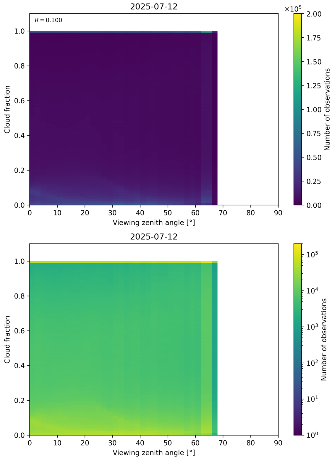
Figure 120: Scatter density plot of “Viewing zenith angle” against “Cloud fraction” for 2025-07-11 to 2025-07-13.
