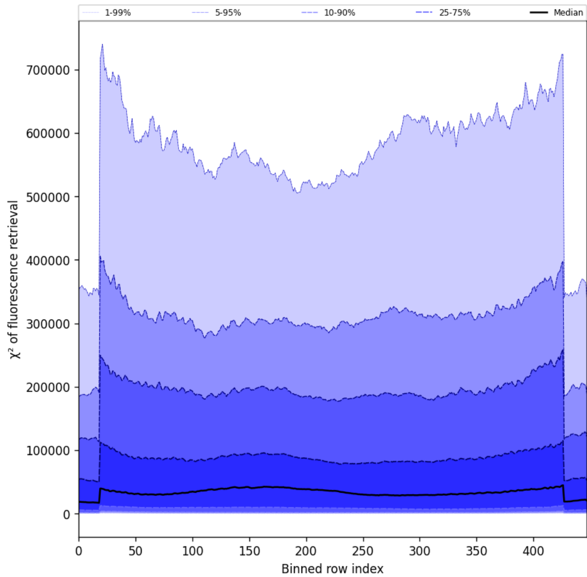
Figure 59: Along track statistics of “ \chi^2 of fluorescence retrieval” for 2025-07-11 to 2025-07-13
