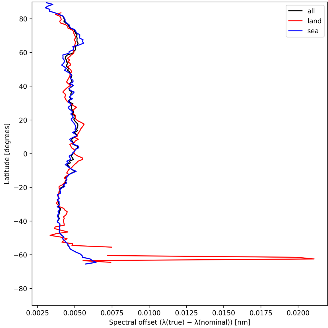
Figure 28: Zonal average of “Spectral offset ( \lambda_{\text{true}} - \lambda_{\text{nominal}} )” for 2025-07-11 to 2025-07-13.
