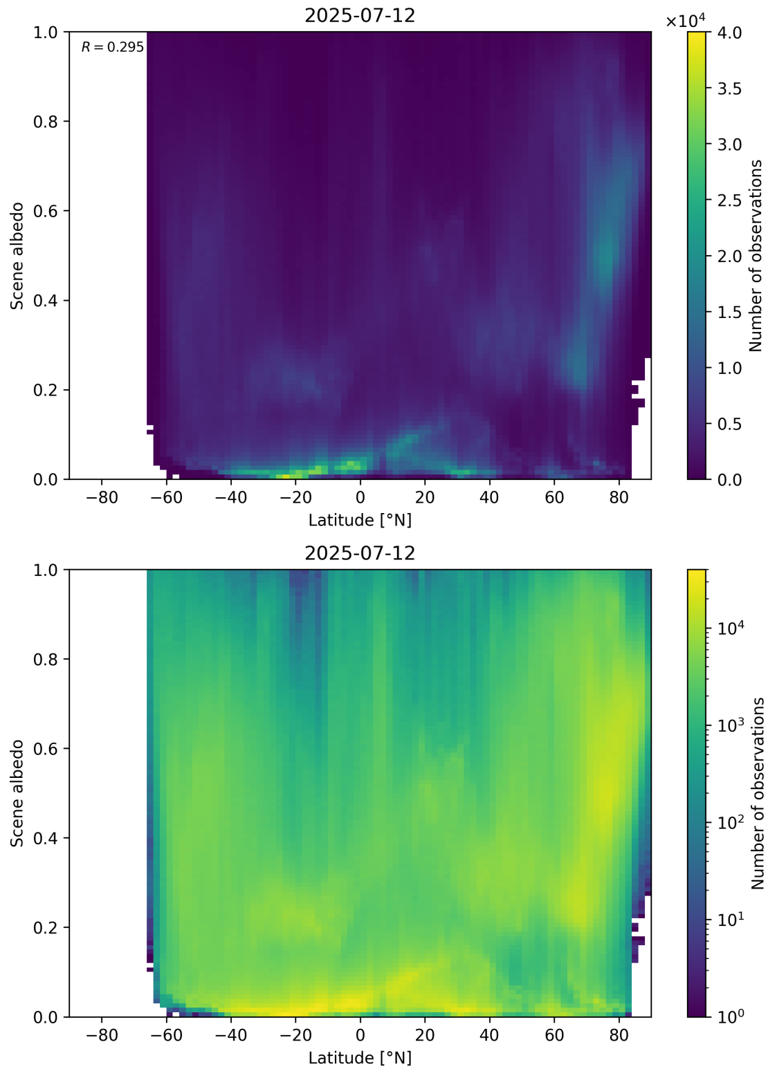
Figure 95: Scatter density plot of “Latitude” against “Scene albedo” for 2025-07-11 to 2025-07-13.
