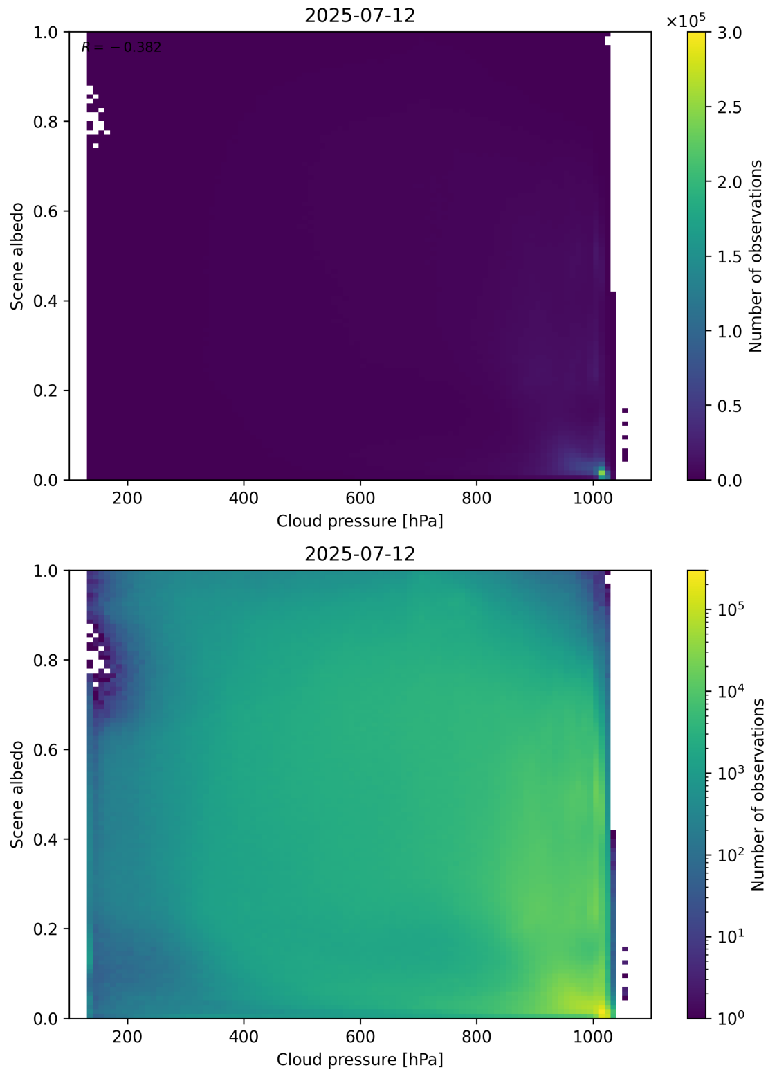
Figure 83: Scatter density plot of “Cloud pressure” against “Scene albedo” for 2025-07-11 to 2025-07-13.
