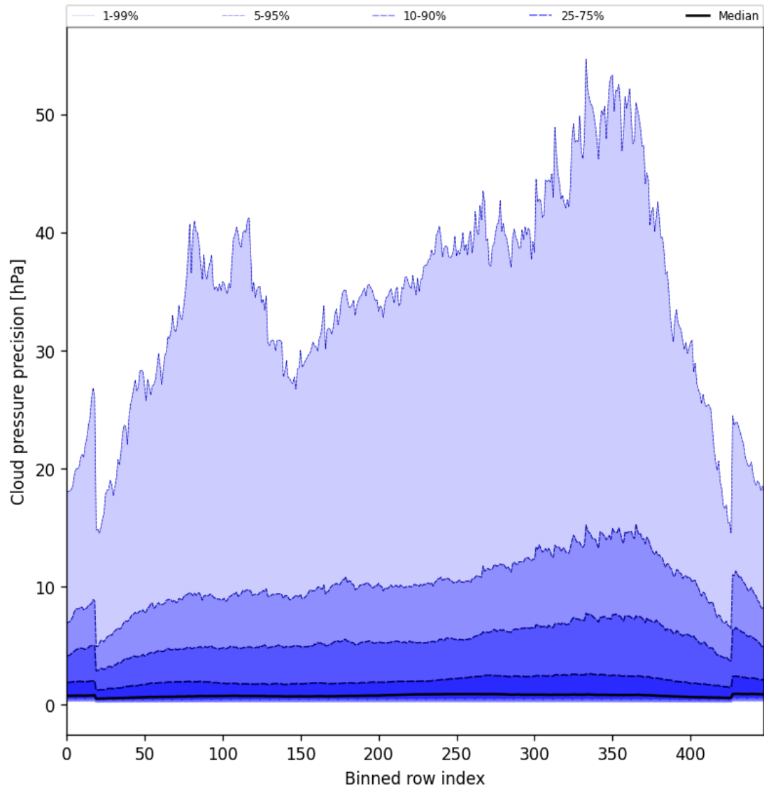
Figure 48: Along track statistics of “Cloud pressure precision” for 2025-07-11 to 2025-07-13
