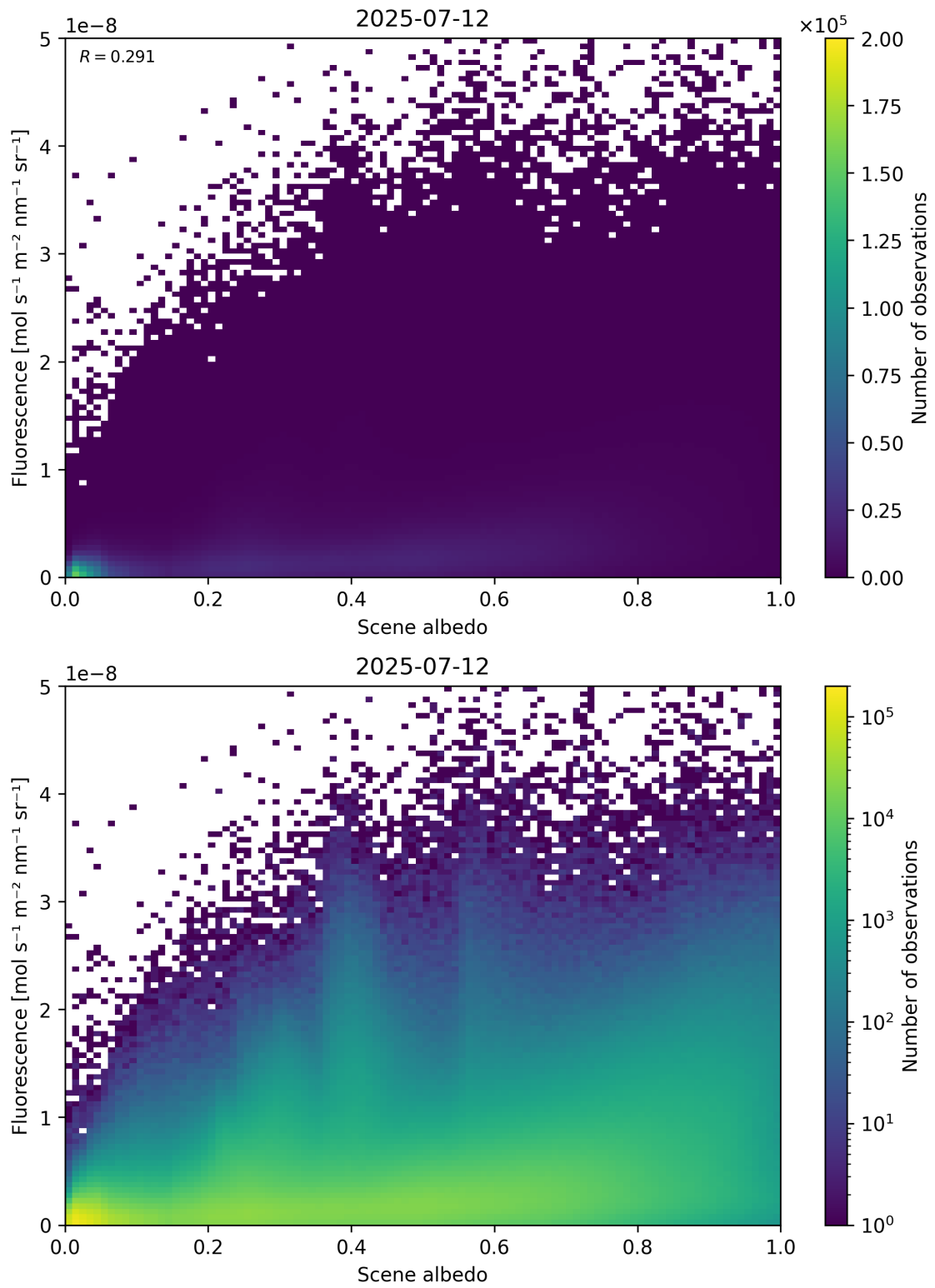
Figure 104: Scatter density plot of “Scene albedo” against “Fluorescence” for 2025-07-11 to 2025-07-13.
