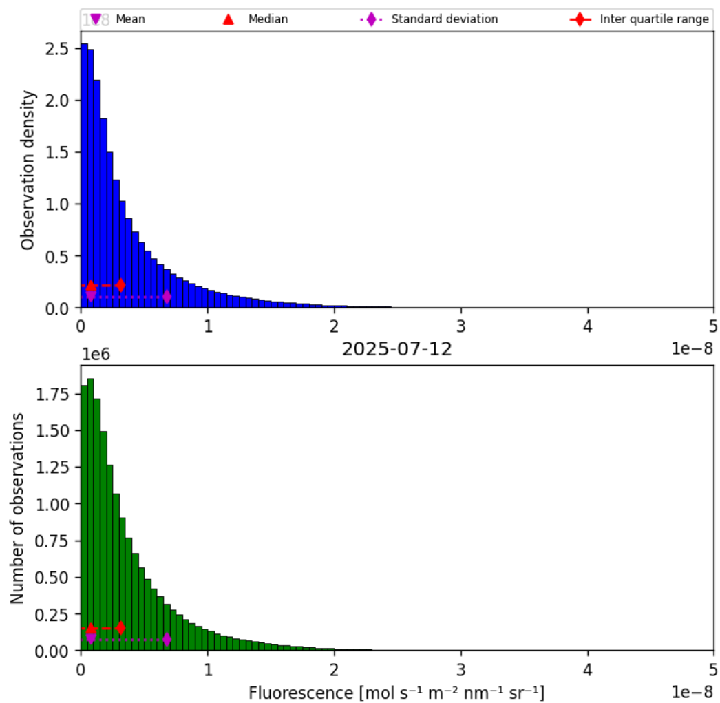
Figure 40: Histogram of “Fluorescence” for 2025-07-11 to 2025-07-13
