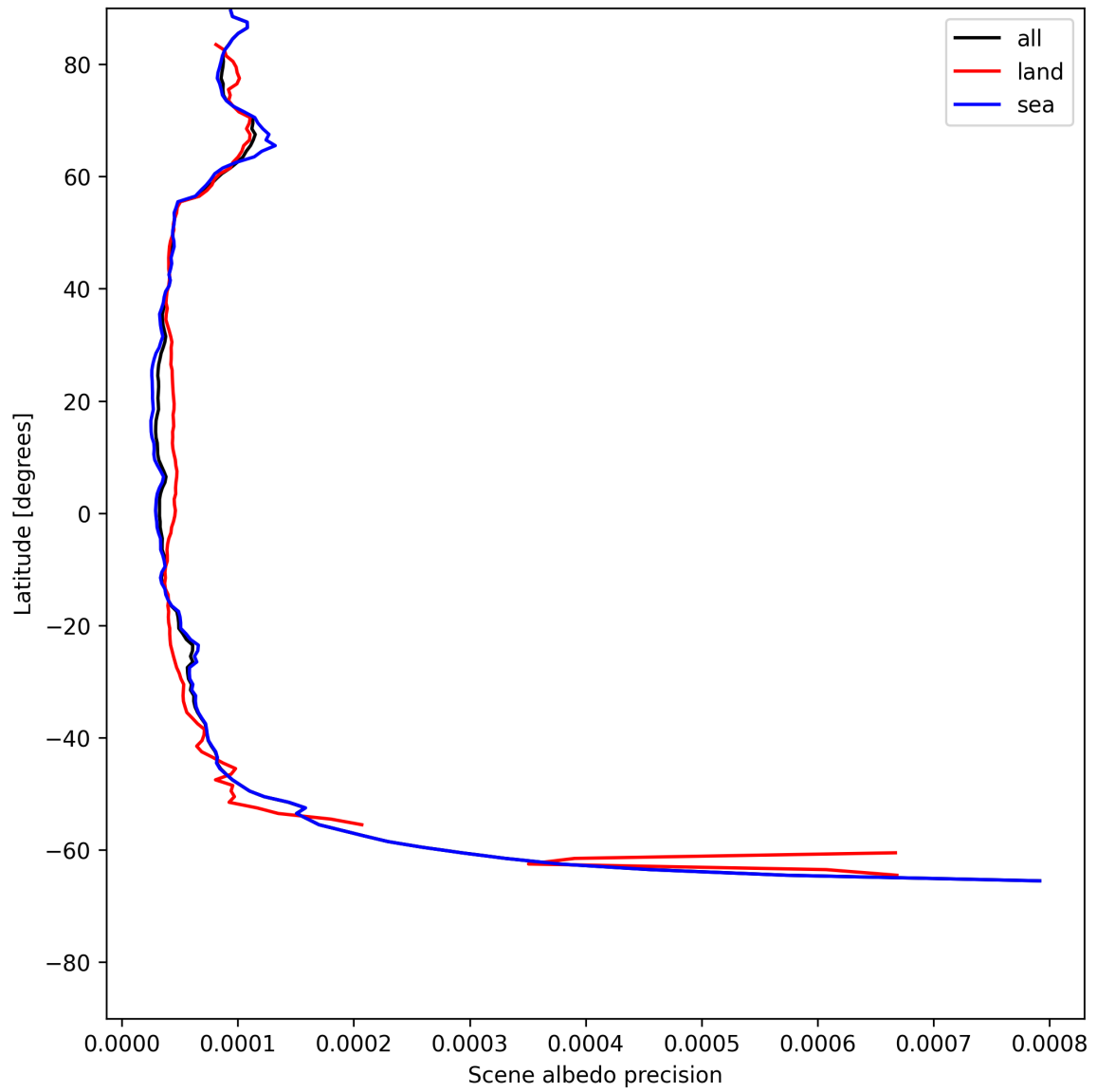
Figure 18: Zonal average of “Scene albedo precision” for 2025-07-11 to 2025-07-13.
