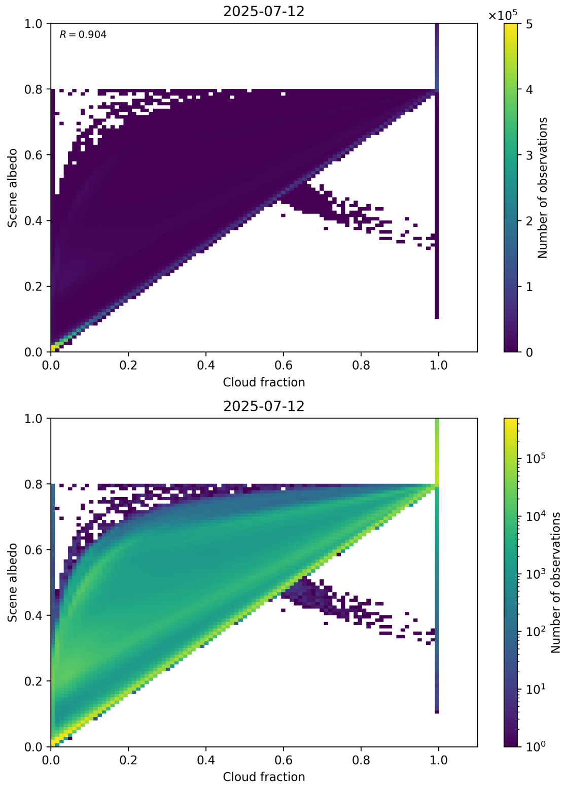
Figure 75: Scatter density plot of “Cloud fraction” against “Scene albedo” for 2025-07-11 to 2025-07-13.
