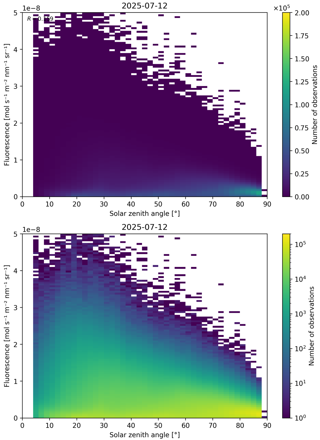
Figure 112: Scatter density plot of “Solar zenith angle” against “Fluorescence” for 2025-07-11 to 2025-07-13.
