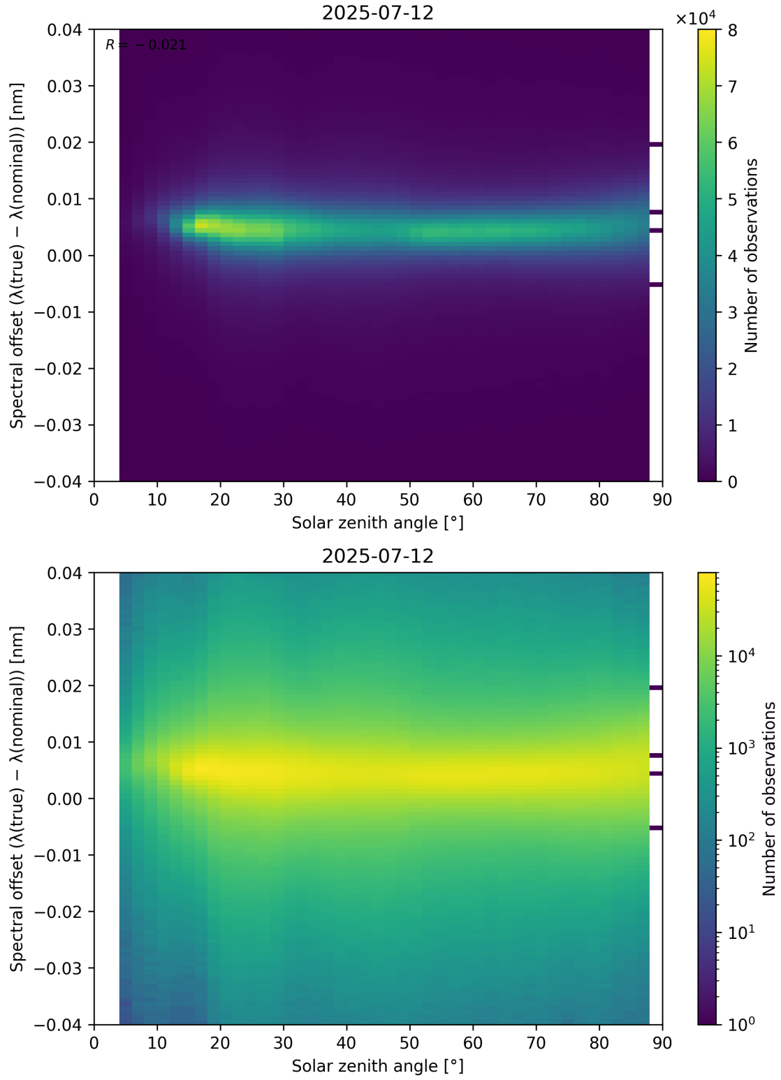
Figure 117: Scatter density plot of “Solar zenith angle” against “Spectral offset ( \lambda_{\text{true}} - \lambda_{\text{nominal}} )” for 2025-07-11 to 2025-07-13.
