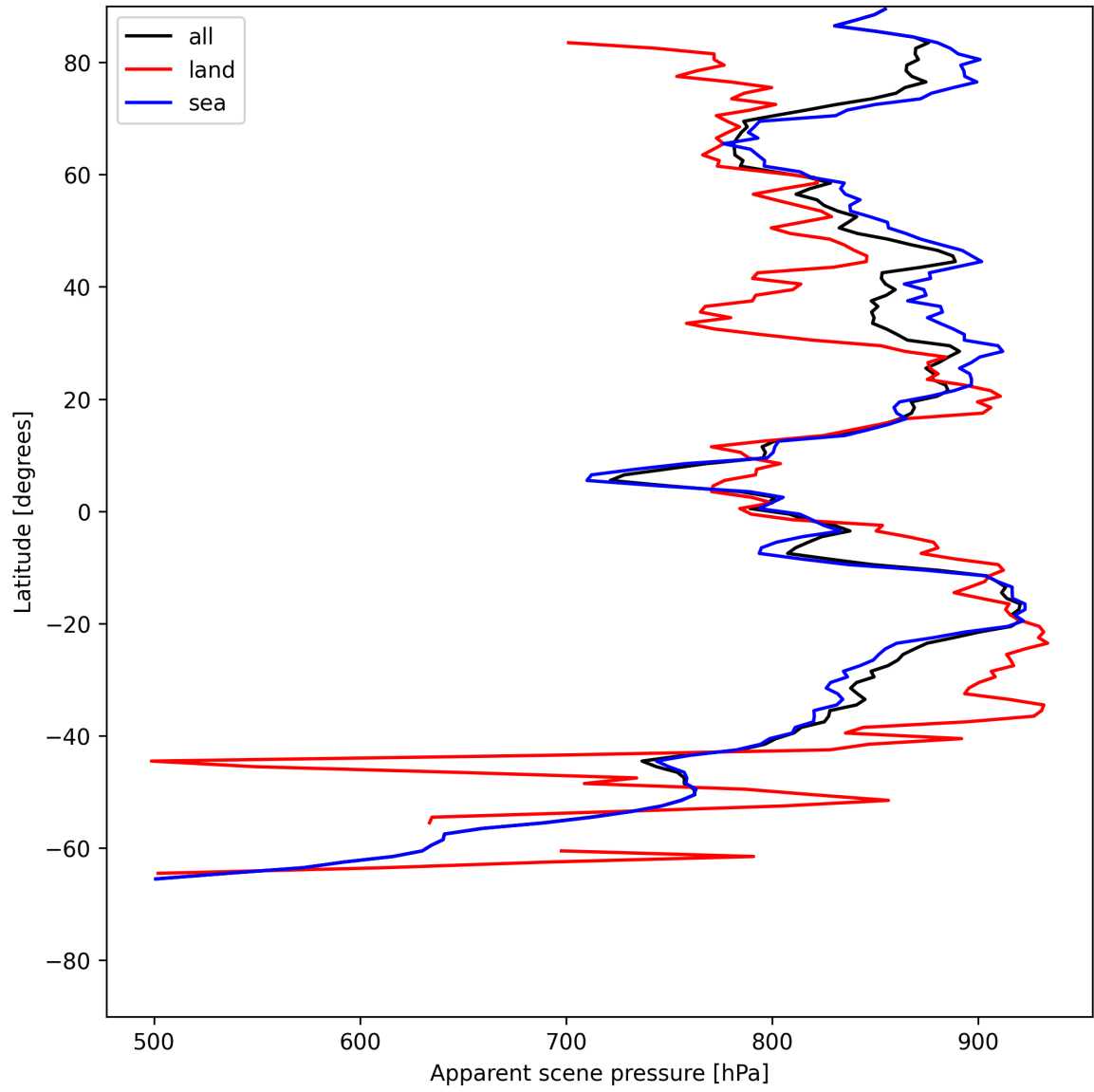
Figure 19: Zonal average of “Apparent scene pressure” for 2025-07-11 to 2025-07-13.
