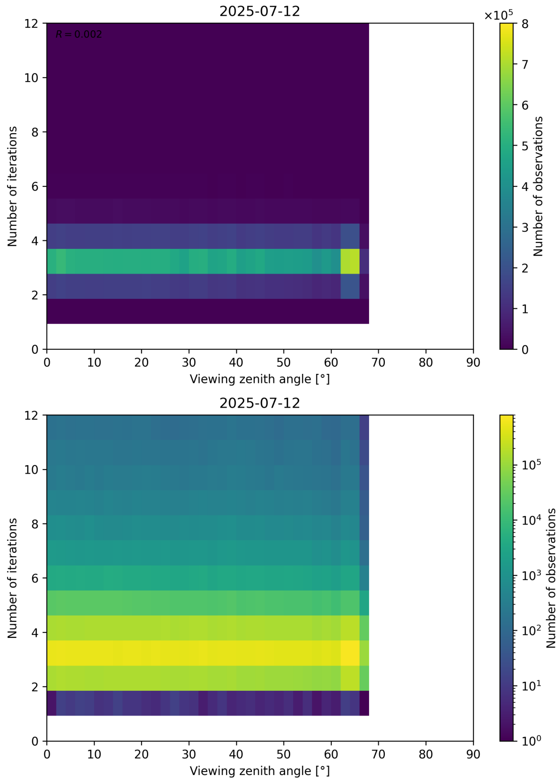
Figure 124: Scatter density plot of “Viewing zenith angle” against “Number of iterations” for 2025-07-11 to 2025-07-13.
