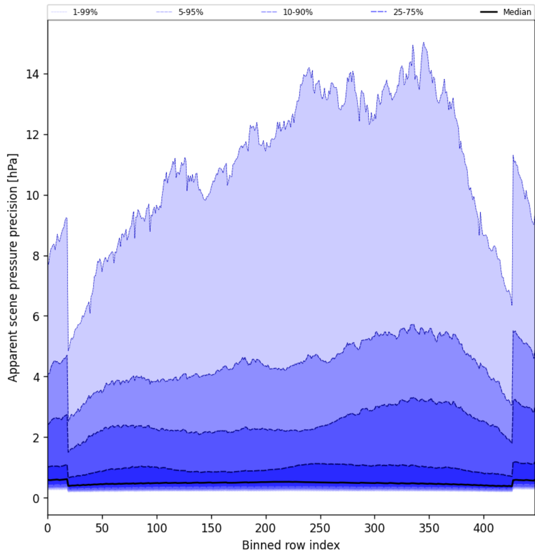
Figure 54: Along track statistics of “Apparent scene pressure precision” for 2025-07-11 to 2025-07-13
