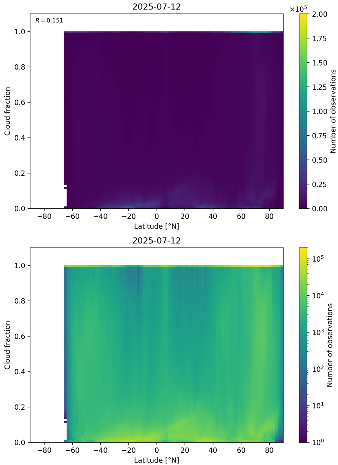
Figure 90: Scatter density plot of “Latitude” against “Cloud fraction” for 2025-07-11 to 2025-07-13.
