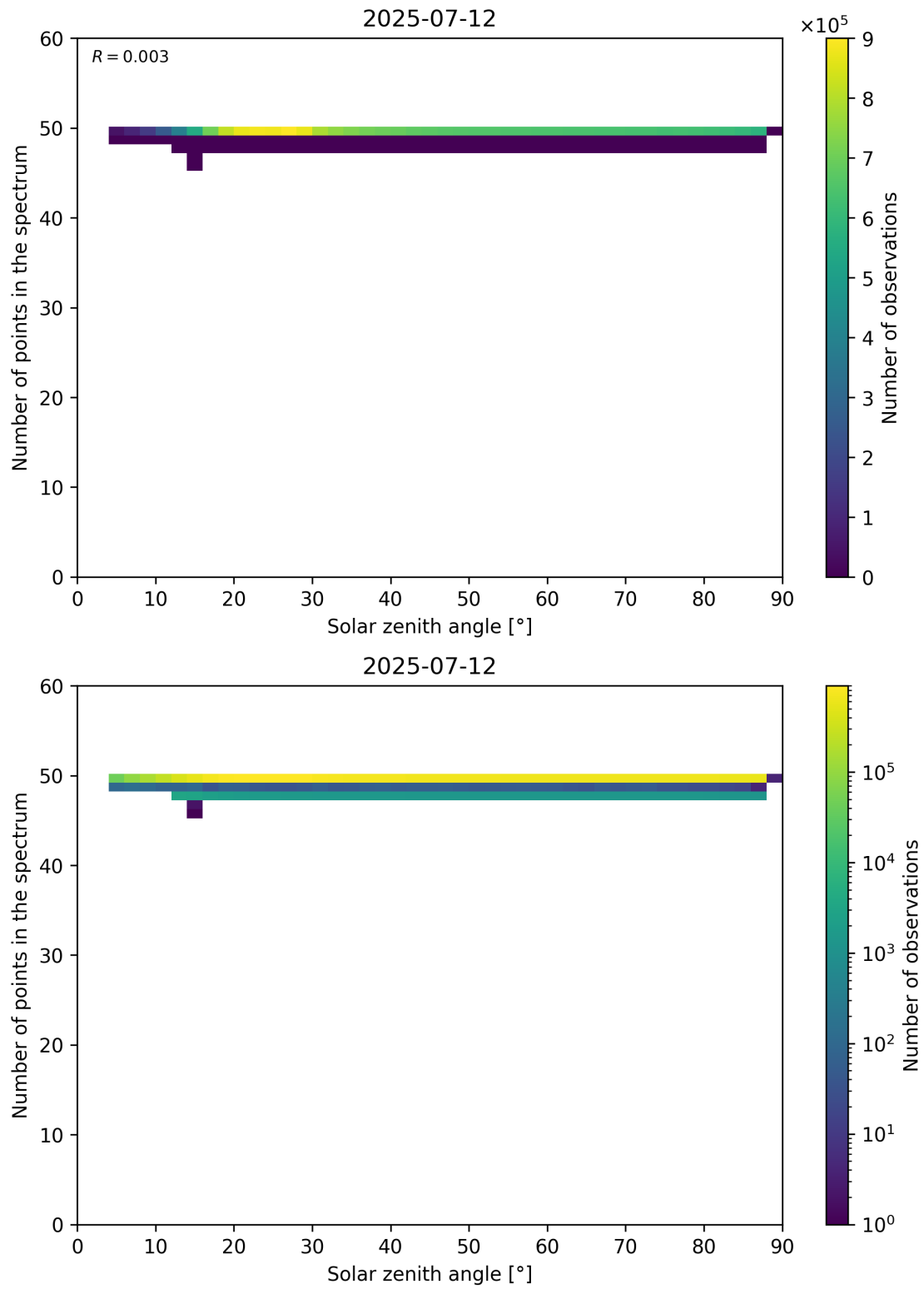
Figure 115: Scatter density plot of “Solar zenith angle” against “Number of points in the spectrum” for 2025-07-11 to 2025-07-13.
