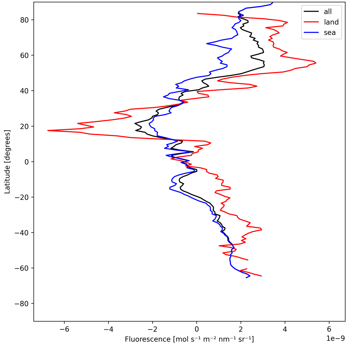
Figure 23: Zonal average of “Fluorescence” for 2025-07-11 to 2025-07-13.
