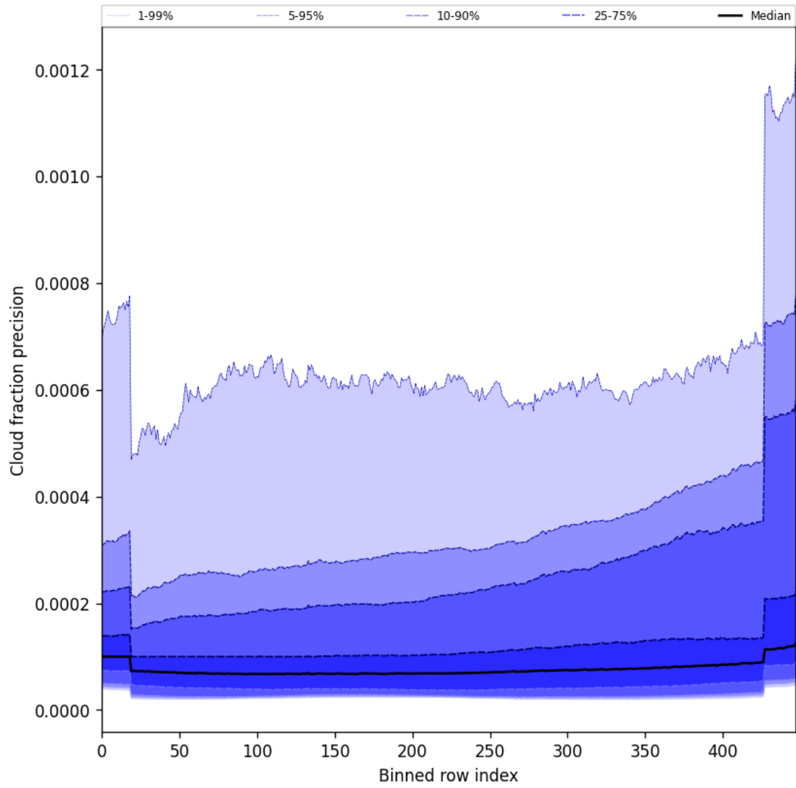
Figure 50: Along track statistics of “Cloud fraction precision” for 2025-07-11 to 2025-07-13
