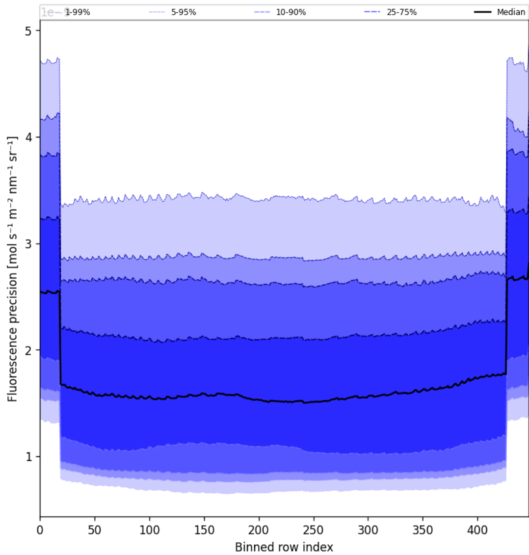
Figure 58: Along track statistics of “Fluorescence precision” for 2025-07-11 to 2025-07-13
