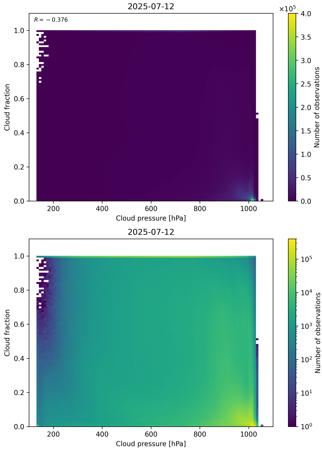
Figure 79: Scatter density plot of “Cloud pressure” against “Cloud fraction” for 2025-07-11 to 2025-07-13.
