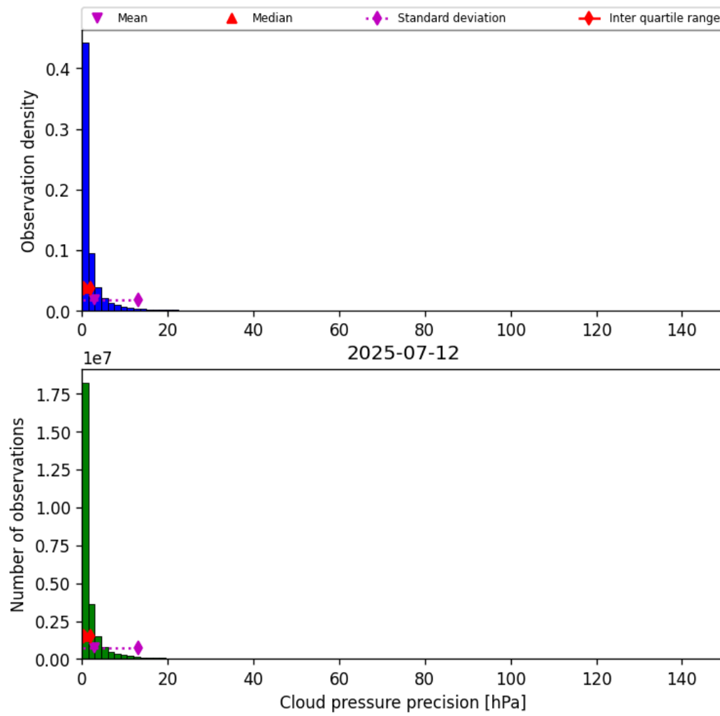
Figure 31: Histogram of “Cloud pressure precision” for 2025-07-11 to 2025-07-13
