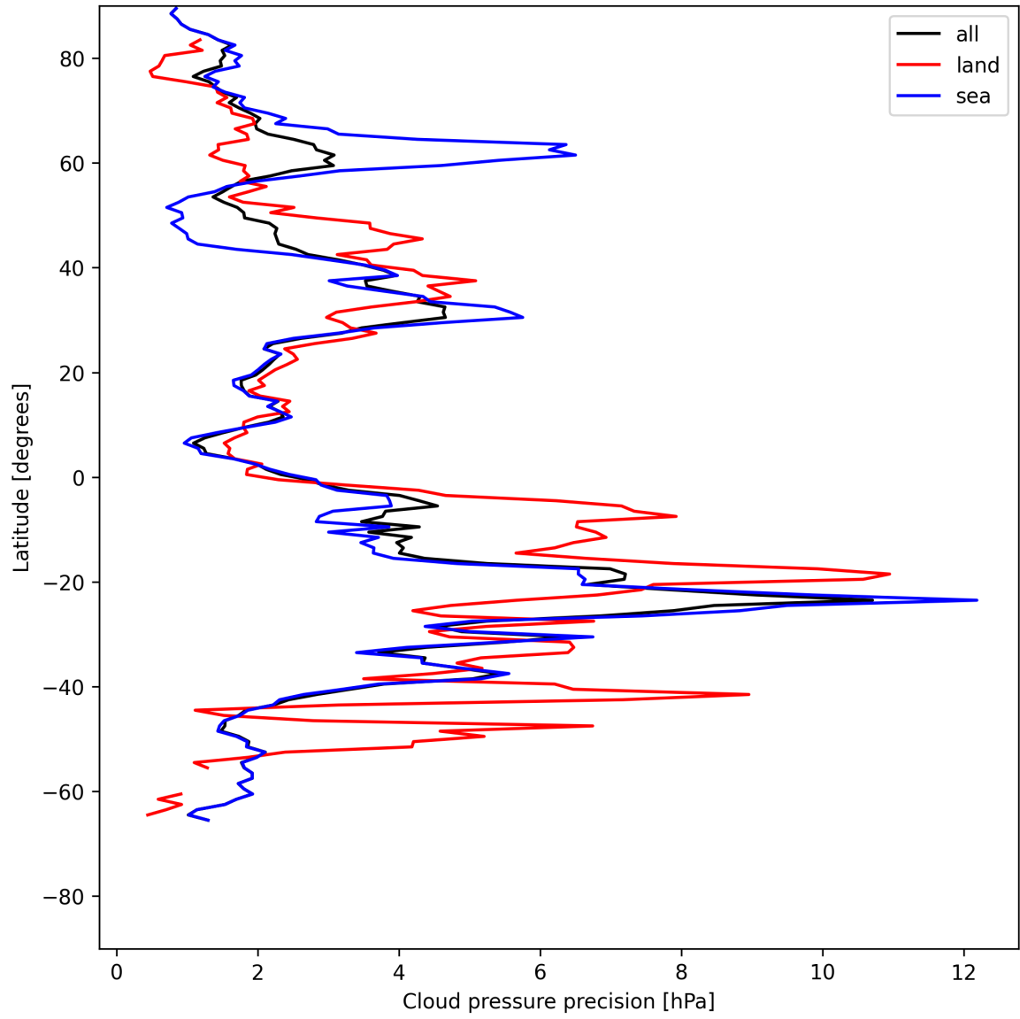
Figure 14: Zonal average of “Cloud pressure precision” for 2025-07-11 to 2025-07-13.
