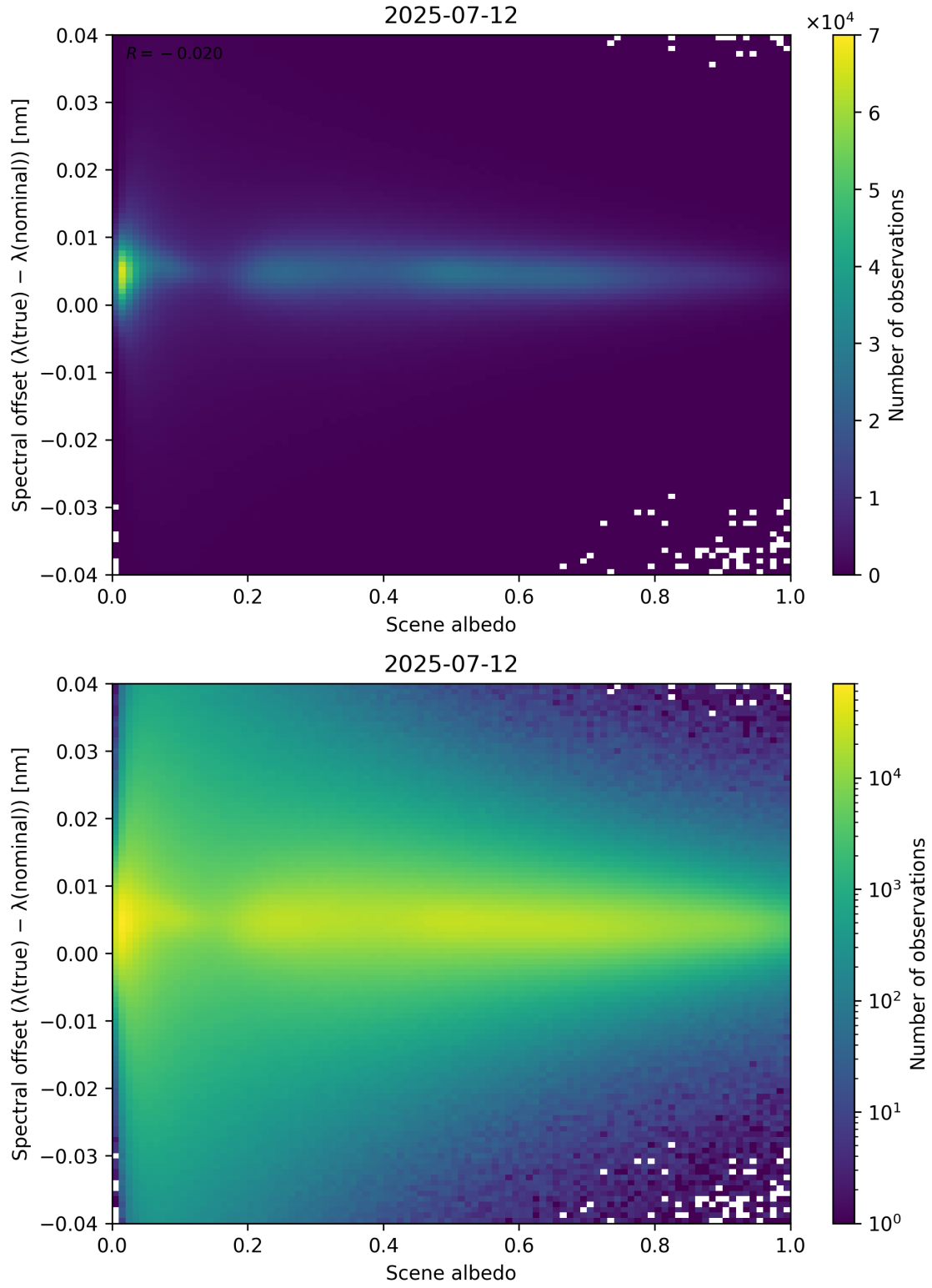
Figure 107: Scatter density plot of “Scene albedo” against “Spectral offset ( \lambda_{\text{true}} - \lambda_{\text{nominal}} )” for 2025-07-11 to 2025-07-13.
