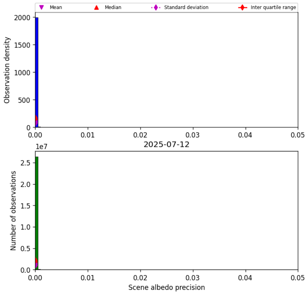
Figure 35: Histogram of “Scene albedo precision” for 2025-07-11 to 2025-07-13
