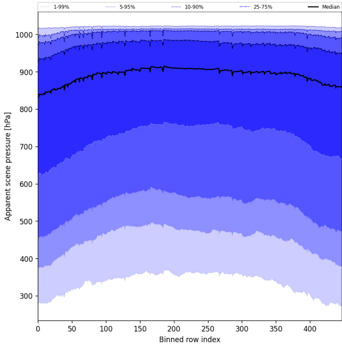
Figure 53: Along track statistics of “Apparent scene pressure” for 2025-07-11 to 2025-07-13
