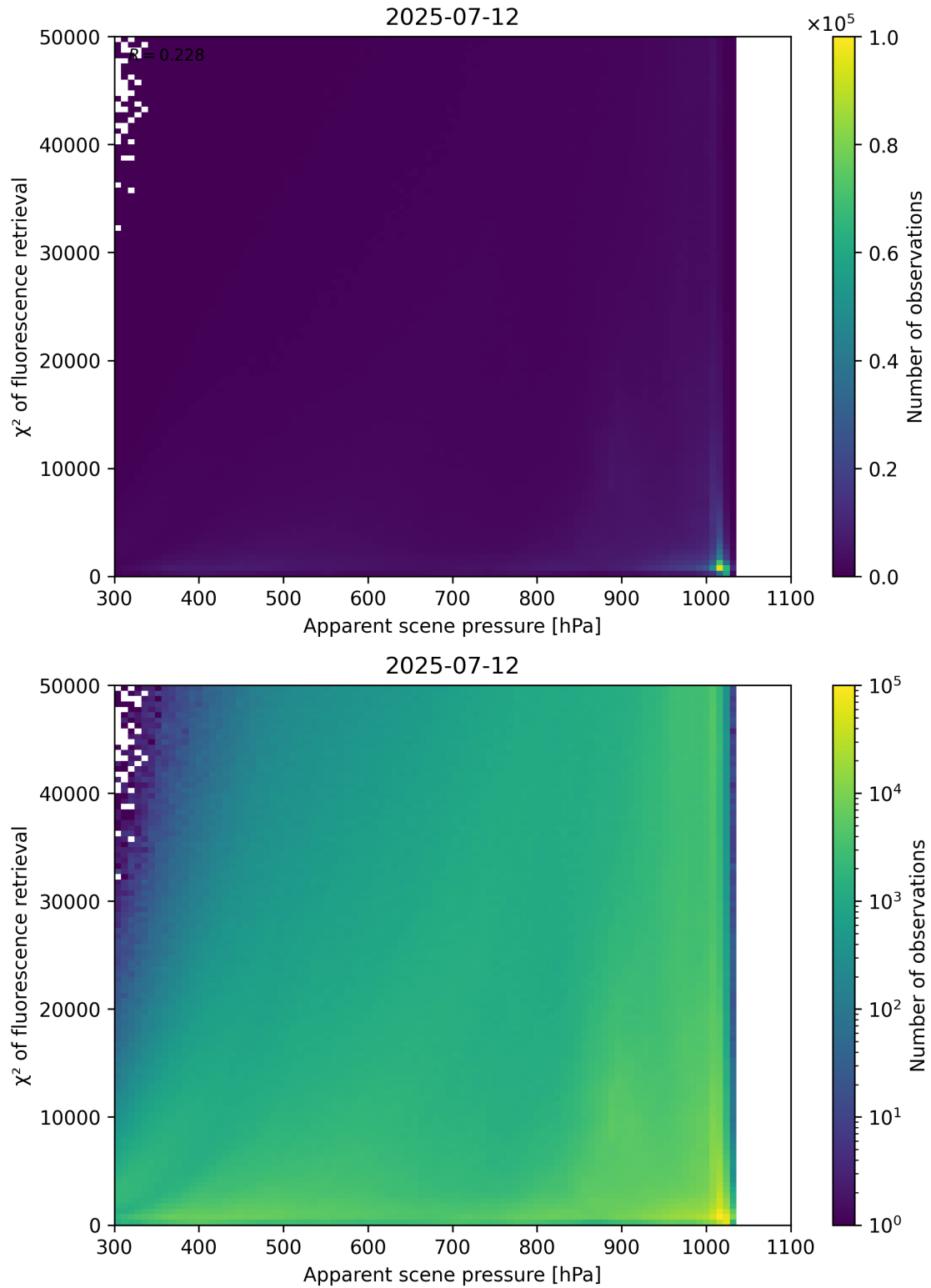
Figure 63: Scatter density plot of “Apparent scene pressure” against “ \chi^2 of fluorescence retrieval” for 2025-07-11 to 2025-07-13.
