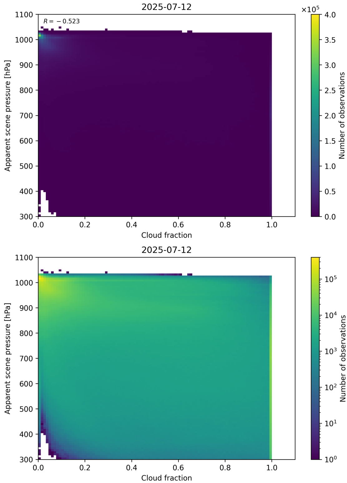
Figure 70: Scatter density plot of “Cloud fraction” against “Apparent scene pressure” for 2025-07-11 to 2025-07-13.
