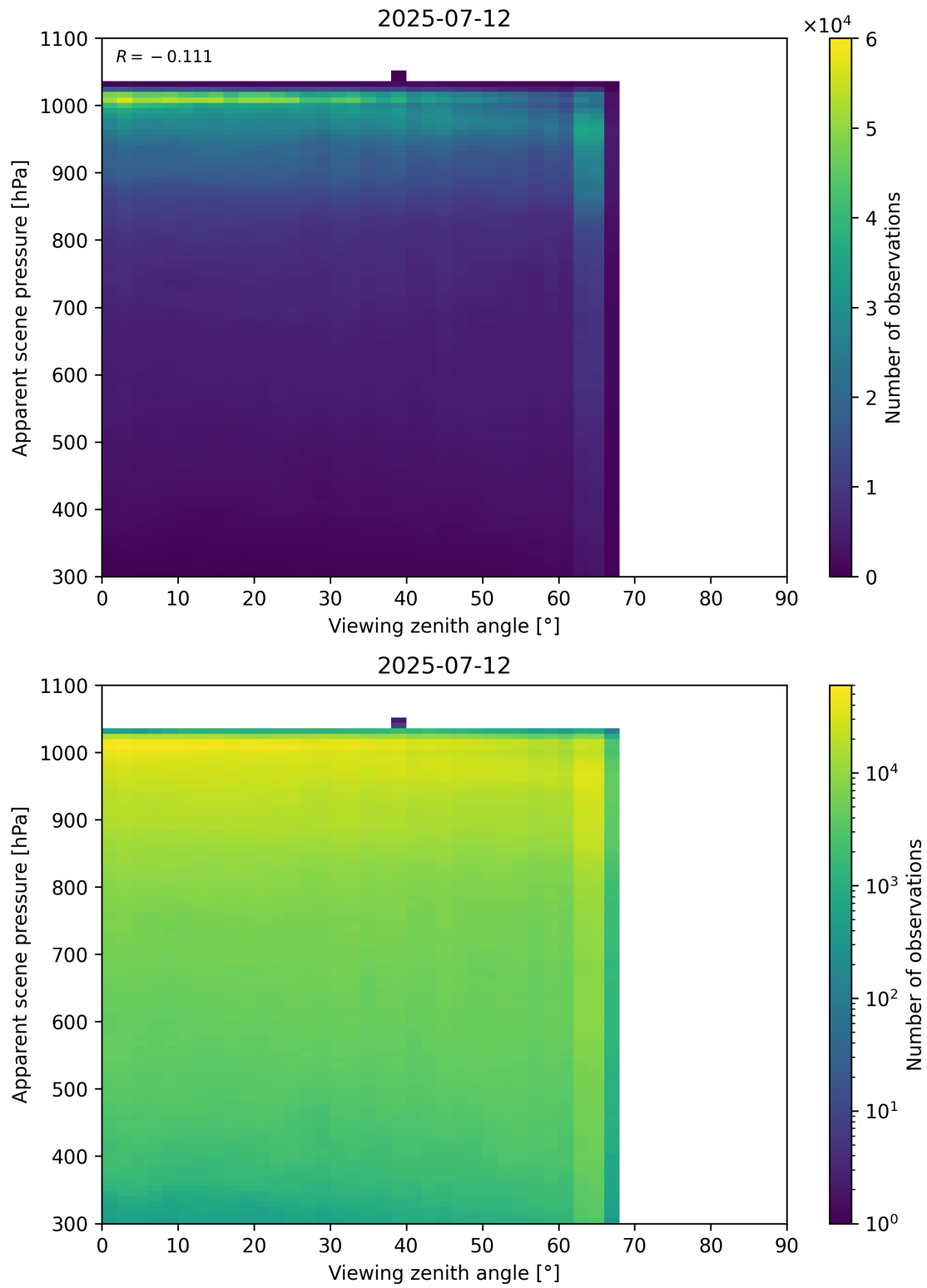
Figure 118: Scatter density plot of “Viewing zenith angle” against “Apparent scene pressure” for 2025-07-11 to 2025-07-13.
