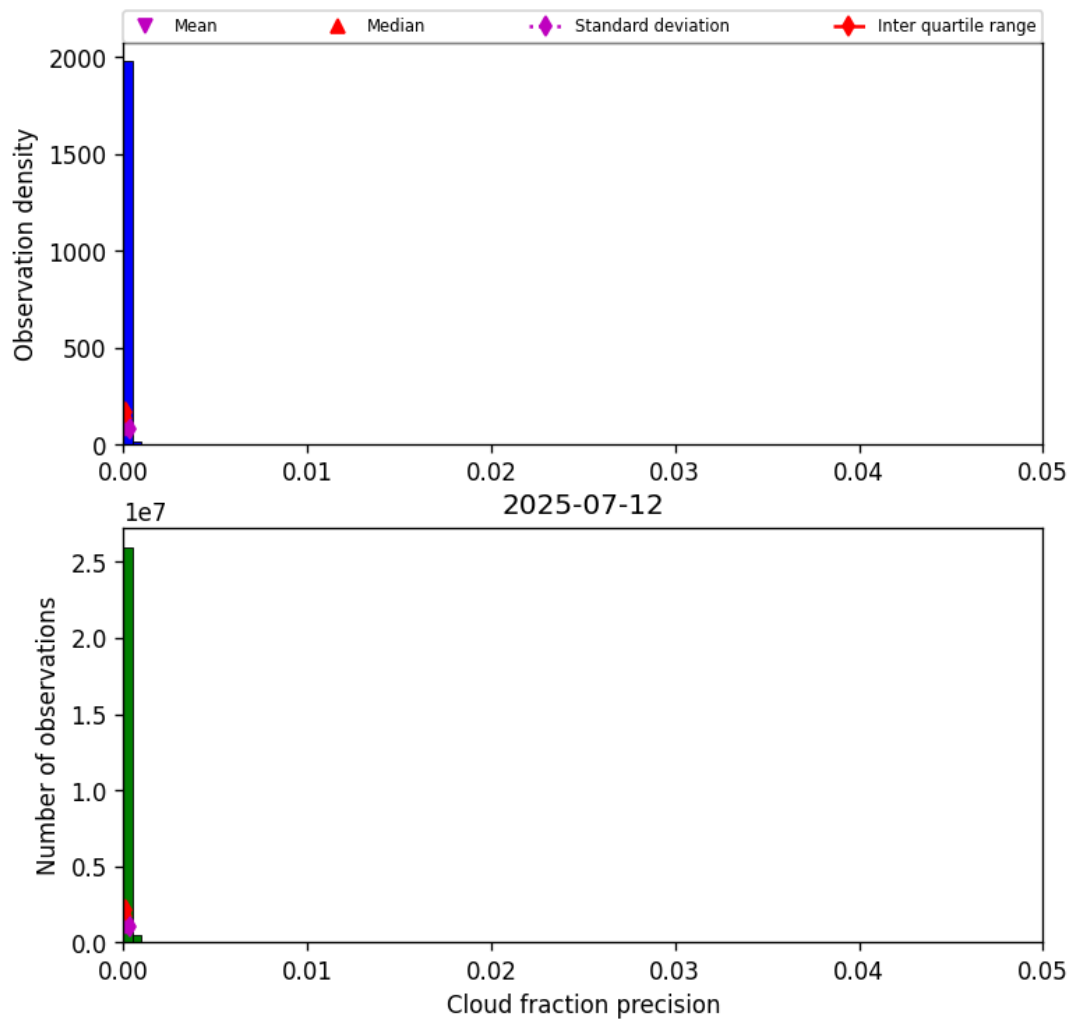
Figure 33: Histogram of “Cloud fraction precision” for 2025-07-11 to 2025-07-13
