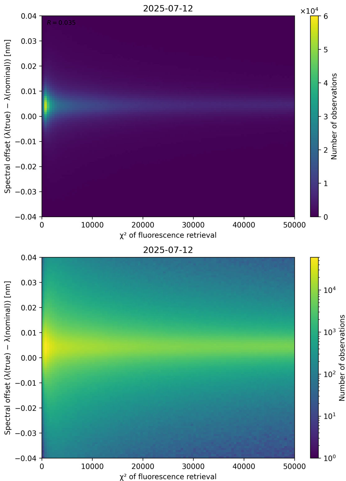
Figure 69: Scatter density plot of “ \chi^2 of fluorescence retrieval” against “Spectral offset ( \lambda_{\text{true}} - \lambda_{\text{nominal}} )” for 2025-07-11 to 2025-07-13.
