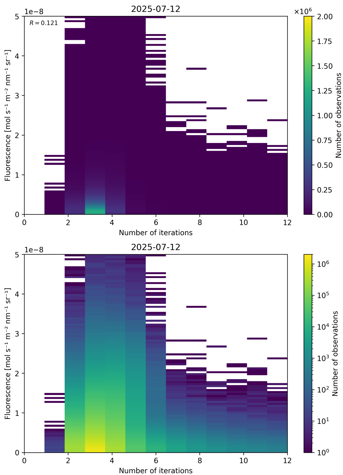
Figure 98: Scatter density plot of “Number of iterations” against “Fluorescence” for 2025-07-11 to 2025-07-13.
