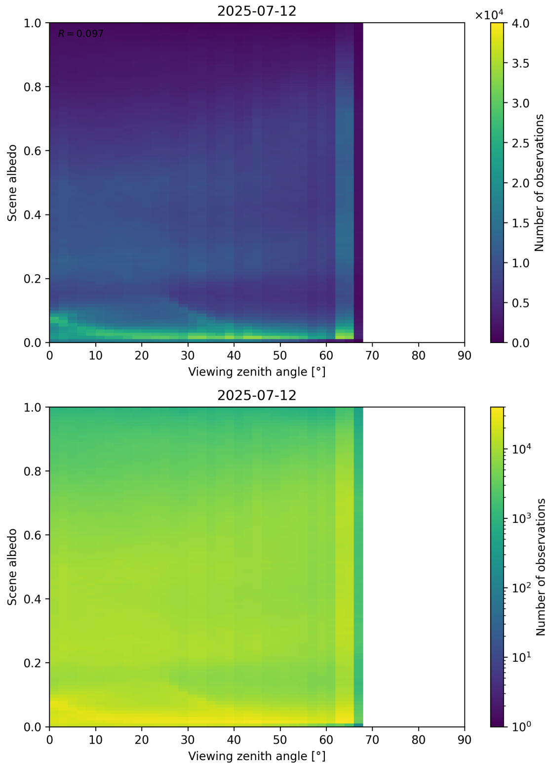
Figure 126: Scatter density plot of “Viewing zenith angle” against “Scene albedo” for 2025-07-11 to 2025-07-13.
