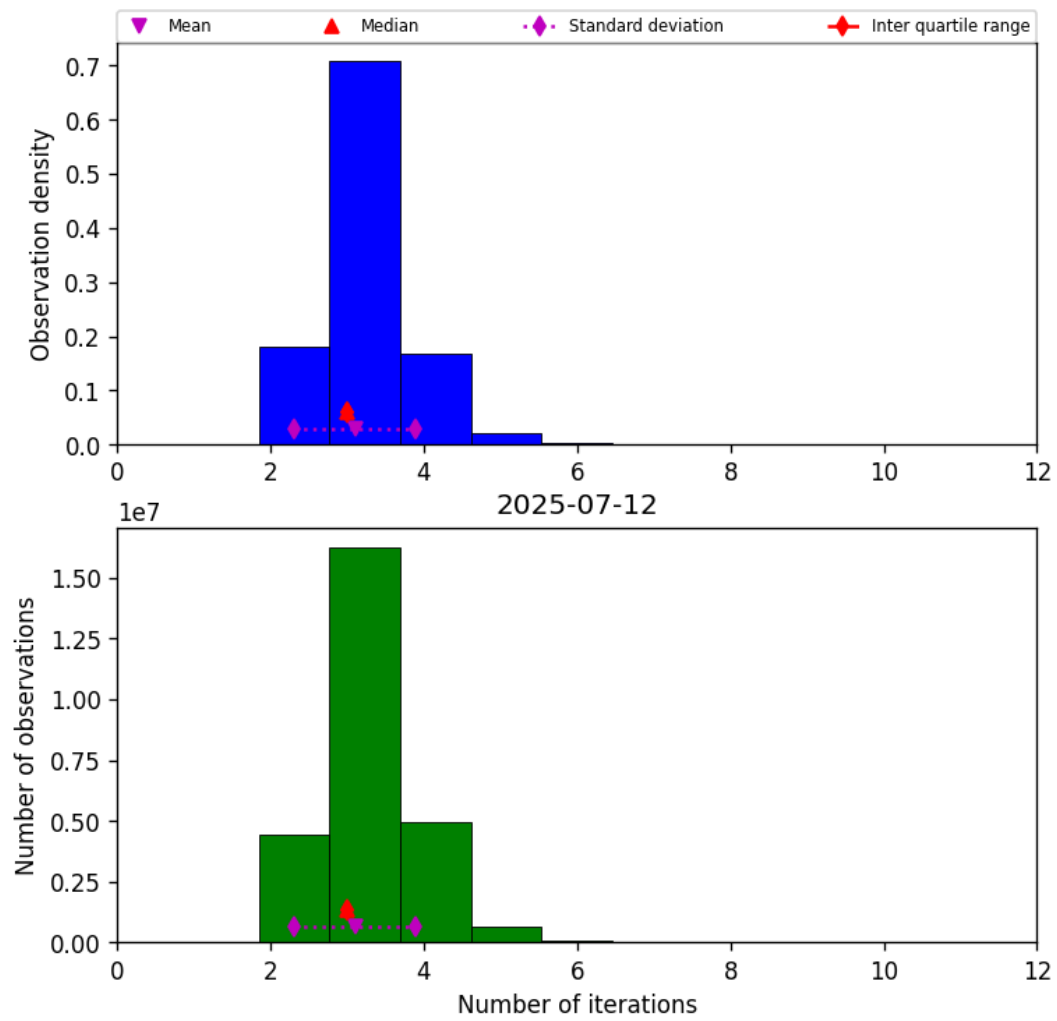
Figure 39: Histogram of “Number of iterations” for 2025-07-11 to 2025-07-13
