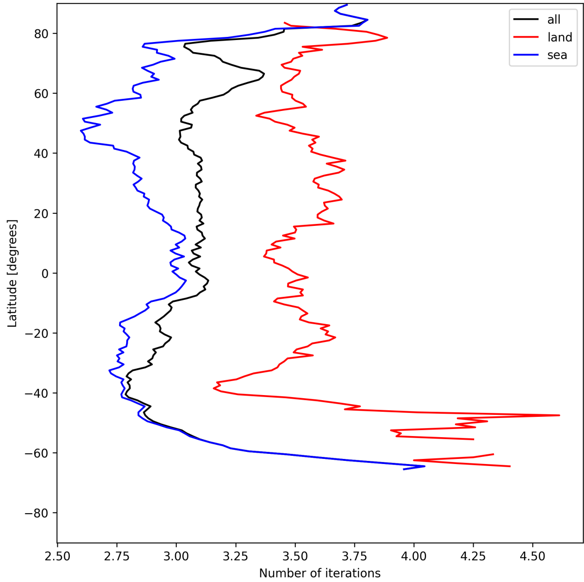
Figure 22: Zonal average of “Number of iterations” for 2025-07-11 to 2025-07-13.
