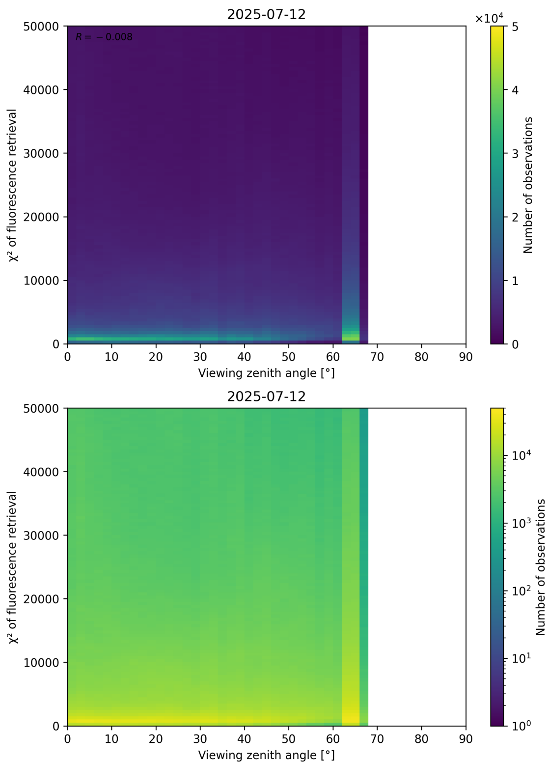
Figure 119: Scatter density plot of “Viewing zenith angle” against “ \chi^2 of fluorescence retrieval” for 2025-07-11 to 2025-07-13.
