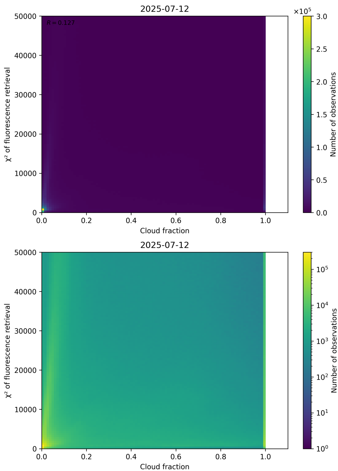
Figure 71: Scatter density plot of “Cloud fraction” against “ \chi^2 of fluorescence retrieval” for 2025-07-11 to 2025-07-13.
