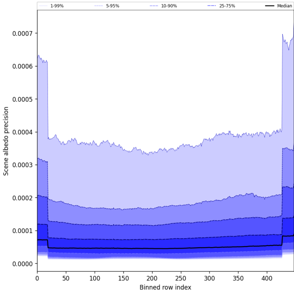
Figure 52: Along track statistics of “Scene albedo precision” for 2025-07-11 to 2025-07-13
