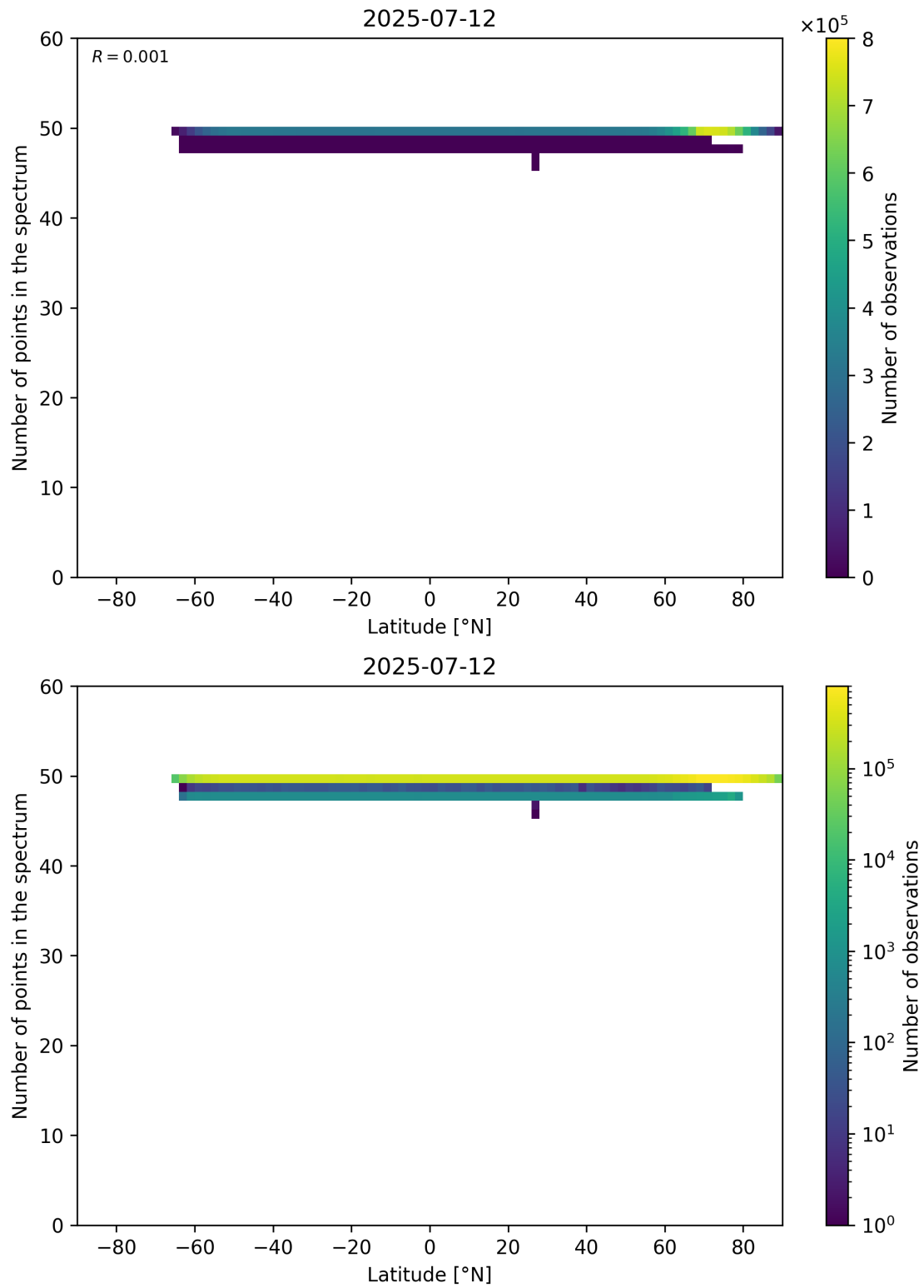
Figure 94: Scatter density plot of “Latitude” against “Number of points in the spectrum” for 2025-07-11 to 2025-07-13.
