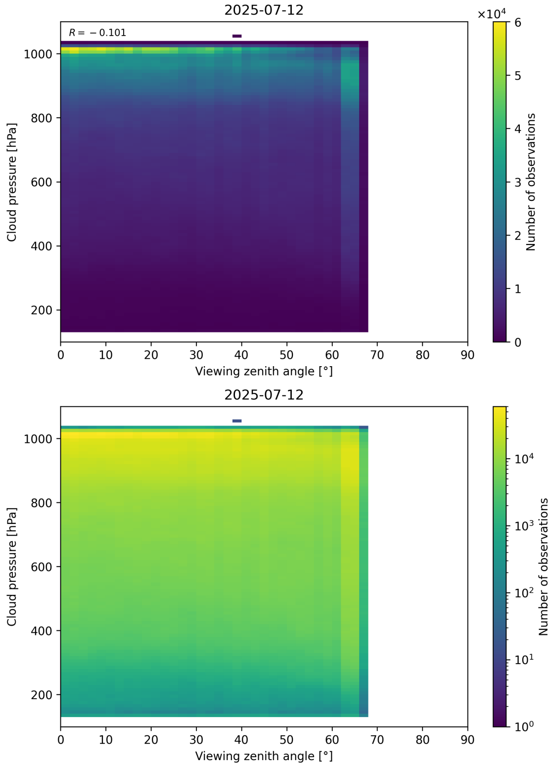
Figure 121: Scatter density plot of “Viewing zenith angle” against “Cloud pressure” for 2025-07-11 to 2025-07-13.
