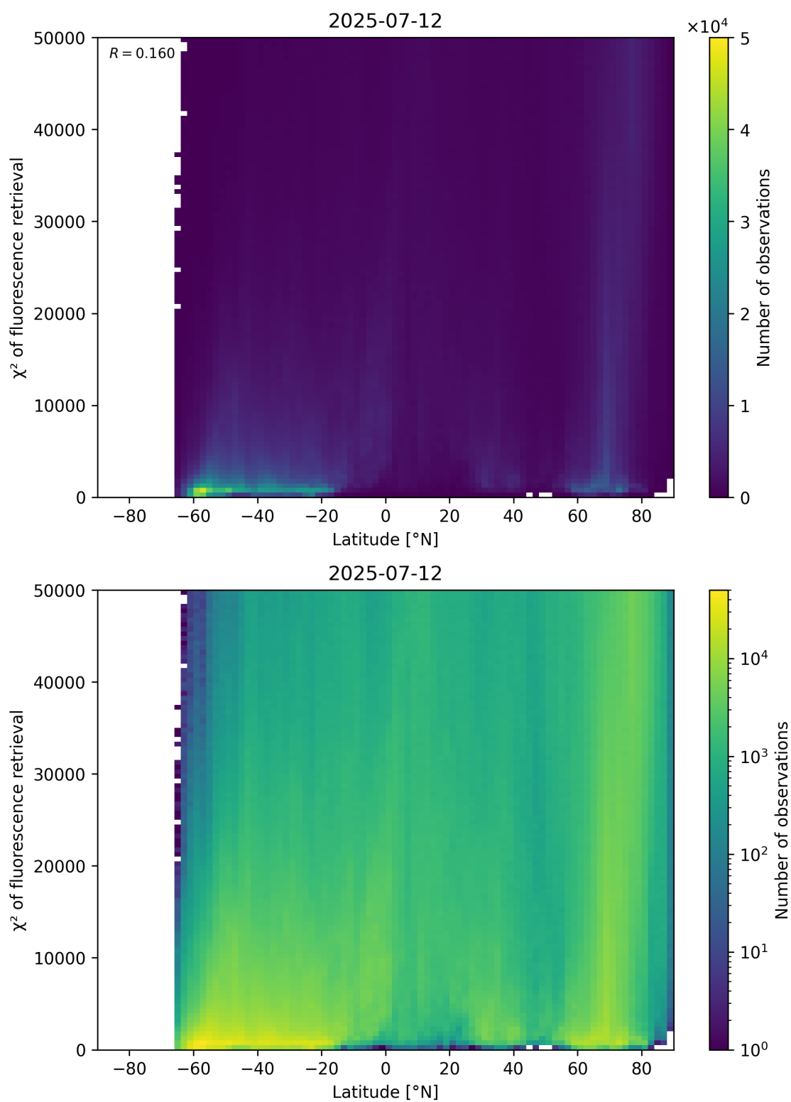
Figure 89: Scatter density plot of “Latitude” against “ \chi^2 of fluorescence retrieval” for 2025-07-11 to 2025-07-13.
