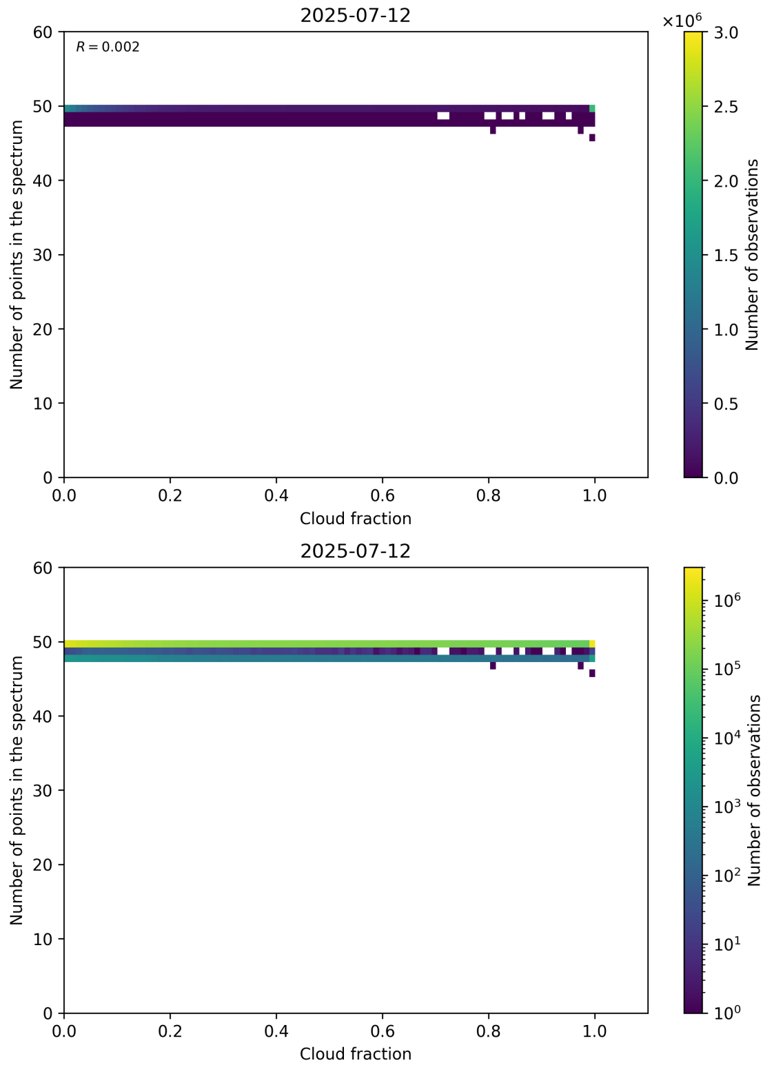
Figure 74: Scatter density plot of “Cloud fraction” against “Number of points in the spectrum” for 2025-07-11 to 2025-07-13.
