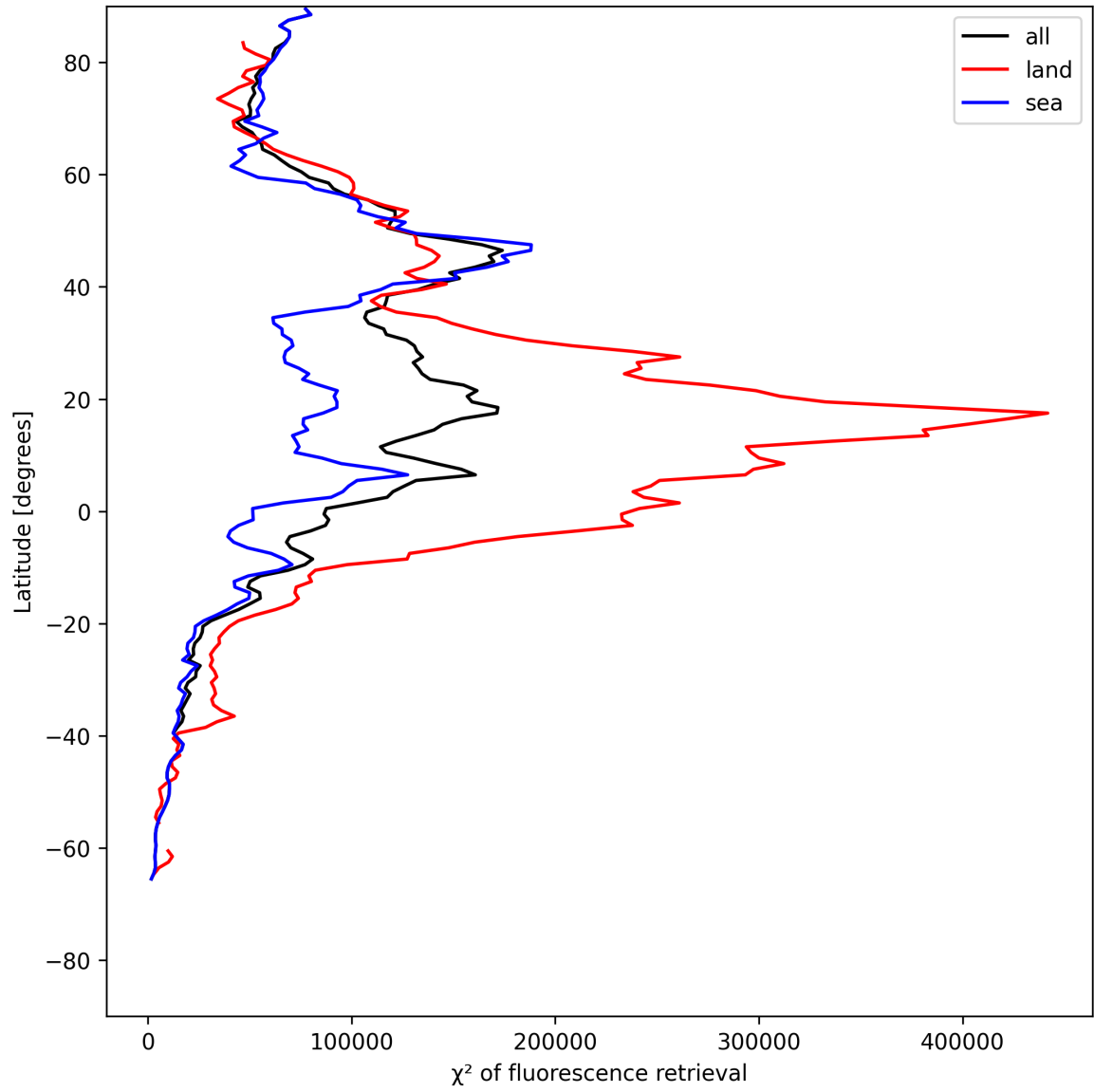
Figure 25: Zonal average of “ \chi^2 of fluorescence retrieval” for 2025-07-11 to 2025-07-13.
