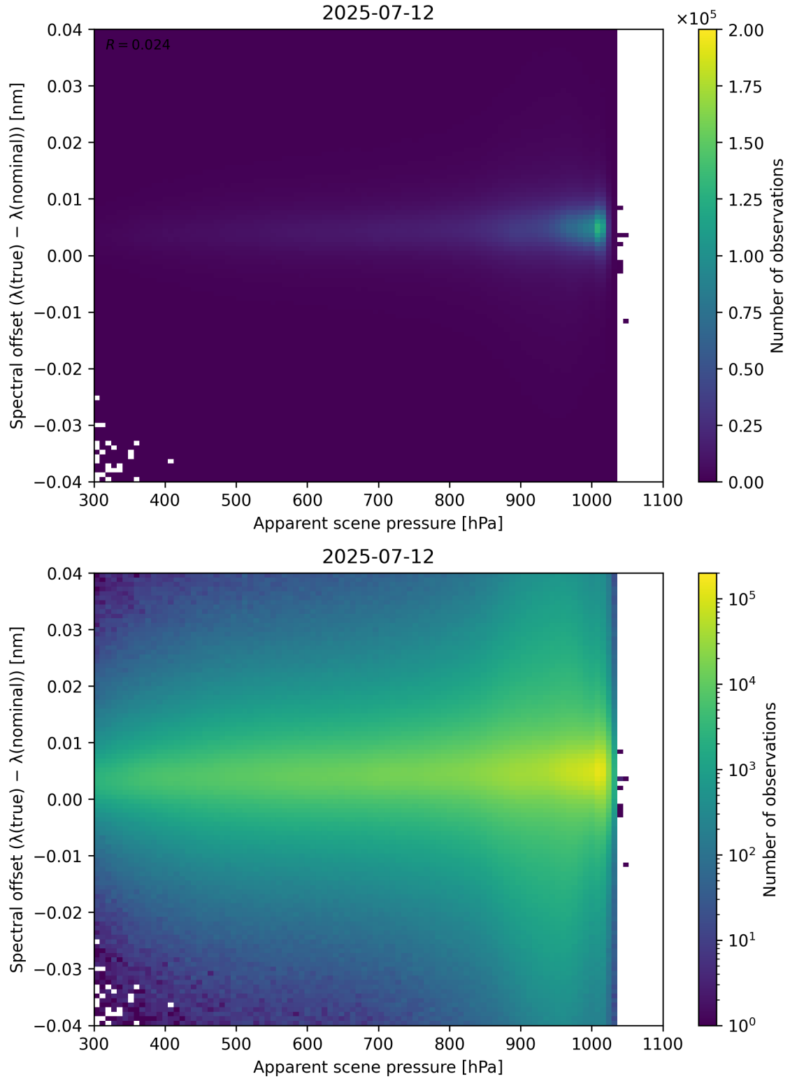
Figure 67: Scatter density plot of “Apparent scene pressure” against “Spectral offset ( \lambda_{\text{true}} - \lambda_{\text{nominal}} )” for 2025-07-11 to 2025-07-13.
