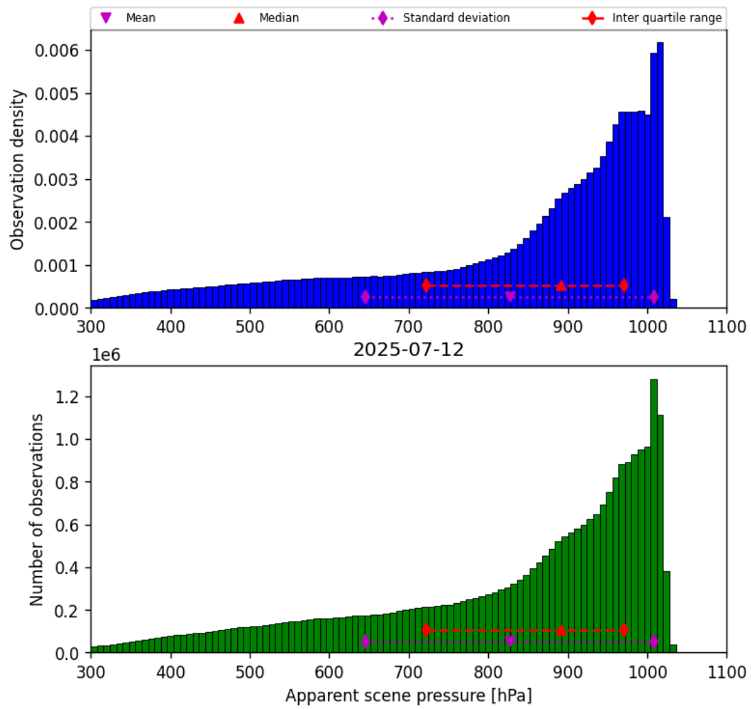
Figure 36: Histogram of “Apparent scene pressure” for 2025-07-11 to 2025-07-13
