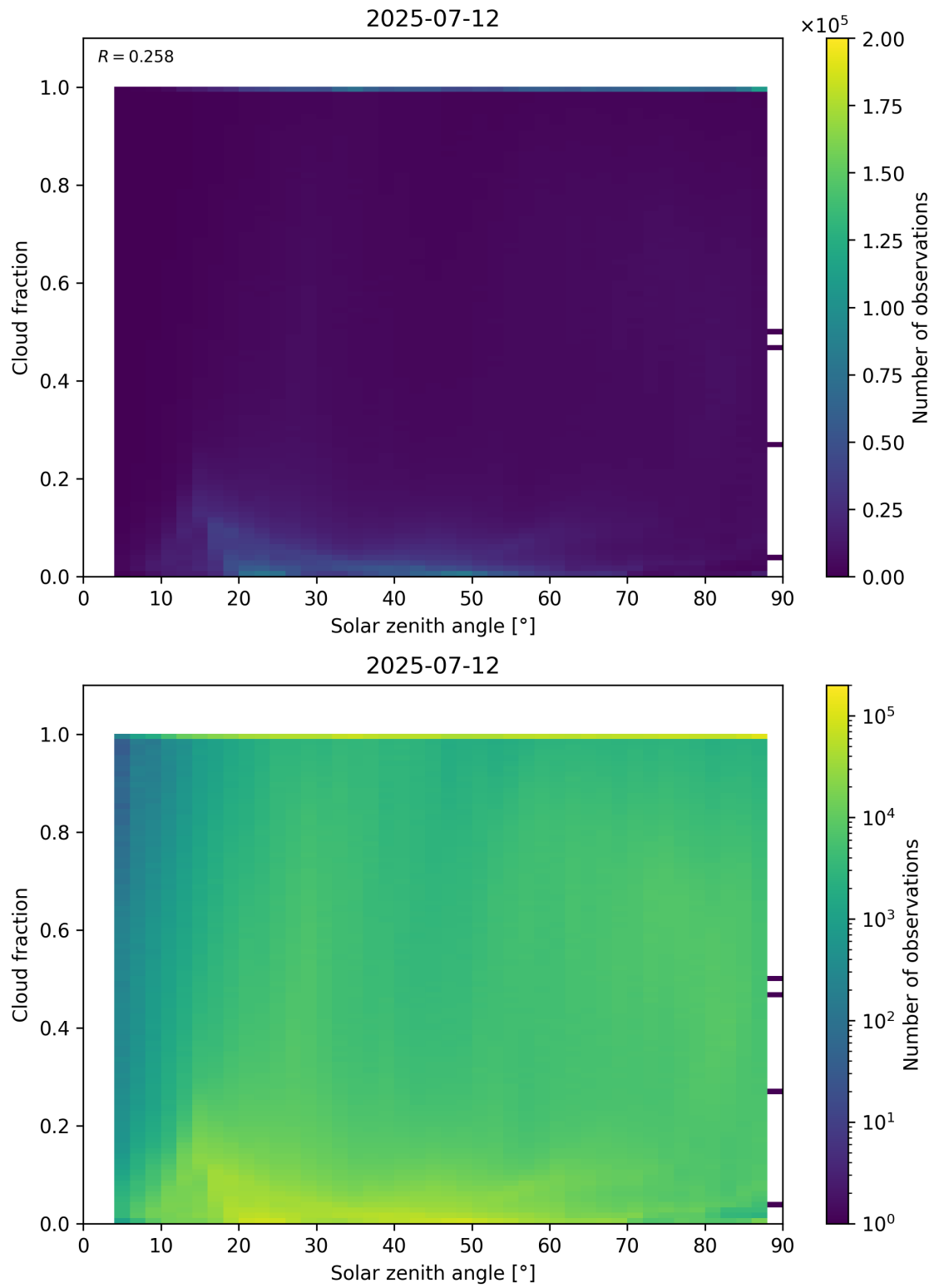
Figure 110: Scatter density plot of “Solar zenith angle” against “Cloud fraction” for 2025-07-11 to 2025-07-13.
