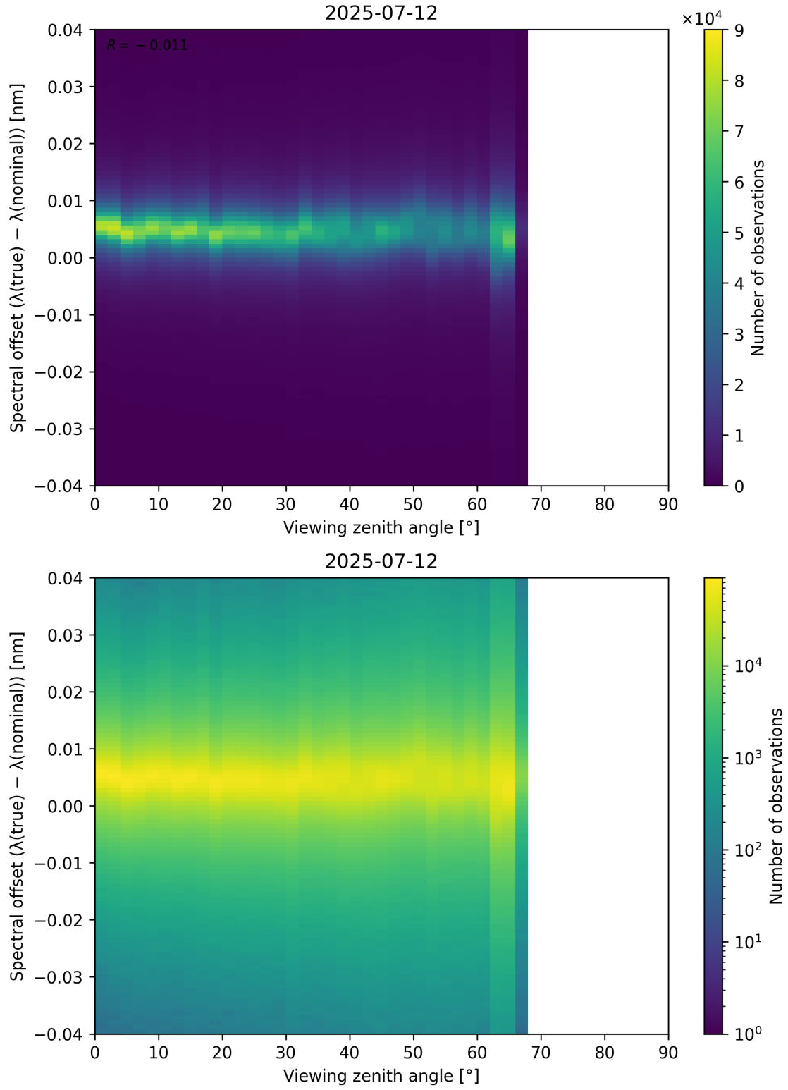
Figure 128: Scatter density plot of “Viewing zenith angle” against “Spectral offset ( \lambda_{\text{true}} - \lambda_{\text{nominal}} )” for 2025-07-11 to 2025-07-13.
