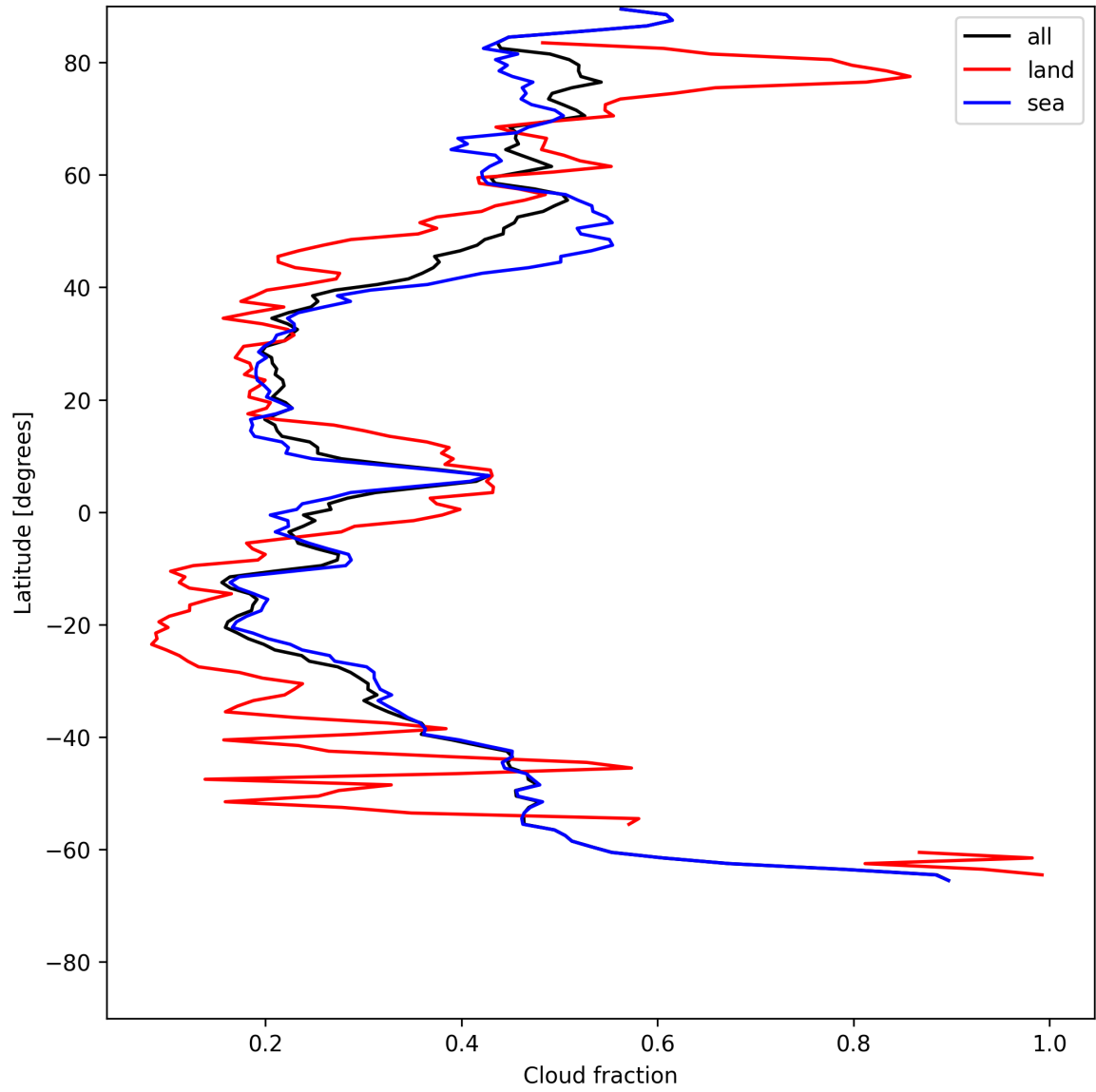
Figure 15: Zonal average of “Cloud fraction” for 2025-07-11 to 2025-07-13.
