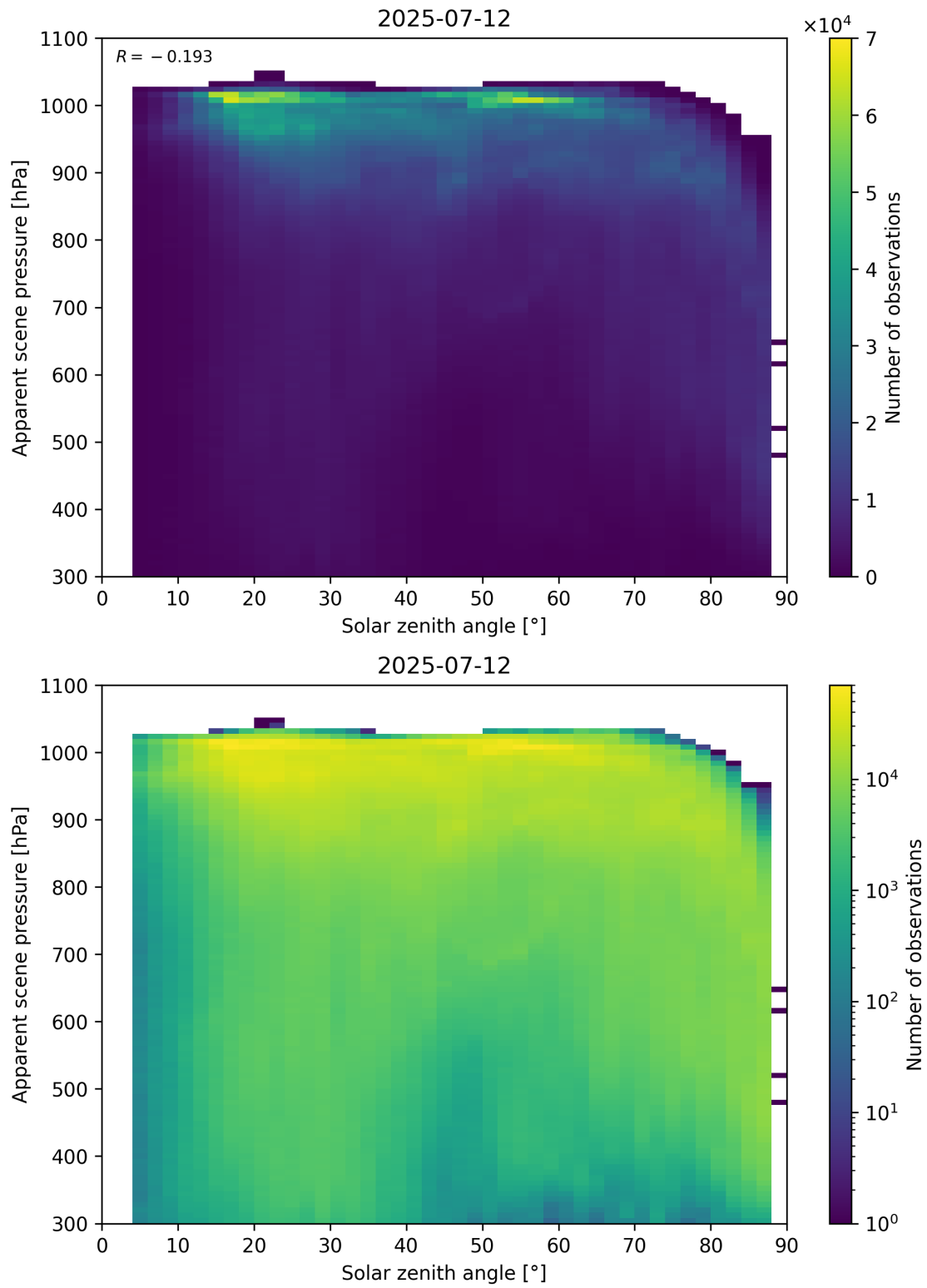
Figure 108: Scatter density plot of “Solar zenith angle” against “Apparent scene pressure” for 2025-07-11 to 2025-07-13.
