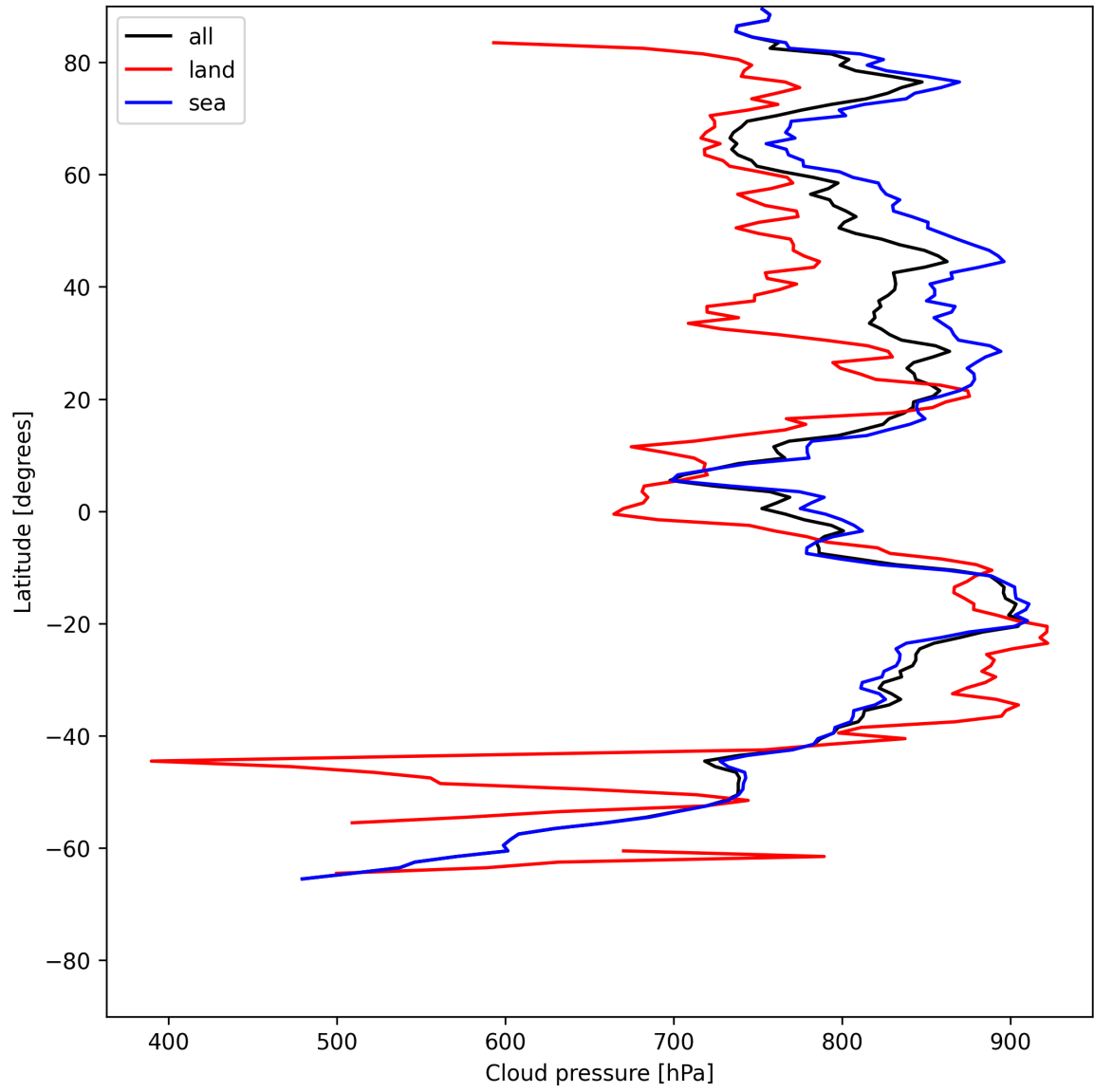
Figure 13: Zonal average of “Cloud pressure” for 2025-07-11 to 2025-07-13.
