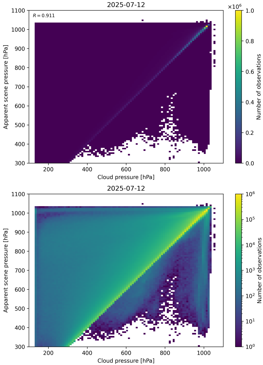
Figure 77: Scatter density plot of “Cloud pressure” against “Apparent scene pressure” for 2025-07-11 to 2025-07-13.
