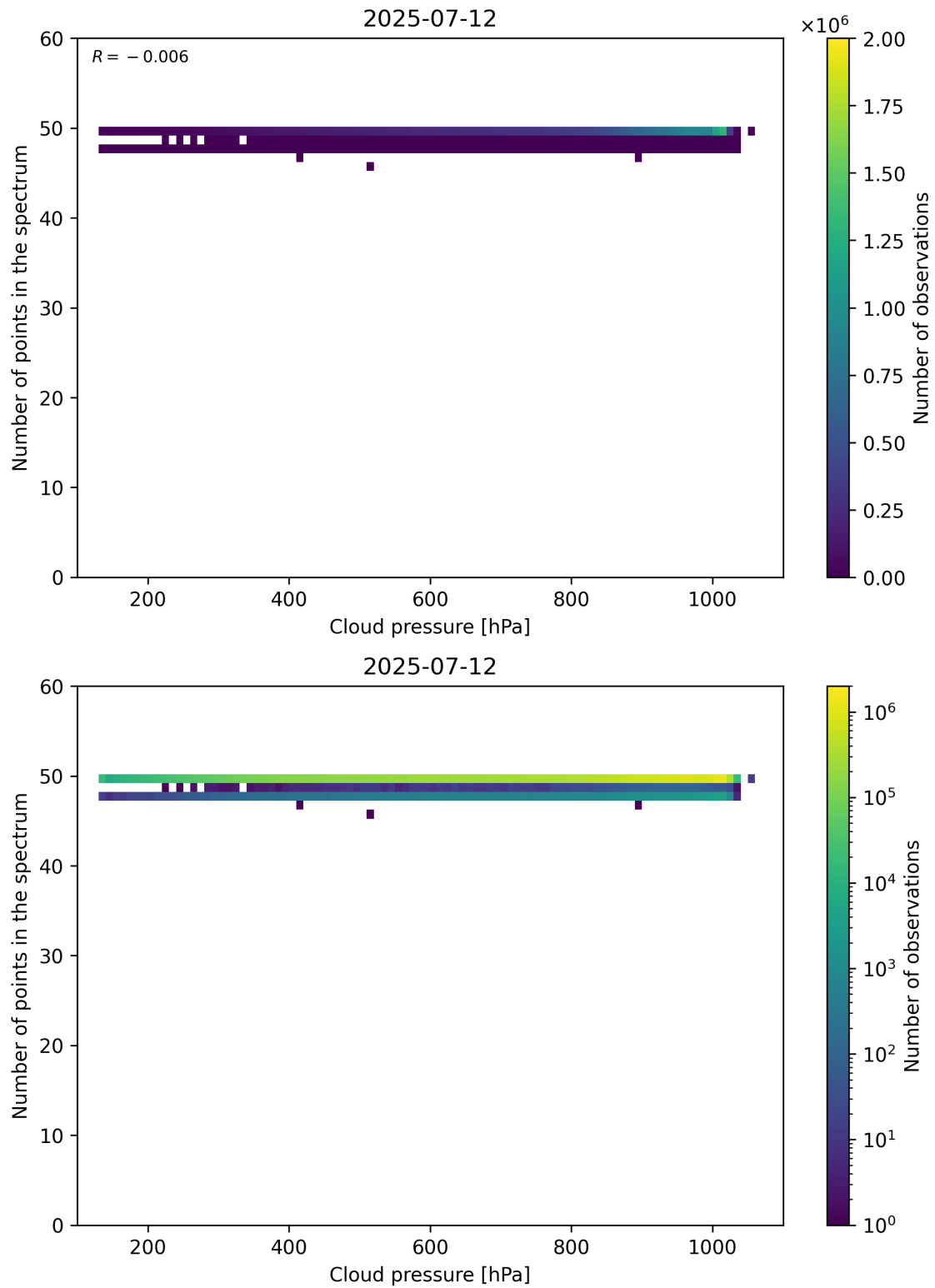
Figure 82: Scatter density plot of “Cloud pressure” against “Number of points in the spectrum” for 2025-07-11 to 2025-07-13.
