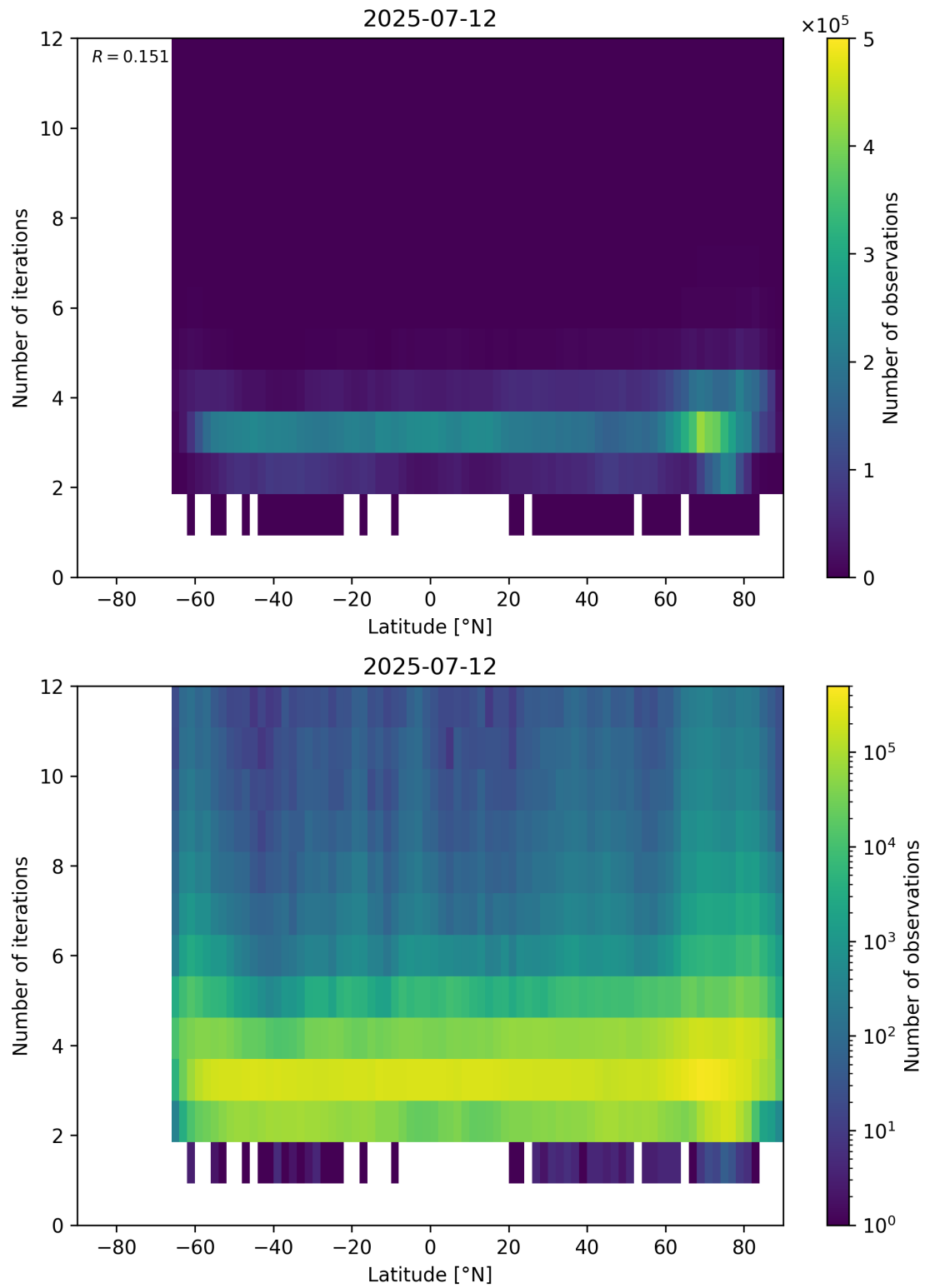
Figure 93: Scatter density plot of “Latitude” against “Number of iterations” for 2025-07-11 to 2025-07-13.
