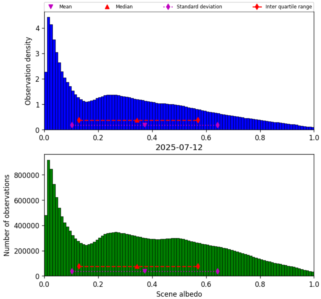
Figure 34: Histogram of “Scene albedo” for 2025-07-11 to 2025-07-13
