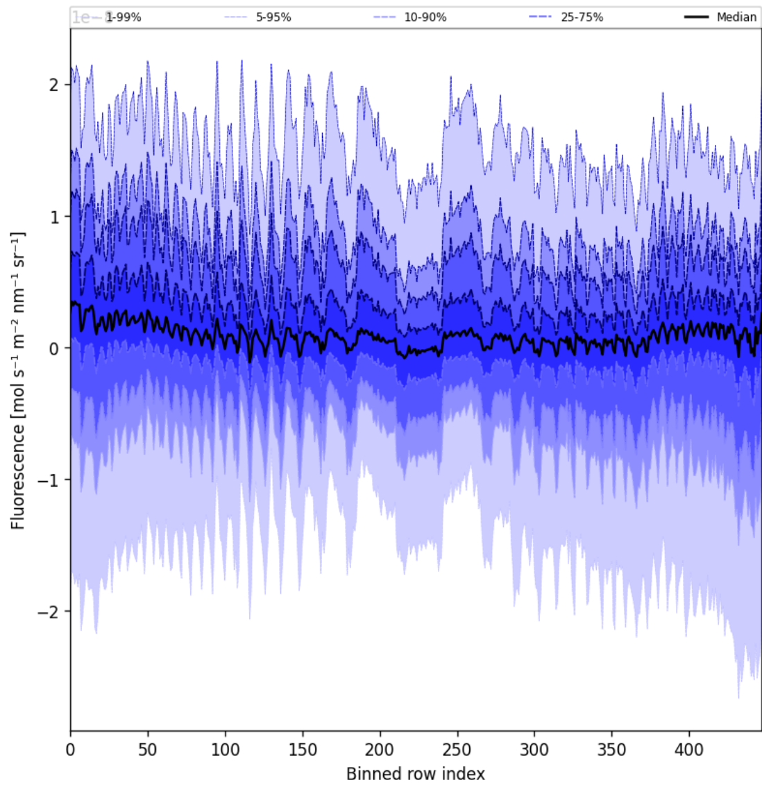
Figure 57: Along track statistics of “Fluorescence” for 2025-07-11 to 2025-07-13
