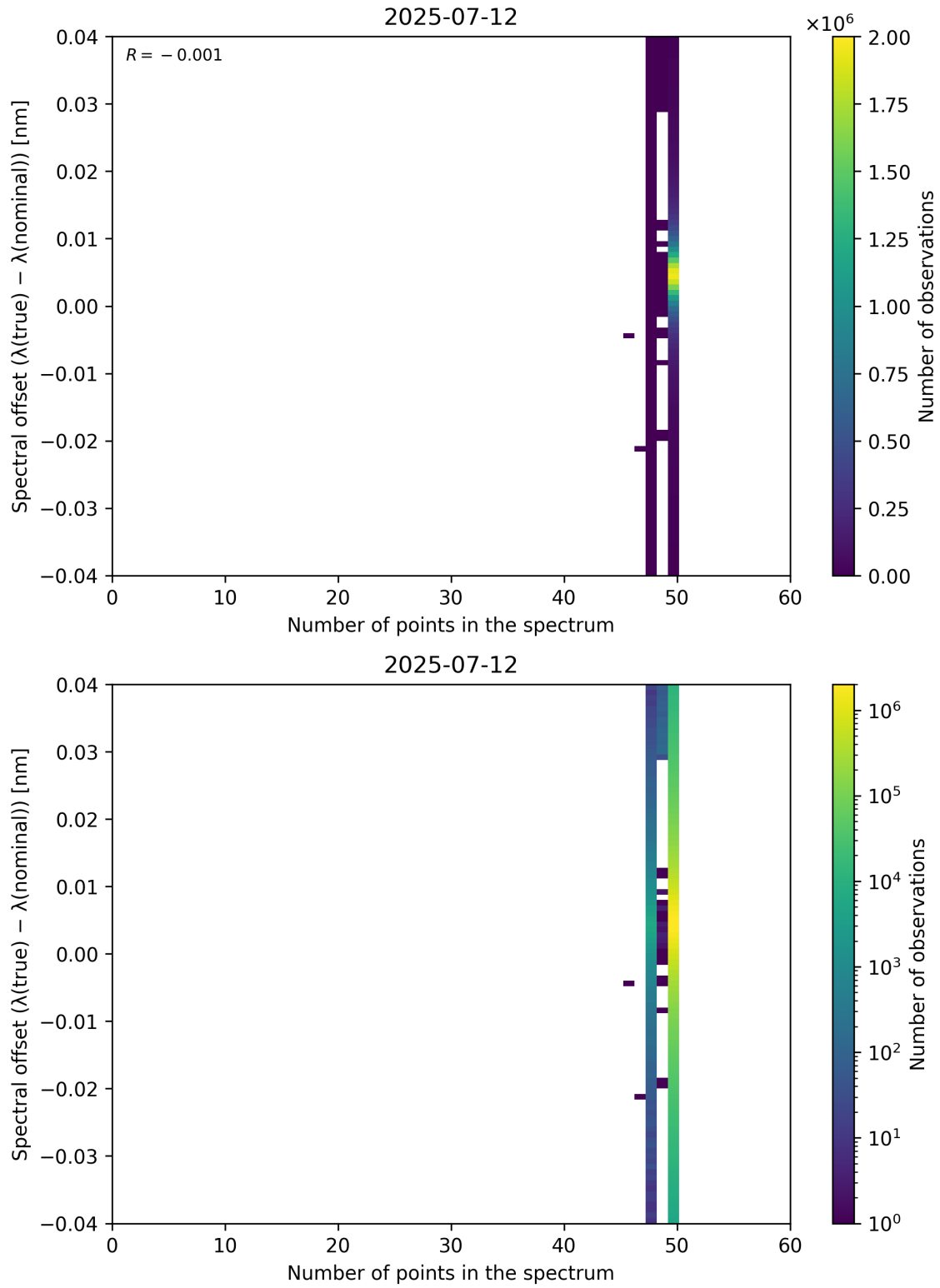
Figure 101: Scatter density plot of “Number of points in the spectrum” against “Spectral offset ( \lambda_{\text{true}} - \lambda_{\text{nominal}} )” for 2025-07-11 to 2025-07-13.
