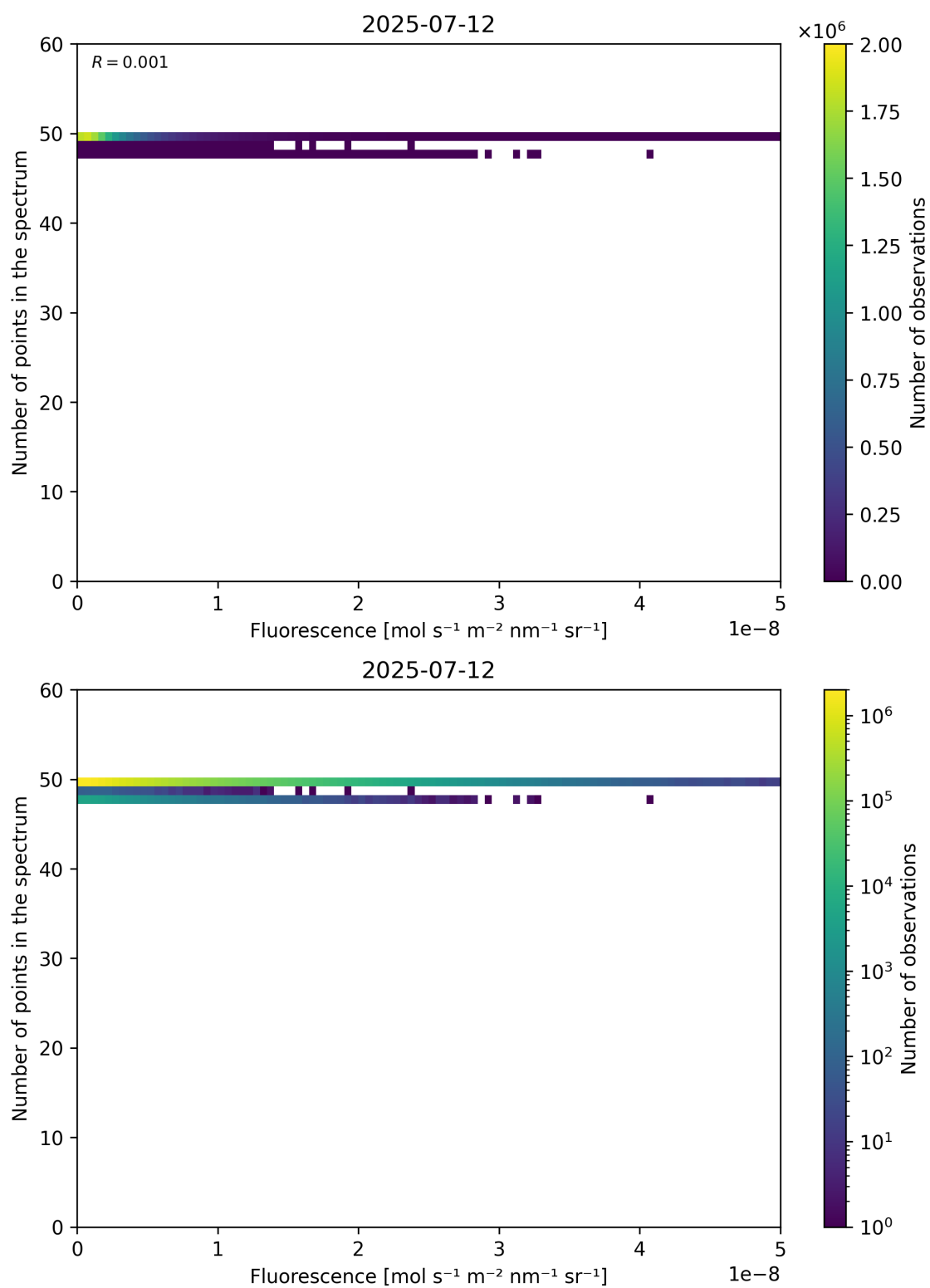
Figure 86: Scatter density plot of “Fluorescence” against “Number of points in the spectrum” for 2025-07-11 to 2025-07-13.
