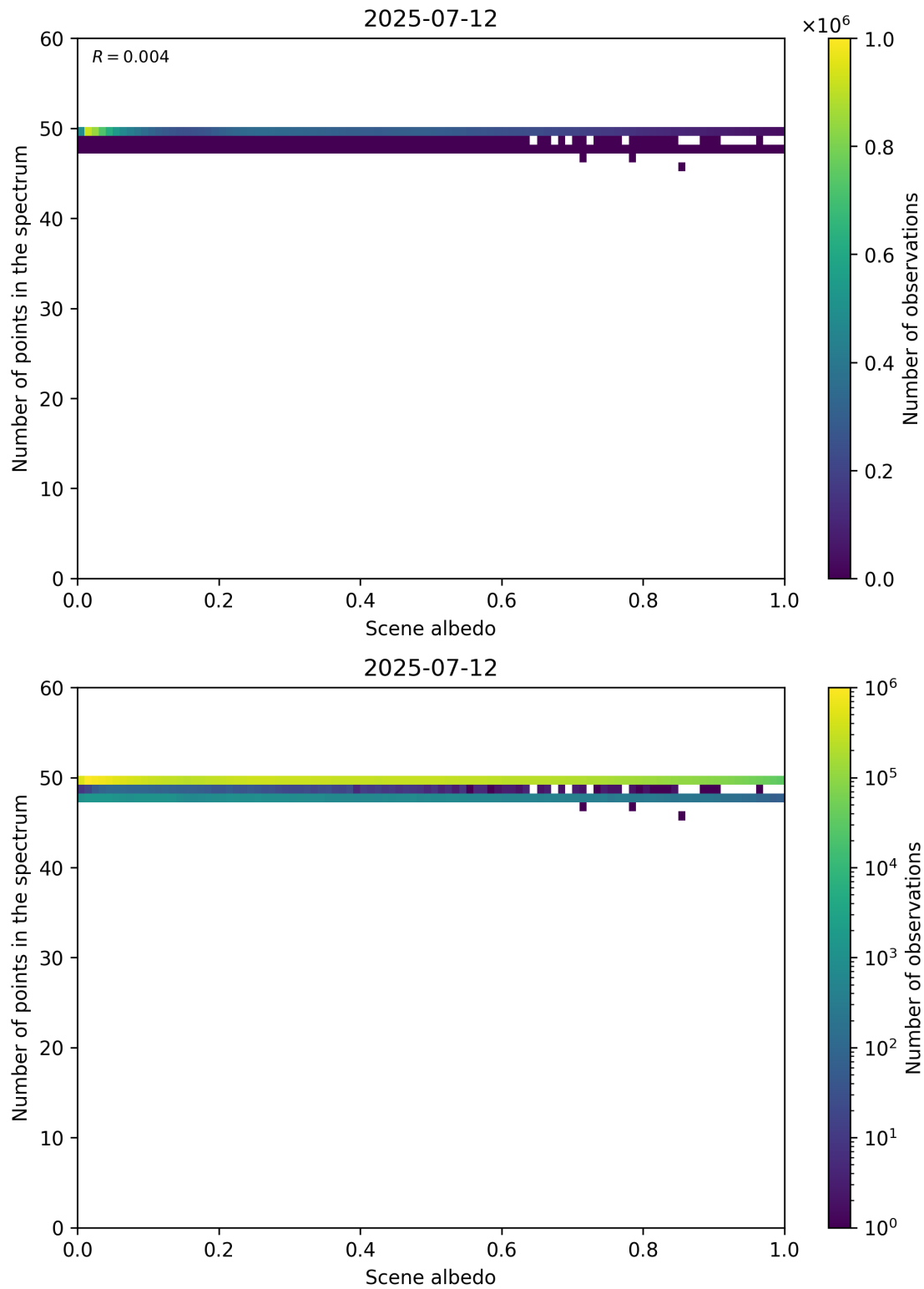
Figure 106: Scatter density plot of “Scene albedo” against “Number of points in the spectrum” for 2025-07-11 to 2025-07-13.
