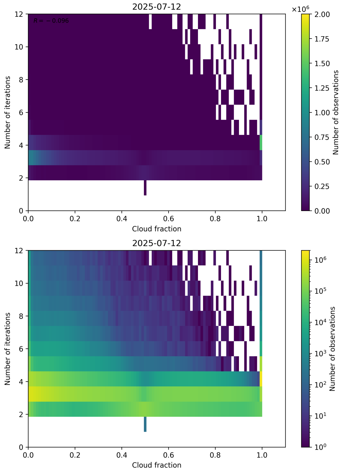
Figure 73: Scatter density plot of “Cloud fraction” against “Number of iterations” for 2025-07-11 to 2025-07-13.
