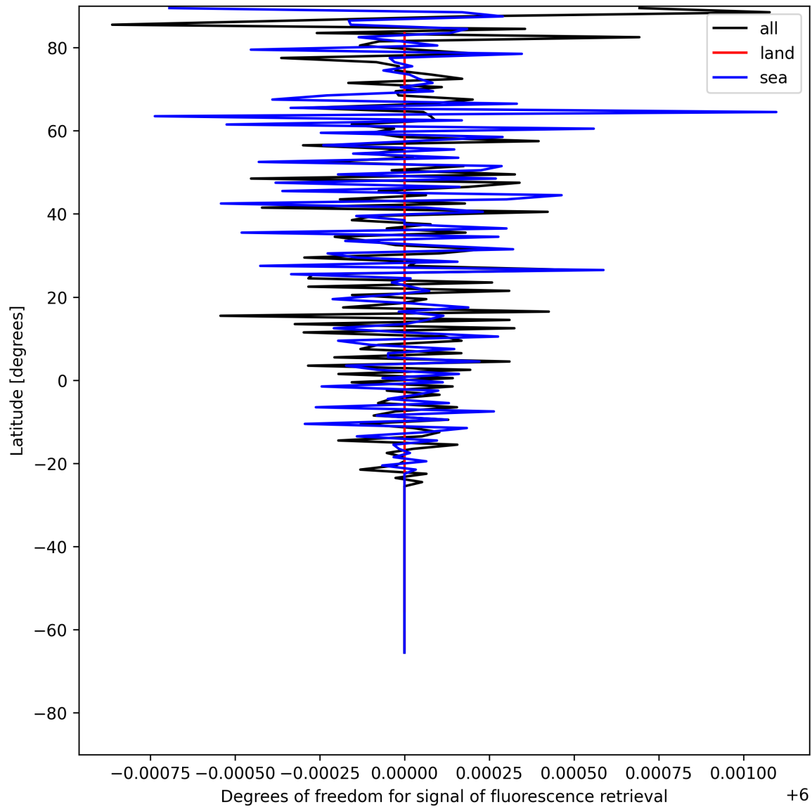
Figure 26: Zonal average of “Degrees of freedom for signal of fluorescence retrieval” for 2025-07-11 to 2025-07-13.
