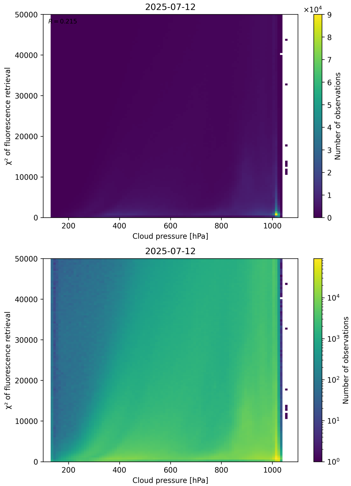
Figure 78: Scatter density plot of “Cloud pressure” against “ \chi^2 of fluorescence retrieval” for 2025-07-11 to 2025-07-13.
