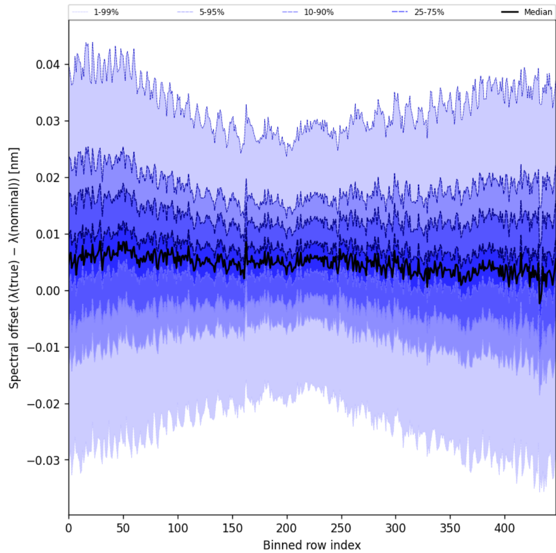
Figure 62: Along track statistics of “Spectral offset ( \lambda_{\text{true}} - \lambda_{\text{nominal}} )” for 2025-07-11 to 2025-07-13
