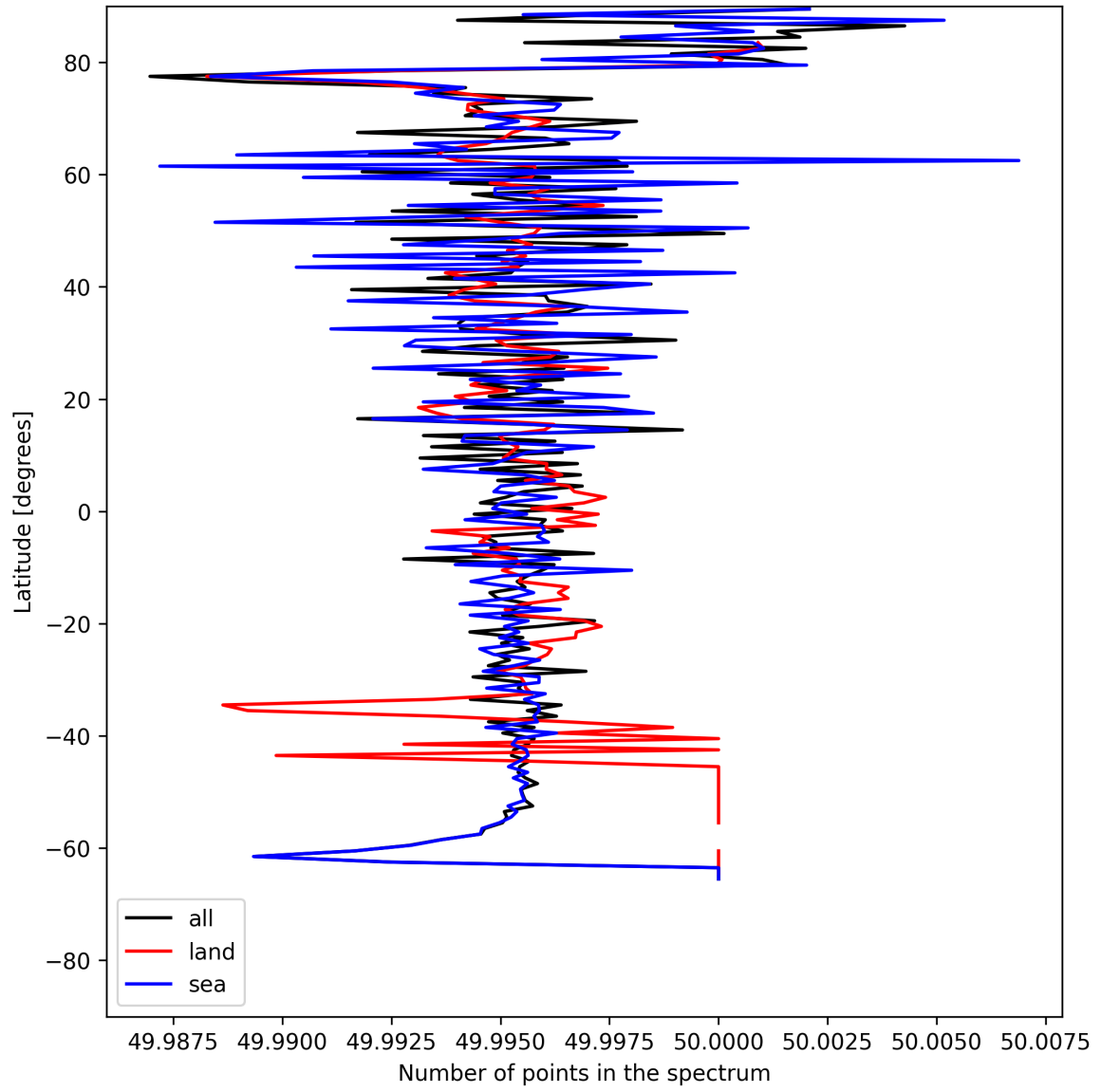
Figure 27: Zonal average of “Number of points in the spectrum” for 2025-07-11 to 2025-07-13.
