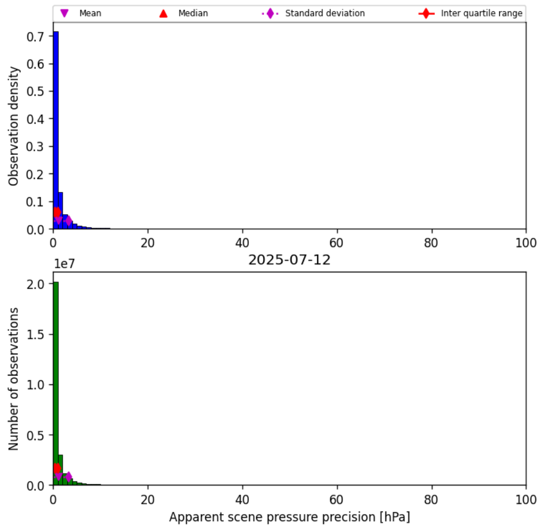
Figure 37: Histogram of “Apparent scene pressure precision” for 2025-07-11 to 2025-07-13
