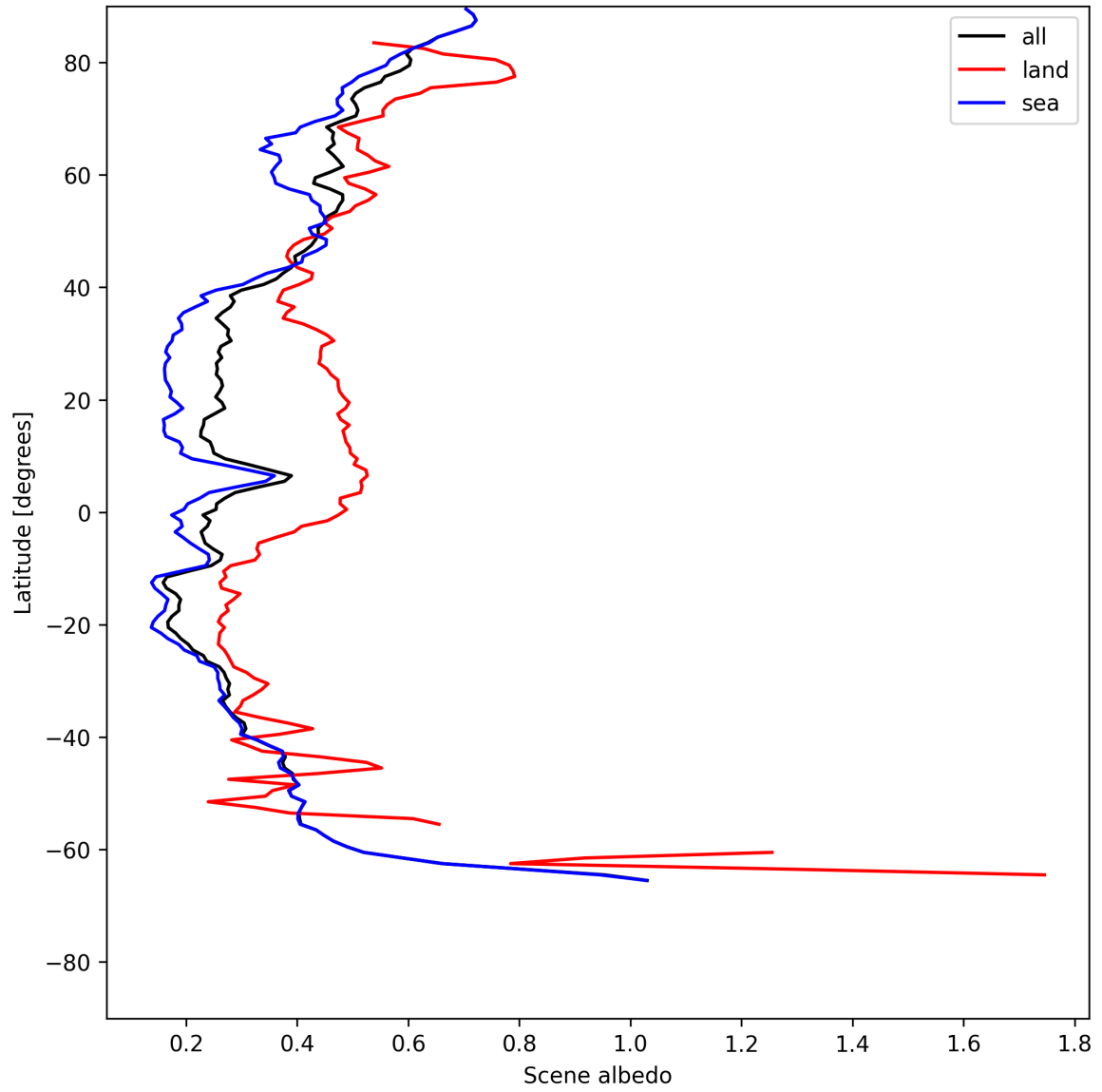
Figure 17: Zonal average of “Scene albedo” for 2025-07-11 to 2025-07-13.
