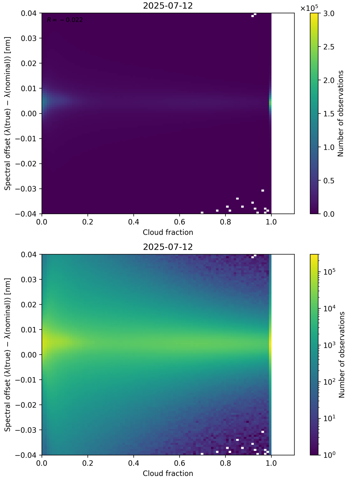
Figure 76: Scatter density plot of “Cloud fraction” against “Spectral offset ( \lambda_{\text{true}} - \lambda_{\text{nominal}} )” for 2025-07-11 to 2025-07-13.
