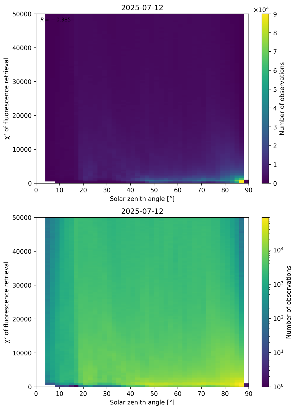
Figure 109: Scatter density plot of “Solar zenith angle” against “ \chi^2 of fluorescence retrieval” for 2025-07-11 to 2025-07-13.
