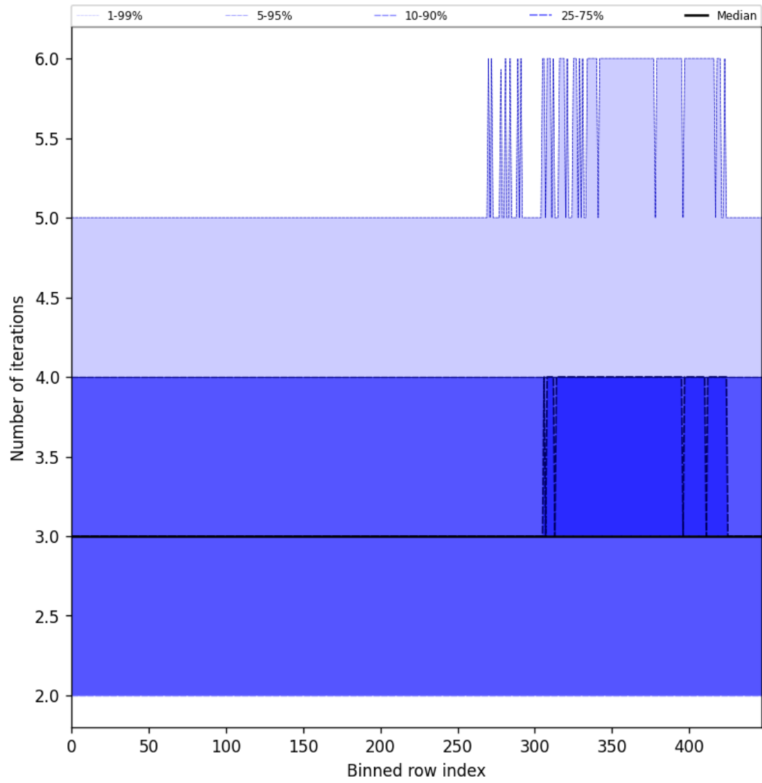
Figure 56: Along track statistics of “Number of iterations” for 2025-07-11 to 2025-07-13
