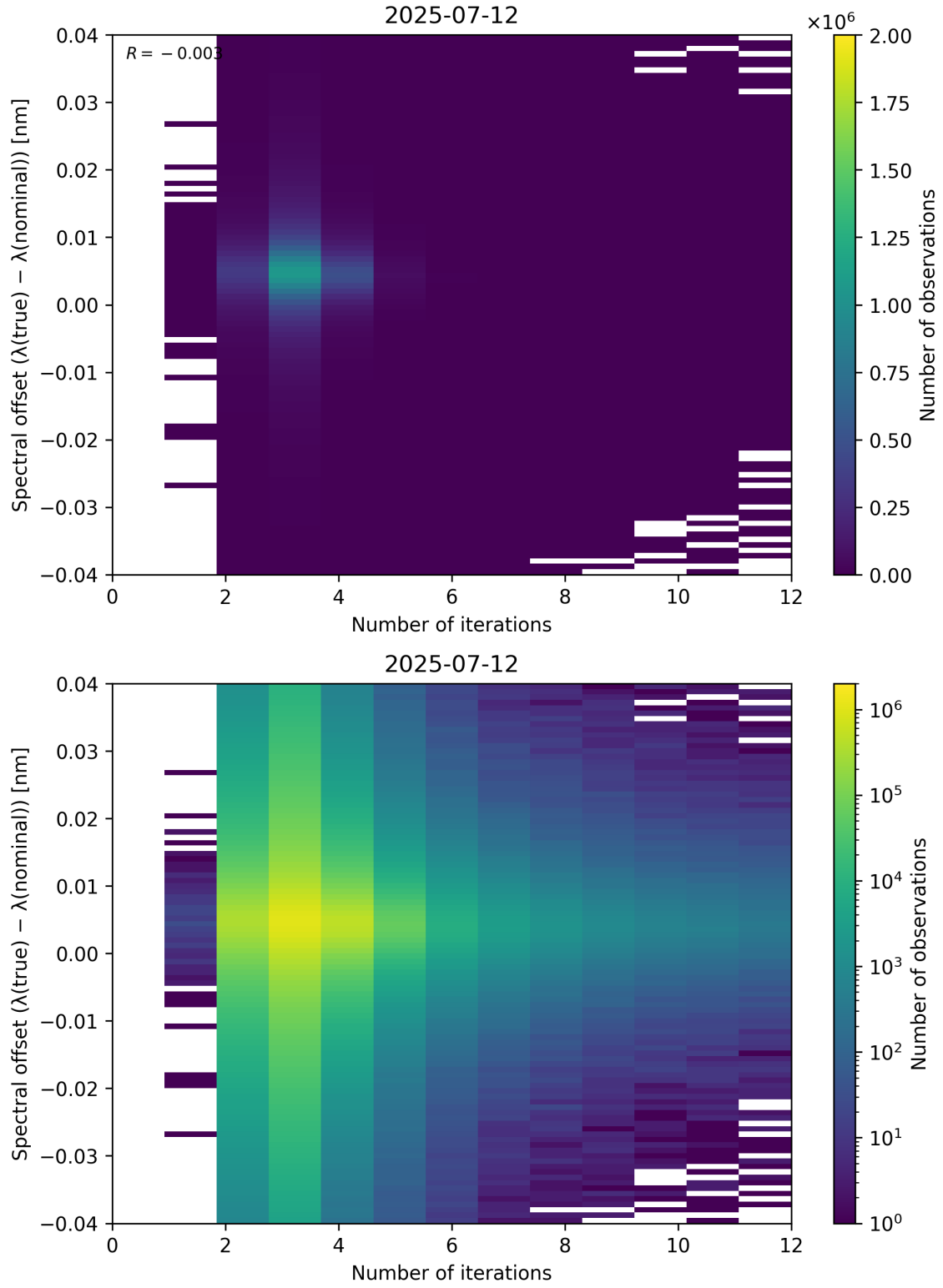
Figure 100: Scatter density plot of “Number of iterations” against “Spectral offset ( \lambda_{\text{true}} - \lambda_{\text{nominal}} )” for 2025-07-11 to 2025-07-13.
