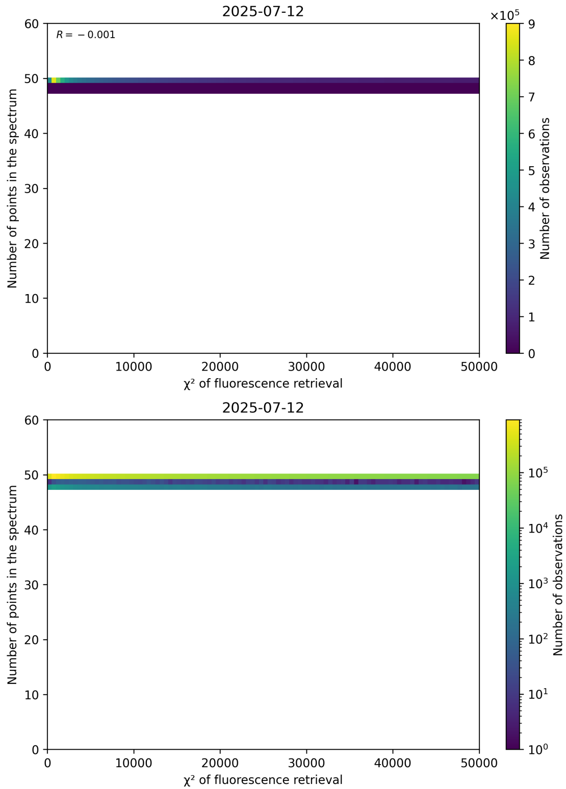
Figure 68: Scatter density plot of “ \chi^2 of fluorescence retrieval” against “Number of points in the spectrum” for 2025-07-11 to 2025-07-13.
