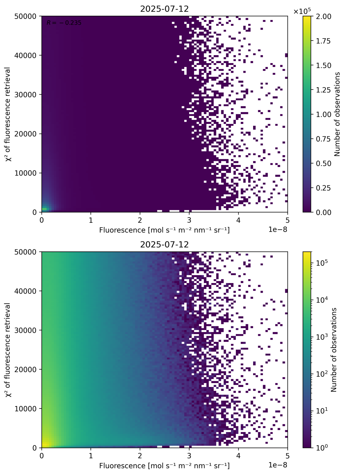
Figure 85: Scatter density plot of “Fluorescence” against “ \chi^2 of fluorescence retrieval” for 2025-07-11 to 2025-07-13.
