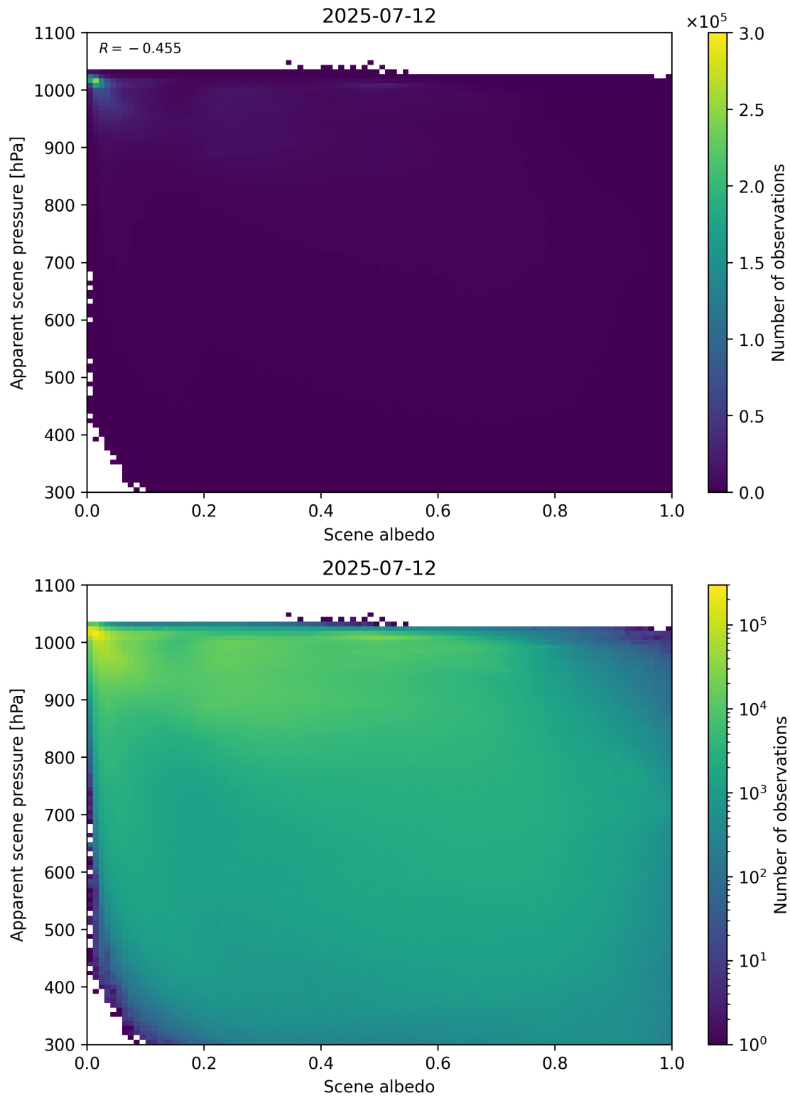
Figure 102: Scatter density plot of “Scene albedo” against “Apparent scene pressure” for 2025-07-11 to 2025-07-13.
