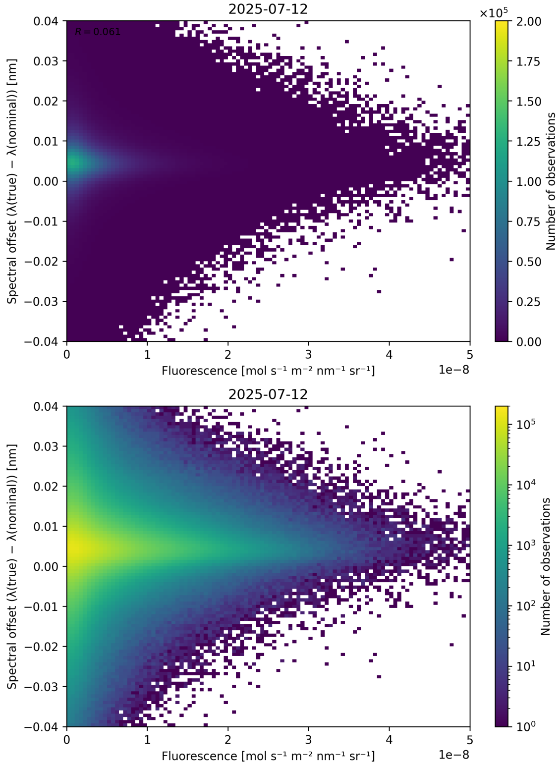
Figure 87: Scatter density plot of “Fluorescence” against “Spectral offset ( \lambda_{\text{true}} - \lambda_{\text{nominal}} )” for 2025-07-11 to 2025-07-13.
