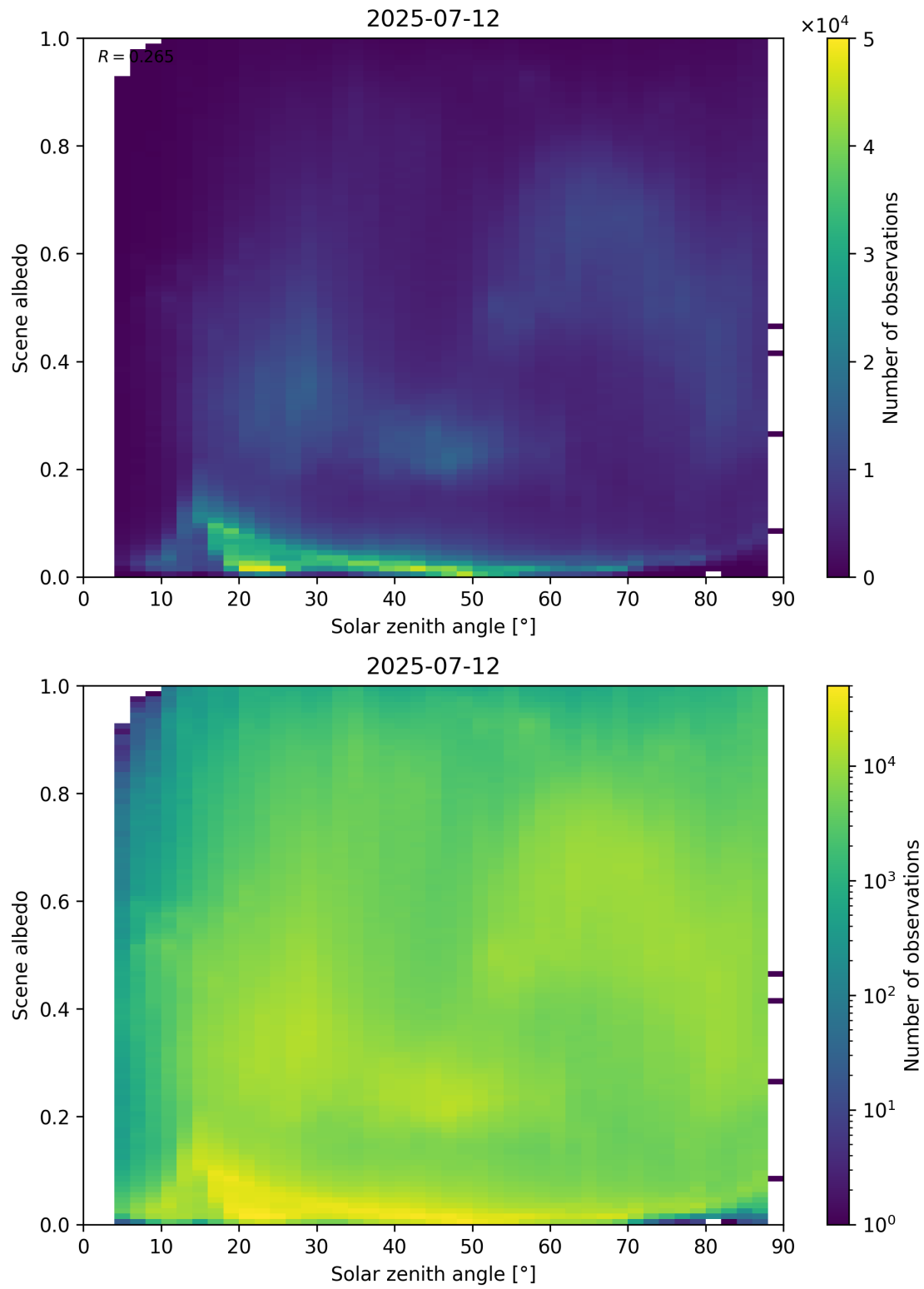
Figure 116: Scatter density plot of “Solar zenith angle” against “Scene albedo” for 2025-07-11 to 2025-07-13.
