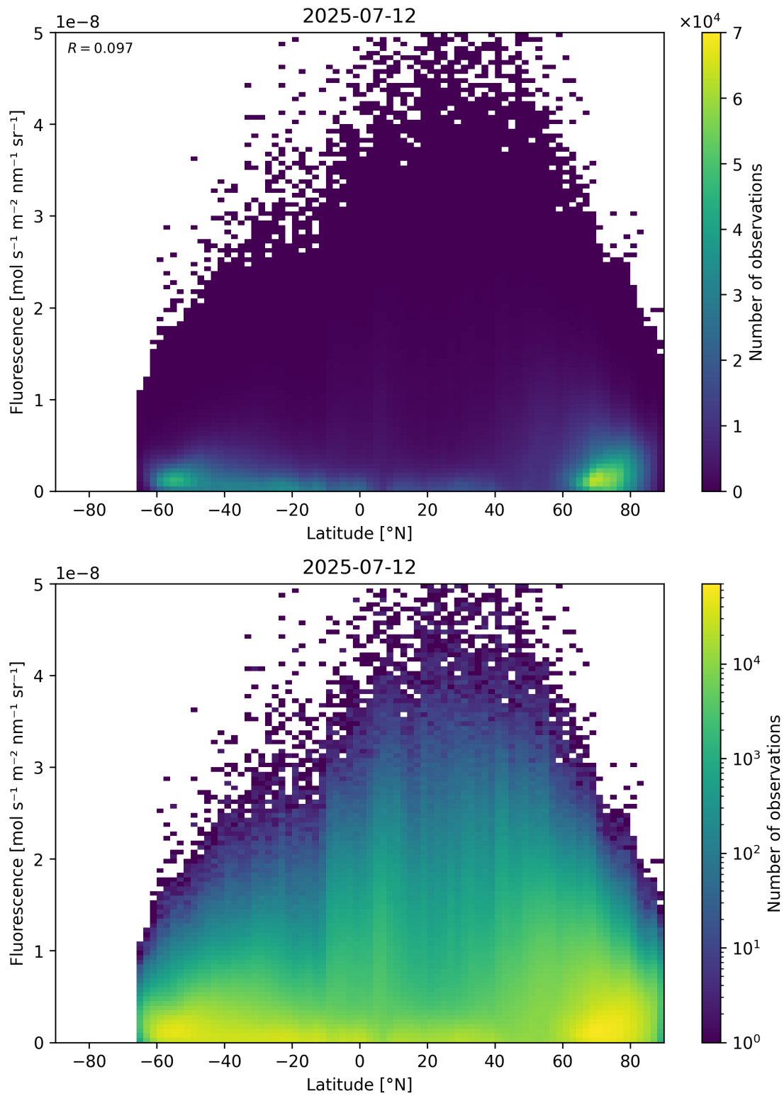
Figure 92: Scatter density plot of “Latitude” against “Fluorescence” for 2025-07-11 to 2025-07-13.
