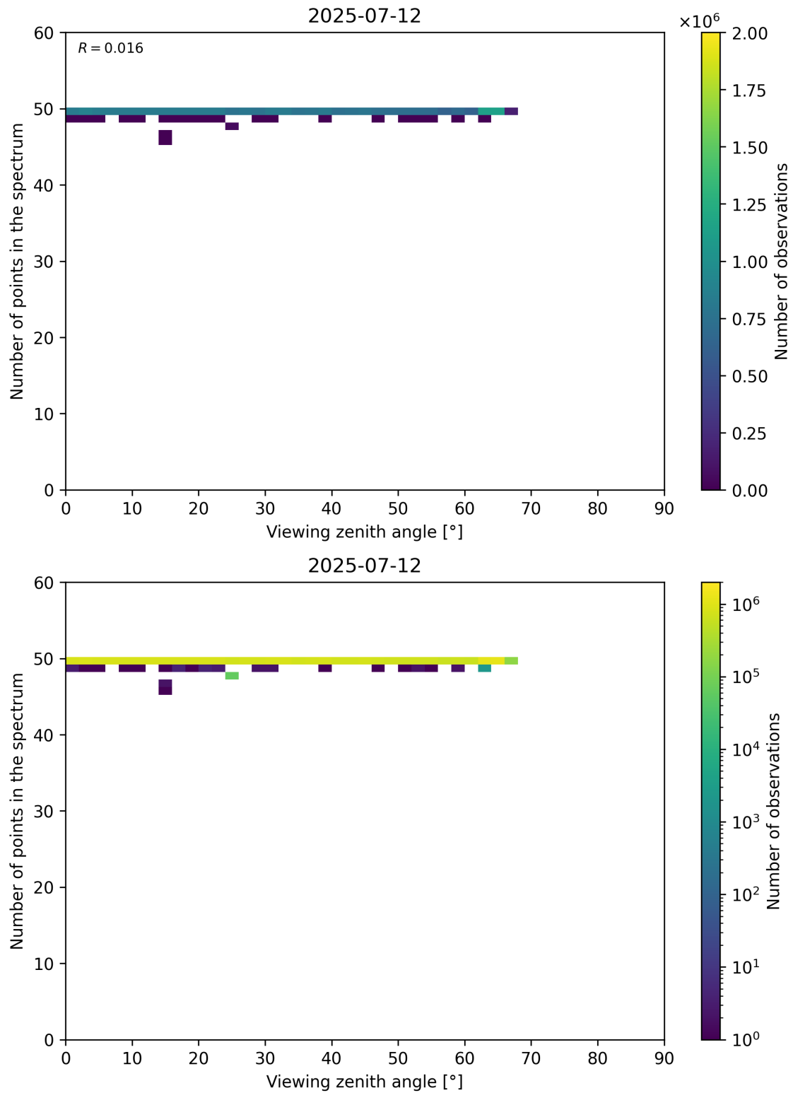
Figure 125: Scatter density plot of “Viewing zenith angle” against “Number of points in the spectrum” for 2025-07-11 to 2025-07-13.
