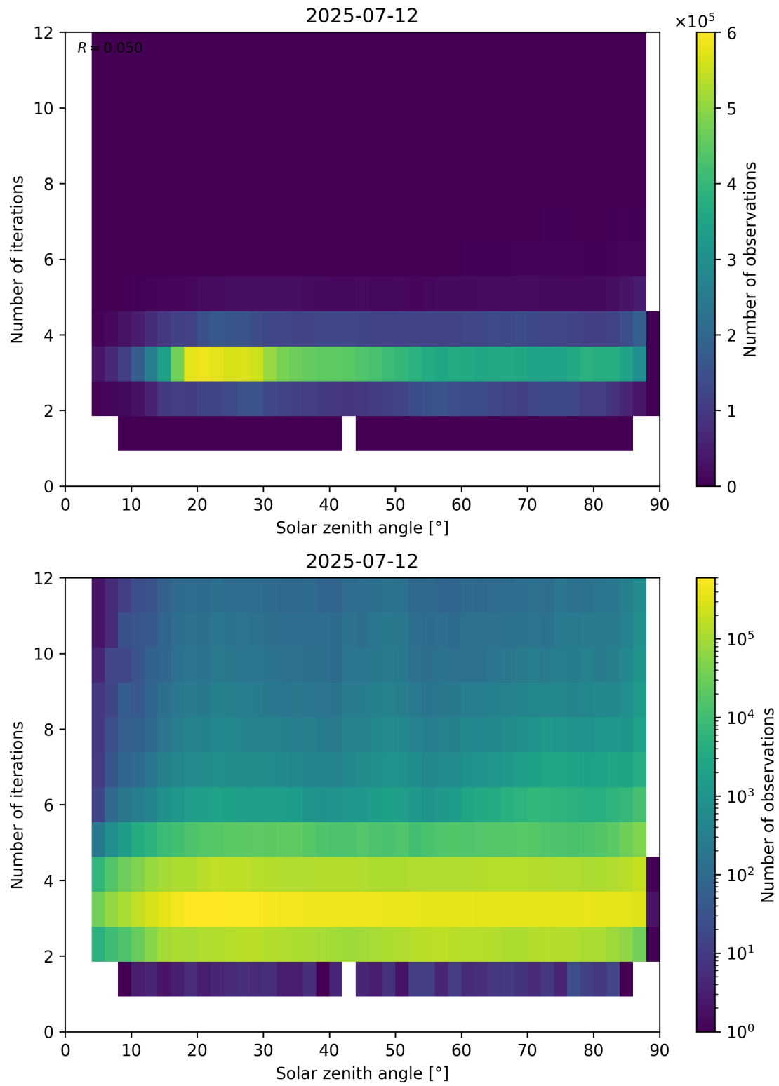
Figure 114: Scatter density plot of “Solar zenith angle” against “Number of iterations” for 2025-07-11 to 2025-07-13.
