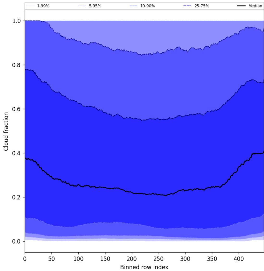
Figure 49: Along track statistics of “Cloud fraction” for 2025-07-11 to 2025-07-13
