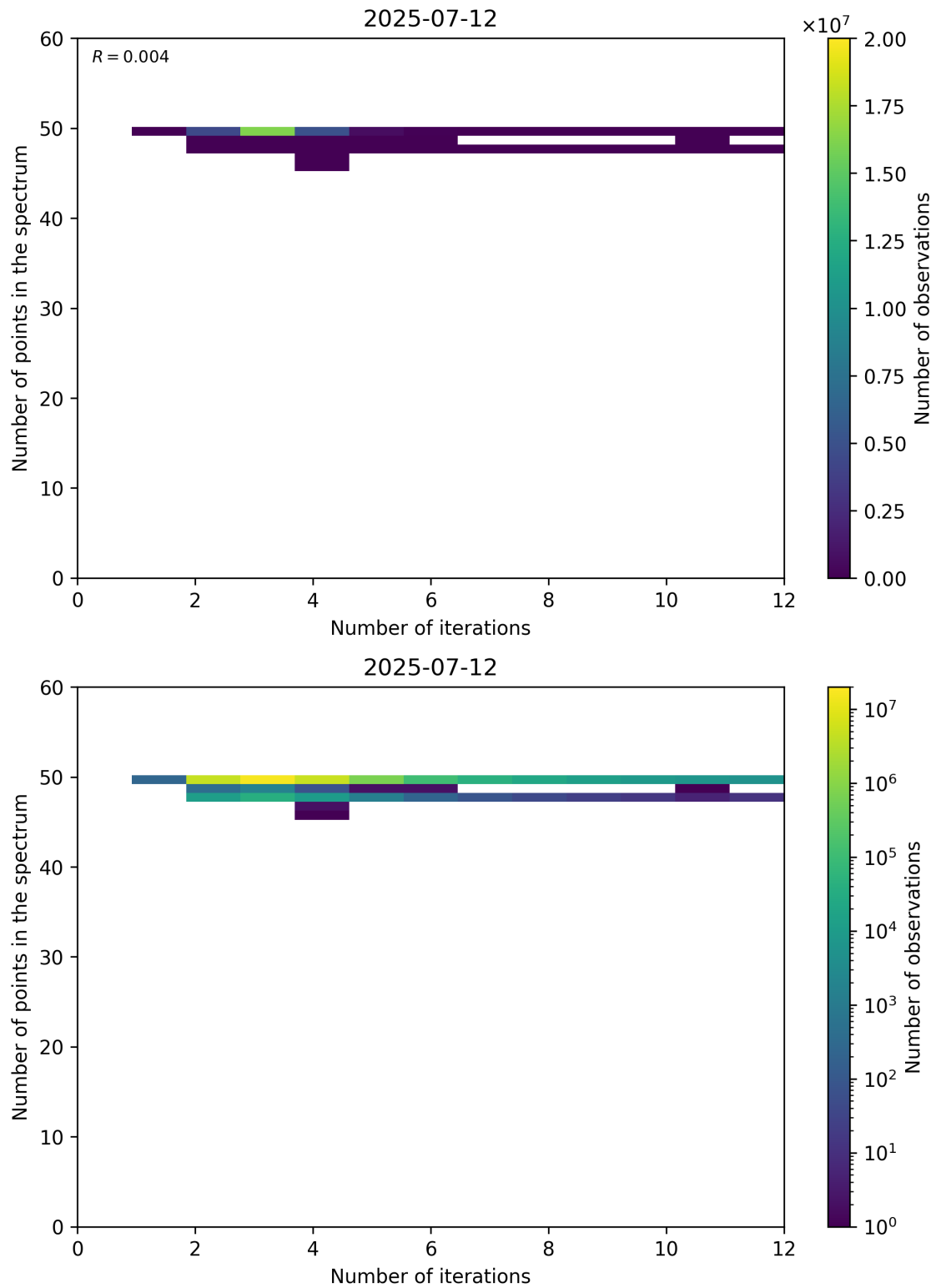
Figure 99: Scatter density plot of “Number of iterations” against “Number of points in the spectrum” for 2025-07-11 to 2025-07-13.
