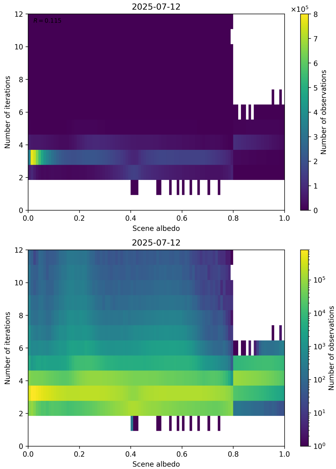
Figure 105: Scatter density plot of “Scene albedo” against “Number of iterations” for 2025-07-11 to 2025-07-13.
