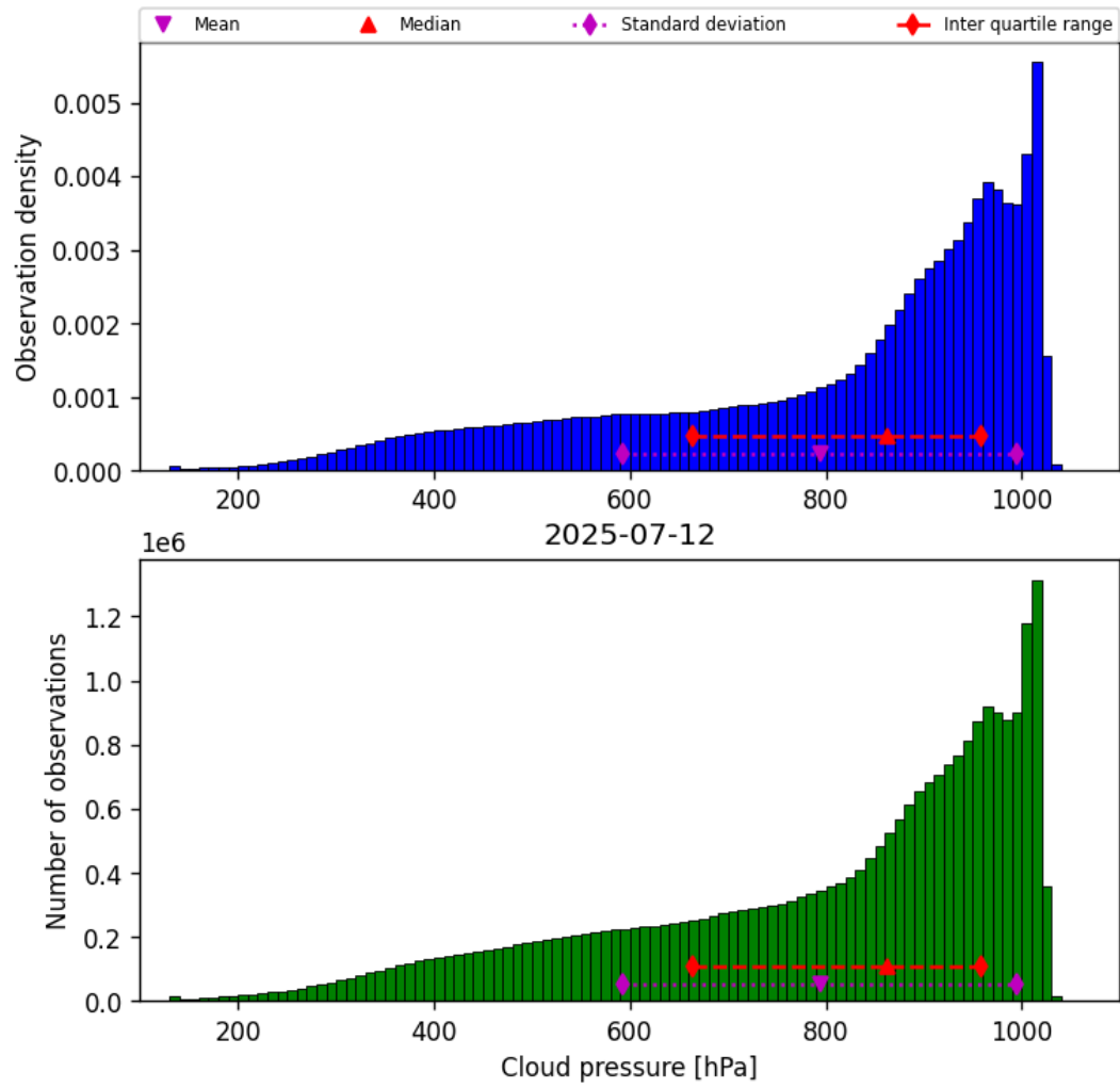
Figure 30: Histogram of “Cloud pressure” for 2025-07-11 to 2025-07-13
