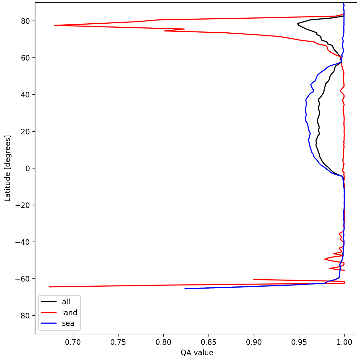
Figure 12: Zonal average of “QA value” for 2025-07-11 to 2025-07-13.
