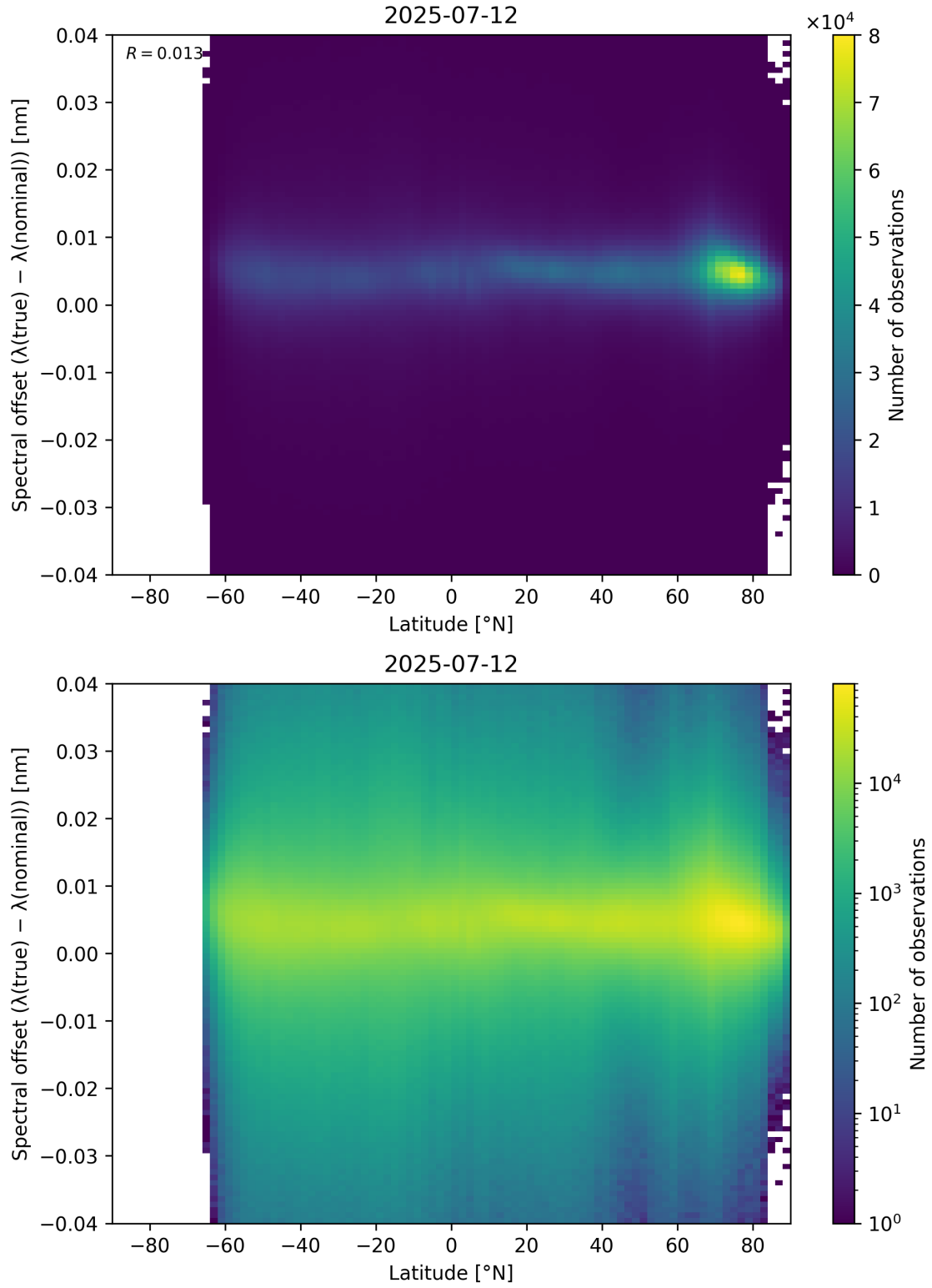
Figure 96: Scatter density plot of “Latitude” against “Spectral offset ( \lambda_{\text{true}} - \lambda_{\text{nominal}} )” for 2025-07-11 to 2025-07-13.
